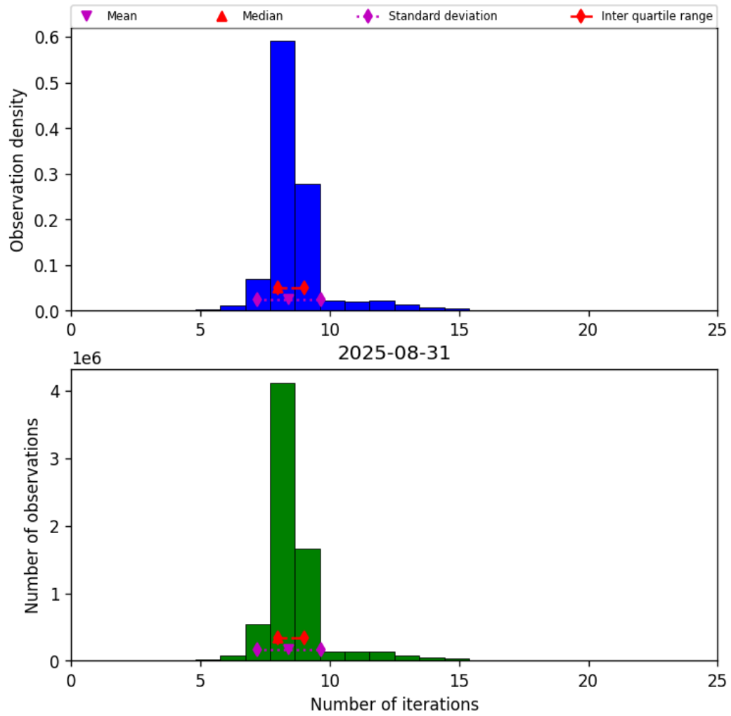
Figure 19: Histogram of “Number of iterations” for 2025-08-31 to 2025-09-01
