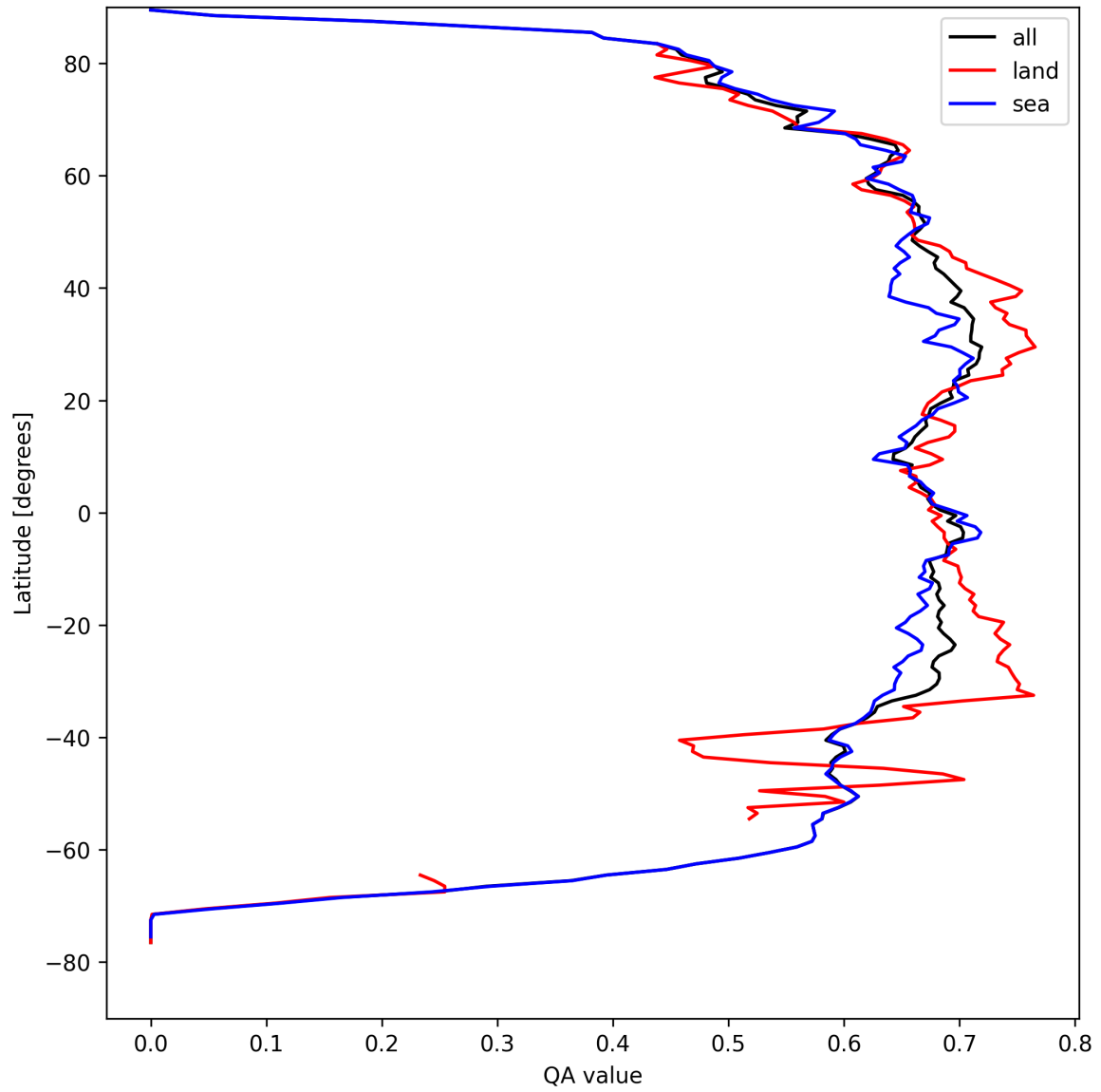
Figure 6: Zonal average of “QA value” for 2025-08-31 to 2025-09-01.
