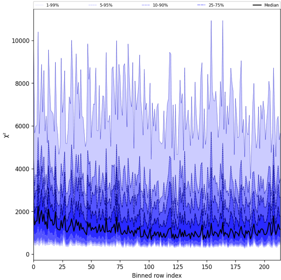
Figure 24: Along track statistics of “ \chi^2 ” for 2025-08-31 to 2025-09-01
