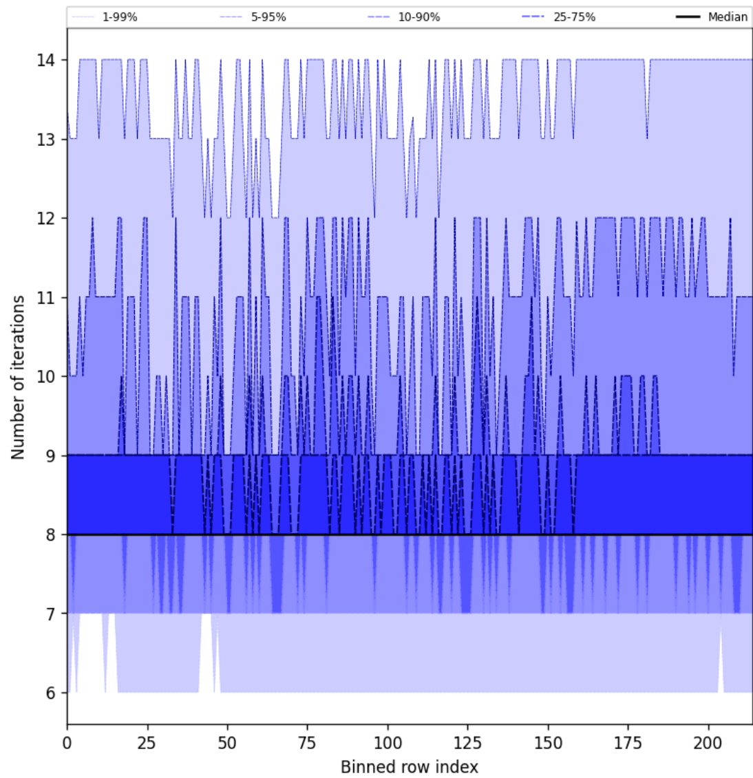
Figure 26: Along track statistics of “Number of iterations” for 2025-08-31 to 2025-09-01
