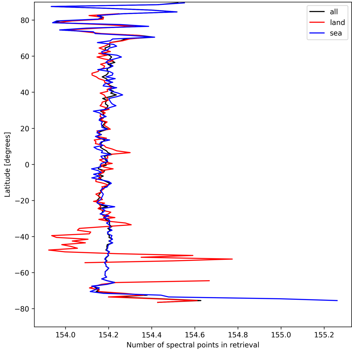
Figure 9: Zonal average of “Number of spectral points in retrieval” for 2025-08-31 to 2025-09-01.
