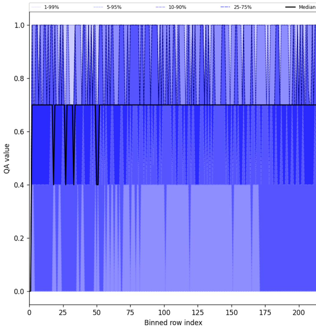
Figure 20: Along track statistics of “QA value” for 2025-08-31 to 2025-09-01
