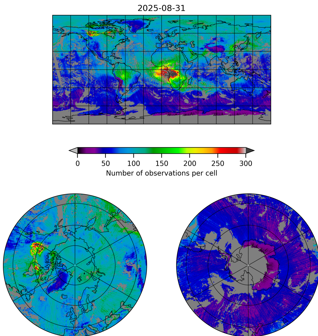
Figure 5: Map of the number of observations for 2025-08-31 to 2025-09-01
