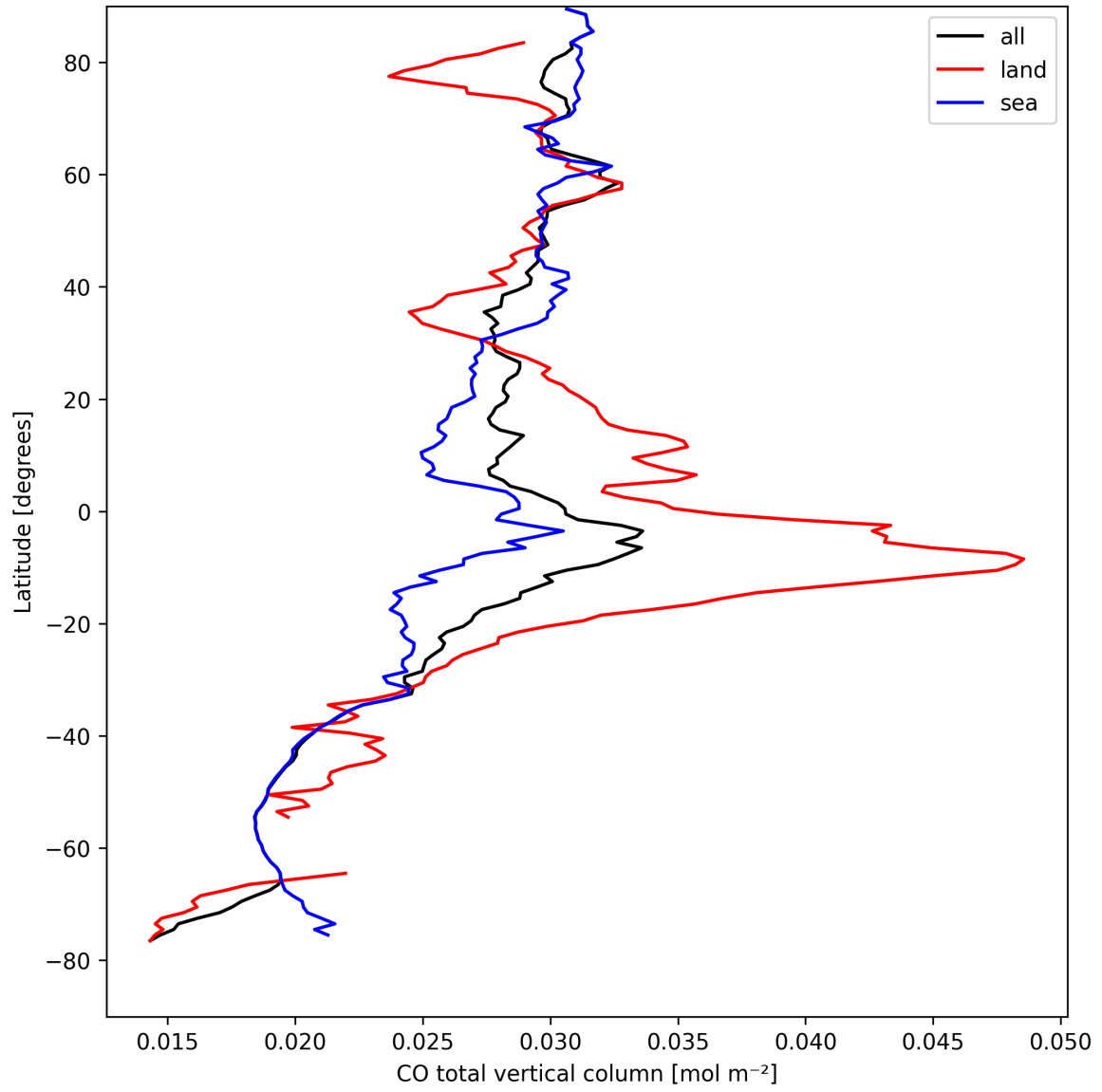
Figure 7: Zonal average of “CO total vertical column” for 2025-08-31 to 2025-09-01.
