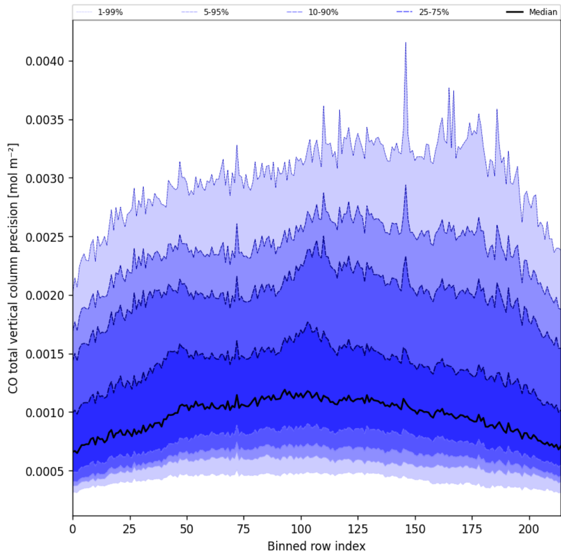
Figure 22: Along track statistics of “CO total vertical column precision” for 2025-08-31 to 2025-09-01
