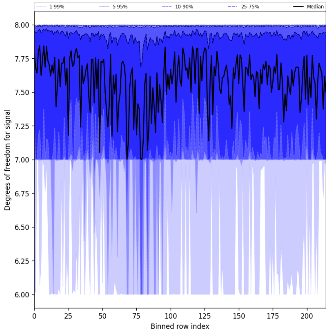
Figure 25: Along track statistics of “Degrees of freedom for signal” for 2025-08-31 to 2025-09-01
