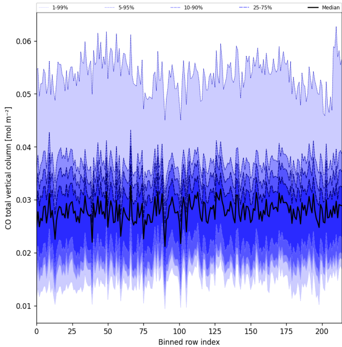
Figure 21: Along track statistics of “CO total vertical column” for 2025-08-31 to 2025-09-01
