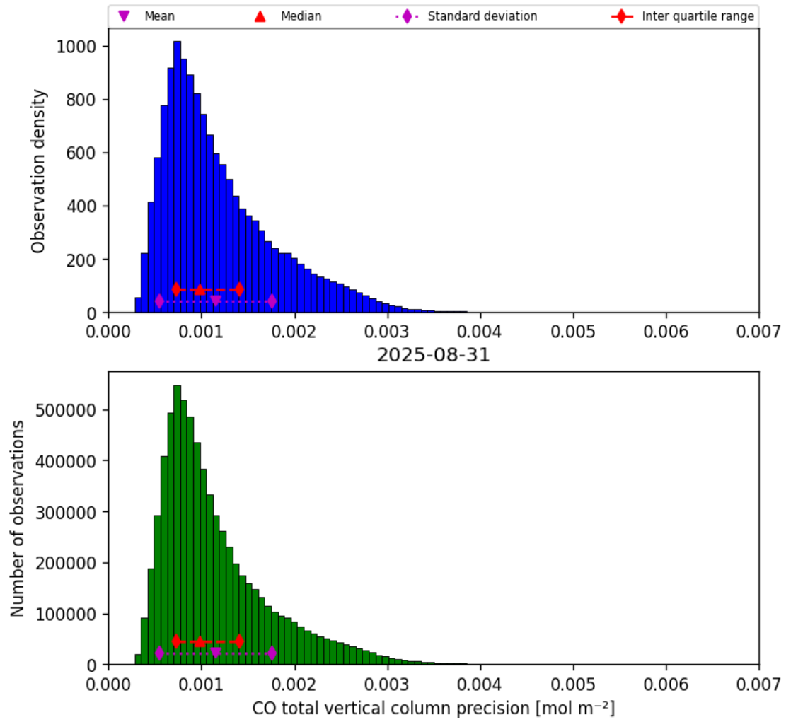
Figure 15: Histogram of “CO total vertical column precision” for 2025-08-31 to 2025-09-01
