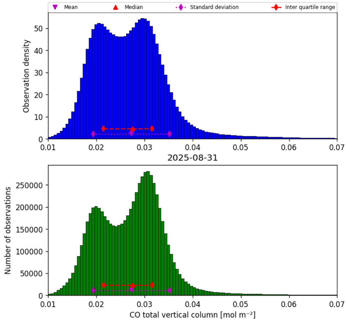
Figure 14: Histogram of “CO total vertical column” for 2025-08-31 to 2025-09-01
