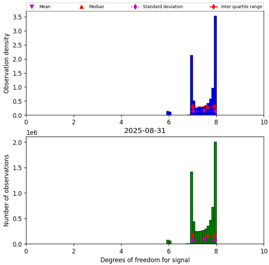
Figure 18: Histogram of “Degrees of freedom for signal” for 2025-08-31 to 2025-09-01
