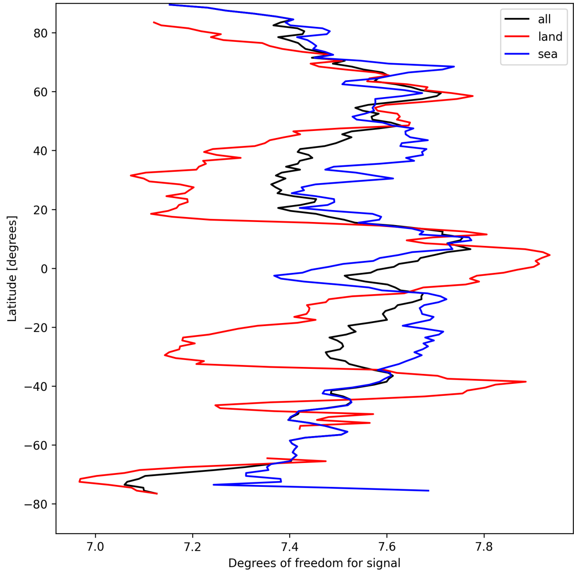
Figure 11: Zonal average of “Degrees of freedom for signal” for 2025-08-31 to 2025-09-01.
