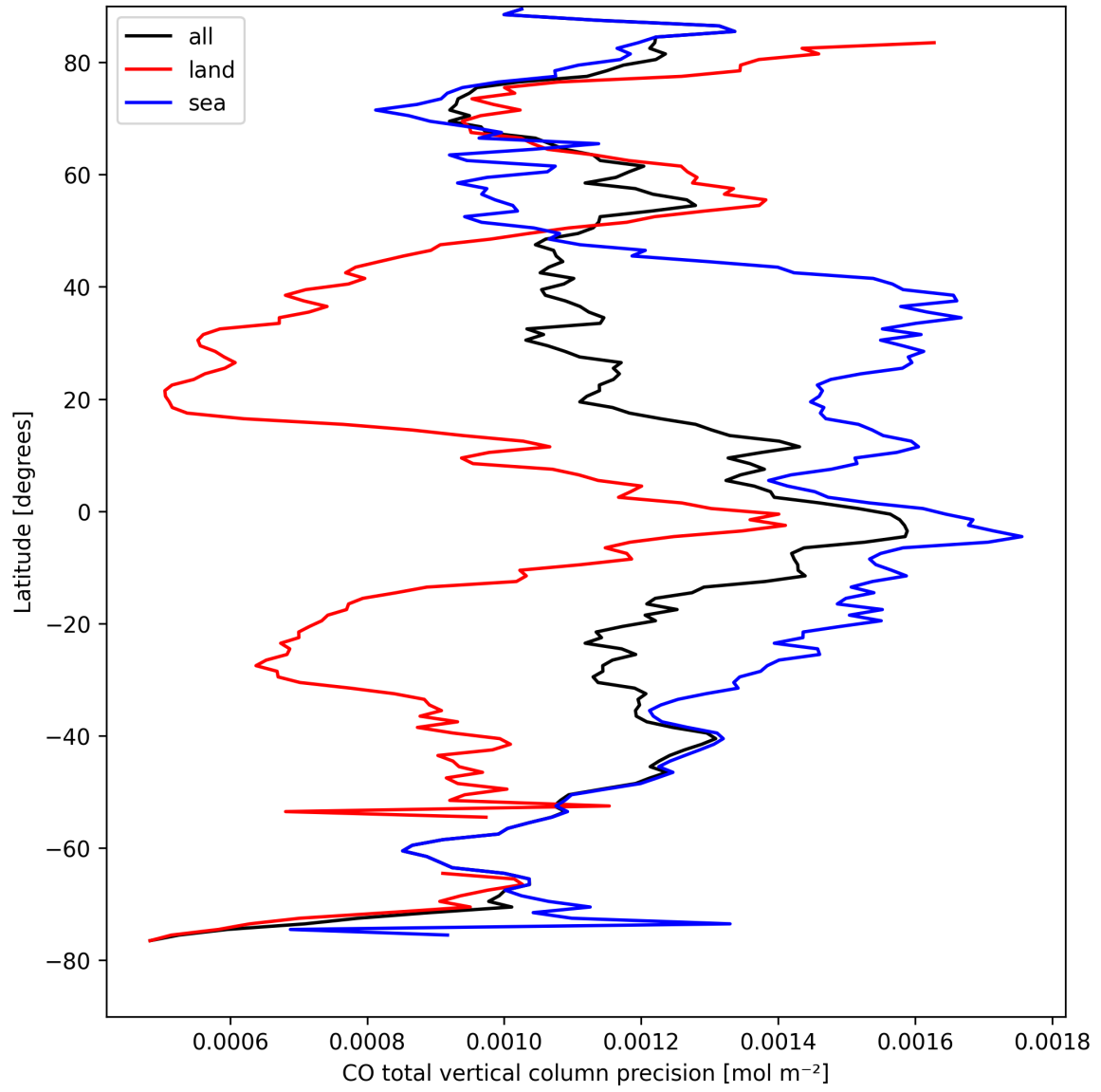
Figure 8: Zonal average of “CO total vertical column precision” for 2025-08-31 to 2025-09-01.
