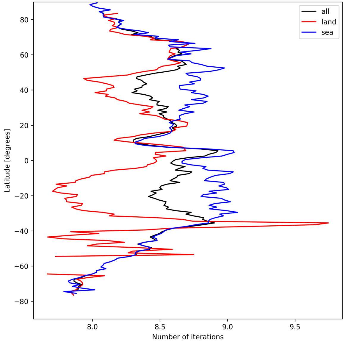
Figure 12: Zonal average of “Number of iterations” for 2025-08-31 to 2025-09-01.
