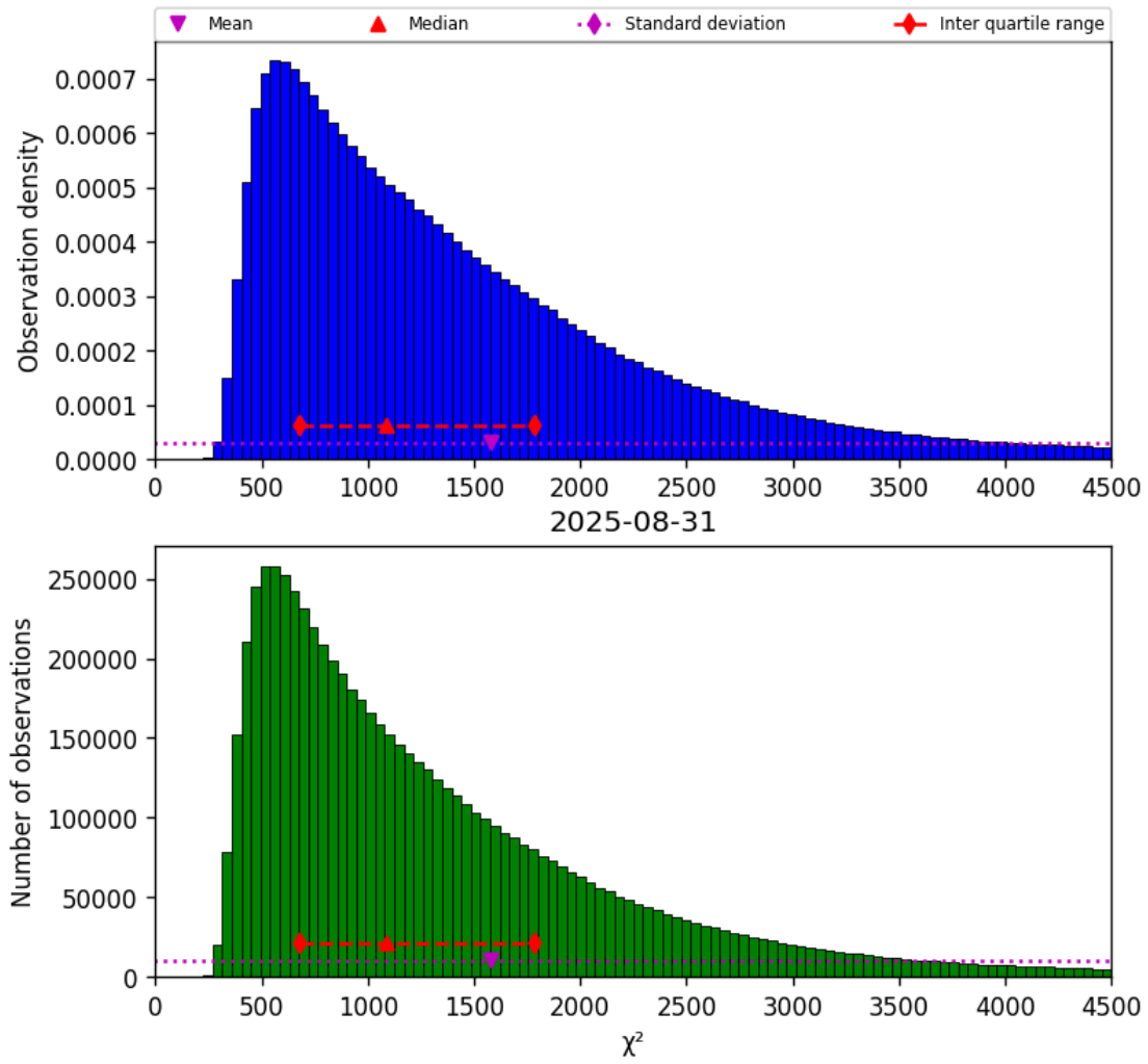
Figure 17: Histogram of " \chi^2 " for 2025-08-31 to 2025-09-01
