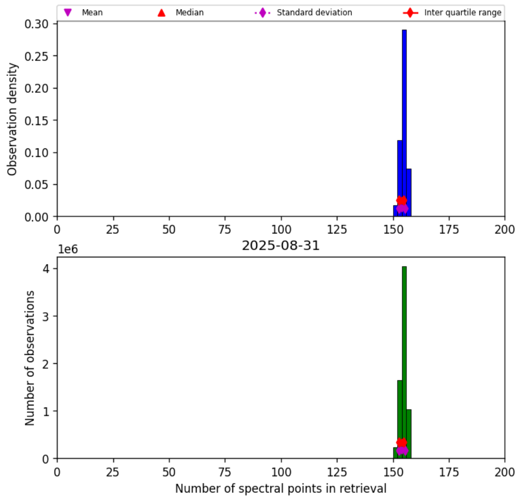
Figure 16: Histogram of “Number of spectral points in retrieval” for 2025-08-31 to 2025-09-01
