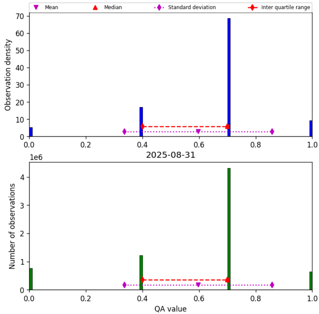
Figure 13: Histogram of “QA value” for 2025-08-31 to 2025-09-01
