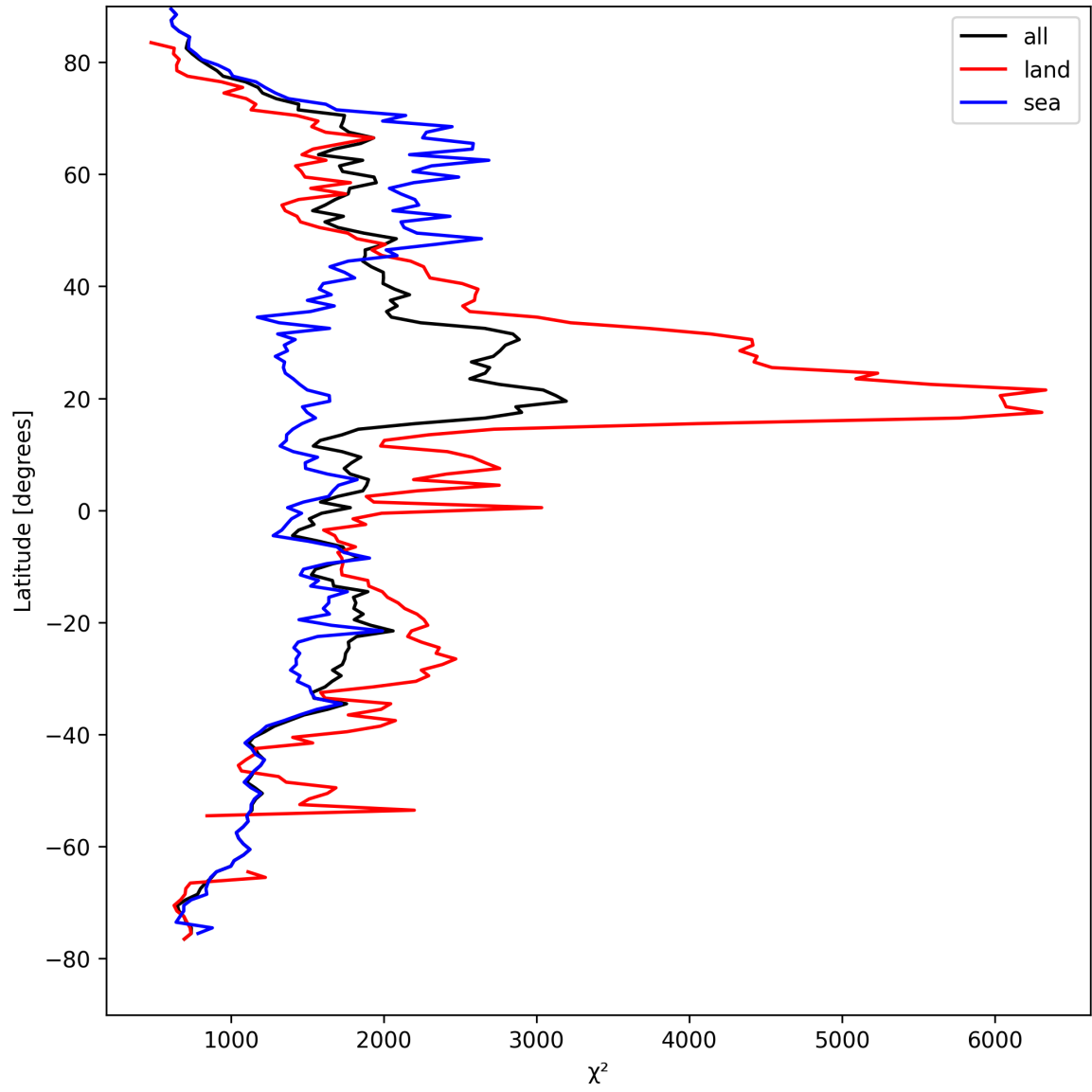
Figure 10: Zonal average of “ \chi^2 ” for 2025-08-31 to 2025-09-01.
