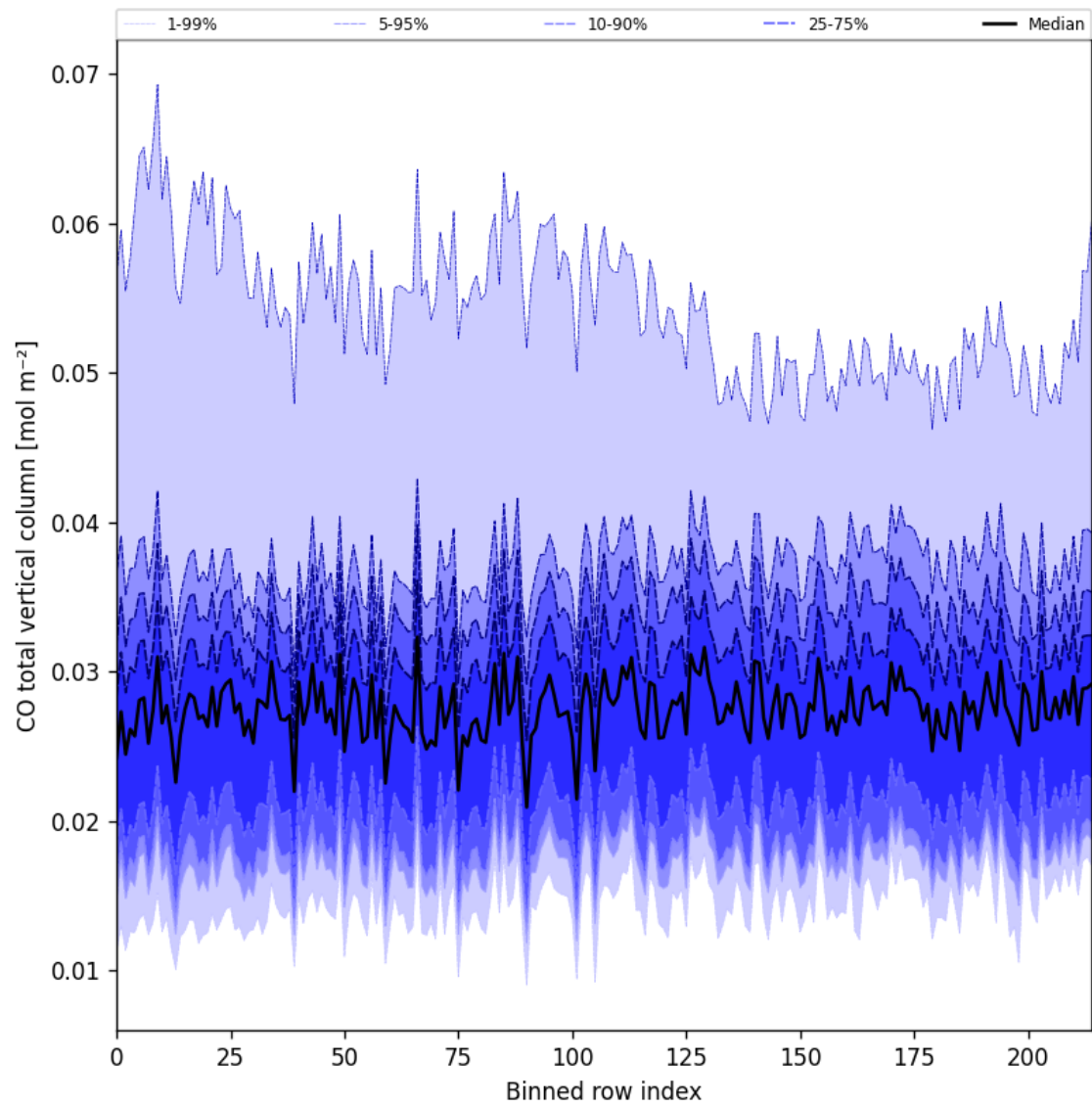
Figure 21: Along track statistics of “CO total vertical column” for 2025-09-01 to 2025-09-02
