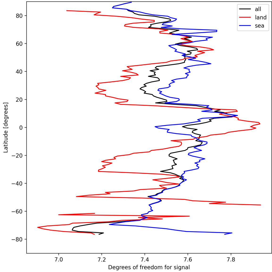
Figure 11: Zonal average of “Degrees of freedom for signal” for 2025-09-01 to 2025-09-02.
