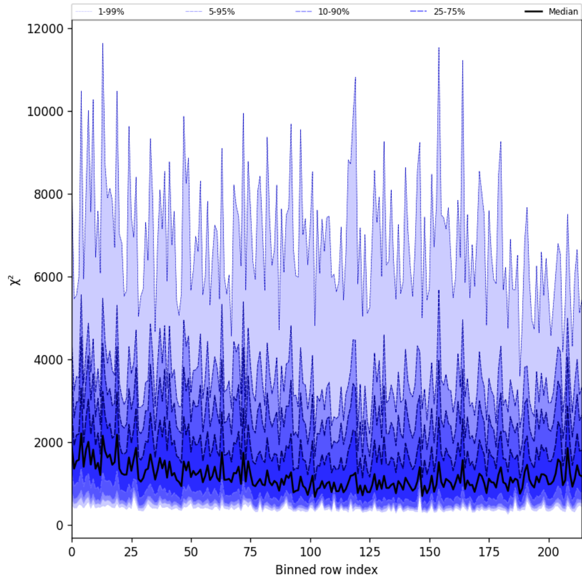
Figure 24: Along track statistics of “ \chi^2 ” for 2025-09-01 to 2025-09-02
