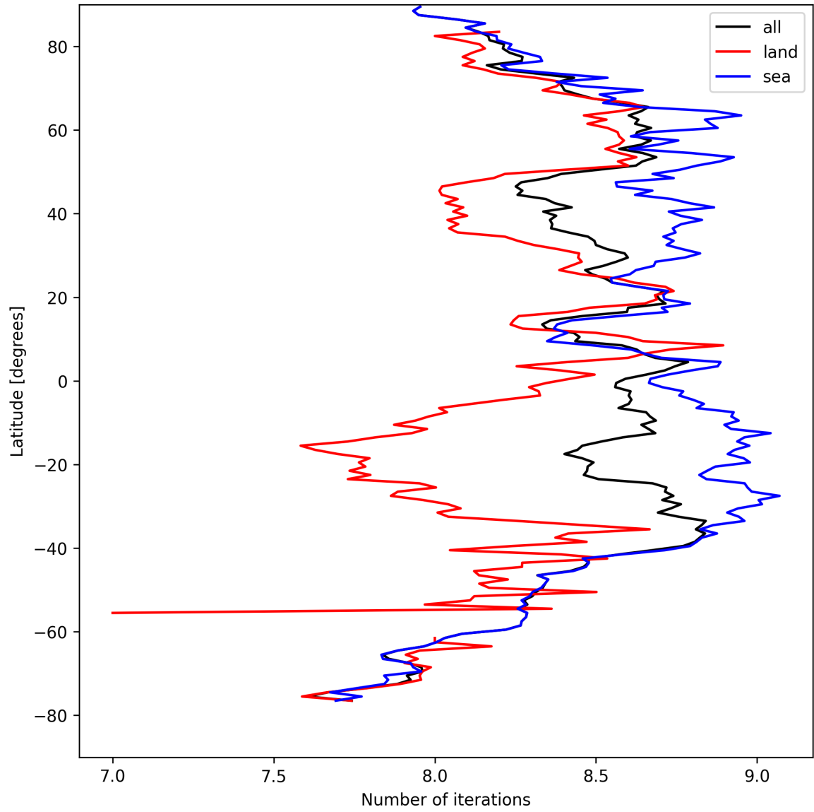
Figure 12: Zonal average of “Number of iterations” for 2025-09-01 to 2025-09-02.
