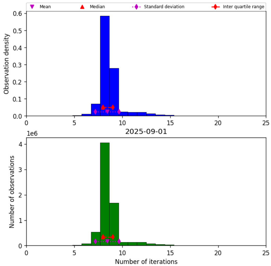
Figure 19: Histogram of “Number of iterations” for 2025-09-01 to 2025-09-02
