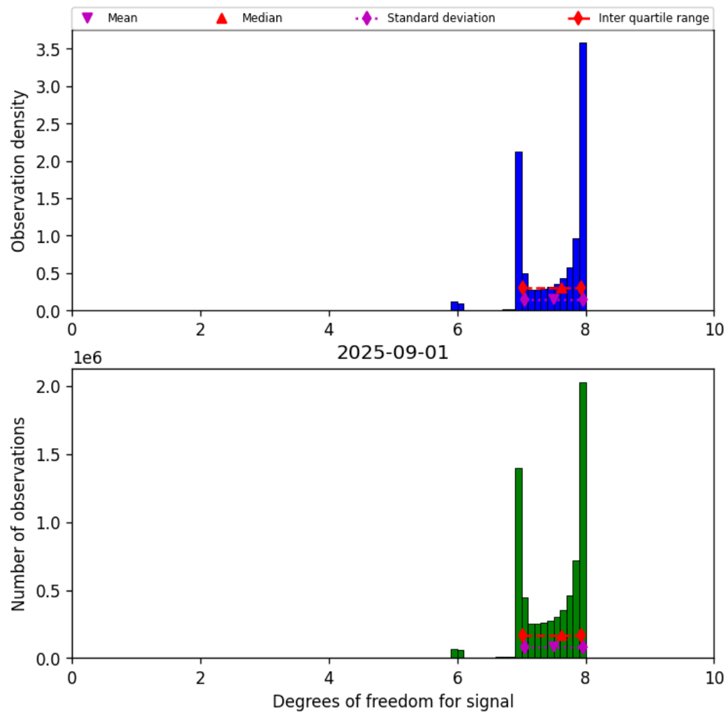
Figure 18: Histogram of “Degrees of freedom for signal” for 2025-09-01 to 2025-09-02
