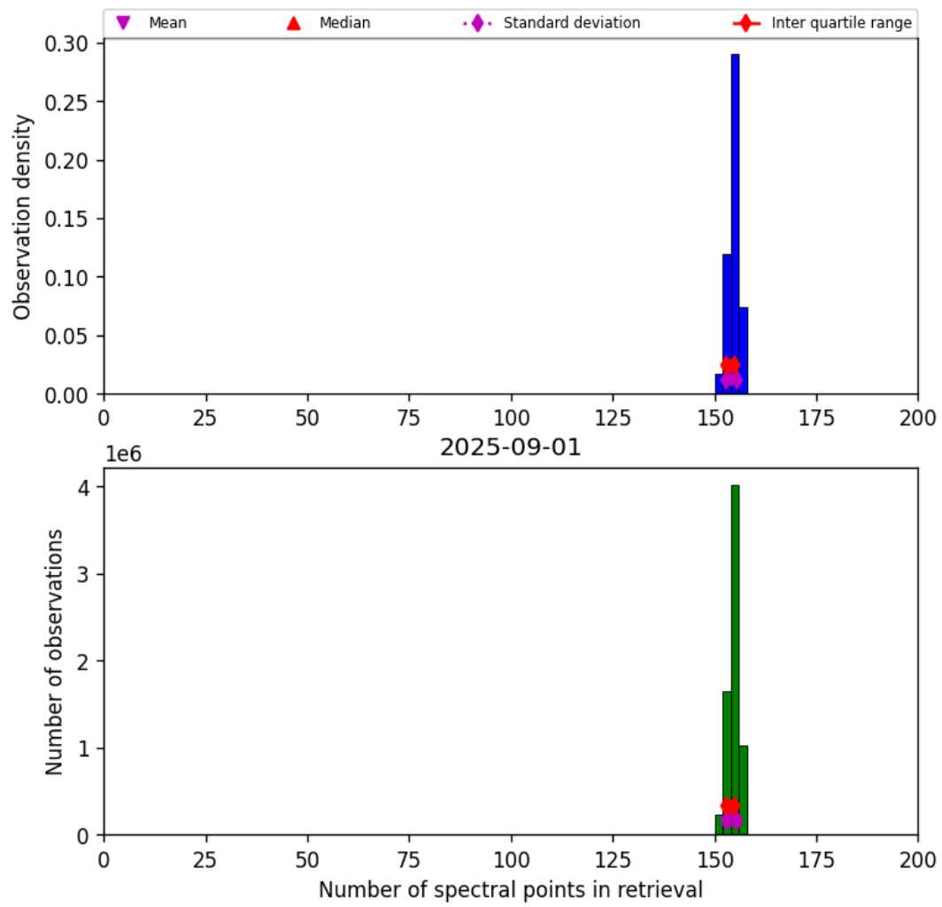
Figure 16: Histogram of “Number of spectral points in retrieval” for 2025-09-01 to 2025-09-02
