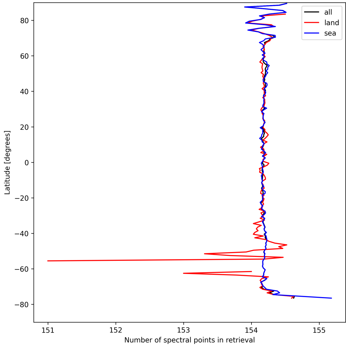
Figure 9: Zonal average of “Number of spectral points in retrieval” for 2025-09-01 to 2025-09-02.
