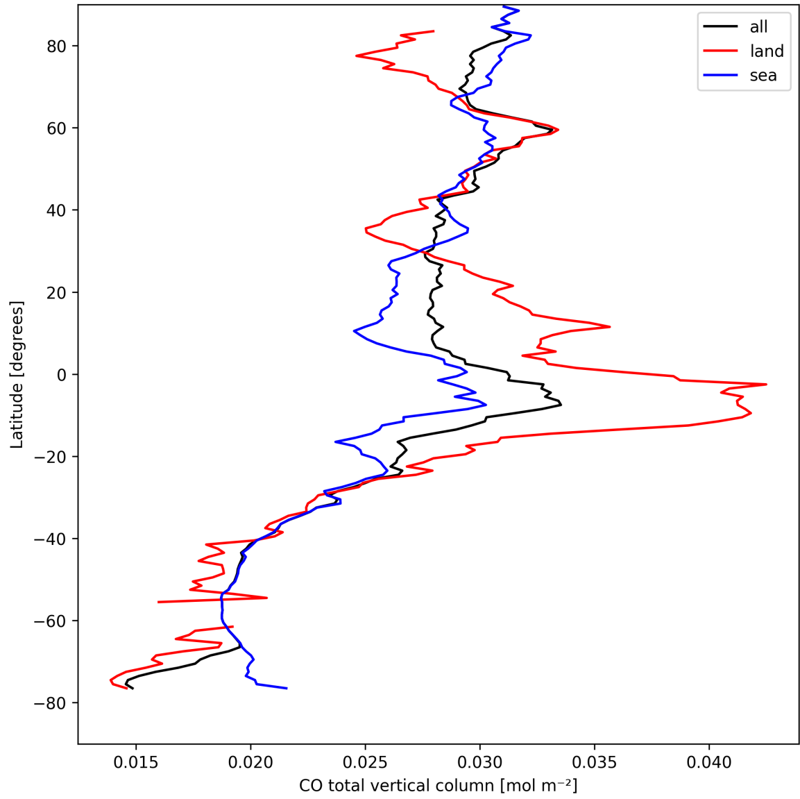
Figure 7: Zonal average of “CO total vertical column” for 2025-09-01 to 2025-09-02.
