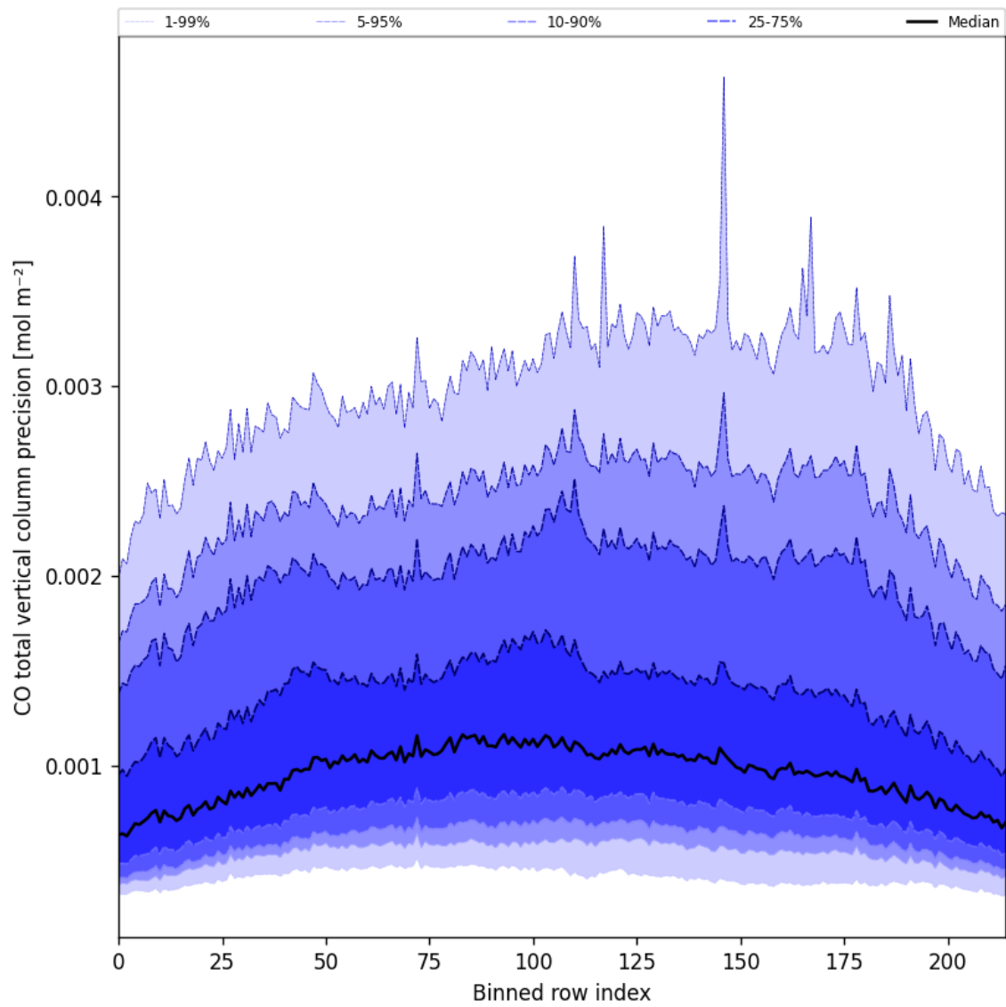
Figure 22: Along track statistics of “CO total vertical column precision” for 2025-09-01 to 2025-09-02
