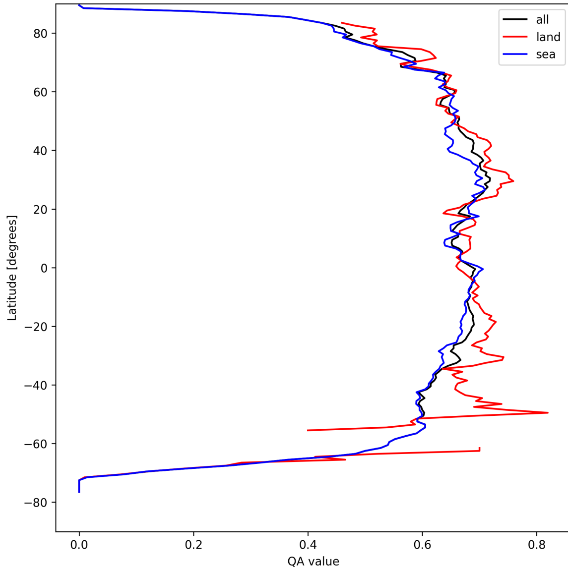
Figure 6: Zonal average of “QA value” for 2025-09-01 to 2025-09-02.
