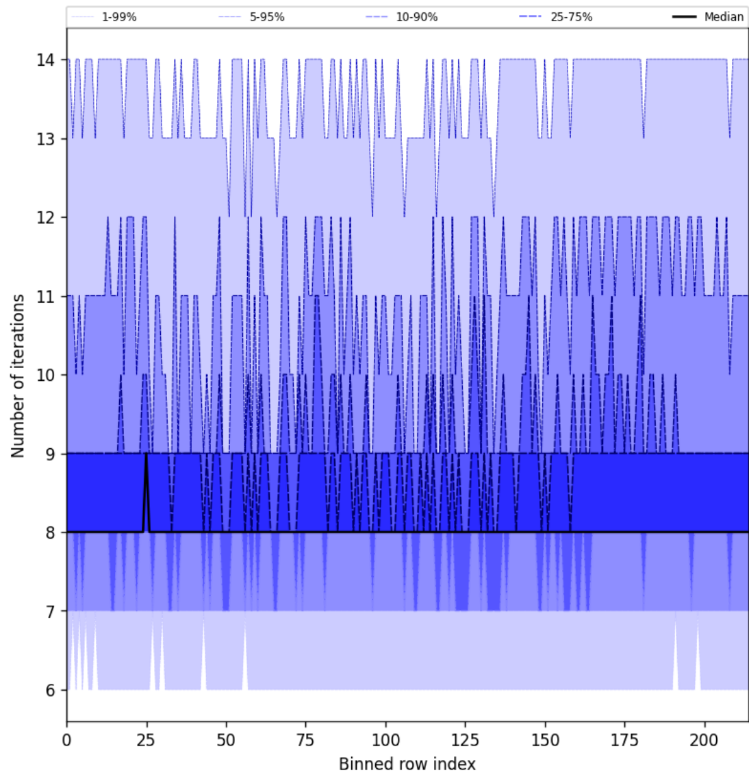
Figure 26: Along track statistics of “Number of iterations” for 2025-09-01 to 2025-09-02
