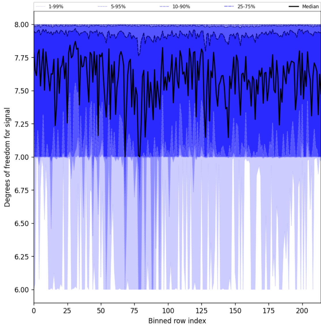
Figure 25: Along track statistics of “Degrees of freedom for signal” for 2025-09-01 to 2025-09-02
