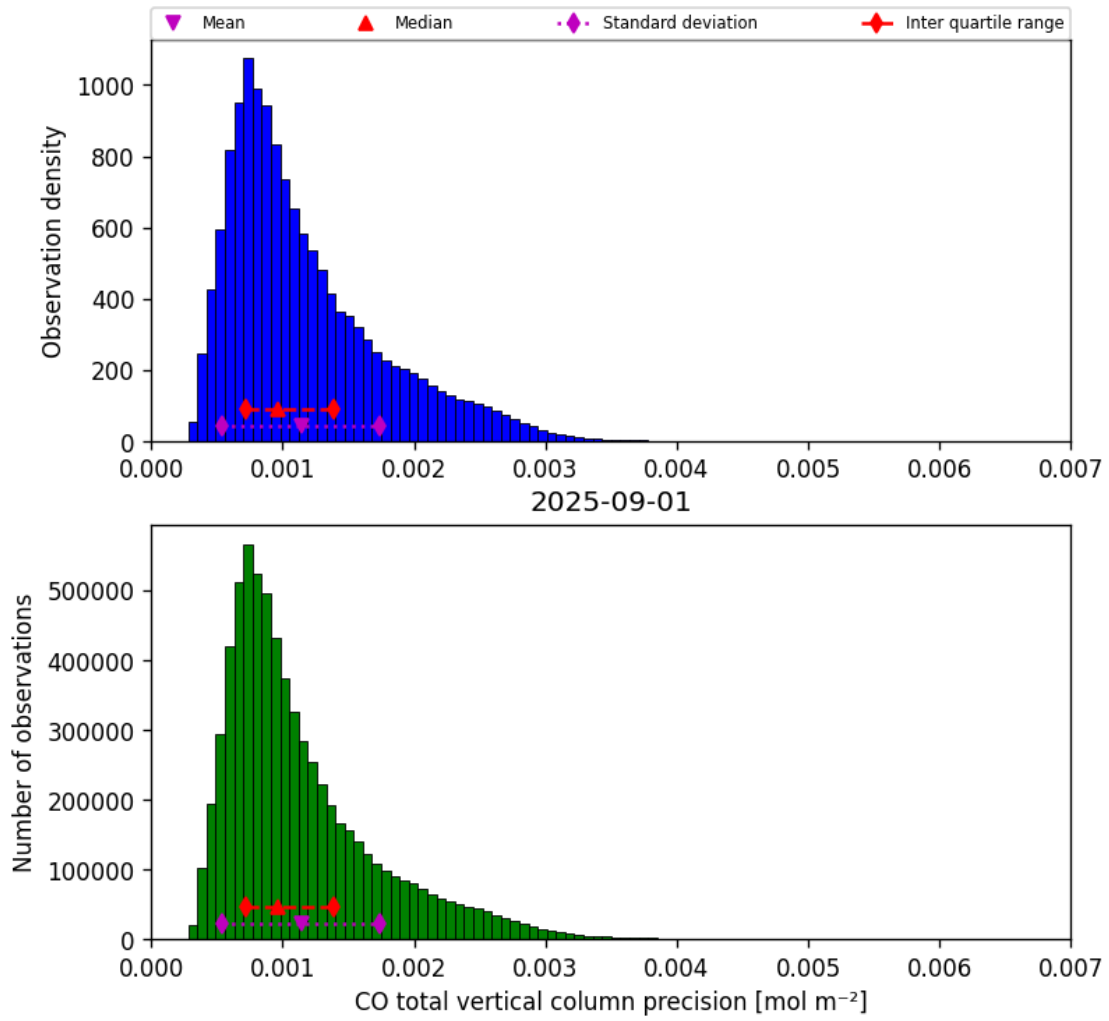
Figure 15: Histogram of “CO total vertical column precision” for 2025-09-01 to 2025-09-02
