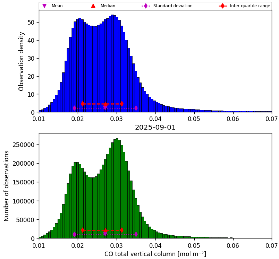
Figure 14: Histogram of “CO total vertical column” for 2025-09-01 to 2025-09-02
