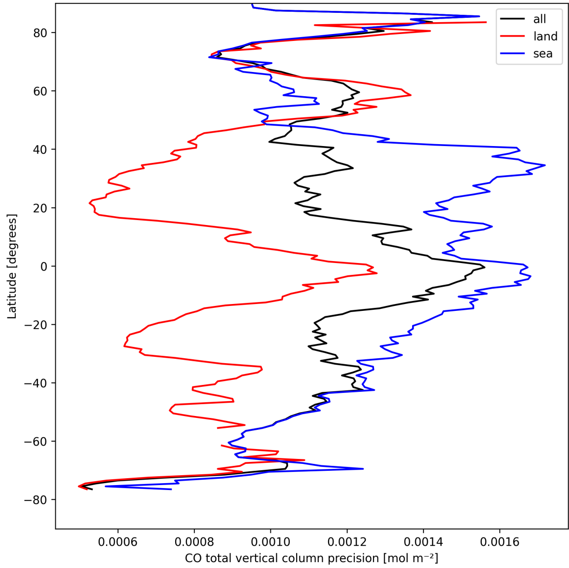
Figure 8: Zonal average of “CO total vertical column precision” for 2025-09-01 to 2025-09-02.
