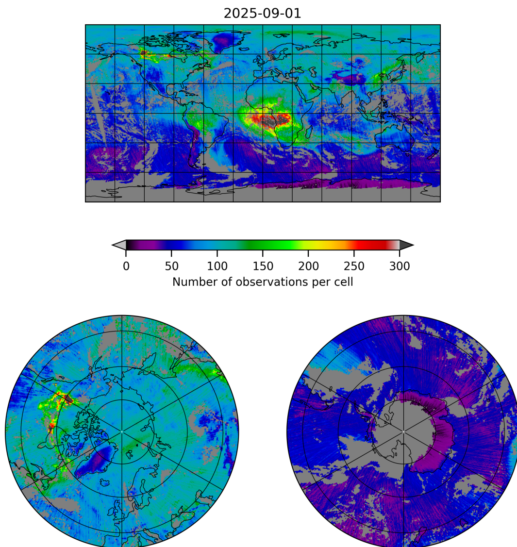
Figure 5: Map of the number of observations for 2025-09-01 to 2025-09-02
