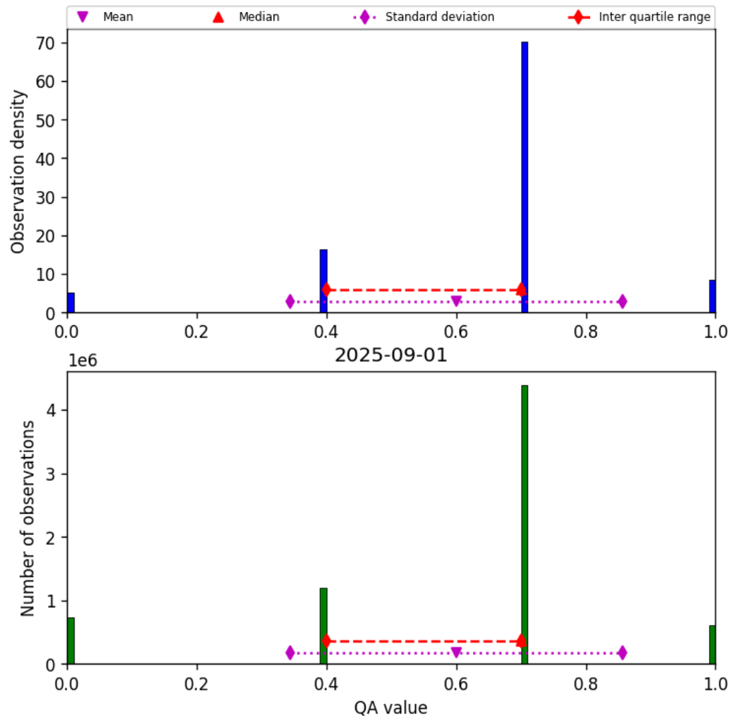
Figure 13: Histogram of “QA value” for 2025-09-01 to 2025-09-02
