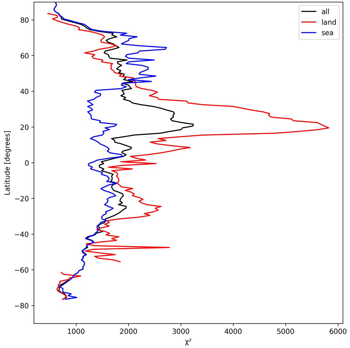
Figure 10: Zonal average of “ \chi^2 ” for 2025-09-01 to 2025-09-02.
