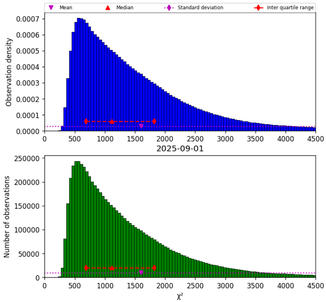
Figure 17: Histogram of " \chi^2 " for 2025-09-01 to 2025-09-02
