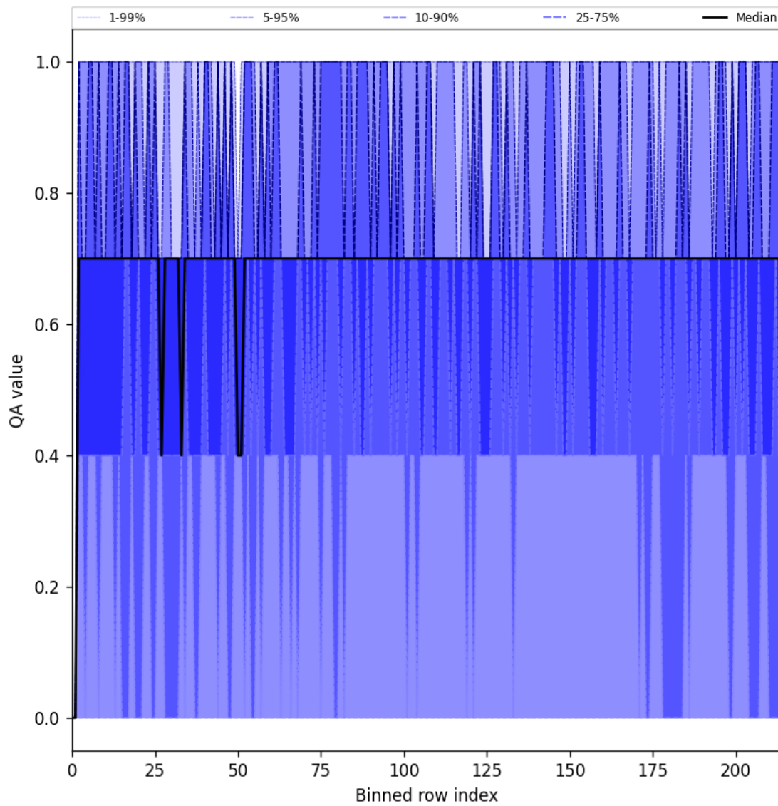
Figure 20: Along track statistics of “QA value” for 2025-09-01 to 2025-09-02
