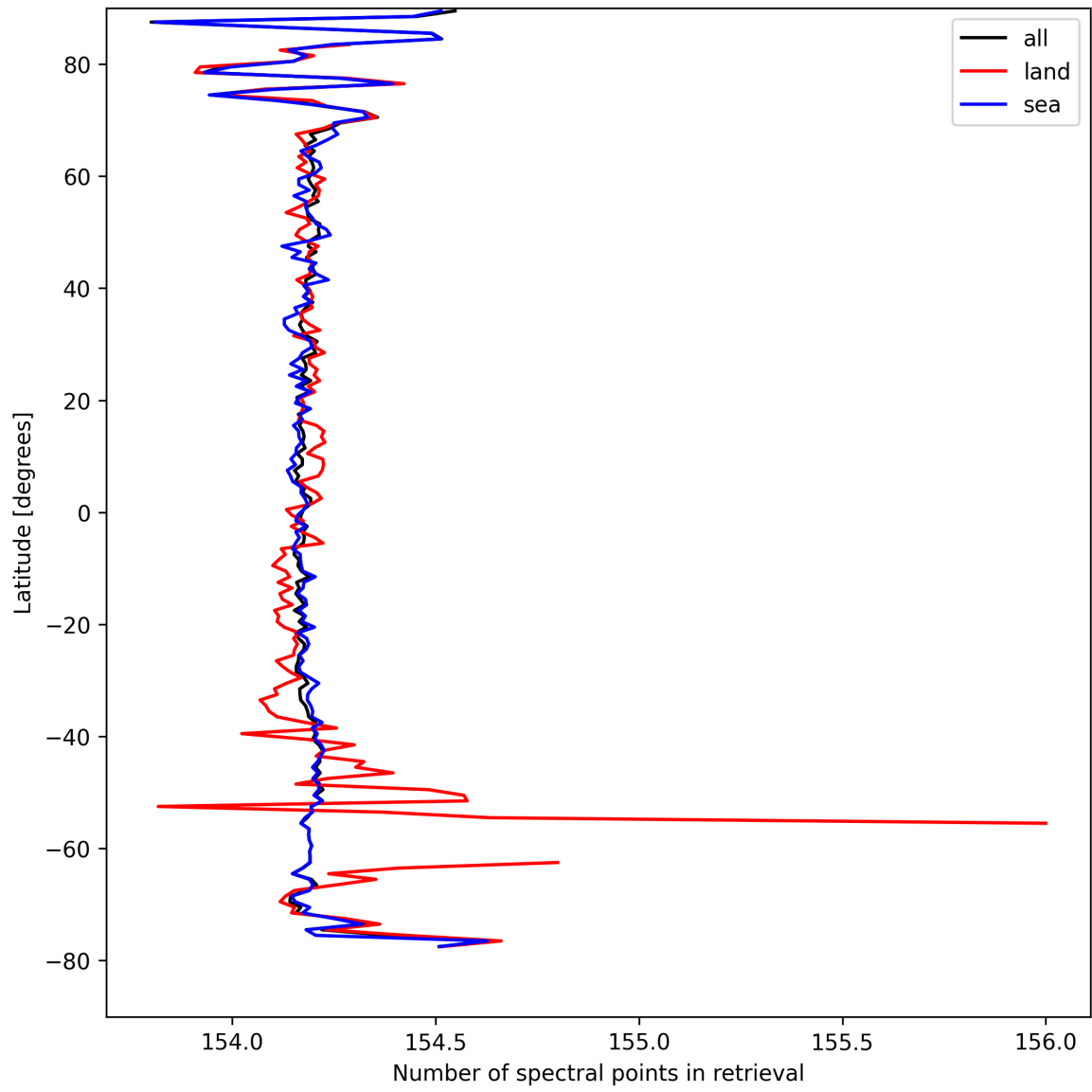
Figure 9: Zonal average of “Number of spectral points in retrieval” for 2025-09-03 to 2025-09-04.
