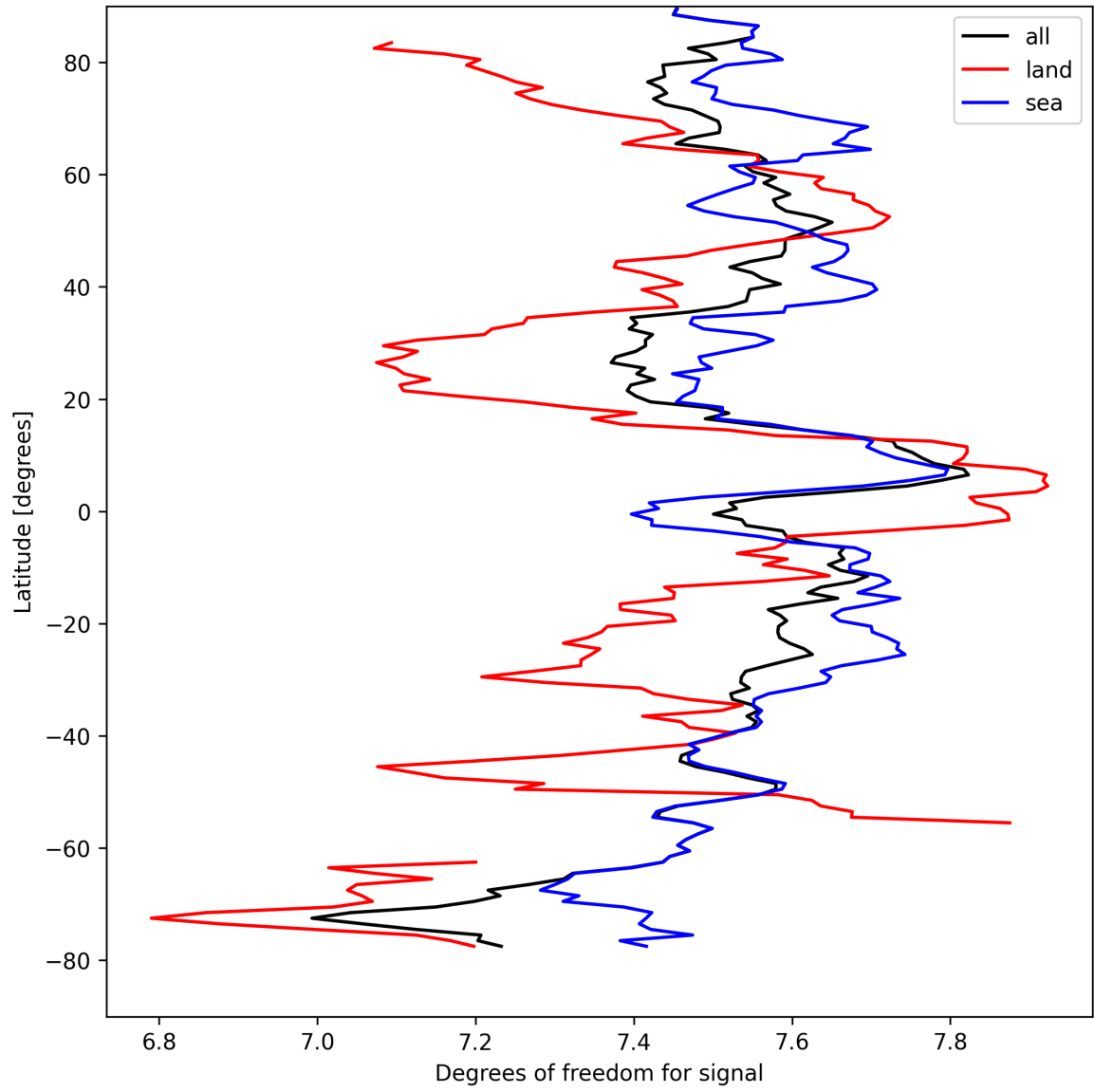
Figure 11: Zonal average of “Degrees of freedom for signal” for 2025-09-03 to 2025-09-04.
