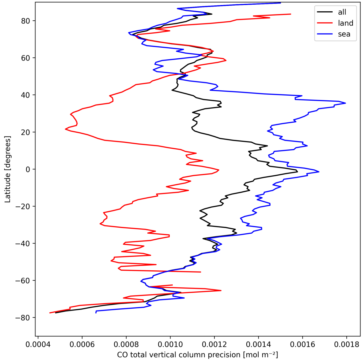
Figure 8: Zonal average of "CO total vertical column precision" for 2025-09-03 to 2025-09-04.
