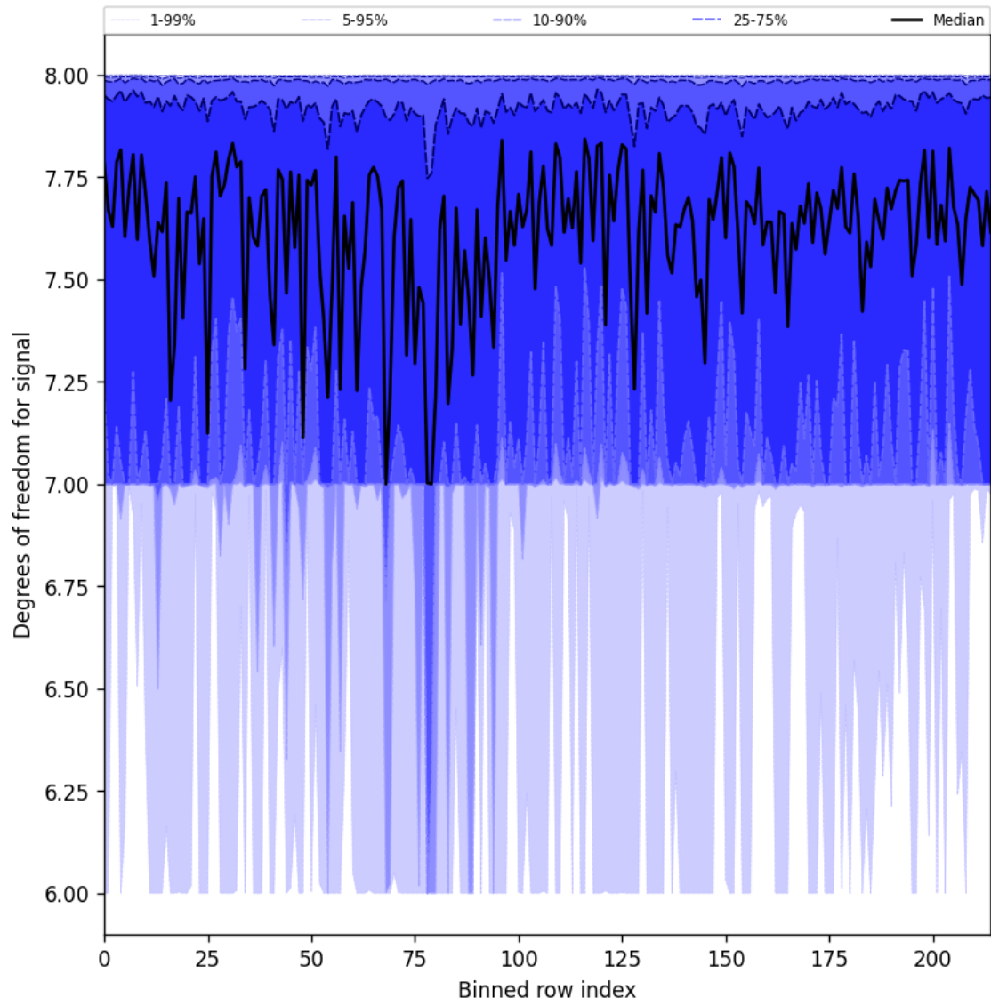
Figure 25: Along track statistics of “Degrees of freedom for signal” for 2025-09-03 to 2025-09-04
