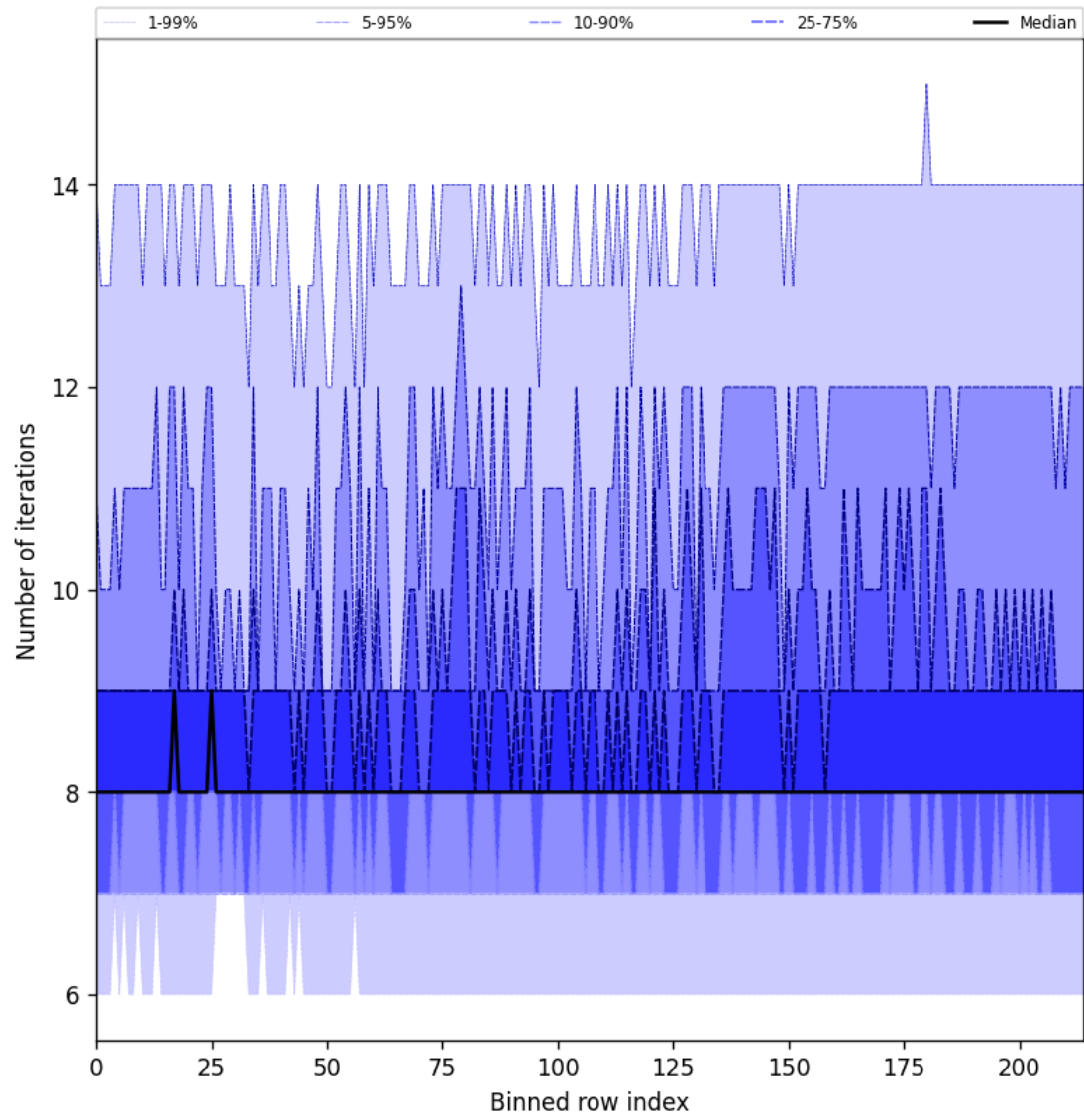
Figure 26: Along track statistics of “Number of iterations” for 2025-09-03 to 2025-09-04
