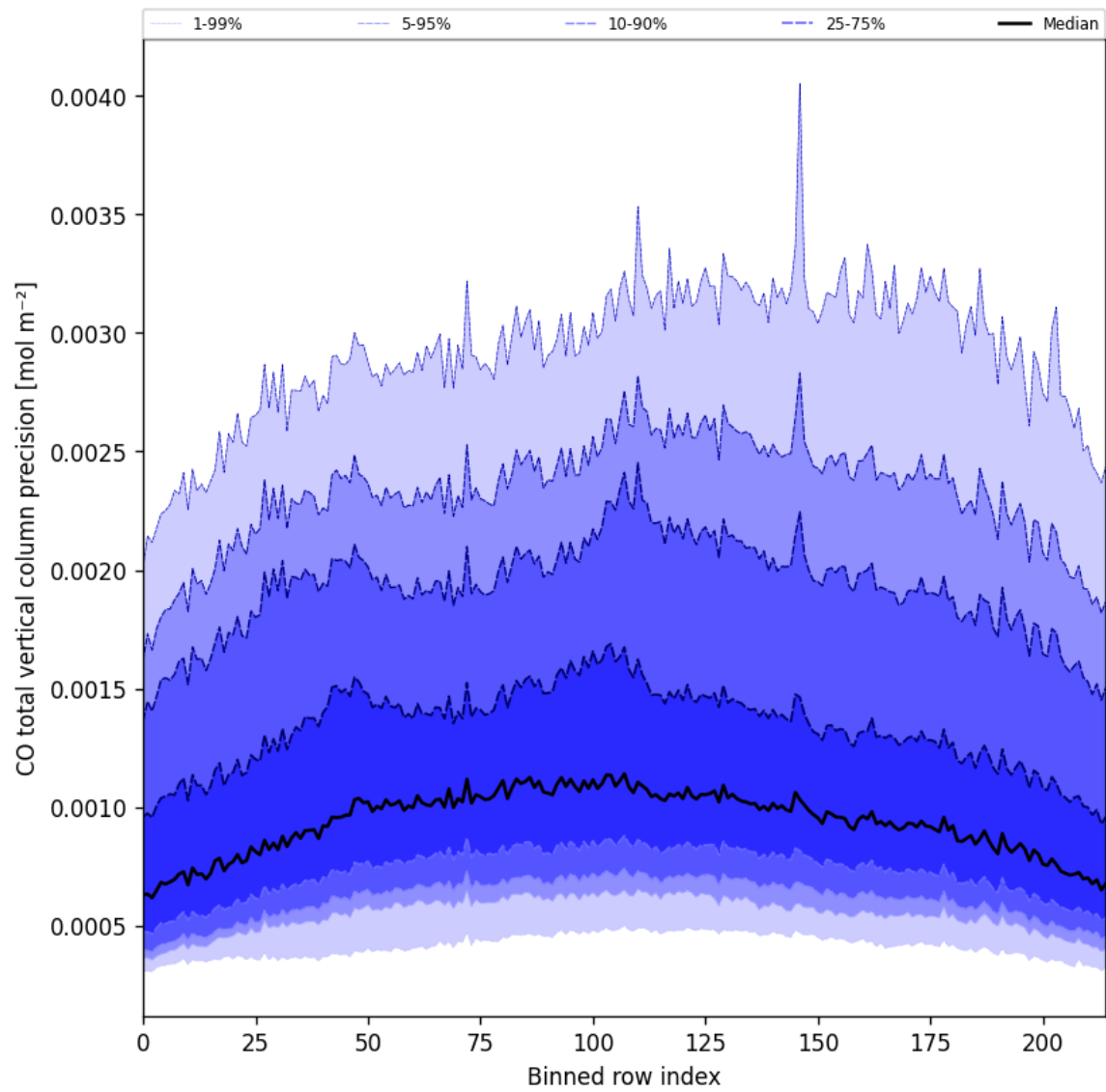
Figure 22: Along track statistics of “CO total vertical column precision” for 2025-09-03 to 2025-09-04
