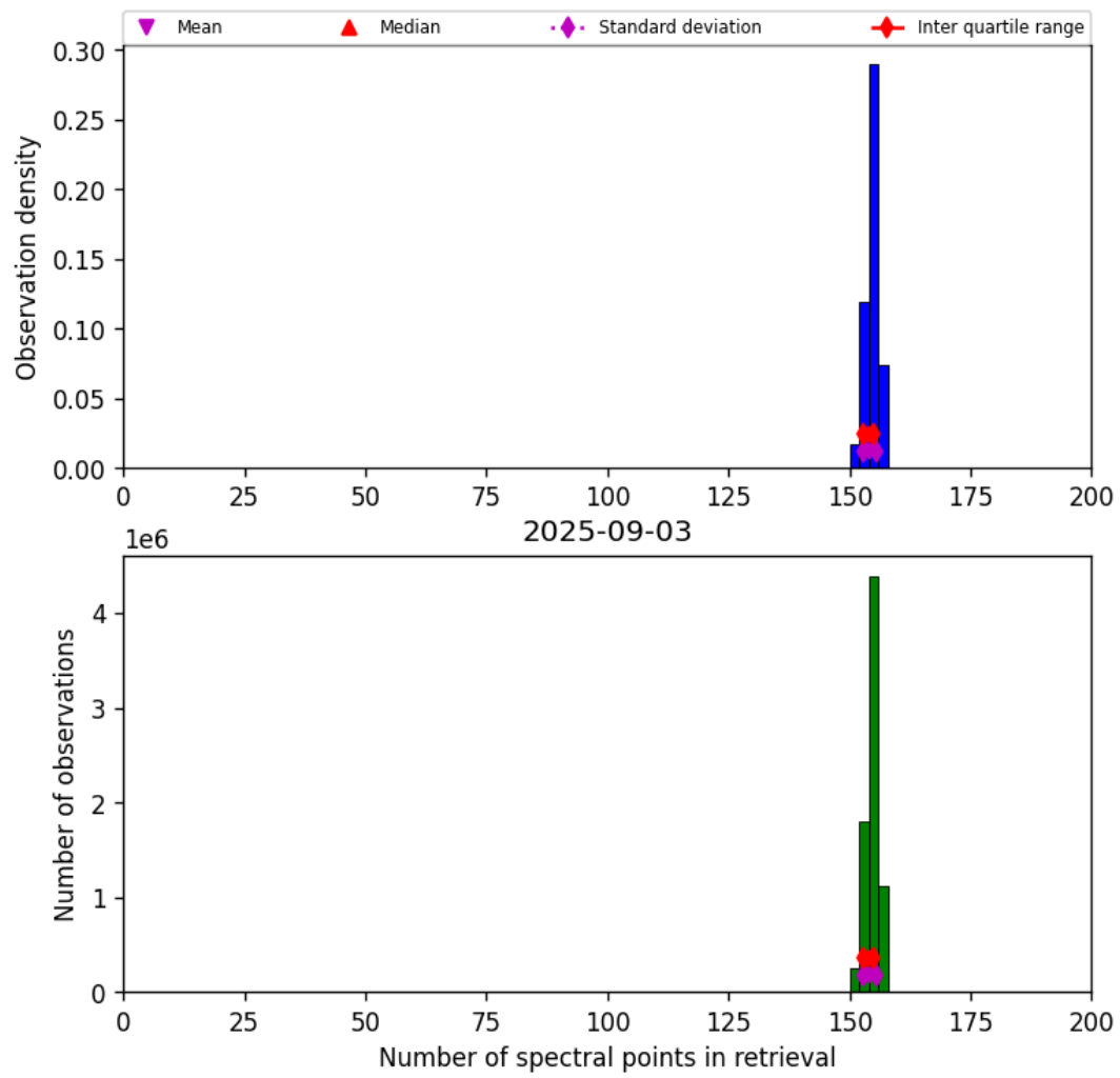
Figure 16: Histogram of “Number of spectral points in retrieval” for 2025-09-03 to 2025-09-04
