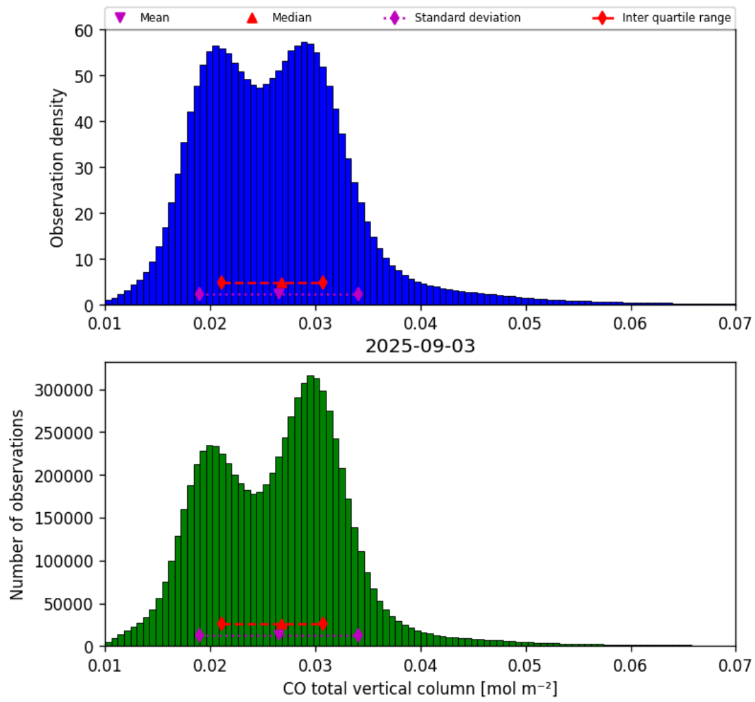
Figure 14: Histogram of “CO total vertical column” for 2025-09-03 to 2025-09-04
