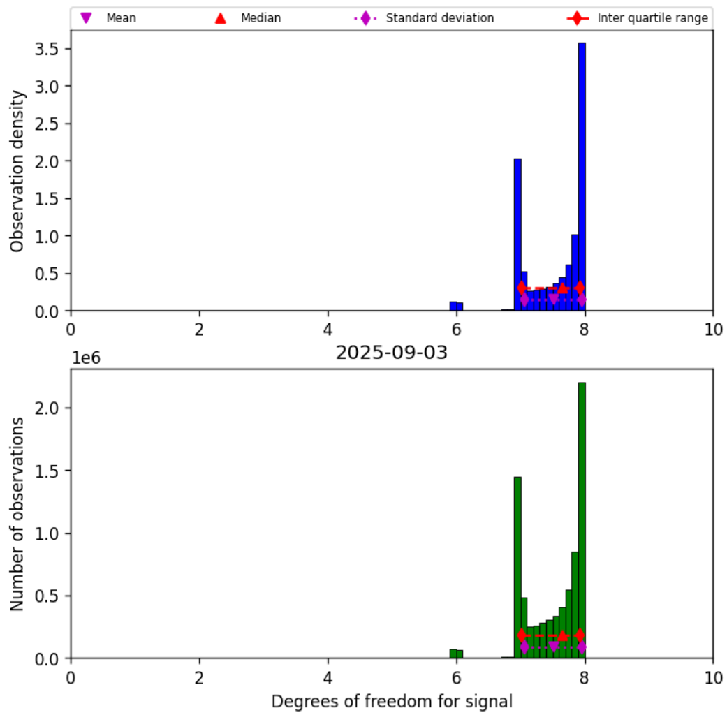
Figure 18: Histogram of “Degrees of freedom for signal” for 2025-09-03 to 2025-09-04
