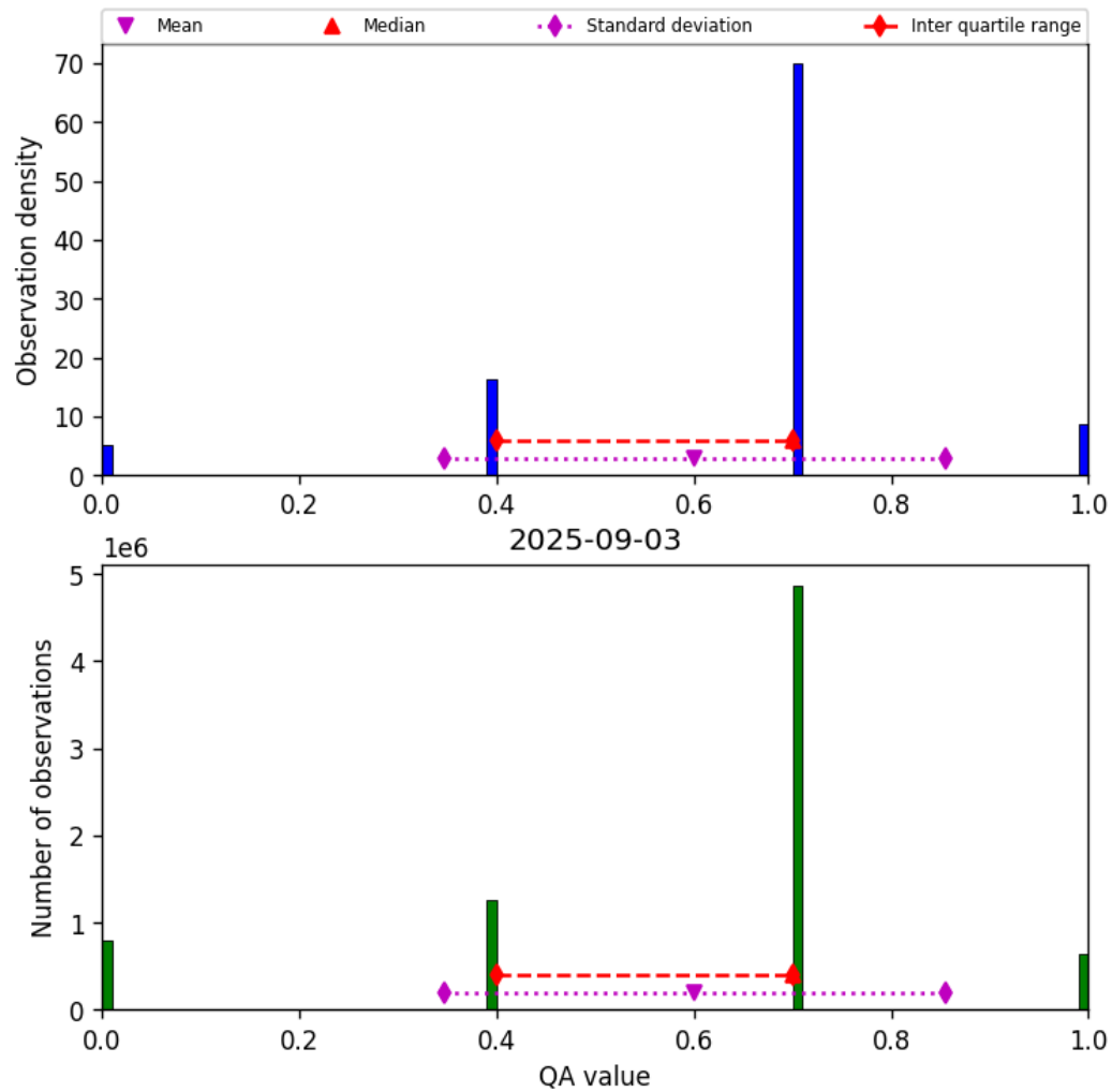
Figure 13: Histogram of “QA value” for 2025-09-03 to 2025-09-04
