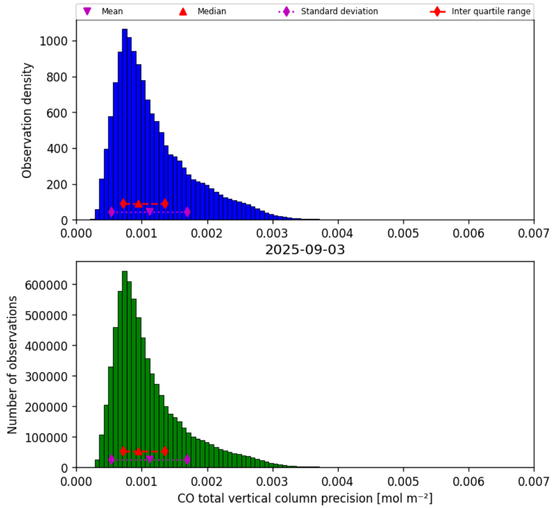
Figure 15: Histogram of “CO total vertical column precision” for 2025-09-03 to 2025-09-04
