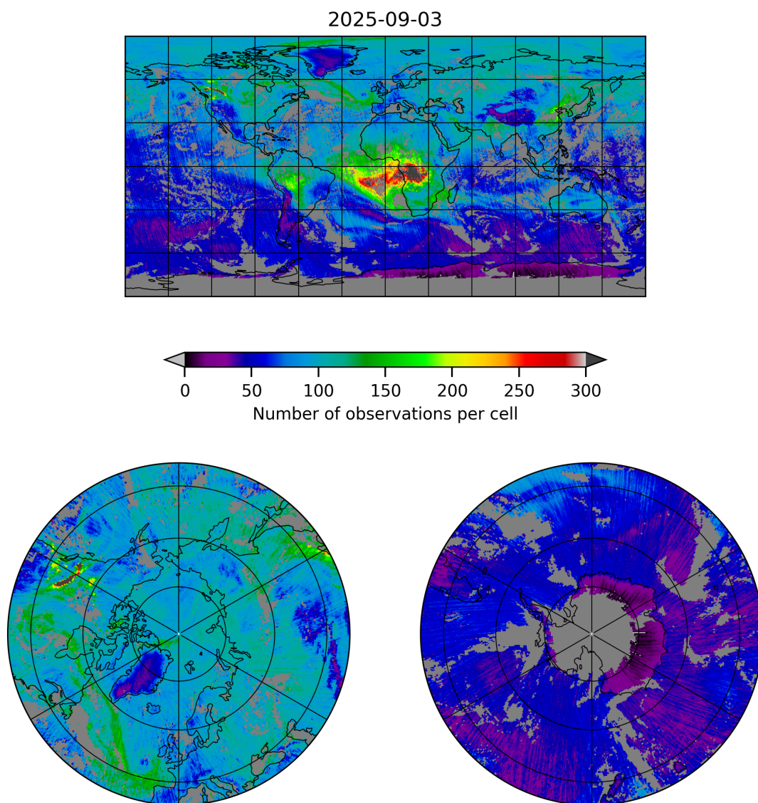
Figure 5: Map of the number of observations for 2025-09-03 to 2025-09-04
