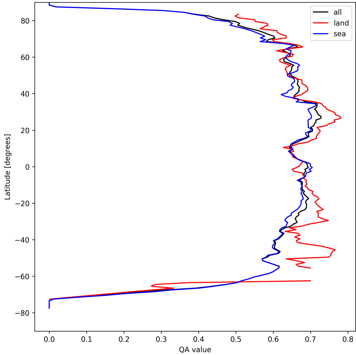
Figure 6: Zonal average of “QA value” for 2025-09-03 to 2025-09-04.
