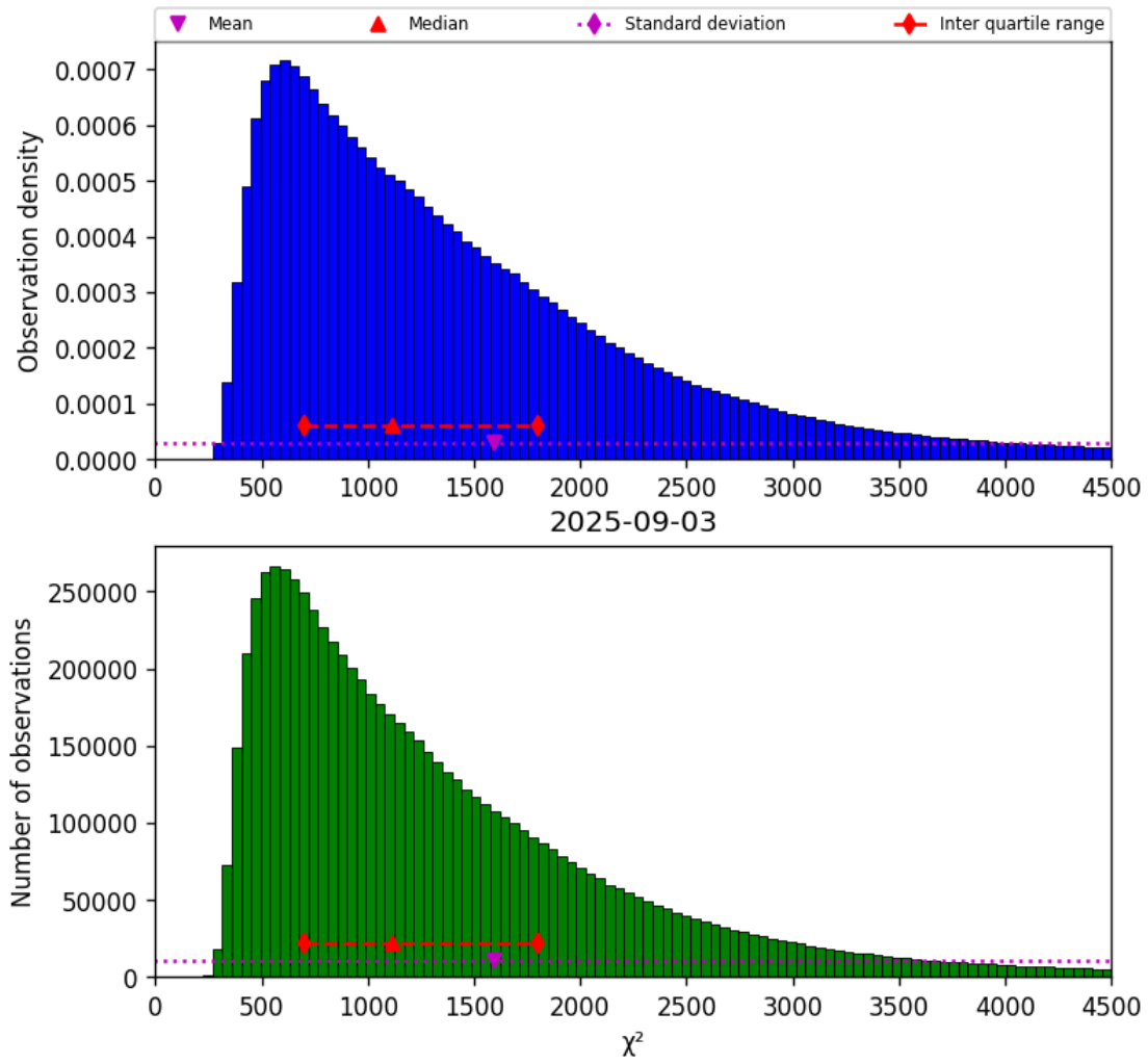
Figure 17: Histogram of “ \chi^2 ” for 2025-09-03 to 2025-09-04
