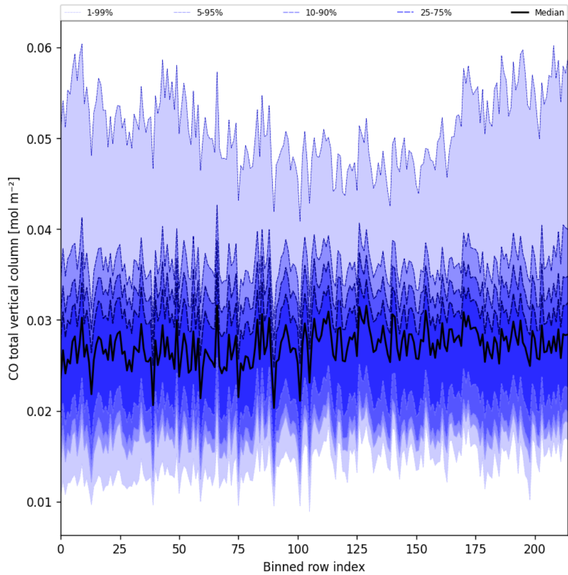
Figure 21: Along track statistics of “CO total vertical column” for 2025-09-03 to 2025-09-04
