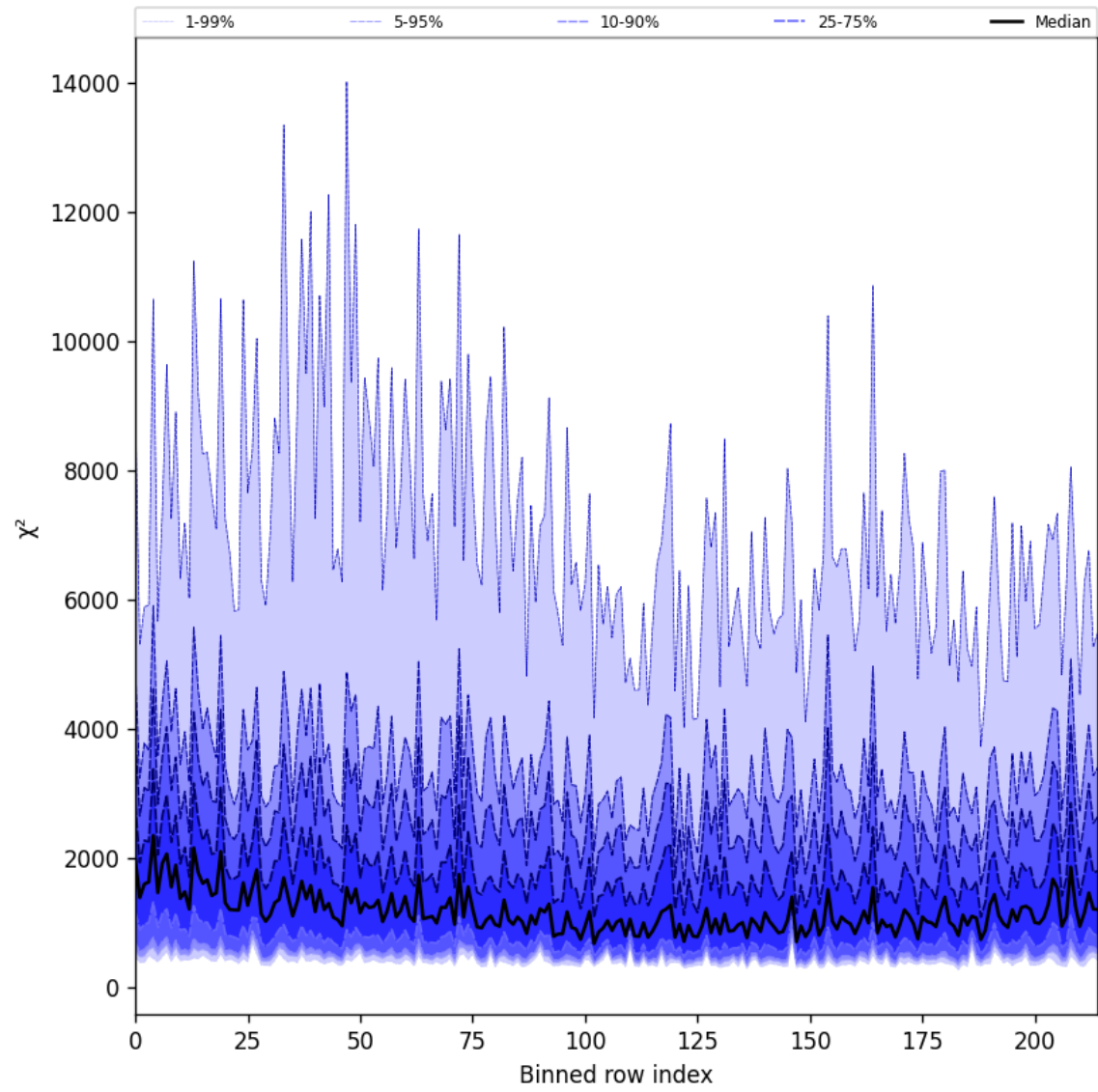
Figure 24: Along track statistics of “ \chi^2 ” for 2025-09-03 to 2025-09-04
