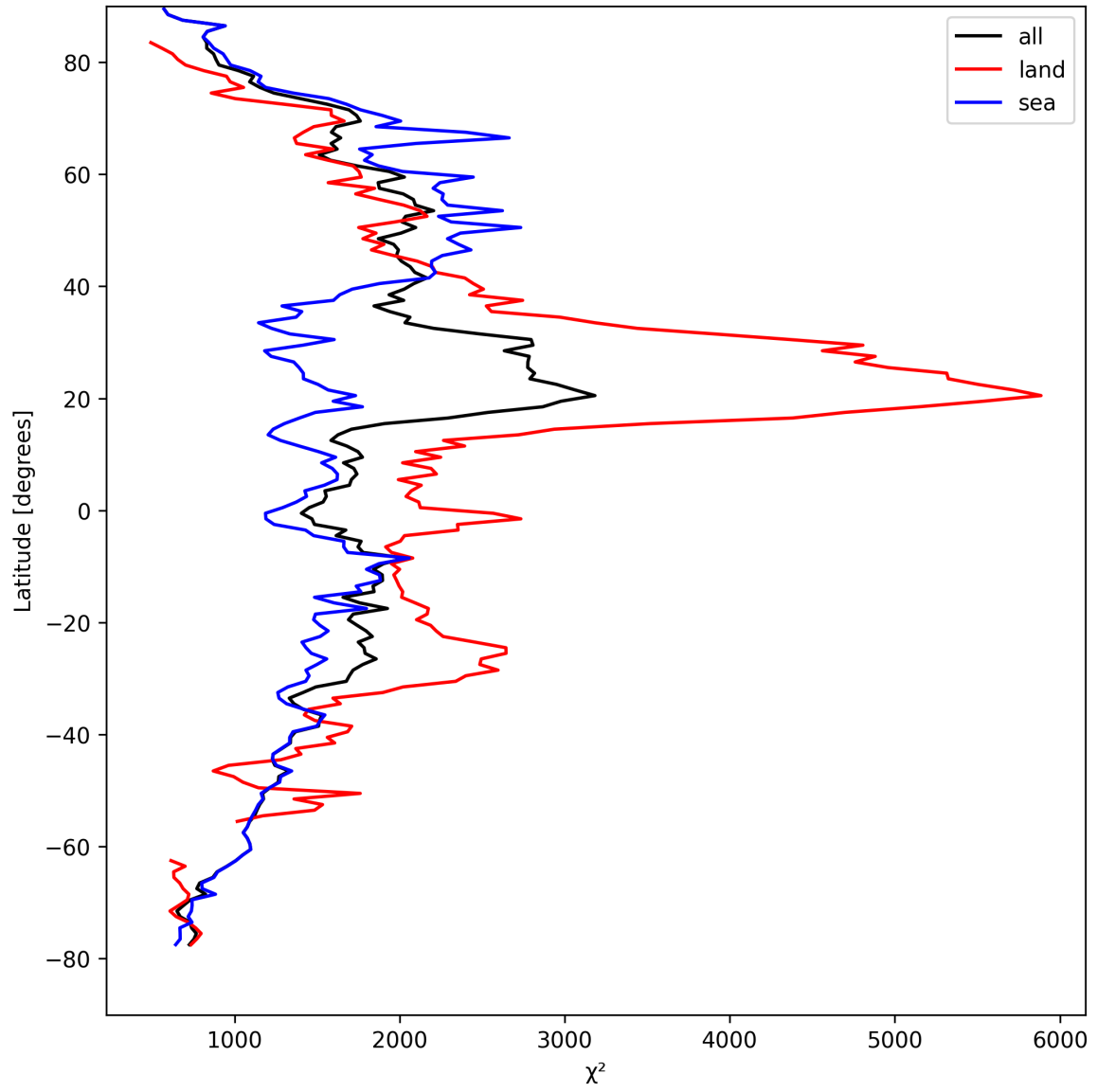
Figure 10: Zonal average of “ \chi^2 ” for 2025-09-03 to 2025-09-04.
