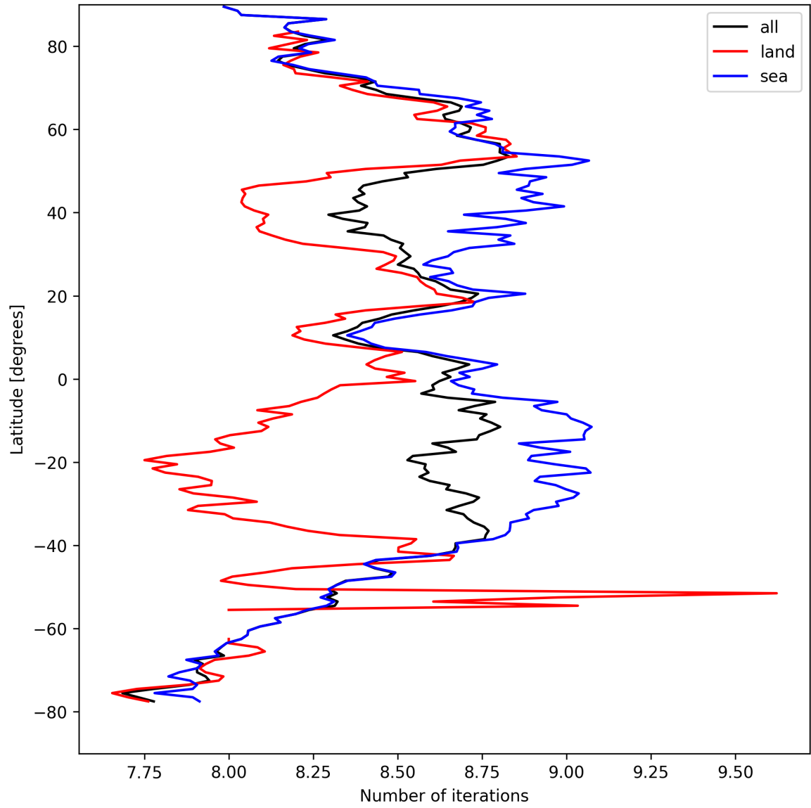
Figure 12: Zonal average of “Number of iterations” for 2025-09-03 to 2025-09-04.
