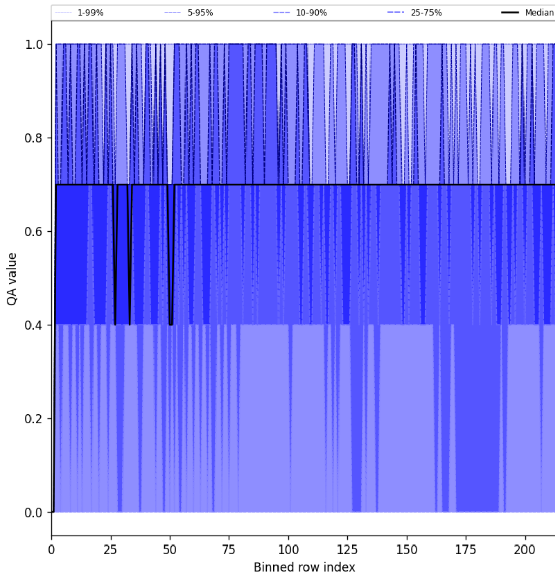
Figure 20: Along track statistics of “QA value” for 2025-09-03 to 2025-09-04
