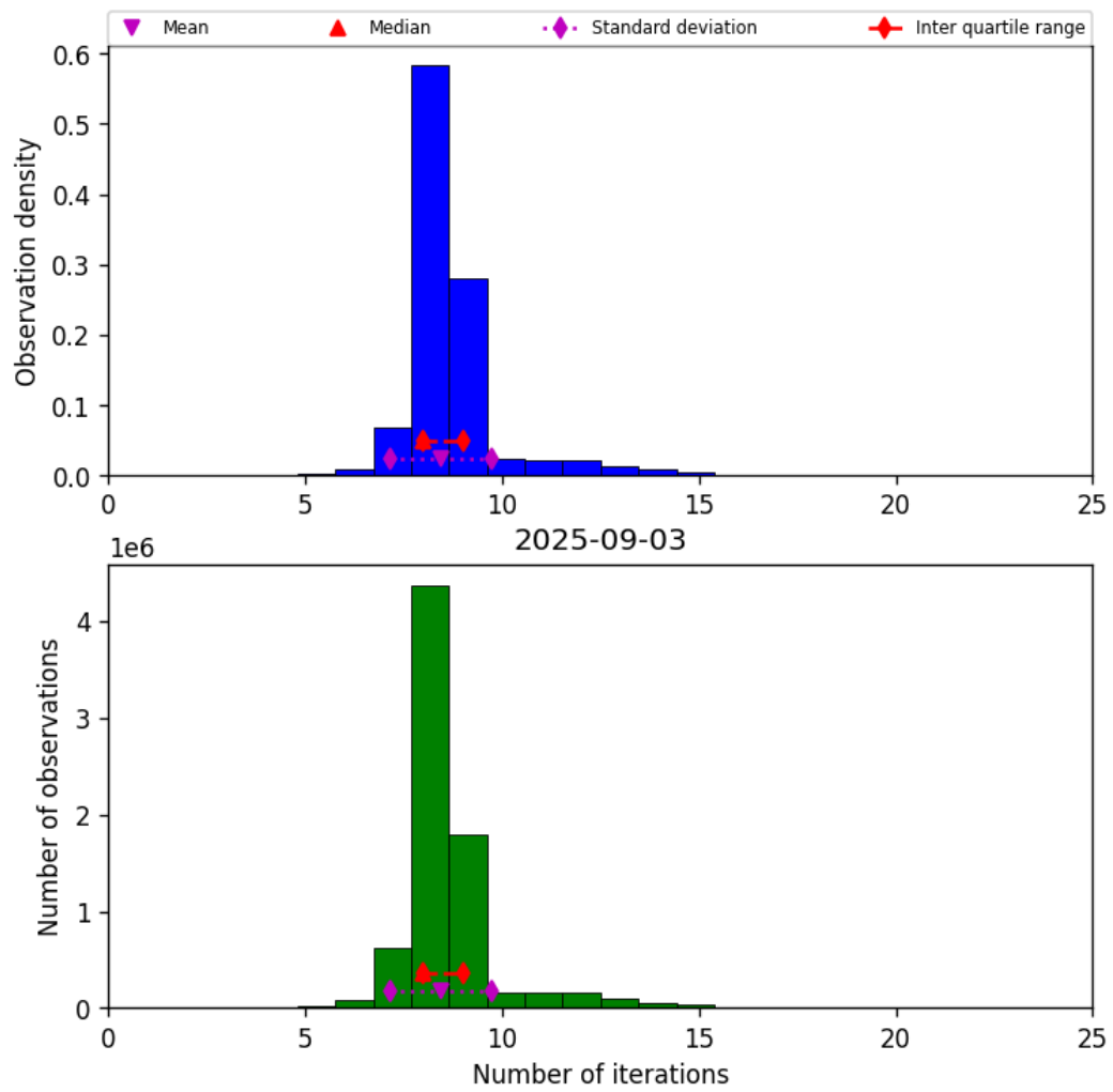
Figure 19: Histogram of “Number of iterations” for 2025-09-03 to 2025-09-04
