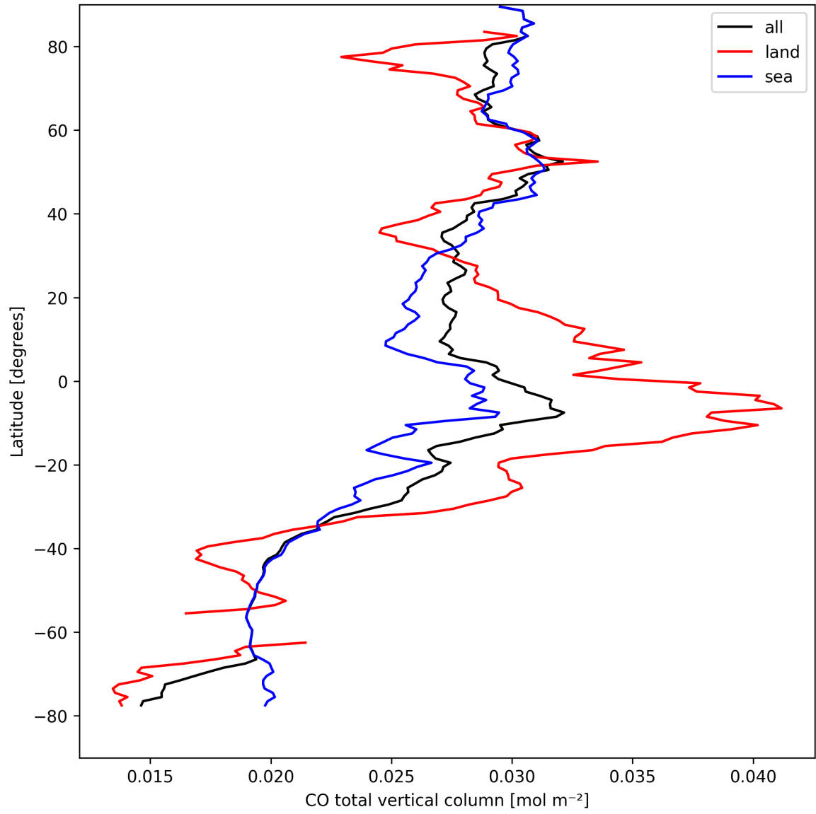
Figure 7: Zonal average of “CO total vertical column” for 2025-09-03 to 2025-09-04.
