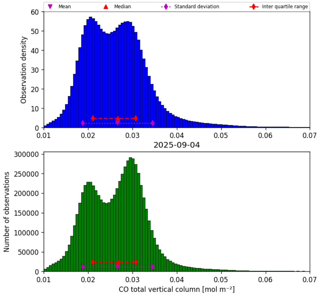
Figure 14: Histogram of “CO total vertical column” for 2025-09-04 to 2025-09-05
