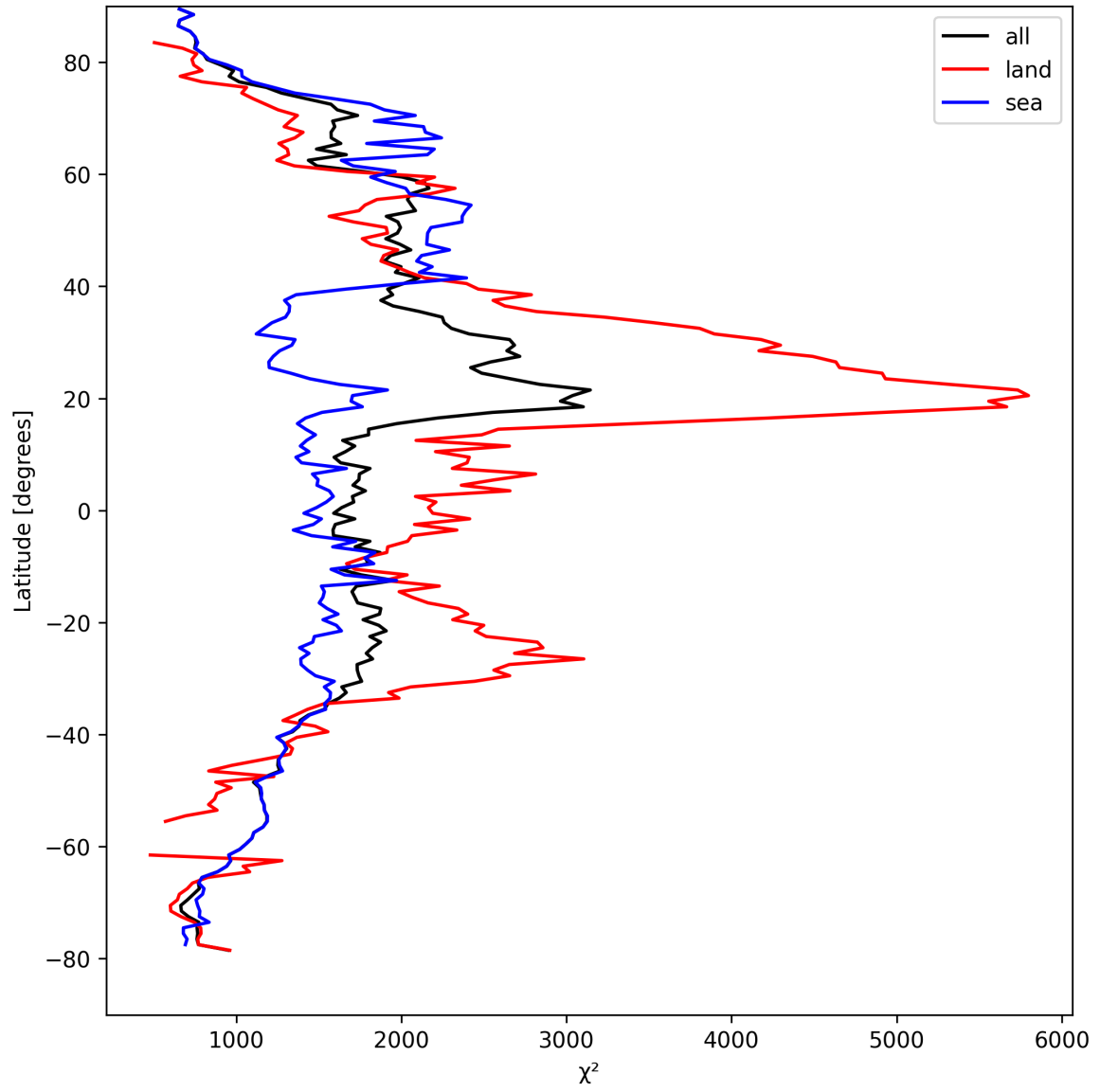
Figure 10: Zonal average of “ \chi^2 ” for 2025-09-04 to 2025-09-05.
