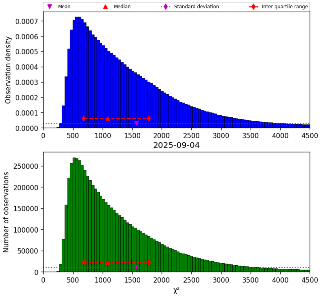
Figure 17: Histogram of “ \chi^2 ” for 2025-09-04 to 2025-09-05
