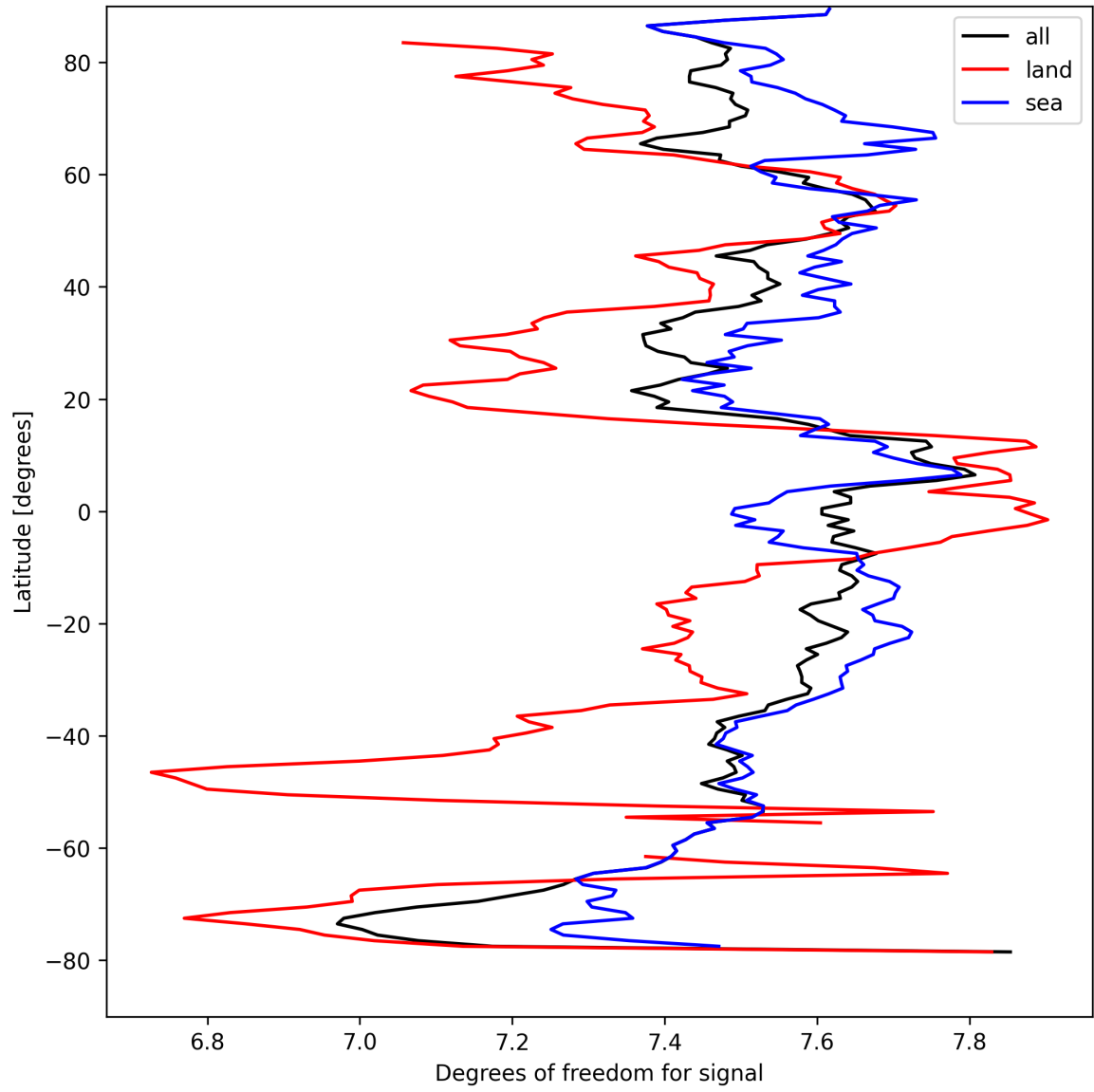
Figure 11: Zonal average of “Degrees of freedom for signal” for 2025-09-04 to 2025-09-05.
