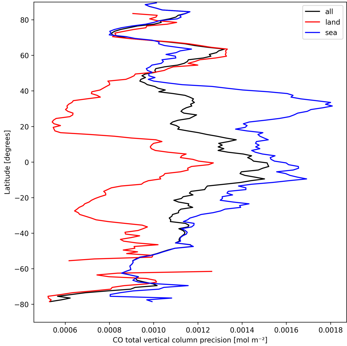
Figure 8: Zonal average of “CO total vertical column precision” for 2025-09-06 to 2025-09-07.
