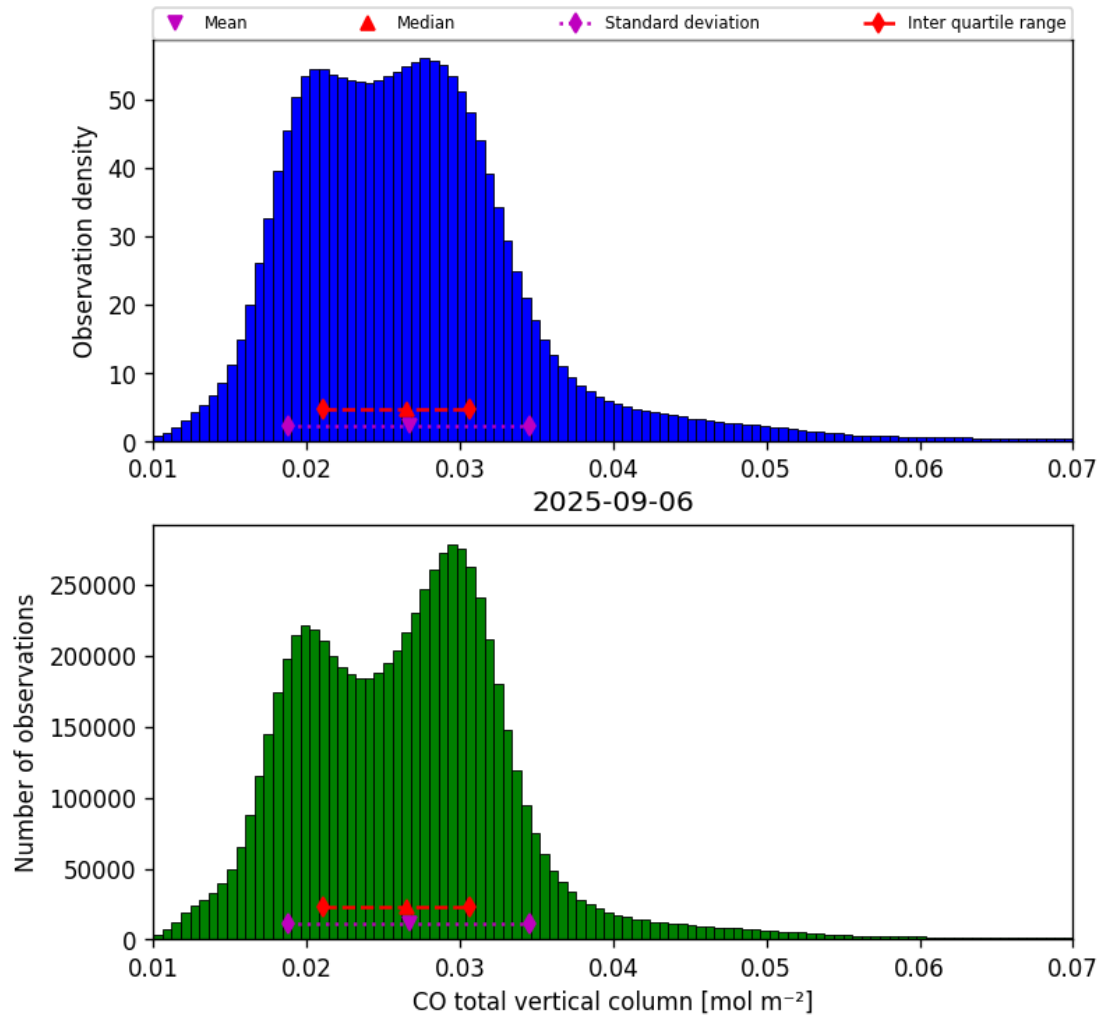
Figure 14: Histogram of “CO total vertical column” for 2025-09-06 to 2025-09-07
