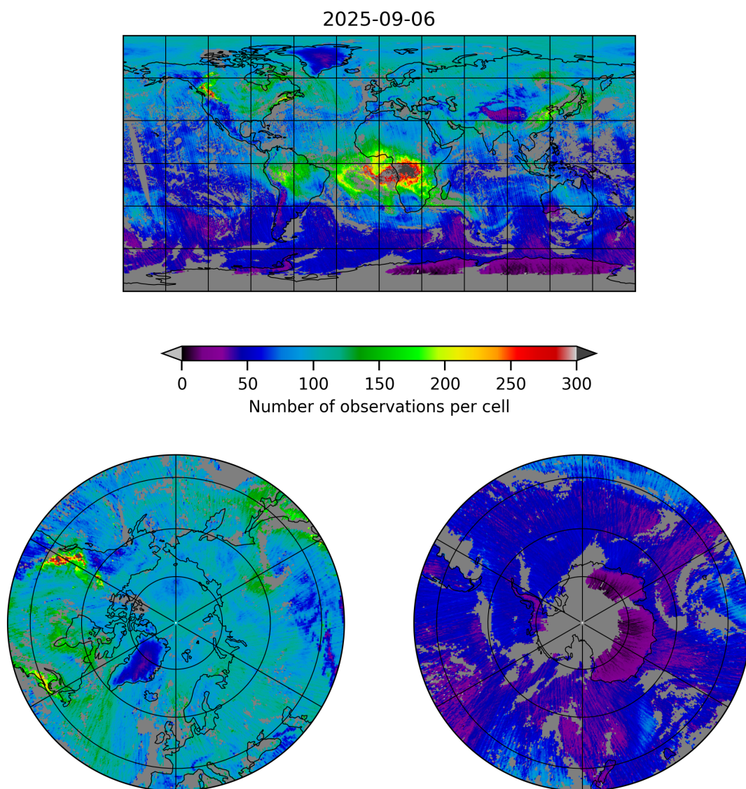
Figure 5: Map of the number of observations for 2025-09-06 to 2025-09-07
