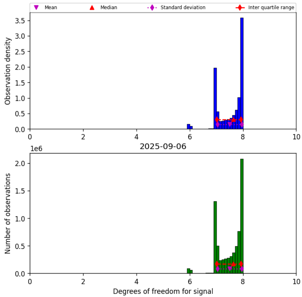
Figure 18: Histogram of “Degrees of freedom for signal” for 2025-09-06 to 2025-09-07
