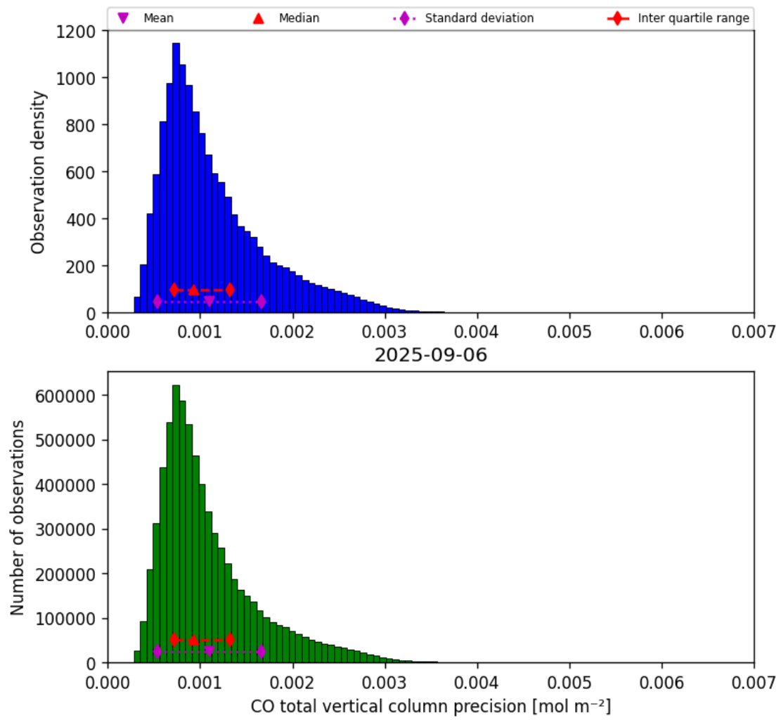
Figure 15: Histogram of “CO total vertical column precision” for 2025-09-06 to 2025-09-07
