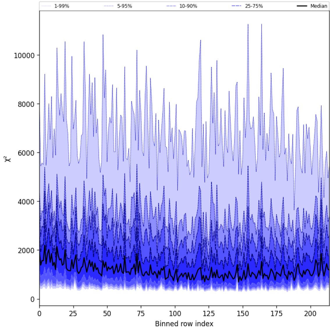
Figure 24: Along track statistics of “ \chi^2 ” for 2025-09-06 to 2025-09-07
