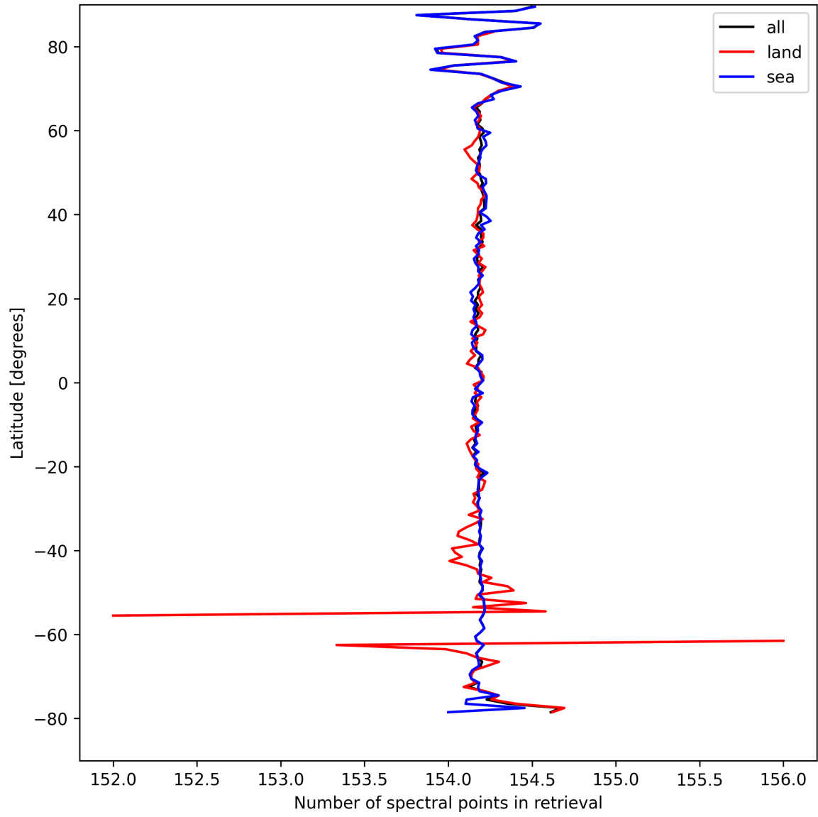
Figure 9: Zonal average of “Number of spectral points in retrieval” for 2025-09-06 to 2025-09-07.
