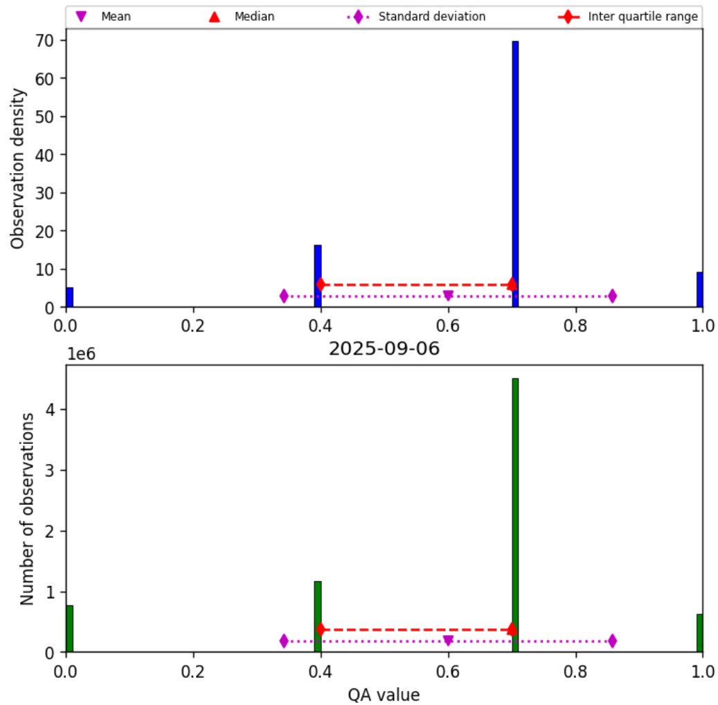
Figure 13: Histogram of “QA value” for 2025-09-06 to 2025-09-07
