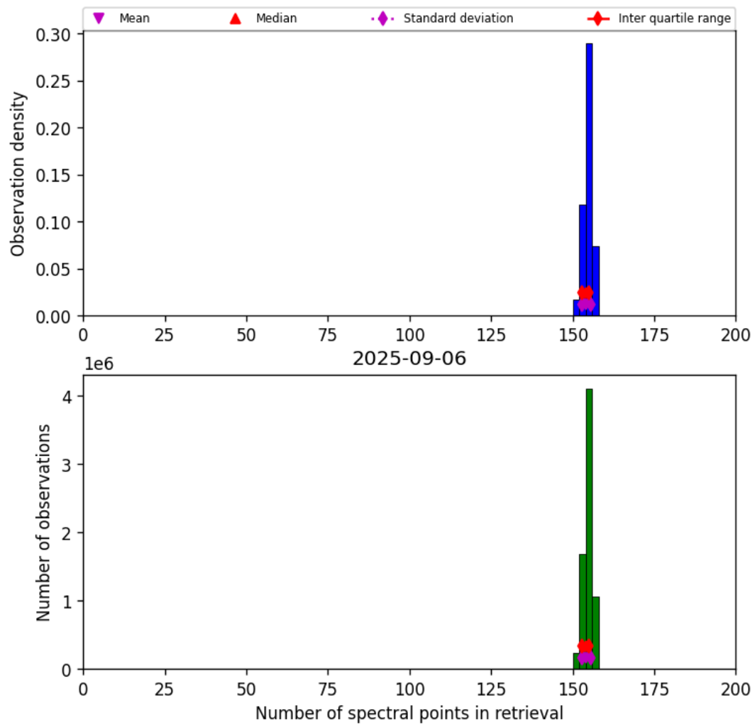
Figure 16: Histogram of “Number of spectral points in retrieval” for 2025-09-06 to 2025-09-07
