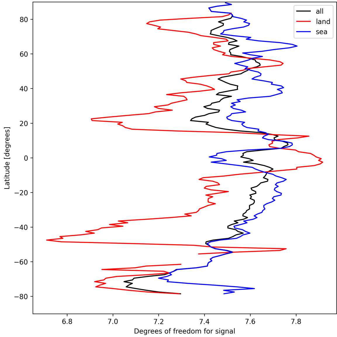
Figure 11: Zonal average of “Degrees of freedom for signal” for 2025-09-06 to 2025-09-07.
