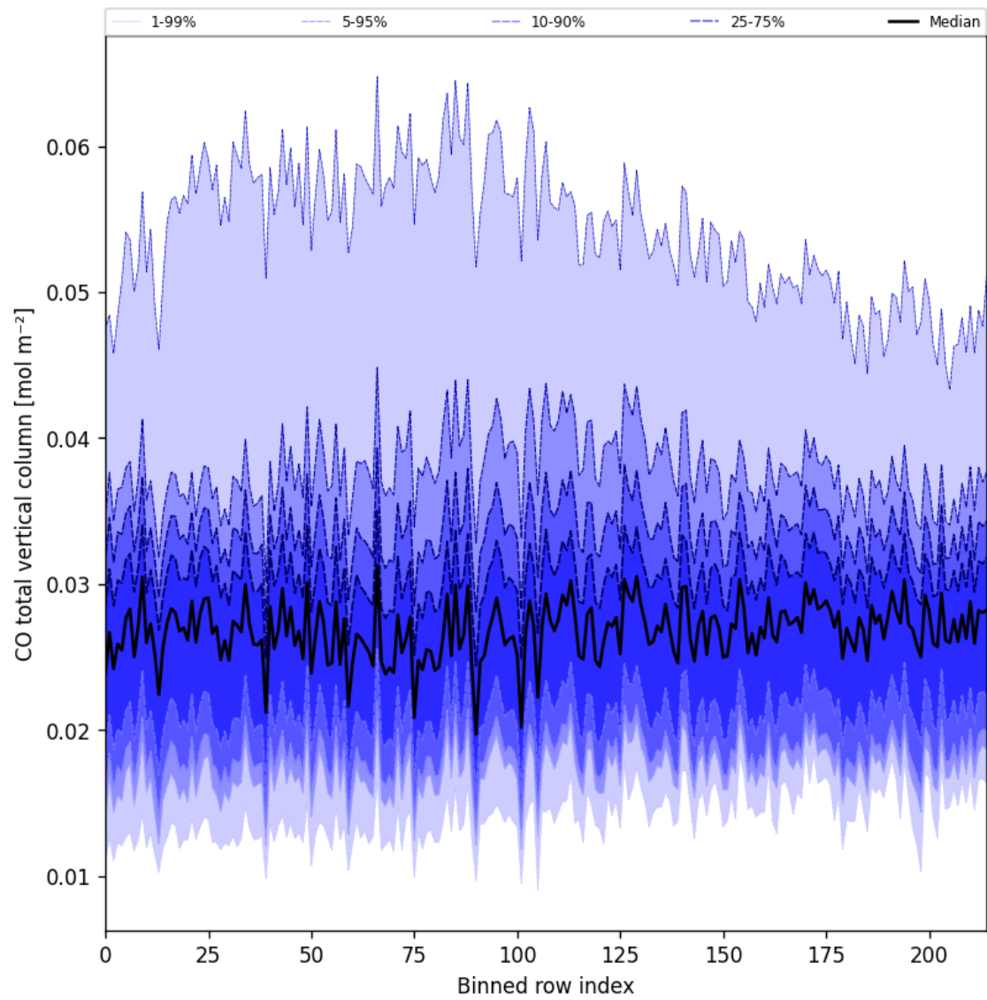
Figure 21: Along track statistics of “CO total vertical column” for 2025-09-06 to 2025-09-07
