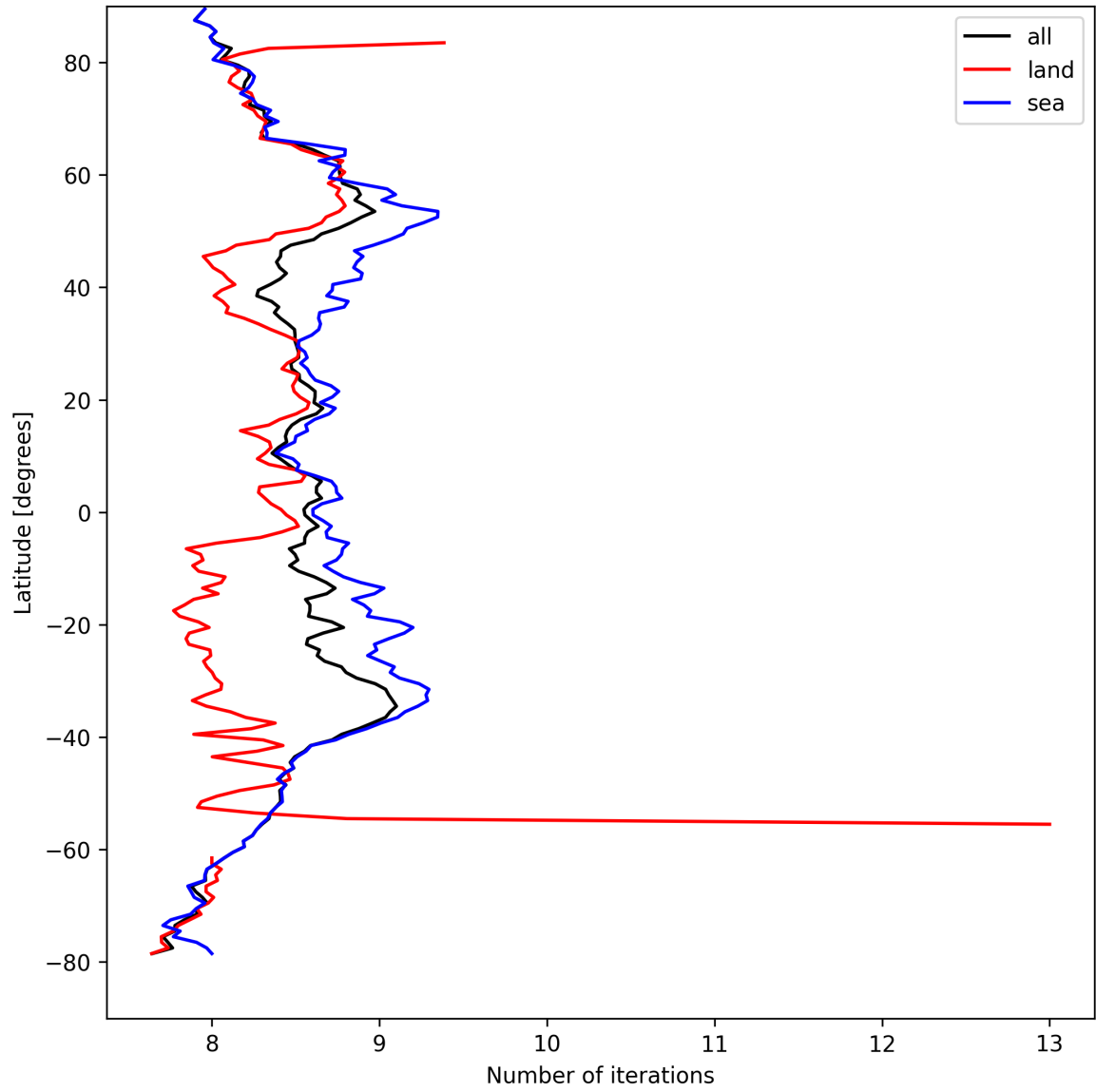
Figure 12: Zonal average of “Number of iterations” for 2025-09-06 to 2025-09-07.
