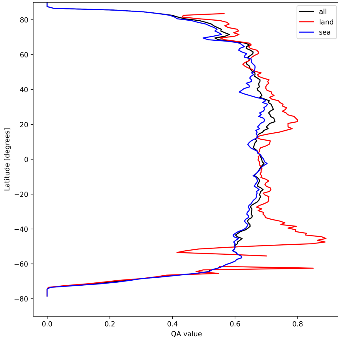
Figure 6: Zonal average of “QA value” for 2025-09-06 to 2025-09-07.
