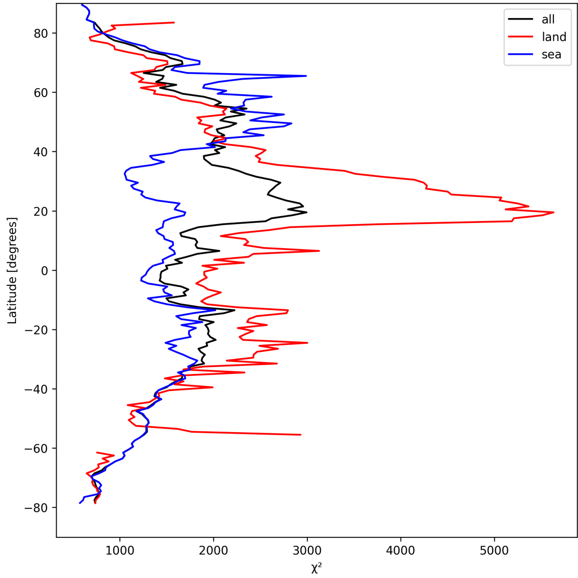
Figure 10: Zonal average of “ \chi^2 ” for 2025-09-06 to 2025-09-07.
