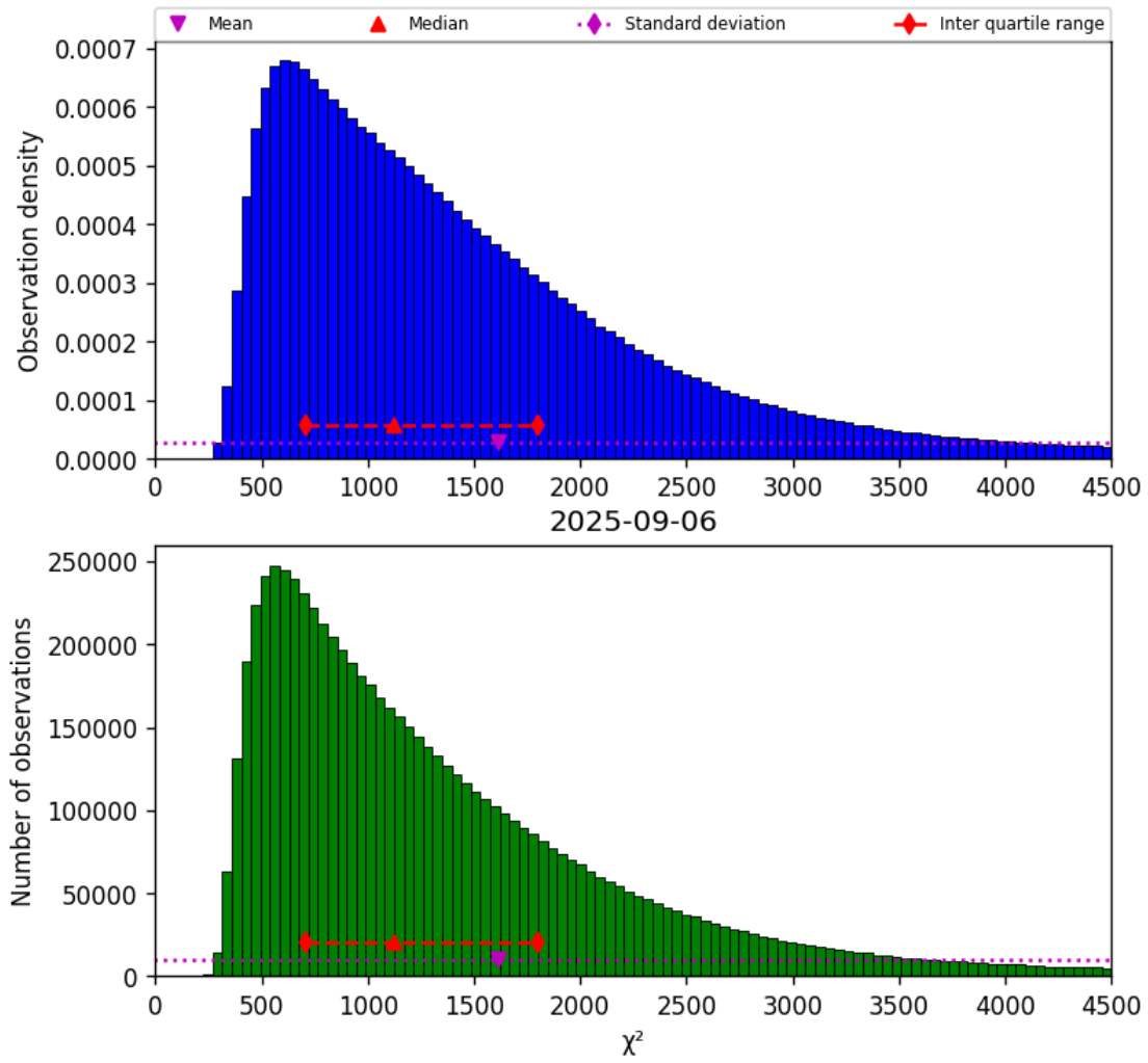
Figure 17: Histogram of " \chi^2 " for 2025-09-06 to 2025-09-07
