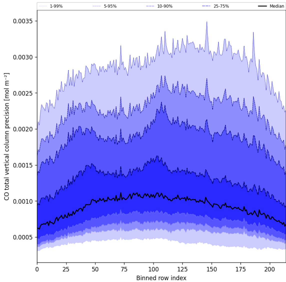
Figure 22: Along track statistics of “CO total vertical column precision” for 2025-09-06 to 2025-09-07
