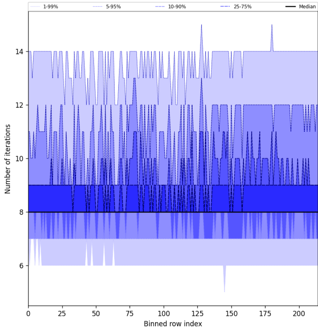
Figure 26: Along track statistics of “Number of iterations” for 2025-09-06 to 2025-09-07
