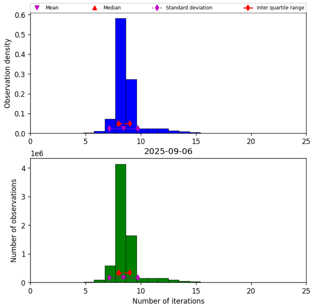
Figure 19: Histogram of “Number of iterations” for 2025-09-06 to 2025-09-07
