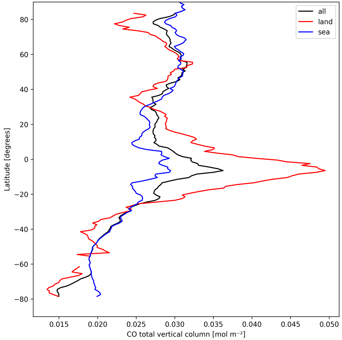
Figure 7: Zonal average of “CO total vertical column” for 2025-09-06 to 2025-09-07.
