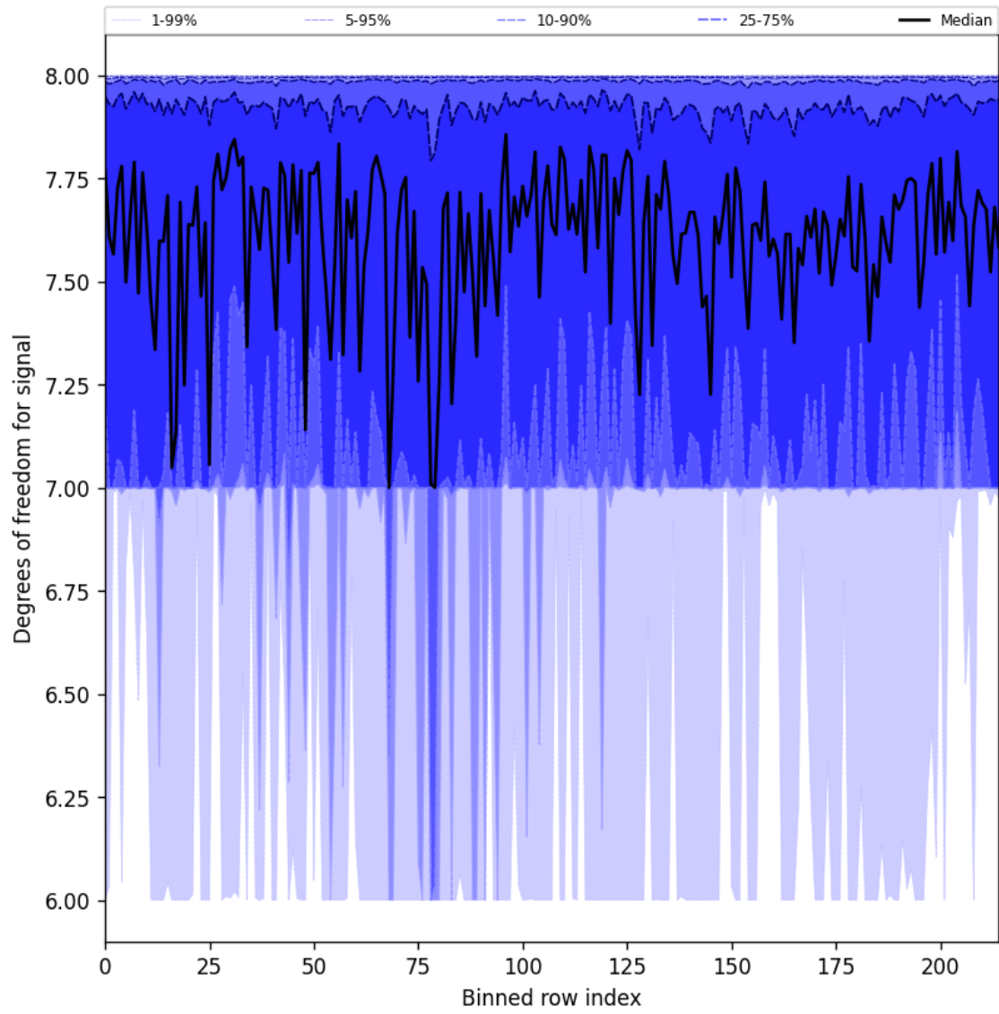
Figure 25: Along track statistics of “Degrees of freedom for signal” for 2025-09-06 to 2025-09-07
