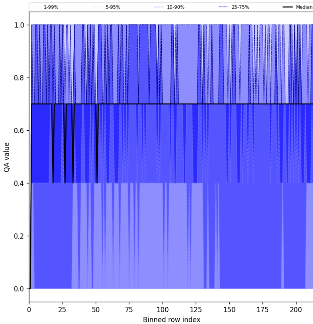
Figure 20: Along track statistics of “QA value” for 2025-09-06 to 2025-09-07
