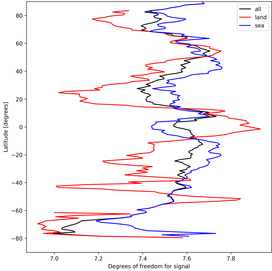
Figure 11: Zonal average of “Degrees of freedom for signal” for 2025-09-07 to 2025-09-07.
