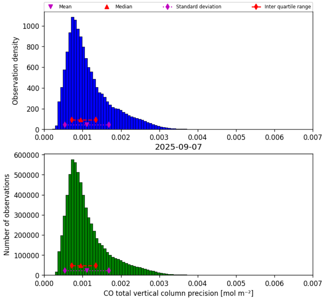
Figure 15: Histogram of “CO total vertical column precision” for 2025-09-07 to 2025-09-07
