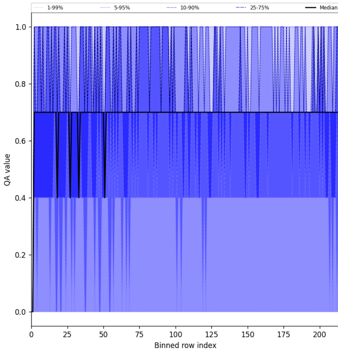
Figure 20: Along track statistics of “QA value” for 2025-09-07 to 2025-09-07
