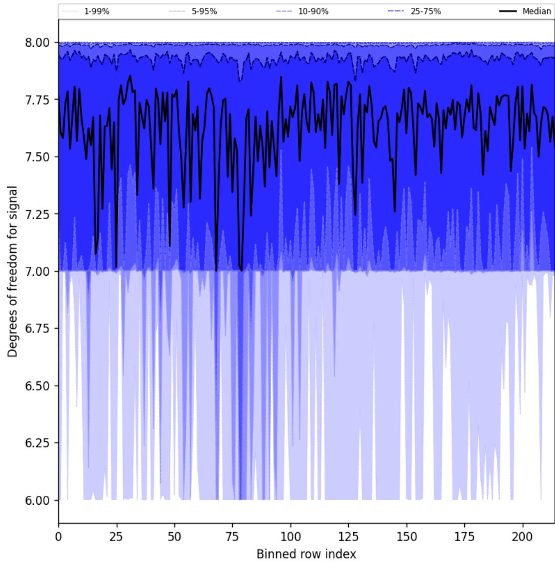
Figure 25: Along track statistics of “Degrees of freedom for signal” for 2025-09-07 to 2025-09-07
