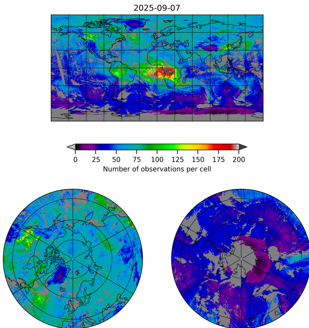
Figure 5: Map of the number of observations for 2025-09-07 to 2025-09-07
