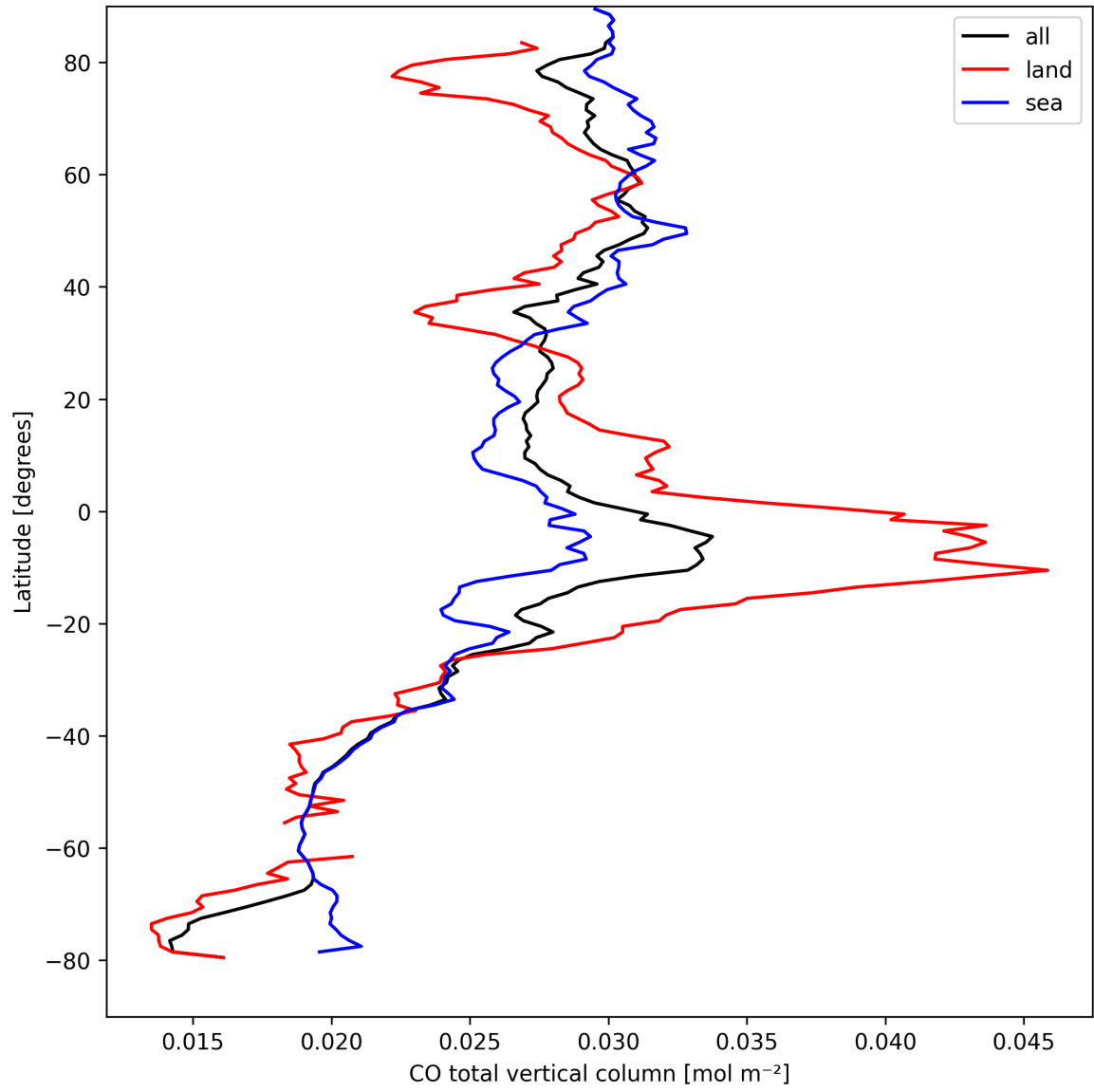
Figure 7: Zonal average of “CO total vertical column” for 2025-09-07 to 2025-09-07.
