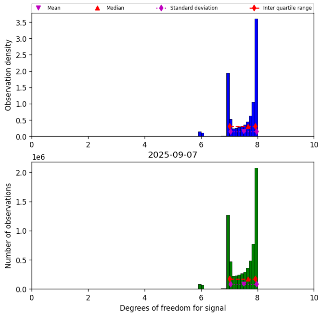
Figure 18: Histogram of “Degrees of freedom for signal” for 2025-09-07 to 2025-09-07
