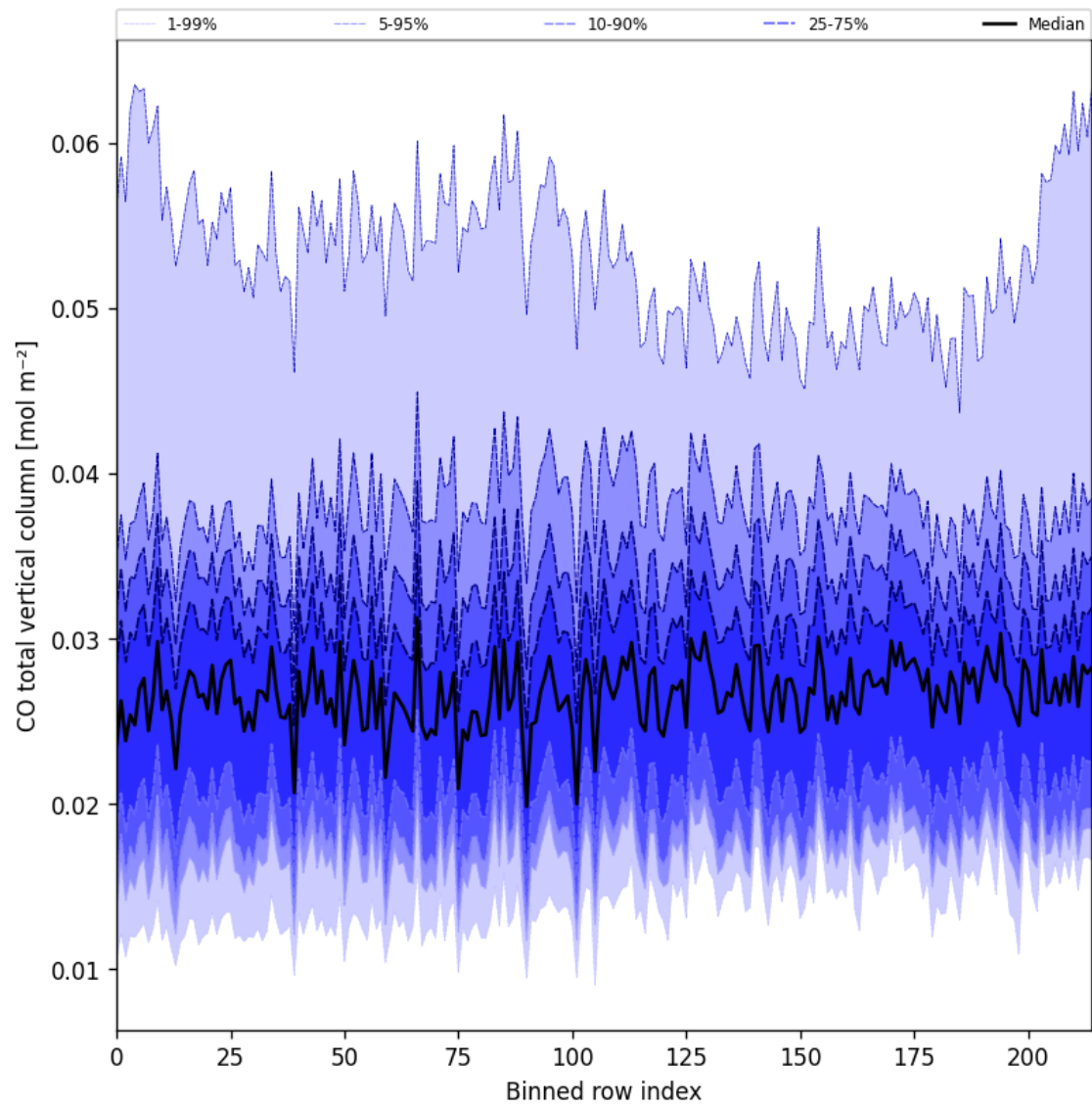
Figure 21: Along track statistics of “CO total vertical column” for 2025-09-07 to 2025-09-07
