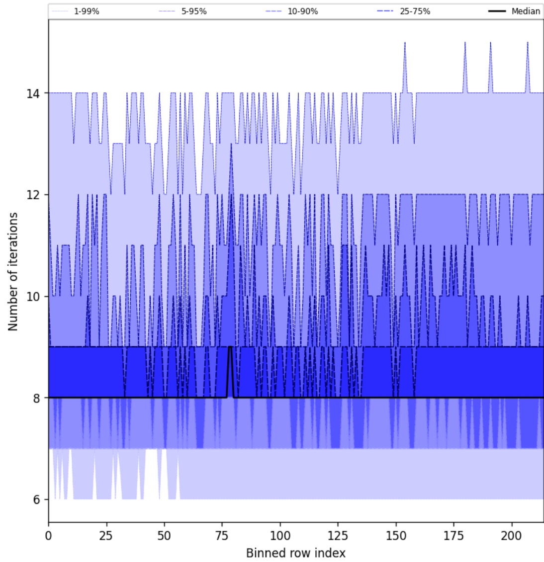
Figure 26: Along track statistics of “Number of iterations” for 2025-09-07 to 2025-09-07
