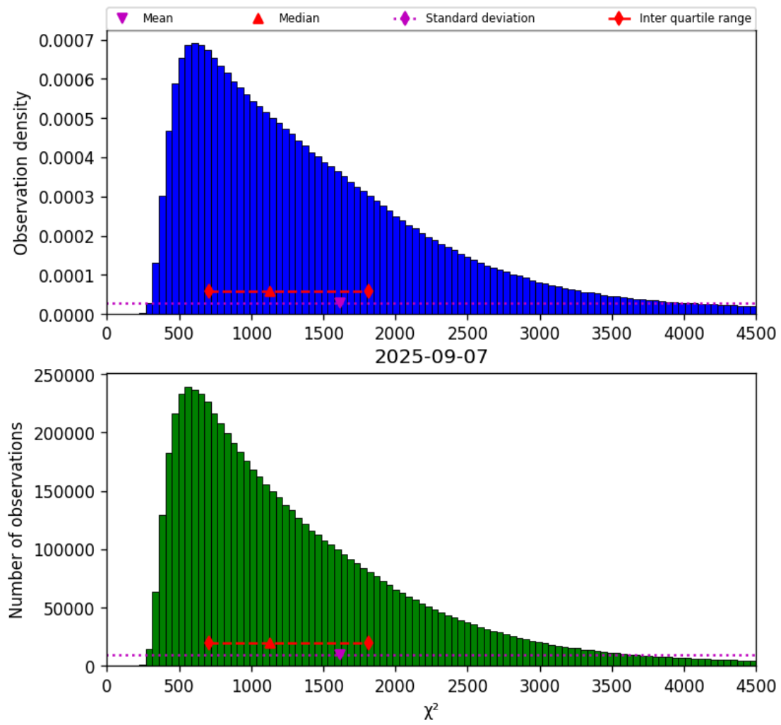
Figure 17: Histogram of " \chi^2 " for 2025-09-07 to 2025-09-07
