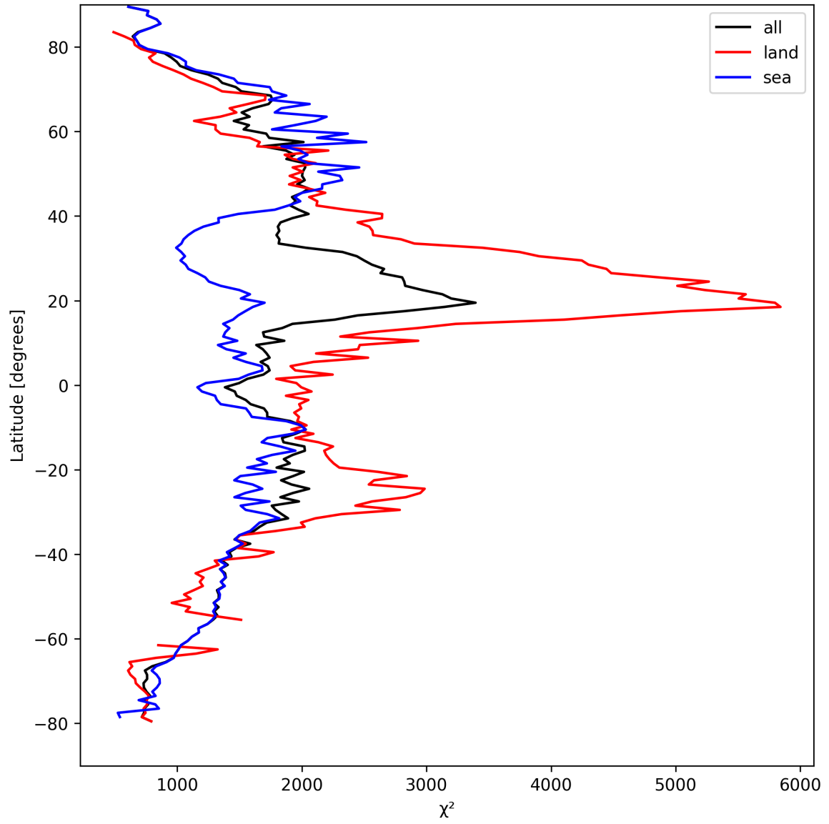
Figure 10: Zonal average of “ \chi^2 ” for 2025-09-07 to 2025-09-07.
