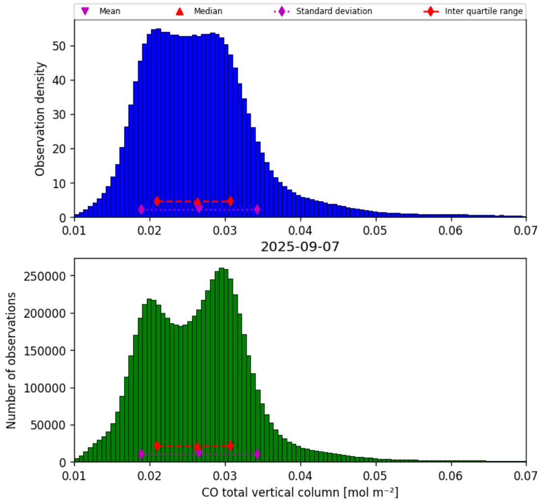
Figure 14: Histogram of “CO total vertical column” for 2025-09-07 to 2025-09-07
