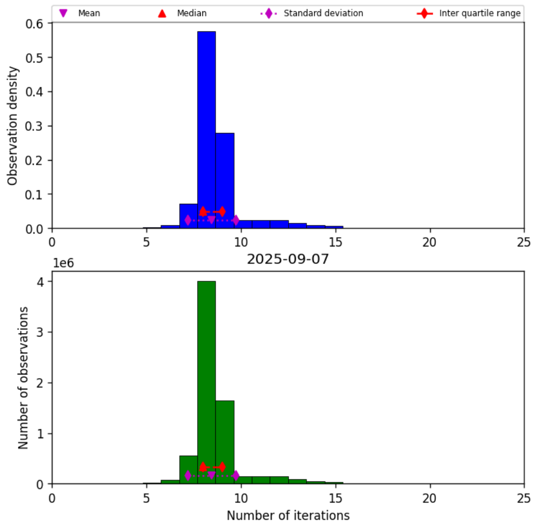
Figure 19: Histogram of “Number of iterations” for 2025-09-07 to 2025-09-07
