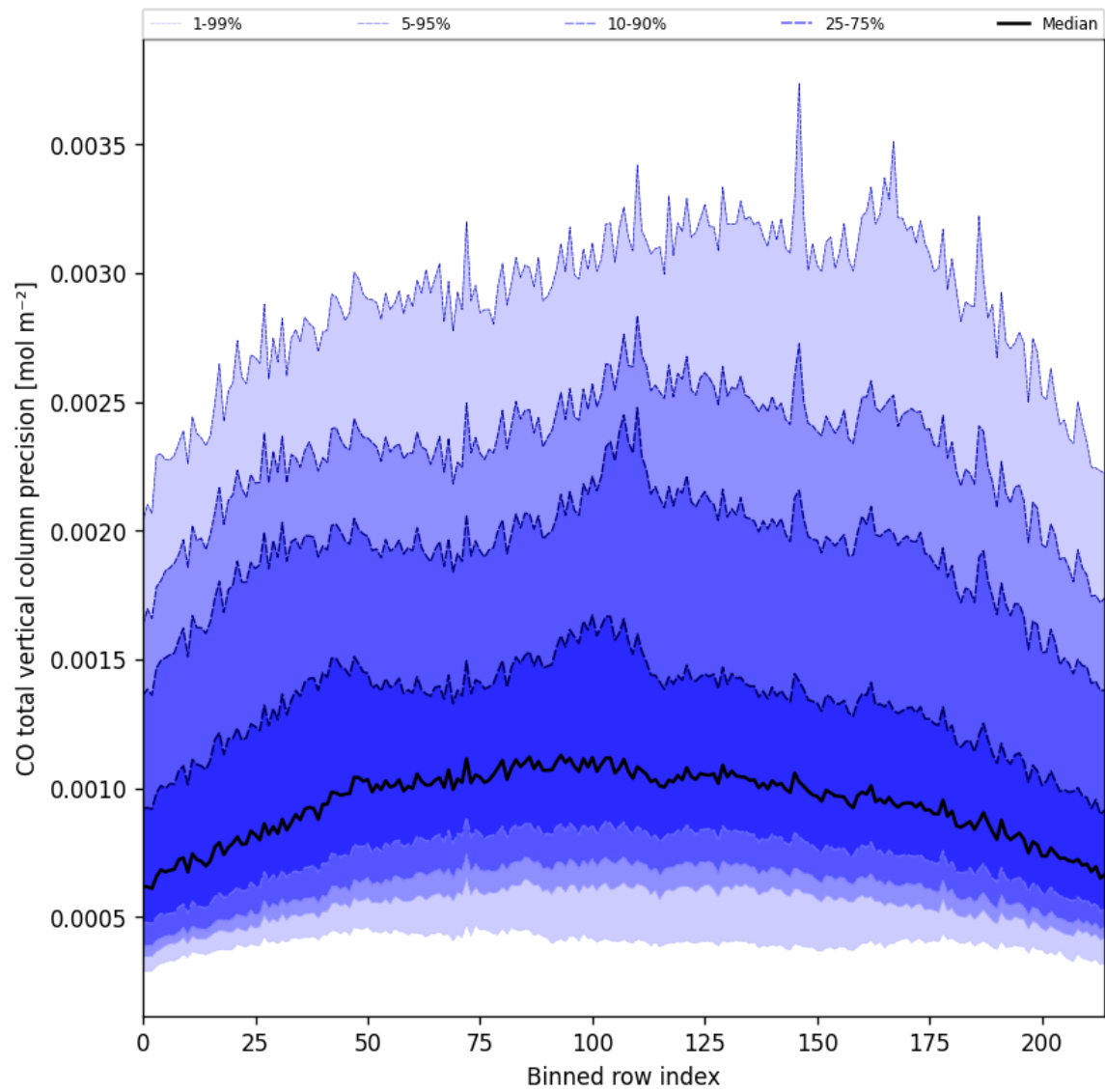
Figure 22: Along track statistics of “CO total vertical column precision” for 2025-09-07 to 2025-09-07
