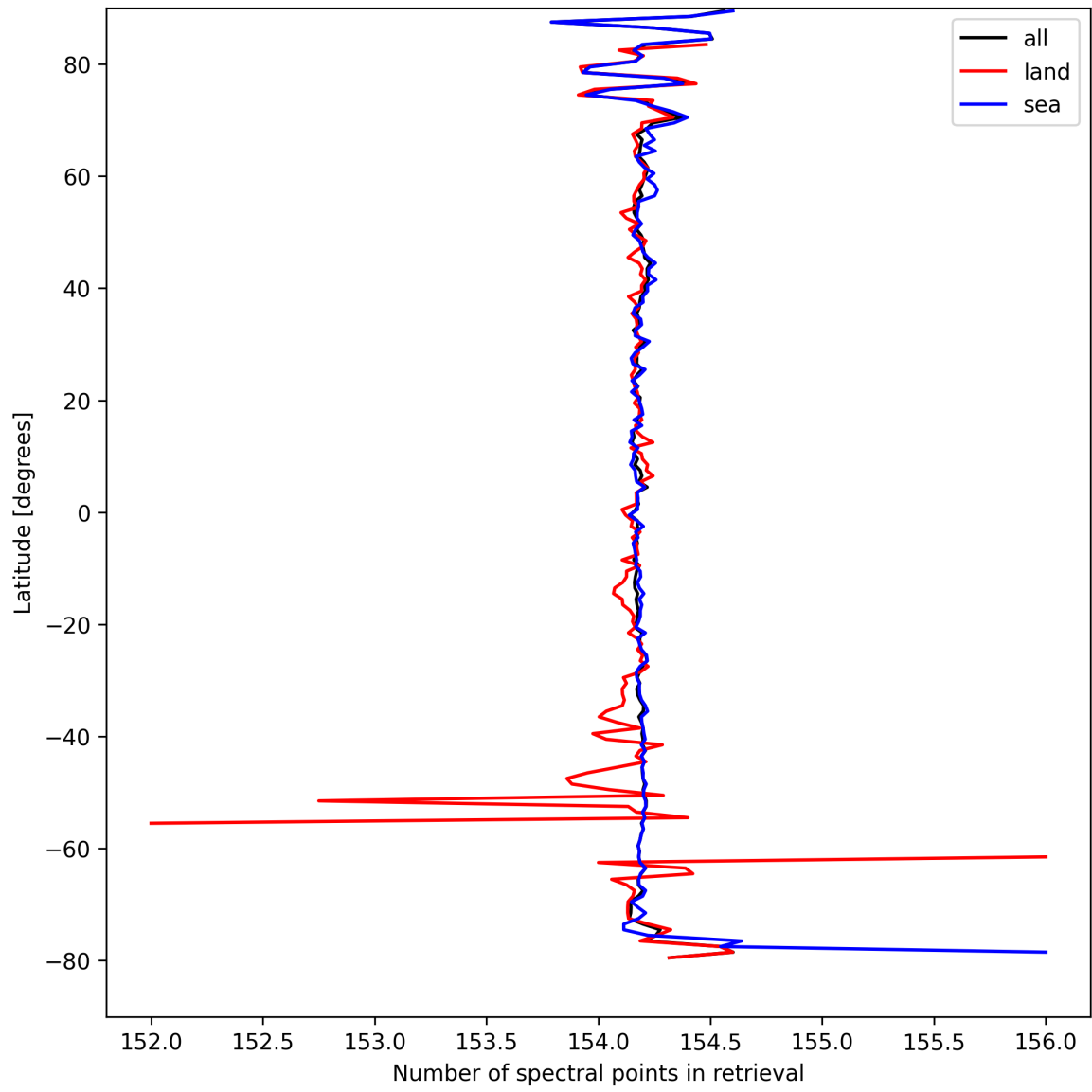
Figure 9: Zonal average of “Number of spectral points in retrieval” for 2025-09-07 to 2025-09-07.
