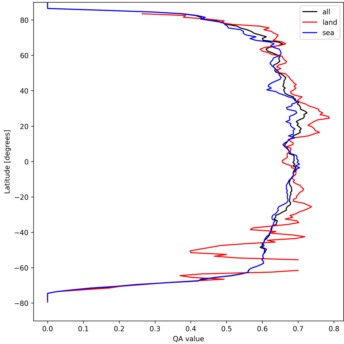
Figure 6: Zonal average of “QA value” for 2025-09-07 to 2025-09-07.
