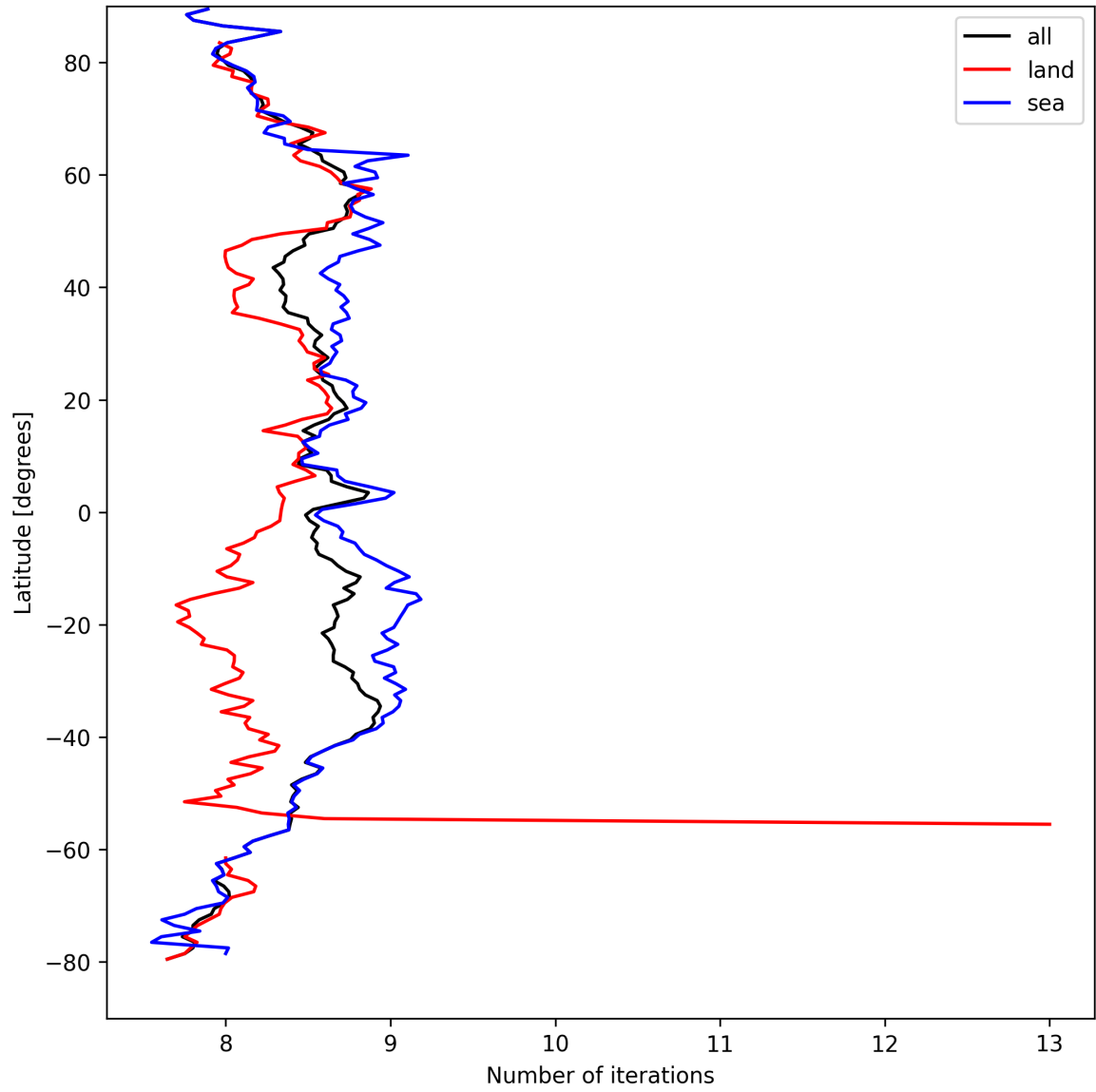
Figure 12: Zonal average of “Number of iterations” for 2025-09-07 to 2025-09-07.
