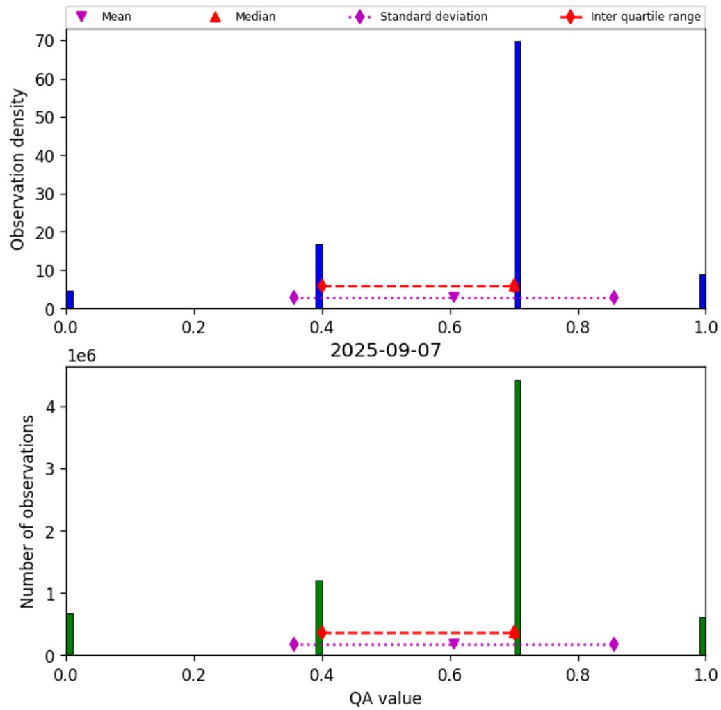
Figure 13: Histogram of “QA value” for 2025-09-07 to 2025-09-07
