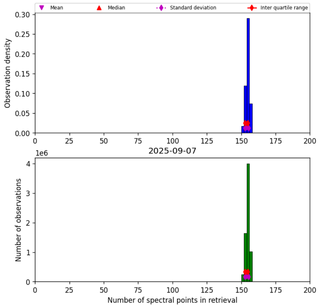
Figure 16: Histogram of “Number of spectral points in retrieval” for 2025-09-07 to 2025-09-07
