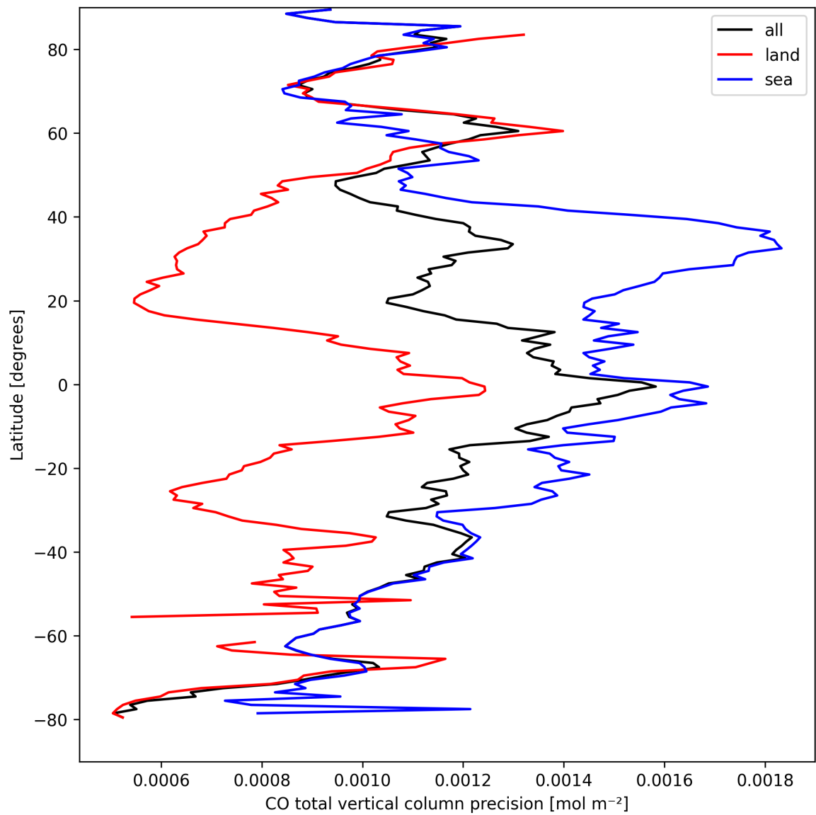
Figure 8: Zonal average of “CO total vertical column precision” for 2025-09-07 to 2025-09-07.
