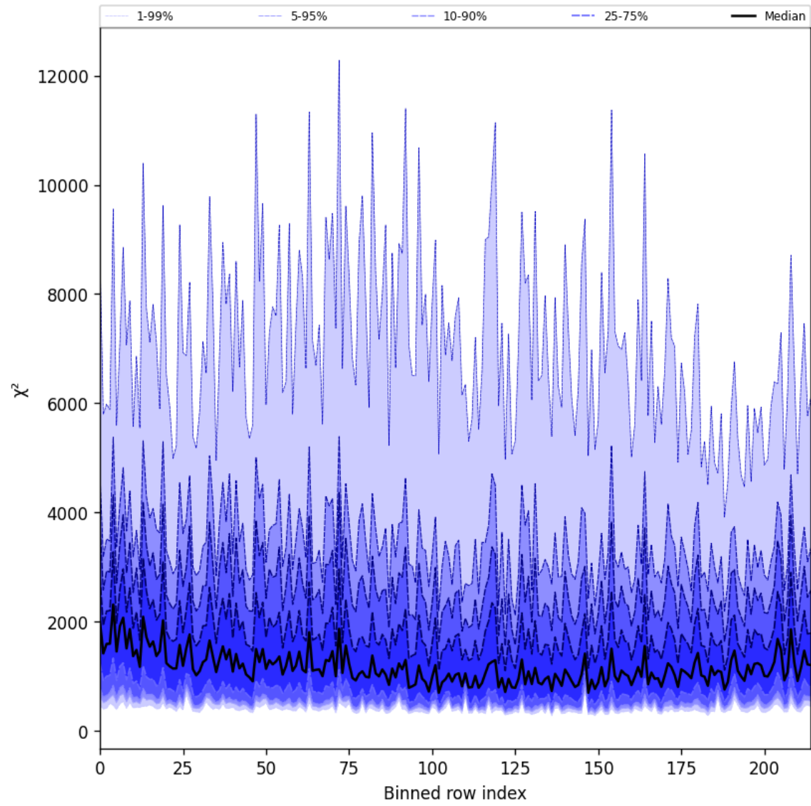
Figure 24: Along track statistics of “ \chi^2 ” for 2025-09-07 to 2025-09-07
