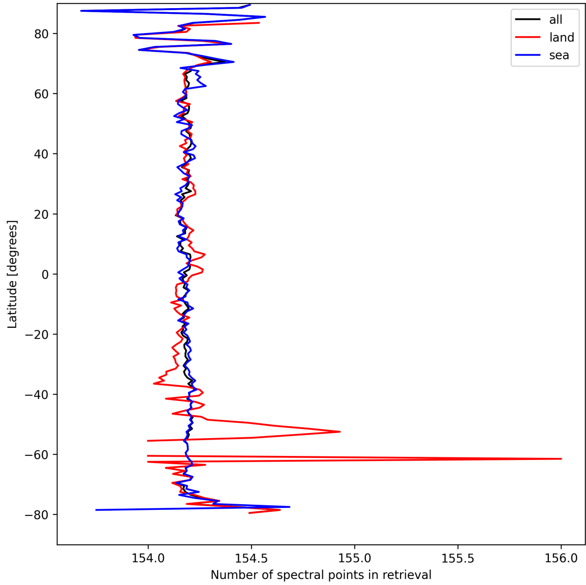
Figure 9: Zonal average of “Number of spectral points in retrieval” for 2025-09-08 to 2025-09-08.
