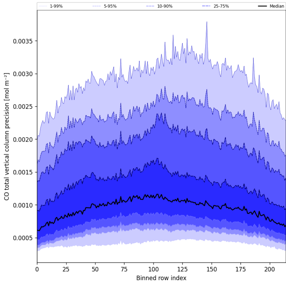
Figure 22: Along track statistics of “CO total vertical column precision” for 2025-09-08 to 2025-09-08
