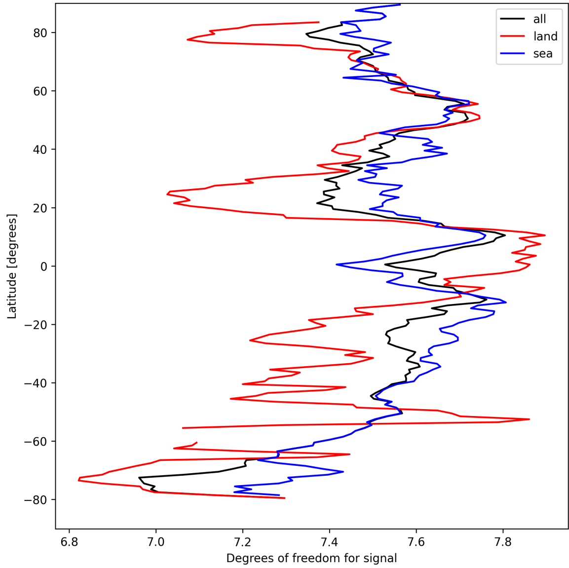
Figure 11: Zonal average of “Degrees of freedom for signal” for 2025-09-08 to 2025-09-08.
