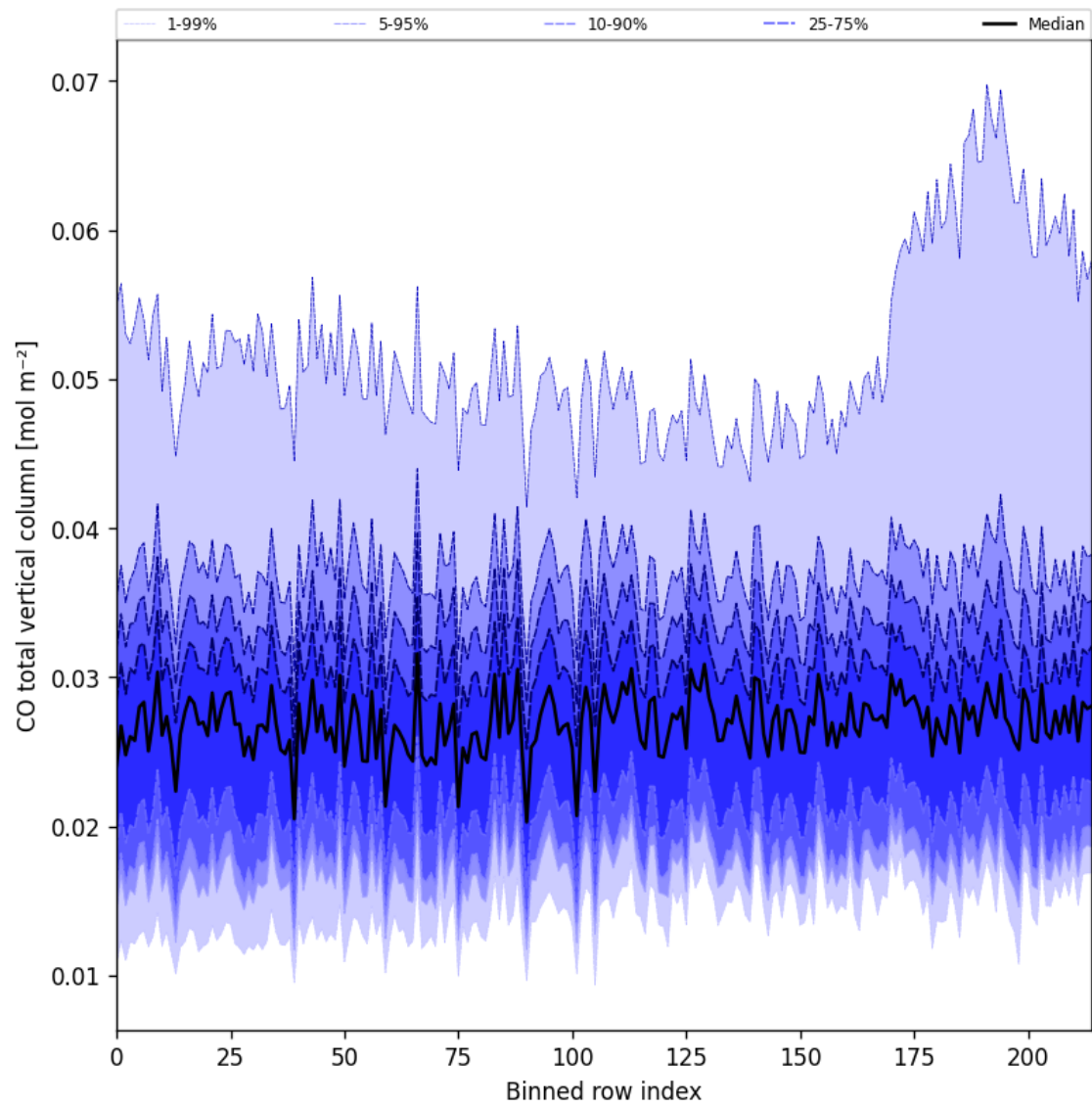
Figure 21: Along track statistics of “CO total vertical column” for 2025-09-08 to 2025-09-08
