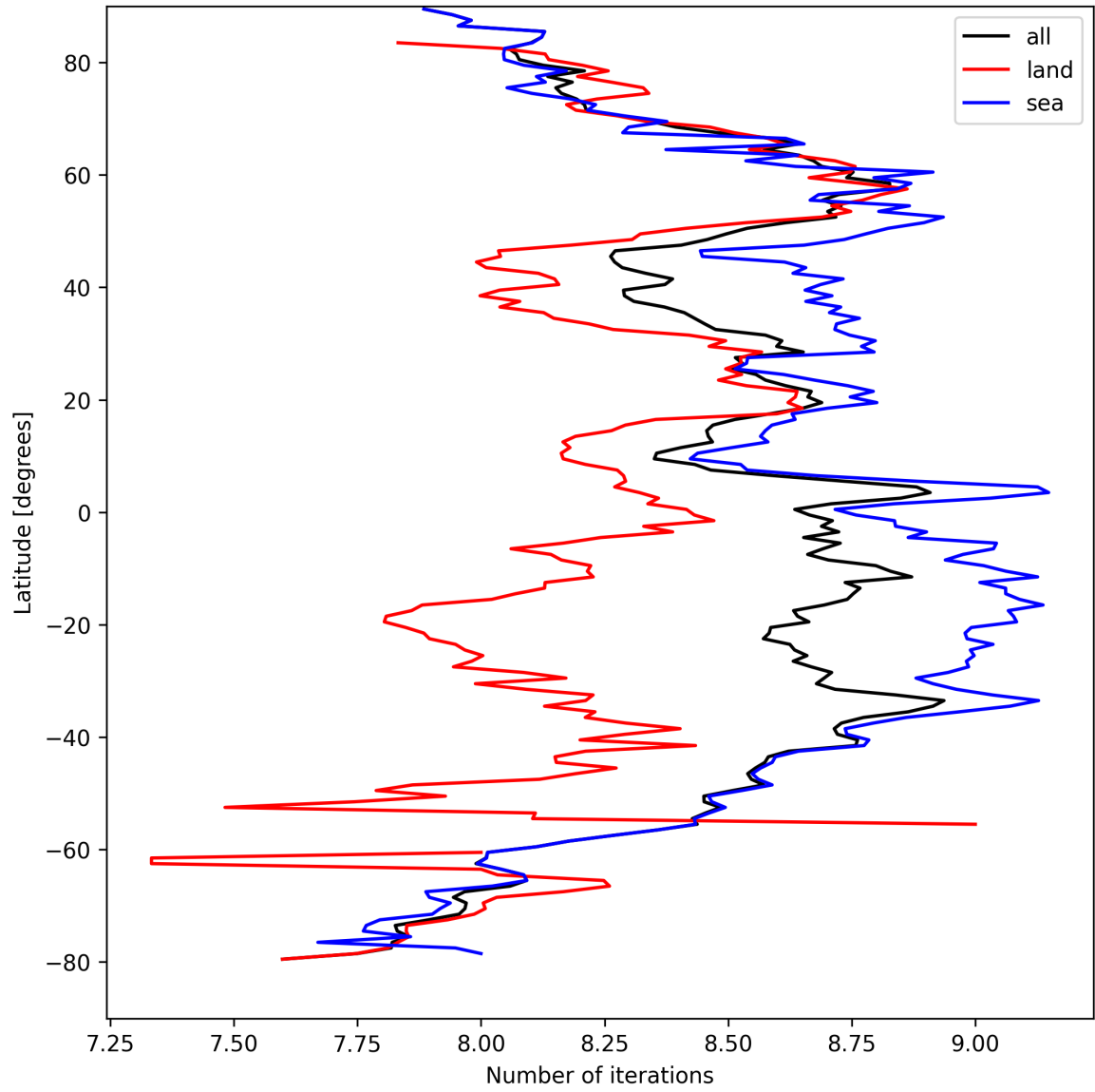
Figure 12: Zonal average of “Number of iterations” for 2025-09-08 to 2025-09-08.
