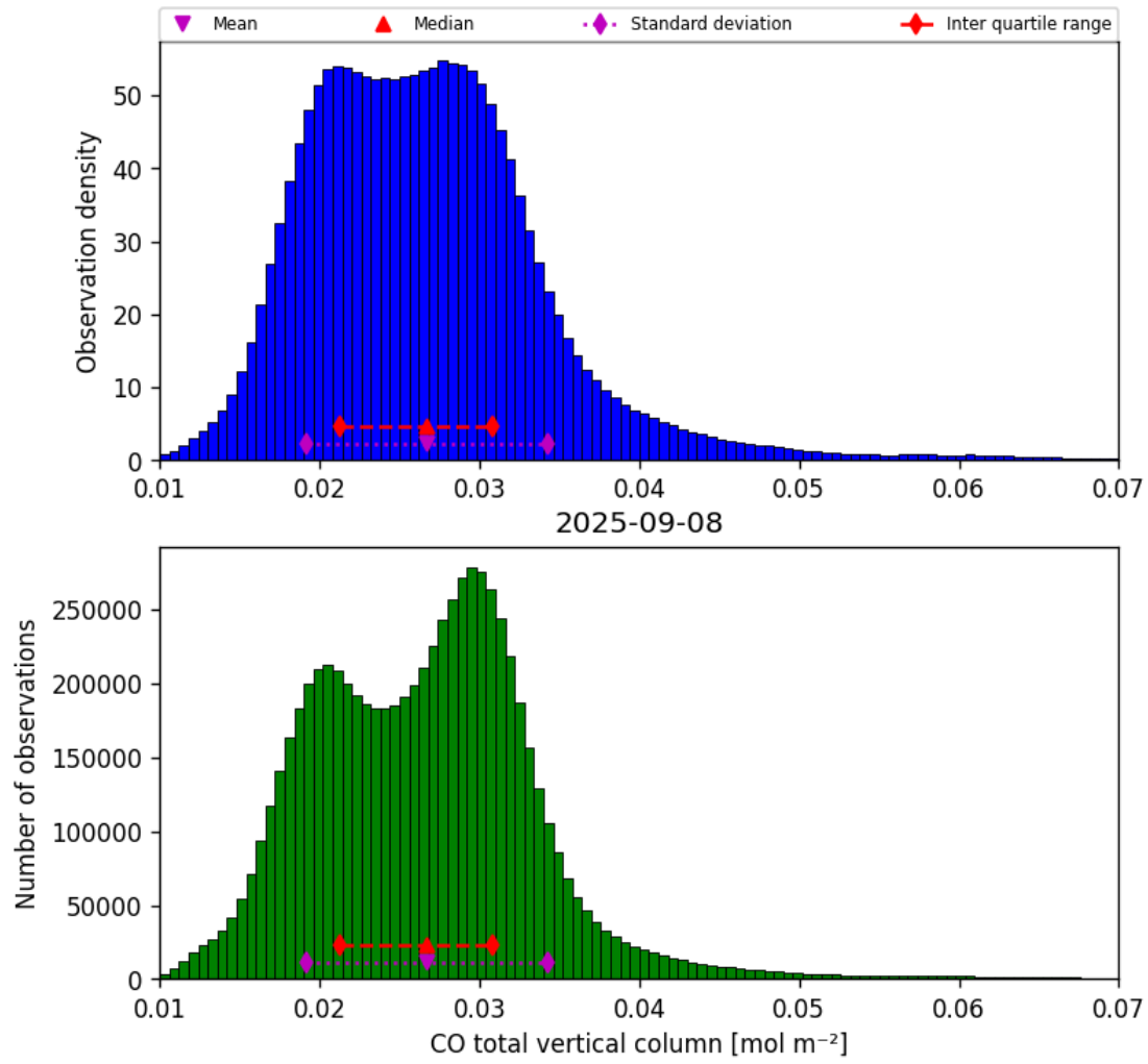
Figure 14: Histogram of “CO total vertical column” for 2025-09-08 to 2025-09-08
