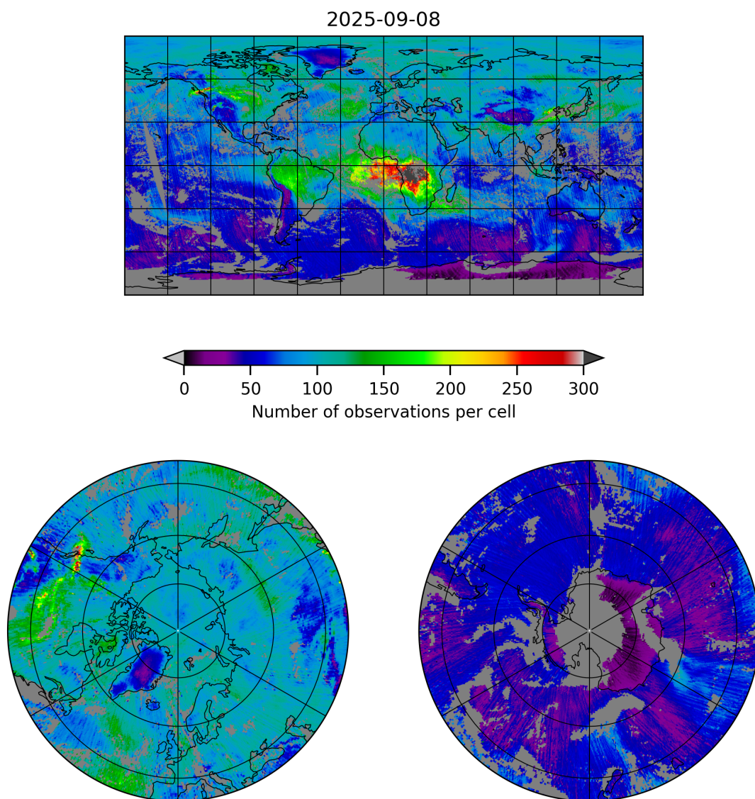
Figure 5: Map of the number of observations for 2025-09-08 to 2025-09-08
