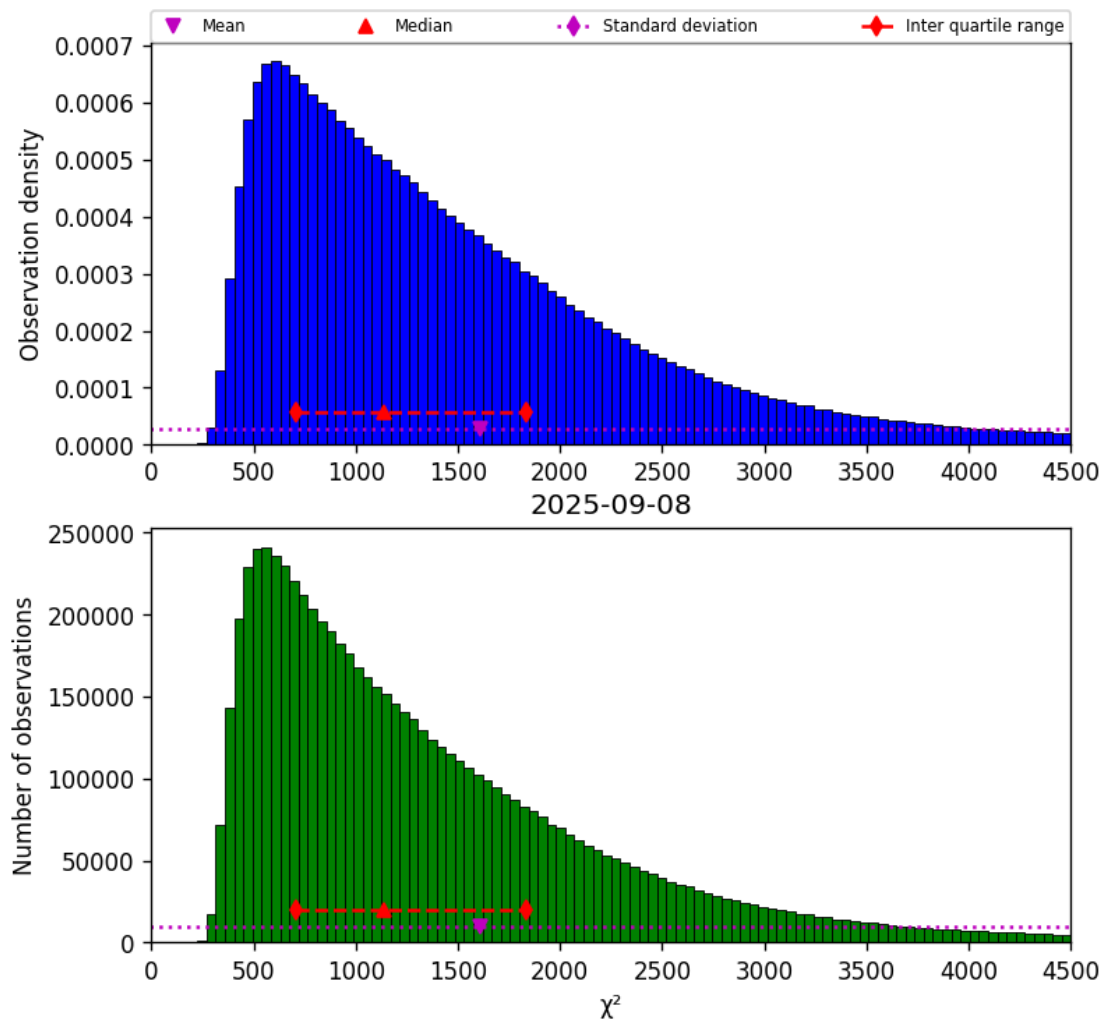
Figure 17: Histogram of " \chi^2 " for 2025-09-08 to 2025-09-08
