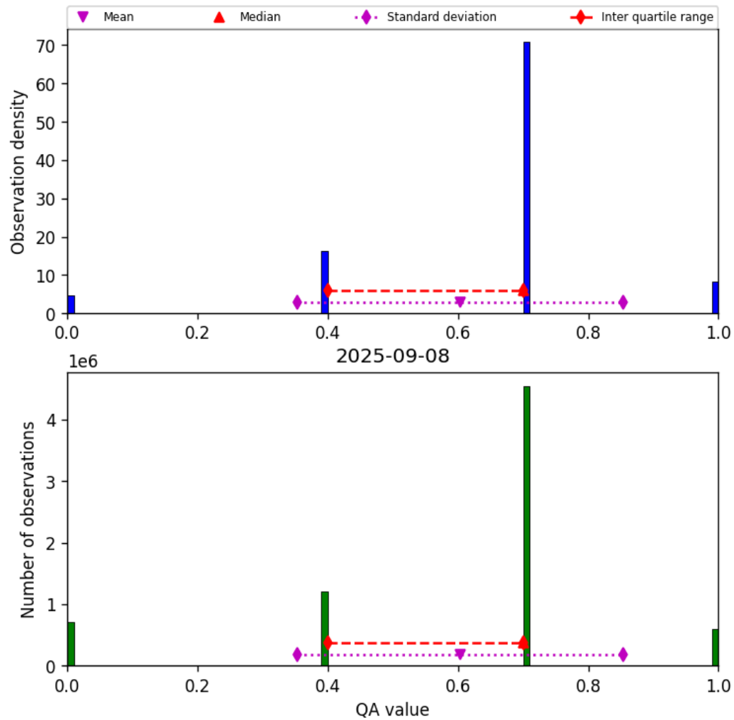
Figure 13: Histogram of “QA value” for 2025-09-08 to 2025-09-08
