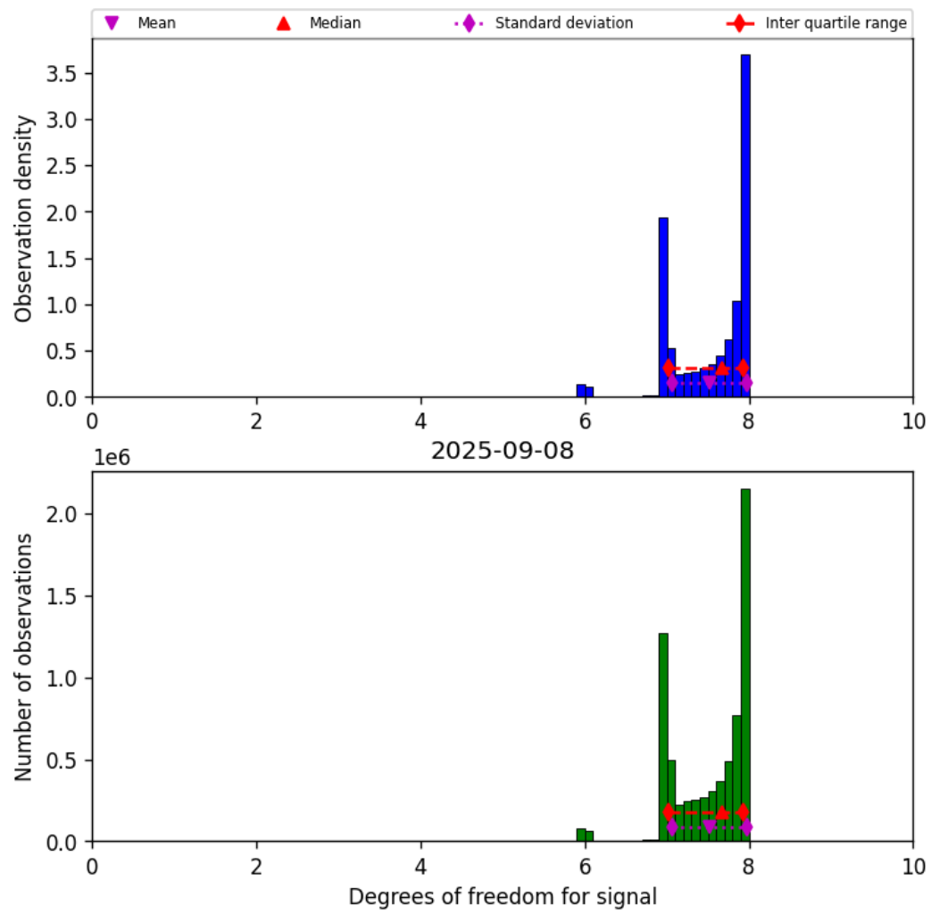
Figure 18: Histogram of “Degrees of freedom for signal” for 2025-09-08 to 2025-09-08
