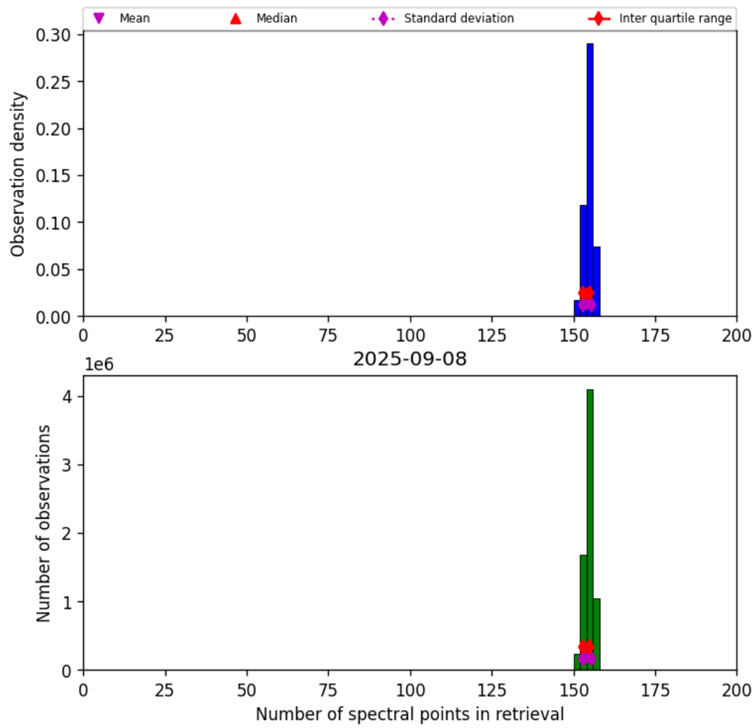
Figure 16: Histogram of “Number of spectral points in retrieval” for 2025-09-08 to 2025-09-08
