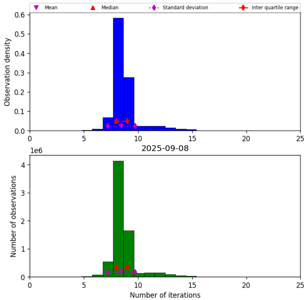
Figure 19: Histogram of “Number of iterations” for 2025-09-08 to 2025-09-08
