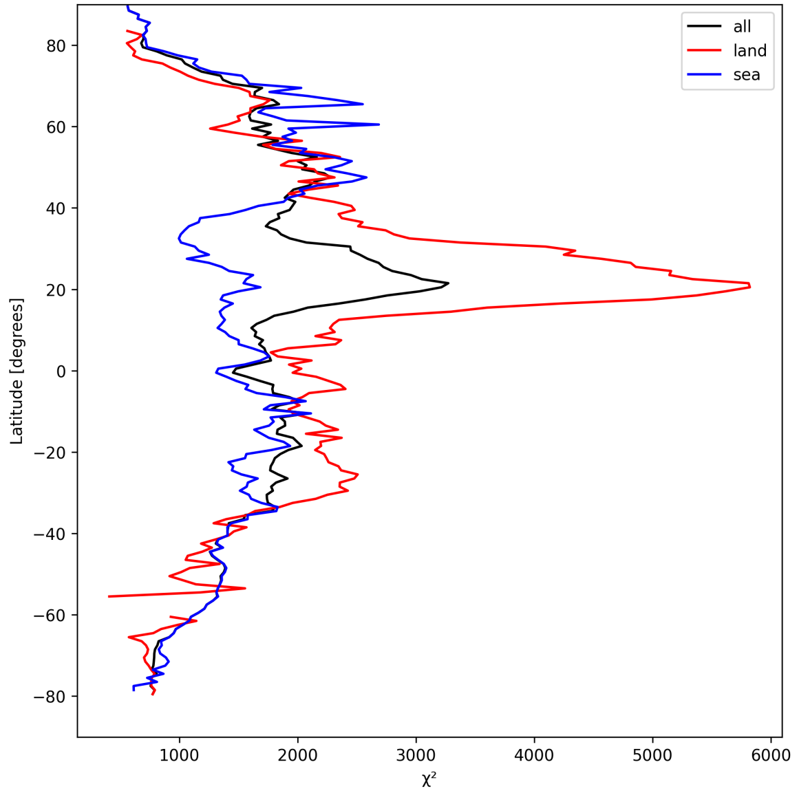
Figure 10: Zonal average of “ \chi^2 ” for 2025-09-08 to 2025-09-08.
