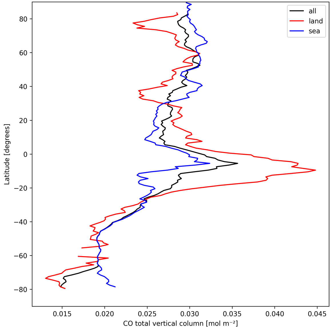
Figure 7: Zonal average of “CO total vertical column” for 2025-09-08 to 2025-09-08.
