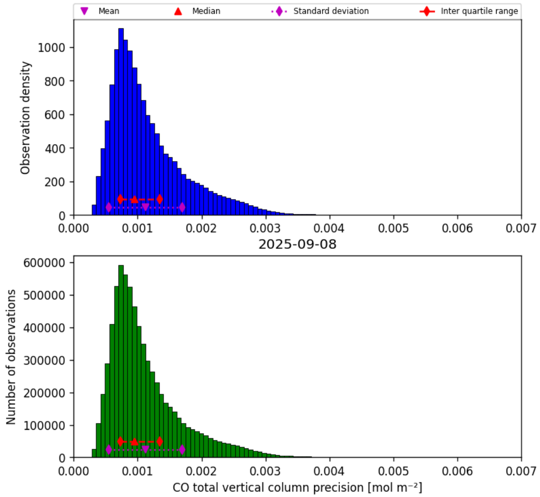
Figure 15: Histogram of “CO total vertical column precision” for 2025-09-08 to 2025-09-08
