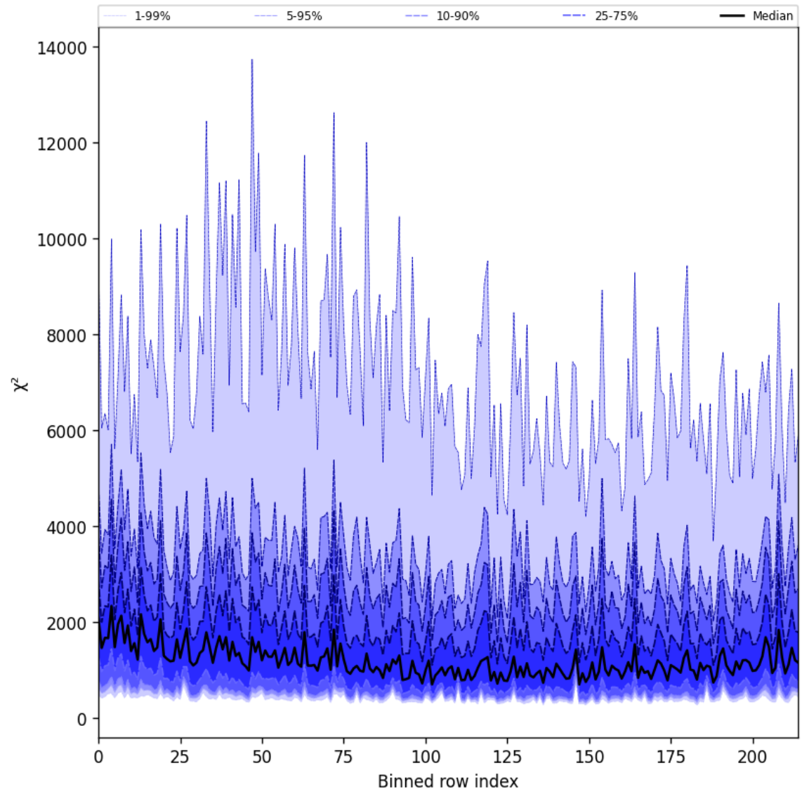
Figure 24: Along track statistics of “ \chi^2 ” for 2025-09-08 to 2025-09-08
