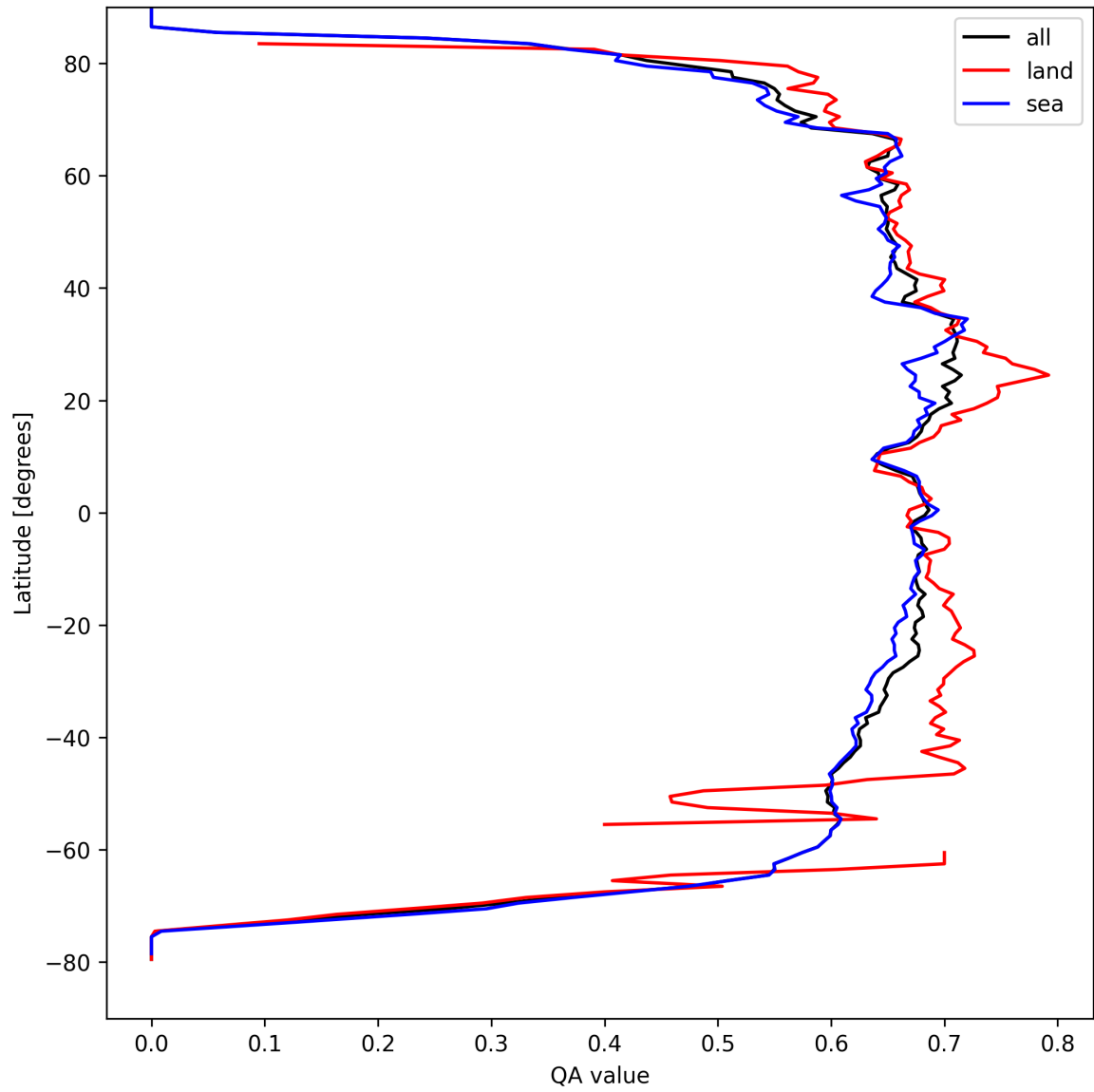
Figure 6: Zonal average of “QA value” for 2025-09-08 to 2025-09-08.
