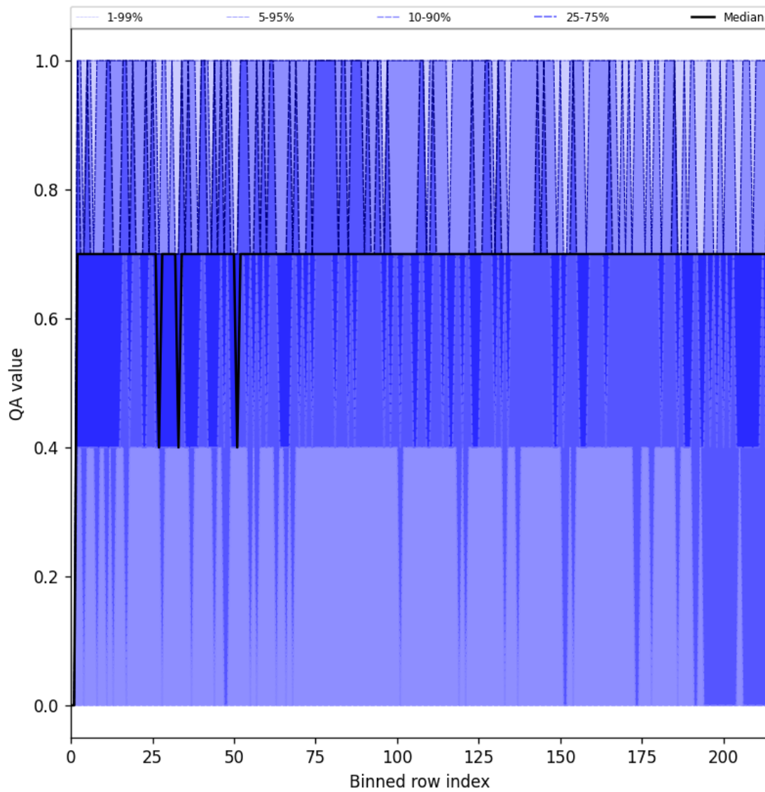
Figure 20: Along track statistics of “QA value” for 2025-09-08 to 2025-09-08
