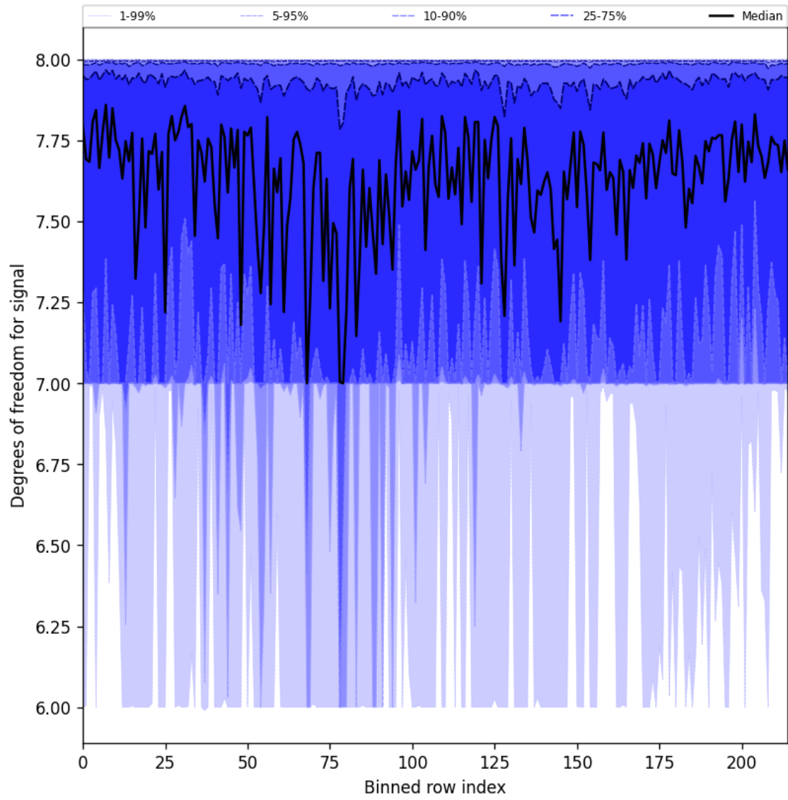
Figure 25: Along track statistics of “Degrees of freedom for signal” for 2025-09-08 to 2025-09-08
