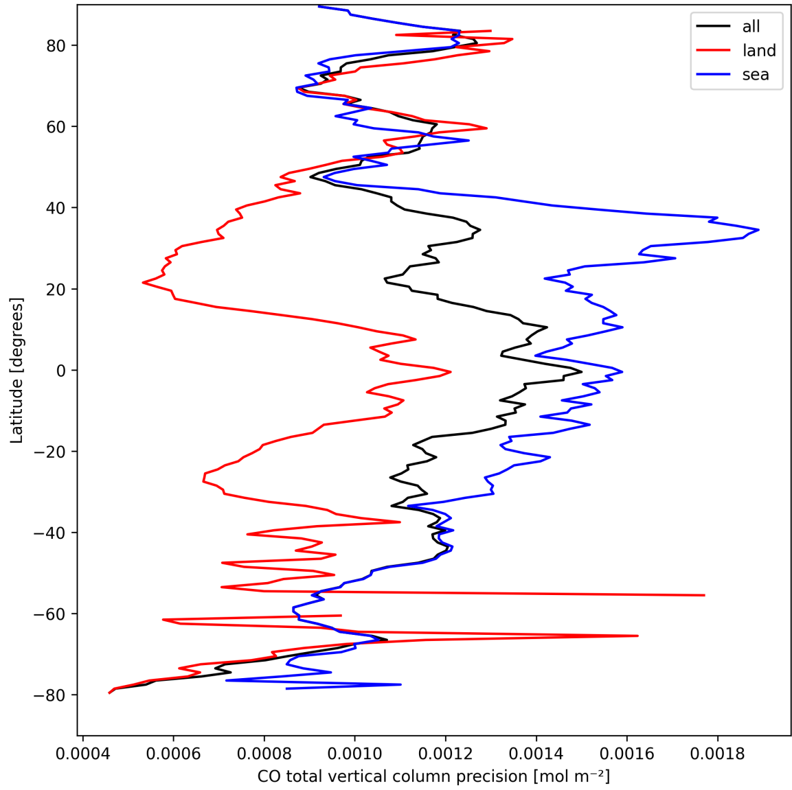
Figure 8: Zonal average of “CO total vertical column precision” for 2025-09-08 to 2025-09-08.
