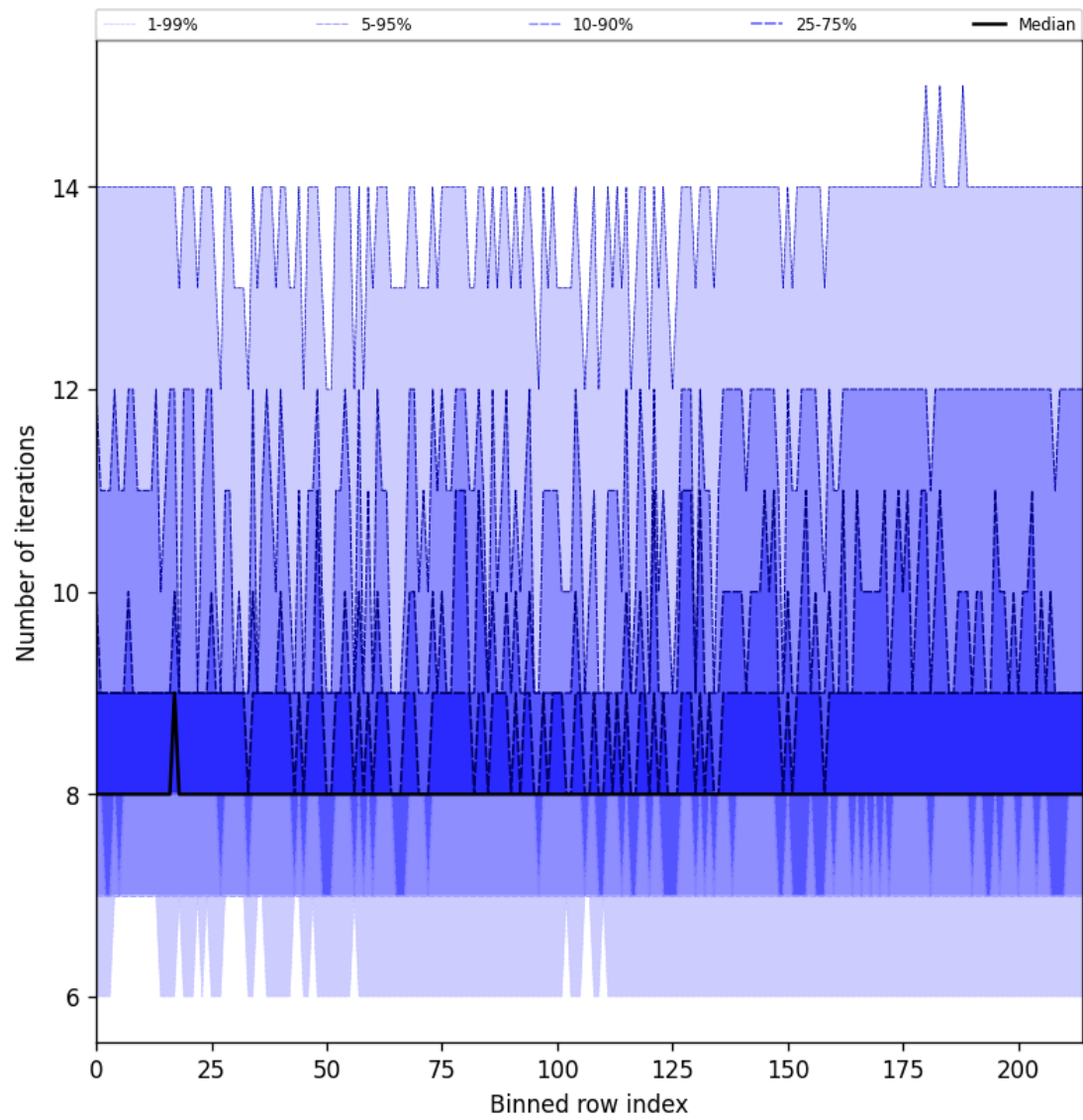
Figure 26: Along track statistics of “Number of iterations” for 2025-09-08 to 2025-09-08
