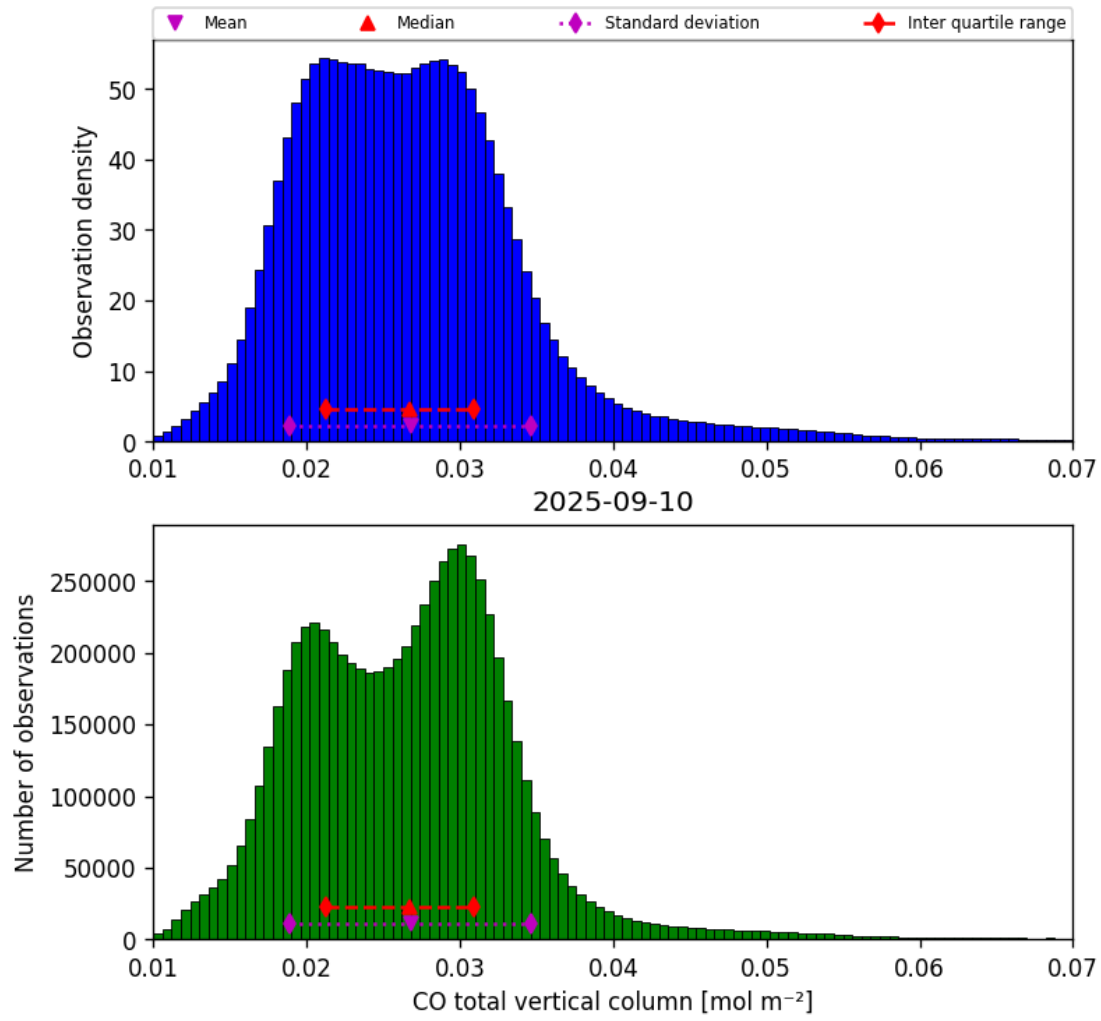
Figure 14: Histogram of “CO total vertical column” for 2025-09-10 to 2025-09-11
