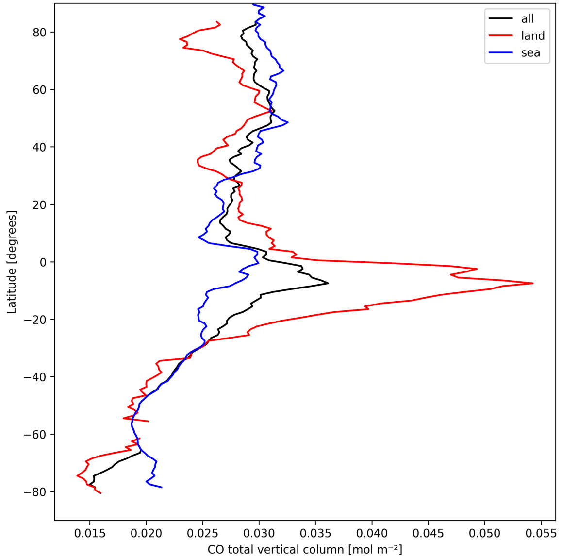
Figure 7: Zonal average of “CO total vertical column” for 2025-09-10 to 2025-09-11.
