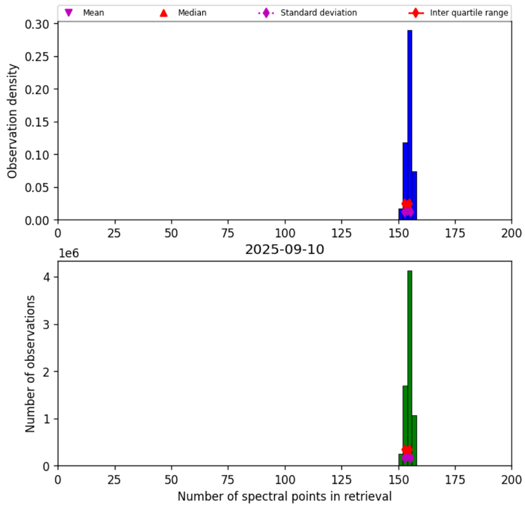
Figure 16: Histogram of “Number of spectral points in retrieval” for 2025-09-10 to 2025-09-11
