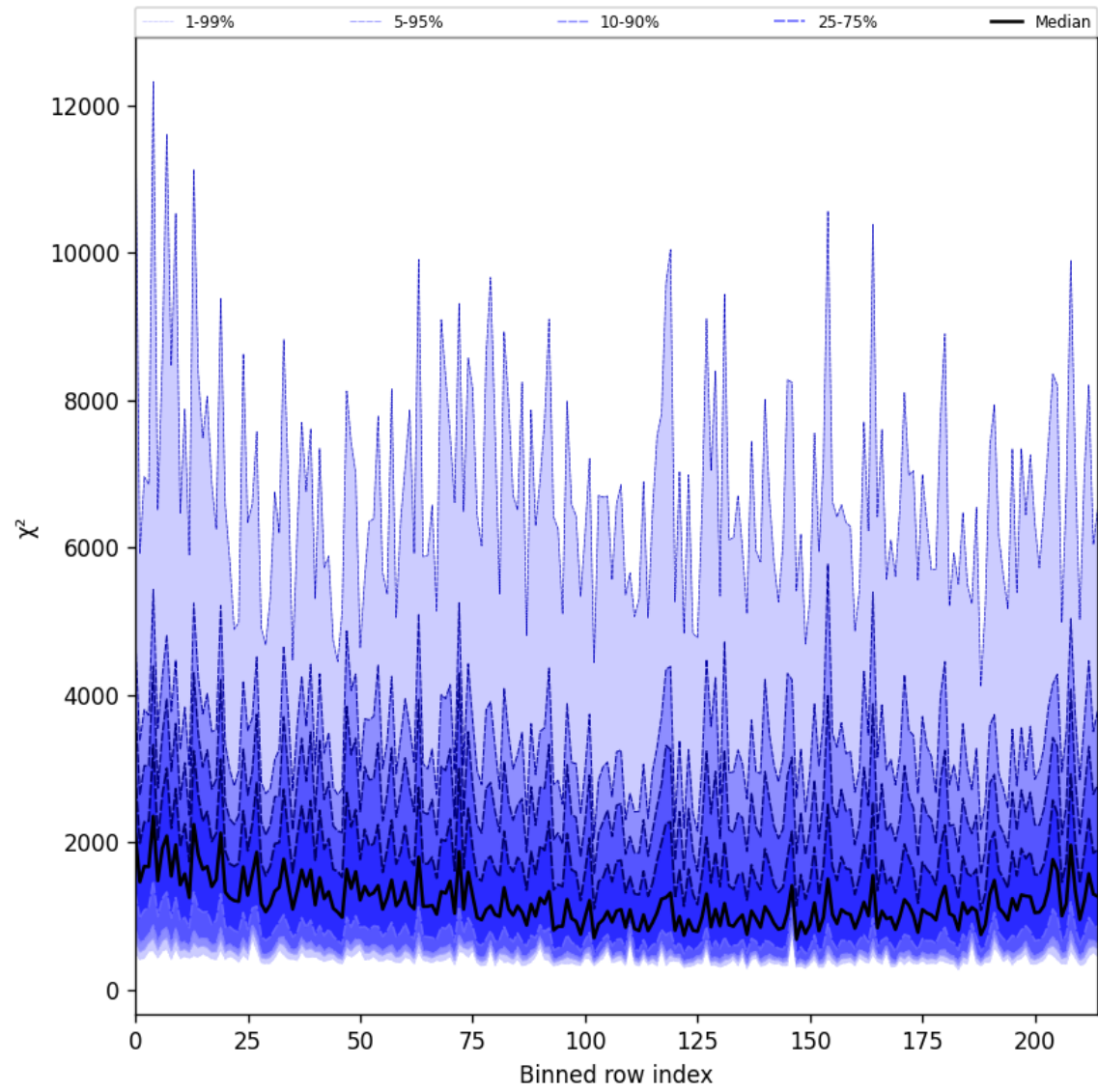
Figure 24: Along track statistics of “ \chi^2 ” for 2025-09-10 to 2025-09-11
