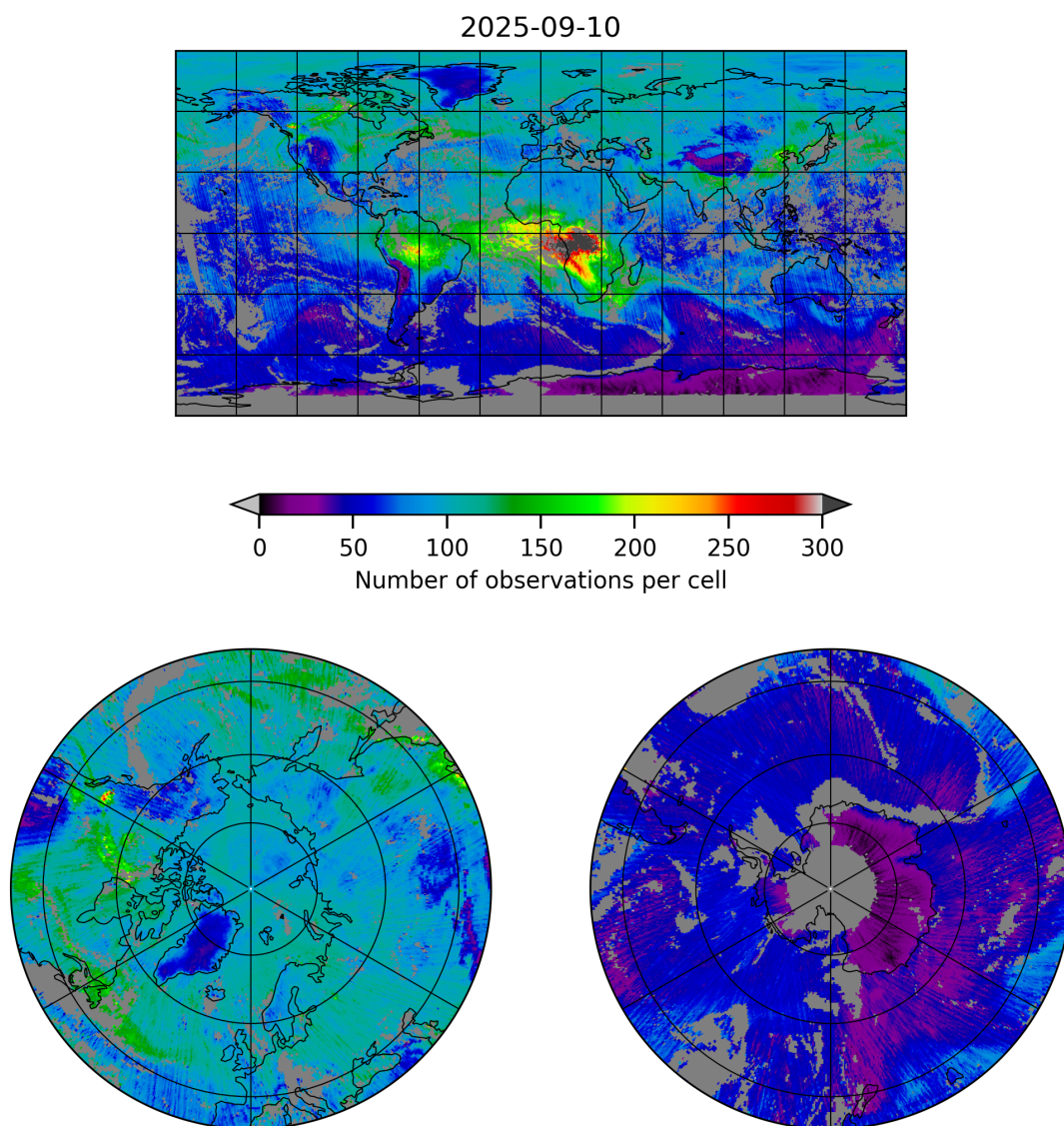
Figure 5: Map of the number of observations for 2025-09-10 to 2025-09-11
