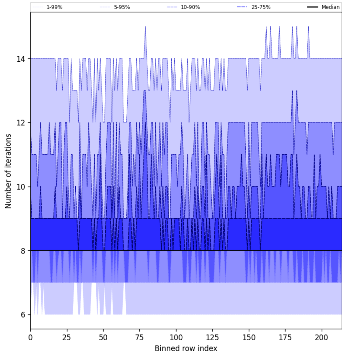
Figure 26: Along track statistics of “Number of iterations” for 2025-09-10 to 2025-09-11
