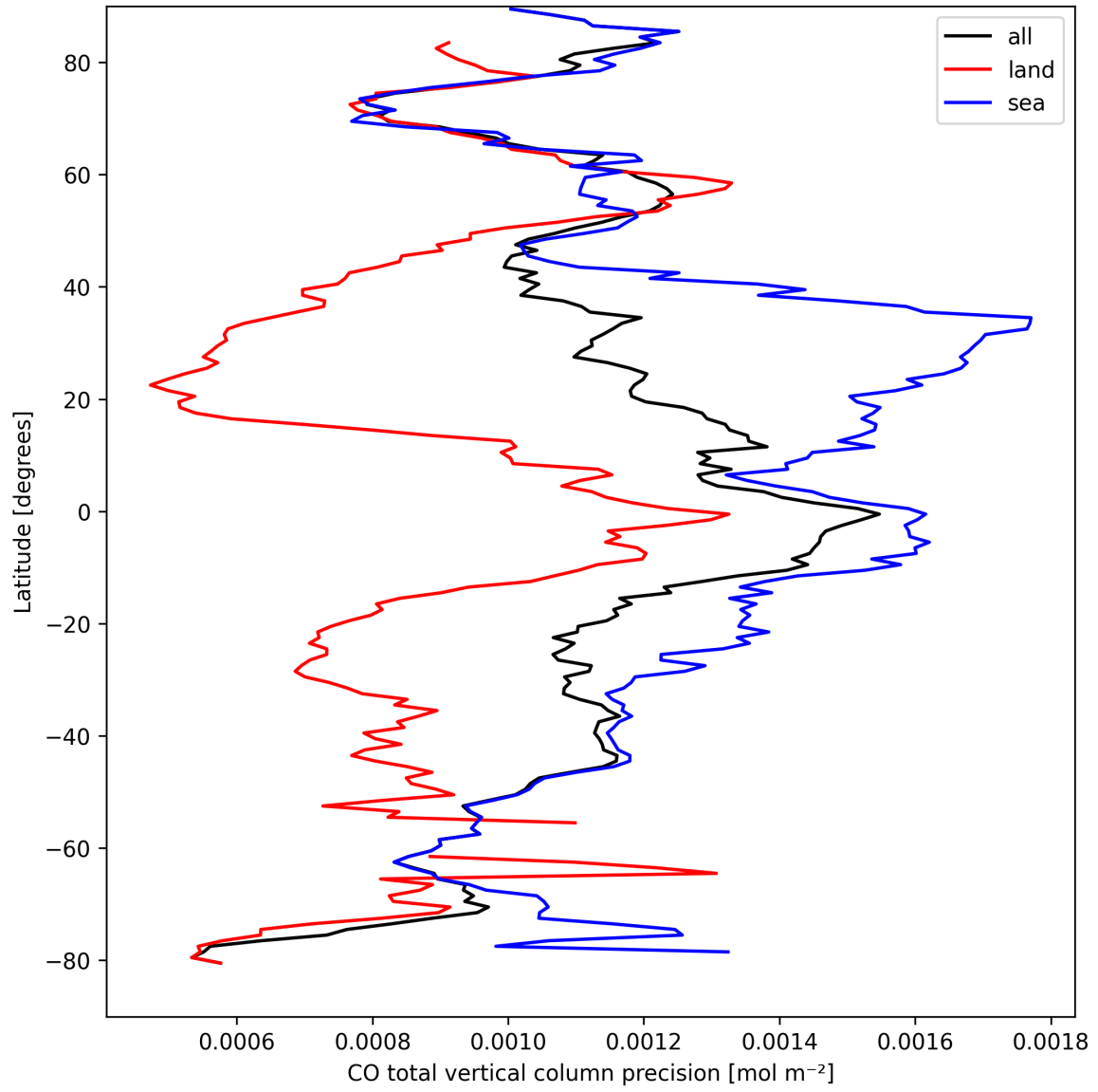
Figure 8: Zonal average of “CO total vertical column precision” for 2025-09-10 to 2025-09-11.
