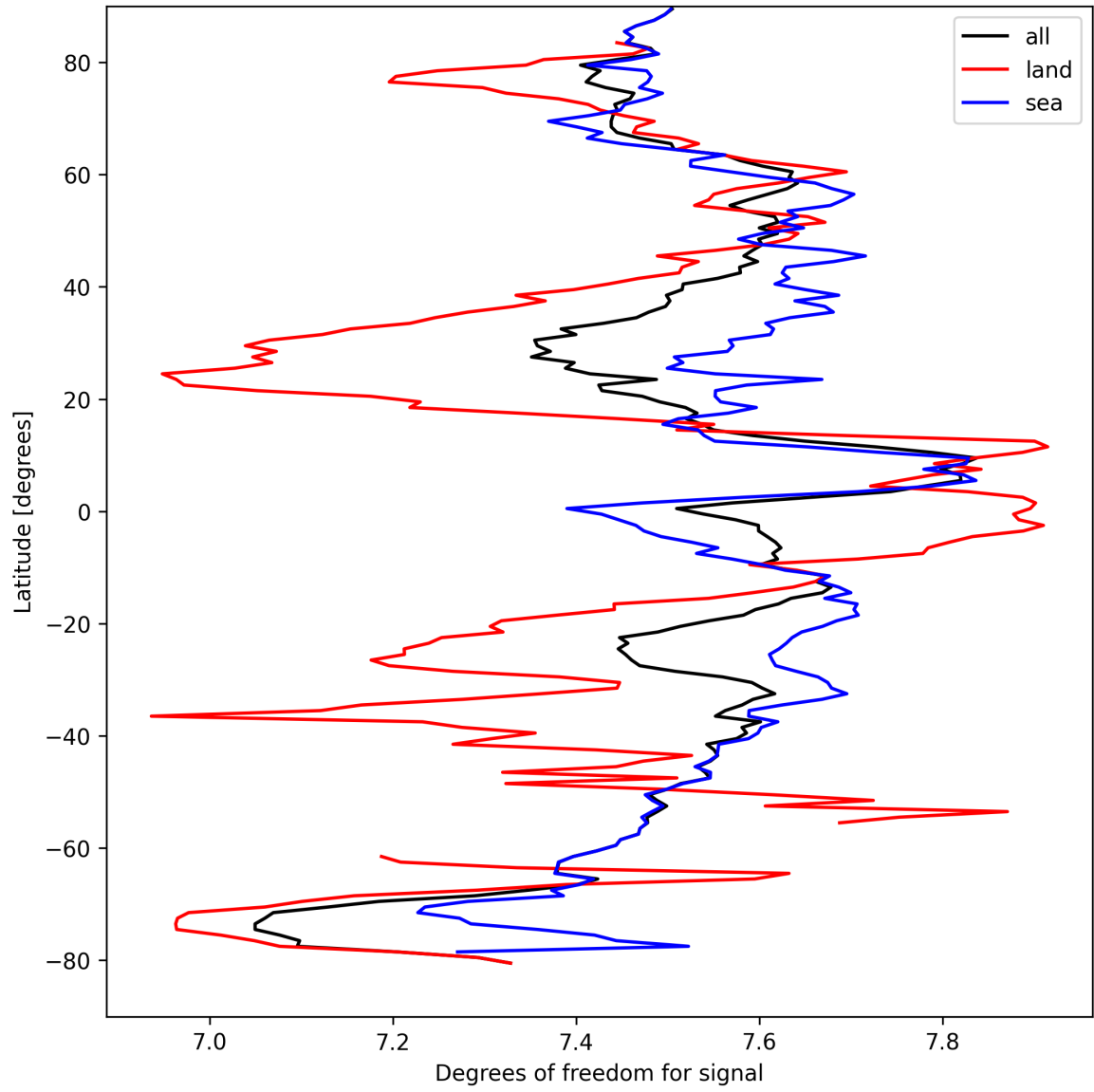
Figure 11: Zonal average of “Degrees of freedom for signal” for 2025-09-10 to 2025-09-11.
