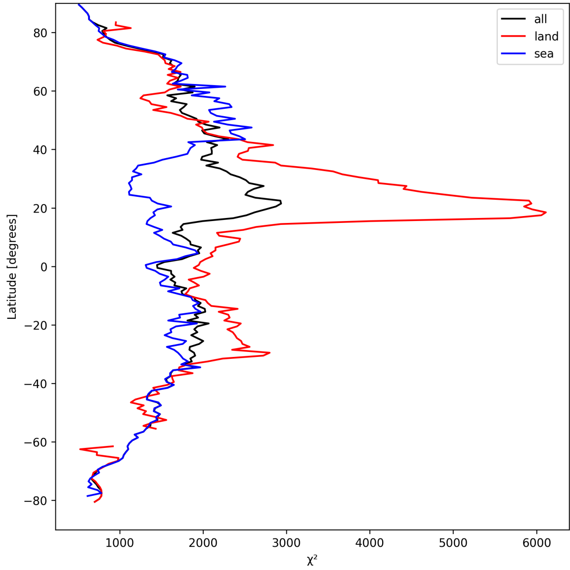
Figure 10: Zonal average of “ \chi^2 ” for 2025-09-10 to 2025-09-11.
