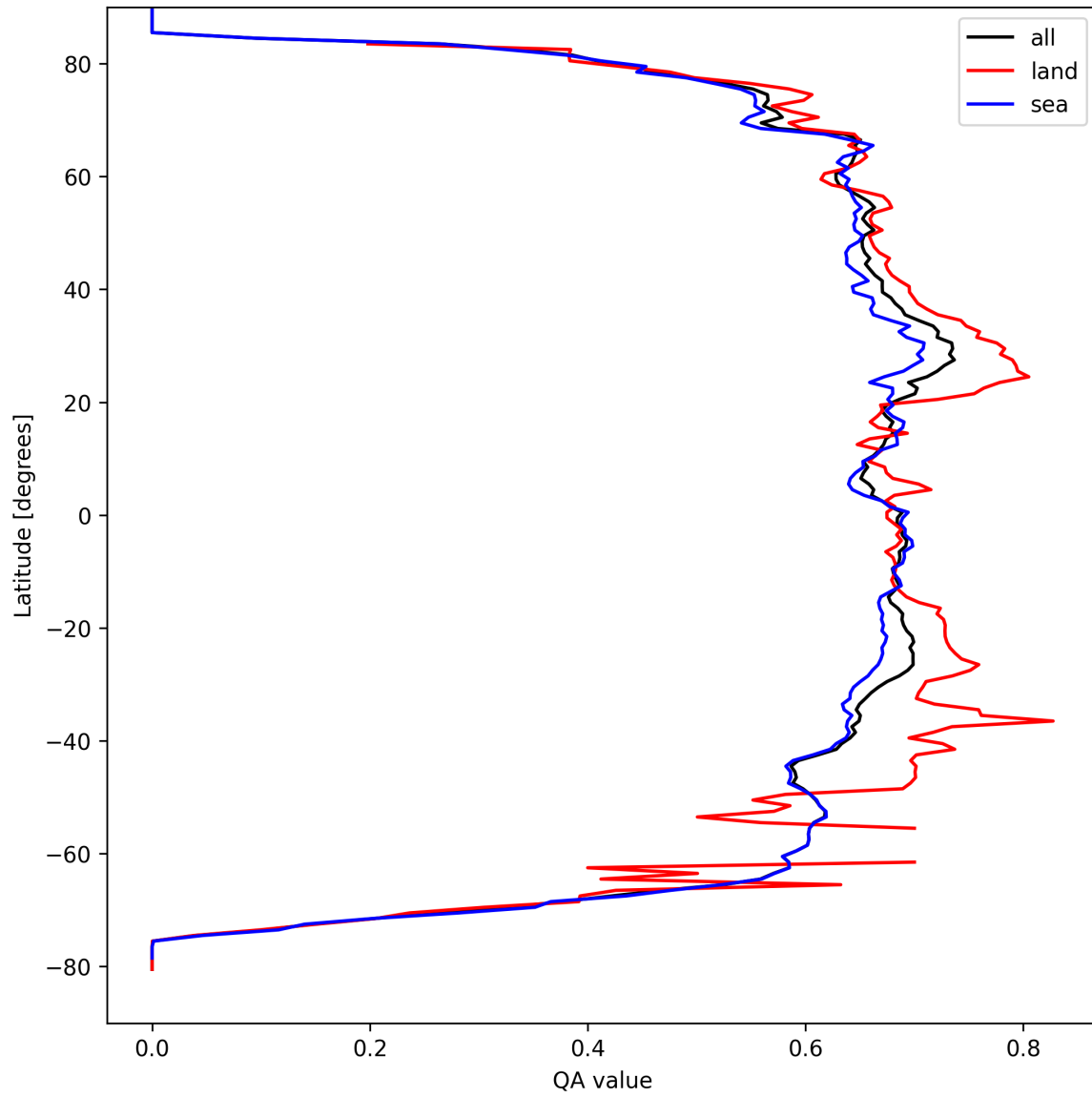
Figure 6: Zonal average of “QA value” for 2025-09-10 to 2025-09-11.
