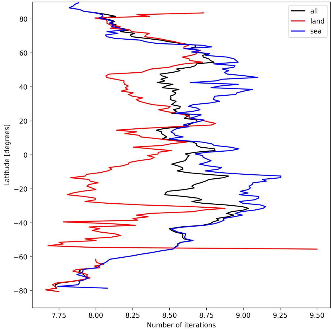
Figure 12: Zonal average of “Number of iterations” for 2025-09-10 to 2025-09-11.
