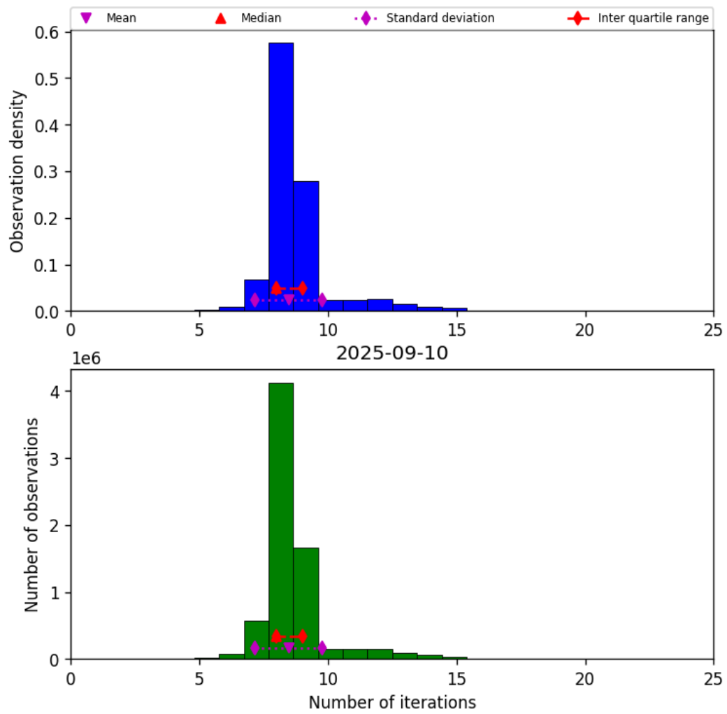
Figure 19: Histogram of “Number of iterations” for 2025-09-10 to 2025-09-11
