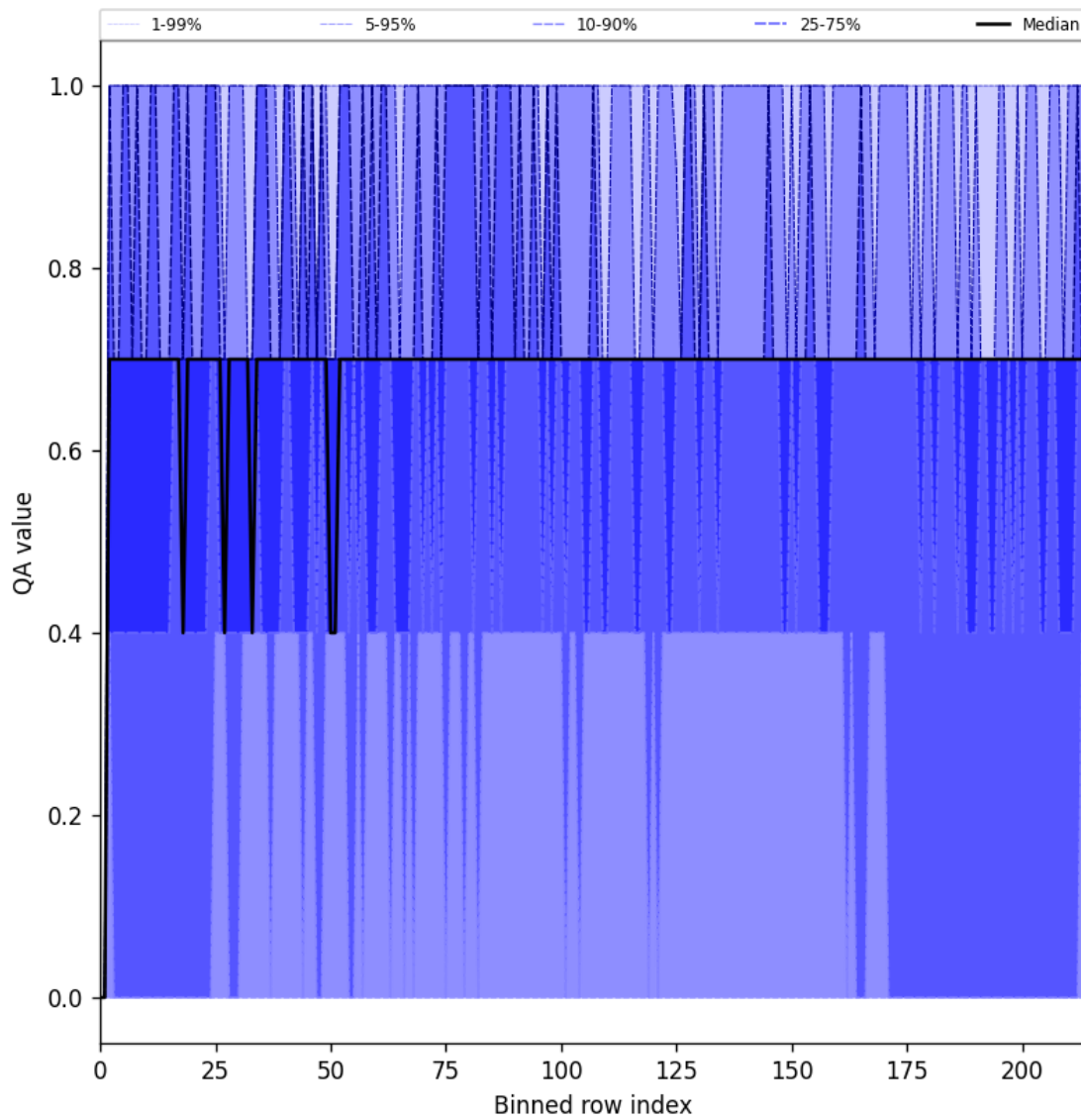
Figure 20: Along track statistics of “QA value” for 2025-09-10 to 2025-09-11
