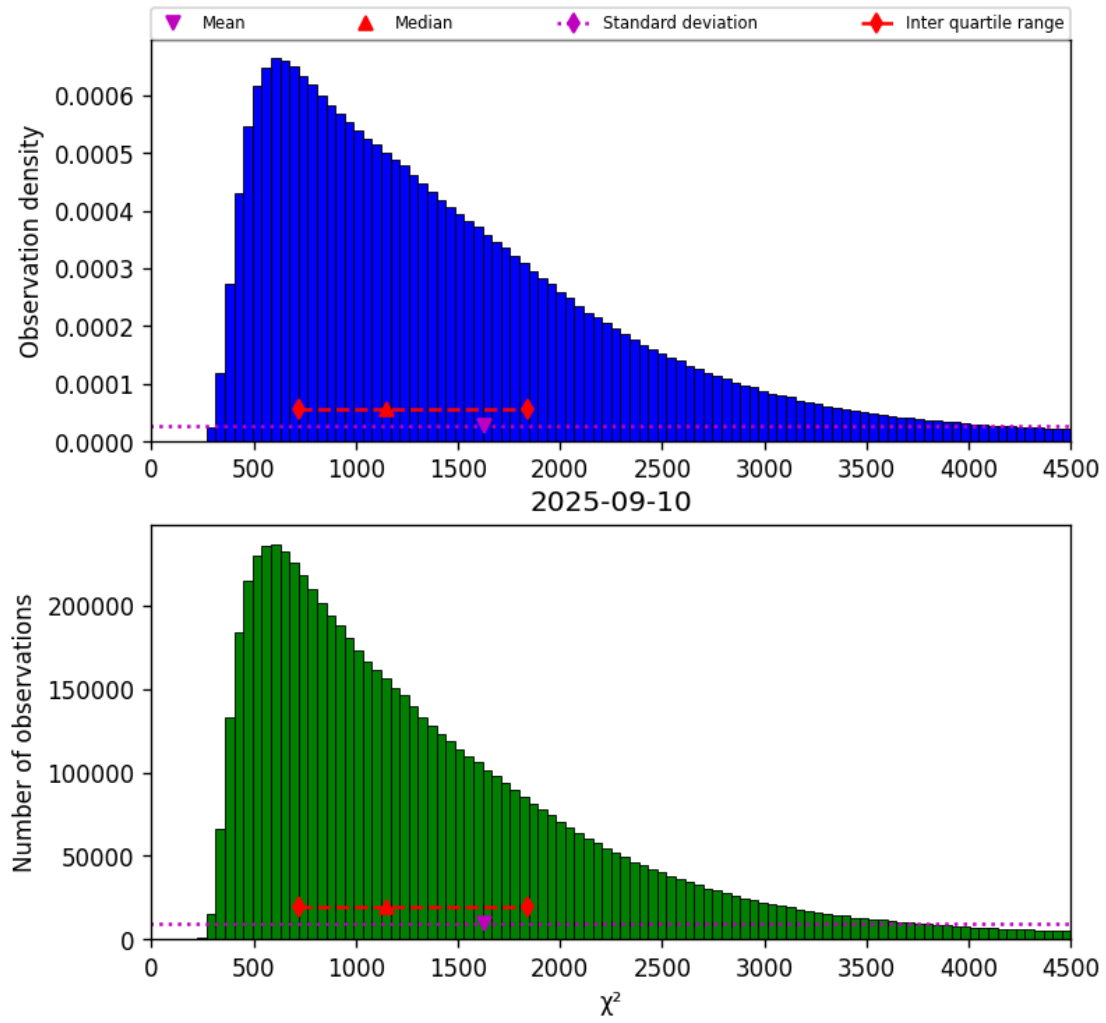
Figure 17: Histogram of “ \chi^2 ” for 2025-09-10 to 2025-09-11
