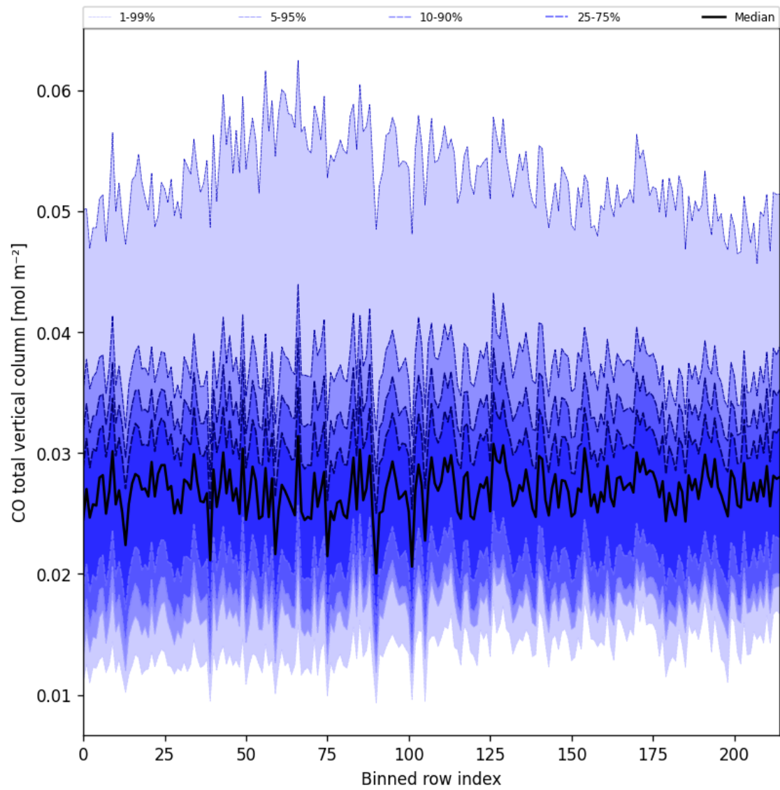
Figure 21: Along track statistics of “CO total vertical column” for 2025-09-10 to 2025-09-11
