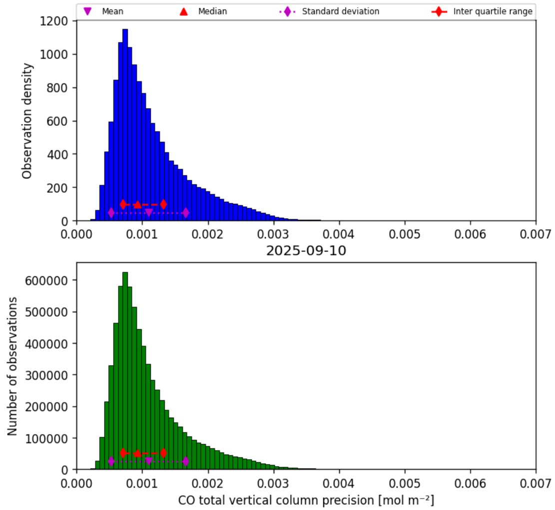
Figure 15: Histogram of “CO total vertical column precision” for 2025-09-10 to 2025-09-11
