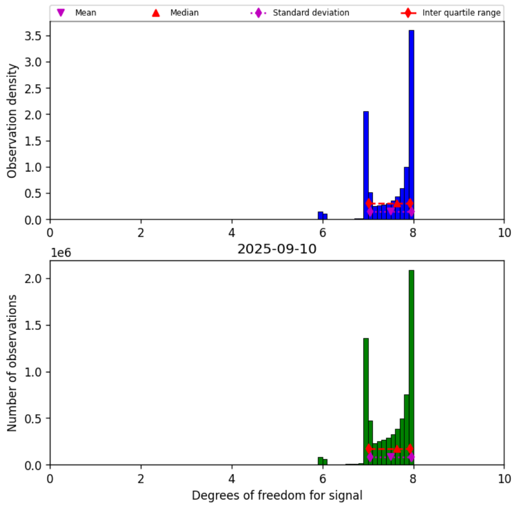
Figure 18: Histogram of “Degrees of freedom for signal” for 2025-09-10 to 2025-09-11
