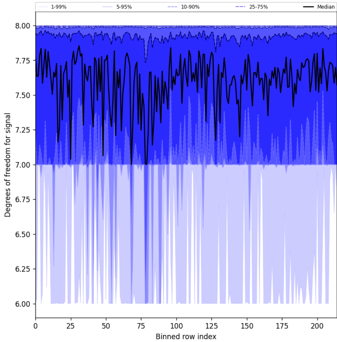
Figure 25: Along track statistics of “Degrees of freedom for signal” for 2025-09-10 to 2025-09-11
