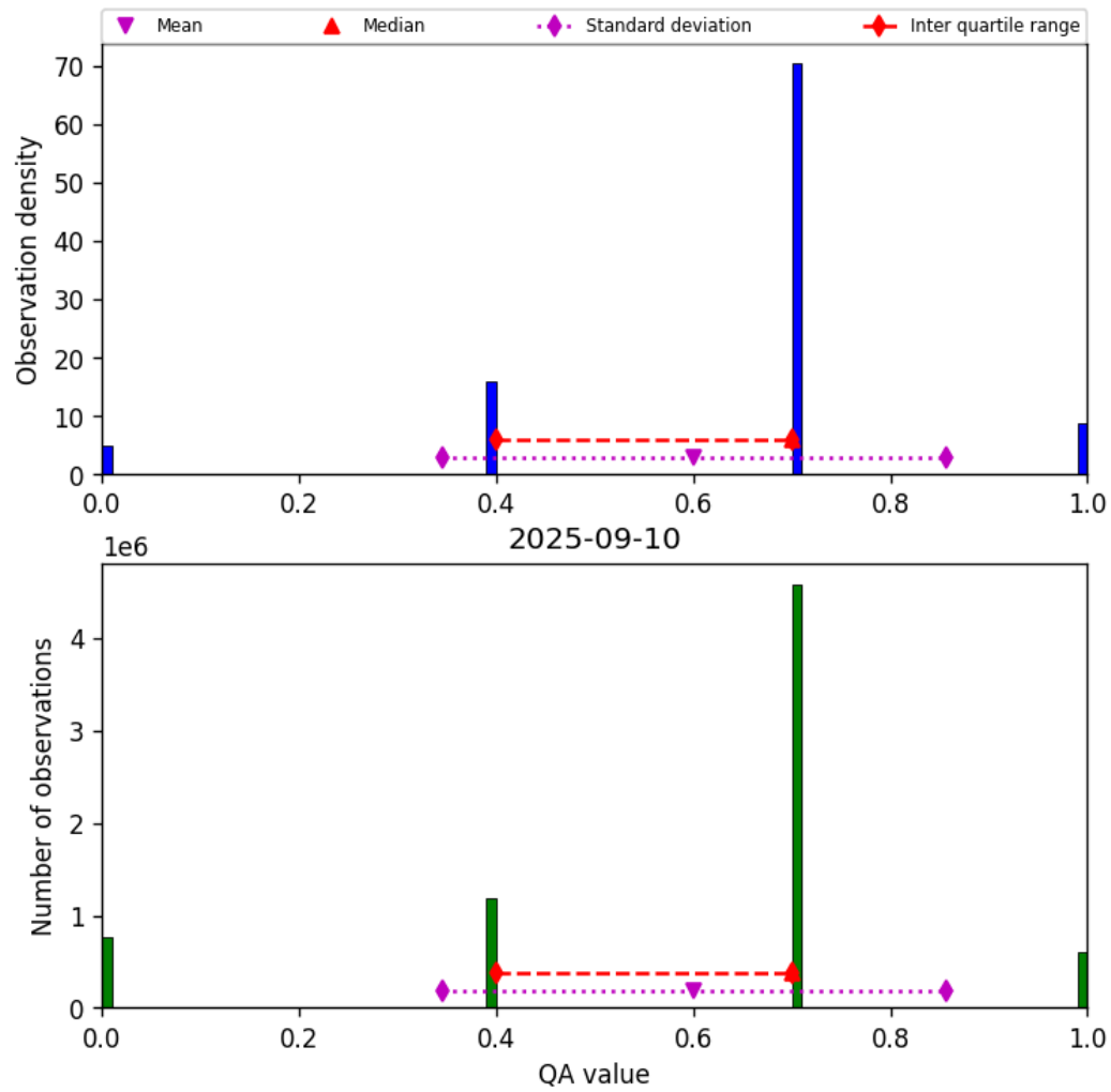
Figure 13: Histogram of “QA value” for 2025-09-10 to 2025-09-11
