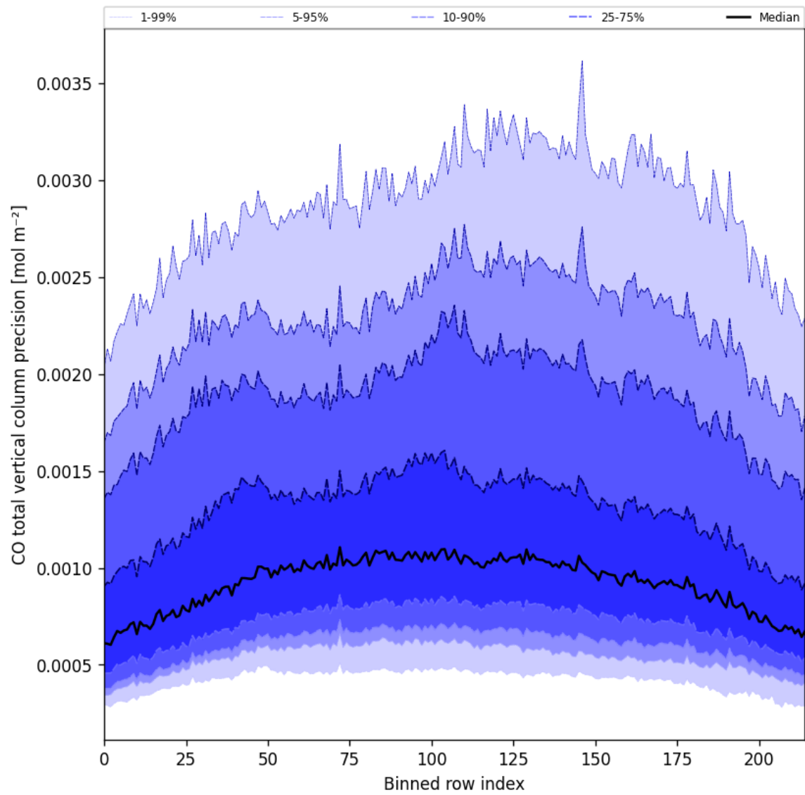
Figure 22: Along track statistics of “CO total vertical column precision” for 2025-09-10 to 2025-09-11
