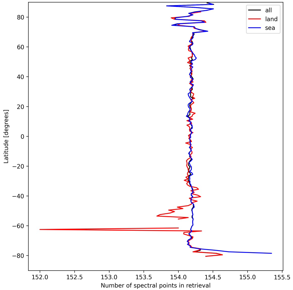
Figure 9: Zonal average of “Number of spectral points in retrieval” for 2025-09-10 to 2025-09-11.
