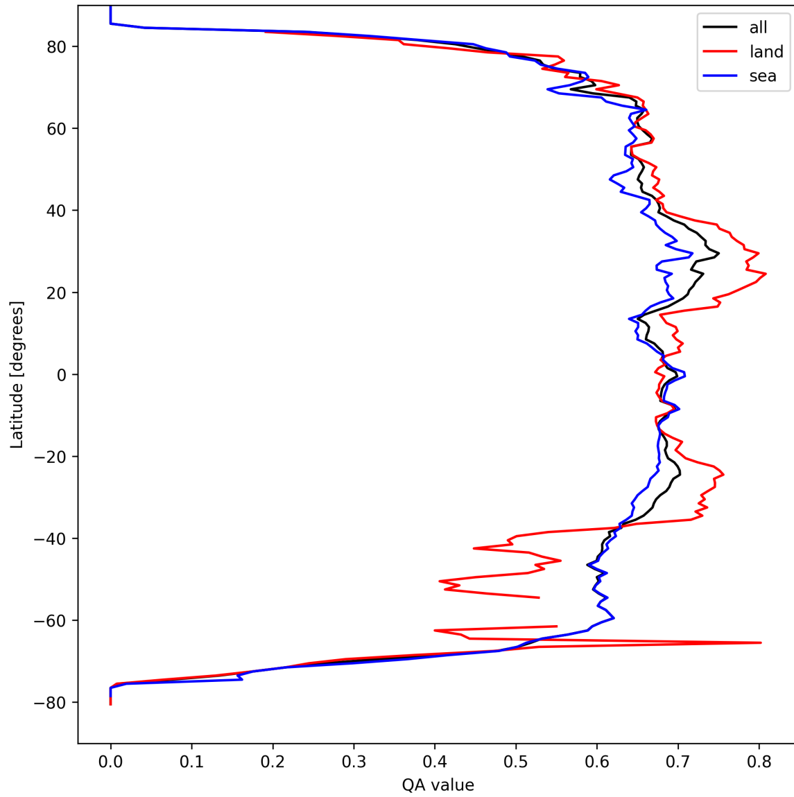
Figure 6: Zonal average of “QA value” for 2025-09-11 to 2025-09-12.
