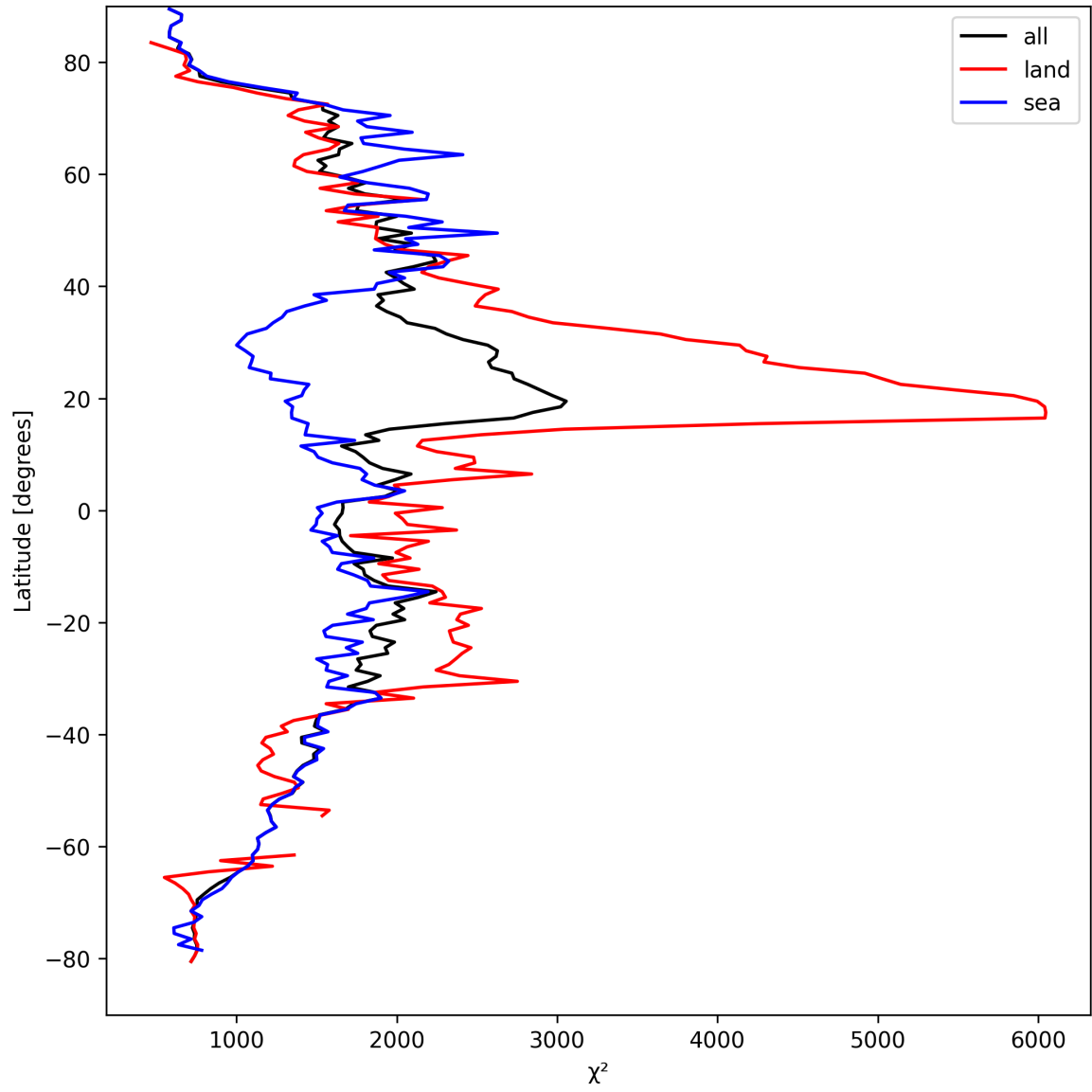
Figure 10: Zonal average of “ \chi^2 ” for 2025-09-11 to 2025-09-12.
