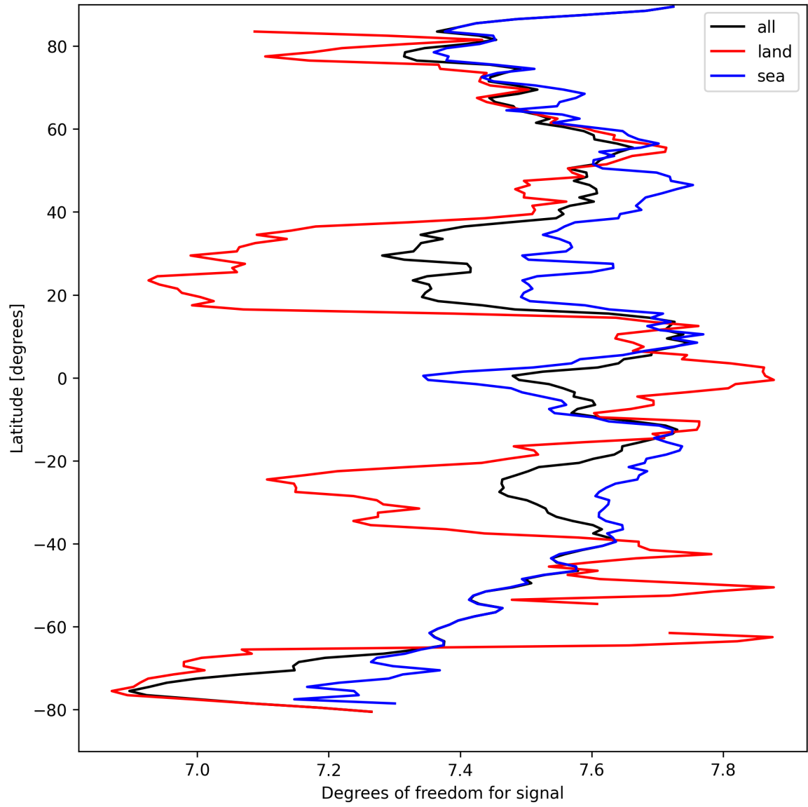
Figure 11: Zonal average of “Degrees of freedom for signal” for 2025-09-11 to 2025-09-12.
