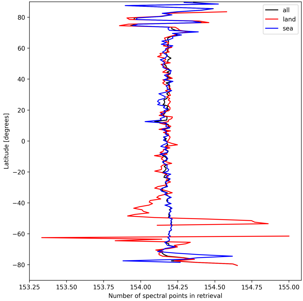
Figure 9: Zonal average of “Number of spectral points in retrieval” for 2025-09-11 to 2025-09-12.
