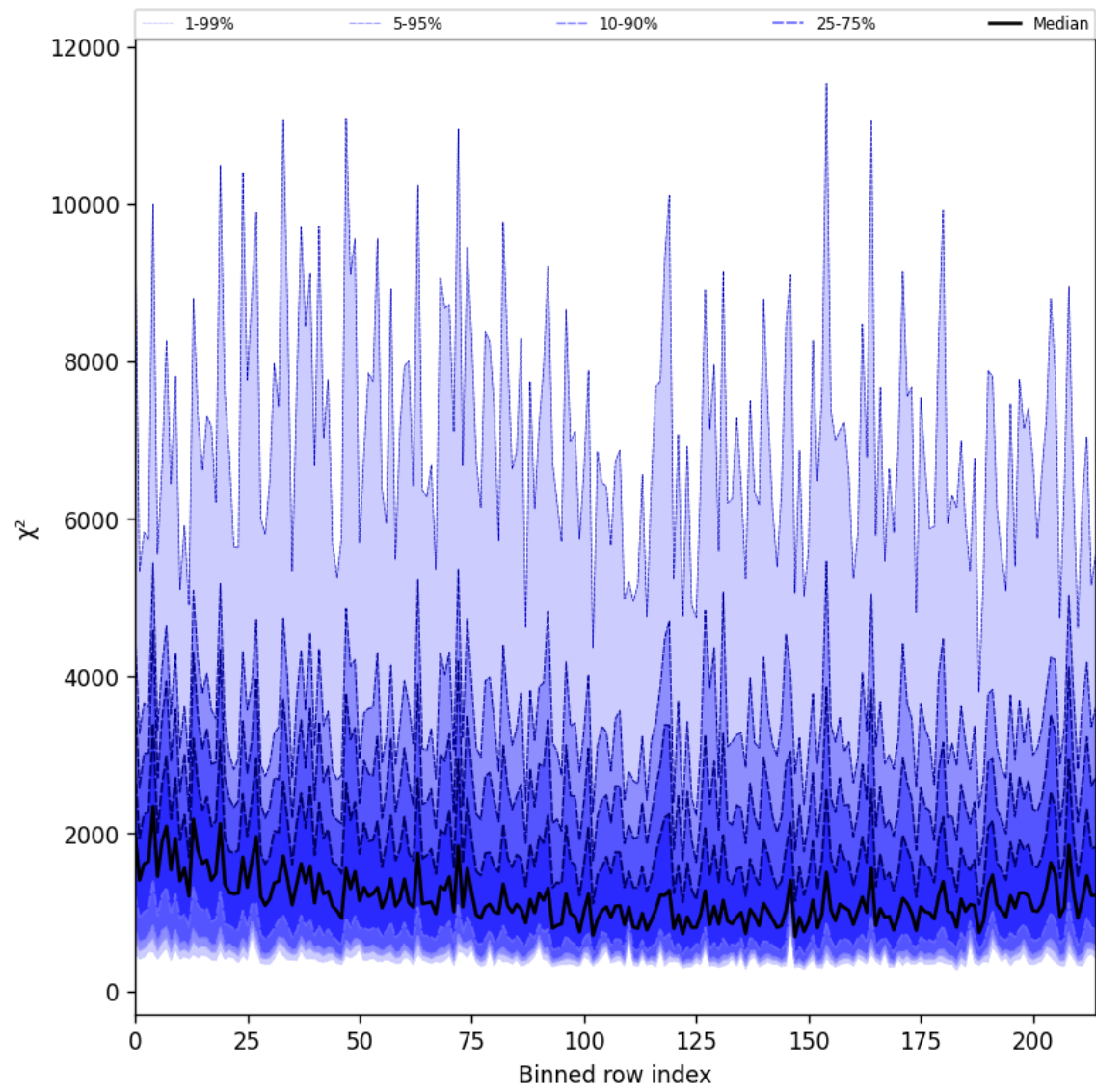
Figure 24: Along track statistics of “ \chi^2 ” for 2025-09-11 to 2025-09-12
