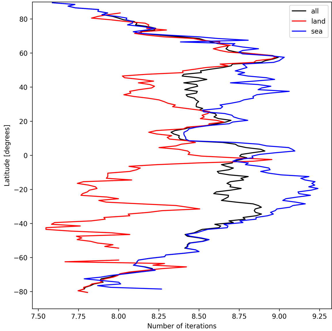
Figure 12: Zonal average of “Number of iterations” for 2025-09-11 to 2025-09-12.
