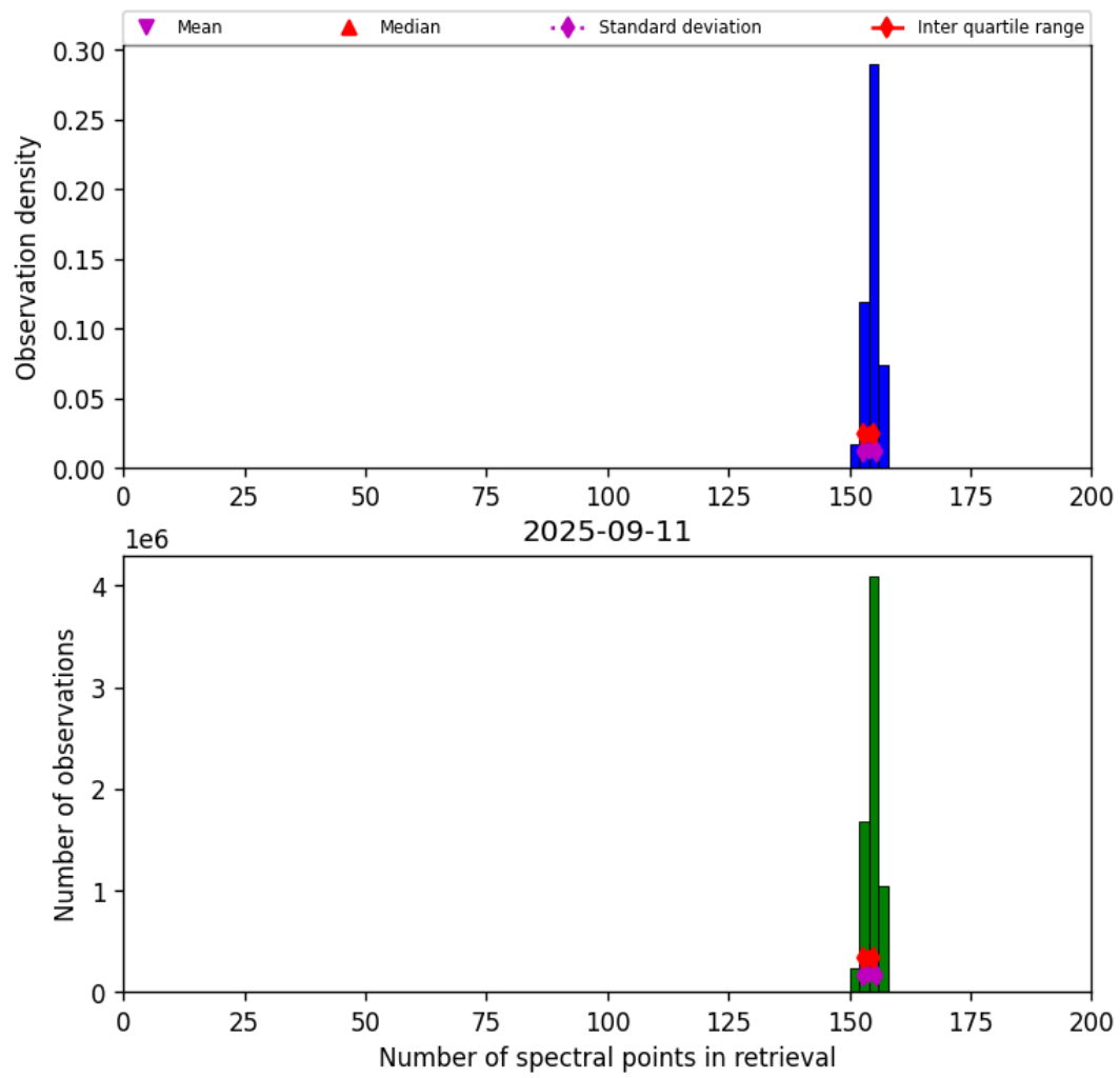
Figure 16: Histogram of “Number of spectral points in retrieval” for 2025-09-11 to 2025-09-12
