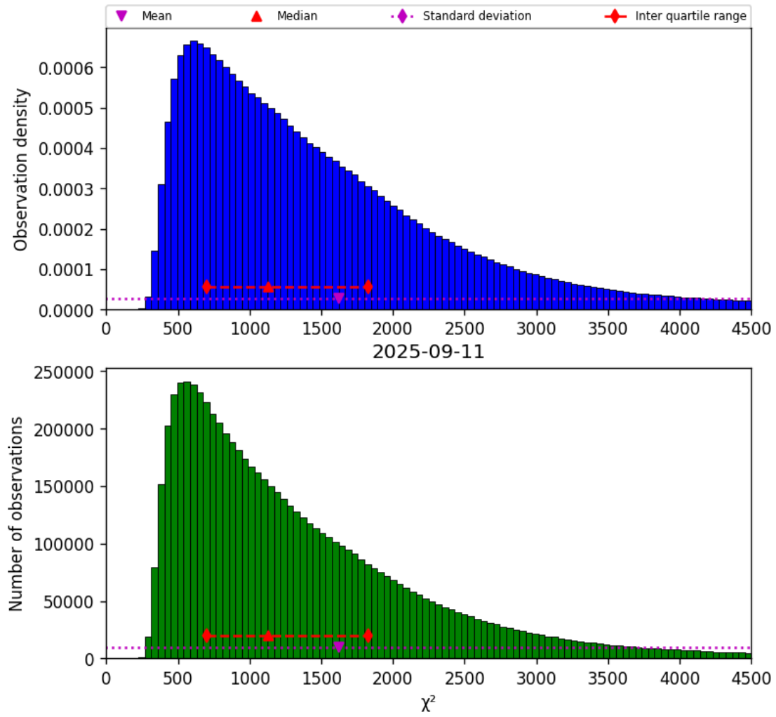
Figure 17: Histogram of “ \chi^2 ” for 2025-09-11 to 2025-09-12
