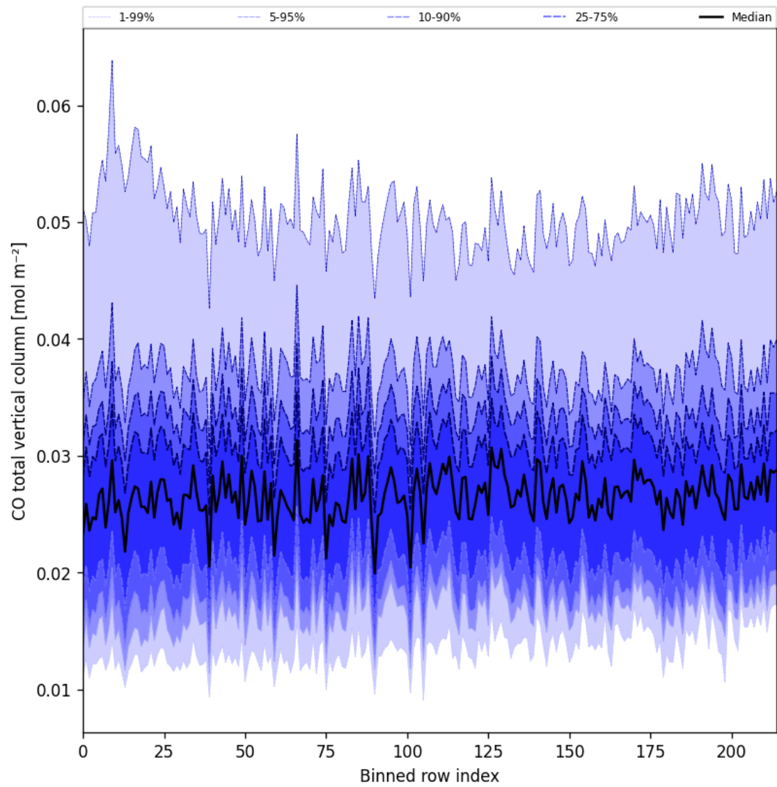
Figure 21: Along track statistics of “CO total vertical column” for 2025-09-11 to 2025-09-12
