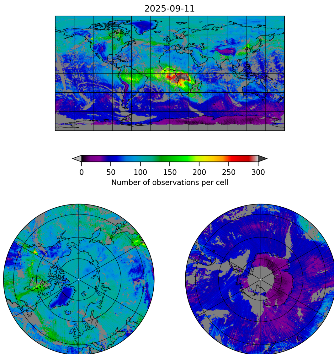
Figure 5: Map of the number of observations for 2025-09-11 to 2025-09-12
