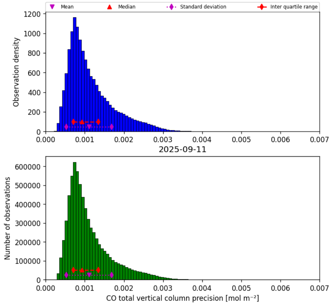
Figure 15: Histogram of “CO total vertical column precision” for 2025-09-11 to 2025-09-12
