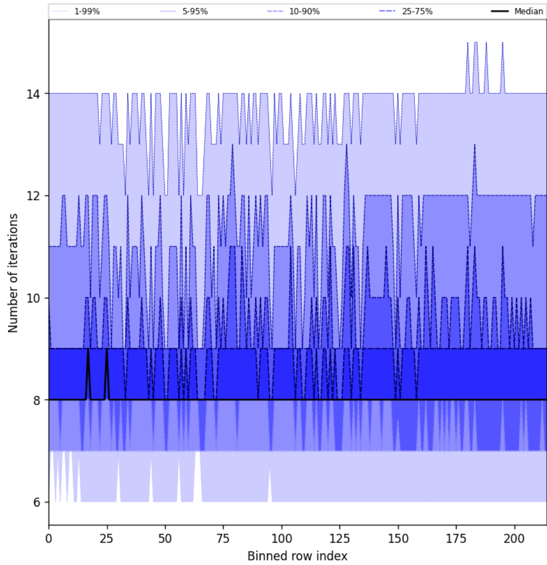
Figure 26: Along track statistics of “Number of iterations” for 2025-09-11 to 2025-09-12
