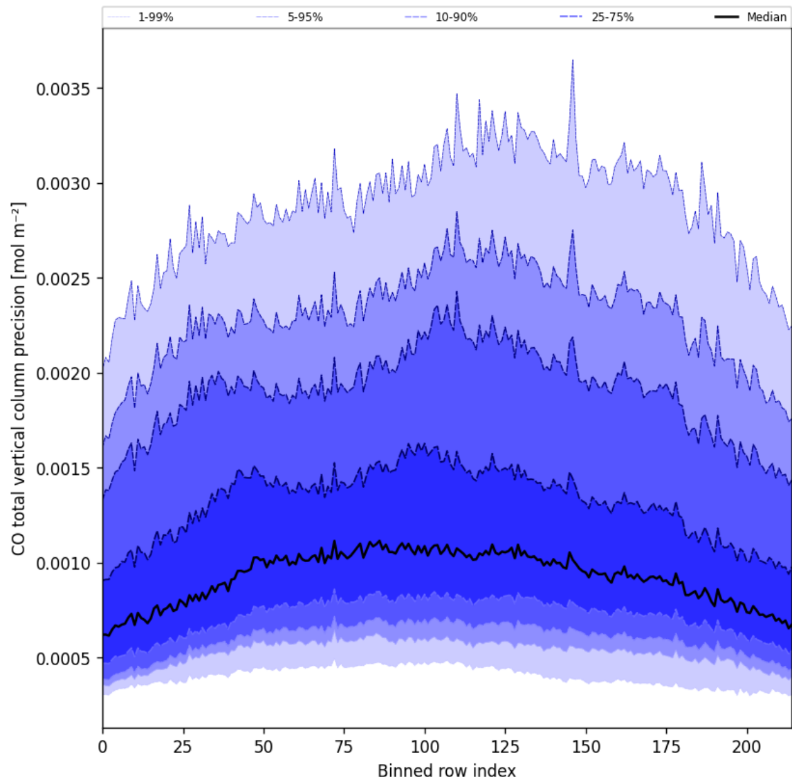
Figure 22: Along track statistics of “CO total vertical column precision” for 2025-09-11 to 2025-09-12
