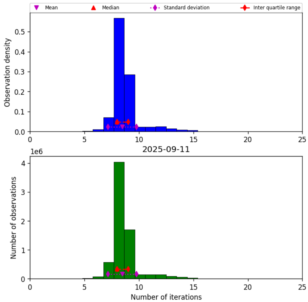
Figure 19: Histogram of “Number of iterations” for 2025-09-11 to 2025-09-12
