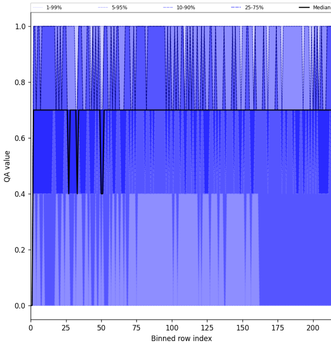
Figure 20: Along track statistics of “QA value” for 2025-09-11 to 2025-09-12
