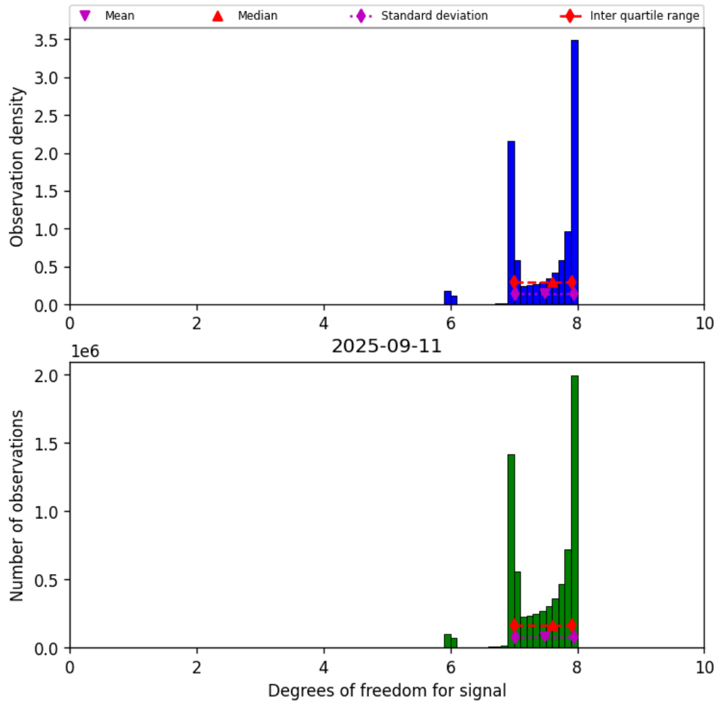
Figure 18: Histogram of “Degrees of freedom for signal” for 2025-09-11 to 2025-09-12
