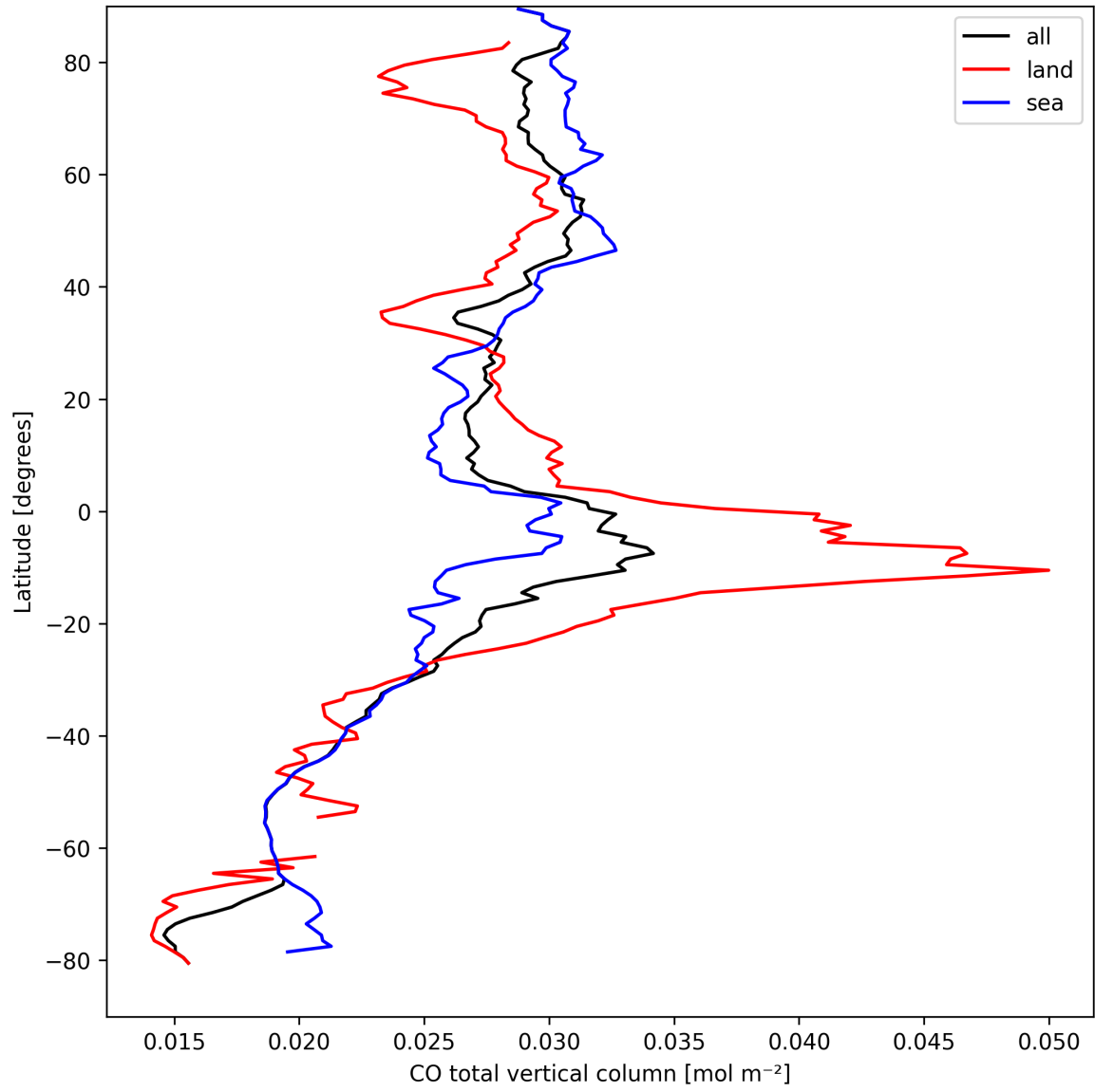
Figure 7: Zonal average of “CO total vertical column” for 2025-09-11 to 2025-09-12.
