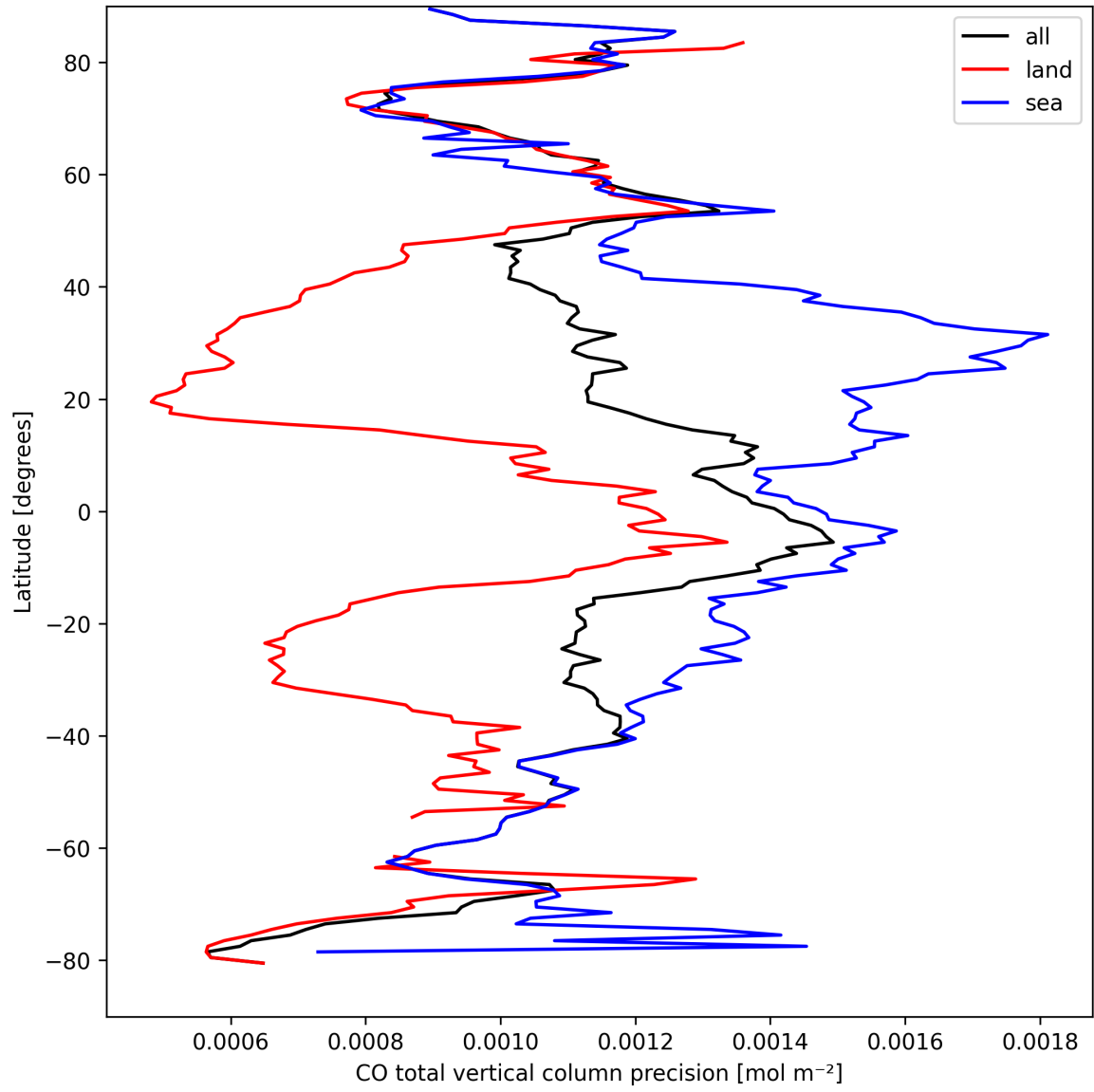
Figure 8: Zonal average of "CO total vertical column precision" for 2025-09-11 to 2025-09-12.
