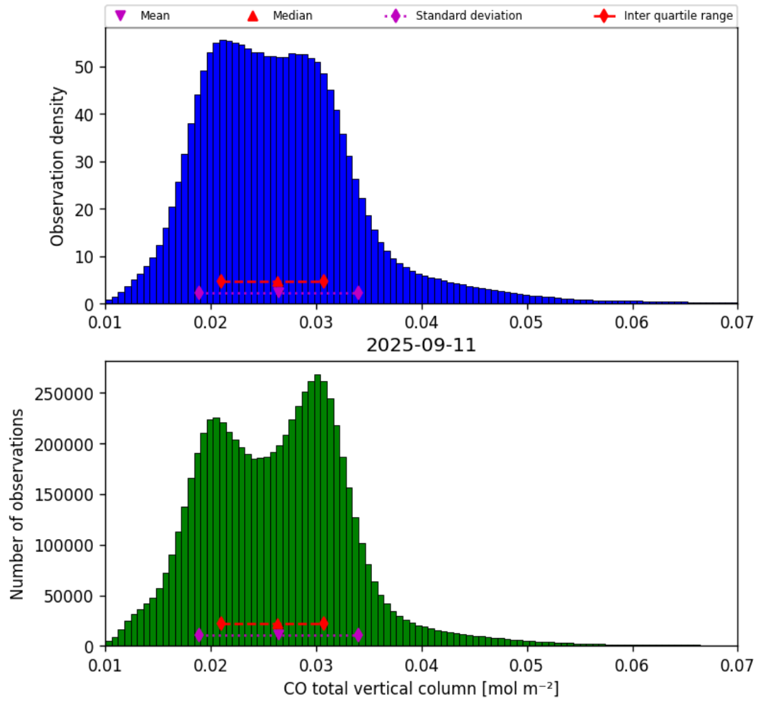
Figure 14: Histogram of “CO total vertical column” for 2025-09-11 to 2025-09-12
