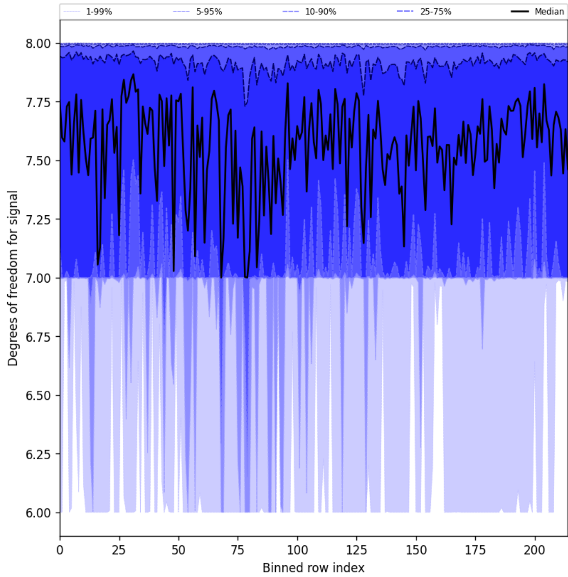
Figure 25: Along track statistics of “Degrees of freedom for signal” for 2025-09-11 to 2025-09-12
