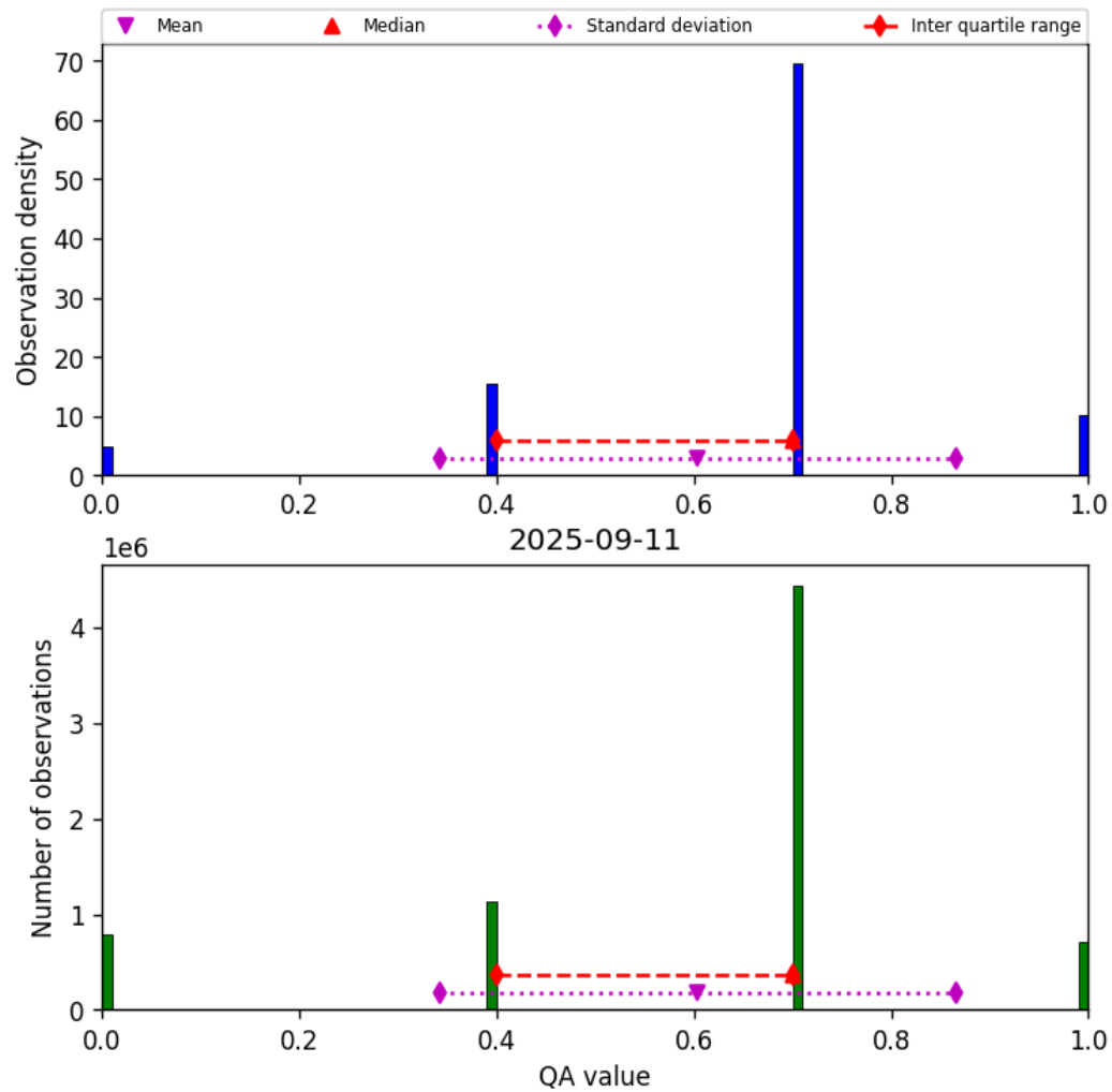
Figure 13: Histogram of “QA value” for 2025-09-11 to 2025-09-12
