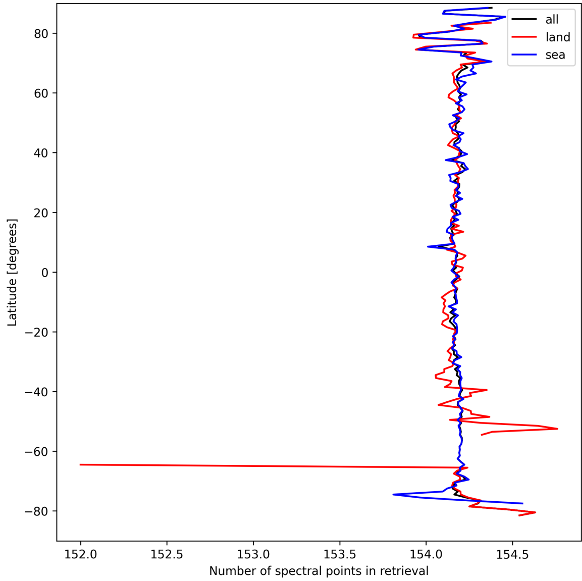
Figure 9: Zonal average of “Number of spectral points in retrieval” for 2025-09-13 to 2025-09-13.
