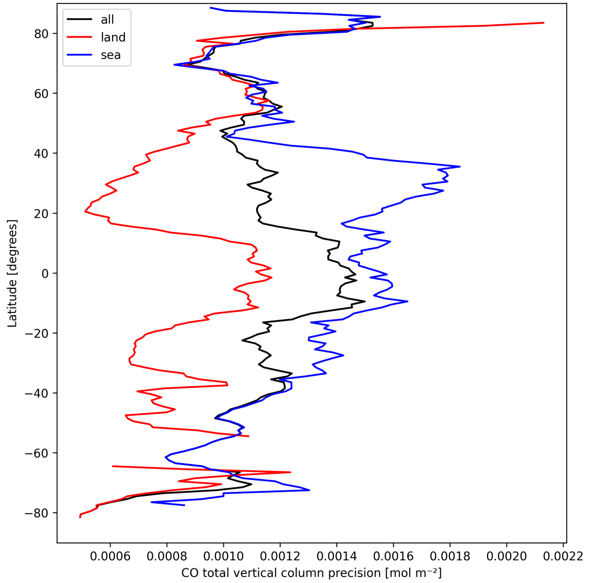
Figure 8: Zonal average of “CO total vertical column precision” for 2025-09-13 to 2025-09-13.
