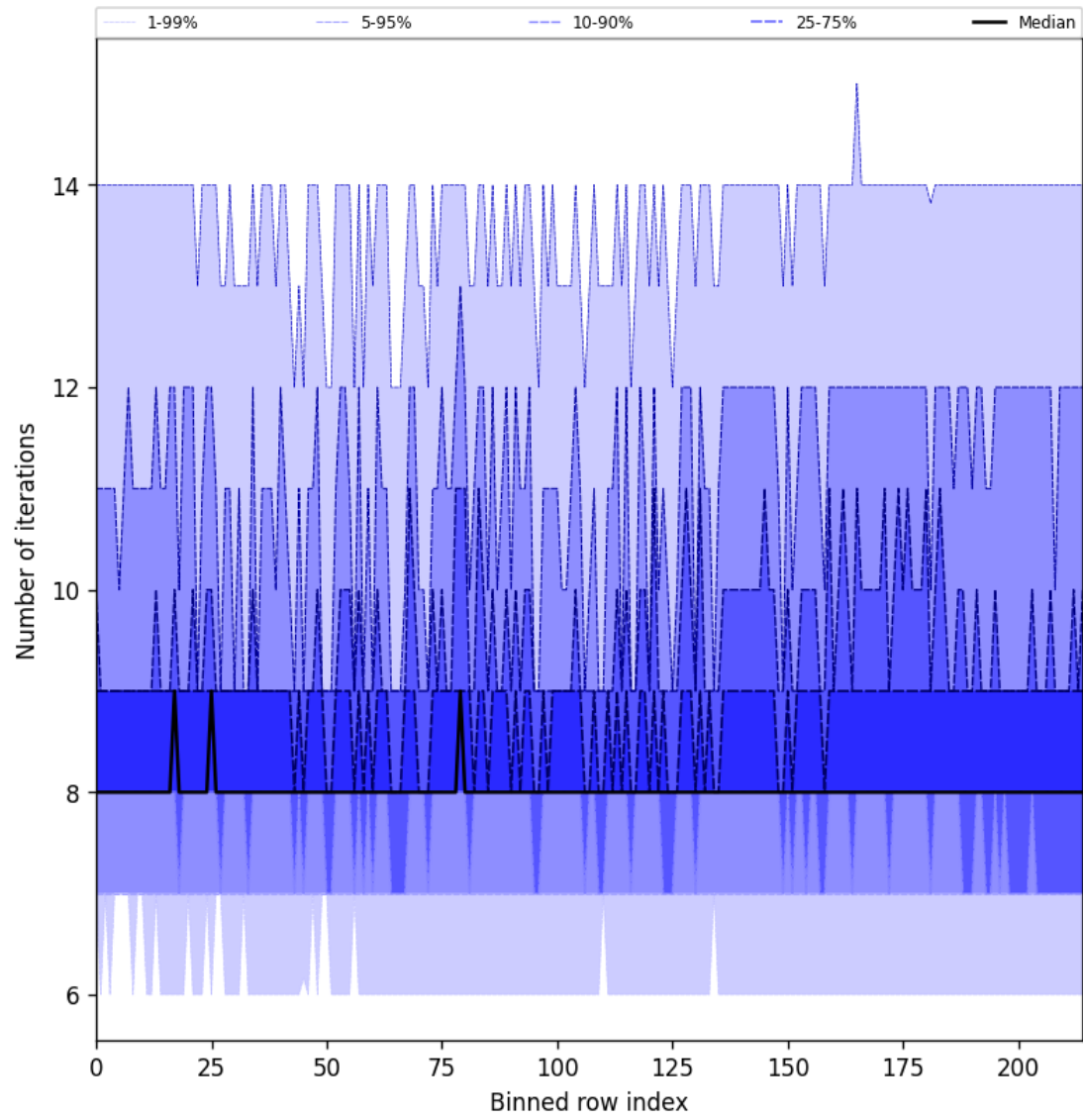
Figure 26: Along track statistics of “Number of iterations” for 2025-09-13 to 2025-09-13
