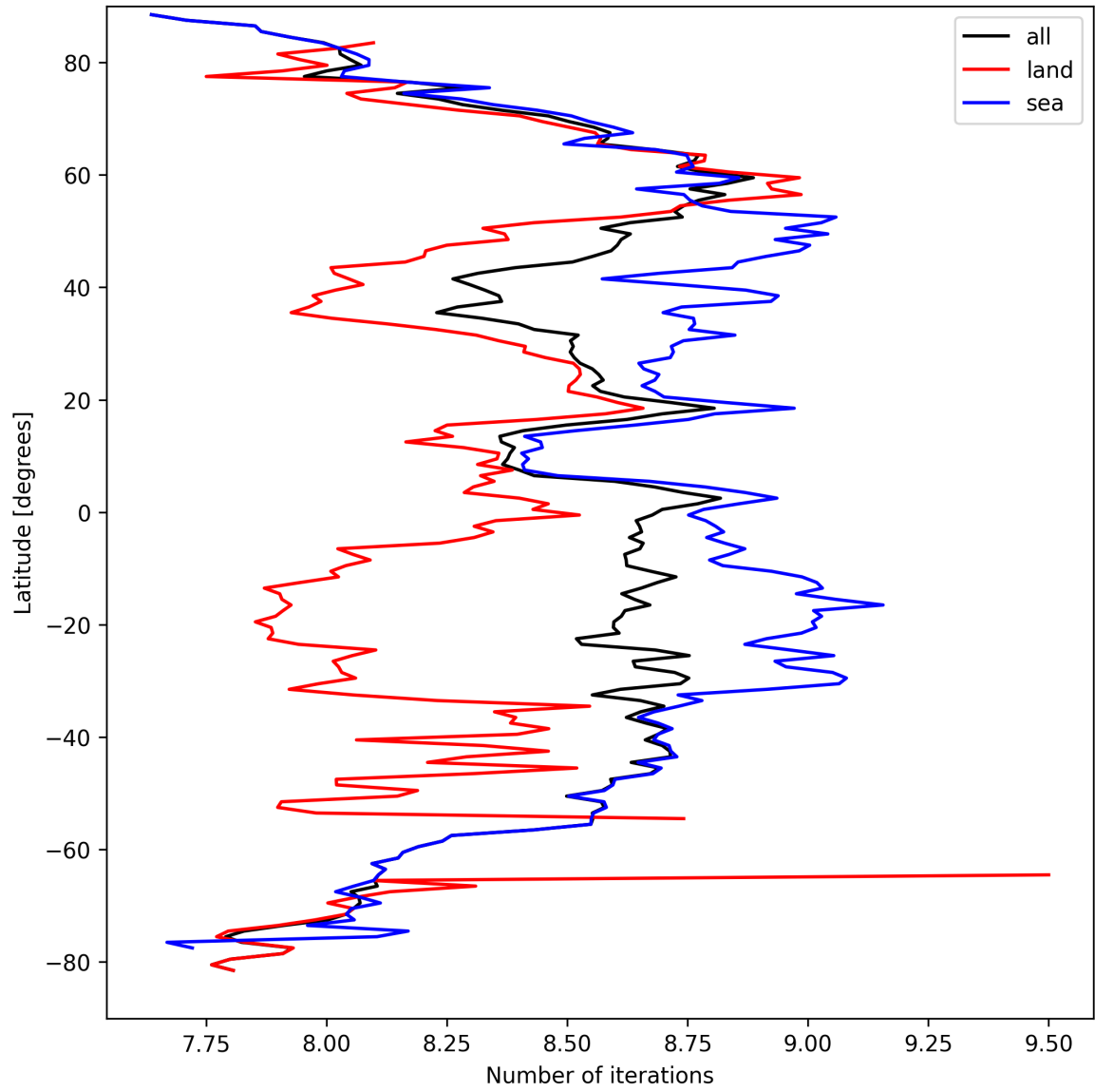
Figure 12: Zonal average of “Number of iterations” for 2025-09-13 to 2025-09-13.
