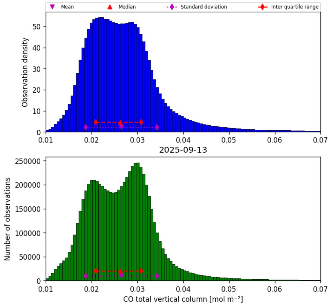
Figure 14: Histogram of “CO total vertical column” for 2025-09-13 to 2025-09-13
