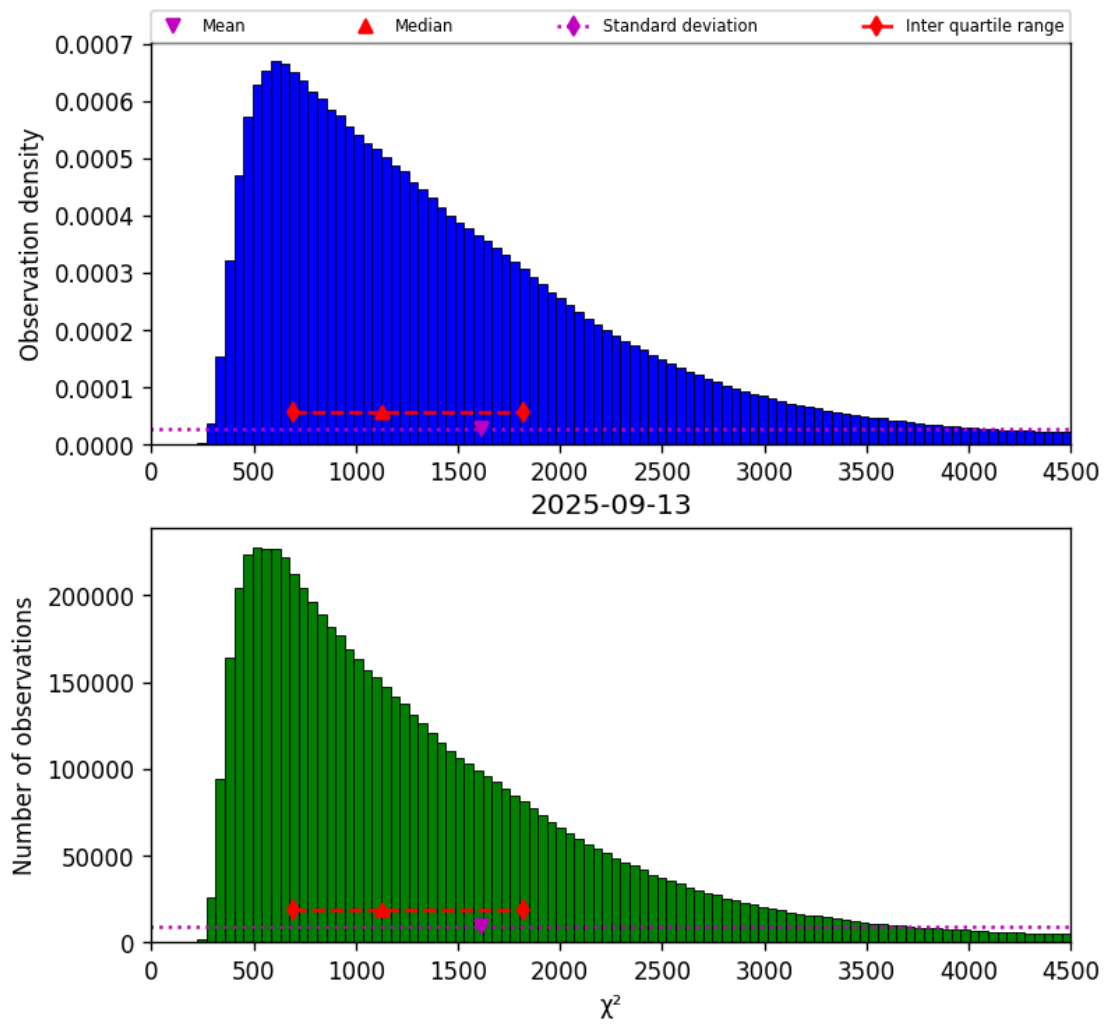
Figure 17: Histogram of " \chi^2 " for 2025-09-13 to 2025-09-13
