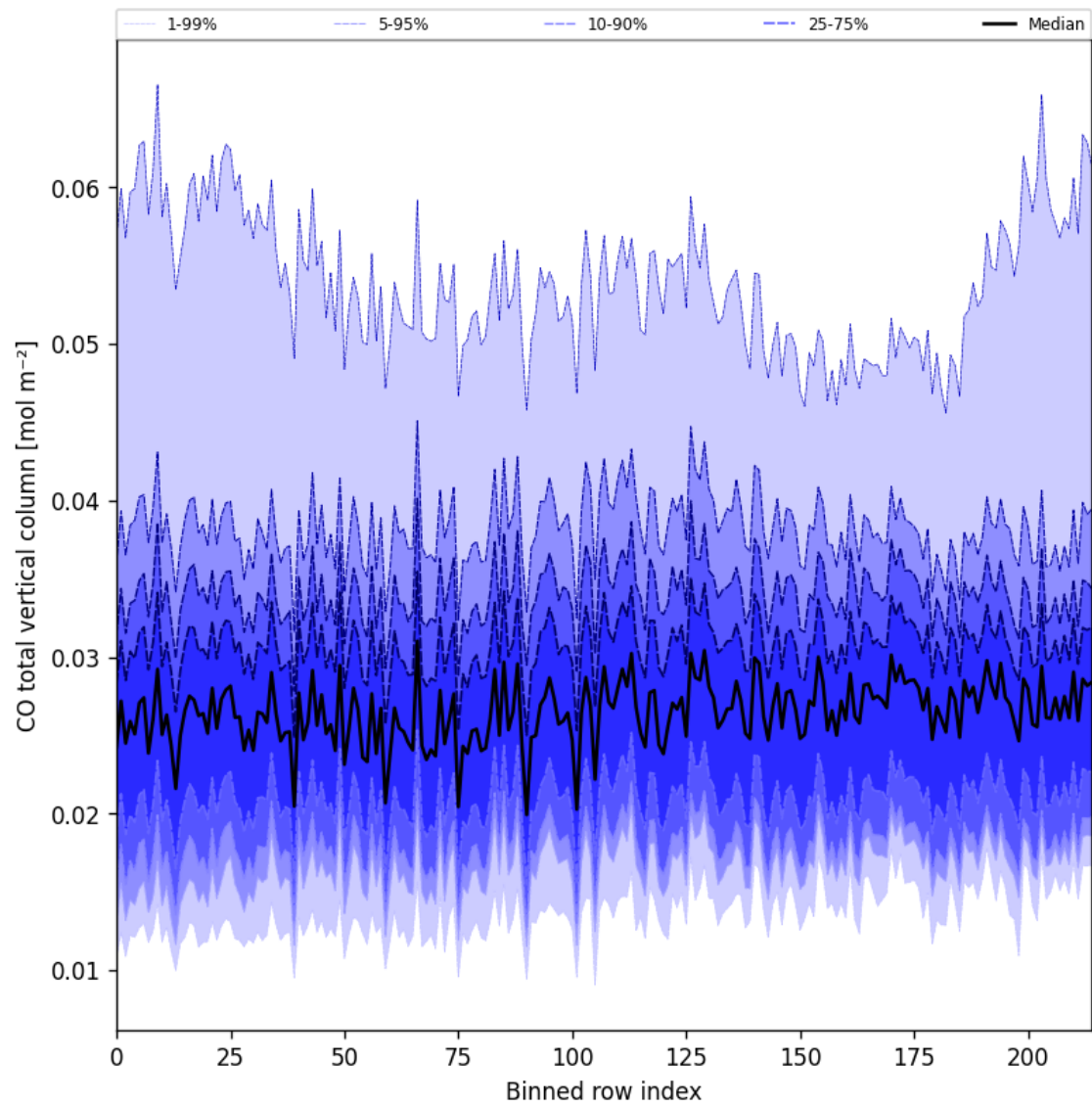
Figure 21: Along track statistics of “CO total vertical column” for 2025-09-13 to 2025-09-13
