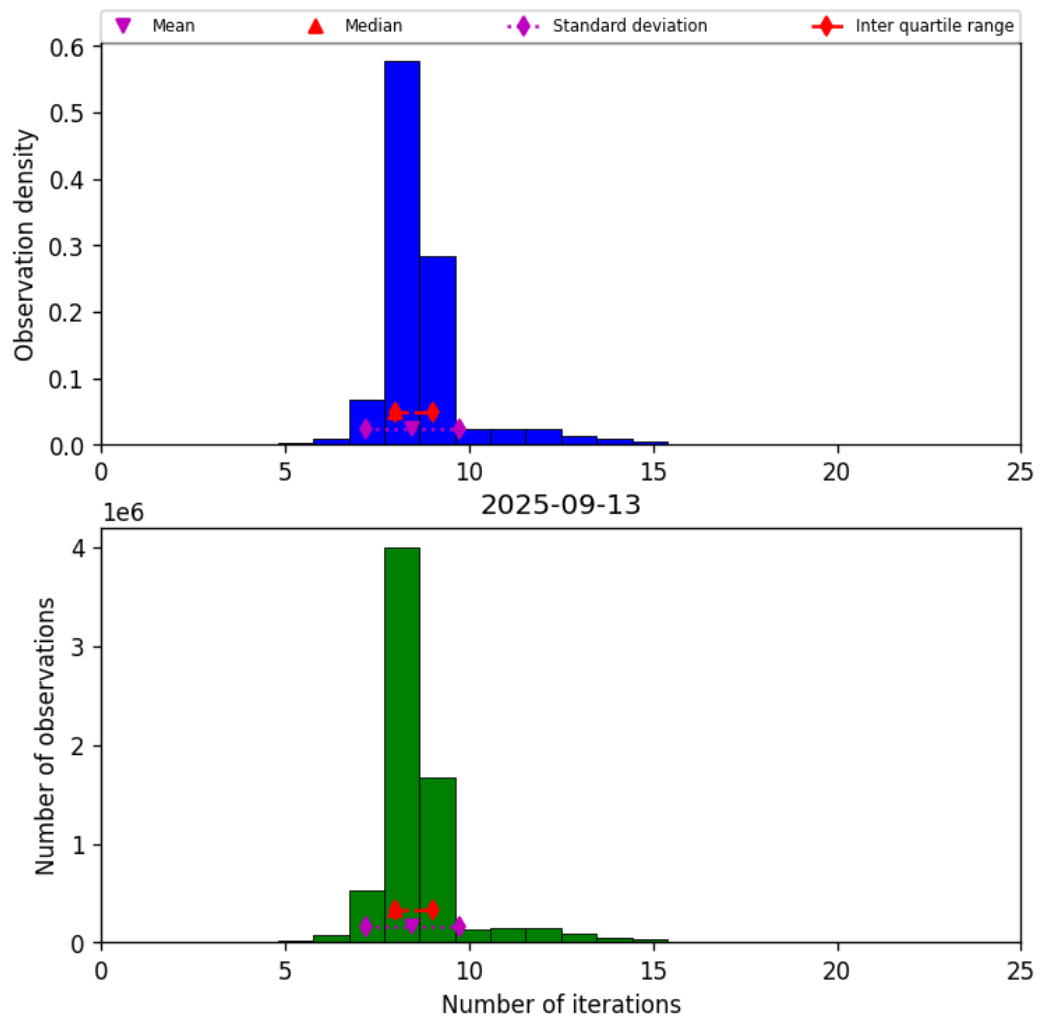
Figure 19: Histogram of “Number of iterations” for 2025-09-13 to 2025-09-13
