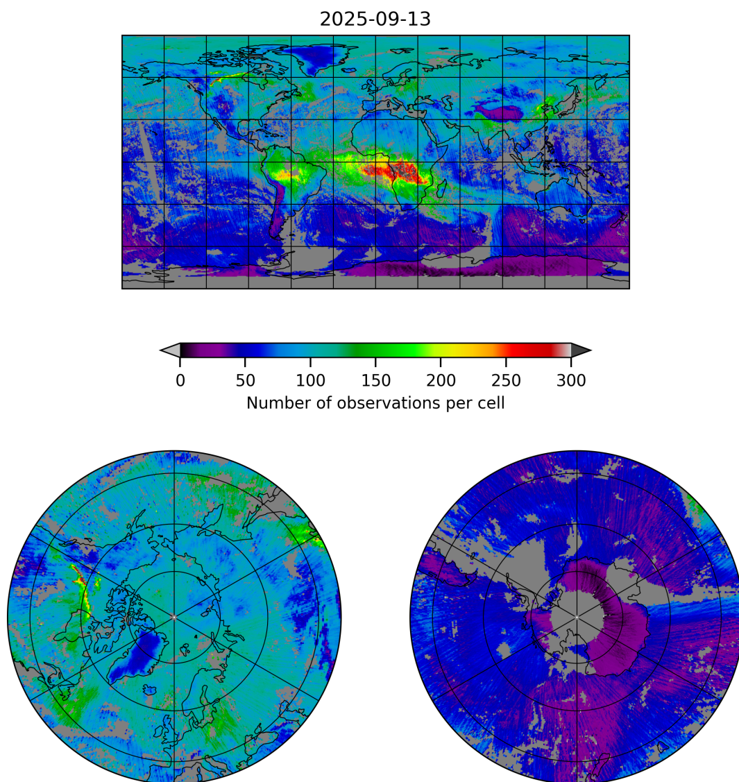
Figure 5: Map of the number of observations for 2025-09-13 to 2025-09-13
