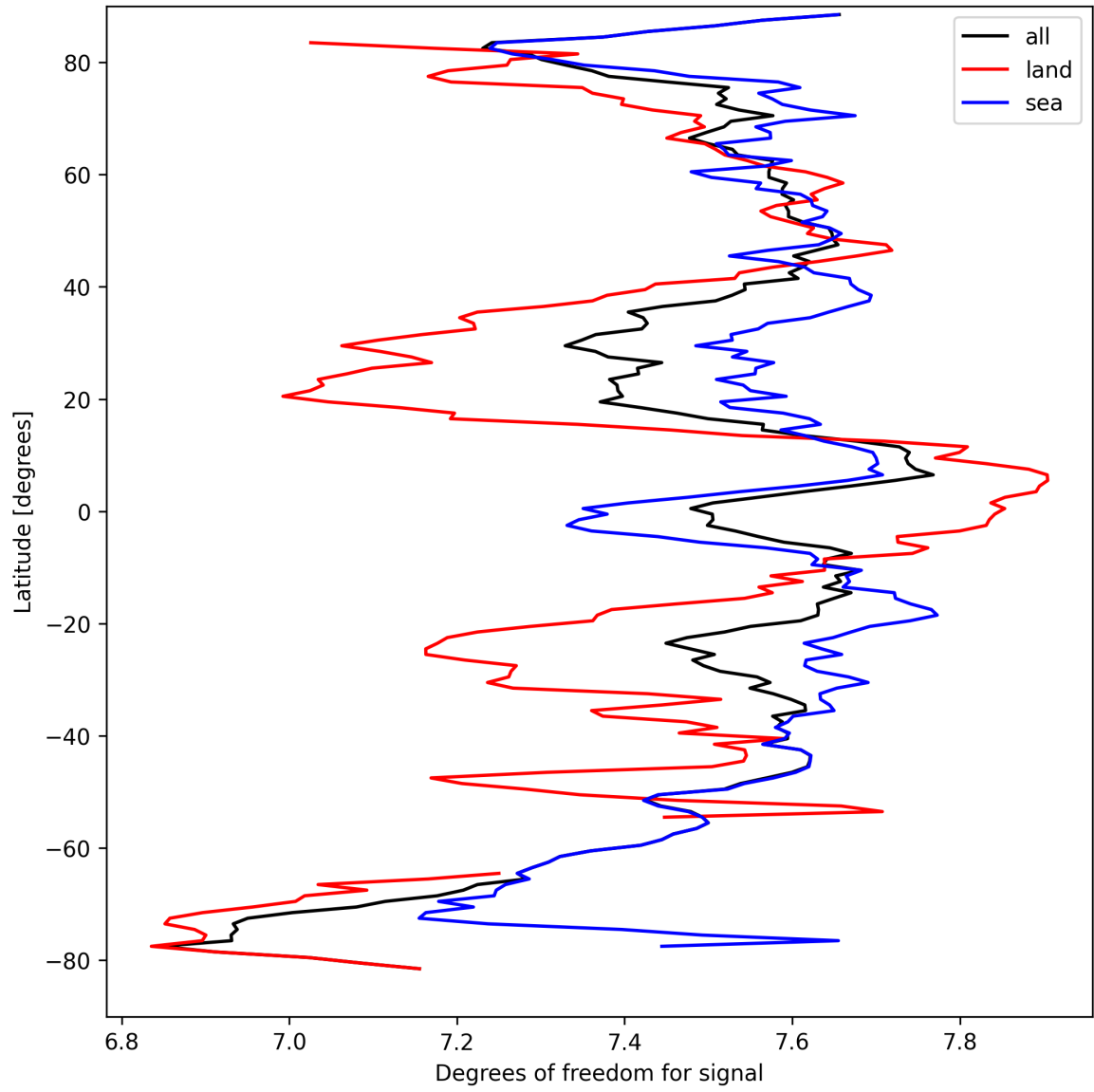
Figure 11: Zonal average of “Degrees of freedom for signal” for 2025-09-13 to 2025-09-13.
