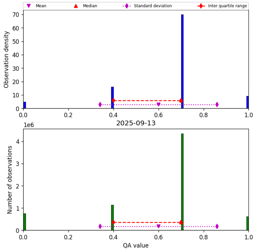
Figure 13: Histogram of “QA value” for 2025-09-13 to 2025-09-13
