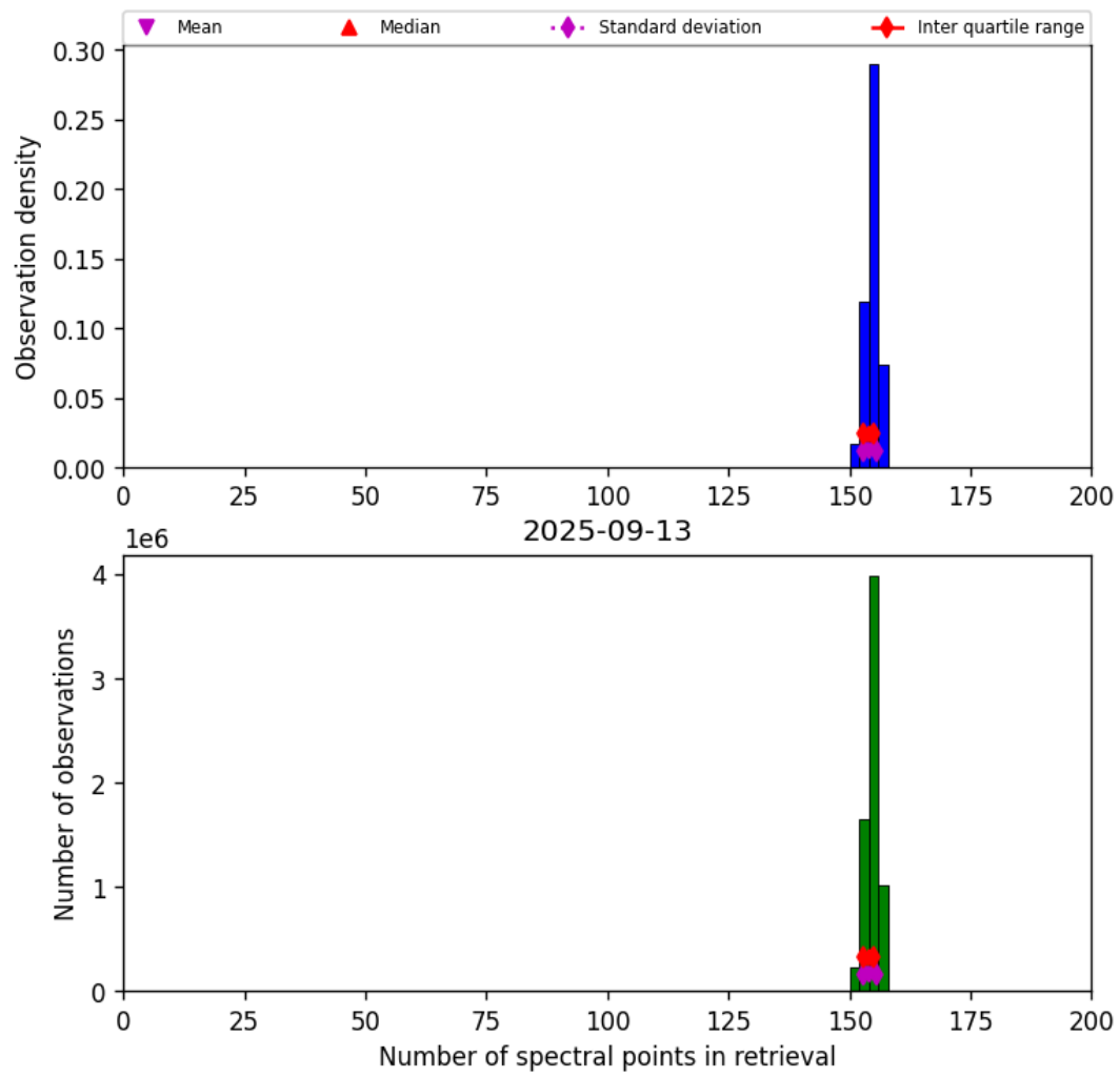
Figure 16: Histogram of “Number of spectral points in retrieval” for 2025-09-13 to 2025-09-13
