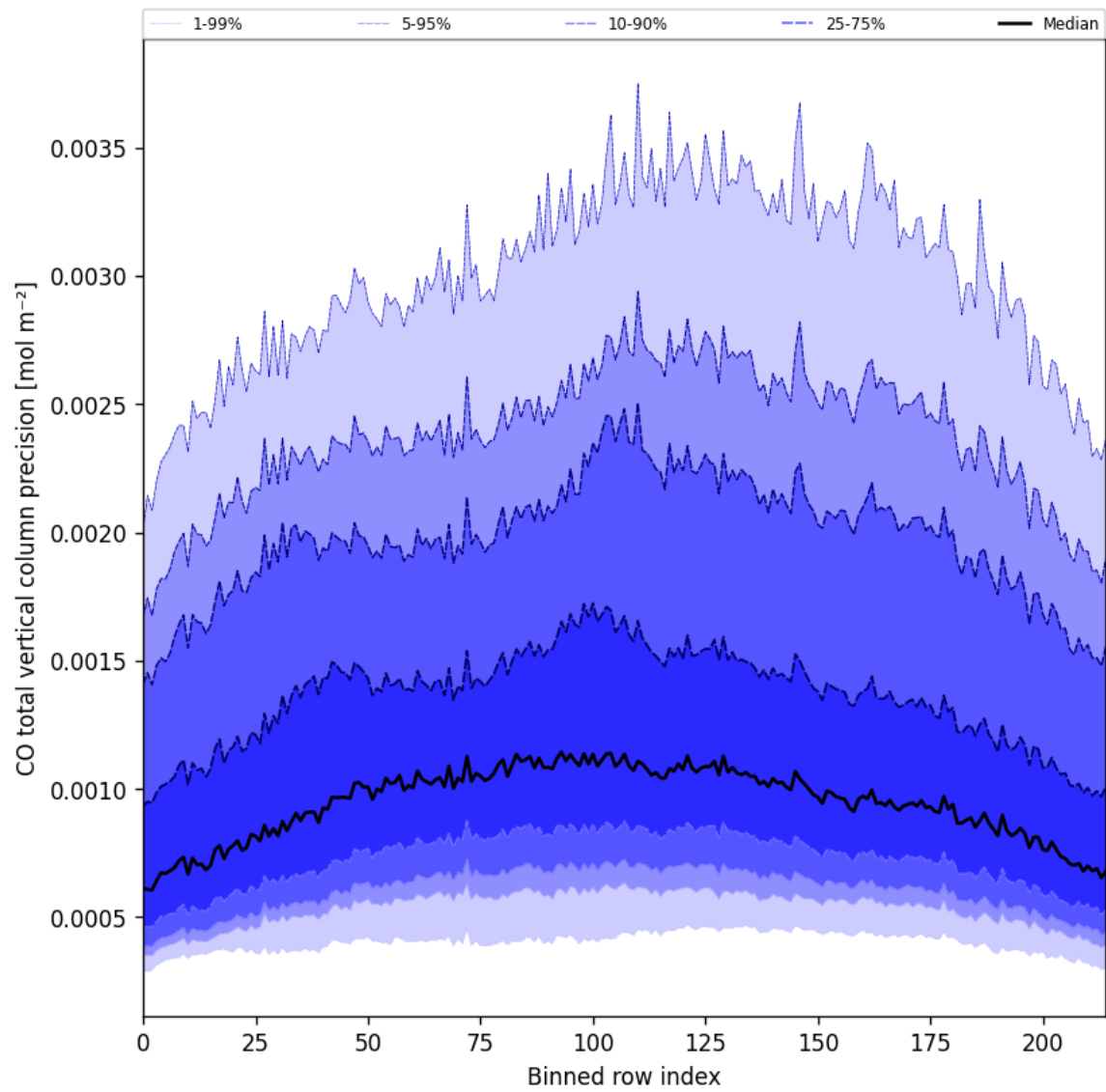
Figure 22: Along track statistics of “CO total vertical column precision” for 2025-09-13 to 2025-09-13
