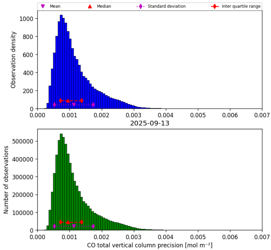
Figure 15: Histogram of "CO total vertical column precision" for 2025-09-13 to 2025-09-13
