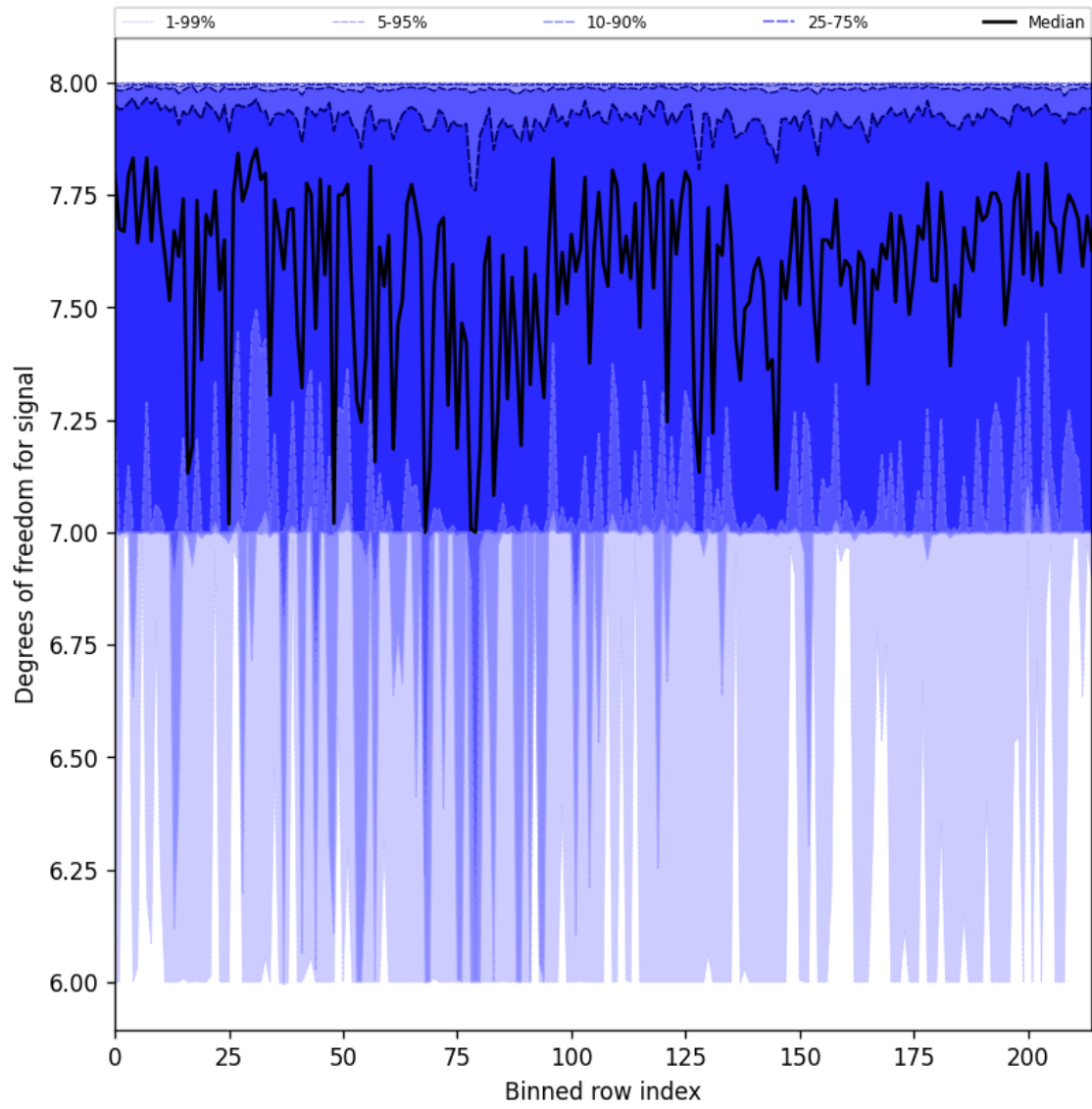
Figure 25: Along track statistics of “Degrees of freedom for signal” for 2025-09-13 to 2025-09-13
