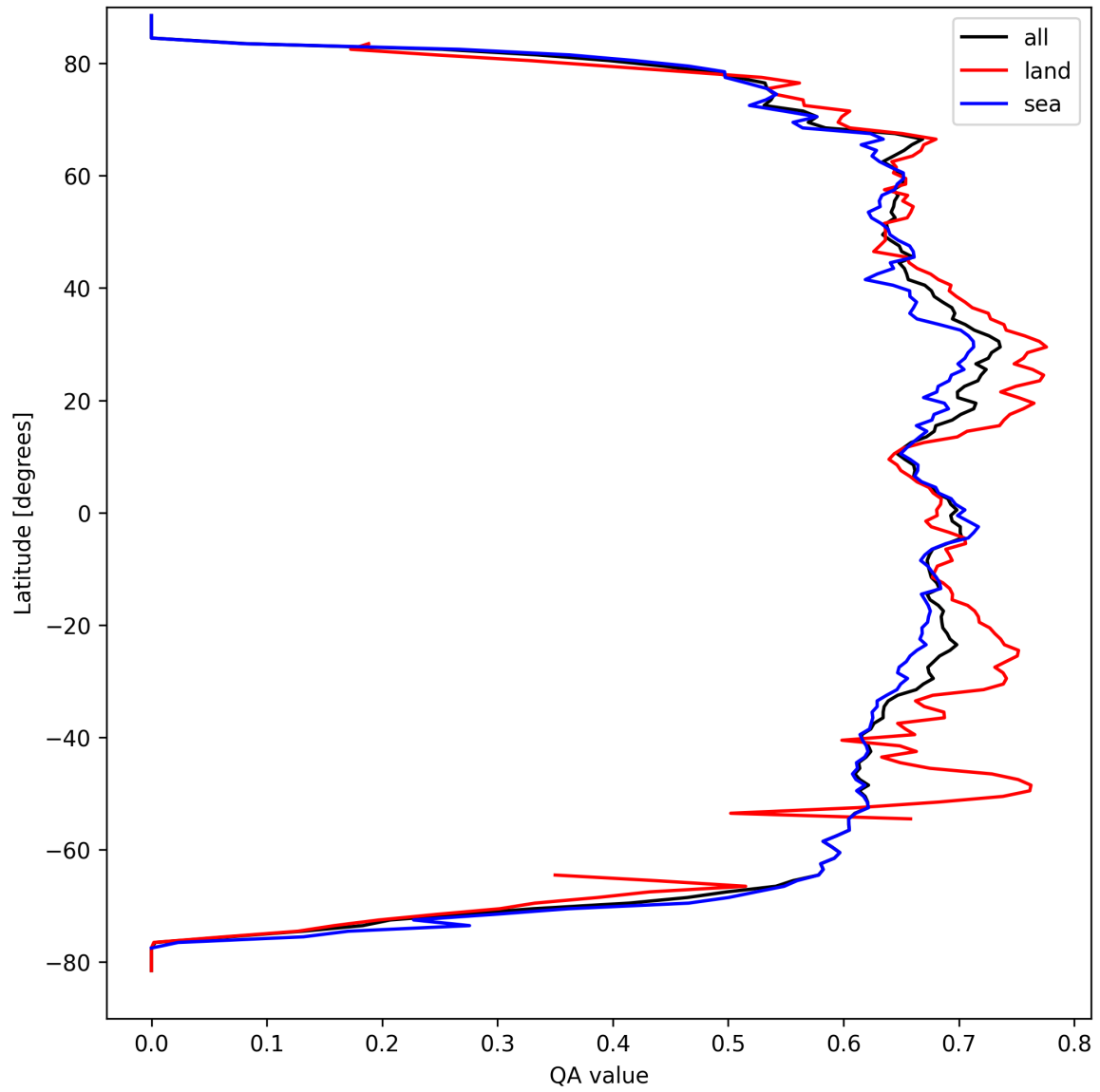
Figure 6: Zonal average of “QA value” for 2025-09-13 to 2025-09-13.
