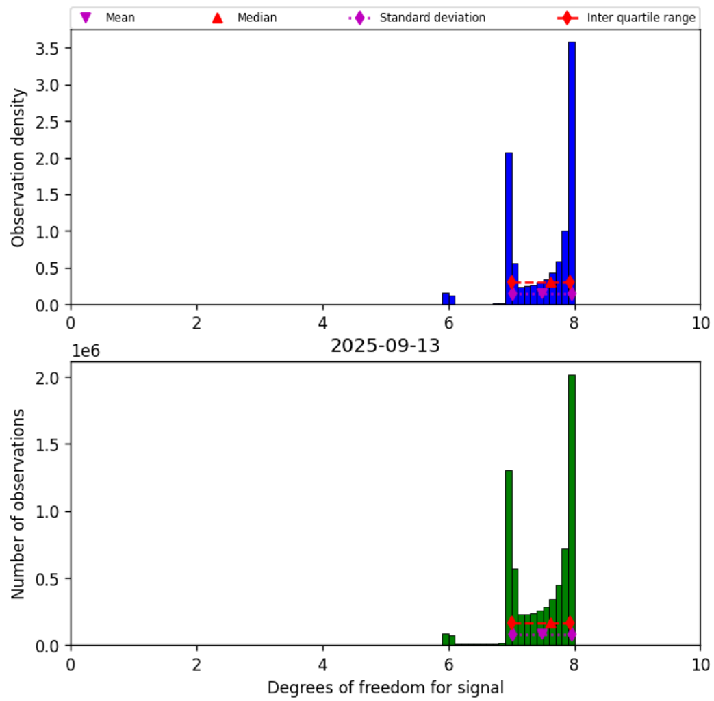
Figure 18: Histogram of “Degrees of freedom for signal” for 2025-09-13 to 2025-09-13
