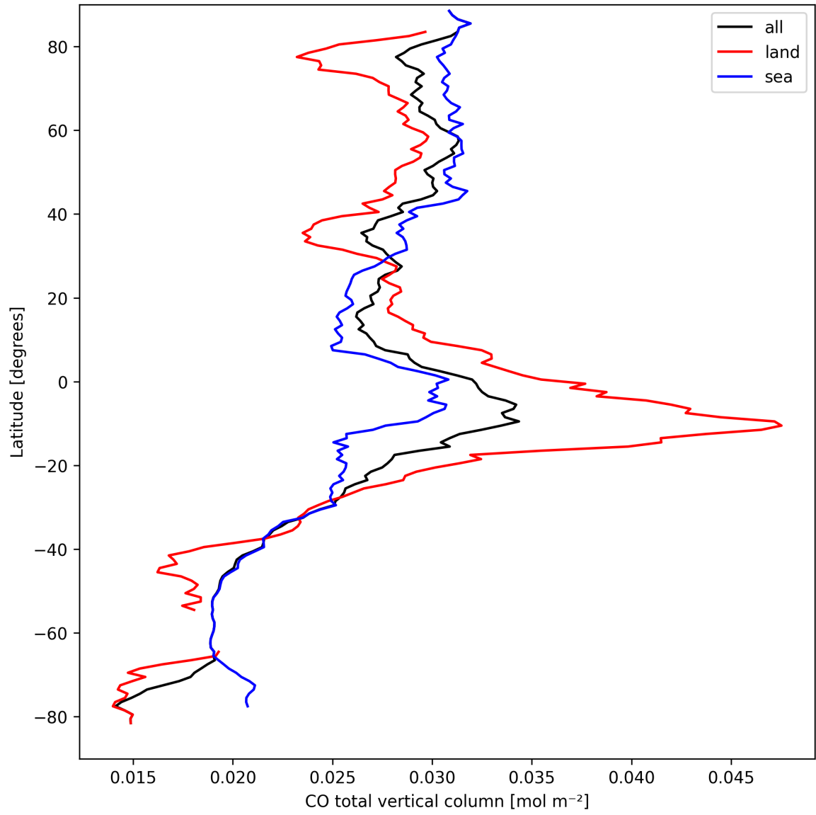
Figure 7: Zonal average of “CO total vertical column” for 2025-09-13 to 2025-09-13.
