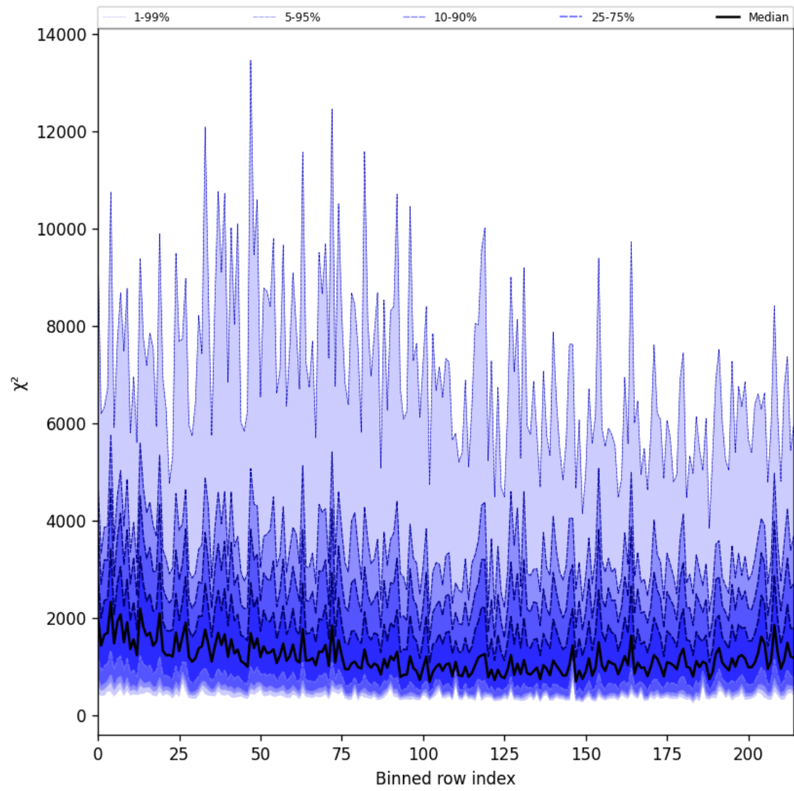
Figure 24: Along track statistics of “ \chi^2 ” for 2025-09-13 to 2025-09-13
