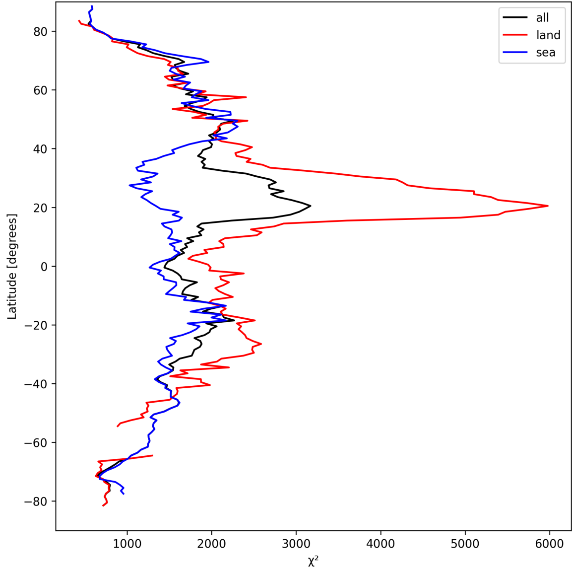
Figure 10: Zonal average of “ \chi^2 ” for 2025-09-13 to 2025-09-13.
