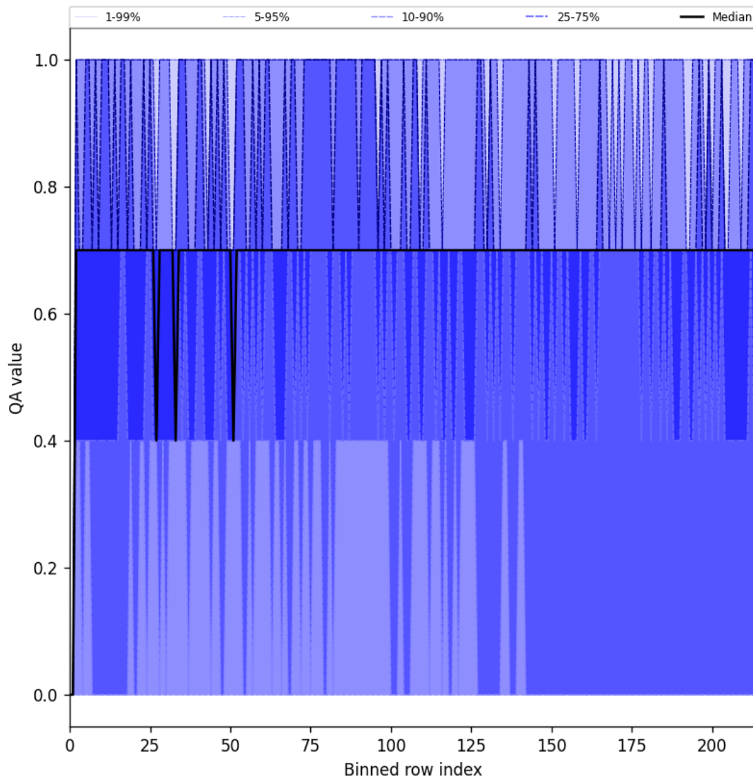
Figure 20: Along track statistics of “QA value” for 2025-09-13 to 2025-09-13
