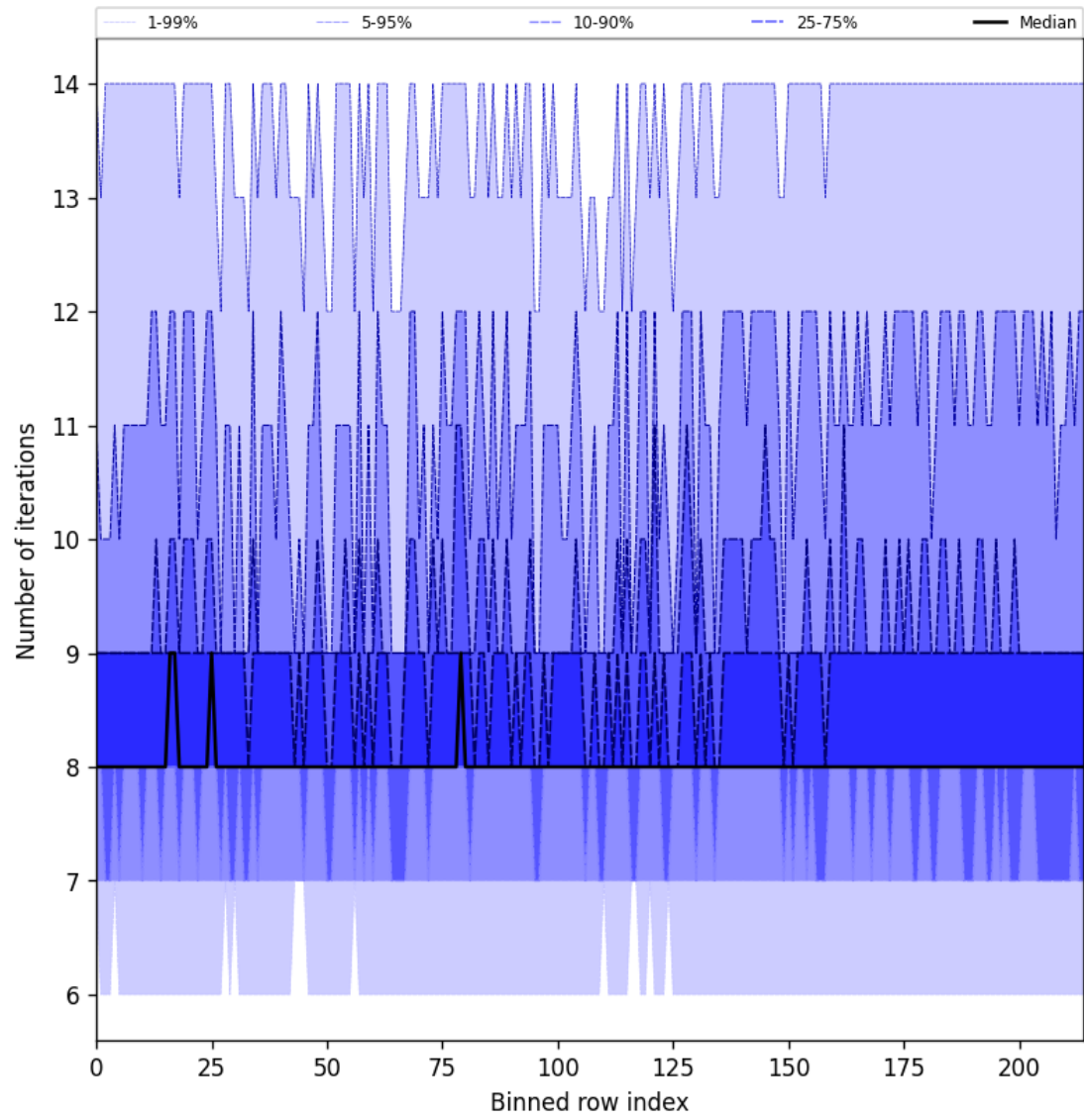
Figure 26: Along track statistics of “Number of iterations” for 2025-09-14 to 2025-09-15
