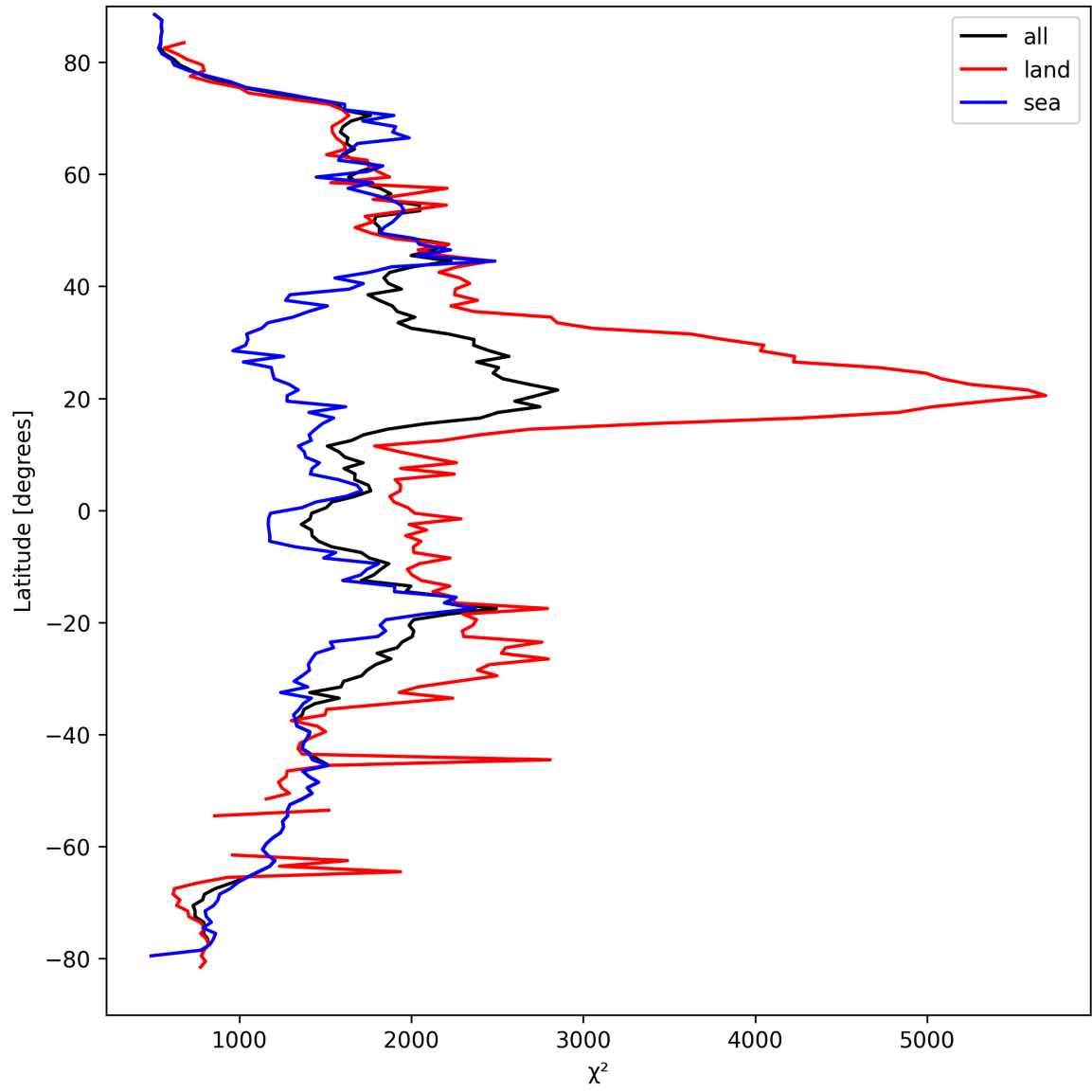
Figure 10: Zonal average of “ \chi^2 ” for 2025-09-14 to 2025-09-15.
