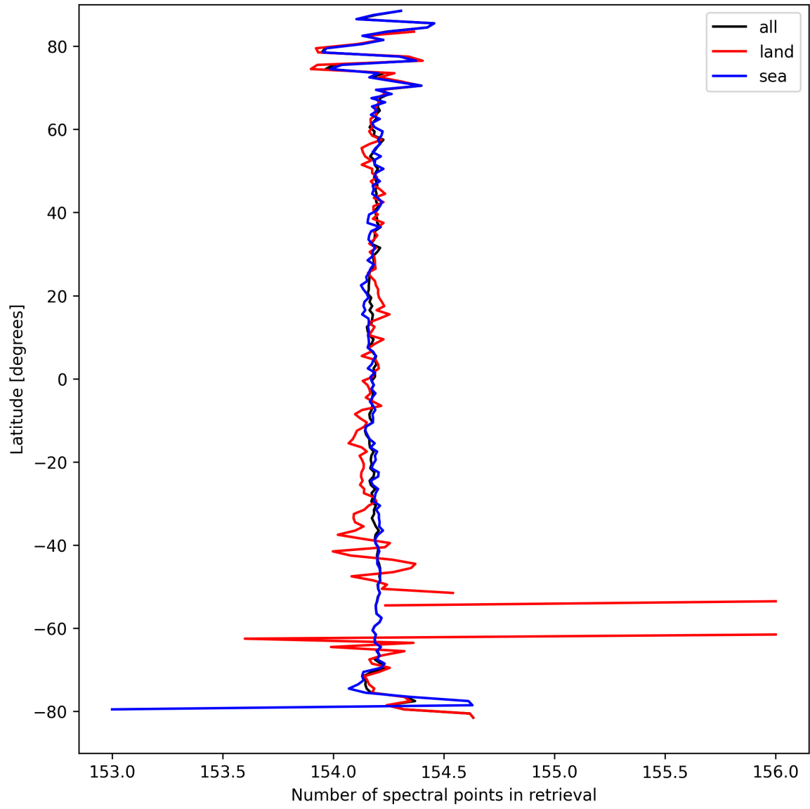
Figure 9: Zonal average of “Number of spectral points in retrieval” for 2025-09-14 to 2025-09-15.
