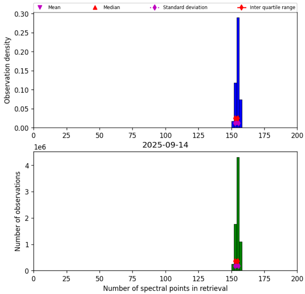
Figure 16: Histogram of “Number of spectral points in retrieval” for 2025-09-14 to 2025-09-15
