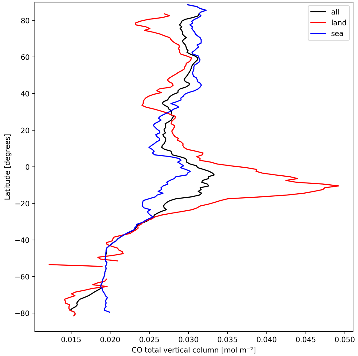
Figure 7: Zonal average of “CO total vertical column” for 2025-09-14 to 2025-09-15.
