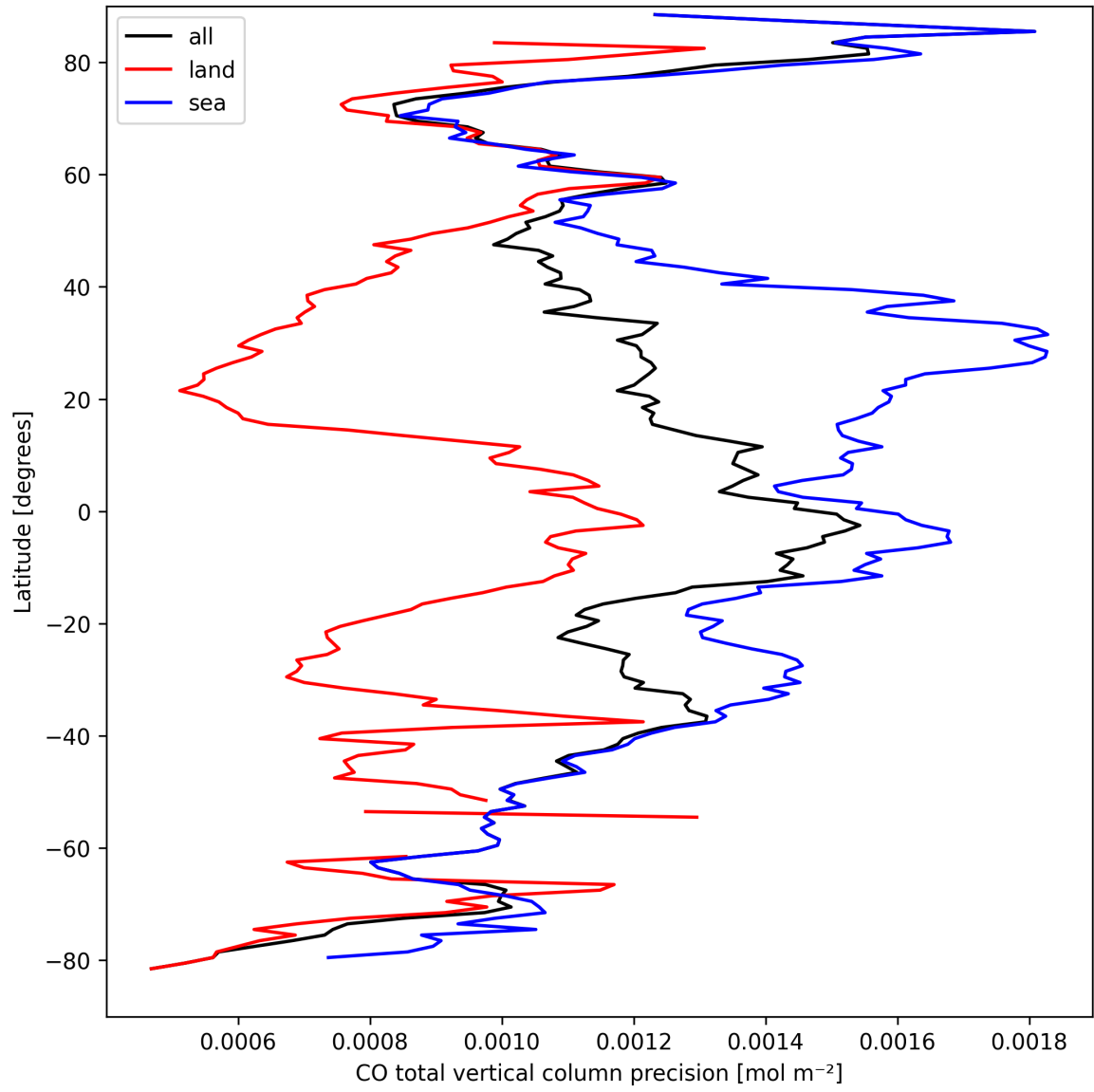
Figure 8: Zonal average of “CO total vertical column precision” for 2025-09-14 to 2025-09-15.
