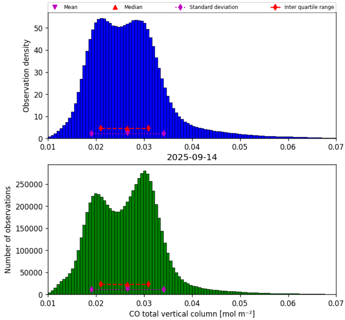
Figure 14: Histogram of “CO total vertical column” for 2025-09-14 to 2025-09-15
