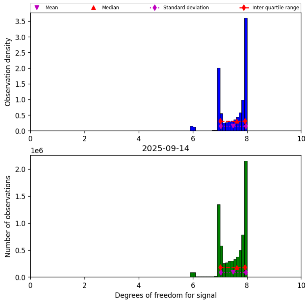
Figure 18: Histogram of “Degrees of freedom for signal” for 2025-09-14 to 2025-09-15
