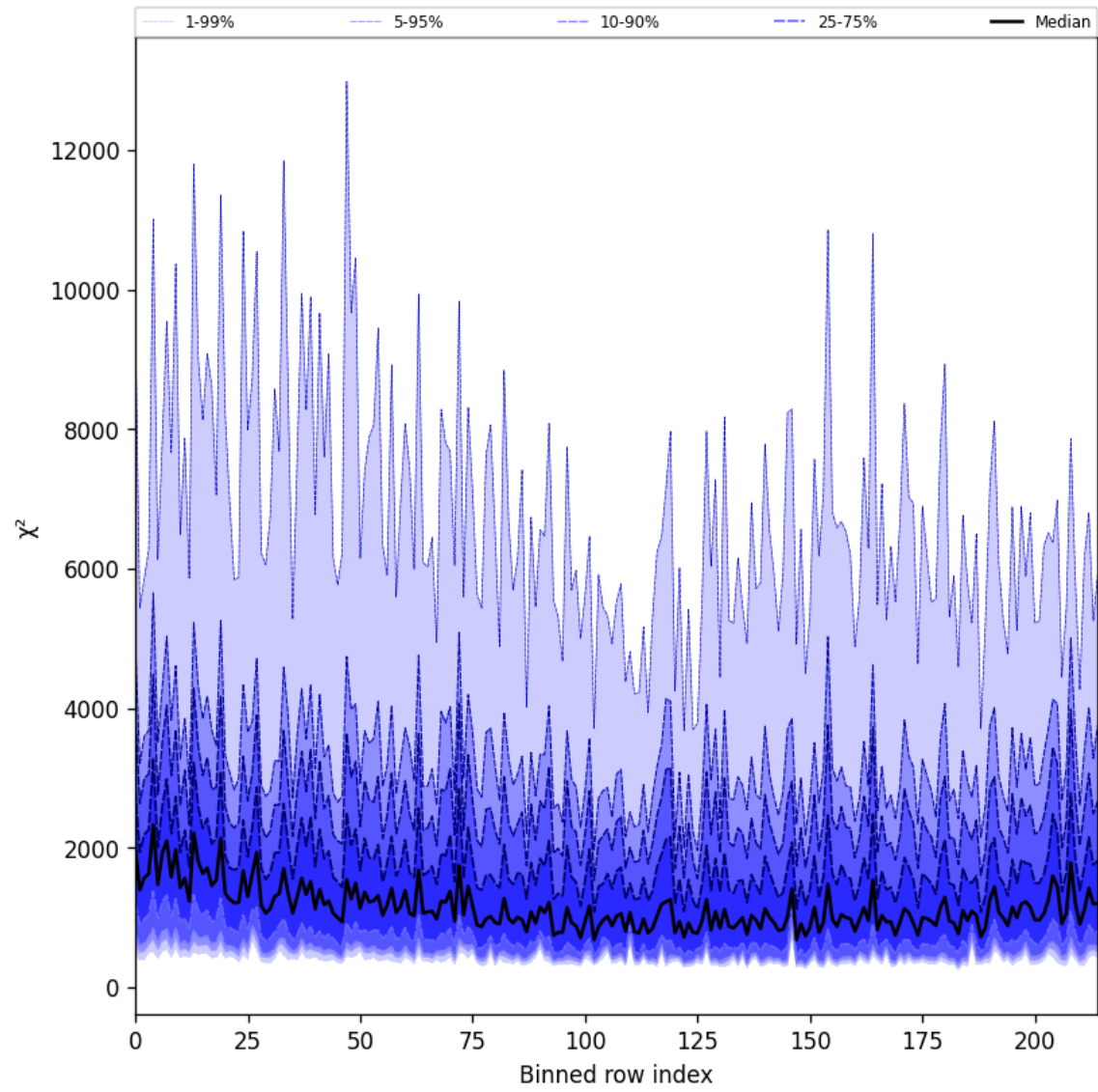
Figure 24: Along track statistics of “ \chi^2 ” for 2025-09-14 to 2025-09-15
