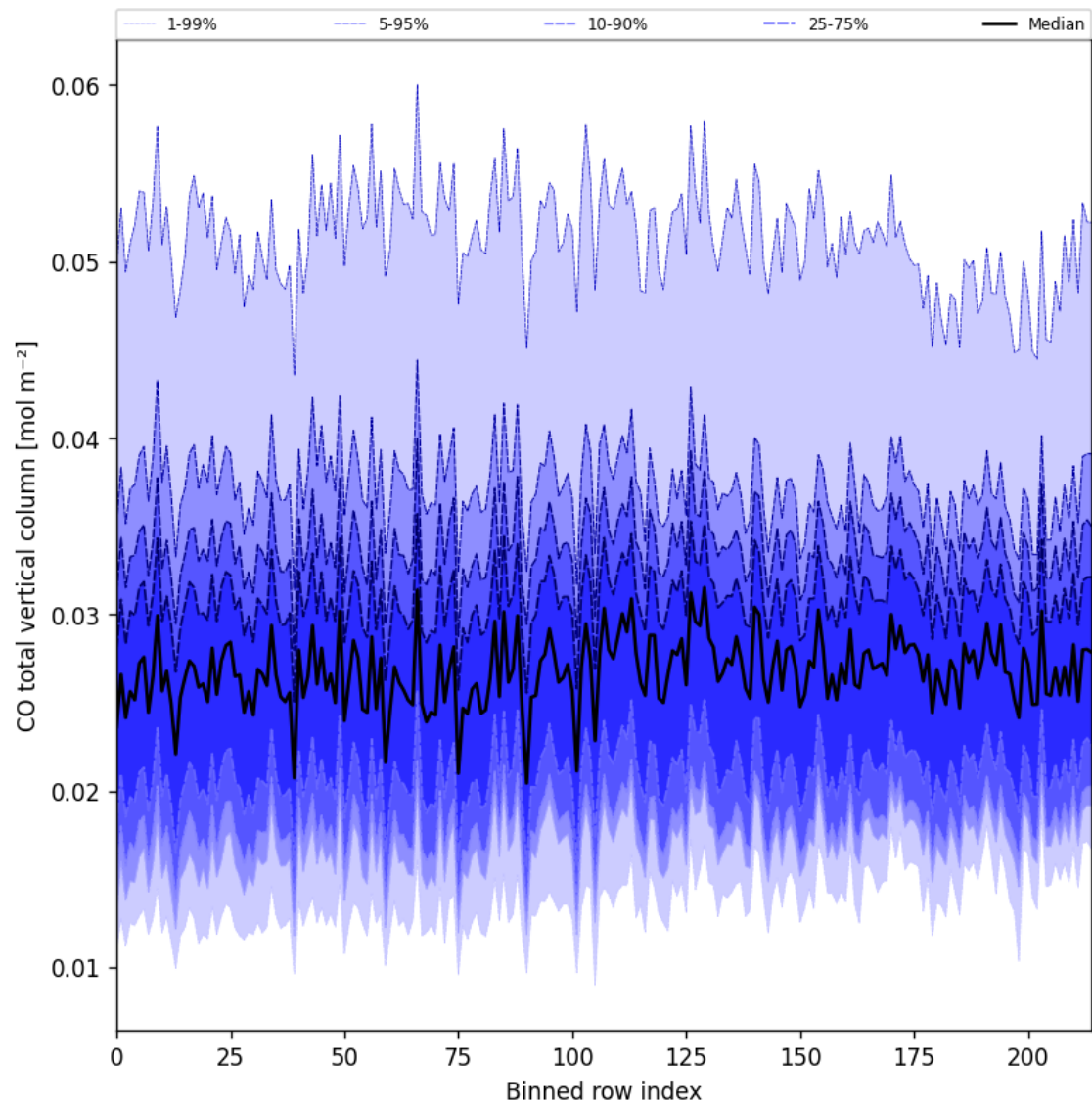
Figure 21: Along track statistics of “CO total vertical column” for 2025-09-14 to 2025-09-15
