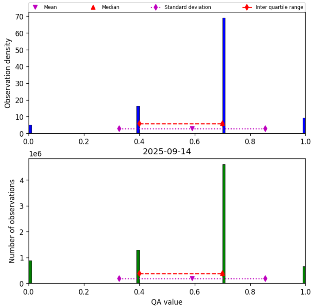
Figure 13: Histogram of “QA value” for 2025-09-14 to 2025-09-15
