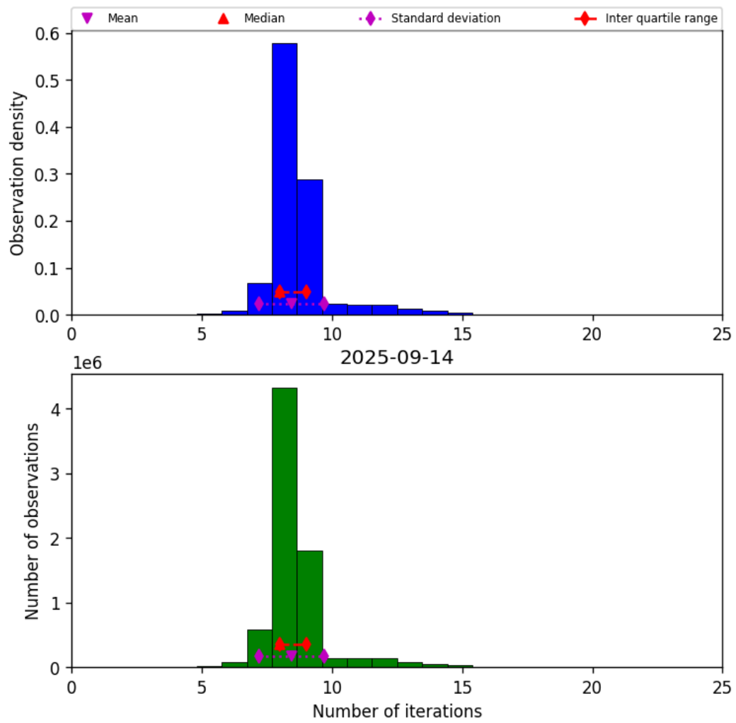
Figure 19: Histogram of “Number of iterations” for 2025-09-14 to 2025-09-15
