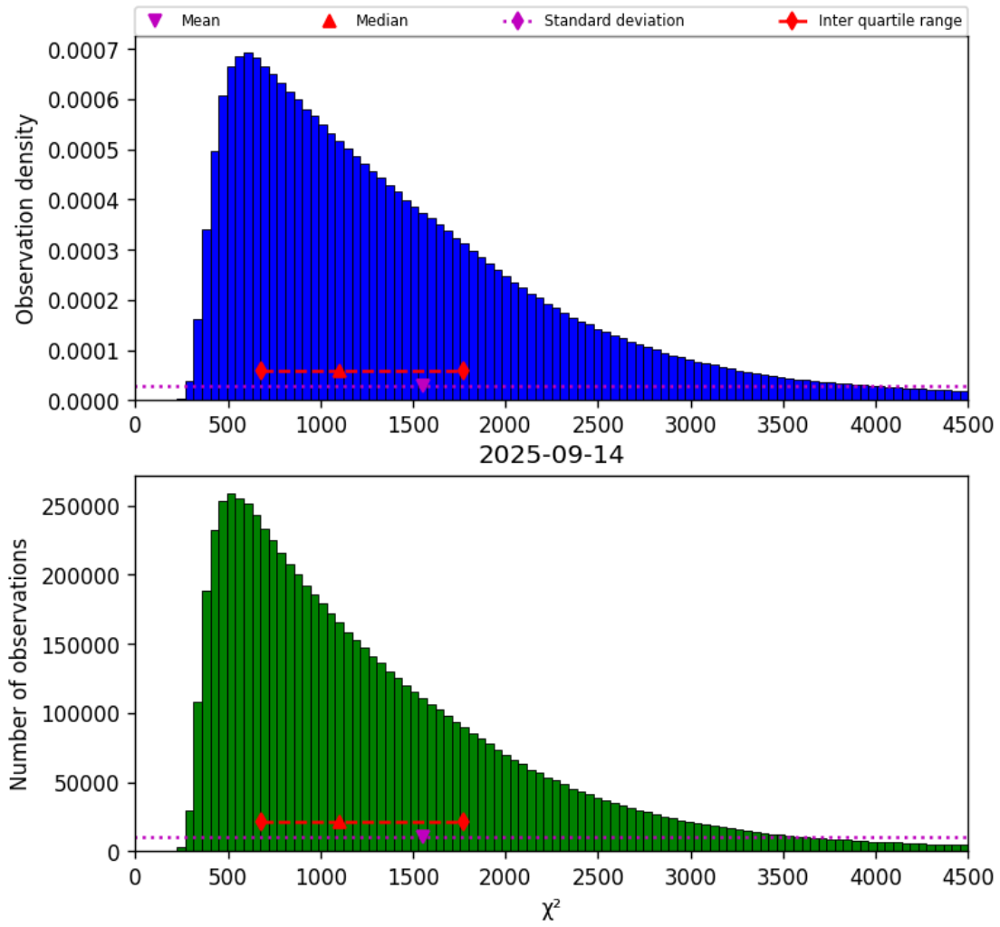
Figure 17: Histogram of “ \chi^2 ” for 2025-09-14 to 2025-09-15
