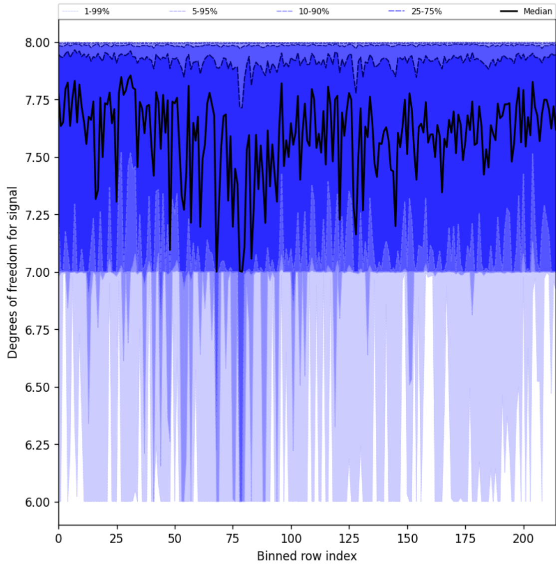
Figure 25: Along track statistics of “Degrees of freedom for signal” for 2025-09-14 to 2025-09-15
