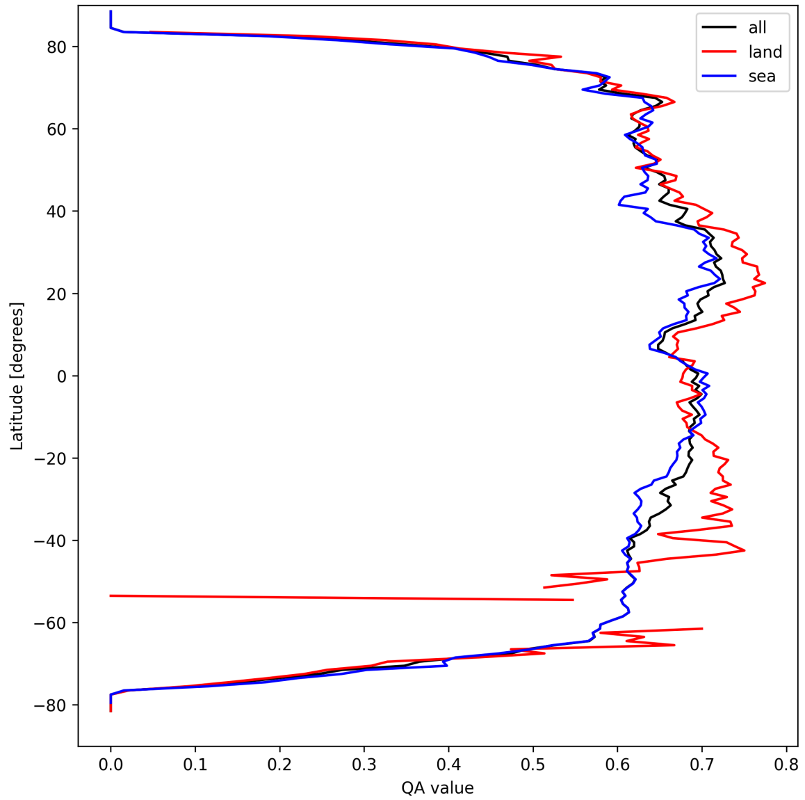
Figure 6: Zonal average of “QA value” for 2025-09-14 to 2025-09-15.
