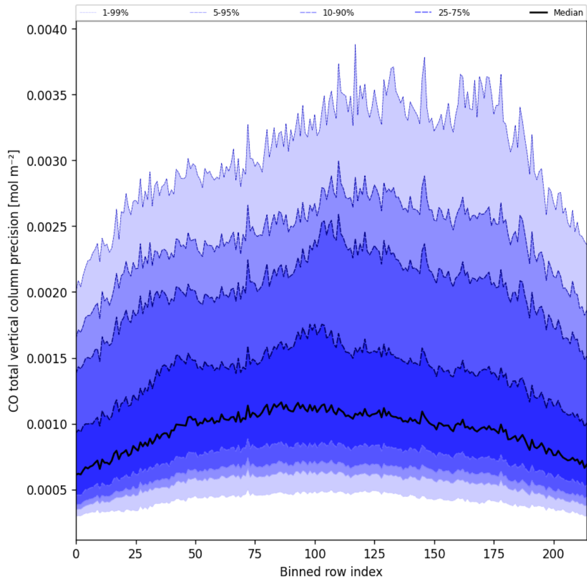
Figure 22: Along track statistics of “CO total vertical column precision” for 2025-09-14 to 2025-09-15
