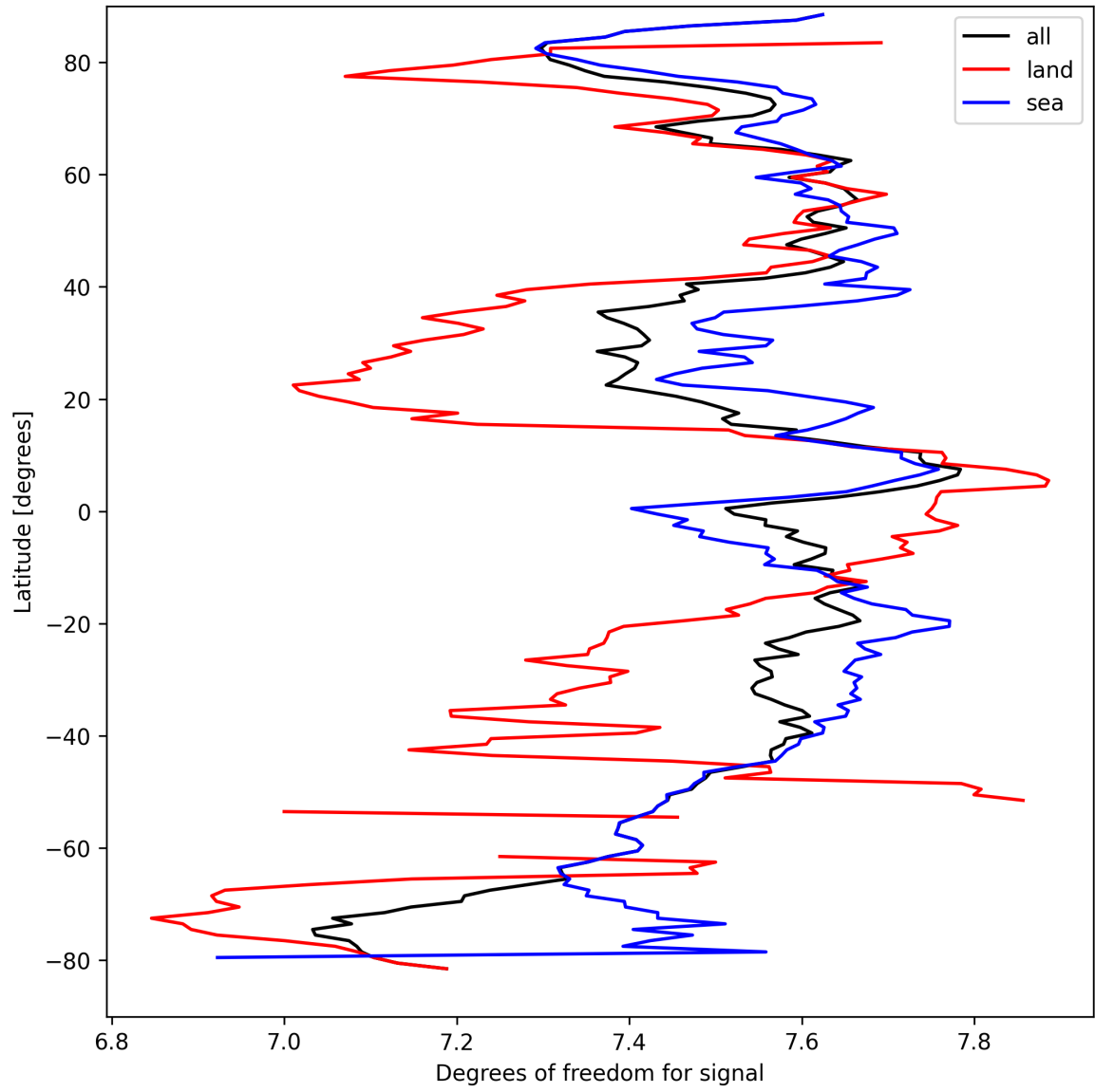
Figure 11: Zonal average of “Degrees of freedom for signal” for 2025-09-14 to 2025-09-15.
