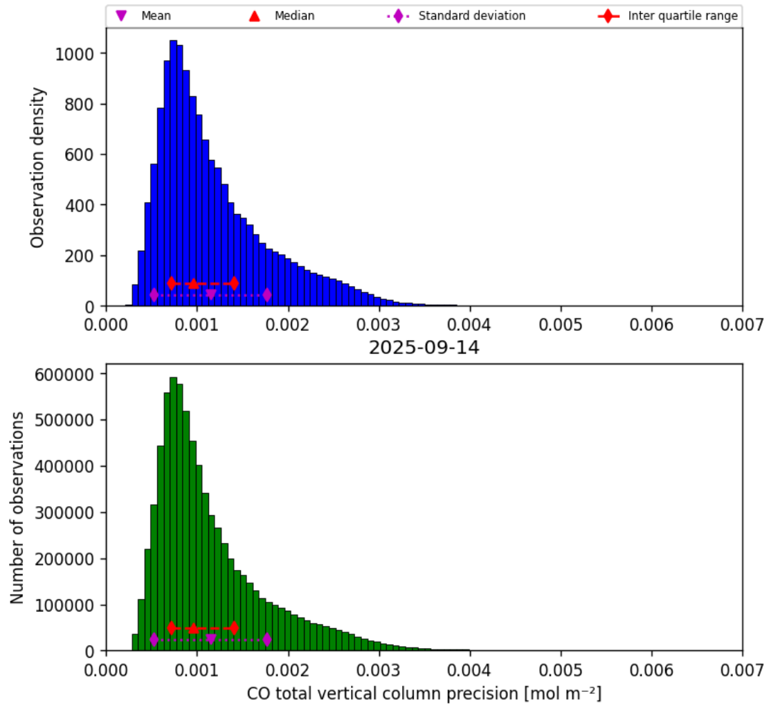
Figure 15: Histogram of “CO total vertical column precision” for 2025-09-14 to 2025-09-15
