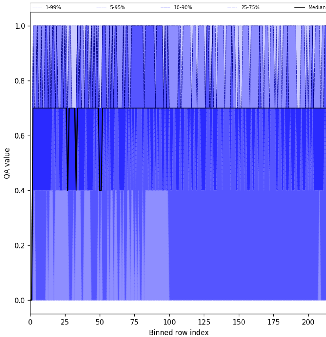
Figure 20: Along track statistics of “QA value” for 2025-09-14 to 2025-09-15
