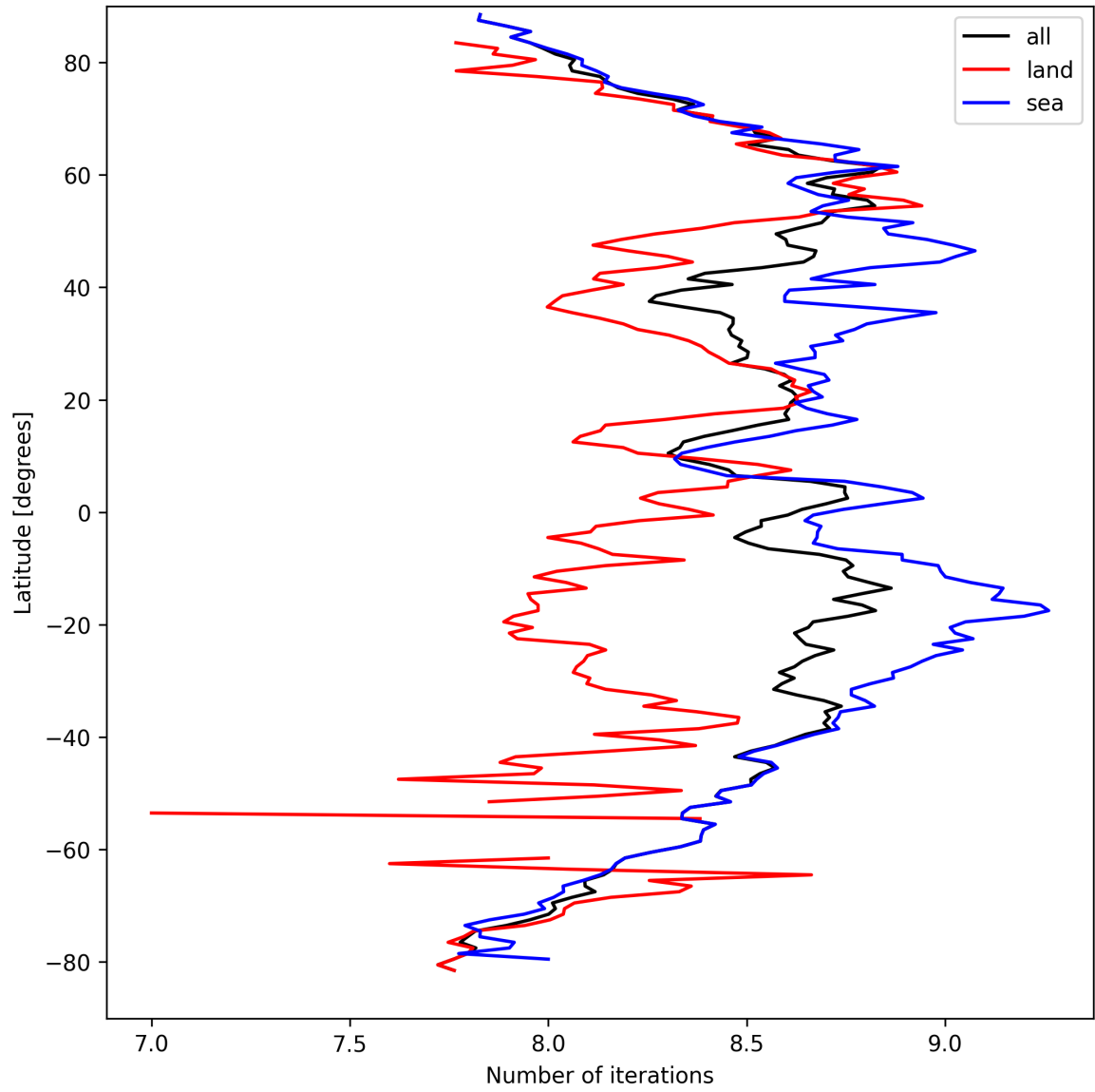
Figure 12: Zonal average of “Number of iterations” for 2025-09-14 to 2025-09-15.
