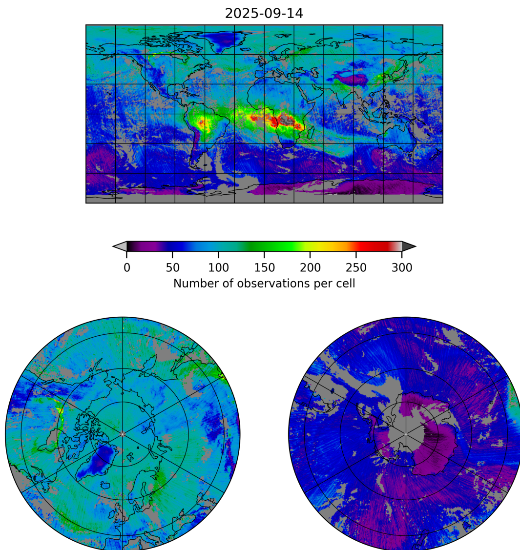
Figure 5: Map of the number of observations for 2025-09-14 to 2025-09-15
