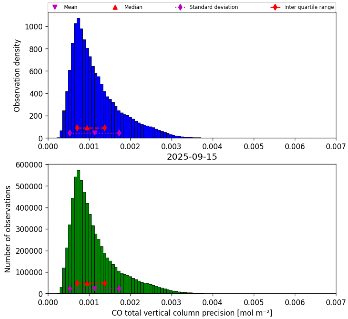
Figure 15: Histogram of “CO total vertical column precision” for 2025-09-15 to 2025-09-16
