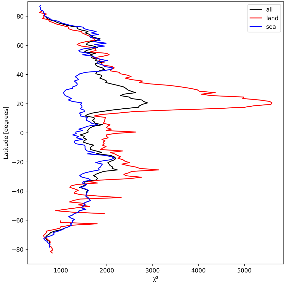
Figure 10: Zonal average of “ \chi^2 ” for 2025-09-15 to 2025-09-16.
