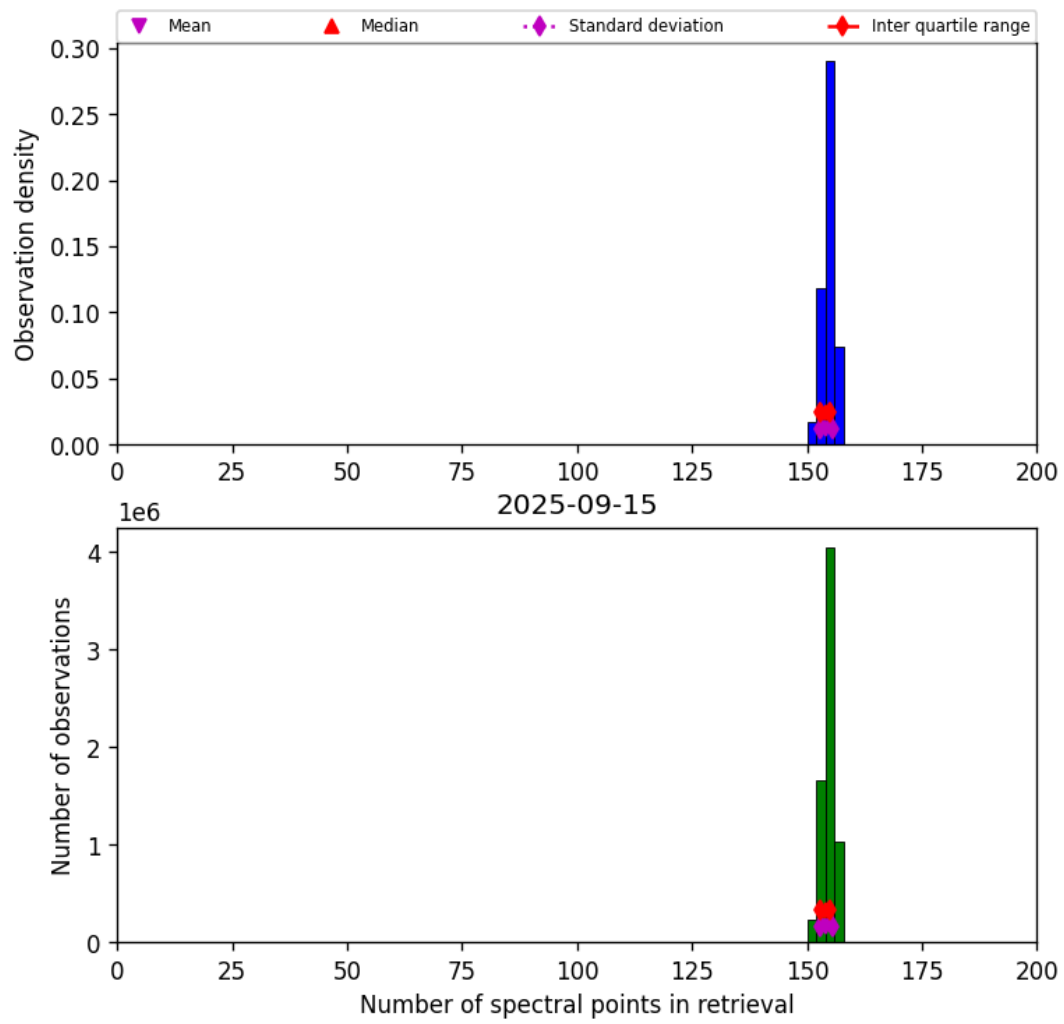
Figure 16: Histogram of “Number of spectral points in retrieval” for 2025-09-15 to 2025-09-16
