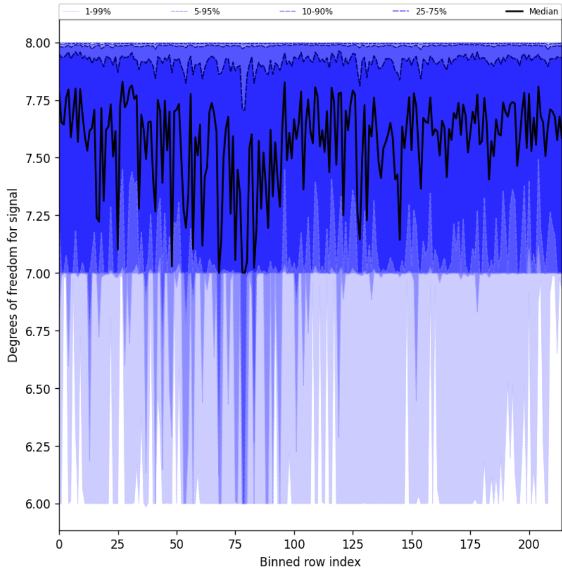
Figure 25: Along track statistics of “Degrees of freedom for signal” for 2025-09-15 to 2025-09-16
