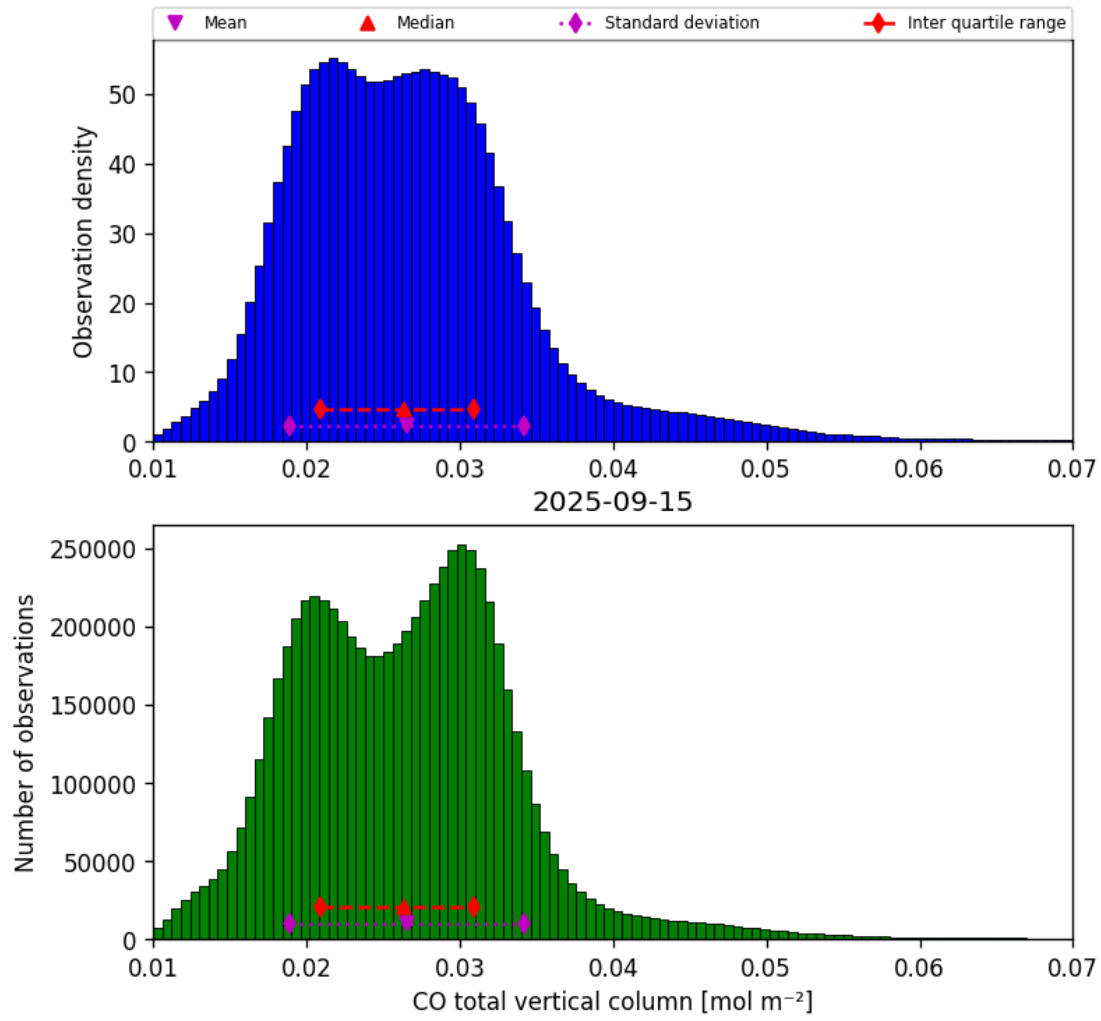
Figure 14: Histogram of “CO total vertical column” for 2025-09-15 to 2025-09-16
