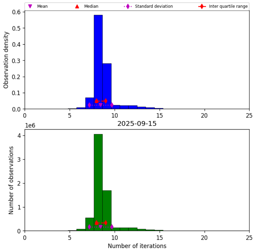
Figure 19: Histogram of “Number of iterations” for 2025-09-15 to 2025-09-16
