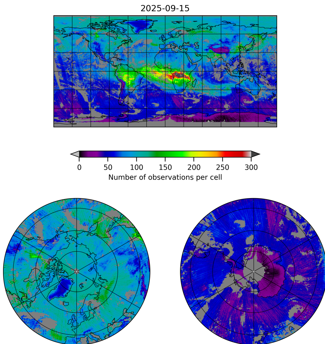
Figure 5: Map of the number of observations for 2025-09-15 to 2025-09-16
