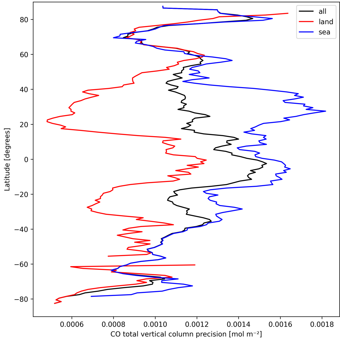
Figure 8: Zonal average of "CO total vertical column precision" for 2025-09-15 to 2025-09-16.
