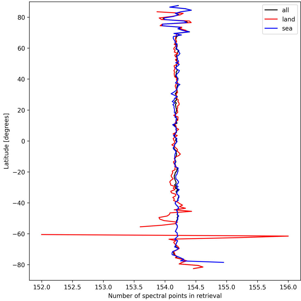
Figure 9: Zonal average of “Number of spectral points in retrieval” for 2025-09-15 to 2025-09-16.
