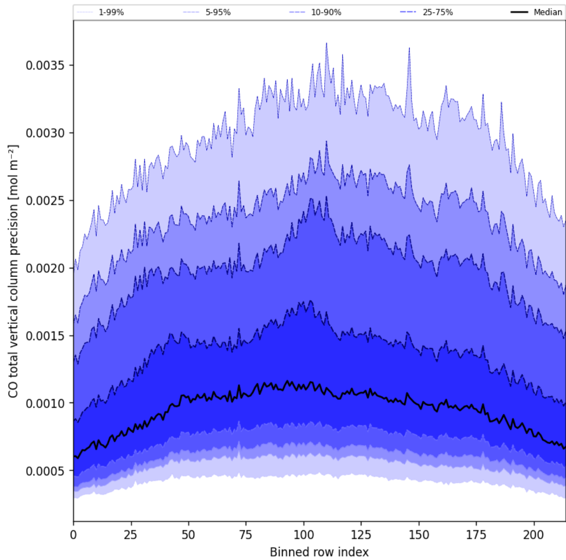
Figure 22: Along track statistics of “CO total vertical column precision” for 2025-09-15 to 2025-09-16
