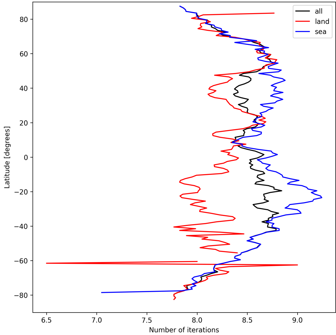
Figure 12: Zonal average of “Number of iterations” for 2025-09-15 to 2025-09-16.
