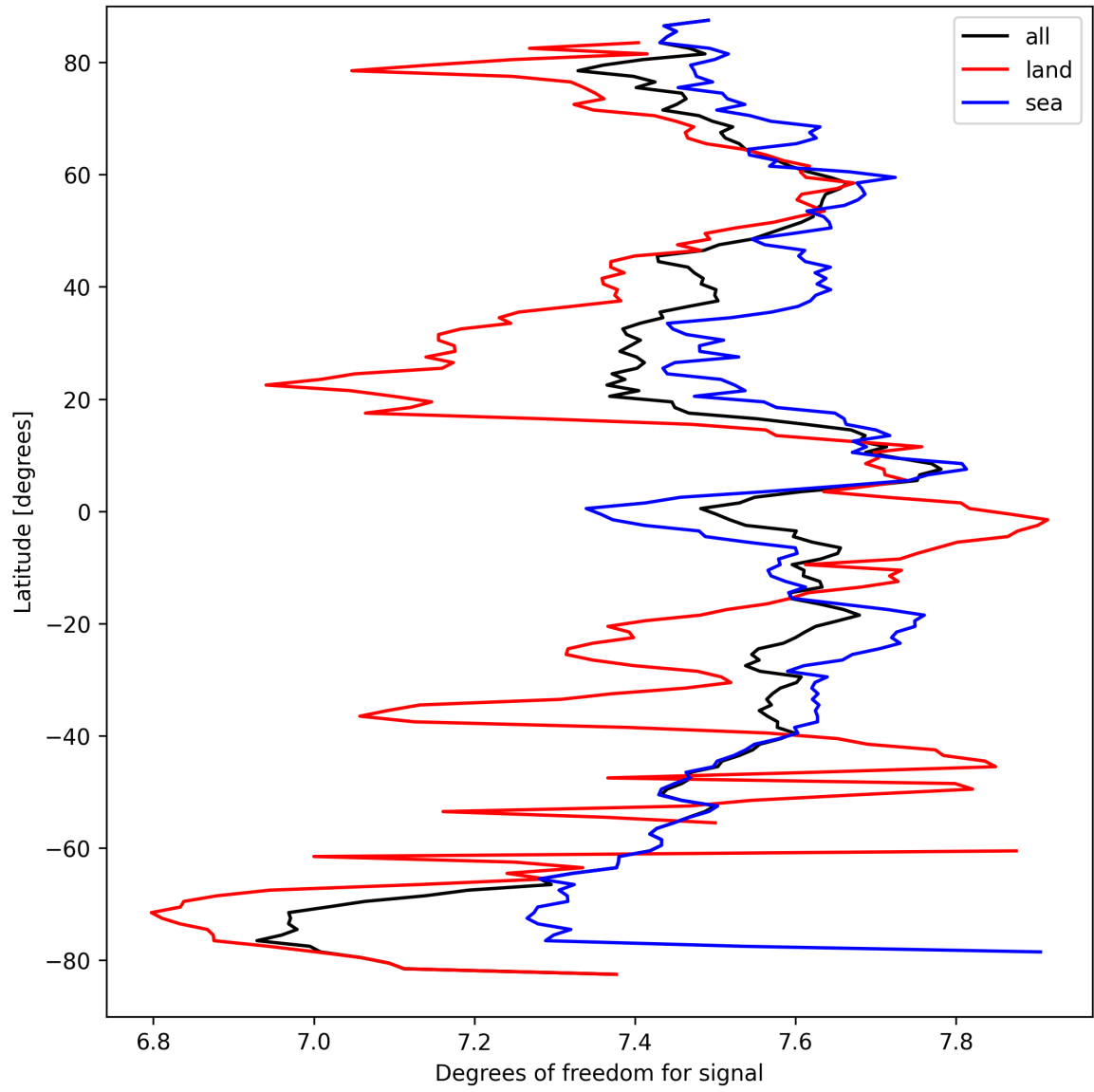
Figure 11: Zonal average of “Degrees of freedom for signal” for 2025-09-15 to 2025-09-16.
