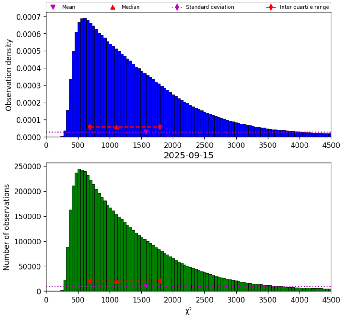
Figure 17: Histogram of " \chi^2 " for 2025-09-15 to 2025-09-16
