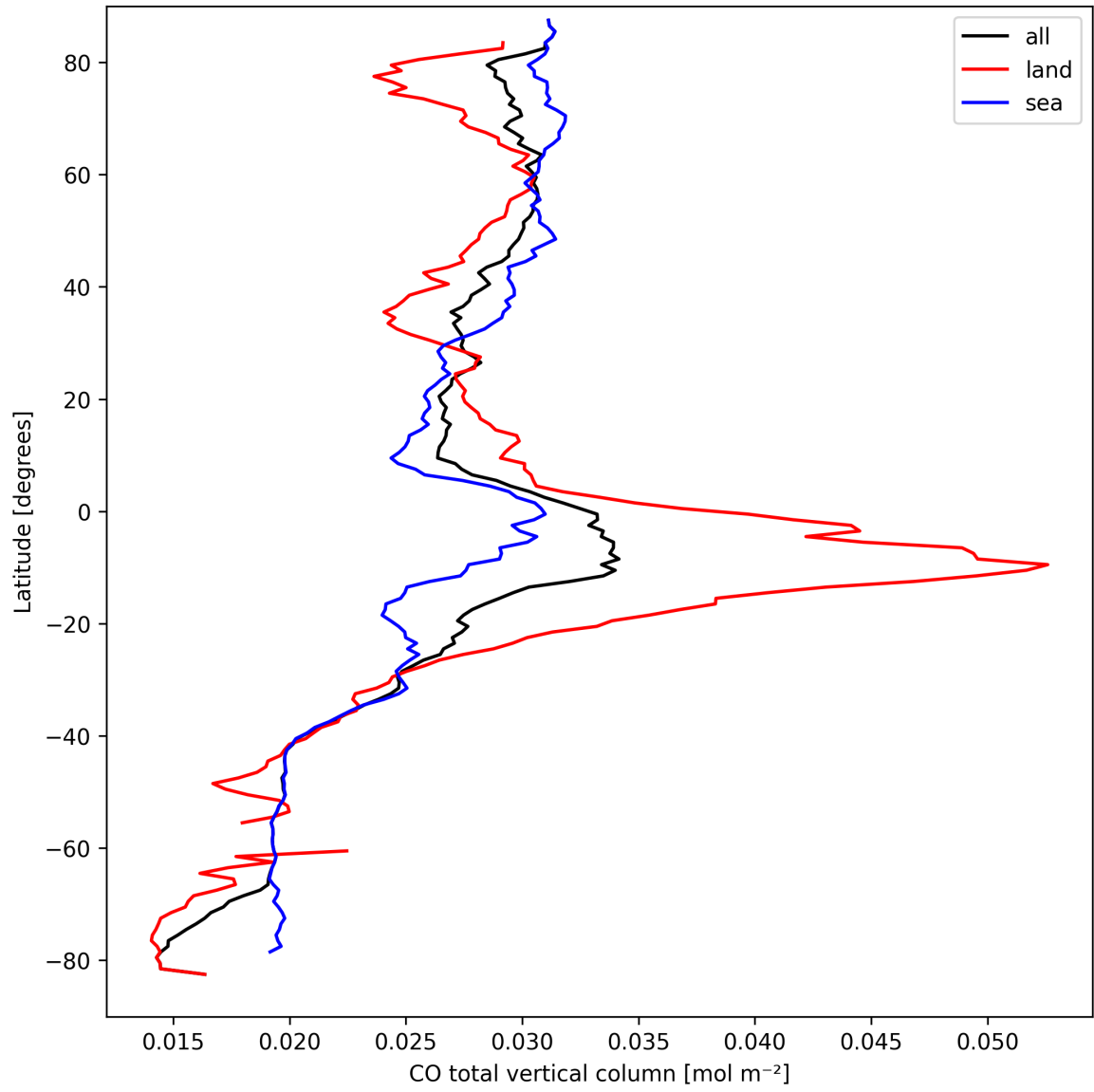
Figure 7: Zonal average of “CO total vertical column” for 2025-09-15 to 2025-09-16.
