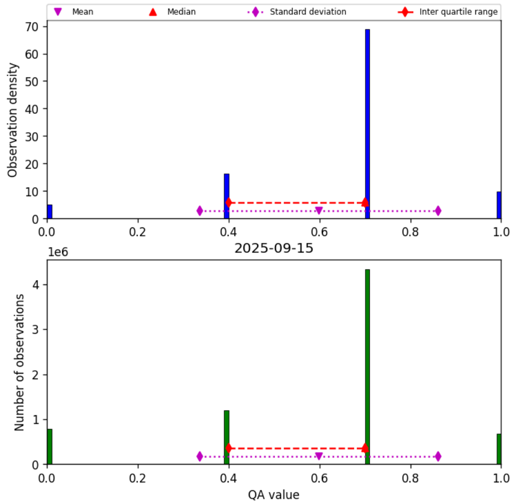
Figure 13: Histogram of “QA value” for 2025-09-15 to 2025-09-16
