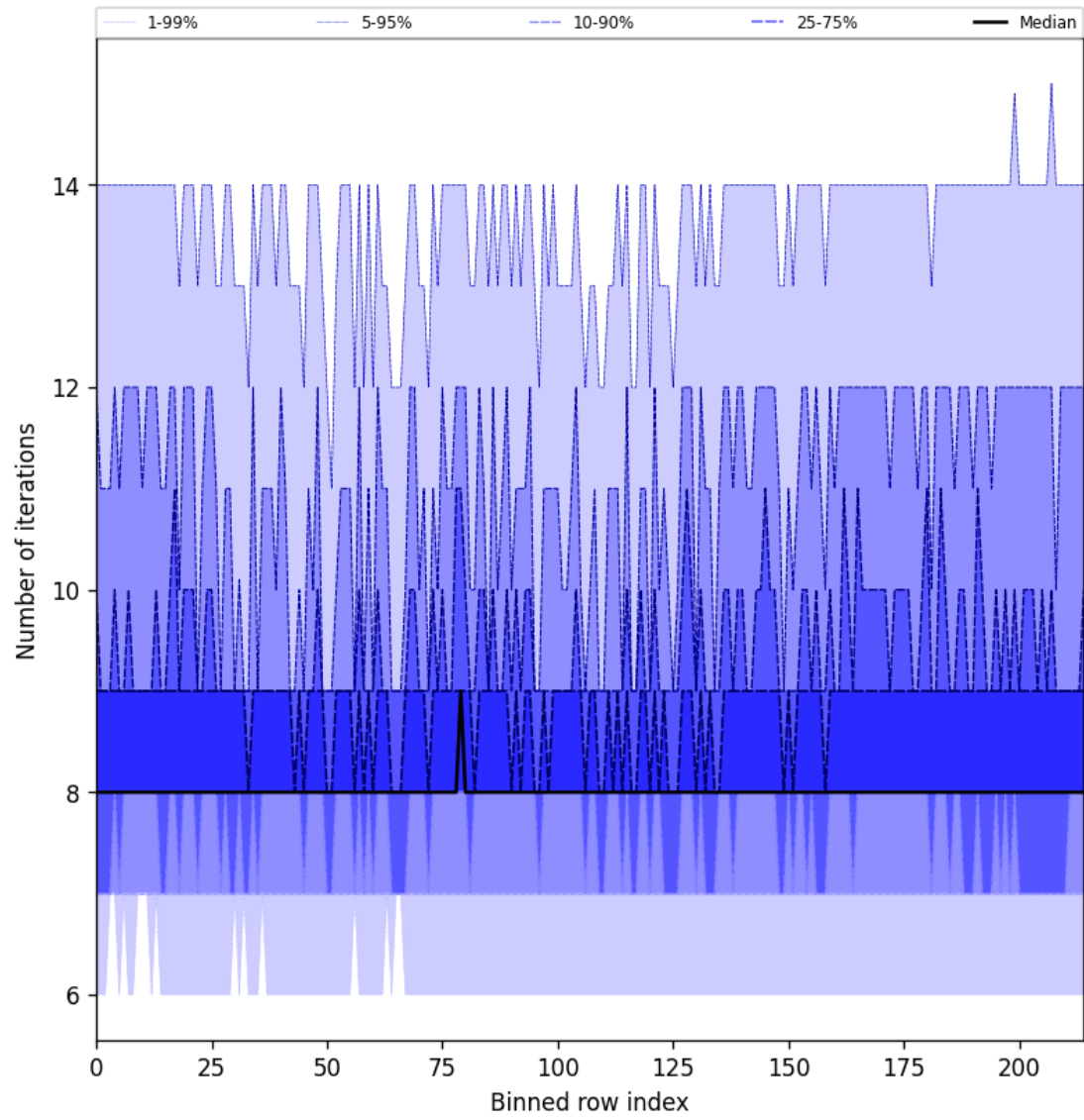
Figure 26: Along track statistics of “Number of iterations” for 2025-09-15 to 2025-09-16
