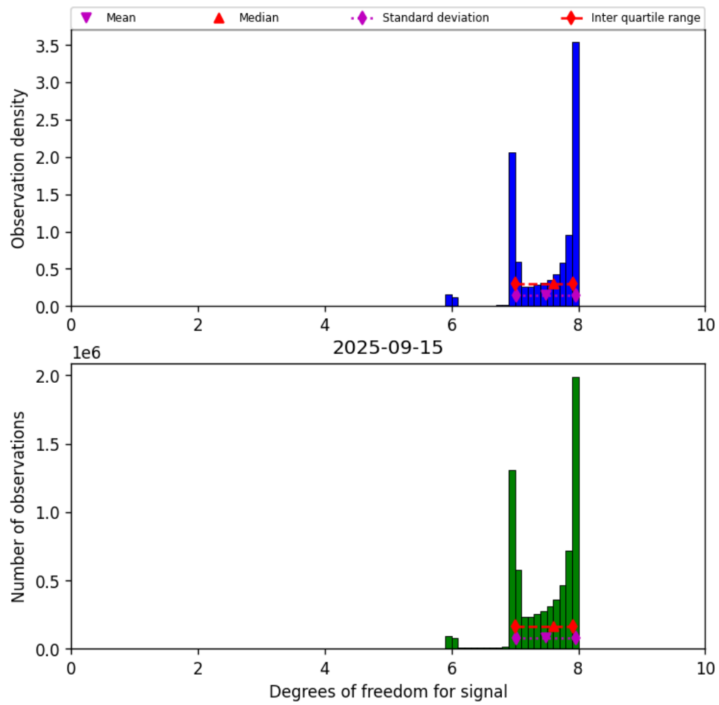
Figure 18: Histogram of “Degrees of freedom for signal” for 2025-09-15 to 2025-09-16
