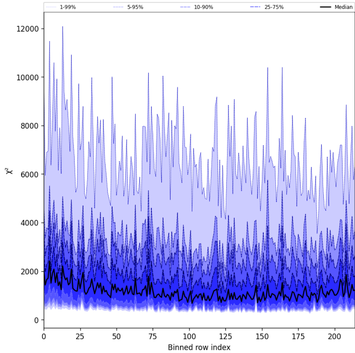
Figure 24: Along track statistics of “ \chi^2 ” for 2025-09-15 to 2025-09-16
