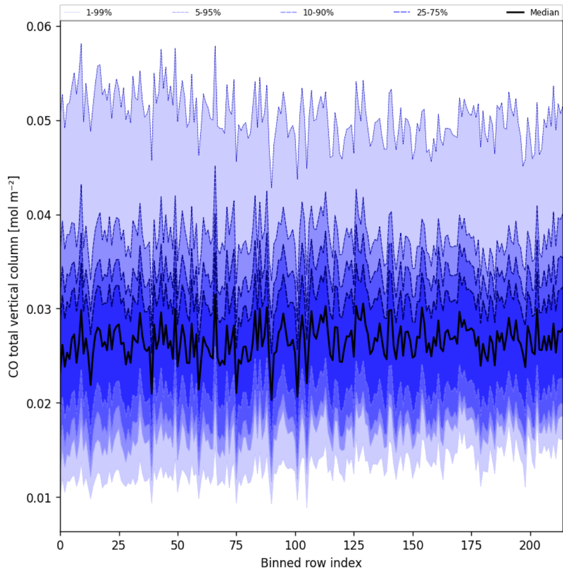
Figure 21: Along track statistics of “CO total vertical column” for 2025-09-15 to 2025-09-16
