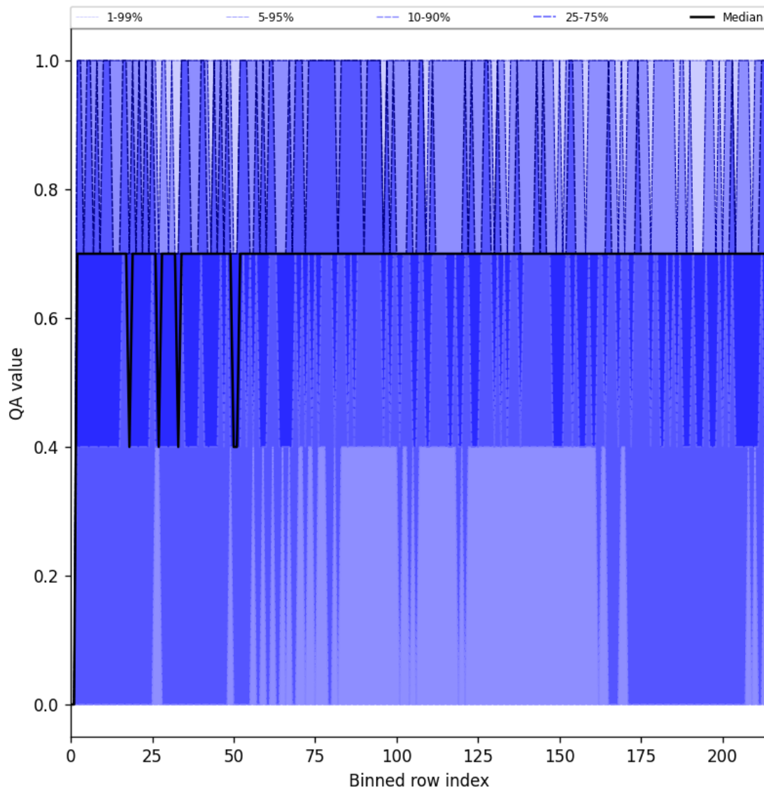
Figure 20: Along track statistics of “QA value” for 2025-09-15 to 2025-09-16
