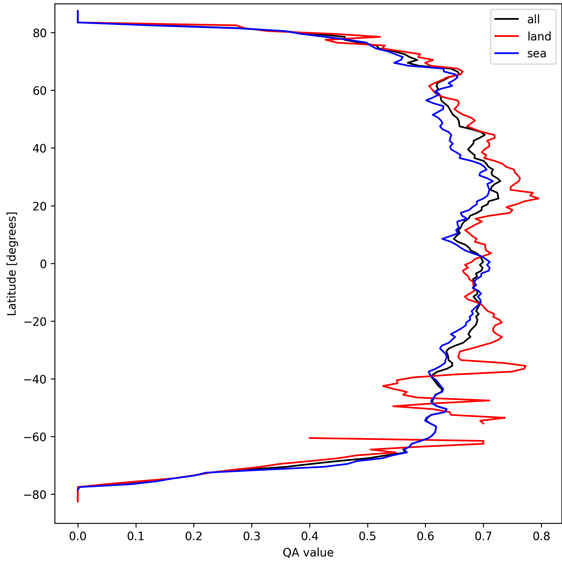
Figure 6: Zonal average of “QA value” for 2025-09-15 to 2025-09-16.
