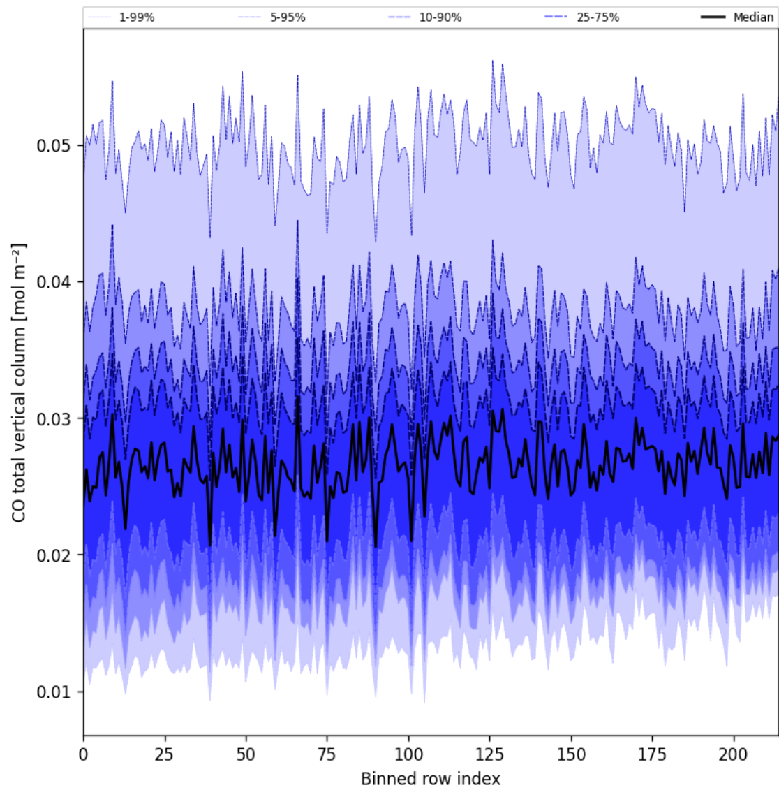
Figure 21: Along track statistics of “CO total vertical column” for 2025-09-16 to 2025-09-17
