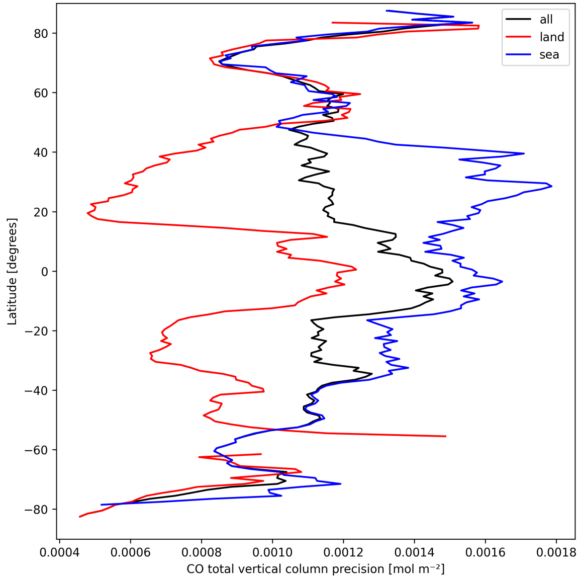
Figure 8: Zonal average of “CO total vertical column precision” for 2025-09-16 to 2025-09-17.
