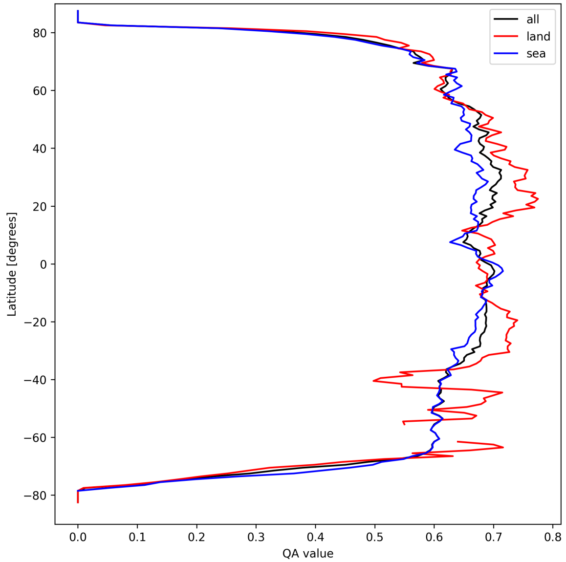
Figure 6: Zonal average of “QA value” for 2025-09-16 to 2025-09-17.
