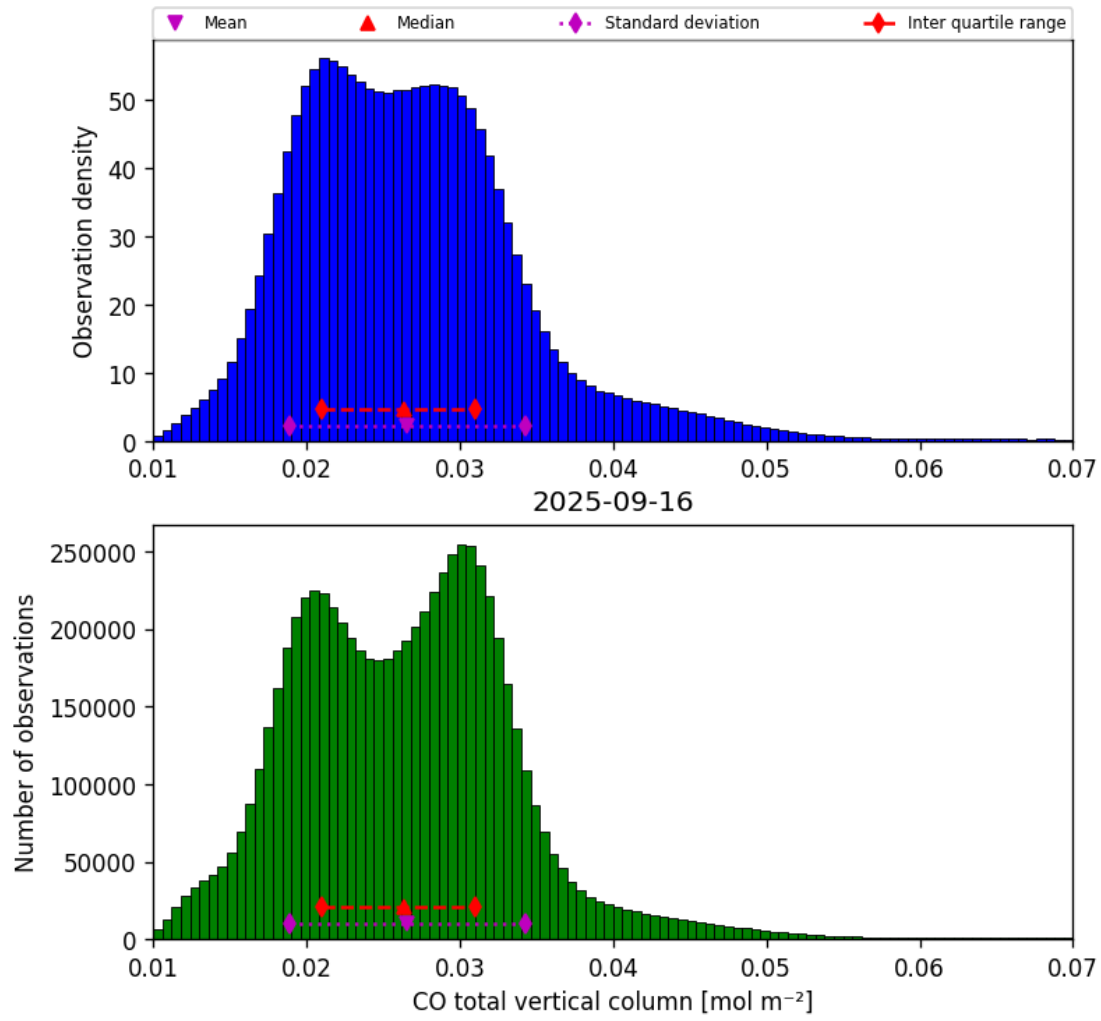
Figure 14: Histogram of “CO total vertical column” for 2025-09-16 to 2025-09-17
