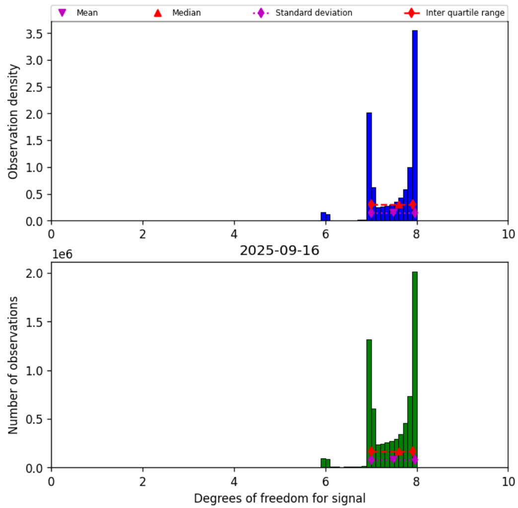
Figure 18: Histogram of “Degrees of freedom for signal” for 2025-09-16 to 2025-09-17
