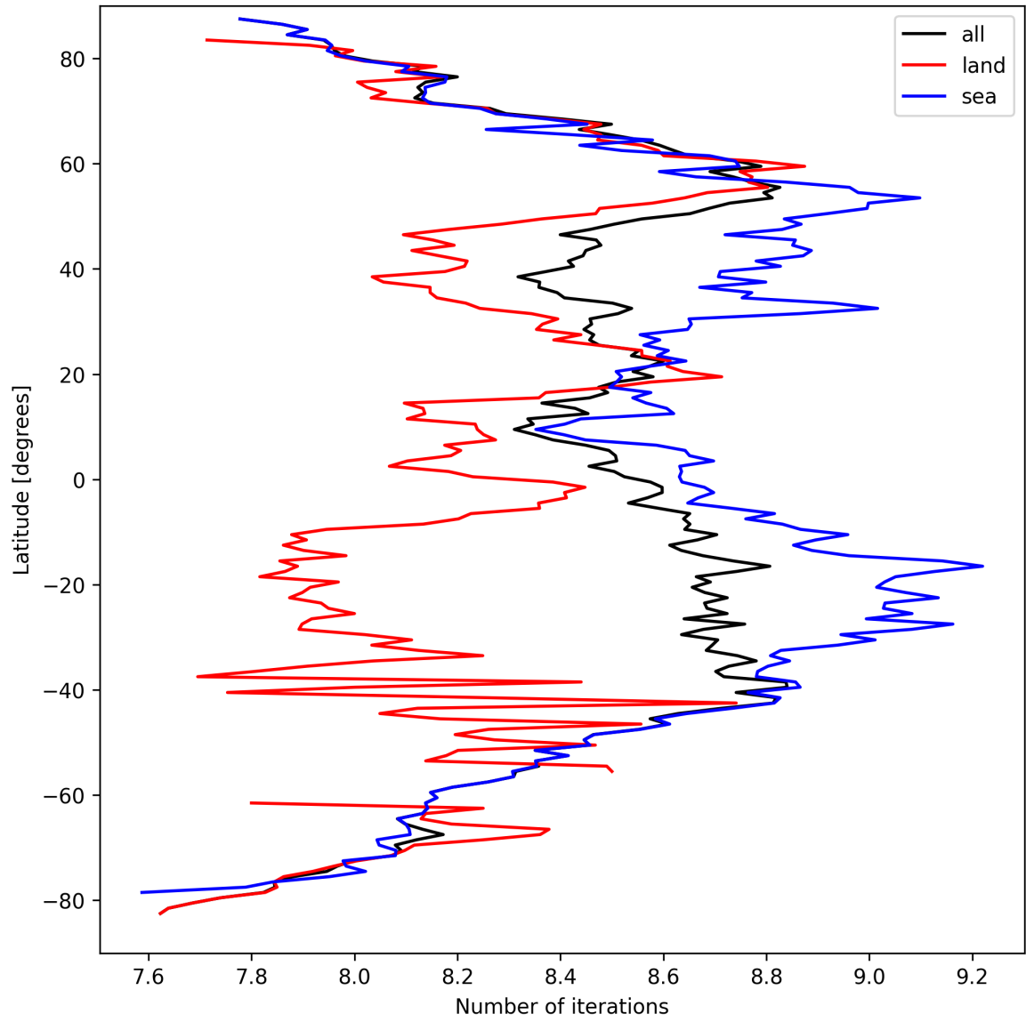
Figure 12: Zonal average of “Number of iterations” for 2025-09-16 to 2025-09-17.
