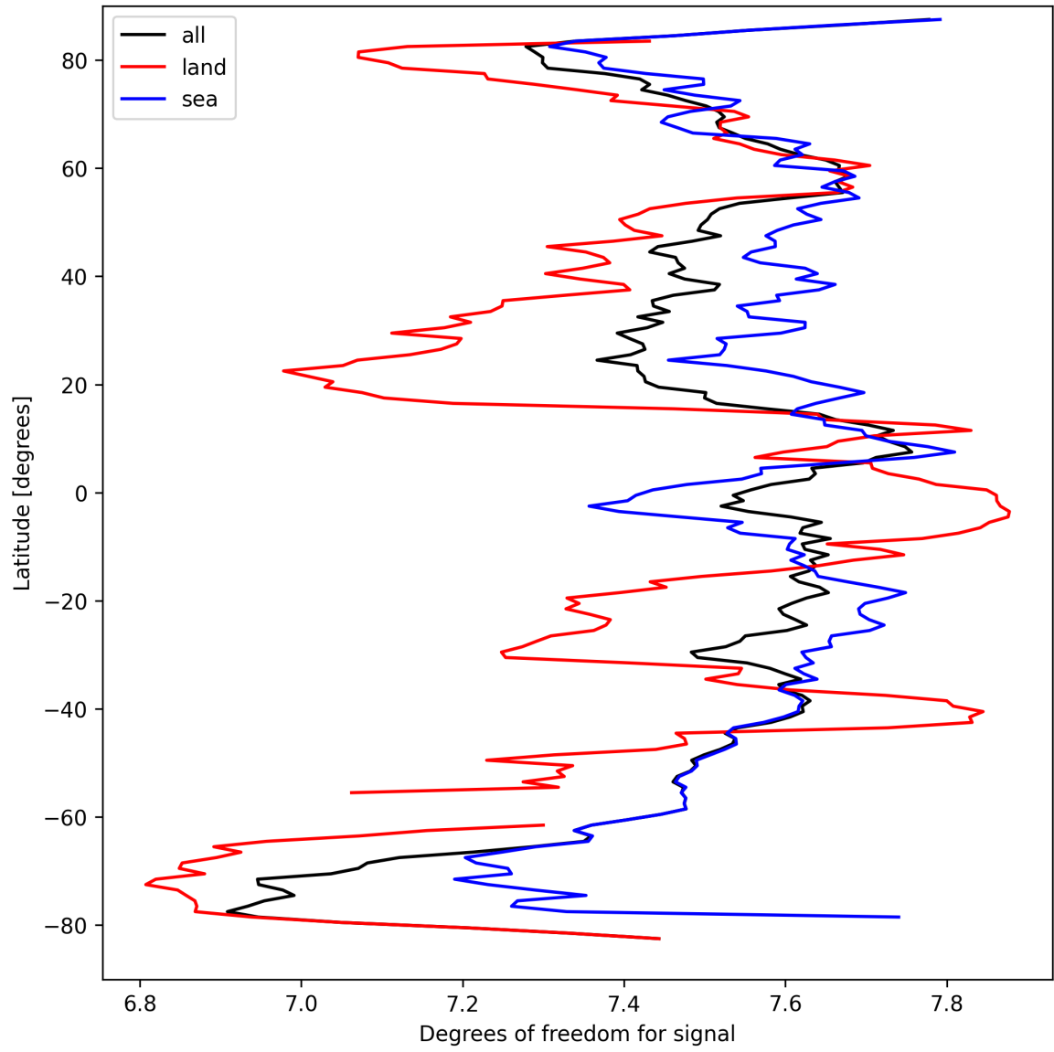
Figure 11: Zonal average of “Degrees of freedom for signal” for 2025-09-16 to 2025-09-17.
