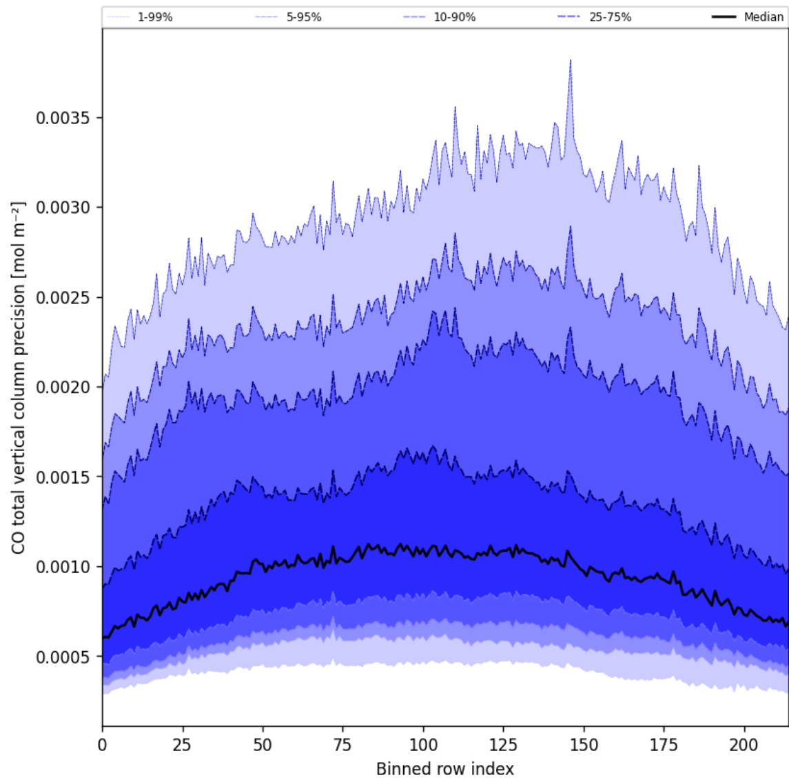
Figure 22: Along track statistics of “CO total vertical column precision” for 2025-09-16 to 2025-09-17
