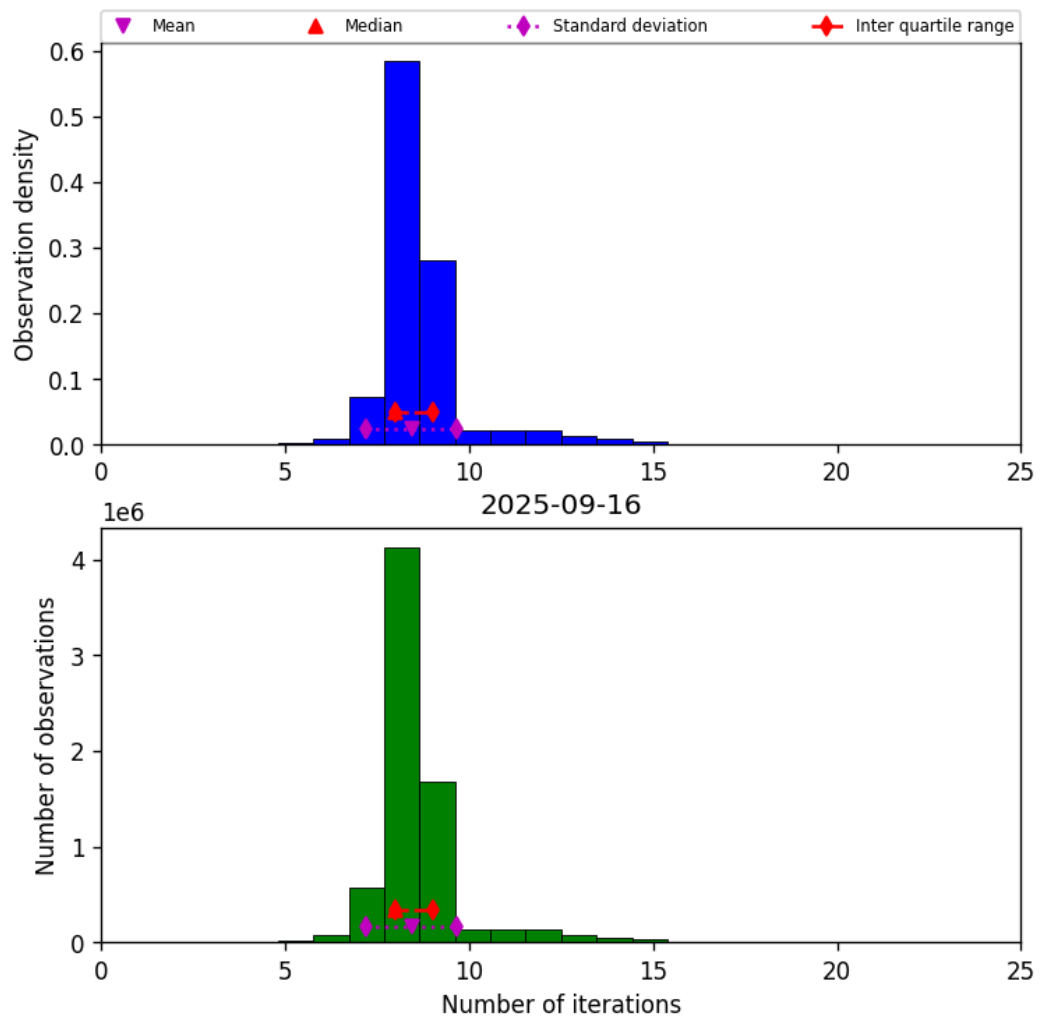
Figure 19: Histogram of “Number of iterations” for 2025-09-16 to 2025-09-17
