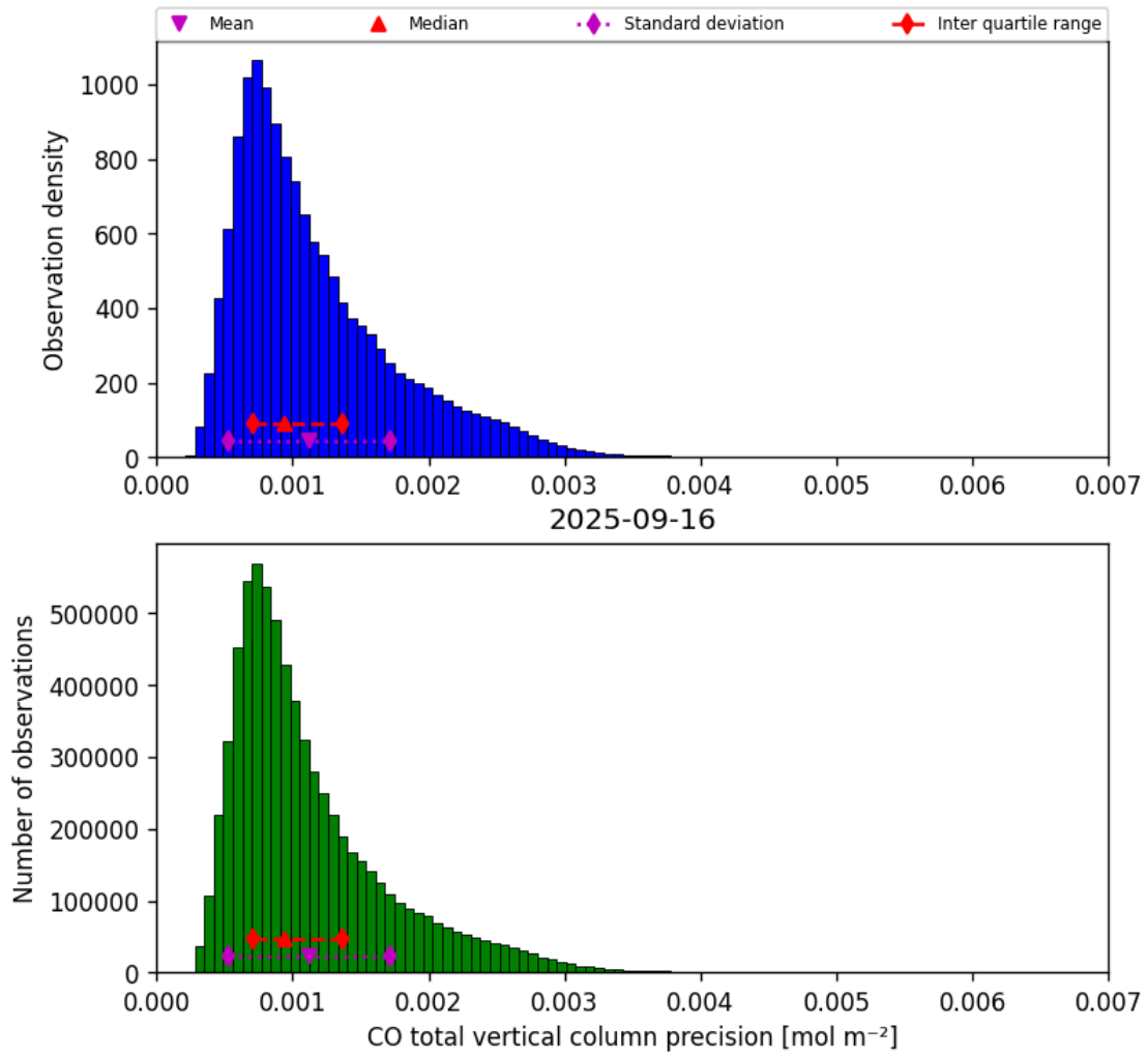
Figure 15: Histogram of “CO total vertical column precision” for 2025-09-16 to 2025-09-17
