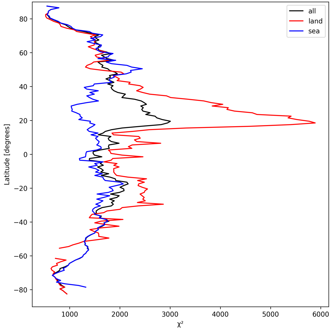
Figure 10: Zonal average of “ \chi^2 ” for 2025-09-16 to 2025-09-17.
