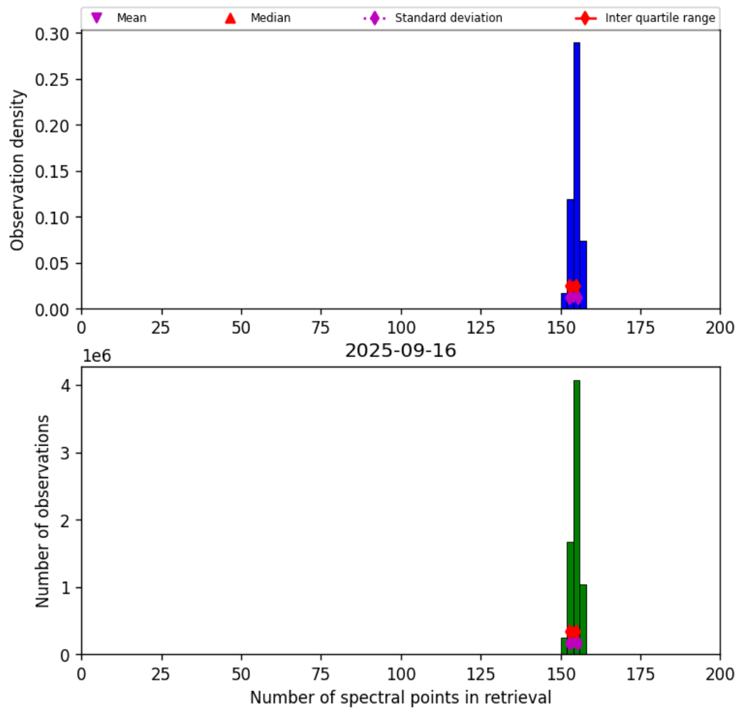
Figure 16: Histogram of “Number of spectral points in retrieval” for 2025-09-16 to 2025-09-17
