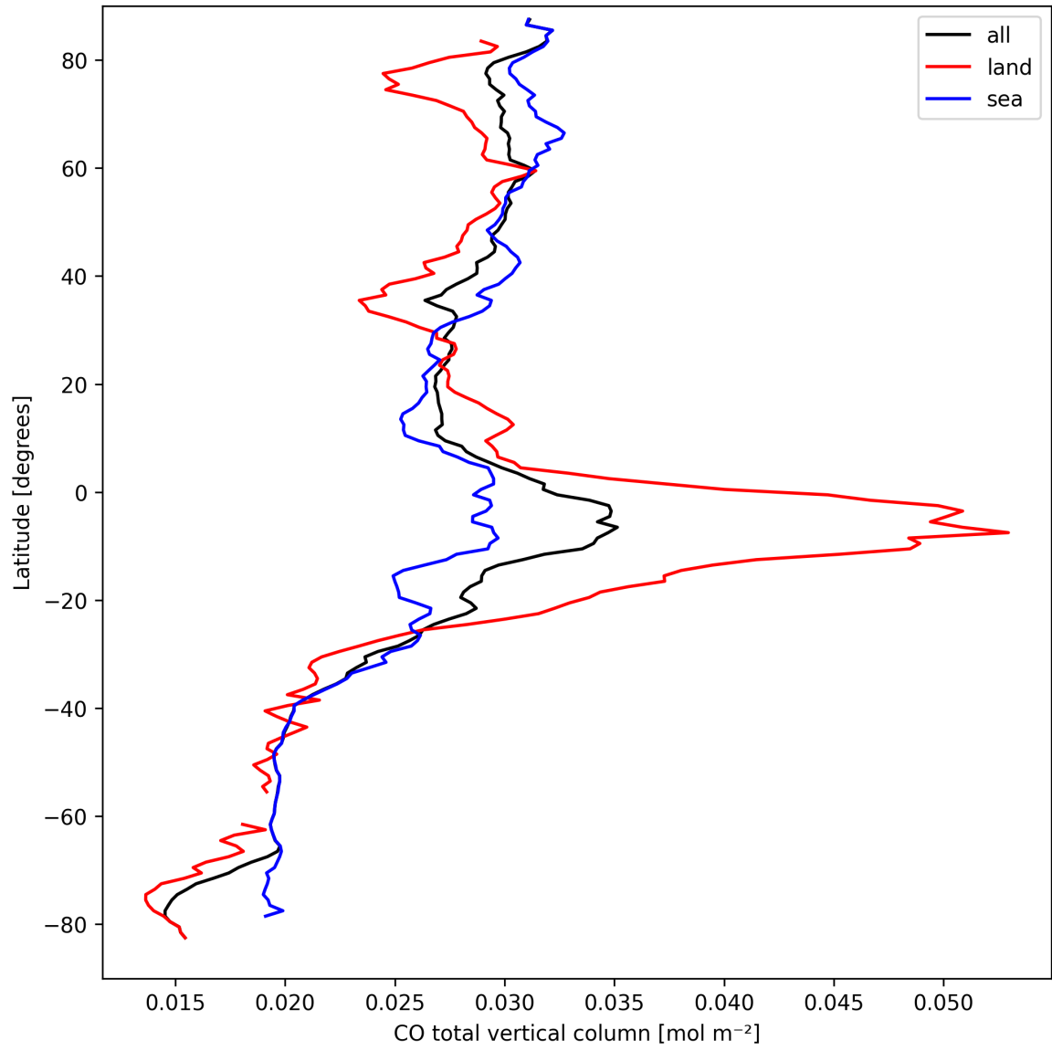
Figure 7: Zonal average of “CO total vertical column” for 2025-09-16 to 2025-09-17.
