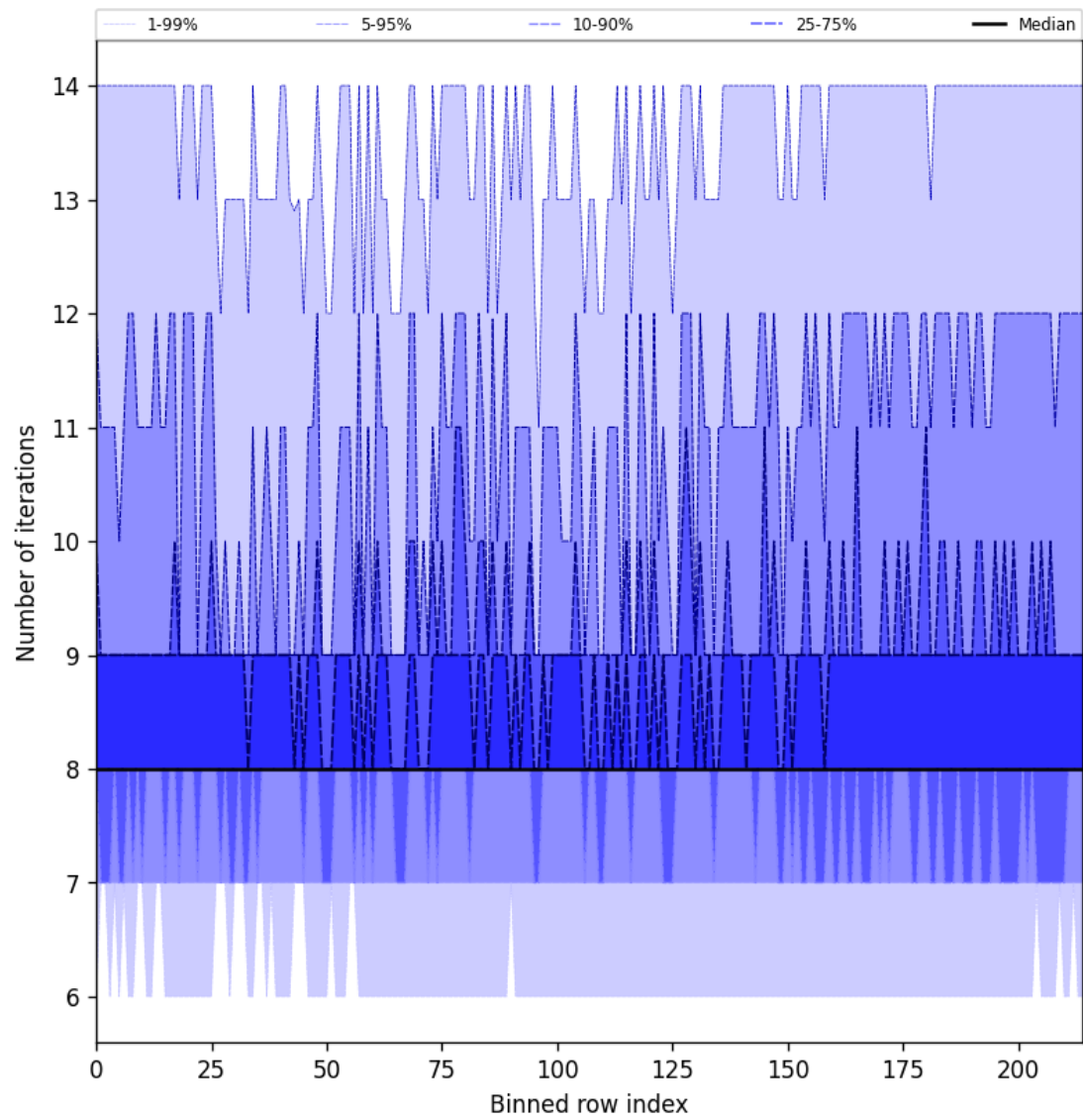
Figure 26: Along track statistics of “Number of iterations” for 2025-09-16 to 2025-09-17
