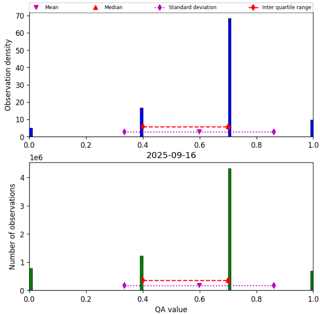
Figure 13: Histogram of “QA value” for 2025-09-16 to 2025-09-17
