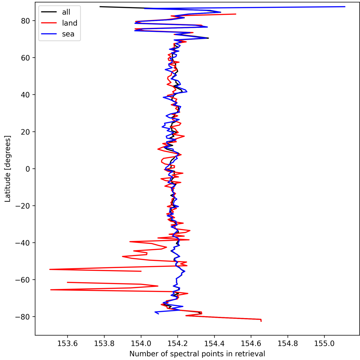
Figure 9: Zonal average of “Number of spectral points in retrieval” for 2025-09-16 to 2025-09-17.
