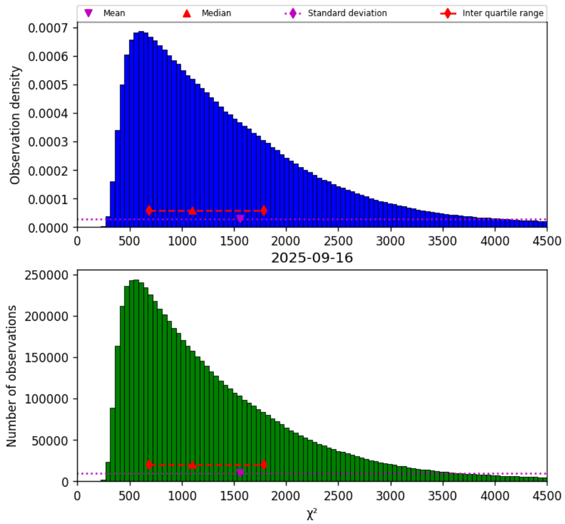
Figure 17: Histogram of “ \chi^2 ” for 2025-09-16 to 2025-09-17
