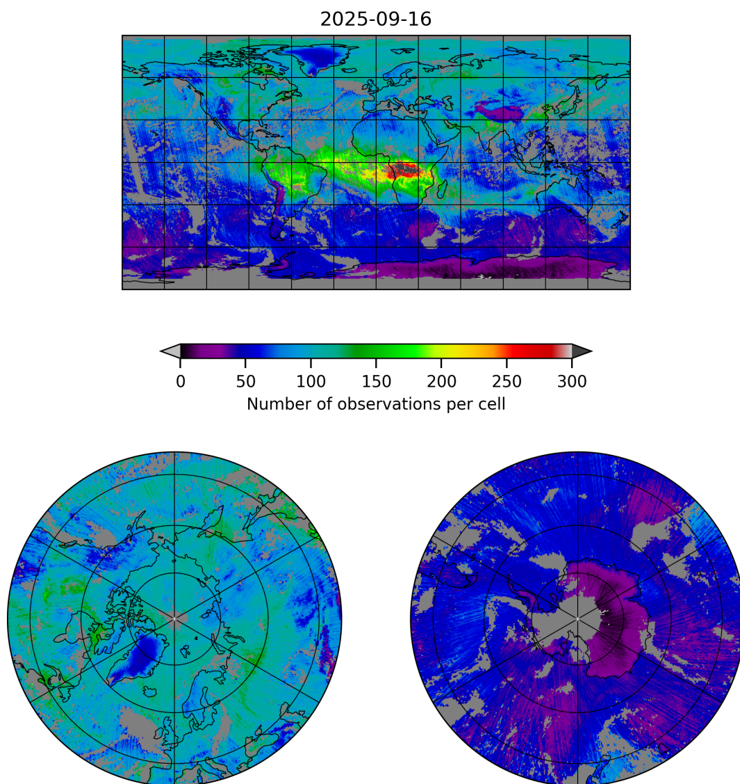
Figure 5: Map of the number of observations for 2025-09-16 to 2025-09-17
