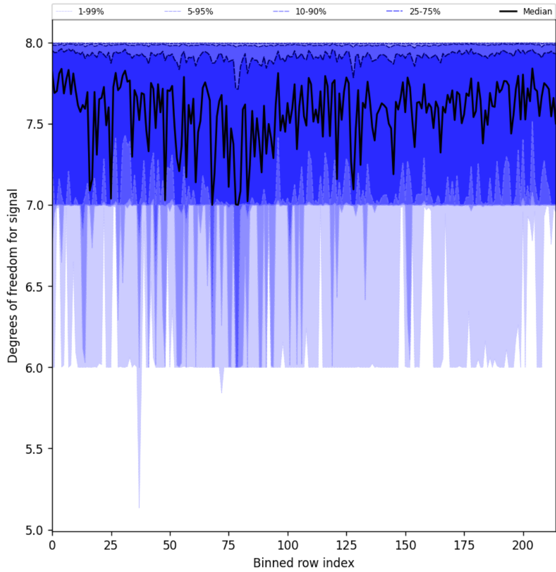
Figure 25: Along track statistics of “Degrees of freedom for signal” for 2025-09-16 to 2025-09-17
