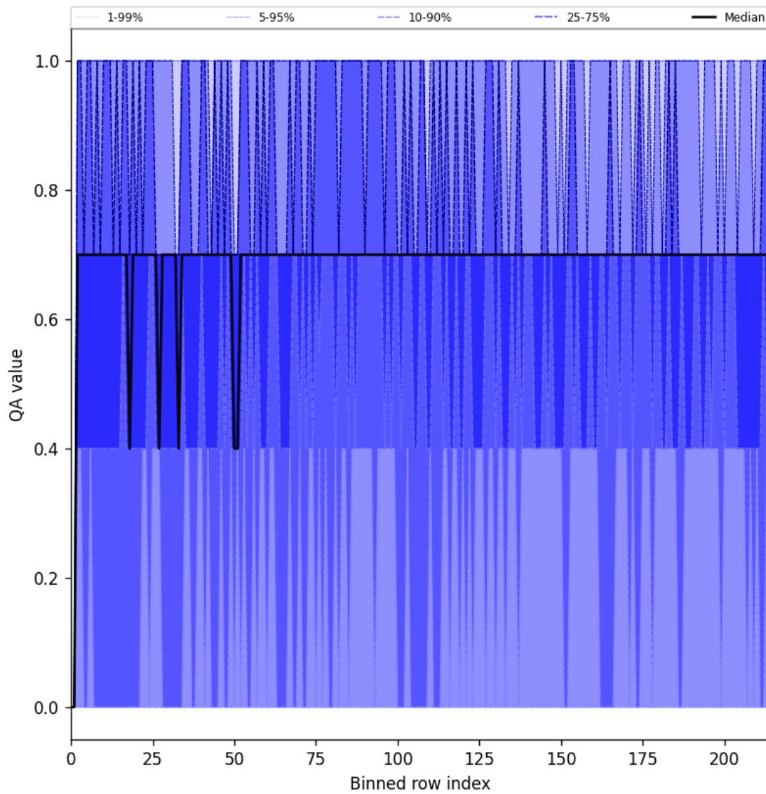
Figure 20: Along track statistics of “QA value” for 2025-09-16 to 2025-09-17
