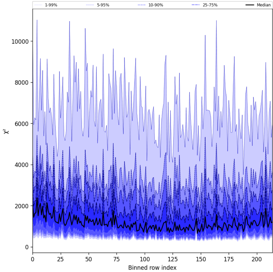
Figure 24: Along track statistics of “ \chi^2 ” for 2025-09-16 to 2025-09-17
