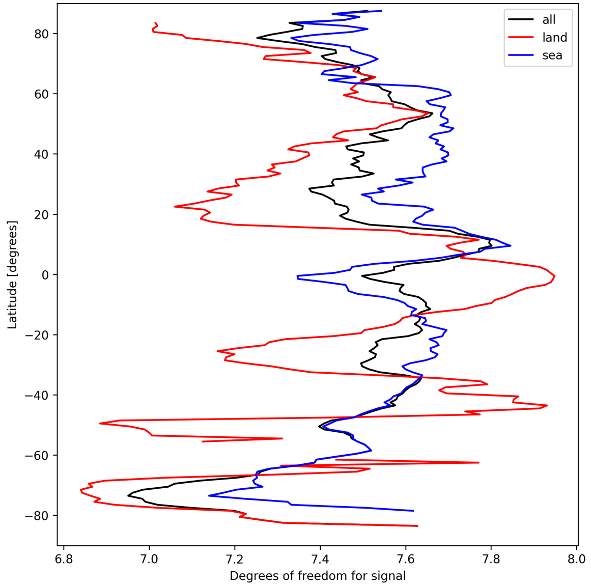
Figure 11: Zonal average of “Degrees of freedom for signal” for 2025-09-17 to 2025-09-18.
