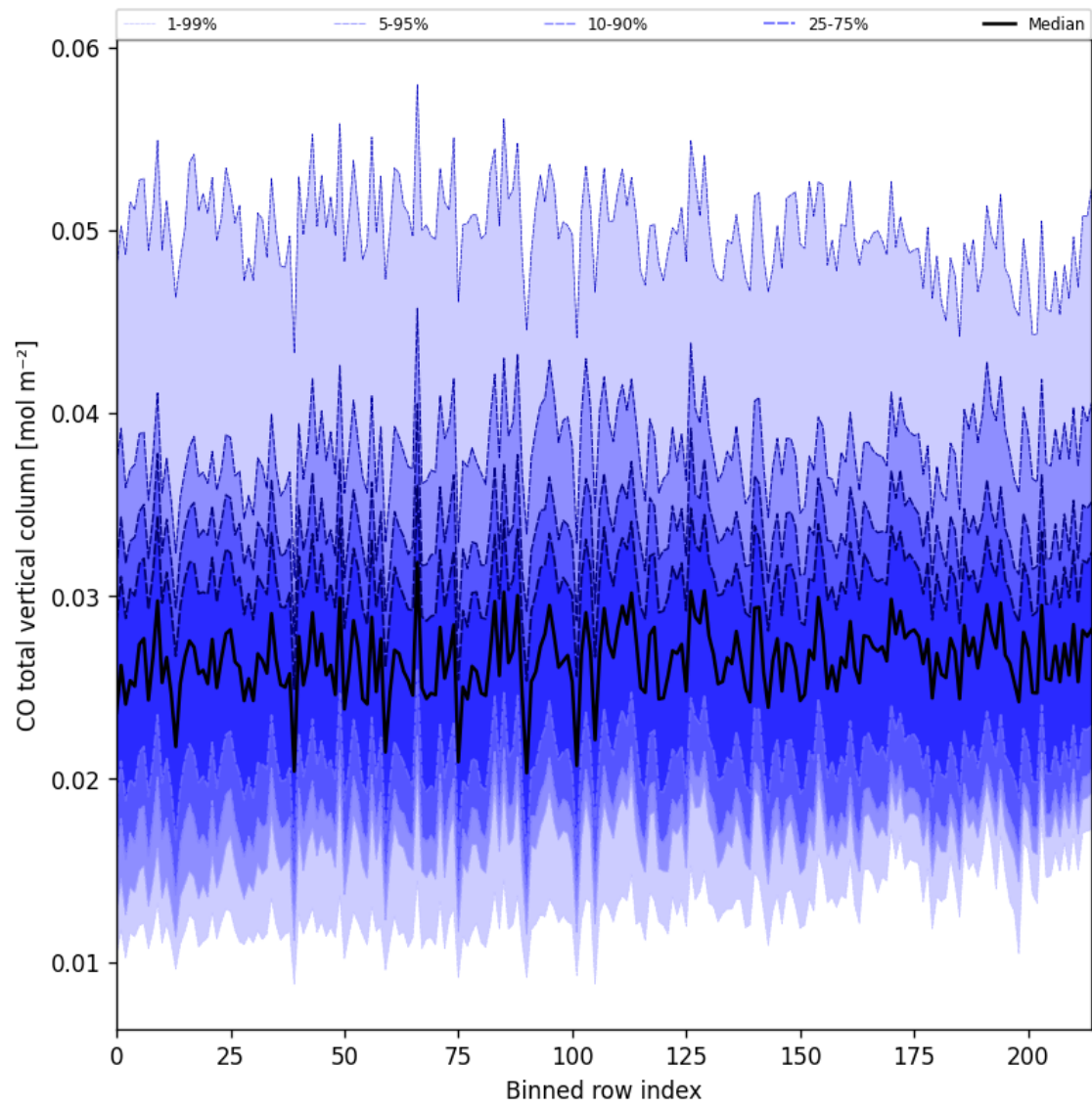
Figure 21: Along track statistics of “CO total vertical column” for 2025-09-17 to 2025-09-18
