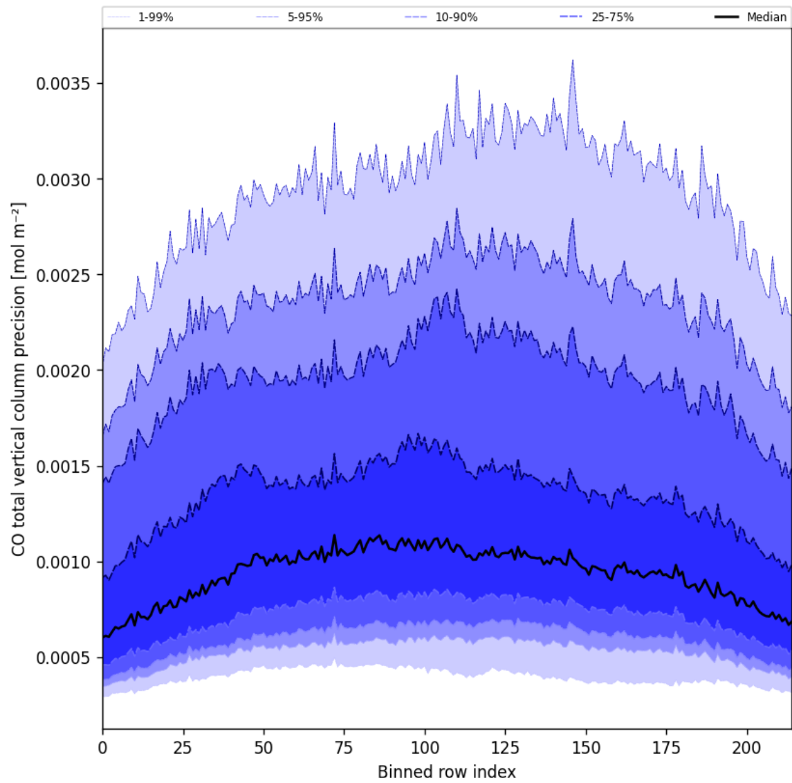
Figure 22: Along track statistics of “CO total vertical column precision” for 2025-09-17 to 2025-09-18
