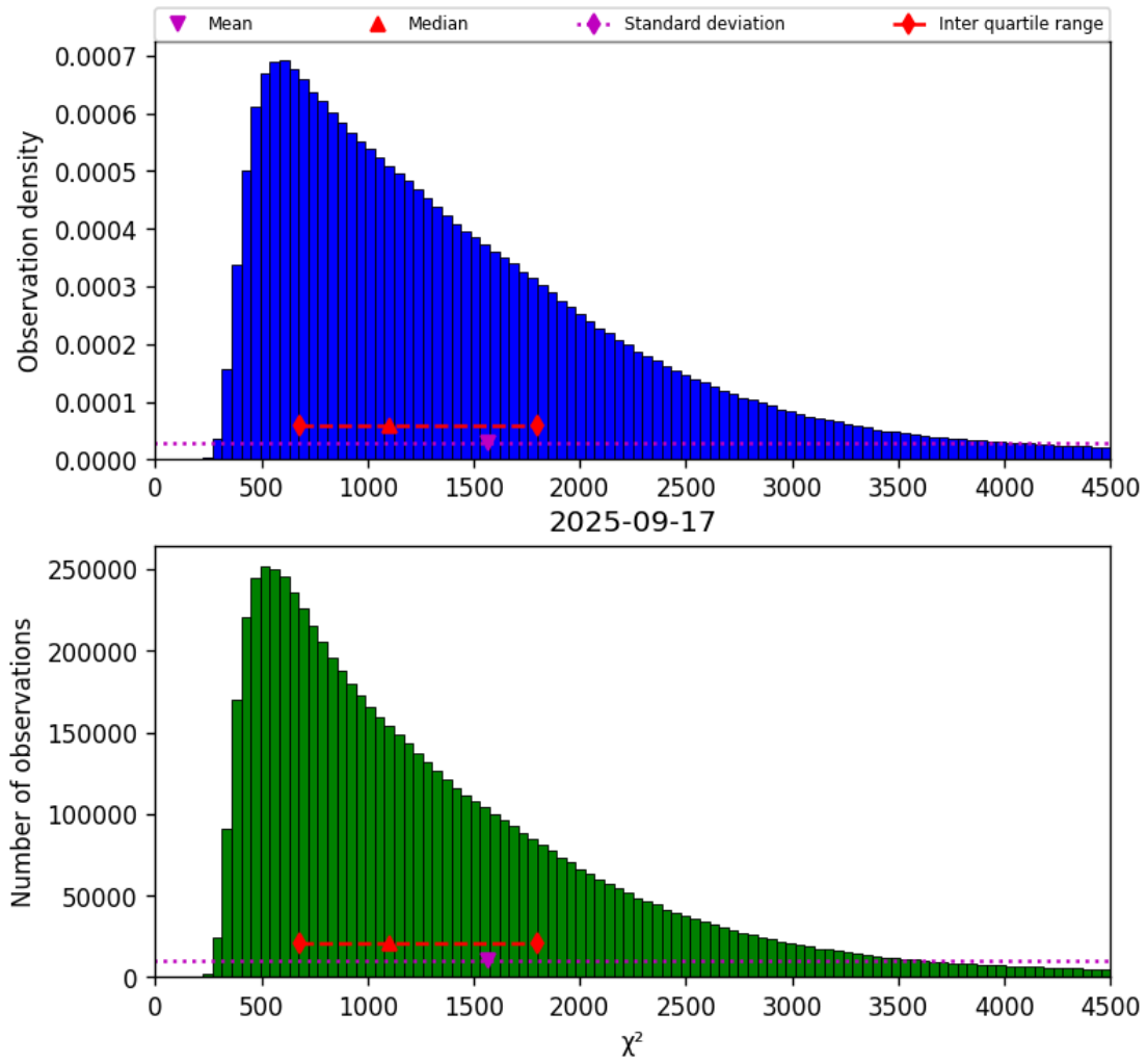
Figure 17: Histogram of " \chi^2 " for 2025-09-17 to 2025-09-18
