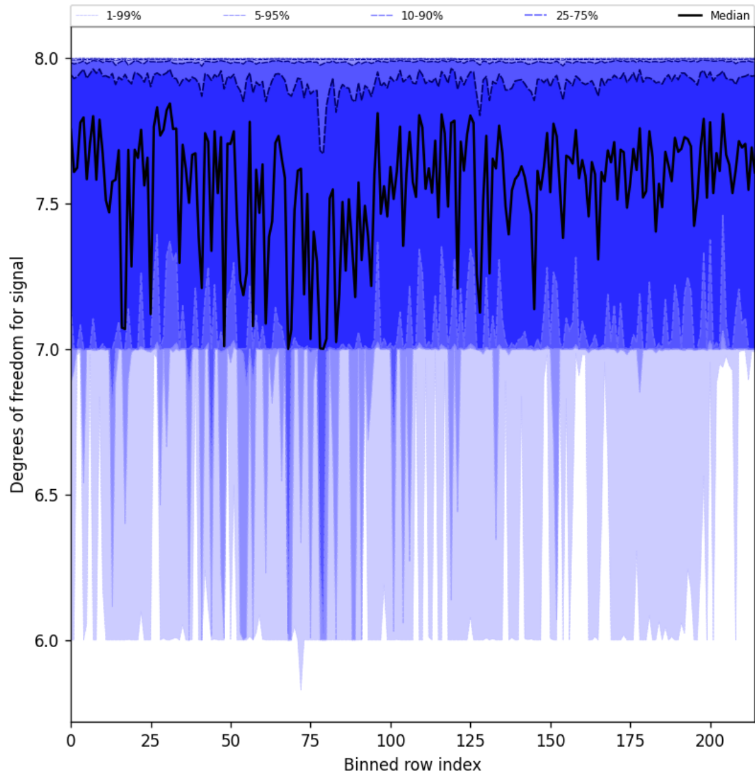
Figure 25: Along track statistics of “Degrees of freedom for signal” for 2025-09-17 to 2025-09-18
