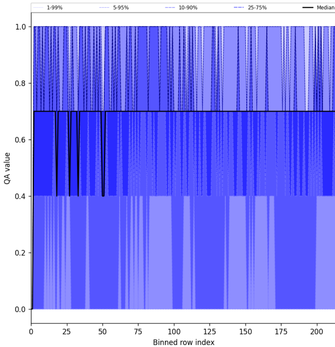
Figure 20: Along track statistics of “QA value” for 2025-09-17 to 2025-09-18
