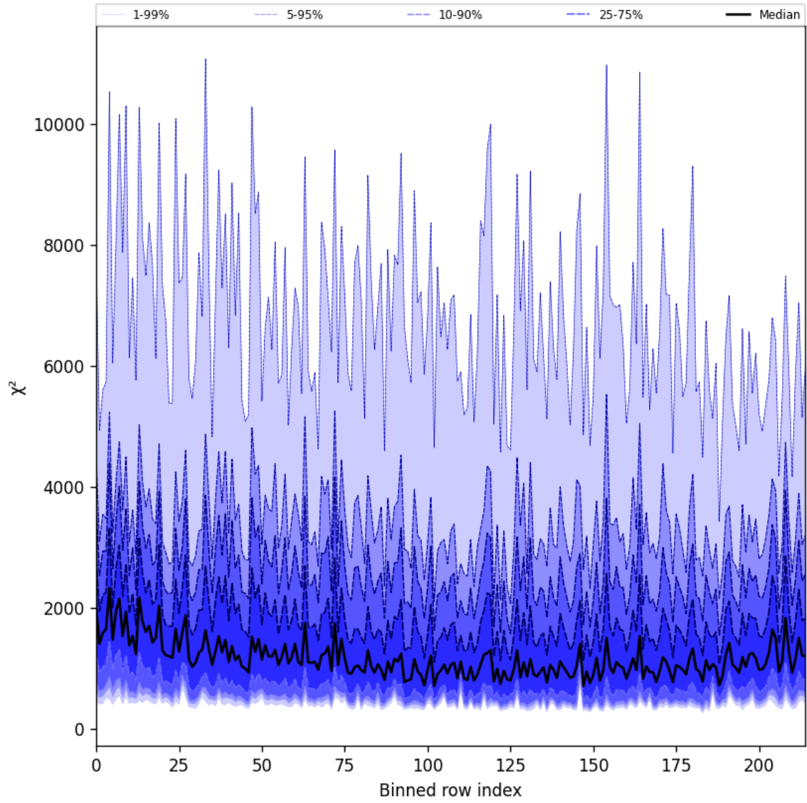
Figure 24: Along track statistics of “ \chi^2 ” for 2025-09-17 to 2025-09-18
