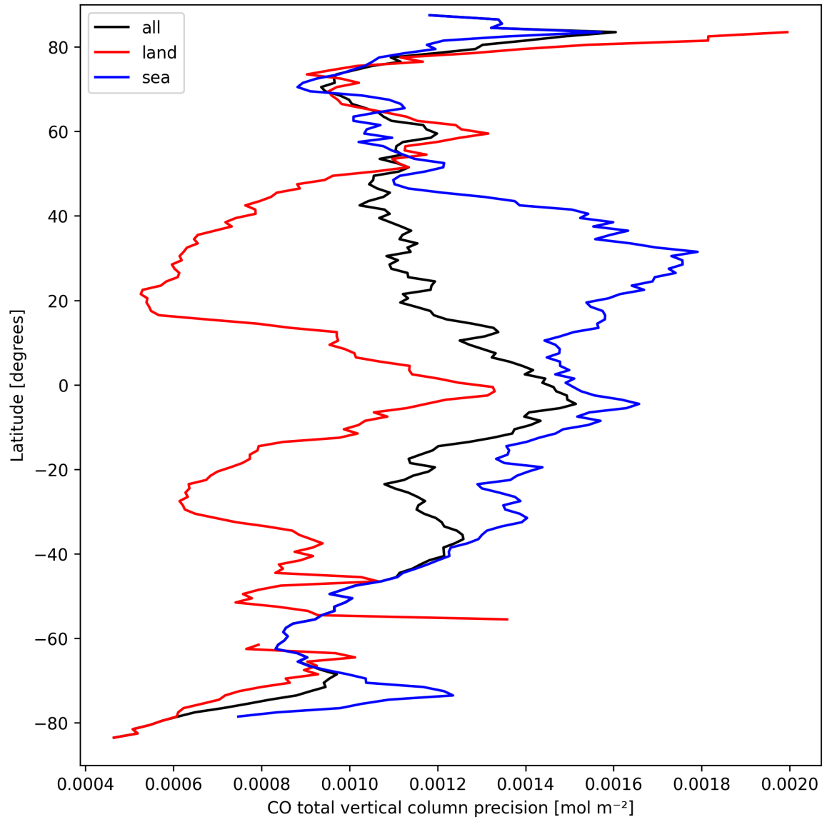
Figure 8: Zonal average of “CO total vertical column precision” for 2025-09-17 to 2025-09-18.
