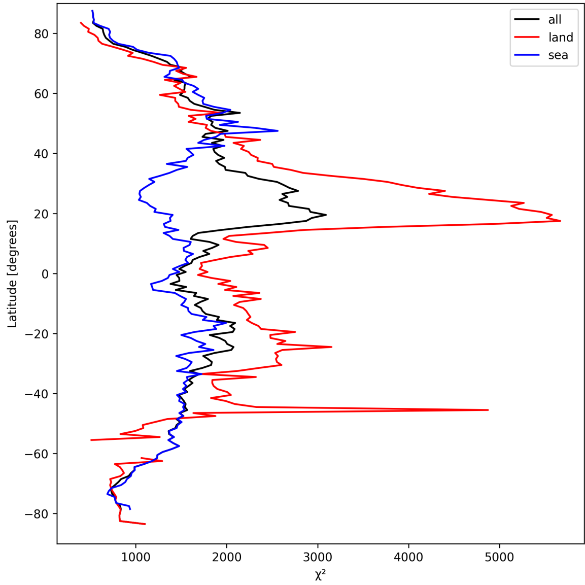
Figure 10: Zonal average of “ \chi^2 ” for 2025-09-17 to 2025-09-18.
