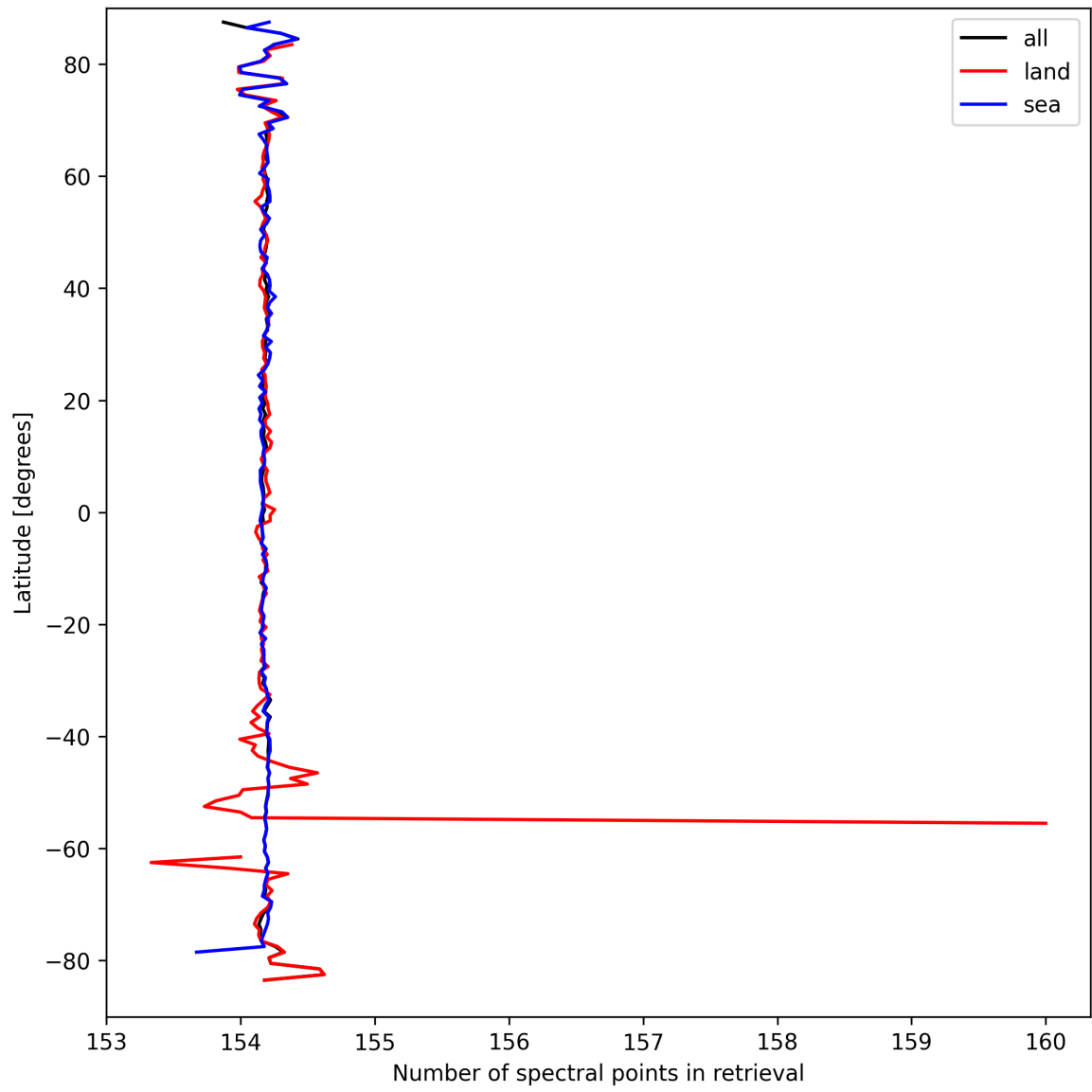
Figure 9: Zonal average of “Number of spectral points in retrieval” for 2025-09-17 to 2025-09-18.
