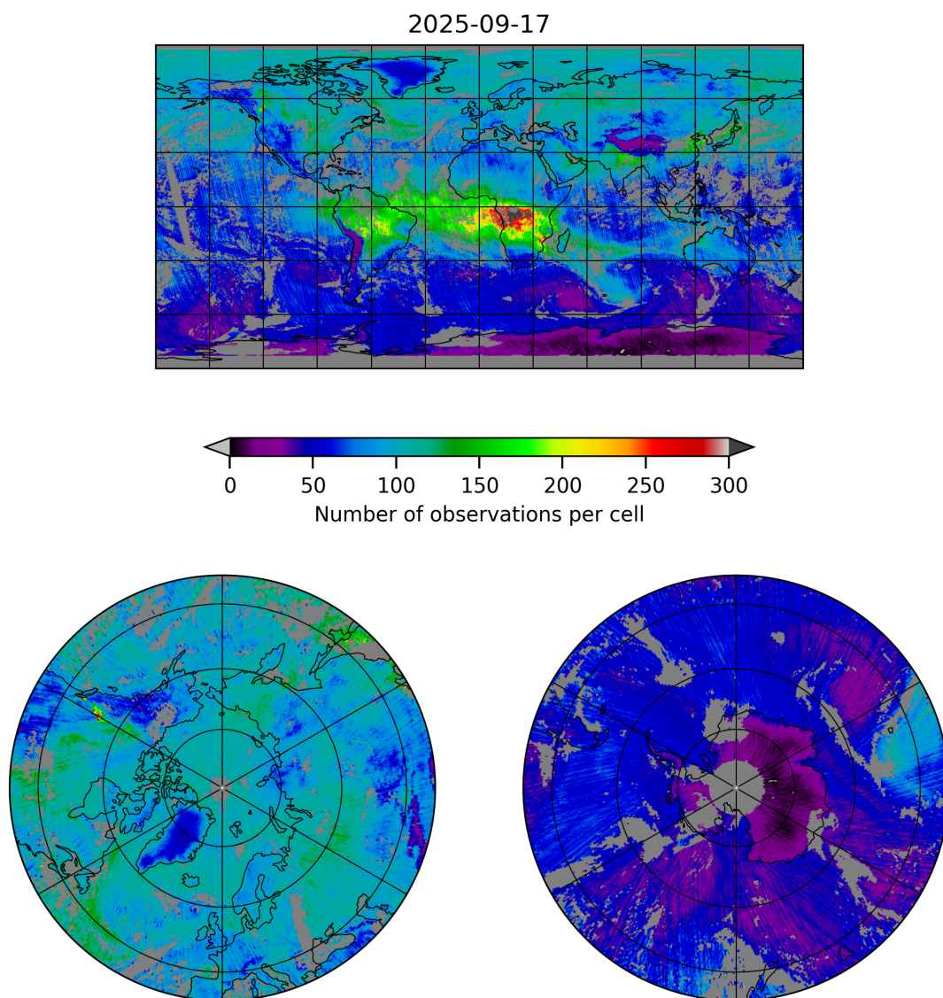
Figure 5: Map of the number of observations for 2025-09-17 to 2025-09-18
