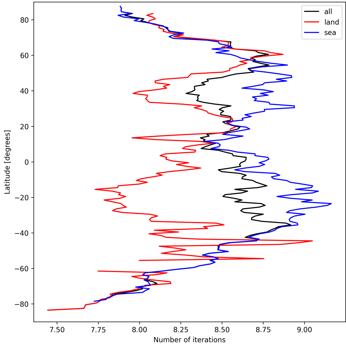
Figure 12: Zonal average of “Number of iterations” for 2025-09-17 to 2025-09-18.
