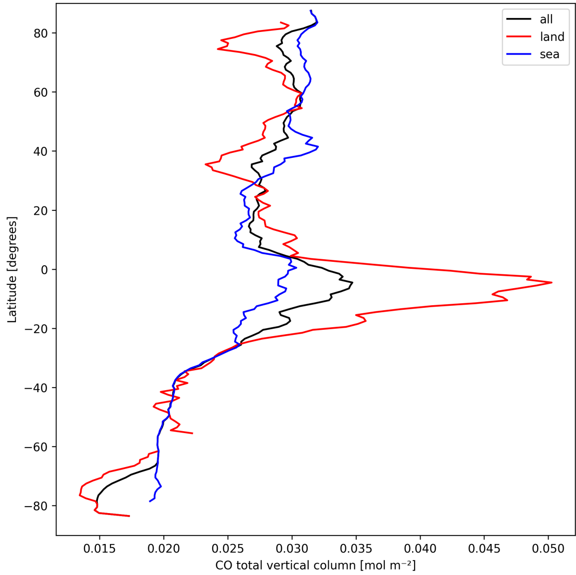
Figure 7: Zonal average of “CO total vertical column” for 2025-09-17 to 2025-09-18.
