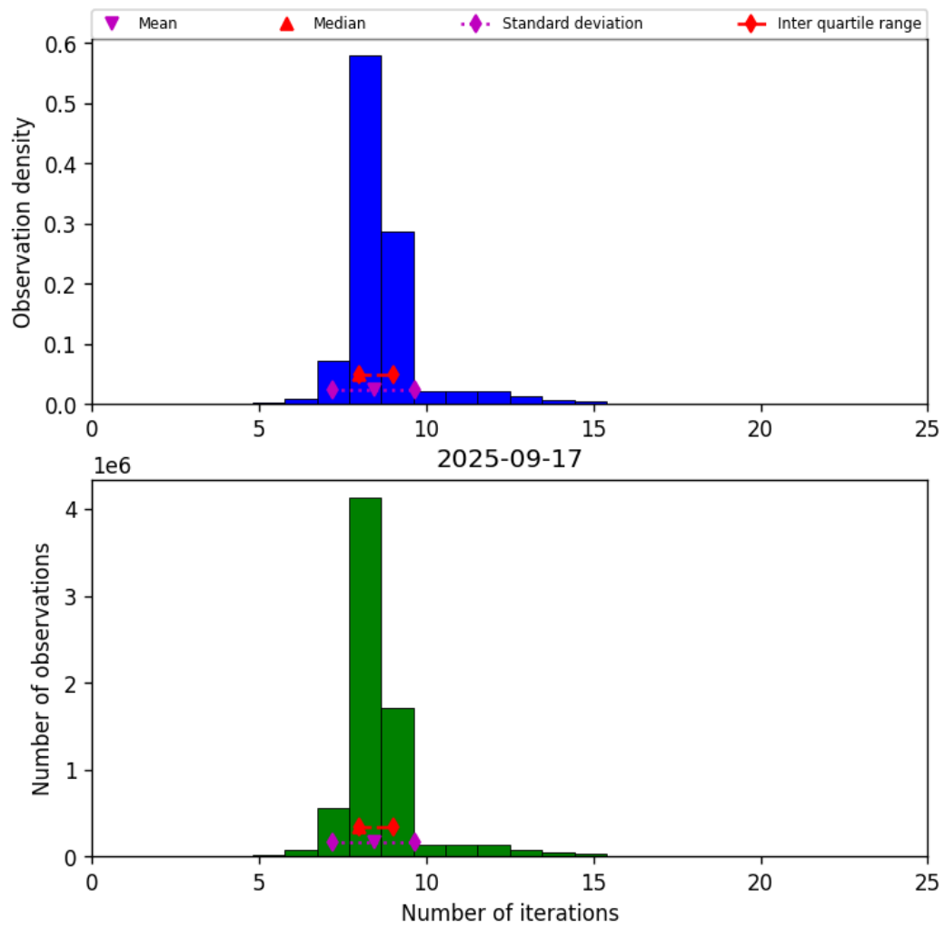
Figure 19: Histogram of “Number of iterations” for 2025-09-17 to 2025-09-18
