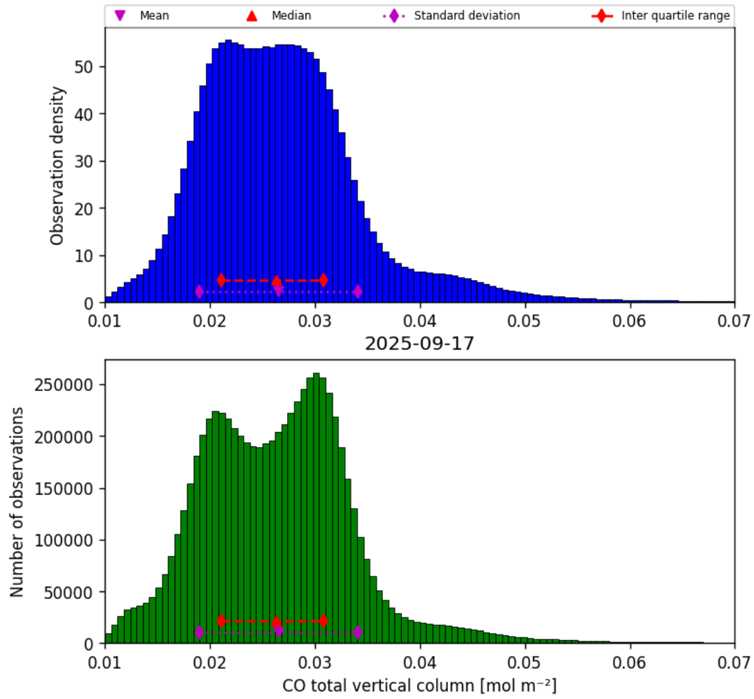
Figure 14: Histogram of “CO total vertical column” for 2025-09-17 to 2025-09-18
