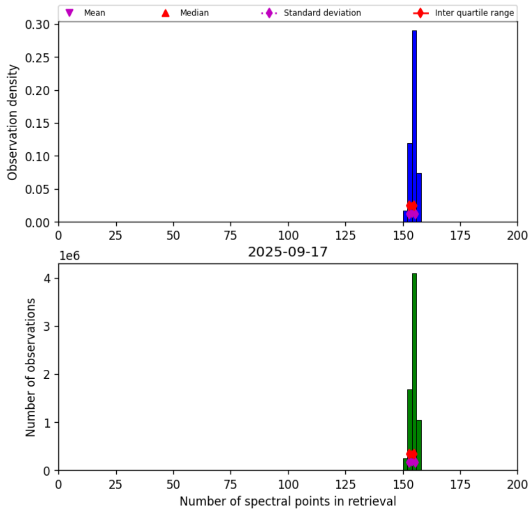
Figure 16: Histogram of “Number of spectral points in retrieval” for 2025-09-17 to 2025-09-18
