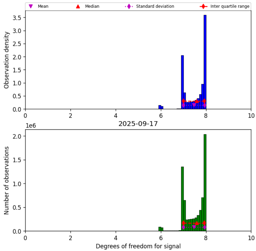
Figure 18: Histogram of “Degrees of freedom for signal” for 2025-09-17 to 2025-09-18
