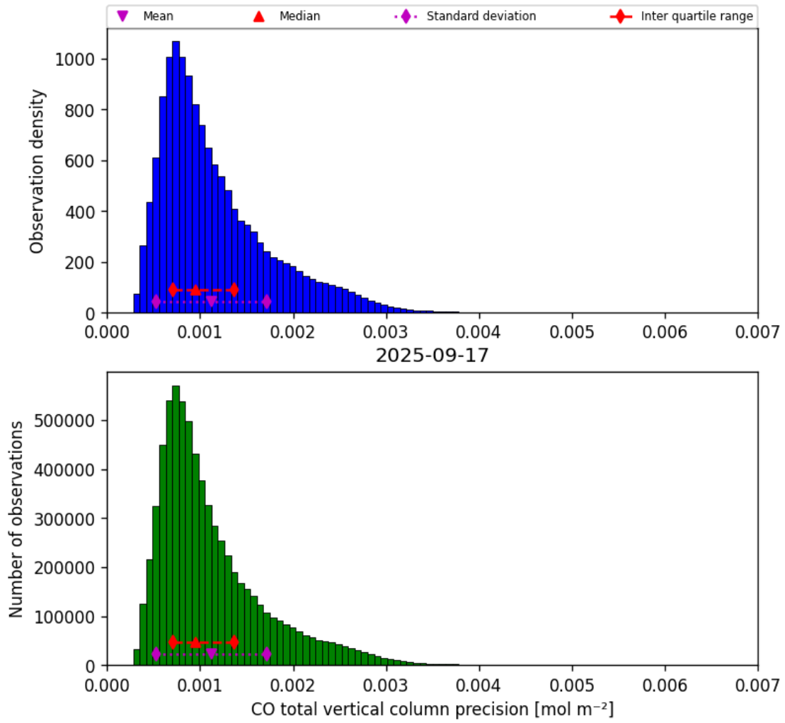
Figure 15: Histogram of “CO total vertical column precision” for 2025-09-17 to 2025-09-18
