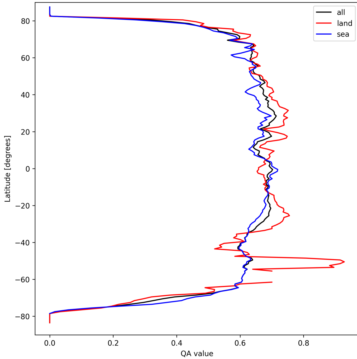
Figure 6: Zonal average of “QA value” for 2025-09-17 to 2025-09-18.
