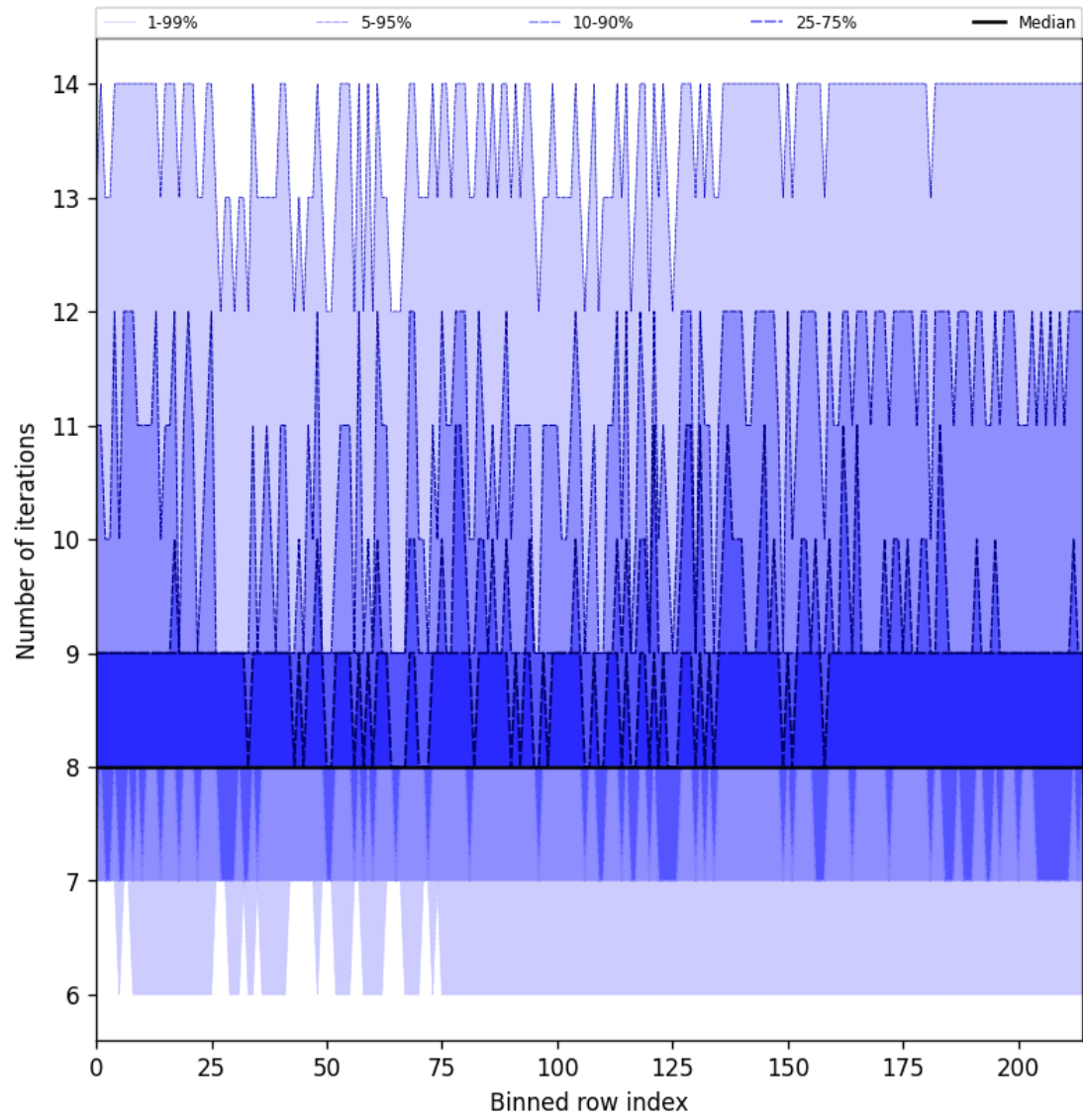
Figure 26: Along track statistics of “Number of iterations” for 2025-09-17 to 2025-09-18
