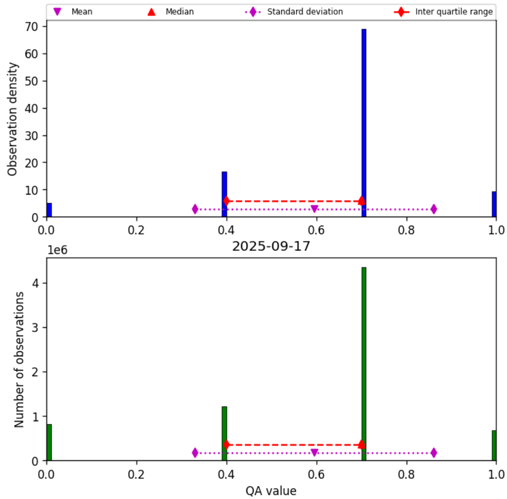
Figure 13: Histogram of “QA value” for 2025-09-17 to 2025-09-18
