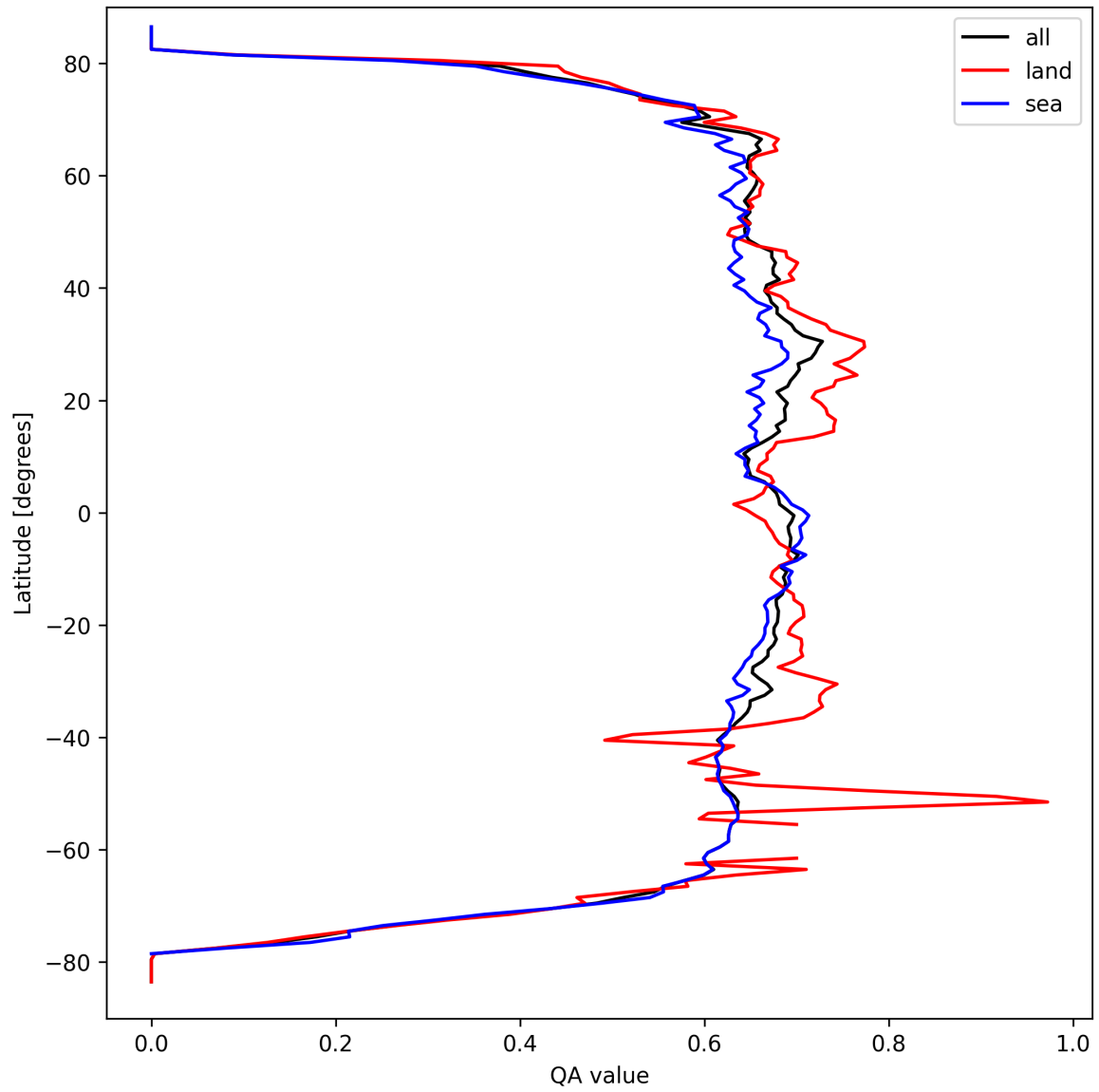
Figure 6: Zonal average of “QA value” for 2025-09-18 to 2025-09-18.
