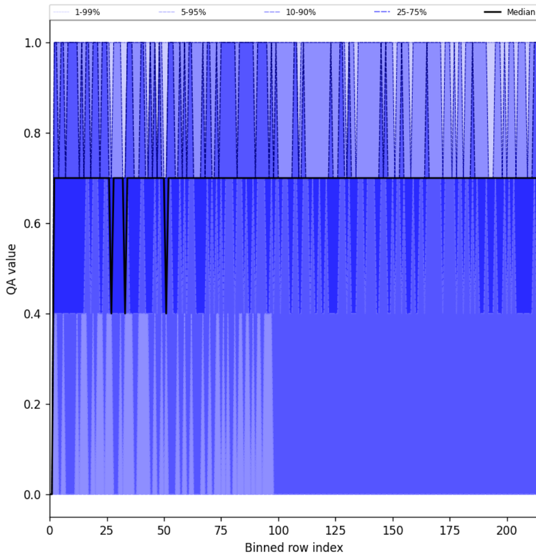
Figure 20: Along track statistics of “QA value” for 2025-09-18 to 2025-09-18
