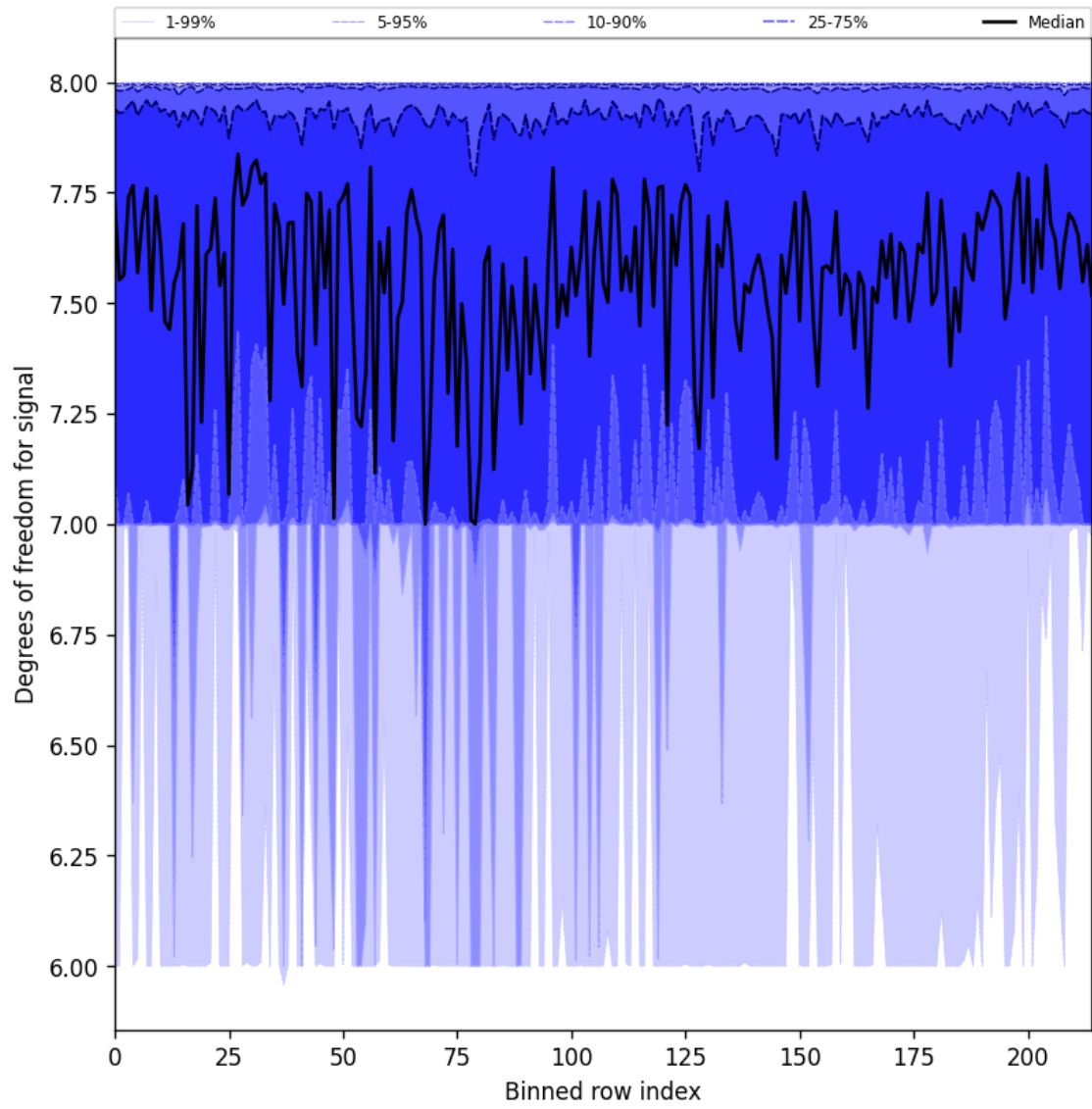
Figure 25: Along track statistics of “Degrees of freedom for signal” for 2025-09-18 to 2025-09-18
