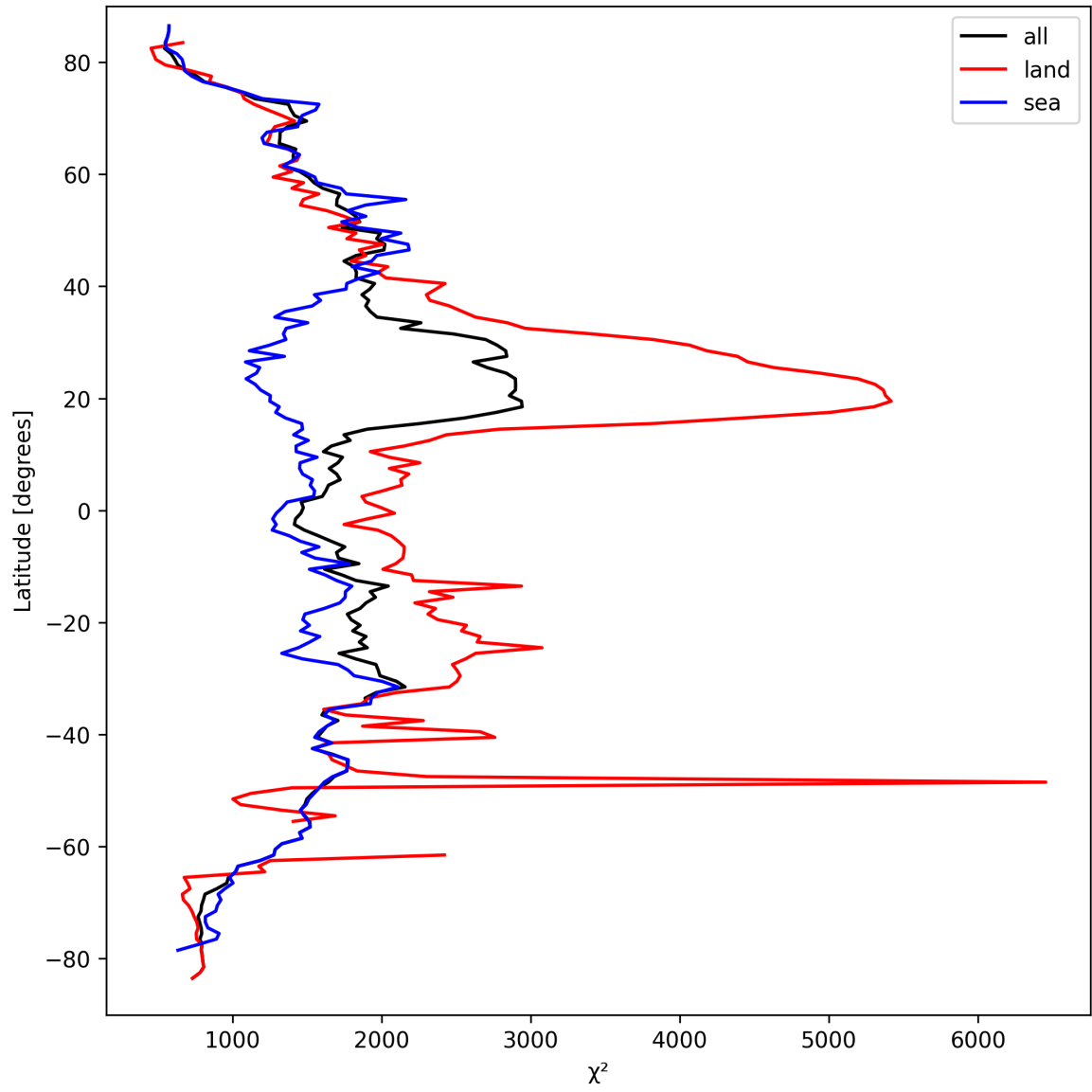
Figure 10: Zonal average of “ \chi^2 ” for 2025-09-18 to 2025-09-18.
