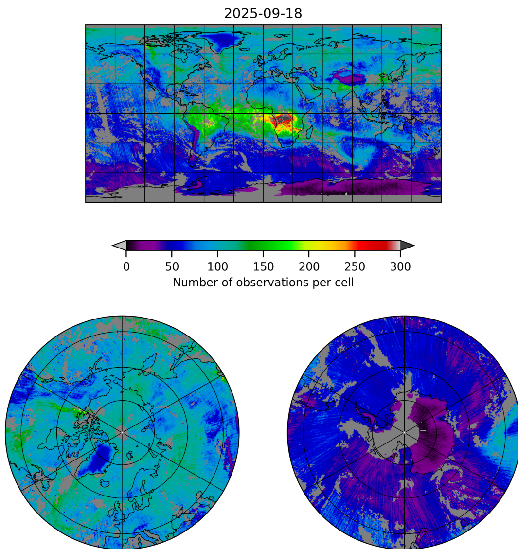
Figure 5: Map of the number of observations for 2025-09-18 to 2025-09-18
