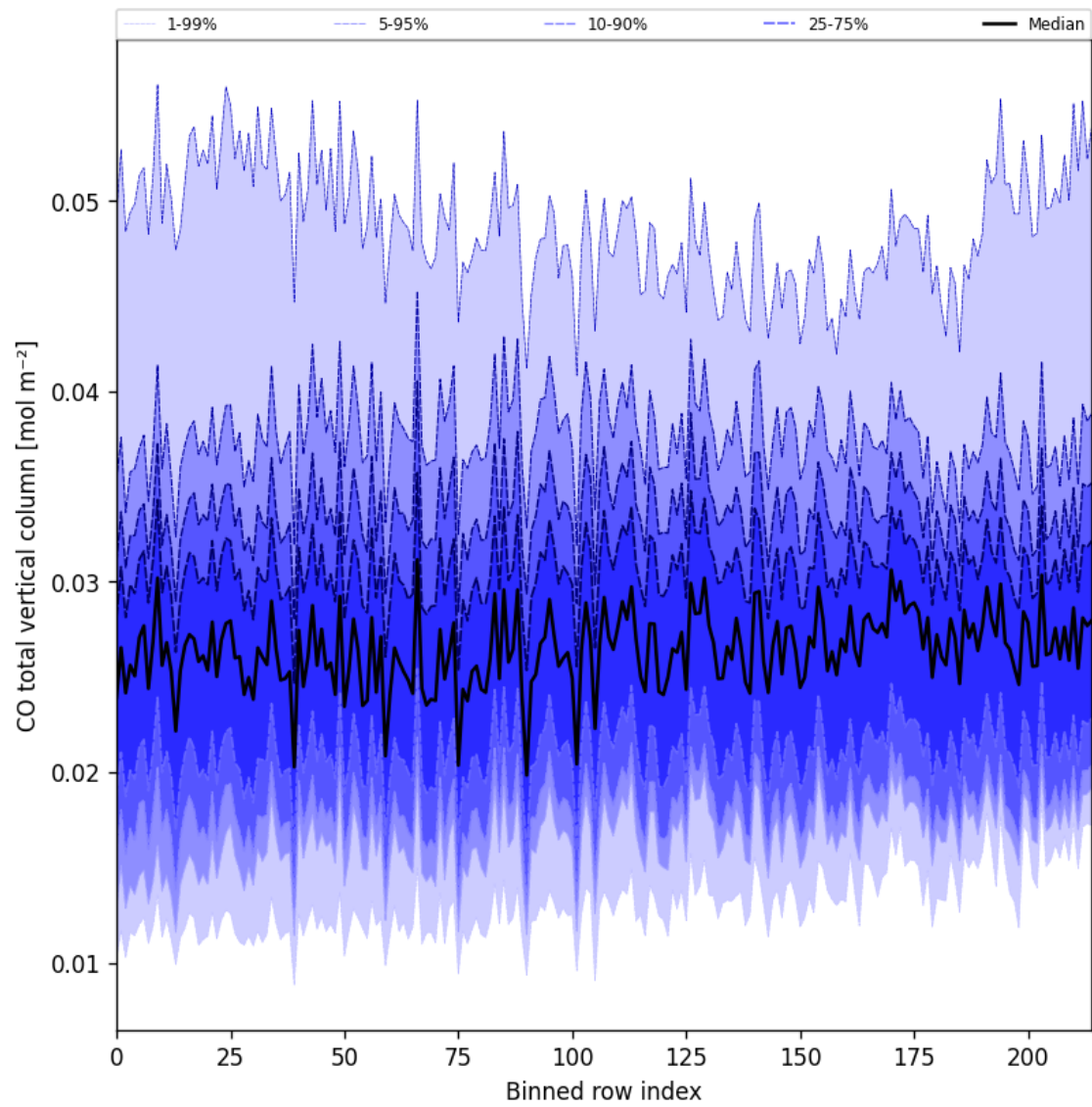
Figure 21: Along track statistics of “CO total vertical column” for 2025-09-18 to 2025-09-18
