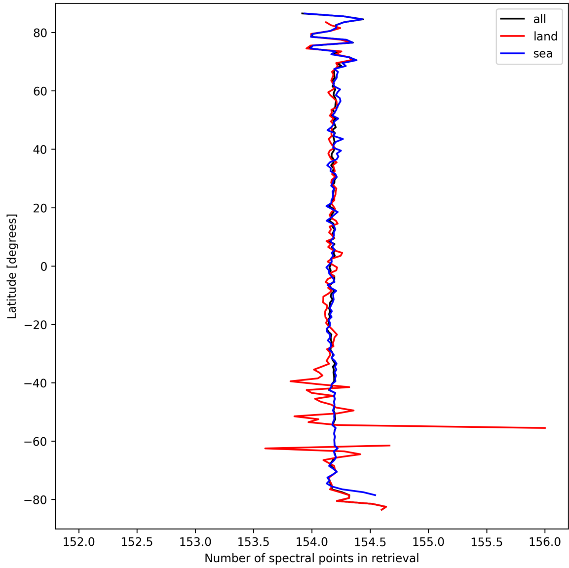
Figure 9: Zonal average of “Number of spectral points in retrieval” for 2025-09-18 to 2025-09-18.
