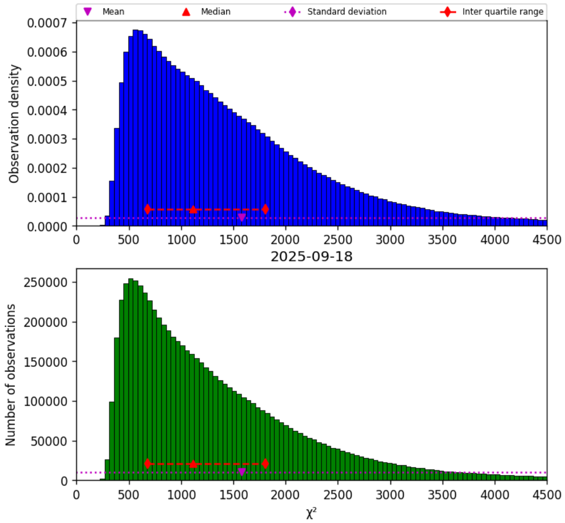
Figure 17: Histogram of " \chi^2 " for 2025-09-18 to 2025-09-18
