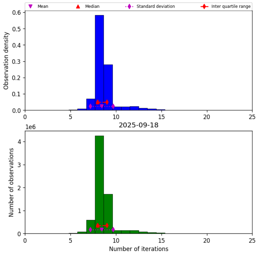
Figure 19: Histogram of “Number of iterations” for 2025-09-18 to 2025-09-18
