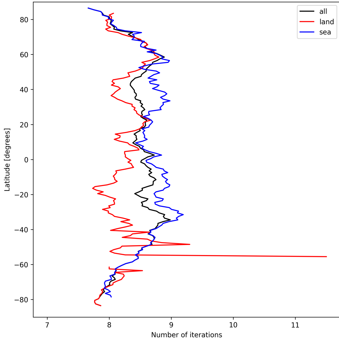
Figure 12: Zonal average of “Number of iterations” for 2025-09-18 to 2025-09-18.
