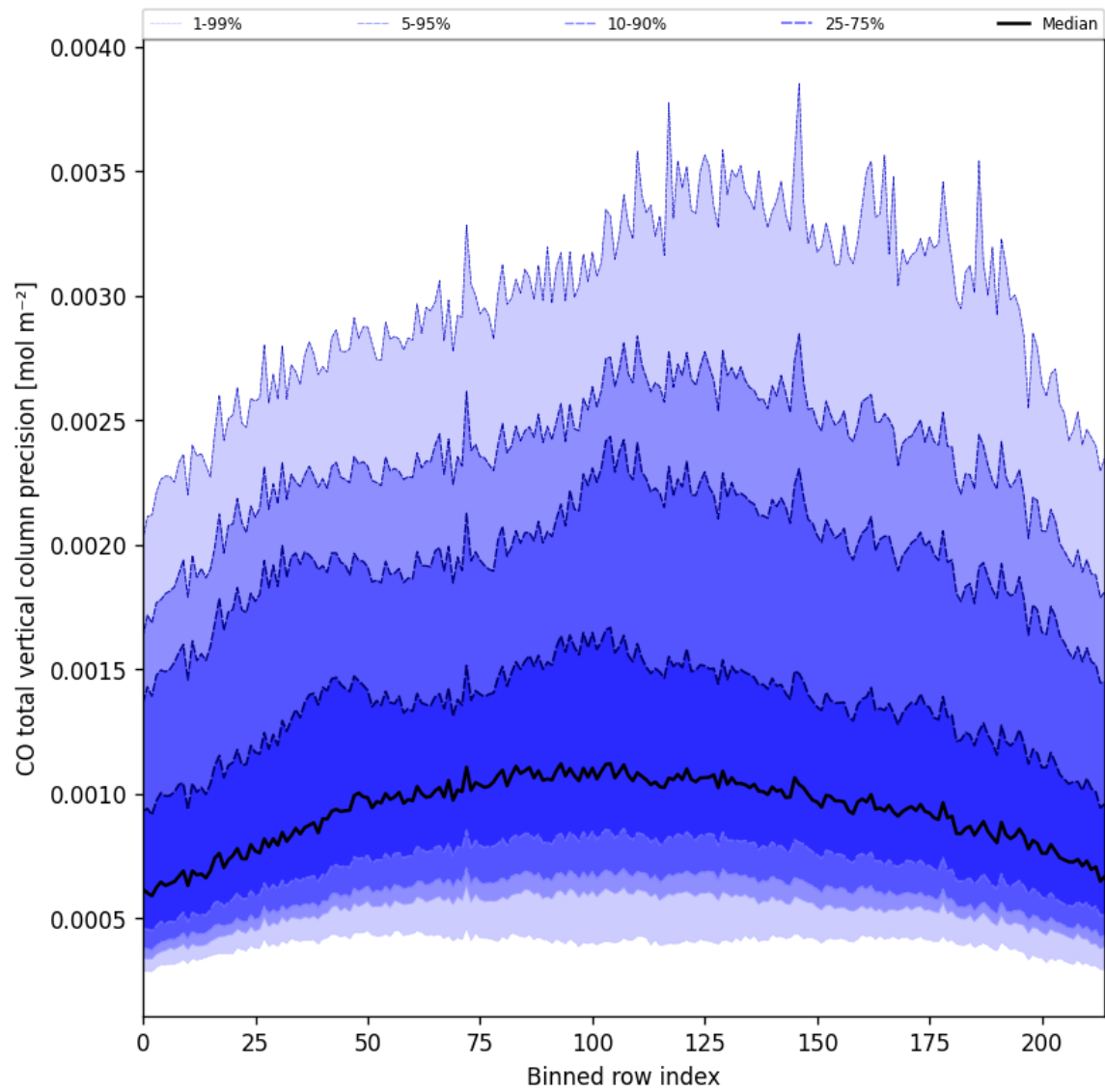
Figure 22: Along track statistics of “CO total vertical column precision” for 2025-09-18 to 2025-09-18
