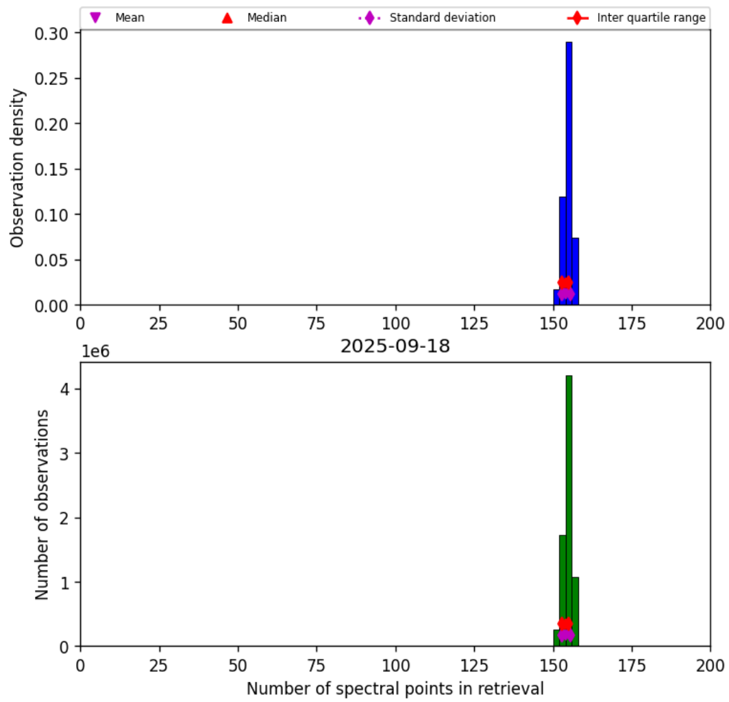
Figure 16: Histogram of “Number of spectral points in retrieval” for 2025-09-18 to 2025-09-18
