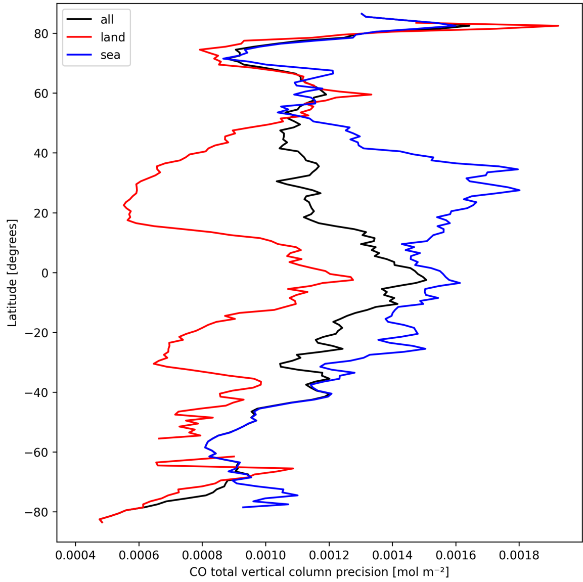
Figure 8: Zonal average of “CO total vertical column precision” for 2025-09-18 to 2025-09-18.
