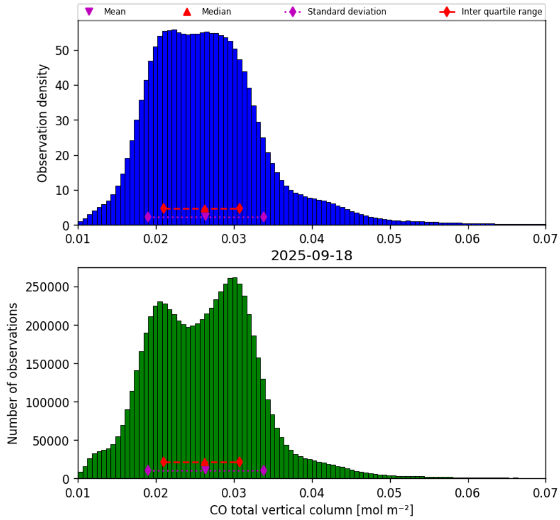
Figure 14: Histogram of “CO total vertical column” for 2025-09-18 to 2025-09-18
