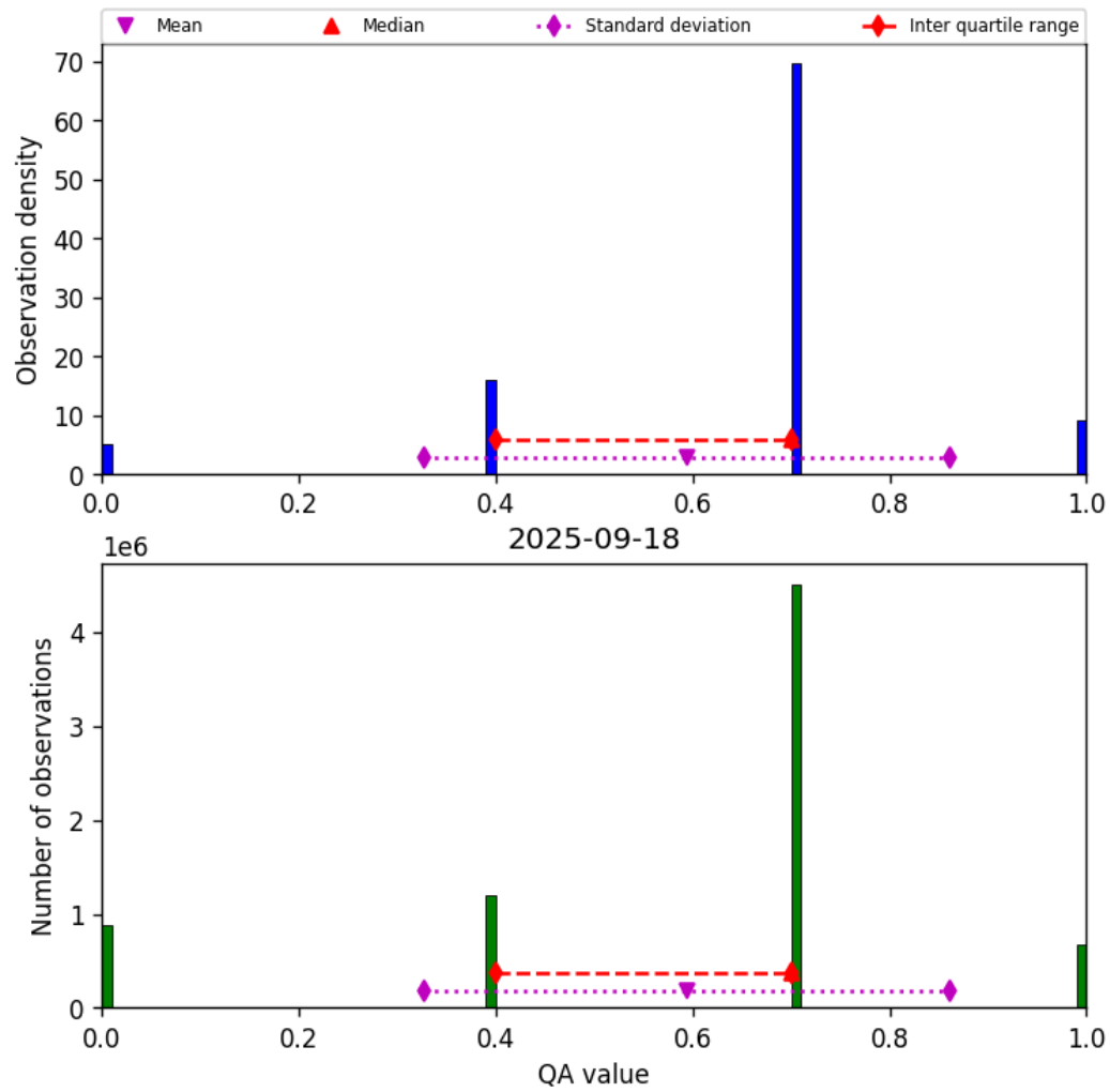
Figure 13: Histogram of “QA value” for 2025-09-18 to 2025-09-18
