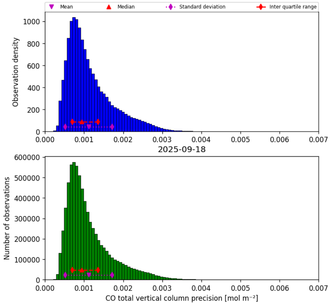
Figure 15: Histogram of “CO total vertical column precision” for 2025-09-18 to 2025-09-18
