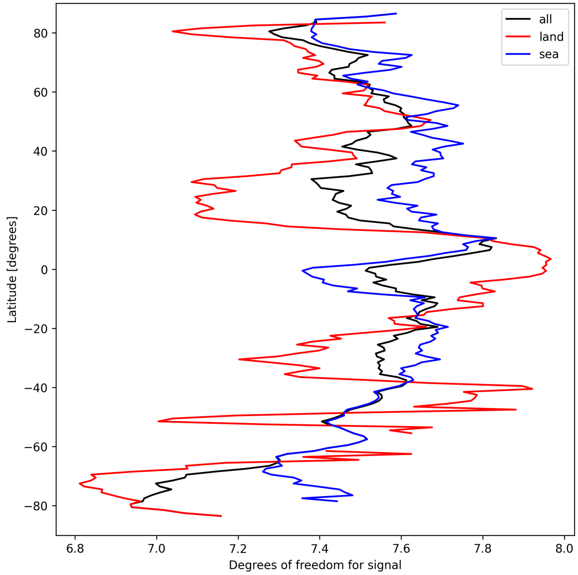
Figure 11: Zonal average of “Degrees of freedom for signal” for 2025-09-18 to 2025-09-18.
