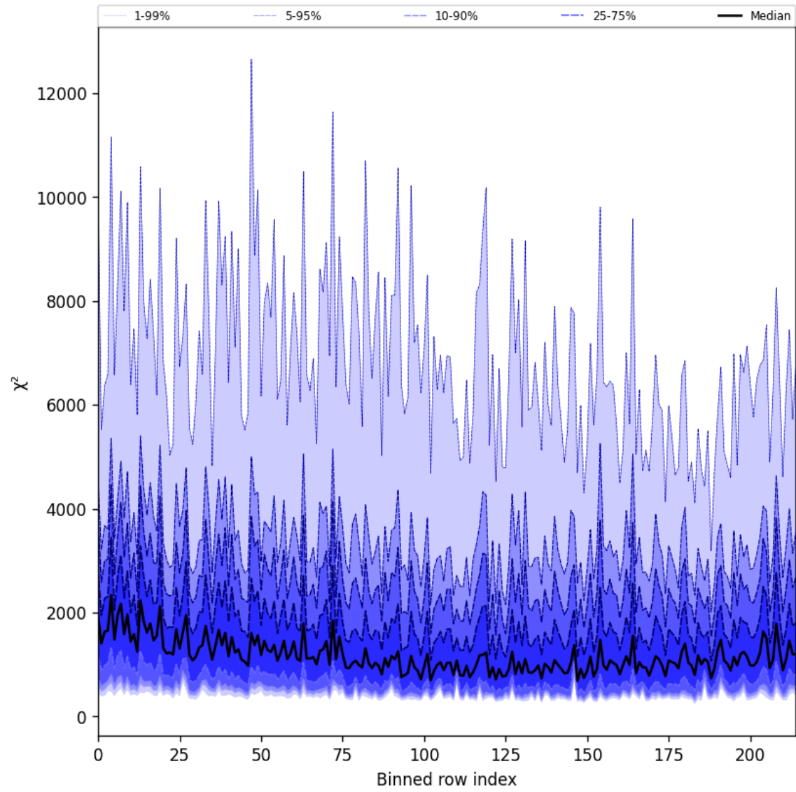
Figure 24: Along track statistics of “ \chi^2 ” for 2025-09-18 to 2025-09-18
