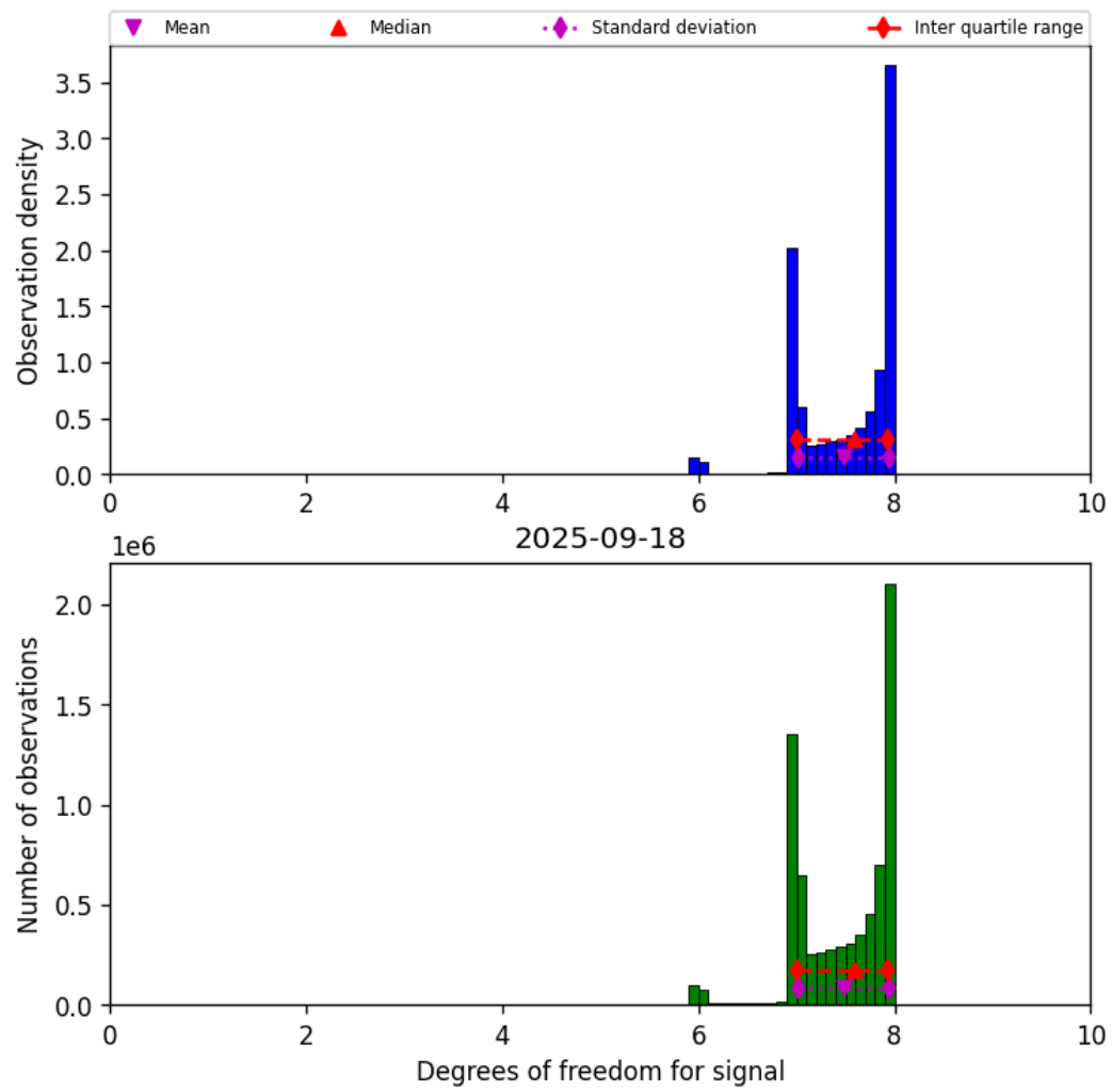
Figure 18: Histogram of “Degrees of freedom for signal” for 2025-09-18 to 2025-09-18
