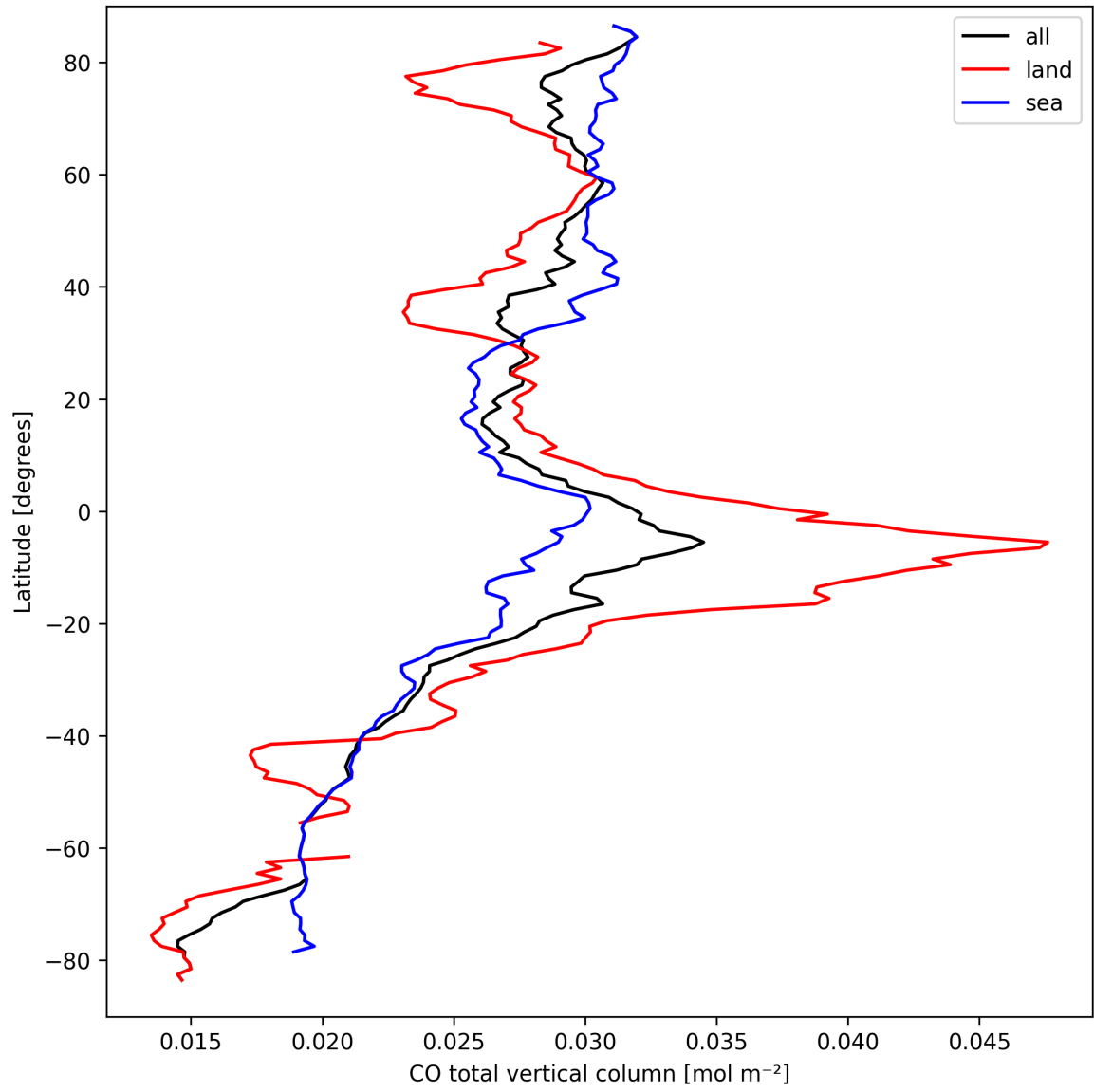
Figure 7: Zonal average of “CO total vertical column” for 2025-09-18 to 2025-09-18.
