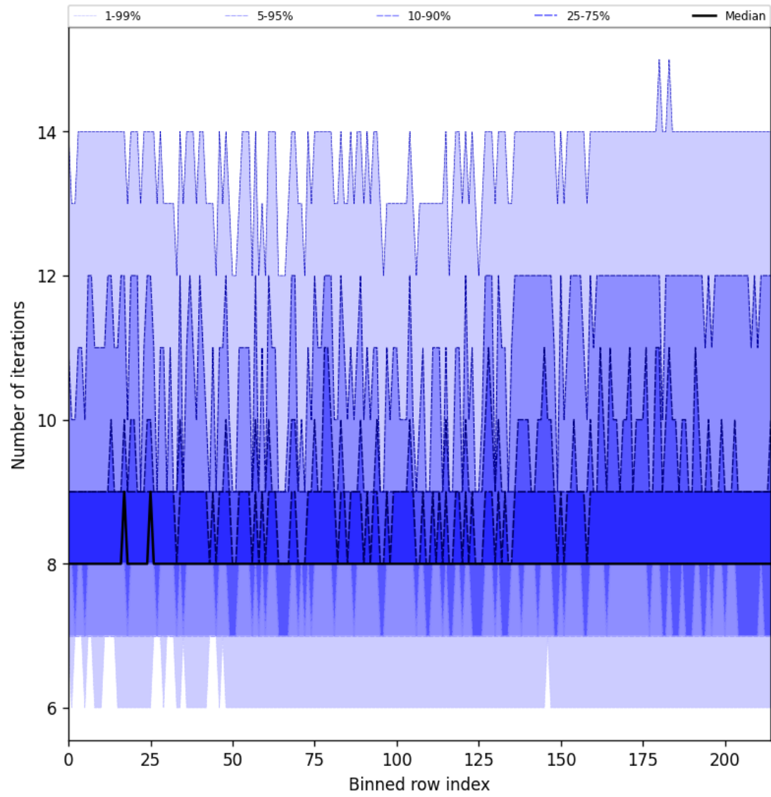
Figure 26: Along track statistics of “Number of iterations” for 2025-09-18 to 2025-09-18
