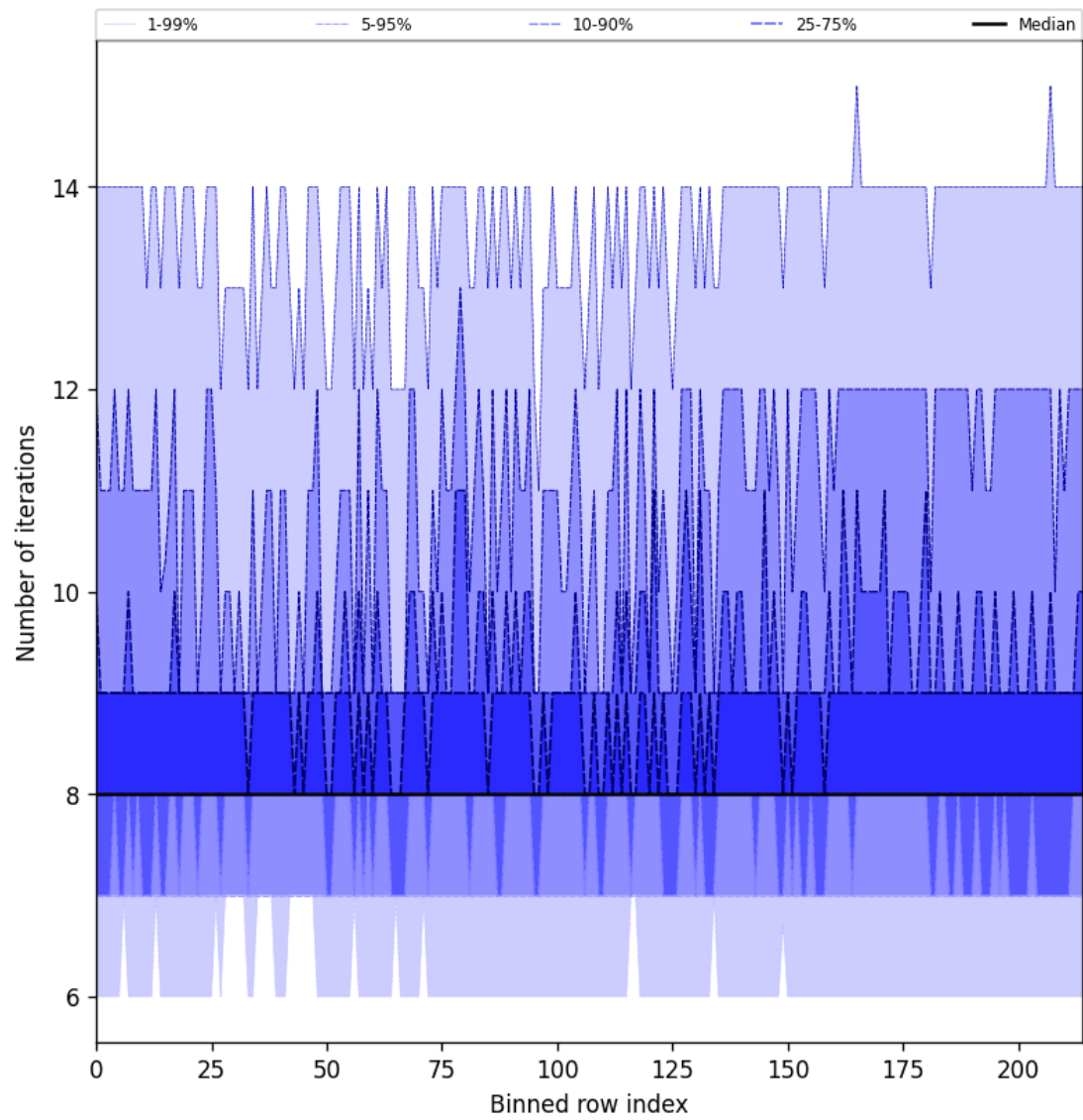
Figure 26: Along track statistics of “Number of iterations” for 2025-09-20 to 2025-09-21
