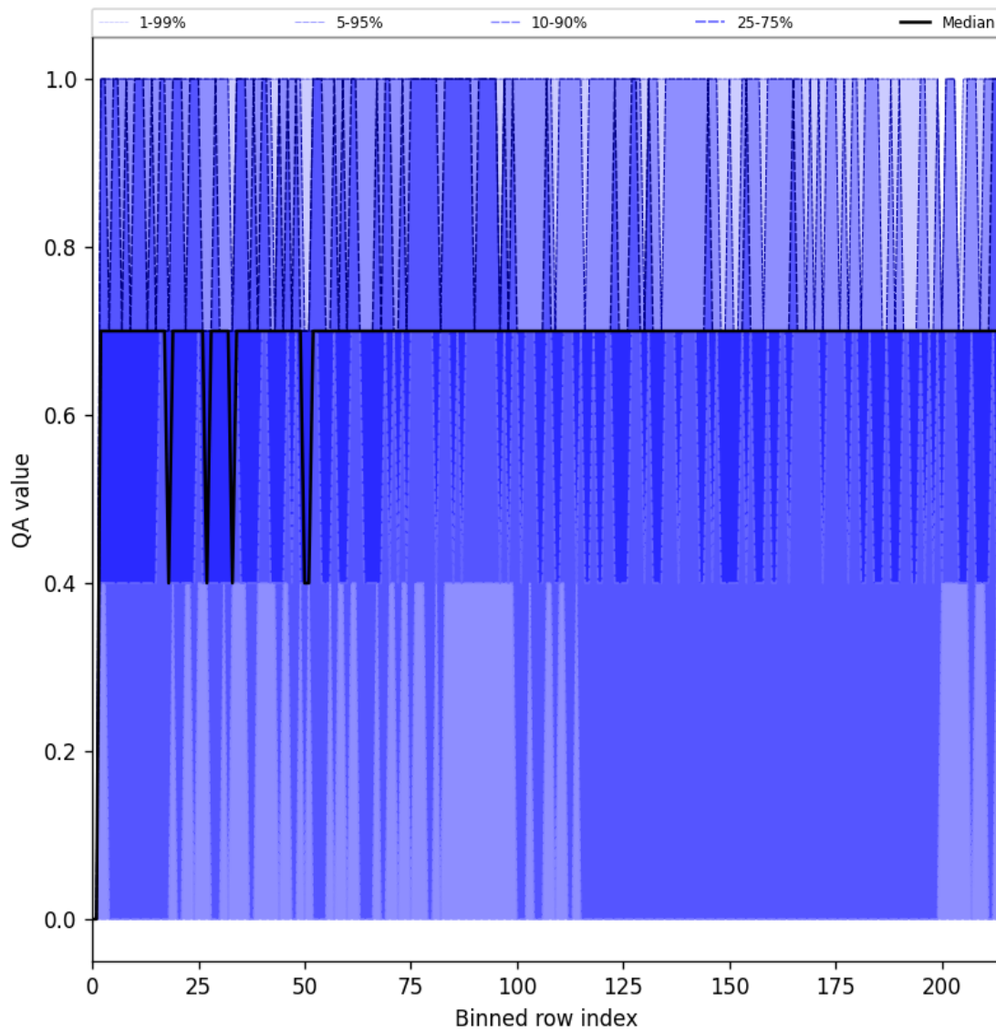
Figure 20: Along track statistics of “QA value” for 2025-09-20 to 2025-09-21
