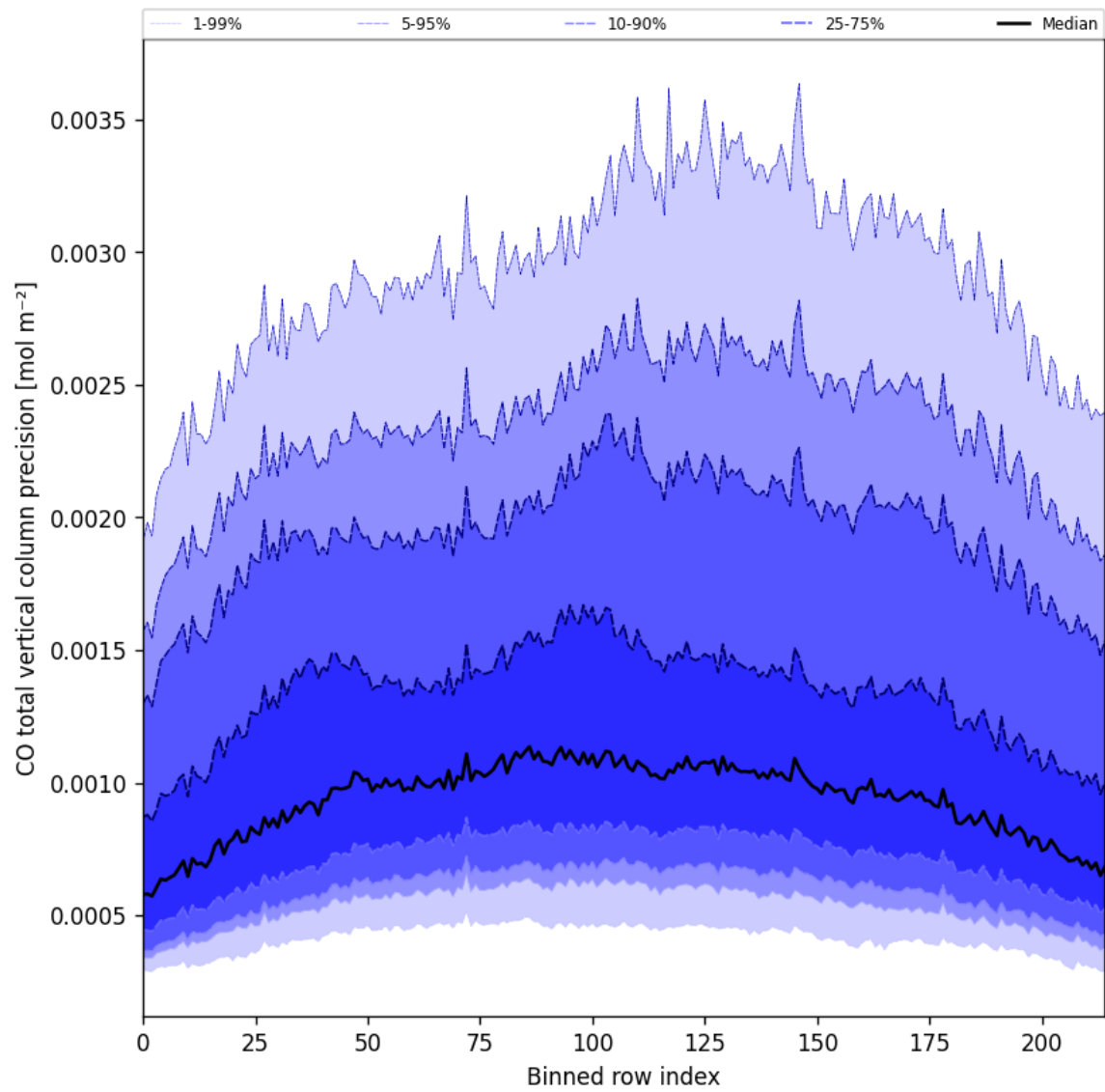
Figure 22: Along track statistics of “CO total vertical column precision” for 2025-09-20 to 2025-09-21
