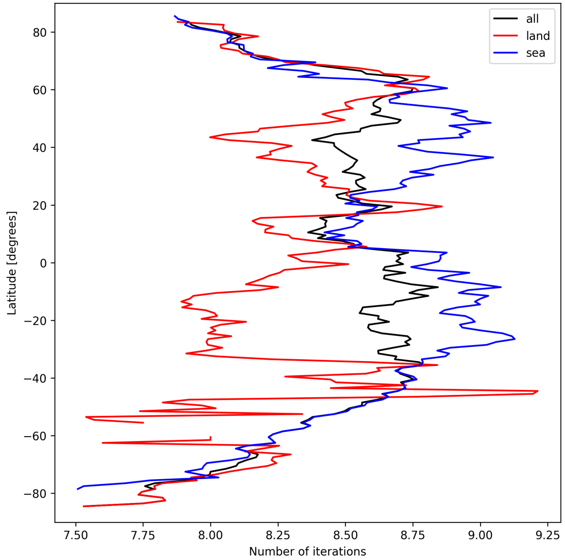
Figure 12: Zonal average of “Number of iterations” for 2025-09-20 to 2025-09-21.
