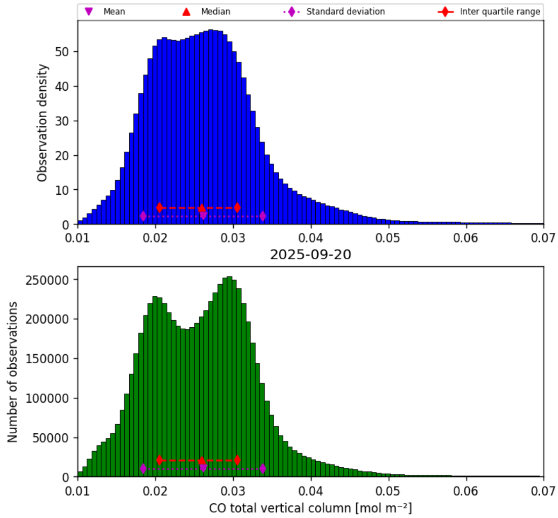
Figure 14: Histogram of “CO total vertical column” for 2025-09-20 to 2025-09-21
