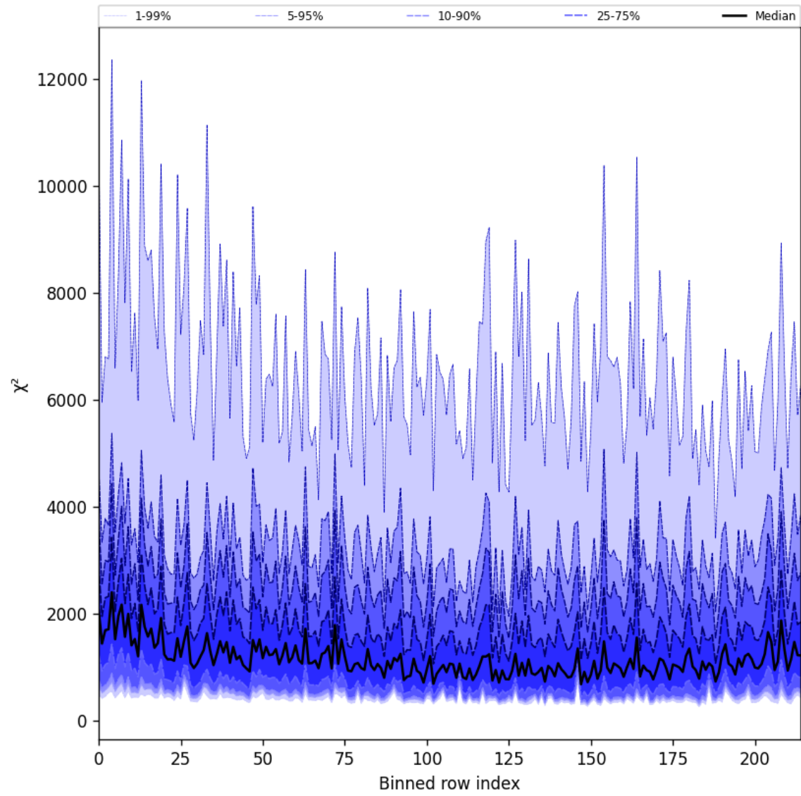
Figure 24: Along track statistics of “ \chi^2 ” for 2025-09-20 to 2025-09-21
