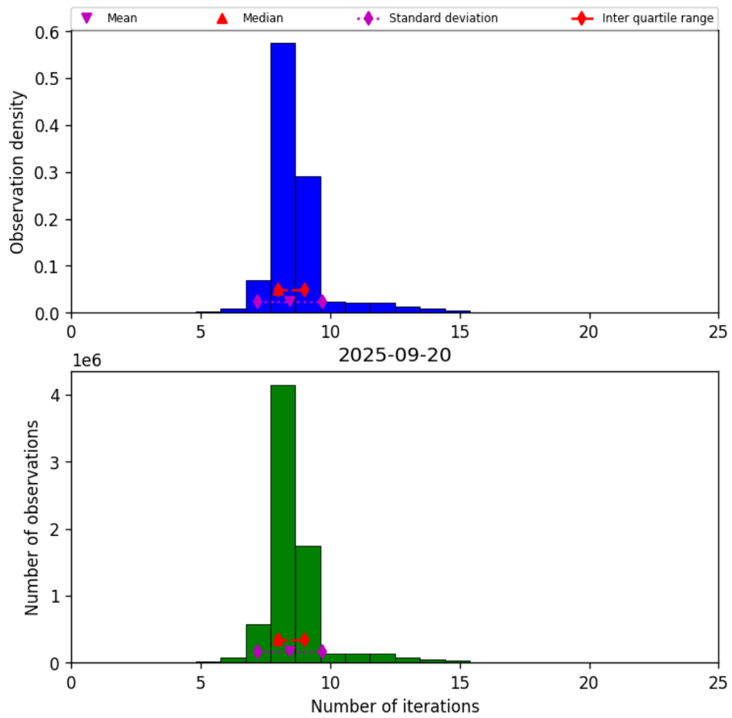
Figure 19: Histogram of “Number of iterations” for 2025-09-20 to 2025-09-21
