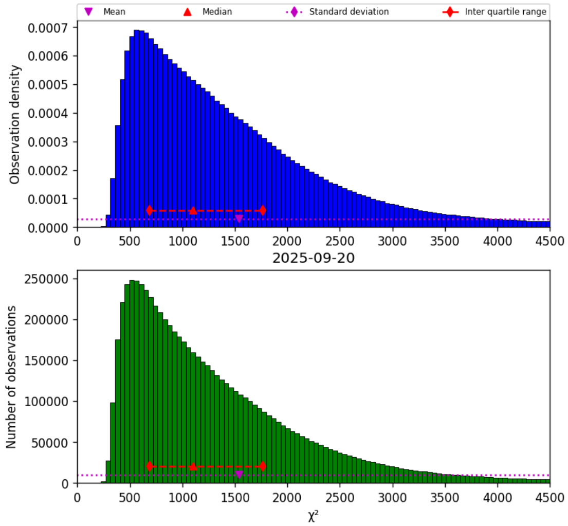
Figure 17: Histogram of " \chi^2 " for 2025-09-20 to 2025-09-21
