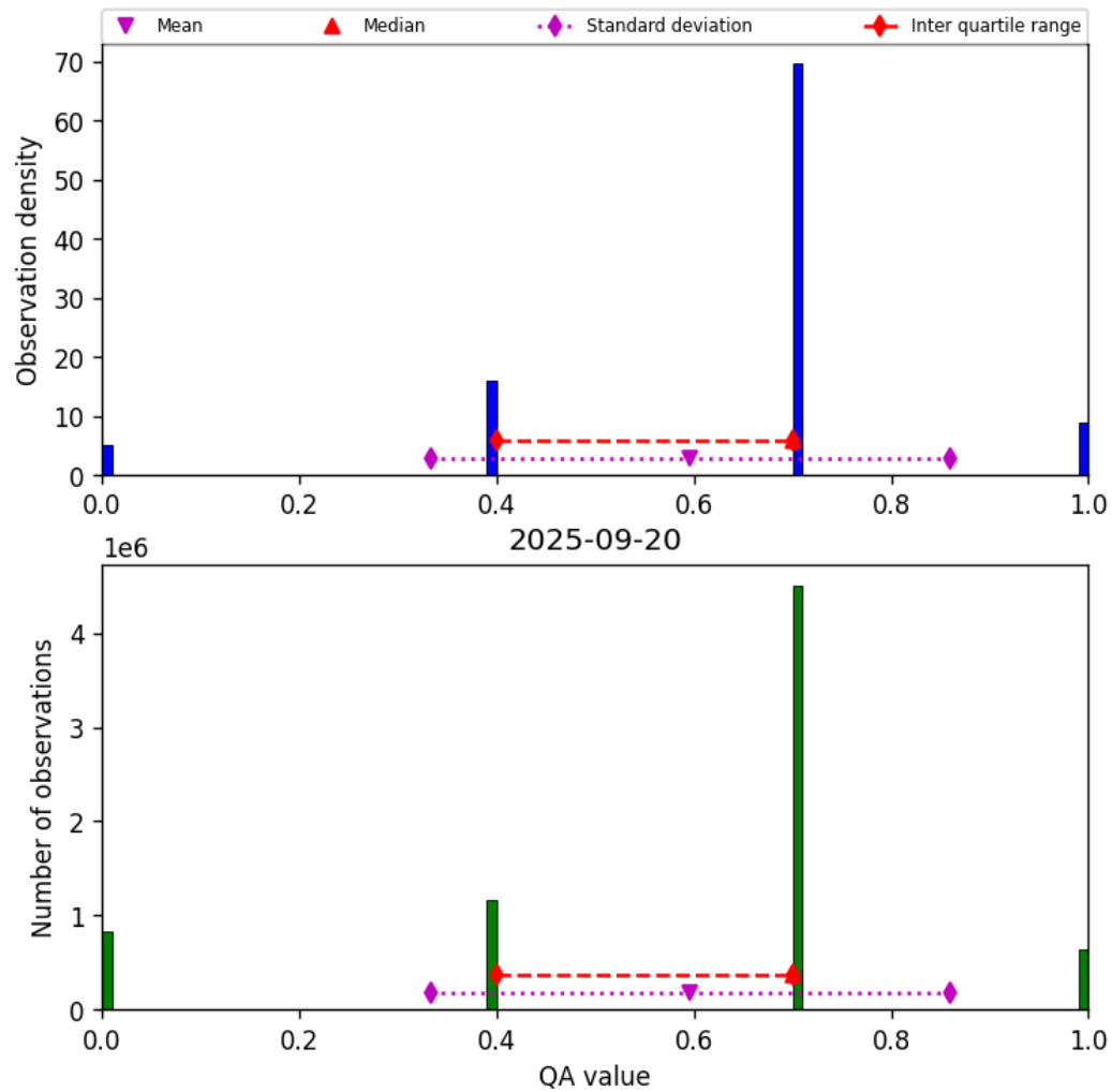
Figure 13: Histogram of “QA value” for 2025-09-20 to 2025-09-21
