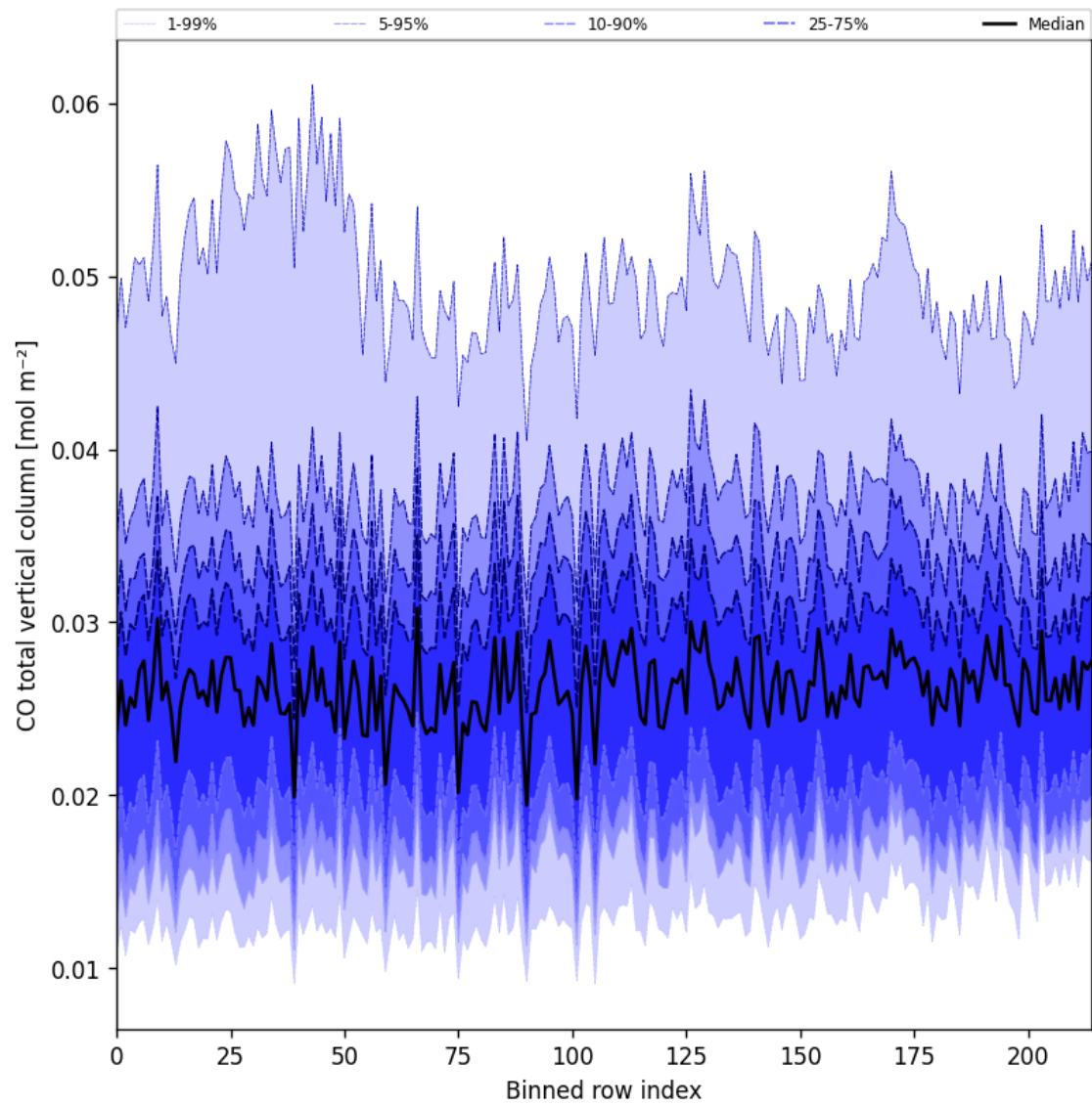
Figure 21: Along track statistics of “CO total vertical column” for 2025-09-20 to 2025-09-21
