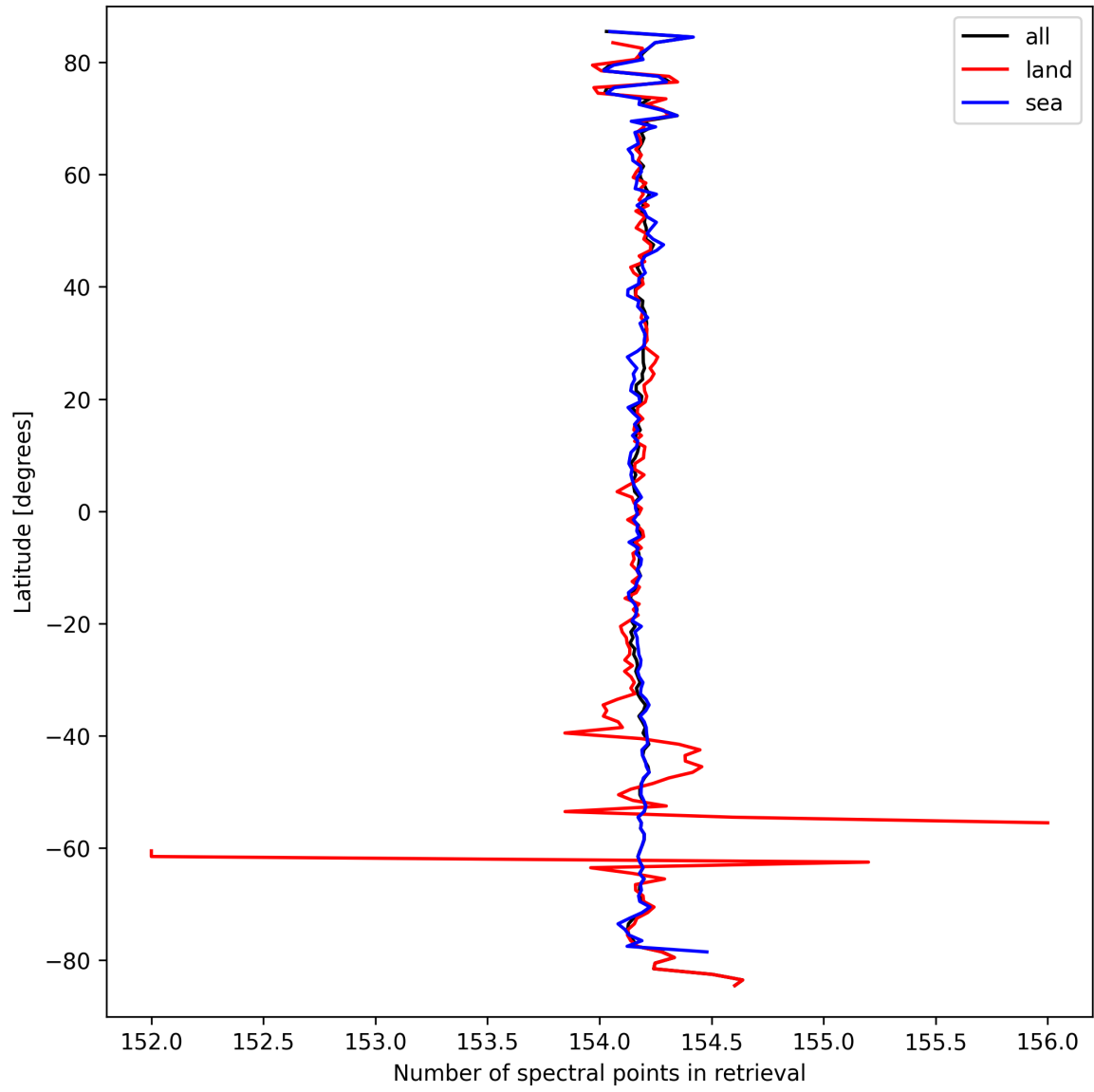
Figure 9: Zonal average of “Number of spectral points in retrieval” for 2025-09-20 to 2025-09-21.
