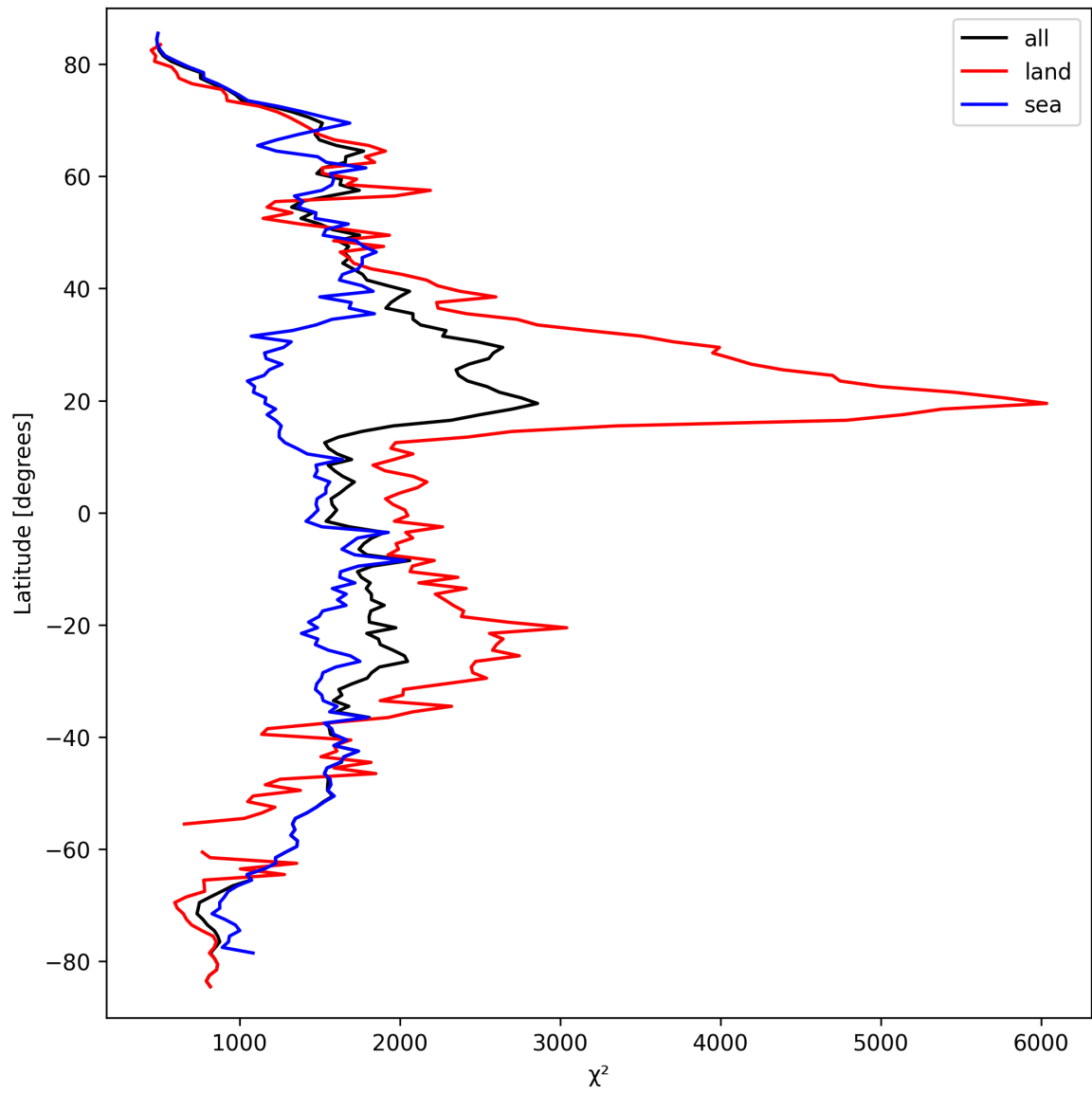
Figure 10: Zonal average of “ \chi^2 ” for 2025-09-20 to 2025-09-21.
