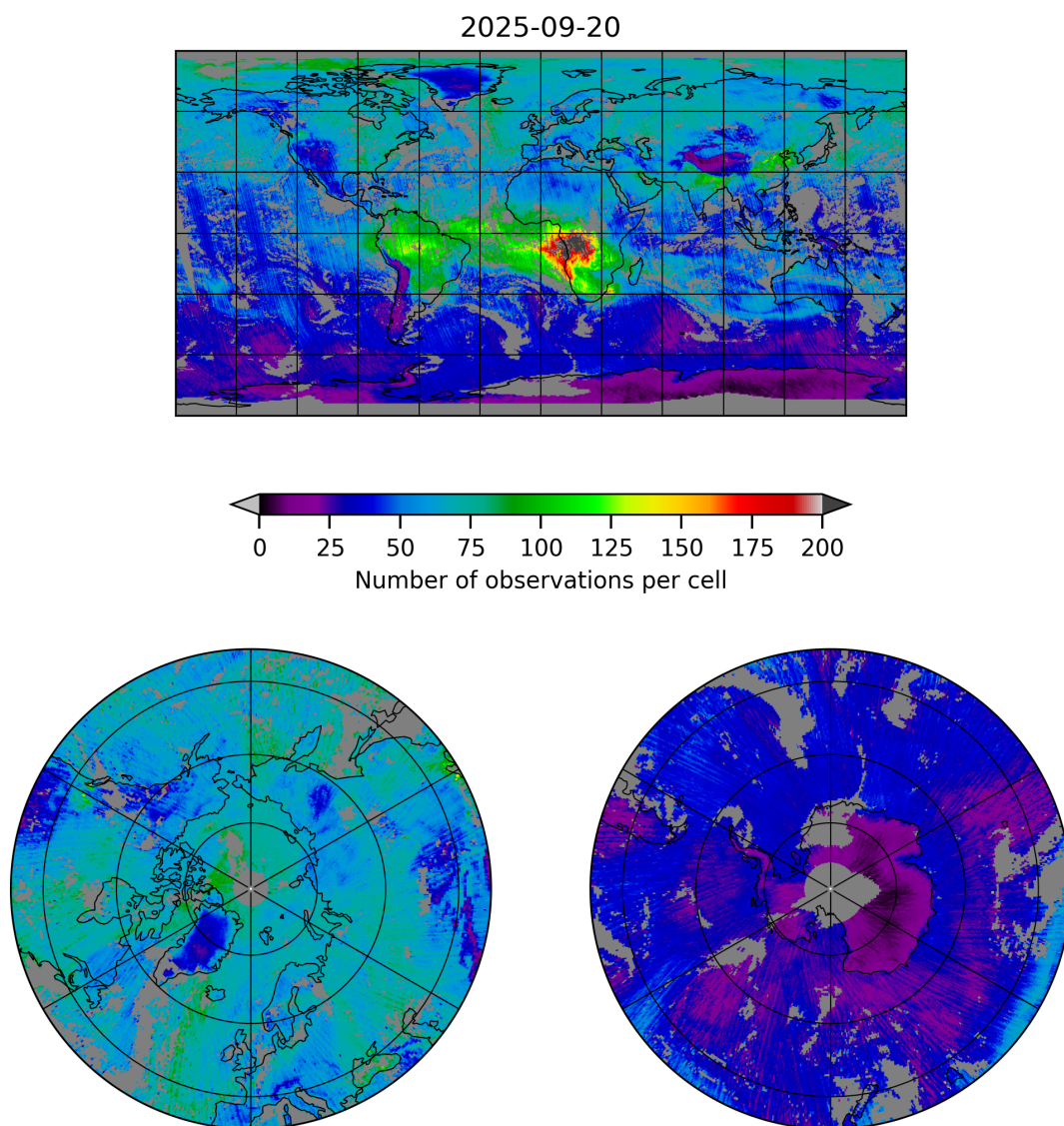
Figure 5: Map of the number of observations for 2025-09-20 to 2025-09-21
