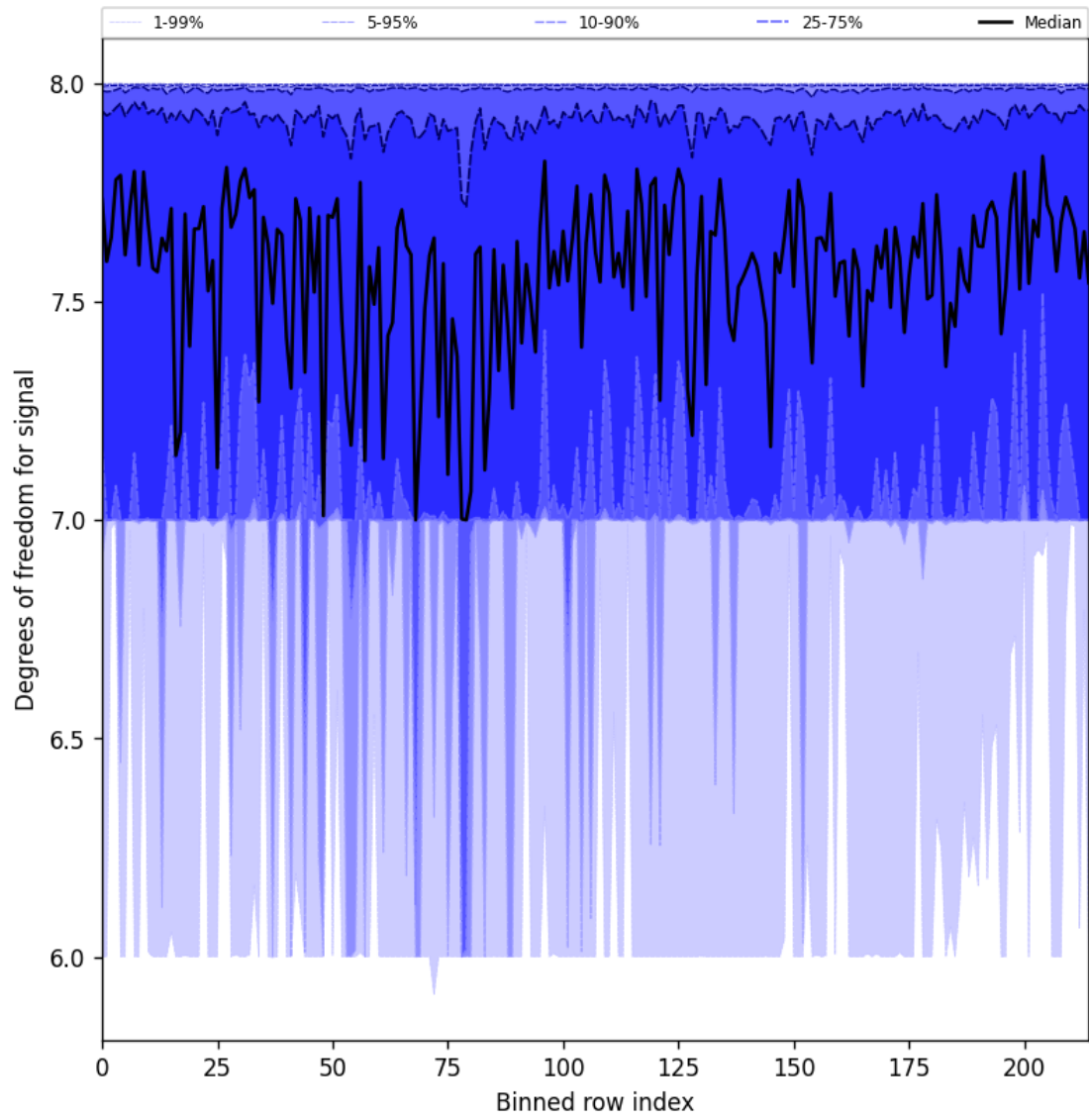
Figure 25: Along track statistics of “Degrees of freedom for signal” for 2025-09-20 to 2025-09-21
