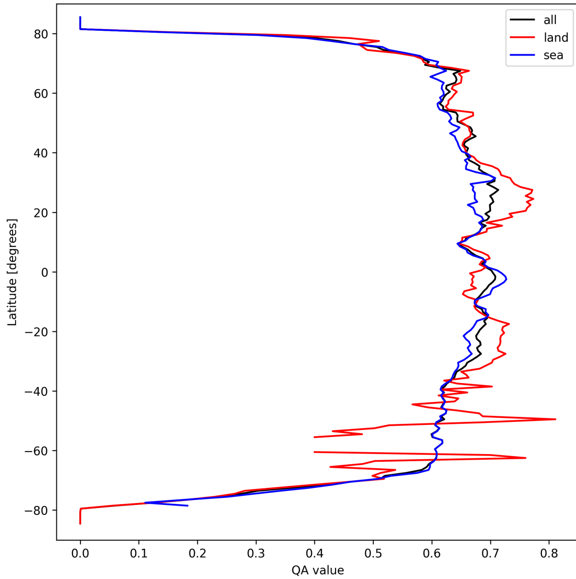
Figure 6: Zonal average of “QA value” for 2025-09-20 to 2025-09-21.
