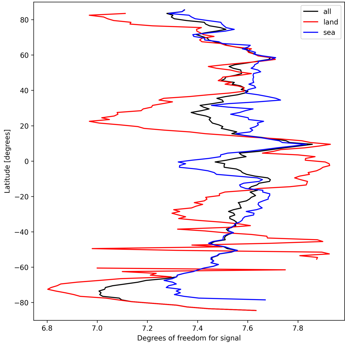
Figure 11: Zonal average of “Degrees of freedom for signal” for 2025-09-20 to 2025-09-21.
