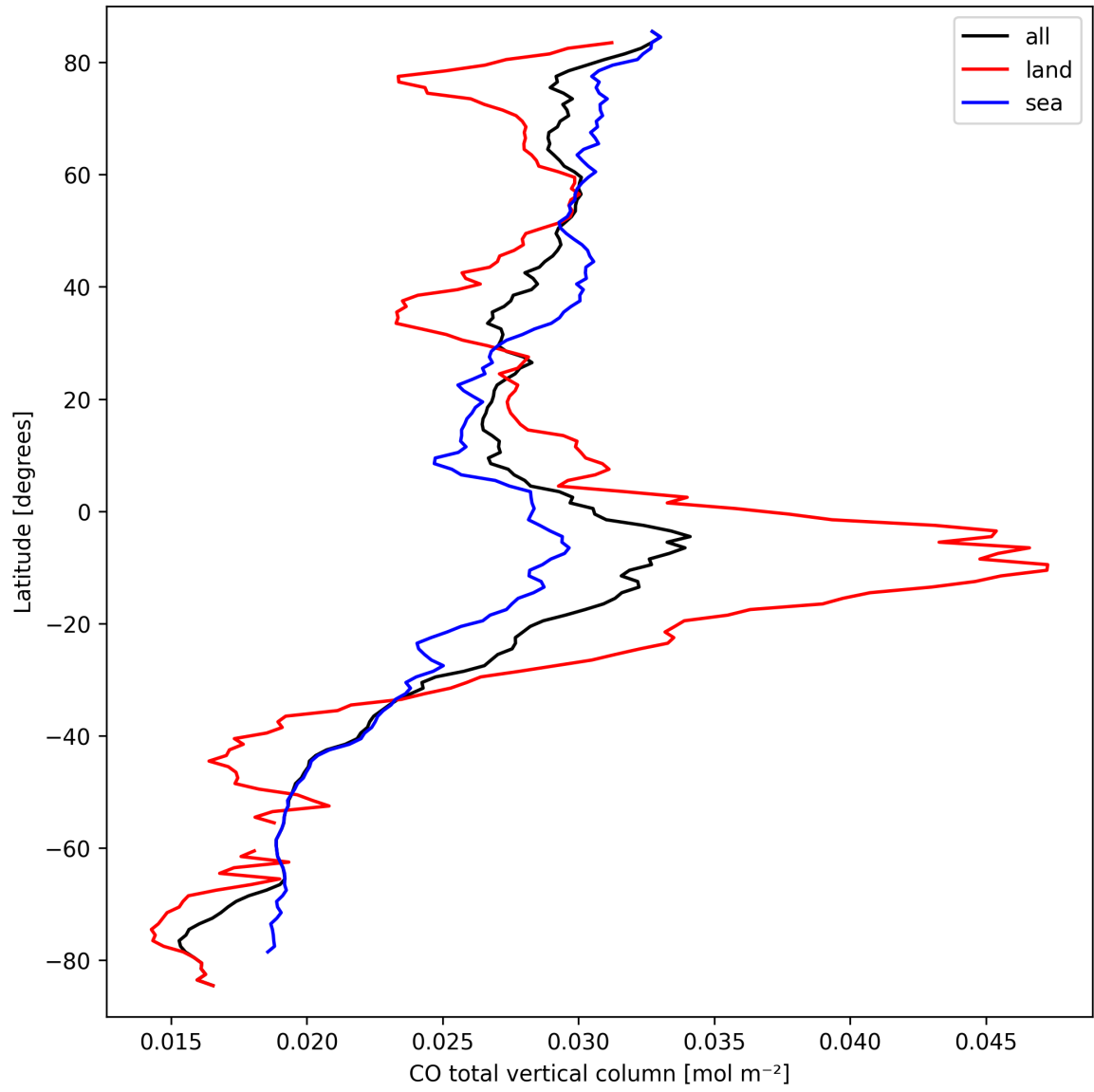
Figure 7: Zonal average of “CO total vertical column” for 2025-09-20 to 2025-09-21.
