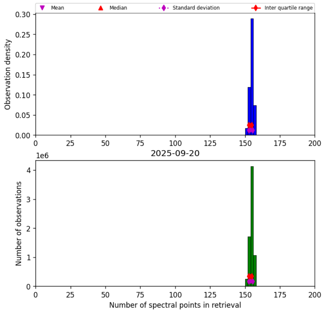
Figure 16: Histogram of “Number of spectral points in retrieval” for 2025-09-20 to 2025-09-21
