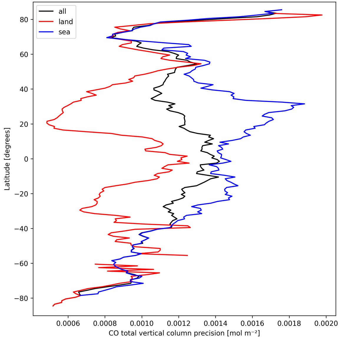
Figure 8: Zonal average of “CO total vertical column precision” for 2025-09-20 to 2025-09-21.
