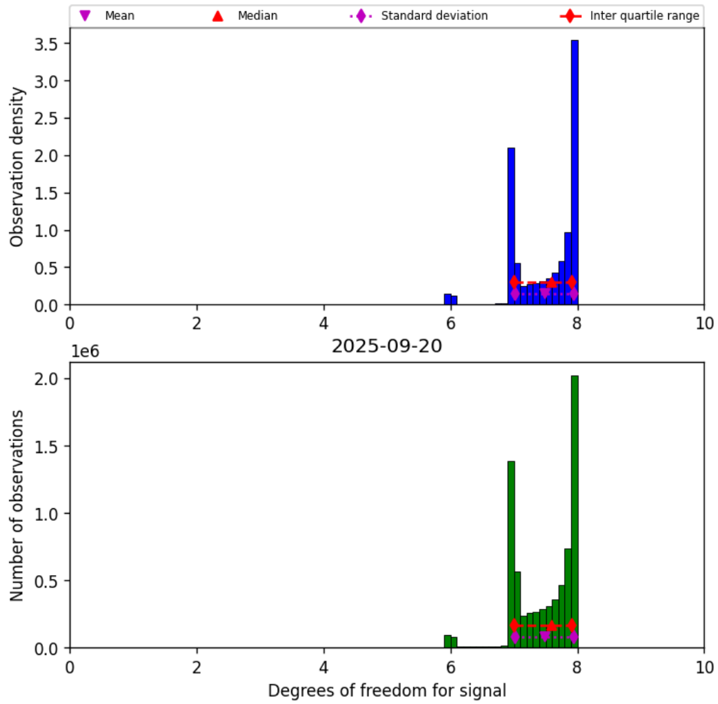
Figure 18: Histogram of “Degrees of freedom for signal” for 2025-09-20 to 2025-09-21
