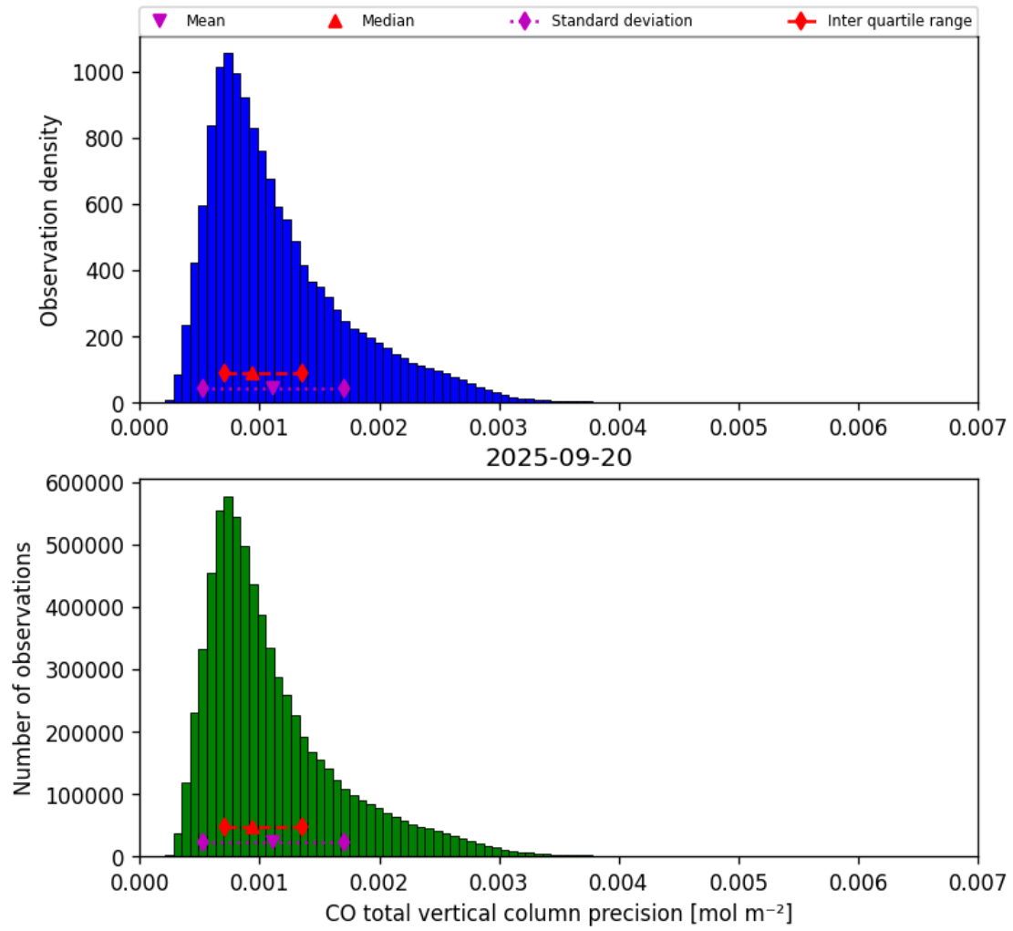
Figure 15: Histogram of “CO total vertical column precision” for 2025-09-20 to 2025-09-21
