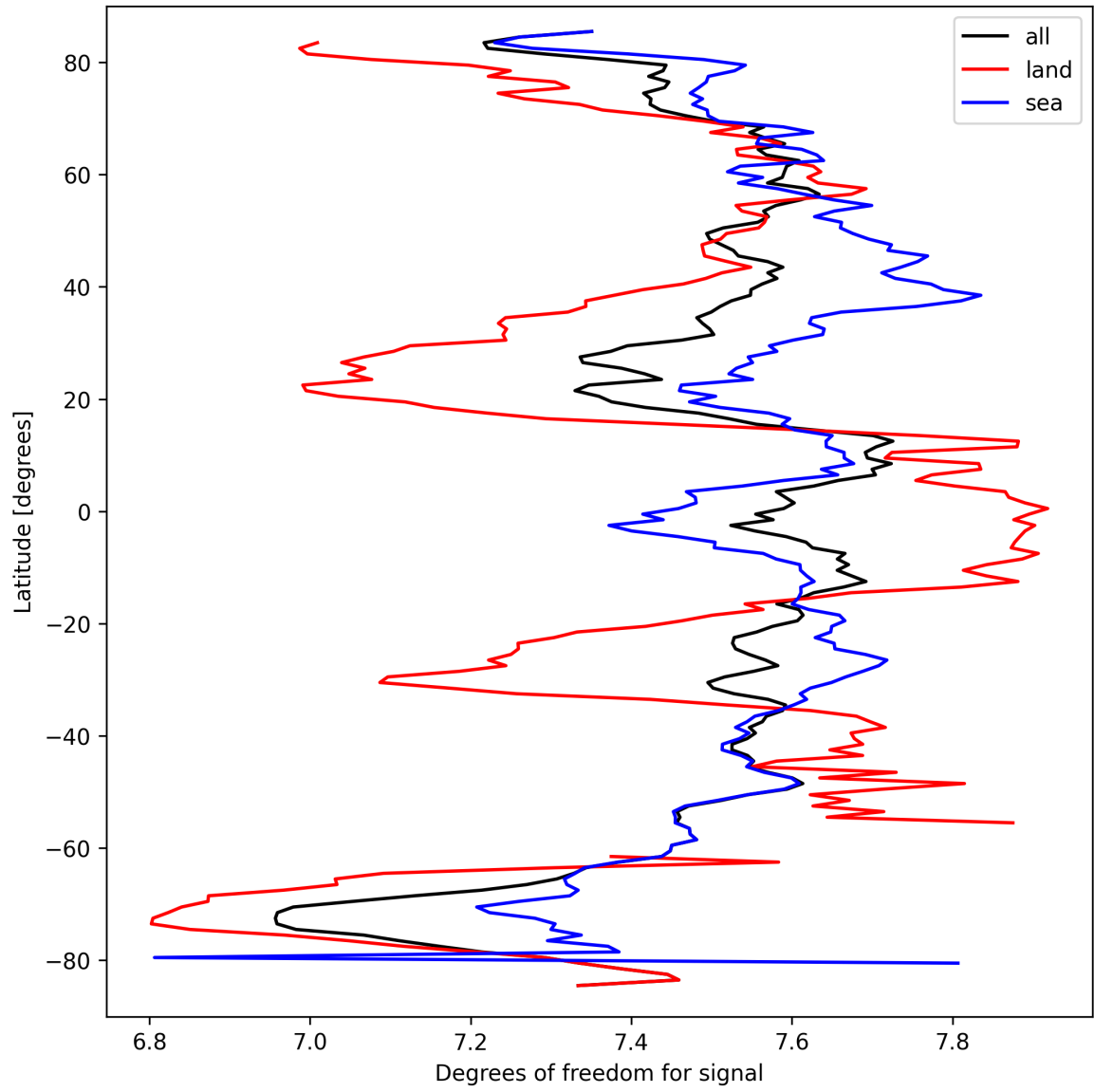
Figure 11: Zonal average of “Degrees of freedom for signal” for 2025-09-21 to 2025-09-22.
