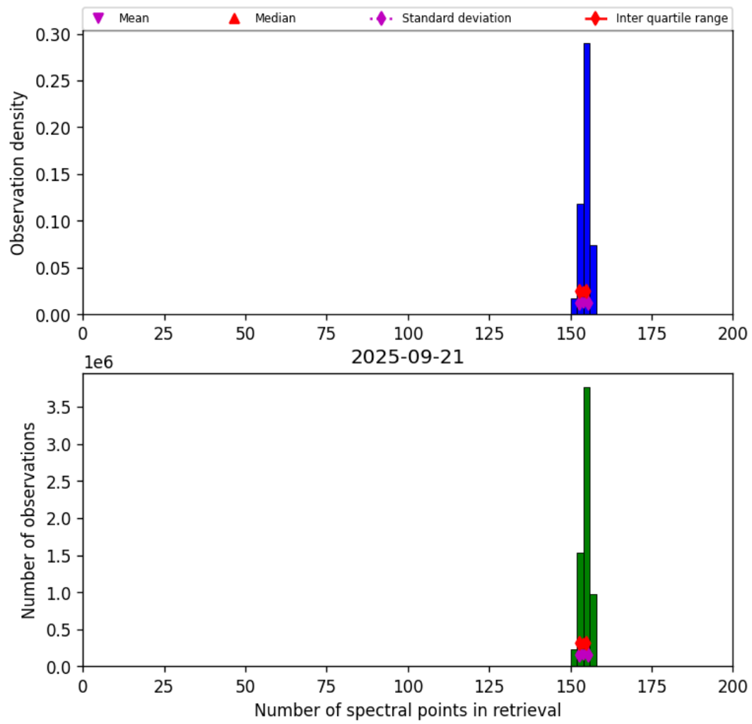
Figure 16: Histogram of “Number of spectral points in retrieval” for 2025-09-21 to 2025-09-22
