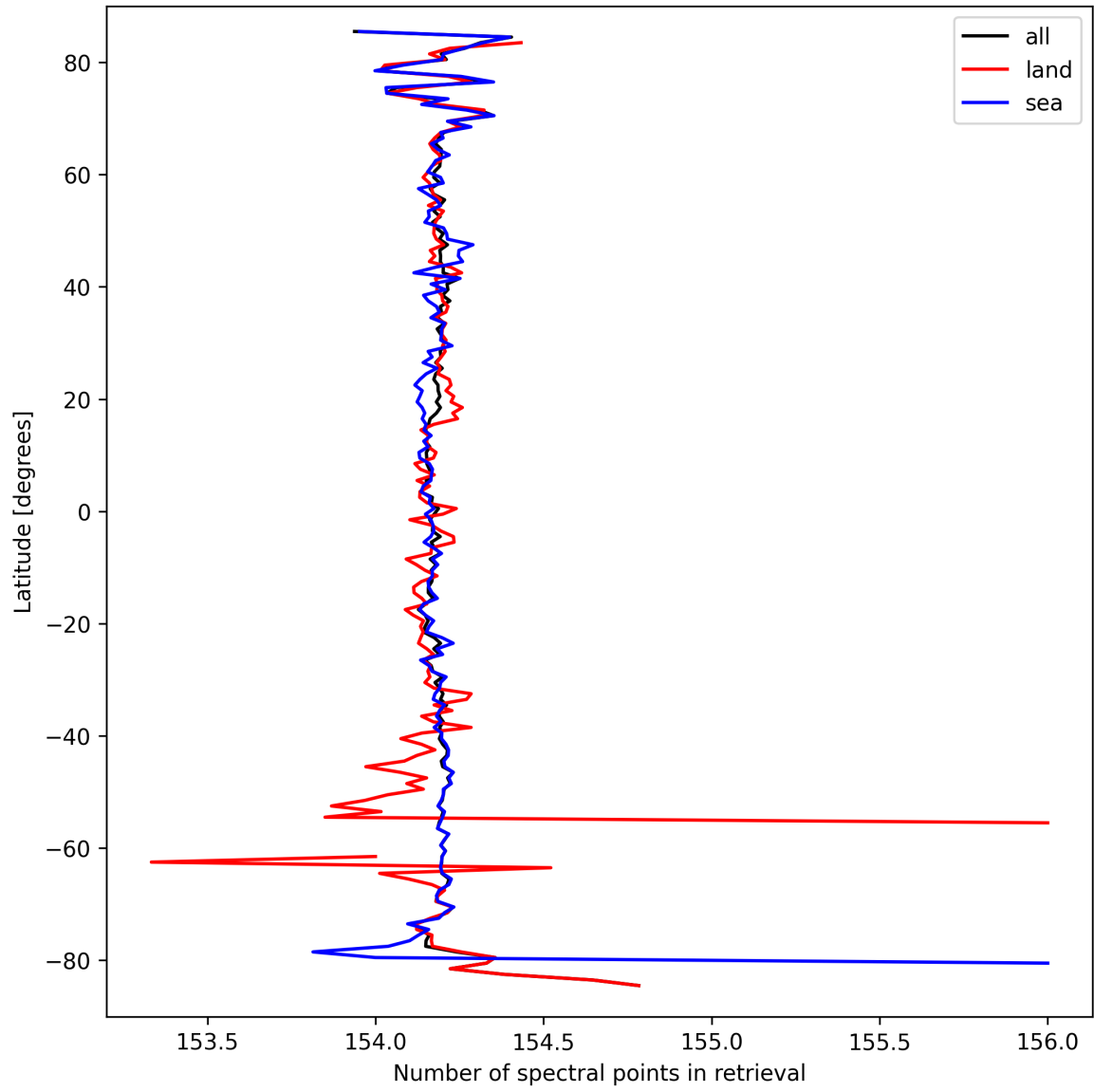
Figure 9: Zonal average of “Number of spectral points in retrieval” for 2025-09-21 to 2025-09-22.
