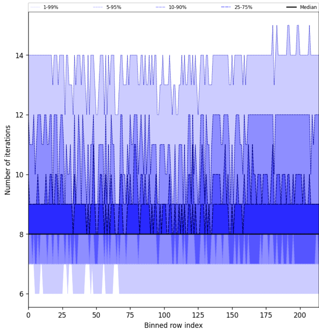
Figure 26: Along track statistics of “Number of iterations” for 2025-09-21 to 2025-09-22
