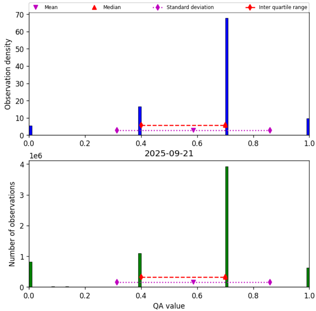
Figure 13: Histogram of “QA value” for 2025-09-21 to 2025-09-22
