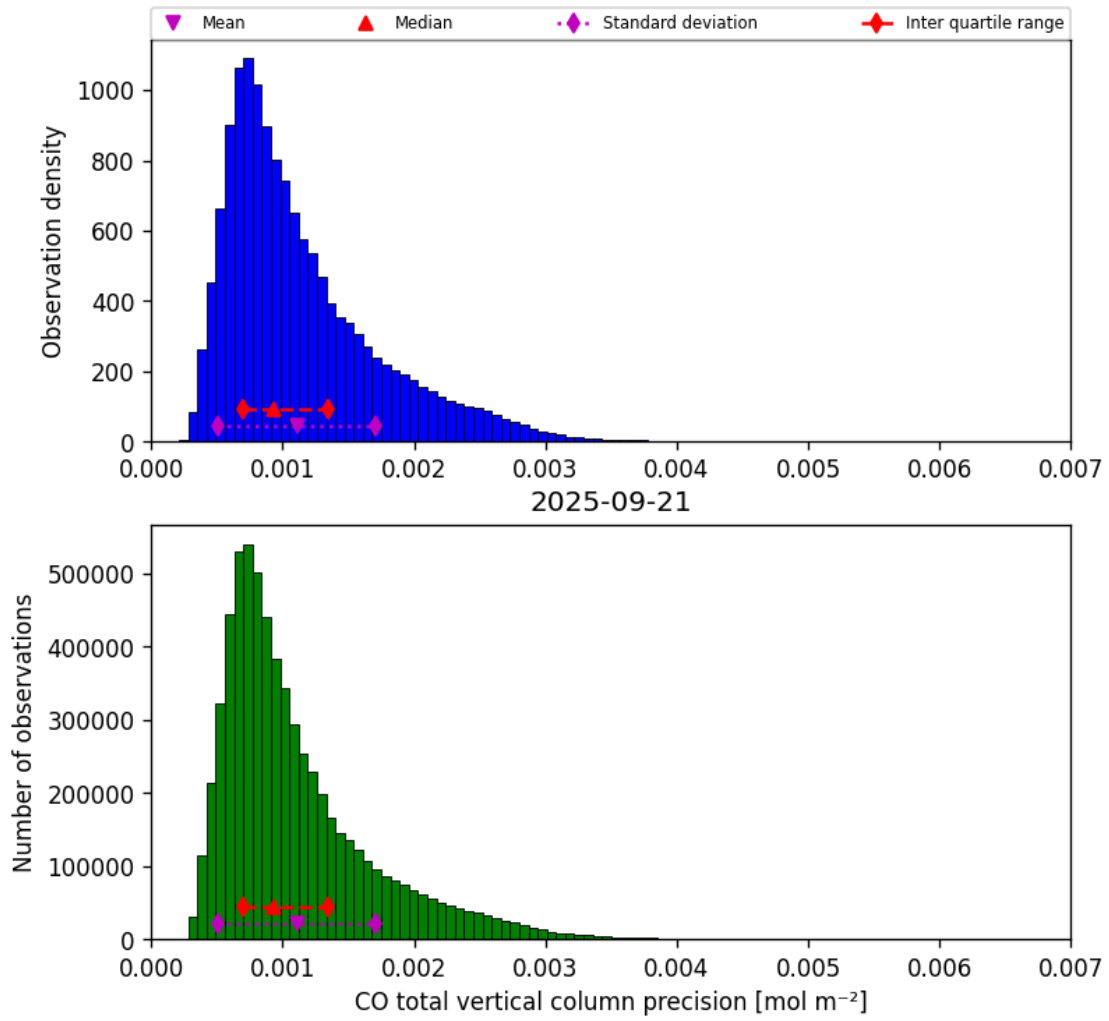
Figure 15: Histogram of “CO total vertical column precision” for 2025-09-21 to 2025-09-22
