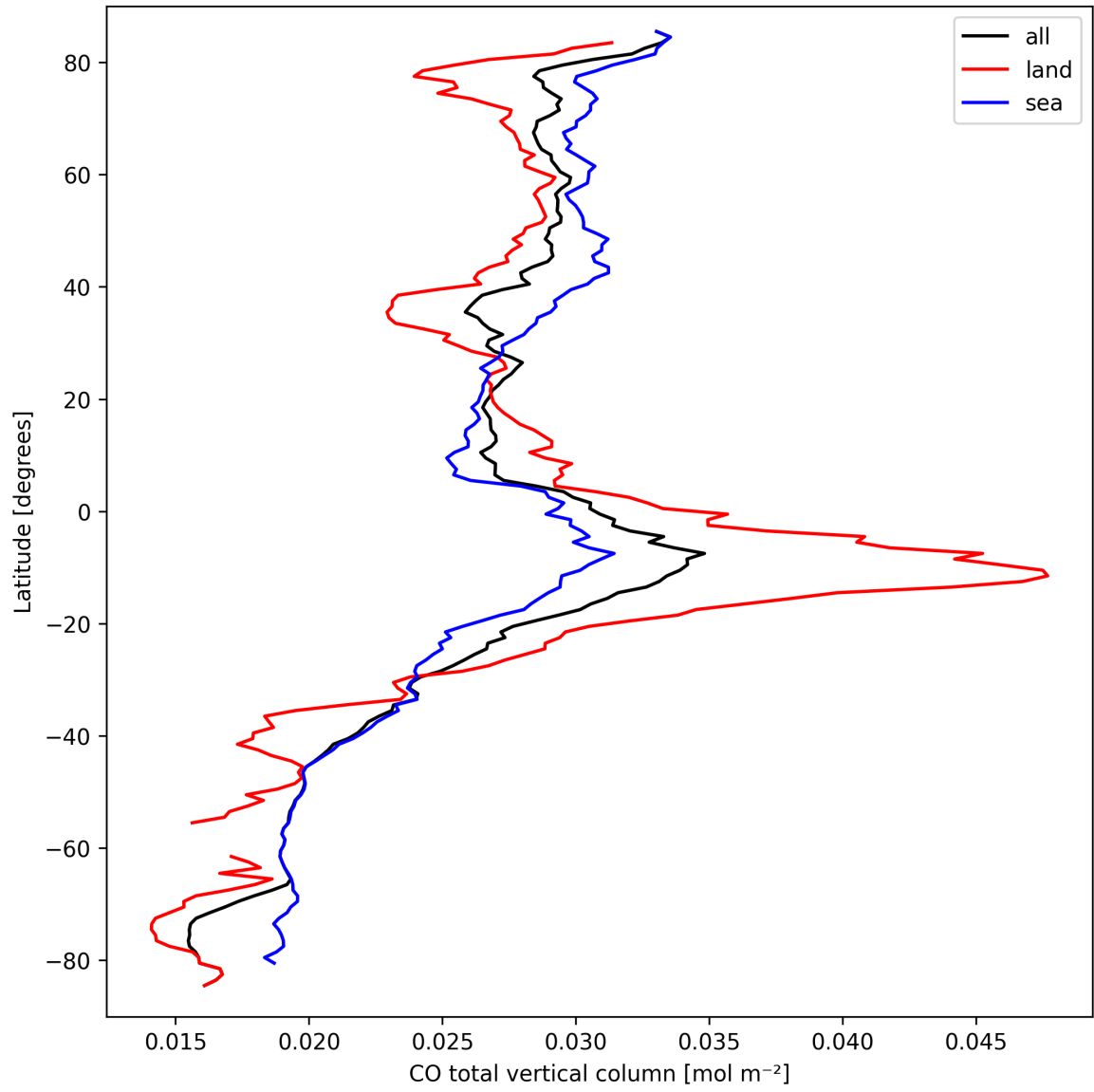
Figure 7: Zonal average of “CO total vertical column” for 2025-09-21 to 2025-09-22.
