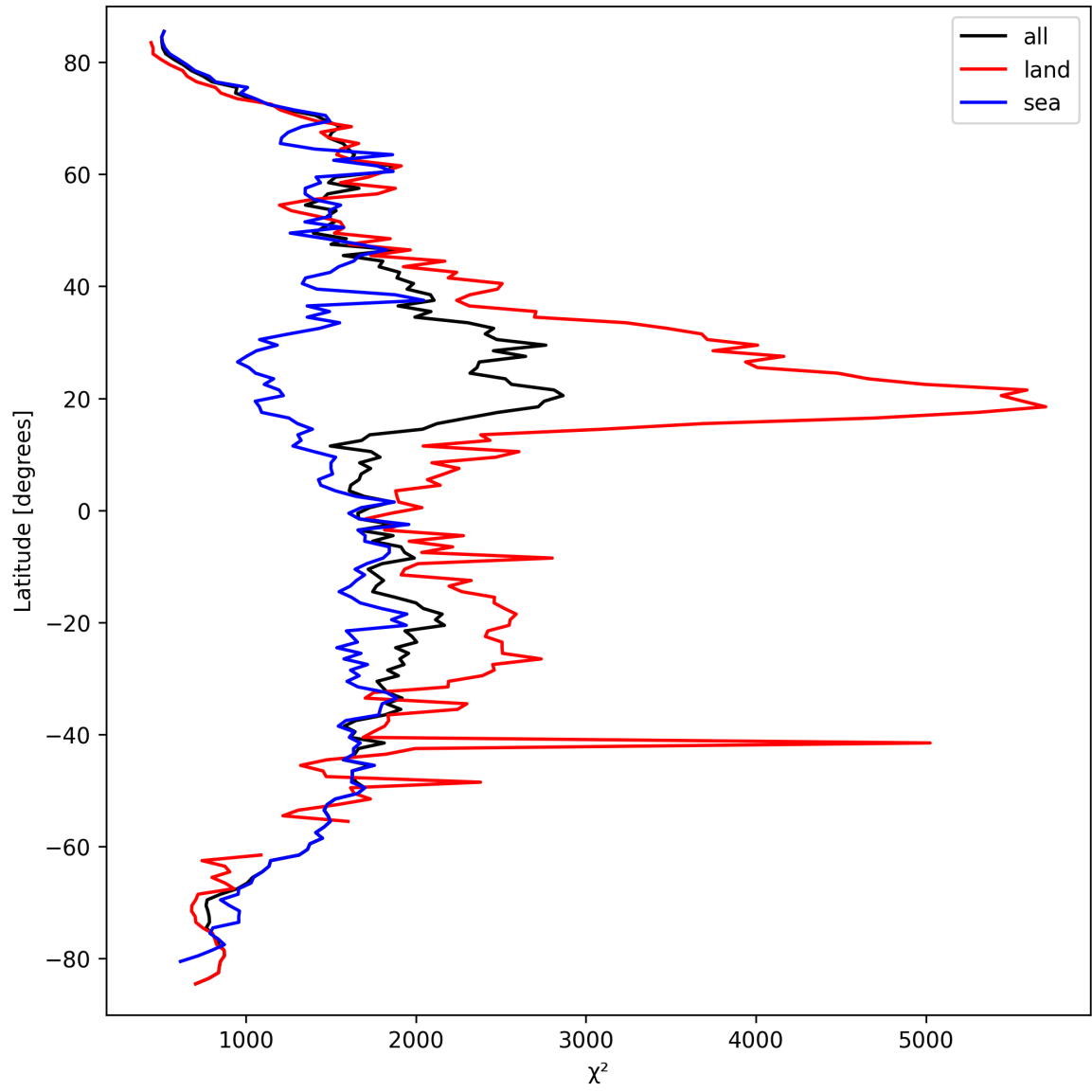
Figure 10: Zonal average of “ \chi^2 ” for 2025-09-21 to 2025-09-22.
