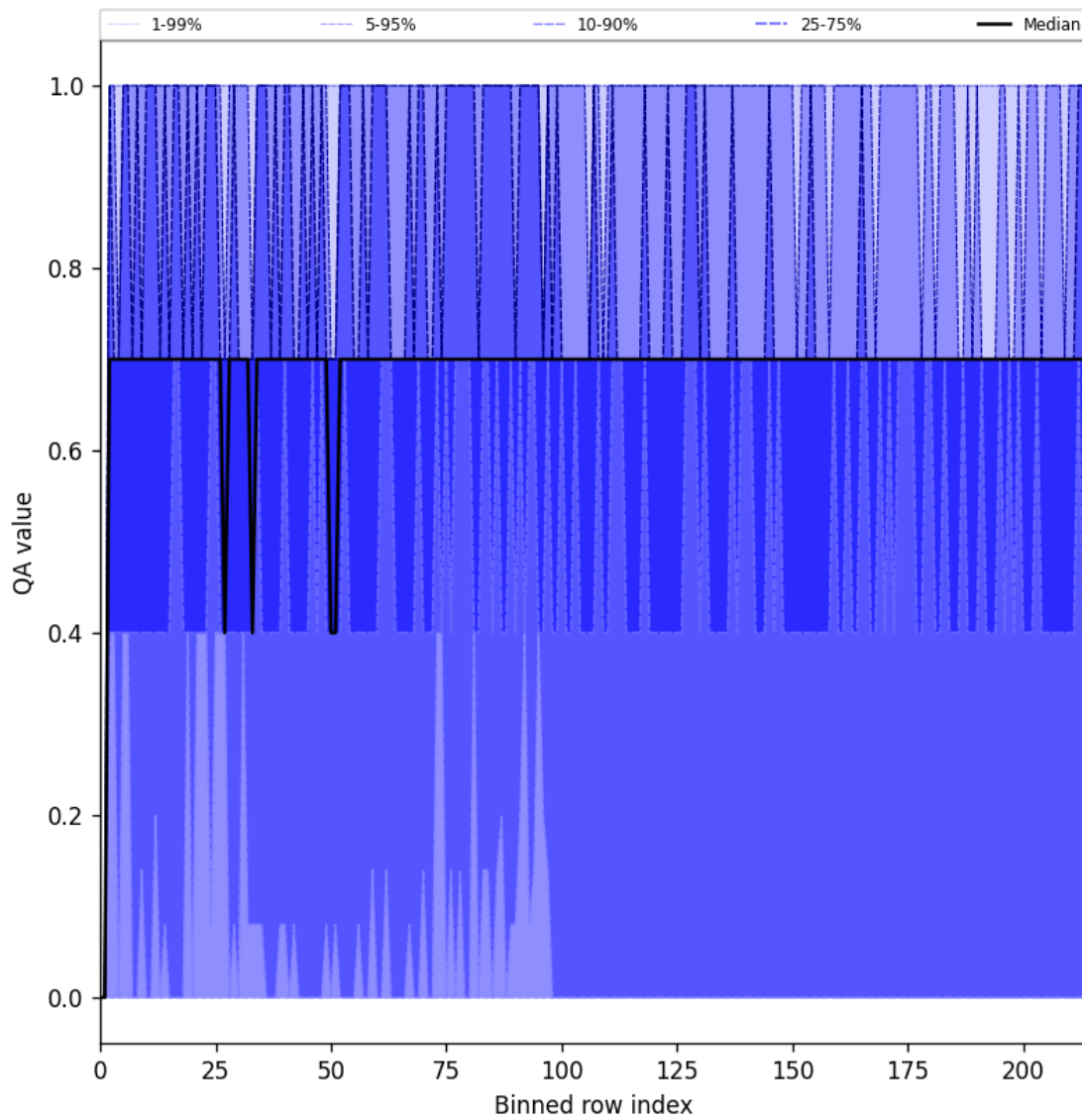
Figure 20: Along track statistics of “QA value” for 2025-09-21 to 2025-09-22
