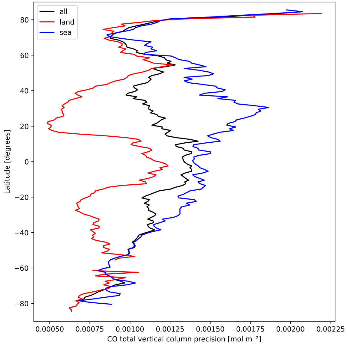
Figure 8: Zonal average of “CO total vertical column precision” for 2025-09-21 to 2025-09-22.
