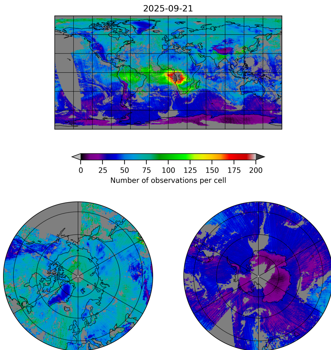
Figure 5: Map of the number of observations for 2025-09-21 to 2025-09-22
