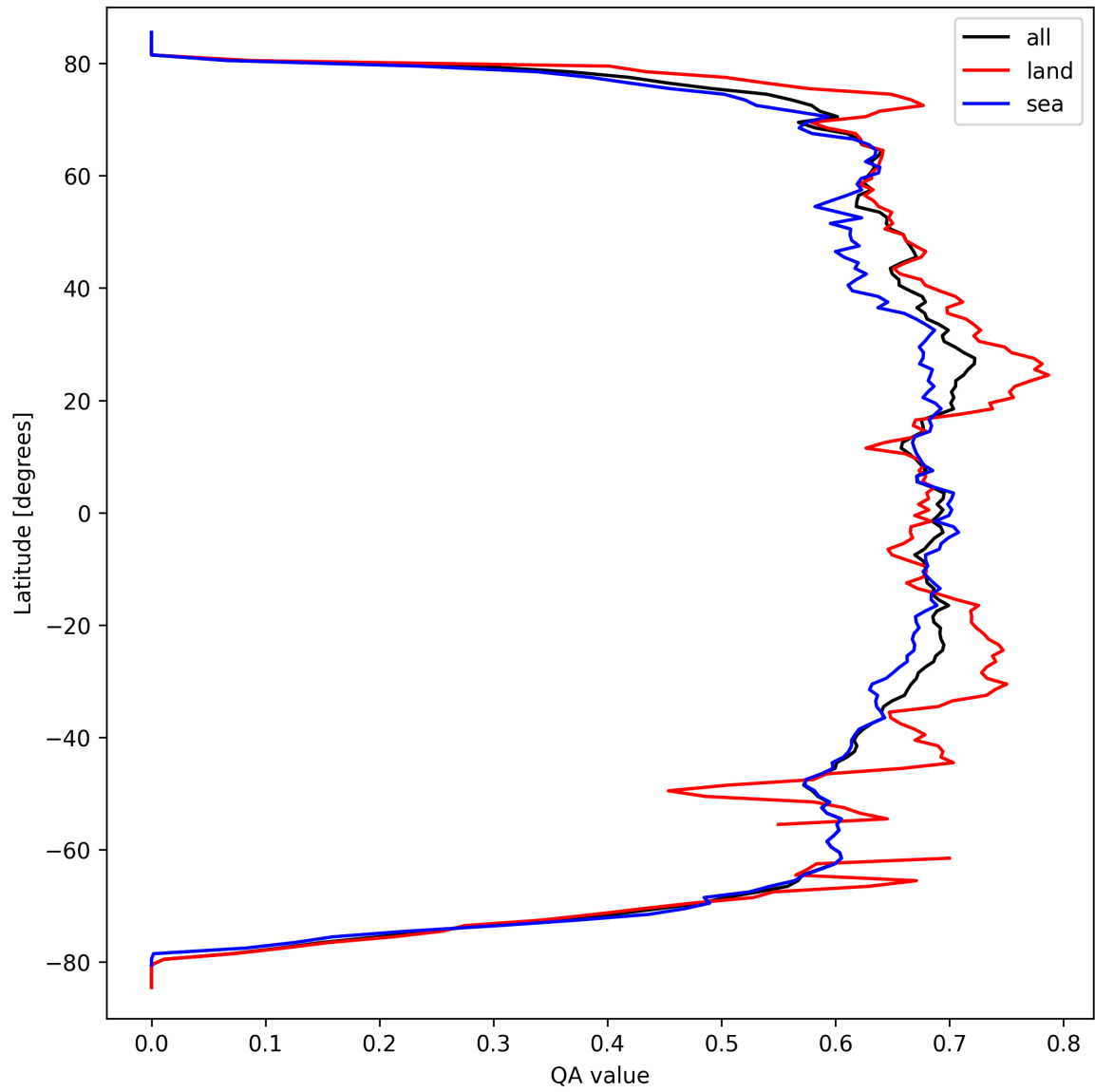
Figure 6: Zonal average of “QA value” for 2025-09-21 to 2025-09-22.
