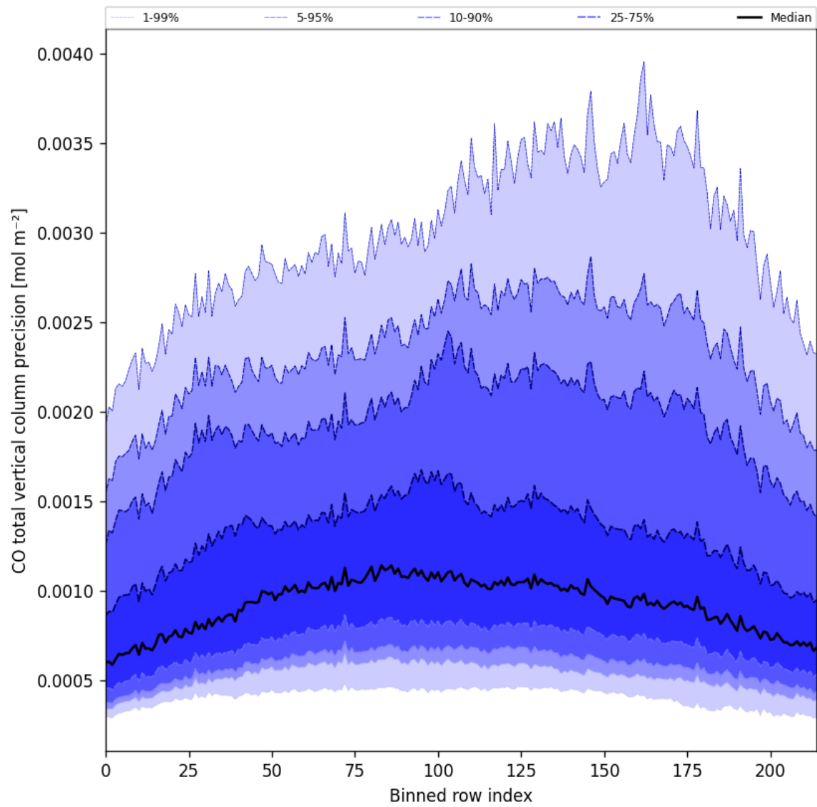
Figure 22: Along track statistics of “CO total vertical column precision” for 2025-09-21 to 2025-09-22
