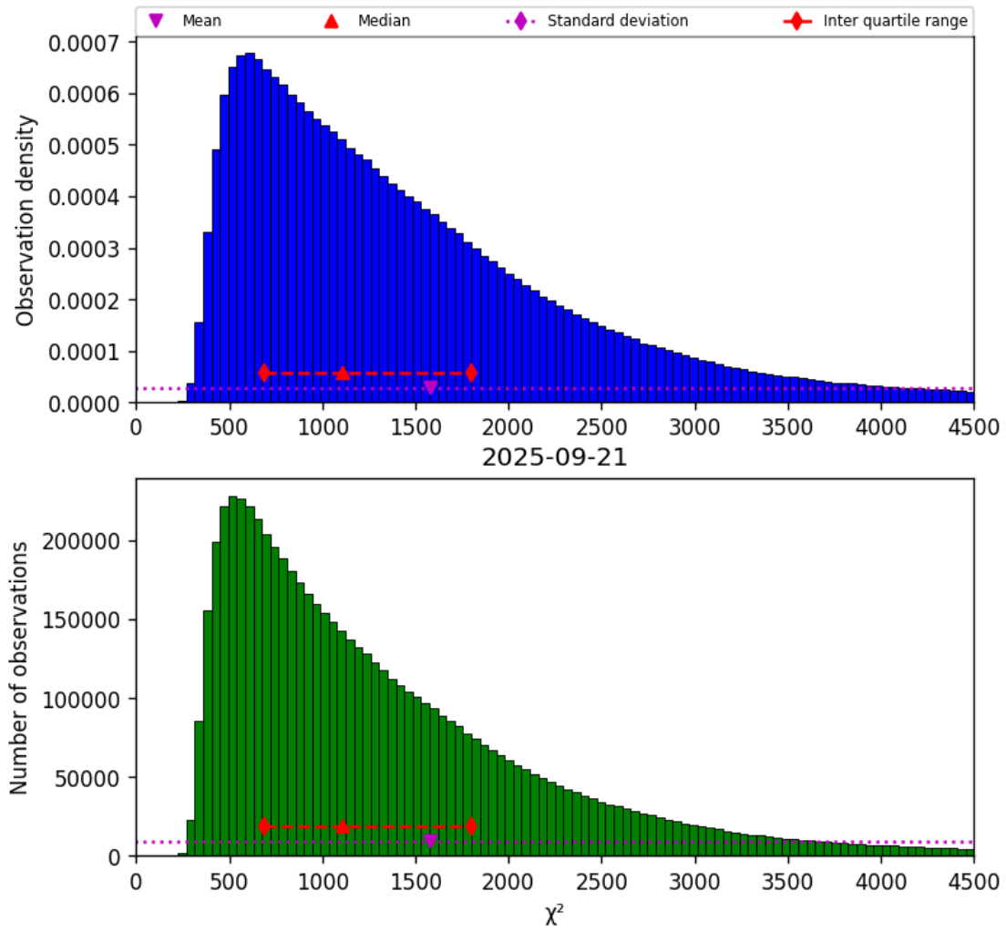
Figure 17: Histogram of “ \chi^2 ” for 2025-09-21 to 2025-09-22
