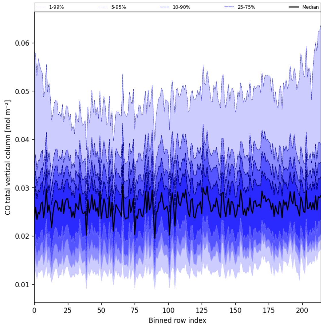
Figure 21: Along track statistics of “CO total vertical column” for 2025-09-21 to 2025-09-22
