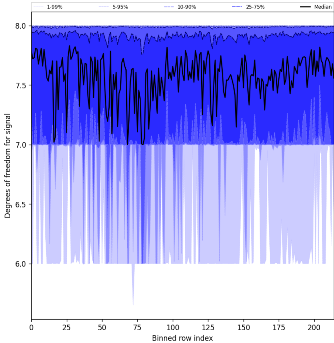
Figure 25: Along track statistics of “Degrees of freedom for signal” for 2025-09-21 to 2025-09-22
