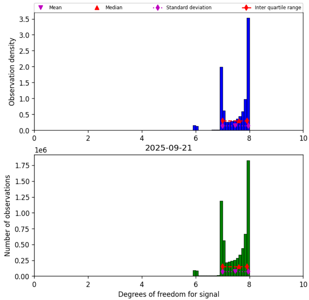
Figure 18: Histogram of “Degrees of freedom for signal” for 2025-09-21 to 2025-09-22
