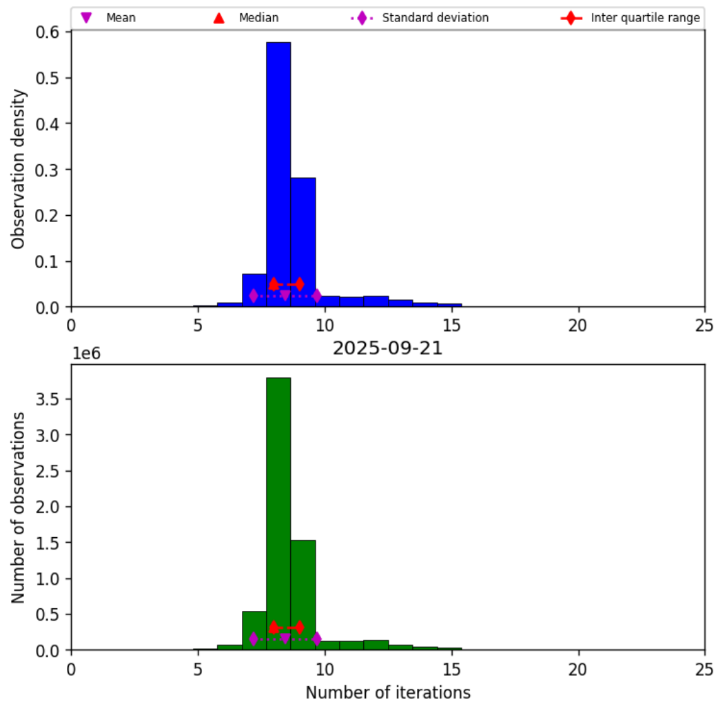
Figure 19: Histogram of “Number of iterations” for 2025-09-21 to 2025-09-22
