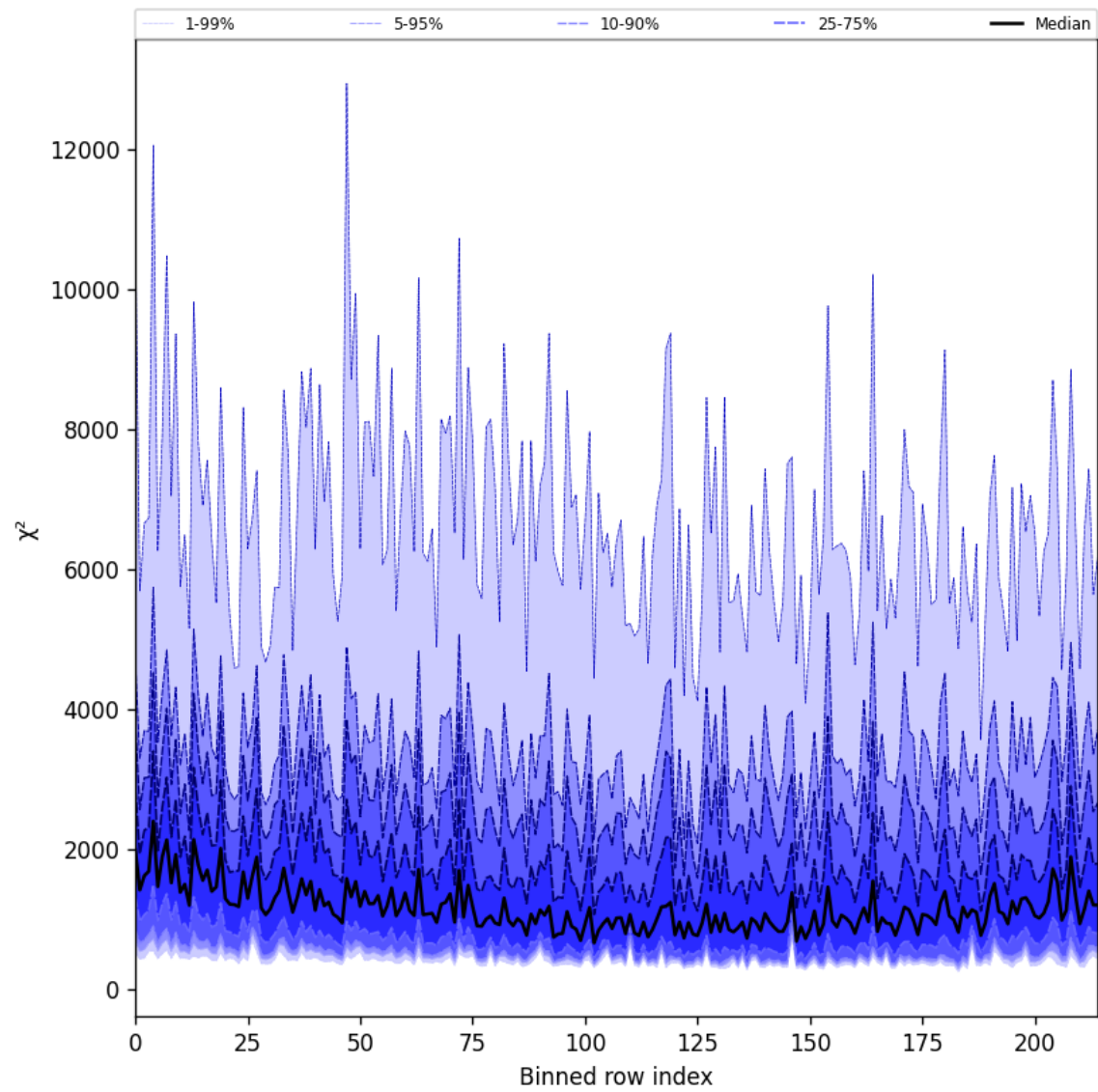
Figure 24: Along track statistics of “ \chi^2 ” for 2025-09-21 to 2025-09-22
