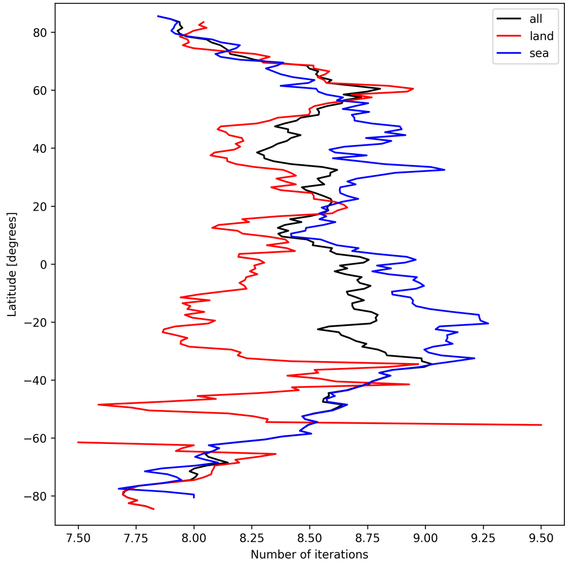
Figure 12: Zonal average of “Number of iterations” for 2025-09-21 to 2025-09-22.
