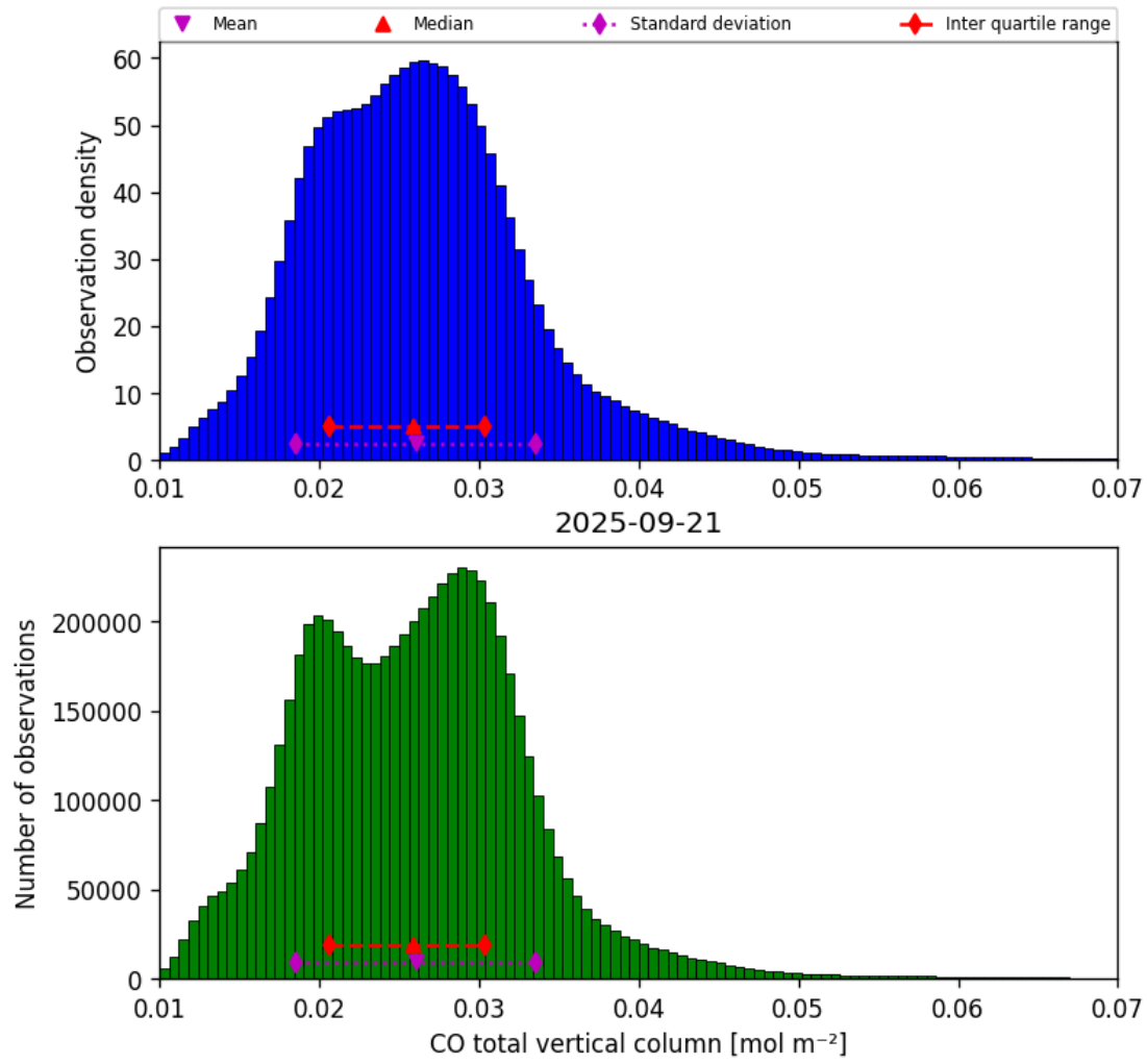
Figure 14: Histogram of “CO total vertical column” for 2025-09-21 to 2025-09-22
