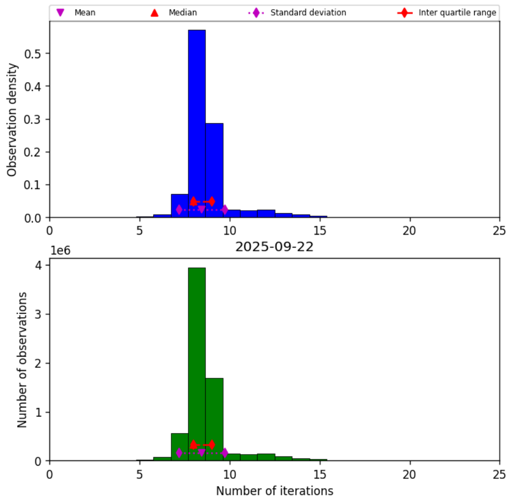
Figure 19: Histogram of “Number of iterations” for 2025-09-22 to 2025-09-23
