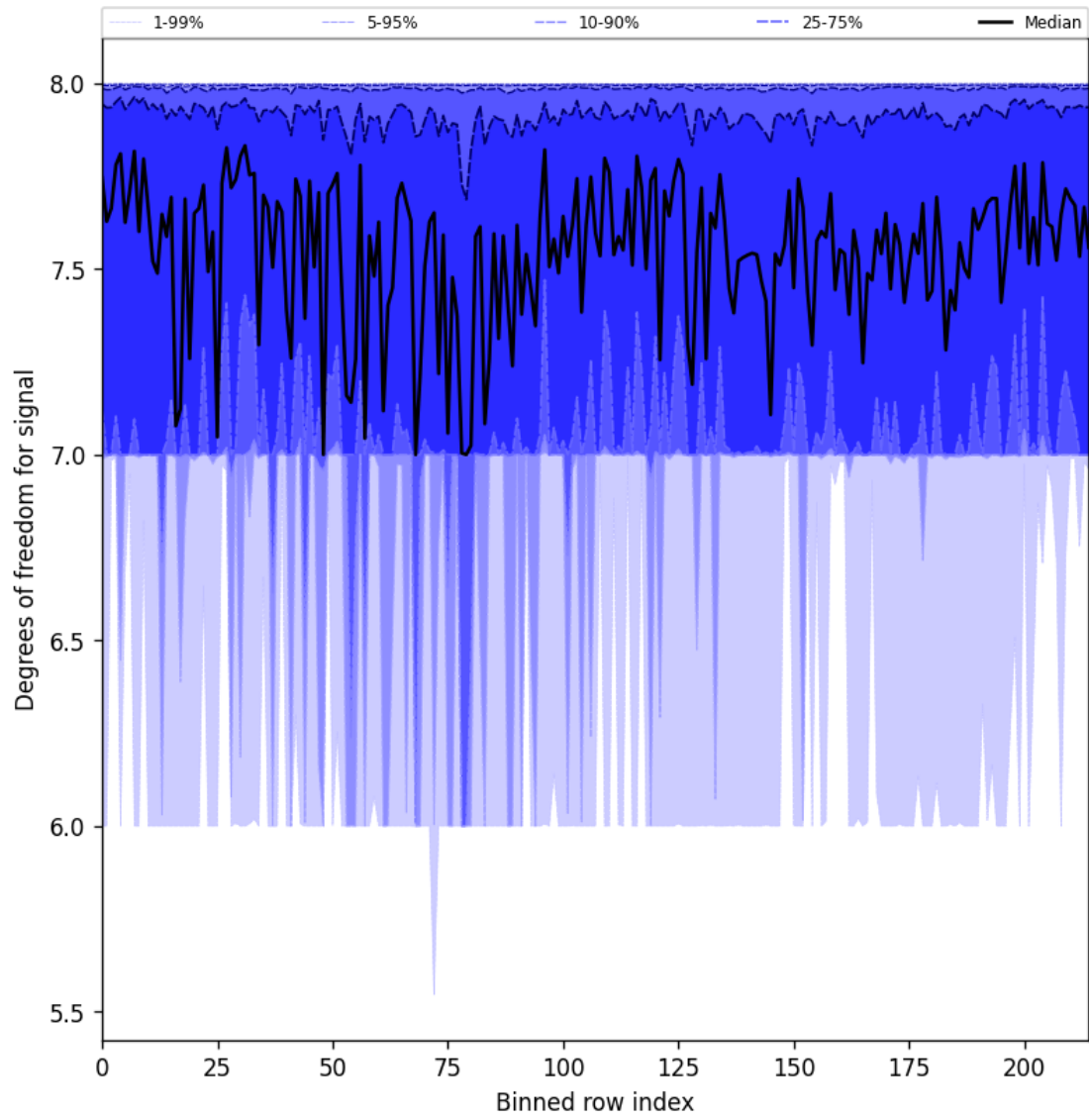
Figure 25: Along track statistics of “Degrees of freedom for signal” for 2025-09-22 to 2025-09-23
