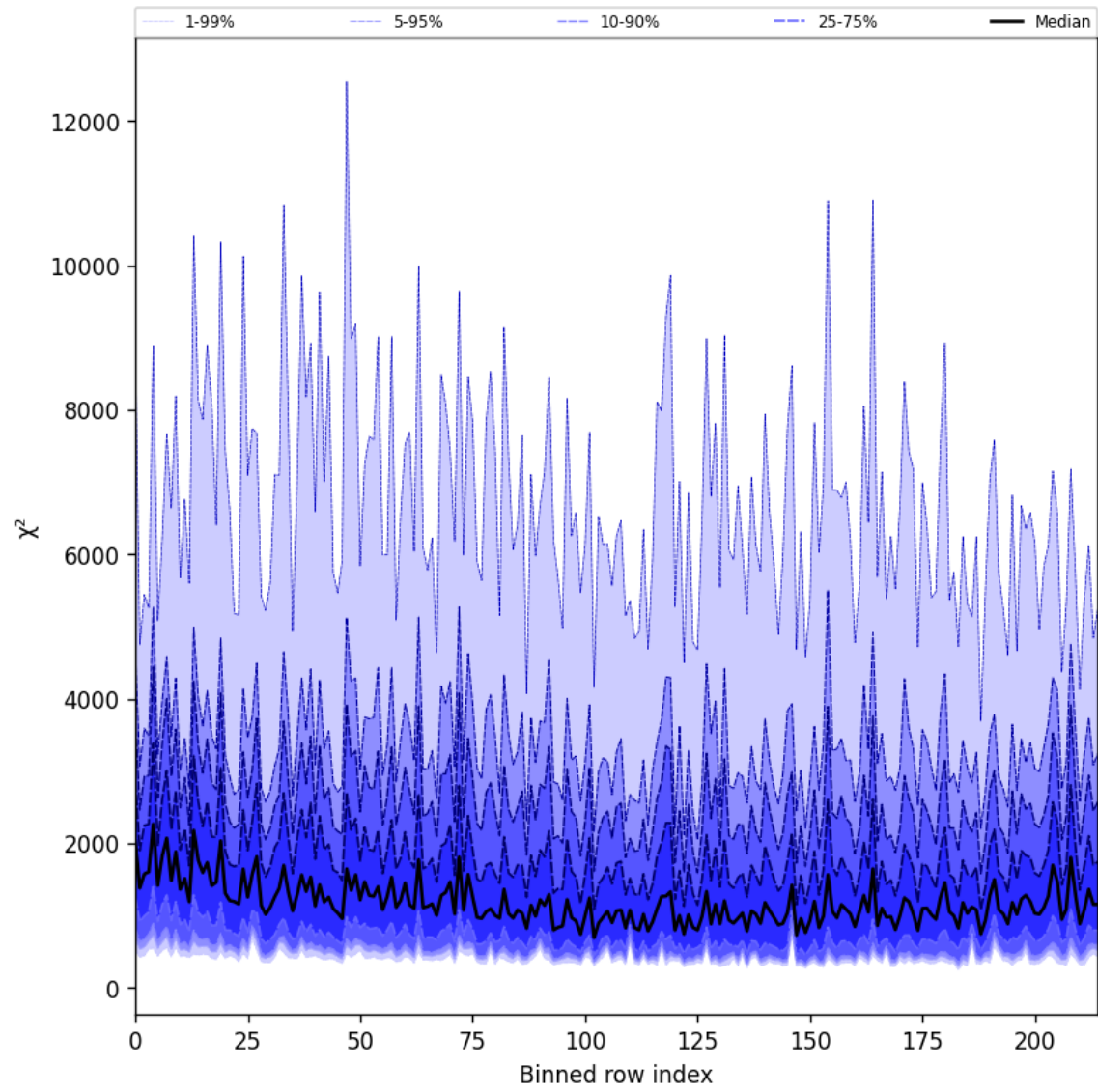
Figure 24: Along track statistics of “ \chi^2 ” for 2025-09-22 to 2025-09-23
