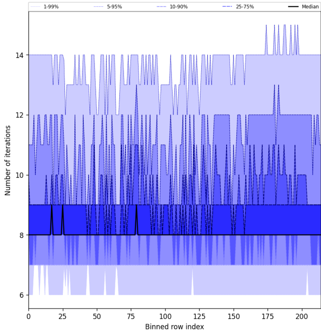
Figure 26: Along track statistics of “Number of iterations” for 2025-09-22 to 2025-09-23
