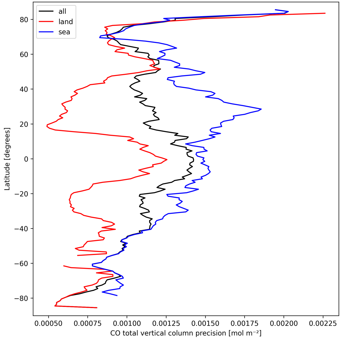
Figure 8: Zonal average of “CO total vertical column precision” for 2025-09-22 to 2025-09-23.
