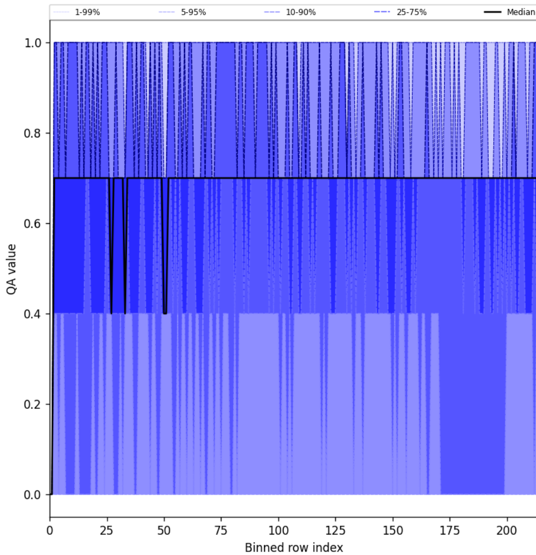
Figure 20: Along track statistics of “QA value” for 2025-09-22 to 2025-09-23
