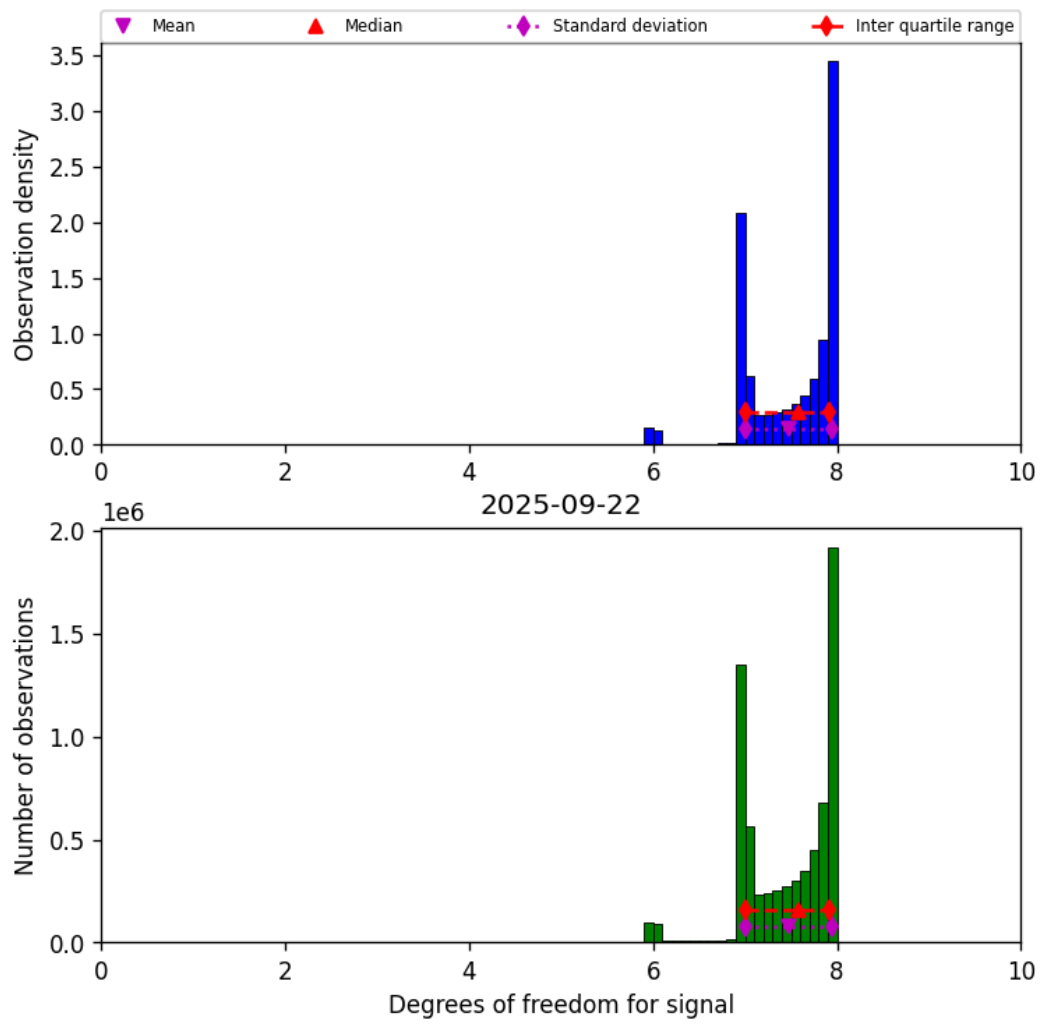
Figure 18: Histogram of “Degrees of freedom for signal” for 2025-09-22 to 2025-09-23
