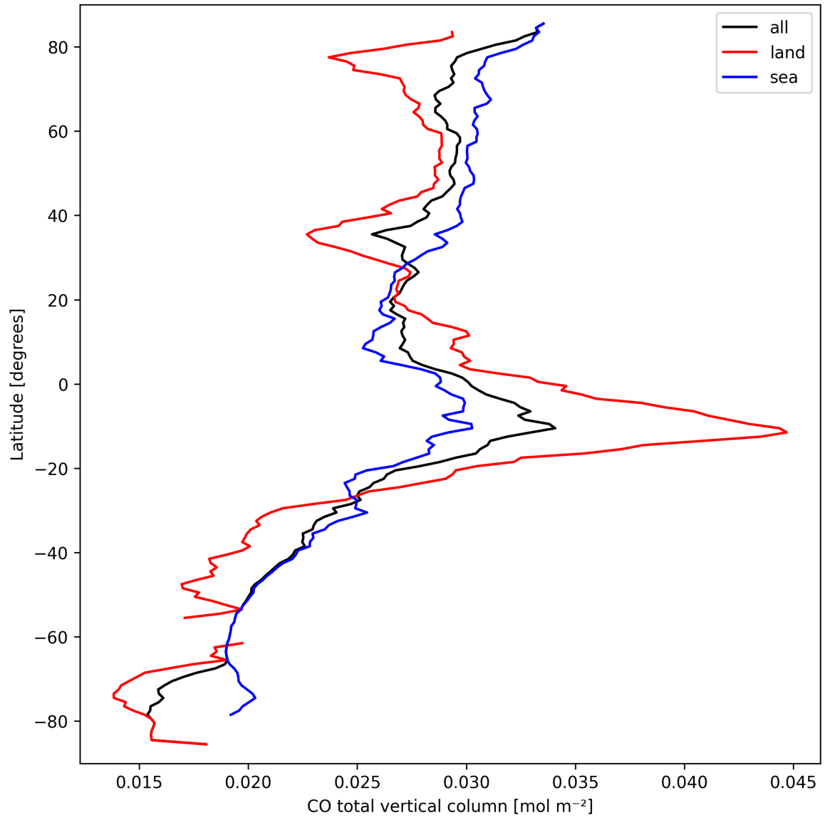
Figure 7: Zonal average of “CO total vertical column” for 2025-09-22 to 2025-09-23.
