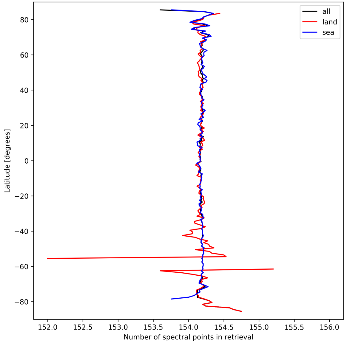
Figure 9: Zonal average of “Number of spectral points in retrieval” for 2025-09-22 to 2025-09-23.
