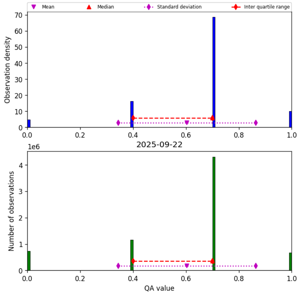
Figure 13: Histogram of “QA value” for 2025-09-22 to 2025-09-23
