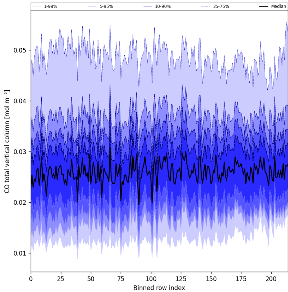
Figure 21: Along track statistics of “CO total vertical column” for 2025-09-22 to 2025-09-23
