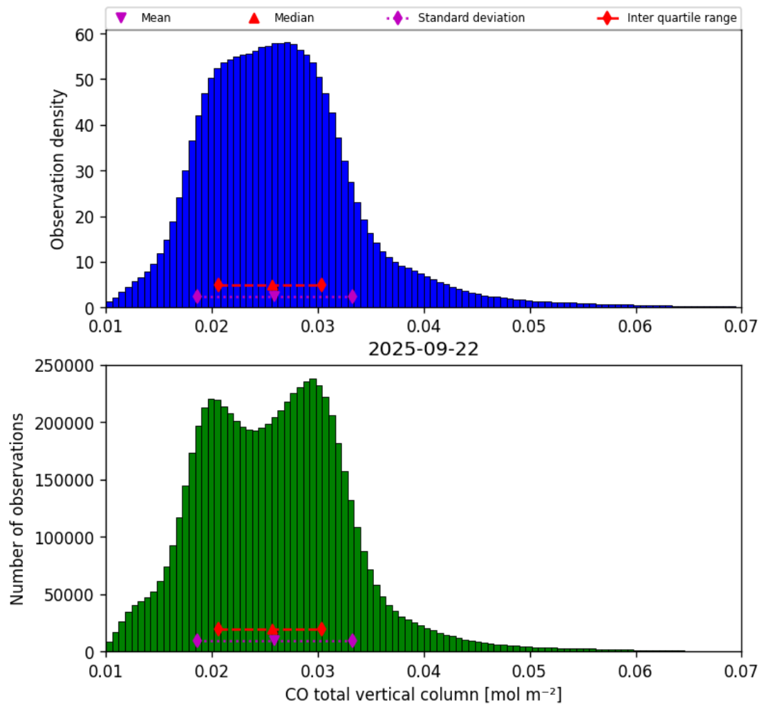
Figure 14: Histogram of “CO total vertical column” for 2025-09-22 to 2025-09-23
