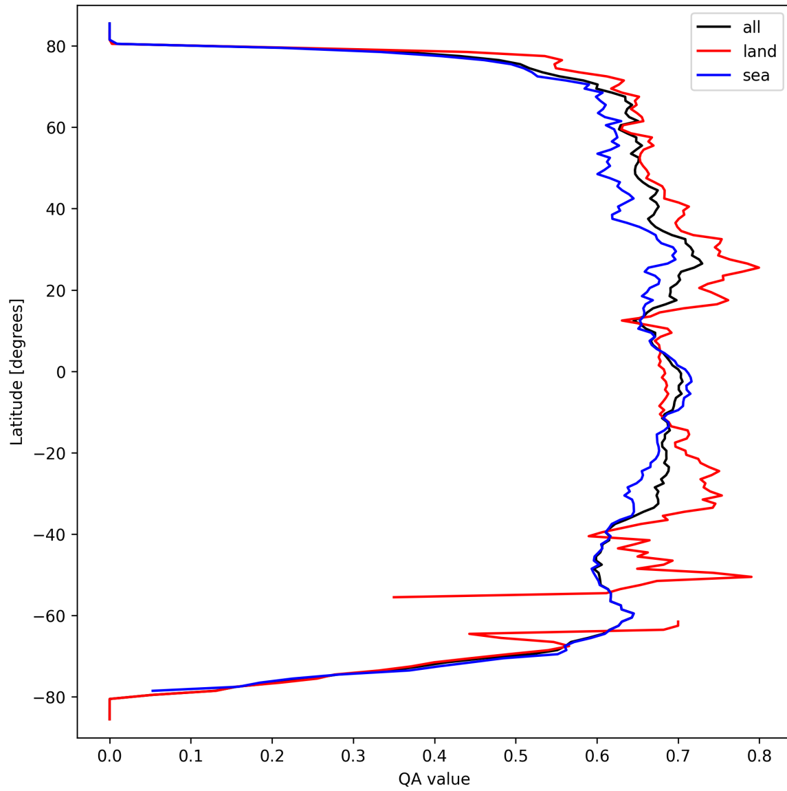
Figure 6: Zonal average of “QA value” for 2025-09-22 to 2025-09-23.
