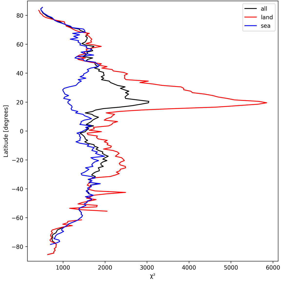
Figure 10: Zonal average of “ \chi^2 ” for 2025-09-22 to 2025-09-23.
