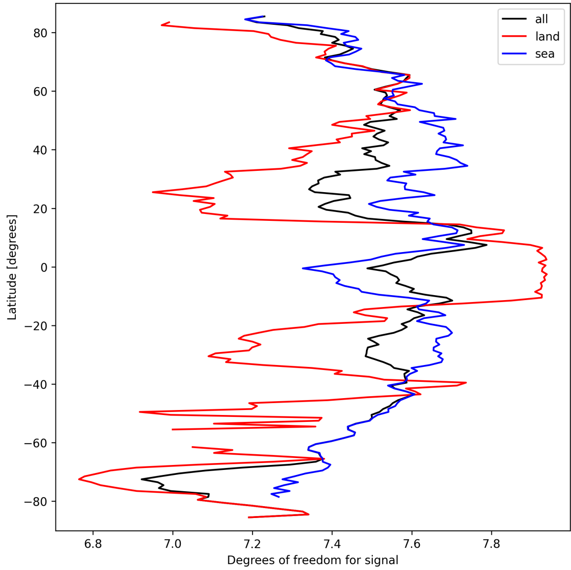
Figure 11: Zonal average of “Degrees of freedom for signal” for 2025-09-22 to 2025-09-23.
