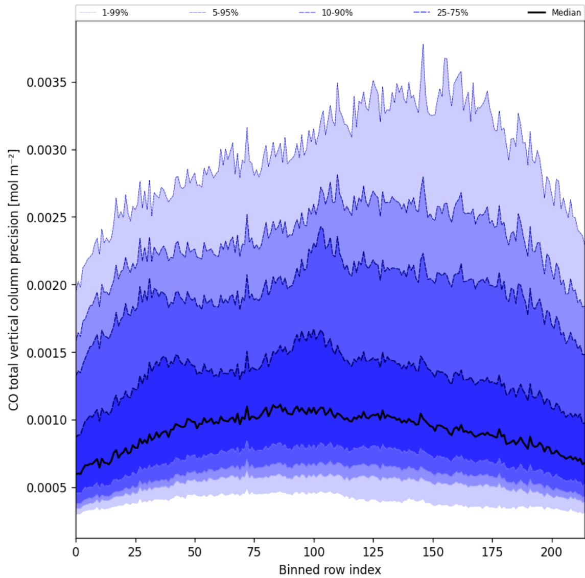
Figure 22: Along track statistics of “CO total vertical column precision” for 2025-09-22 to 2025-09-23
