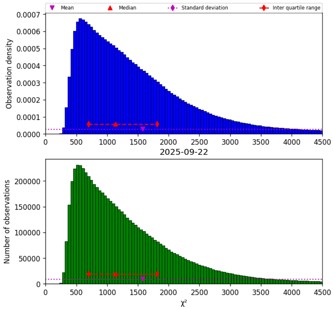
Figure 17: Histogram of " \chi^2 " for 2025-09-22 to 2025-09-23
