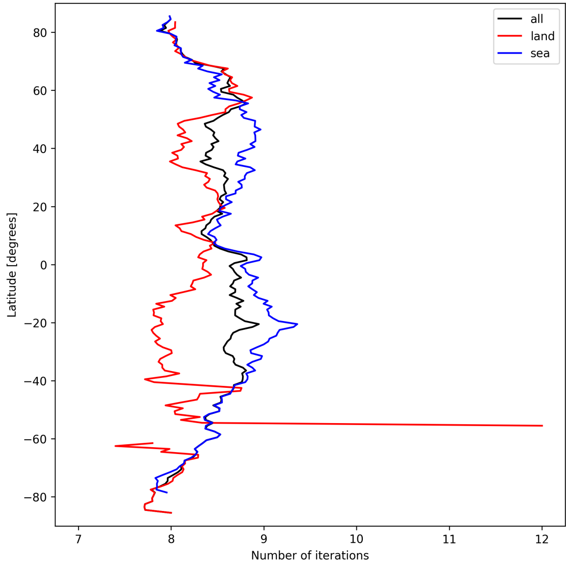
Figure 12: Zonal average of “Number of iterations” for 2025-09-22 to 2025-09-23.
