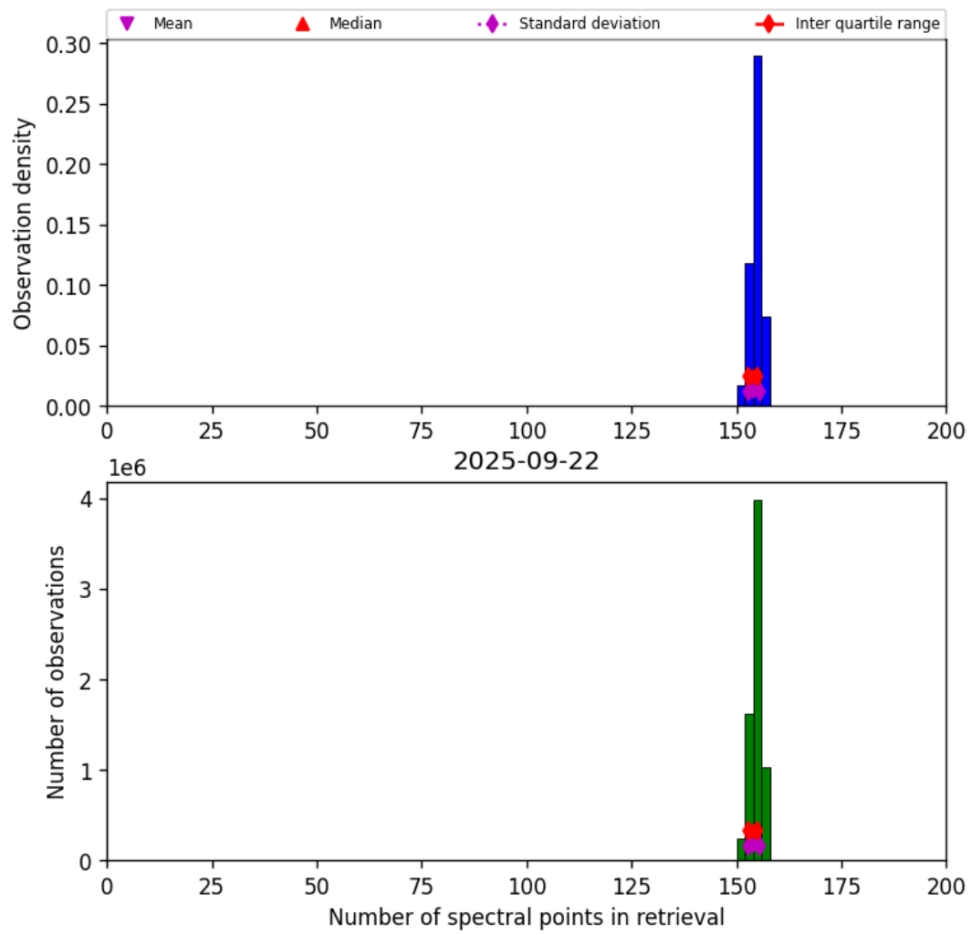
Figure 16: Histogram of “Number of spectral points in retrieval” for 2025-09-22 to 2025-09-23
