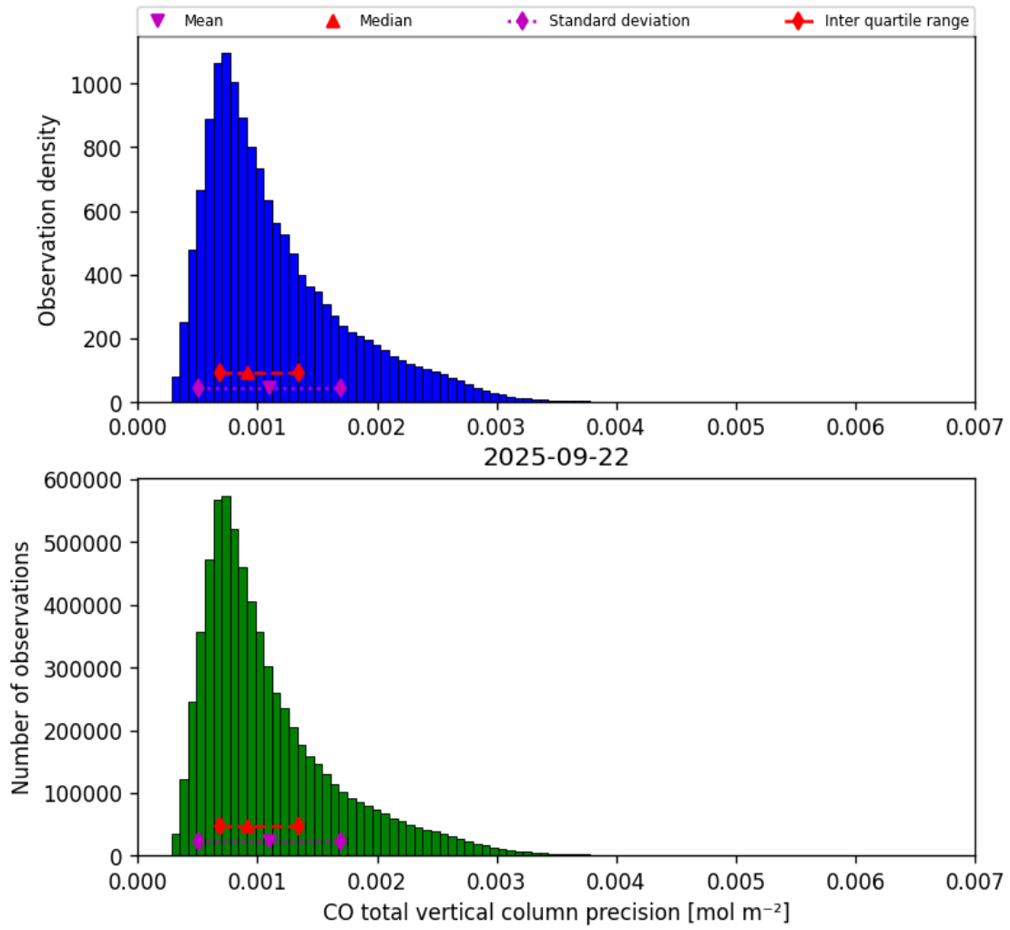
Figure 15: Histogram of “CO total vertical column precision” for 2025-09-22 to 2025-09-23
