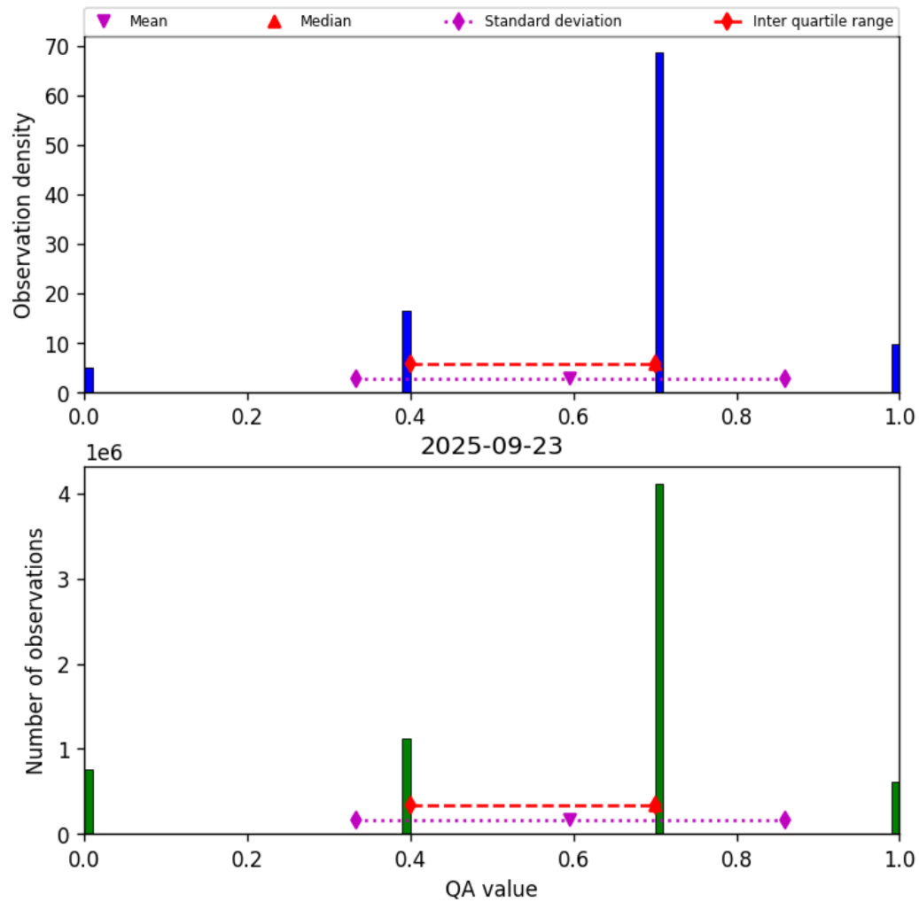
Figure 13: Histogram of “QA value” for 2025-09-23 to 2025-09-23
