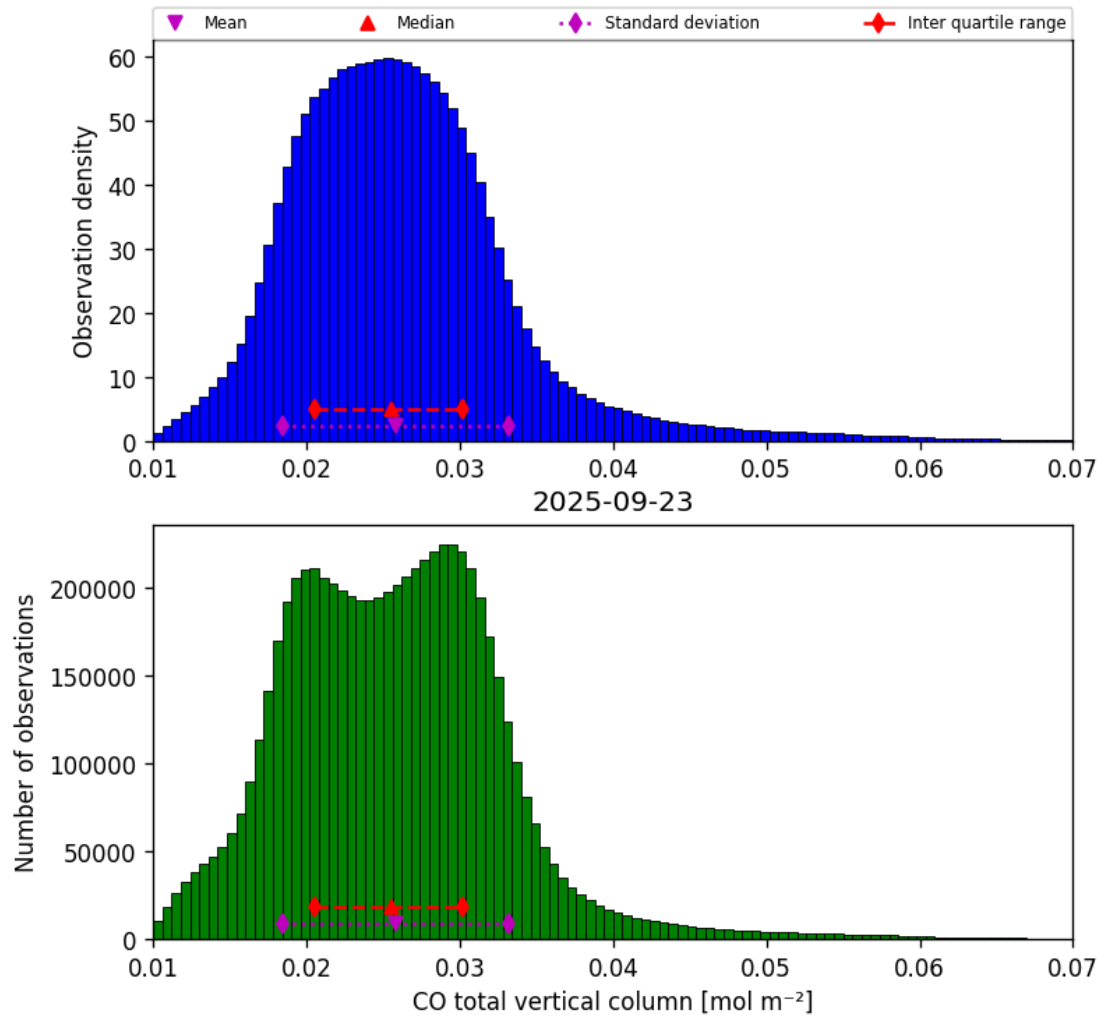
Figure 14: Histogram of “CO total vertical column” for 2025-09-23 to 2025-09-23
