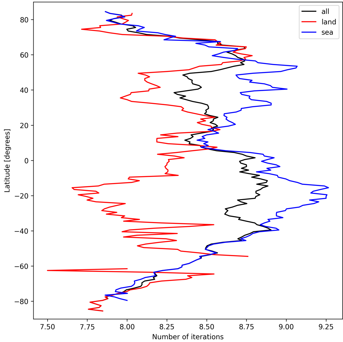
Figure 12: Zonal average of “Number of iterations” for 2025-09-23 to 2025-09-23.
