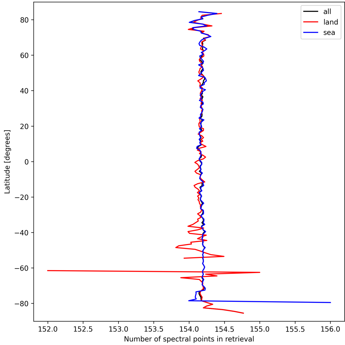
Figure 9: Zonal average of “Number of spectral points in retrieval” for 2025-09-23 to 2025-09-23.
