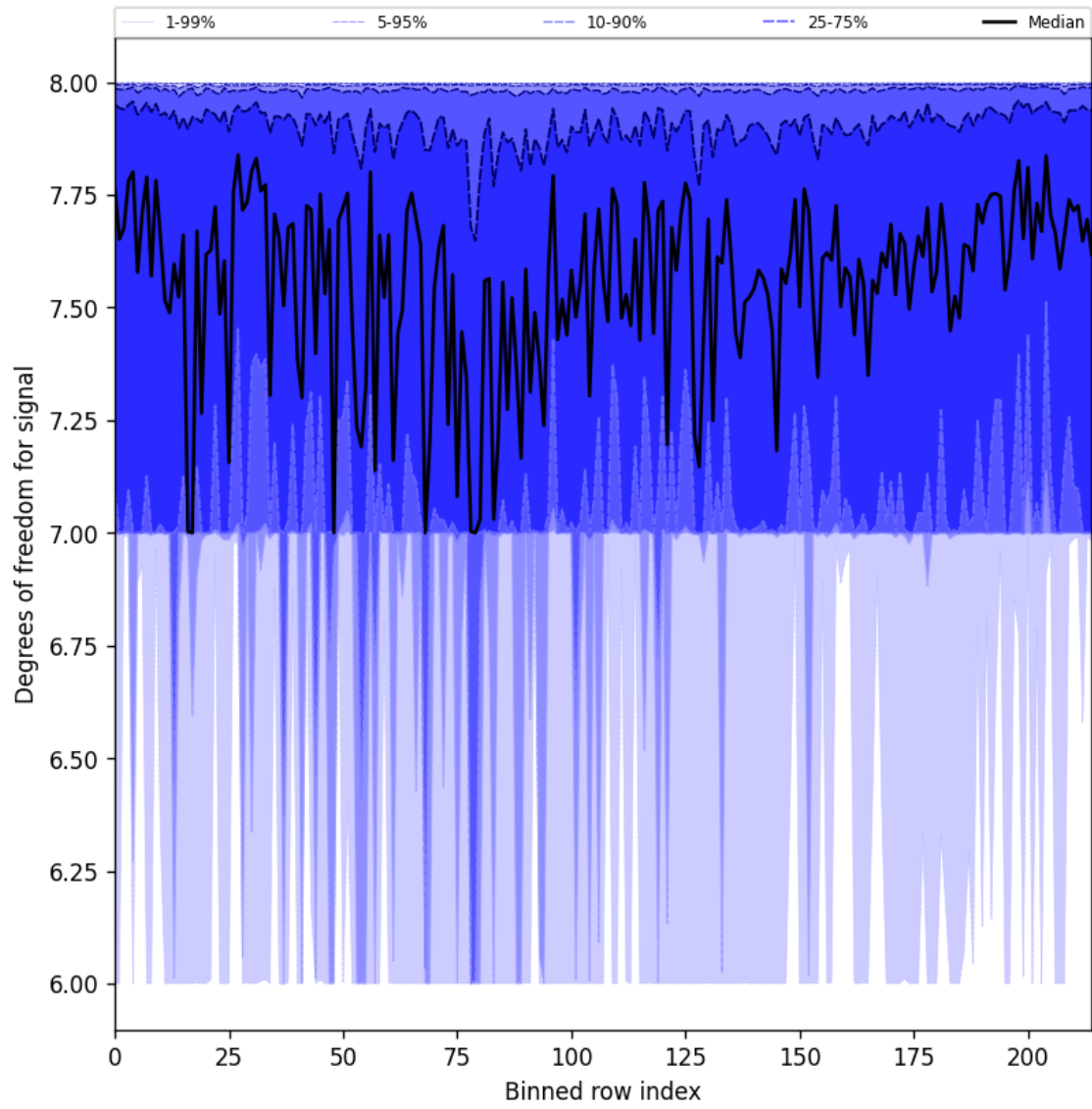
Figure 25: Along track statistics of “Degrees of freedom for signal” for 2025-09-23 to 2025-09-23
