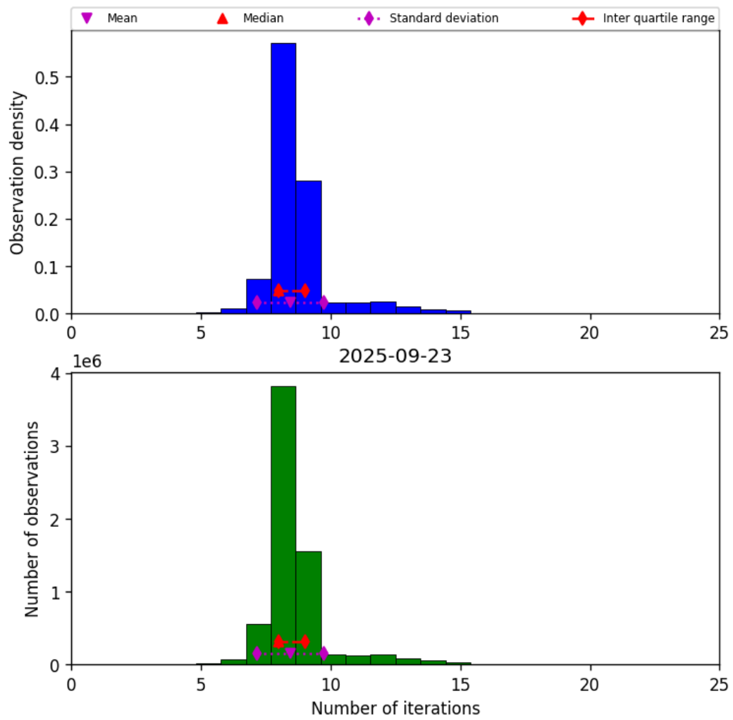
Figure 19: Histogram of “Number of iterations” for 2025-09-23 to 2025-09-23
