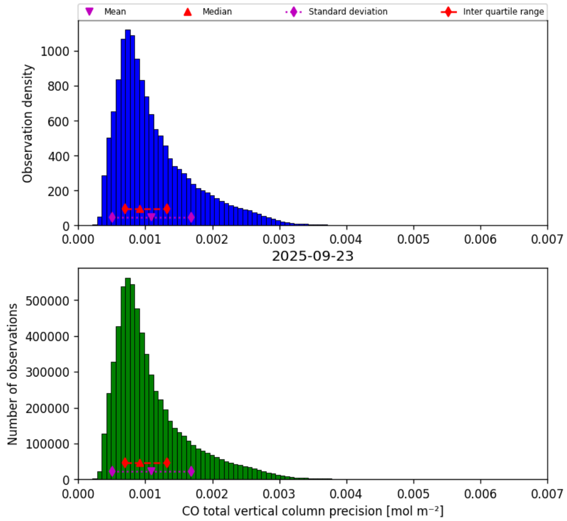
Figure 15: Histogram of “CO total vertical column precision” for 2025-09-23 to 2025-09-23
