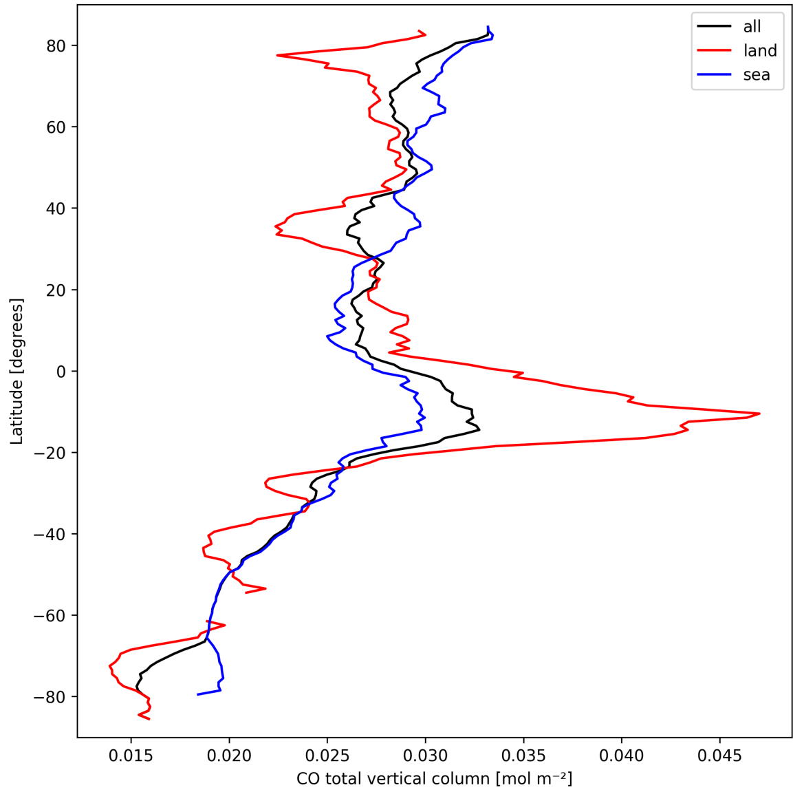
Figure 7: Zonal average of “CO total vertical column” for 2025-09-23 to 2025-09-23.
