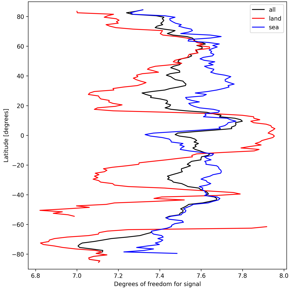
Figure 11: Zonal average of “Degrees of freedom for signal” for 2025-09-23 to 2025-09-23.
