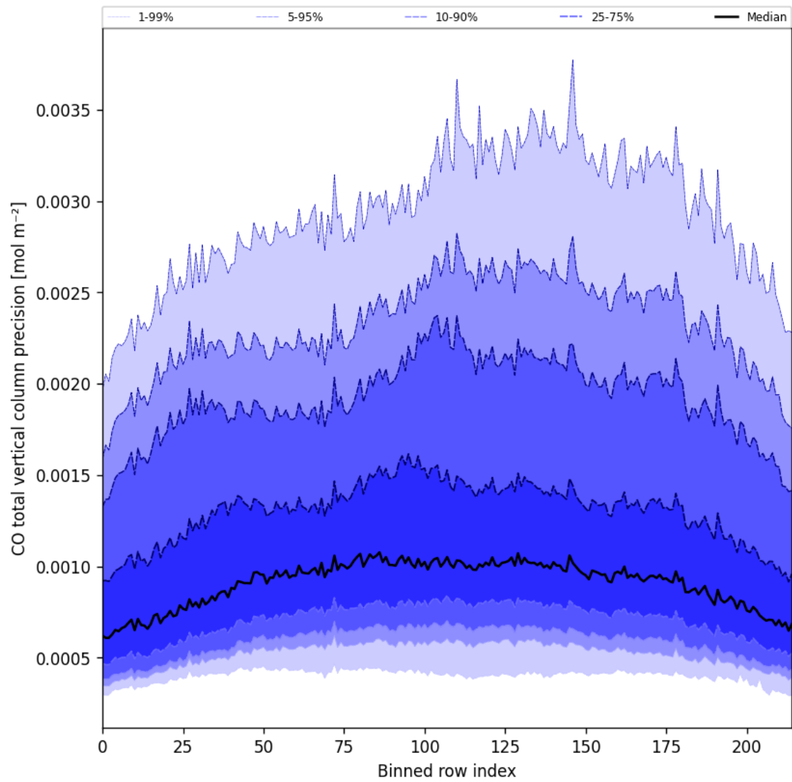
Figure 22: Along track statistics of “CO total vertical column precision” for 2025-09-23 to 2025-09-23
