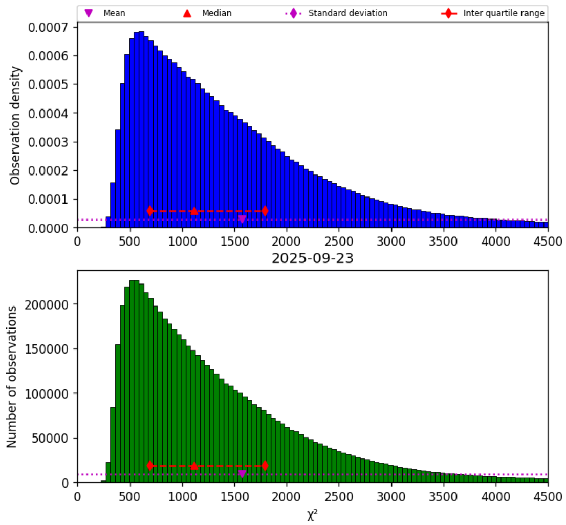
Figure 17: Histogram of " \chi^2 " for 2025-09-23 to 2025-09-23
