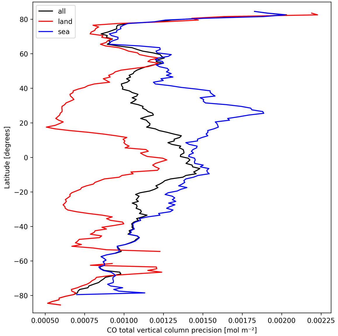
Figure 8: Zonal average of “CO total vertical column precision” for 2025-09-23 to 2025-09-23.
