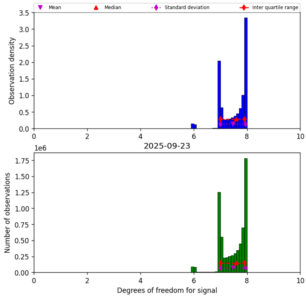
Figure 18: Histogram of “Degrees of freedom for signal” for 2025-09-23 to 2025-09-23
