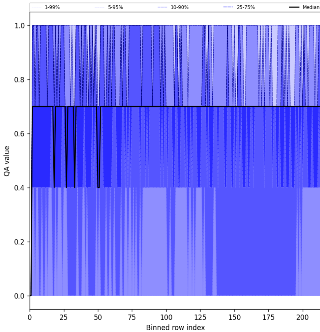
Figure 20: Along track statistics of “QA value” for 2025-09-23 to 2025-09-23
