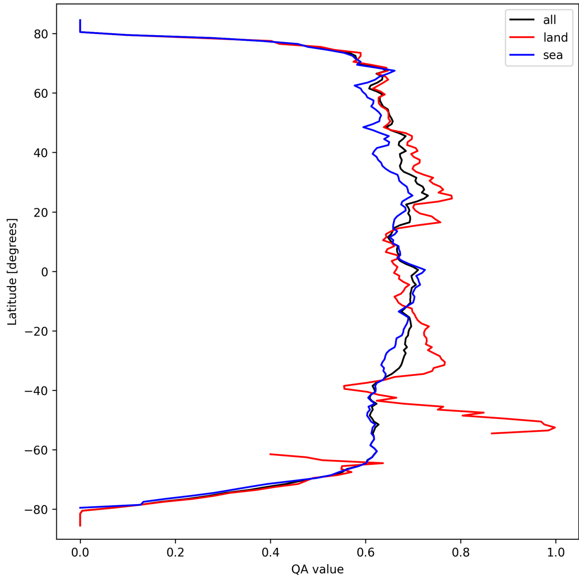
Figure 6: Zonal average of “QA value” for 2025-09-23 to 2025-09-23.
