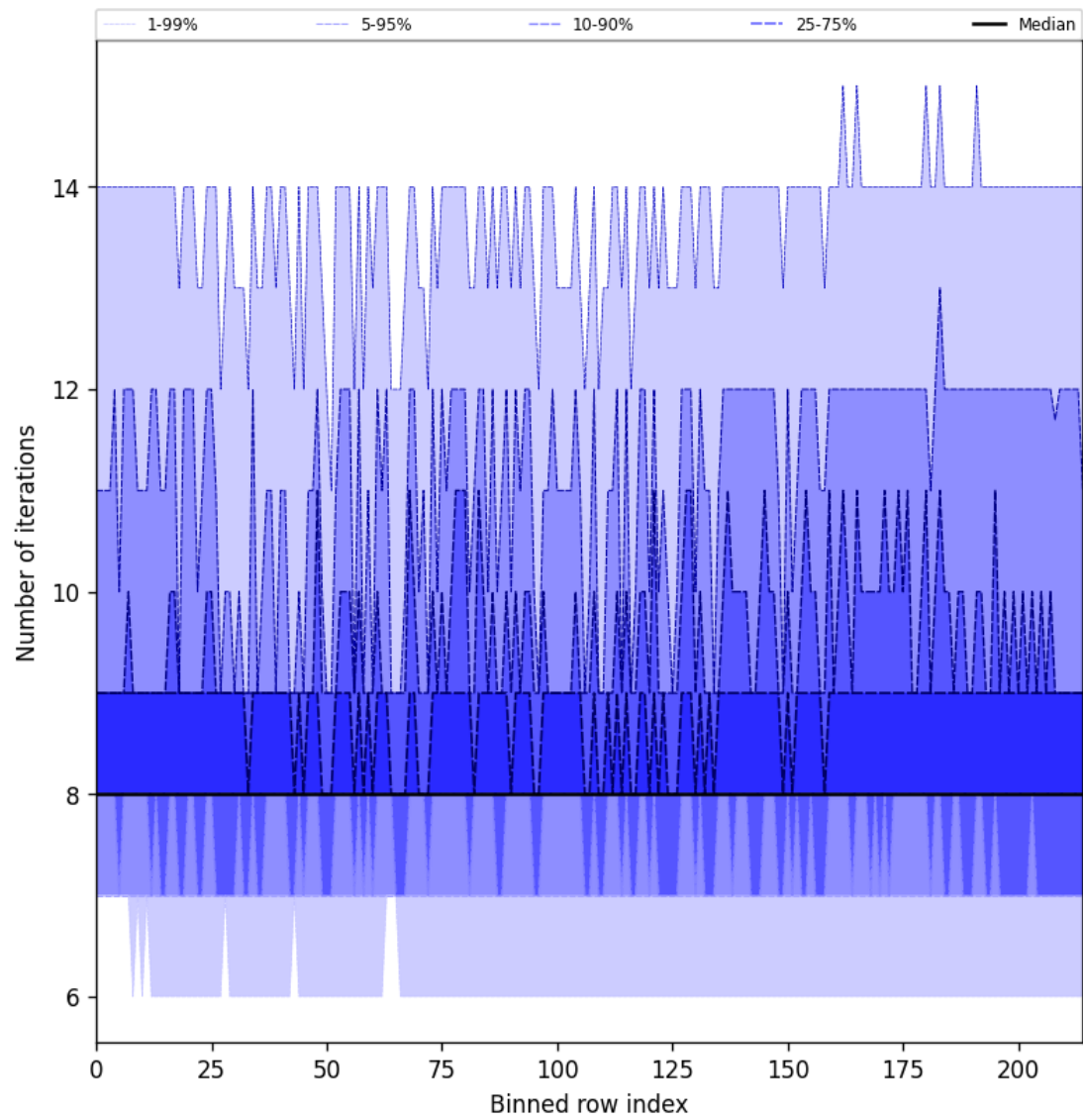
Figure 26: Along track statistics of “Number of iterations” for 2025-09-23 to 2025-09-23
