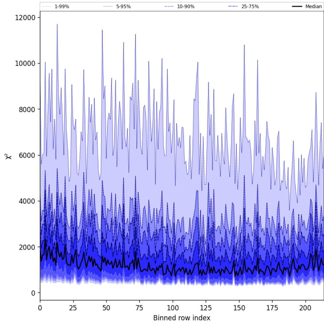
Figure 24: Along track statistics of “ \chi^2 ” for 2025-09-23 to 2025-09-23
