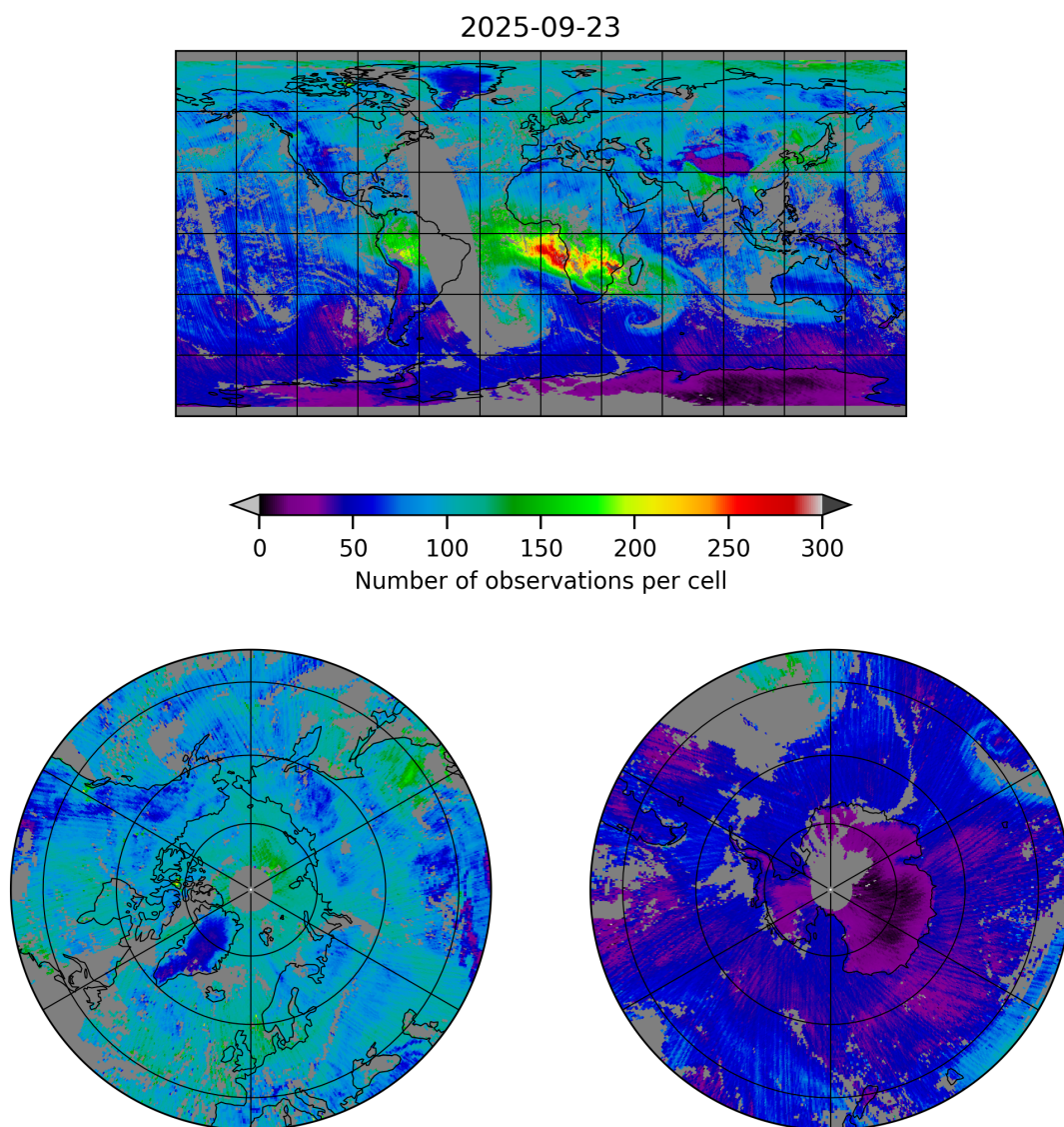
Figure 5: Map of the number of observations for 2025-09-23 to 2025-09-23
