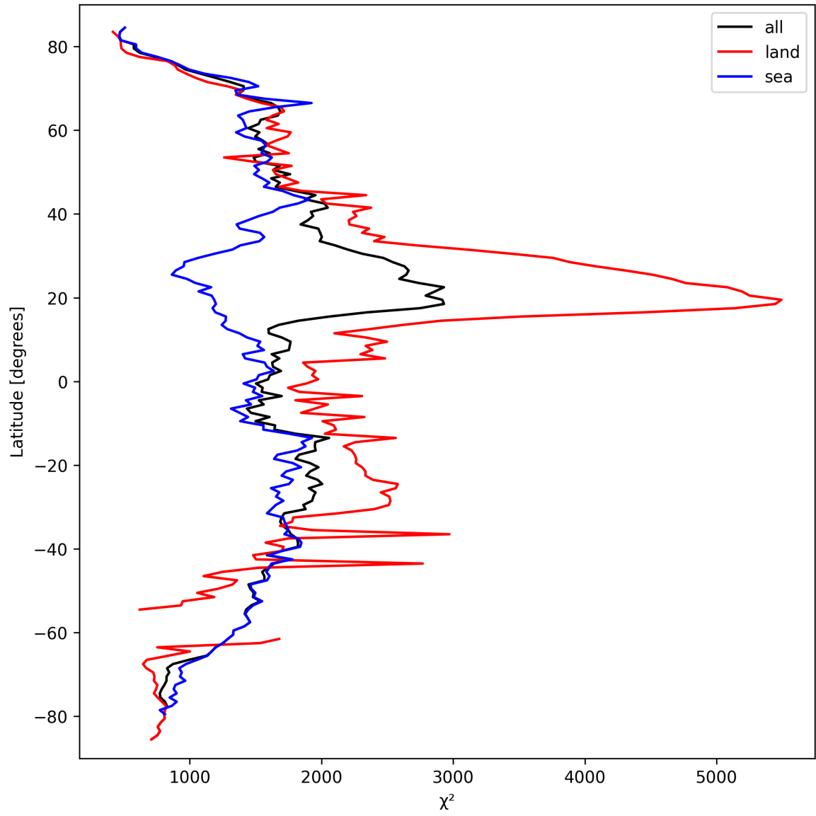
Figure 10: Zonal average of “ \chi^2 ” for 2025-09-23 to 2025-09-23.
