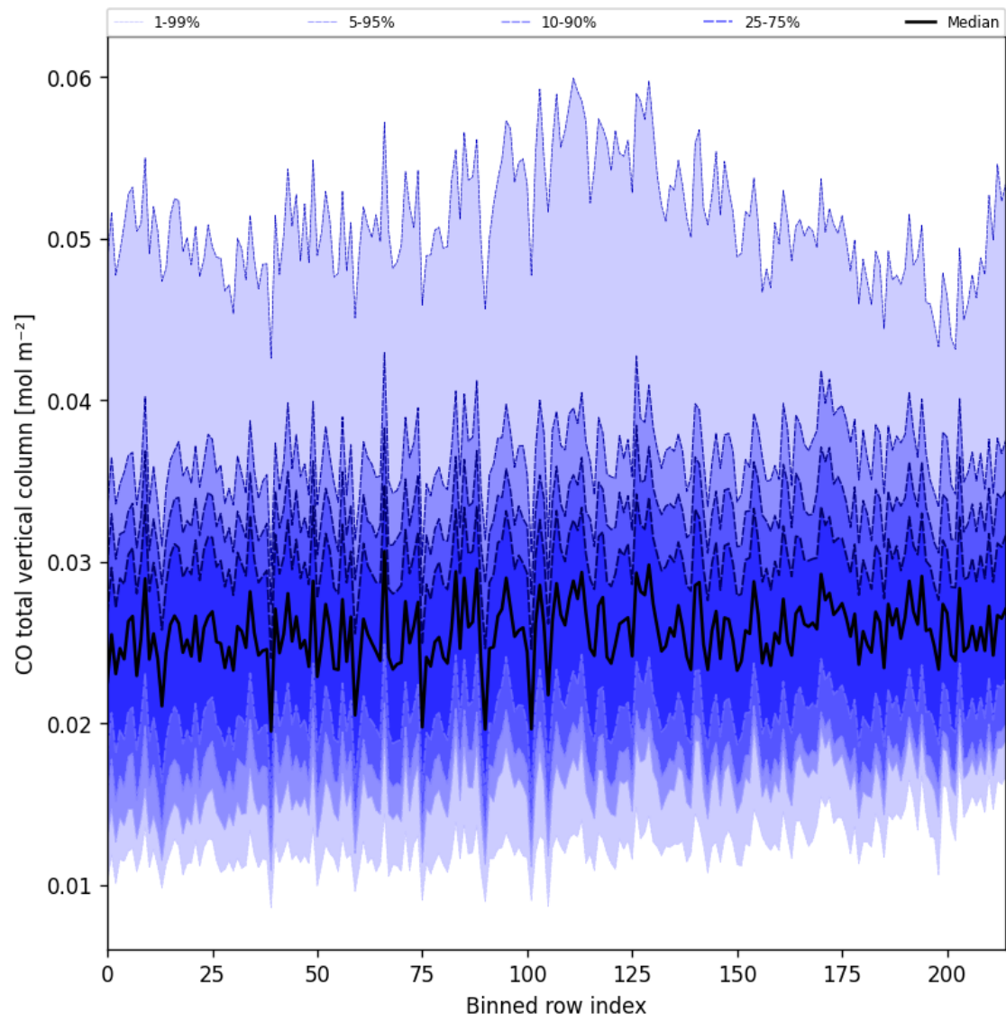
Figure 21: Along track statistics of “CO total vertical column” for 2025-09-23 to 2025-09-23
