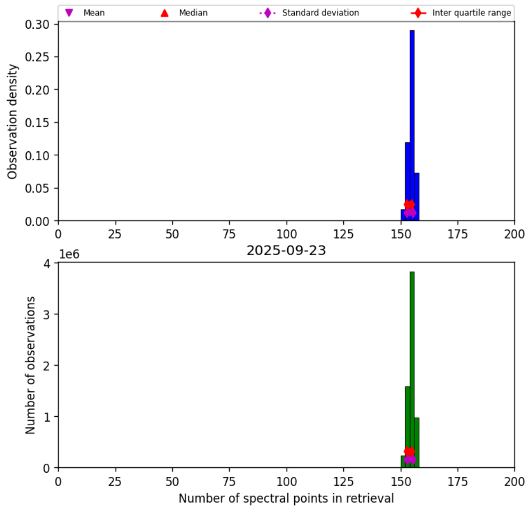
Figure 16: Histogram of “Number of spectral points in retrieval” for 2025-09-23 to 2025-09-23
