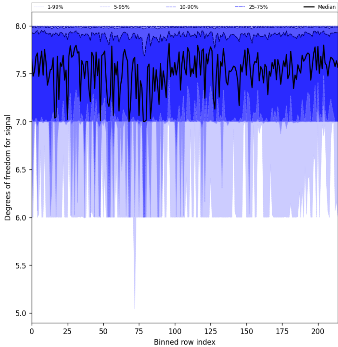
Figure 25: Along track statistics of “Degrees of freedom for signal” for 2025-09-25 to 2025-09-26
