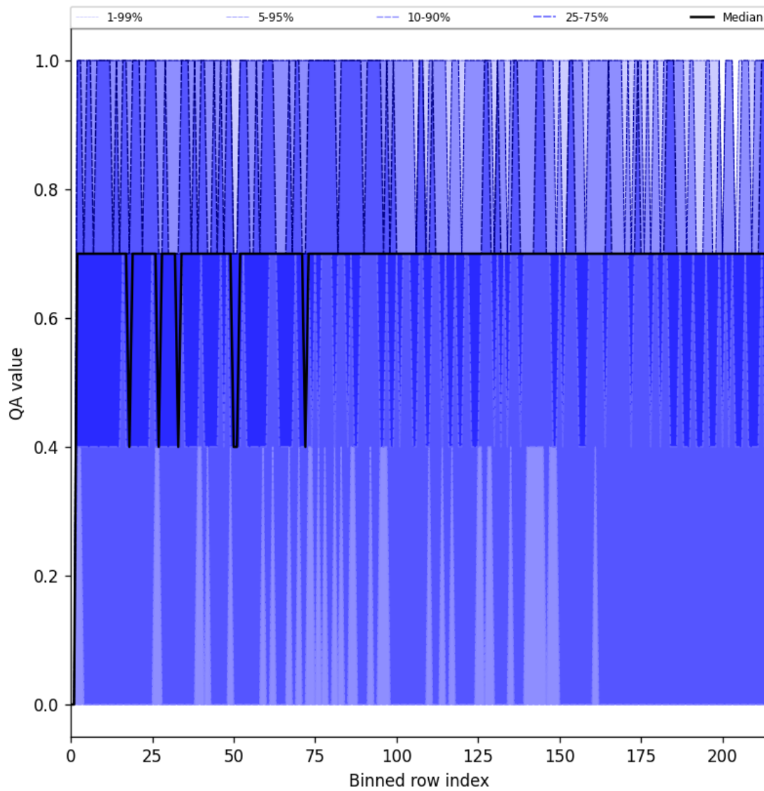
Figure 20: Along track statistics of “QA value” for 2025-09-25 to 2025-09-26
