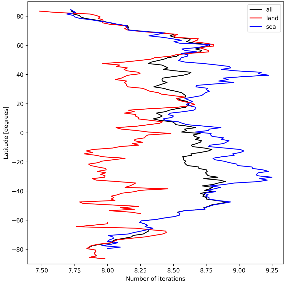
Figure 12: Zonal average of “Number of iterations” for 2025-09-25 to 2025-09-26.
