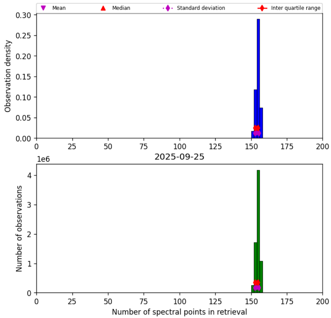
Figure 16: Histogram of “Number of spectral points in retrieval” for 2025-09-25 to 2025-09-26
