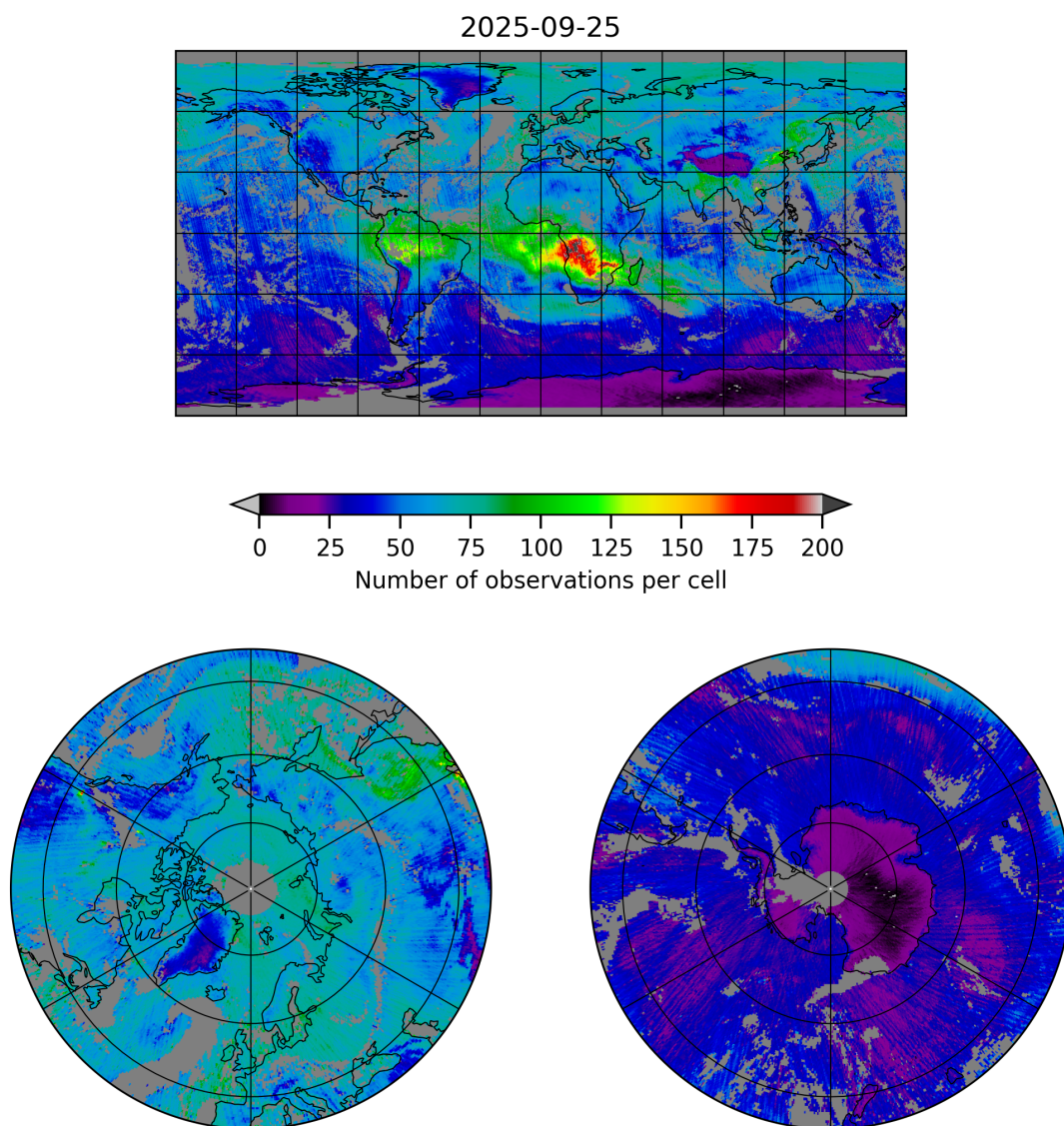
Figure 5: Map of the number of observations for 2025-09-25 to 2025-09-26
