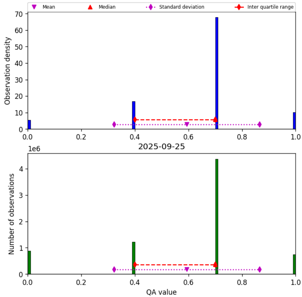
Figure 13: Histogram of “QA value” for 2025-09-25 to 2025-09-26
