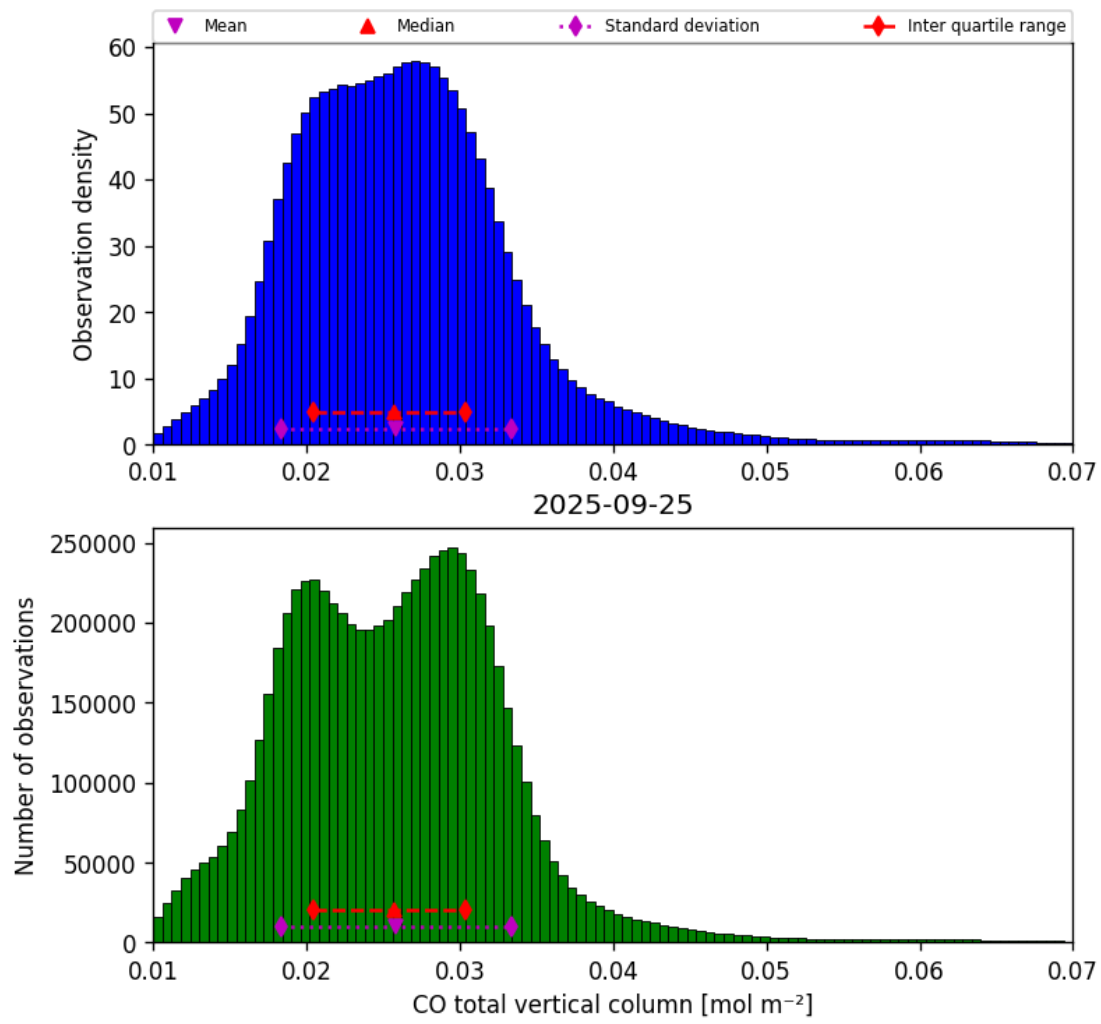
Figure 14: Histogram of “CO total vertical column” for 2025-09-25 to 2025-09-26
