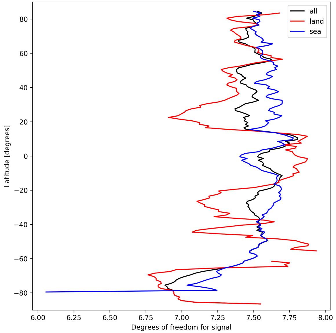
Figure 11: Zonal average of “Degrees of freedom for signal” for 2025-09-25 to 2025-09-26.
