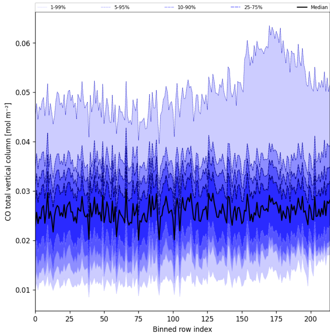
Figure 21: Along track statistics of “CO total vertical column” for 2025-09-25 to 2025-09-26
