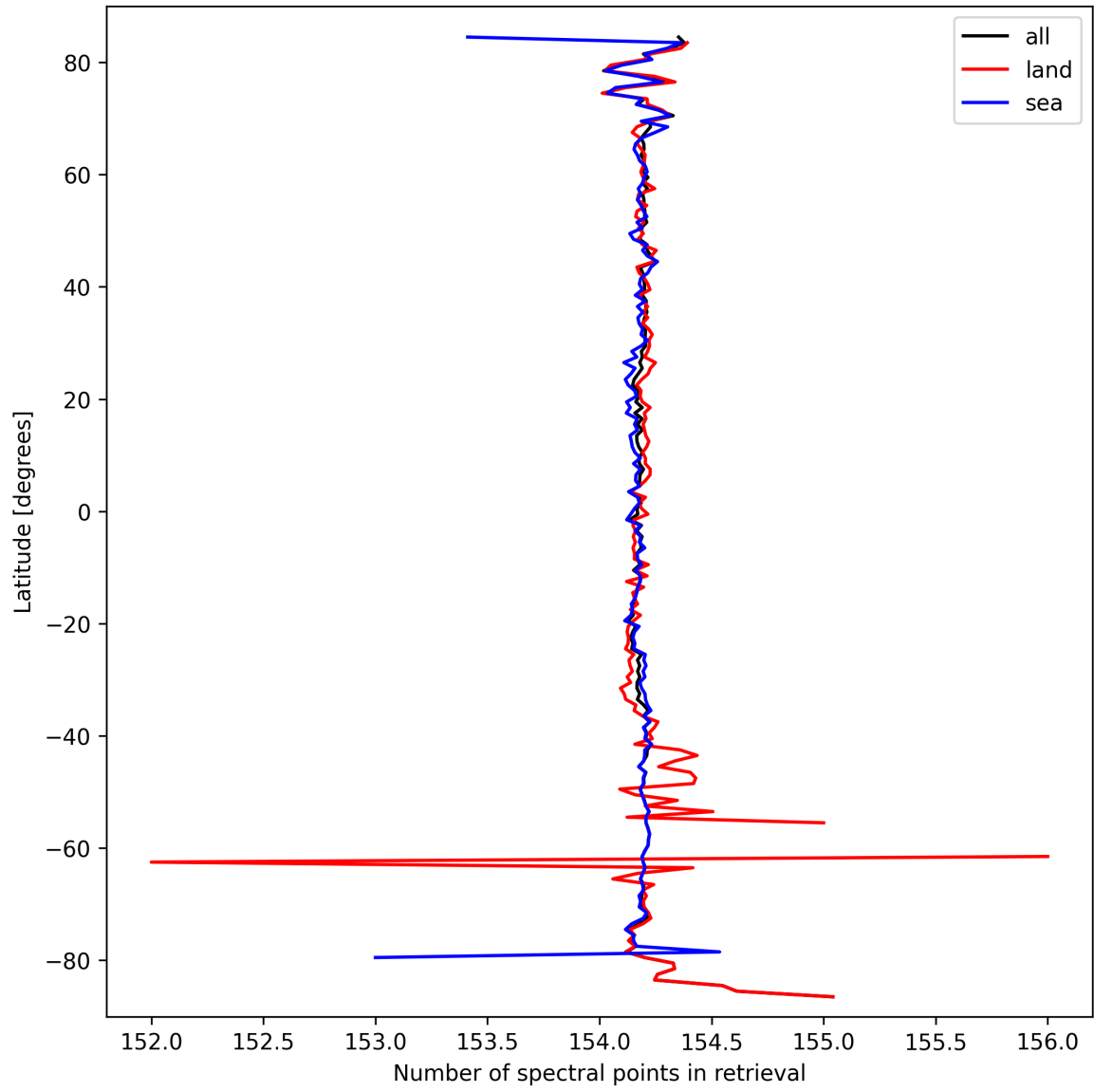
Figure 9: Zonal average of “Number of spectral points in retrieval” for 2025-09-25 to 2025-09-26.
