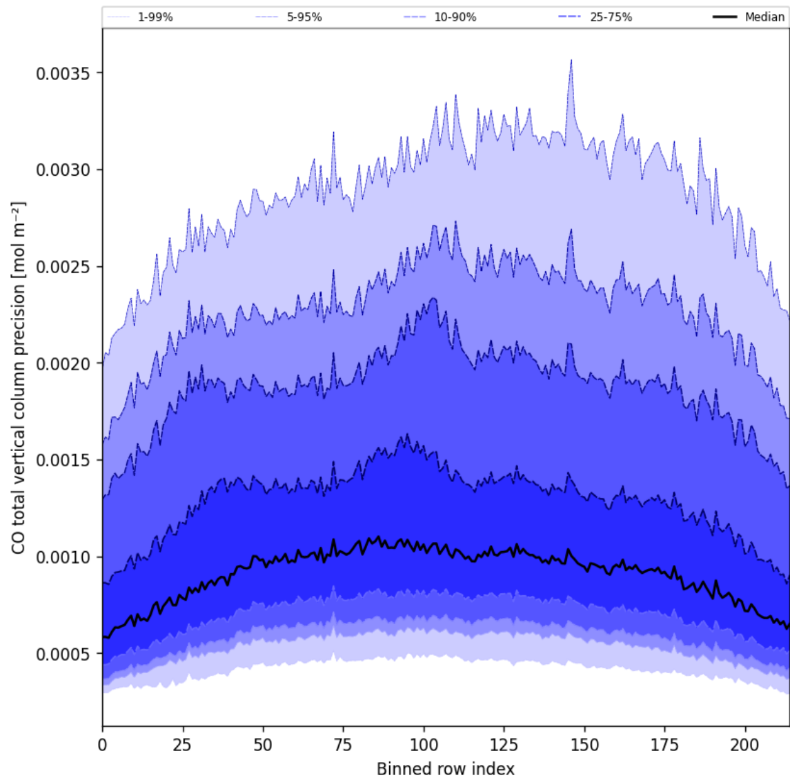
Figure 22: Along track statistics of “CO total vertical column precision” for 2025-09-25 to 2025-09-26
