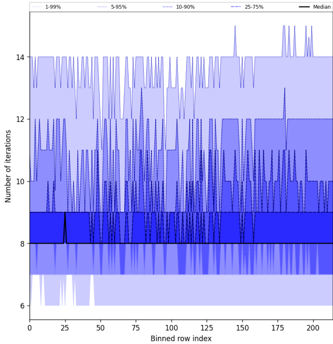
Figure 26: Along track statistics of “Number of iterations” for 2025-09-25 to 2025-09-26
