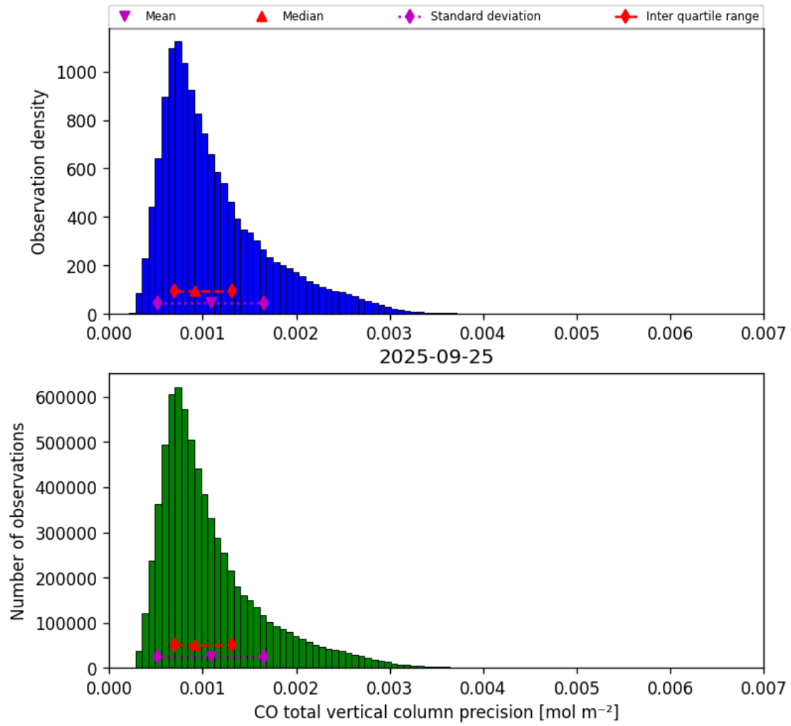
Figure 15: Histogram of “CO total vertical column precision” for 2025-09-25 to 2025-09-26
