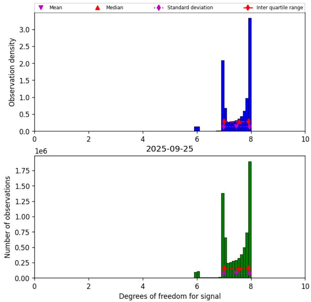
Figure 18: Histogram of “Degrees of freedom for signal” for 2025-09-25 to 2025-09-26
