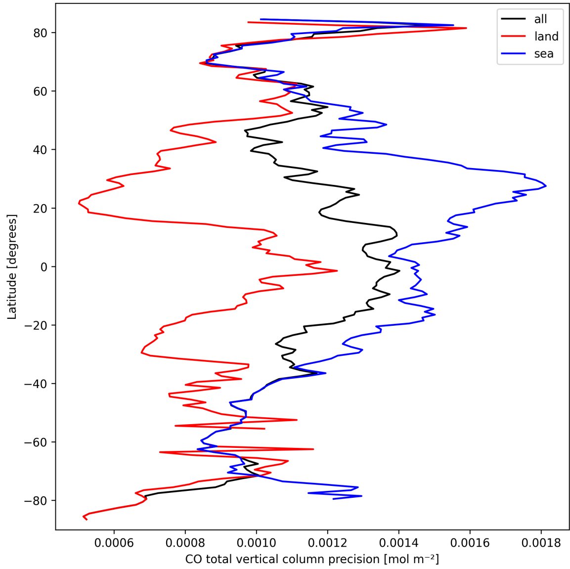
Figure 8: Zonal average of “CO total vertical column precision” for 2025-09-25 to 2025-09-26.
