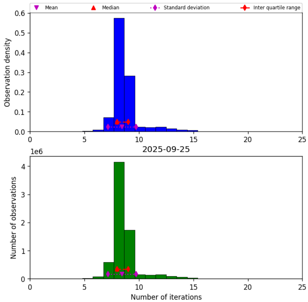
Figure 19: Histogram of “Number of iterations” for 2025-09-25 to 2025-09-26
