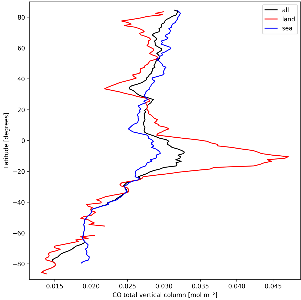
Figure 7: Zonal average of “CO total vertical column” for 2025-09-25 to 2025-09-26.
