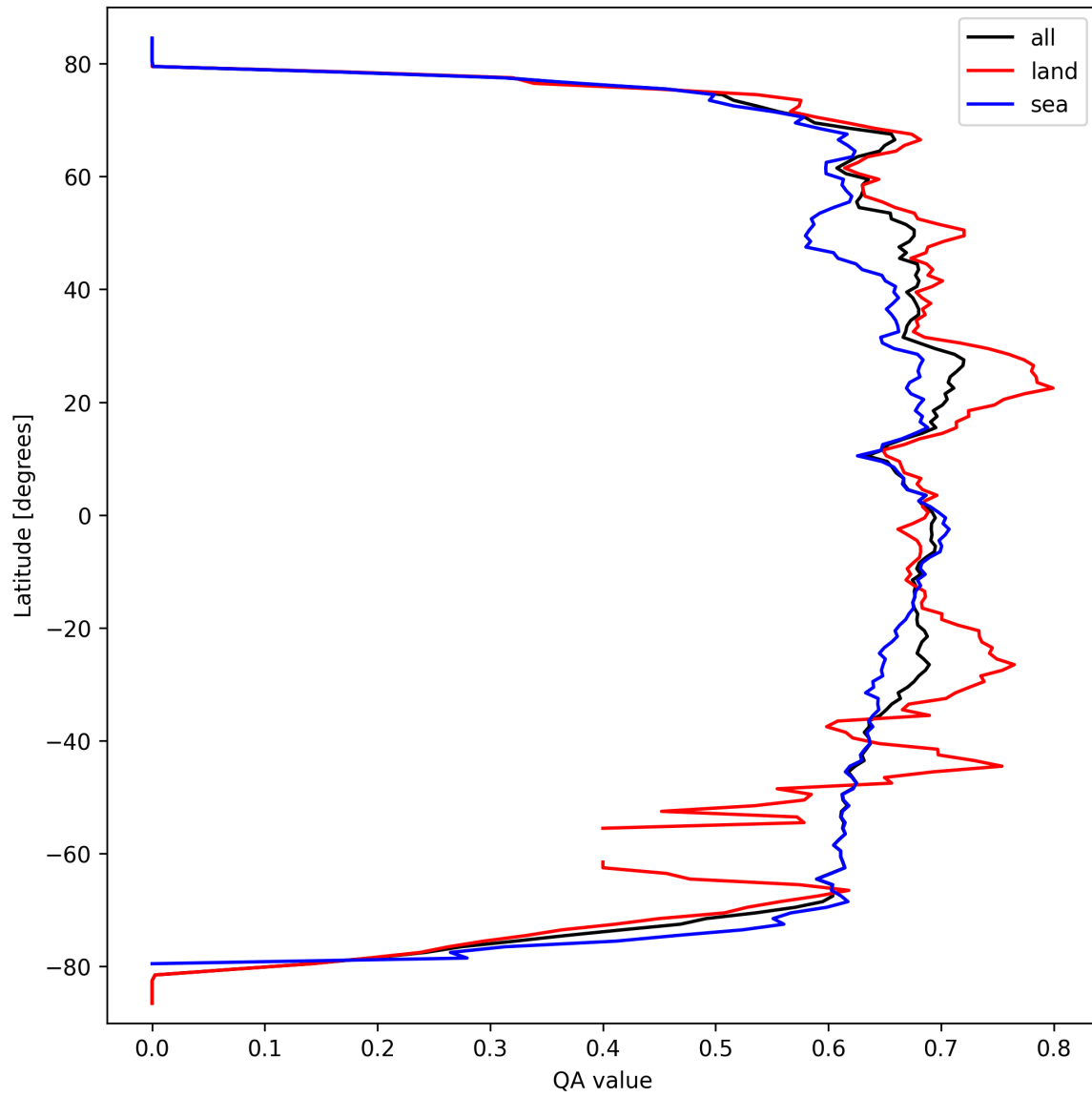
Figure 6: Zonal average of “QA value” for 2025-09-25 to 2025-09-26.
