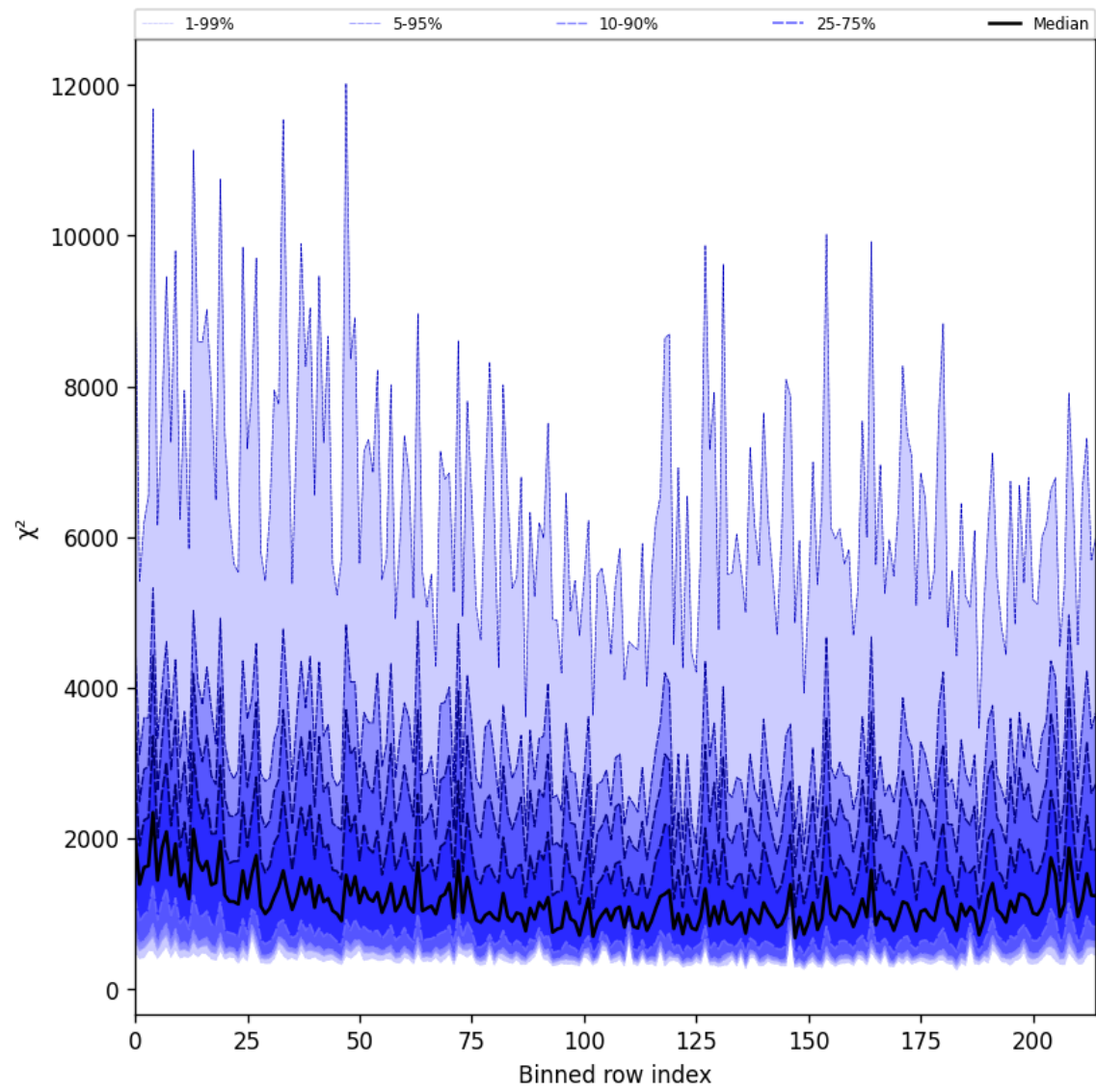
Figure 24: Along track statistics of “ \chi^2 ” for 2025-09-25 to 2025-09-26
