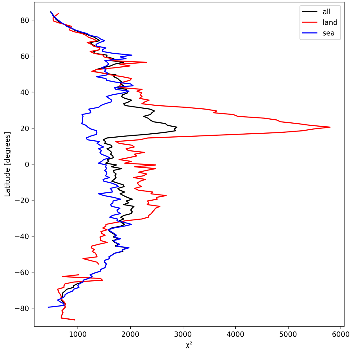
Figure 10: Zonal average of “ \chi^2 ” for 2025-09-25 to 2025-09-26.
