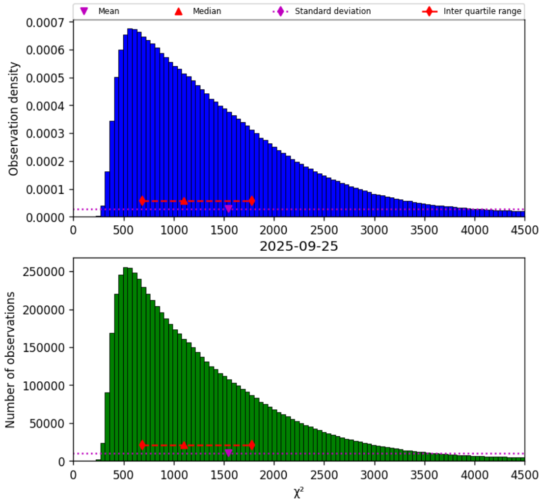
Figure 17: Histogram of “ \chi^2 ” for 2025-09-25 to 2025-09-26
