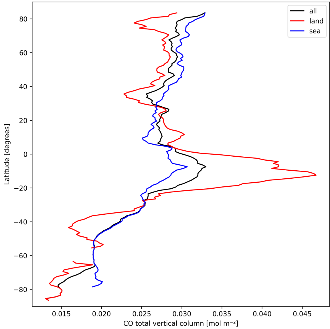
Figure 7: Zonal average of “CO total vertical column” for 2025-09-26 to 2025-09-27.
