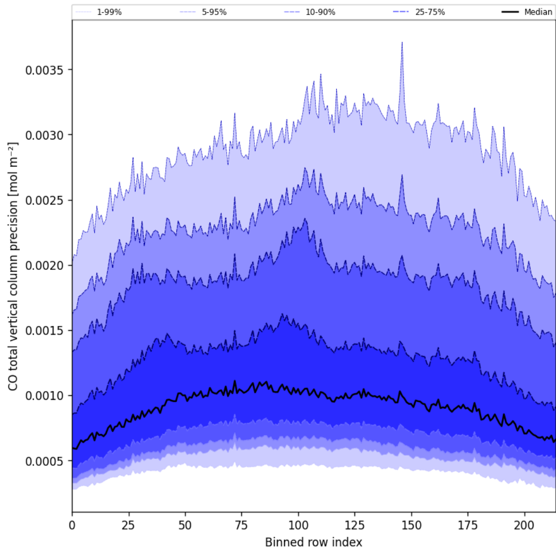
Figure 22: Along track statistics of “CO total vertical column precision” for 2025-09-26 to 2025-09-27
