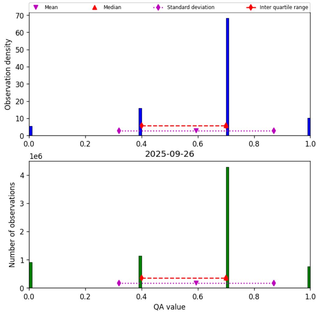
Figure 13: Histogram of “QA value” for 2025-09-26 to 2025-09-27
