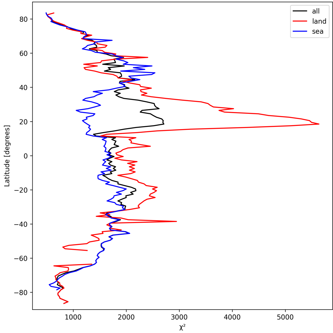
Figure 10: Zonal average of “ \chi^2 ” for 2025-09-26 to 2025-09-27.
