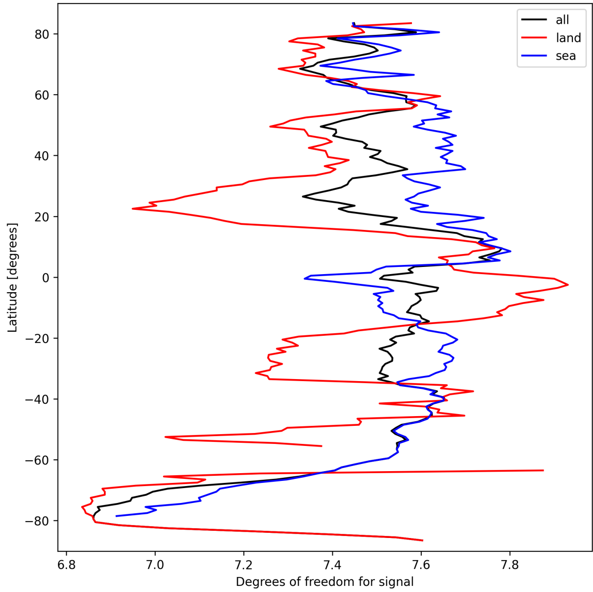
Figure 11: Zonal average of “Degrees of freedom for signal” for 2025-09-26 to 2025-09-27.
