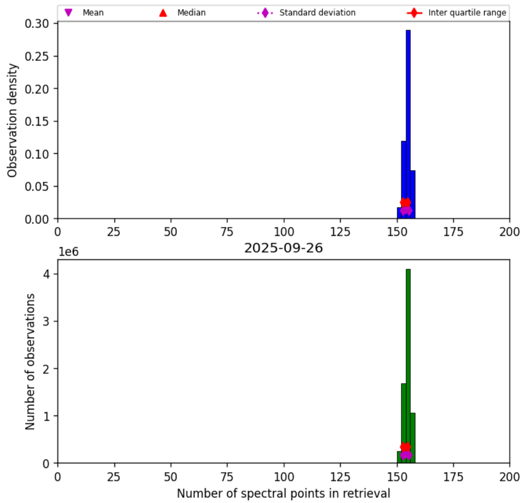
Figure 16: Histogram of “Number of spectral points in retrieval” for 2025-09-26 to 2025-09-27
