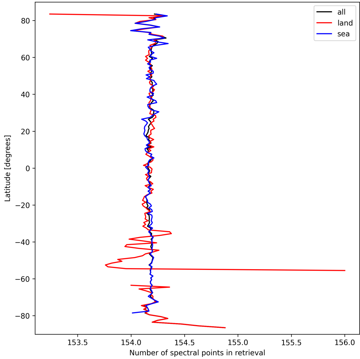
Figure 9: Zonal average of “Number of spectral points in retrieval” for 2025-09-26 to 2025-09-27.
