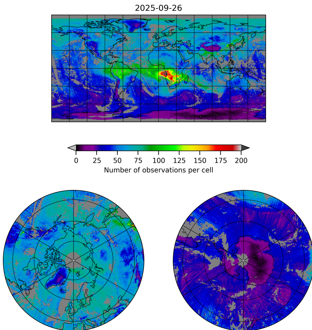
Figure 5: Map of the number of observations for 2025-09-26 to 2025-09-27
