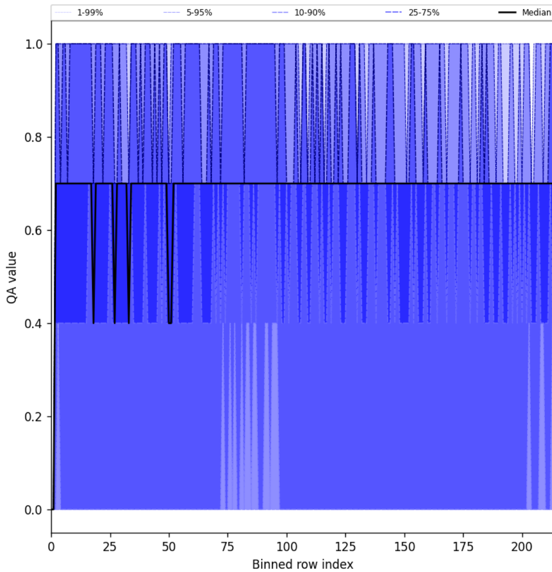
Figure 20: Along track statistics of “QA value” for 2025-09-26 to 2025-09-27
