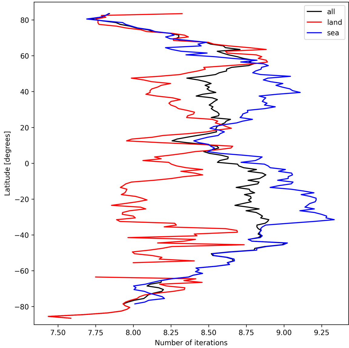
Figure 12: Zonal average of “Number of iterations” for 2025-09-26 to 2025-09-27.
