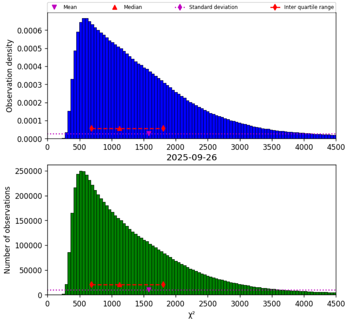
Figure 17: Histogram of " \chi^2 " for 2025-09-26 to 2025-09-27
