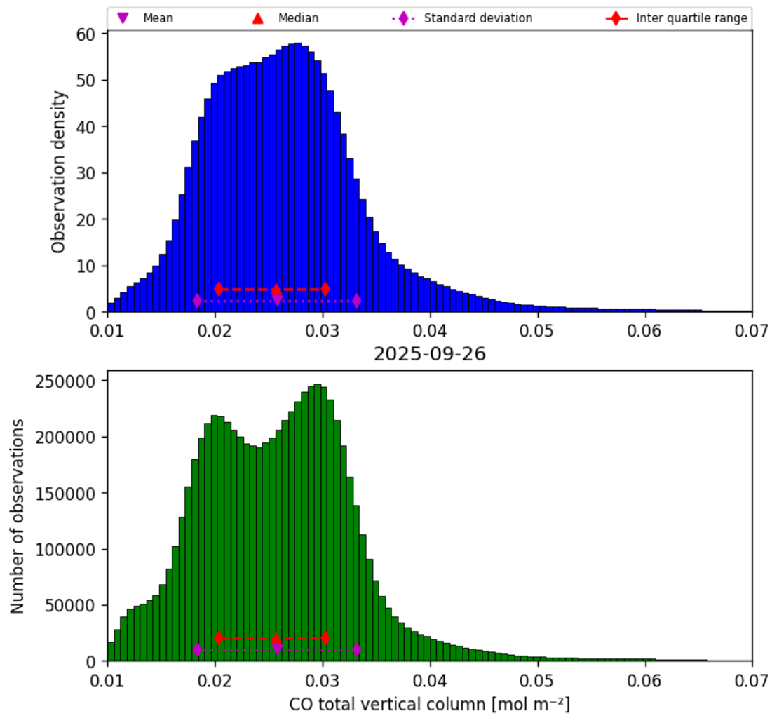
Figure 14: Histogram of “CO total vertical column” for 2025-09-26 to 2025-09-27
