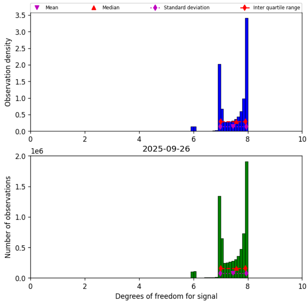
Figure 18: Histogram of “Degrees of freedom for signal” for 2025-09-26 to 2025-09-27
