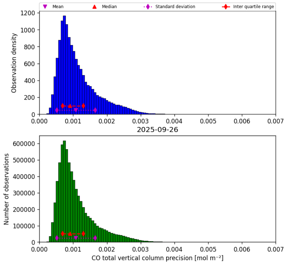
Figure 15: Histogram of “CO total vertical column precision” for 2025-09-26 to 2025-09-27
