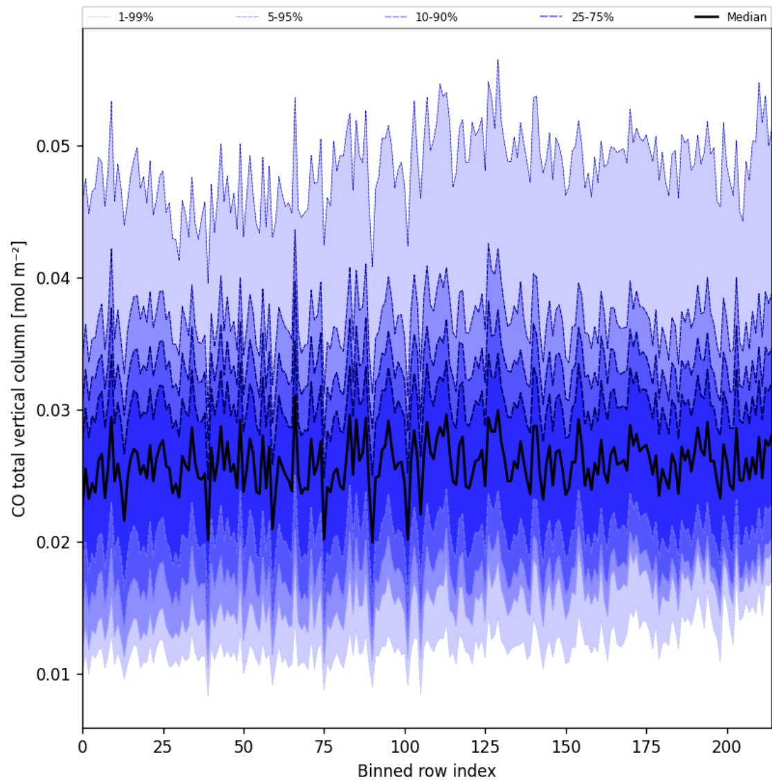
Figure 21: Along track statistics of “CO total vertical column” for 2025-09-26 to 2025-09-27
