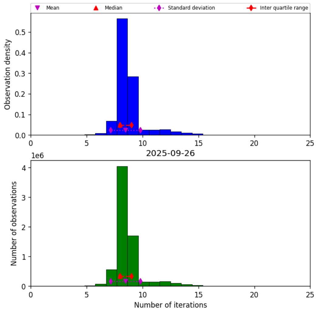
Figure 19: Histogram of “Number of iterations” for 2025-09-26 to 2025-09-27
