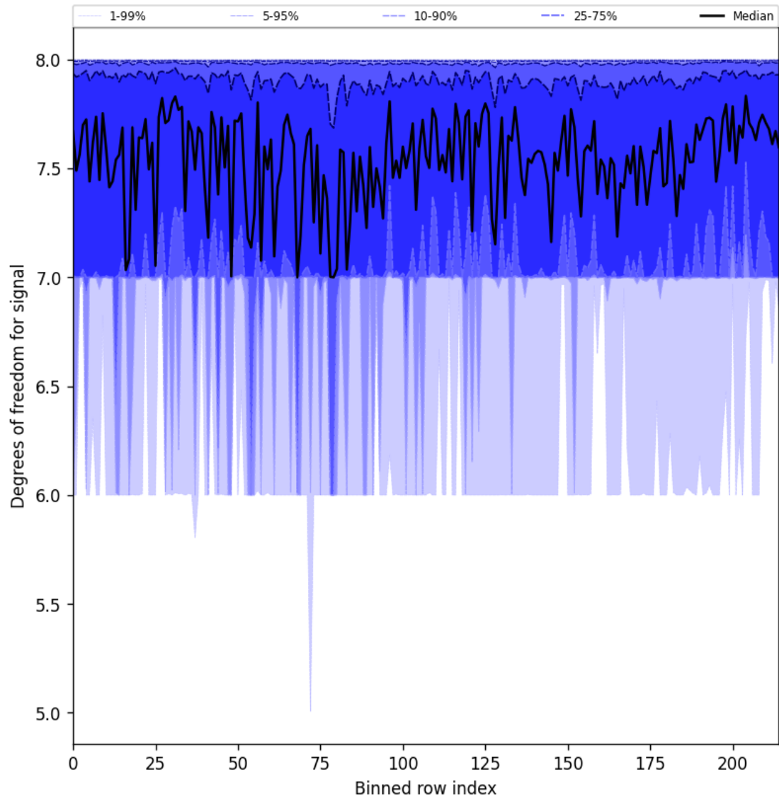
Figure 25: Along track statistics of “Degrees of freedom for signal” for 2025-09-26 to 2025-09-27
