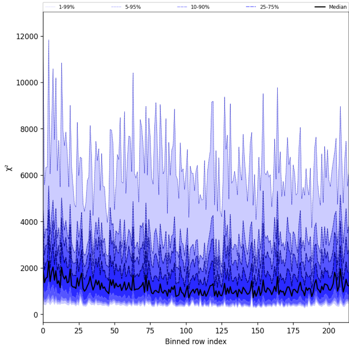
Figure 24: Along track statistics of “ \chi^2 ” for 2025-09-26 to 2025-09-27
