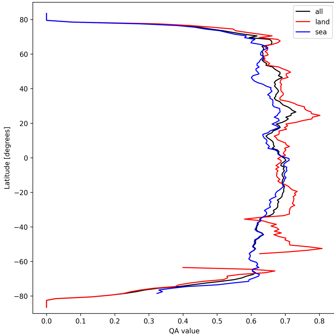
Figure 6: Zonal average of “QA value” for 2025-09-26 to 2025-09-27.
