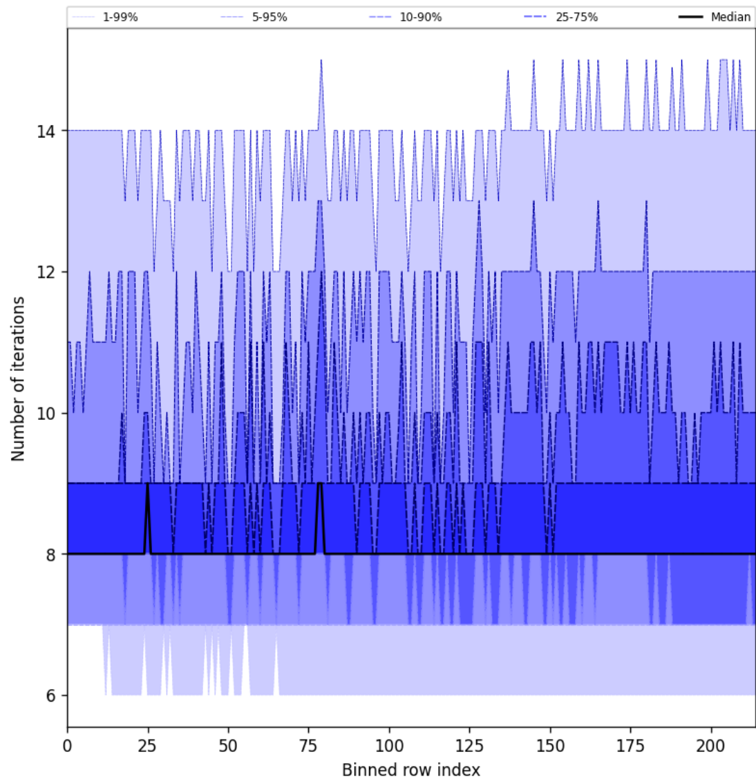
Figure 26: Along track statistics of “Number of iterations” for 2025-09-26 to 2025-09-27
