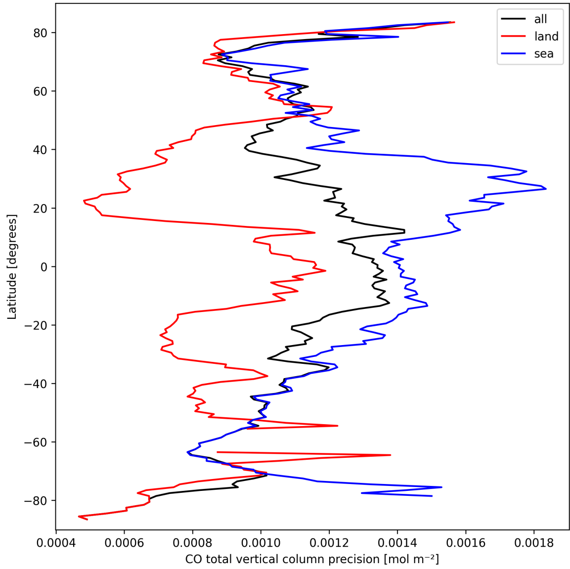
Figure 8: Zonal average of “CO total vertical column precision” for 2025-09-26 to 2025-09-27.
