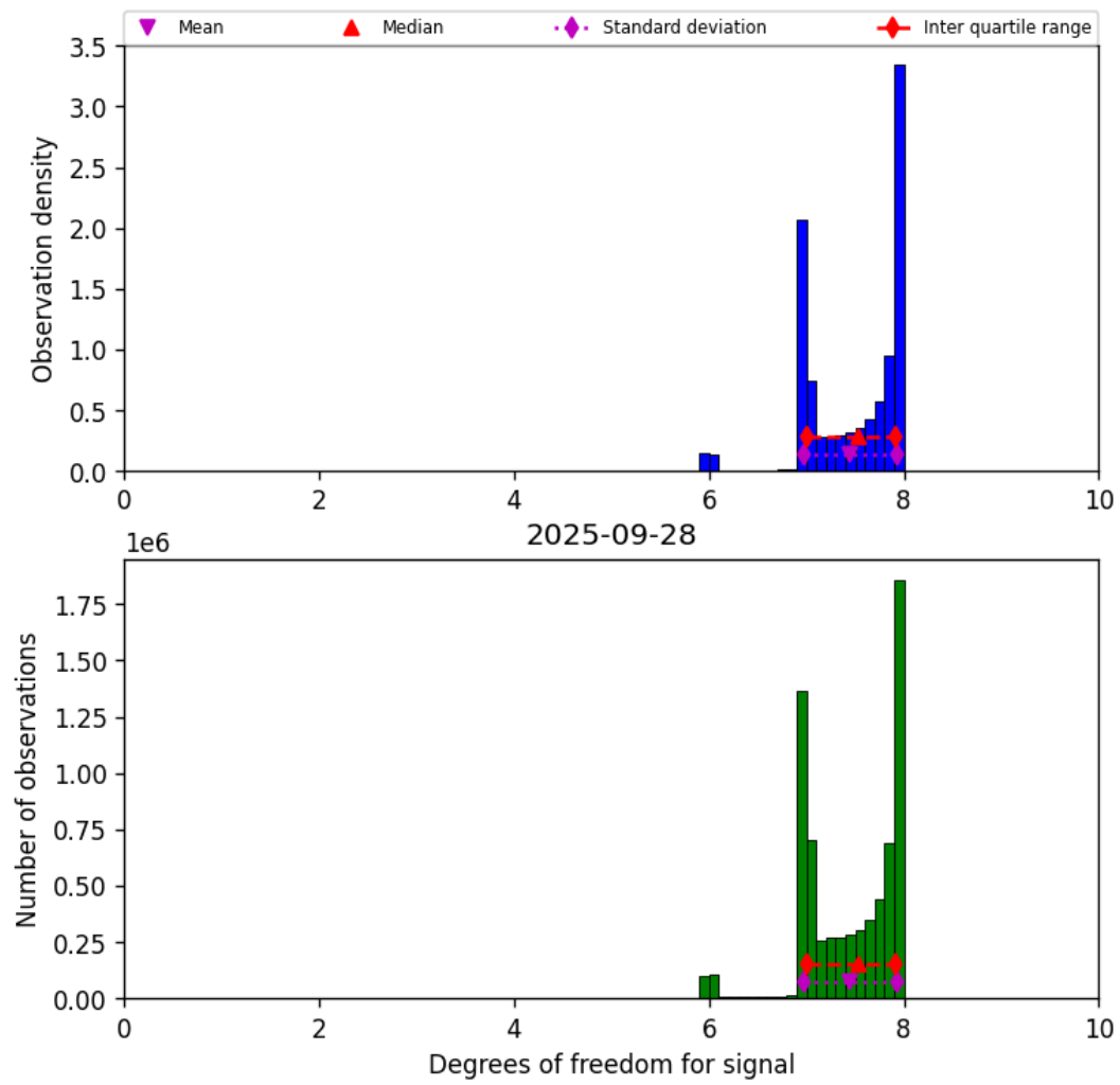
Figure 18: Histogram of “Degrees of freedom for signal” for 2025-09-28 to 2025-09-29
