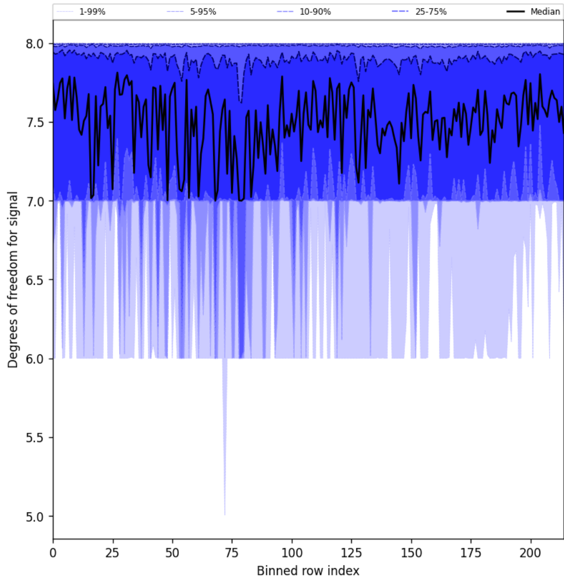
Figure 25: Along track statistics of “Degrees of freedom for signal” for 2025-09-28 to 2025-09-29
