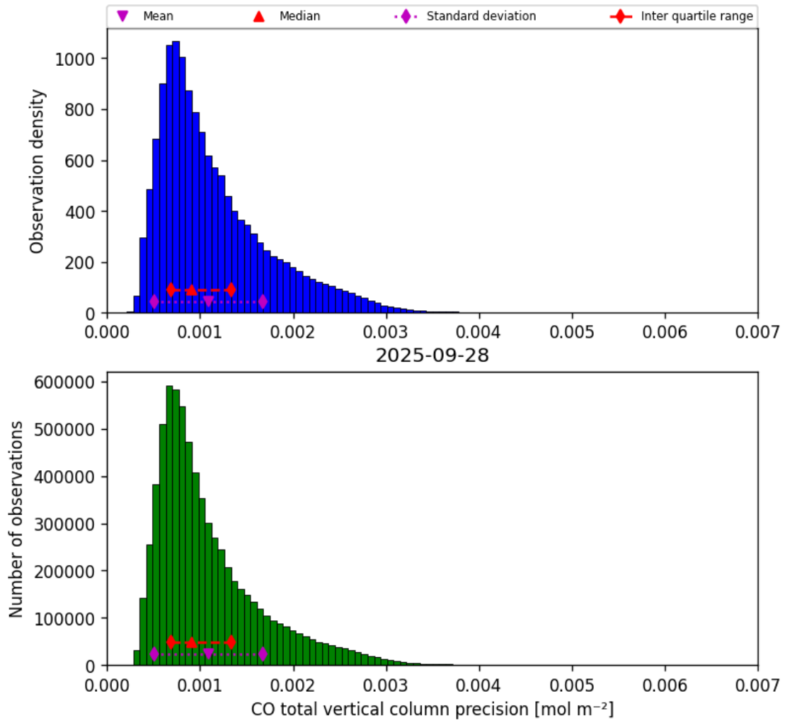
Figure 15: Histogram of “CO total vertical column precision” for 2025-09-28 to 2025-09-29
