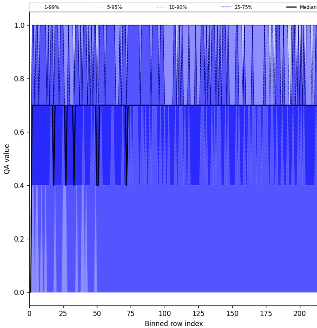
Figure 20: Along track statistics of “QA value” for 2025-09-28 to 2025-09-29
