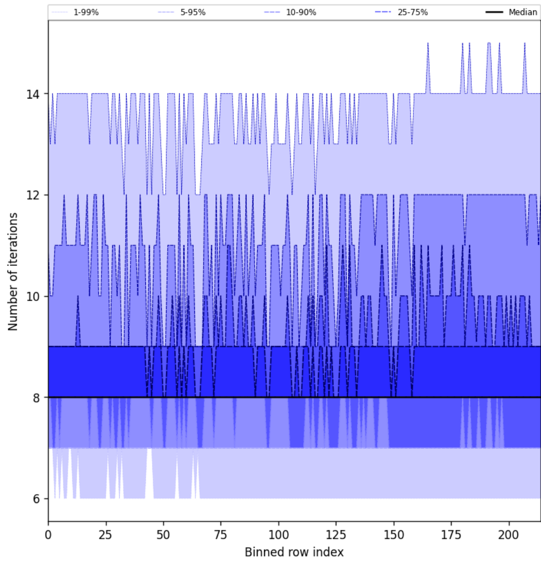
Figure 26: Along track statistics of “Number of iterations” for 2025-09-28 to 2025-09-29
