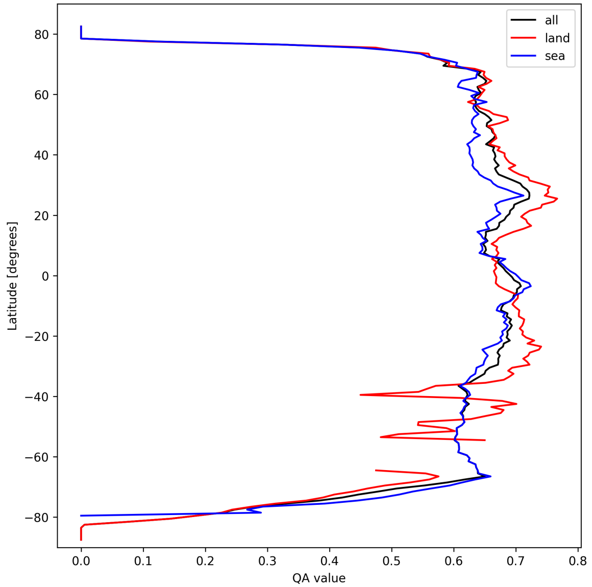
Figure 6: Zonal average of “QA value” for 2025-09-28 to 2025-09-29.
