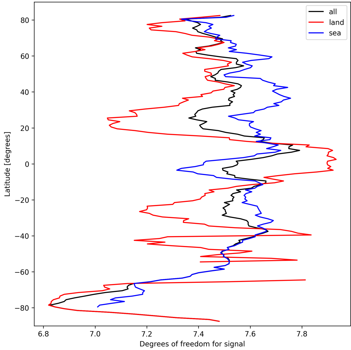
Figure 11: Zonal average of “Degrees of freedom for signal” for 2025-09-28 to 2025-09-29.
