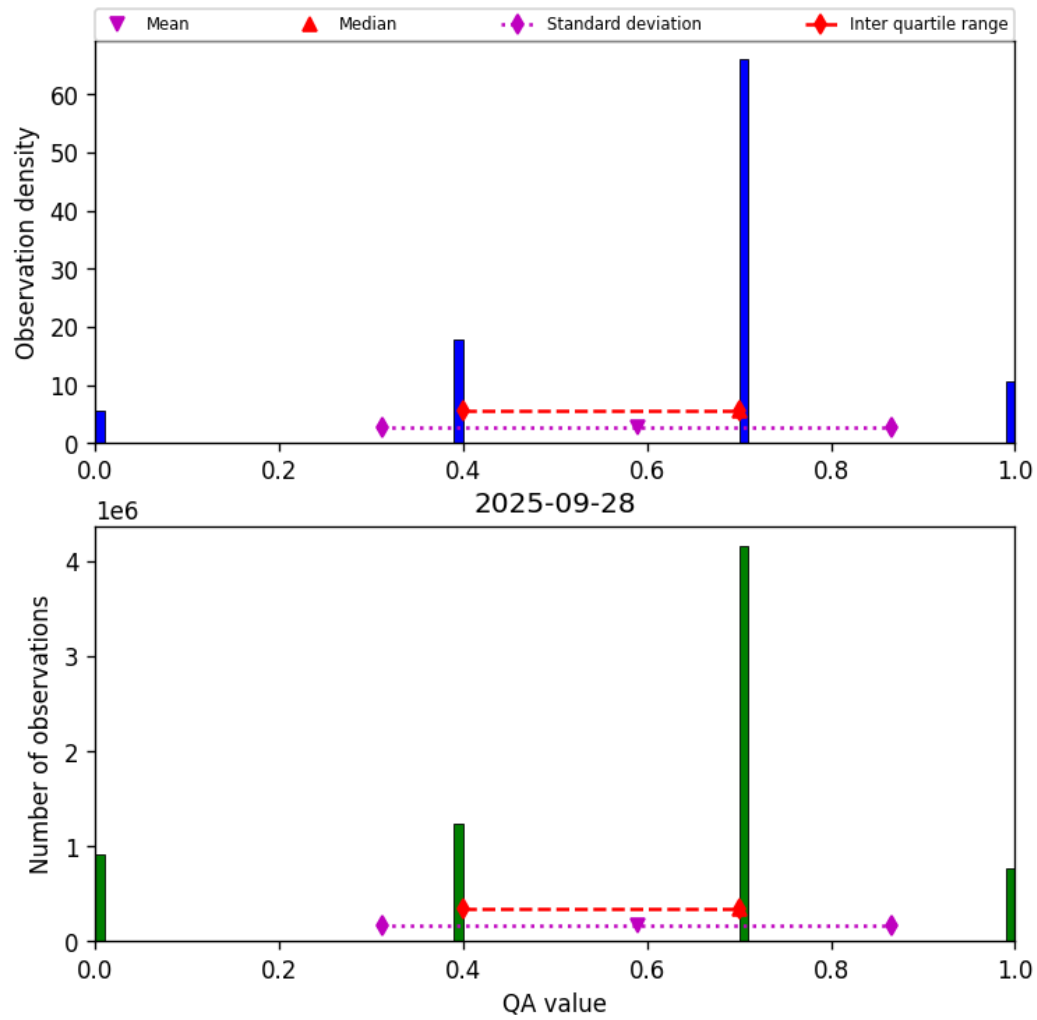
Figure 13: Histogram of “QA value” for 2025-09-28 to 2025-09-29
