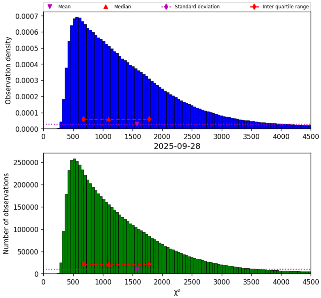
Figure 17: Histogram of “ \chi^2 ” for 2025-09-28 to 2025-09-29
