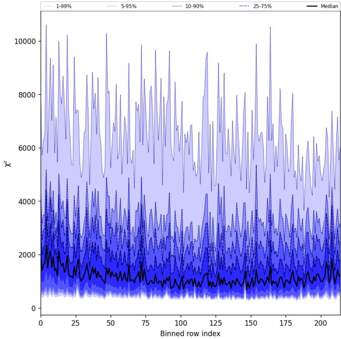
Figure 24: Along track statistics of “ \chi^2 ” for 2025-09-28 to 2025-09-29
