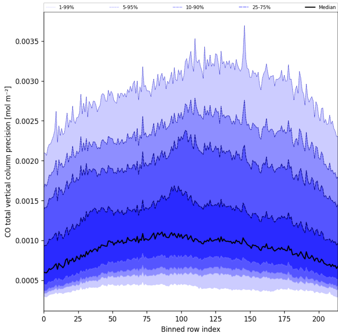
Figure 22: Along track statistics of “CO total vertical column precision” for 2025-09-28 to 2025-09-29
