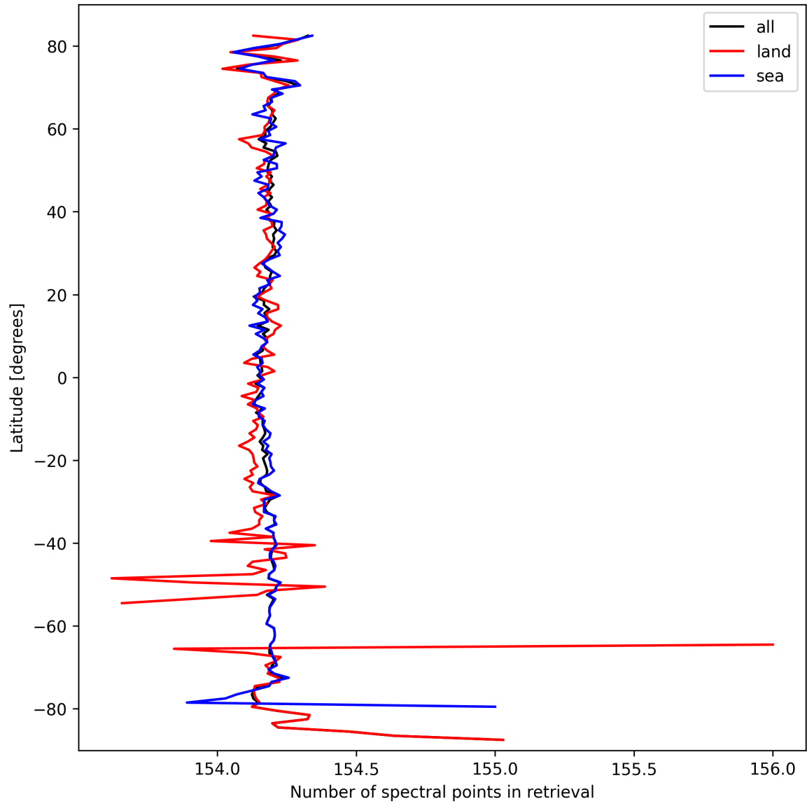
Figure 9: Zonal average of “Number of spectral points in retrieval” for 2025-09-28 to 2025-09-29.
