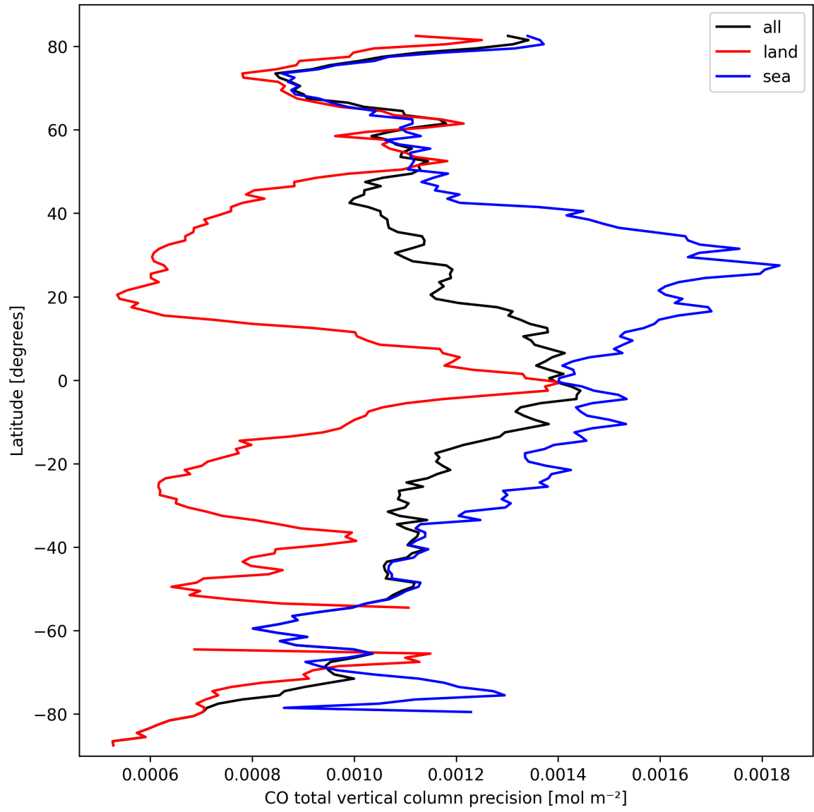
Figure 8: Zonal average of “CO total vertical column precision” for 2025-09-28 to 2025-09-29.
