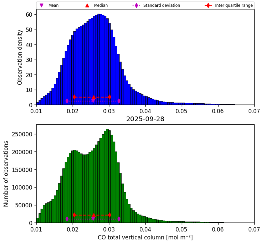
Figure 14: Histogram of “CO total vertical column” for 2025-09-28 to 2025-09-29
