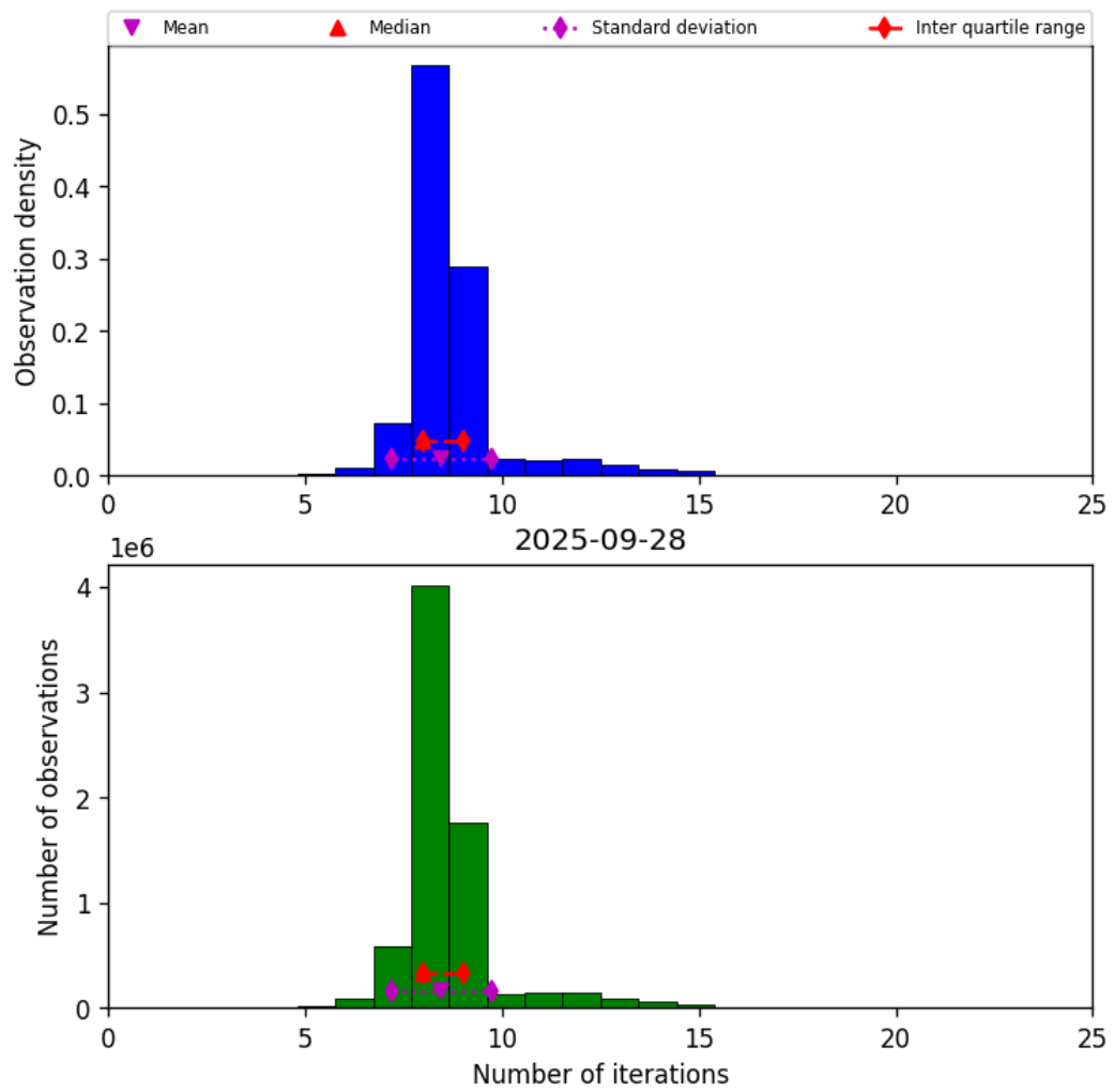
Figure 19: Histogram of “Number of iterations” for 2025-09-28 to 2025-09-29
