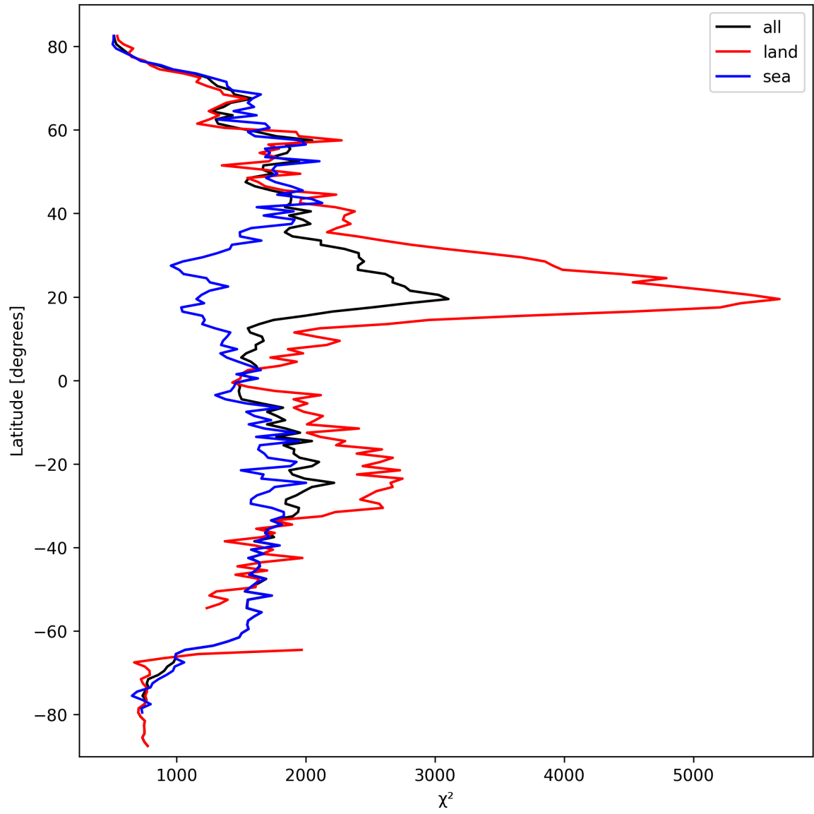
Figure 10: Zonal average of “ \chi^2 ” for 2025-09-28 to 2025-09-29.
