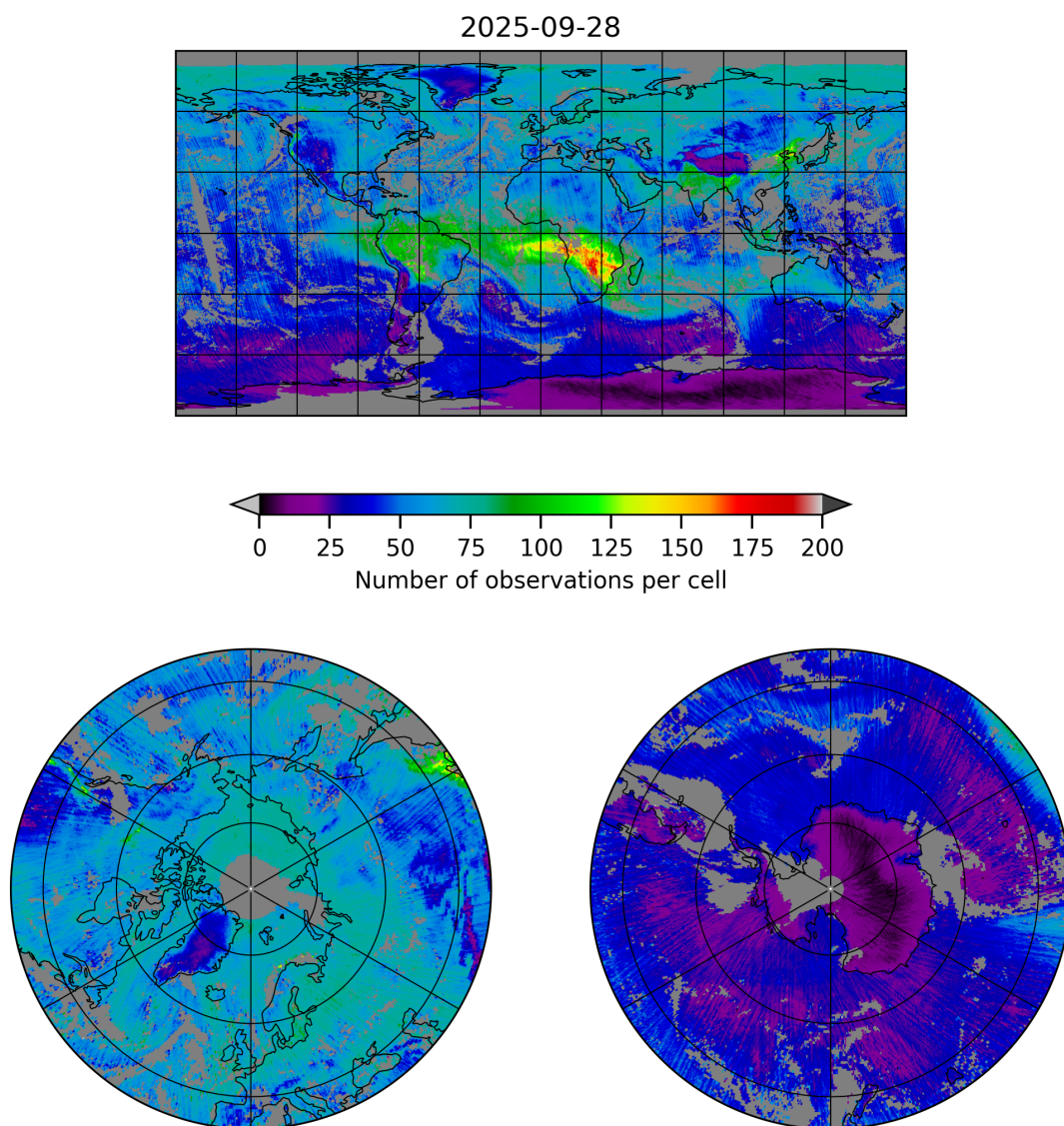
Figure 5: Map of the number of observations for 2025-09-28 to 2025-09-29
