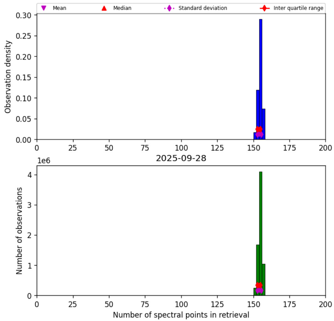
Figure 16: Histogram of “Number of spectral points in retrieval” for 2025-09-28 to 2025-09-29
