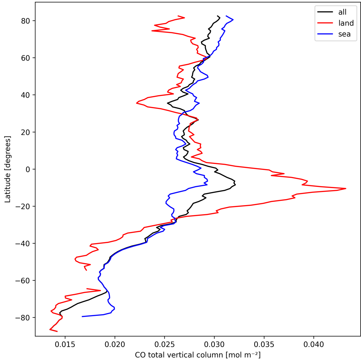
Figure 7: Zonal average of “CO total vertical column” for 2025-09-28 to 2025-09-29.
