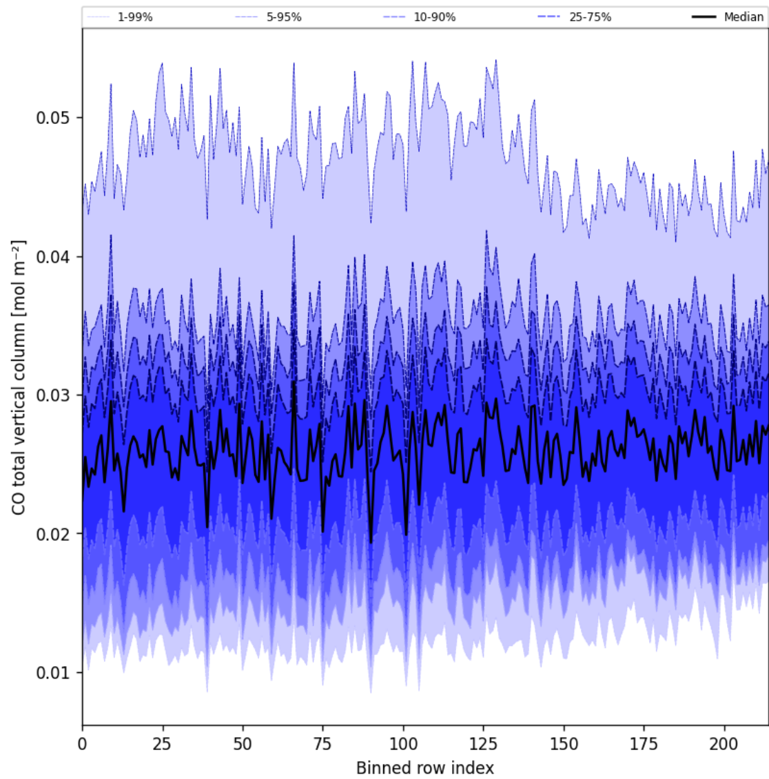
Figure 21: Along track statistics of “CO total vertical column” for 2025-09-28 to 2025-09-29
