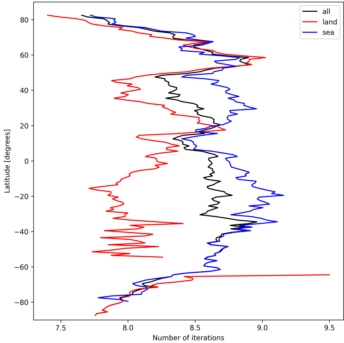
Figure 12: Zonal average of “Number of iterations” for 2025-09-28 to 2025-09-29.
