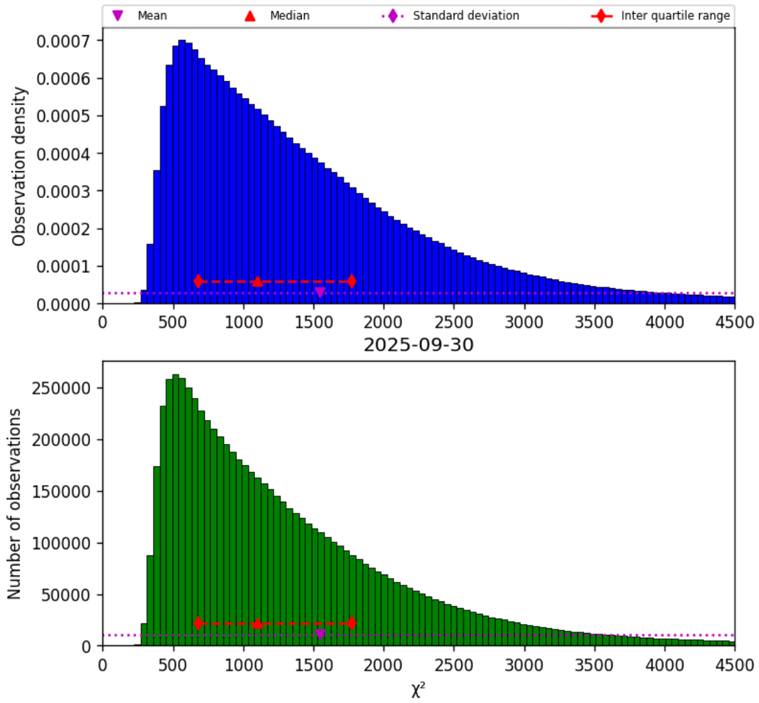
Figure 17: Histogram of “ \chi^2 ” for 2025-09-30 to 2025-10-01
