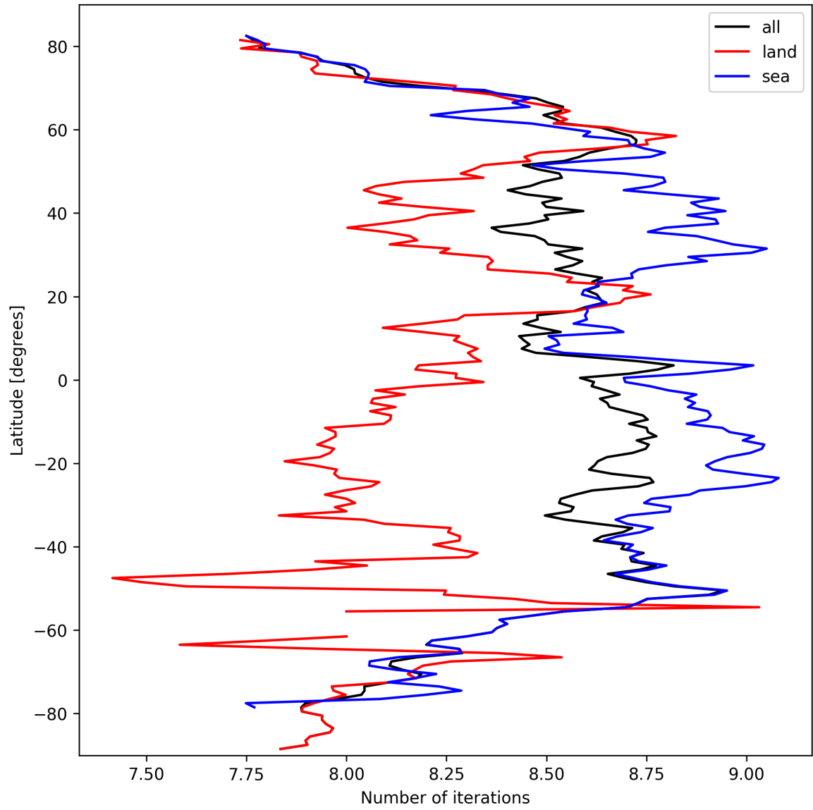
Figure 12: Zonal average of “Number of iterations” for 2025-09-30 to 2025-10-01.
