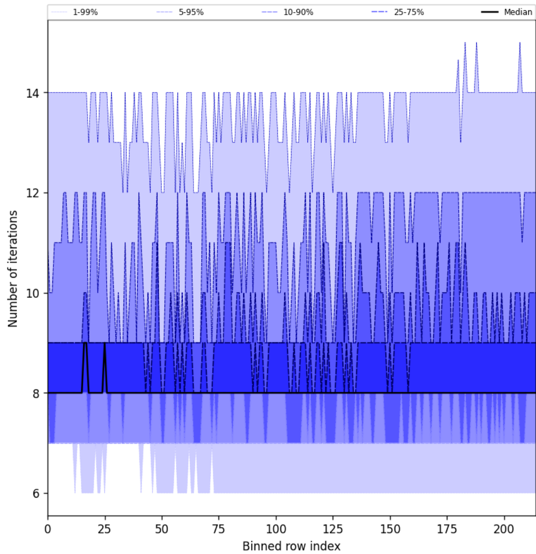
Figure 26: Along track statistics of “Number of iterations” for 2025-09-30 to 2025-10-01
