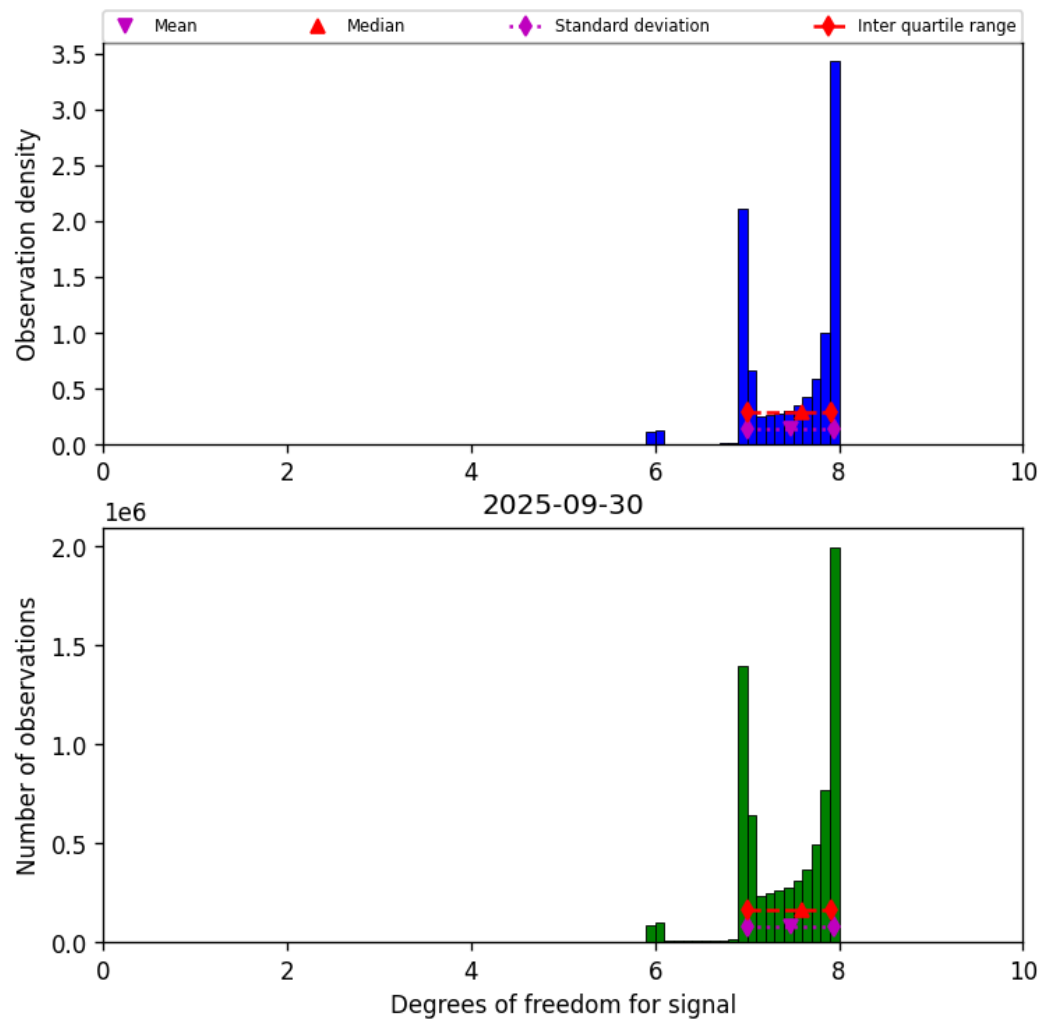
Figure 18: Histogram of “Degrees of freedom for signal” for 2025-09-30 to 2025-10-01
