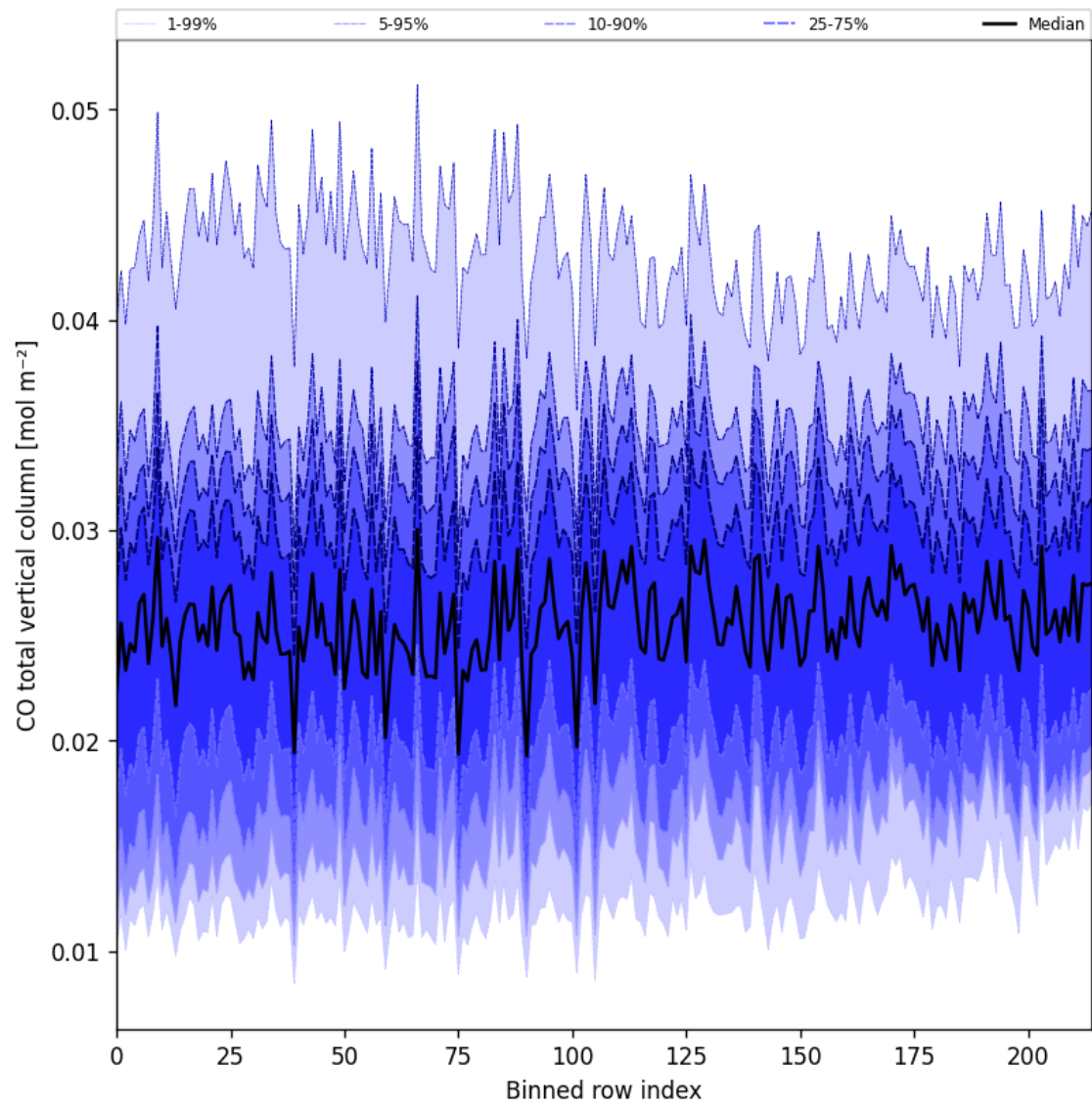
Figure 21: Along track statistics of “CO total vertical column” for 2025-09-30 to 2025-10-01
