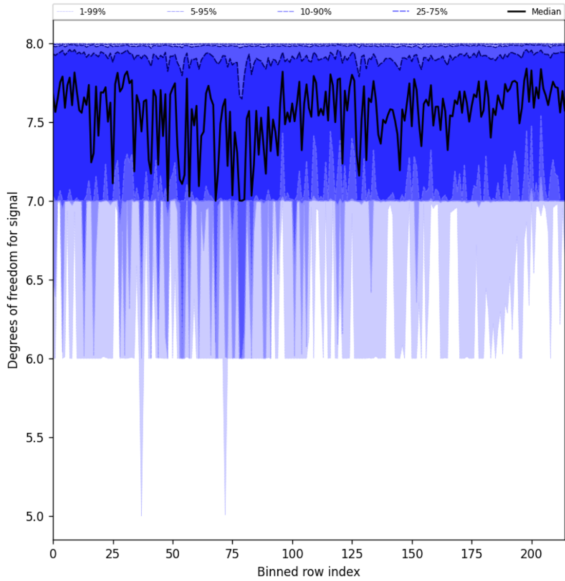
Figure 25: Along track statistics of “Degrees of freedom for signal” for 2025-09-30 to 2025-10-01
