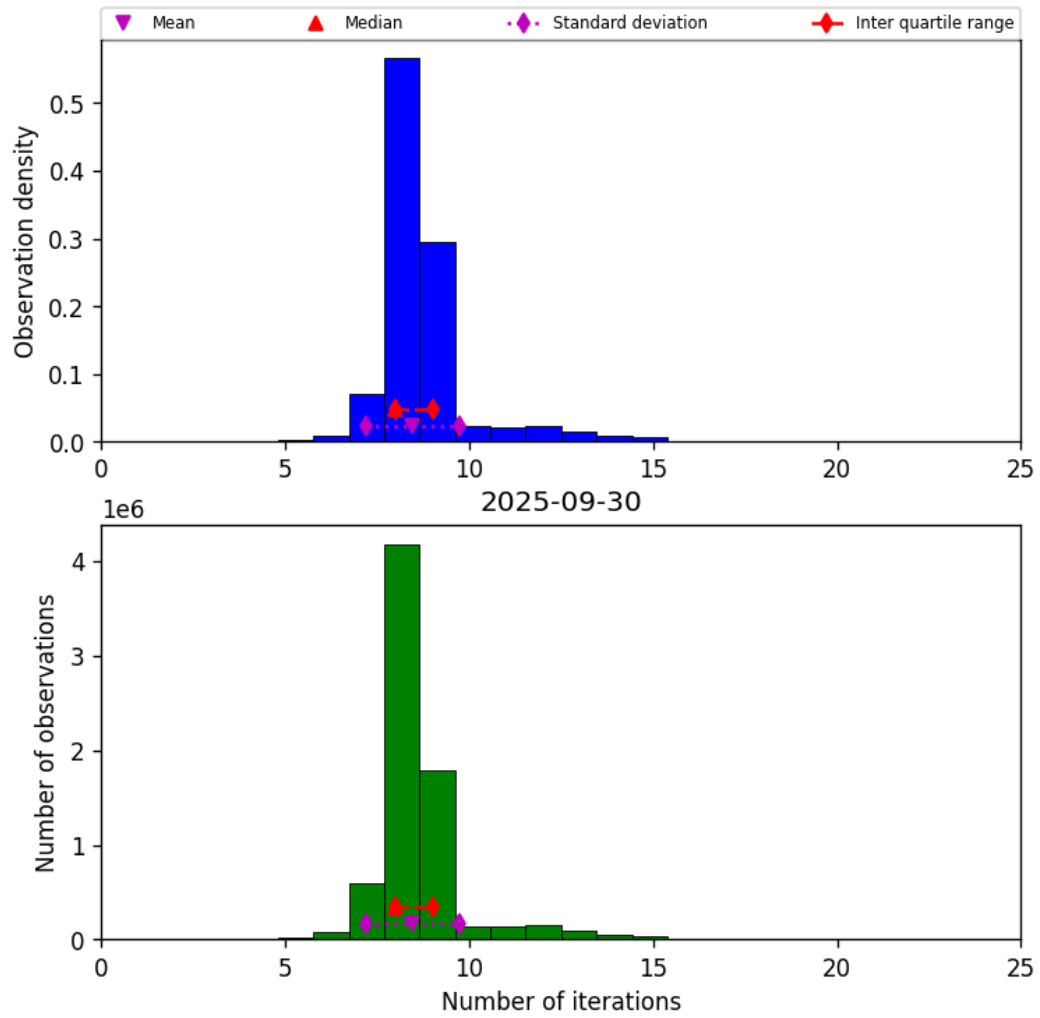
Figure 19: Histogram of “Number of iterations” for 2025-09-30 to 2025-10-01
