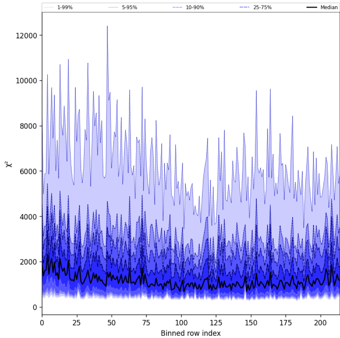
Figure 24: Along track statistics of “ \chi^2 ” for 2025-09-30 to 2025-10-01
