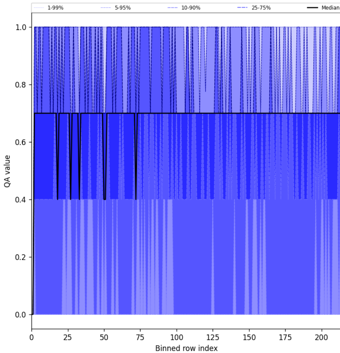
Figure 20: Along track statistics of “QA value” for 2025-09-30 to 2025-10-01
