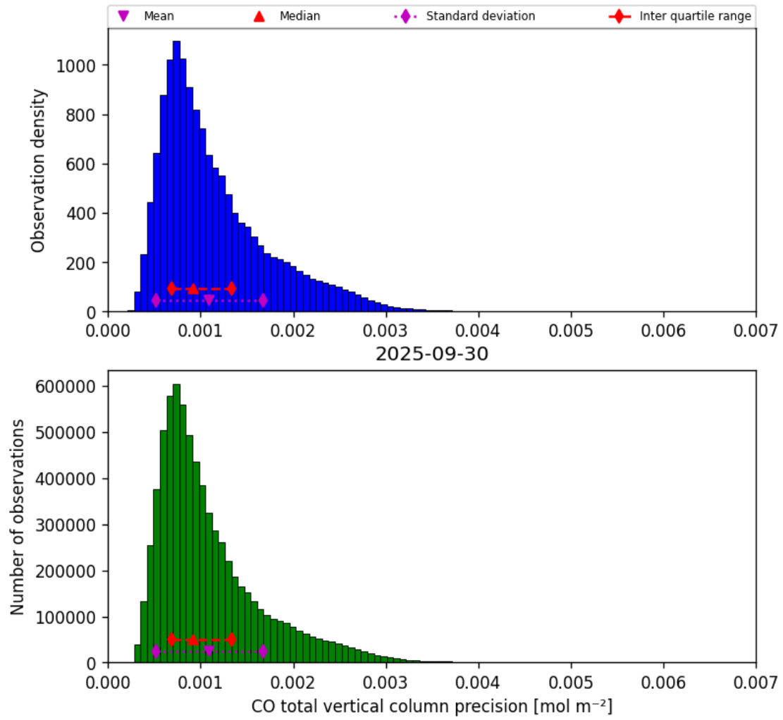
Figure 15: Histogram of “CO total vertical column precision” for 2025-09-30 to 2025-10-01
