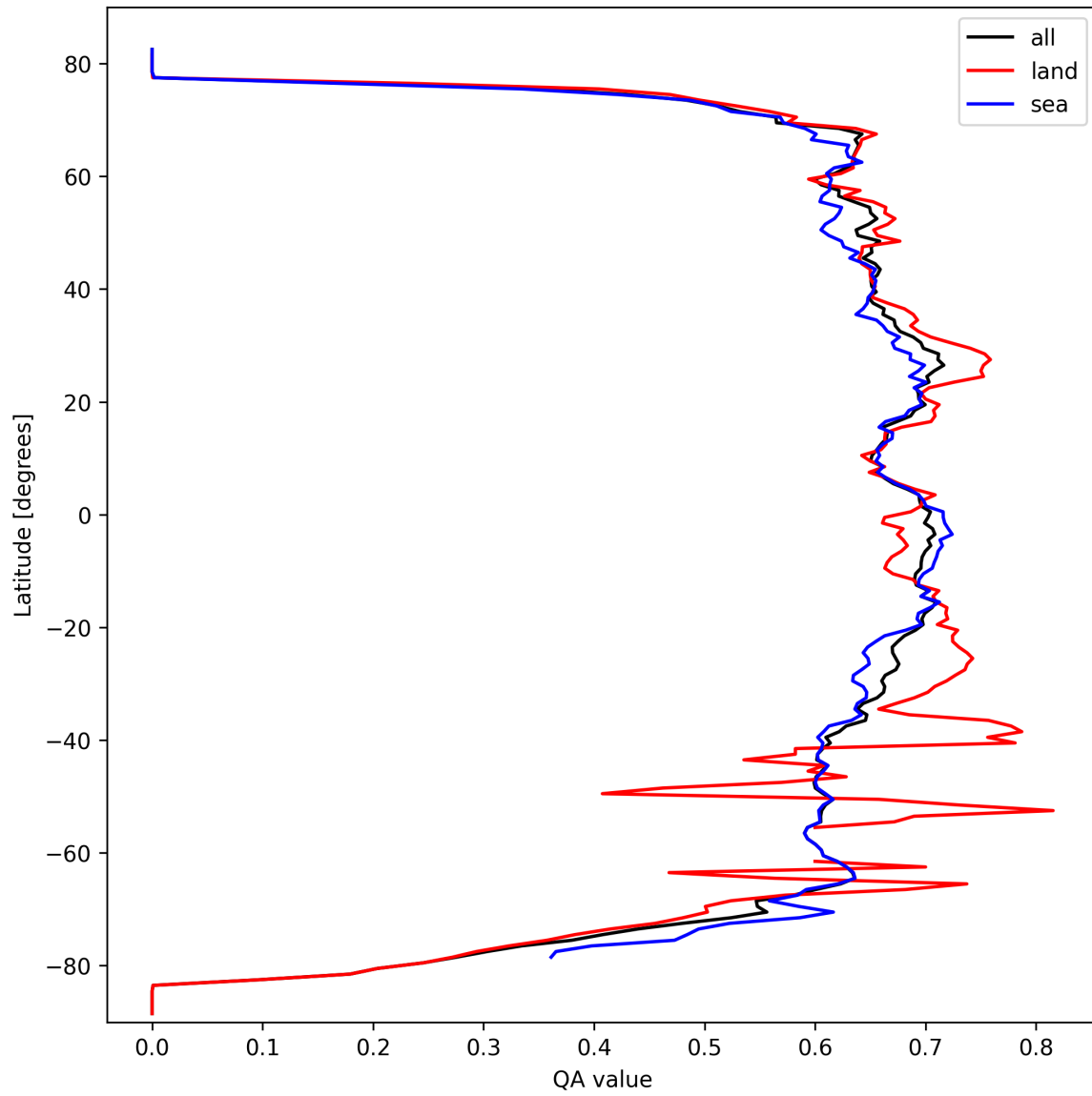
Figure 6: Zonal average of “QA value” for 2025-09-30 to 2025-10-01.
