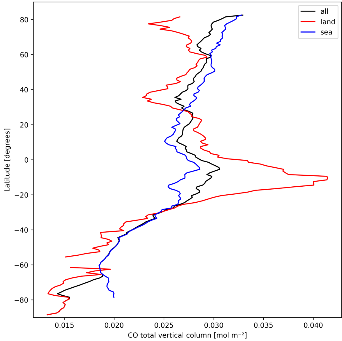
Figure 7: Zonal average of “CO total vertical column” for 2025-09-30 to 2025-10-01.
