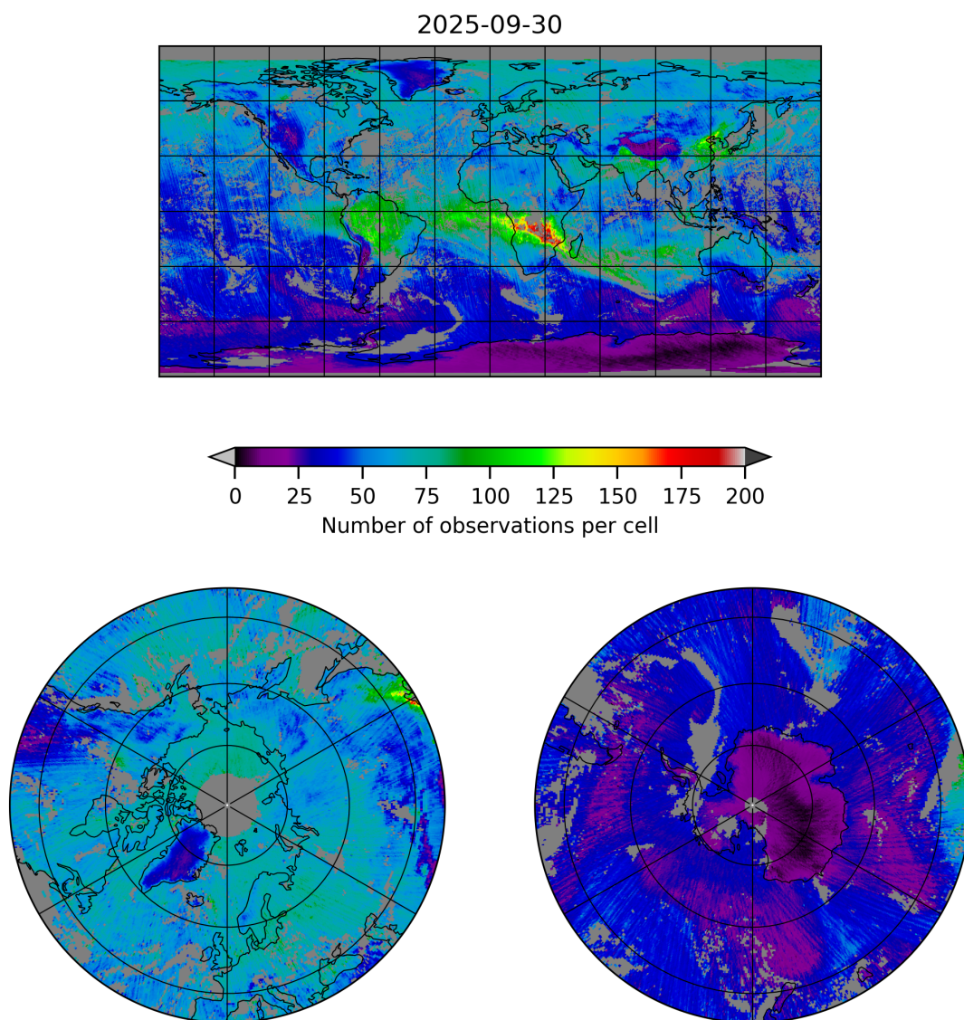
Figure 5: Map of the number of observations for 2025-09-30 to 2025-10-01
