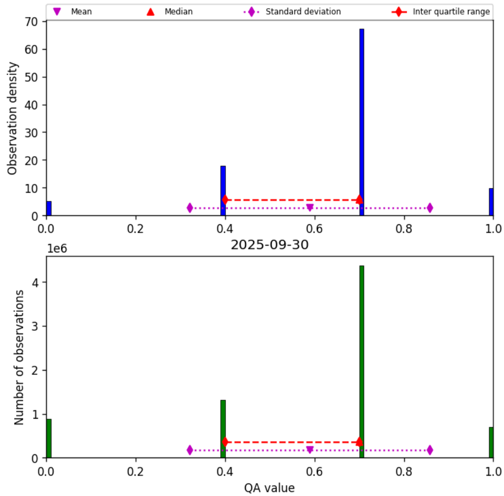
Figure 13: Histogram of “QA value” for 2025-09-30 to 2025-10-01
