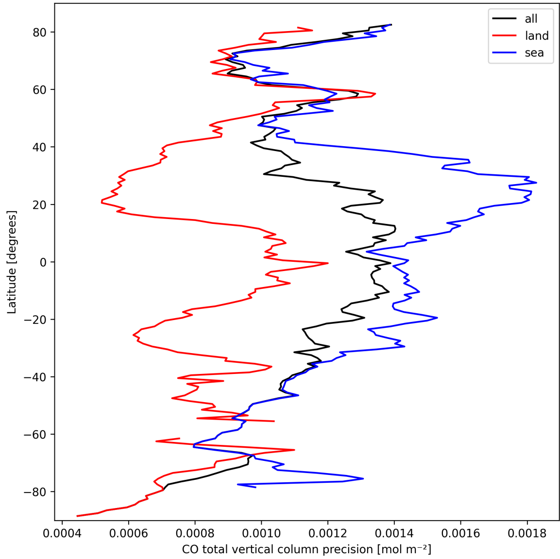
Figure 8: Zonal average of “CO total vertical column precision” for 2025-09-30 to 2025-10-01.
