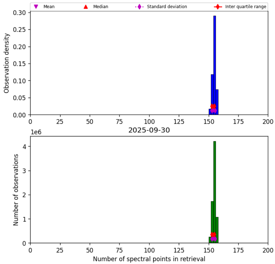
Figure 16: Histogram of “Number of spectral points in retrieval” for 2025-09-30 to 2025-10-01
