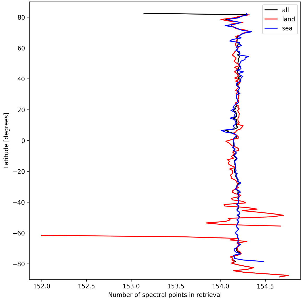
Figure 9: Zonal average of “Number of spectral points in retrieval” for 2025-09-30 to 2025-10-01.
