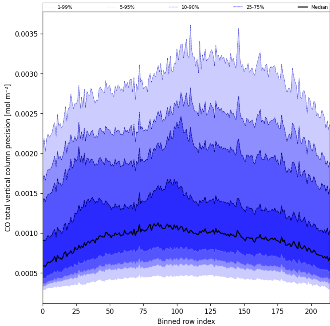
Figure 22: Along track statistics of “CO total vertical column precision” for 2025-09-30 to 2025-10-01
