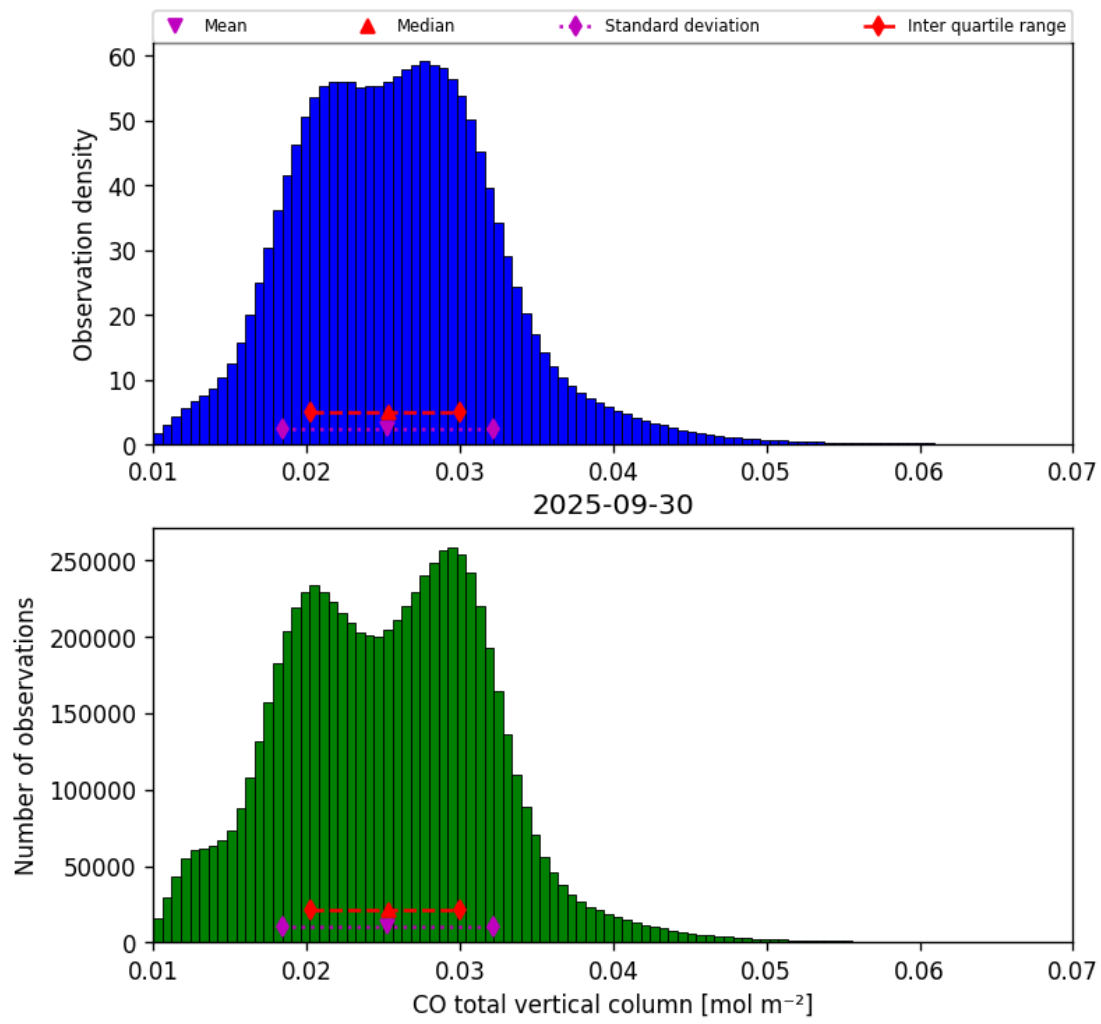
Figure 14: Histogram of “CO total vertical column” for 2025-09-30 to 2025-10-01
