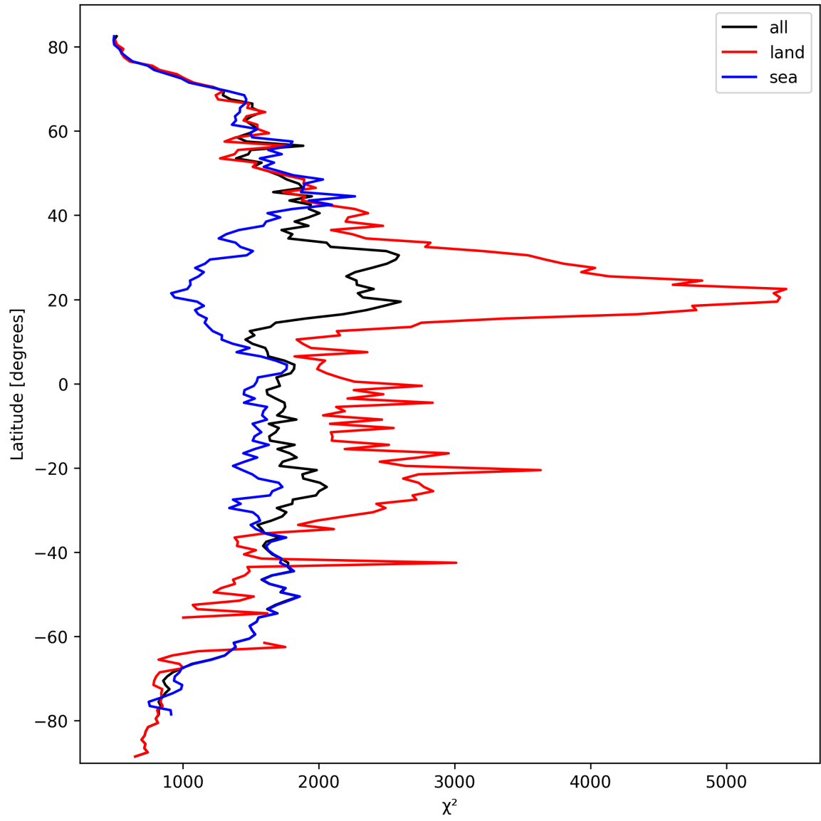
Figure 10: Zonal average of “ \chi^2 ” for 2025-09-30 to 2025-10-01.
