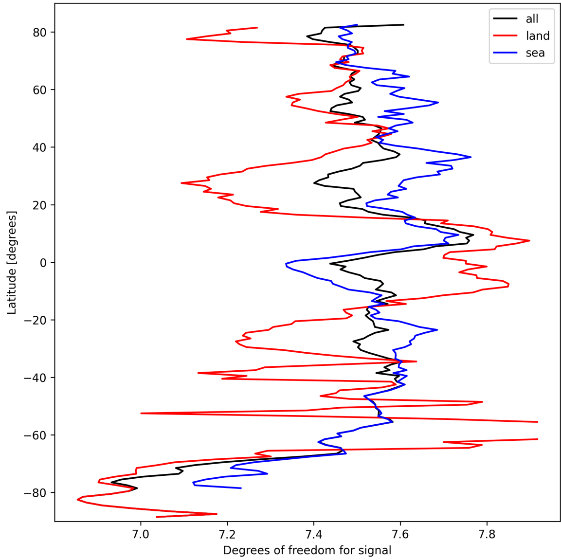
Figure 11: Zonal average of “Degrees of freedom for signal” for 2025-09-30 to 2025-10-01.
