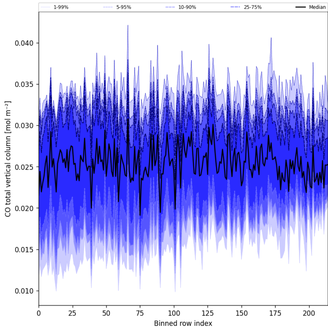
Figure 21: Along track statistics of “CO total vertical column” for 2025-10-02 to 2025-10-03
