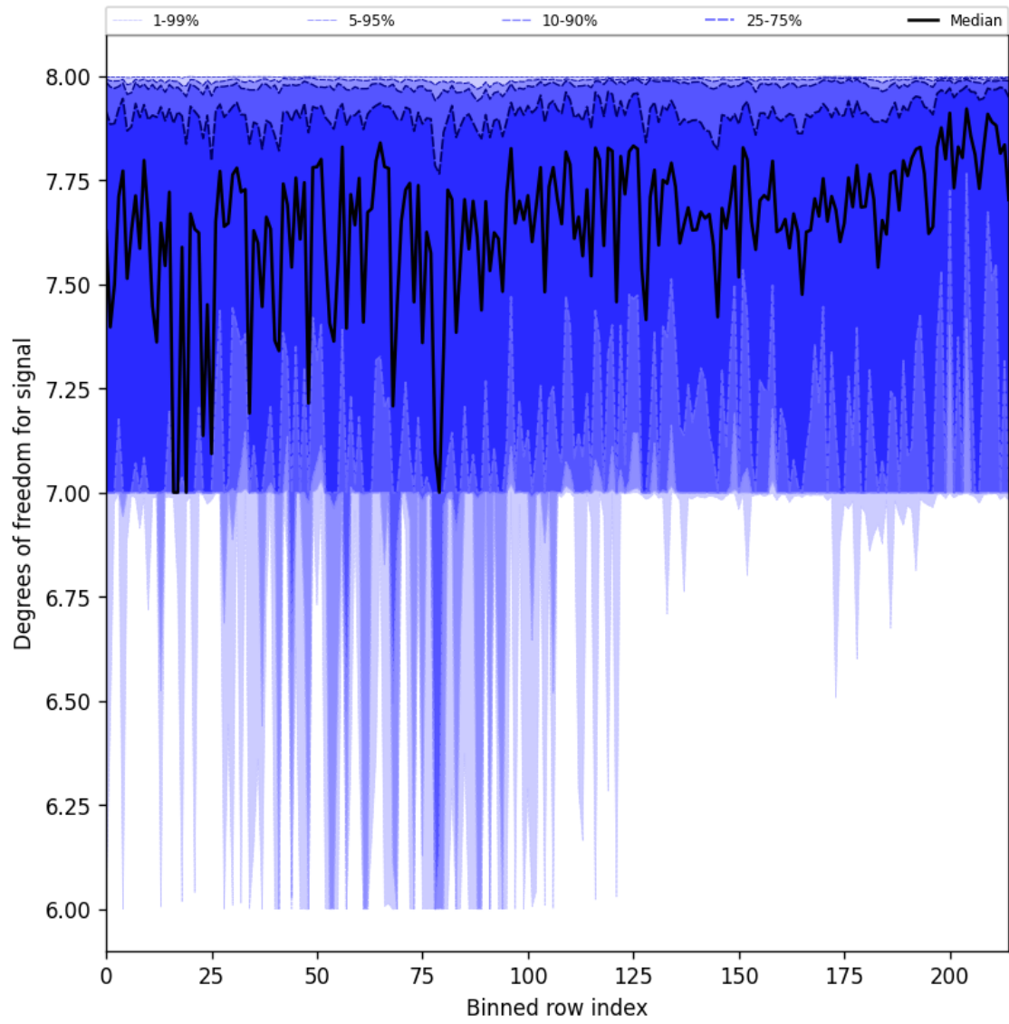
Figure 25: Along track statistics of “Degrees of freedom for signal” for 2025-10-02 to 2025-10-03
