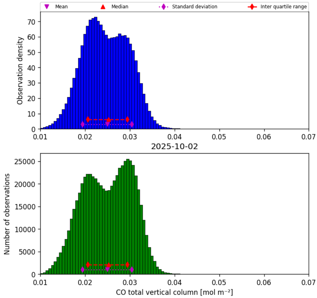
Figure 14: Histogram of “CO total vertical column” for 2025-10-02 to 2025-10-03
