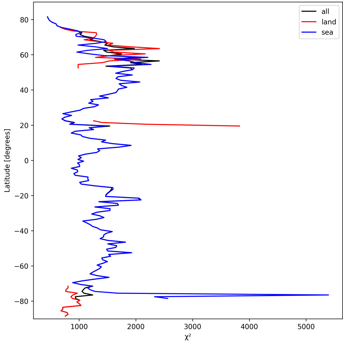
Figure 10: Zonal average of “ \chi^2 ” for 2025-10-02 to 2025-10-03.
