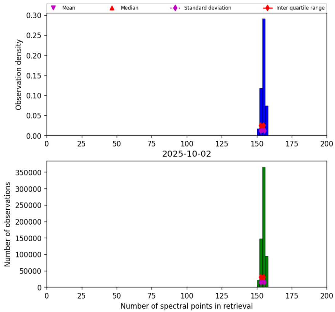
Figure 16: Histogram of “Number of spectral points in retrieval” for 2025-10-02 to 2025-10-03
