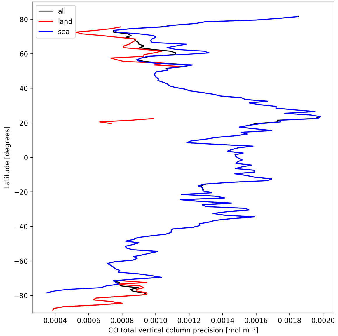
Figure 8: Zonal average of “CO total vertical column precision” for 2025-10-02 to 2025-10-03.
