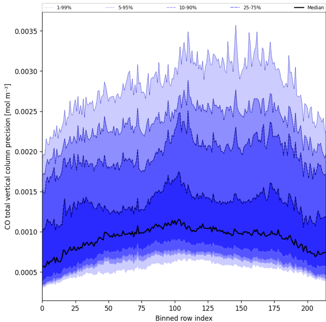
Figure 22: Along track statistics of “CO total vertical column precision” for 2025-10-02 to 2025-10-03
