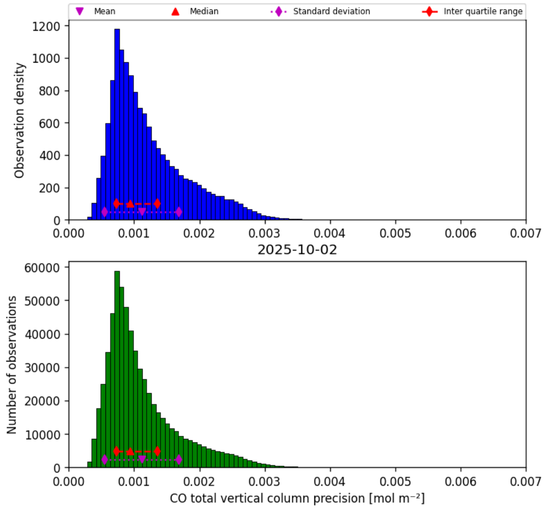
Figure 15: Histogram of “CO total vertical column precision” for 2025-10-02 to 2025-10-03
