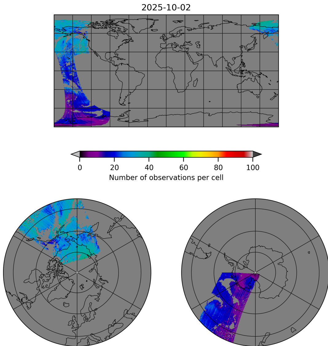
Figure 5: Map of the number of observations for 2025-10-02 to 2025-10-03
