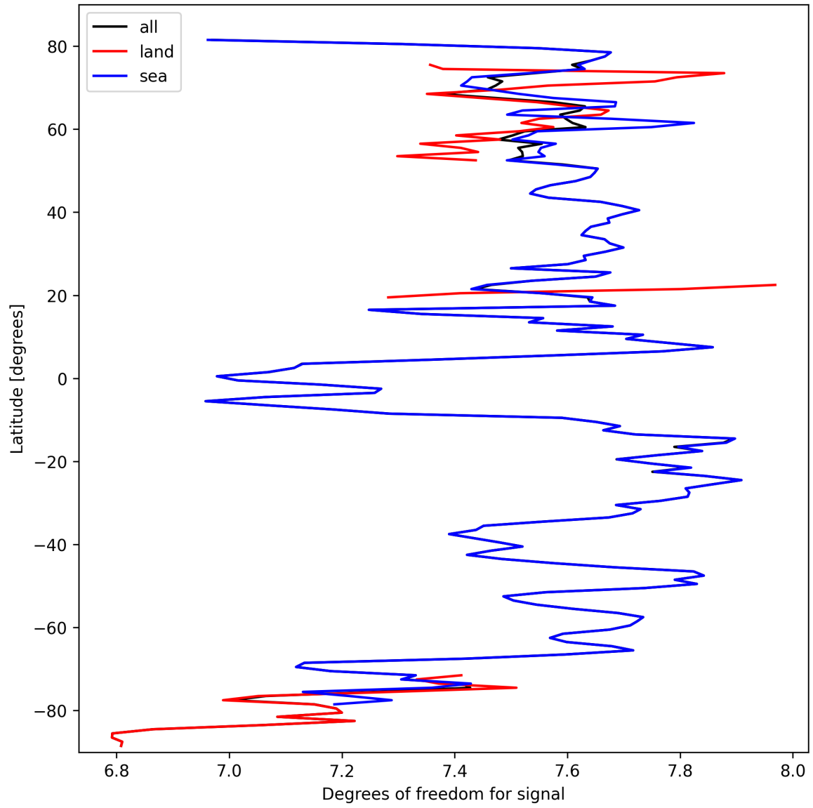
Figure 11: Zonal average of “Degrees of freedom for signal” for 2025-10-02 to 2025-10-03.
