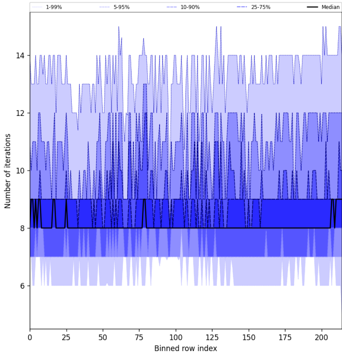
Figure 26: Along track statistics of “Number of iterations” for 2025-10-02 to 2025-10-03
