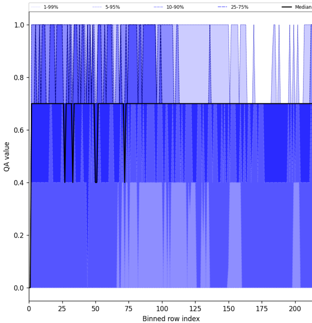
Figure 20: Along track statistics of “QA value” for 2025-10-02 to 2025-10-03
