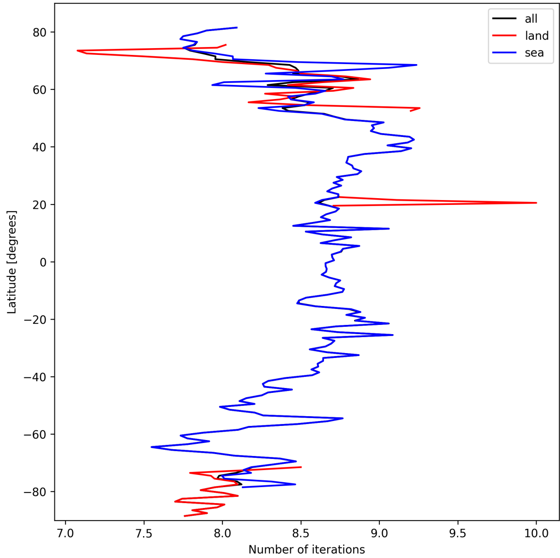
Figure 12: Zonal average of “Number of iterations” for 2025-10-02 to 2025-10-03.
