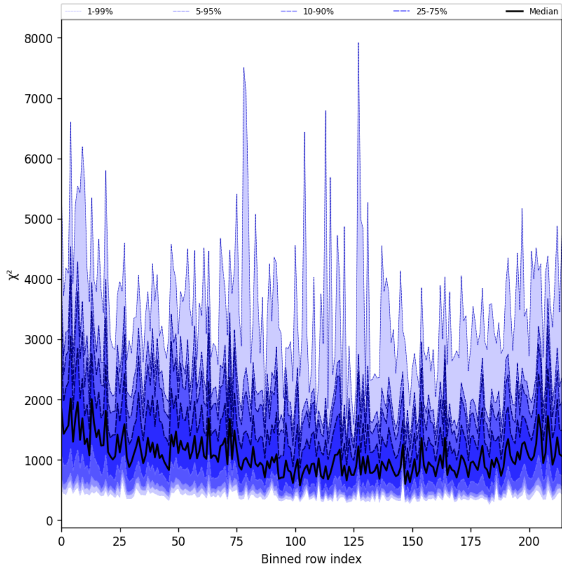
Figure 24: Along track statistics of “ \chi^2 ” for 2025-10-02 to 2025-10-03
