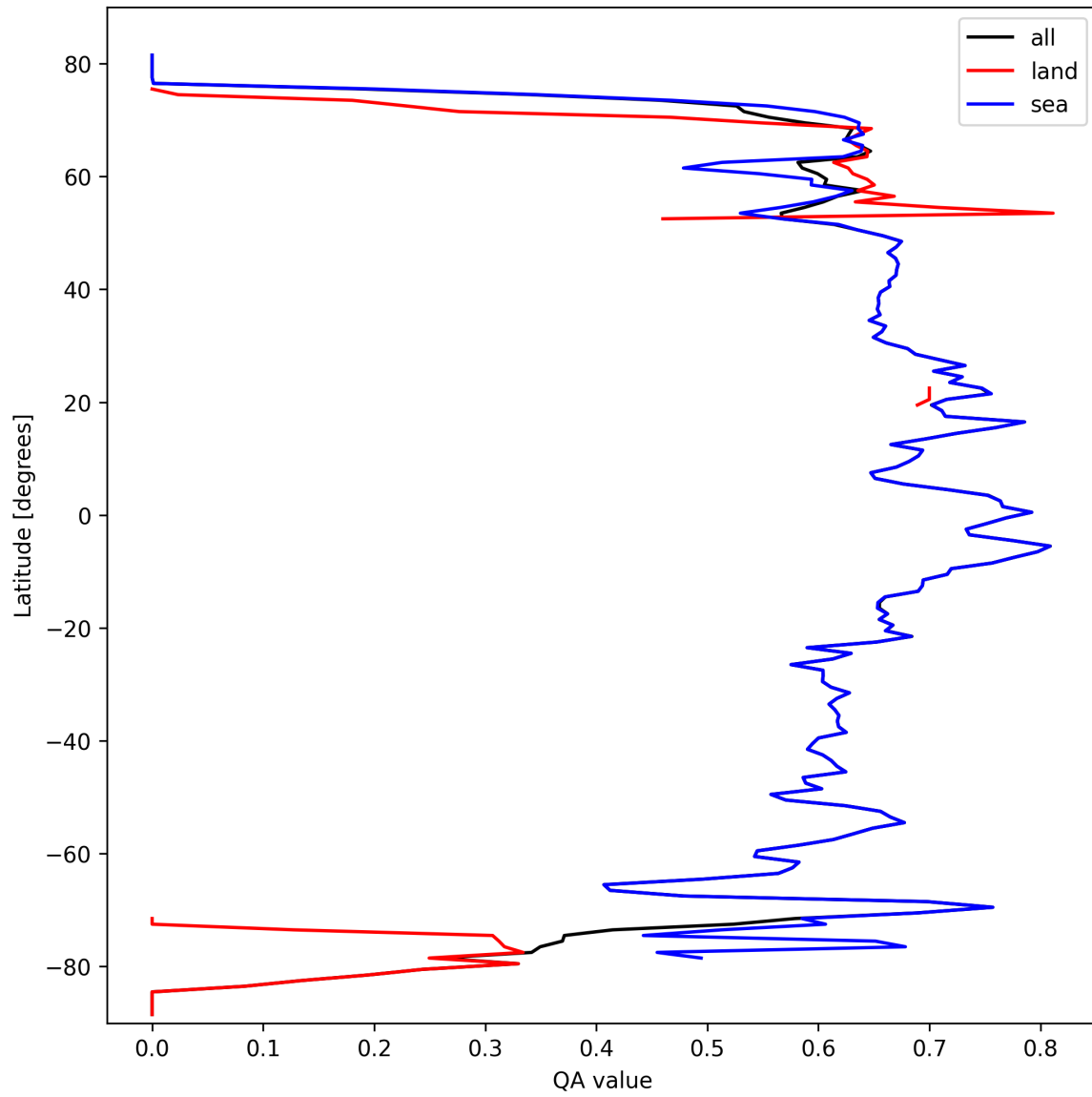
Figure 6: Zonal average of “QA value” for 2025-10-02 to 2025-10-03.
