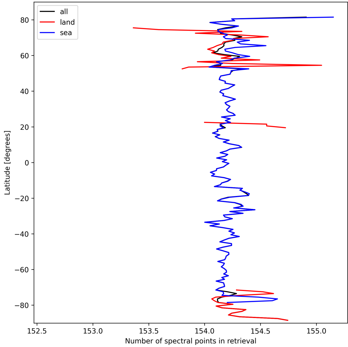
Figure 9: Zonal average of “Number of spectral points in retrieval” for 2025-10-02 to 2025-10-03.
