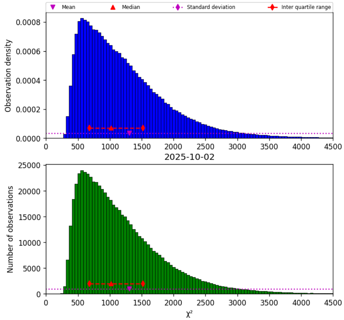
Figure 17: Histogram of “ \chi^2 ” for 2025-10-02 to 2025-10-03
