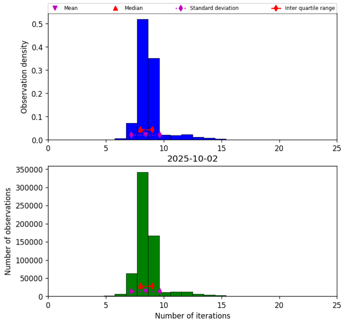
Figure 19: Histogram of “Number of iterations” for 2025-10-02 to 2025-10-03
