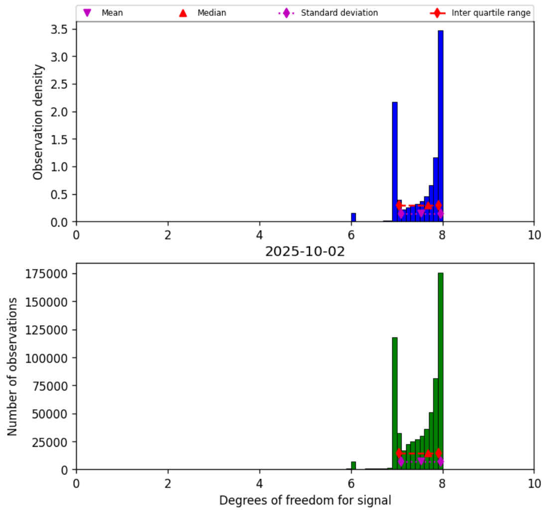
Figure 18: Histogram of “Degrees of freedom for signal” for 2025-10-02 to 2025-10-03
