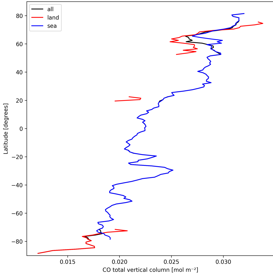
Figure 7: Zonal average of “CO total vertical column” for 2025-10-02 to 2025-10-03.
