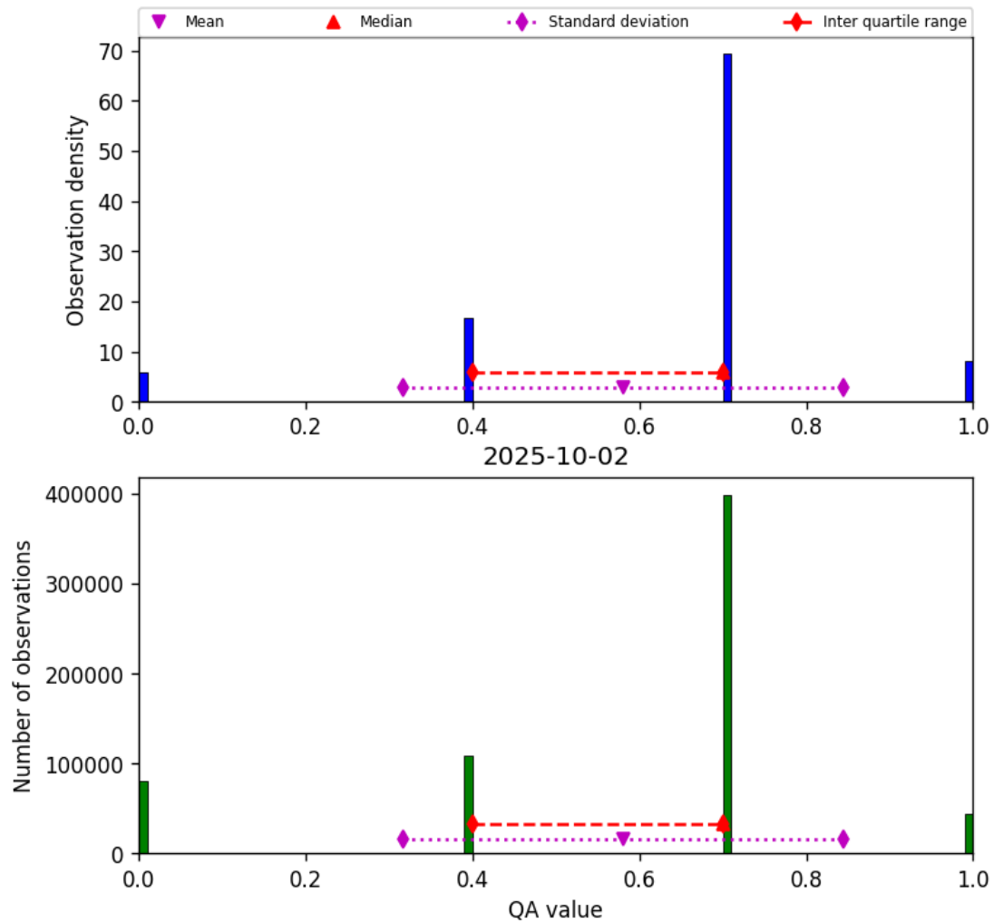
Figure 13: Histogram of “QA value” for 2025-10-02 to 2025-10-03
