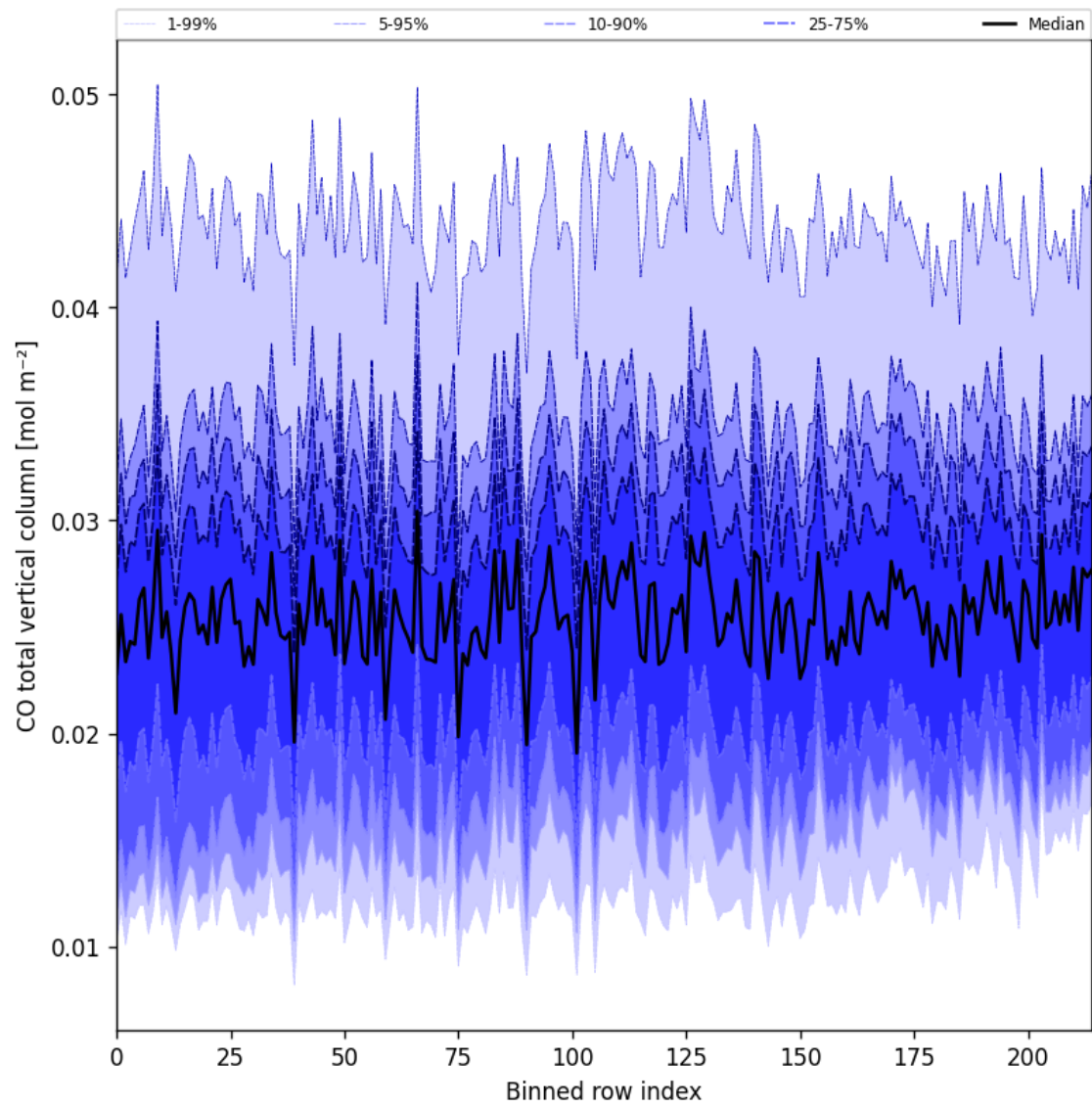
Figure 21: Along track statistics of “CO total vertical column” for 2025-10-03 to 2025-10-04
