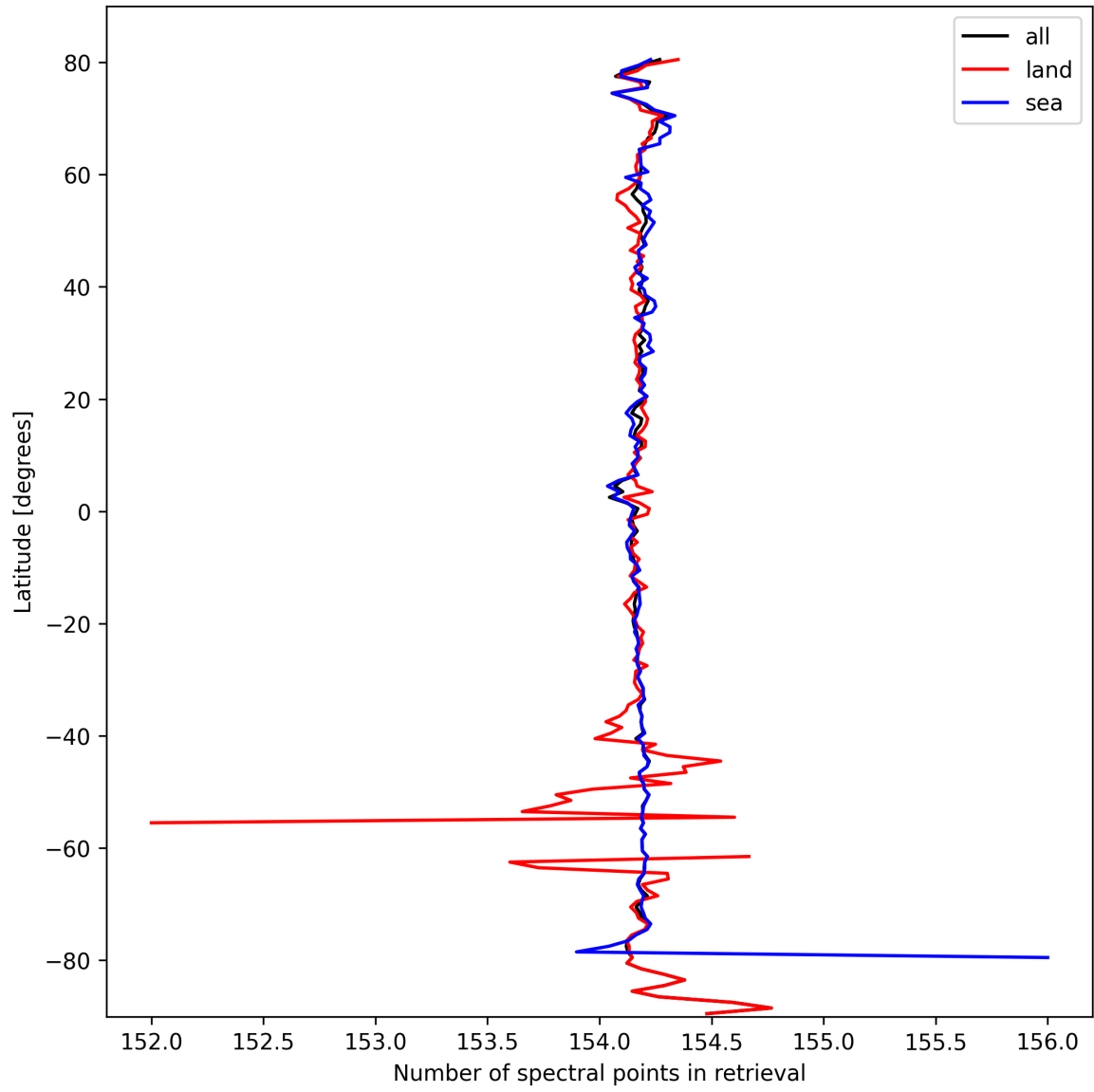
Figure 9: Zonal average of “Number of spectral points in retrieval” for 2025-10-03 to 2025-10-04.
