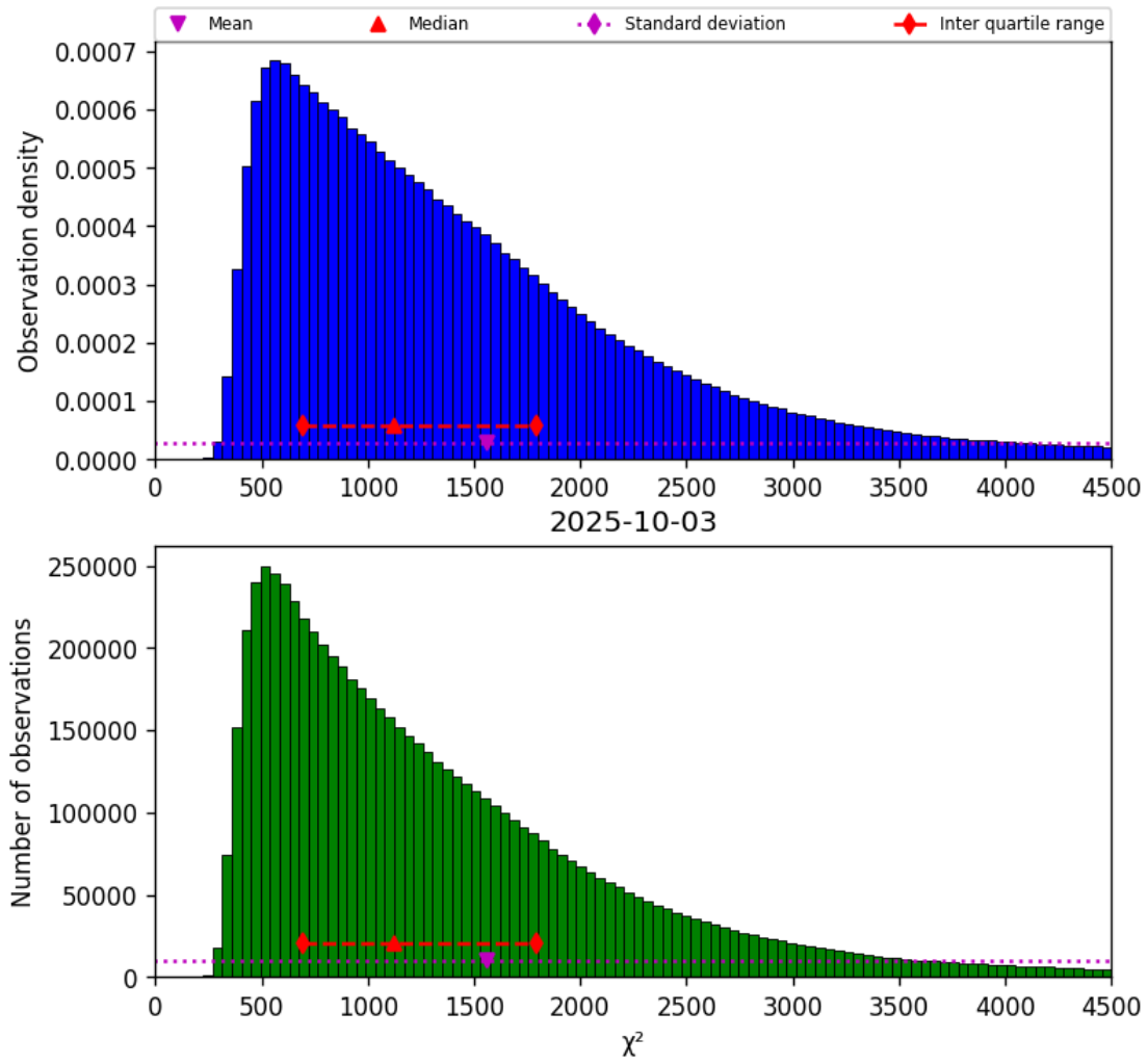
Figure 17: Histogram of " \chi^2 " for 2025-10-03 to 2025-10-04
