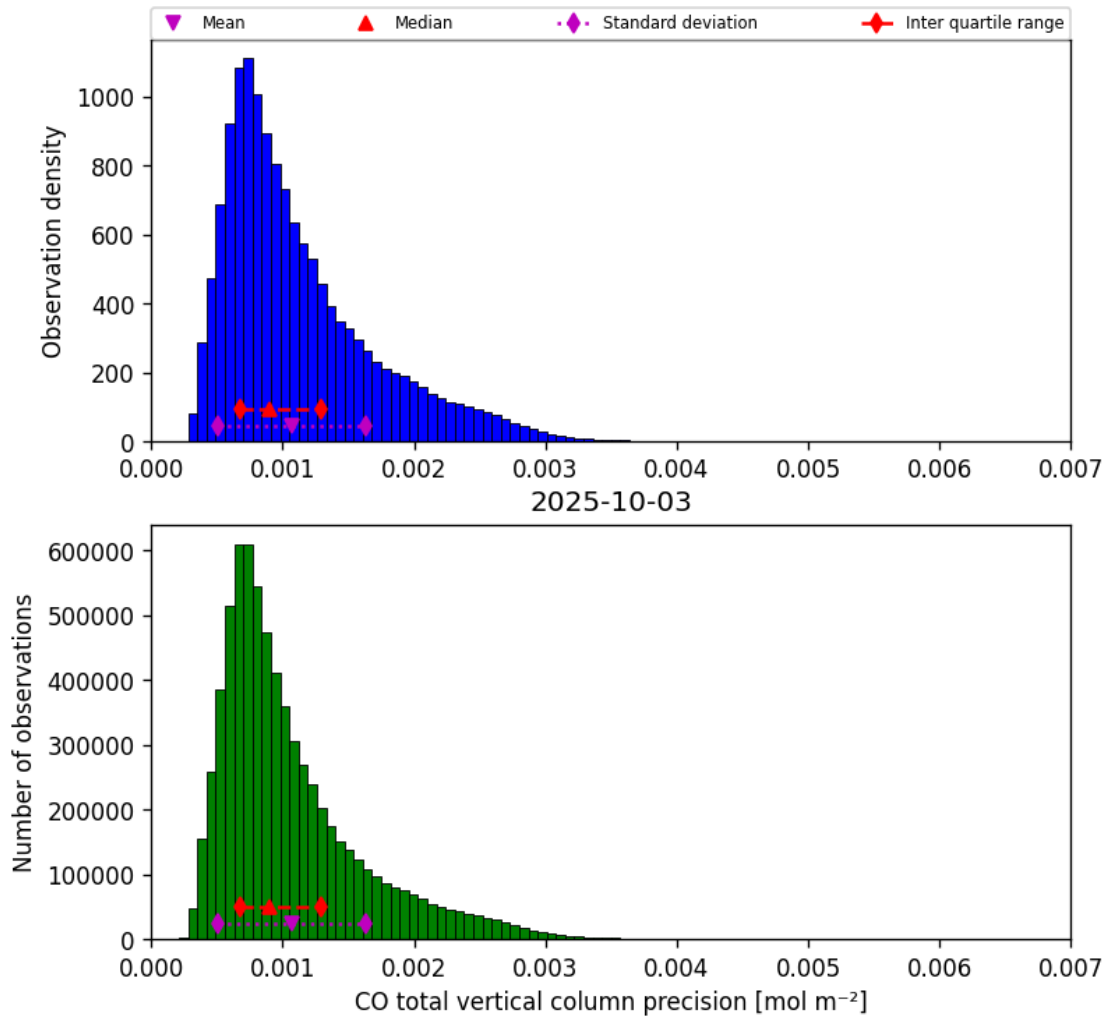
Figure 15: Histogram of “CO total vertical column precision” for 2025-10-03 to 2025-10-04
