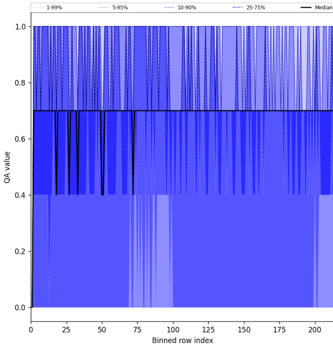
Figure 20: Along track statistics of “QA value” for 2025-10-03 to 2025-10-04
