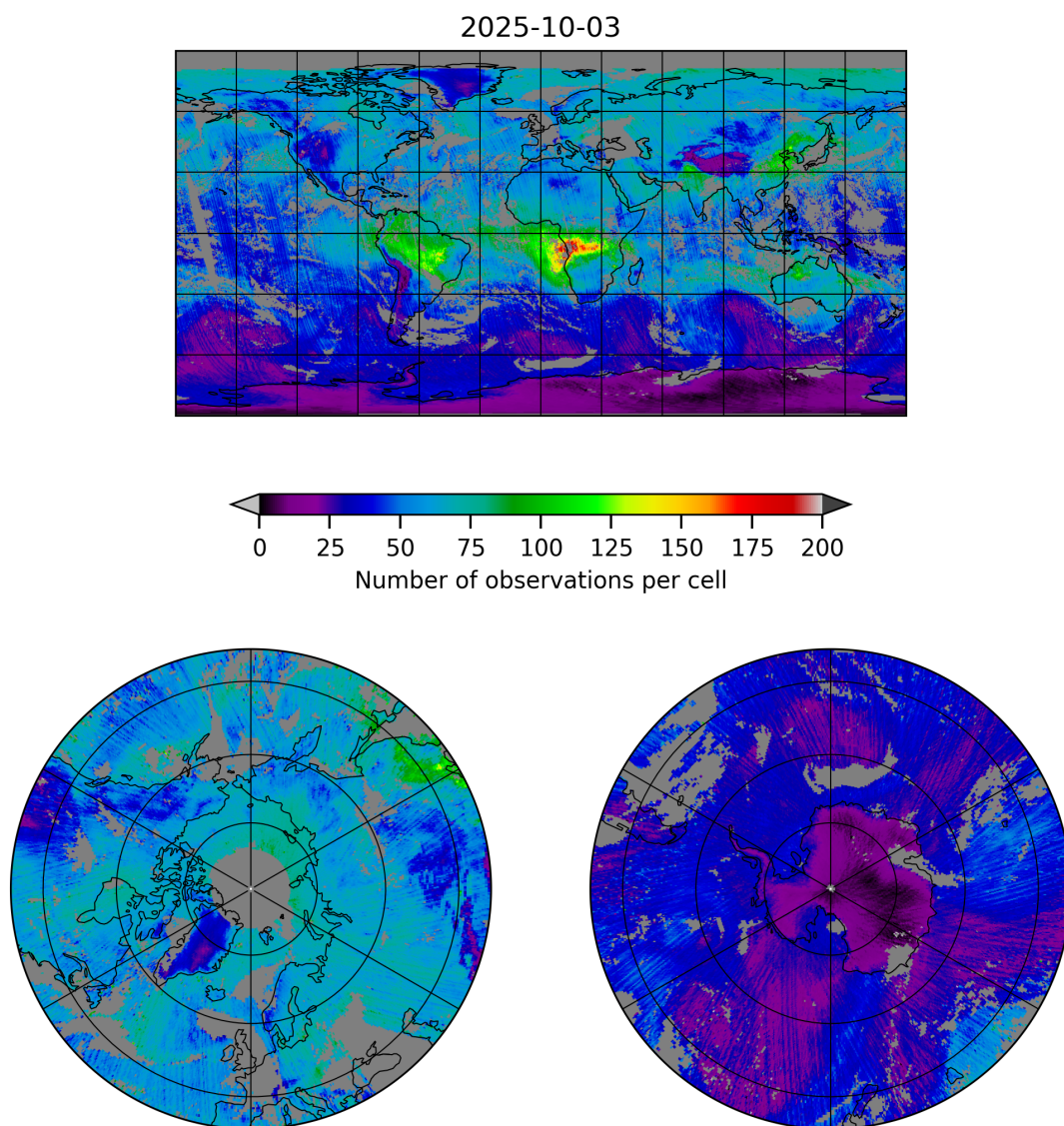
Figure 5: Map of the number of observations for 2025-10-03 to 2025-10-04
