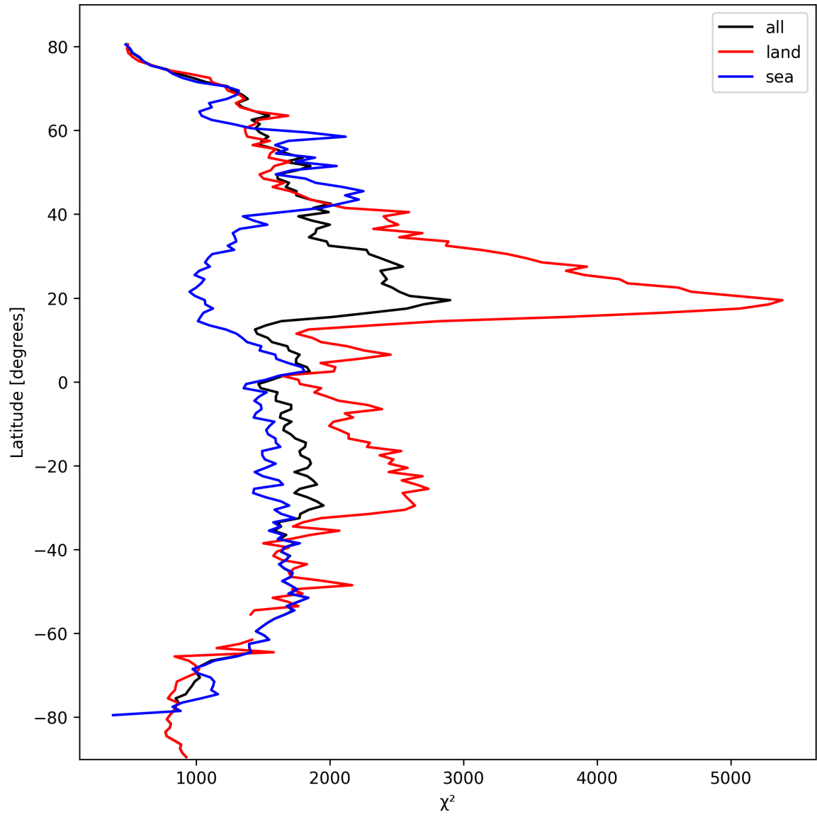
Figure 10: Zonal average of “ \chi^2 ” for 2025-10-03 to 2025-10-04.
