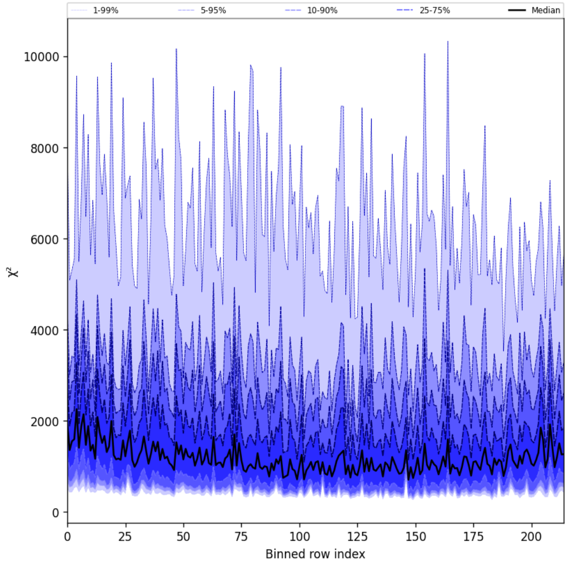
Figure 24: Along track statistics of “ \chi^2 ” for 2025-10-03 to 2025-10-04
