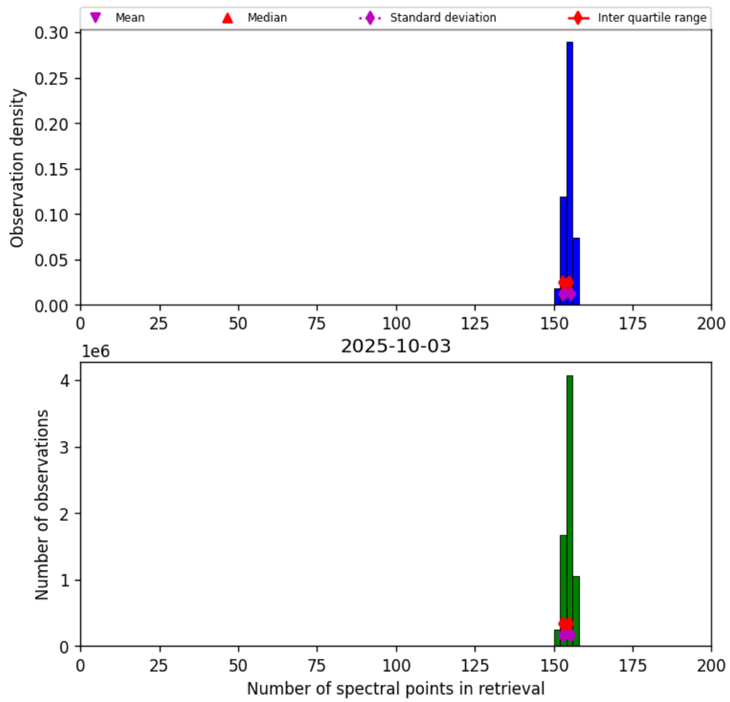
Figure 16: Histogram of “Number of spectral points in retrieval” for 2025-10-03 to 2025-10-04
