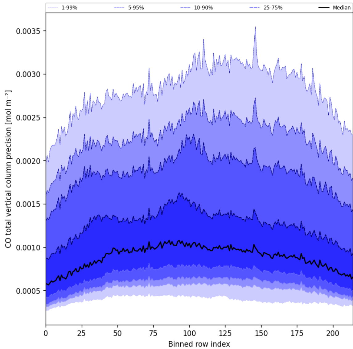
Figure 22: Along track statistics of “CO total vertical column precision” for 2025-10-03 to 2025-10-04
