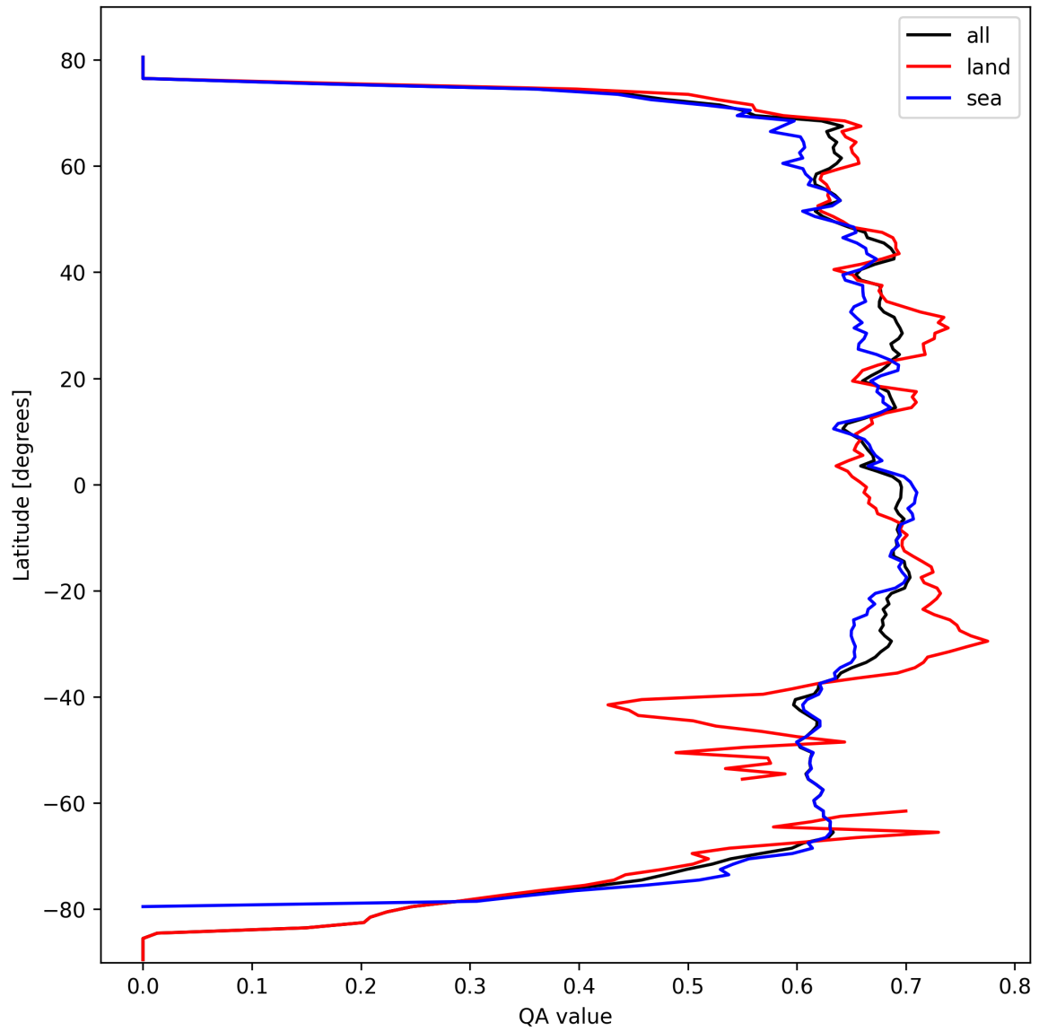
Figure 6: Zonal average of “QA value” for 2025-10-03 to 2025-10-04.
