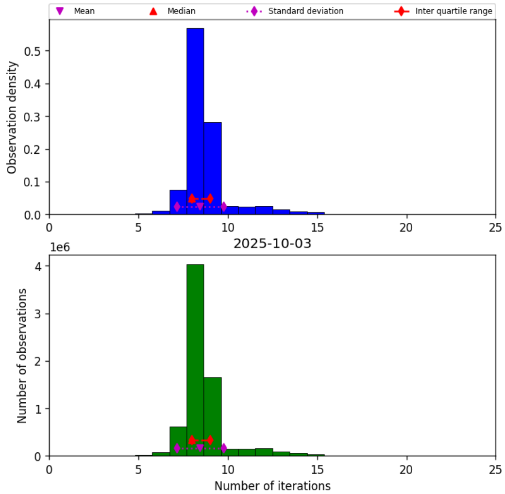
Figure 19: Histogram of “Number of iterations” for 2025-10-03 to 2025-10-04
