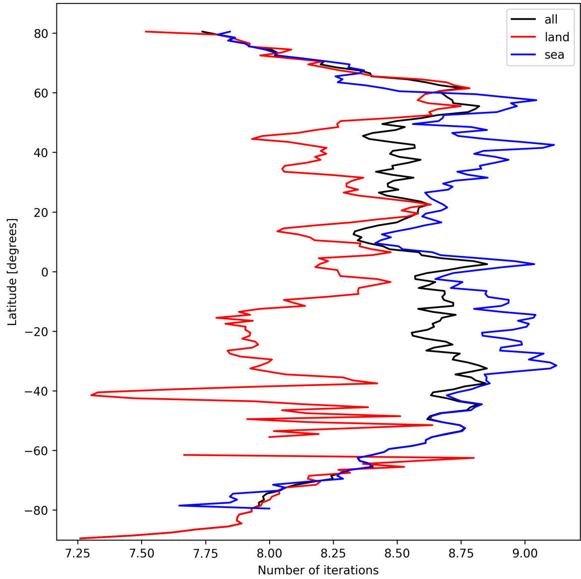
Figure 12: Zonal average of “Number of iterations” for 2025-10-03 to 2025-10-04.
