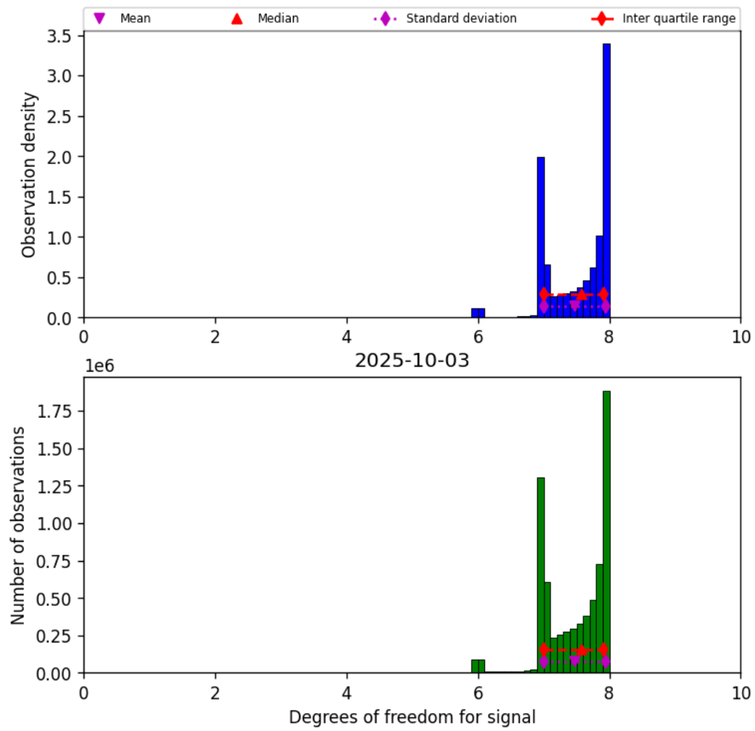
Figure 18: Histogram of “Degrees of freedom for signal” for 2025-10-03 to 2025-10-04
