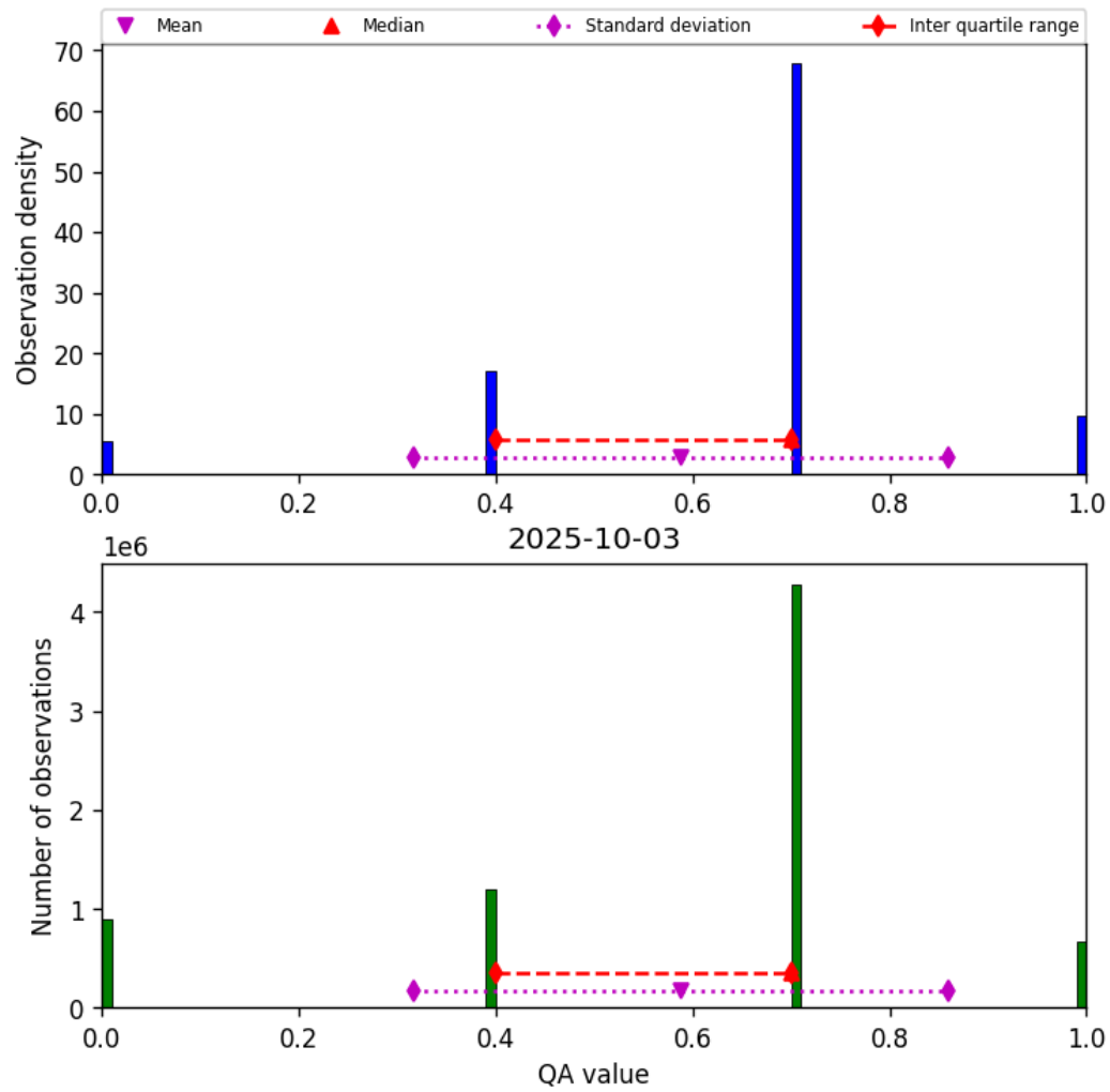
Figure 13: Histogram of “QA value” for 2025-10-03 to 2025-10-04
