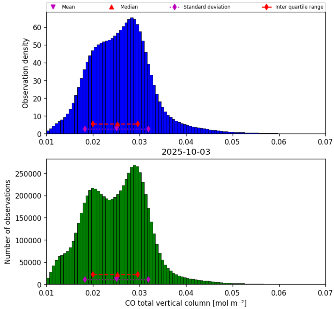
Figure 14: Histogram of “CO total vertical column” for 2025-10-03 to 2025-10-04
