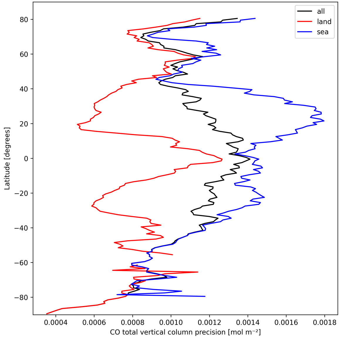
Figure 8: Zonal average of “CO total vertical column precision” for 2025-10-03 to 2025-10-04.
