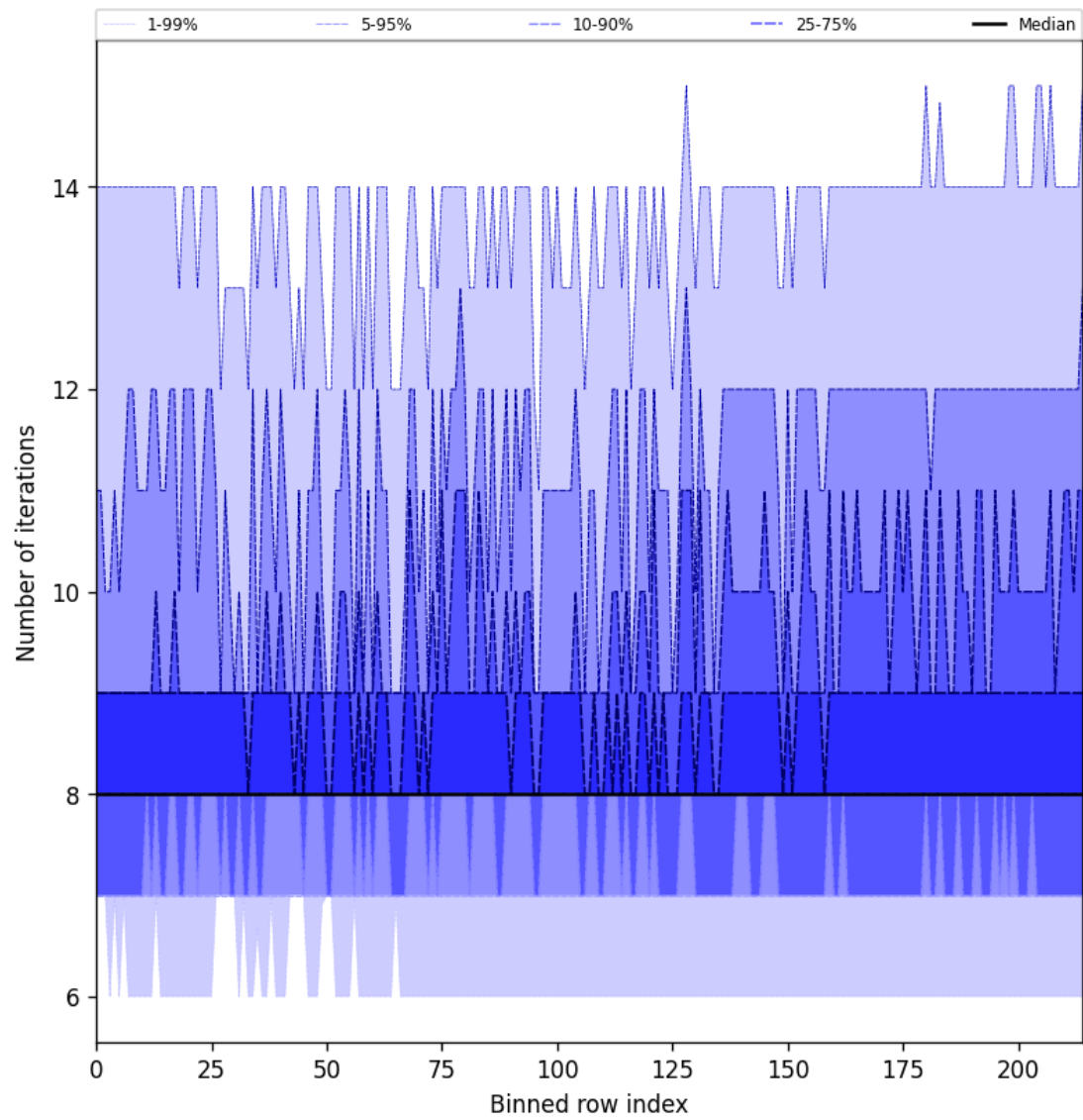
Figure 26: Along track statistics of “Number of iterations” for 2025-10-03 to 2025-10-04
