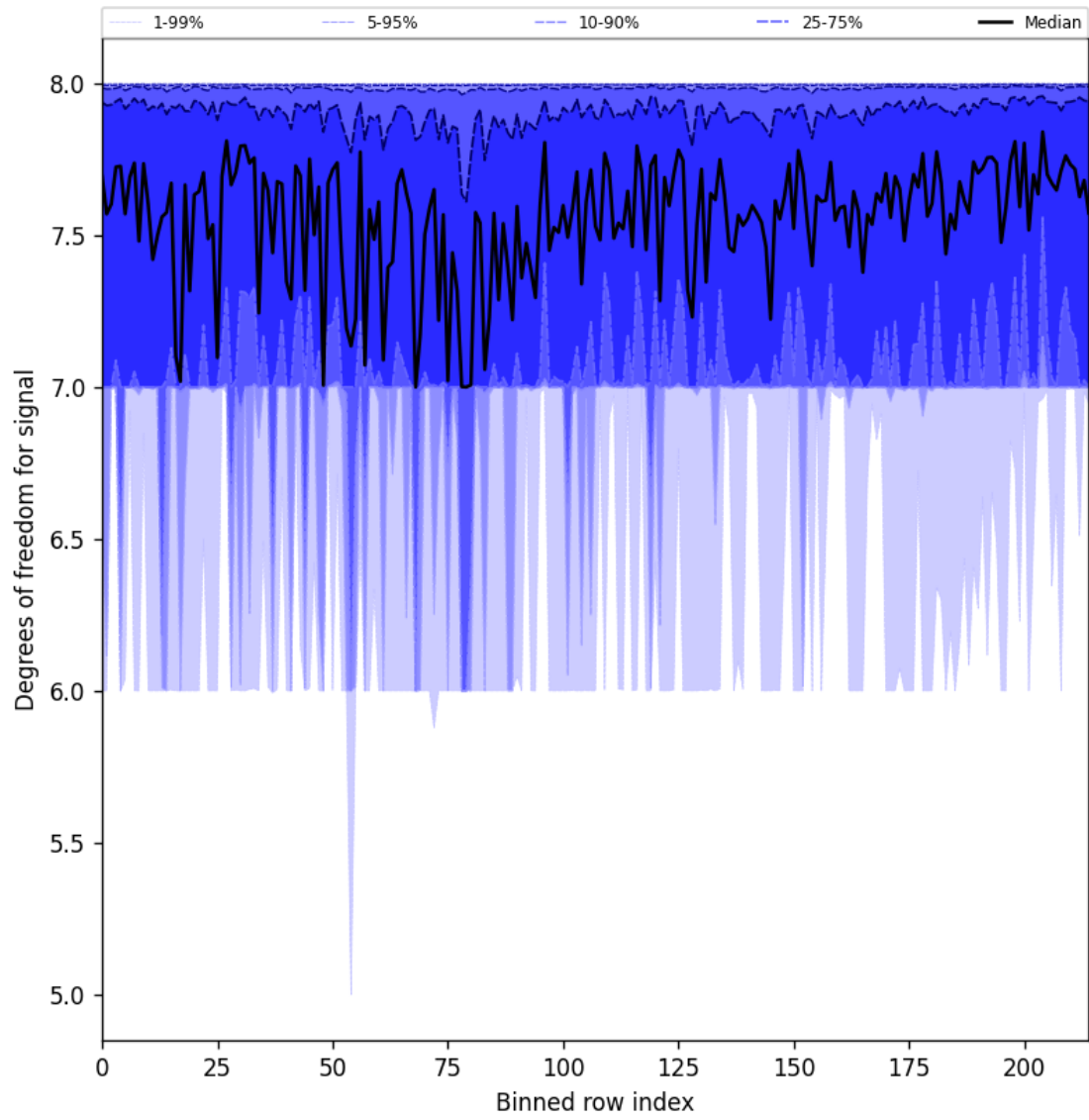
Figure 25: Along track statistics of “Degrees of freedom for signal” for 2025-10-03 to 2025-10-04
