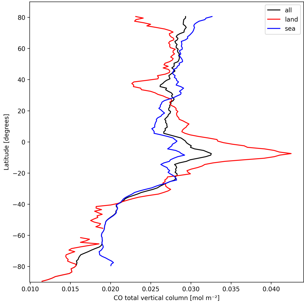
Figure 7: Zonal average of “CO total vertical column” for 2025-10-03 to 2025-10-04.
