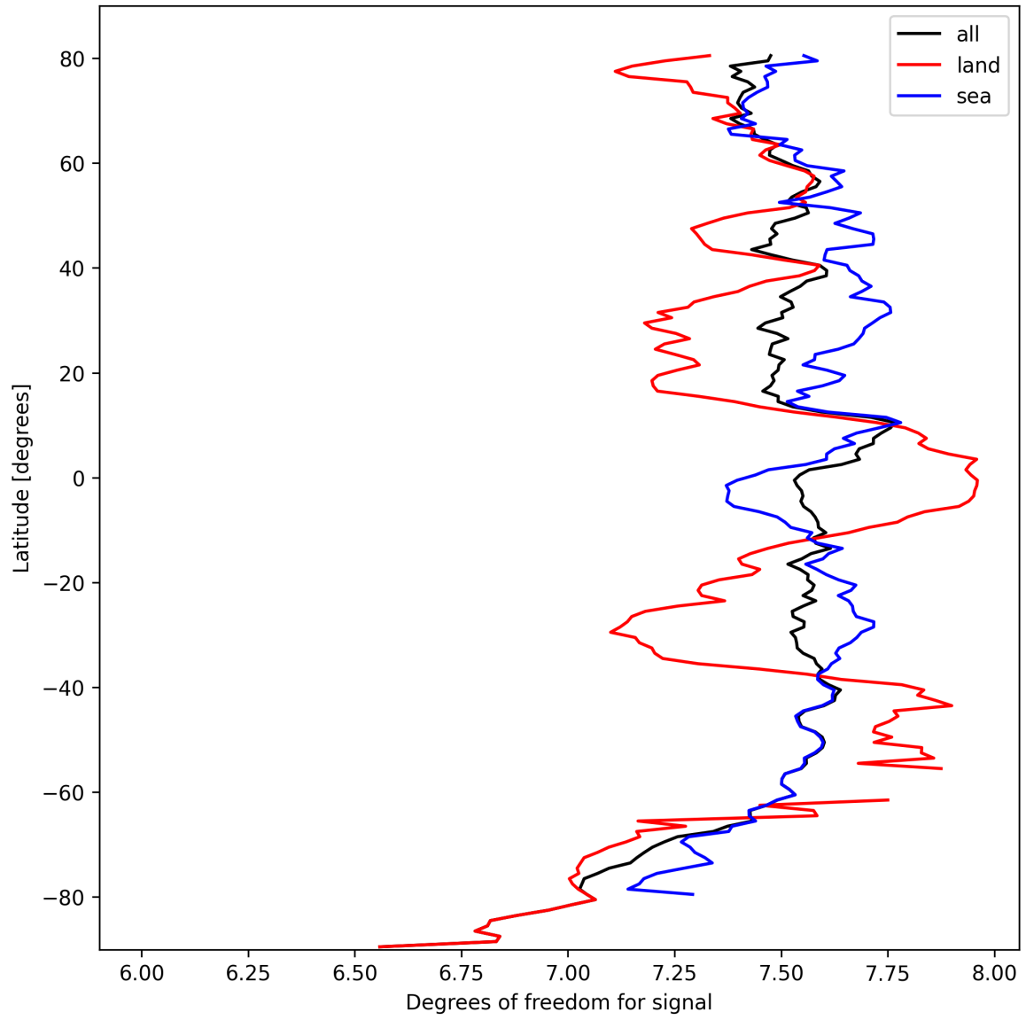
Figure 11: Zonal average of “Degrees of freedom for signal” for 2025-10-03 to 2025-10-04.
