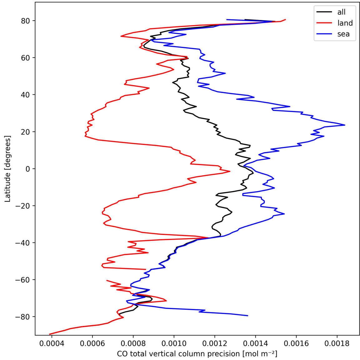
Figure 8: Zonal average of “CO total vertical column precision” for 2025-10-04 to 2025-10-04.
