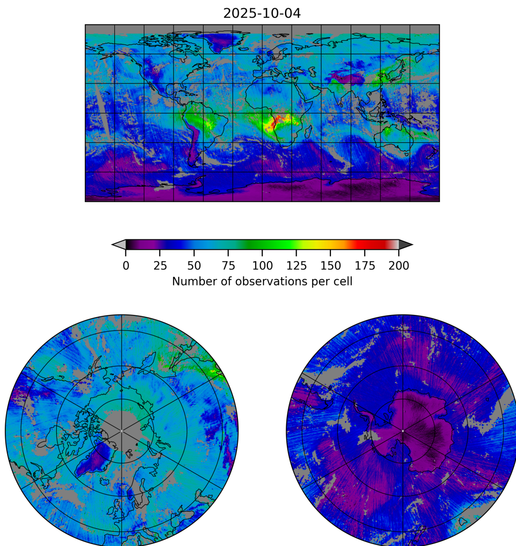
Figure 5: Map of the number of observations for 2025-10-04 to 2025-10-04
