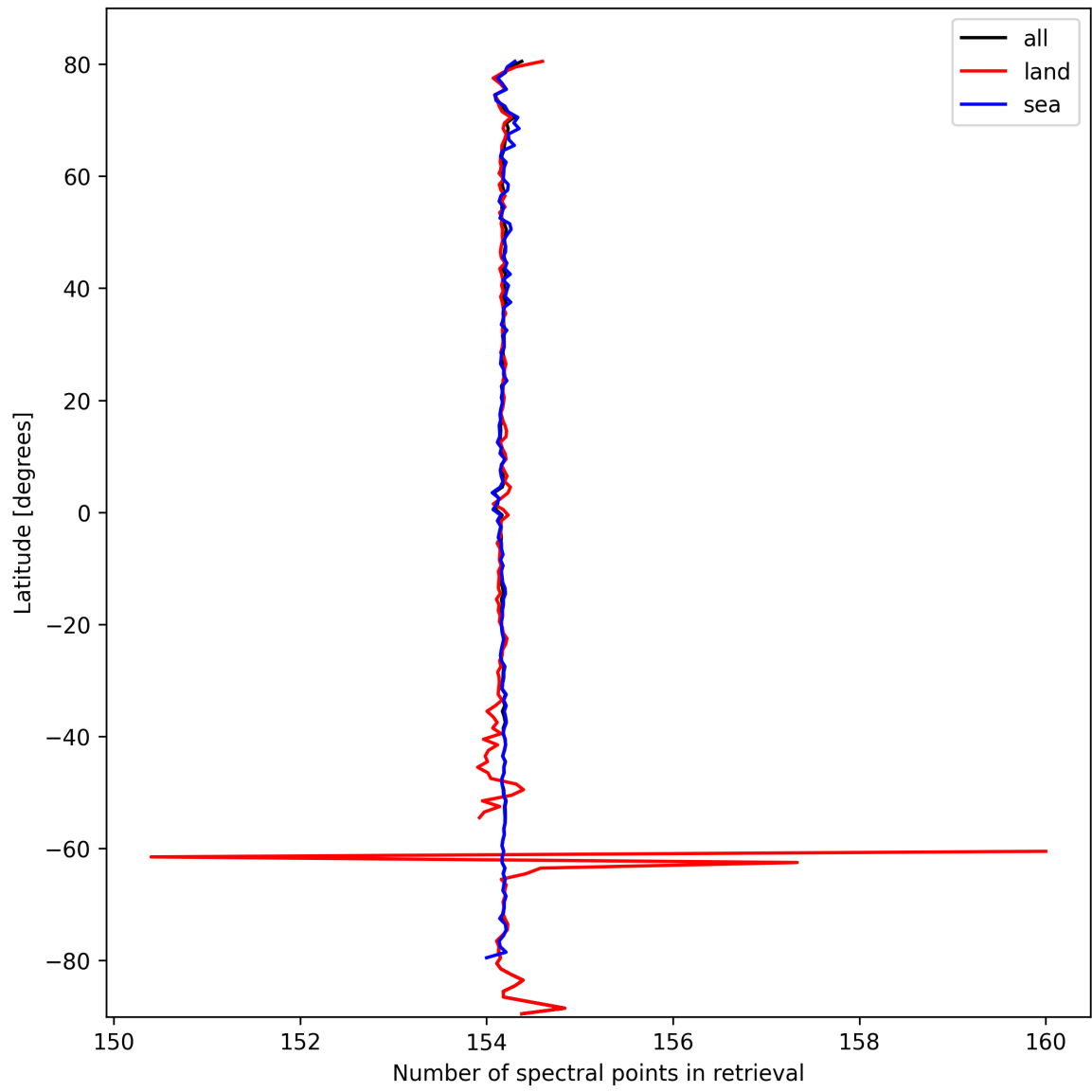
Figure 9: Zonal average of “Number of spectral points in retrieval” for 2025-10-04 to 2025-10-04.
