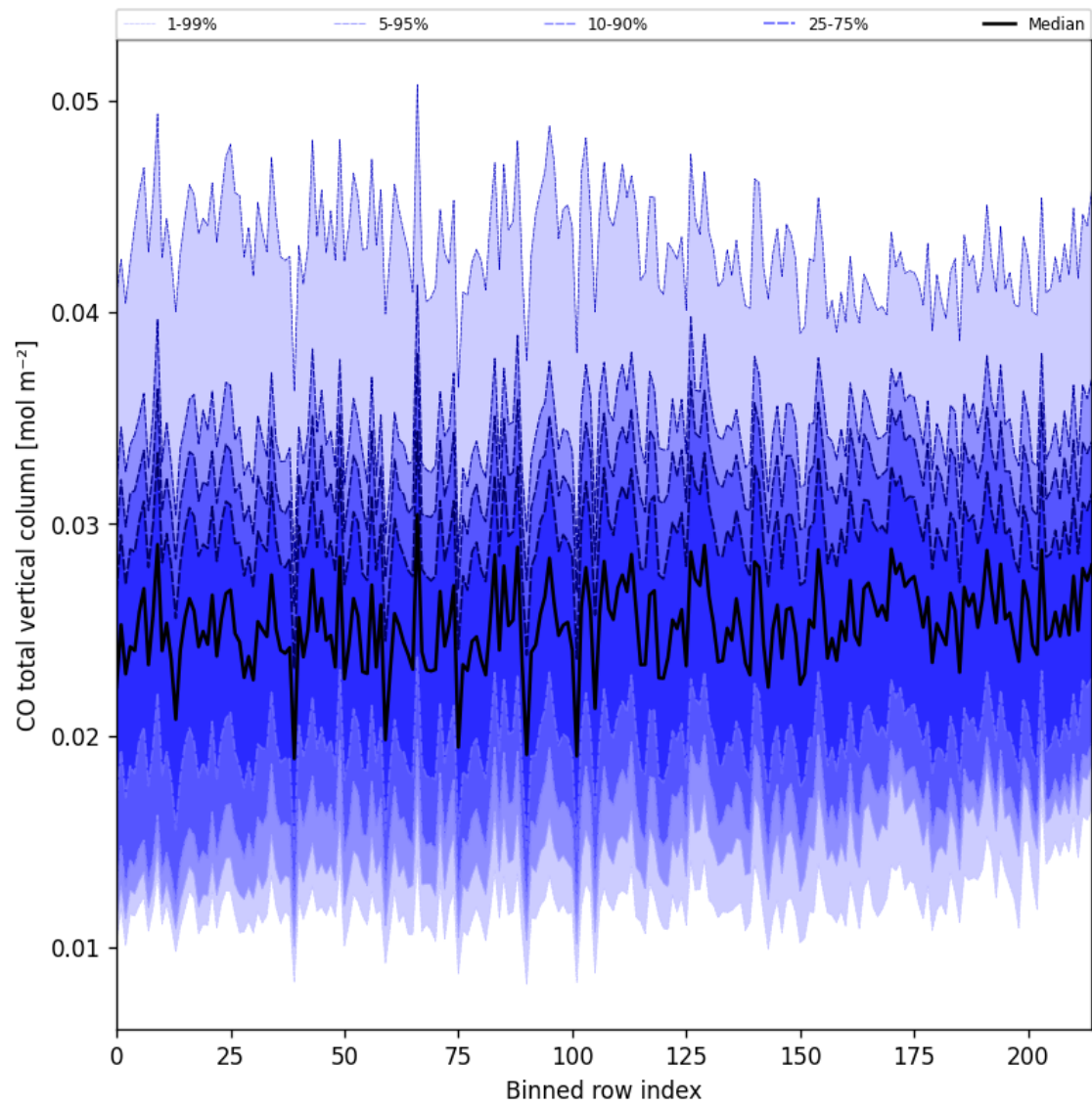
Figure 21: Along track statistics of “CO total vertical column” for 2025-10-04 to 2025-10-04
