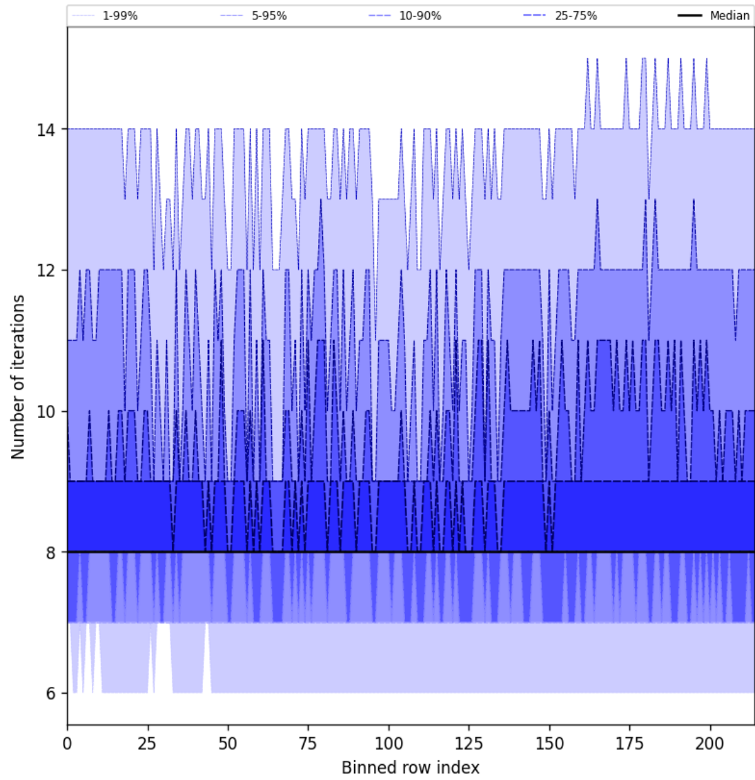
Figure 26: Along track statistics of “Number of iterations” for 2025-10-04 to 2025-10-04
