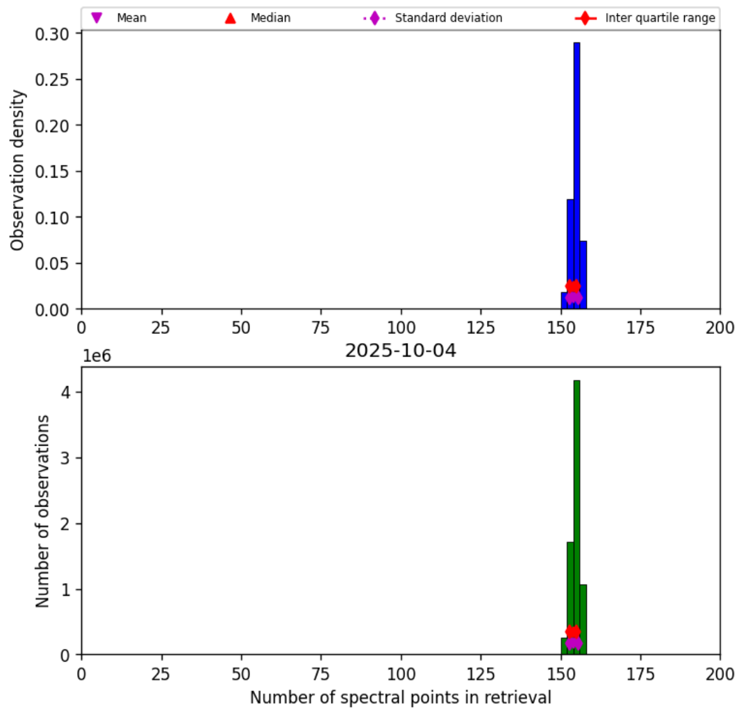
Figure 16: Histogram of “Number of spectral points in retrieval” for 2025-10-04 to 2025-10-04
