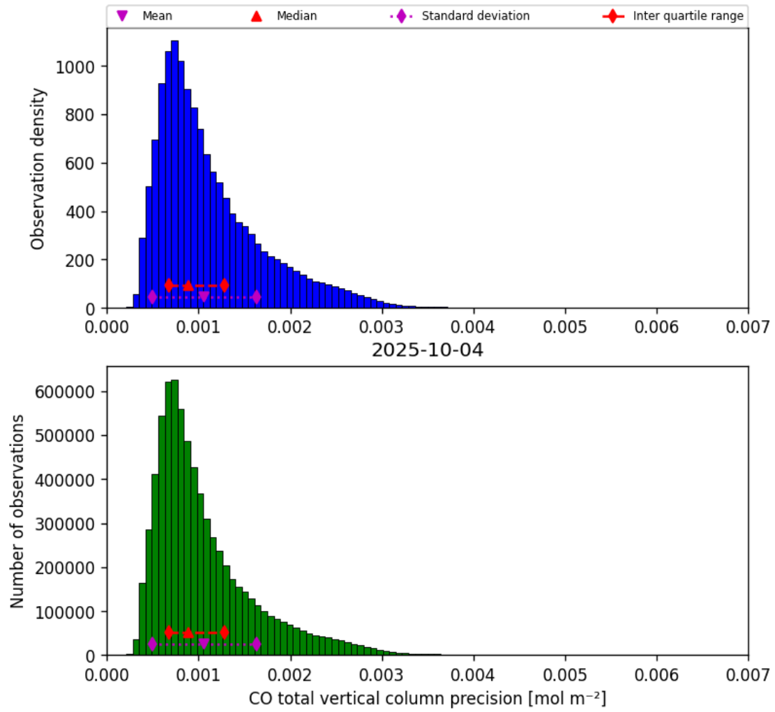
Figure 15: Histogram of “CO total vertical column precision” for 2025-10-04 to 2025-10-04
