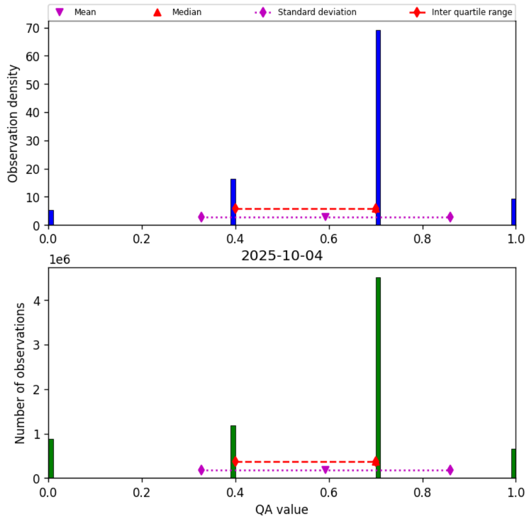
Figure 13: Histogram of “QA value” for 2025-10-04 to 2025-10-04
