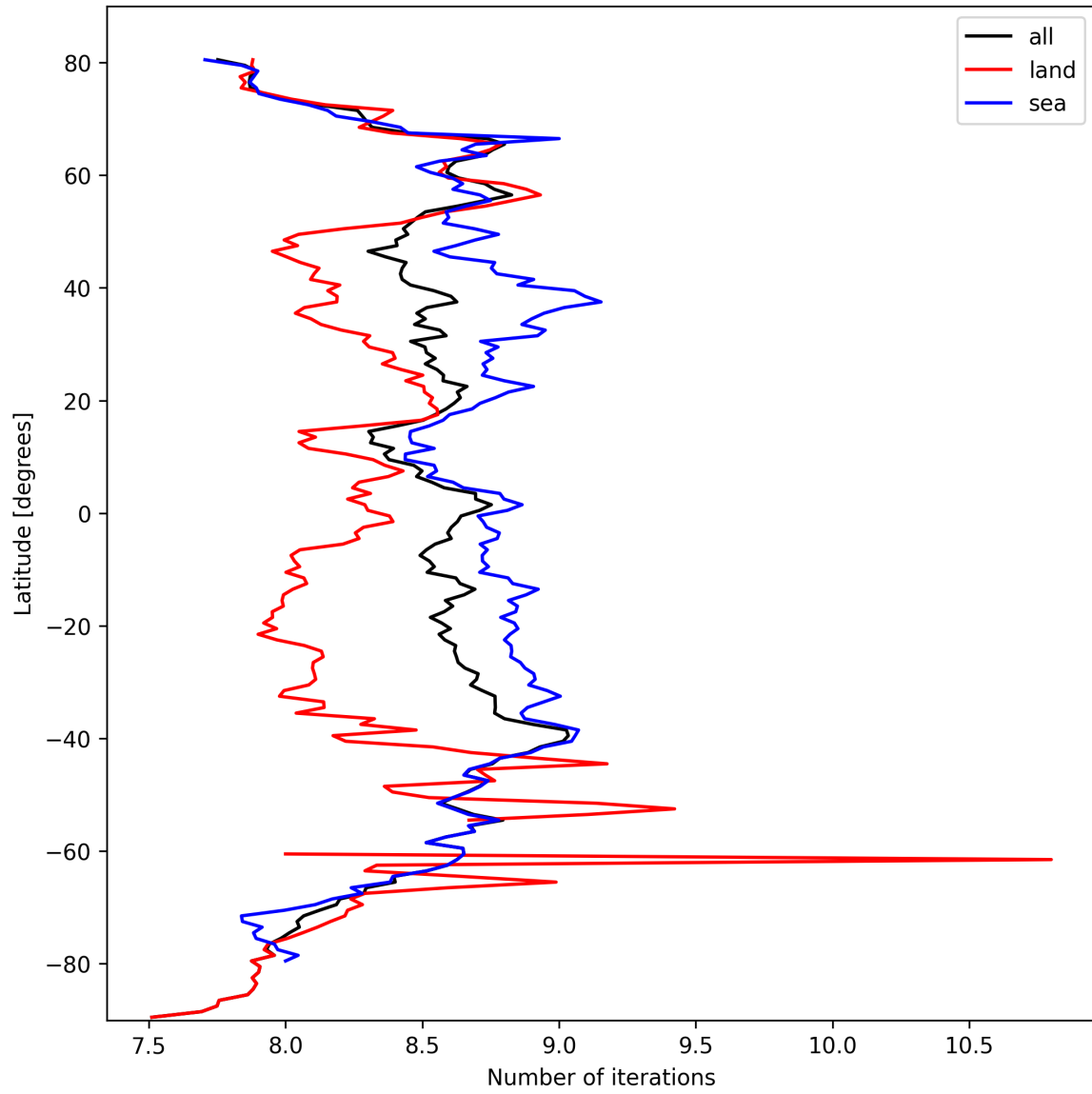
Figure 12: Zonal average of “Number of iterations” for 2025-10-04 to 2025-10-04.
