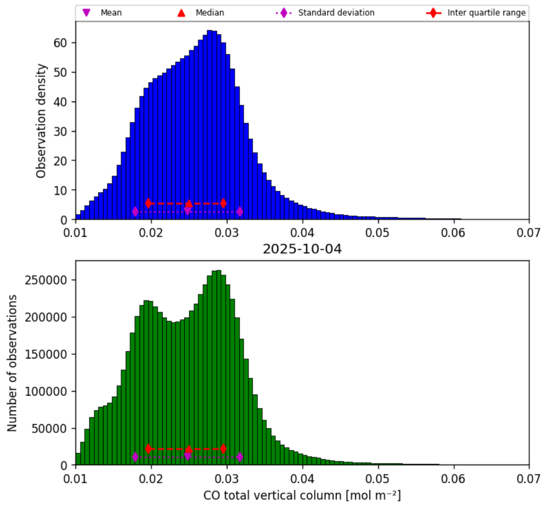
Figure 14: Histogram of “CO total vertical column” for 2025-10-04 to 2025-10-04
