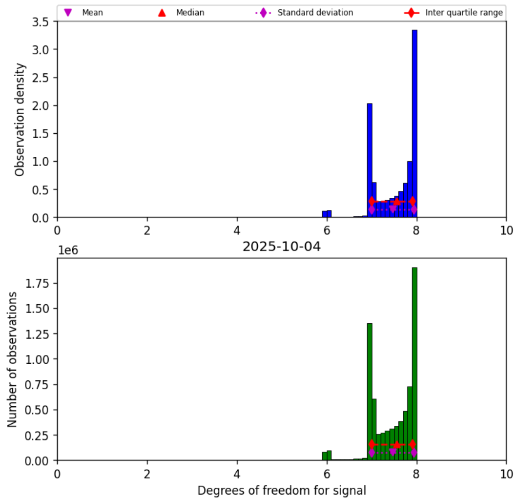
Figure 18: Histogram of “Degrees of freedom for signal” for 2025-10-04 to 2025-10-04
