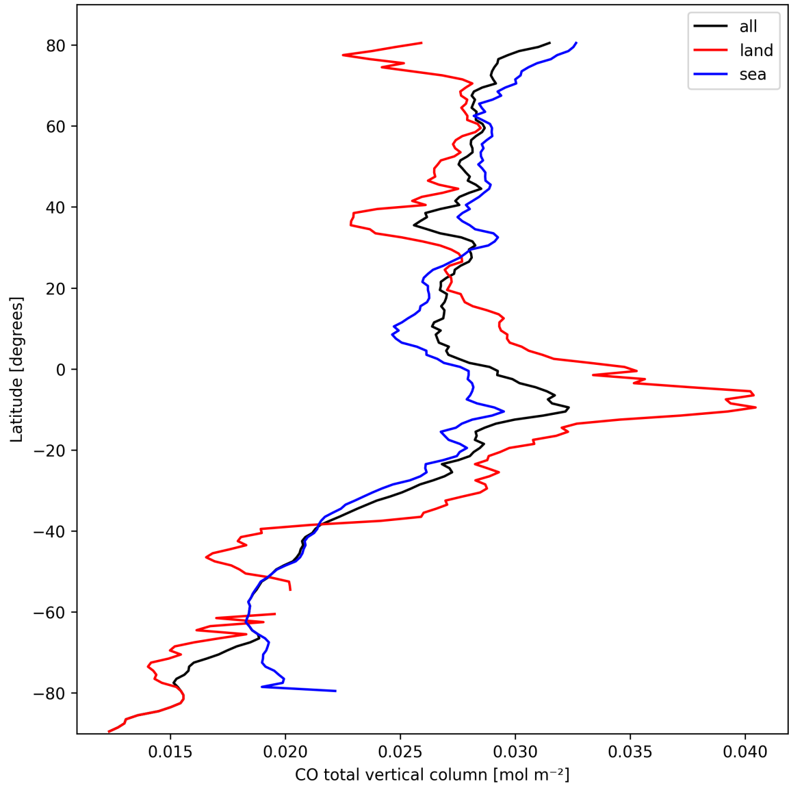
Figure 7: Zonal average of “CO total vertical column” for 2025-10-04 to 2025-10-04.
