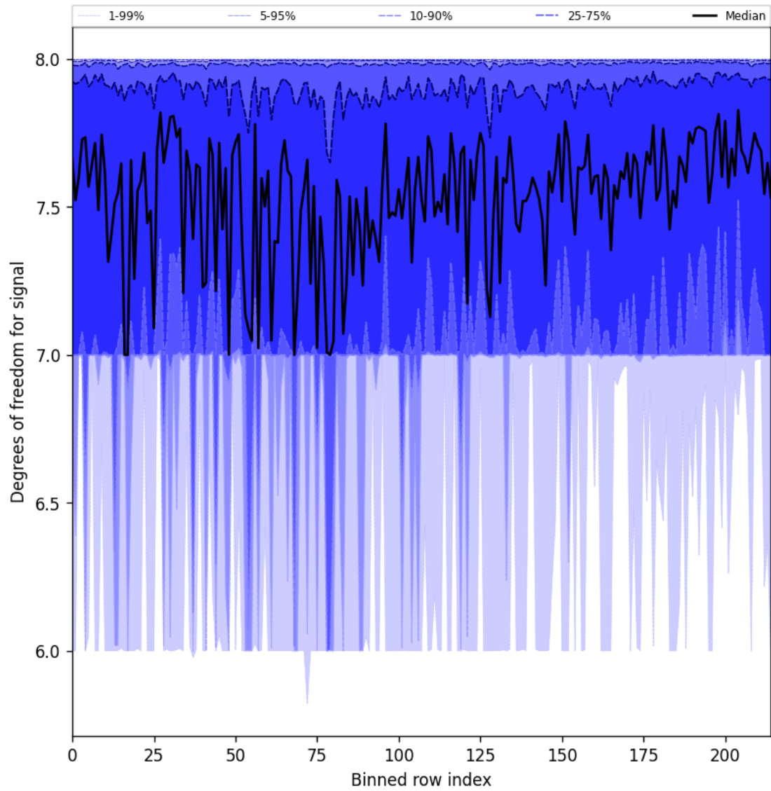
Figure 25: Along track statistics of “Degrees of freedom for signal” for 2025-10-04 to 2025-10-04
