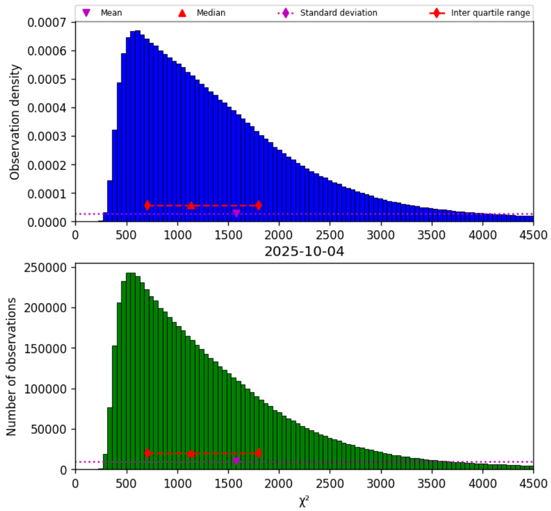
Figure 17: Histogram of " \chi^2 " for 2025-10-04 to 2025-10-04
