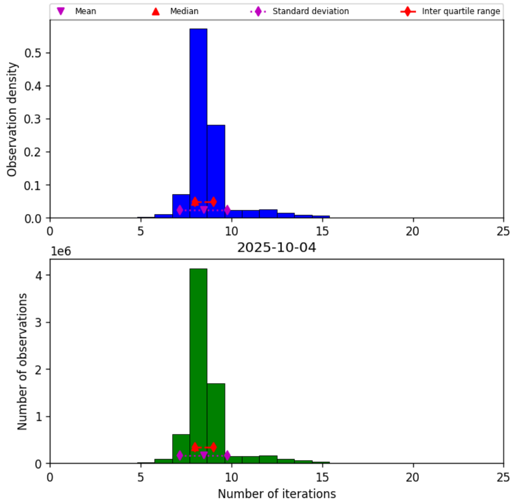
Figure 19: Histogram of “Number of iterations” for 2025-10-04 to 2025-10-04
