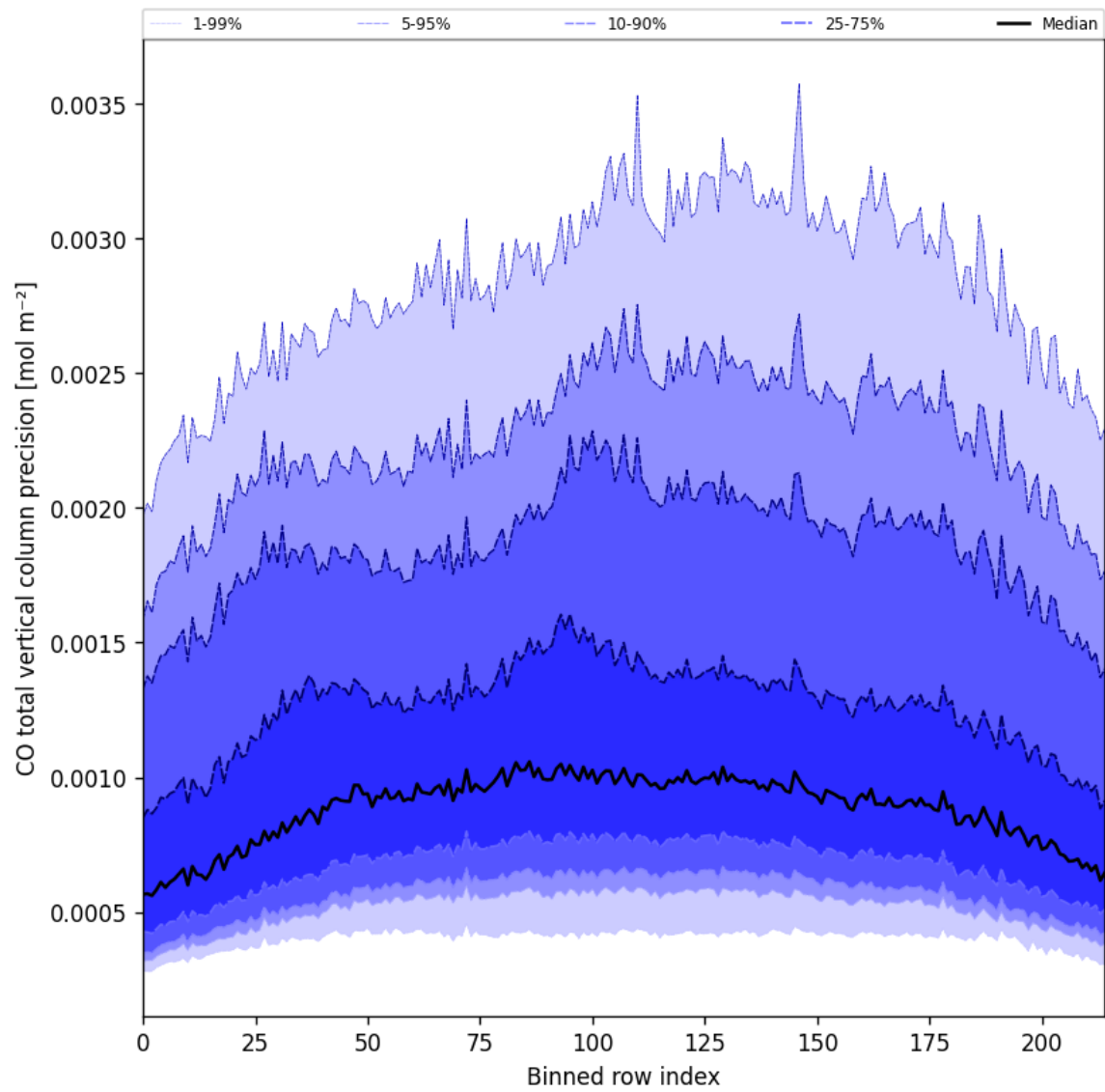
Figure 22: Along track statistics of “CO total vertical column precision” for 2025-10-04 to 2025-10-04
