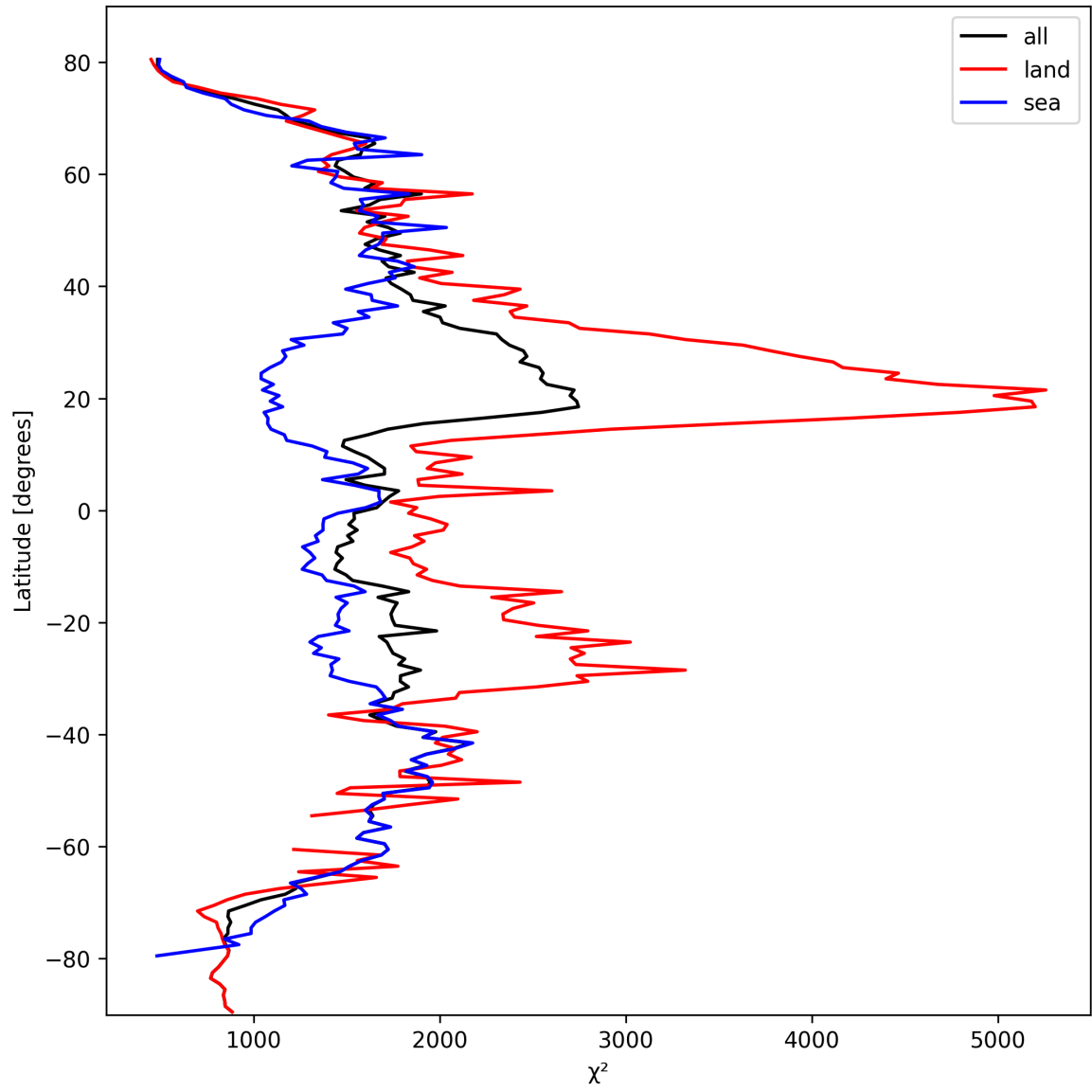
Figure 10: Zonal average of “ \chi^2 ” for 2025-10-04 to 2025-10-04.
