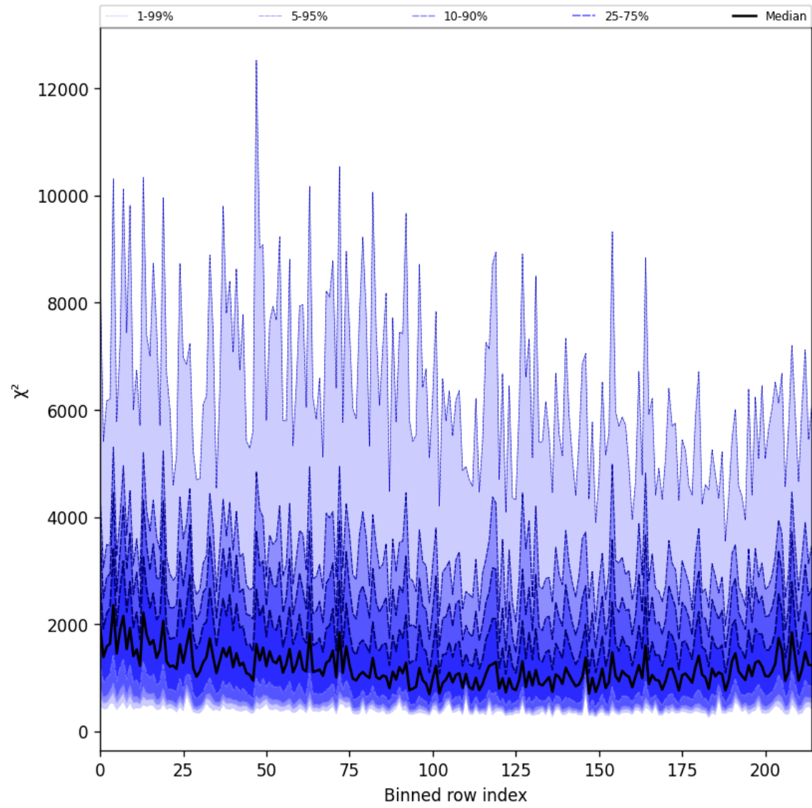
Figure 24: Along track statistics of “ \chi^2 ” for 2025-10-04 to 2025-10-04
