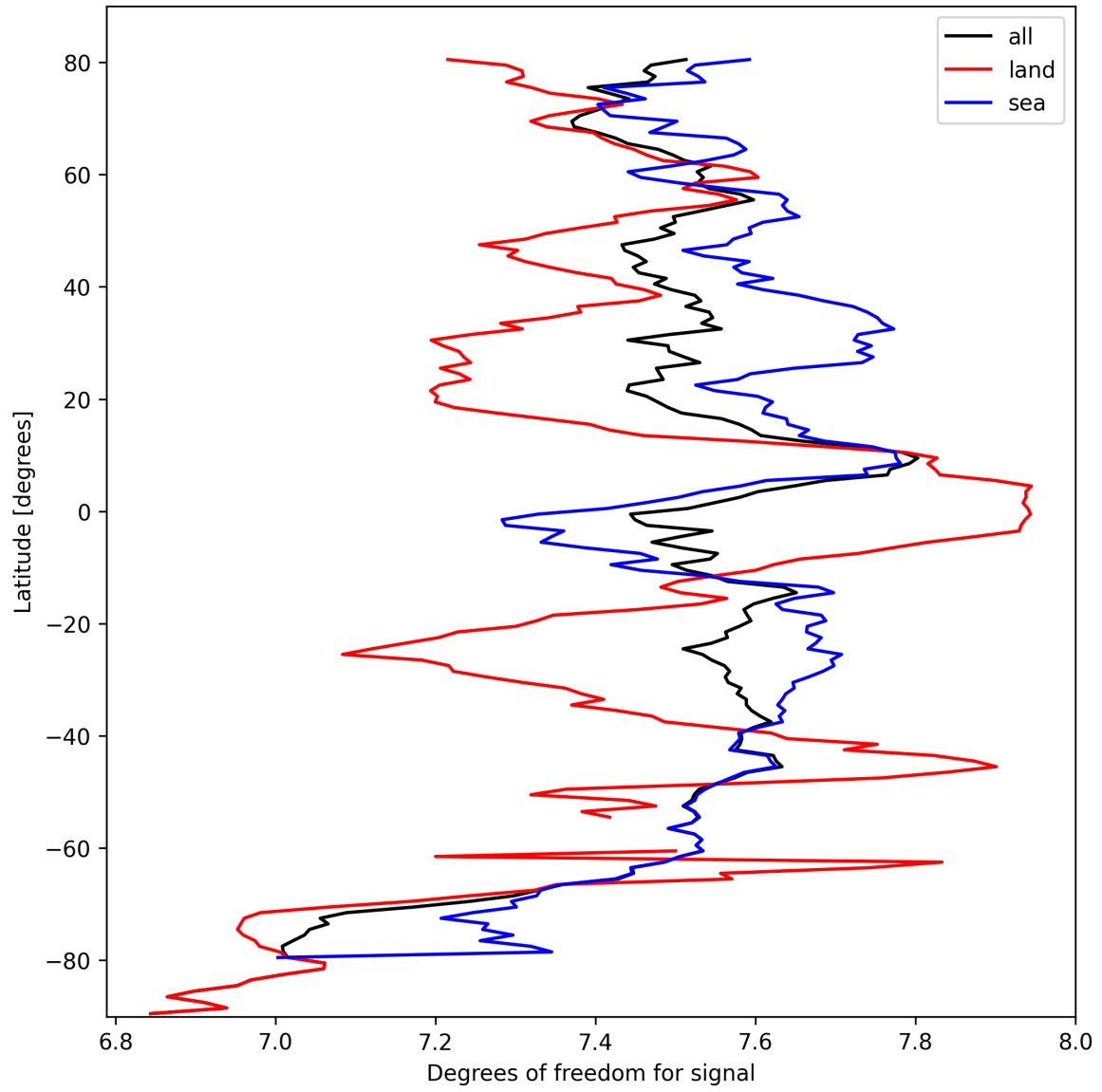
Figure 11: Zonal average of “Degrees of freedom for signal” for 2025-10-04 to 2025-10-04.
