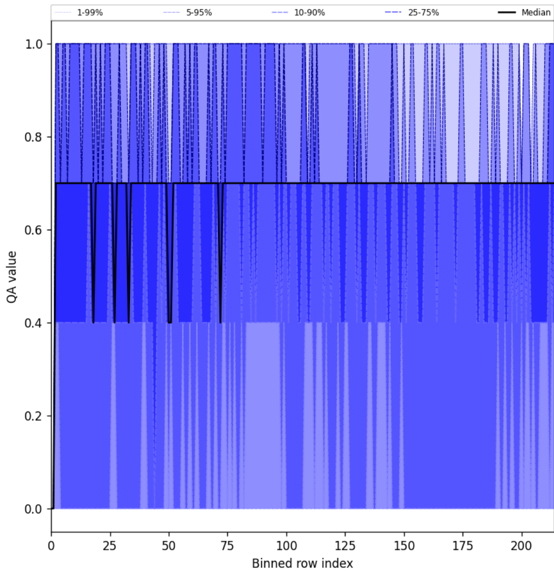
Figure 20: Along track statistics of “QA value” for 2025-10-04 to 2025-10-04
