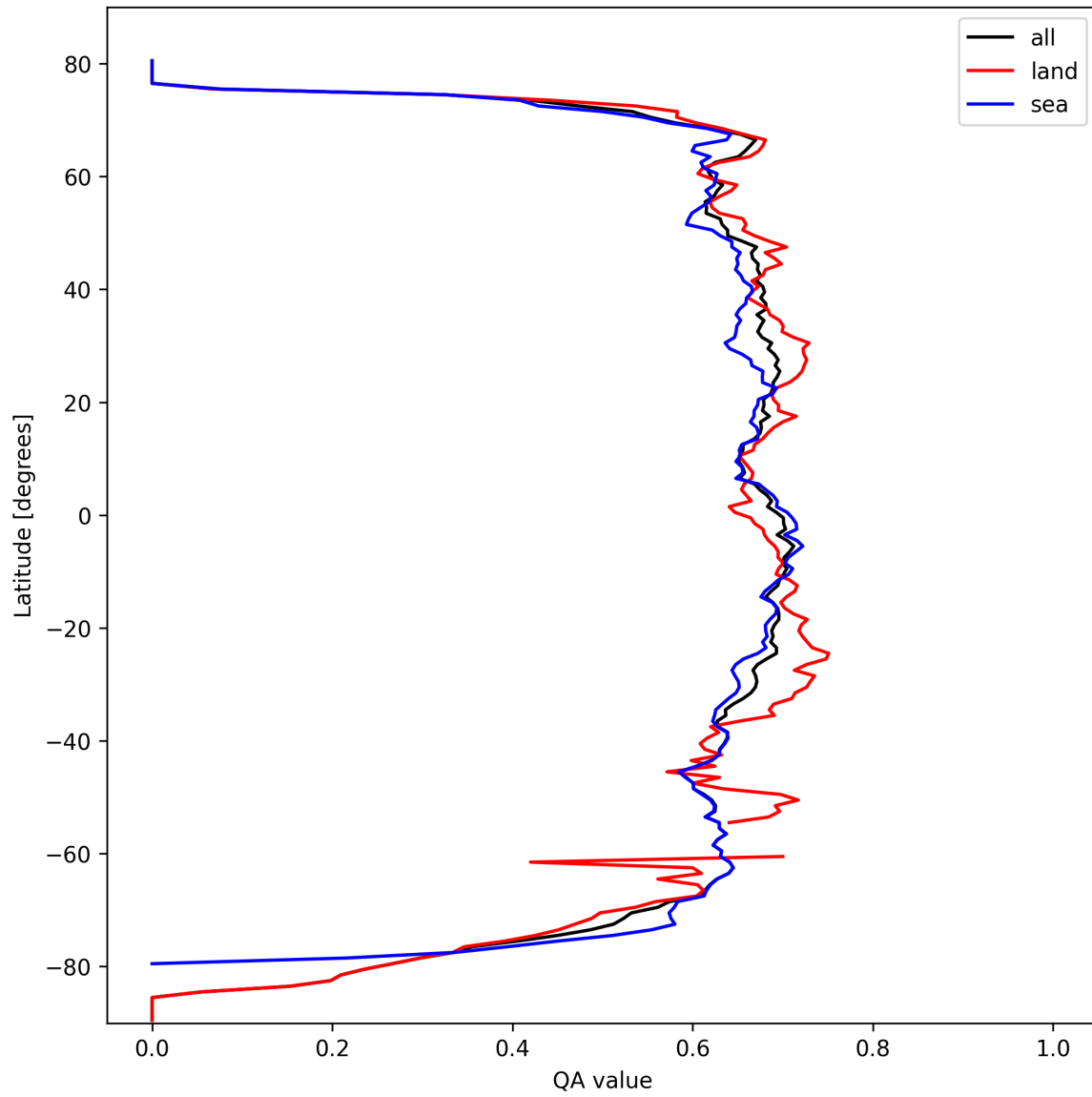
Figure 6: Zonal average of “QA value” for 2025-10-04 to 2025-10-04.
