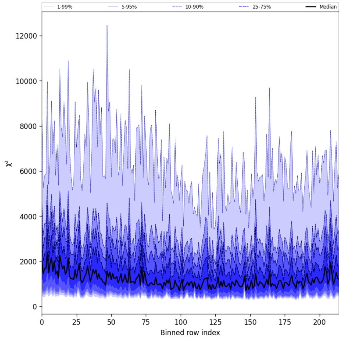
Figure 24: Along track statistics of “ \chi^2 ” for 2025-10-05 to 2025-10-06
