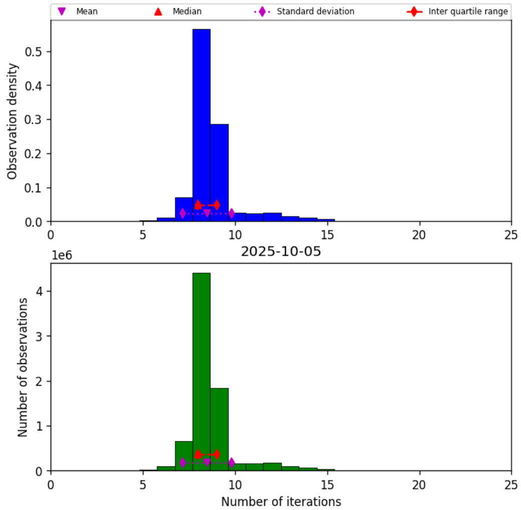
Figure 19: Histogram of “Number of iterations” for 2025-10-05 to 2025-10-06
