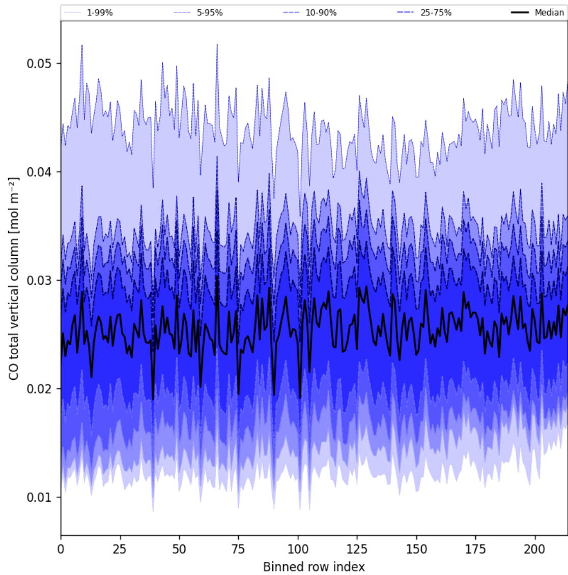
Figure 21: Along track statistics of “CO total vertical column” for 2025-10-05 to 2025-10-06
