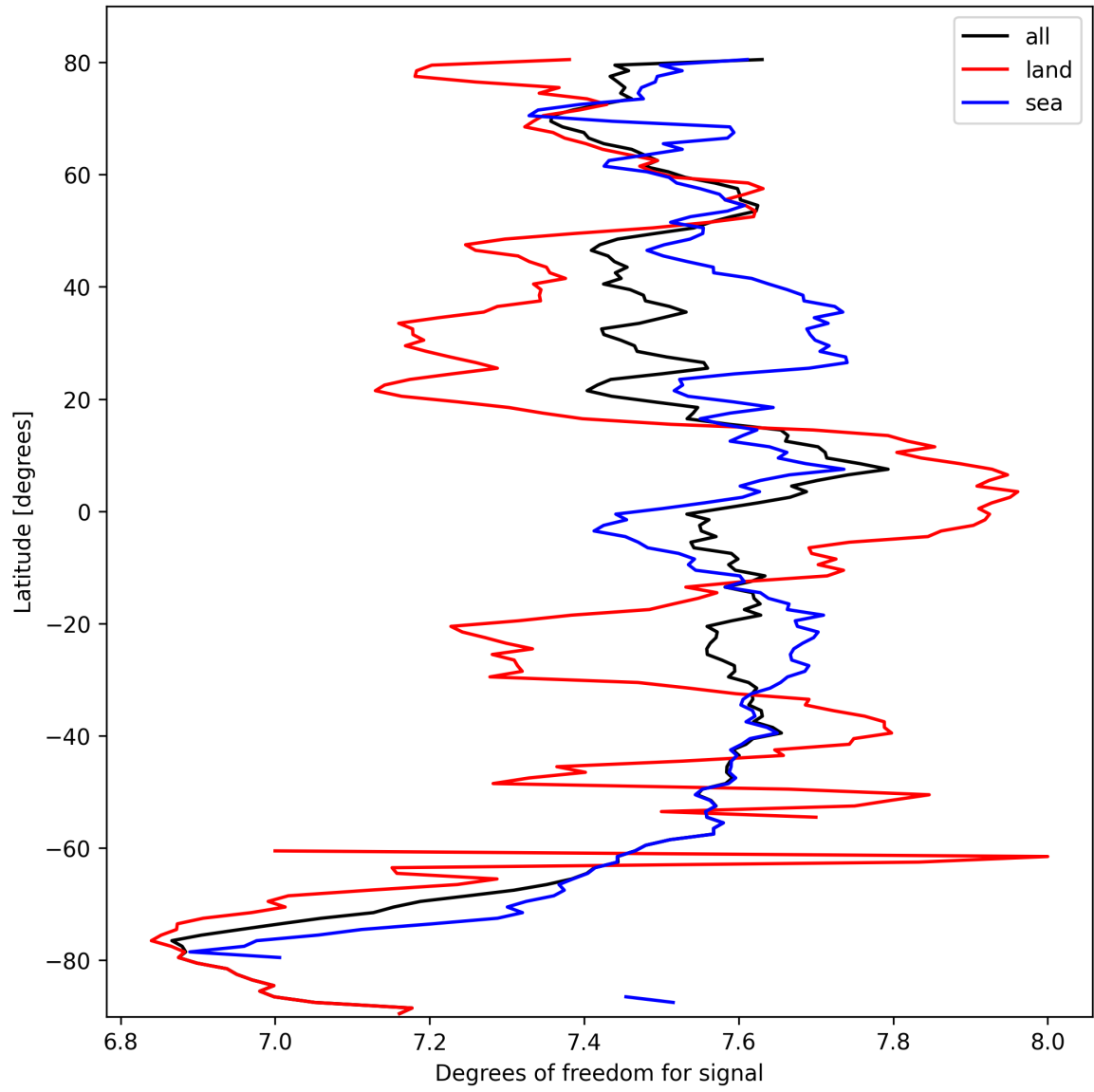
Figure 11: Zonal average of “Degrees of freedom for signal” for 2025-10-05 to 2025-10-06.
