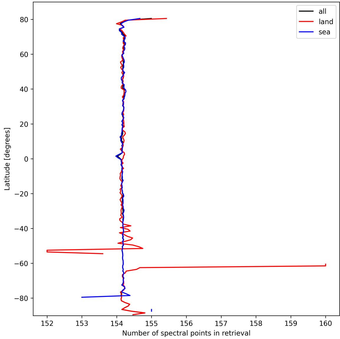
Figure 9: Zonal average of “Number of spectral points in retrieval” for 2025-10-05 to 2025-10-06.
