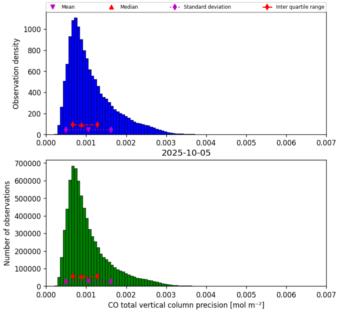
Figure 15: Histogram of “CO total vertical column precision” for 2025-10-05 to 2025-10-06
