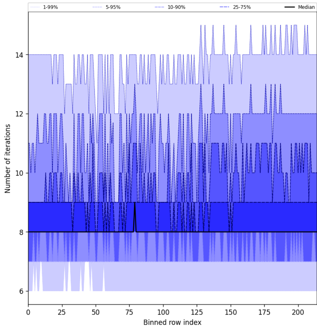
Figure 26: Along track statistics of “Number of iterations” for 2025-10-05 to 2025-10-06
