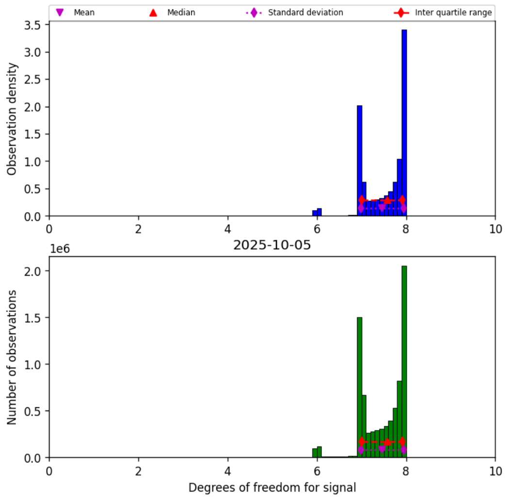
Figure 18: Histogram of “Degrees of freedom for signal” for 2025-10-05 to 2025-10-06
