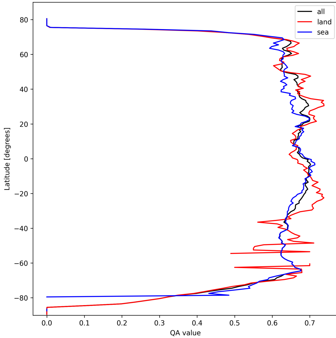
Figure 6: Zonal average of “QA value” for 2025-10-05 to 2025-10-06.
