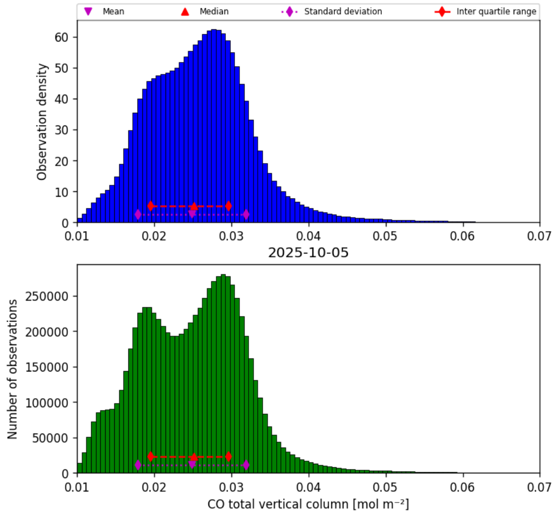
Figure 14: Histogram of “CO total vertical column” for 2025-10-05 to 2025-10-06
