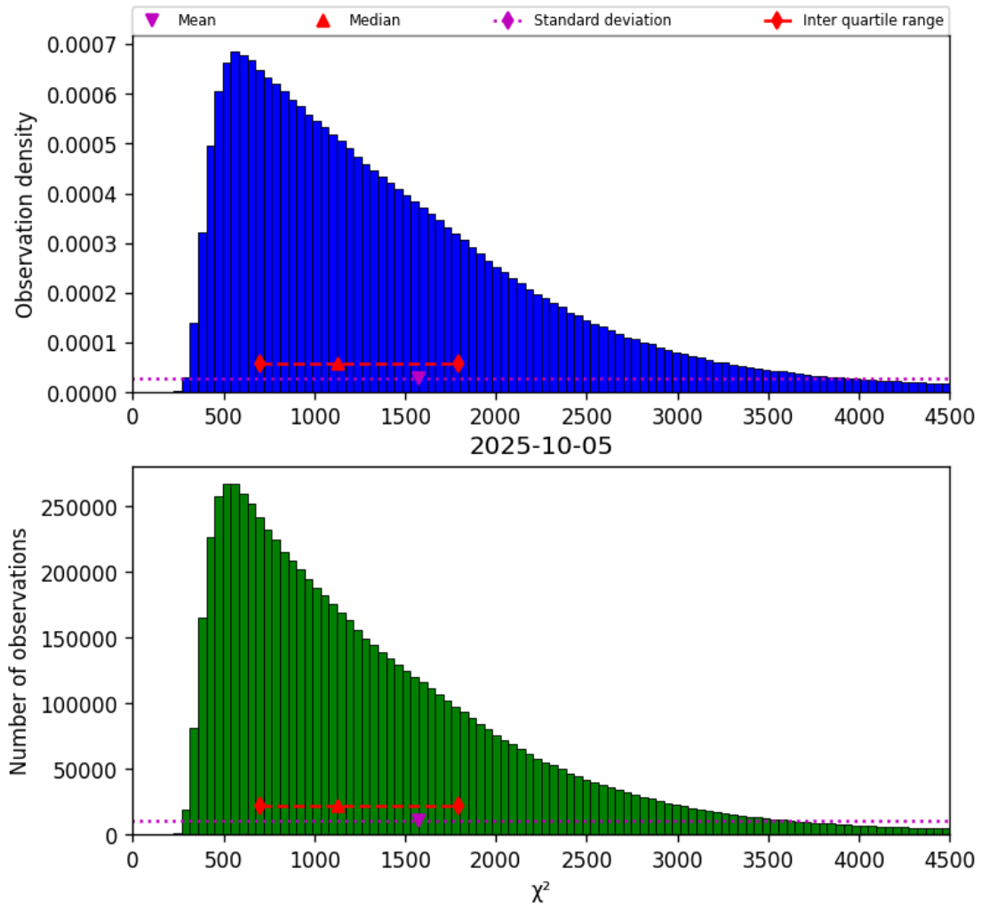
Figure 17: Histogram of " \chi^2 " for 2025-10-05 to 2025-10-06
