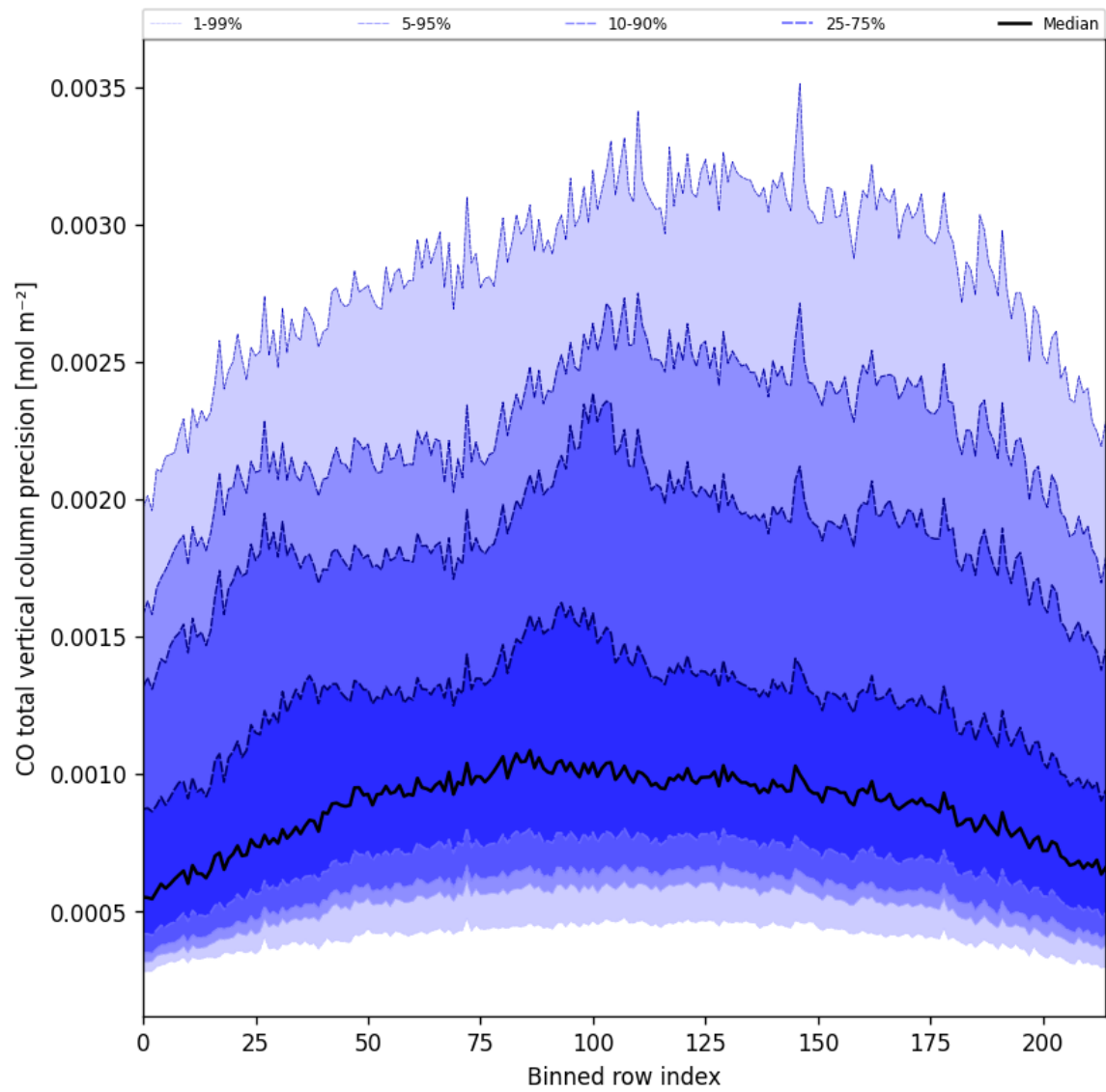
Figure 22: Along track statistics of “CO total vertical column precision” for 2025-10-05 to 2025-10-06
