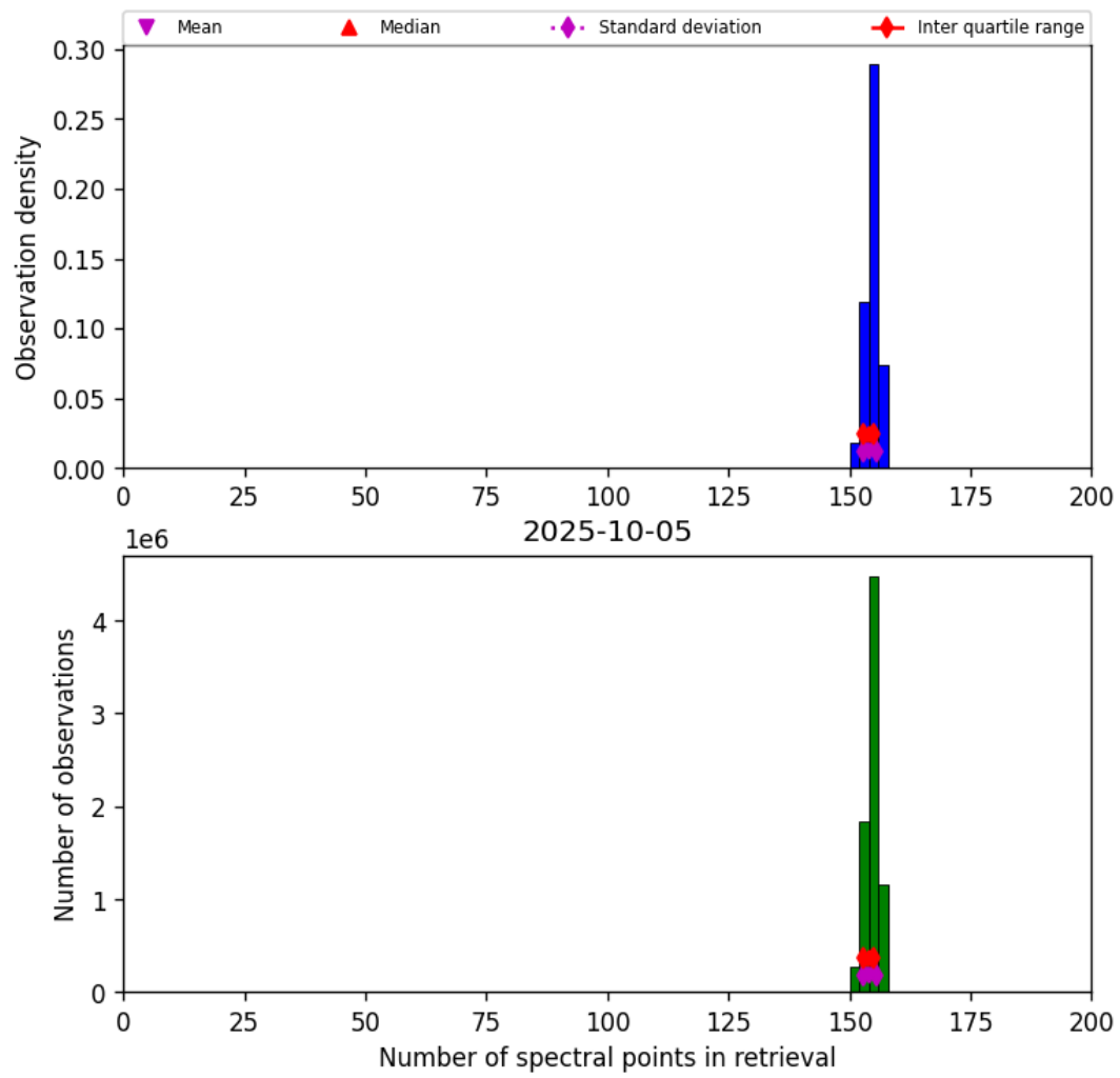
Figure 16: Histogram of “Number of spectral points in retrieval” for 2025-10-05 to 2025-10-06
