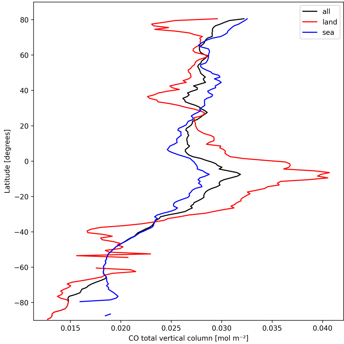
Figure 7: Zonal average of “CO total vertical column” for 2025-10-05 to 2025-10-06.
