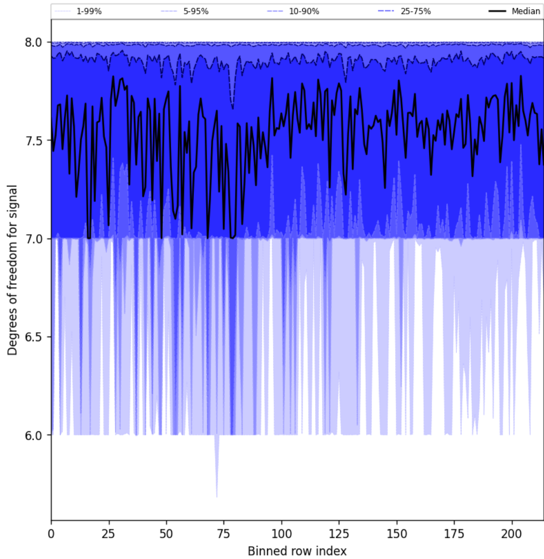
Figure 25: Along track statistics of “Degrees of freedom for signal” for 2025-10-05 to 2025-10-06
