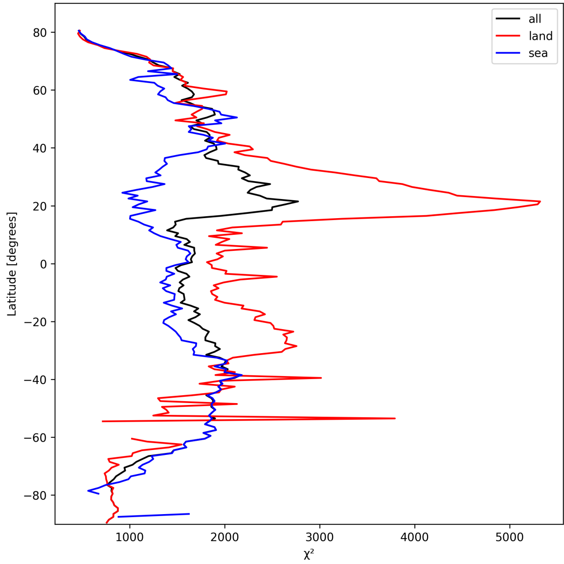
Figure 10: Zonal average of “ \chi^2 ” for 2025-10-05 to 2025-10-06.
