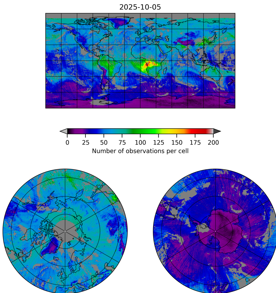
Figure 5: Map of the number of observations for 2025-10-05 to 2025-10-06
