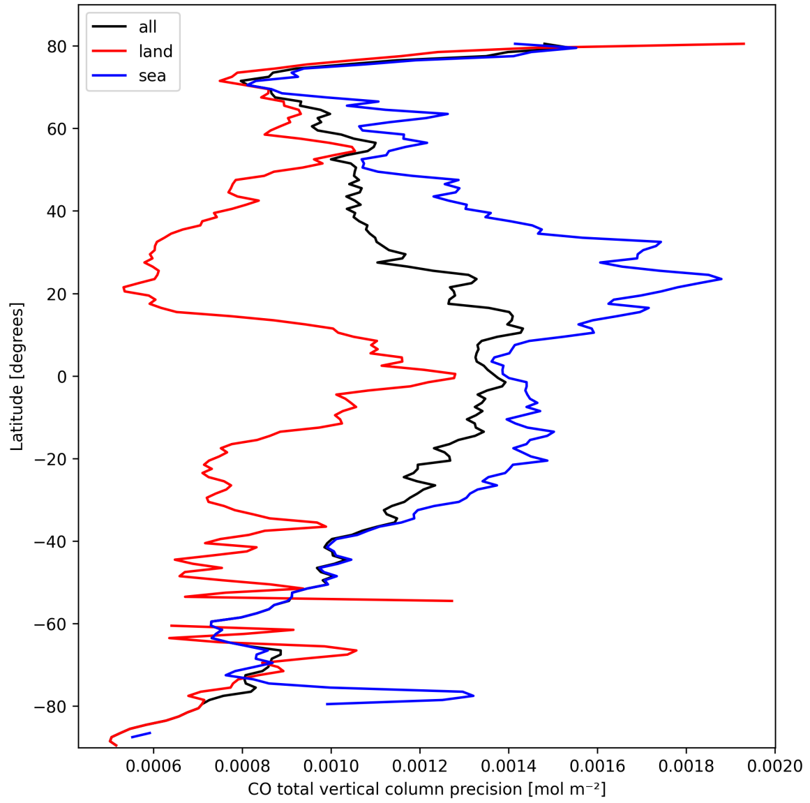
Figure 8: Zonal average of “CO total vertical column precision” for 2025-10-05 to 2025-10-06.
