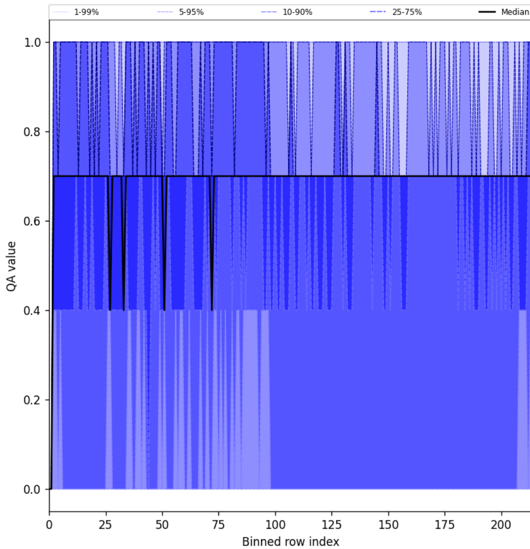
Figure 20: Along track statistics of “QA value” for 2025-10-05 to 2025-10-06
