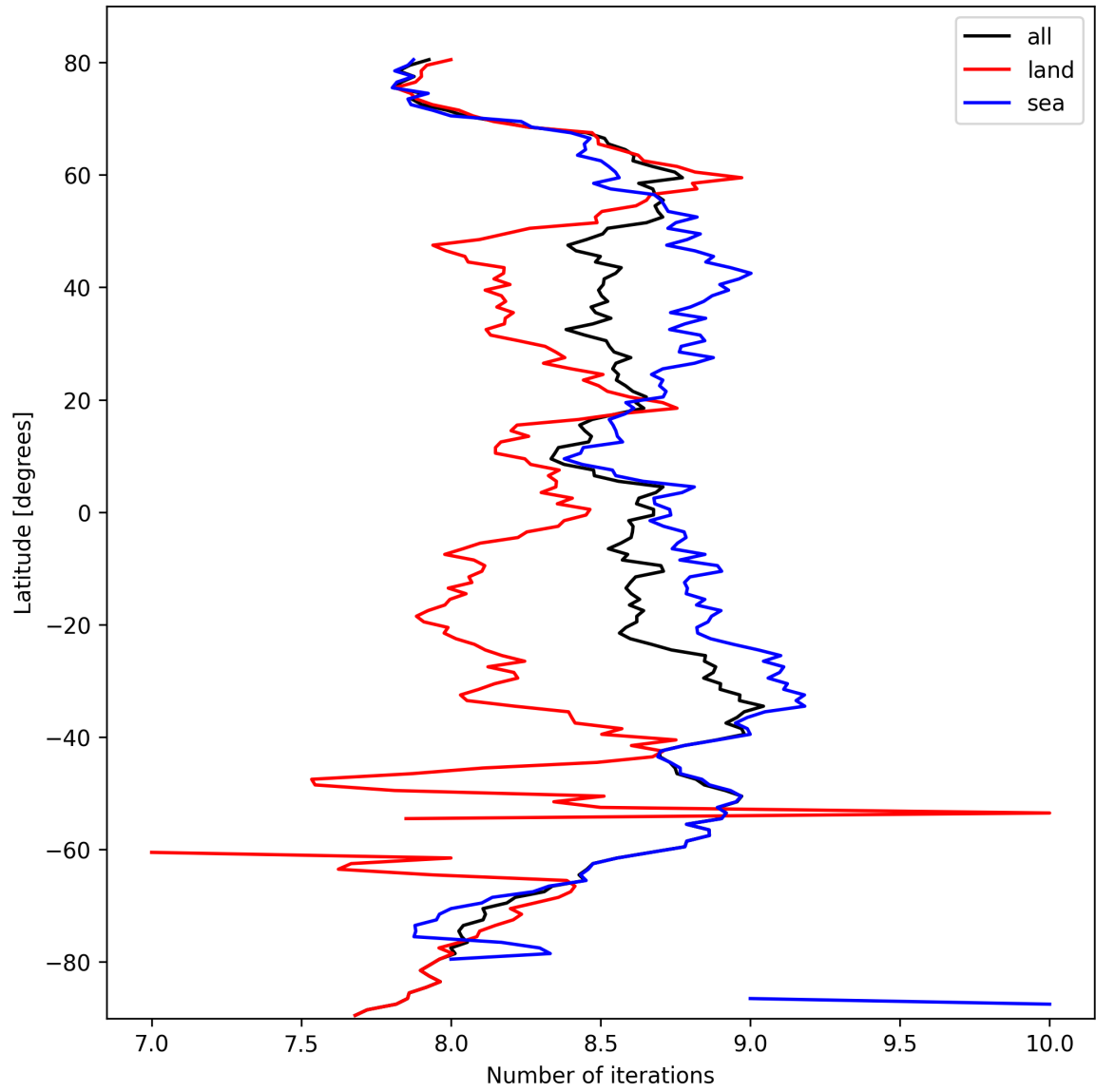
Figure 12: Zonal average of “Number of iterations” for 2025-10-05 to 2025-10-06.
