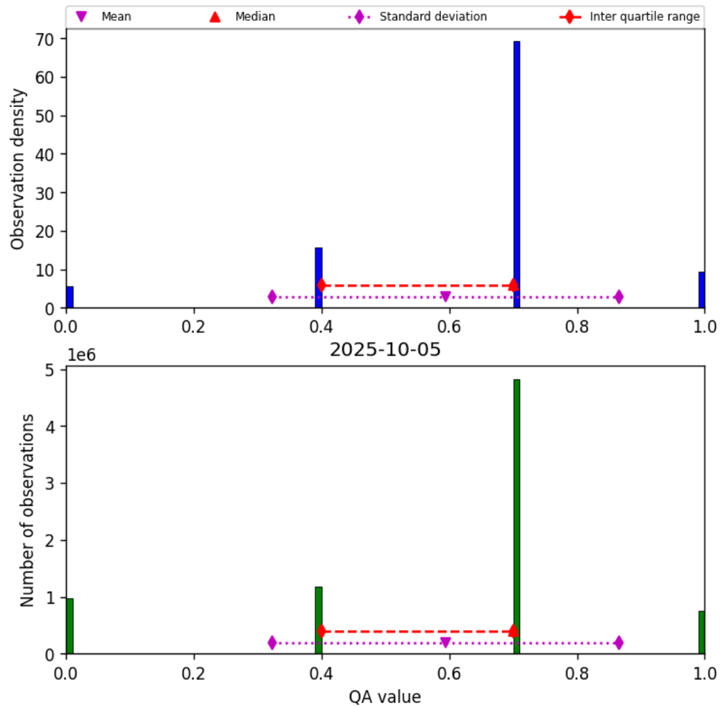
Figure 13: Histogram of “QA value” for 2025-10-05 to 2025-10-06
