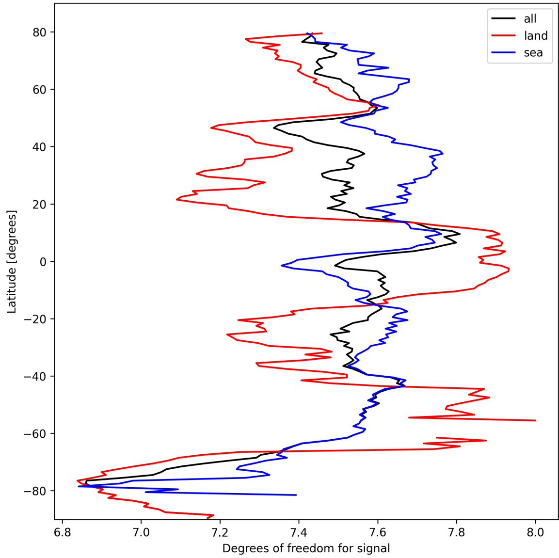
Figure 11: Zonal average of “Degrees of freedom for signal” for 2025-10-06 to 2025-10-07.
