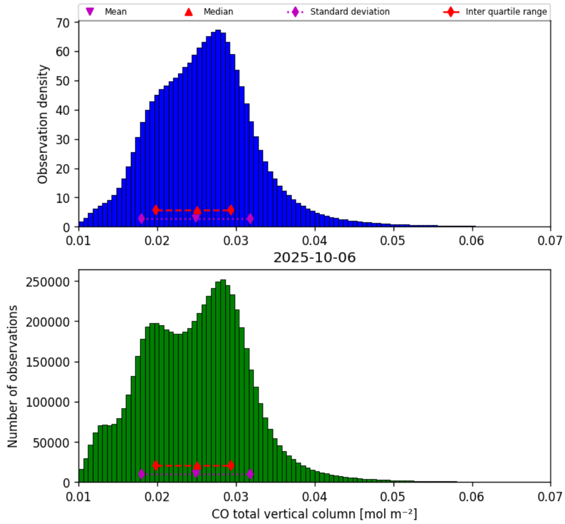
Figure 14: Histogram of “CO total vertical column” for 2025-10-06 to 2025-10-07
