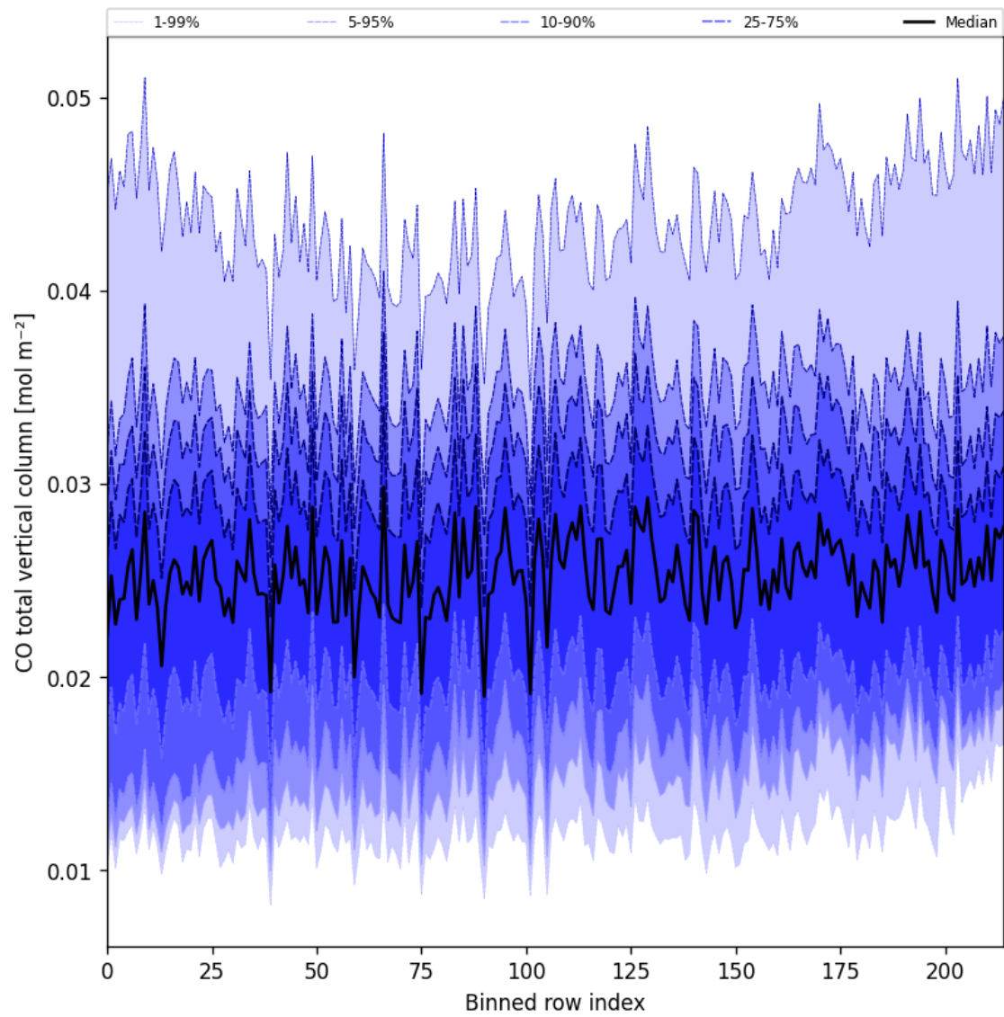
Figure 21: Along track statistics of “CO total vertical column” for 2025-10-06 to 2025-10-07
