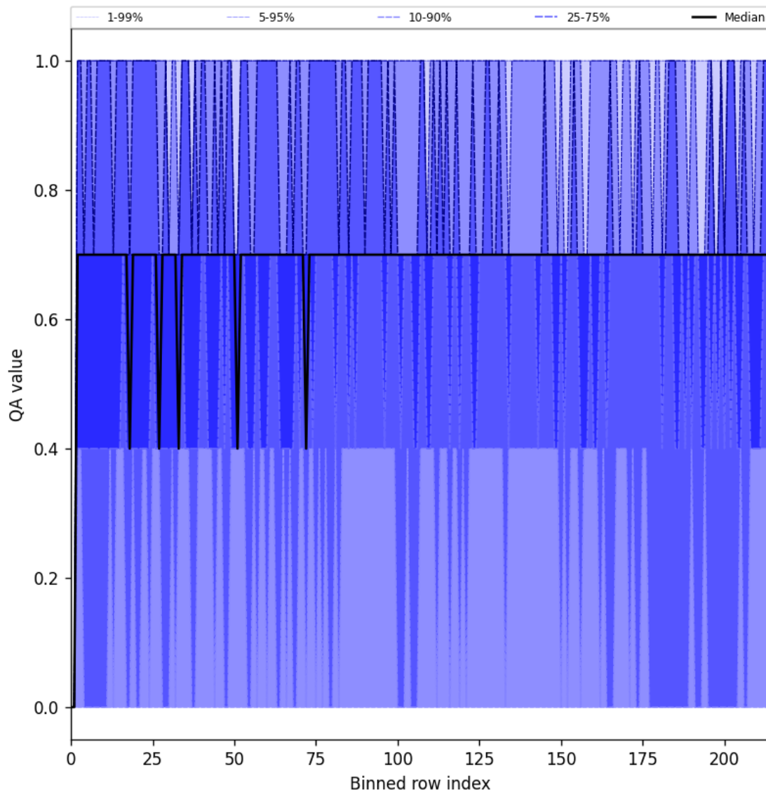
Figure 20: Along track statistics of “QA value” for 2025-10-06 to 2025-10-07
