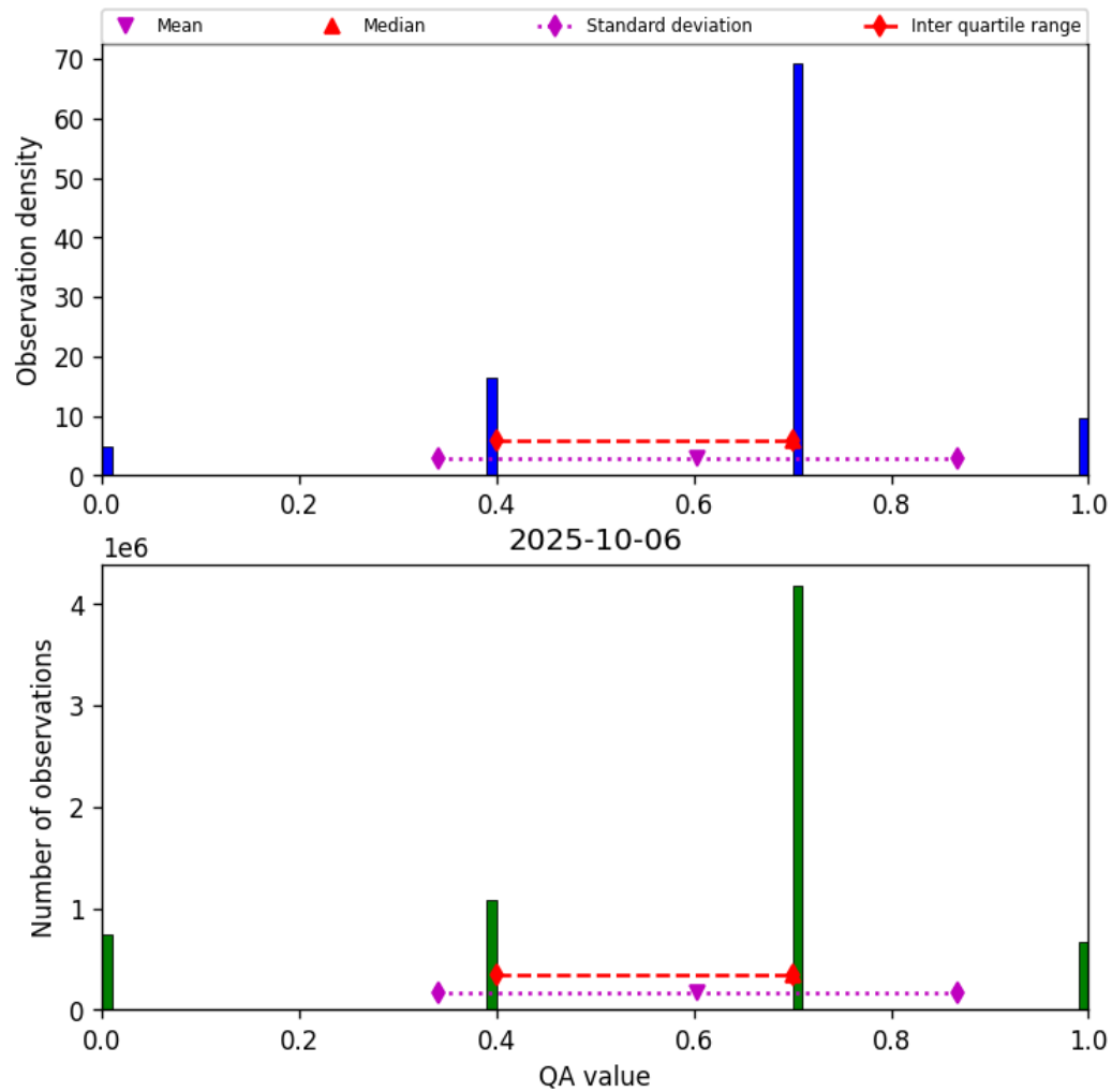
Figure 13: Histogram of “QA value” for 2025-10-06 to 2025-10-07
