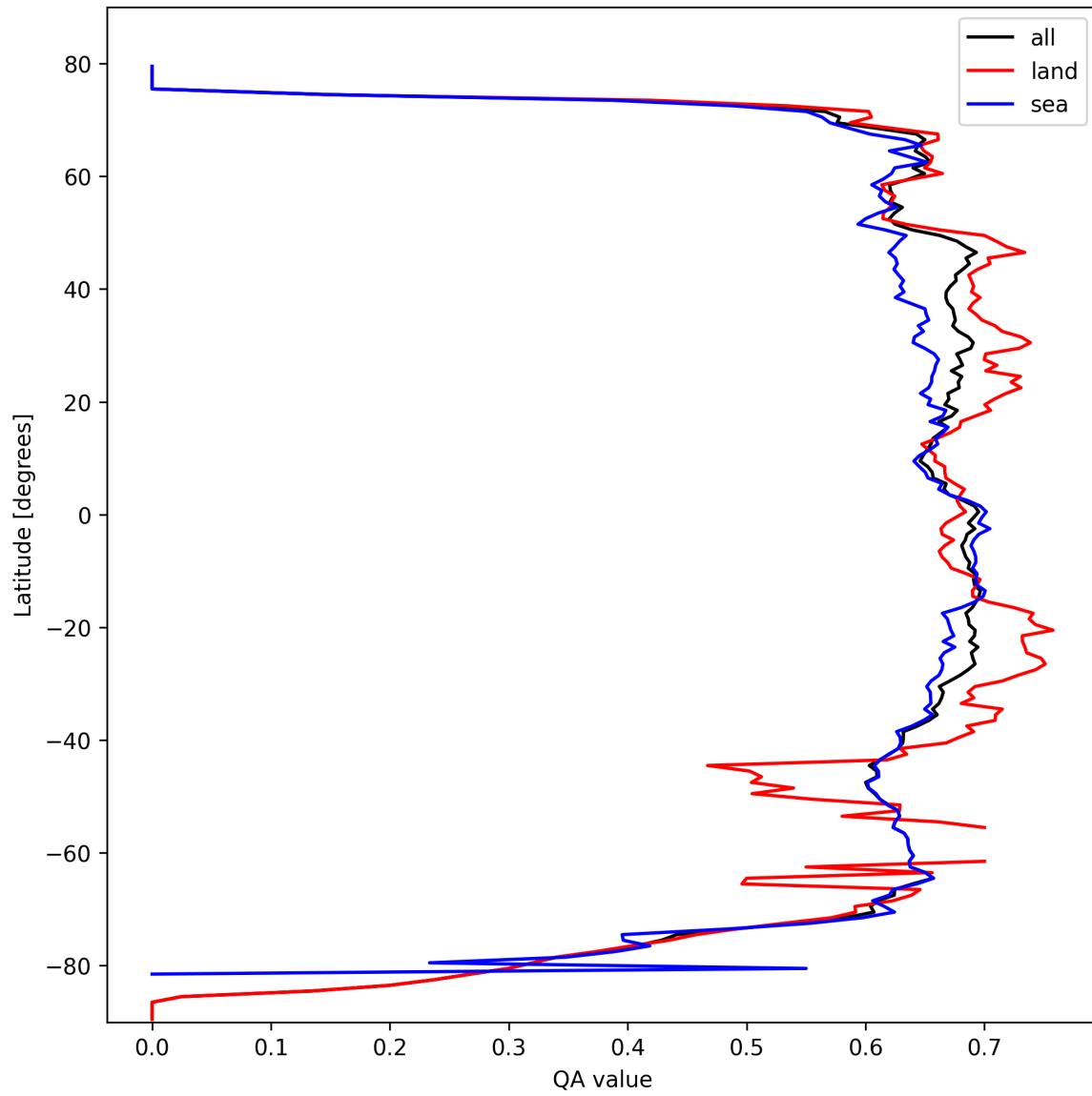
Figure 6: Zonal average of “QA value” for 2025-10-06 to 2025-10-07.
