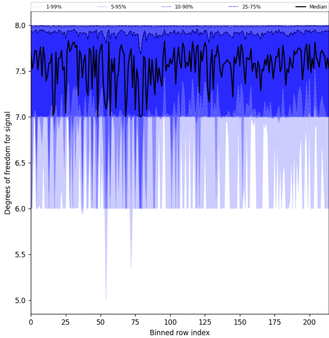
Figure 25: Along track statistics of “Degrees of freedom for signal” for 2025-10-06 to 2025-10-07
