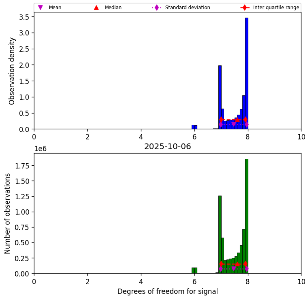
Figure 18: Histogram of “Degrees of freedom for signal” for 2025-10-06 to 2025-10-07
