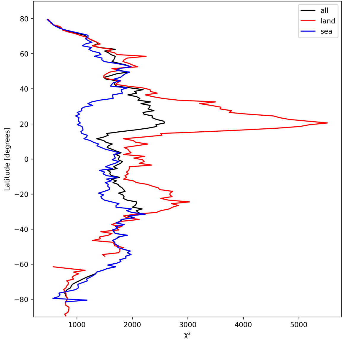
Figure 10: Zonal average of “ \chi^2 ” for 2025-10-06 to 2025-10-07.
