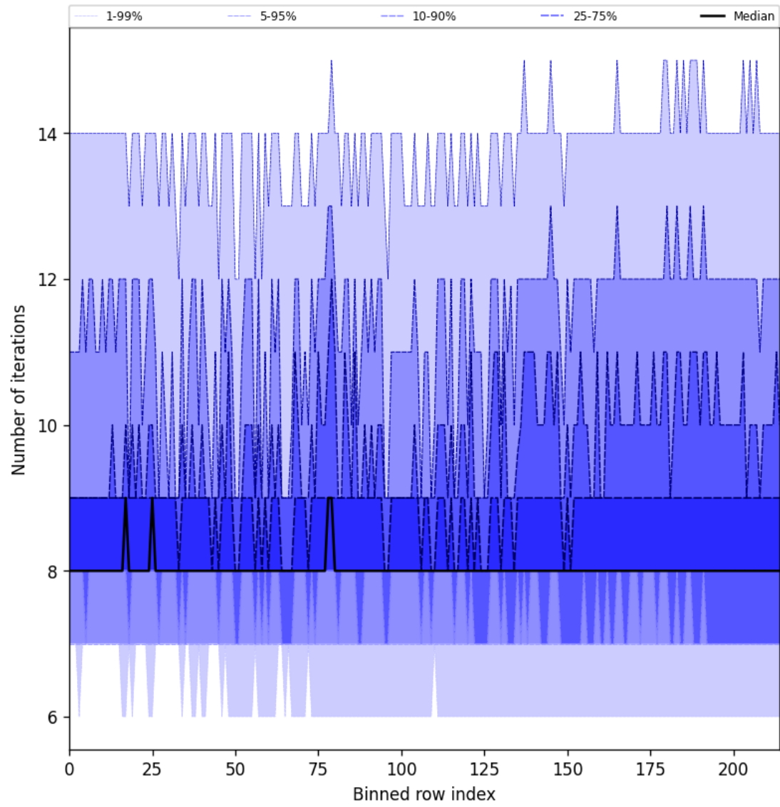
Figure 26: Along track statistics of “Number of iterations” for 2025-10-06 to 2025-10-07
