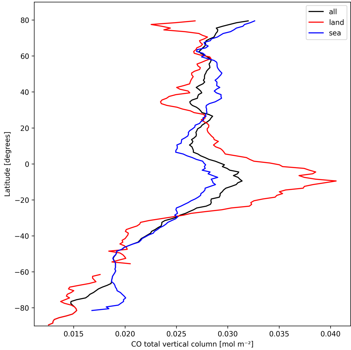
Figure 7: Zonal average of “CO total vertical column” for 2025-10-06 to 2025-10-07.
