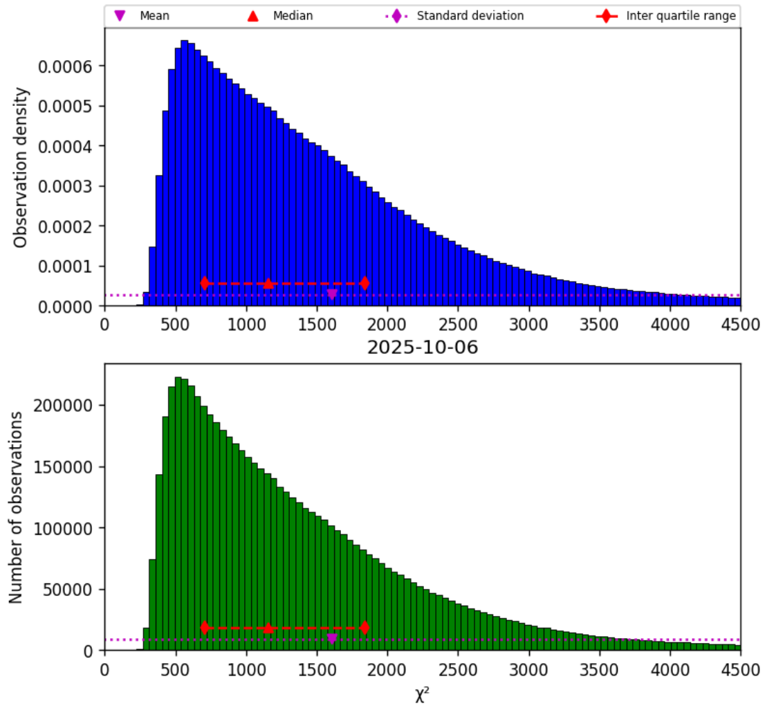
Figure 17: Histogram of “ \chi^2 ” for 2025-10-06 to 2025-10-07
