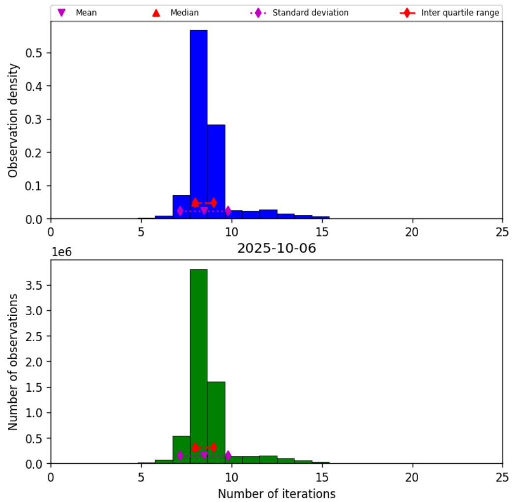
Figure 19: Histogram of “Number of iterations” for 2025-10-06 to 2025-10-07
