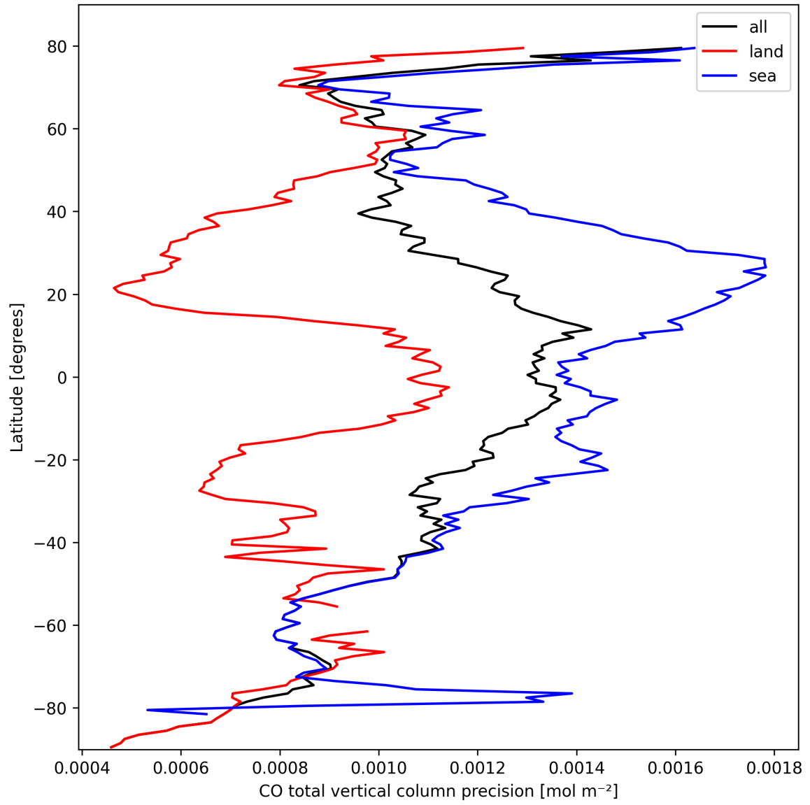
Figure 8: Zonal average of “CO total vertical column precision” for 2025-10-06 to 2025-10-07.
