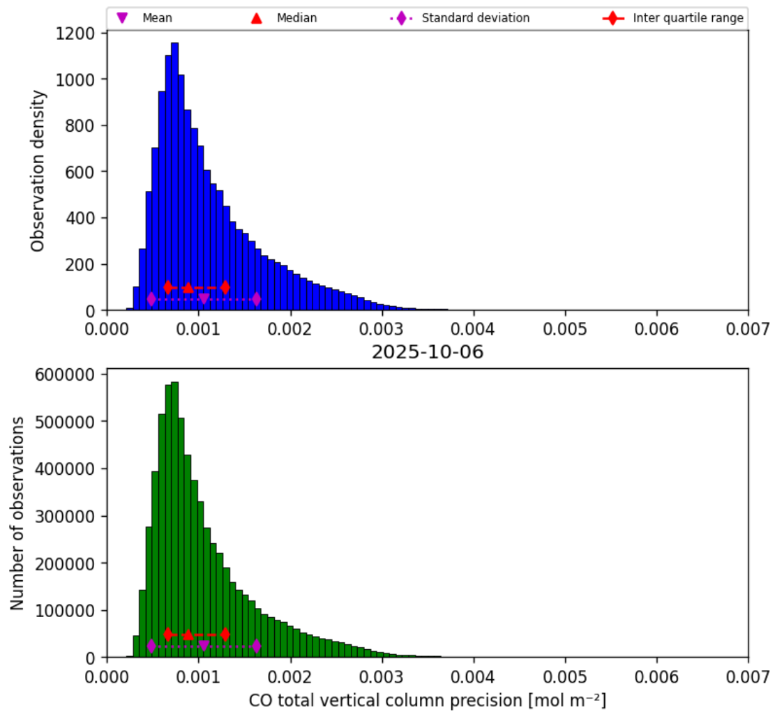
Figure 15: Histogram of “CO total vertical column precision” for 2025-10-06 to 2025-10-07
