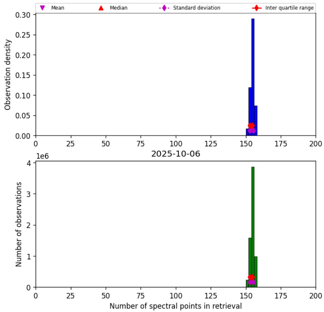
Figure 16: Histogram of "Number of spectral points in retrieval" for 2025-10-06 to 2025-10-07
