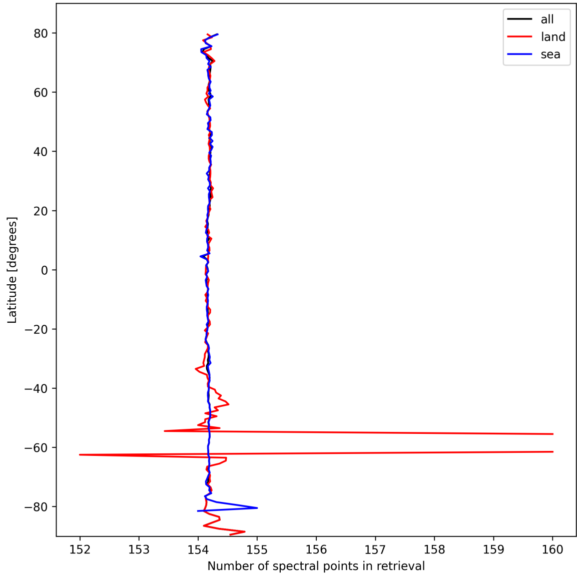
Figure 9: Zonal average of “Number of spectral points in retrieval” for 2025-10-06 to 2025-10-07.
