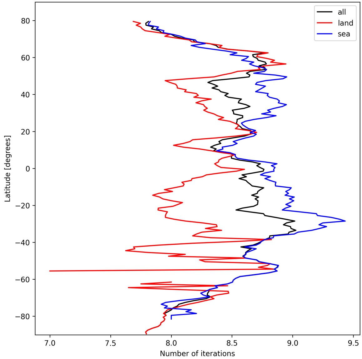
Figure 12: Zonal average of “Number of iterations” for 2025-10-06 to 2025-10-07.
