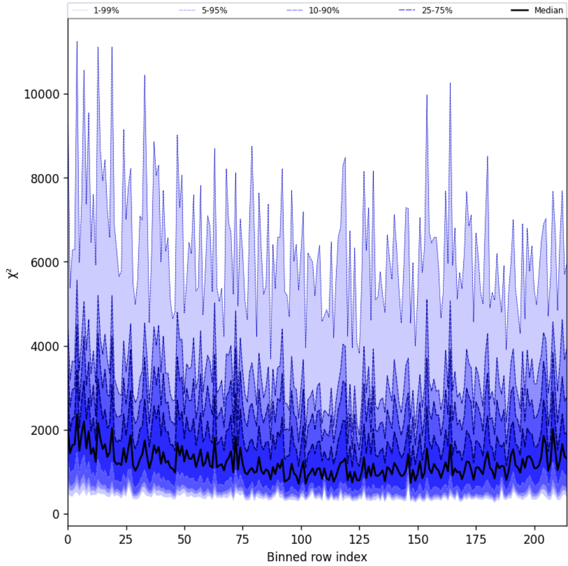
Figure 24: Along track statistics of “ \chi^2 ” for 2025-10-06 to 2025-10-07
