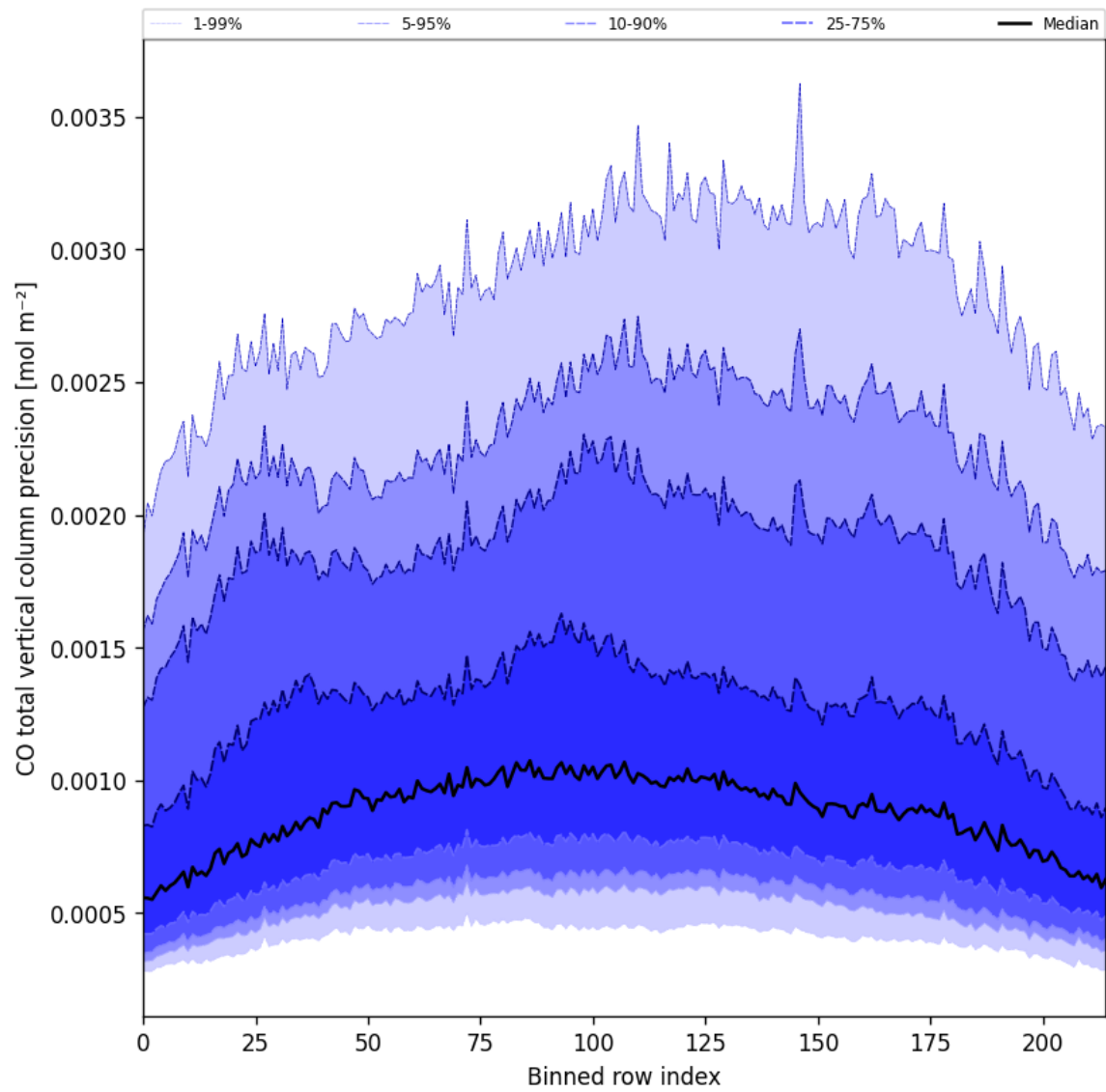
Figure 22: Along track statistics of “CO total vertical column precision” for 2025-10-06 to 2025-10-07
