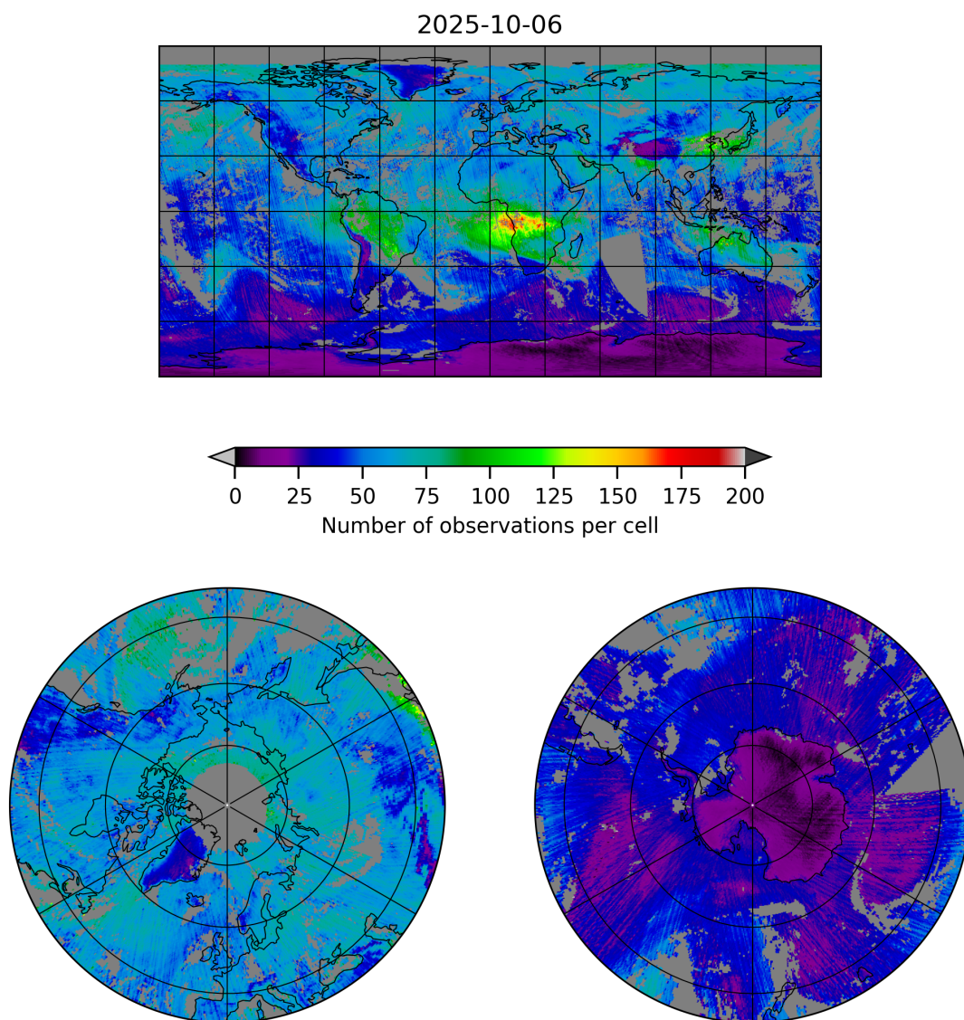
Figure 5: Map of the number of observations for 2025-10-06 to 2025-10-07
