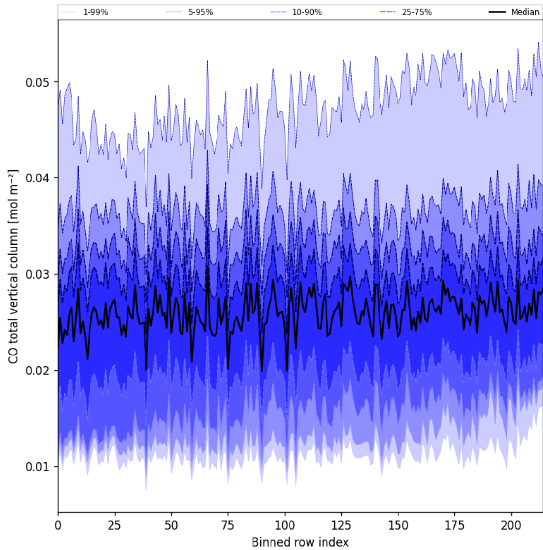
Figure 21: Along track statistics of “CO total vertical column” for 2025-10-07 to 2025-10-07
