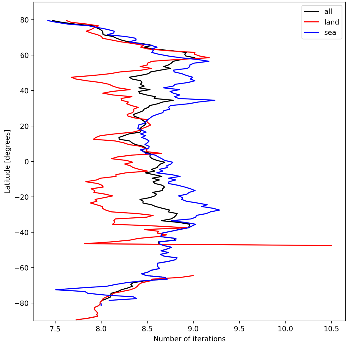
Figure 12: Zonal average of “Number of iterations” for 2025-10-07 to 2025-10-07.
