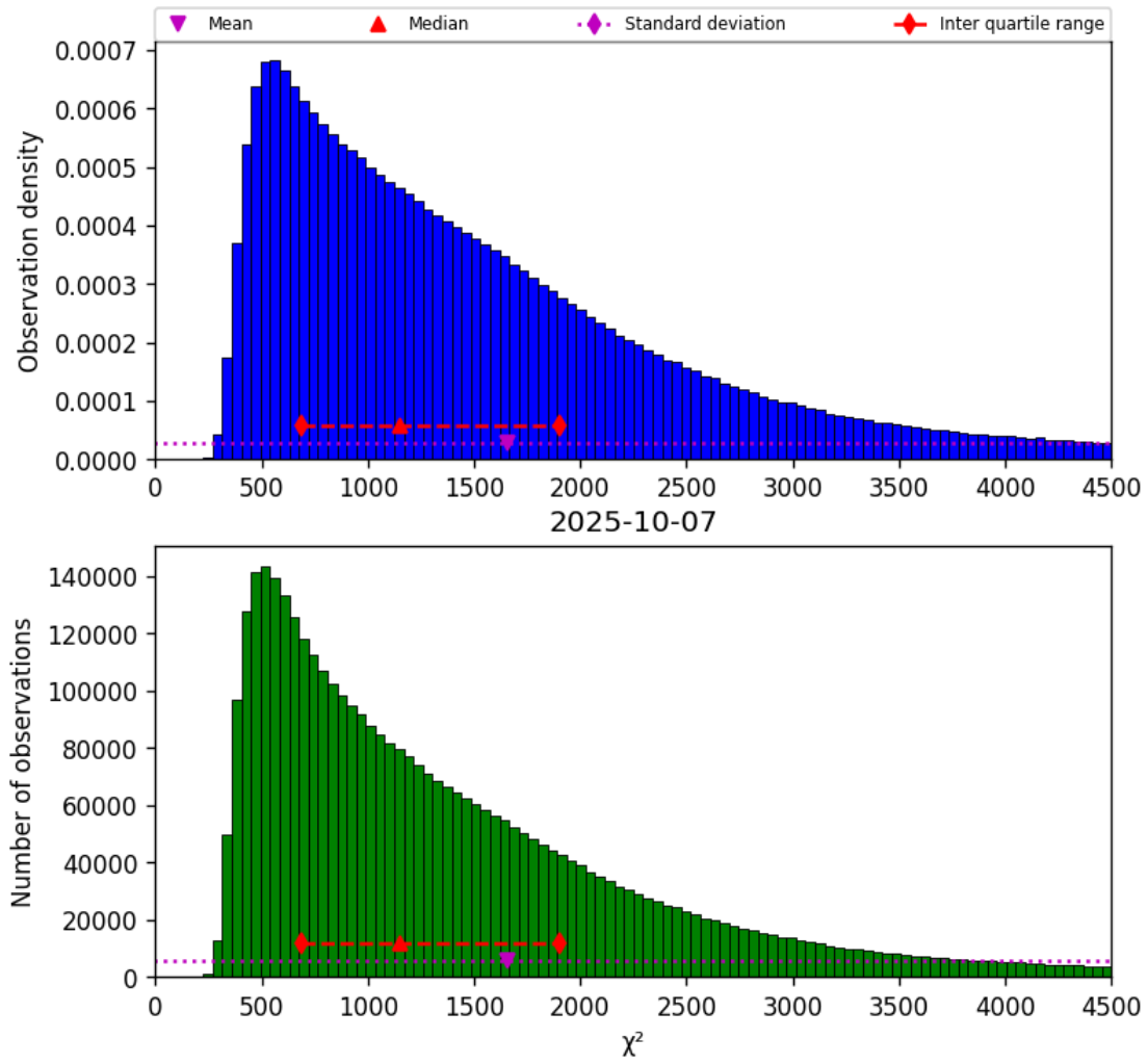
Figure 17: Histogram of " \chi^2 " for 2025-10-07 to 2025-10-07
