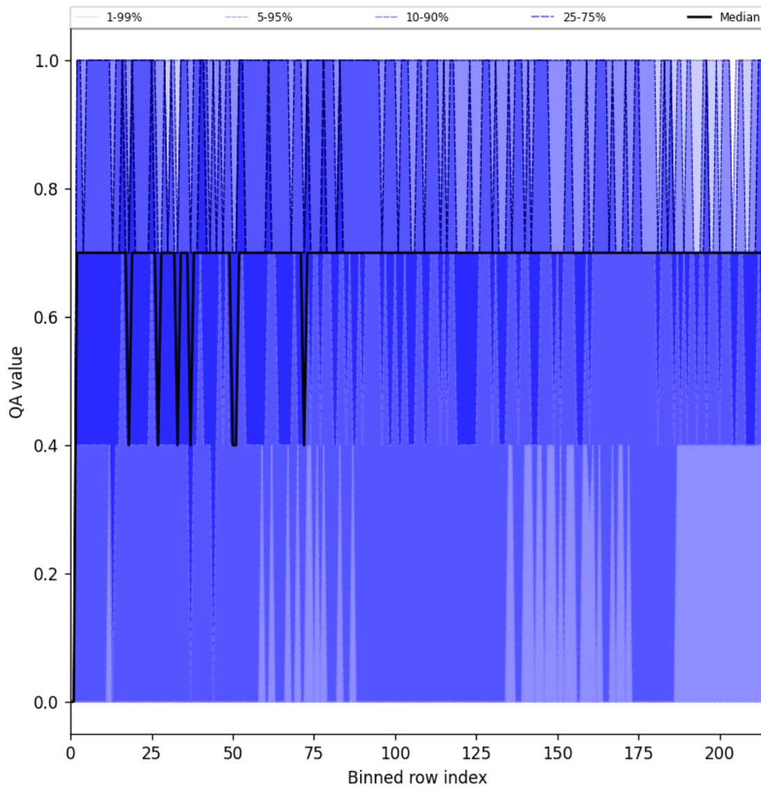
Figure 20: Along track statistics of “QA value” for 2025-10-07 to 2025-10-07
