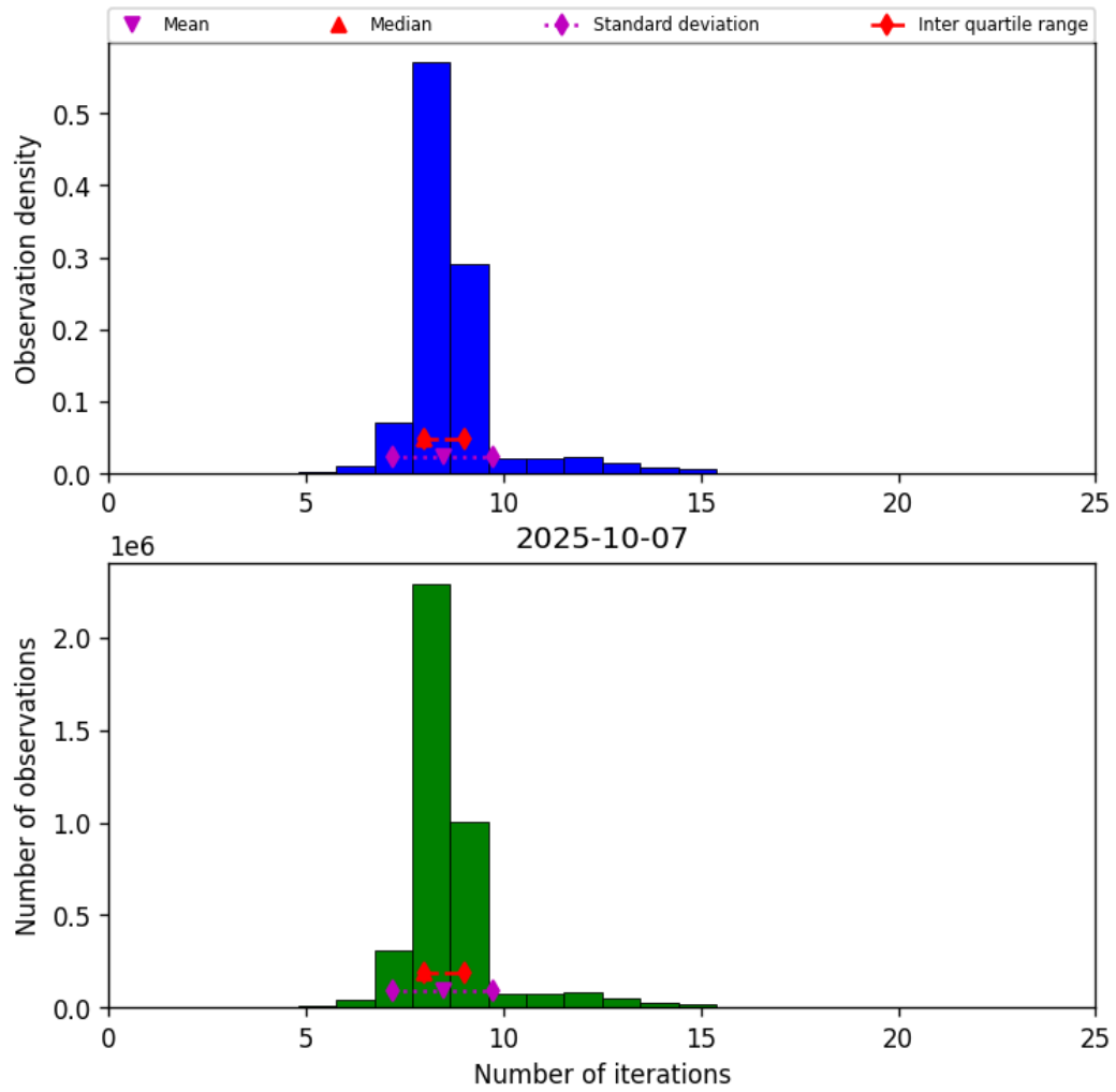
Figure 19: Histogram of “Number of iterations” for 2025-10-07 to 2025-10-07
