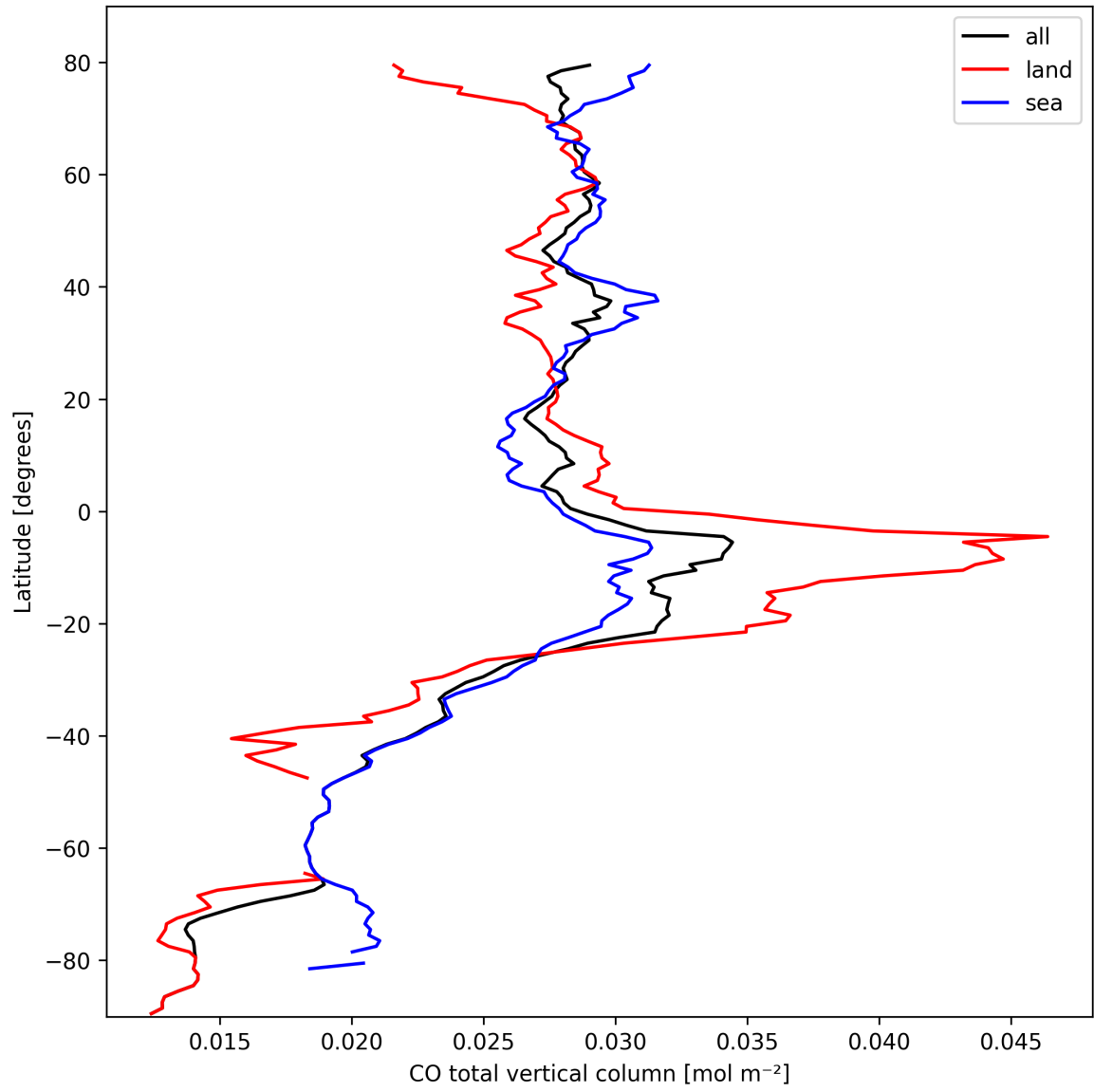
Figure 7: Zonal average of “CO total vertical column” for 2025-10-07 to 2025-10-07.
