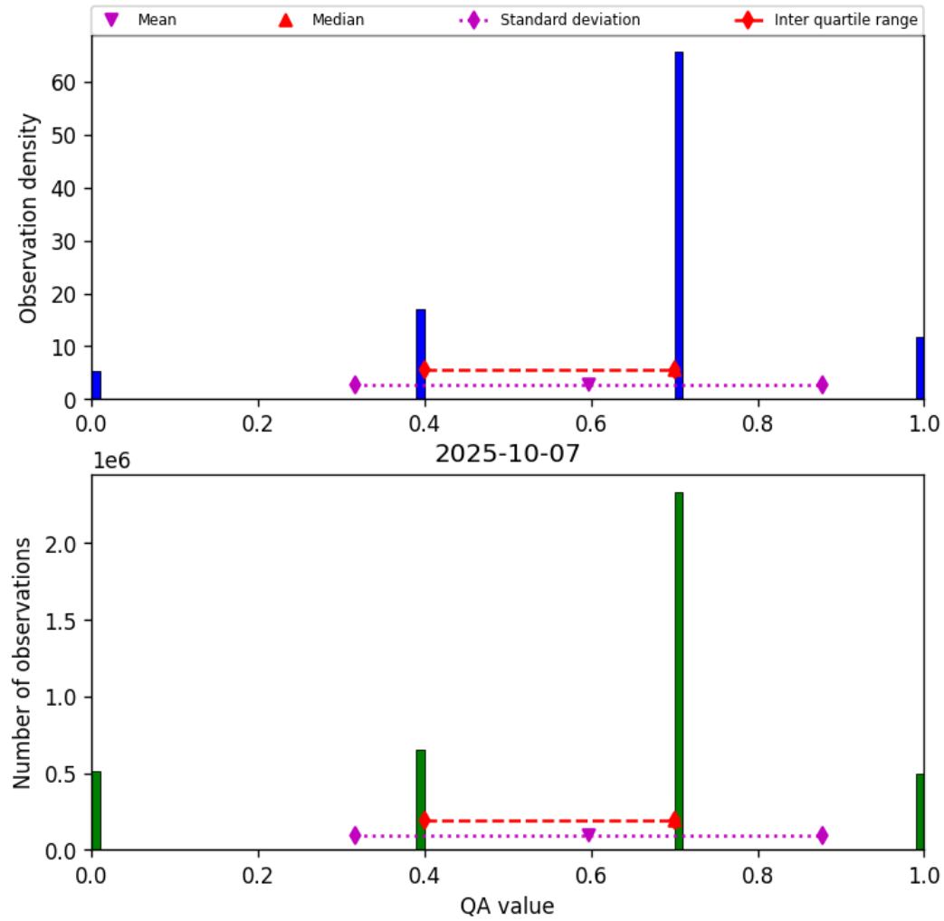
Figure 13: Histogram of “QA value” for 2025-10-07 to 2025-10-07
