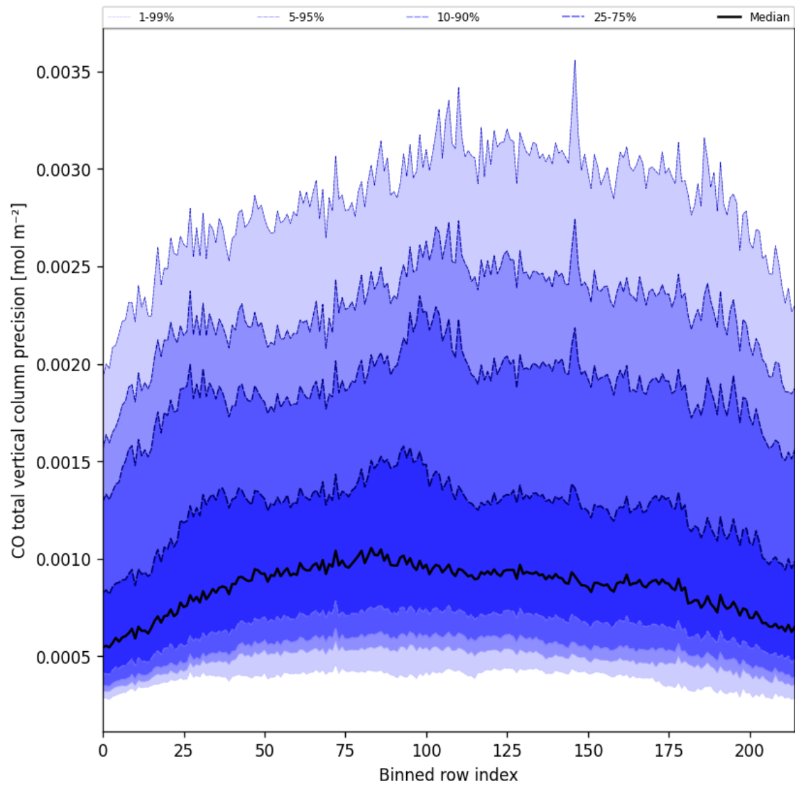
Figure 22: Along track statistics of “CO total vertical column precision” for 2025-10-07 to 2025-10-07
