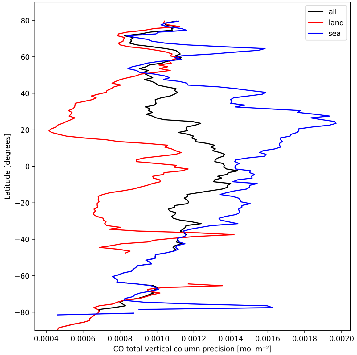
Figure 8: Zonal average of “CO total vertical column precision” for 2025-10-07 to 2025-10-07.
