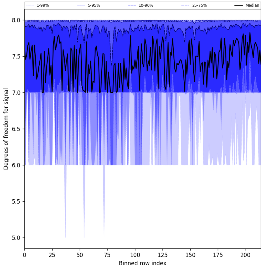
Figure 25: Along track statistics of “Degrees of freedom for signal” for 2025-10-07 to 2025-10-07
