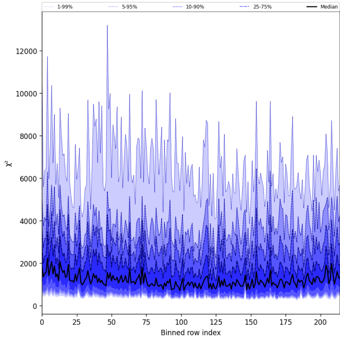
Figure 24: Along track statistics of “ \chi^2 ” for 2025-10-07 to 2025-10-07
