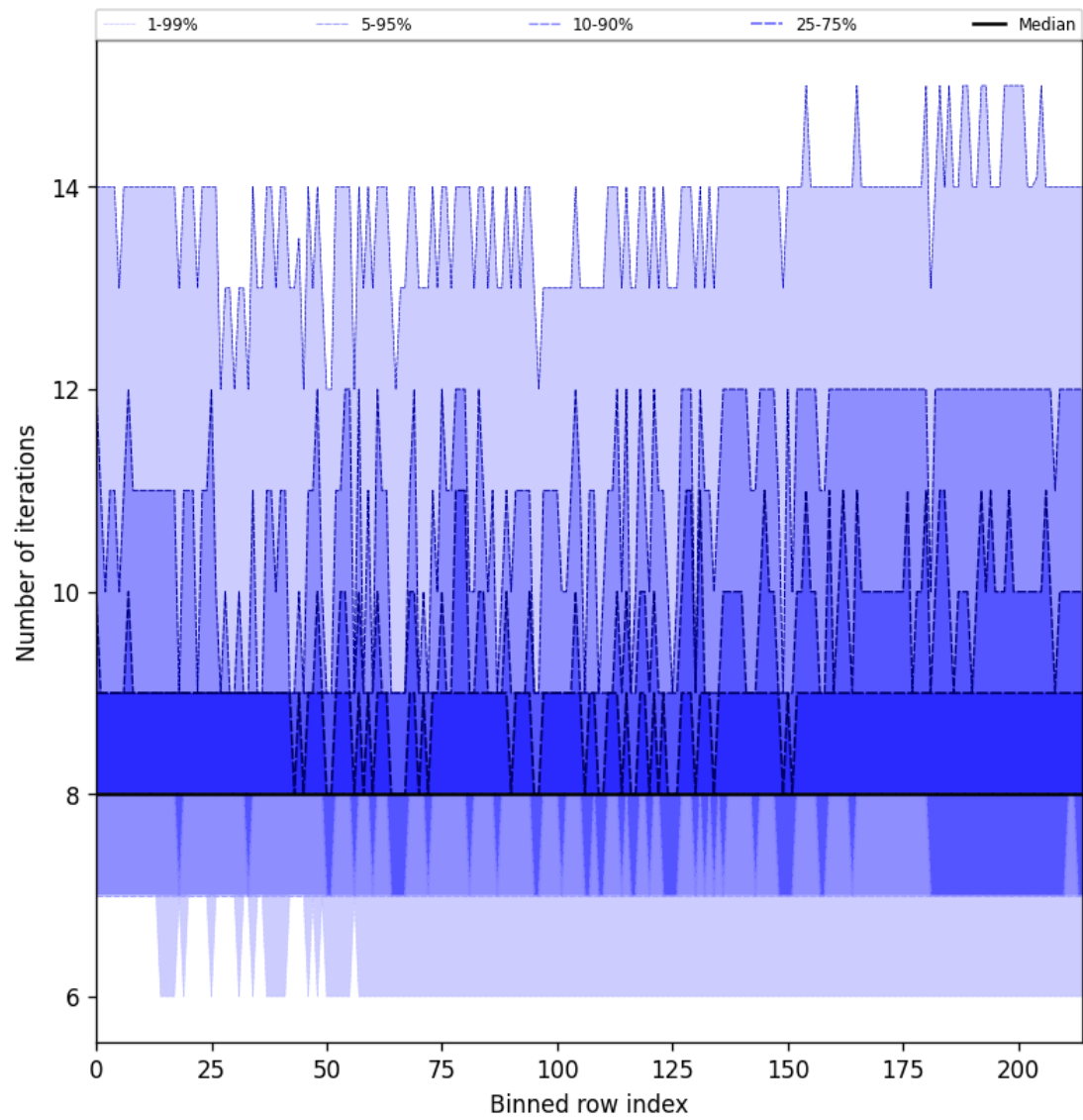
Figure 26: Along track statistics of “Number of iterations” for 2025-10-07 to 2025-10-07
