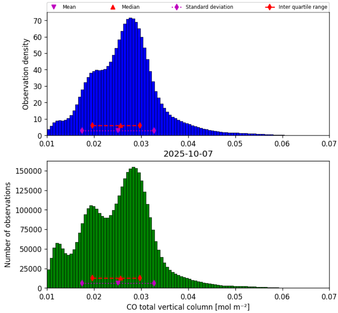
Figure 14: Histogram of “CO total vertical column” for 2025-10-07 to 2025-10-07
