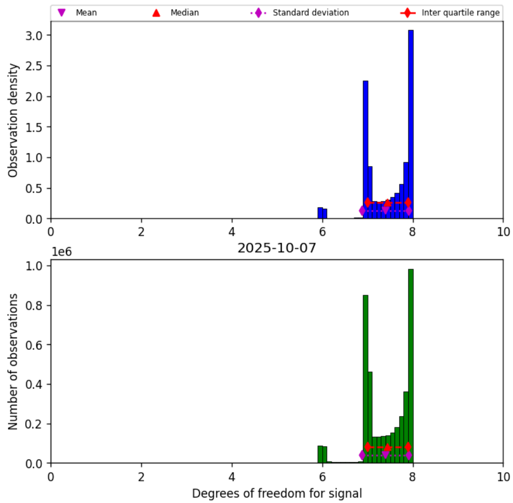
Figure 18: Histogram of “Degrees of freedom for signal” for 2025-10-07 to 2025-10-07
