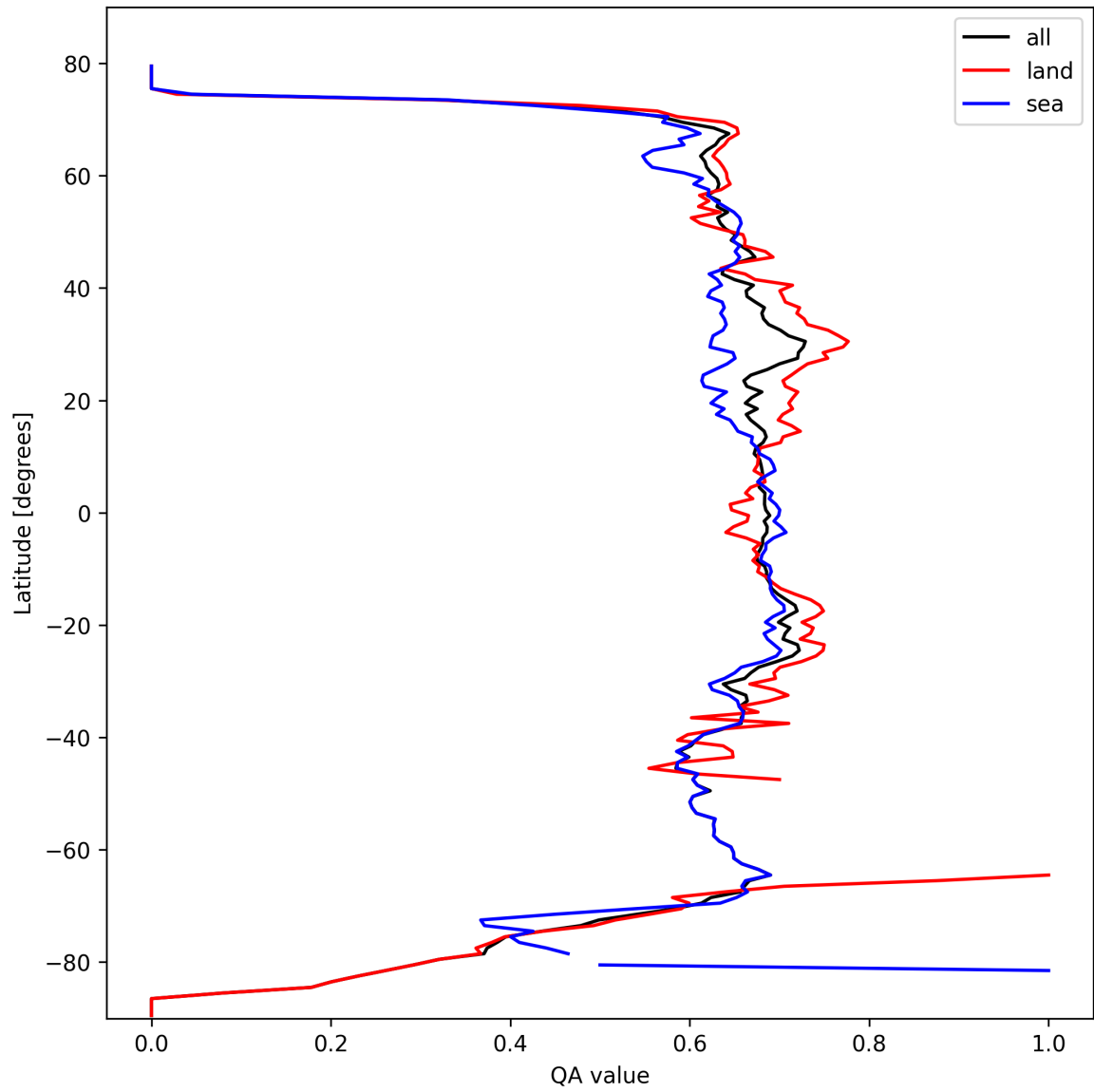
Figure 6: Zonal average of “QA value” for 2025-10-07 to 2025-10-07.
