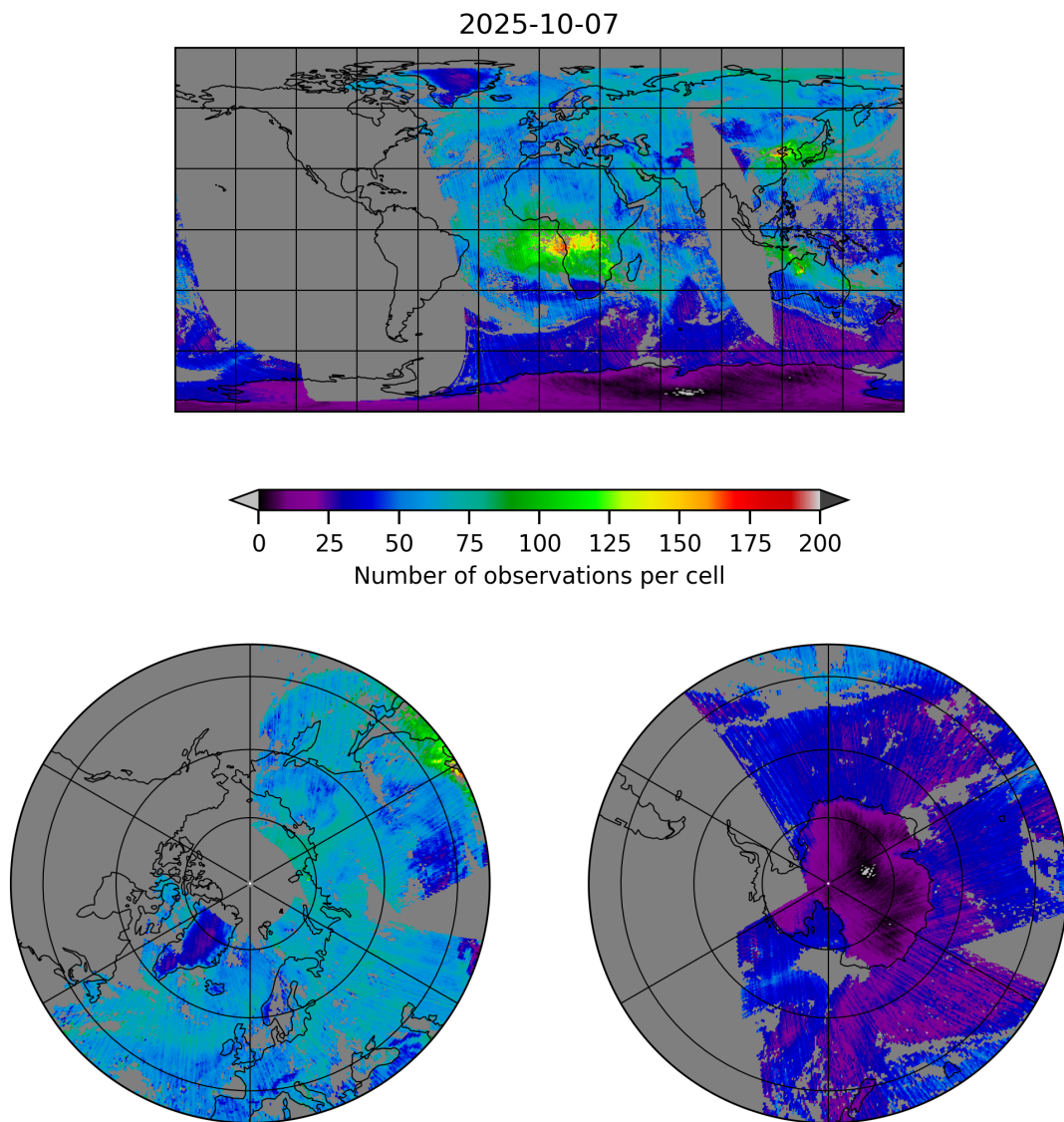
Figure 5: Map of the number of observations for 2025-10-07 to 2025-10-07
