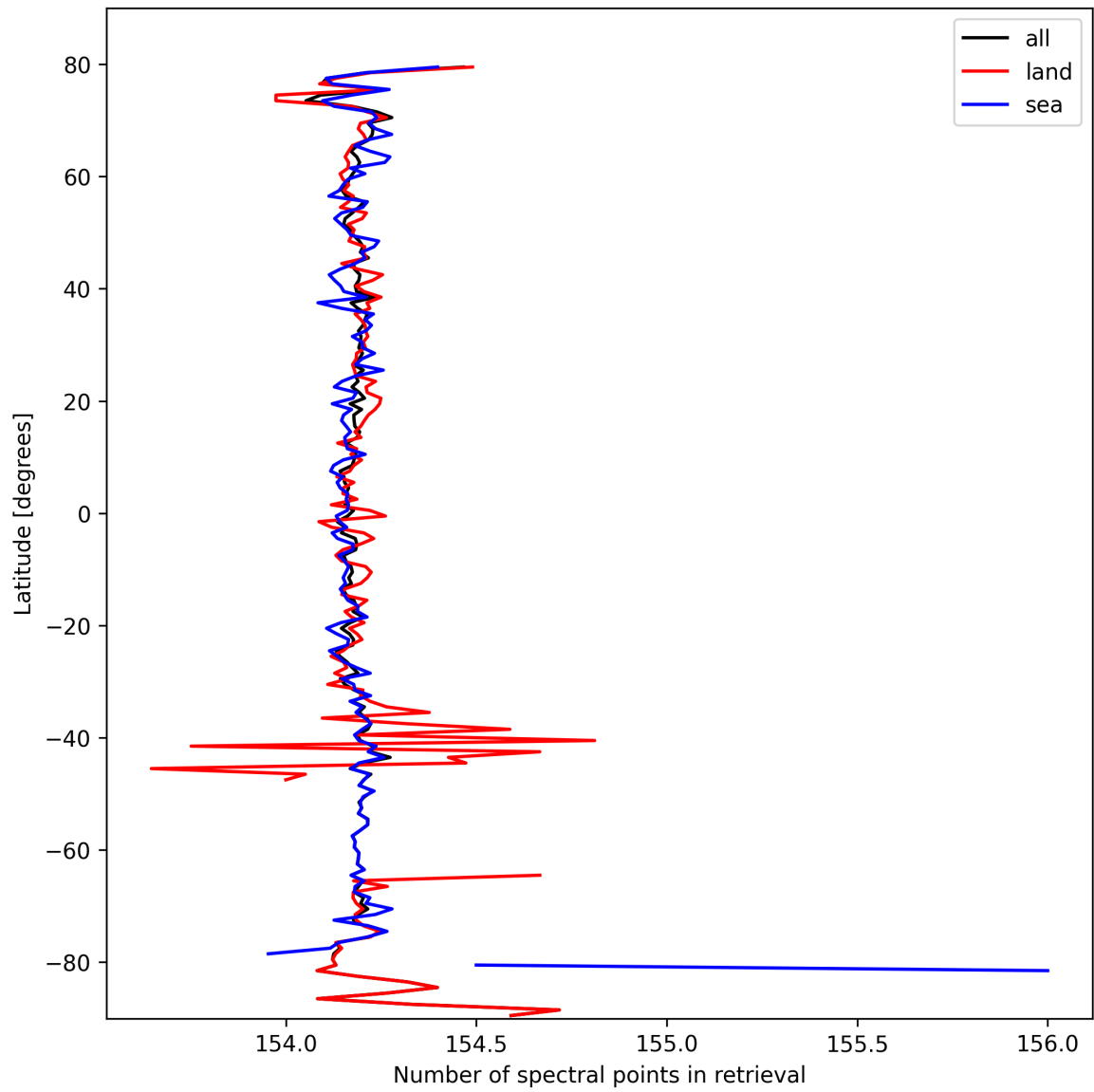
Figure 9: Zonal average of “Number of spectral points in retrieval” for 2025-10-07 to 2025-10-07.
