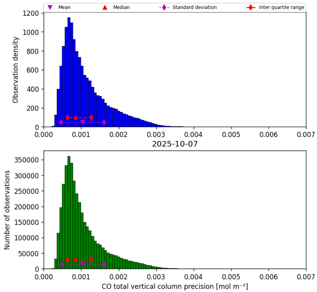
Figure 15: Histogram of “CO total vertical column precision” for 2025-10-07 to 2025-10-07
