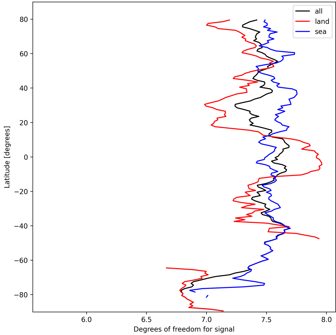
Figure 11: Zonal average of “Degrees of freedom for signal” for 2025-10-07 to 2025-10-07.
