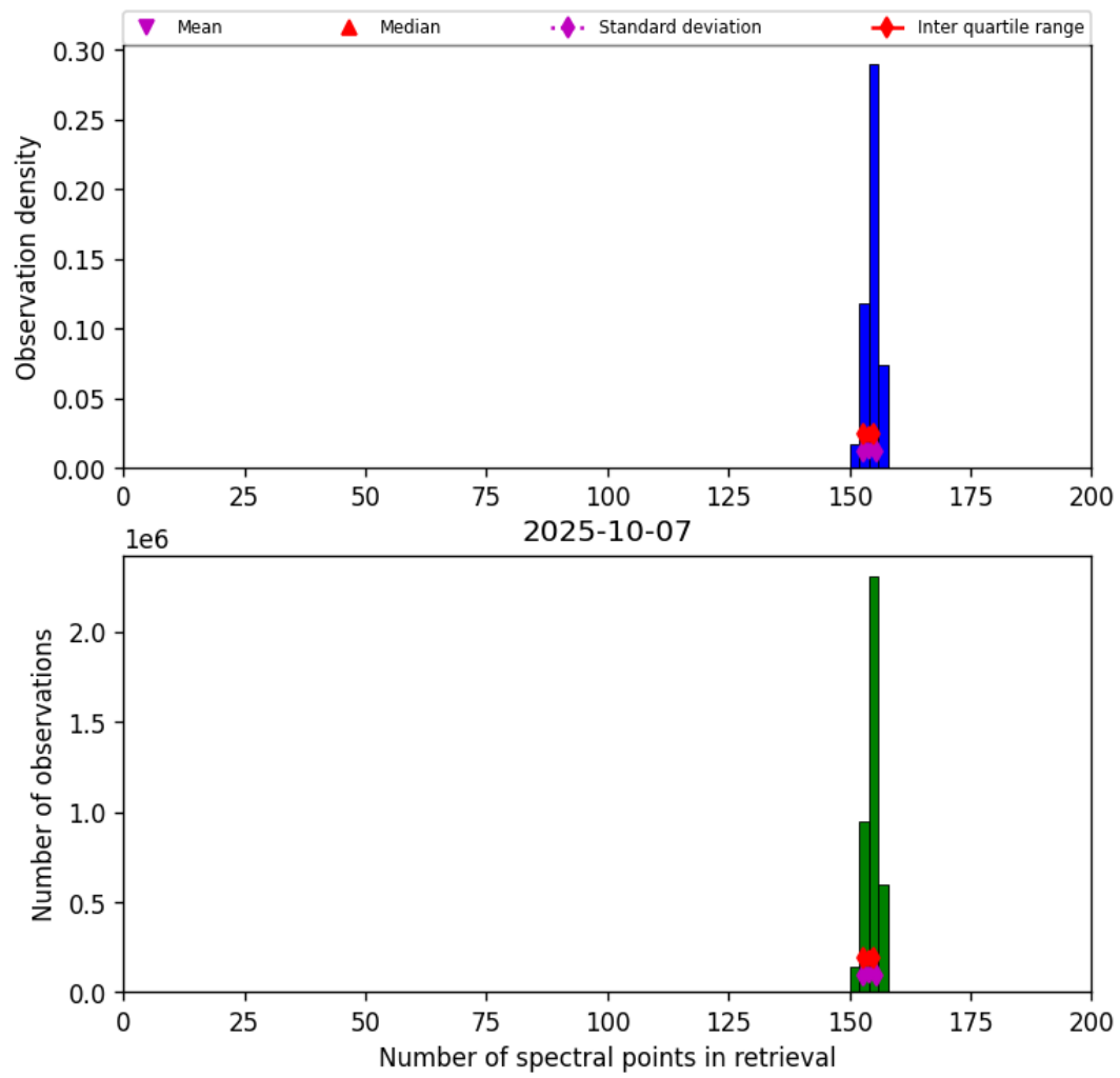
Figure 16: Histogram of “Number of spectral points in retrieval” for 2025-10-07 to 2025-10-07
