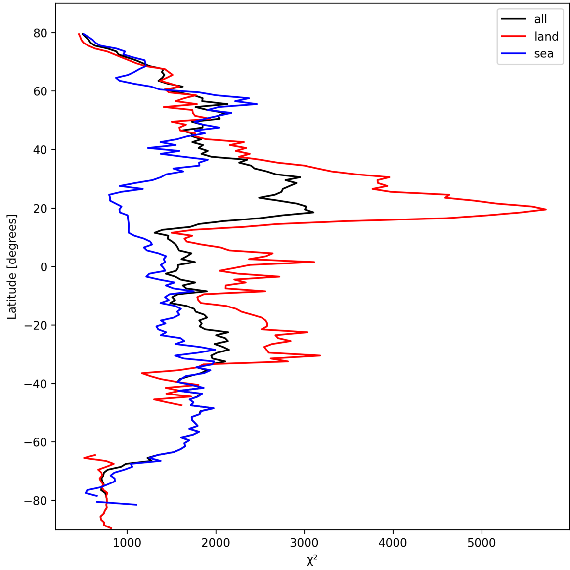
Figure 10: Zonal average of “ \chi^2 ” for 2025-10-07 to 2025-10-07.
