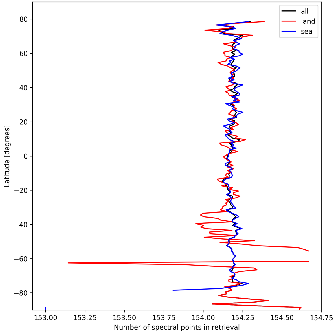
Figure 9: Zonal average of “Number of spectral points in retrieval” for 2025-10-08 to 2025-10-09.
