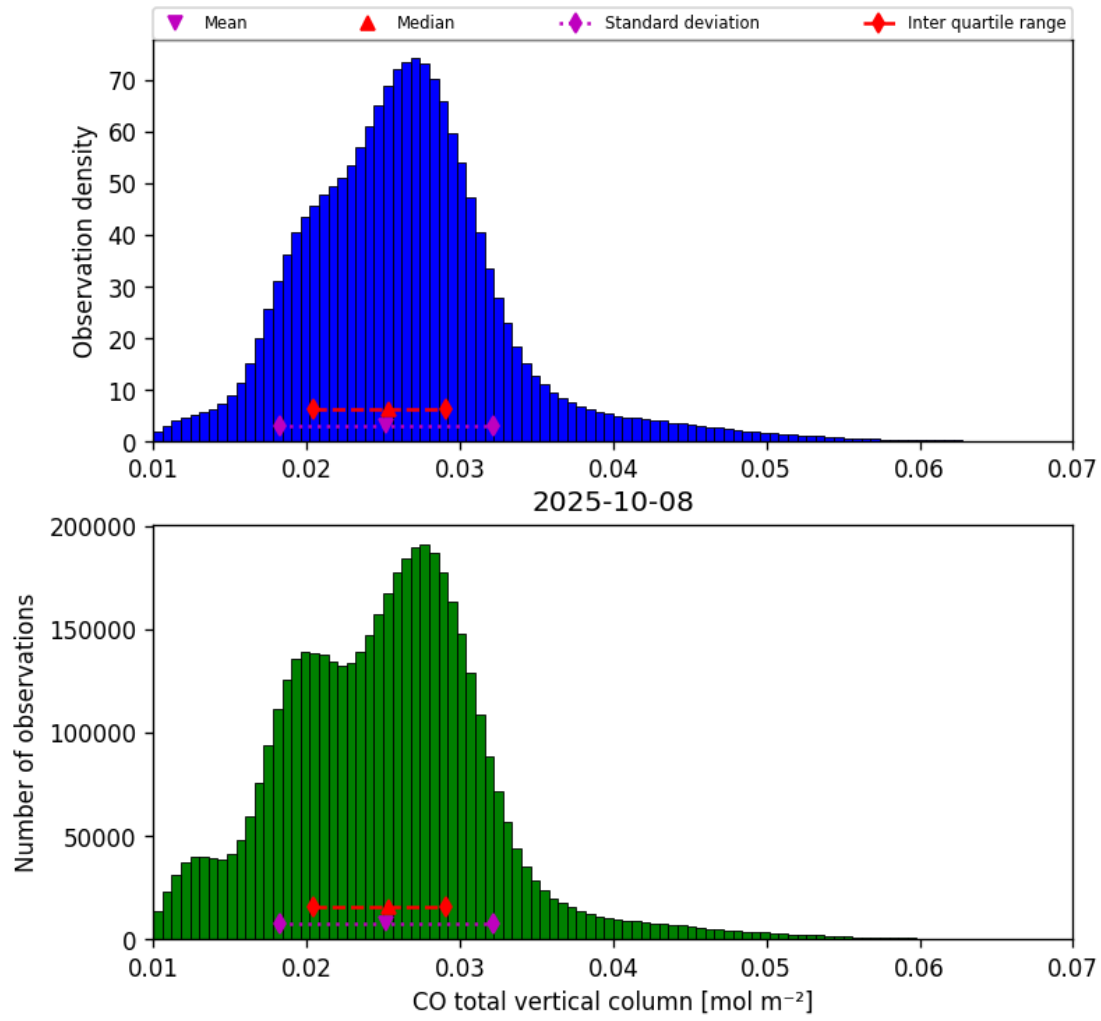
Figure 14: Histogram of “CO total vertical column” for 2025-10-08 to 2025-10-09
