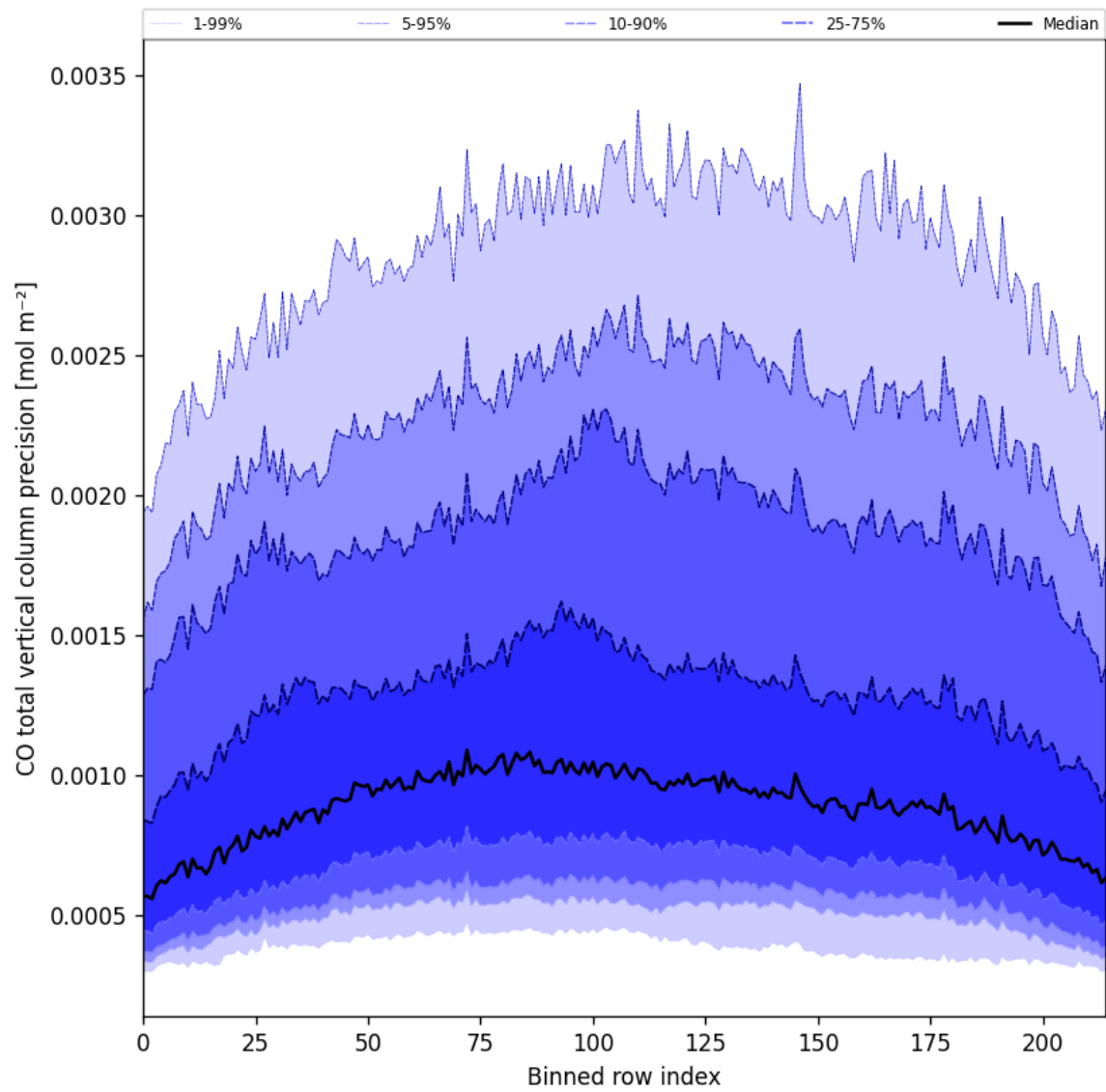
Figure 22: Along track statistics of “CO total vertical column precision” for 2025-10-08 to 2025-10-09
