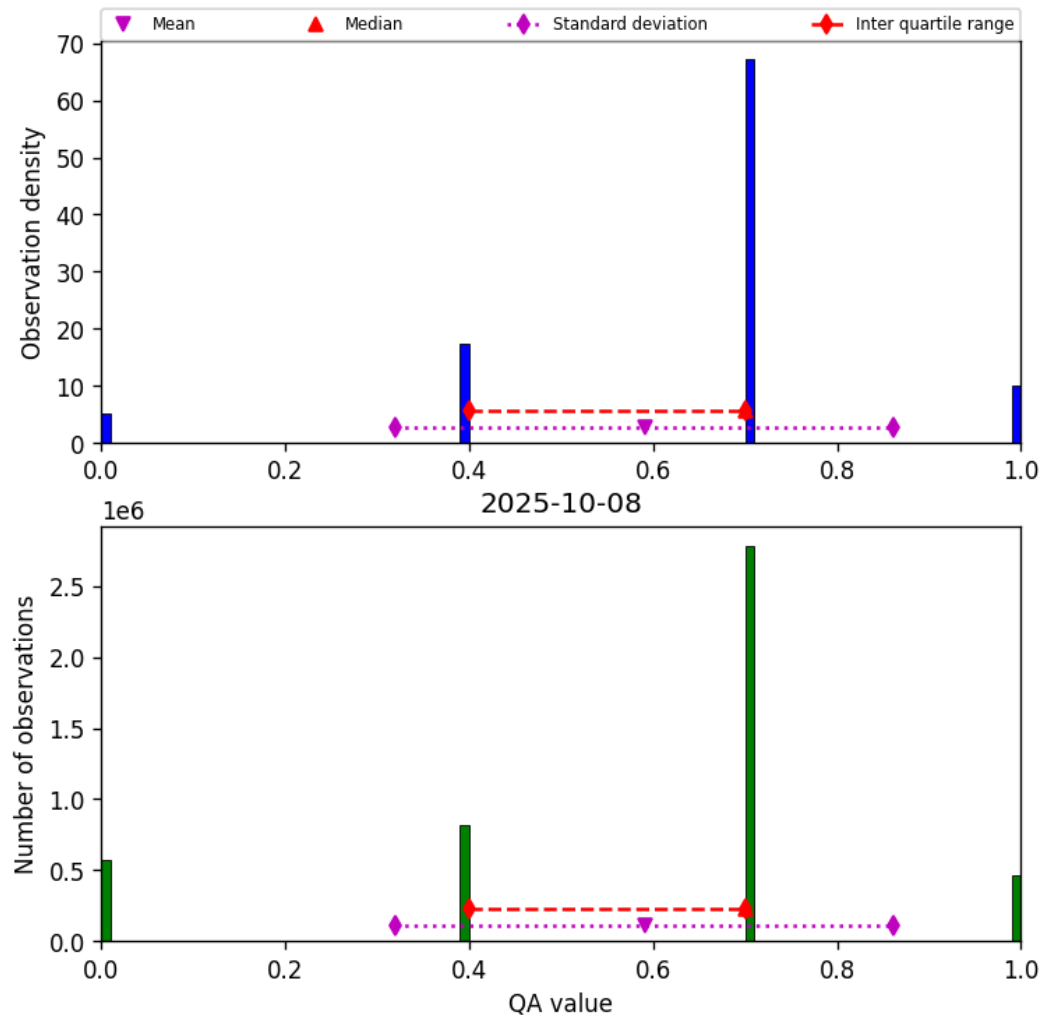
Figure 13: Histogram of “QA value” for 2025-10-08 to 2025-10-09
