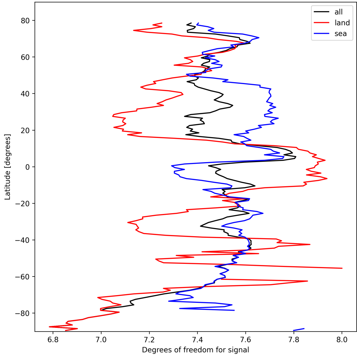
Figure 11: Zonal average of “Degrees of freedom for signal” for 2025-10-08 to 2025-10-09.
