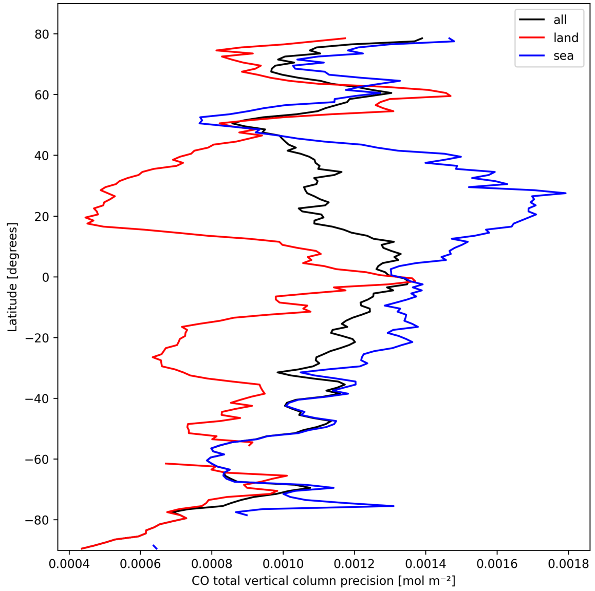
Figure 8: Zonal average of “CO total vertical column precision” for 2025-10-08 to 2025-10-09.
