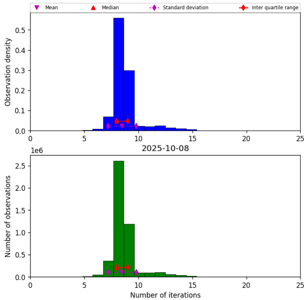
Figure 19: Histogram of “Number of iterations” for 2025-10-08 to 2025-10-09
