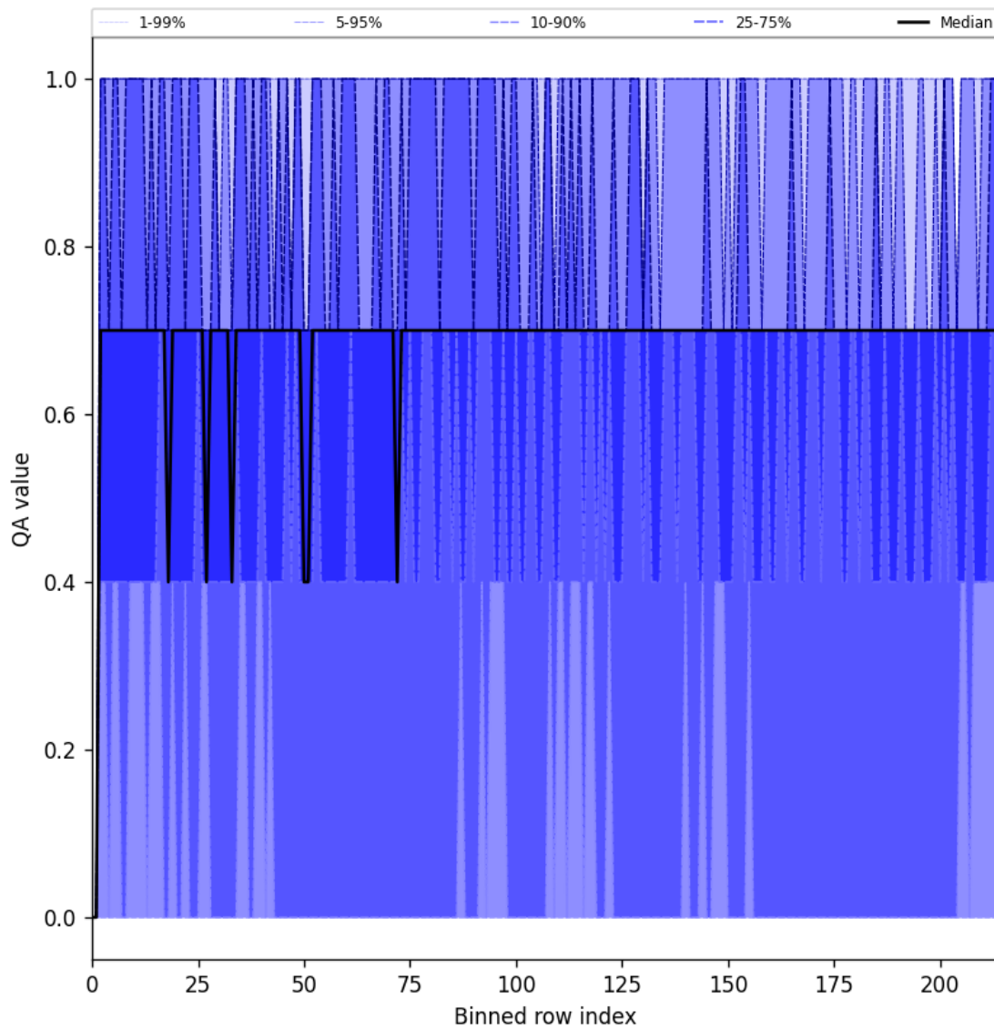
Figure 20: Along track statistics of “QA value” for 2025-10-08 to 2025-10-09
