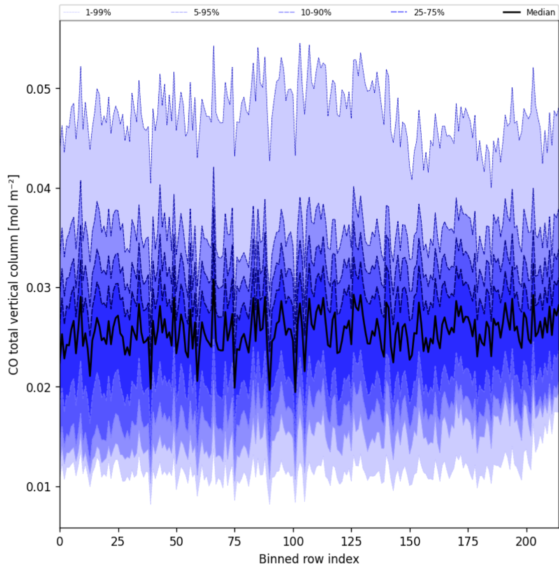
Figure 21: Along track statistics of “CO total vertical column” for 2025-10-08 to 2025-10-09
