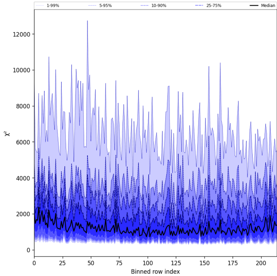
Figure 24: Along track statistics of “ \chi^2 ” for 2025-10-08 to 2025-10-09
