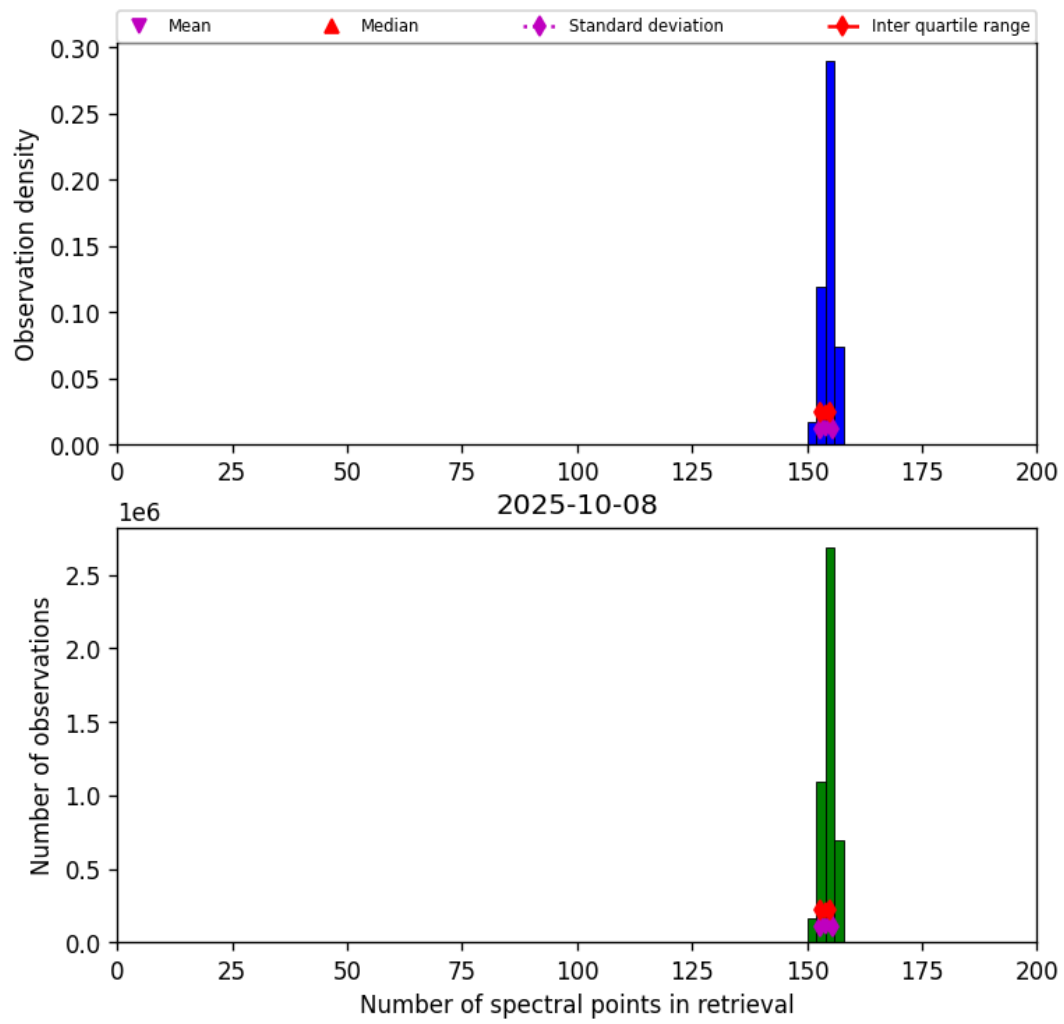
Figure 16: Histogram of “Number of spectral points in retrieval” for 2025-10-08 to 2025-10-09
