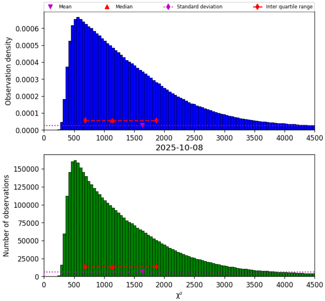
Figure 17: Histogram of “ \chi^2 ” for 2025-10-08 to 2025-10-09
