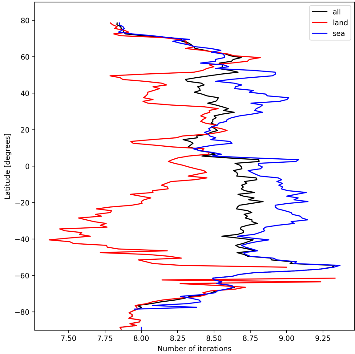
Figure 12: Zonal average of “Number of iterations” for 2025-10-08 to 2025-10-09.
