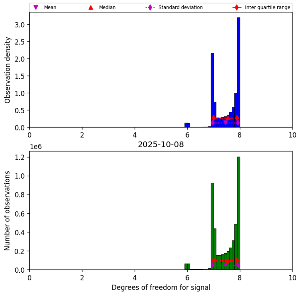
Figure 18: Histogram of “Degrees of freedom for signal” for 2025-10-08 to 2025-10-09
