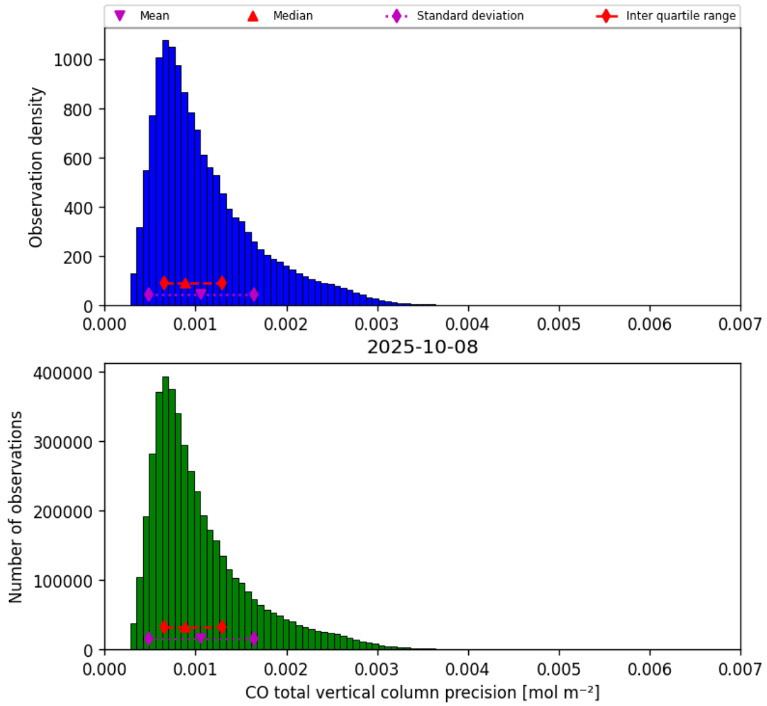
Figure 15: Histogram of “CO total vertical column precision” for 2025-10-08 to 2025-10-09
