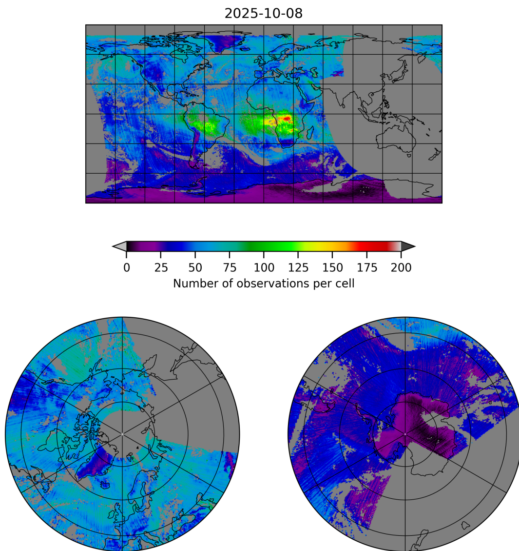
Figure 5: Map of the number of observations for 2025-10-08 to 2025-10-09
