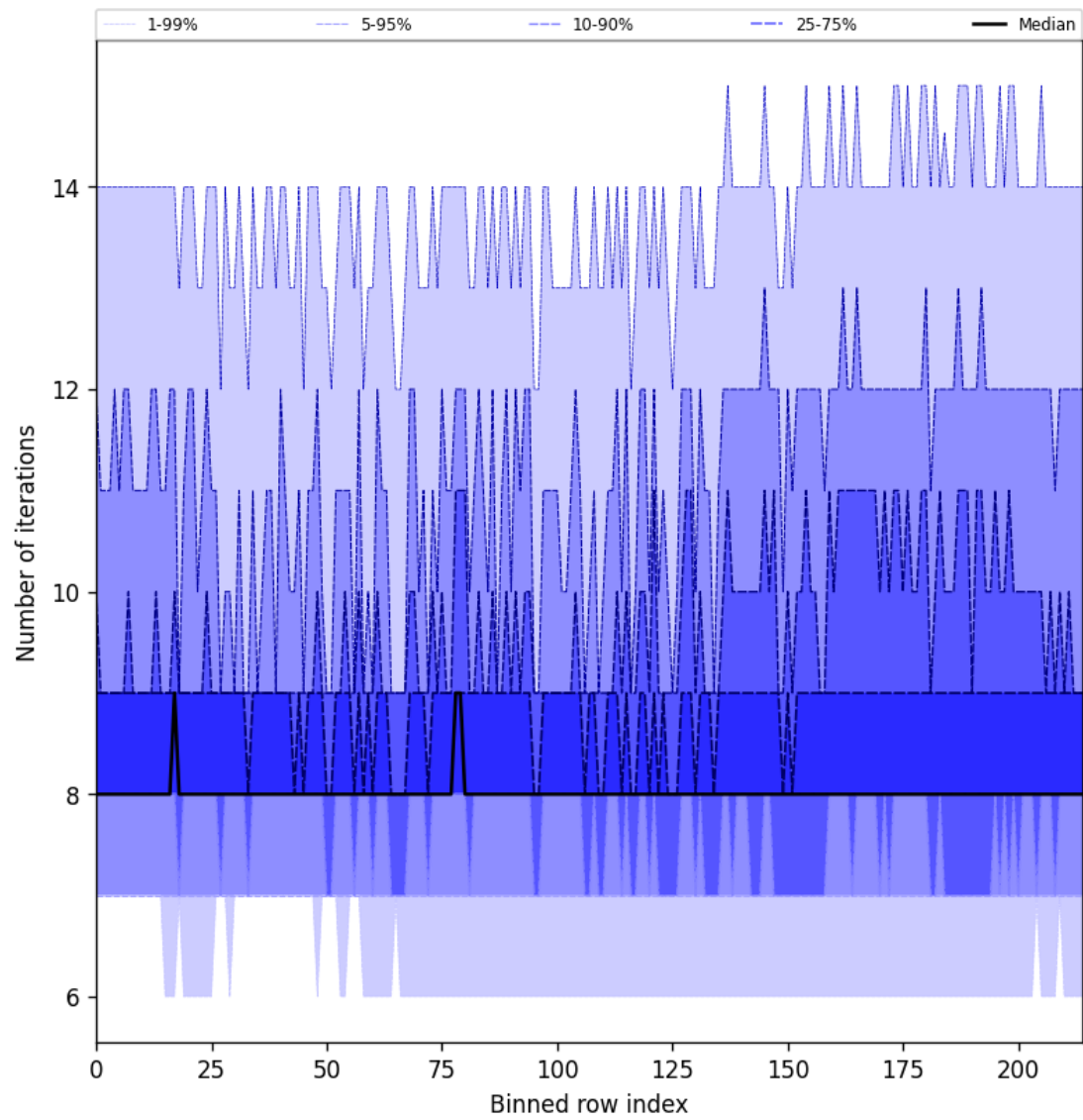
Figure 26: Along track statistics of “Number of iterations” for 2025-10-08 to 2025-10-09
