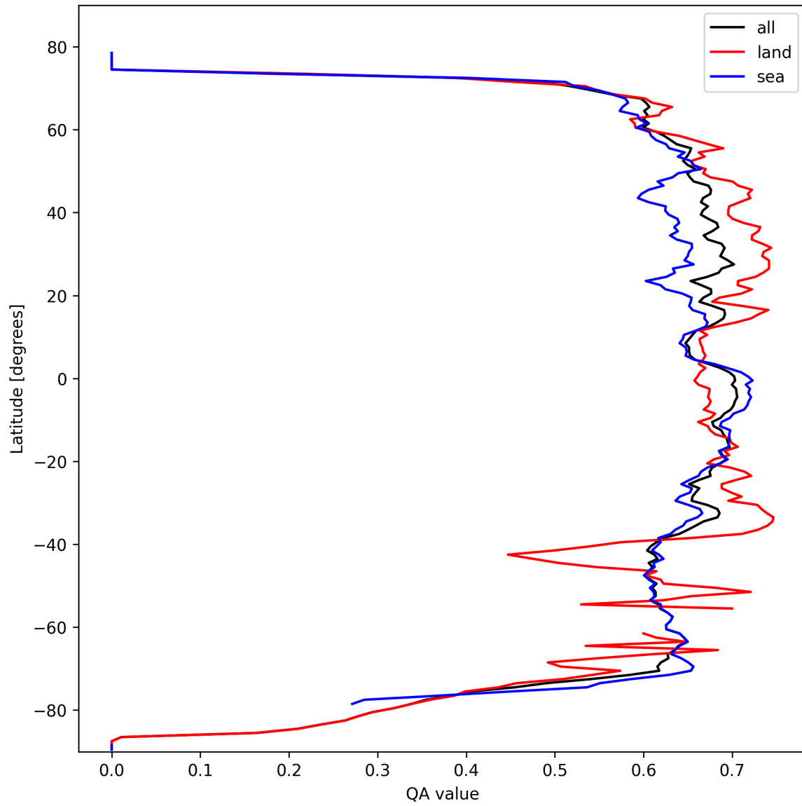
Figure 6: Zonal average of “QA value” for 2025-10-08 to 2025-10-09.
