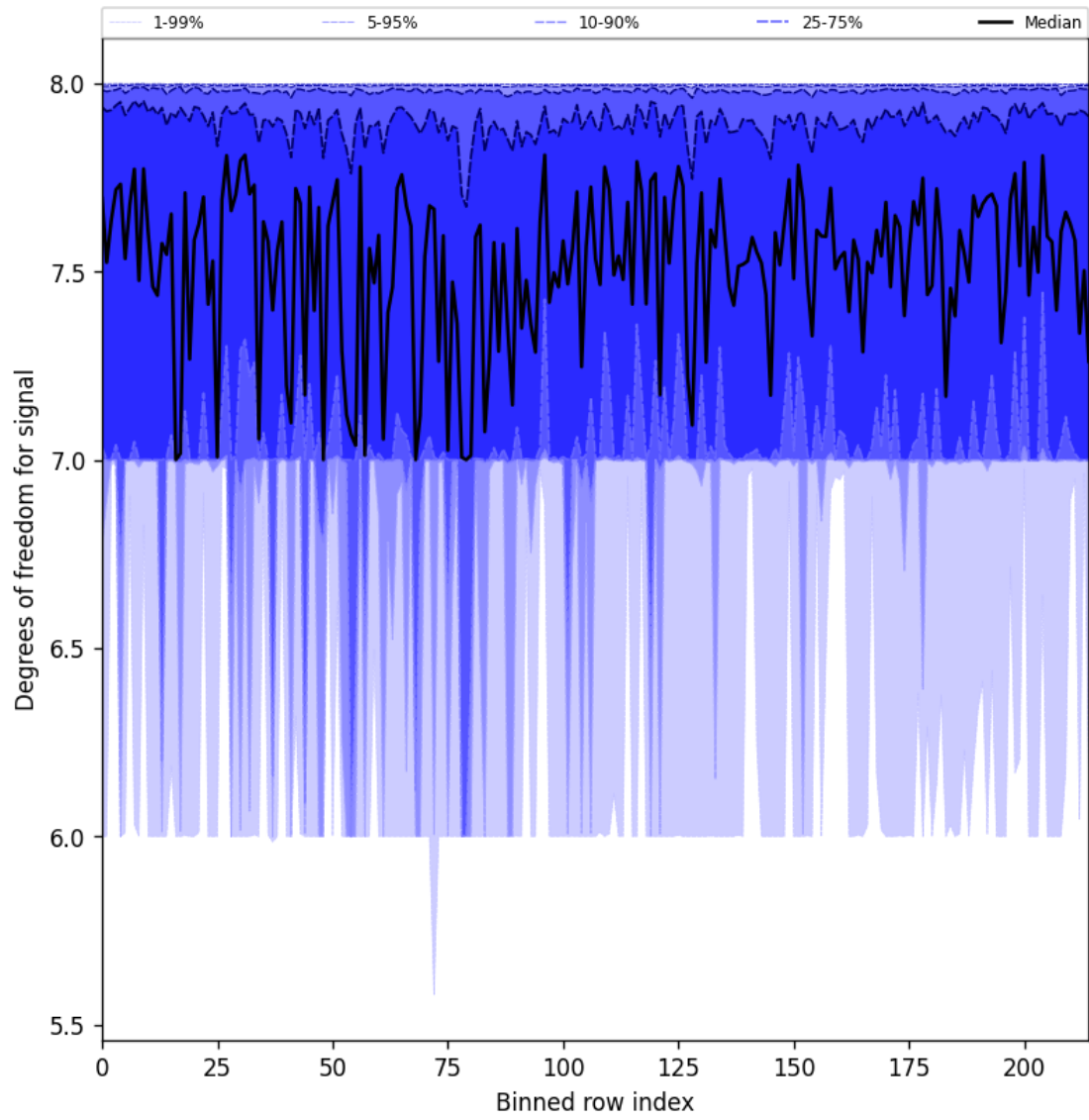
Figure 25: Along track statistics of “Degrees of freedom for signal” for 2025-10-08 to 2025-10-09
