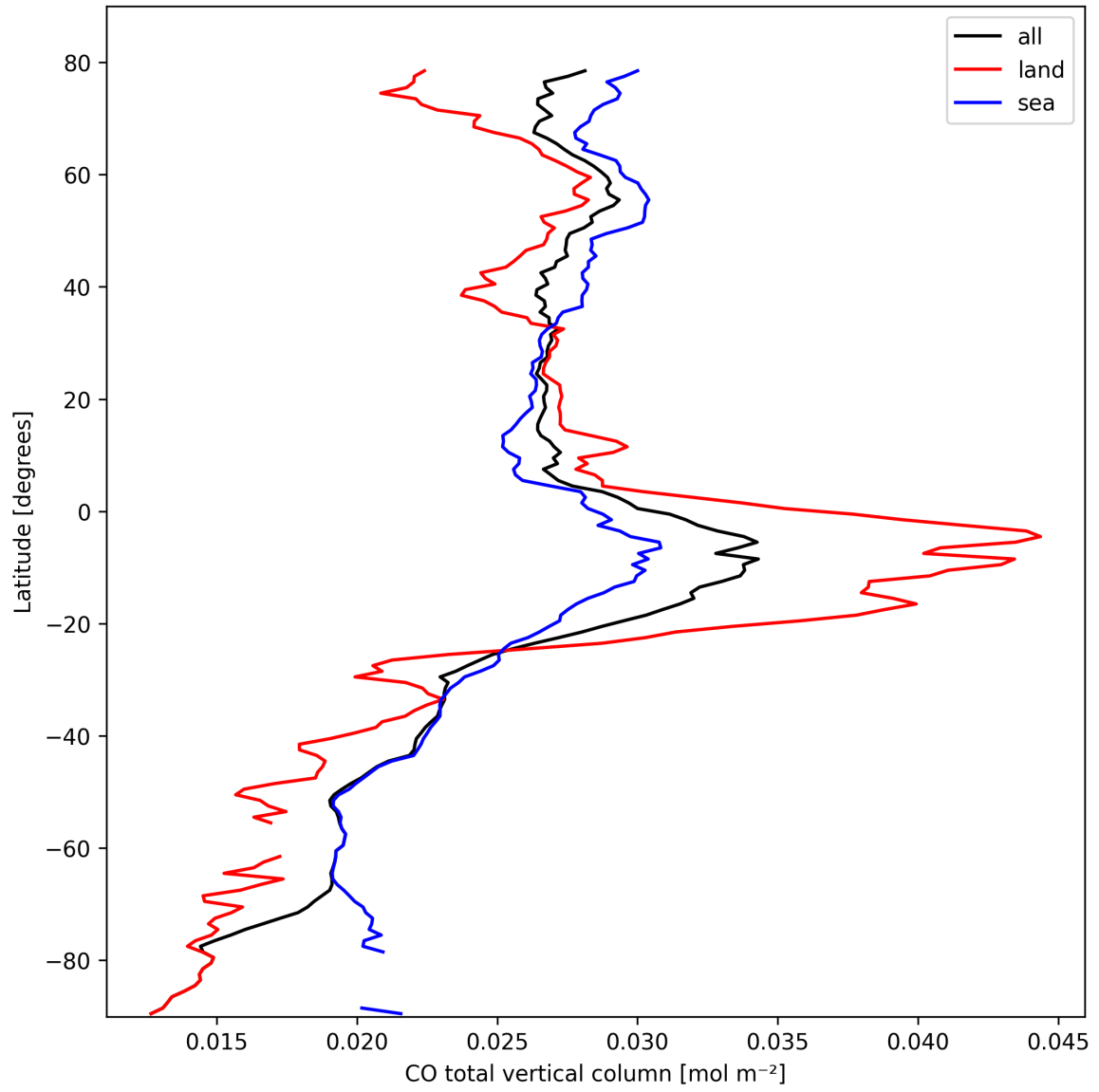
Figure 7: Zonal average of “CO total vertical column” for 2025-10-08 to 2025-10-09.
