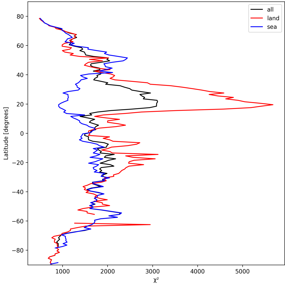
Figure 10: Zonal average of “ \chi^2 ” for 2025-10-08 to 2025-10-09.
