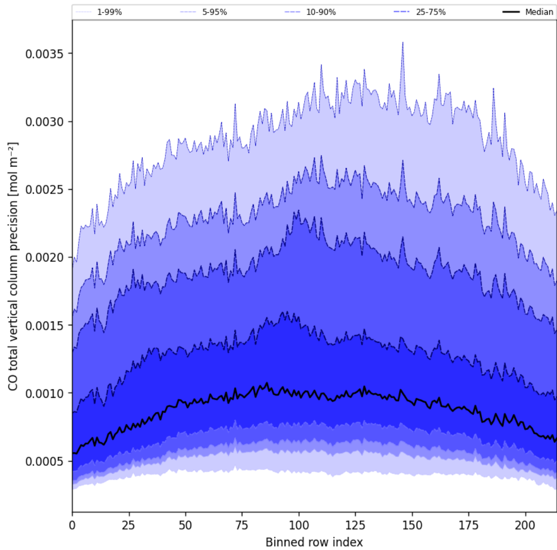
Figure 22: Along track statistics of “CO total vertical column precision” for 2025-10-09 to 2025-10-09
