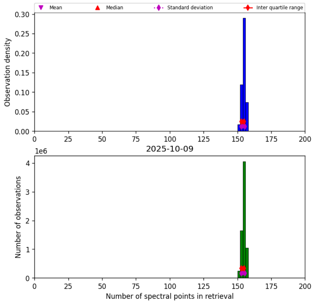
Figure 16: Histogram of “Number of spectral points in retrieval” for 2025-10-09 to 2025-10-09
