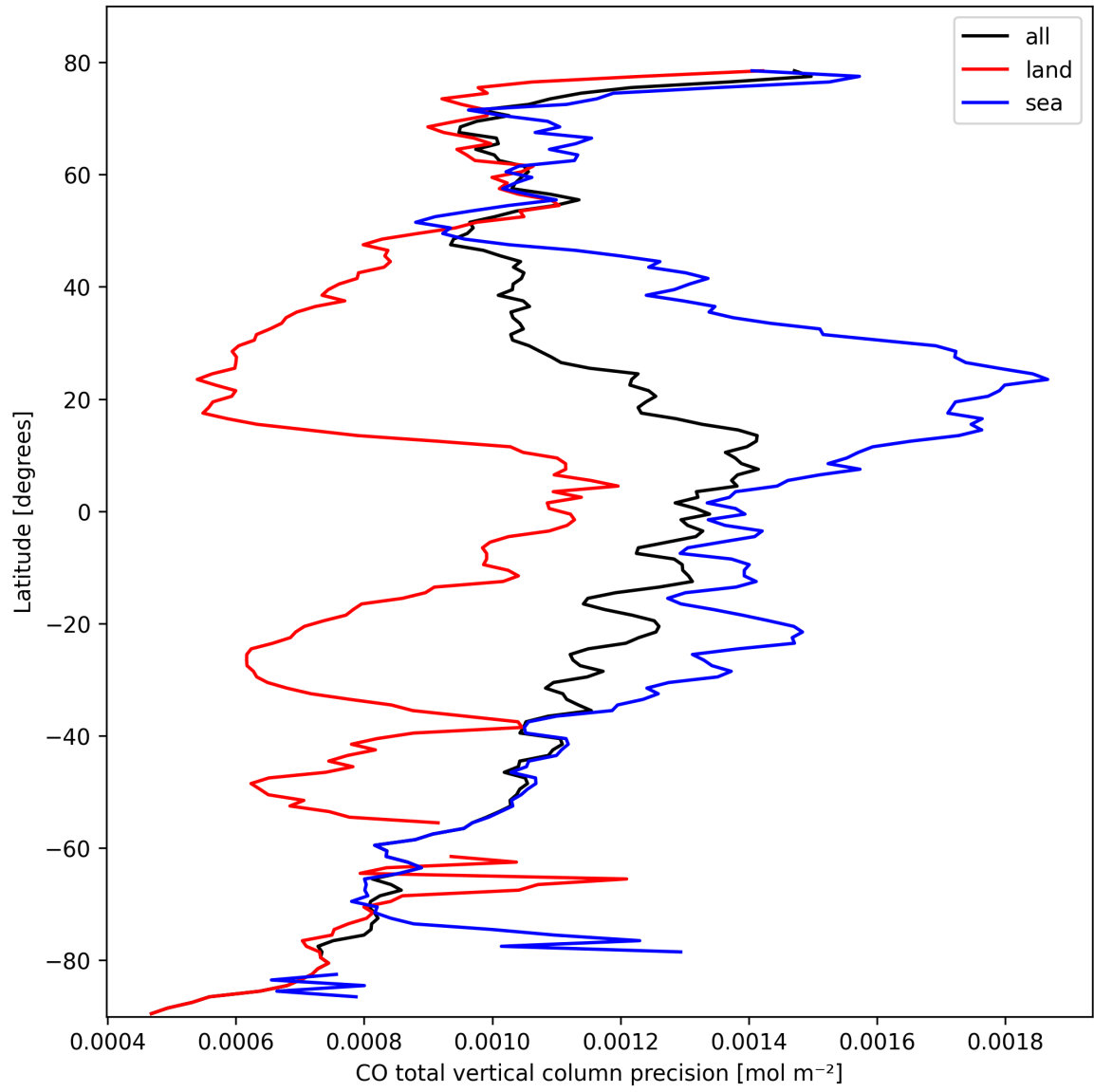
Figure 8: Zonal average of “CO total vertical column precision” for 2025-10-09 to 2025-10-09.
