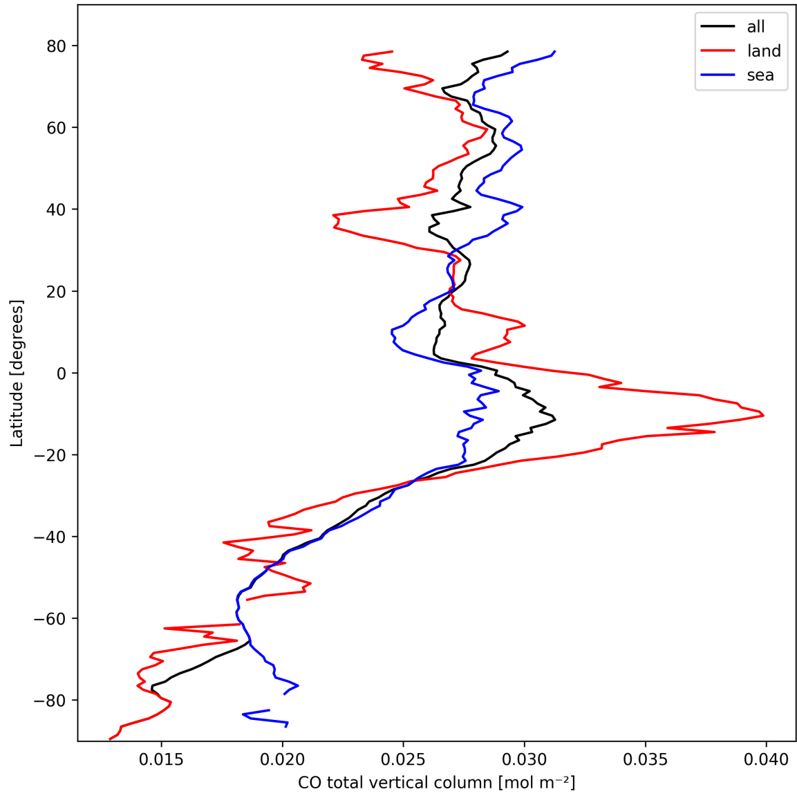
Figure 7: Zonal average of “CO total vertical column” for 2025-10-09 to 2025-10-09.
