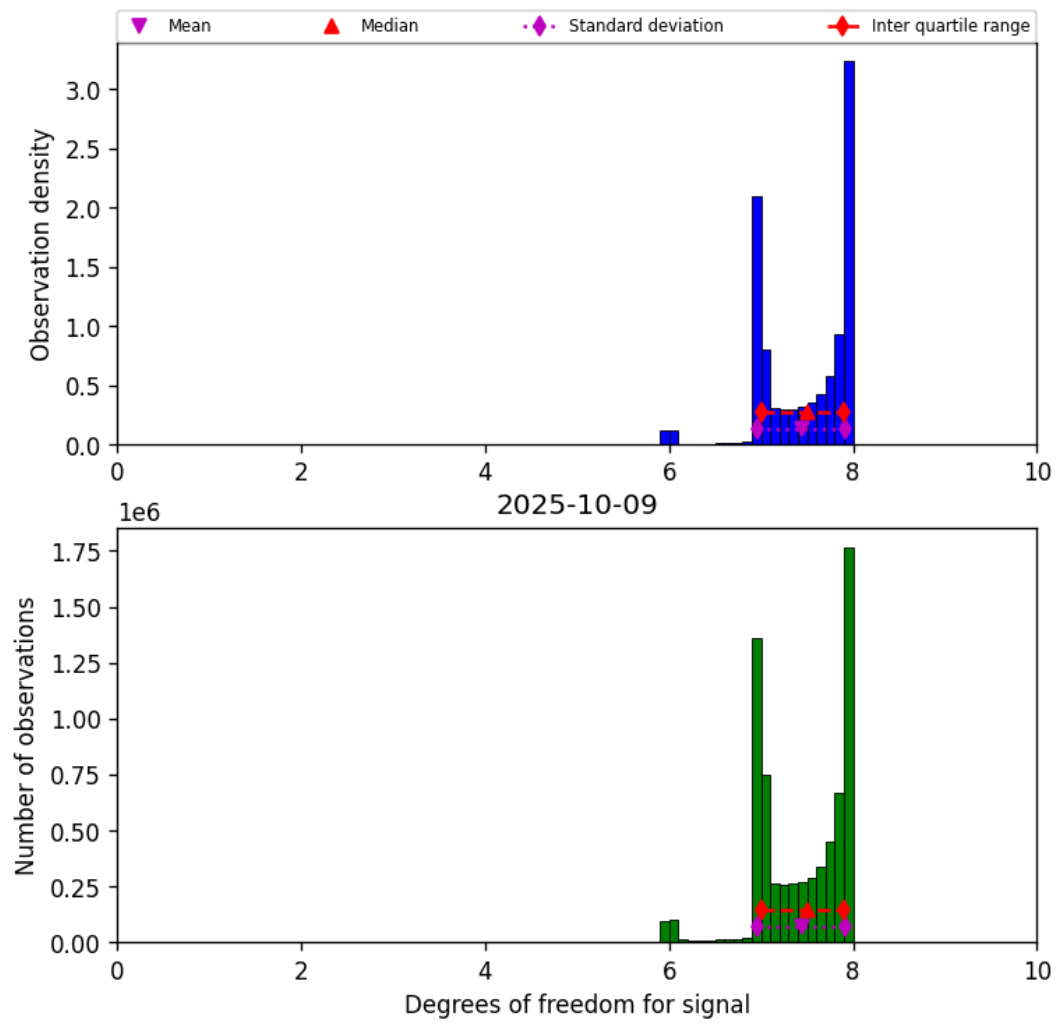
Figure 18: Histogram of “Degrees of freedom for signal” for 2025-10-09 to 2025-10-09
