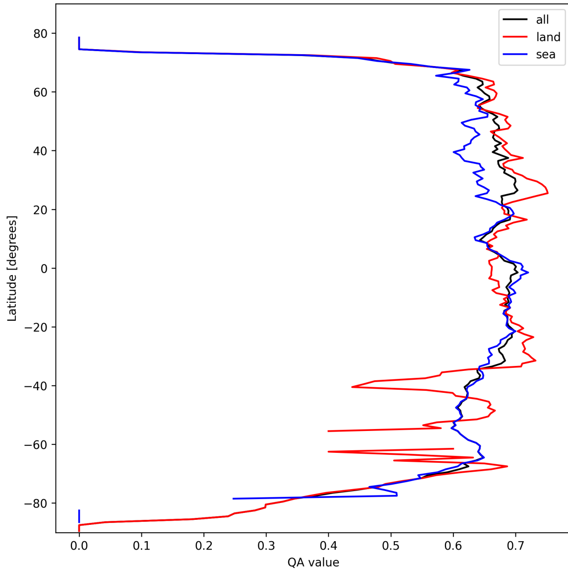
Figure 6: Zonal average of “QA value” for 2025-10-09 to 2025-10-09.
