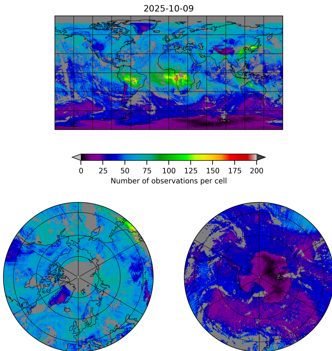
Figure 5: Map of the number of observations for 2025-10-09 to 2025-10-09
