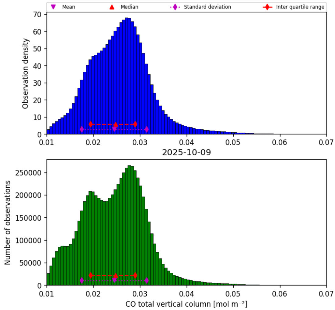
Figure 14: Histogram of “CO total vertical column” for 2025-10-09 to 2025-10-09
