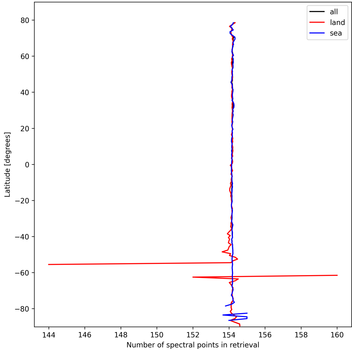
Figure 9: Zonal average of “Number of spectral points in retrieval” for 2025-10-09 to 2025-10-09.
