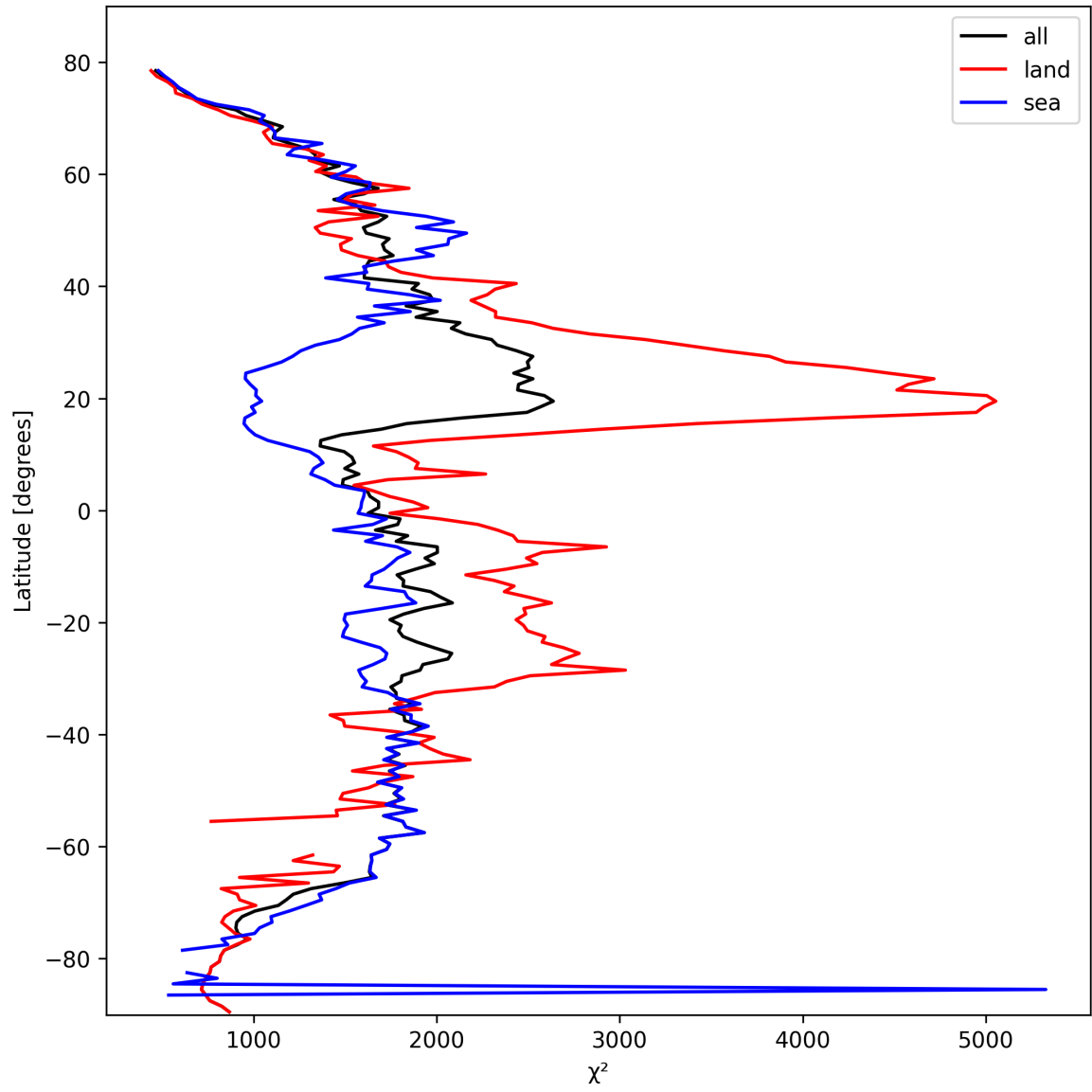
Figure 10: Zonal average of “ \chi^2 ” for 2025-10-09 to 2025-10-09.
