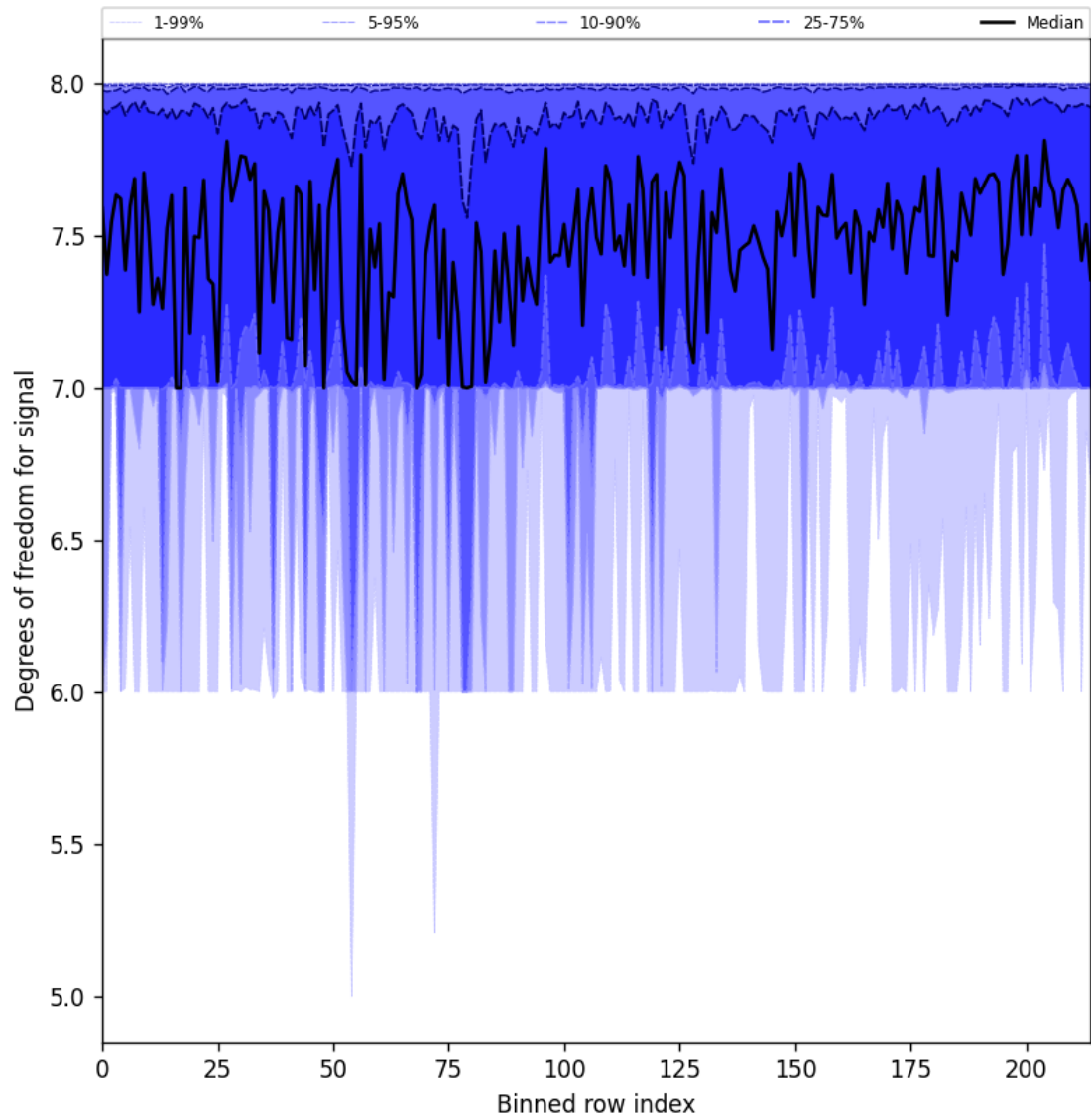
Figure 25: Along track statistics of “Degrees of freedom for signal” for 2025-10-09 to 2025-10-09
