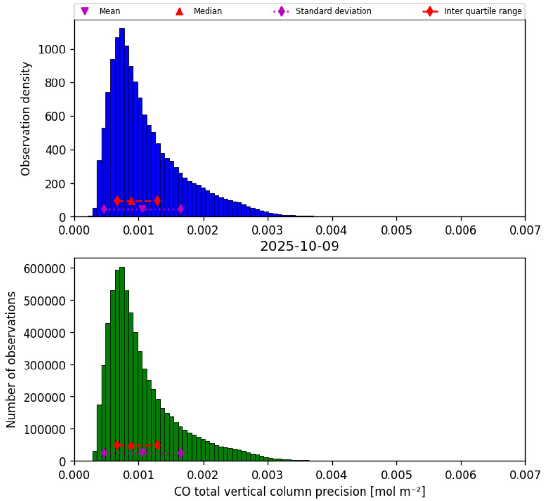
Figure 15: Histogram of “CO total vertical column precision” for 2025-10-09 to 2025-10-09
