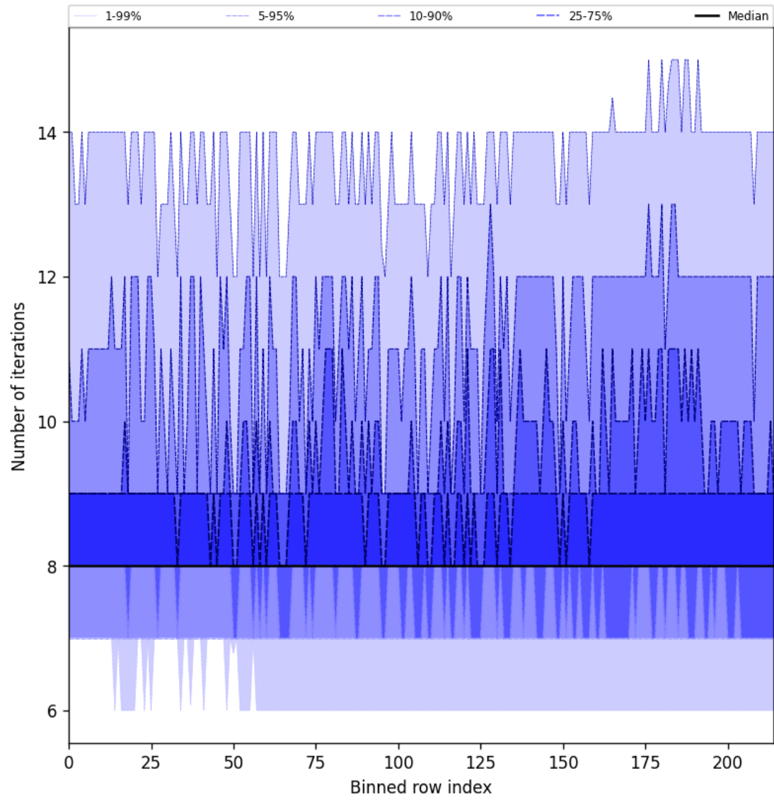
Figure 26: Along track statistics of “Number of iterations” for 2025-10-09 to 2025-10-09
