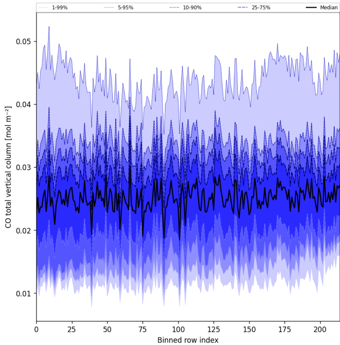
Figure 21: Along track statistics of “CO total vertical column” for 2025-10-09 to 2025-10-09
