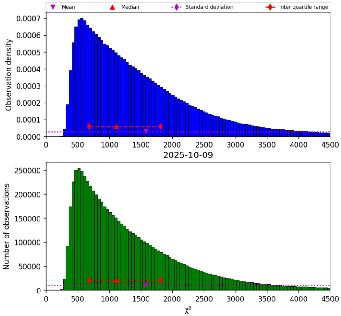
Figure 17: Histogram of " \chi^2 " for 2025-10-09 to 2025-10-09
