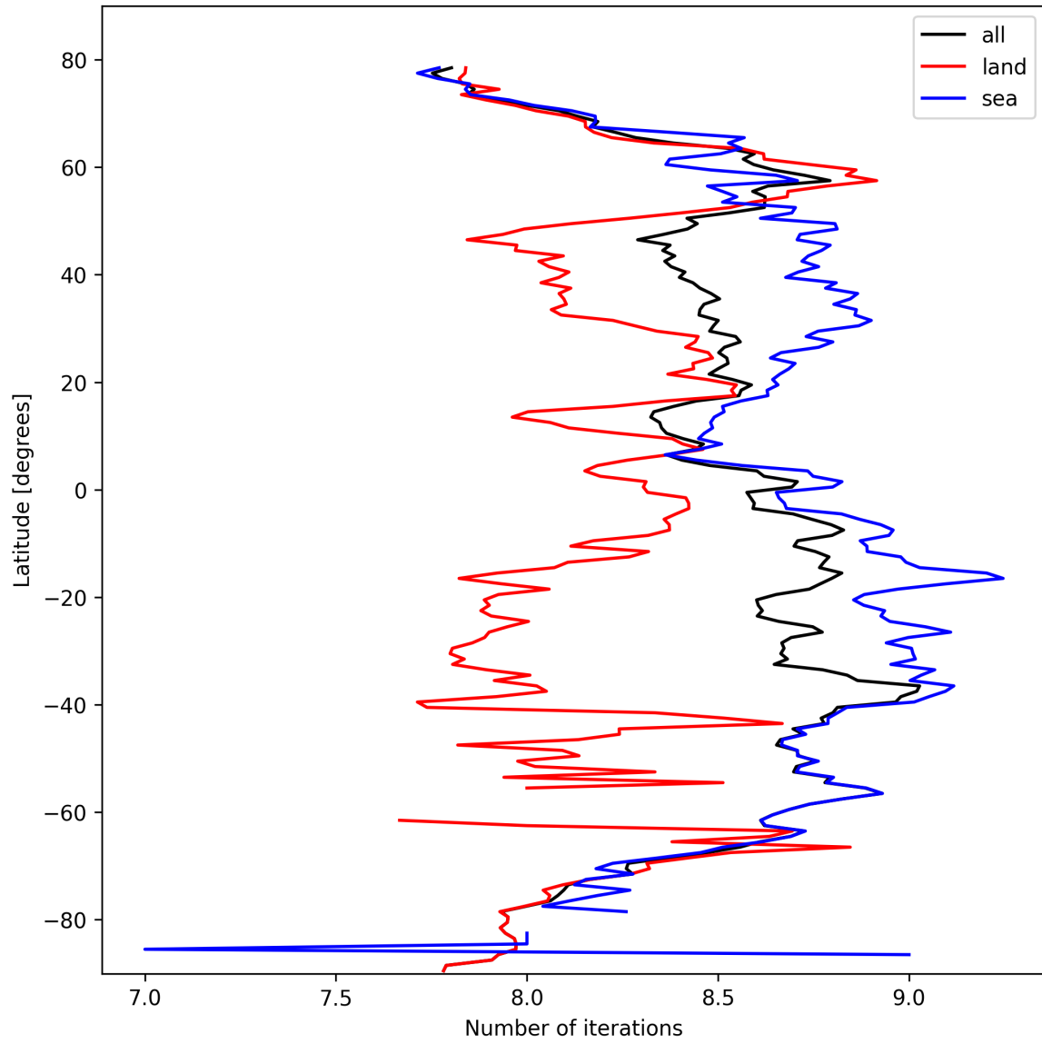
Figure 12: Zonal average of “Number of iterations” for 2025-10-09 to 2025-10-09.
