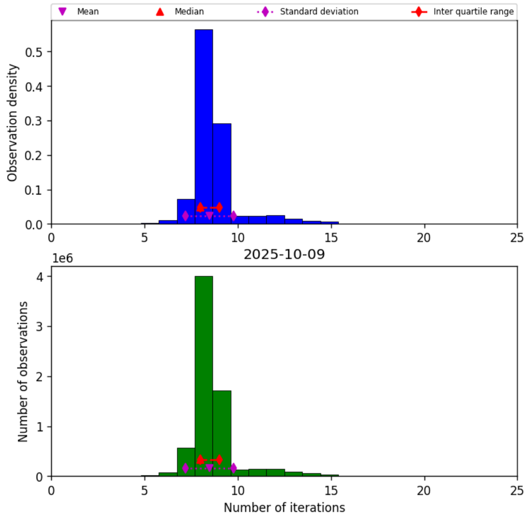
Figure 19: Histogram of “Number of iterations” for 2025-10-09 to 2025-10-09
