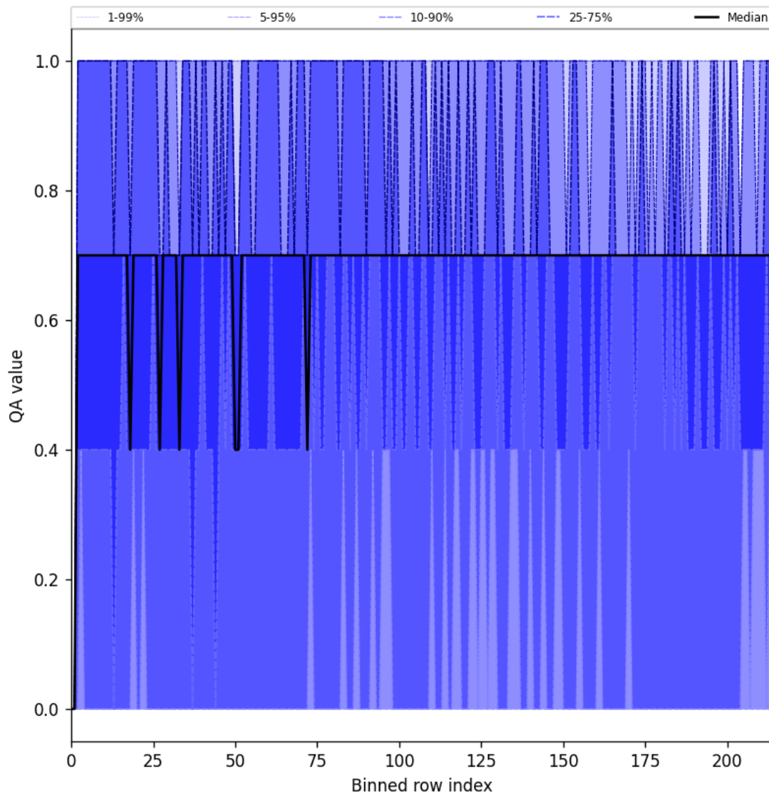
Figure 20: Along track statistics of “QA value” for 2025-10-09 to 2025-10-09
