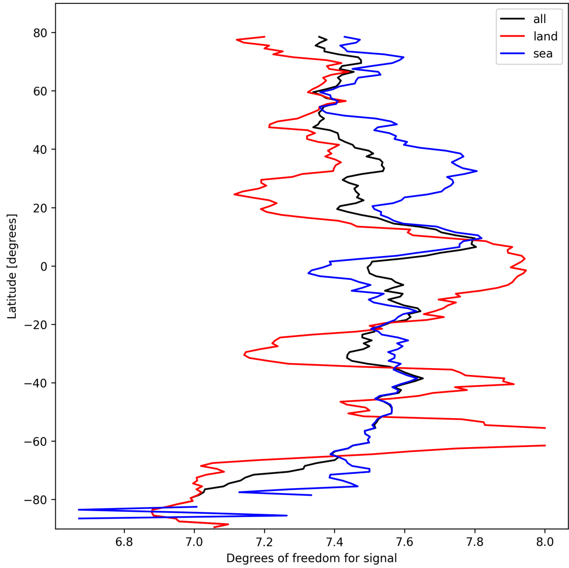
Figure 11: Zonal average of “Degrees of freedom for signal” for 2025-10-09 to 2025-10-09.
