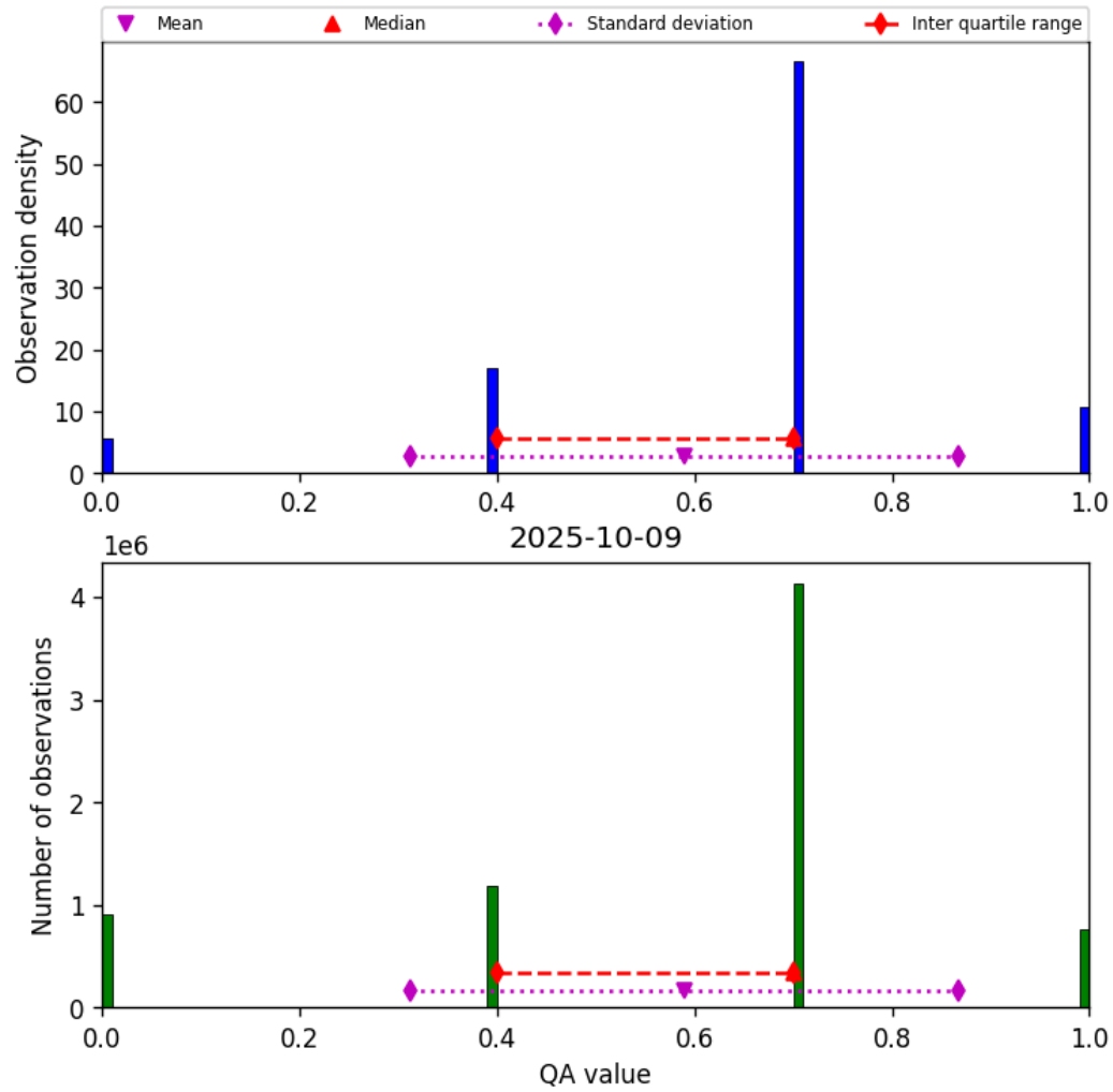
Figure 13: Histogram of “QA value” for 2025-10-09 to 2025-10-09
