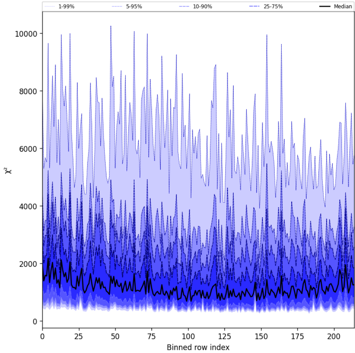
Figure 24: Along track statistics of “ \chi^2 ” for 2025-10-09 to 2025-10-09
