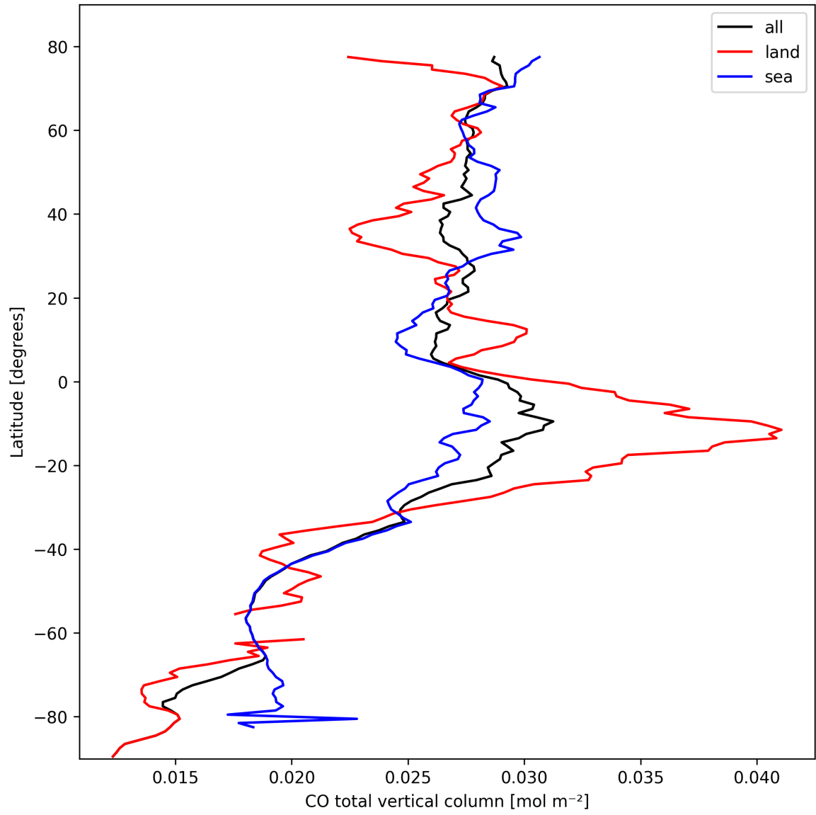
Figure 7: Zonal average of “CO total vertical column” for 2025-10-11 to 2025-10-12.
