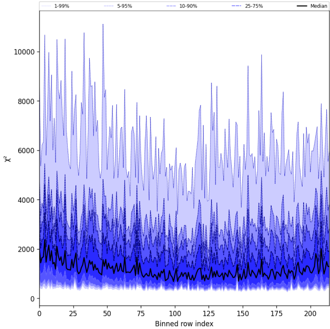
Figure 24: Along track statistics of “ \chi^2 ” for 2025-10-11 to 2025-10-12
