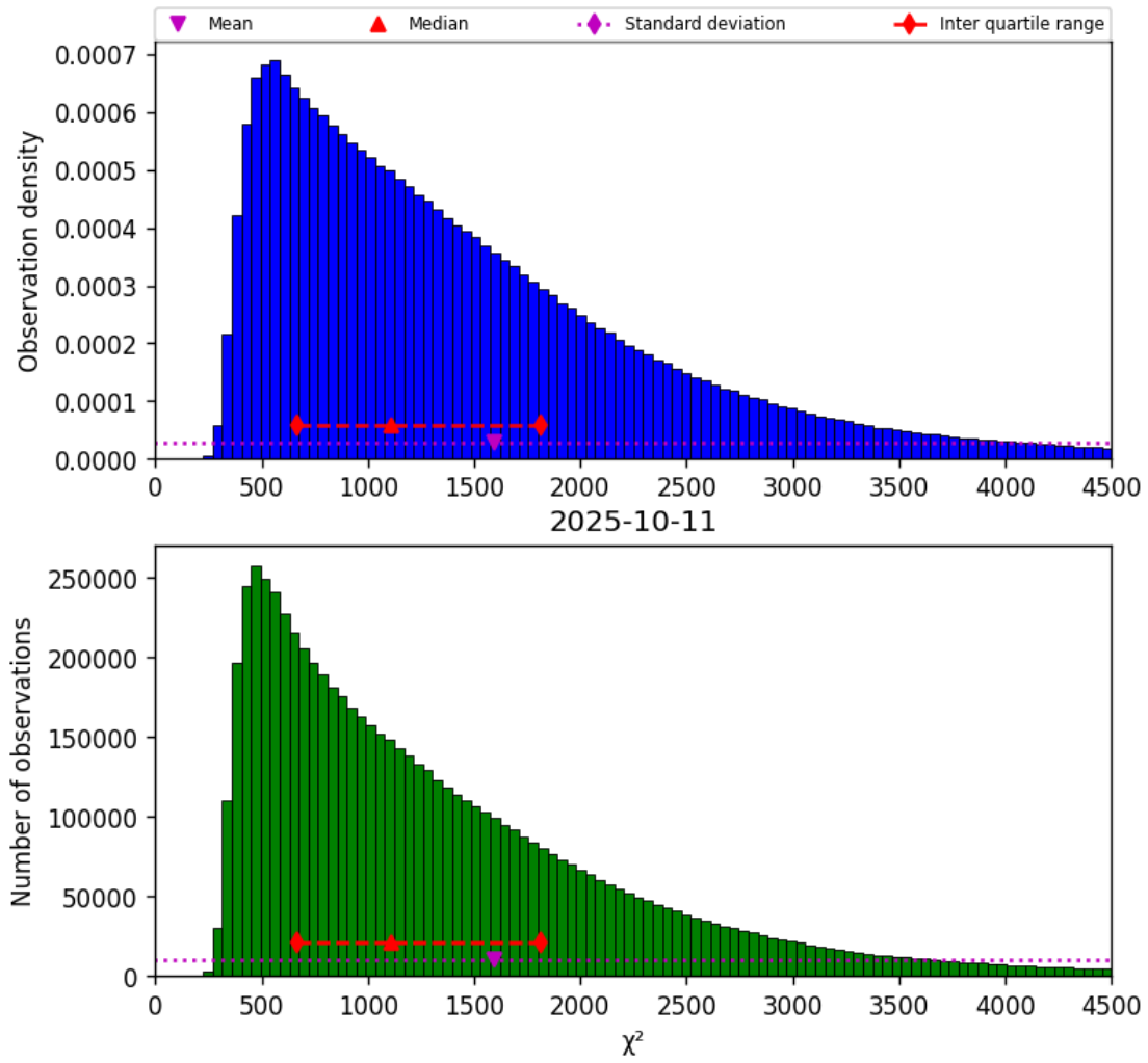
Figure 17: Histogram of “ \chi^2 ” for 2025-10-11 to 2025-10-12
