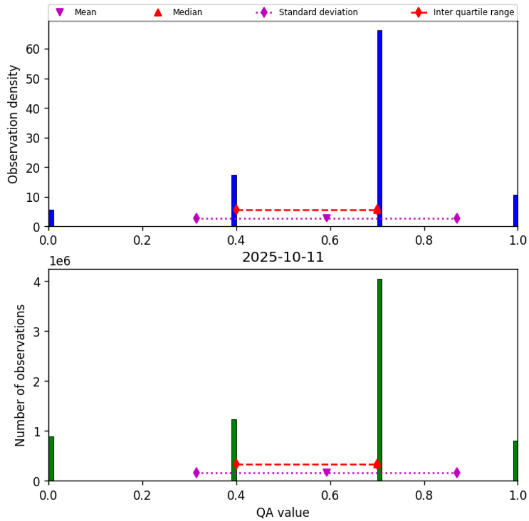
Figure 13: Histogram of “QA value” for 2025-10-11 to 2025-10-12
