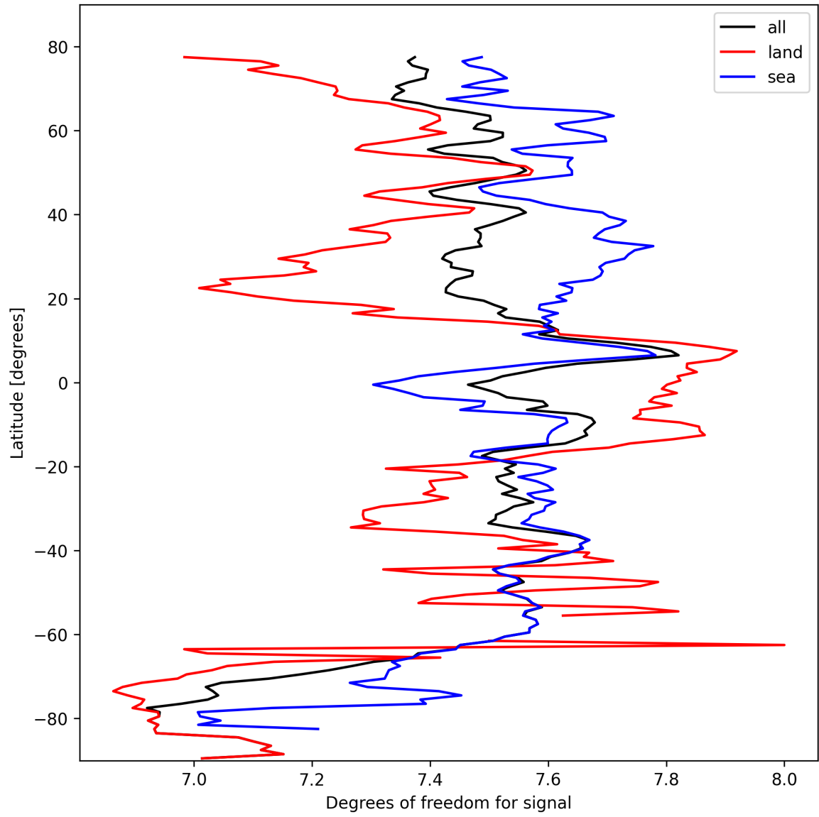
Figure 11: Zonal average of “Degrees of freedom for signal” for 2025-10-11 to 2025-10-12.
