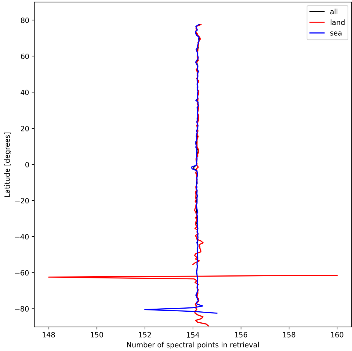
Figure 9: Zonal average of “Number of spectral points in retrieval” for 2025-10-11 to 2025-10-12.
