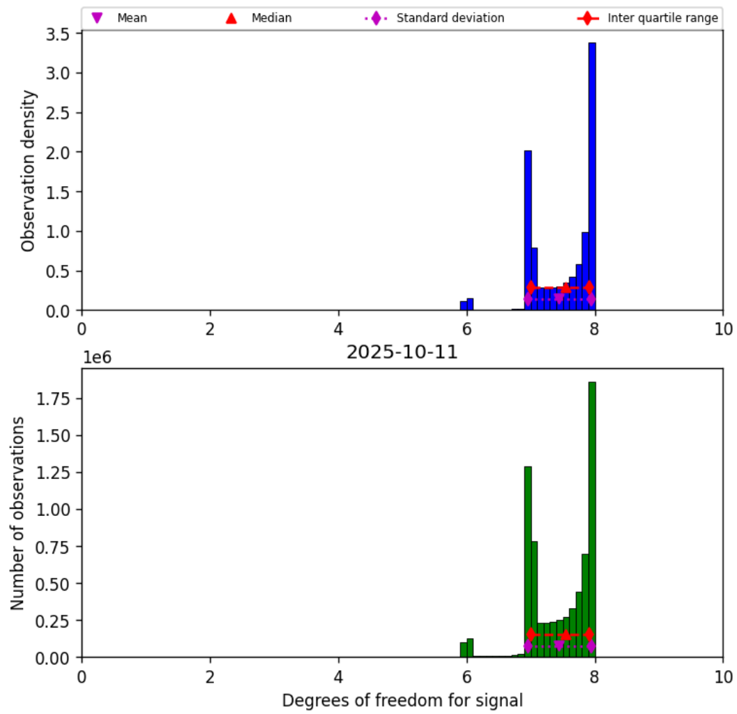
Figure 18: Histogram of “Degrees of freedom for signal” for 2025-10-11 to 2025-10-12
