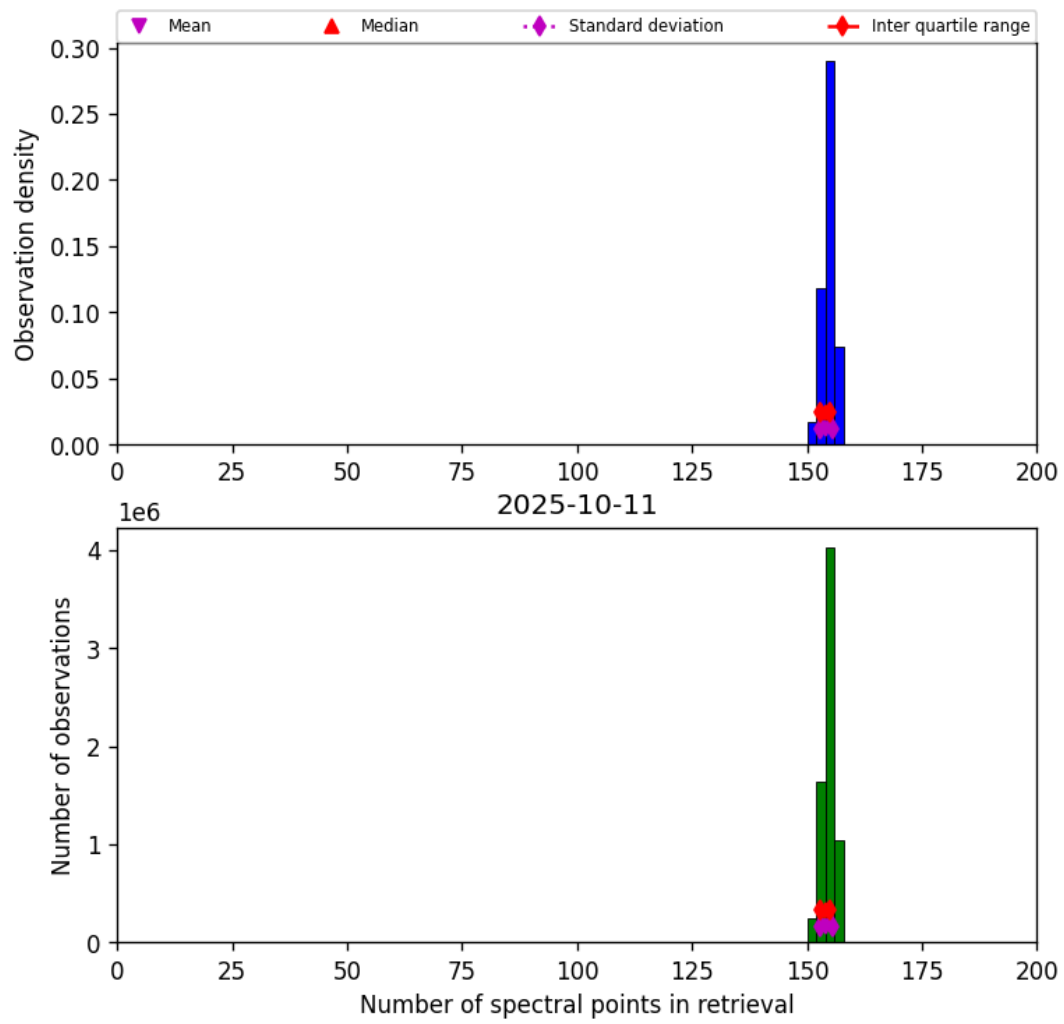
Figure 16: Histogram of “Number of spectral points in retrieval” for 2025-10-11 to 2025-10-12
