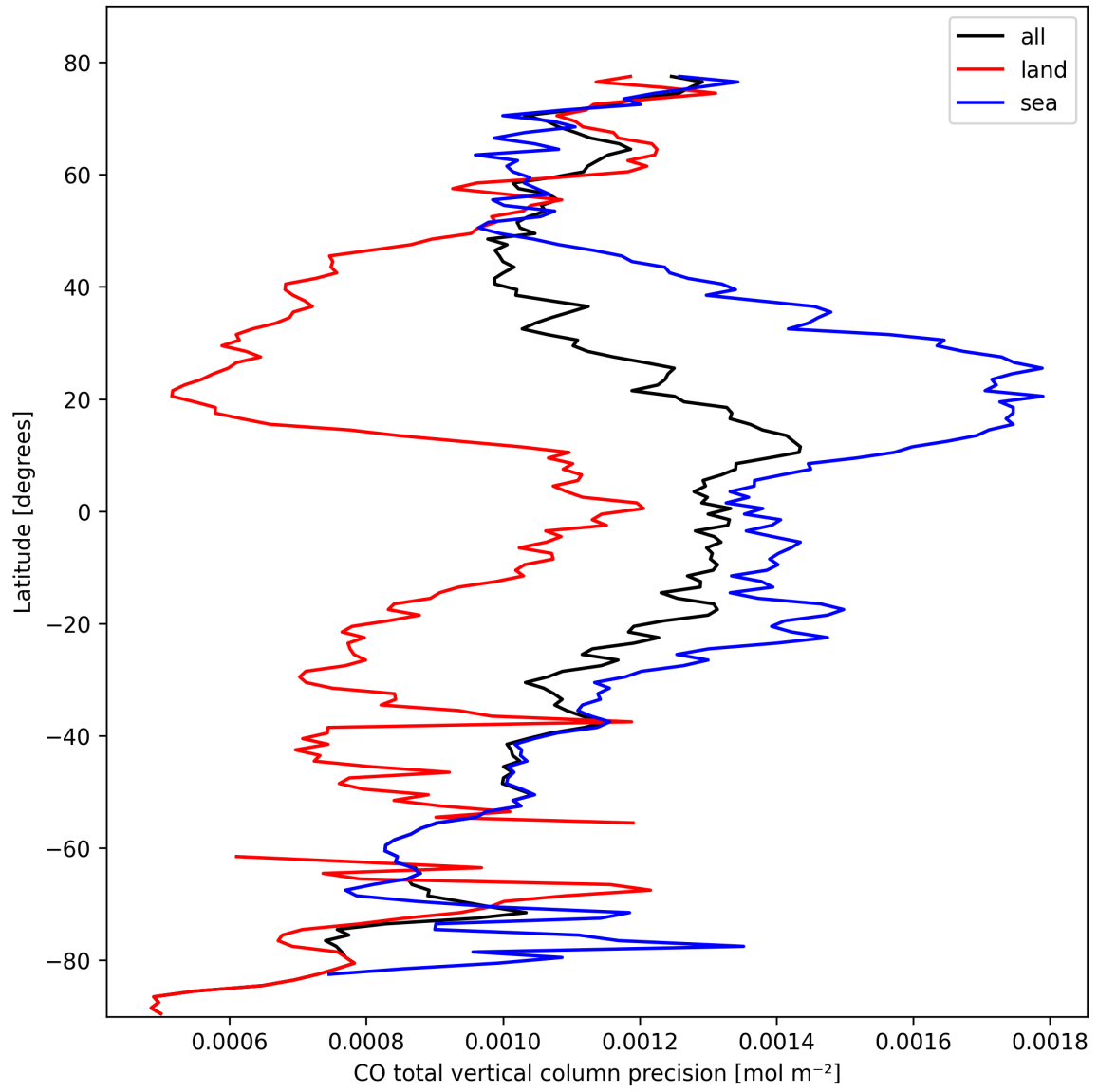
Figure 8: Zonal average of “CO total vertical column precision” for 2025-10-11 to 2025-10-12.
