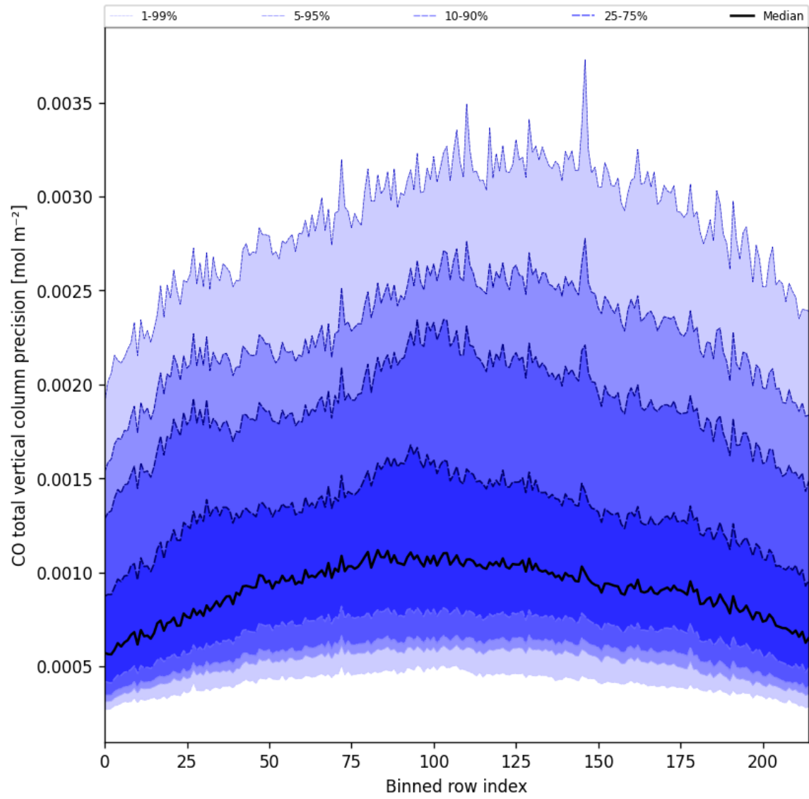
Figure 22: Along track statistics of “CO total vertical column precision” for 2025-10-11 to 2025-10-12
