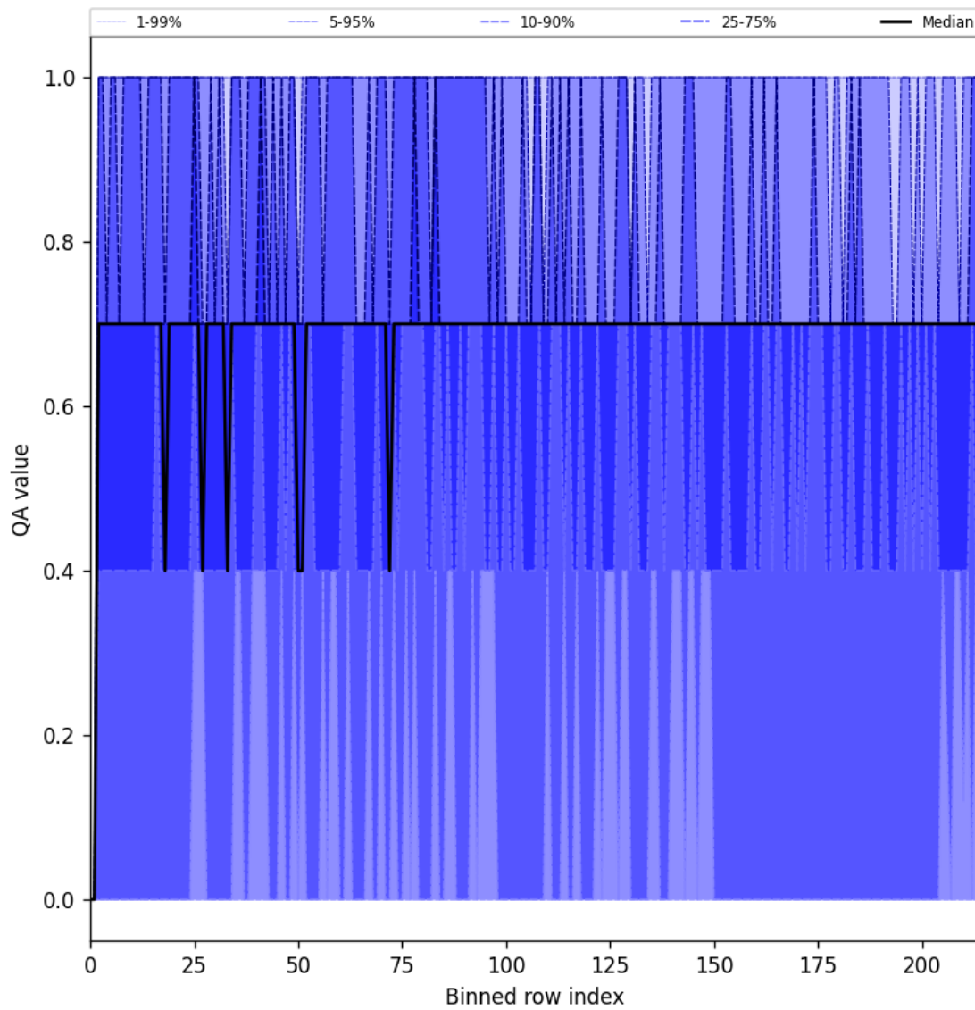
Figure 20: Along track statistics of “QA value” for 2025-10-11 to 2025-10-12
