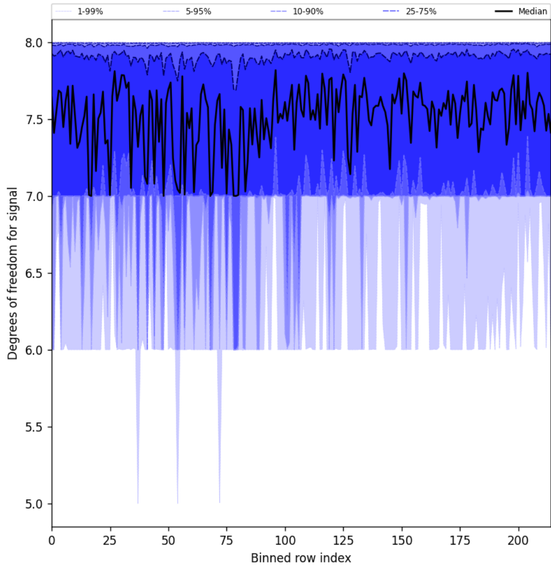
Figure 25: Along track statistics of “Degrees of freedom for signal” for 2025-10-11 to 2025-10-12
