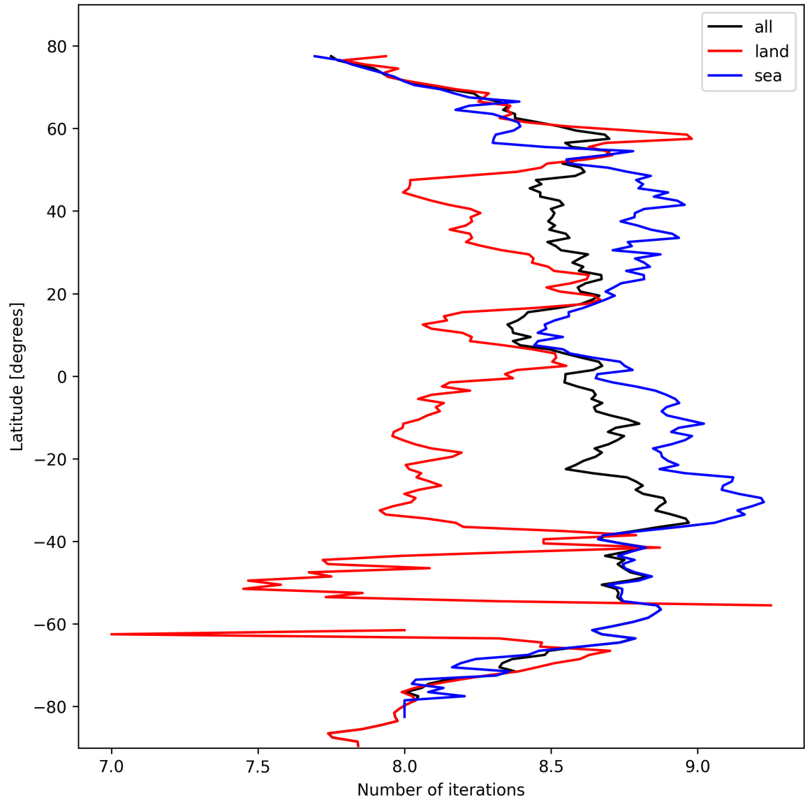
Figure 12: Zonal average of “Number of iterations” for 2025-10-11 to 2025-10-12.
