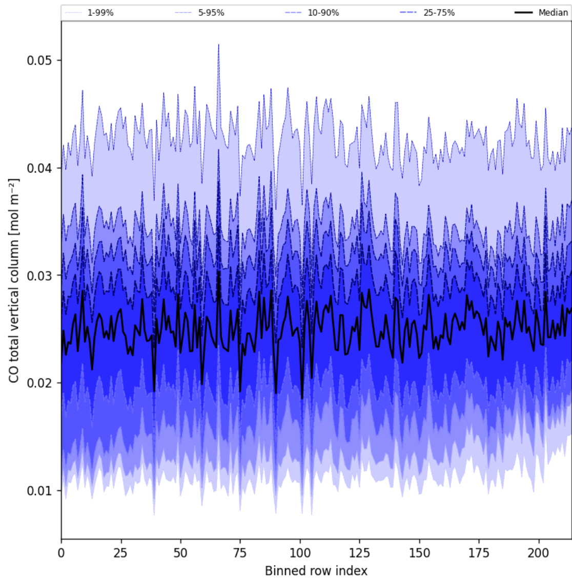
Figure 21: Along track statistics of “CO total vertical column” for 2025-10-11 to 2025-10-12
