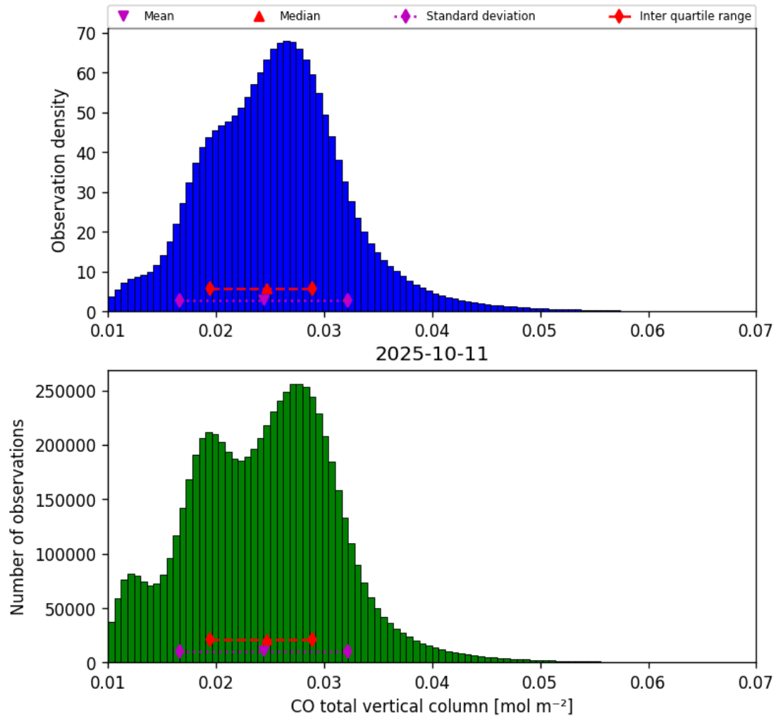
Figure 14: Histogram of “CO total vertical column” for 2025-10-11 to 2025-10-12
