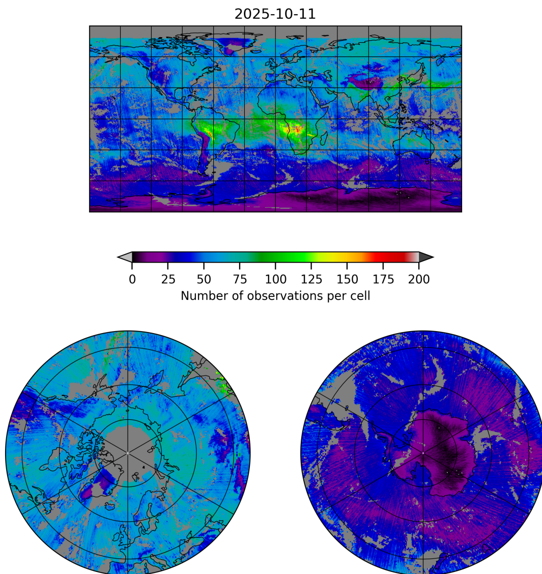
Figure 5: Map of the number of observations for 2025-10-11 to 2025-10-12
