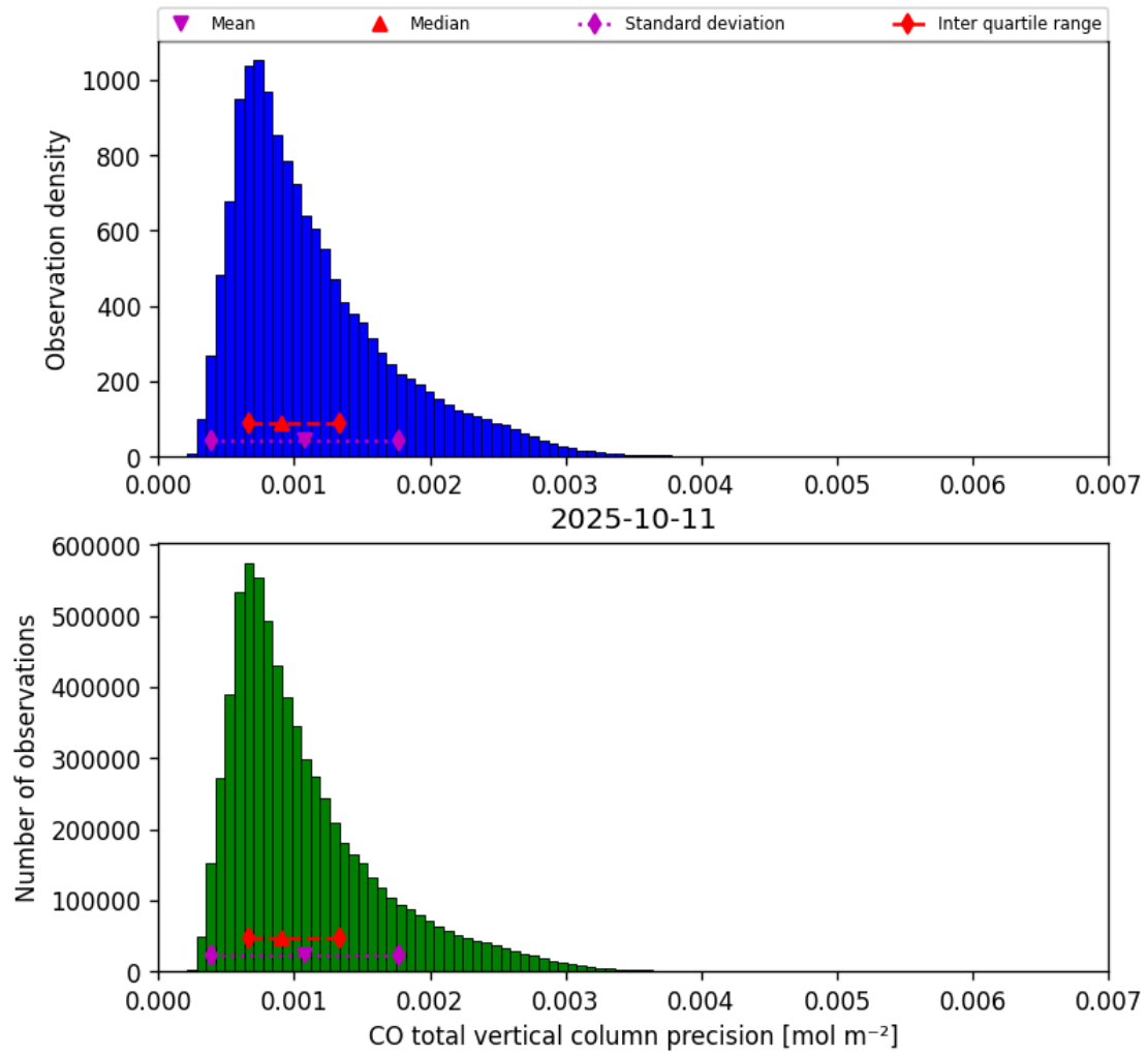
Figure 15: Histogram of “CO total vertical column precision” for 2025-10-11 to 2025-10-12
