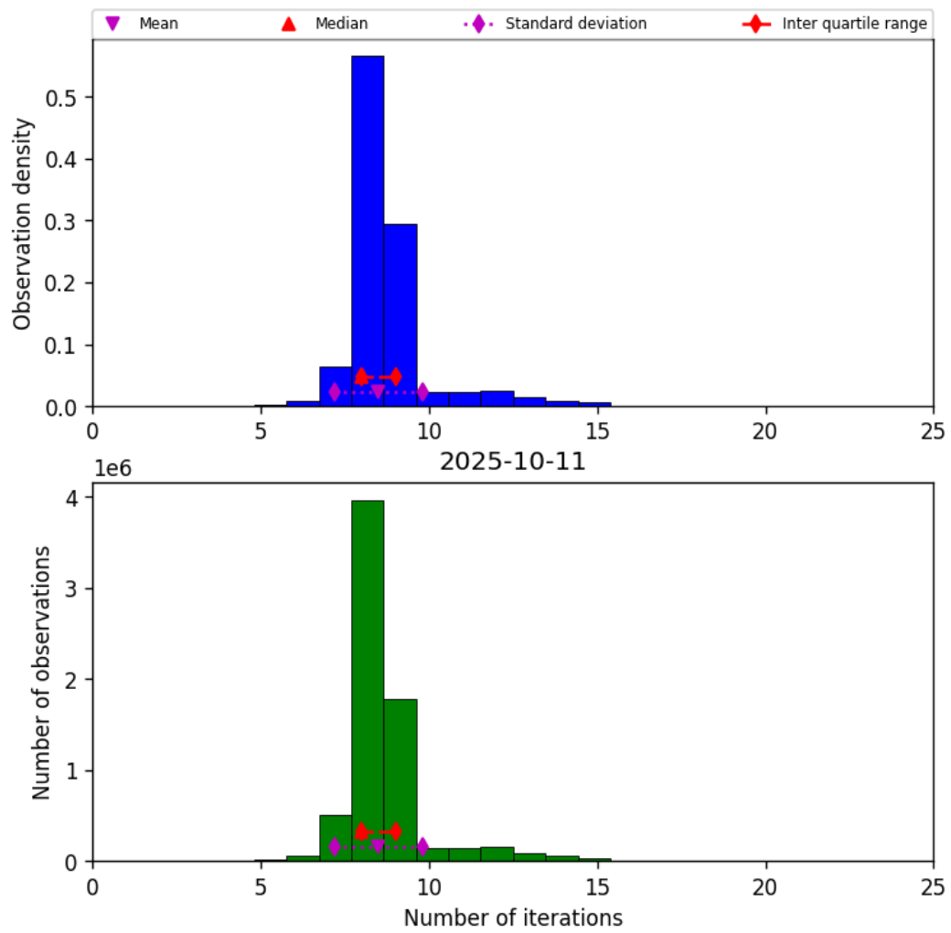
Figure 19: Histogram of “Number of iterations” for 2025-10-11 to 2025-10-12
