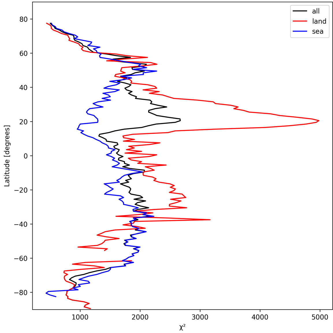
Figure 10: Zonal average of “ \chi^2 ” for 2025-10-11 to 2025-10-12.
