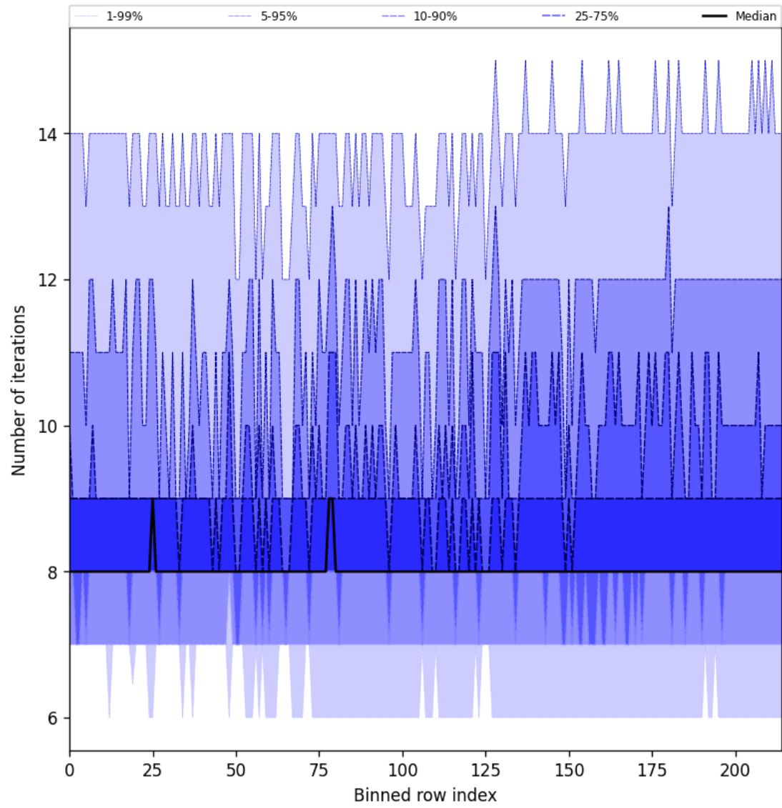
Figure 26: Along track statistics of “Number of iterations” for 2025-10-11 to 2025-10-12
