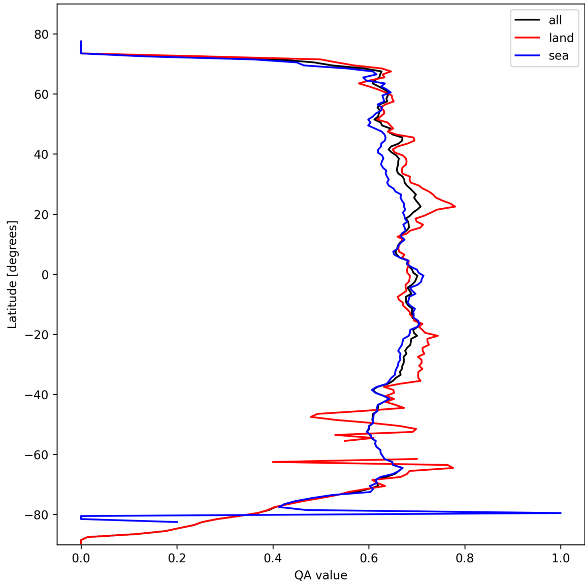
Figure 6: Zonal average of “QA value” for 2025-10-11 to 2025-10-12.
