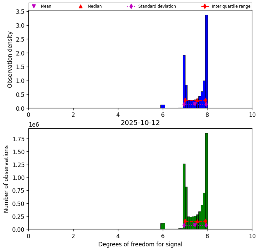
Figure 18: Histogram of “Degrees of freedom for signal” for 2025-10-12 to 2025-10-13
