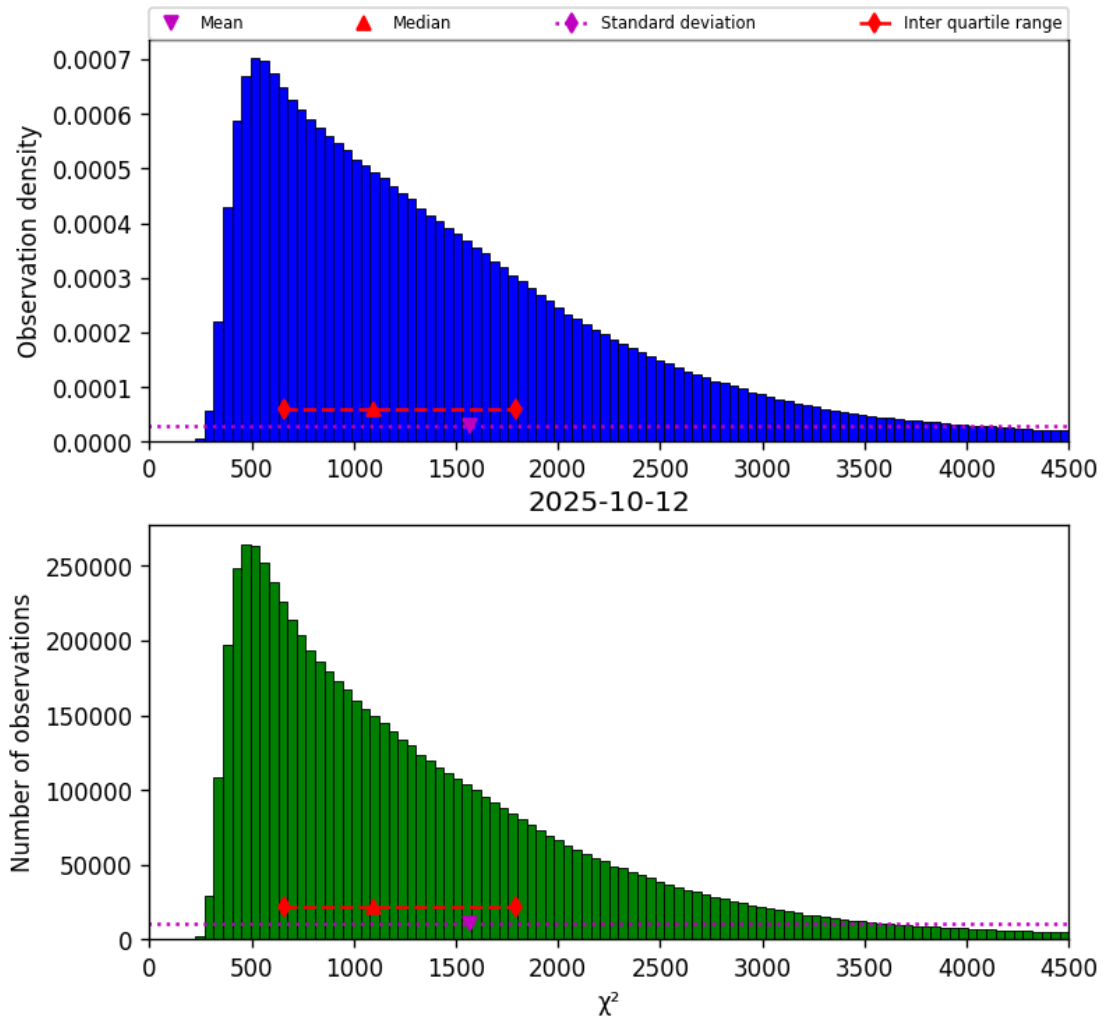
Figure 17: Histogram of “ \chi^2 ” for 2025-10-12 to 2025-10-13
