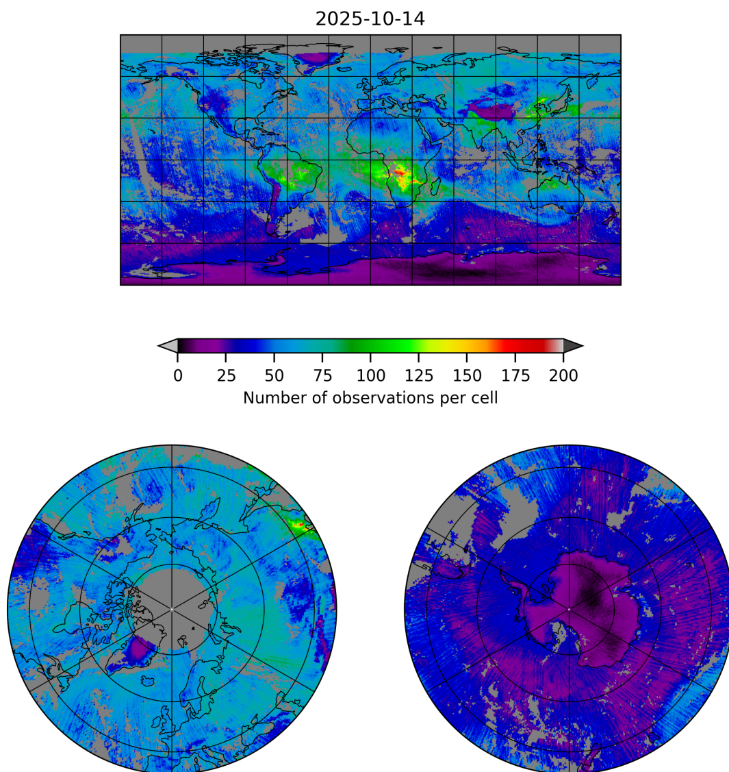
Figure 5: Map of the number of observations for 2025-10-14 to 2025-10-15
