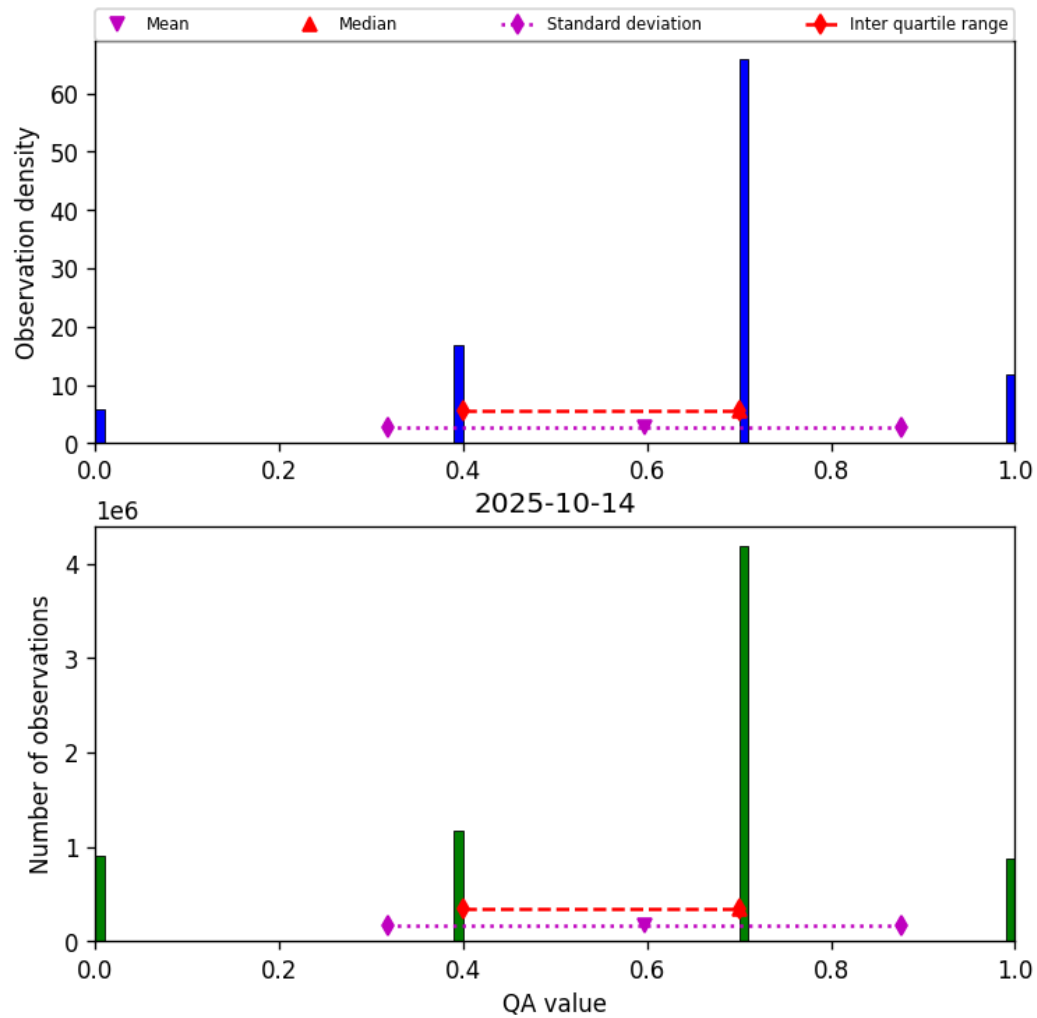
Figure 13: Histogram of “QA value” for 2025-10-14 to 2025-10-15
