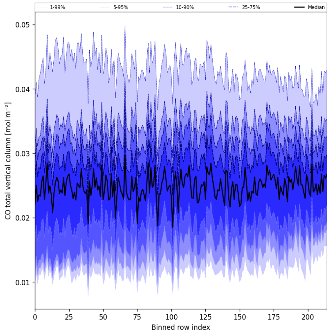
Figure 21: Along track statistics of “CO total vertical column” for 2025-10-14 to 2025-10-15
