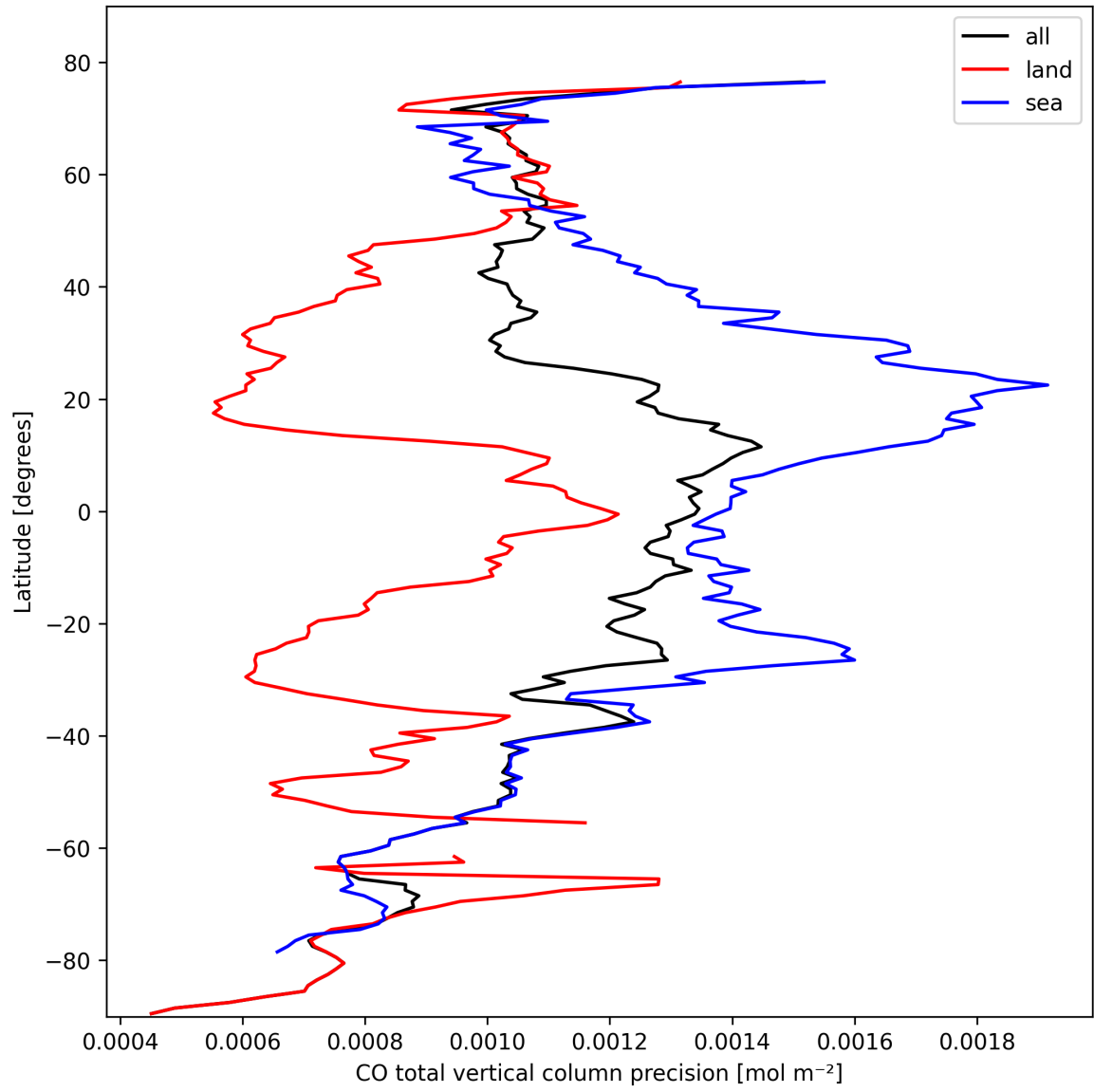
Figure 8: Zonal average of “CO total vertical column precision” for 2025-10-14 to 2025-10-15.
