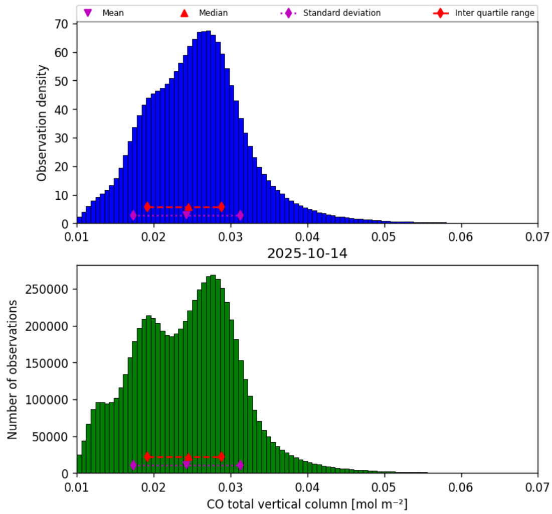
Figure 14: Histogram of “CO total vertical column” for 2025-10-14 to 2025-10-15
