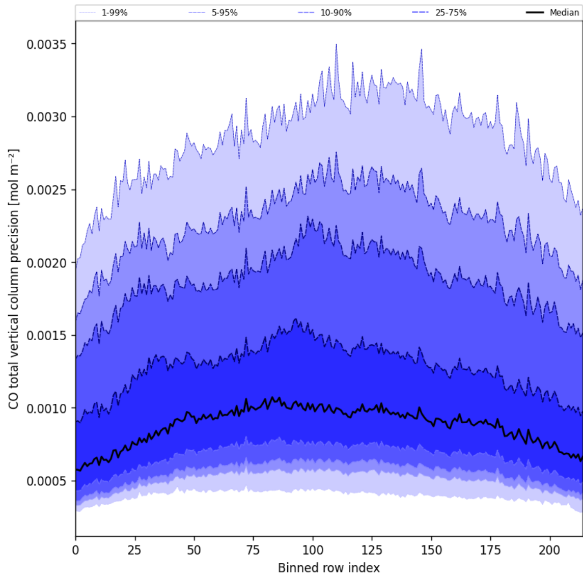
Figure 22: Along track statistics of “CO total vertical column precision” for 2025-10-14 to 2025-10-15
