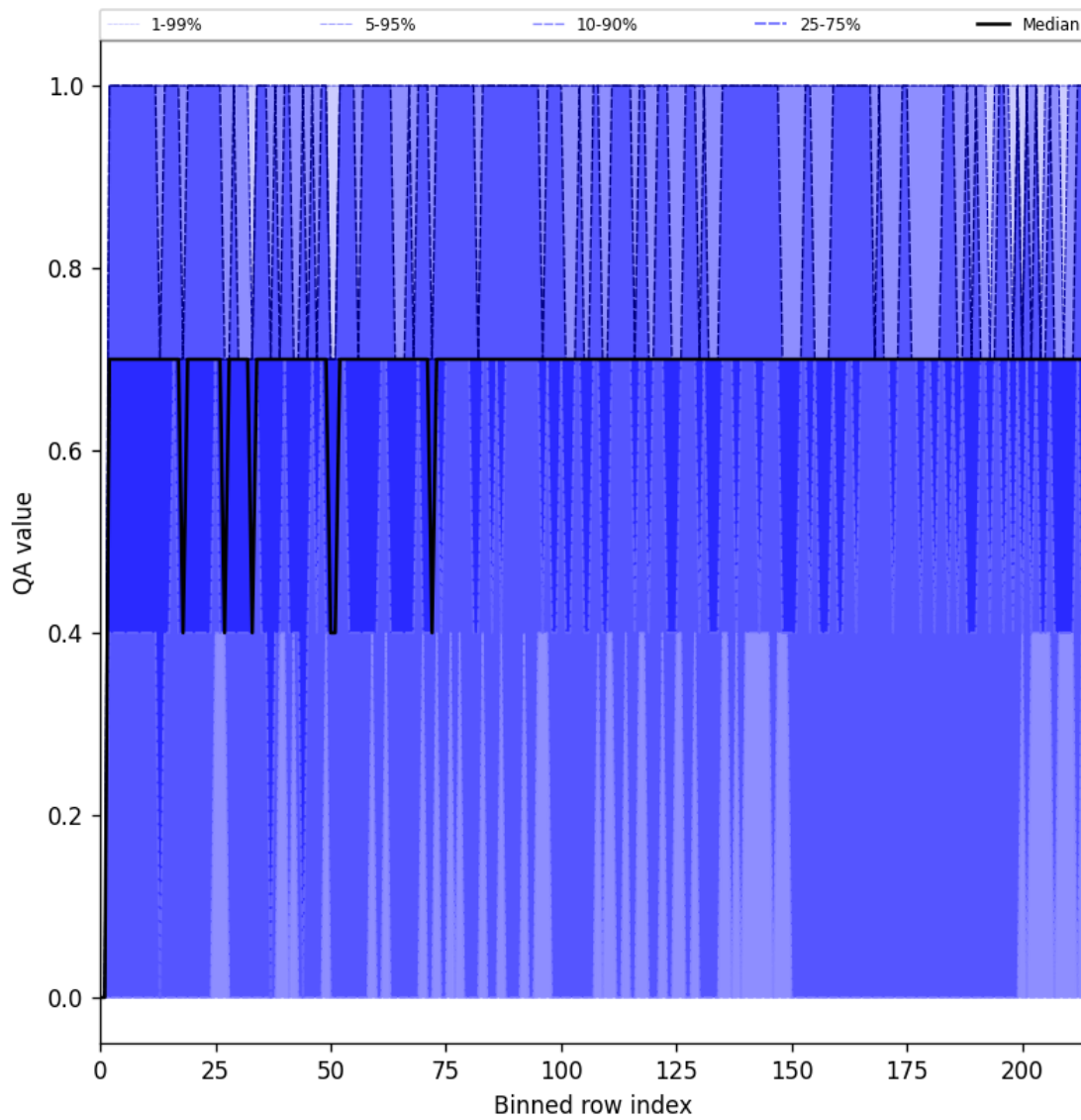
Figure 20: Along track statistics of “QA value” for 2025-10-14 to 2025-10-15
