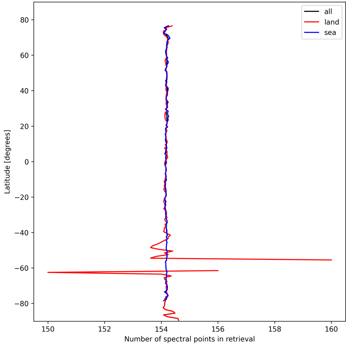
Figure 9: Zonal average of “Number of spectral points in retrieval” for 2025-10-14 to 2025-10-15.
