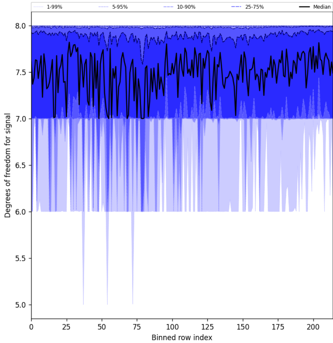
Figure 25: Along track statistics of “Degrees of freedom for signal” for 2025-10-14 to 2025-10-15
