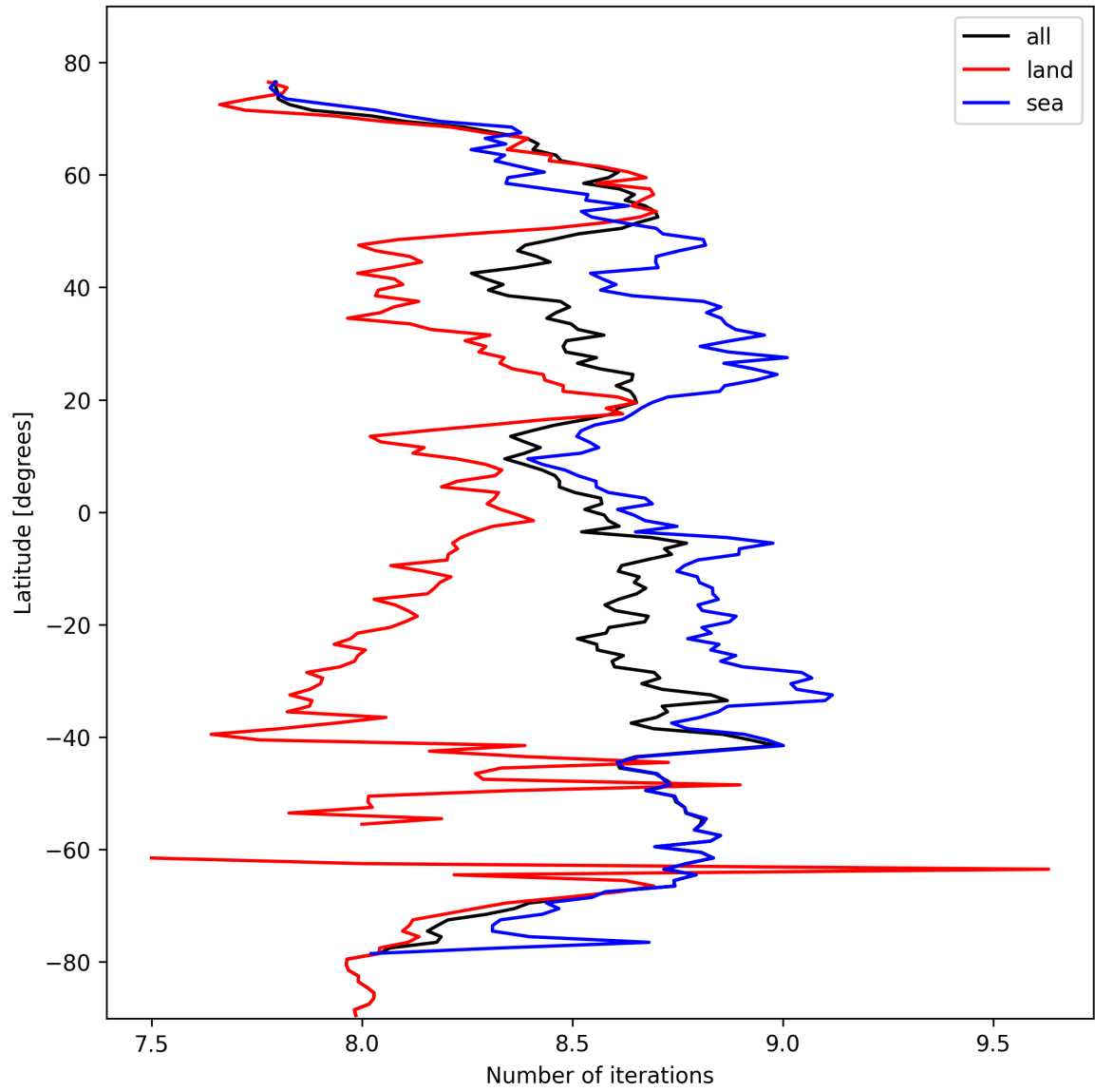
Figure 12: Zonal average of “Number of iterations” for 2025-10-14 to 2025-10-15.
