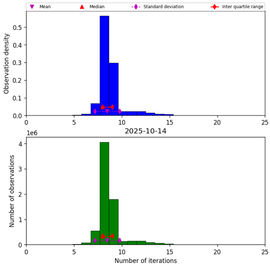
Figure 19: Histogram of “Number of iterations” for 2025-10-14 to 2025-10-15
