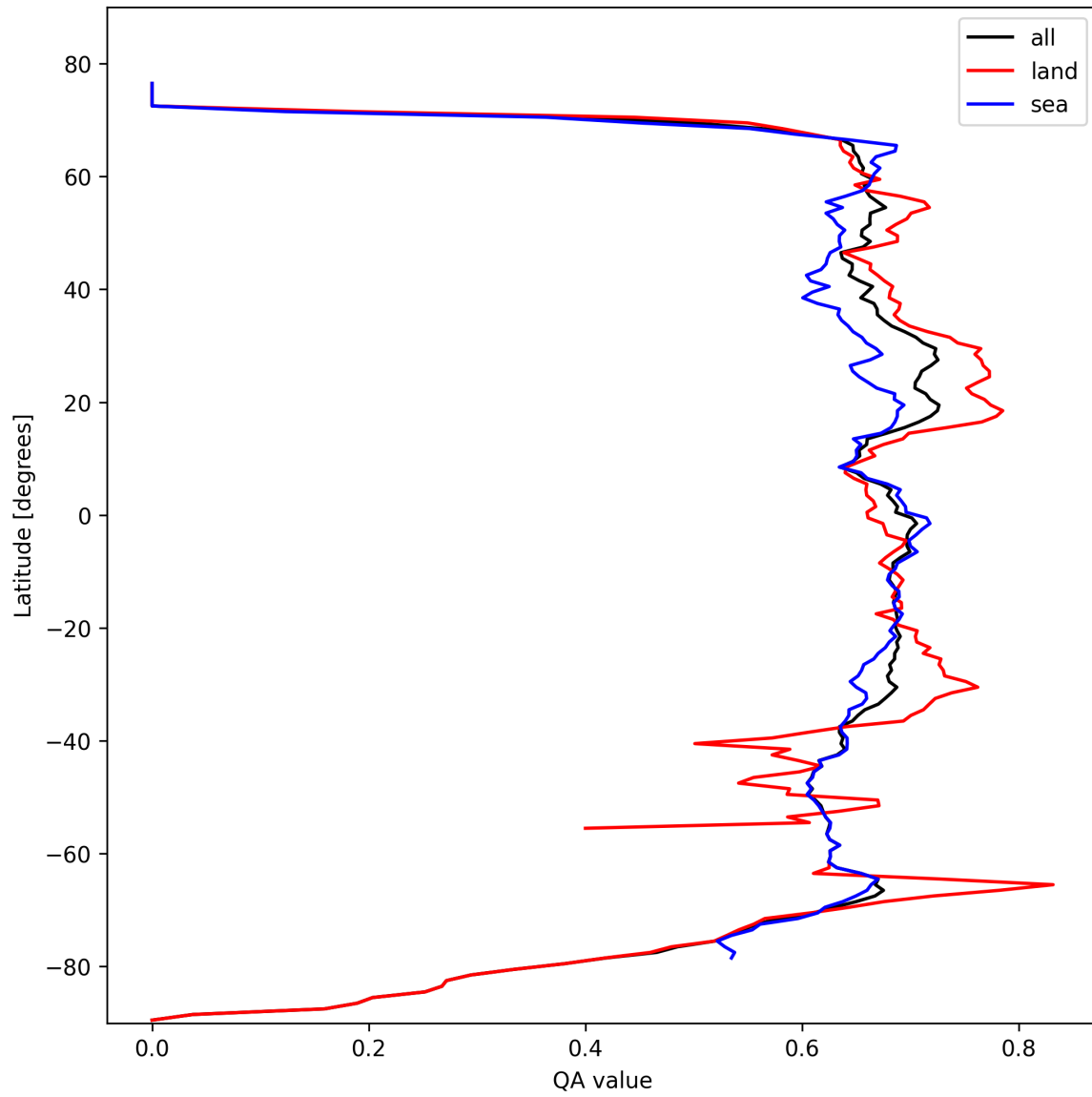
Figure 6: Zonal average of “QA value” for 2025-10-14 to 2025-10-15.
