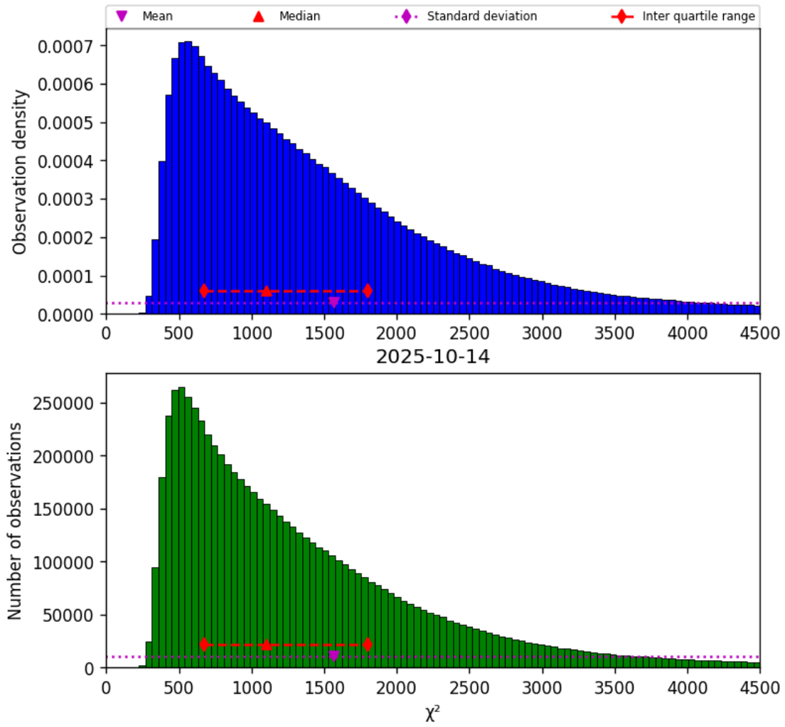
Figure 17: Histogram of “ \chi^2 ” for 2025-10-14 to 2025-10-15
