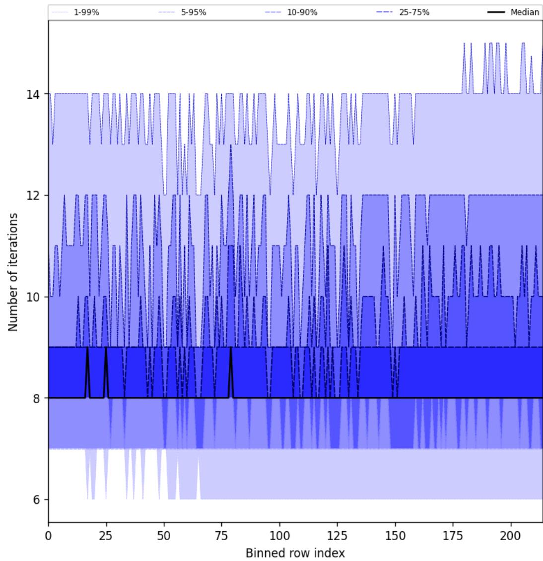
Figure 26: Along track statistics of “Number of iterations” for 2025-10-14 to 2025-10-15
