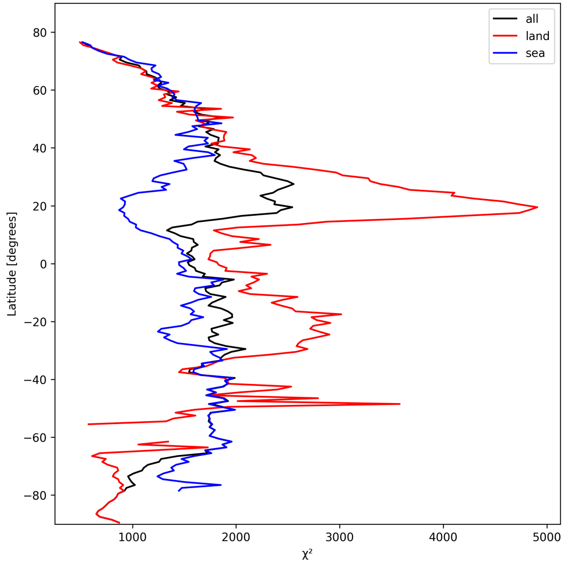
Figure 10: Zonal average of “ \chi^2 ” for 2025-10-14 to 2025-10-15.
