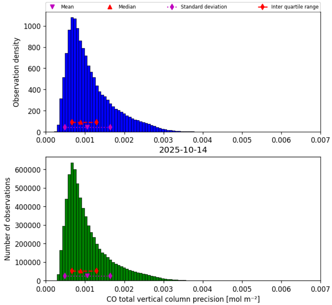
Figure 15: Histogram of “CO total vertical column precision” for 2025-10-14 to 2025-10-15
