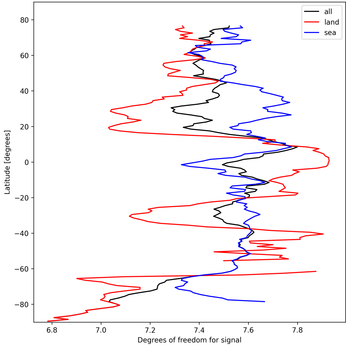
Figure 11: Zonal average of “Degrees of freedom for signal” for 2025-10-14 to 2025-10-15.
