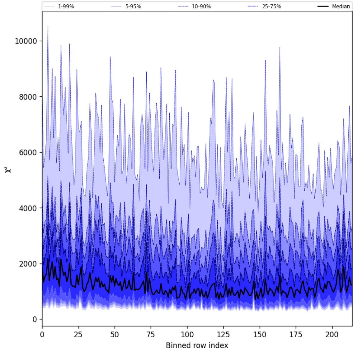
Figure 24: Along track statistics of “ \chi^2 ” for 2025-10-14 to 2025-10-15
