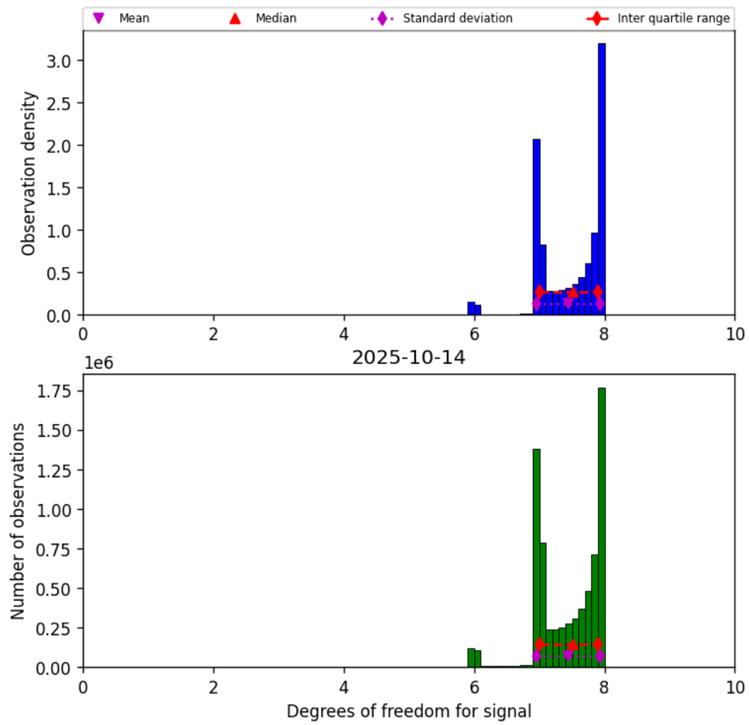
Figure 18: Histogram of “Degrees of freedom for signal” for 2025-10-14 to 2025-10-15
