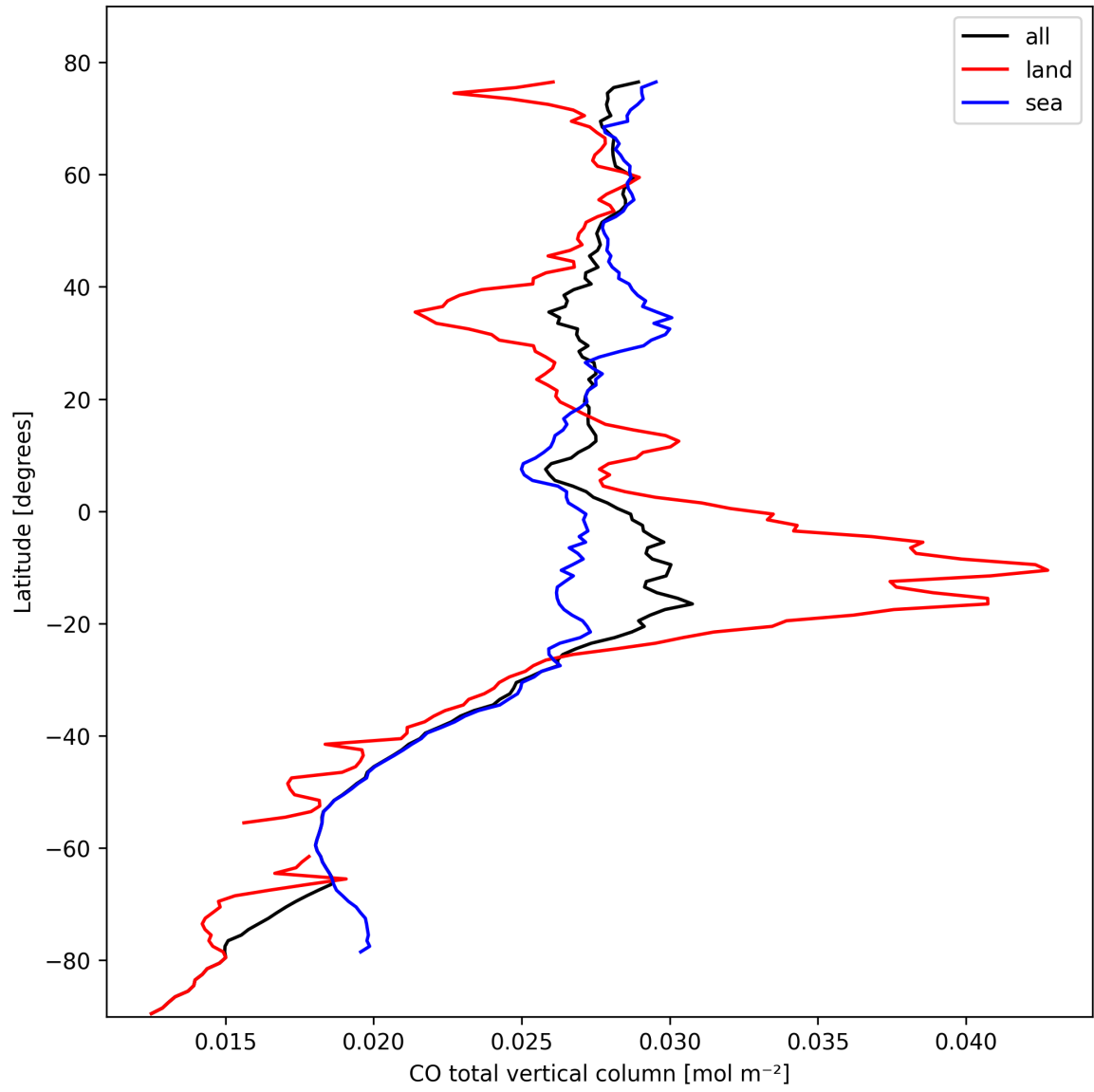
Figure 7: Zonal average of “CO total vertical column” for 2025-10-14 to 2025-10-15.
