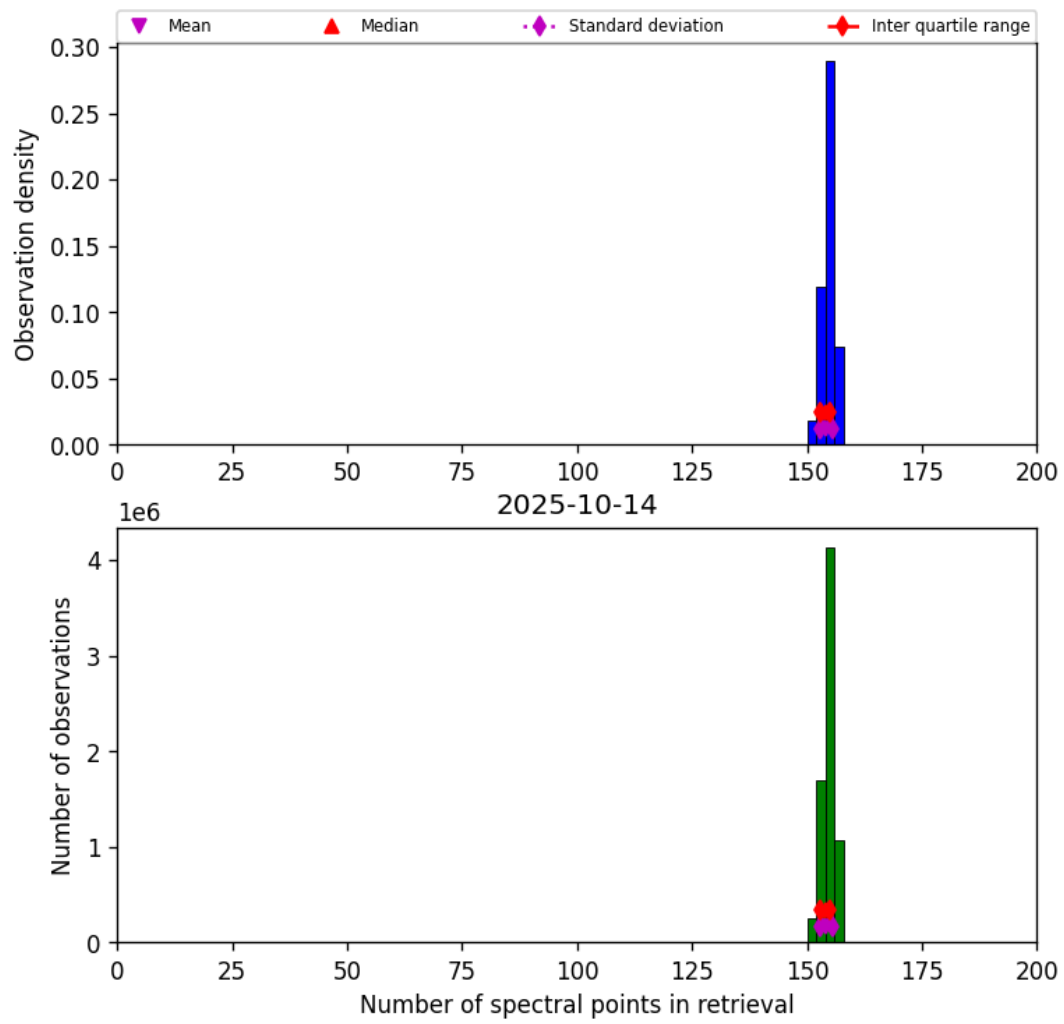
Figure 16: Histogram of “Number of spectral points in retrieval” for 2025-10-14 to 2025-10-15
