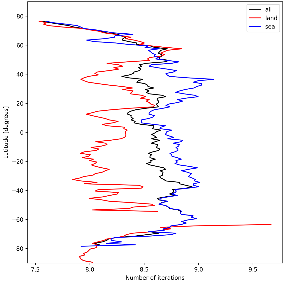
Figure 12: Zonal average of “Number of iterations” for 2025-10-15 to 2025-10-15.
