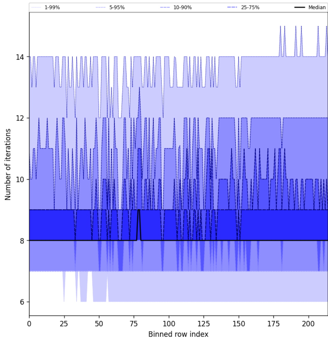
Figure 26: Along track statistics of “Number of iterations” for 2025-10-15 to 2025-10-15
