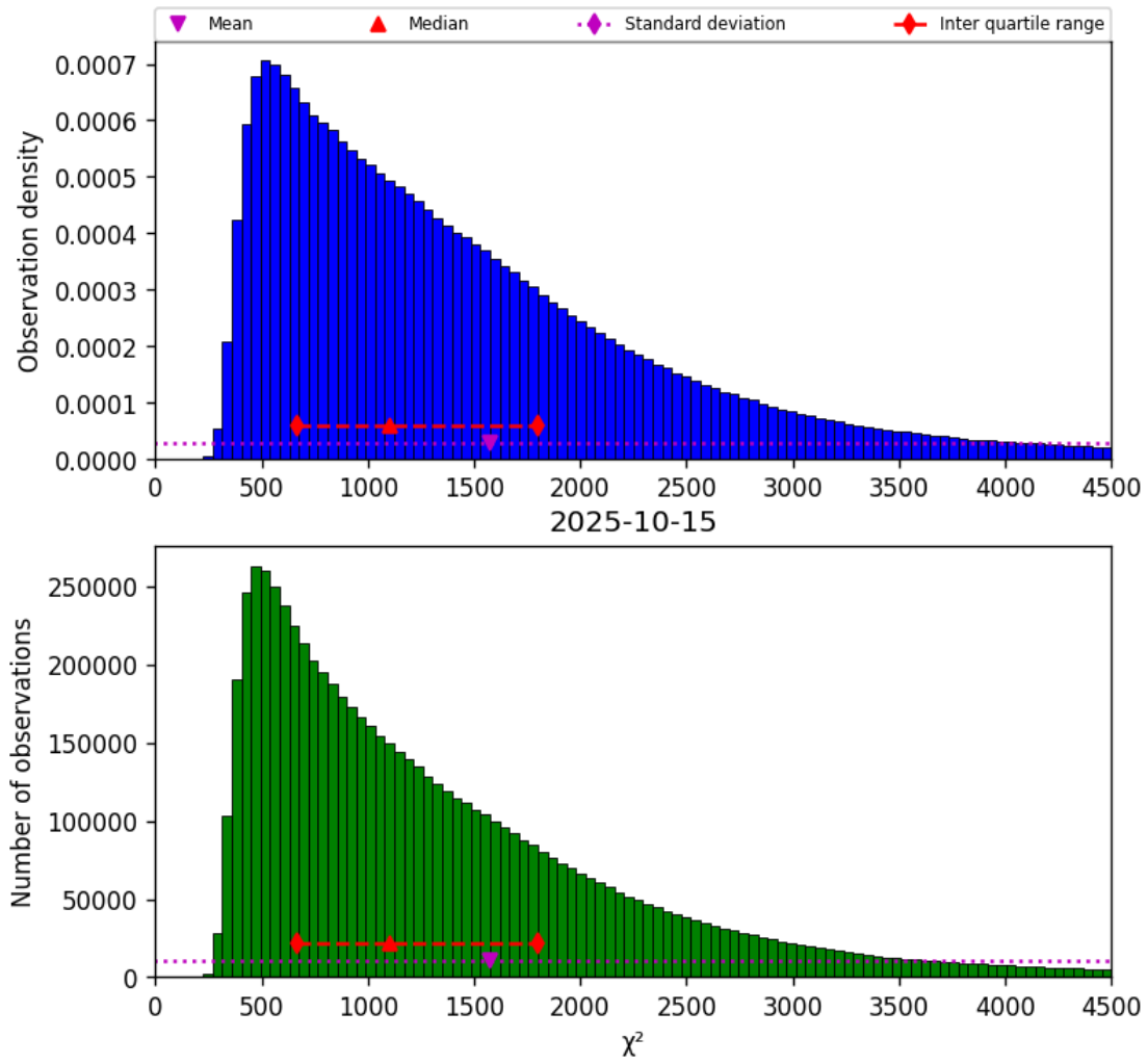
Figure 17: Histogram of “ \chi^2 ” for 2025-10-15 to 2025-10-15
