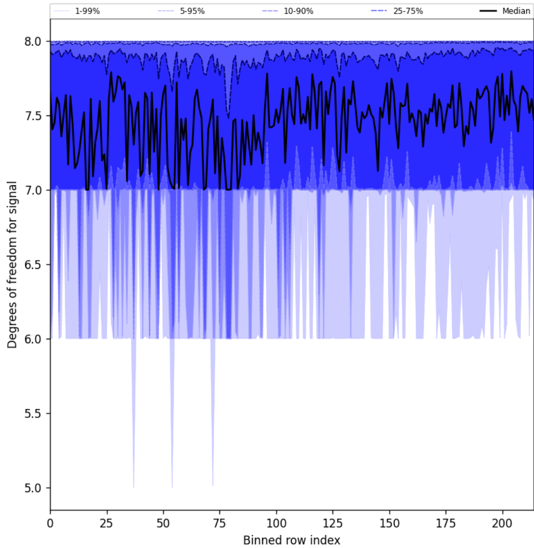
Figure 25: Along track statistics of “Degrees of freedom for signal” for 2025-10-15 to 2025-10-15
