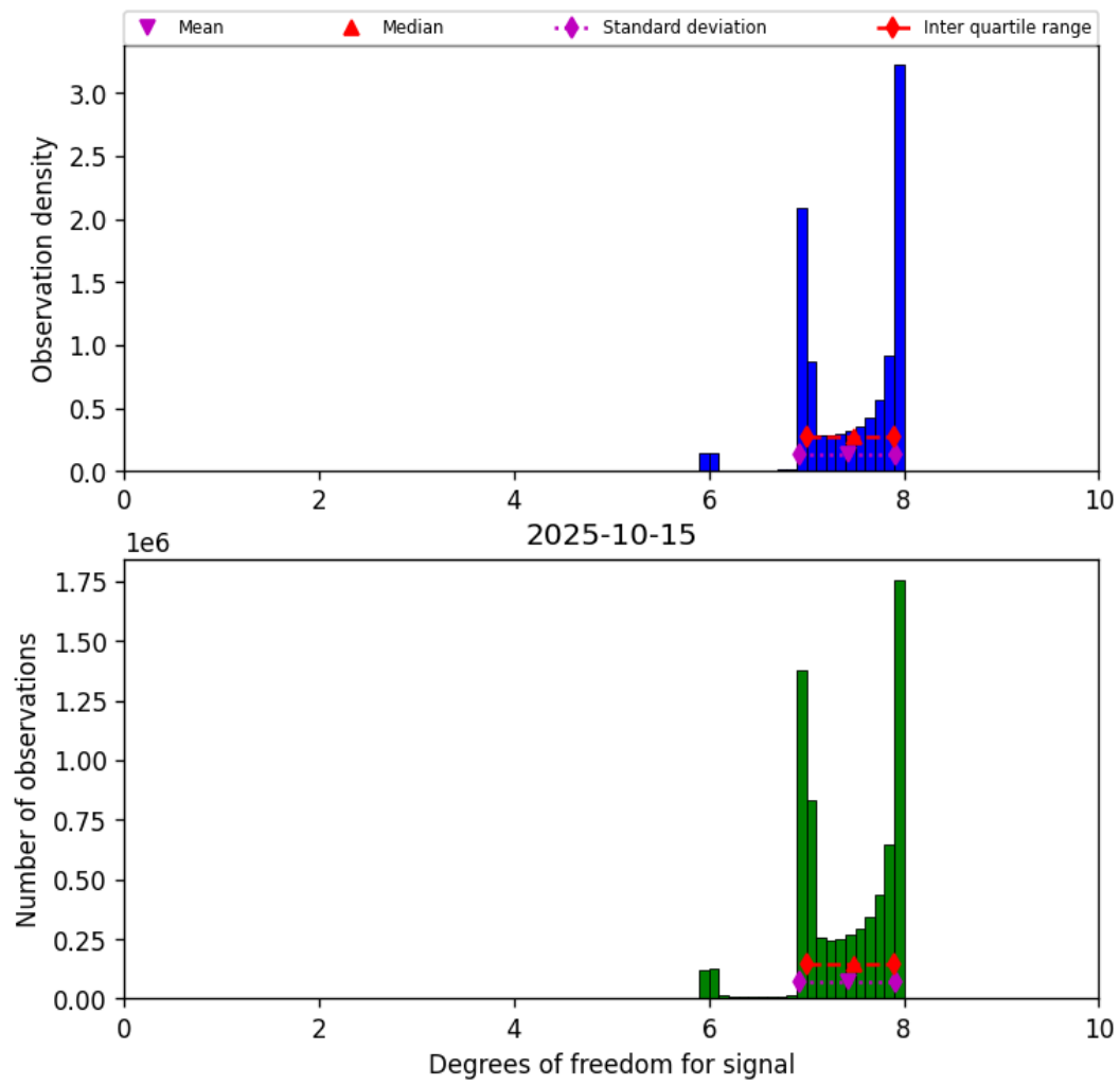
Figure 18: Histogram of “Degrees of freedom for signal” for 2025-10-15 to 2025-10-15
