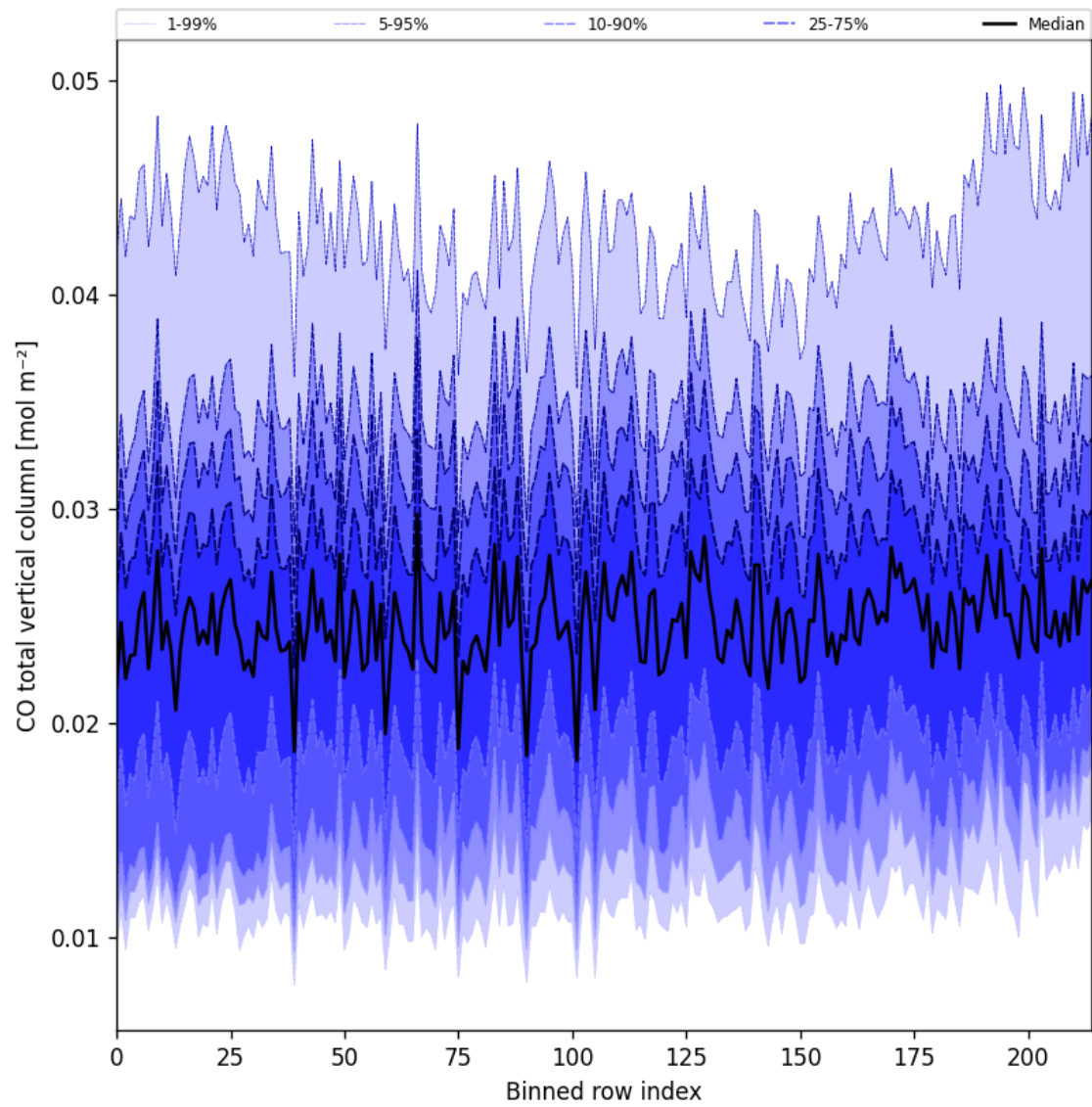
Figure 21: Along track statistics of “CO total vertical column” for 2025-10-15 to 2025-10-15
