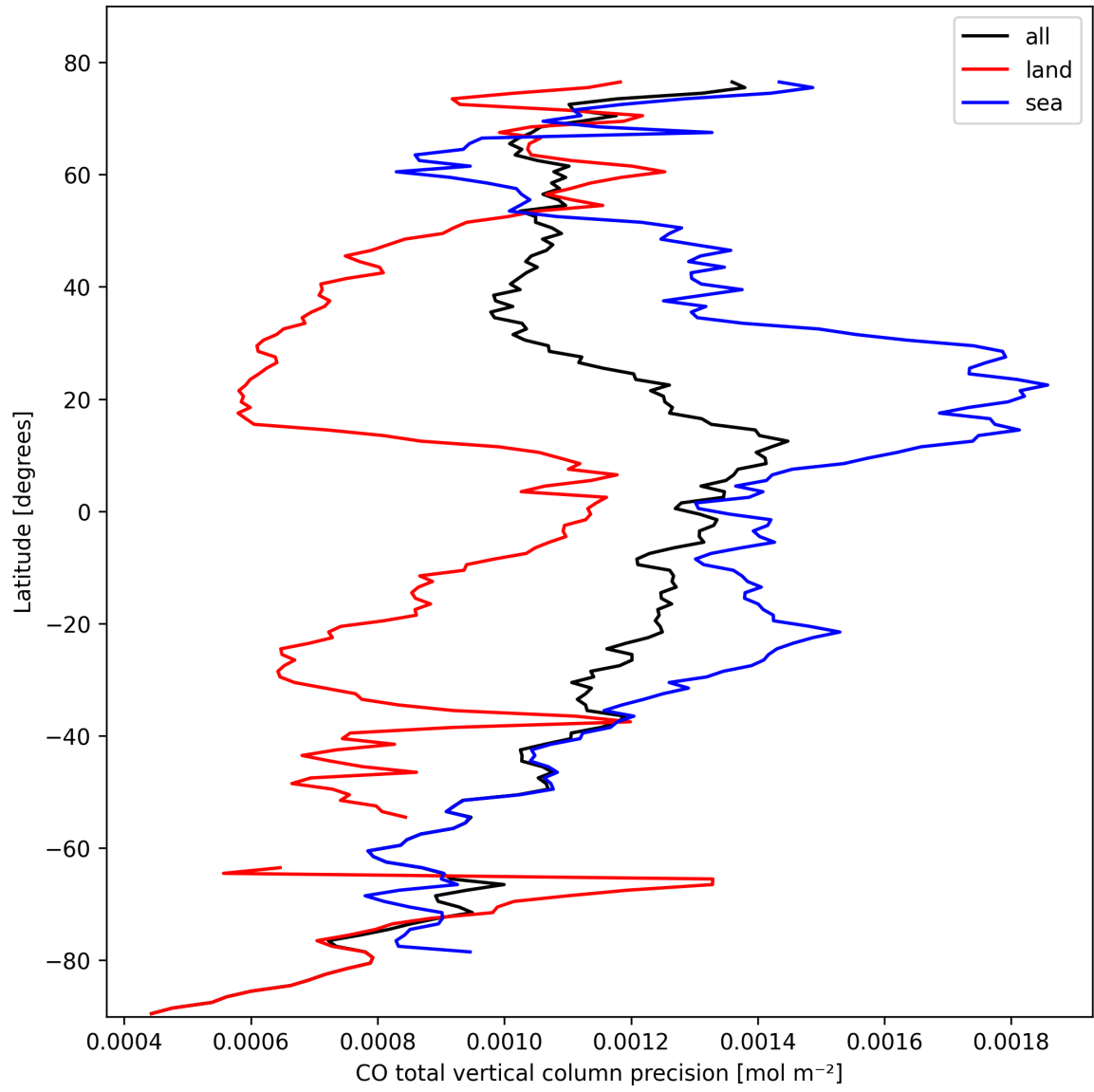
Figure 8: Zonal average of "CO total vertical column precision" for 2025-10-15 to 2025-10-15.
