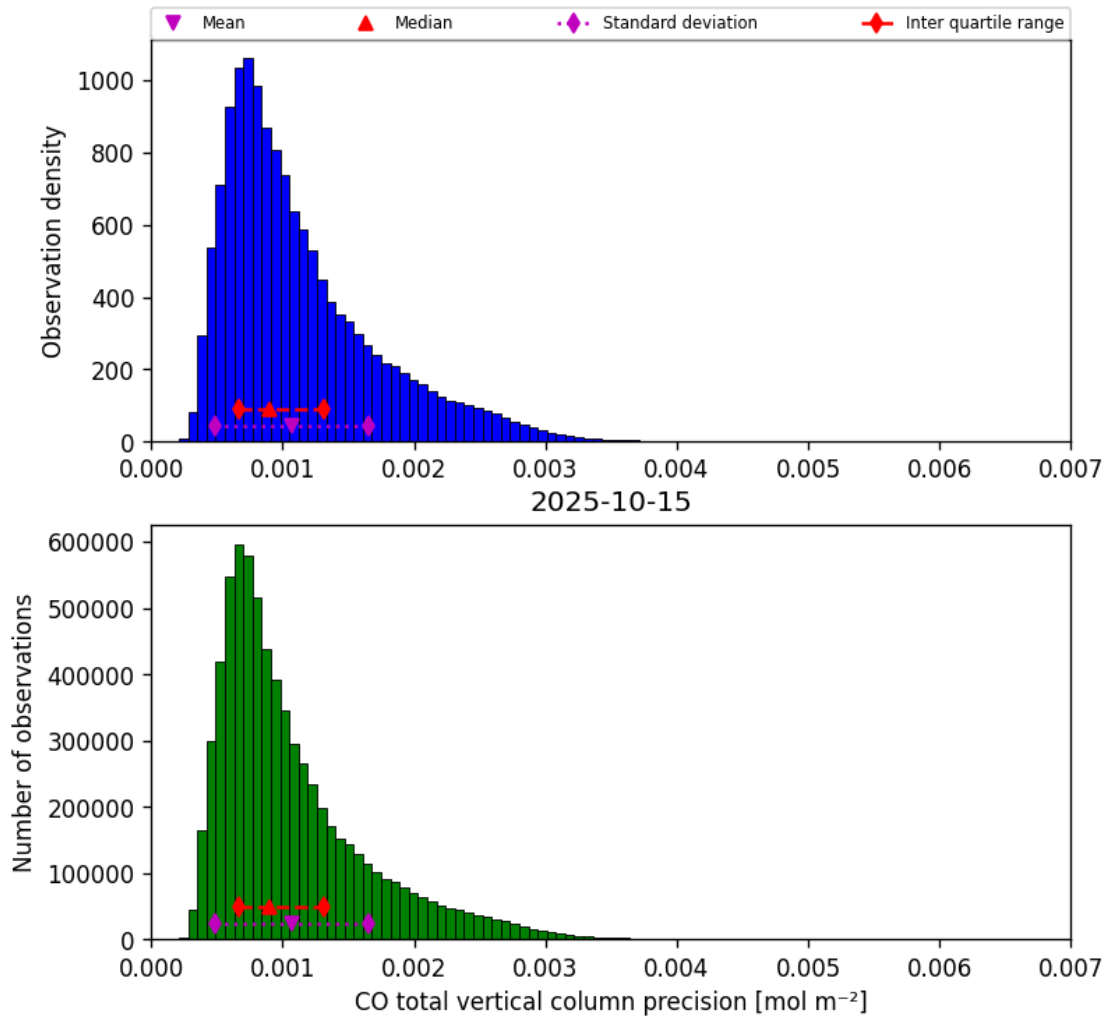
Figure 15: Histogram of “CO total vertical column precision” for 2025-10-15 to 2025-10-15
