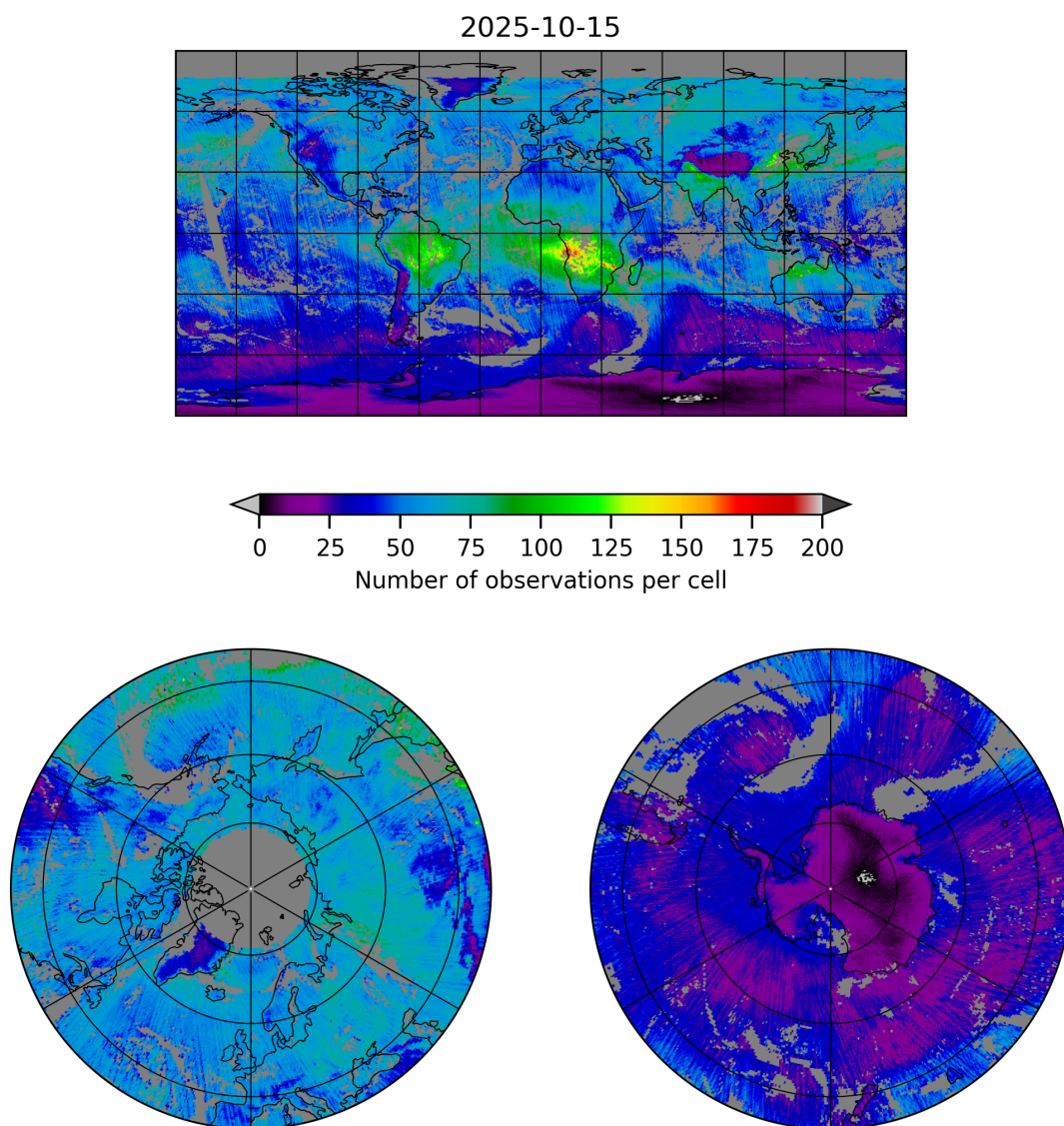
Figure 5: Map of the number of observations for 2025-10-15 to 2025-10-15
