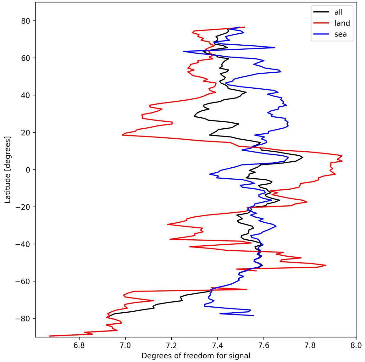
Figure 11: Zonal average of “Degrees of freedom for signal” for 2025-10-15 to 2025-10-15.
