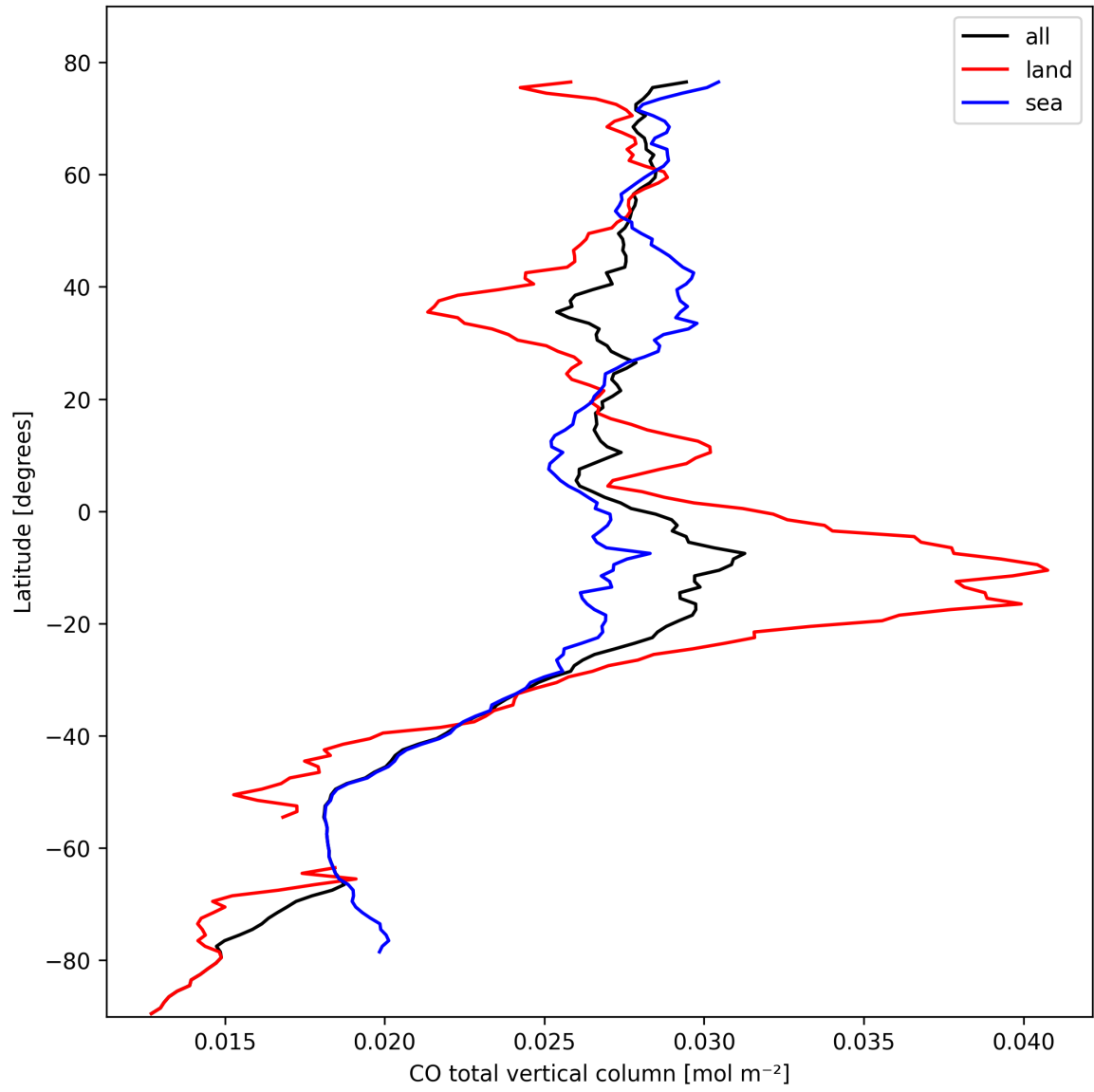
Figure 7: Zonal average of “CO total vertical column” for 2025-10-15 to 2025-10-15.
