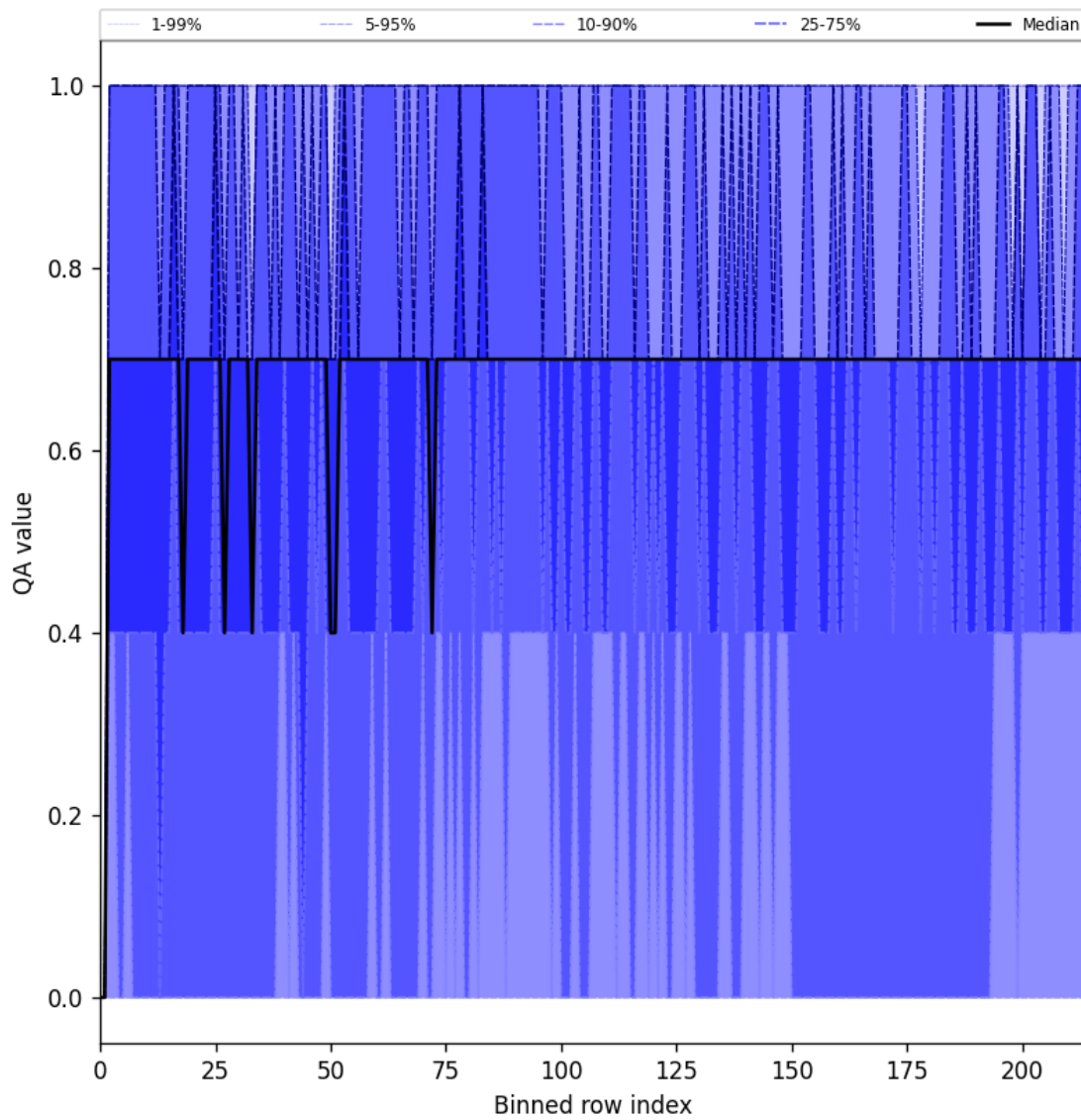
Figure 20: Along track statistics of “QA value” for 2025-10-15 to 2025-10-15
