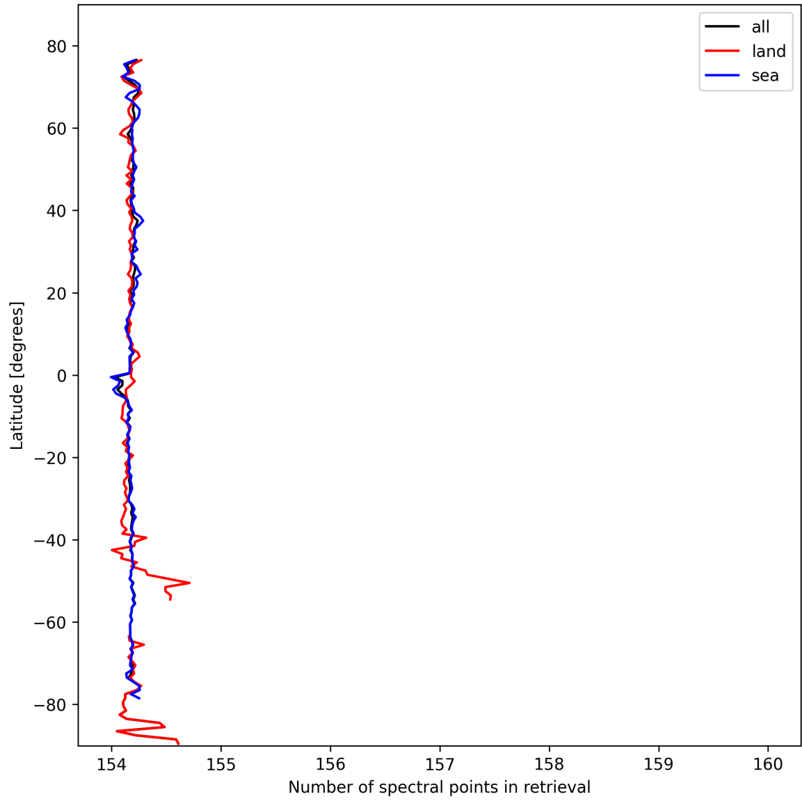
Figure 9: Zonal average of “Number of spectral points in retrieval” for 2025-10-15 to 2025-10-15.
