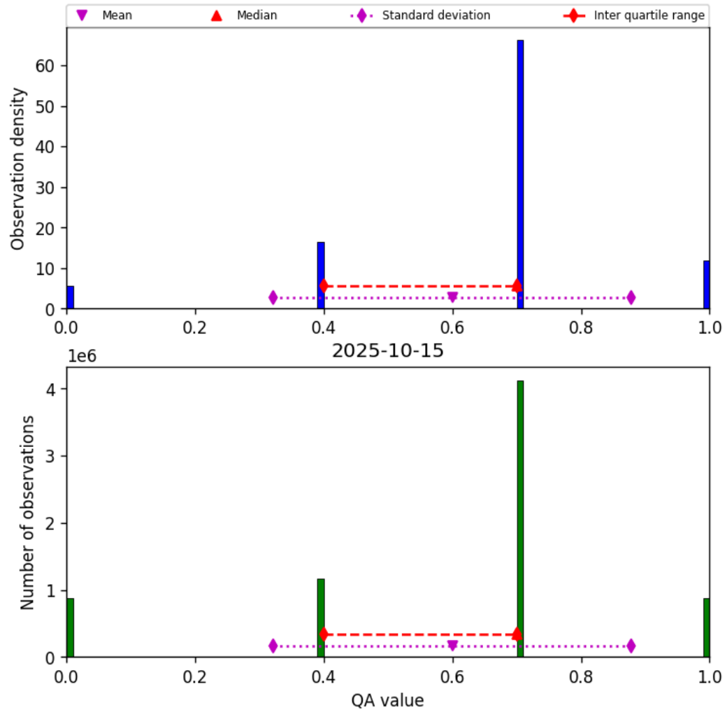
Figure 13: Histogram of “QA value” for 2025-10-15 to 2025-10-15
