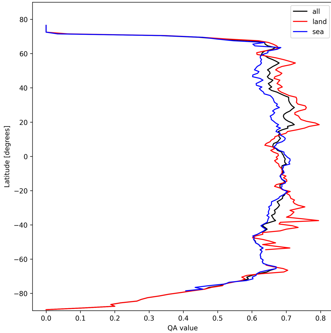
Figure 6: Zonal average of “QA value” for 2025-10-15 to 2025-10-15.
