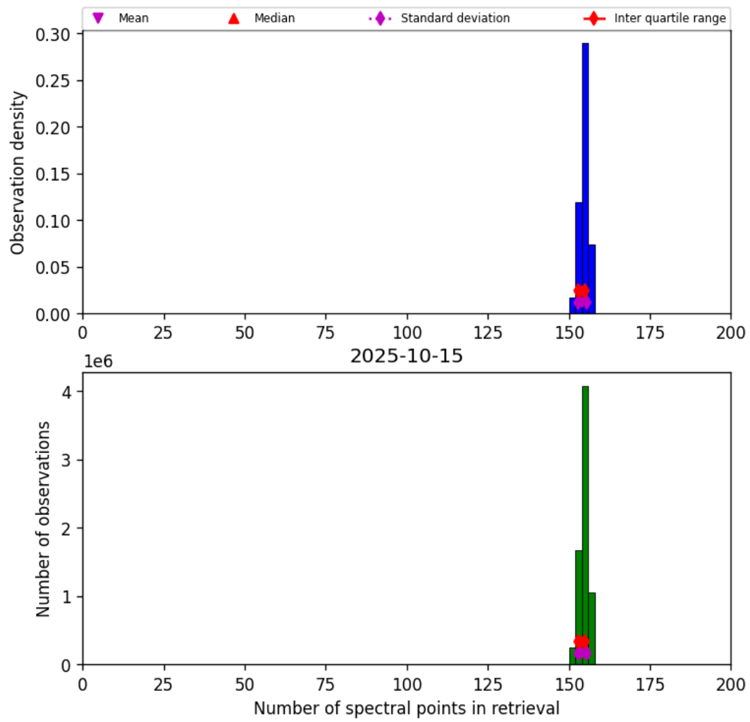
Figure 16: Histogram of “Number of spectral points in retrieval” for 2025-10-15 to 2025-10-15
