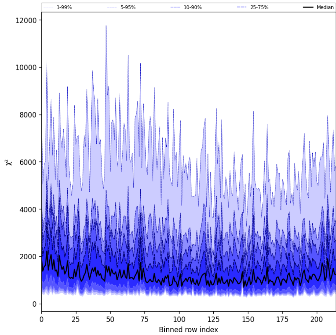
Figure 24: Along track statistics of “ \chi^2 ” for 2025-10-15 to 2025-10-15
