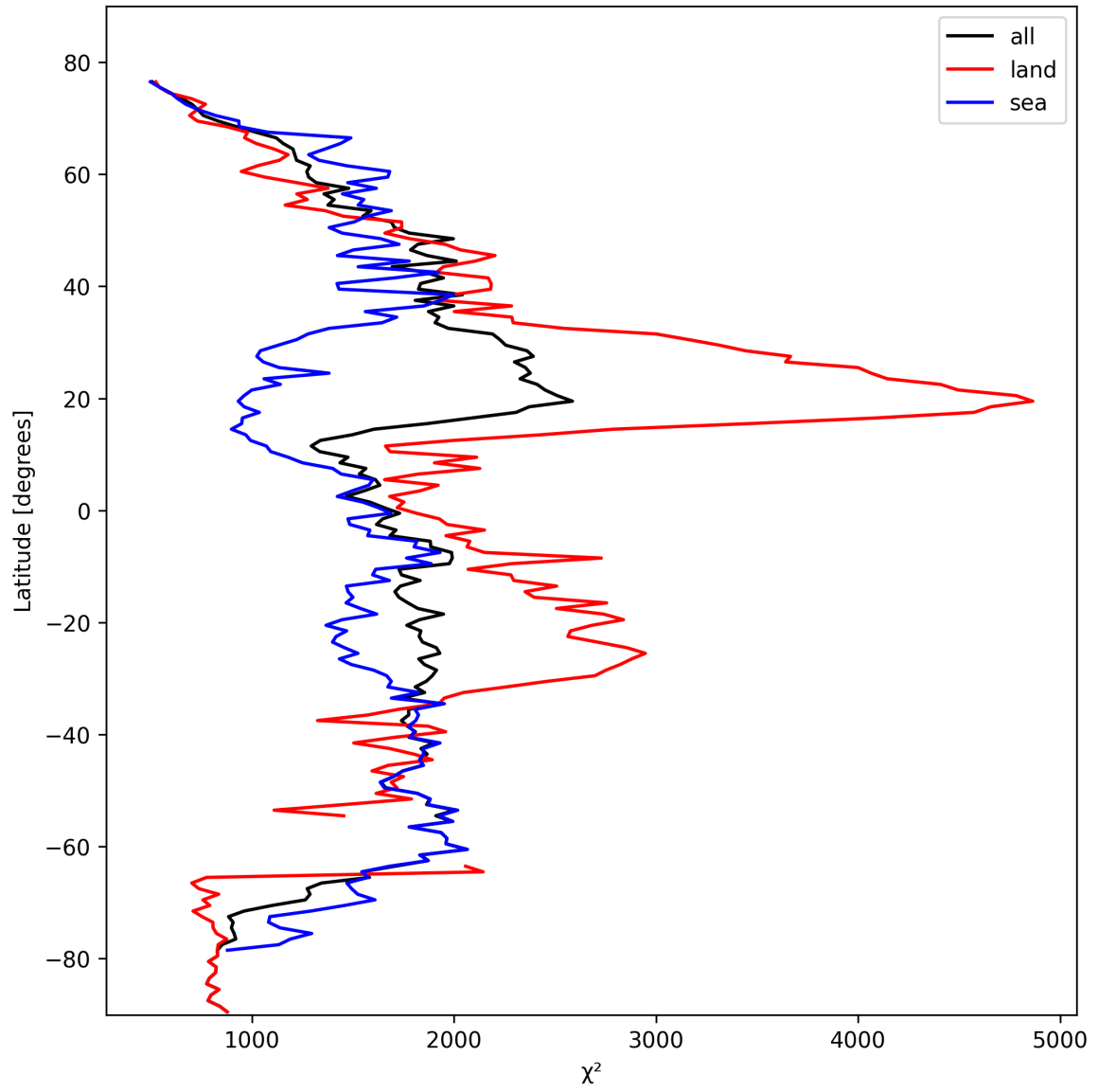
Figure 10: Zonal average of “ \chi^2 ” for 2025-10-15 to 2025-10-15.
