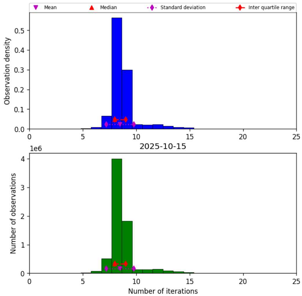
Figure 19: Histogram of “Number of iterations” for 2025-10-15 to 2025-10-15
