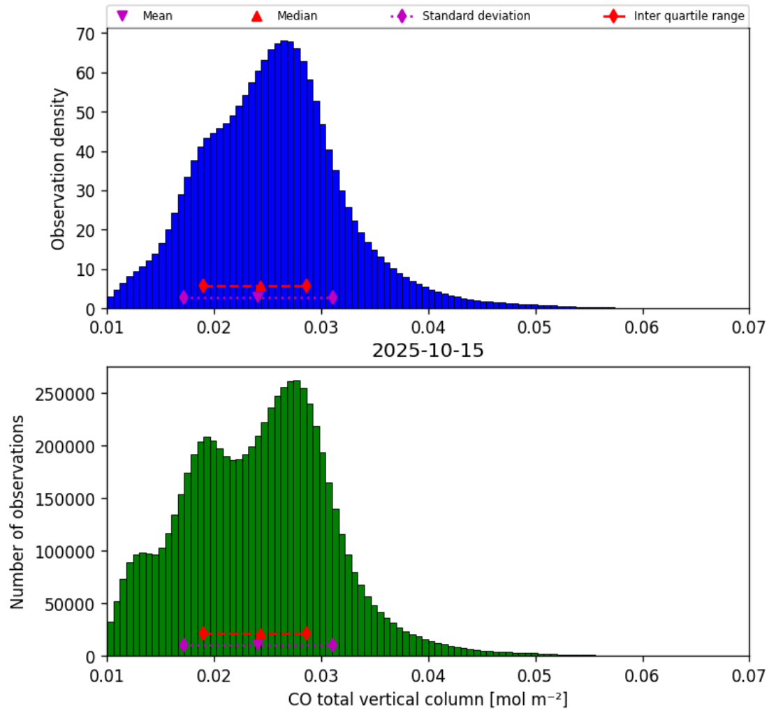
Figure 14: Histogram of “CO total vertical column” for 2025-10-15 to 2025-10-15
