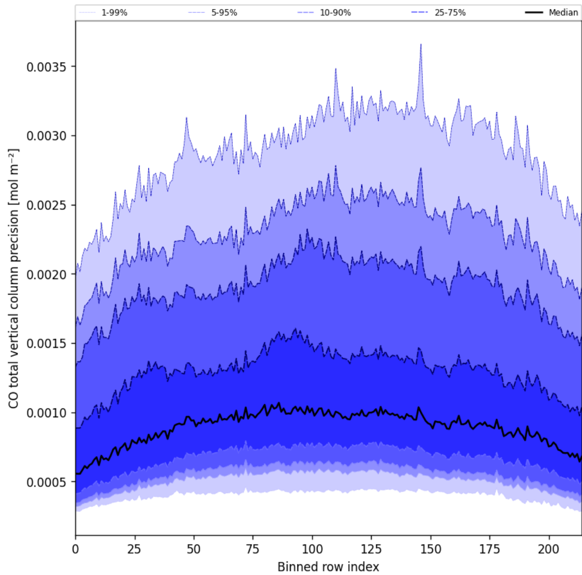
Figure 22: Along track statistics of “CO total vertical column precision” for 2025-10-15 to 2025-10-15
