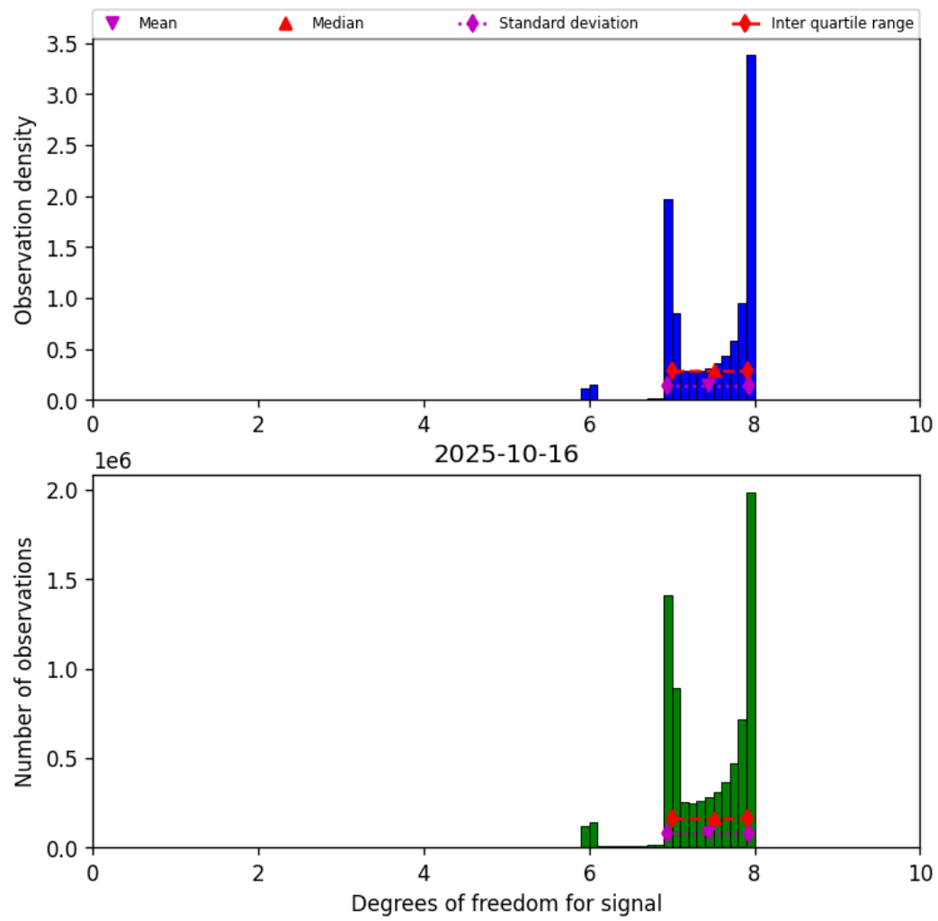
Figure 18: Histogram of “Degrees of freedom for signal” for 2025-10-16 to 2025-10-17
