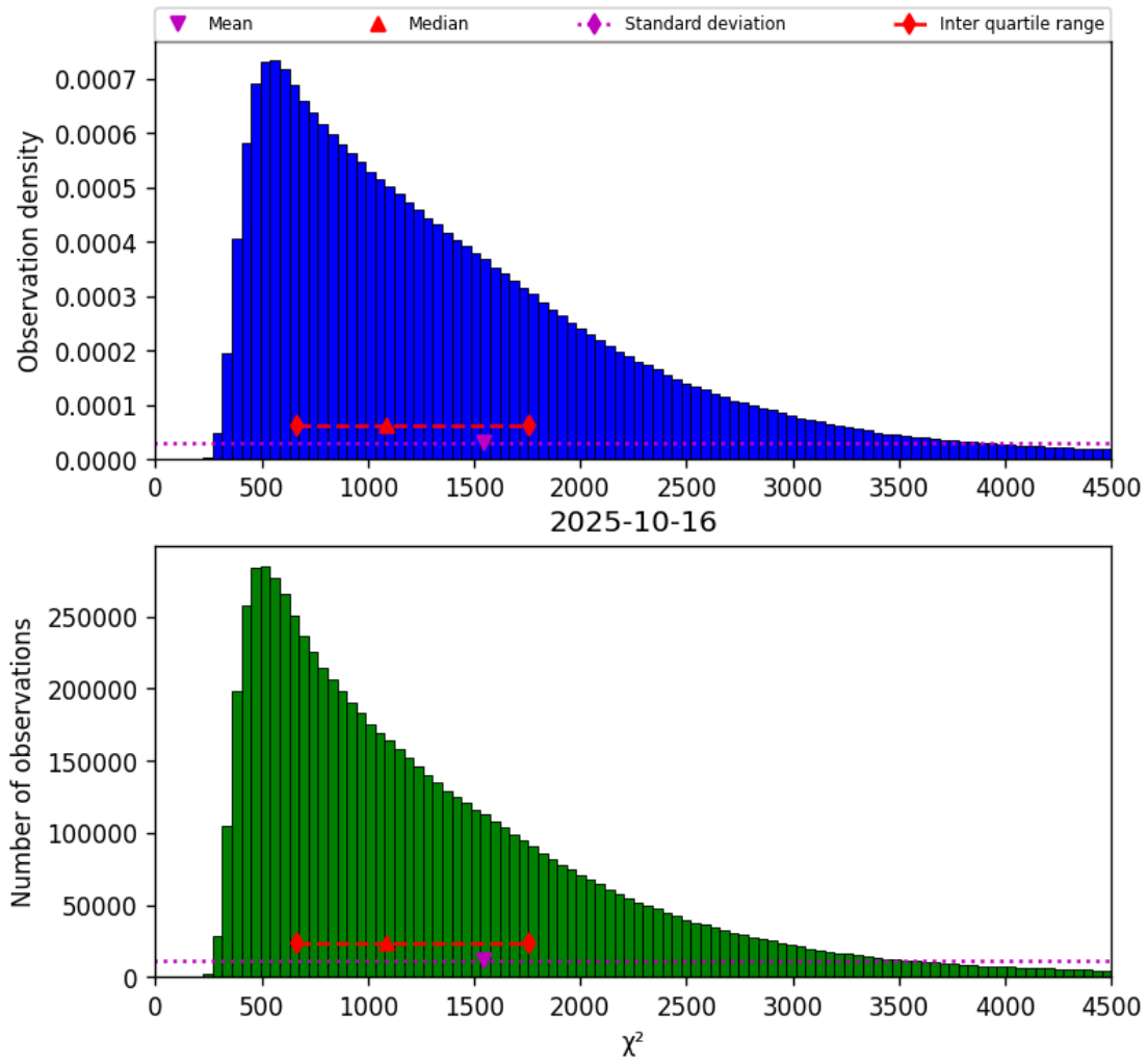
Figure 17: Histogram of “ \chi^2 ” for 2025-10-16 to 2025-10-17
