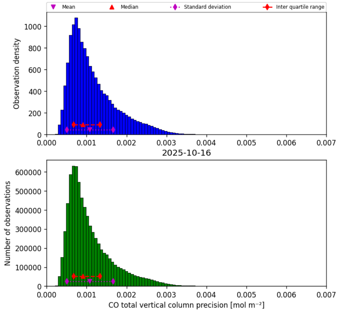
Figure 15: Histogram of “CO total vertical column precision” for 2025-10-16 to 2025-10-17
