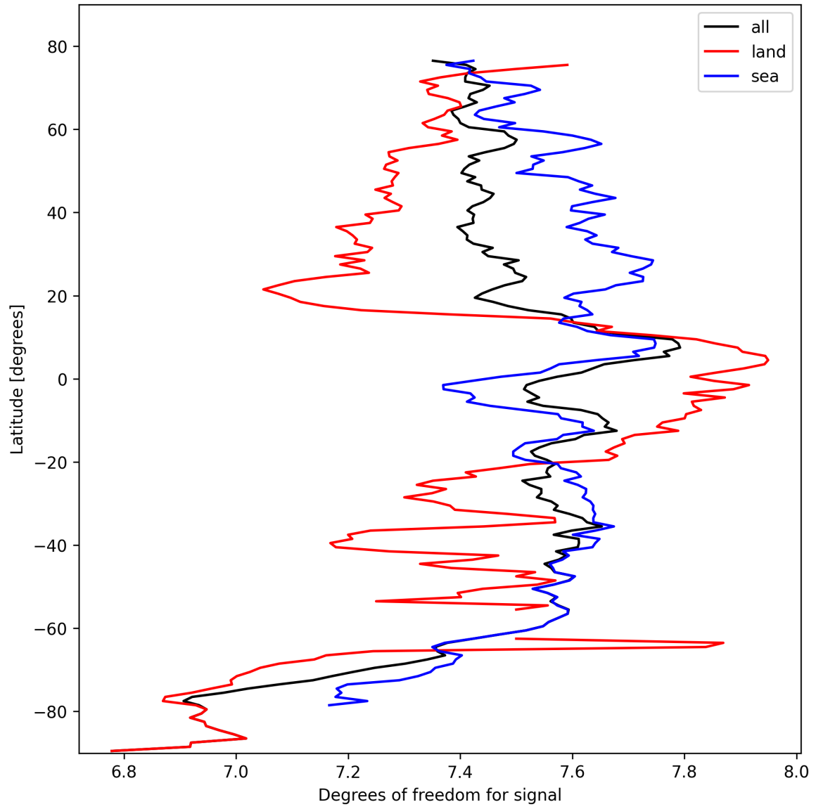
Figure 11: Zonal average of “Degrees of freedom for signal” for 2025-10-16 to 2025-10-17.
