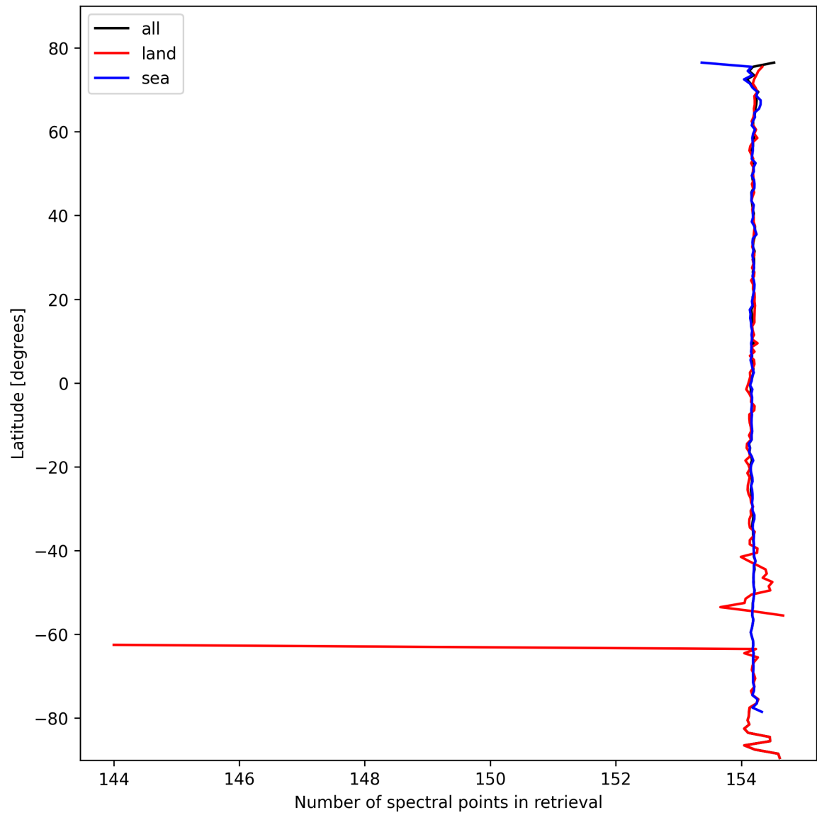
Figure 9: Zonal average of “Number of spectral points in retrieval” for 2025-10-16 to 2025-10-17.
