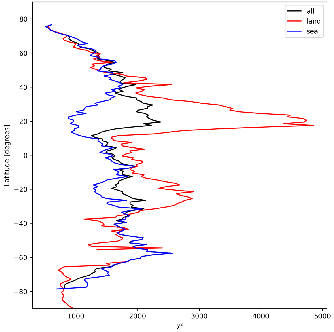
Figure 10: Zonal average of “ \chi^2 ” for 2025-10-16 to 2025-10-17.
