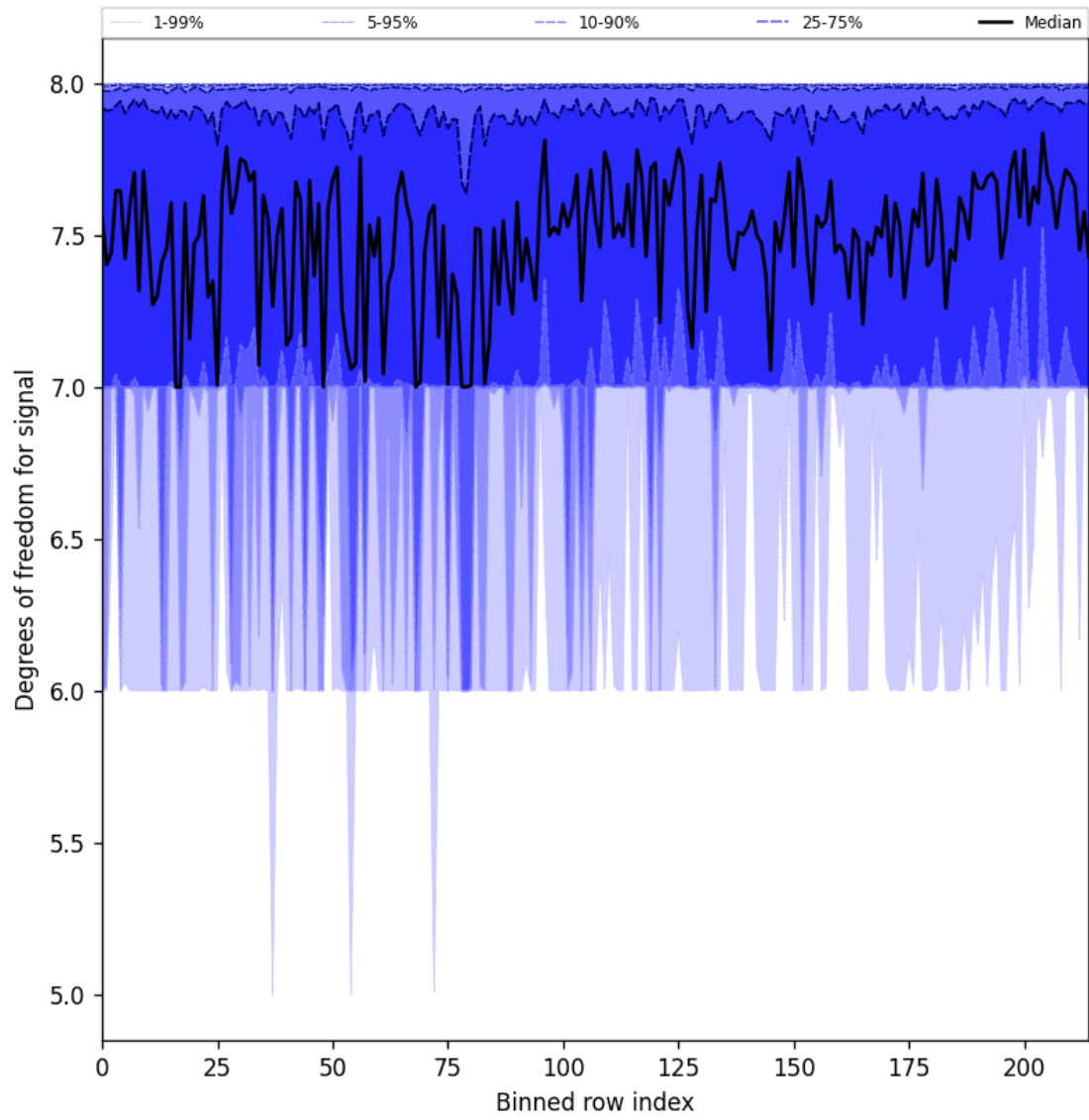
Figure 25: Along track statistics of “Degrees of freedom for signal” for 2025-10-16 to 2025-10-17
