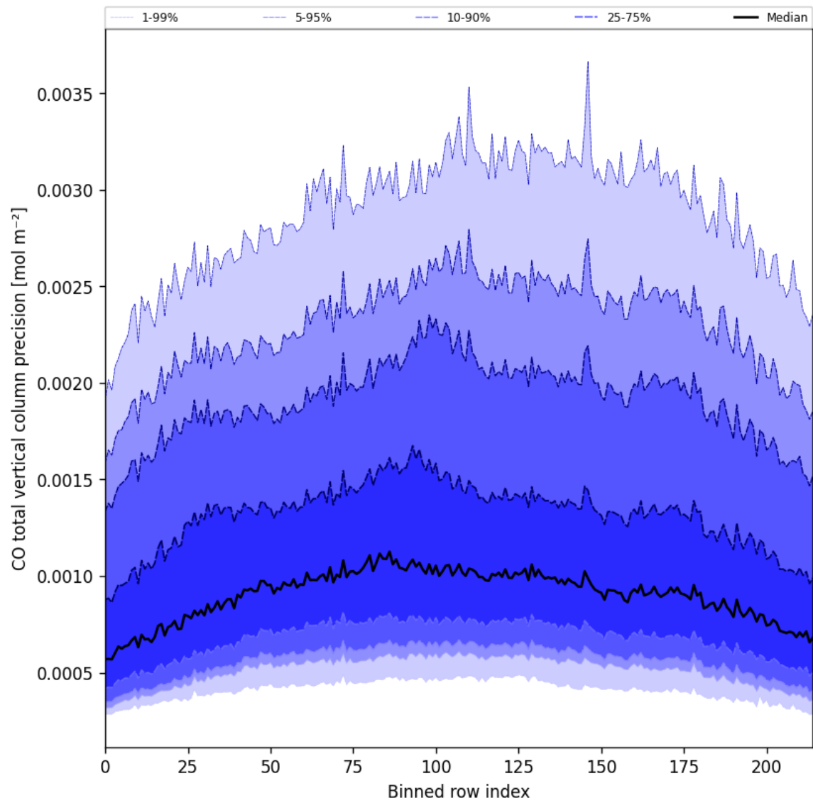
Figure 22: Along track statistics of “CO total vertical column precision” for 2025-10-16 to 2025-10-17
