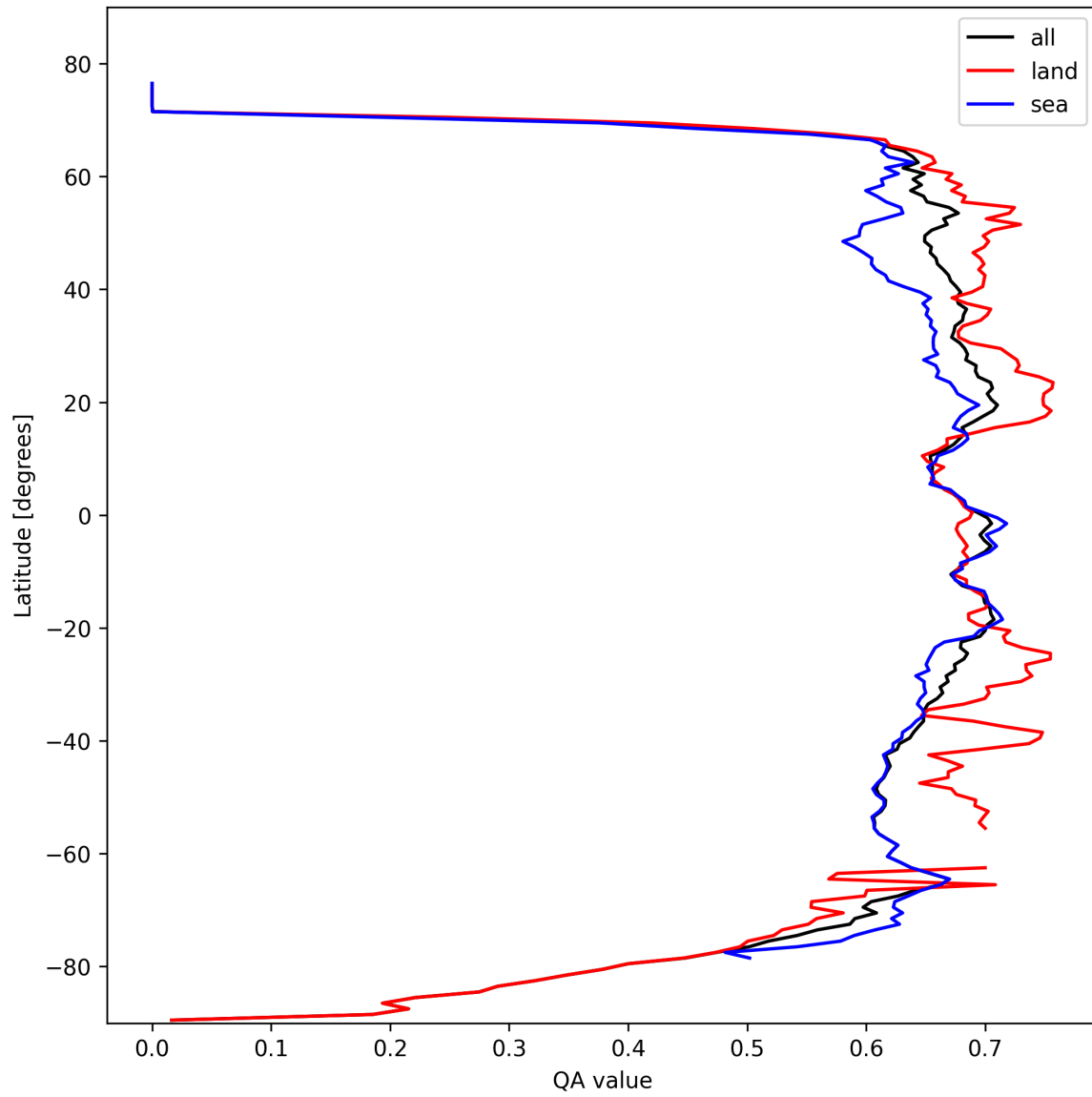
Figure 6: Zonal average of “QA value” for 2025-10-16 to 2025-10-17.
