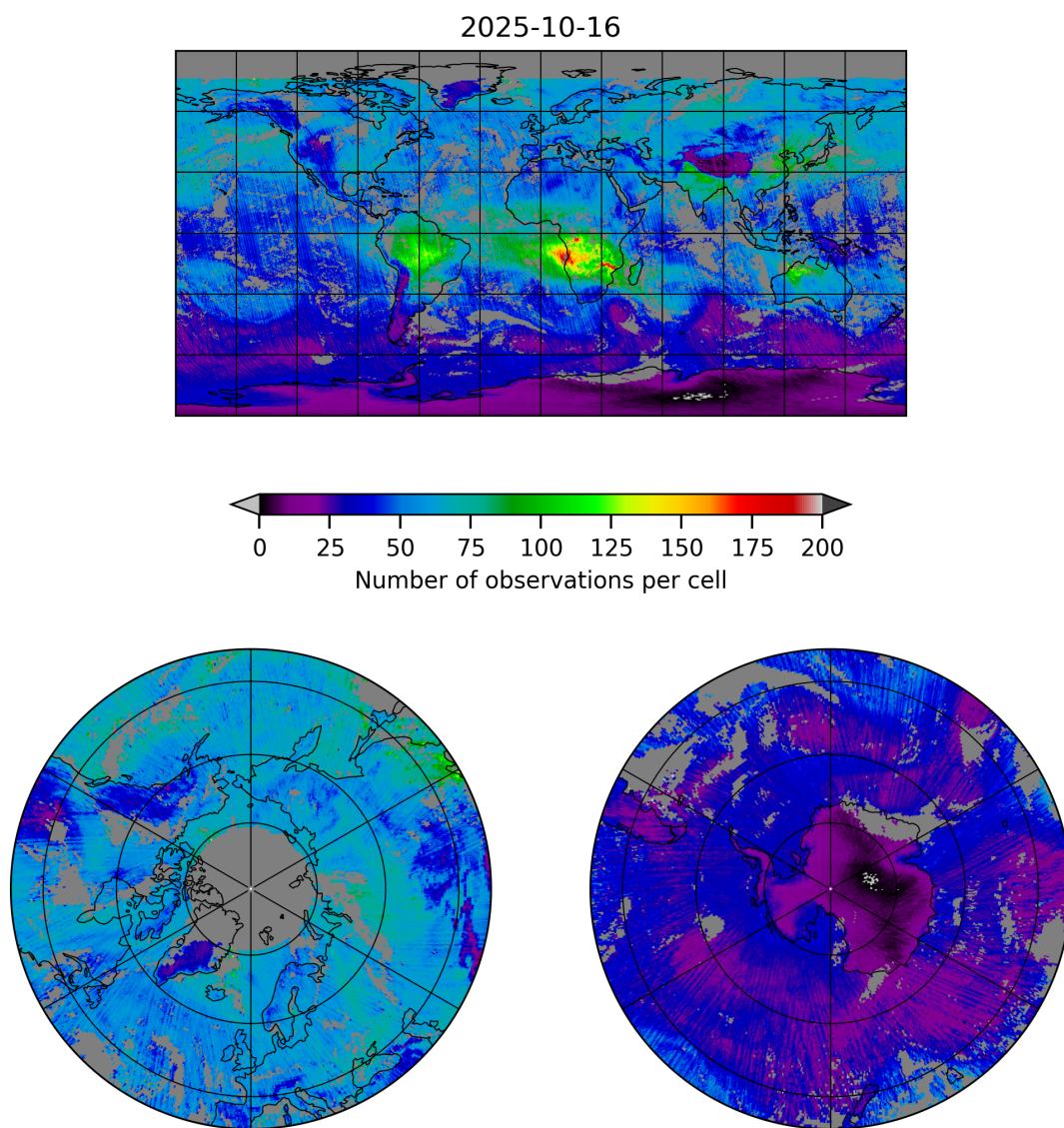
Figure 5: Map of the number of observations for 2025-10-16 to 2025-10-17
