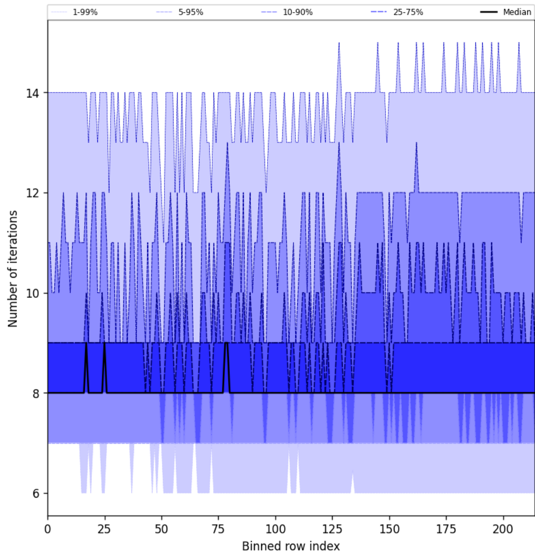
Figure 26: Along track statistics of “Number of iterations” for 2025-10-16 to 2025-10-17
