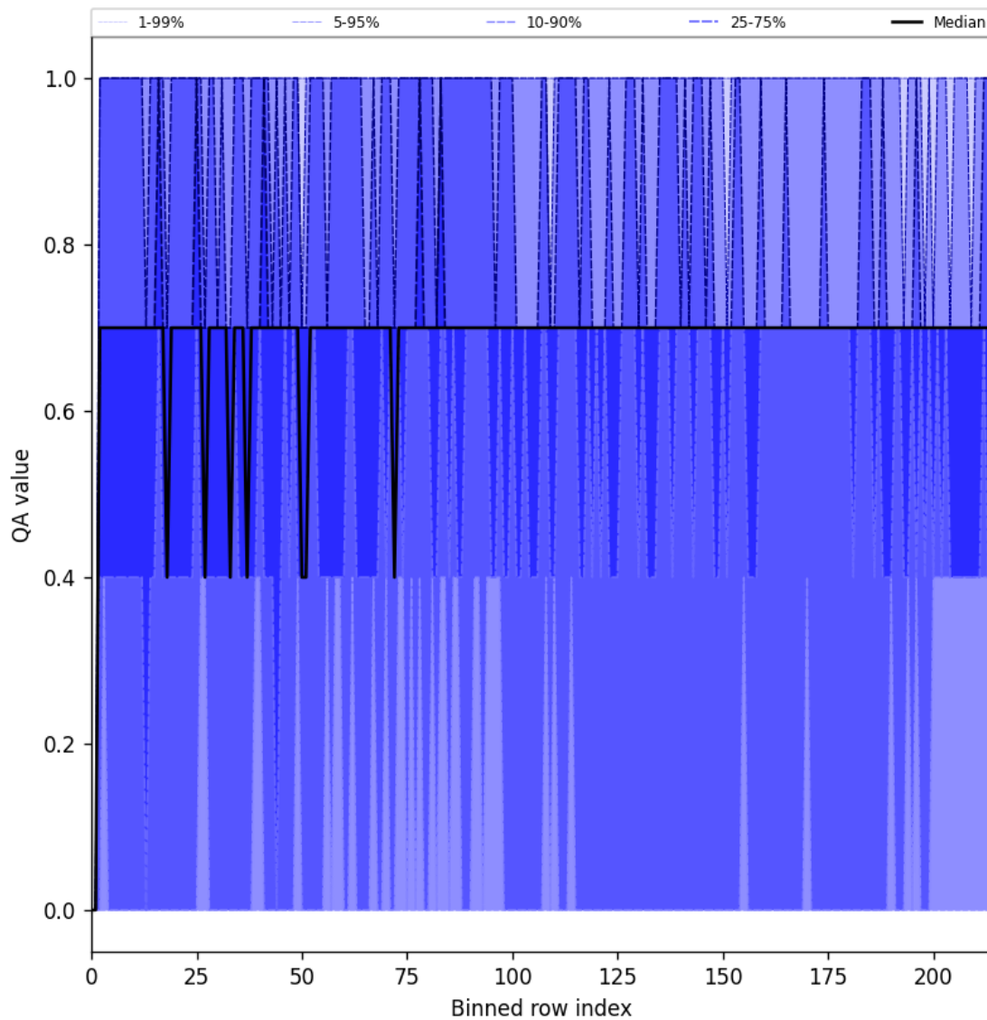
Figure 20: Along track statistics of “QA value” for 2025-10-16 to 2025-10-17
