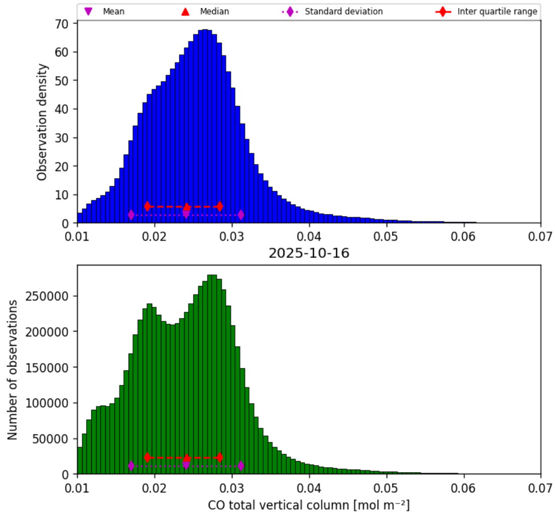
Figure 14: Histogram of “CO total vertical column” for 2025-10-16 to 2025-10-17
