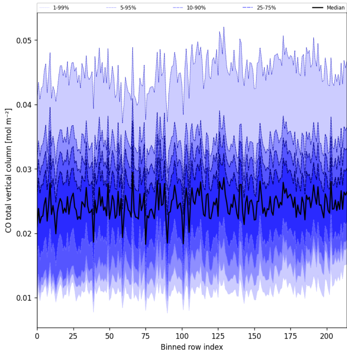
Figure 21: Along track statistics of “CO total vertical column” for 2025-10-16 to 2025-10-17
