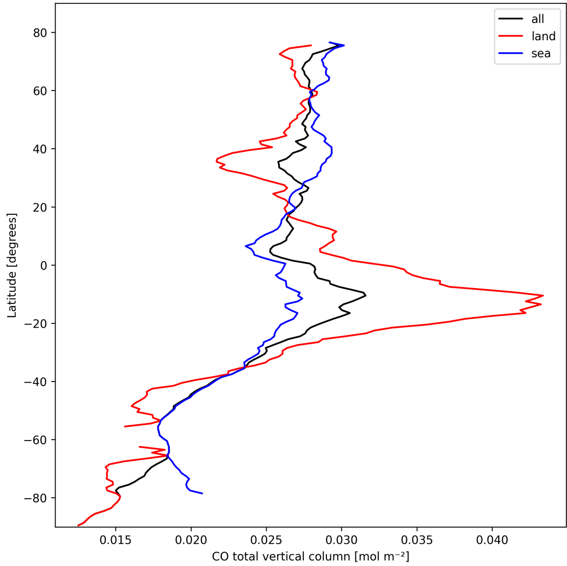
Figure 7: Zonal average of “CO total vertical column” for 2025-10-16 to 2025-10-17.
