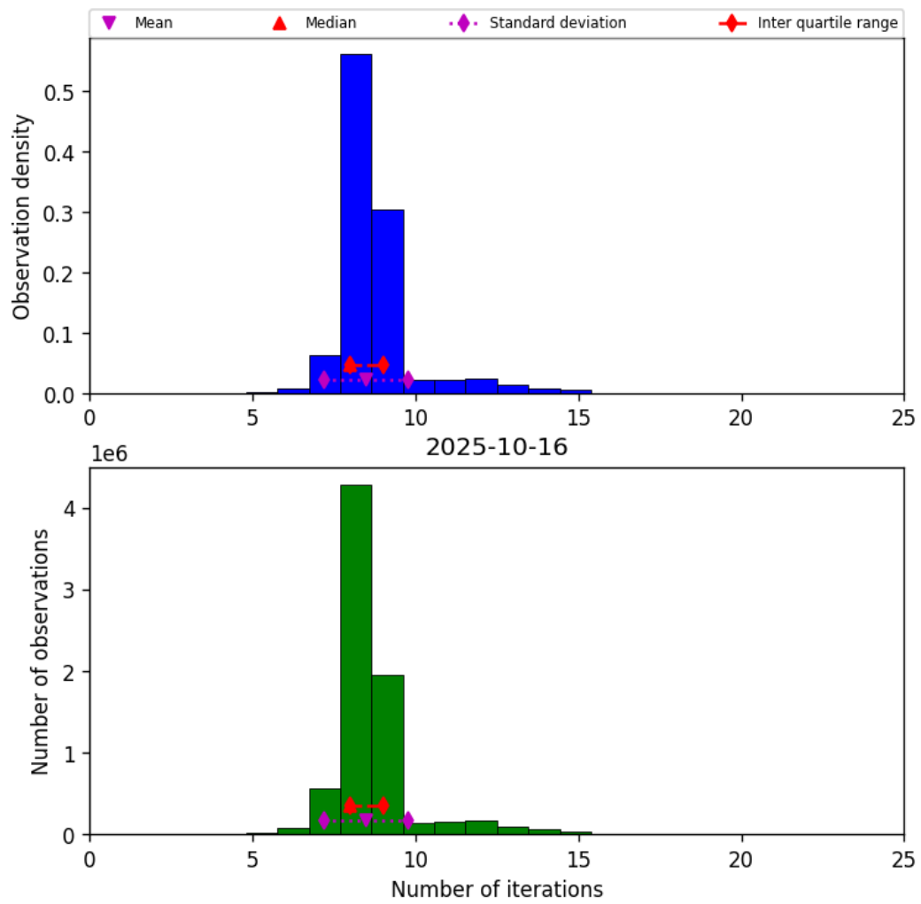
Figure 19: Histogram of “Number of iterations” for 2025-10-16 to 2025-10-17
