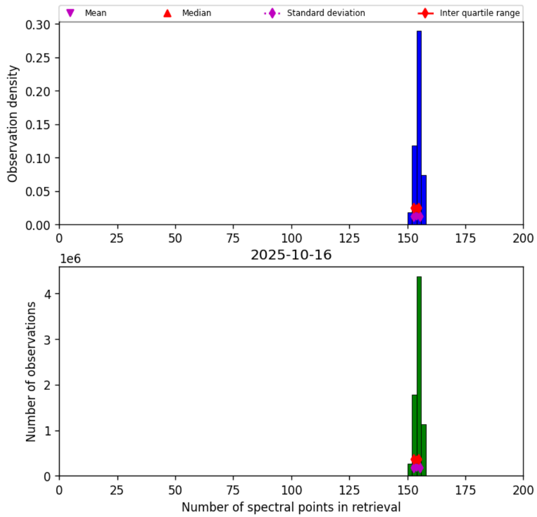
Figure 16: Histogram of “Number of spectral points in retrieval” for 2025-10-16 to 2025-10-17
