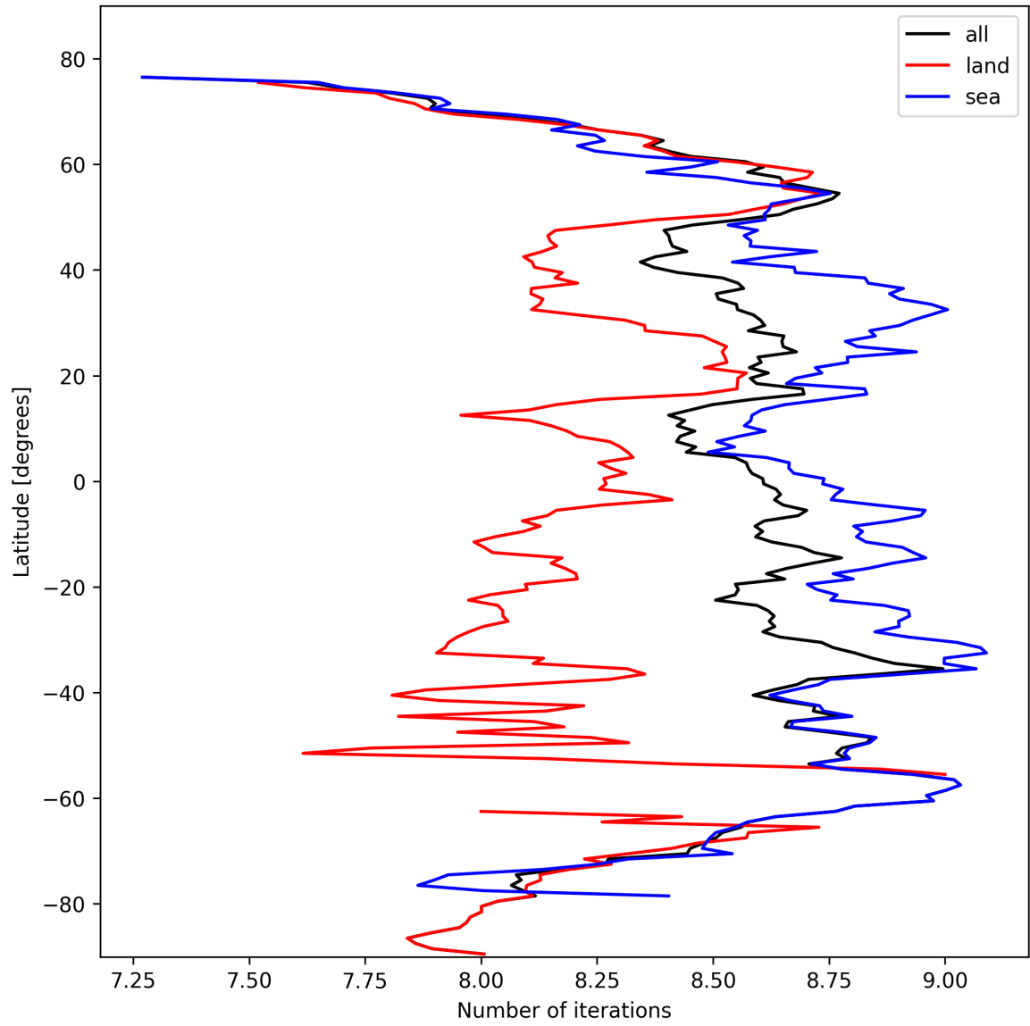
Figure 12: Zonal average of “Number of iterations” for 2025-10-16 to 2025-10-17.
