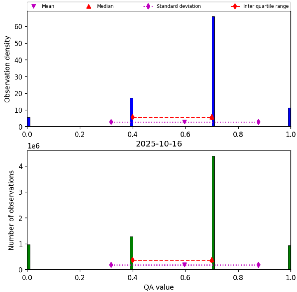
Figure 13: Histogram of “QA value” for 2025-10-16 to 2025-10-17
