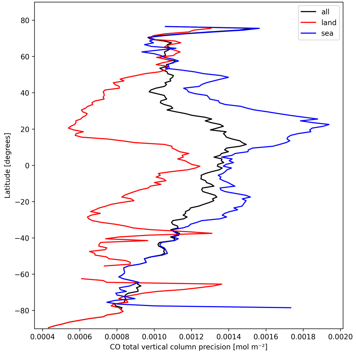
Figure 8: Zonal average of “CO total vertical column precision” for 2025-10-16 to 2025-10-17.
