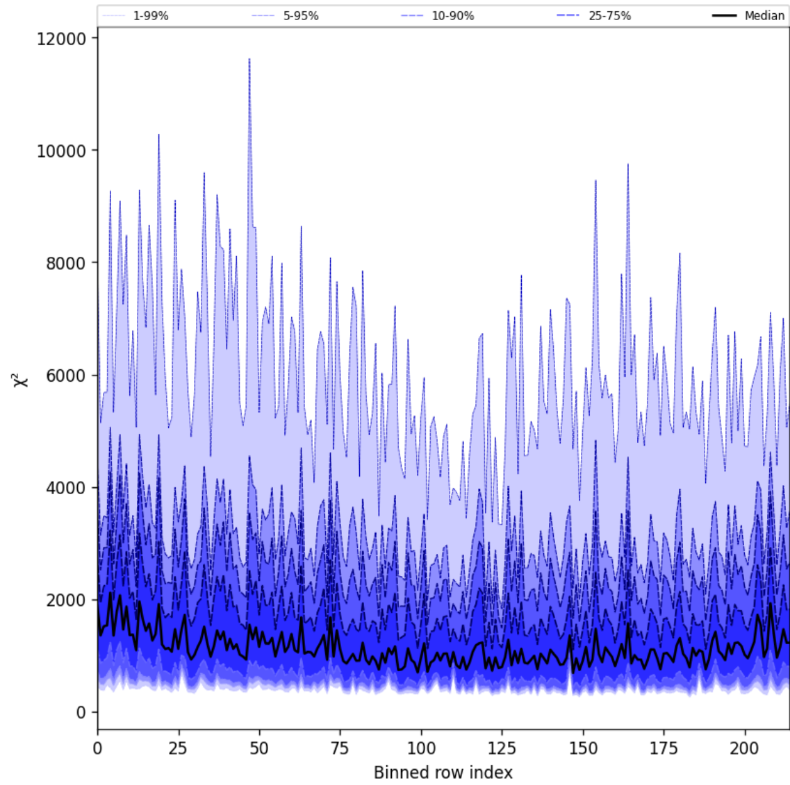
Figure 24: Along track statistics of “ \chi^2 ” for 2025-10-16 to 2025-10-17
