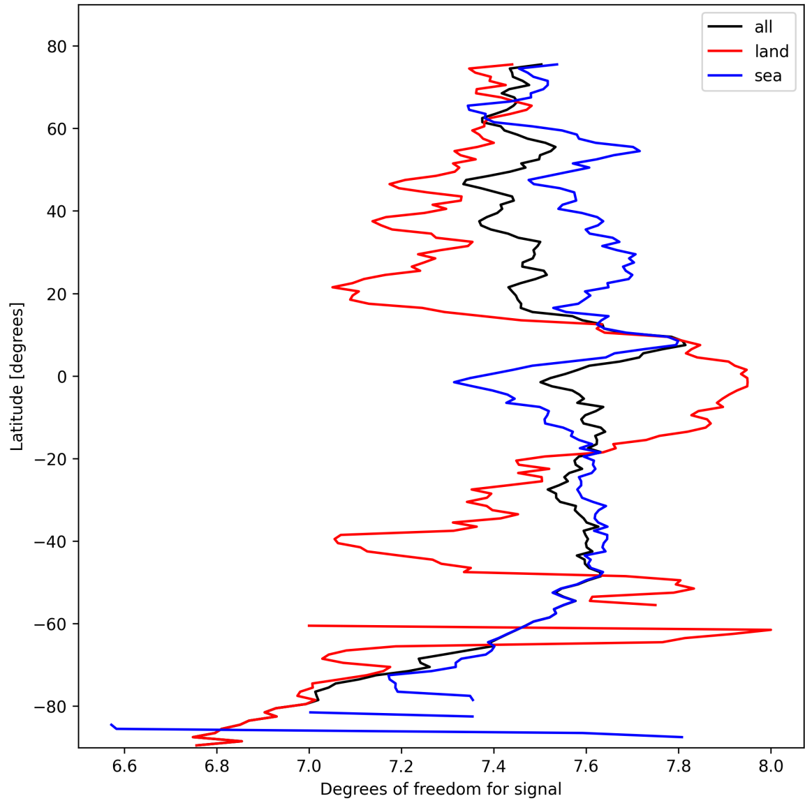
Figure 11: Zonal average of “Degrees of freedom for signal” for 2025-10-17 to 2025-10-18.
