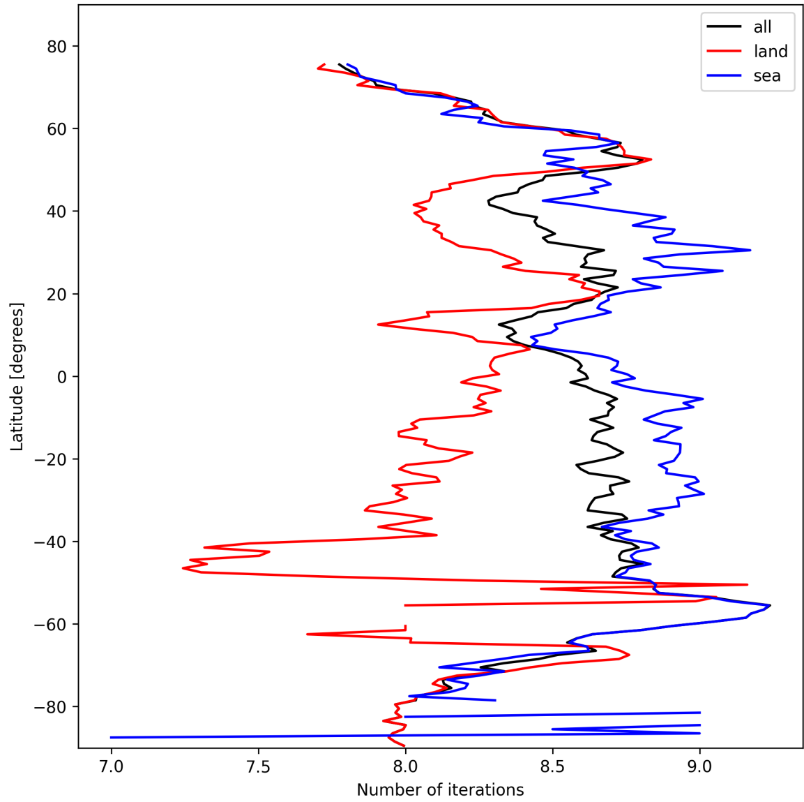
Figure 12: Zonal average of “Number of iterations” for 2025-10-17 to 2025-10-18.
