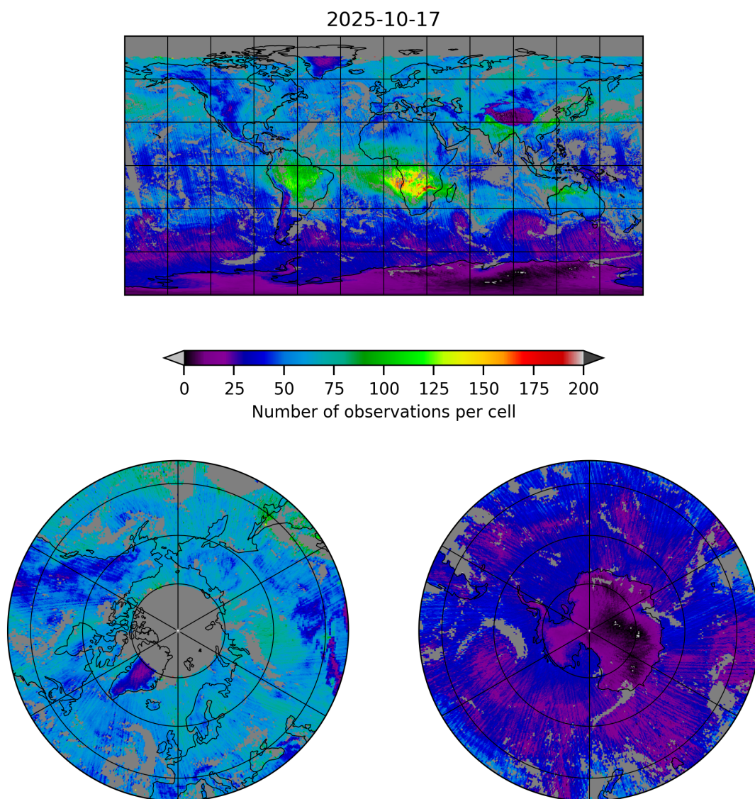
Figure 5: Map of the number of observations for 2025-10-17 to 2025-10-18
