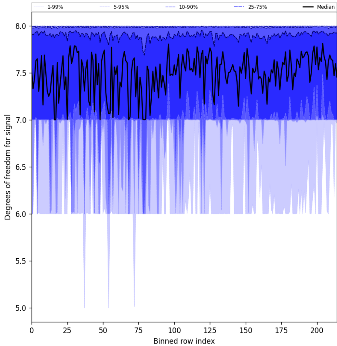
Figure 25: Along track statistics of “Degrees of freedom for signal” for 2025-10-17 to 2025-10-18
