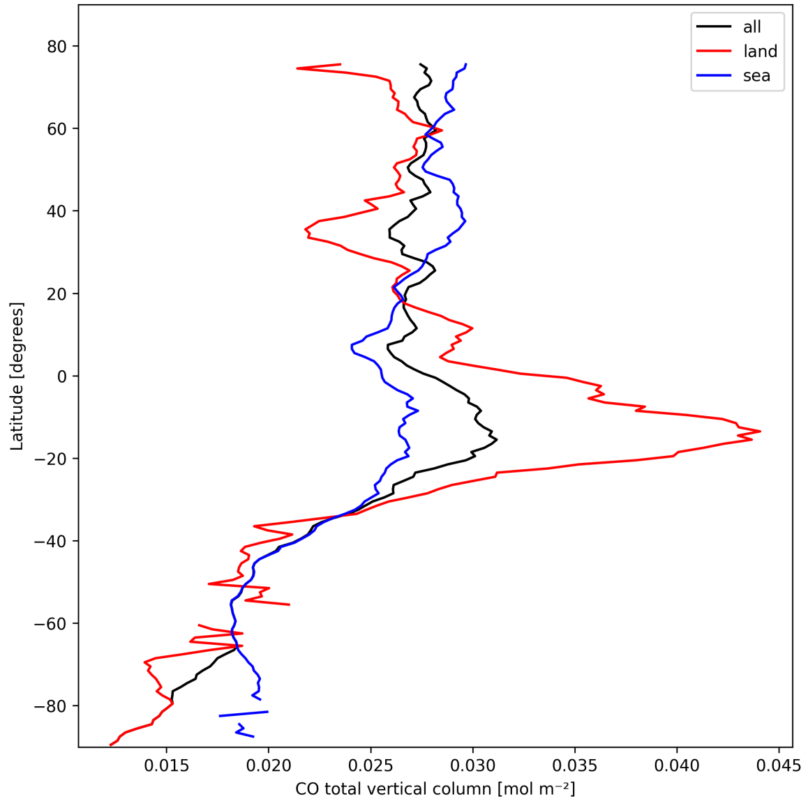
Figure 7: Zonal average of “CO total vertical column” for 2025-10-17 to 2025-10-18.
