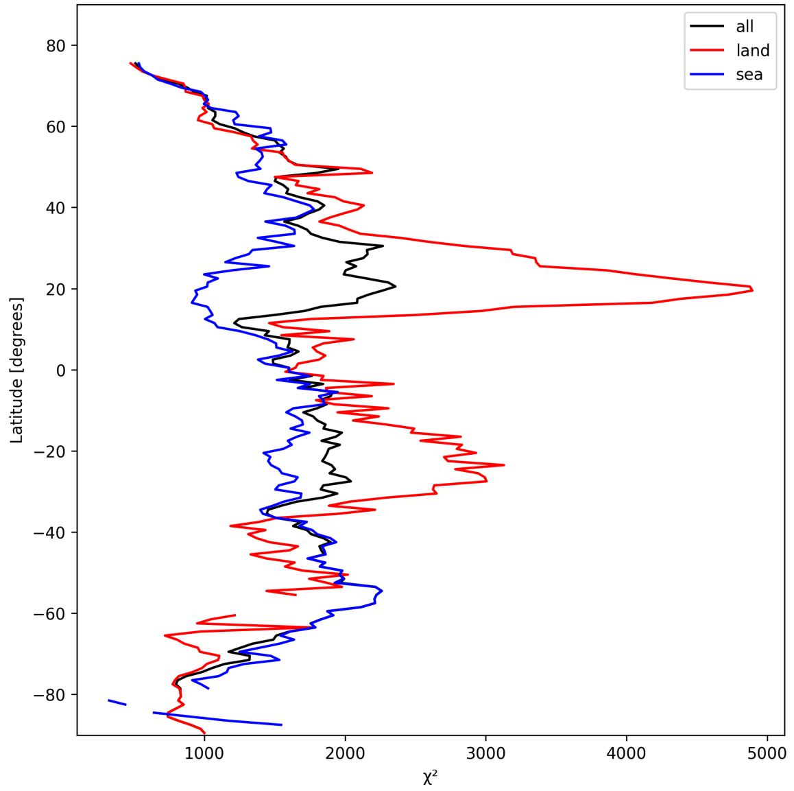
Figure 10: Zonal average of “ \chi^2 ” for 2025-10-17 to 2025-10-18.
