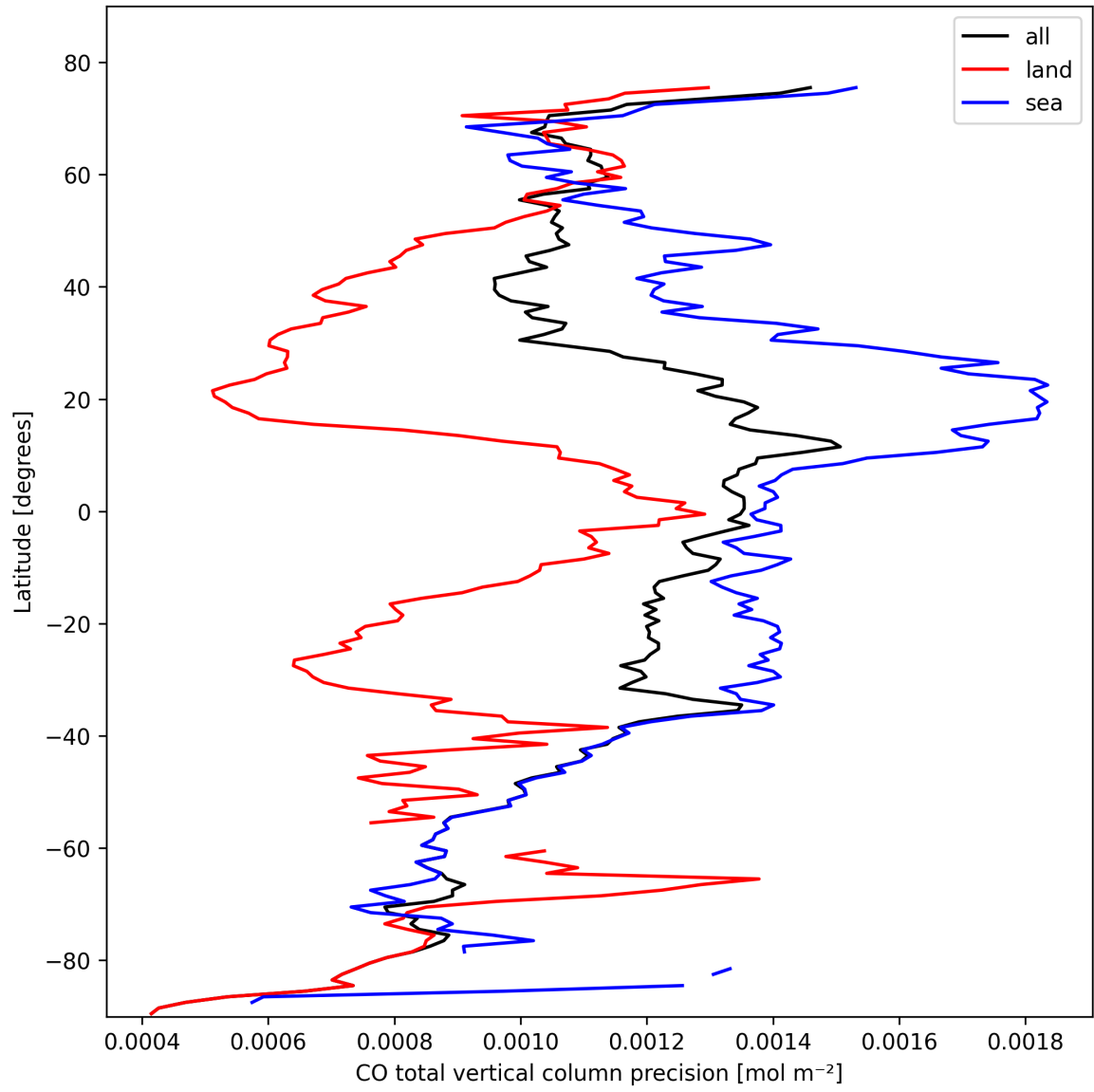
Figure 8: Zonal average of “CO total vertical column precision” for 2025-10-17 to 2025-10-18.
