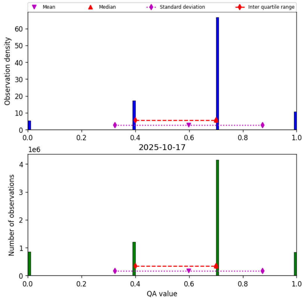
Figure 13: Histogram of “QA value” for 2025-10-17 to 2025-10-18
