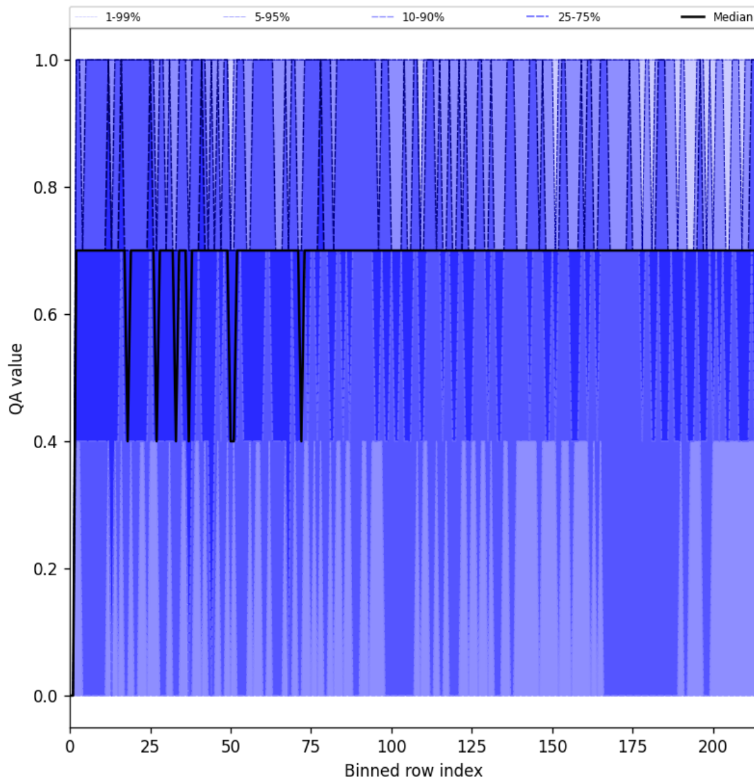
Figure 20: Along track statistics of “QA value” for 2025-10-17 to 2025-10-18
