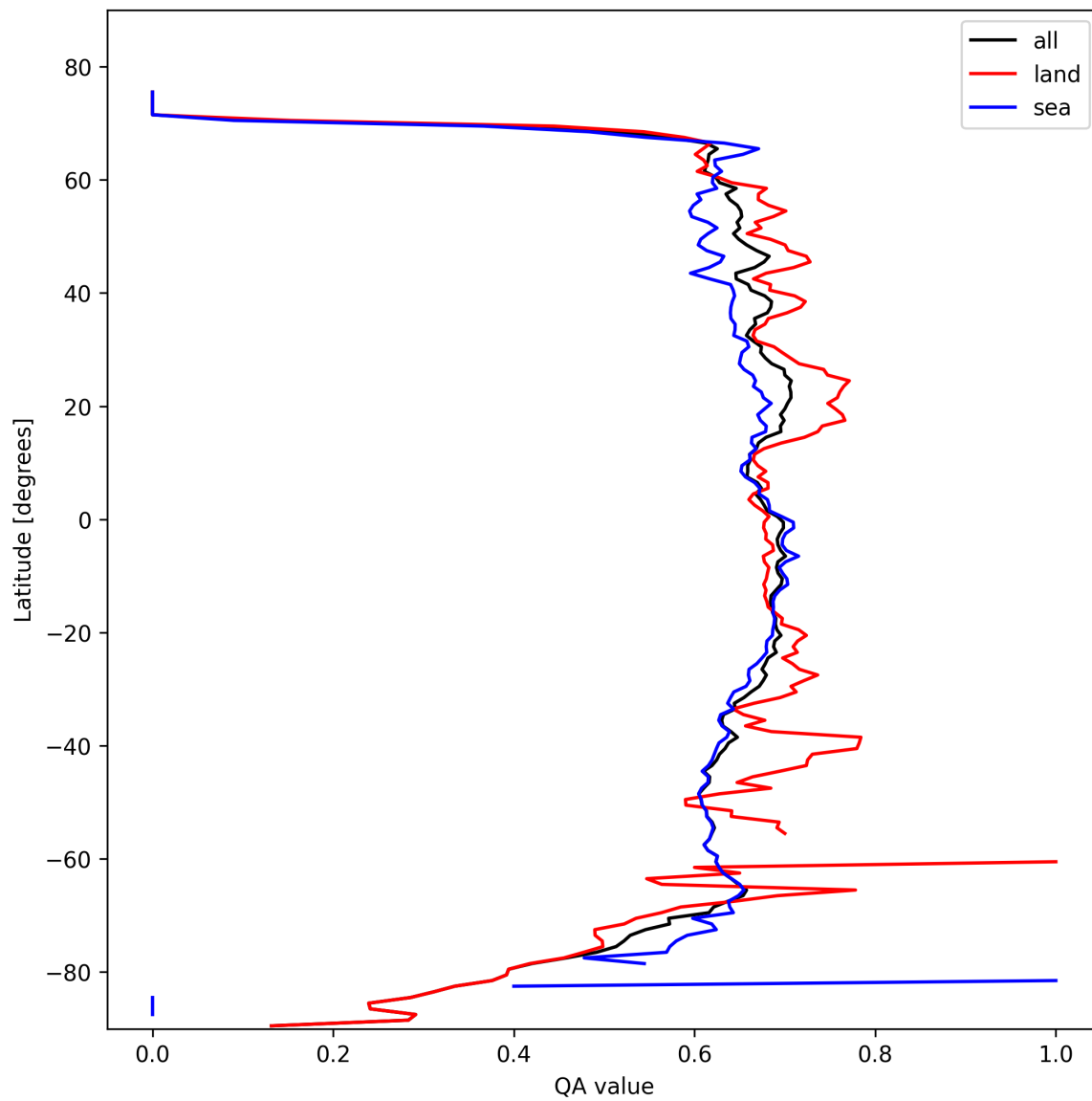
Figure 6: Zonal average of “QA value” for 2025-10-17 to 2025-10-18.
