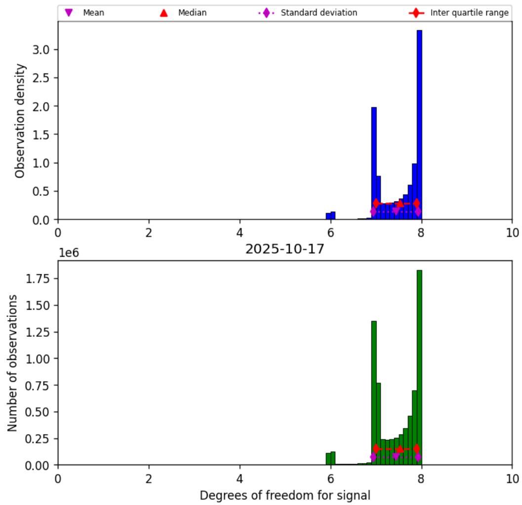
Figure 18: Histogram of “Degrees of freedom for signal” for 2025-10-17 to 2025-10-18
