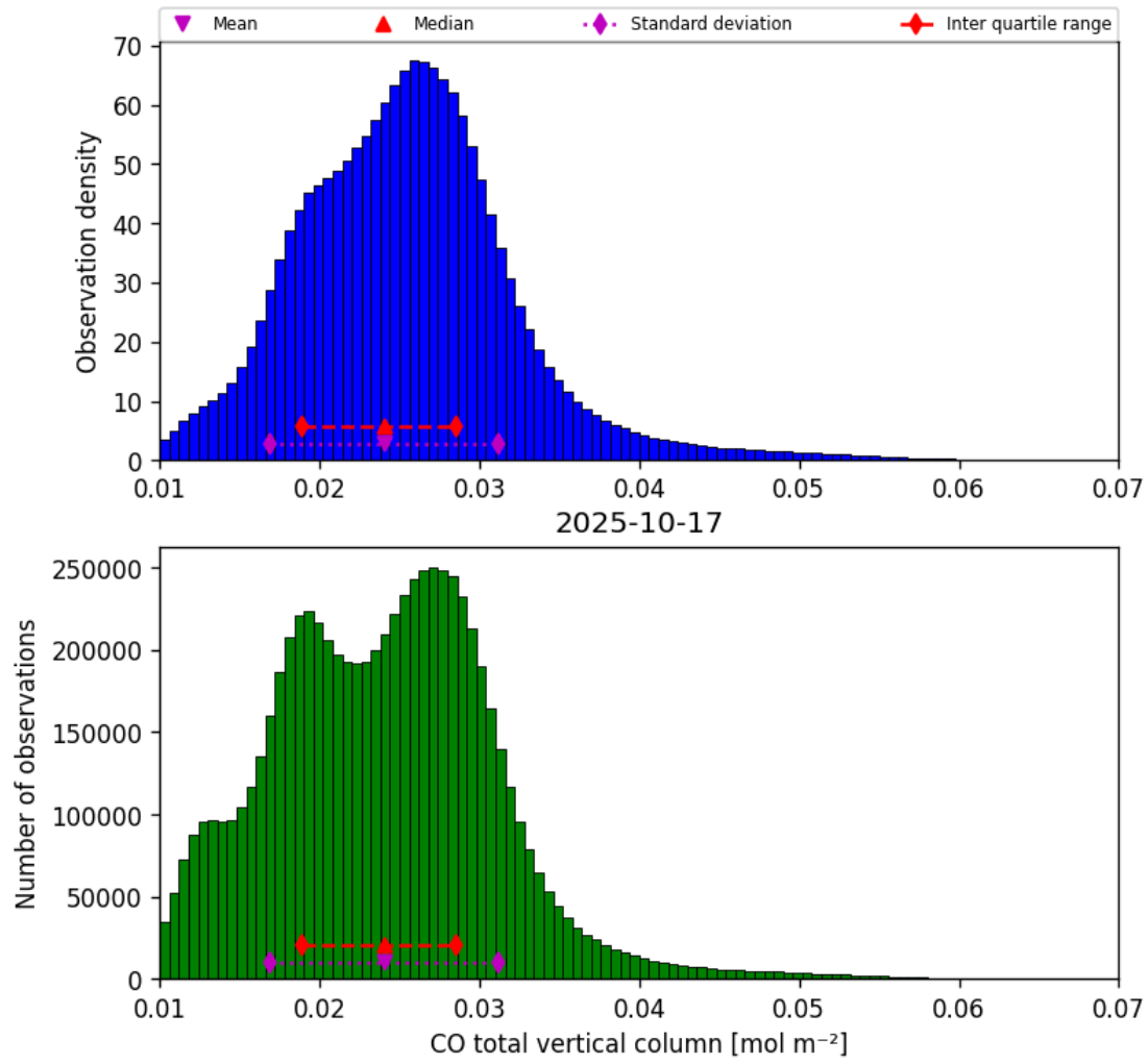
Figure 14: Histogram of “CO total vertical column” for 2025-10-17 to 2025-10-18
