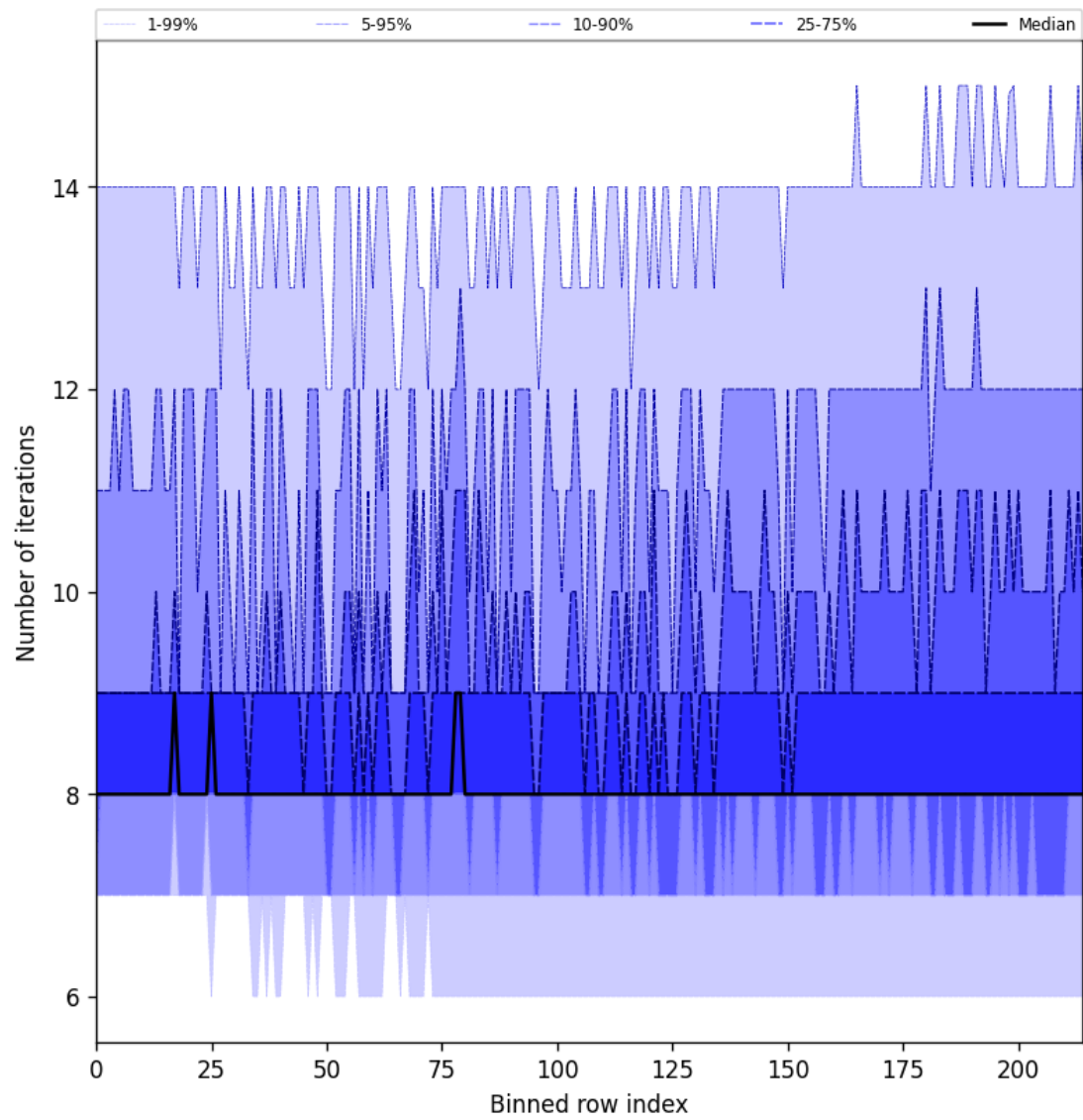
Figure 26: Along track statistics of “Number of iterations” for 2025-10-17 to 2025-10-18
