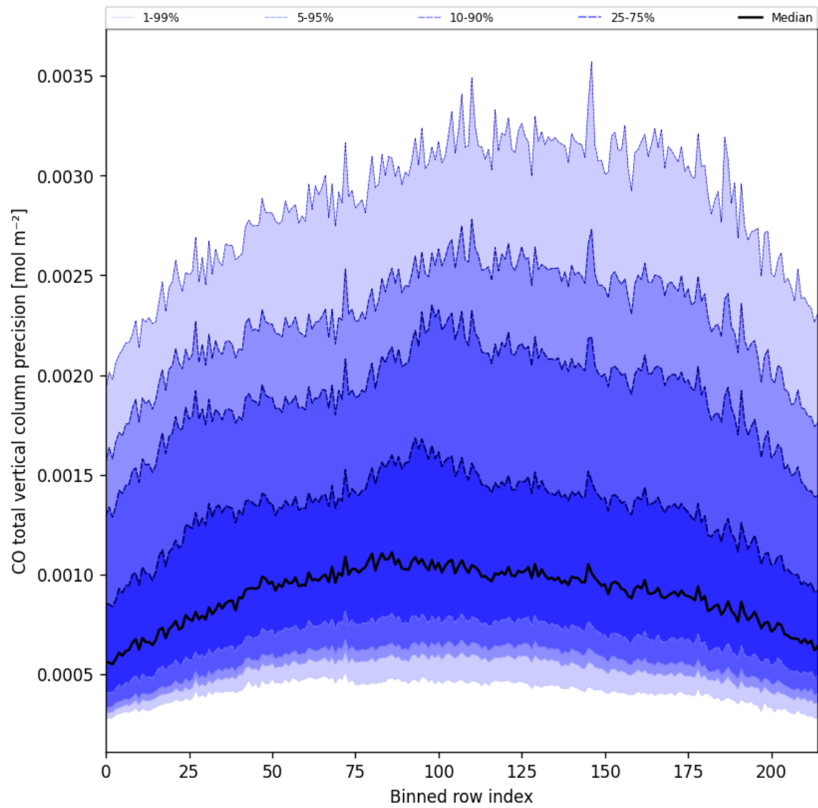
Figure 22: Along track statistics of “CO total vertical column precision” for 2025-10-17 to 2025-10-18
