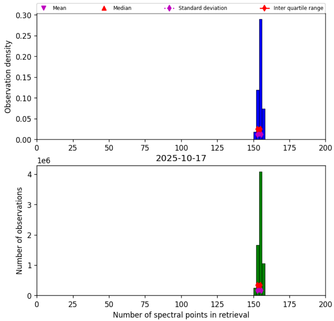
Figure 16: Histogram of “Number of spectral points in retrieval” for 2025-10-17 to 2025-10-18
