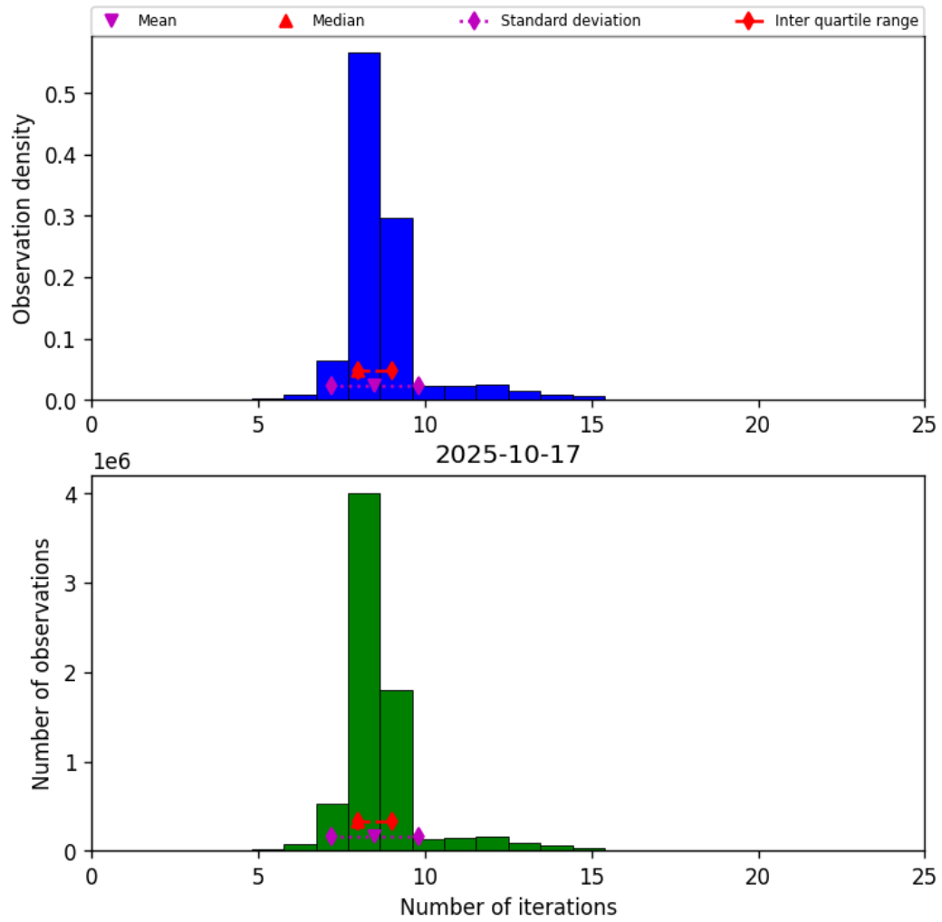
Figure 19: Histogram of “Number of iterations” for 2025-10-17 to 2025-10-18
