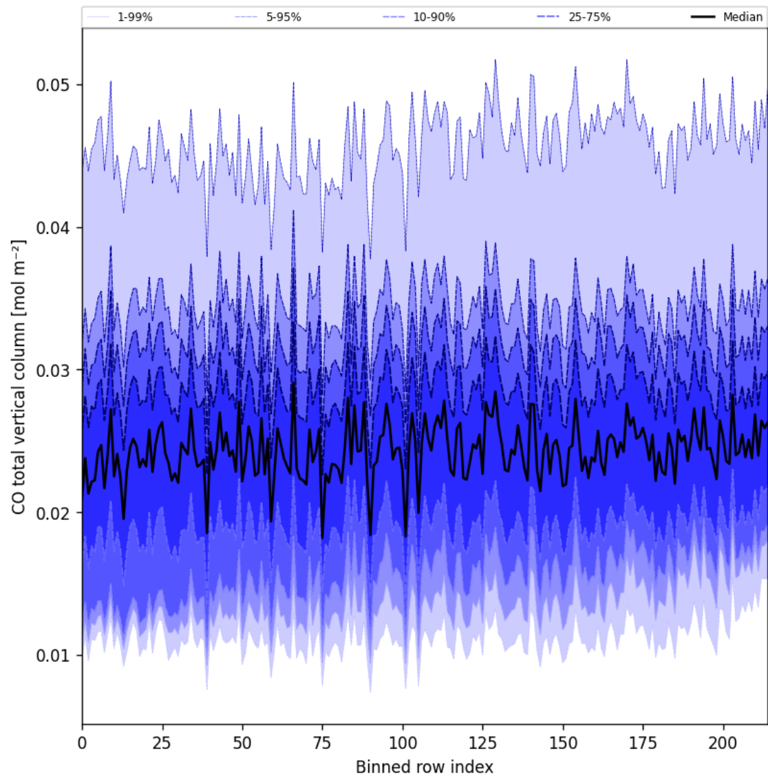
Figure 21: Along track statistics of “CO total vertical column” for 2025-10-17 to 2025-10-18
