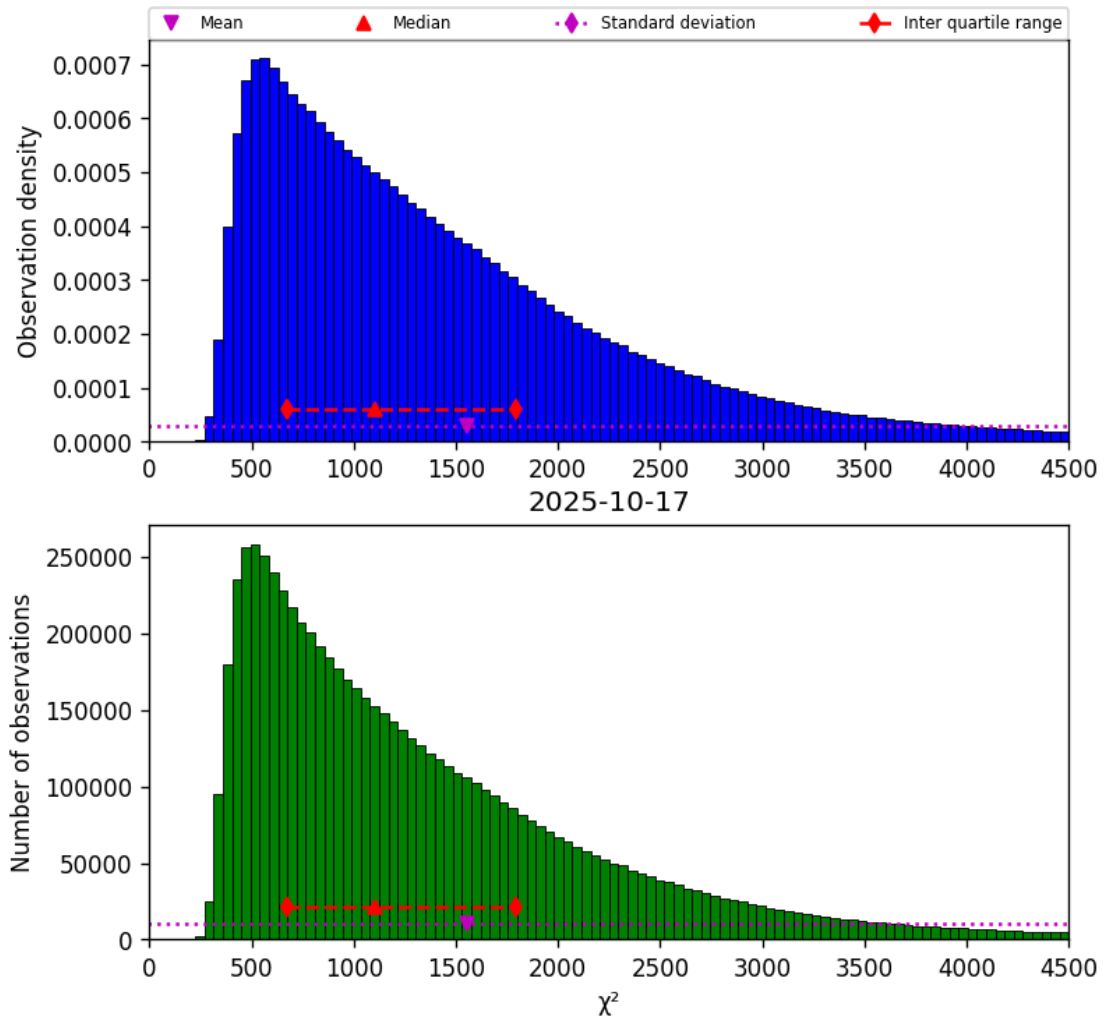
Figure 17: Histogram of “ \chi^2 ” for 2025-10-17 to 2025-10-18
