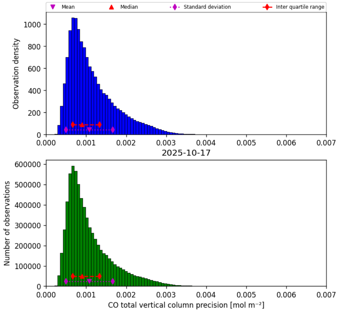
Figure 15: Histogram of “CO total vertical column precision” for 2025-10-17 to 2025-10-18
