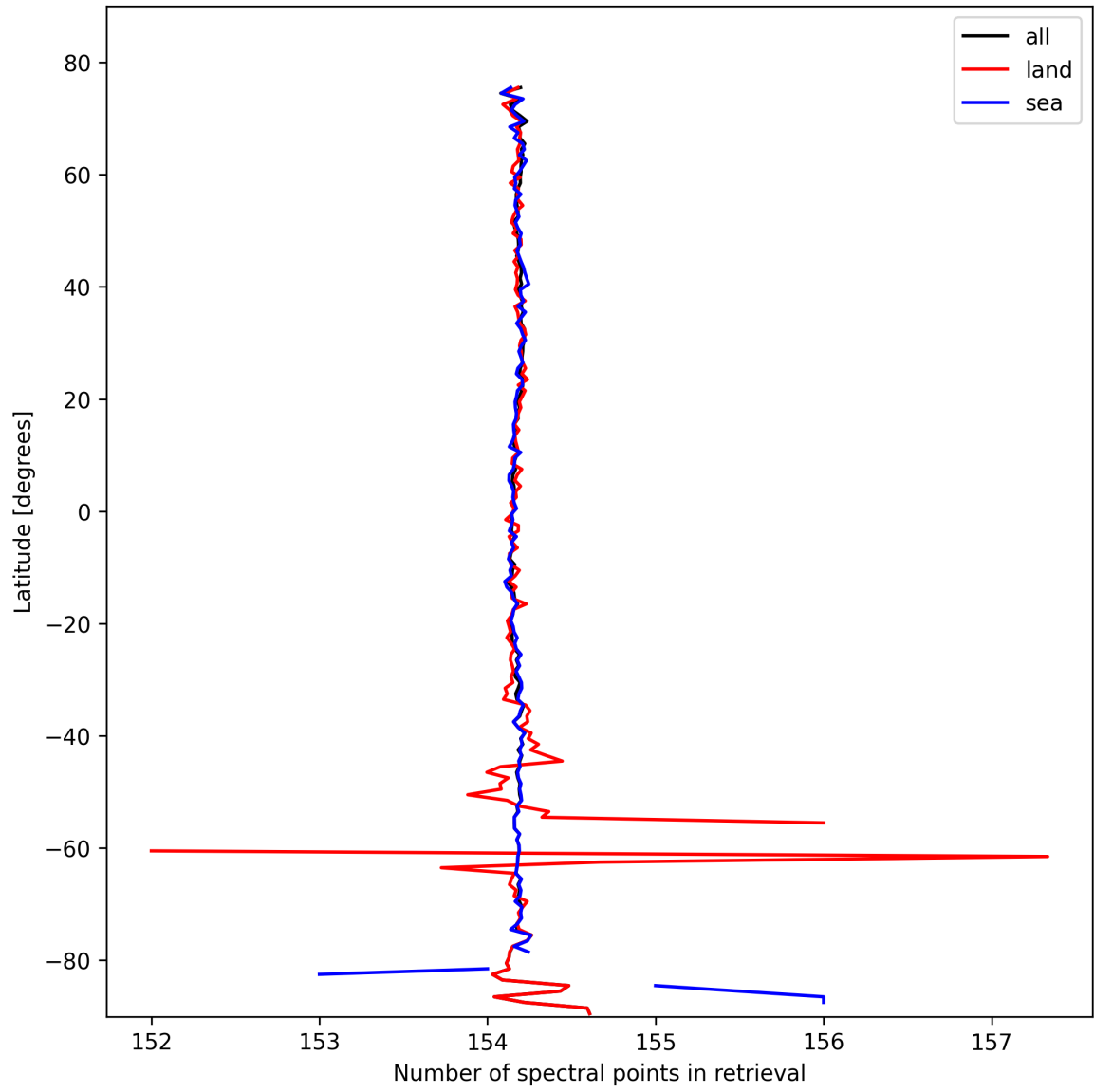
Figure 9: Zonal average of “Number of spectral points in retrieval” for 2025-10-17 to 2025-10-18.
