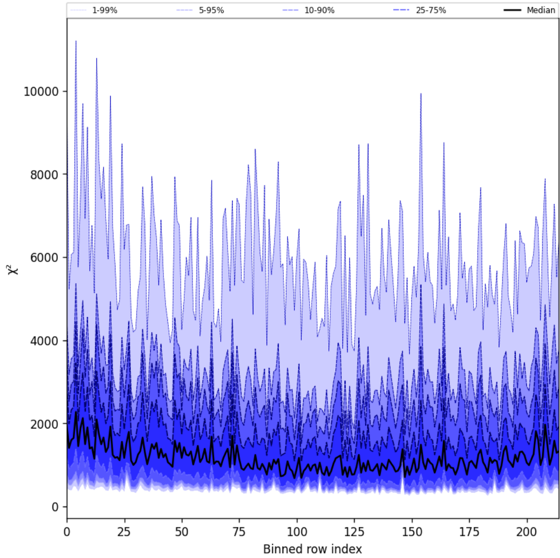
Figure 24: Along track statistics of “ \chi^2 ” for 2025-10-17 to 2025-10-18
