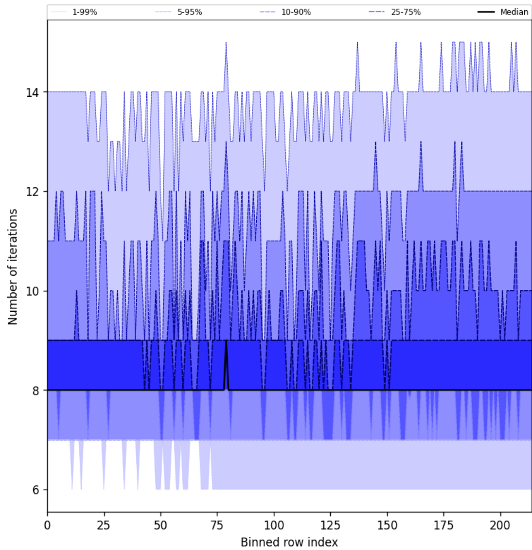
Figure 26: Along track statistics of “Number of iterations” for 2025-10-19 to 2025-10-20
