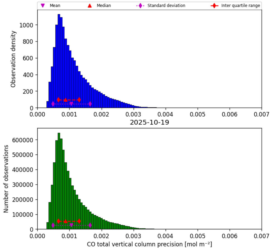
Figure 15: Histogram of “CO total vertical column precision” for 2025-10-19 to 2025-10-20
