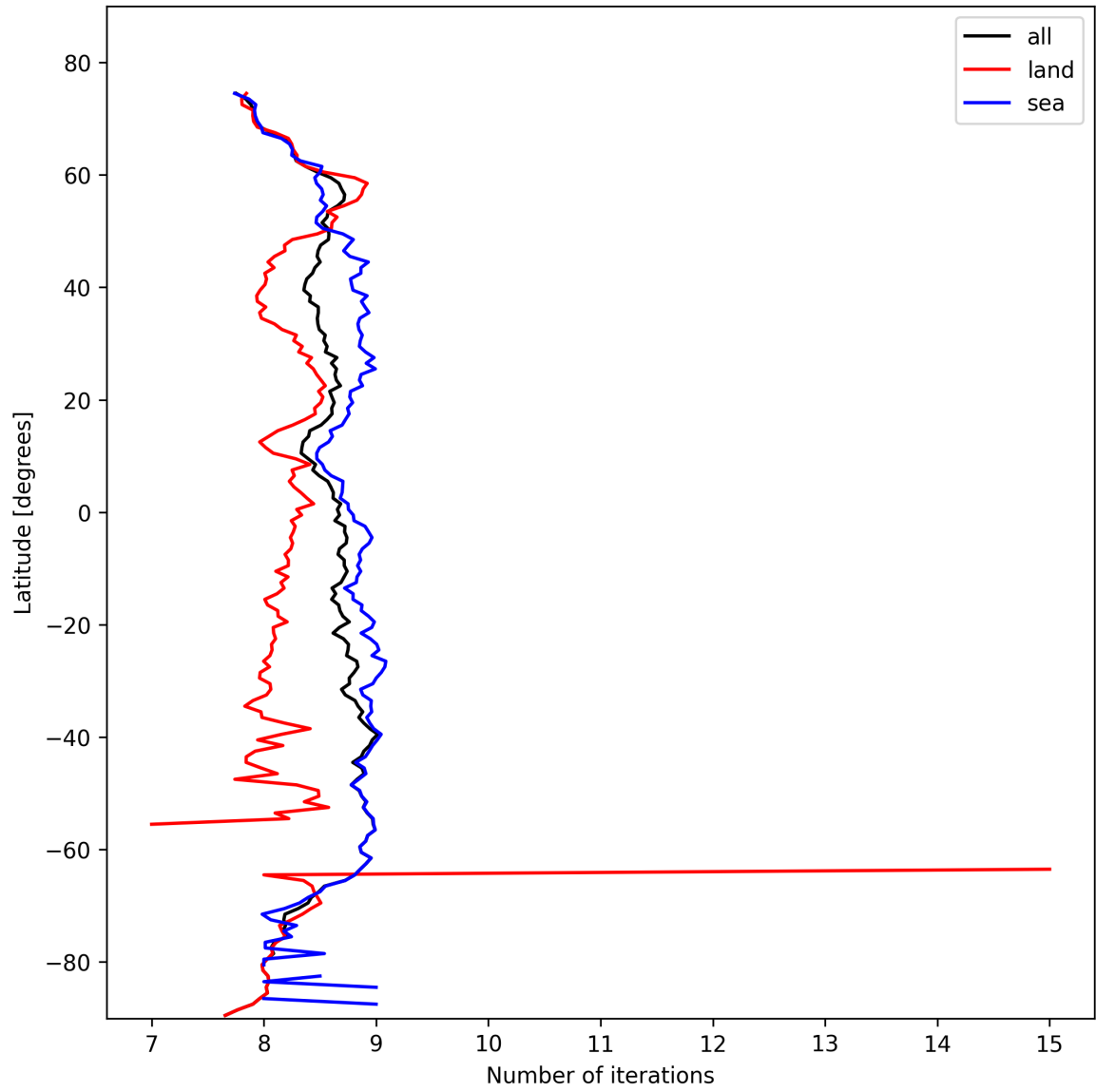
Figure 12: Zonal average of “Number of iterations” for 2025-10-19 to 2025-10-20.
