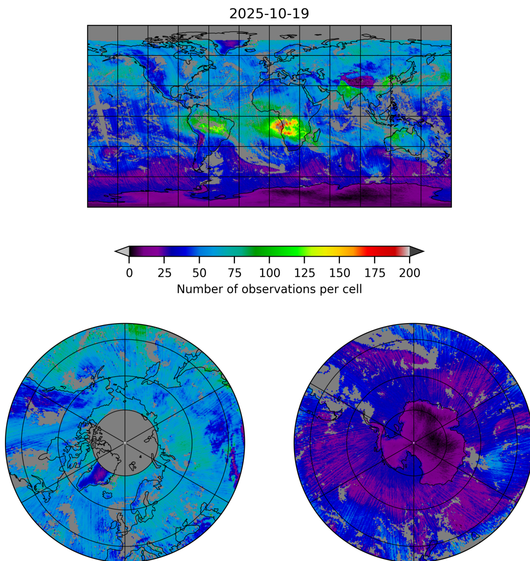
Figure 5: Map of the number of observations for 2025-10-19 to 2025-10-20
