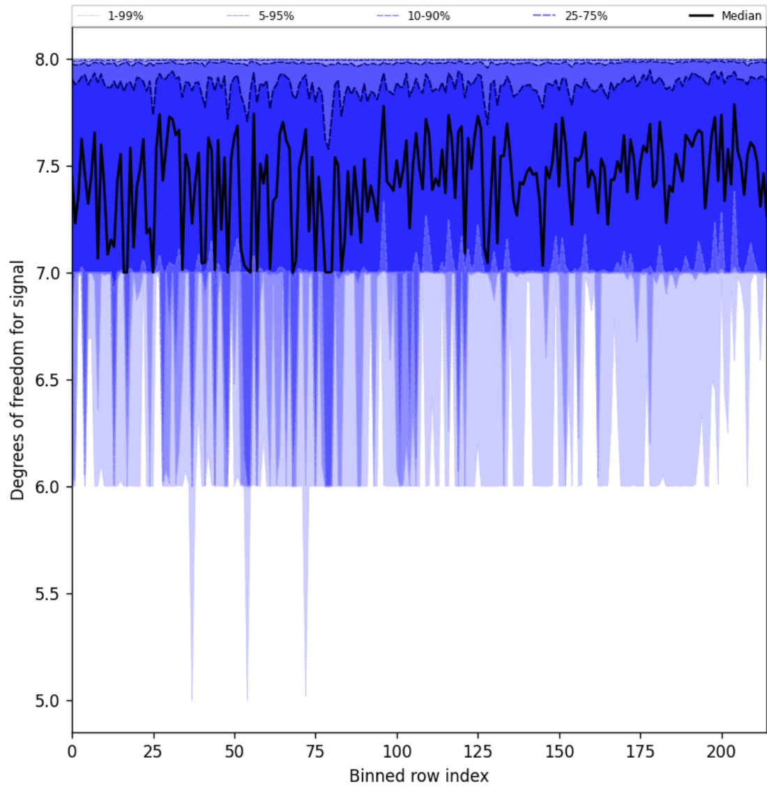
Figure 25: Along track statistics of “Degrees of freedom for signal” for 2025-10-19 to 2025-10-20
