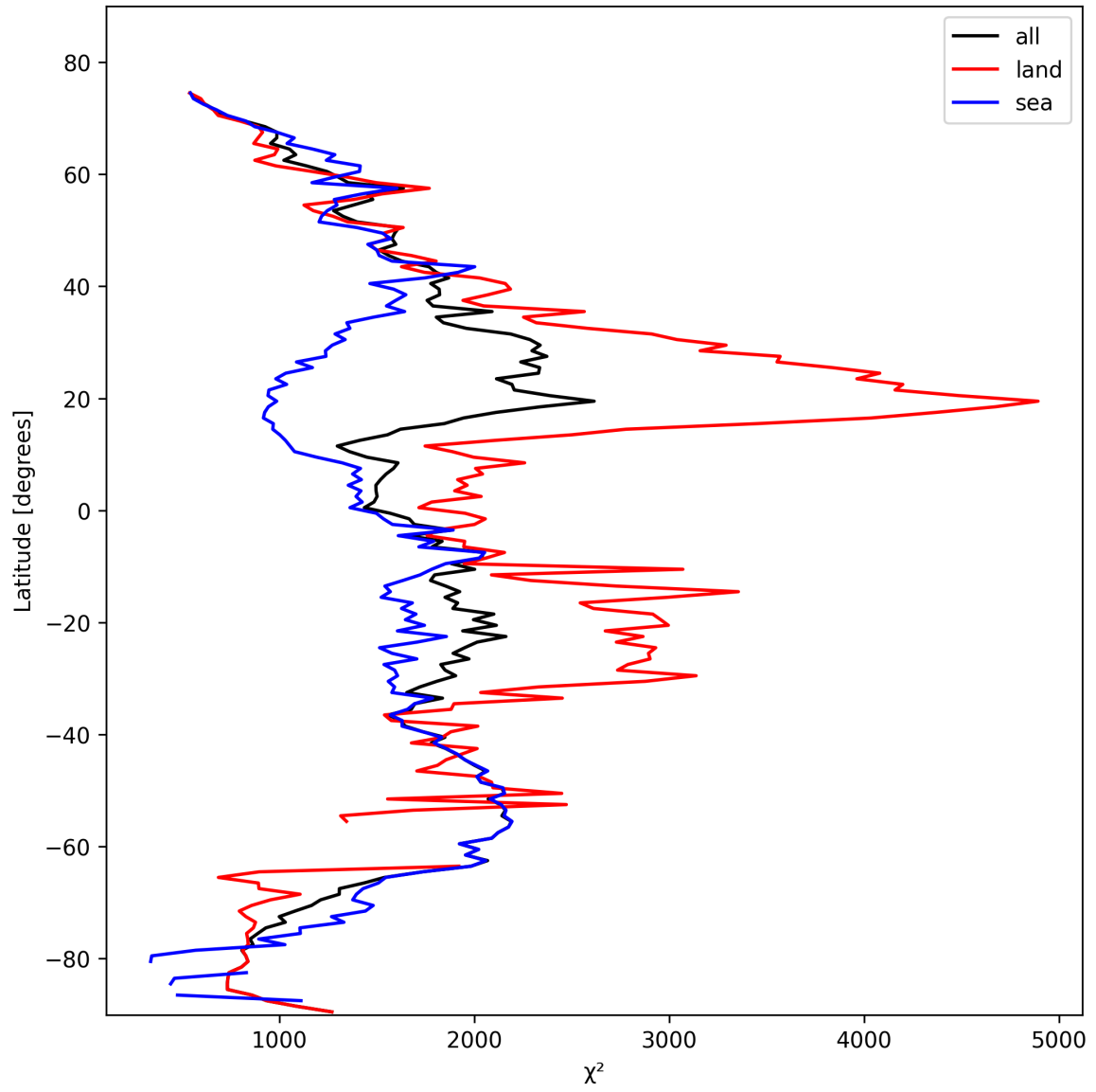
Figure 10: Zonal average of “ \chi^2 ” for 2025-10-19 to 2025-10-20.
