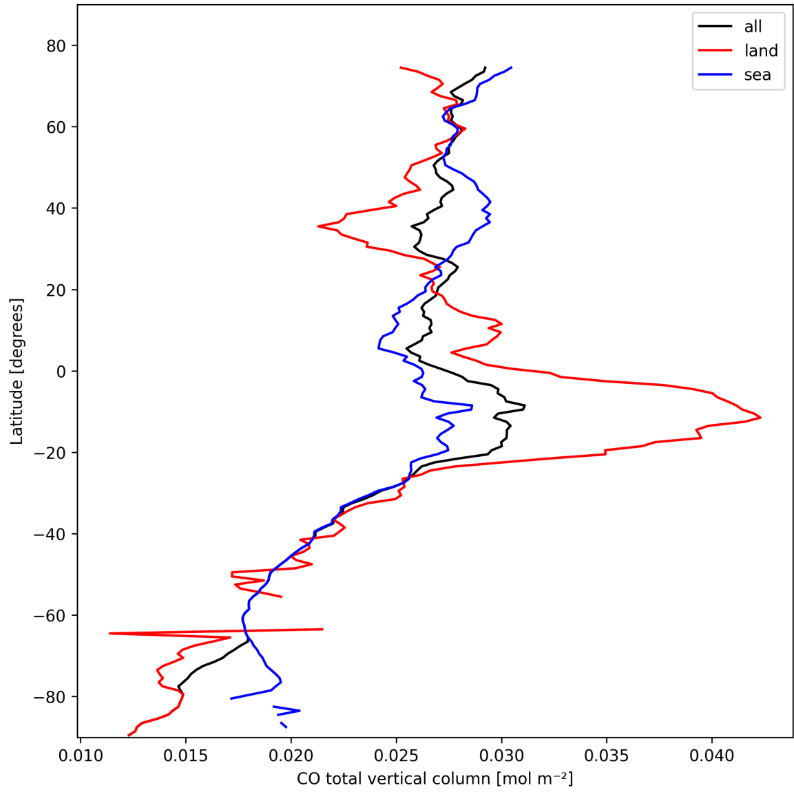
Figure 7: Zonal average of “CO total vertical column” for 2025-10-19 to 2025-10-20.
