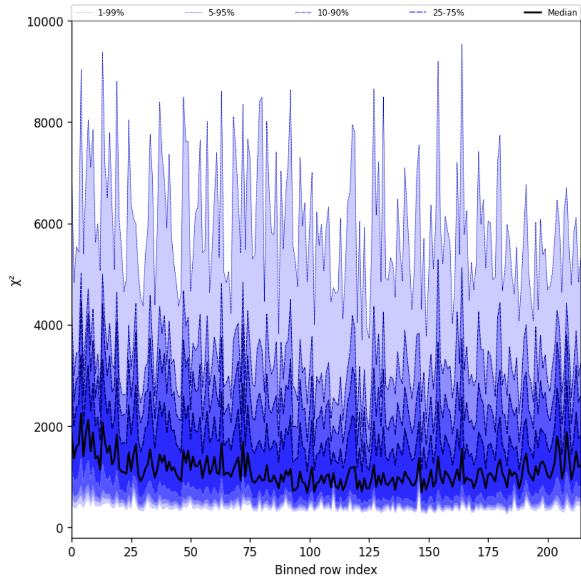
Figure 24: Along track statistics of “ \chi^2 ” for 2025-10-19 to 2025-10-20
