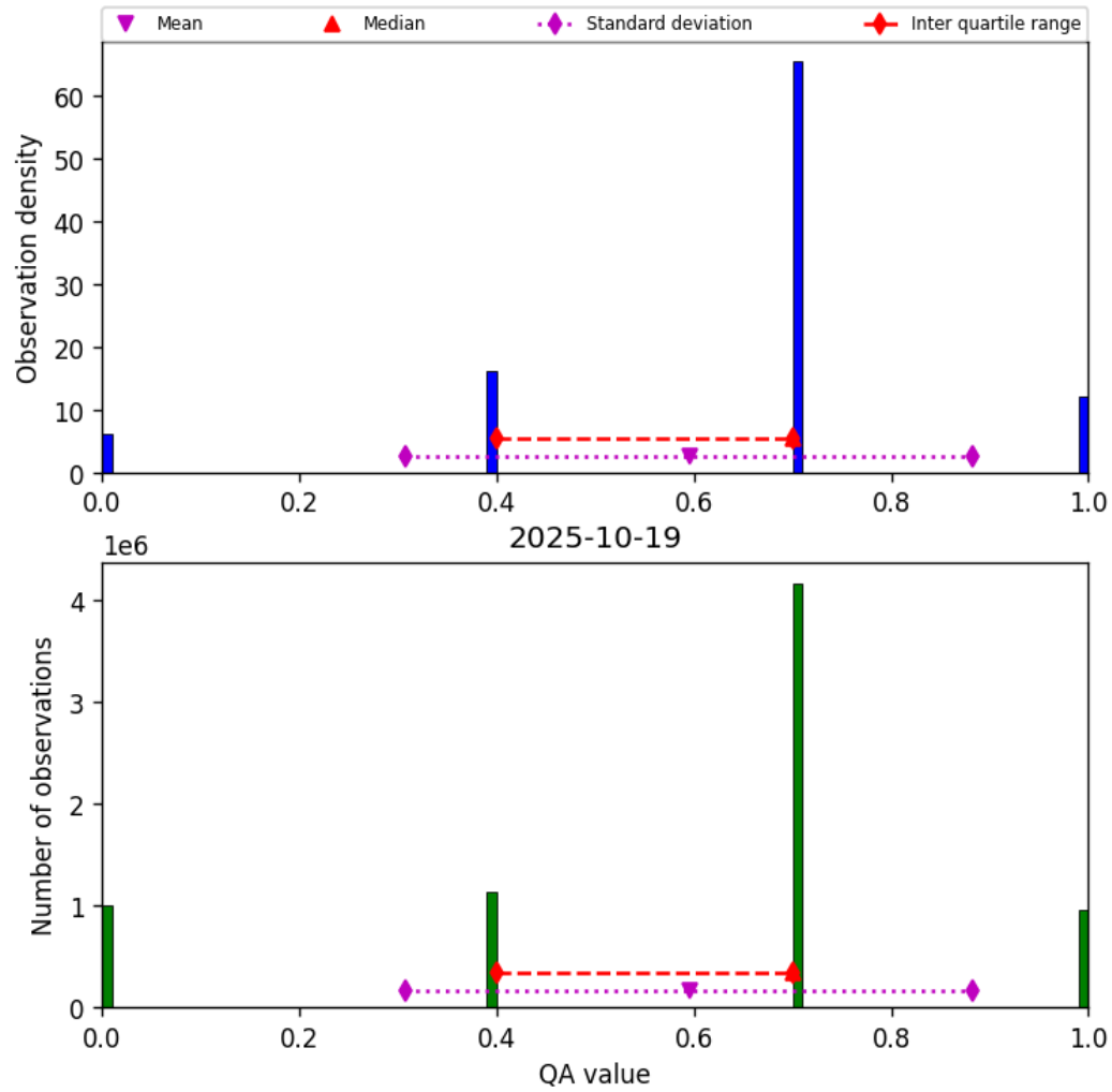
Figure 13: Histogram of “QA value” for 2025-10-19 to 2025-10-20
