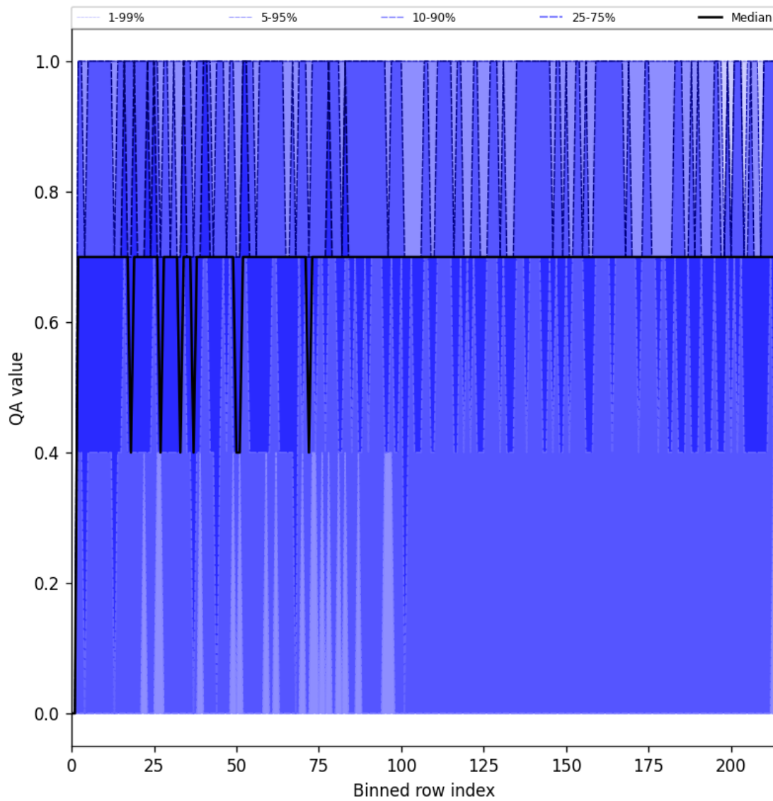
Figure 20: Along track statistics of “QA value” for 2025-10-19 to 2025-10-20
