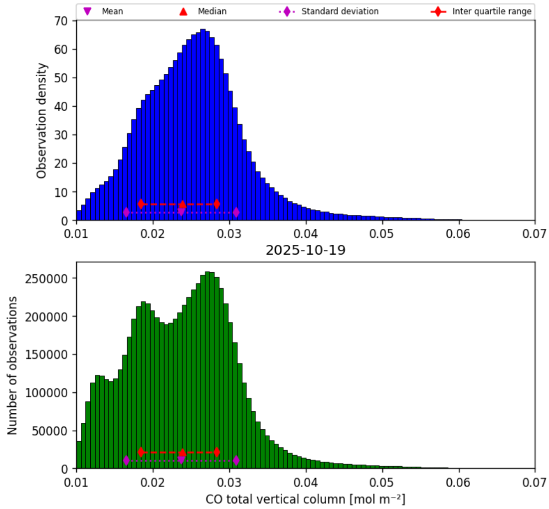
Figure 14: Histogram of “CO total vertical column” for 2025-10-19 to 2025-10-20
