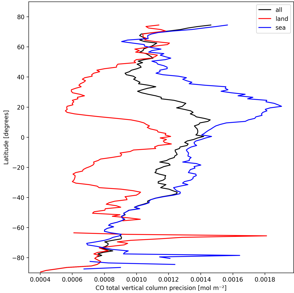
Figure 8: Zonal average of “CO total vertical column precision” for 2025-10-19 to 2025-10-20.
