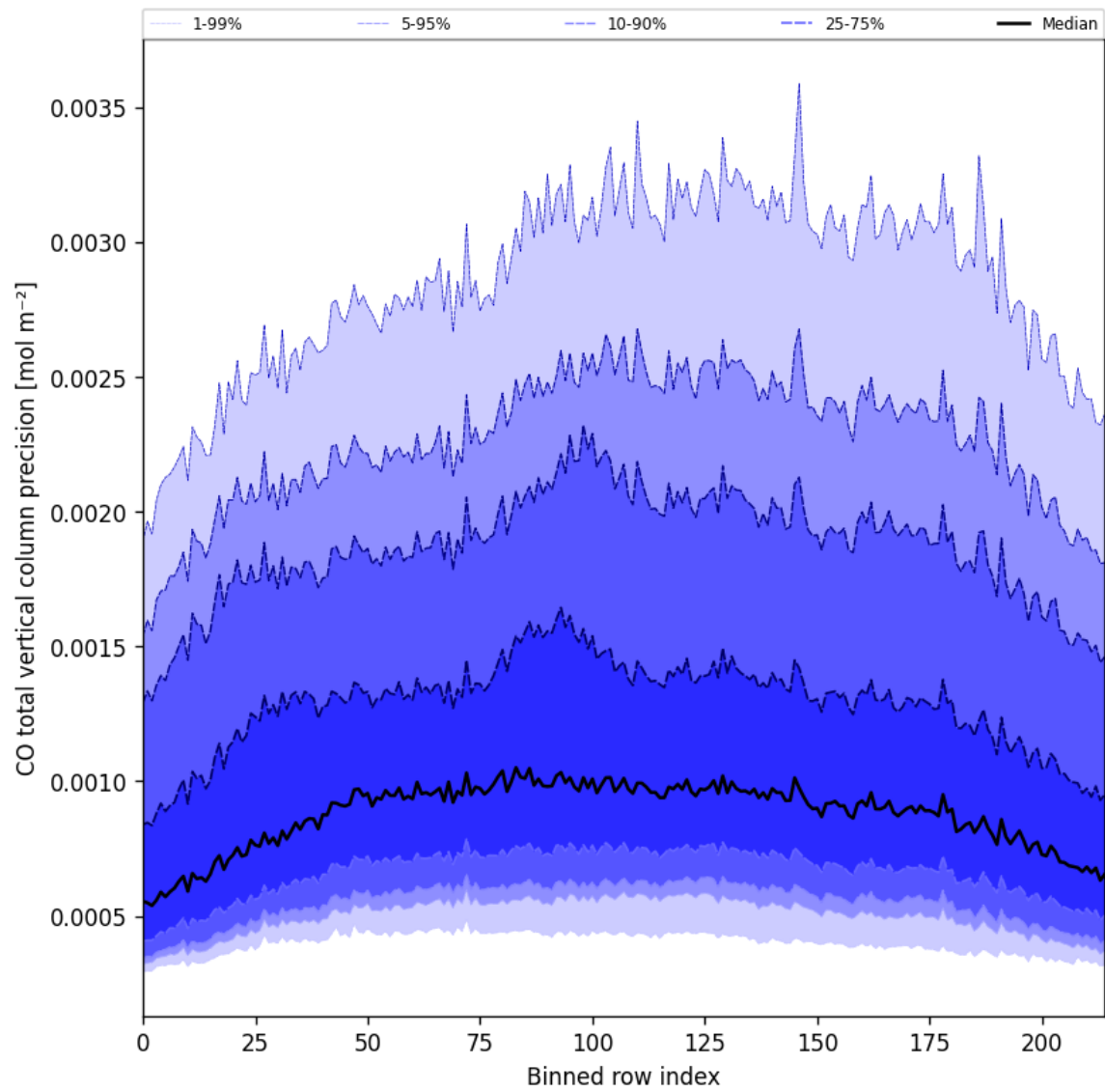
Figure 22: Along track statistics of “CO total vertical column precision” for 2025-10-19 to 2025-10-20
