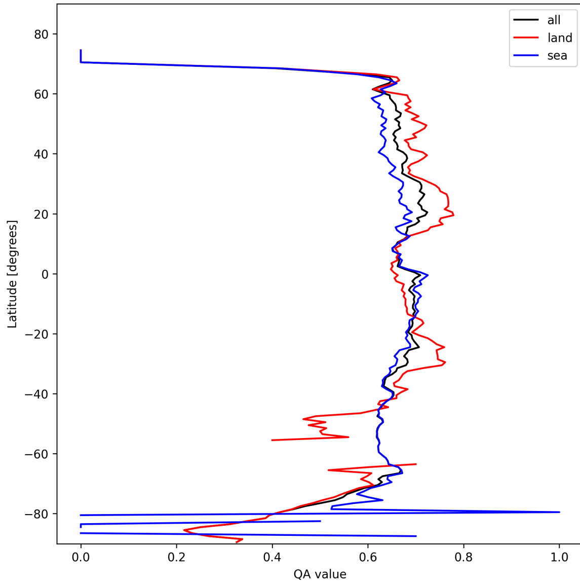
Figure 6: Zonal average of “QA value” for 2025-10-19 to 2025-10-20.
