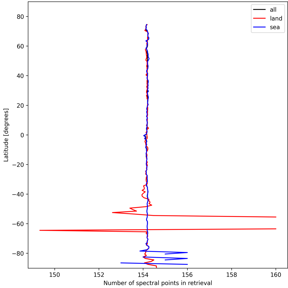
Figure 9: Zonal average of “Number of spectral points in retrieval” for 2025-10-19 to 2025-10-20.
