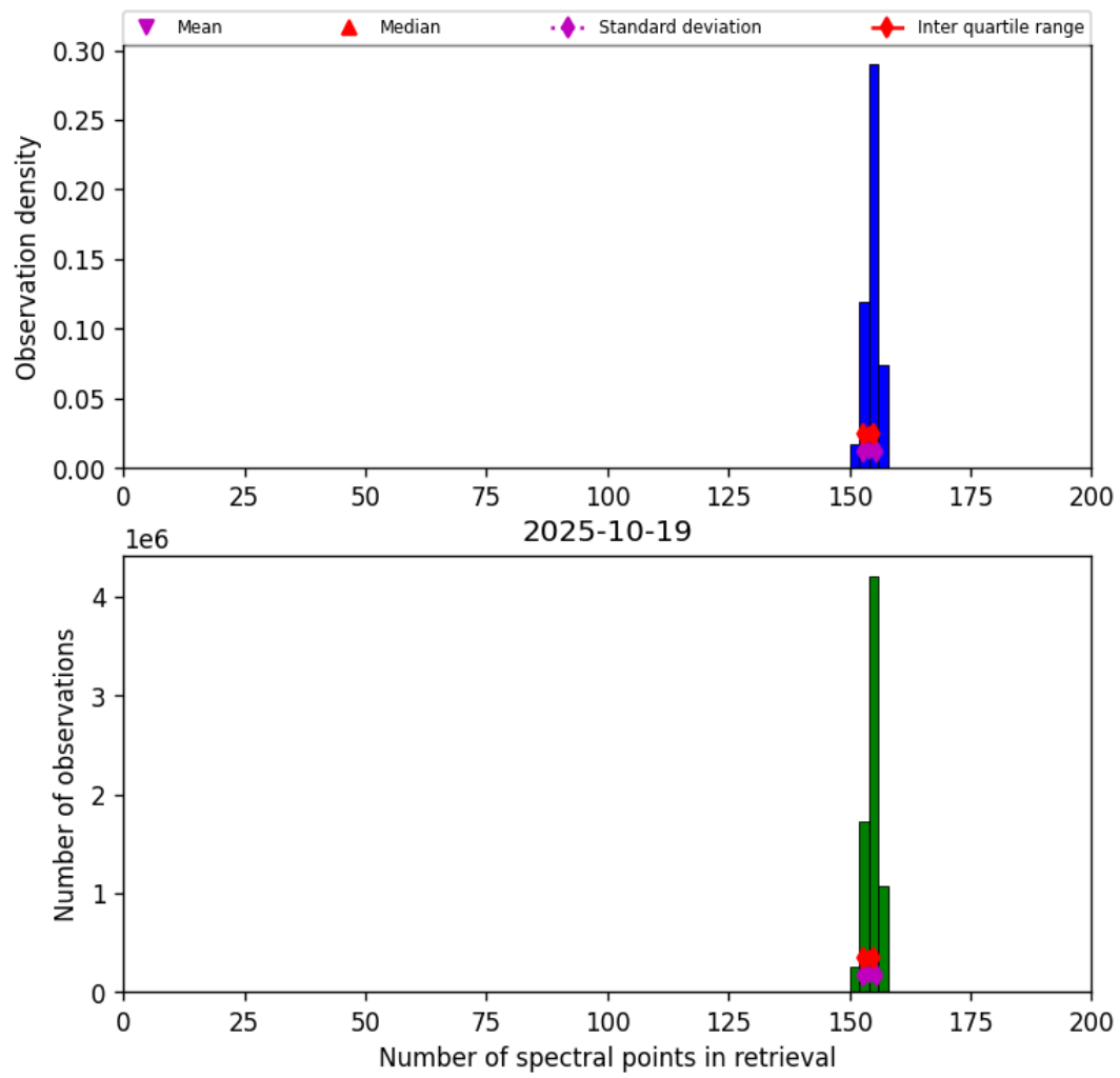
Figure 16: Histogram of “Number of spectral points in retrieval” for 2025-10-19 to 2025-10-20
