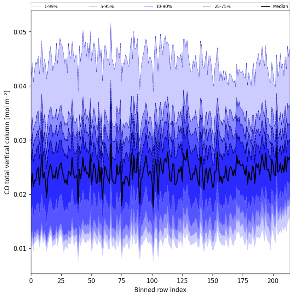
Figure 21: Along track statistics of “CO total vertical column” for 2025-10-19 to 2025-10-20
