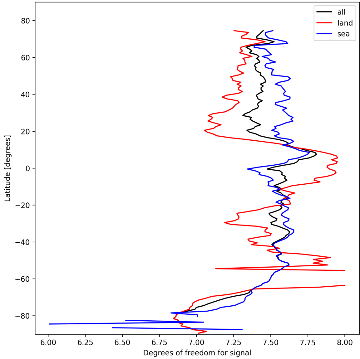
Figure 11: Zonal average of “Degrees of freedom for signal” for 2025-10-19 to 2025-10-20.
