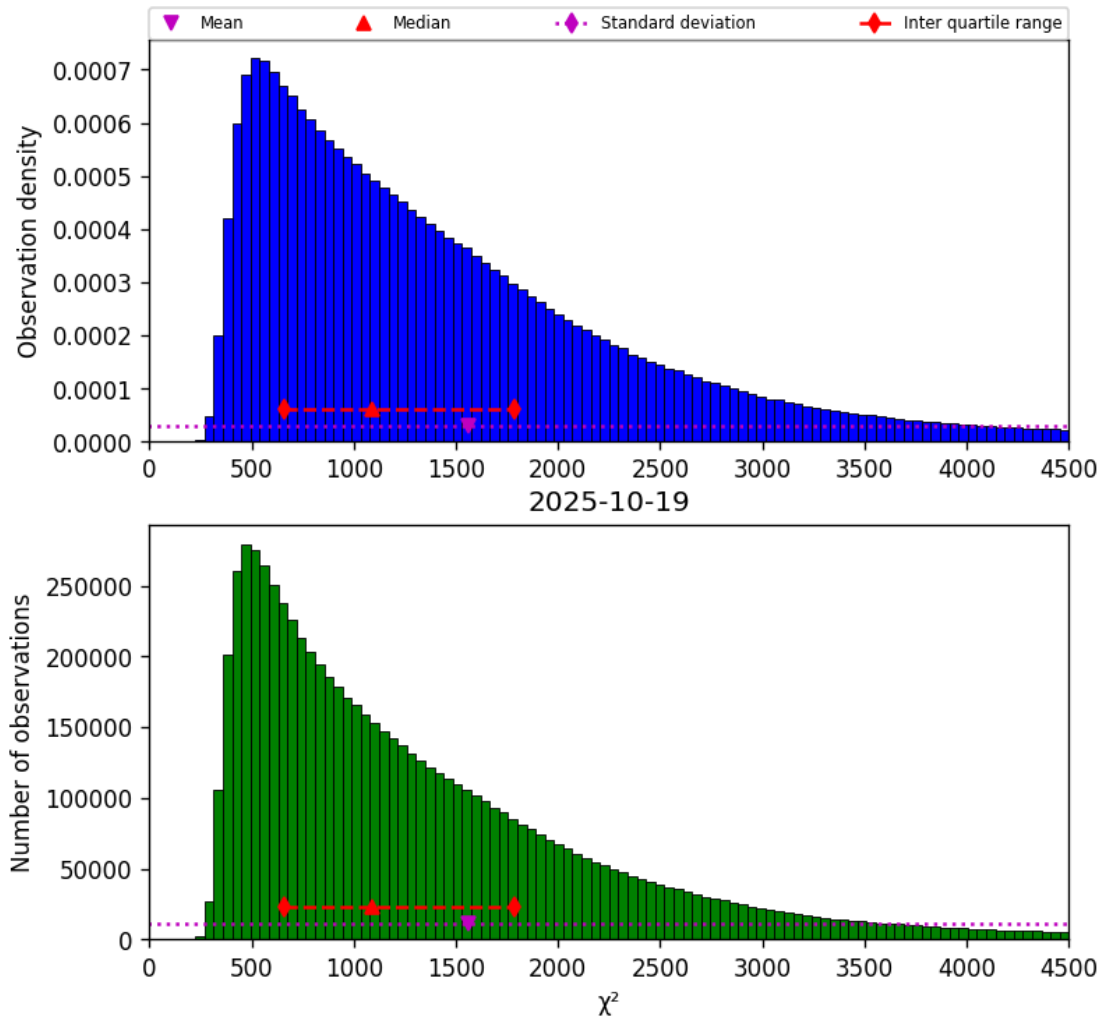
Figure 17: Histogram of “ \chi^2 ” for 2025-10-19 to 2025-10-20
