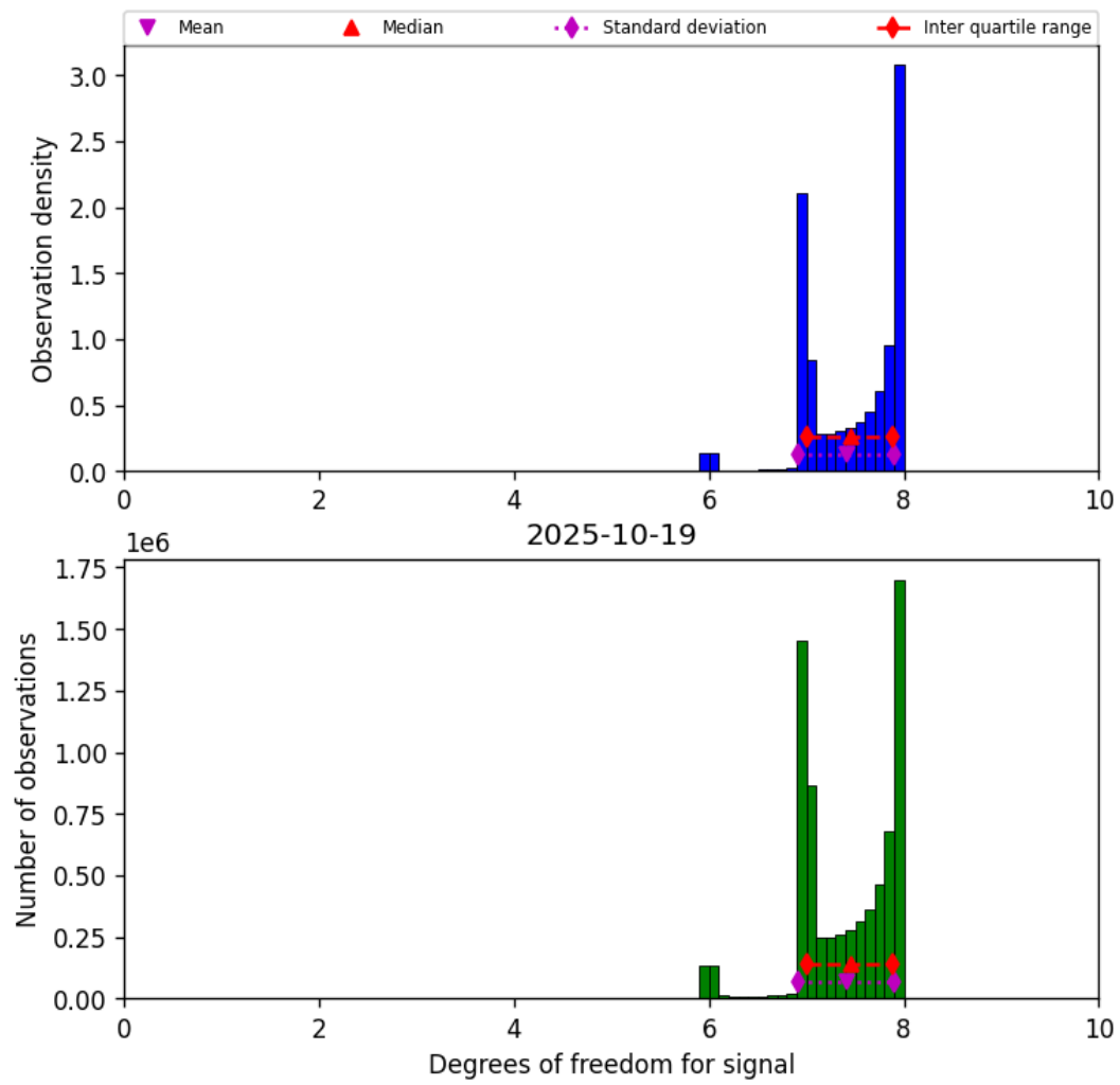
Figure 18: Histogram of “Degrees of freedom for signal” for 2025-10-19 to 2025-10-20
