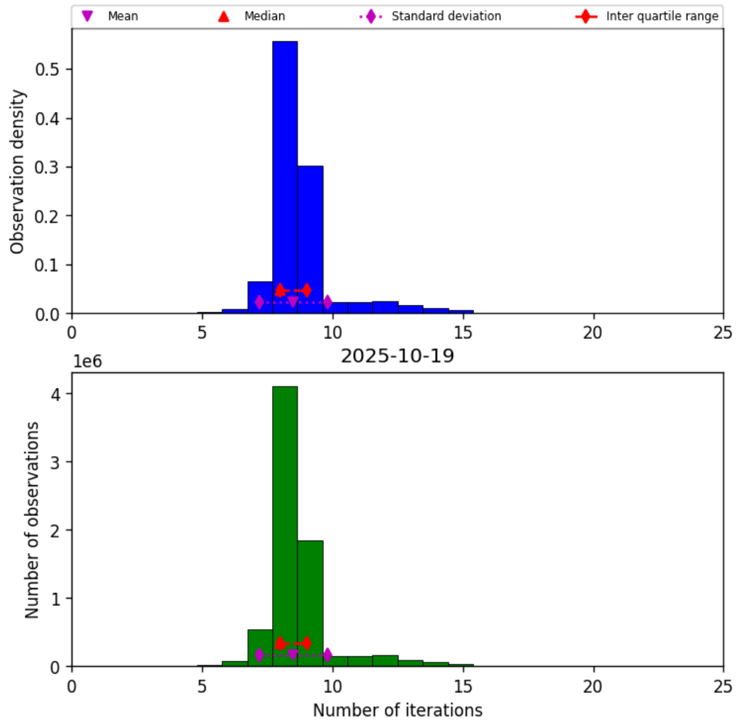
Figure 19: Histogram of “Number of iterations” for 2025-10-19 to 2025-10-20
