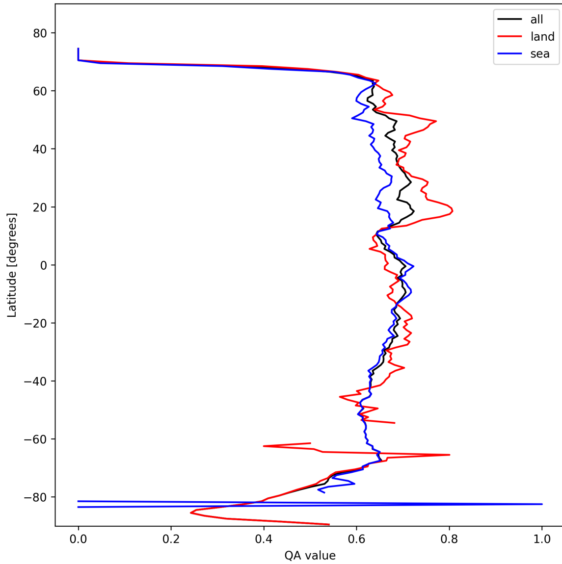
Figure 6: Zonal average of “QA value” for 2025-10-20 to 2025-10-20.
