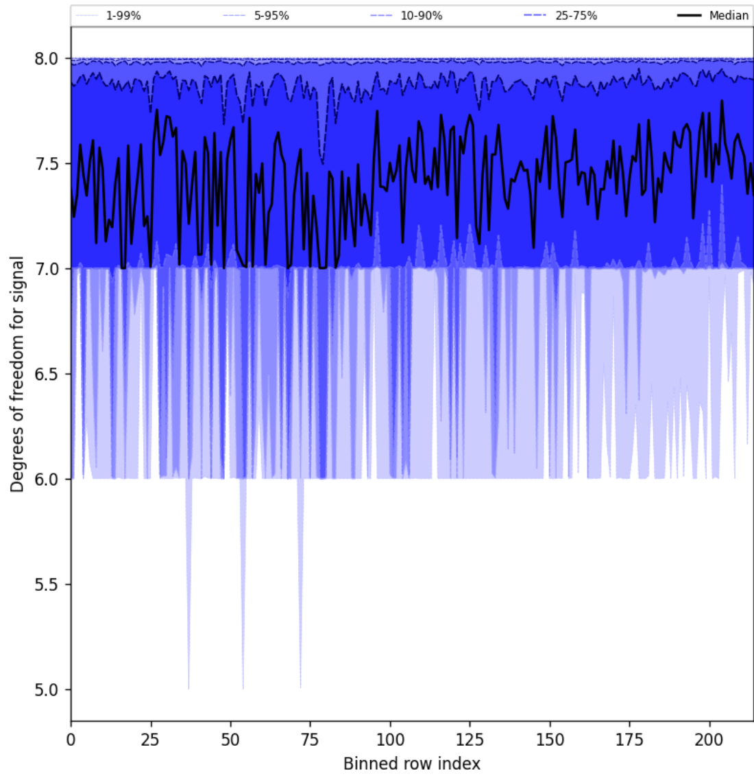
Figure 25: Along track statistics of “Degrees of freedom for signal” for 2025-10-20 to 2025-10-20
