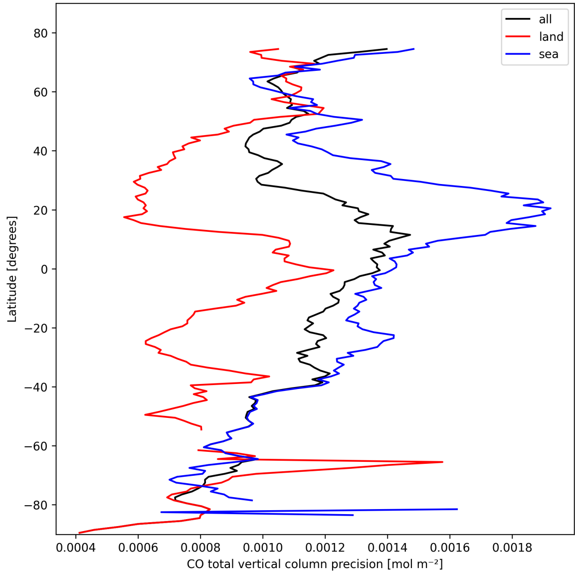
Figure 8: Zonal average of “CO total vertical column precision” for 2025-10-20 to 2025-10-20.
