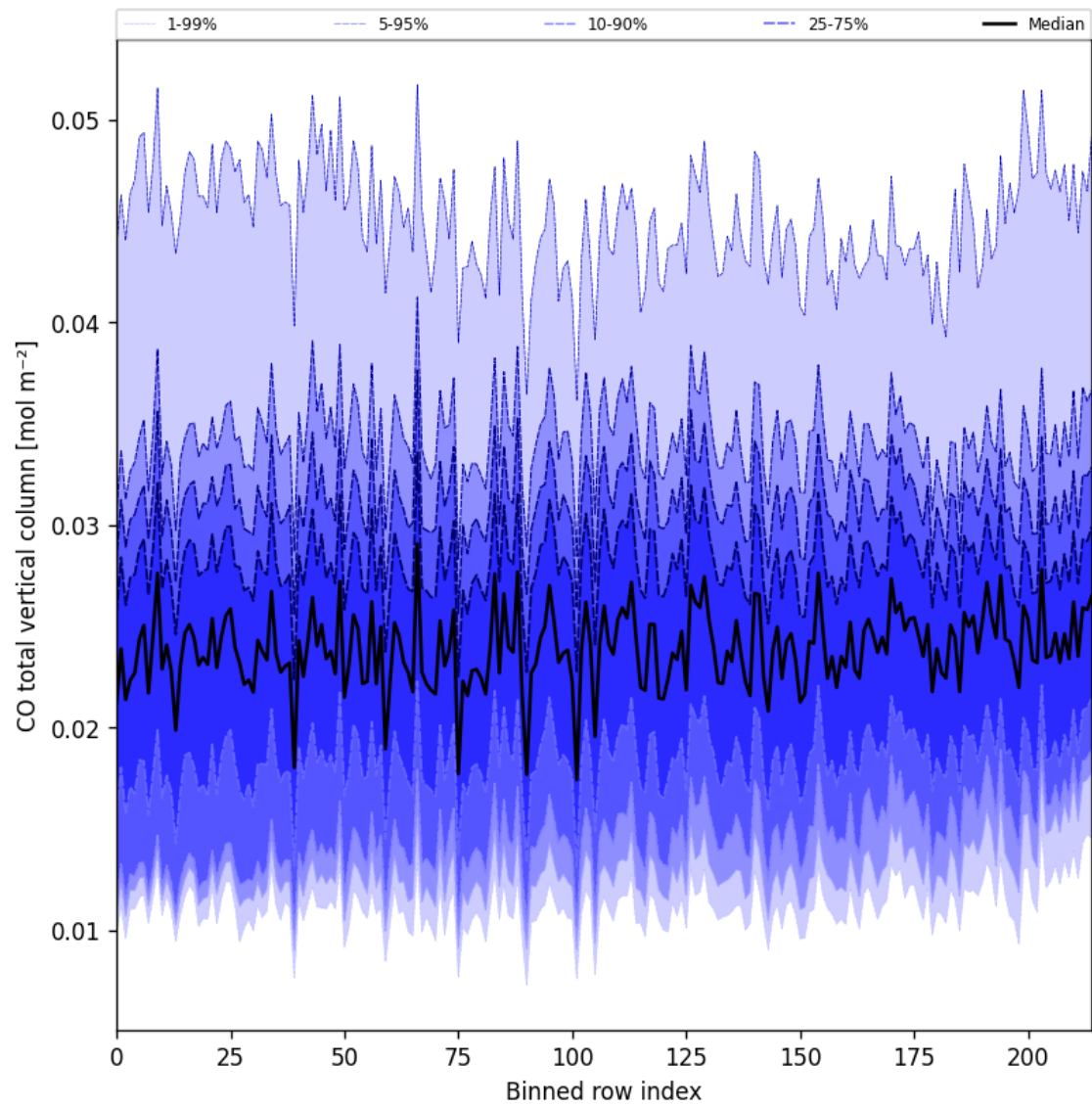
Figure 21: Along track statistics of “CO total vertical column” for 2025-10-20 to 2025-10-20
