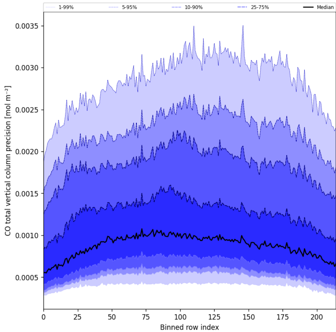
Figure 22: Along track statistics of “CO total vertical column precision” for 2025-10-20 to 2025-10-20
