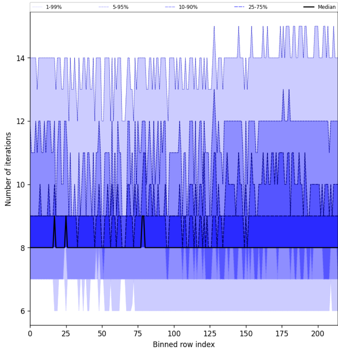
Figure 26: Along track statistics of “Number of iterations” for 2025-10-20 to 2025-10-20
