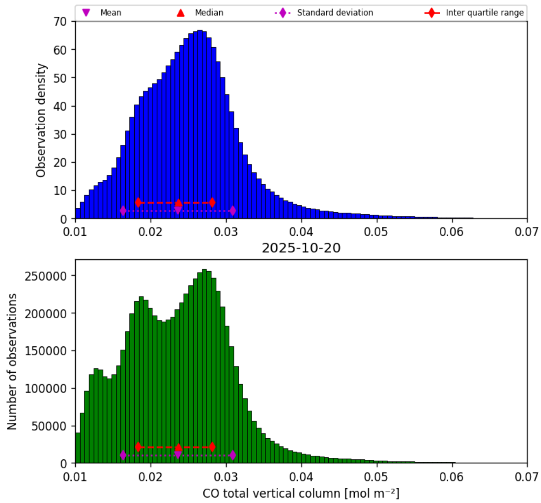
Figure 14: Histogram of “CO total vertical column” for 2025-10-20 to 2025-10-20
