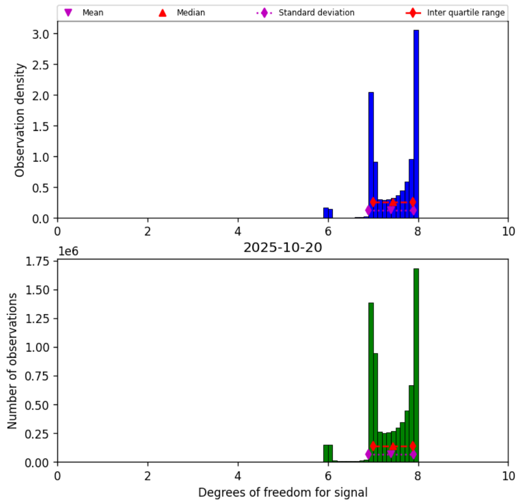
Figure 18: Histogram of “Degrees of freedom for signal” for 2025-10-20 to 2025-10-20
