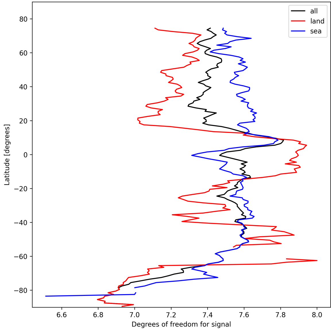
Figure 11: Zonal average of “Degrees of freedom for signal” for 2025-10-20 to 2025-10-20.
