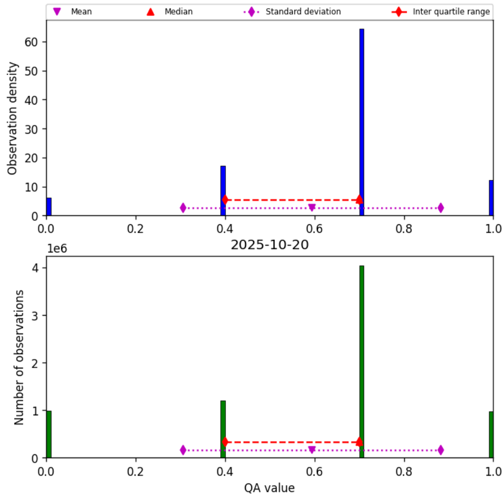
Figure 13: Histogram of “QA value” for 2025-10-20 to 2025-10-20
