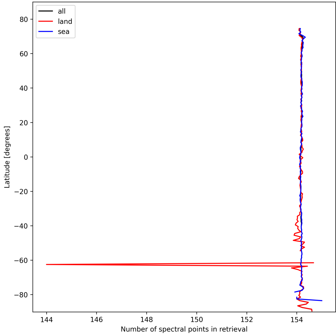
Figure 9: Zonal average of “Number of spectral points in retrieval” for 2025-10-20 to 2025-10-20.
