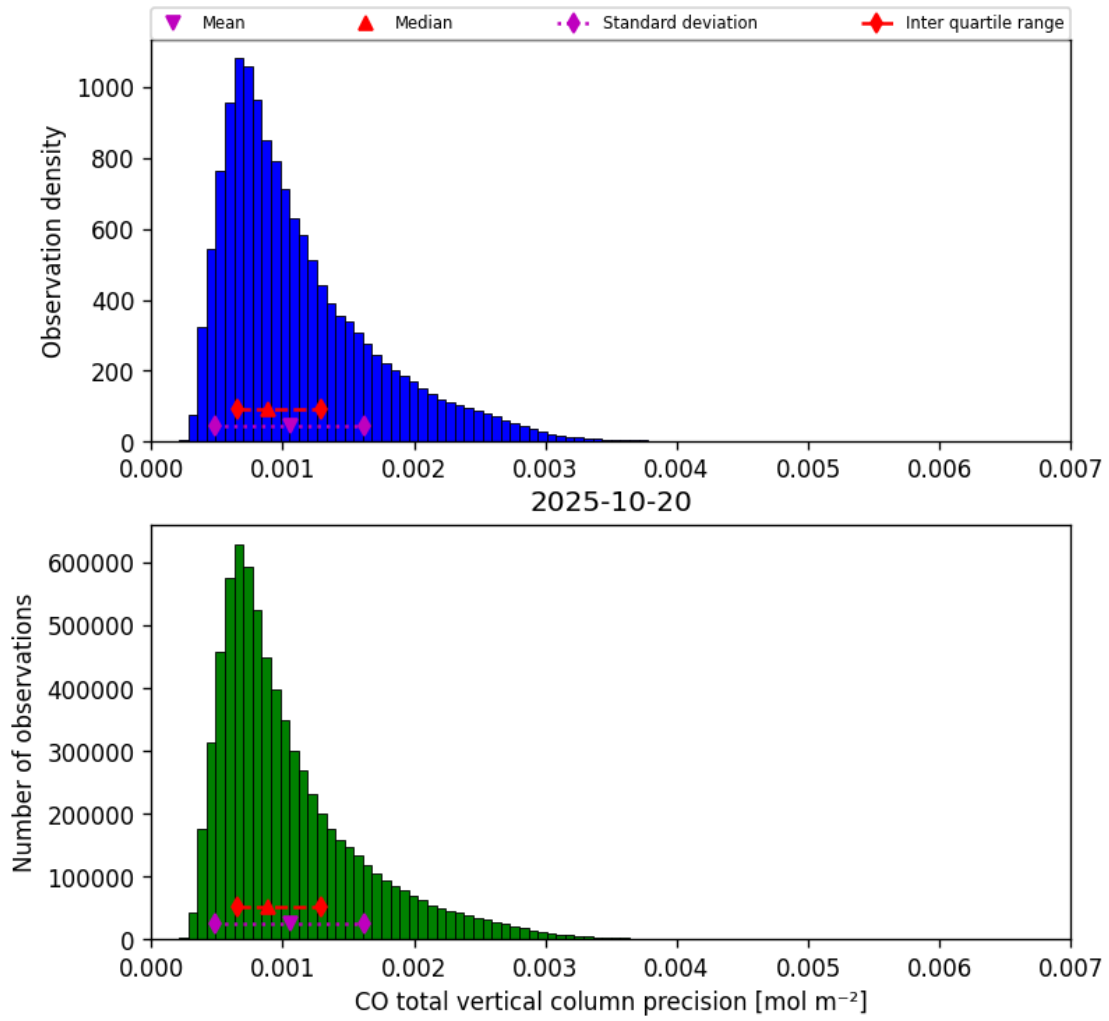
Figure 15: Histogram of “CO total vertical column precision” for 2025-10-20 to 2025-10-20
