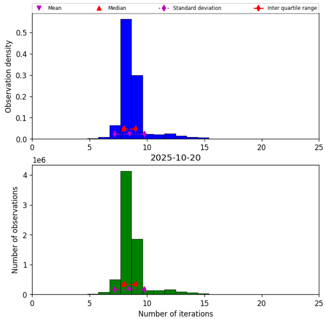
Figure 19: Histogram of “Number of iterations” for 2025-10-20 to 2025-10-20
