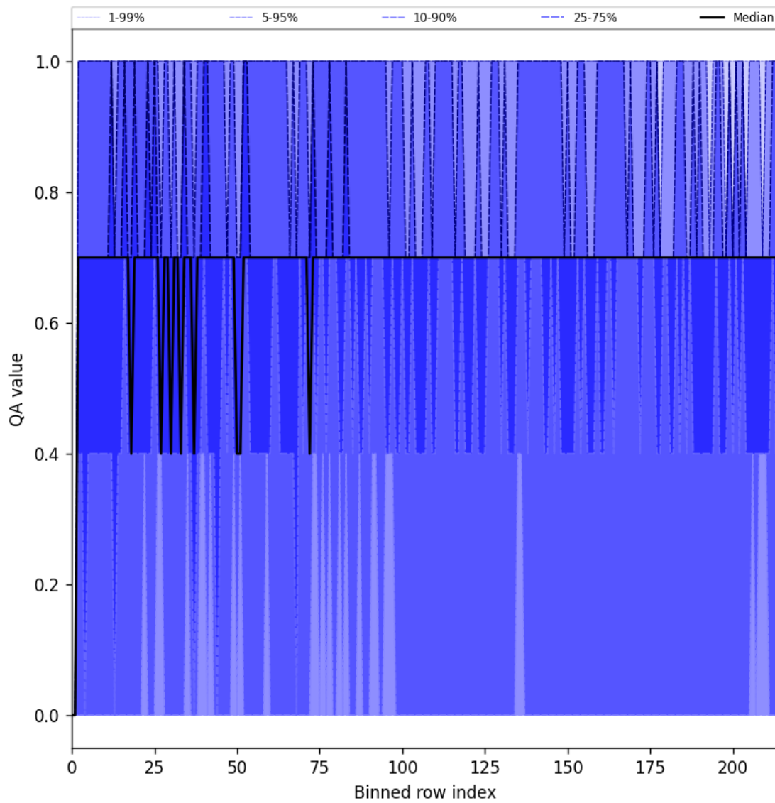
Figure 20: Along track statistics of “QA value” for 2025-10-20 to 2025-10-20
