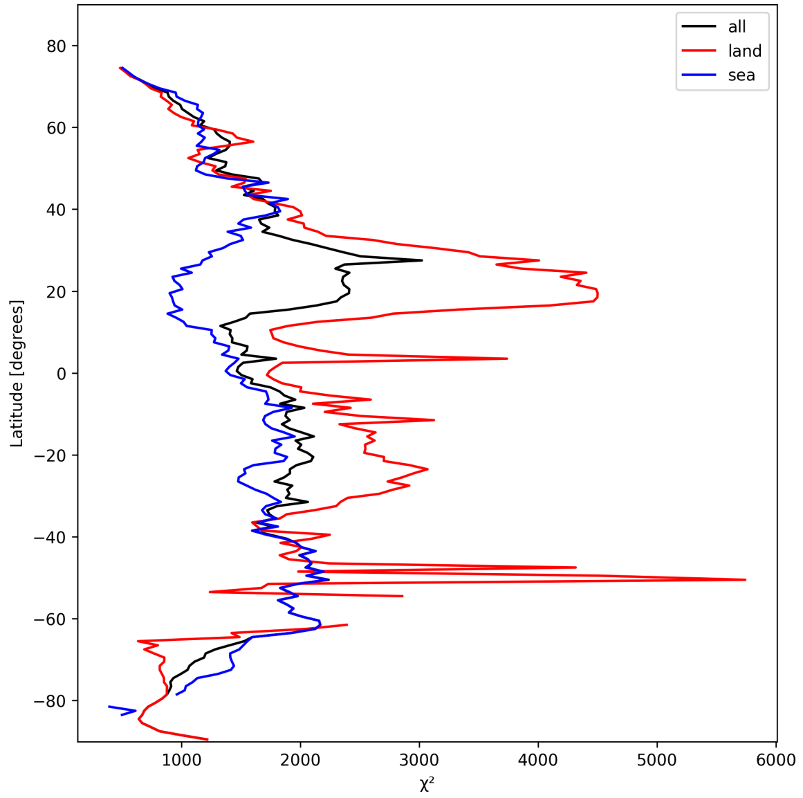
Figure 10: Zonal average of “ \chi^2 ” for 2025-10-20 to 2025-10-20.
