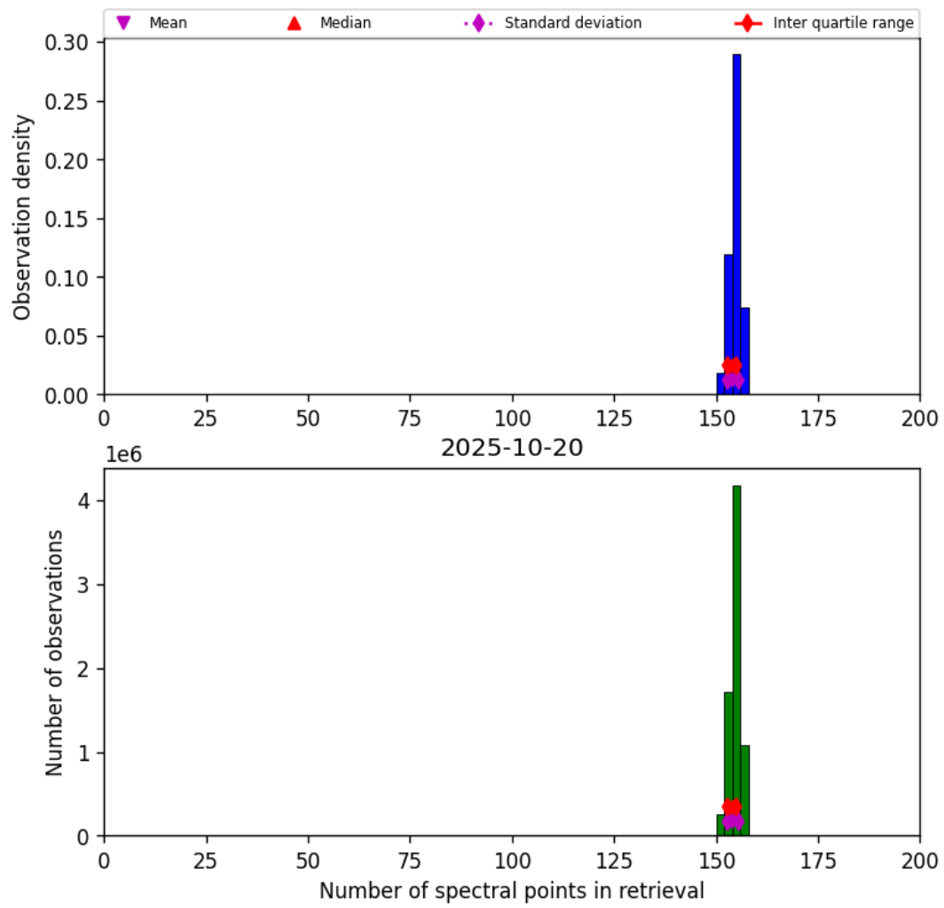
Figure 16: Histogram of “Number of spectral points in retrieval” for 2025-10-20 to 2025-10-20
