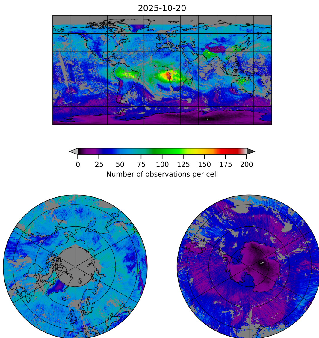
Figure 5: Map of the number of observations for 2025-10-20 to 2025-10-20
