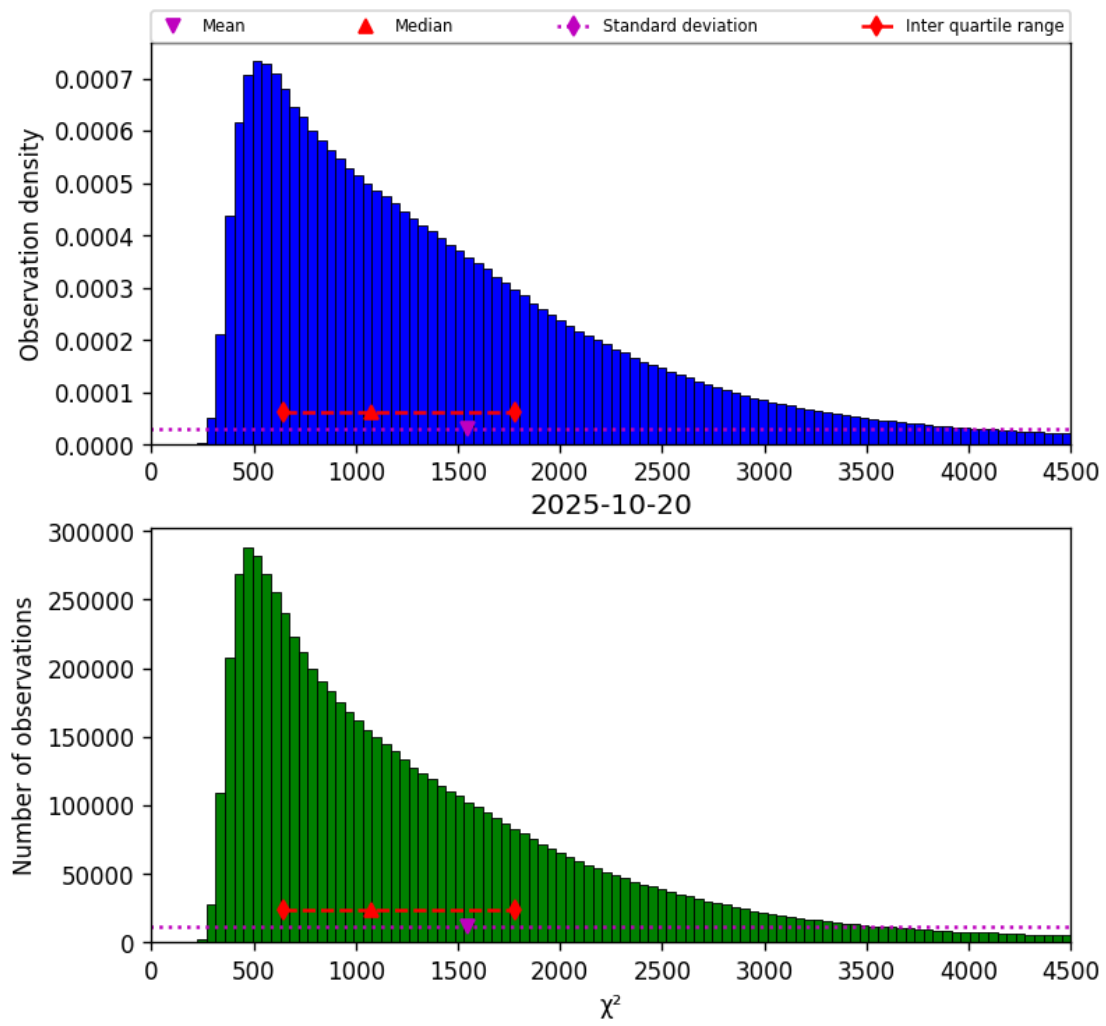
Figure 17: Histogram of " \chi^2 " for 2025-10-20 to 2025-10-20
