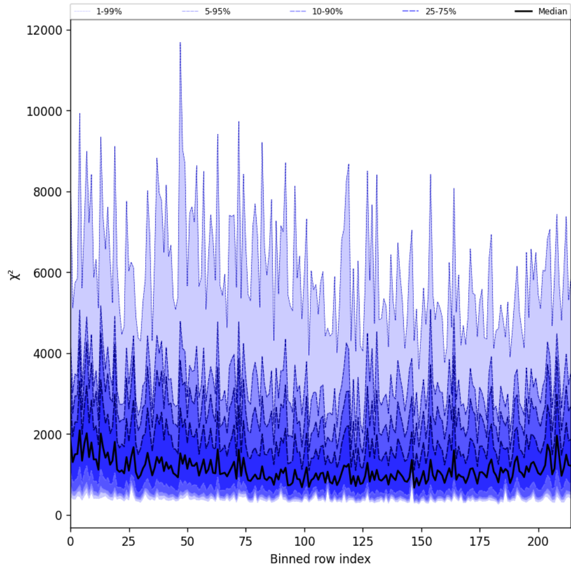
Figure 24: Along track statistics of “ \chi^2 ” for 2025-10-20 to 2025-10-20
