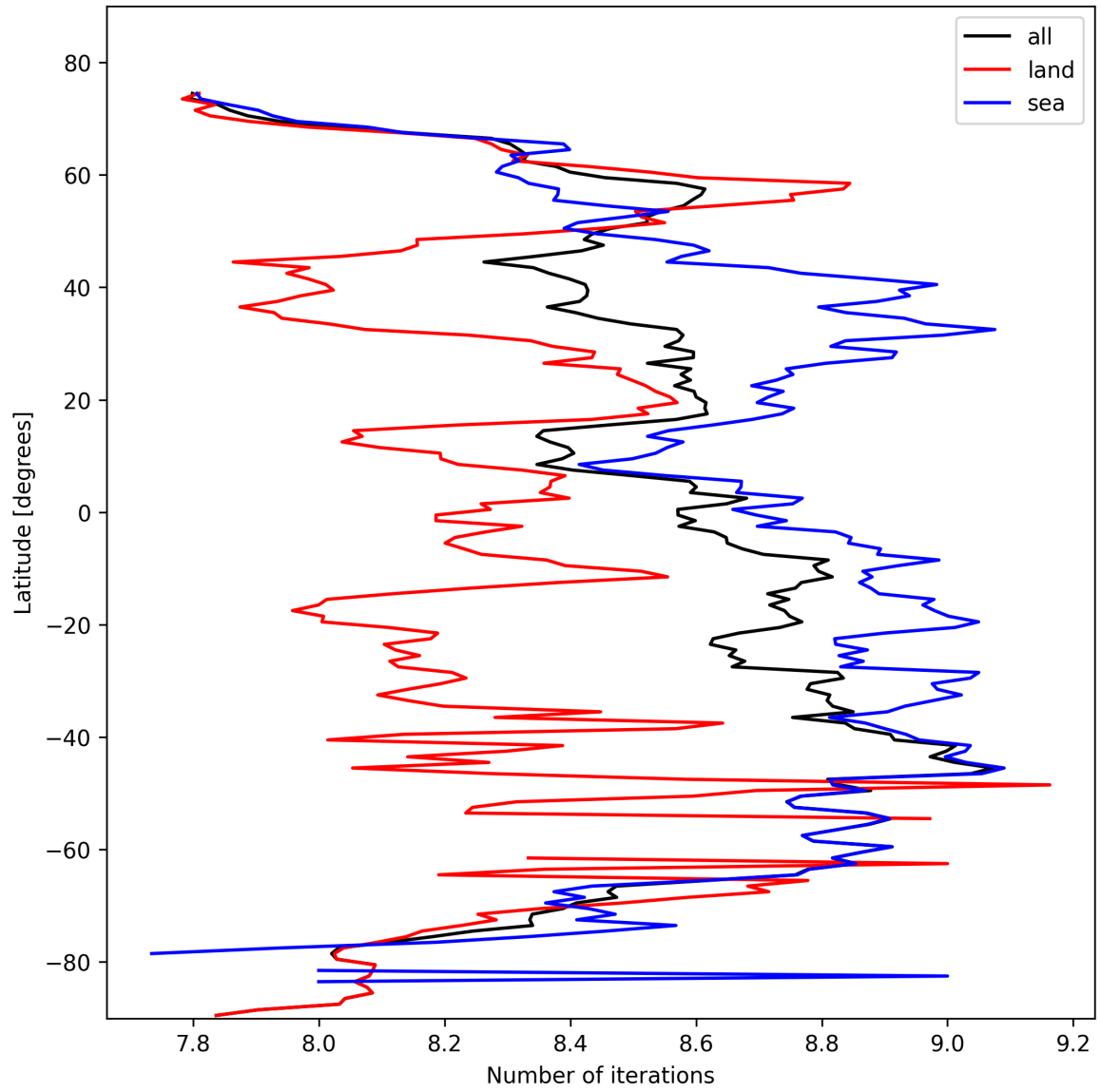
Figure 12: Zonal average of “Number of iterations” for 2025-10-20 to 2025-10-20.
