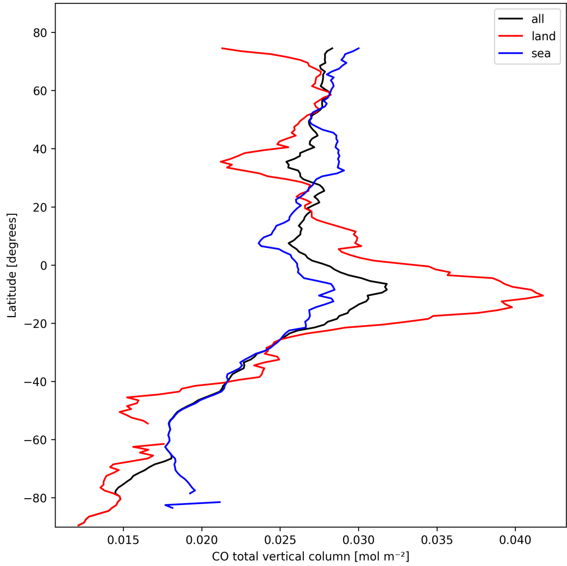
Figure 7: Zonal average of “CO total vertical column” for 2025-10-20 to 2025-10-20.
