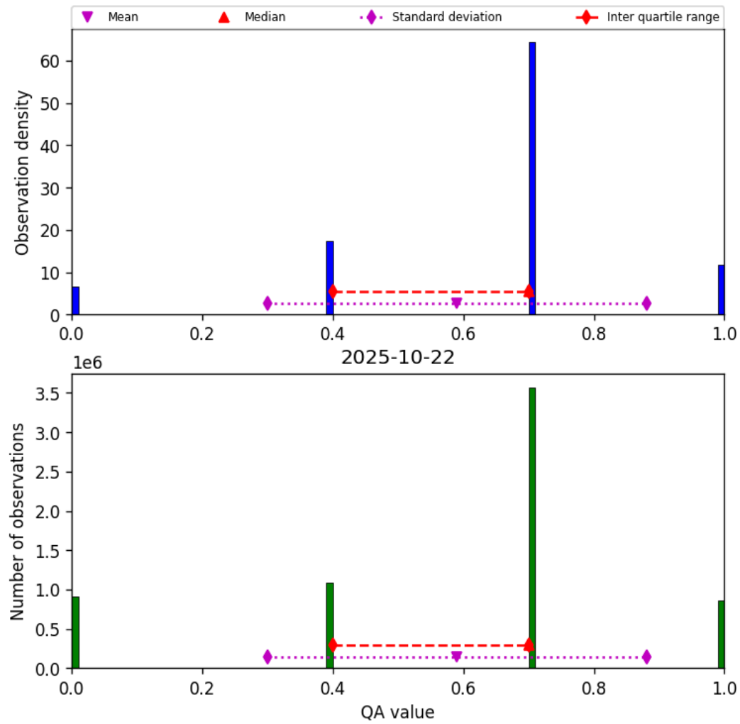
Figure 13: Histogram of “QA value” for 2025-10-22 to 2025-10-23
