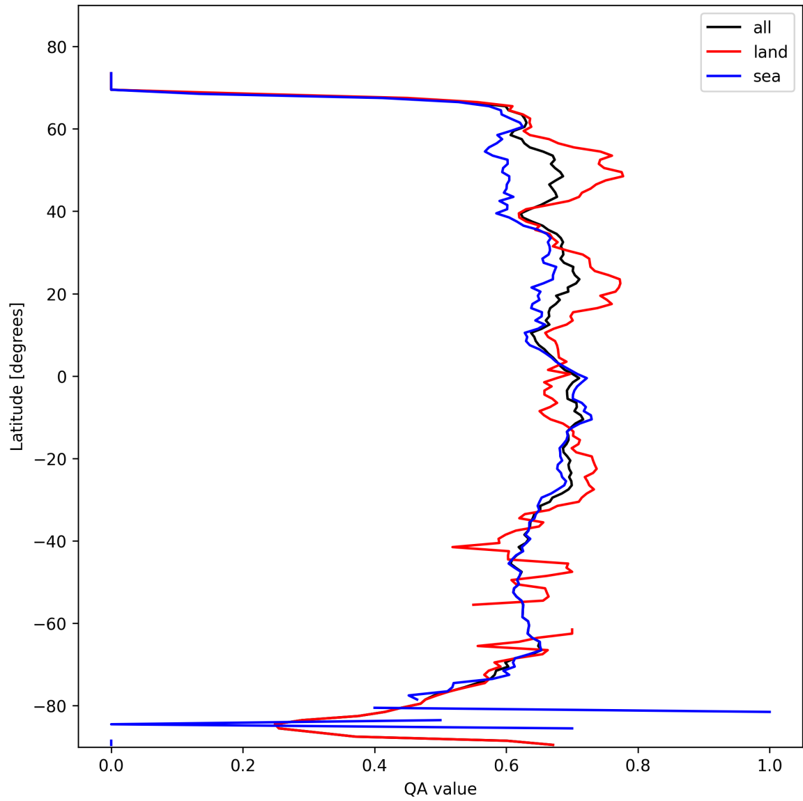
Figure 6: Zonal average of “QA value” for 2025-10-22 to 2025-10-23.
