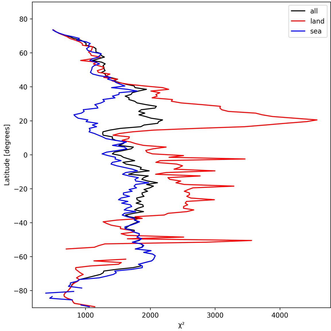
Figure 10: Zonal average of “ \chi^2 ” for 2025-10-22 to 2025-10-23.
