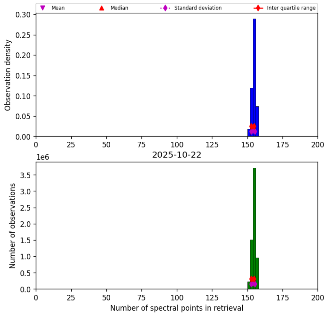
Figure 16: Histogram of “Number of spectral points in retrieval” for 2025-10-22 to 2025-10-23
