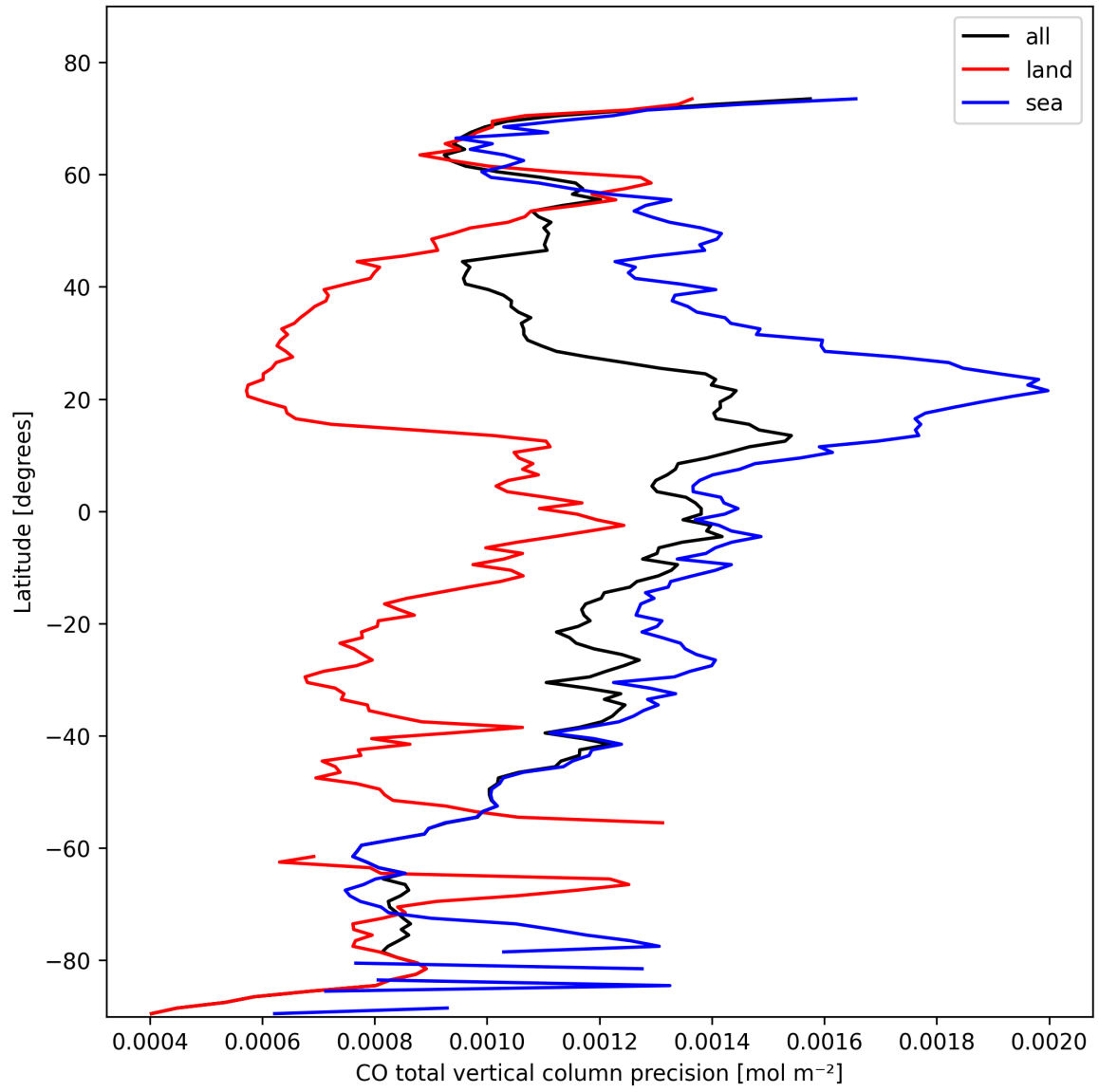
Figure 8: Zonal average of “CO total vertical column precision” for 2025-10-22 to 2025-10-23.
