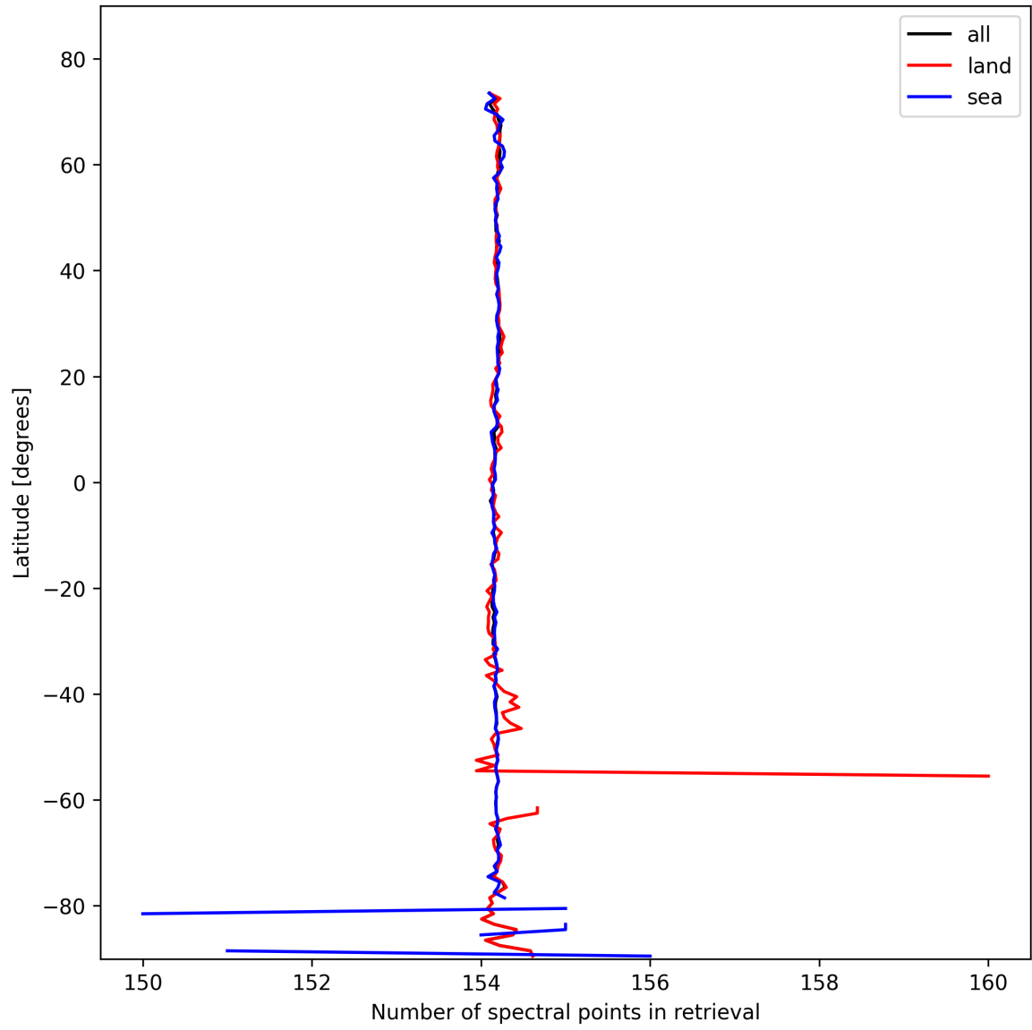
Figure 9: Zonal average of “Number of spectral points in retrieval” for 2025-10-22 to 2025-10-23.
