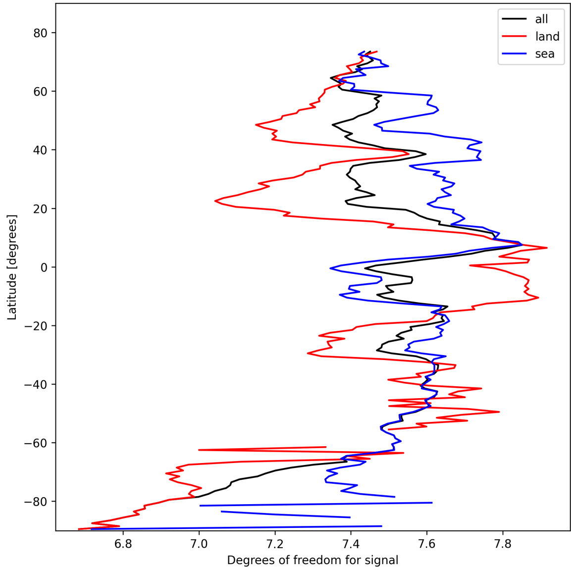
Figure 11: Zonal average of “Degrees of freedom for signal” for 2025-10-22 to 2025-10-23.
