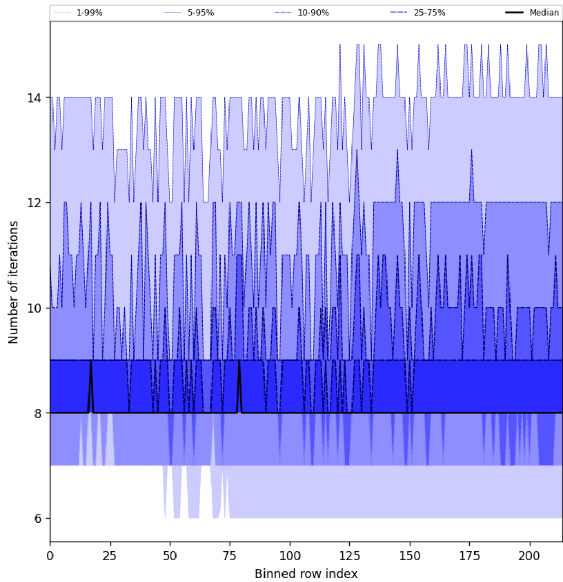
Figure 26: Along track statistics of “Number of iterations” for 2025-10-22 to 2025-10-23
