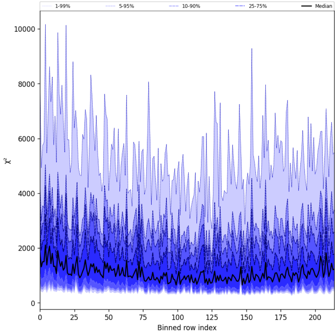
Figure 24: Along track statistics of “ \chi^2 ” for 2025-10-22 to 2025-10-23
