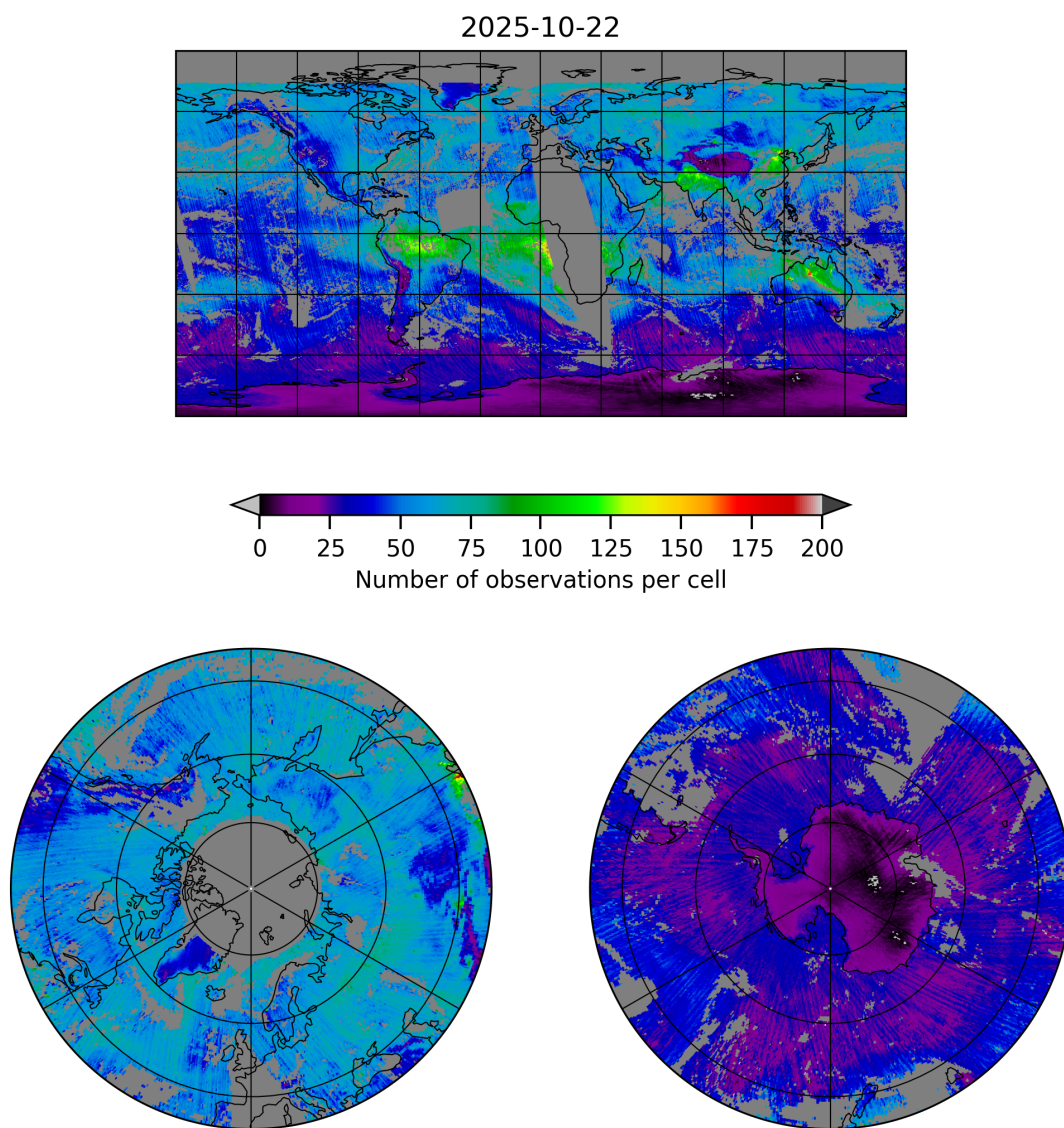
Figure 5: Map of the number of observations for 2025-10-22 to 2025-10-23
