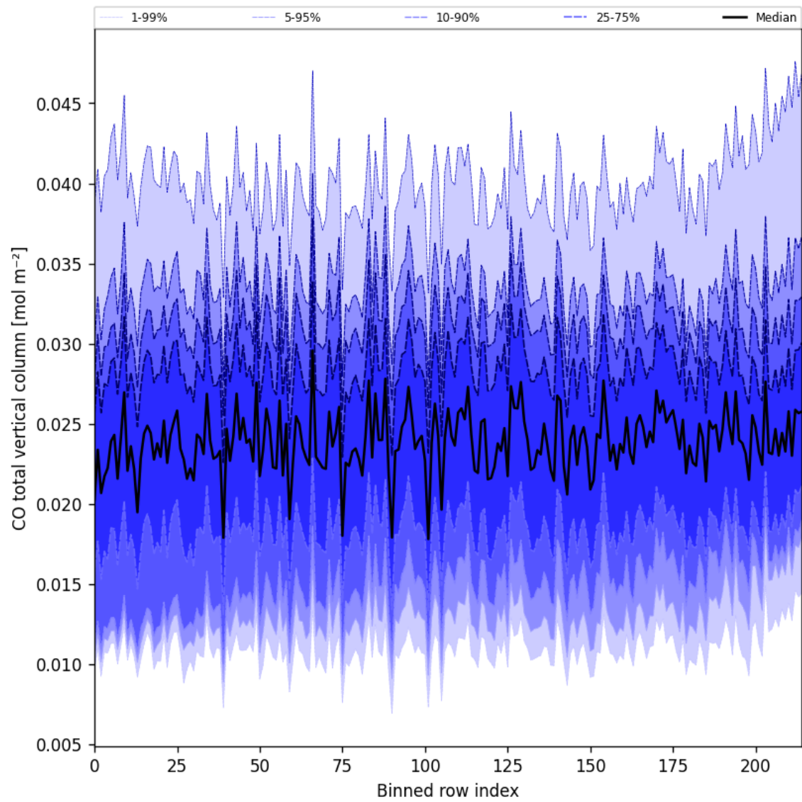
Figure 21: Along track statistics of “CO total vertical column” for 2025-10-22 to 2025-10-23
