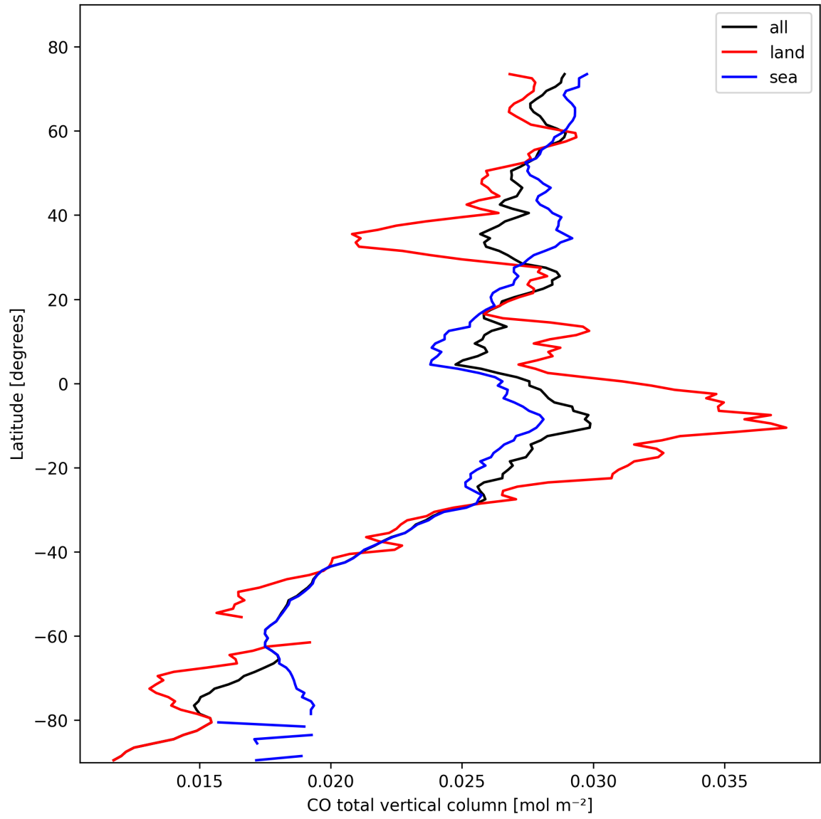
Figure 7: Zonal average of “CO total vertical column” for 2025-10-22 to 2025-10-23.
