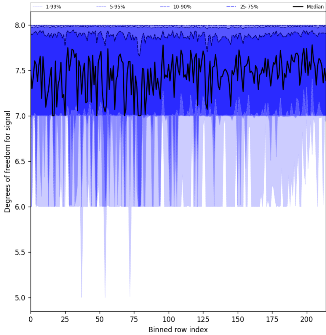
Figure 25: Along track statistics of “Degrees of freedom for signal” for 2025-10-22 to 2025-10-23
