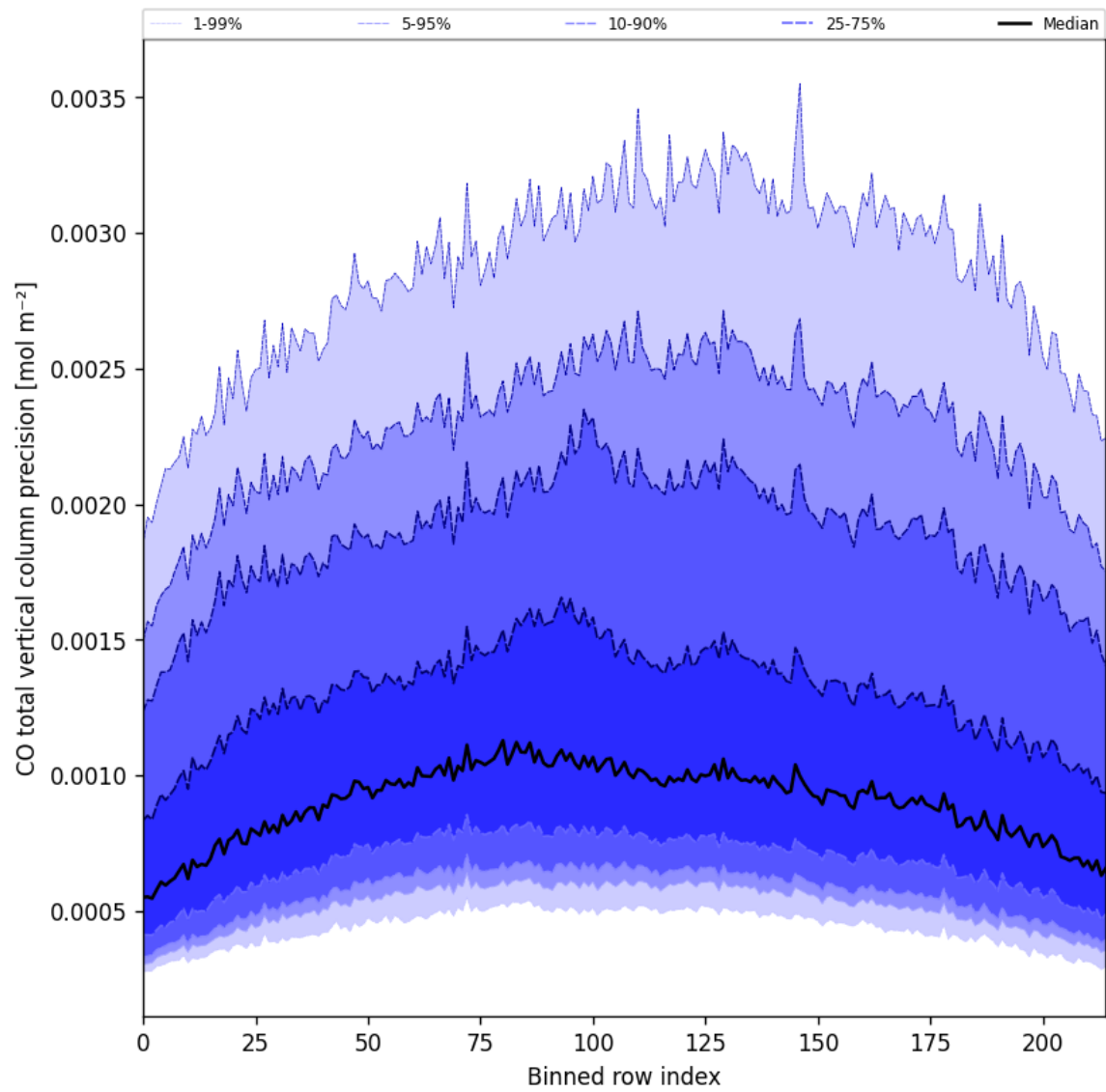
Figure 22: Along track statistics of “CO total vertical column precision” for 2025-10-22 to 2025-10-23
