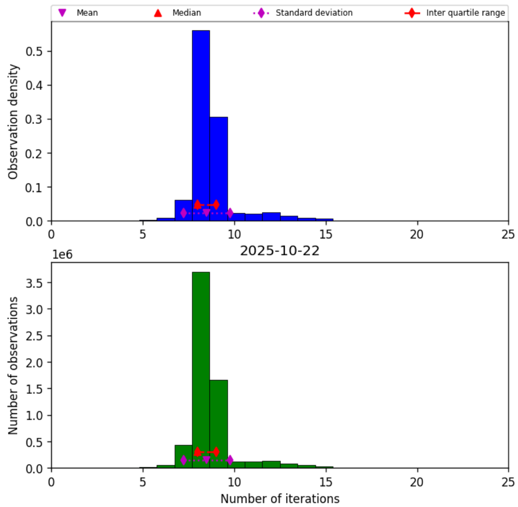
Figure 19: Histogram of “Number of iterations” for 2025-10-22 to 2025-10-23
