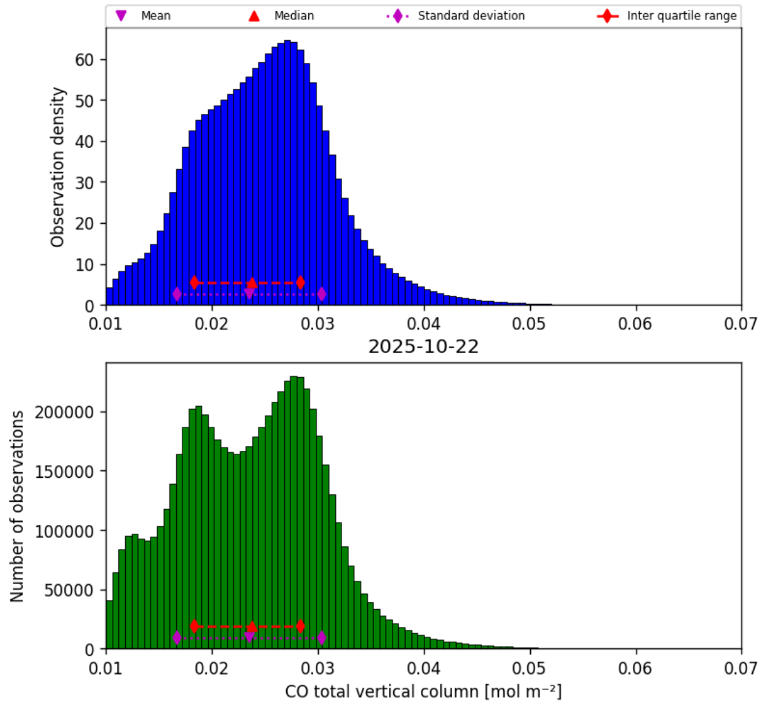
Figure 14: Histogram of “CO total vertical column” for 2025-10-22 to 2025-10-23
