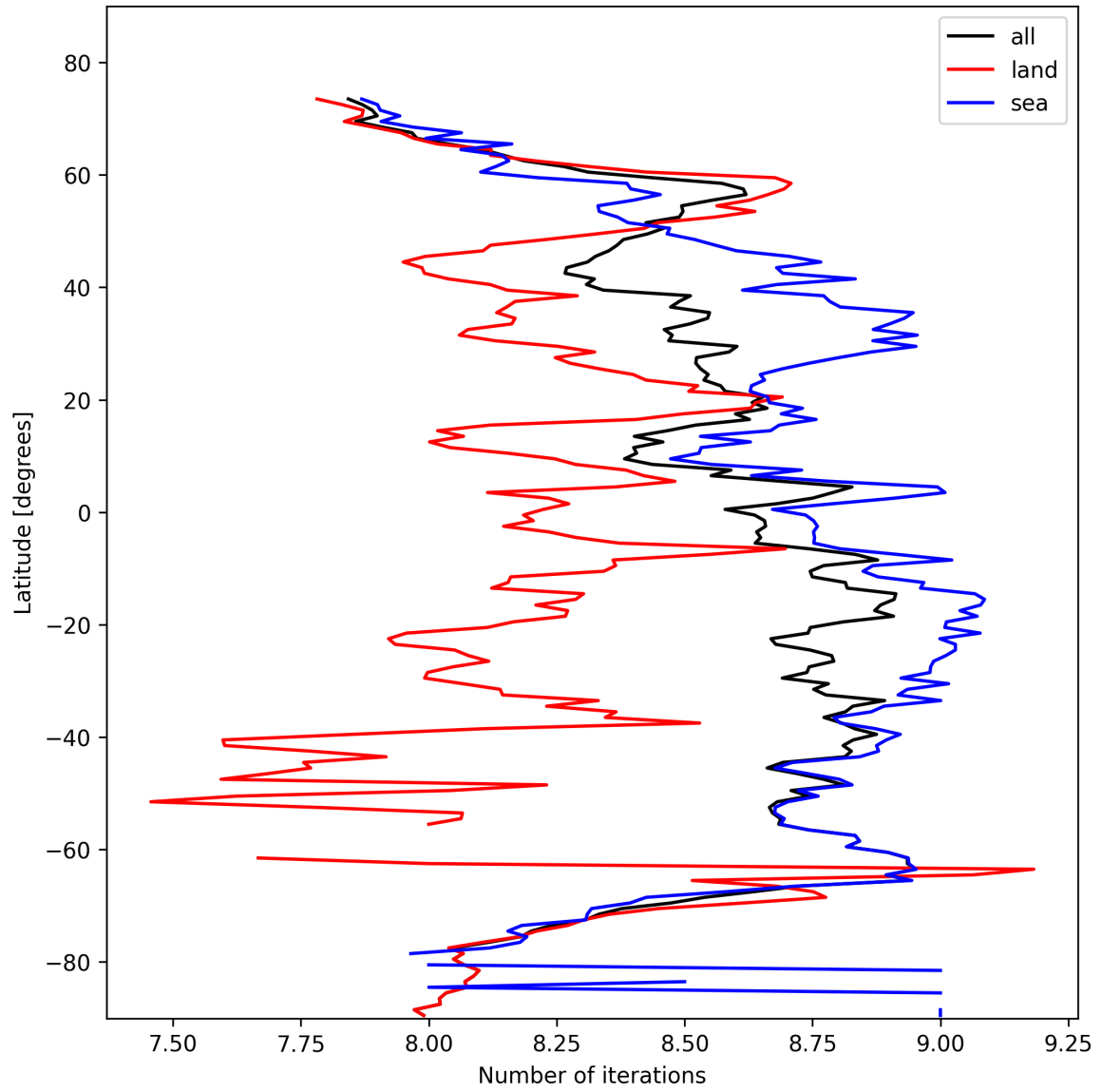
Figure 12: Zonal average of “Number of iterations” for 2025-10-22 to 2025-10-23.
