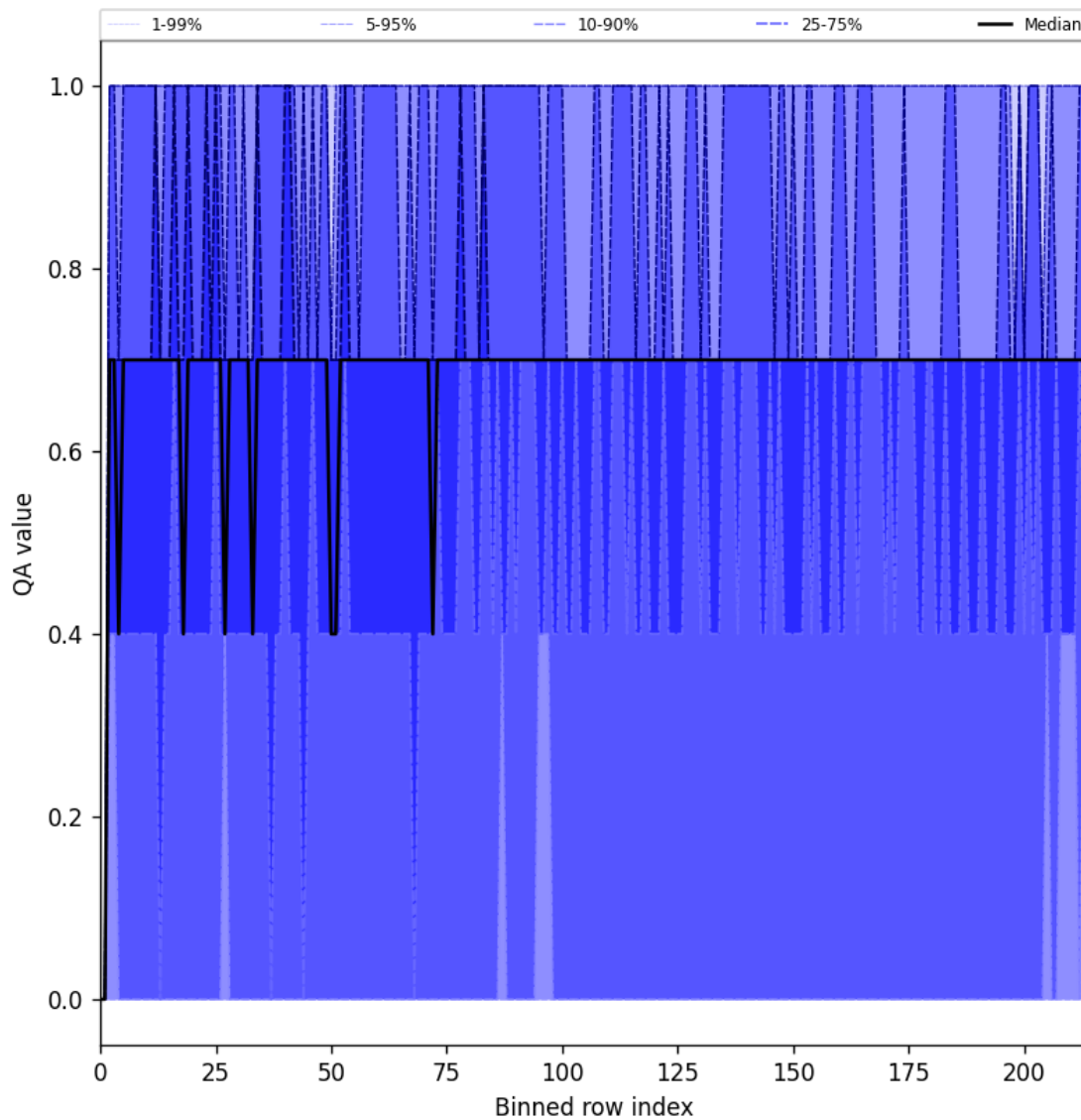
Figure 20: Along track statistics of “QA value” for 2025-10-22 to 2025-10-23
