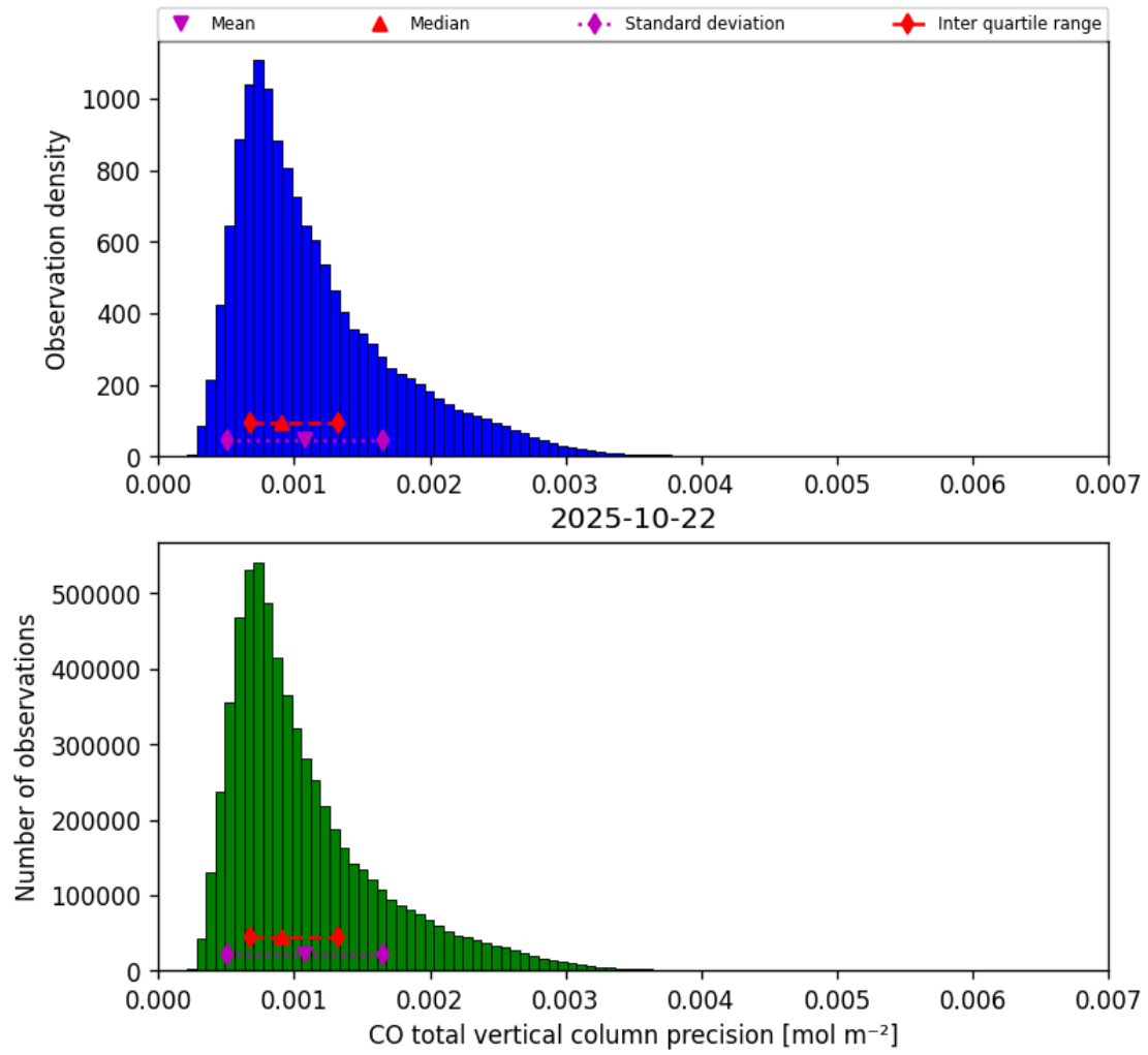
Figure 15: Histogram of “CO total vertical column precision” for 2025-10-22 to 2025-10-23
