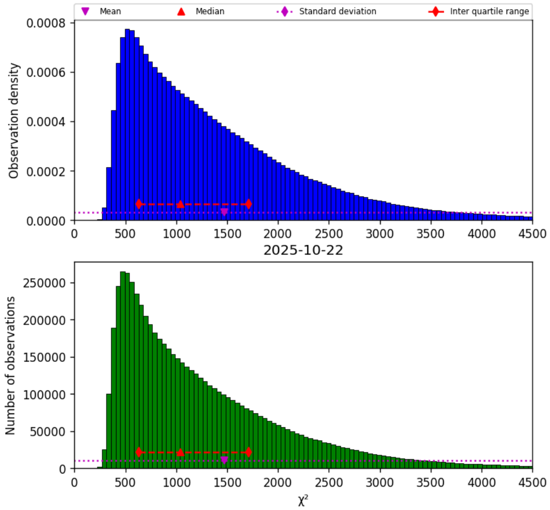
Figure 17: Histogram of “ \chi^2 ” for 2025-10-22 to 2025-10-23
