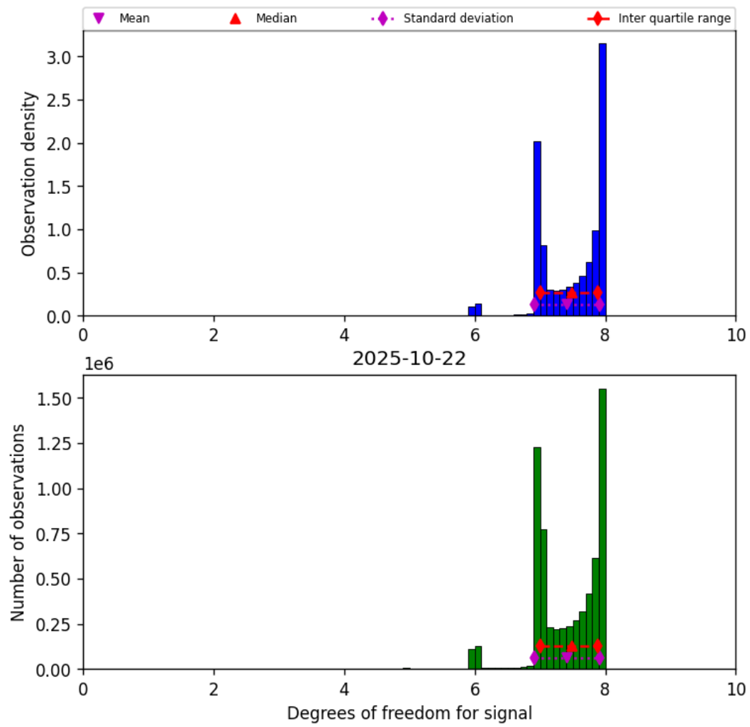
Figure 18: Histogram of “Degrees of freedom for signal” for 2025-10-22 to 2025-10-23
