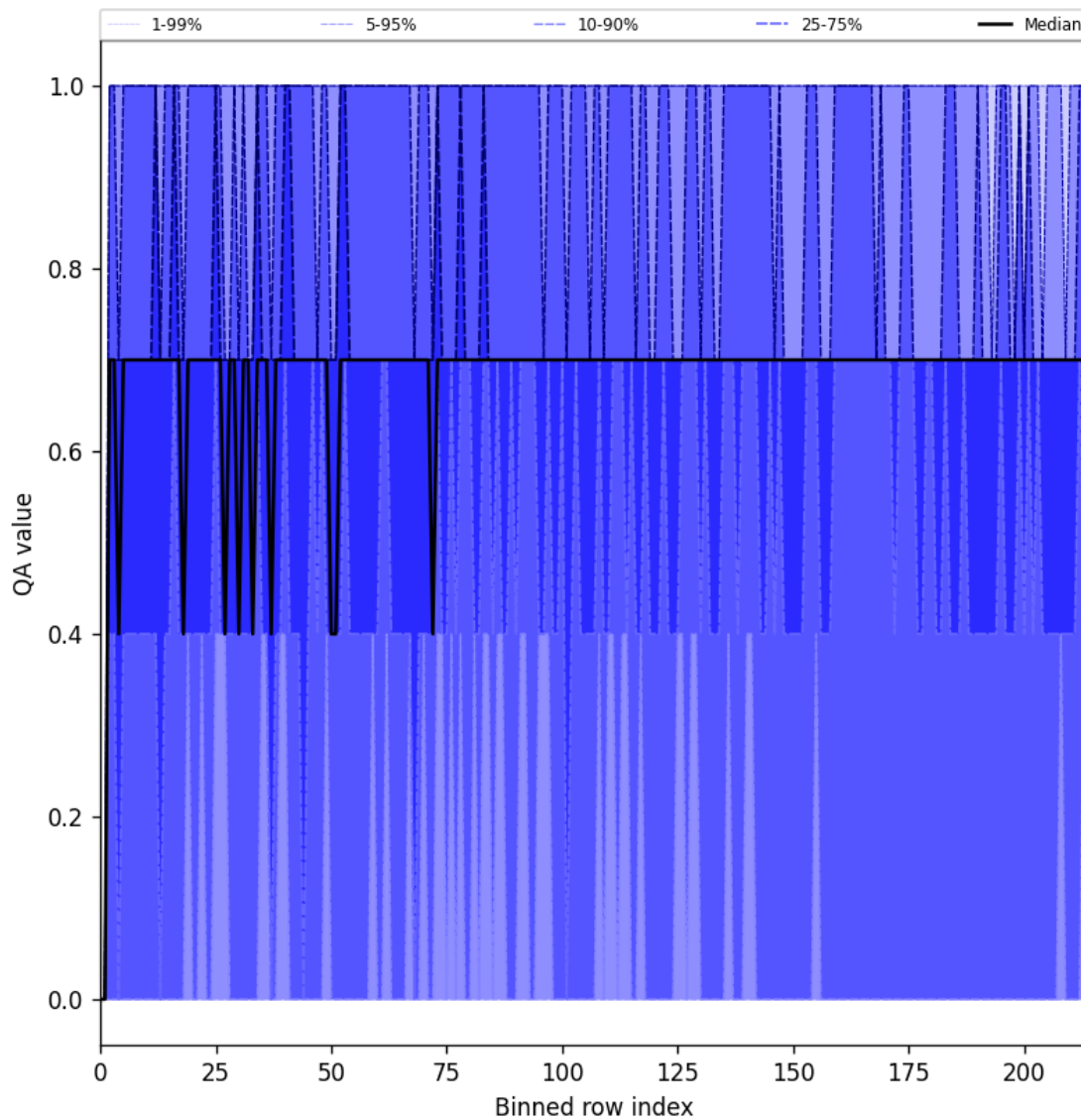
Figure 20: Along track statistics of “QA value” for 2025-10-23 to 2025-10-24
