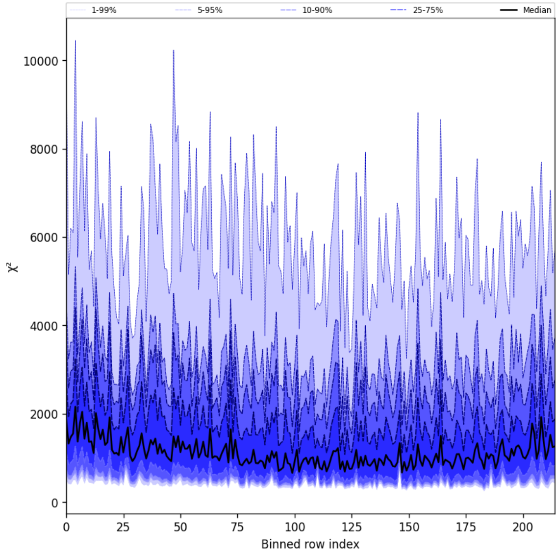
Figure 24: Along track statistics of “ \chi^2 ” for 2025-10-23 to 2025-10-24
