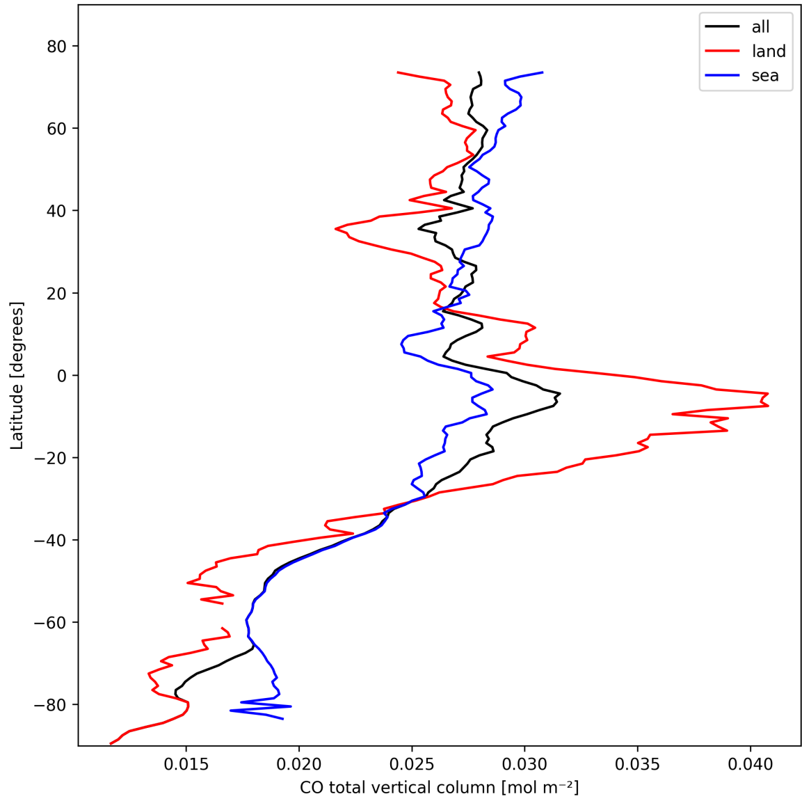
Figure 7: Zonal average of “CO total vertical column” for 2025-10-23 to 2025-10-24.
