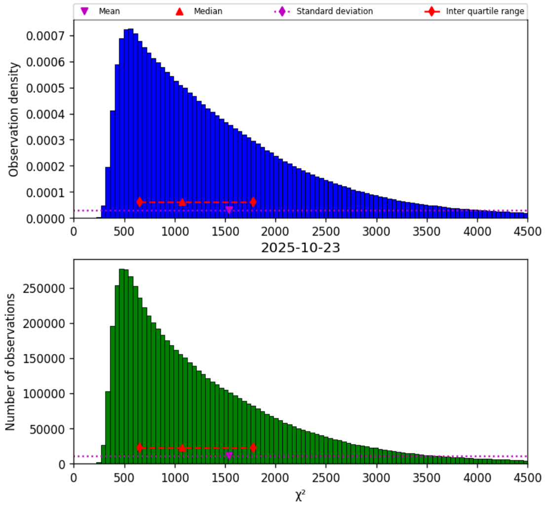
Figure 17: Histogram of “ \chi^2 ” for 2025-10-23 to 2025-10-24
