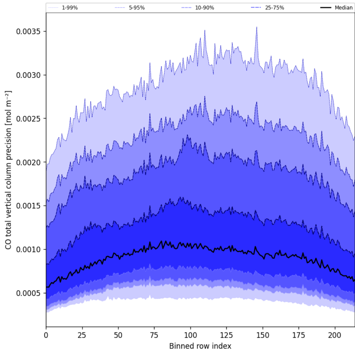
Figure 22: Along track statistics of “CO total vertical column precision” for 2025-10-23 to 2025-10-24
