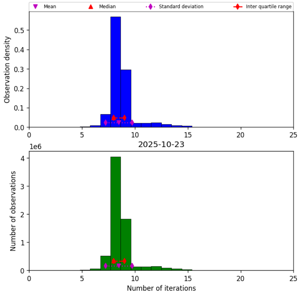
Figure 19: Histogram of “Number of iterations” for 2025-10-23 to 2025-10-24
