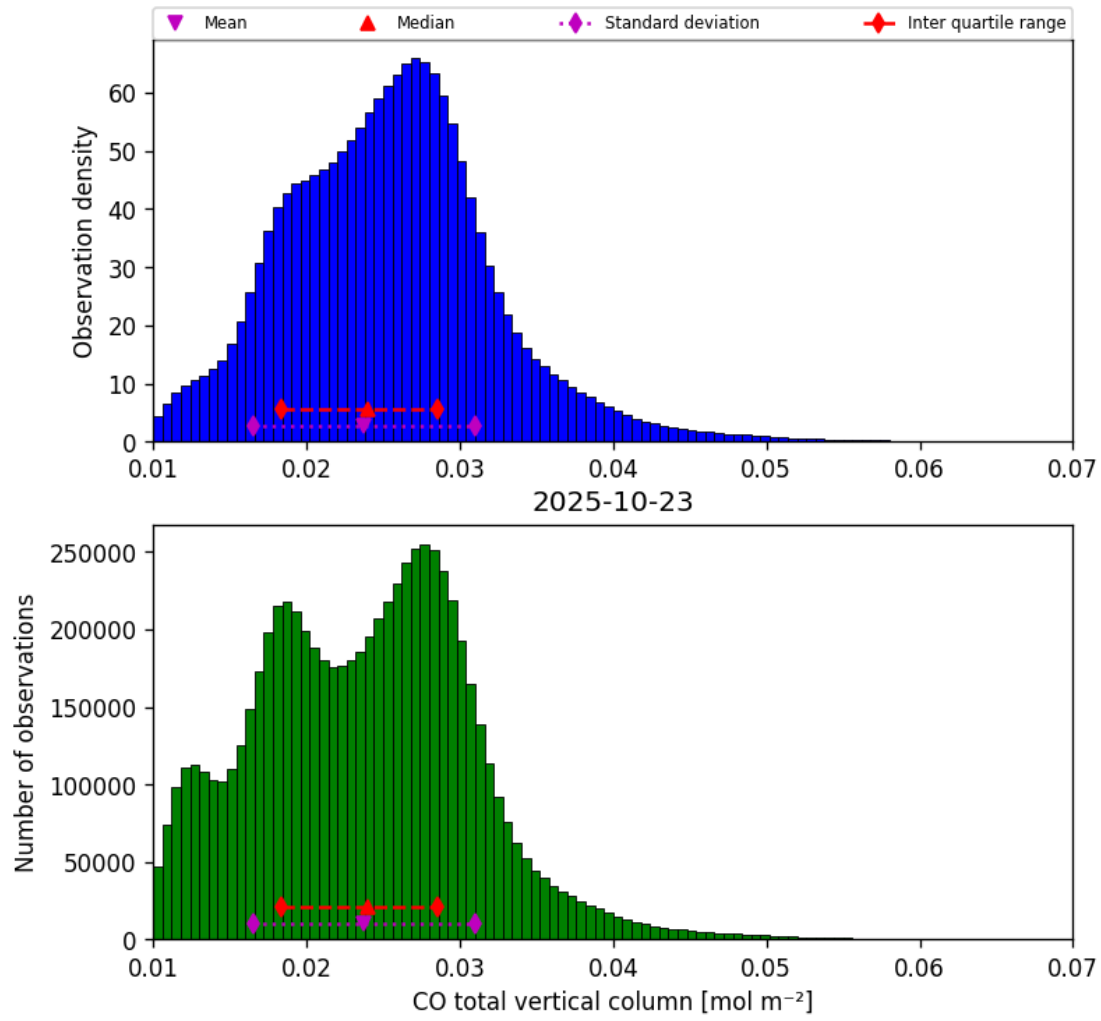
Figure 14: Histogram of “CO total vertical column” for 2025-10-23 to 2025-10-24
