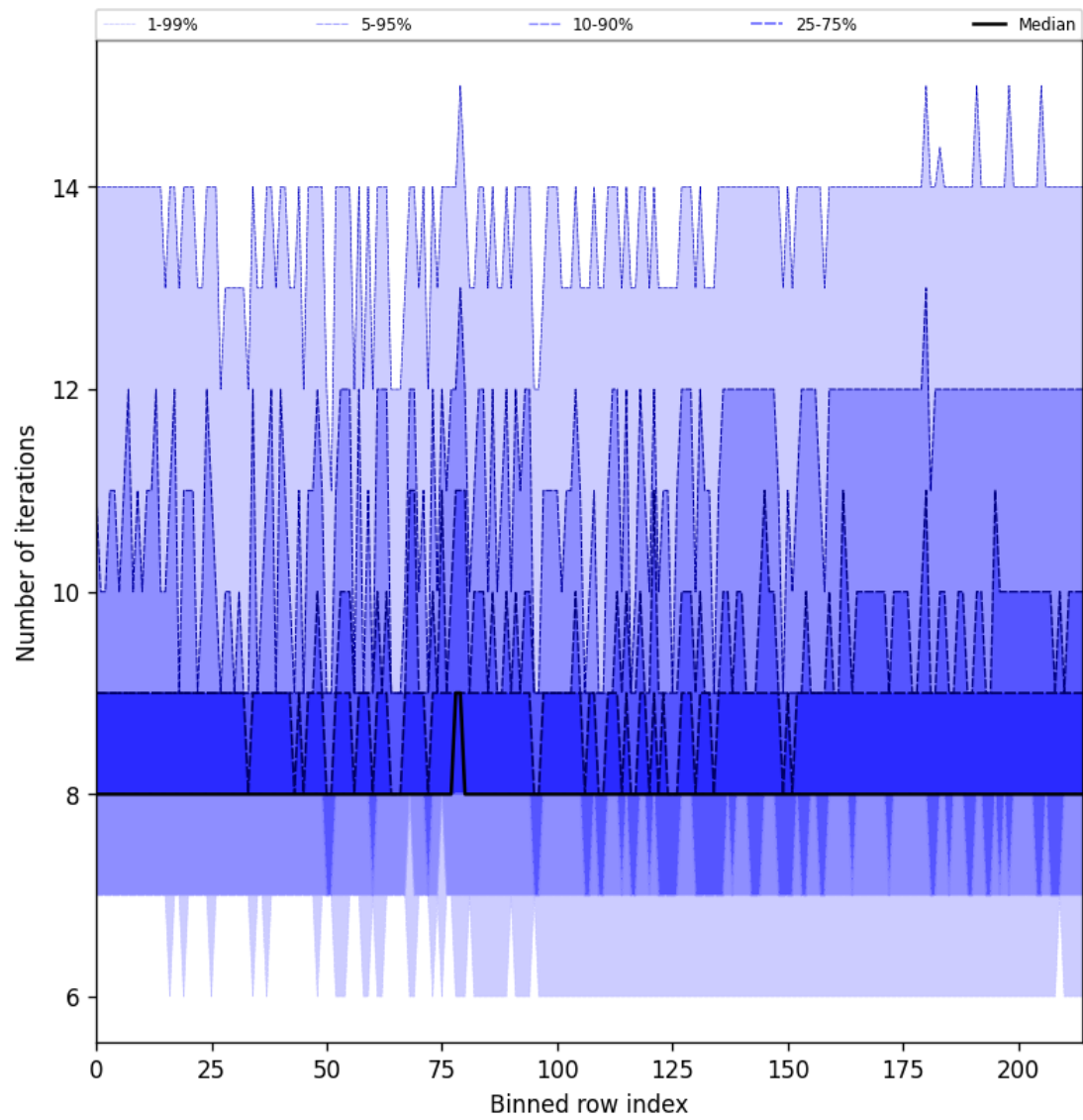
Figure 26: Along track statistics of “Number of iterations” for 2025-10-23 to 2025-10-24
