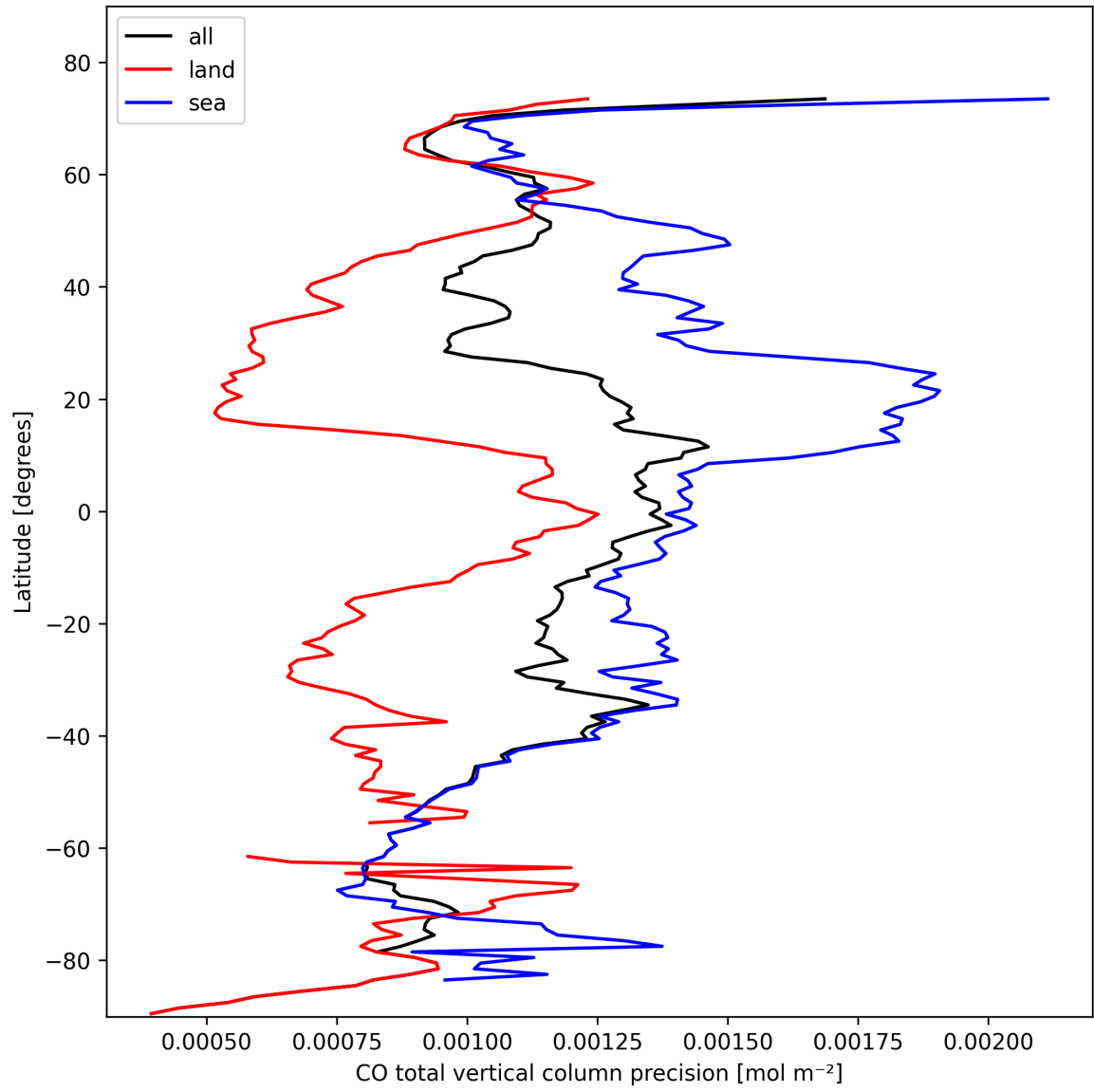
Figure 8: Zonal average of “CO total vertical column precision” for 2025-10-23 to 2025-10-24.
