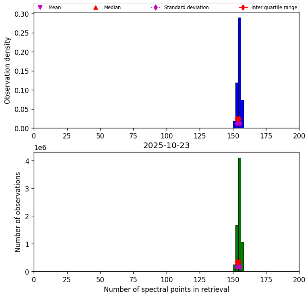
Figure 16: Histogram of “Number of spectral points in retrieval” for 2025-10-23 to 2025-10-24
