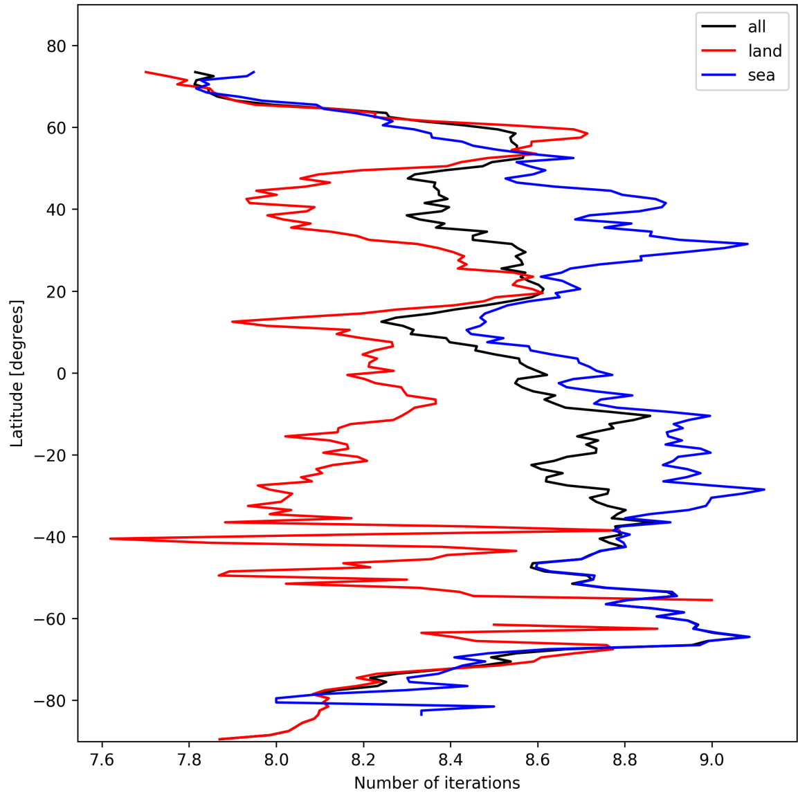
Figure 12: Zonal average of “Number of iterations” for 2025-10-23 to 2025-10-24.
