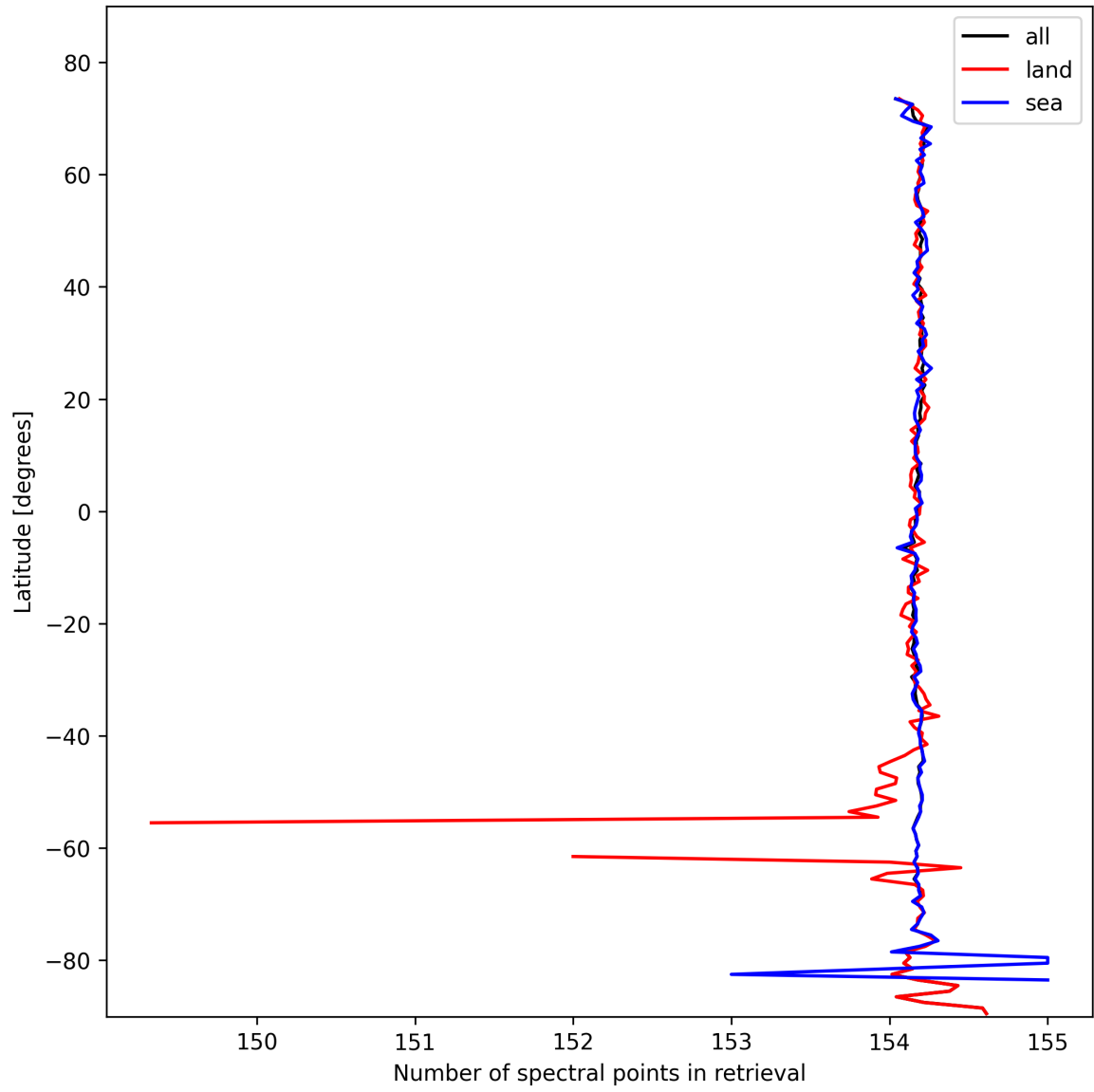
Figure 9: Zonal average of “Number of spectral points in retrieval” for 2025-10-23 to 2025-10-24.
