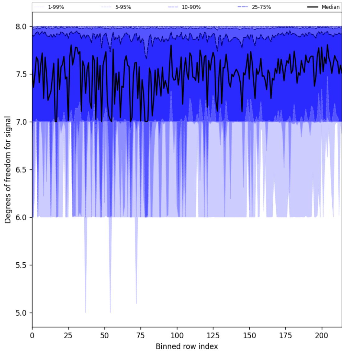
Figure 25: Along track statistics of “Degrees of freedom for signal” for 2025-10-23 to 2025-10-24
