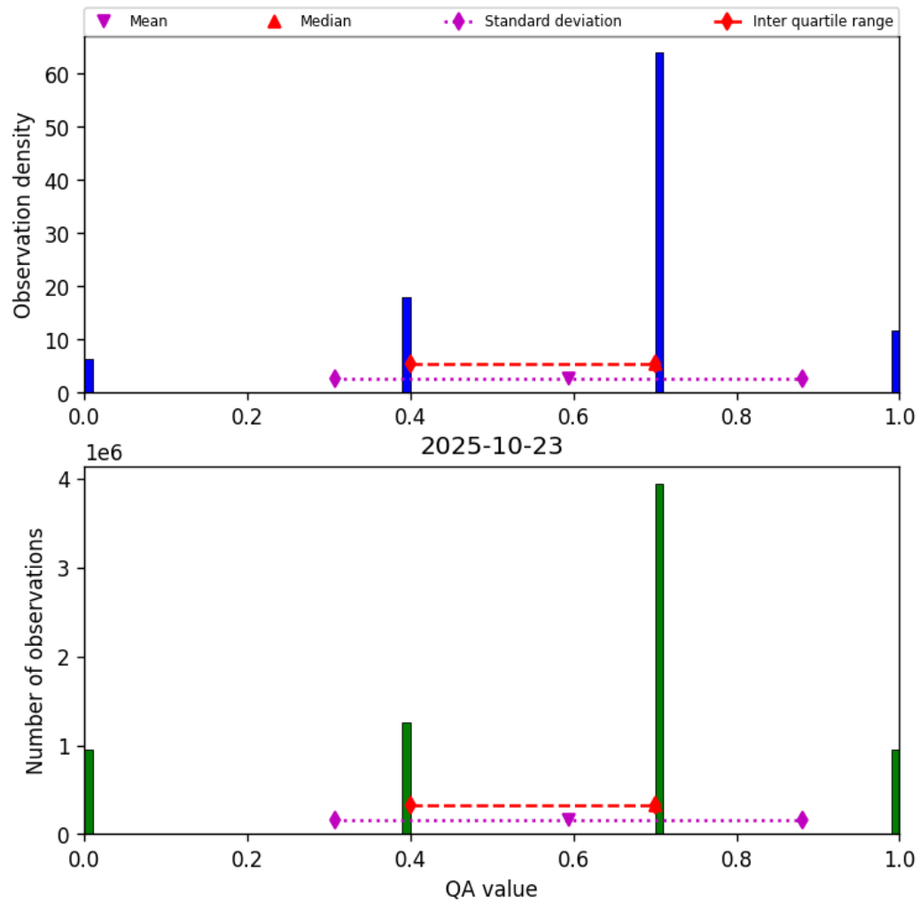
Figure 13: Histogram of “QA value” for 2025-10-23 to 2025-10-24
