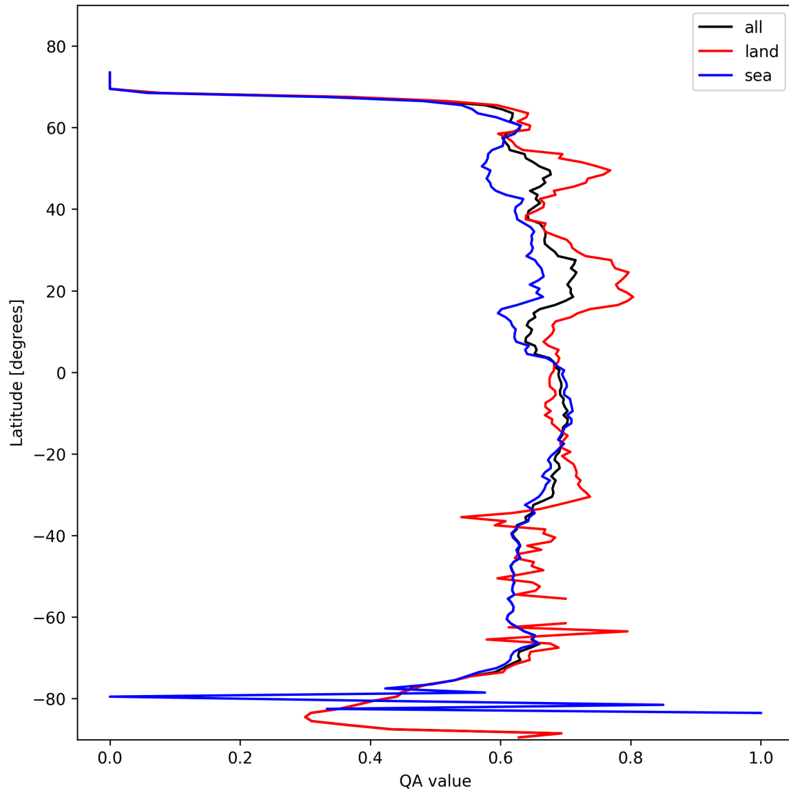
Figure 6: Zonal average of “QA value” for 2025-10-23 to 2025-10-24.
