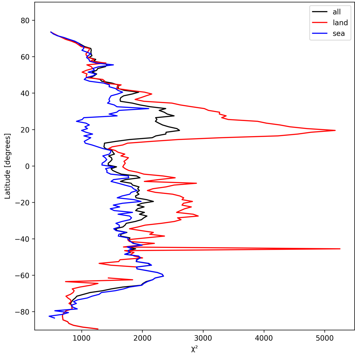
Figure 10: Zonal average of “ \chi^2 ” for 2025-10-23 to 2025-10-24.
