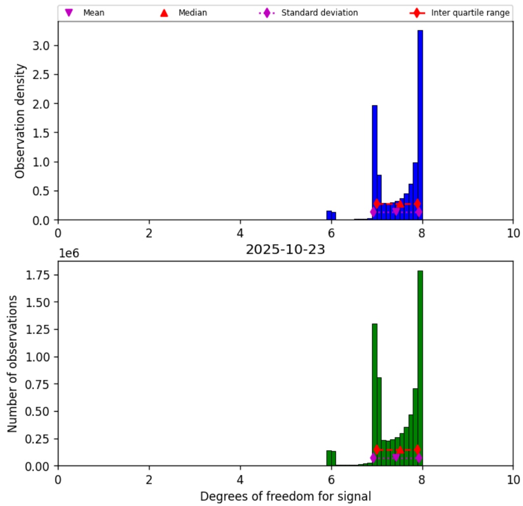
Figure 18: Histogram of “Degrees of freedom for signal” for 2025-10-23 to 2025-10-24
