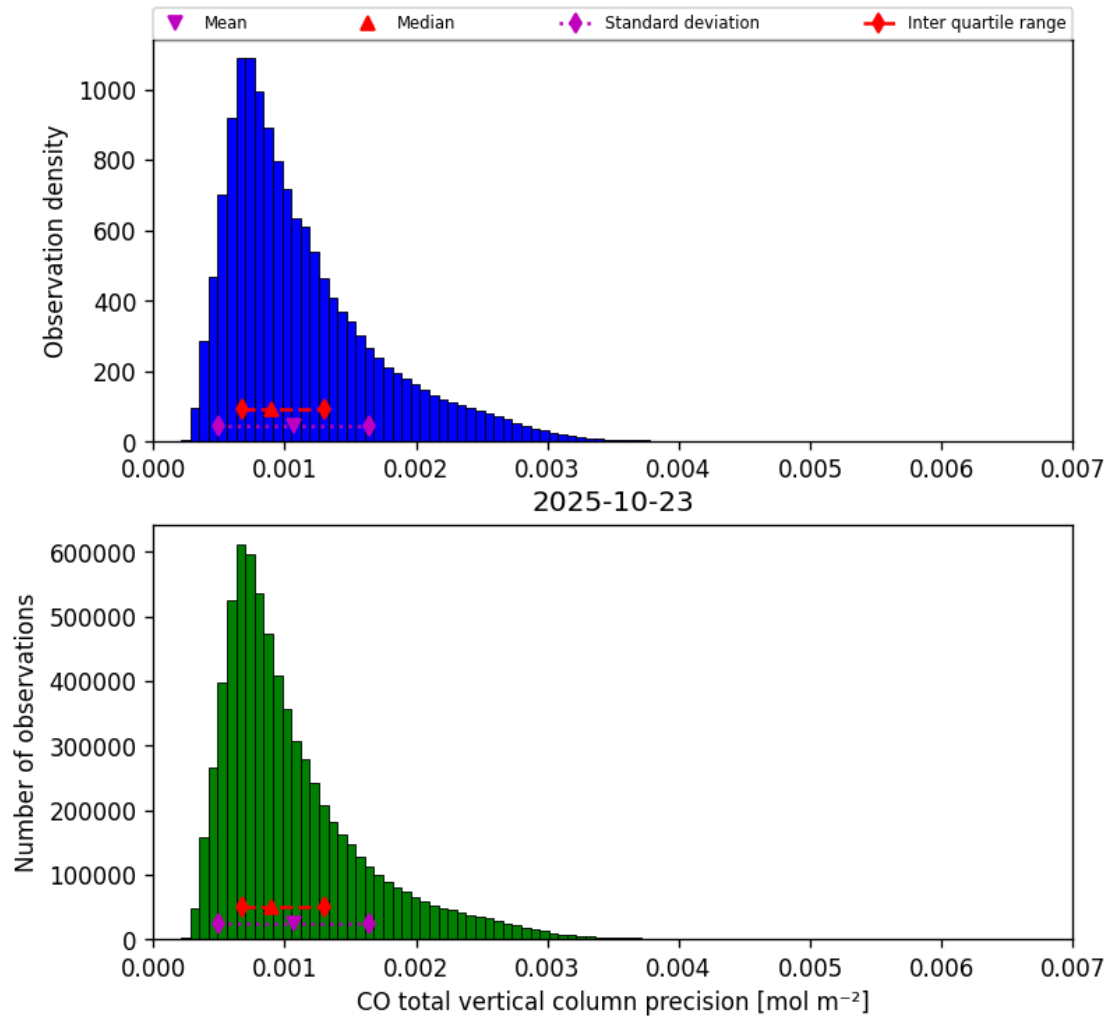
Figure 15: Histogram of “CO total vertical column precision” for 2025-10-23 to 2025-10-24
