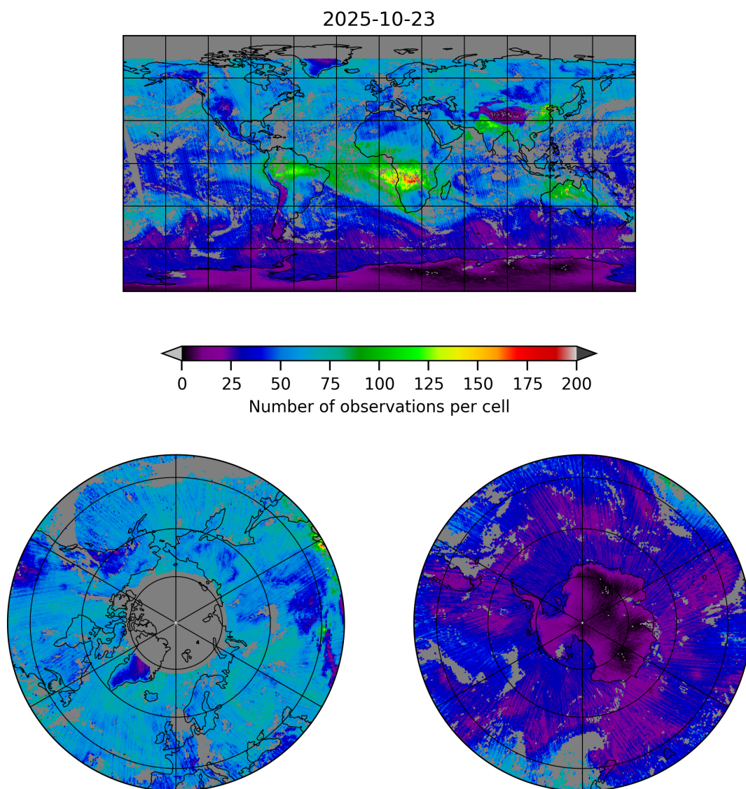
Figure 5: Map of the number of observations for 2025-10-23 to 2025-10-24
