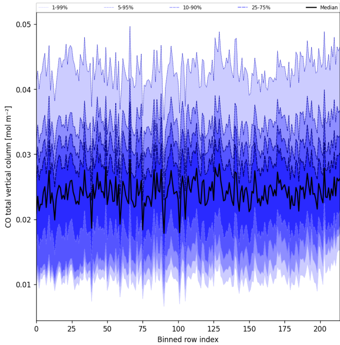
Figure 21: Along track statistics of “CO total vertical column” for 2025-10-23 to 2025-10-24
