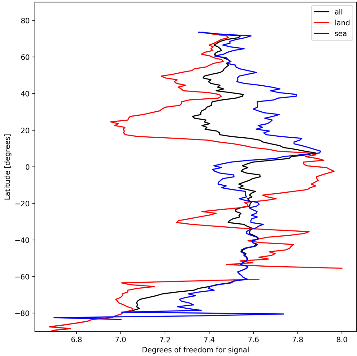
Figure 11: Zonal average of “Degrees of freedom for signal” for 2025-10-23 to 2025-10-24.
