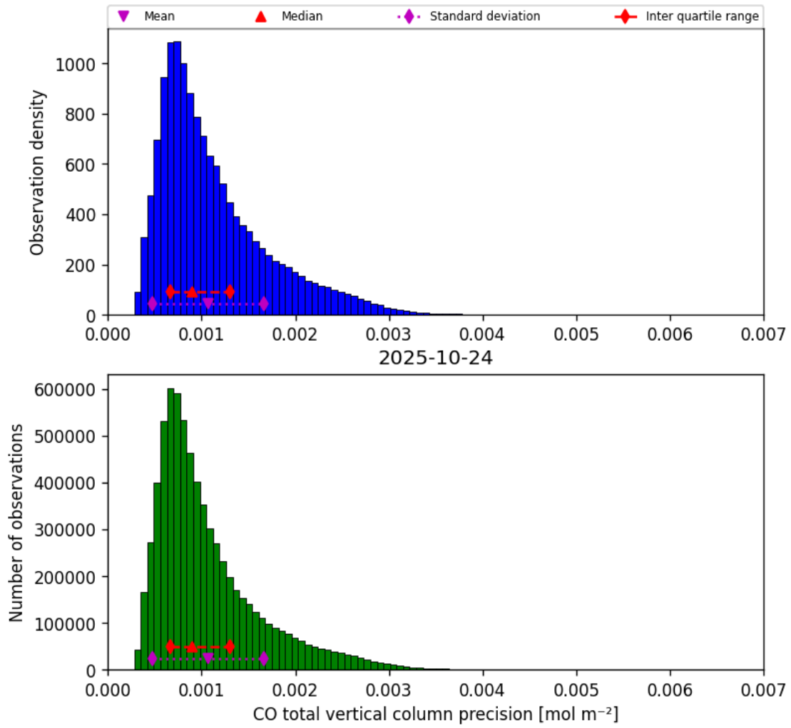
Figure 15: Histogram of “CO total vertical column precision” for 2025-10-24 to 2025-10-25
