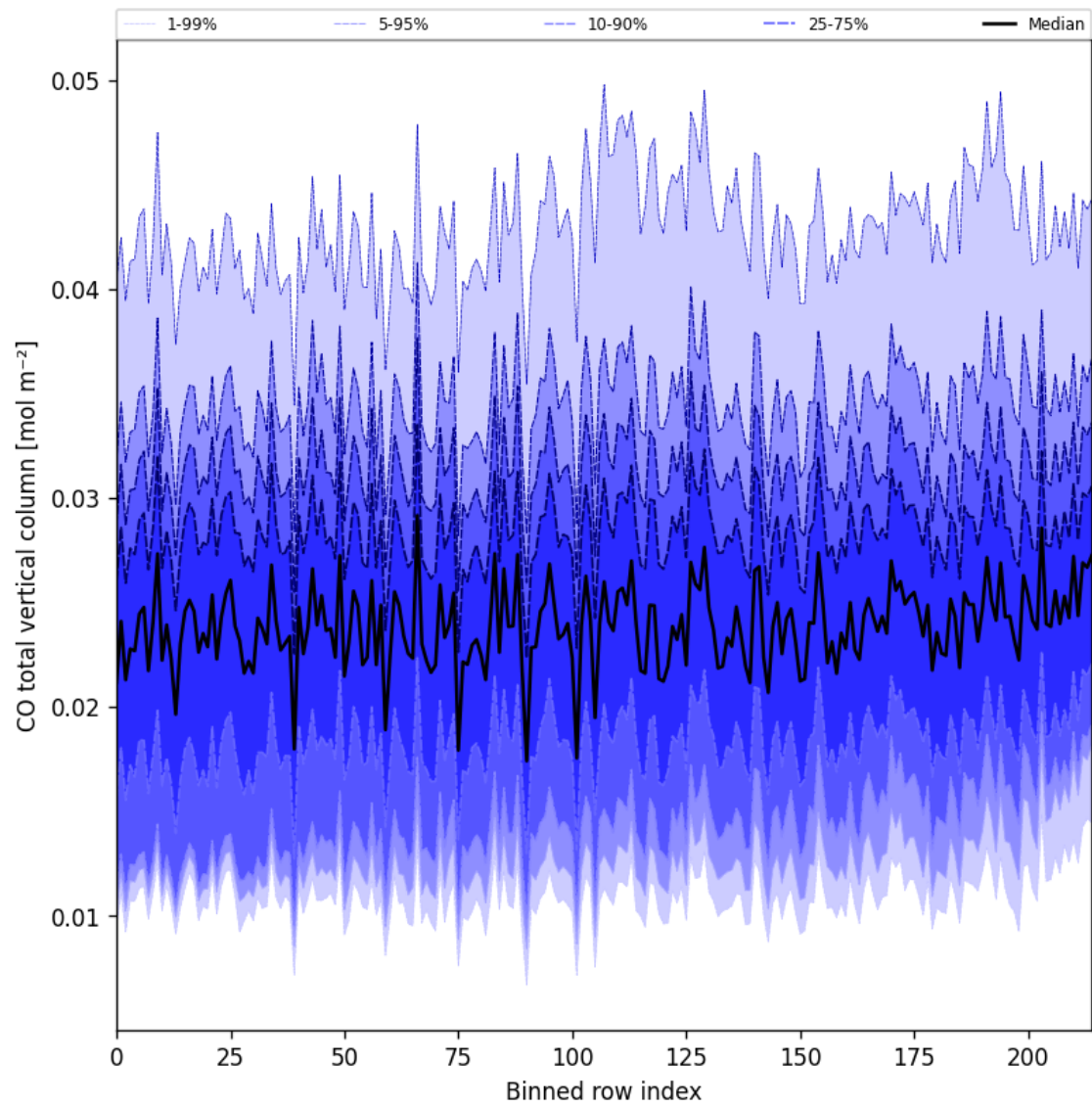
Figure 21: Along track statistics of “CO total vertical column” for 2025-10-24 to 2025-10-25
