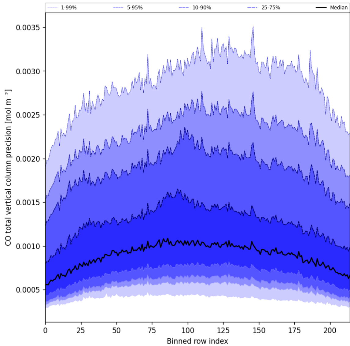
Figure 22: Along track statistics of “CO total vertical column precision” for 2025-10-24 to 2025-10-25
