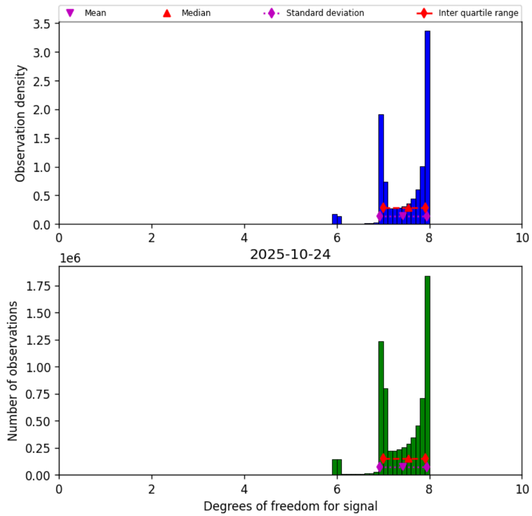
Figure 18: Histogram of “Degrees of freedom for signal” for 2025-10-24 to 2025-10-25
