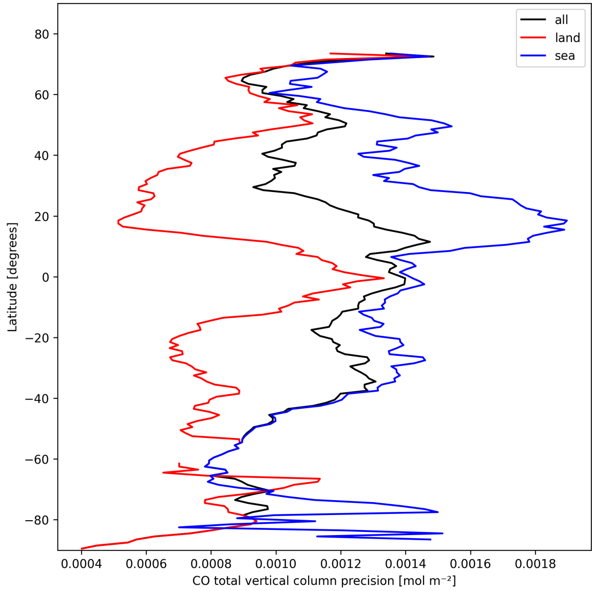
Figure 8: Zonal average of “CO total vertical column precision” for 2025-10-24 to 2025-10-25.
