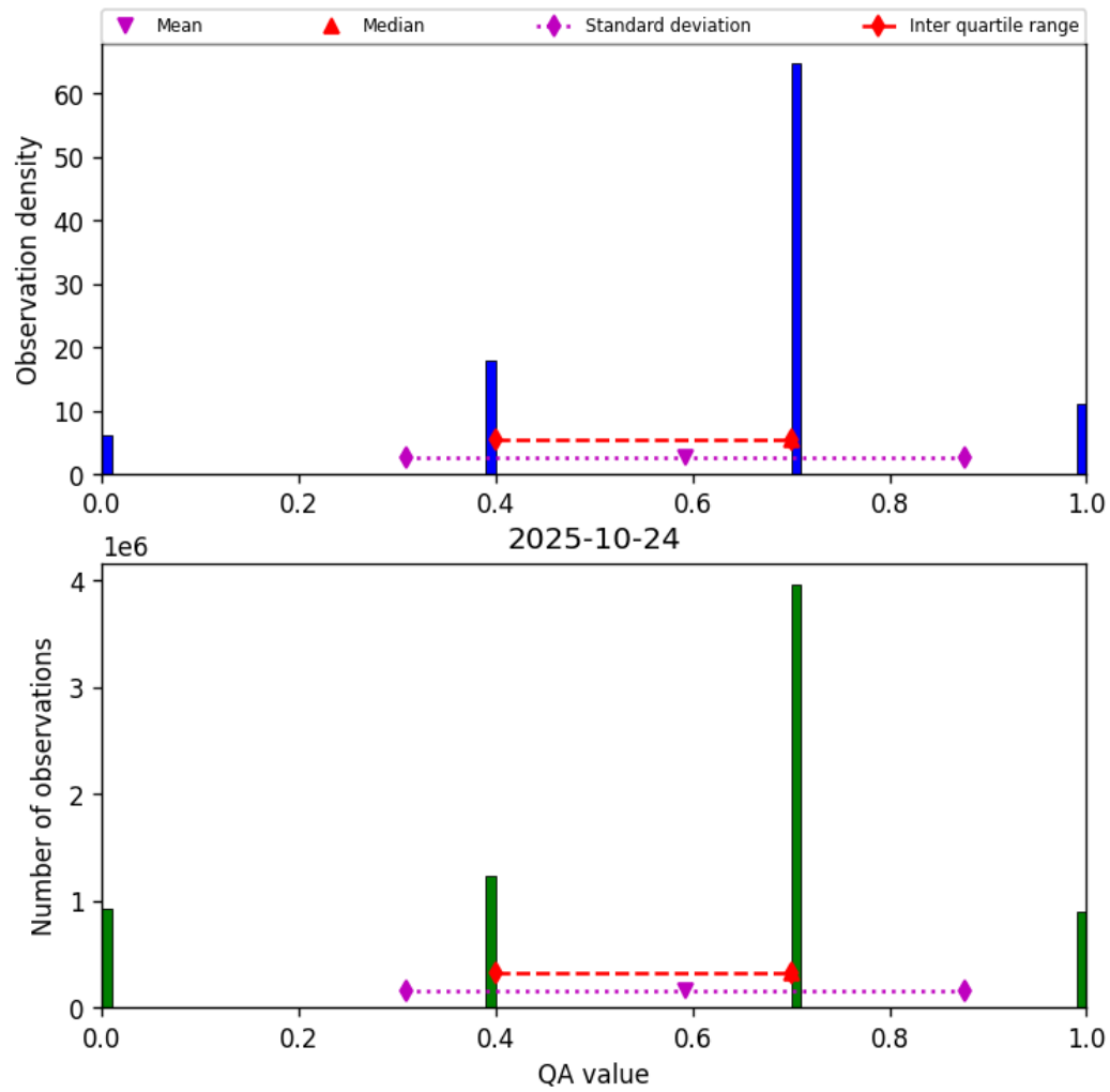
Figure 13: Histogram of “QA value” for 2025-10-24 to 2025-10-25
