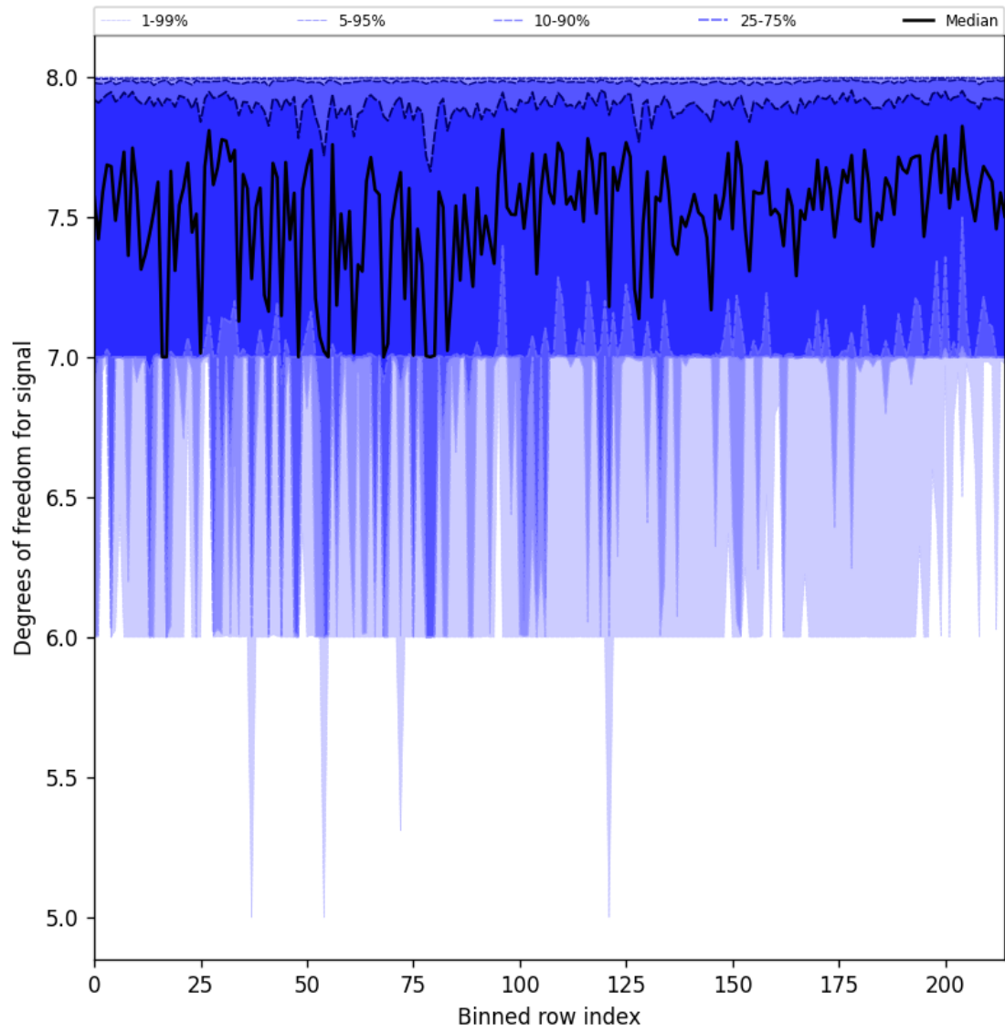
Figure 25: Along track statistics of “Degrees of freedom for signal” for 2025-10-24 to 2025-10-25
