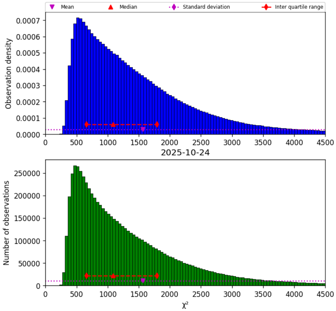
Figure 17: Histogram of “ \chi^2 ” for 2025-10-24 to 2025-10-25
