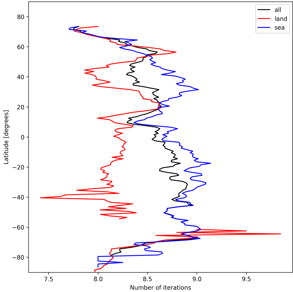
Figure 12: Zonal average of “Number of iterations” for 2025-10-24 to 2025-10-25.
