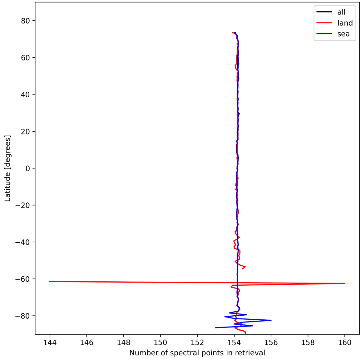
Figure 9: Zonal average of “Number of spectral points in retrieval” for 2025-10-24 to 2025-10-25.
