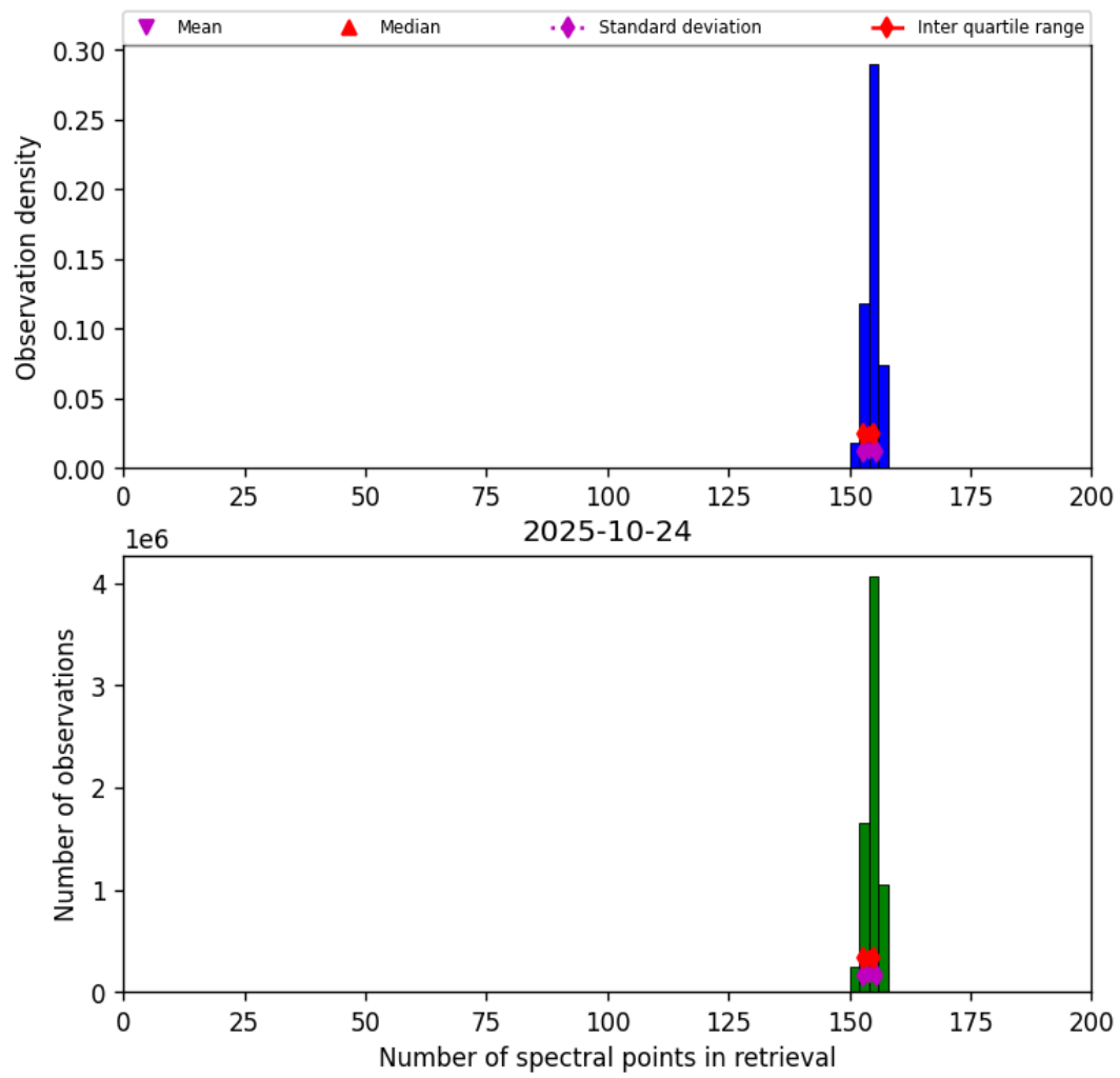
Figure 16: Histogram of “Number of spectral points in retrieval” for 2025-10-24 to 2025-10-25
