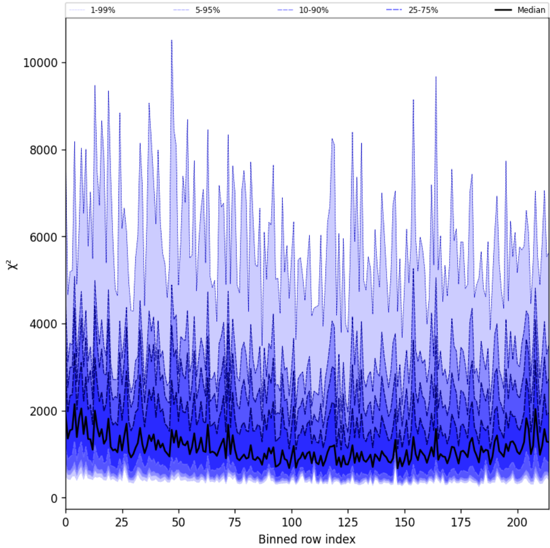
Figure 24: Along track statistics of “ \chi^2 ” for 2025-10-24 to 2025-10-25
