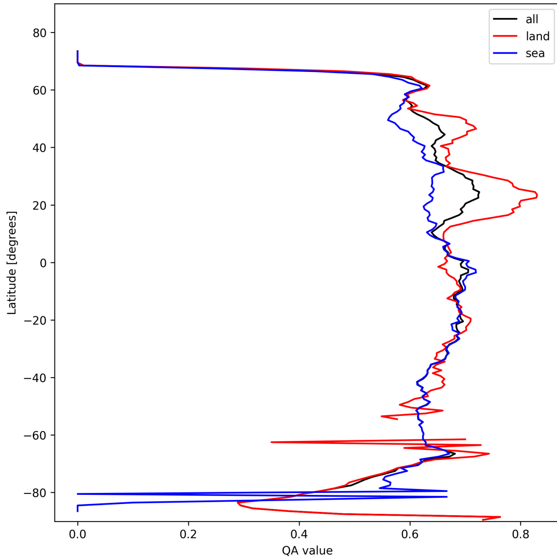
Figure 6: Zonal average of “QA value” for 2025-10-24 to 2025-10-25.
