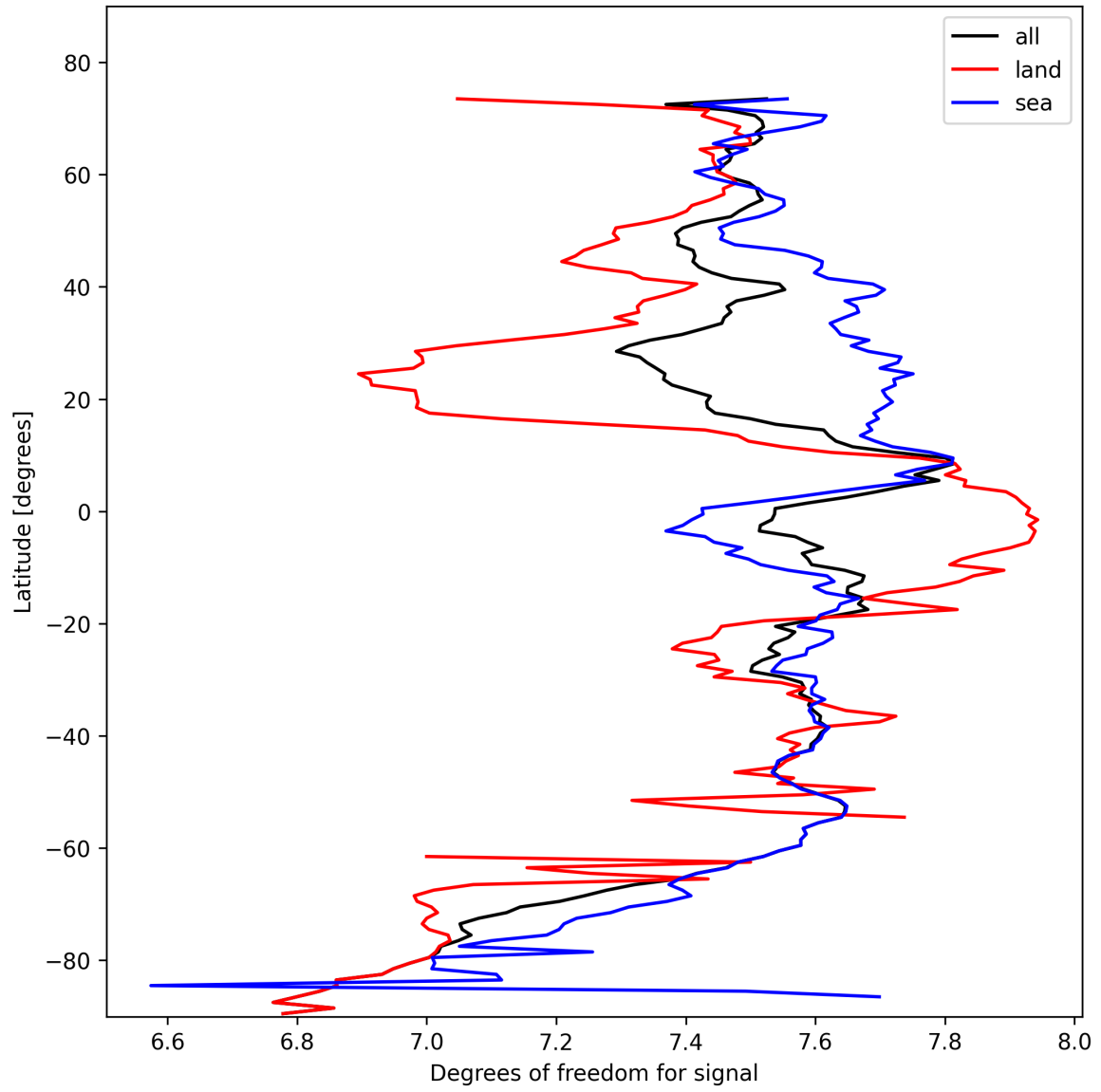
Figure 11: Zonal average of “Degrees of freedom for signal” for 2025-10-24 to 2025-10-25.
