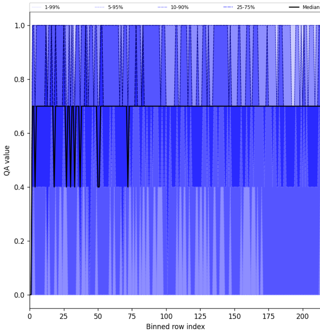
Figure 20: Along track statistics of “QA value” for 2025-10-24 to 2025-10-25
