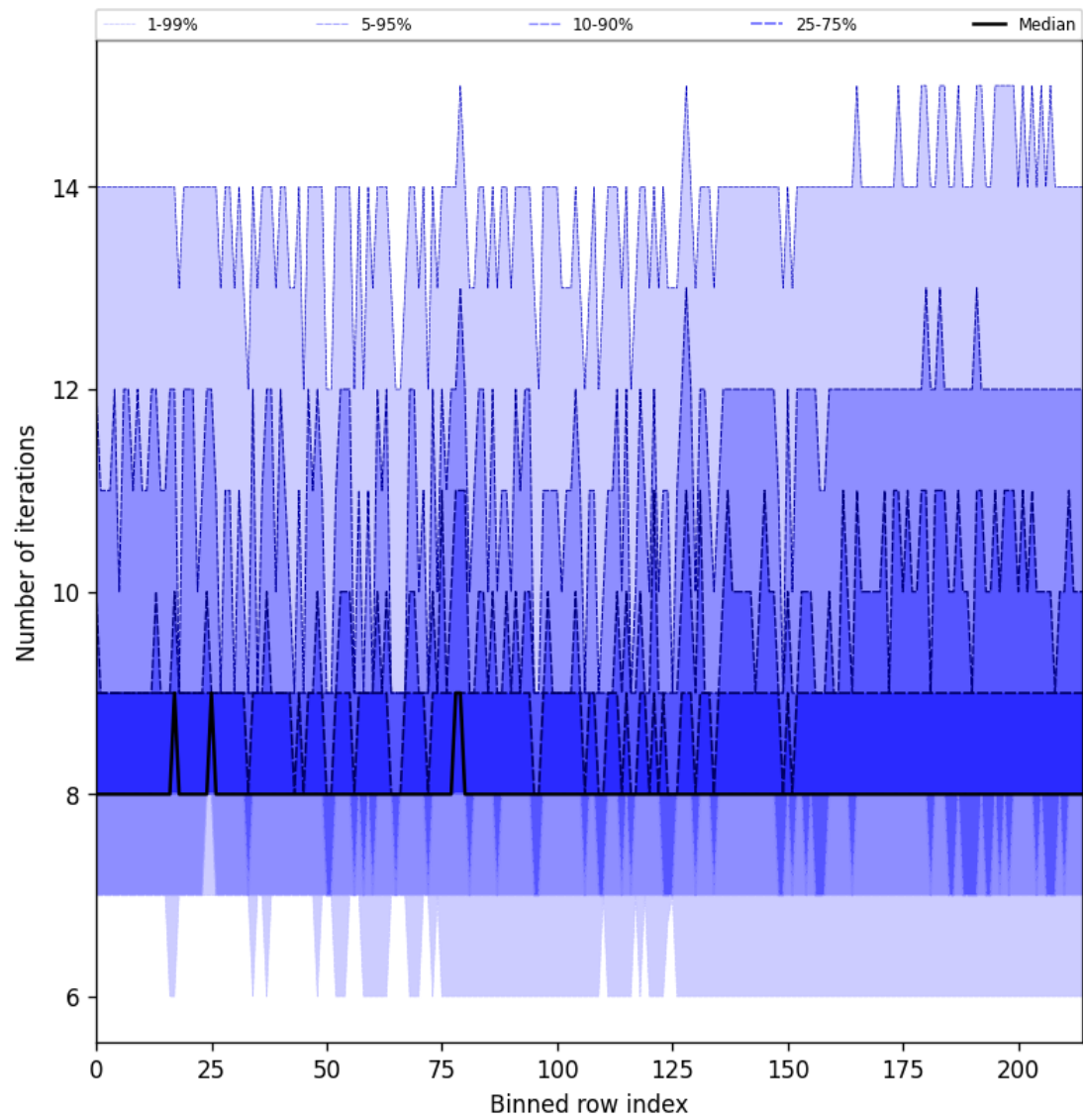
Figure 26: Along track statistics of “Number of iterations” for 2025-10-24 to 2025-10-25
