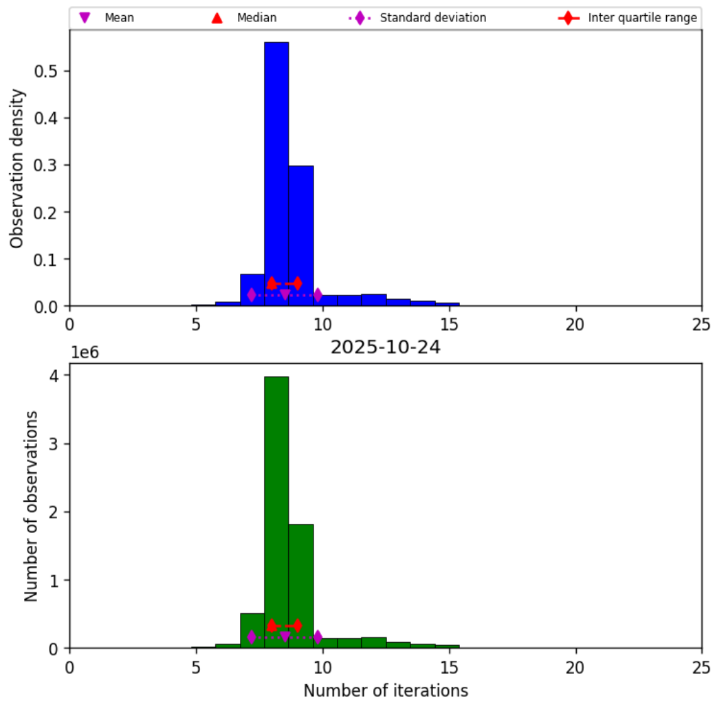
Figure 19: Histogram of “Number of iterations” for 2025-10-24 to 2025-10-25
