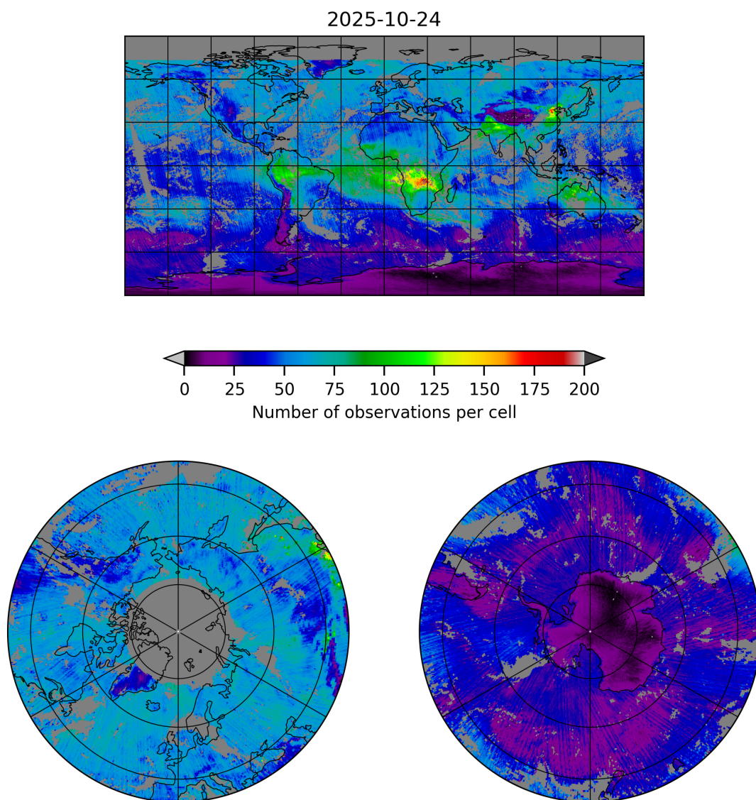
Figure 5: Map of the number of observations for 2025-10-24 to 2025-10-25
