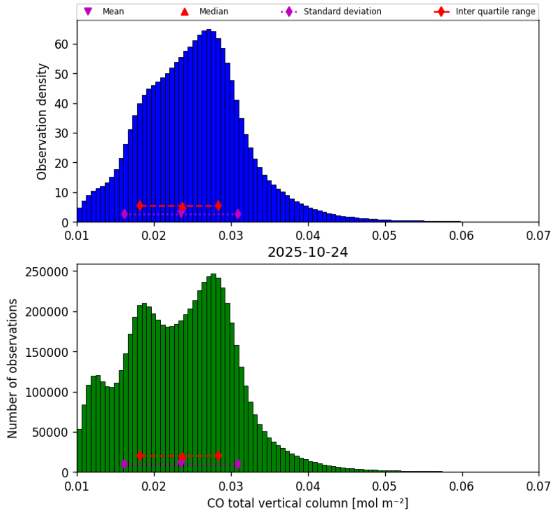
Figure 14: Histogram of “CO total vertical column” for 2025-10-24 to 2025-10-25
