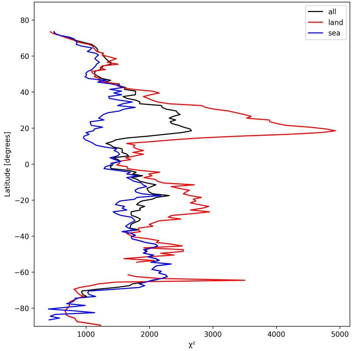
Figure 10: Zonal average of “ \chi^2 ” for 2025-10-24 to 2025-10-25.
