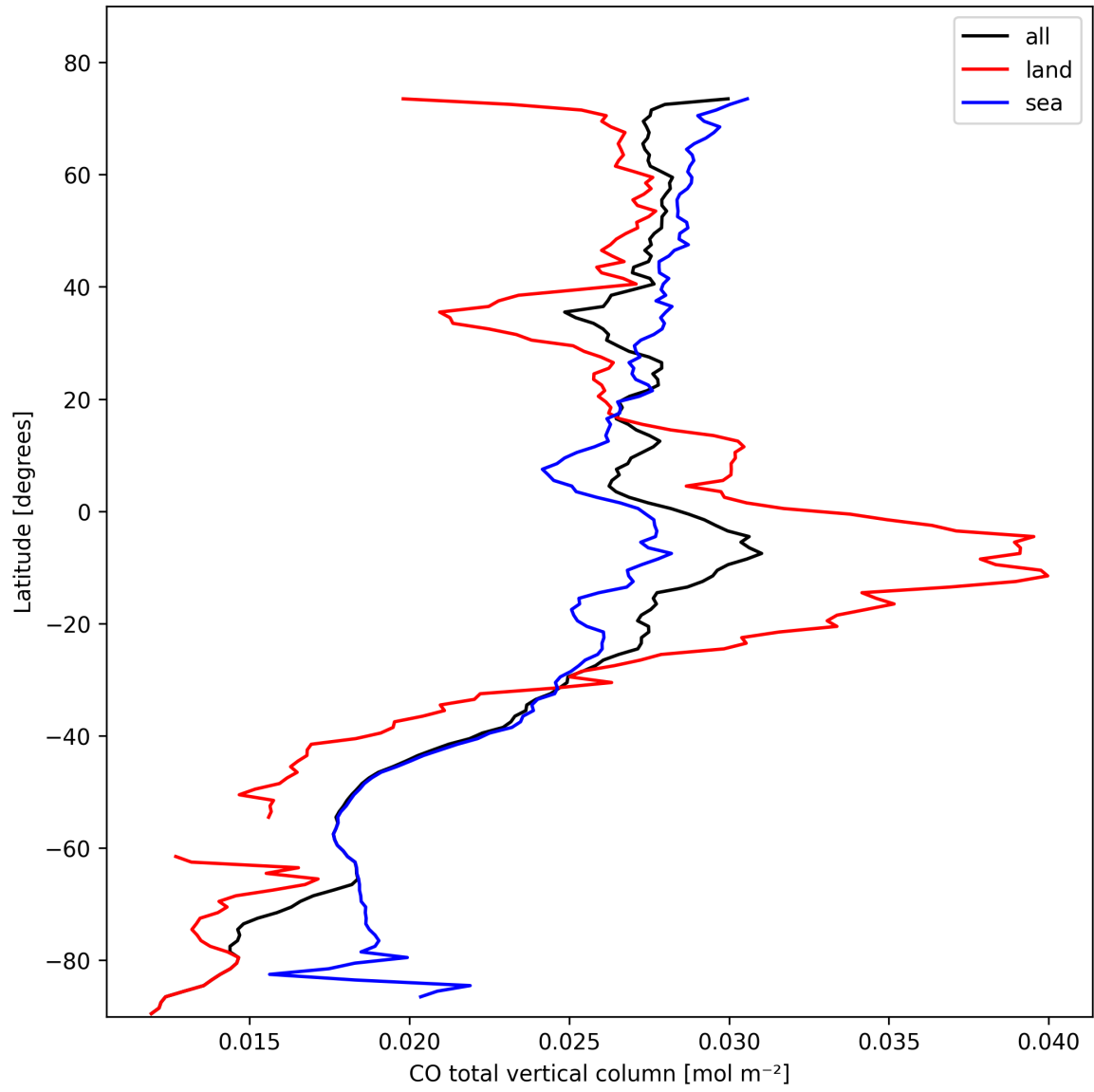
Figure 7: Zonal average of “CO total vertical column” for 2025-10-24 to 2025-10-25.
