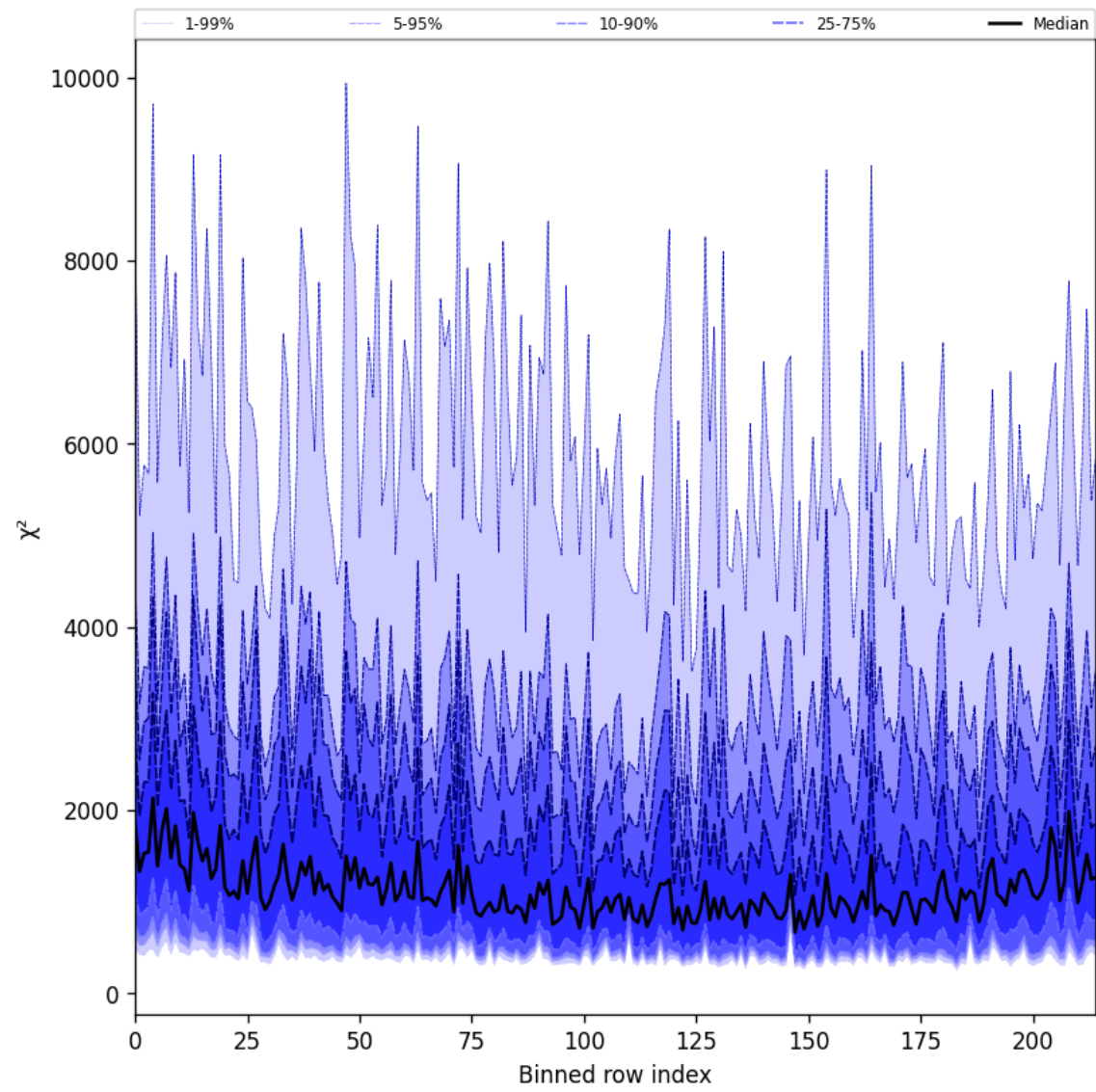
Figure 24: Along track statistics of “ \chi^2 ” for 2025-10-25 to 2025-10-25
