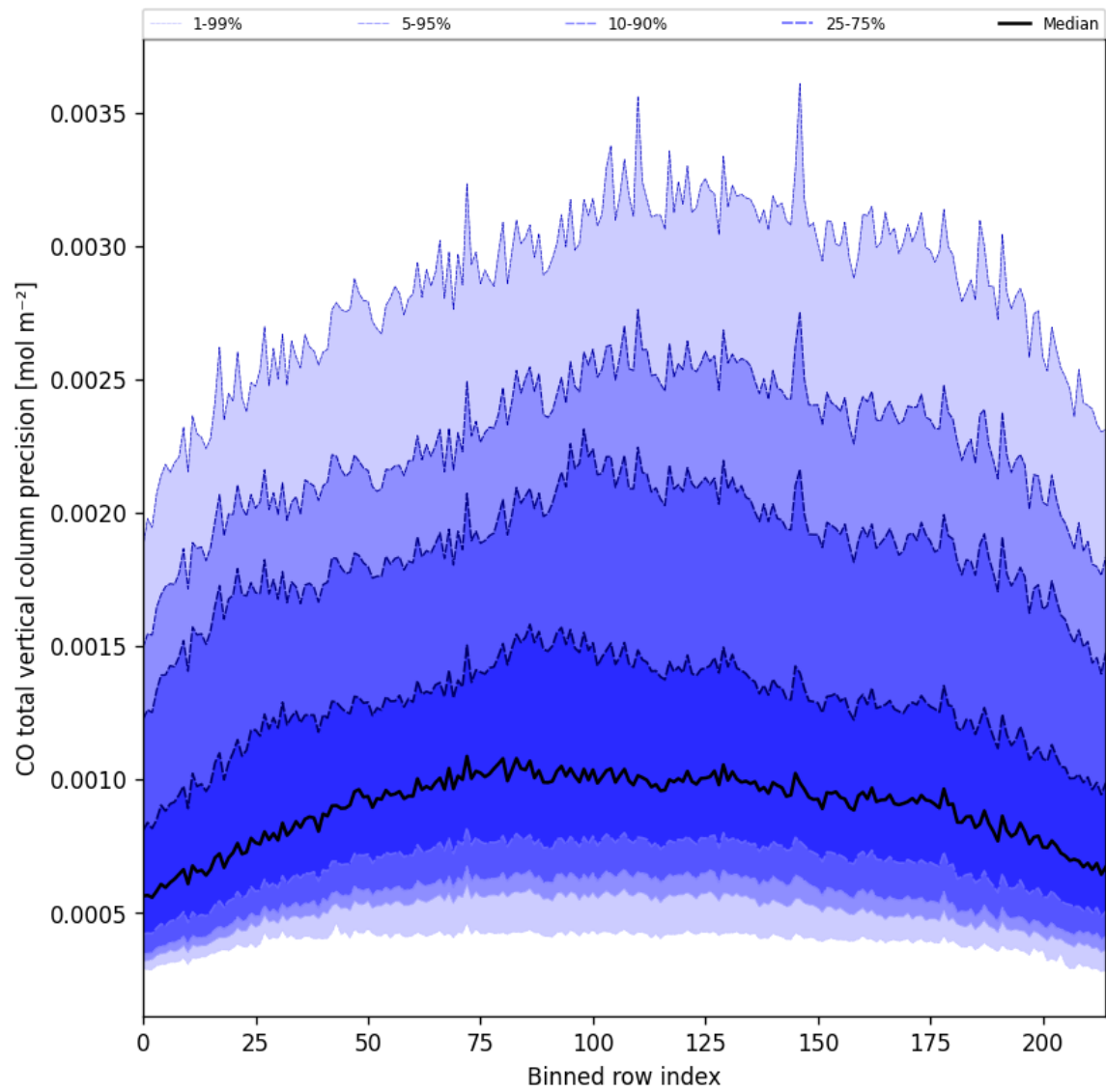
Figure 22: Along track statistics of “CO total vertical column precision” for 2025-10-25 to 2025-10-25
