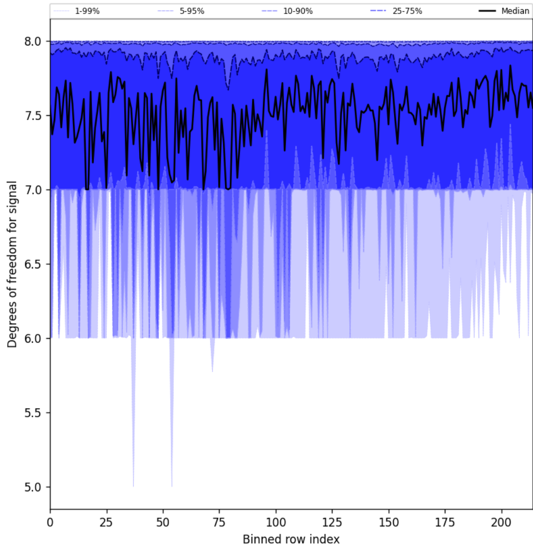
Figure 25: Along track statistics of “Degrees of freedom for signal” for 2025-10-25 to 2025-10-25
