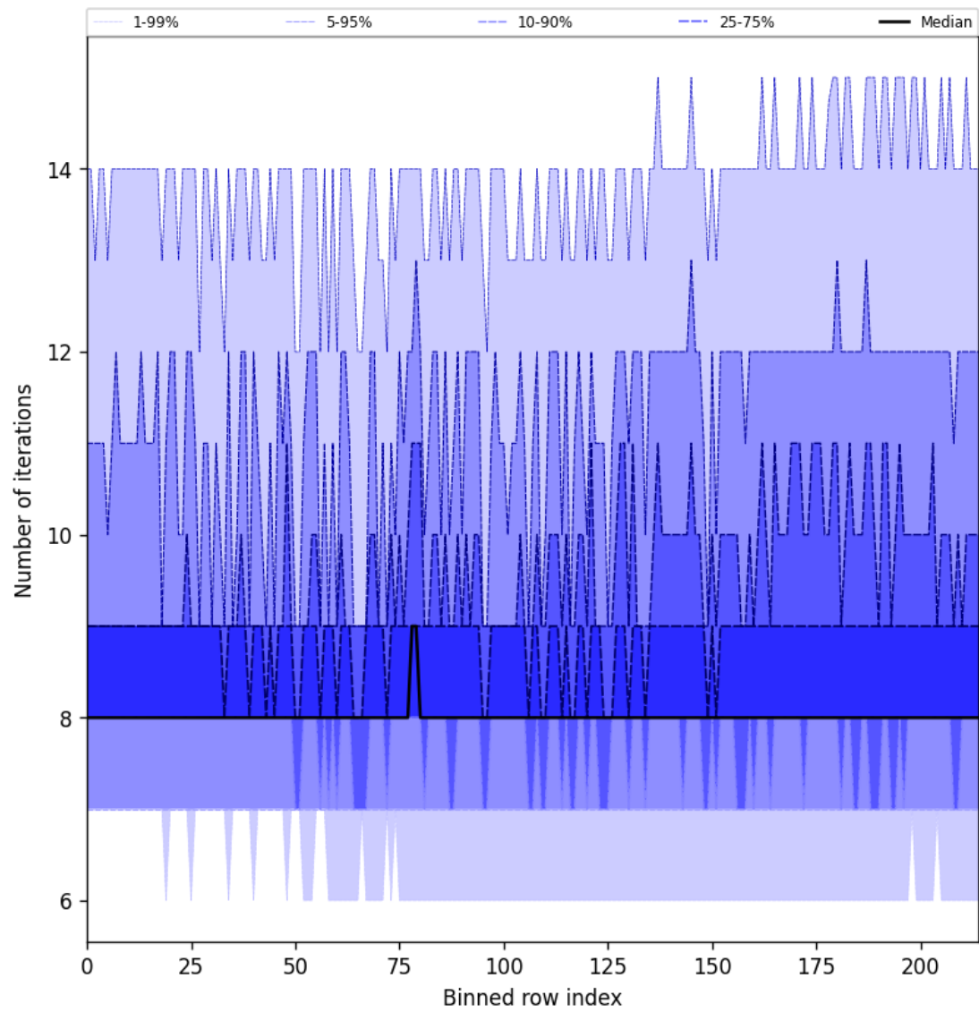
Figure 26: Along track statistics of “Number of iterations” for 2025-10-25 to 2025-10-25
