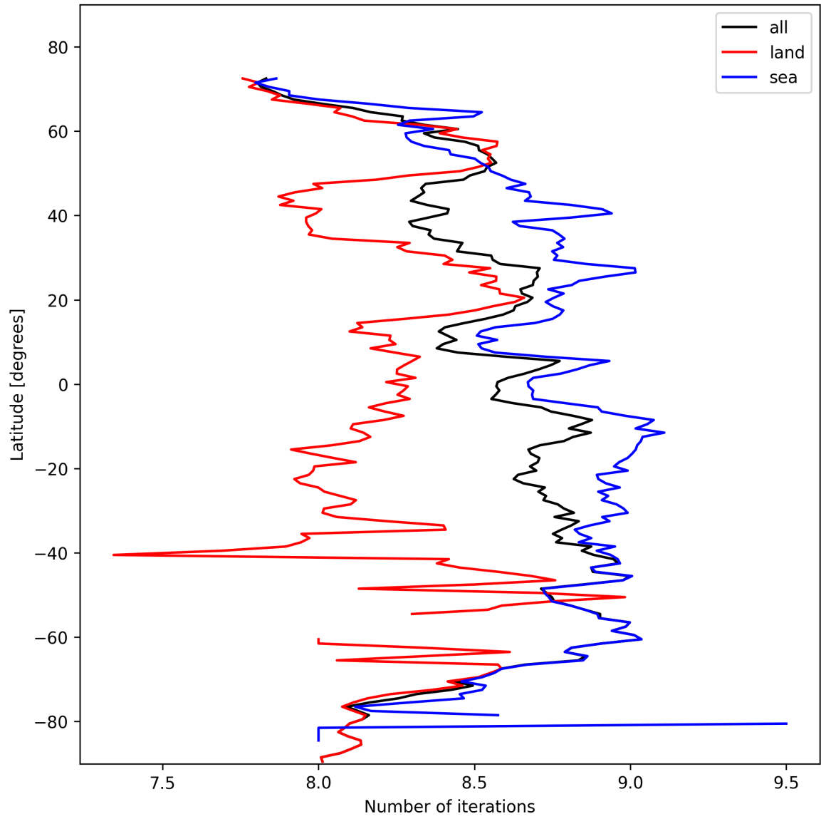
Figure 12: Zonal average of “Number of iterations” for 2025-10-25 to 2025-10-25.
