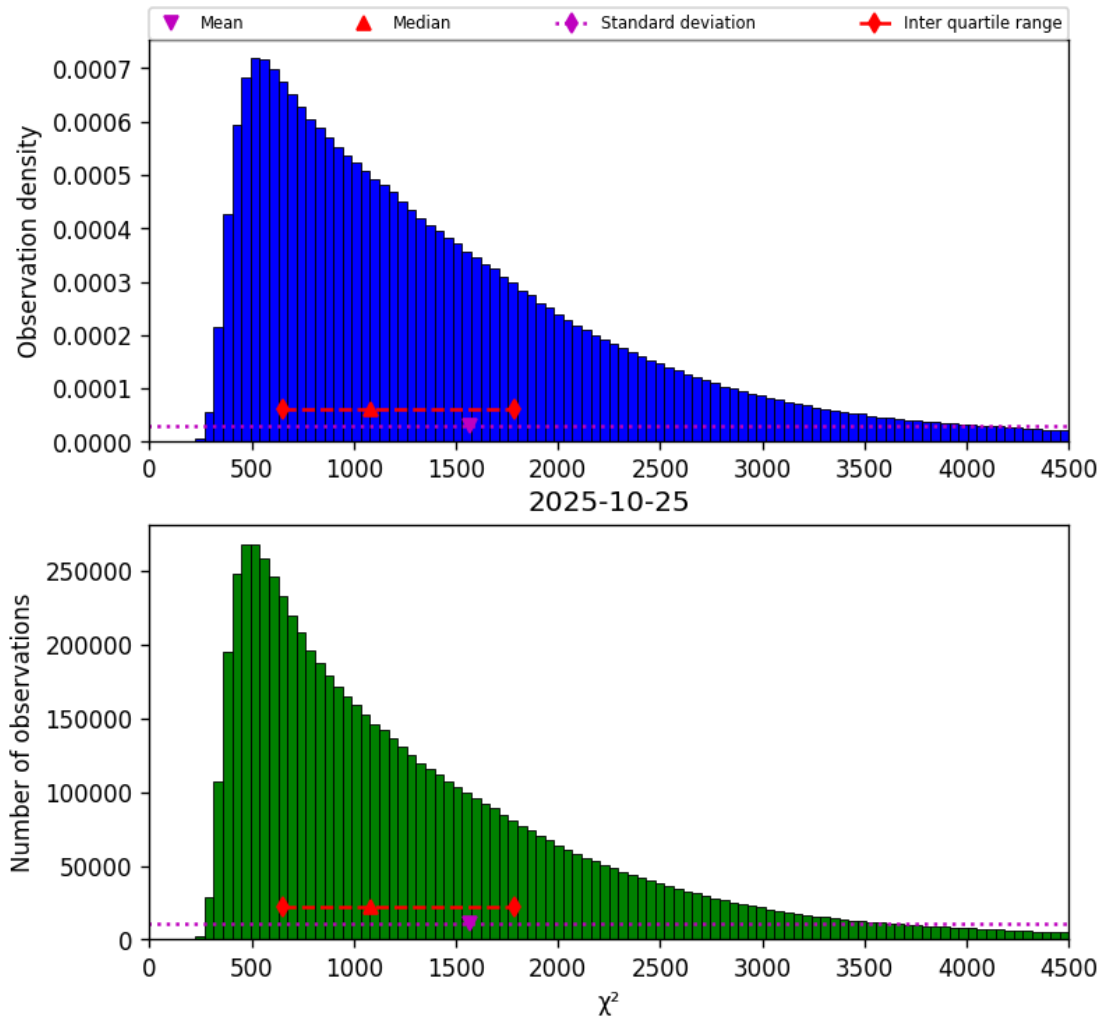
Figure 17: Histogram of “ \chi^2 ” for 2025-10-25 to 2025-10-25
