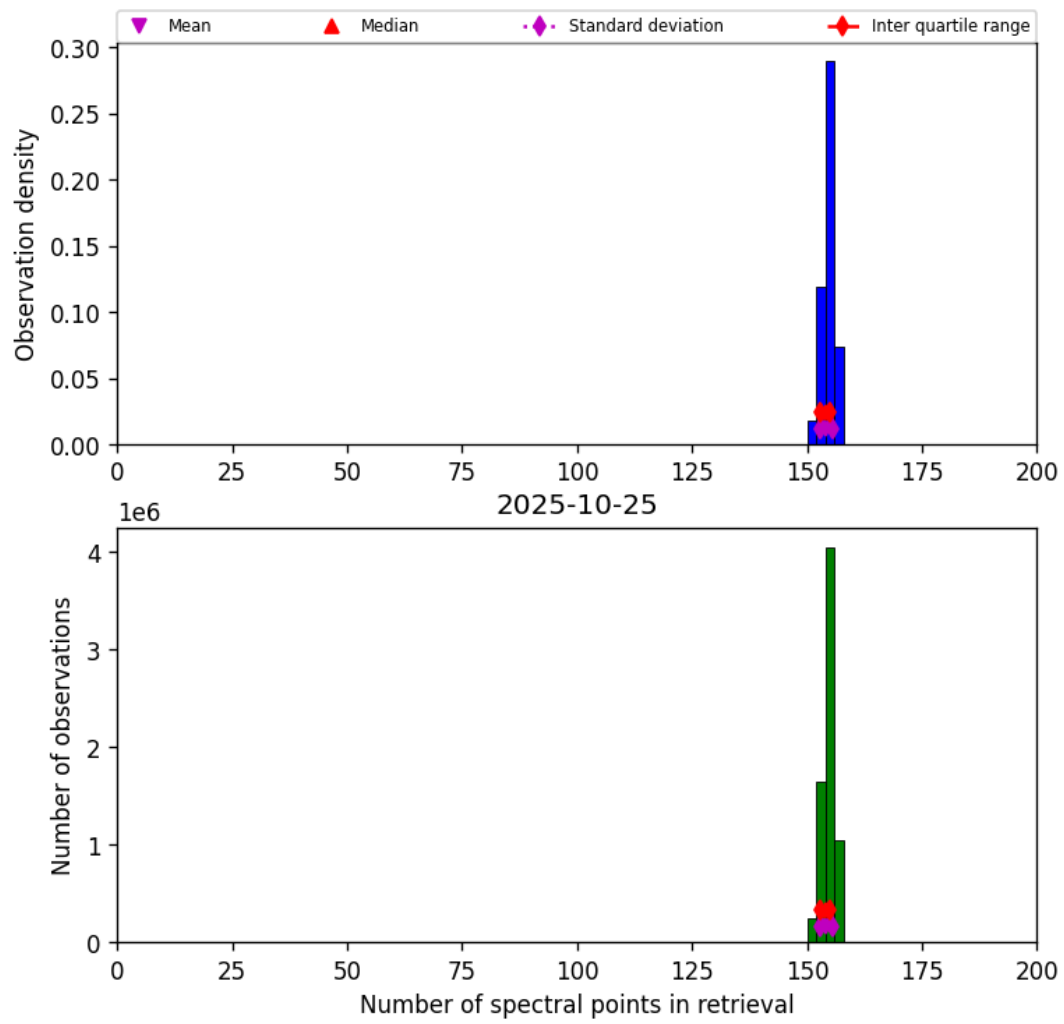
Figure 16: Histogram of “Number of spectral points in retrieval” for 2025-10-25 to 2025-10-25
