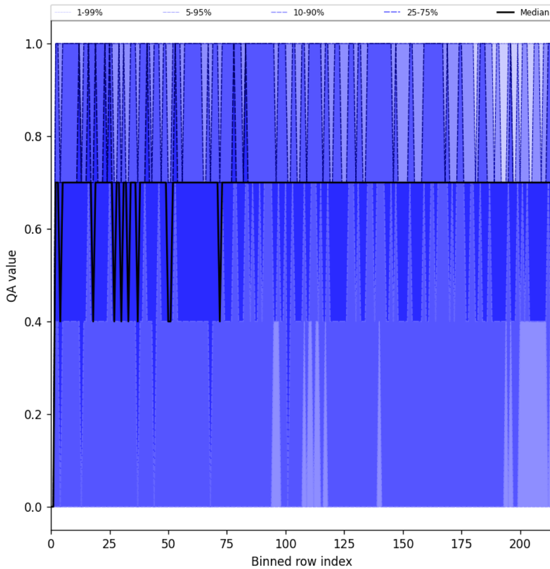
Figure 20: Along track statistics of “QA value” for 2025-10-25 to 2025-10-25
