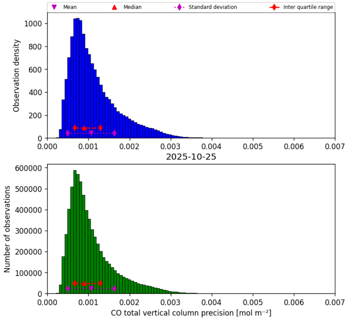
Figure 15: Histogram of “CO total vertical column precision” for 2025-10-25 to 2025-10-25
