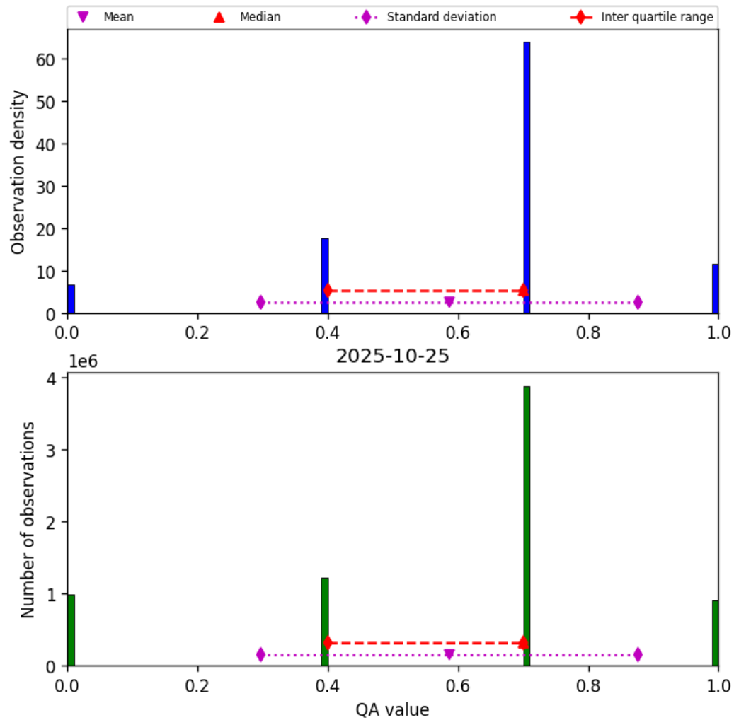
Figure 13: Histogram of “QA value” for 2025-10-25 to 2025-10-25
