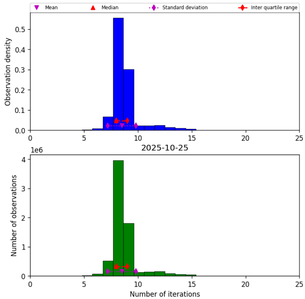
Figure 19: Histogram of “Number of iterations” for 2025-10-25 to 2025-10-25
