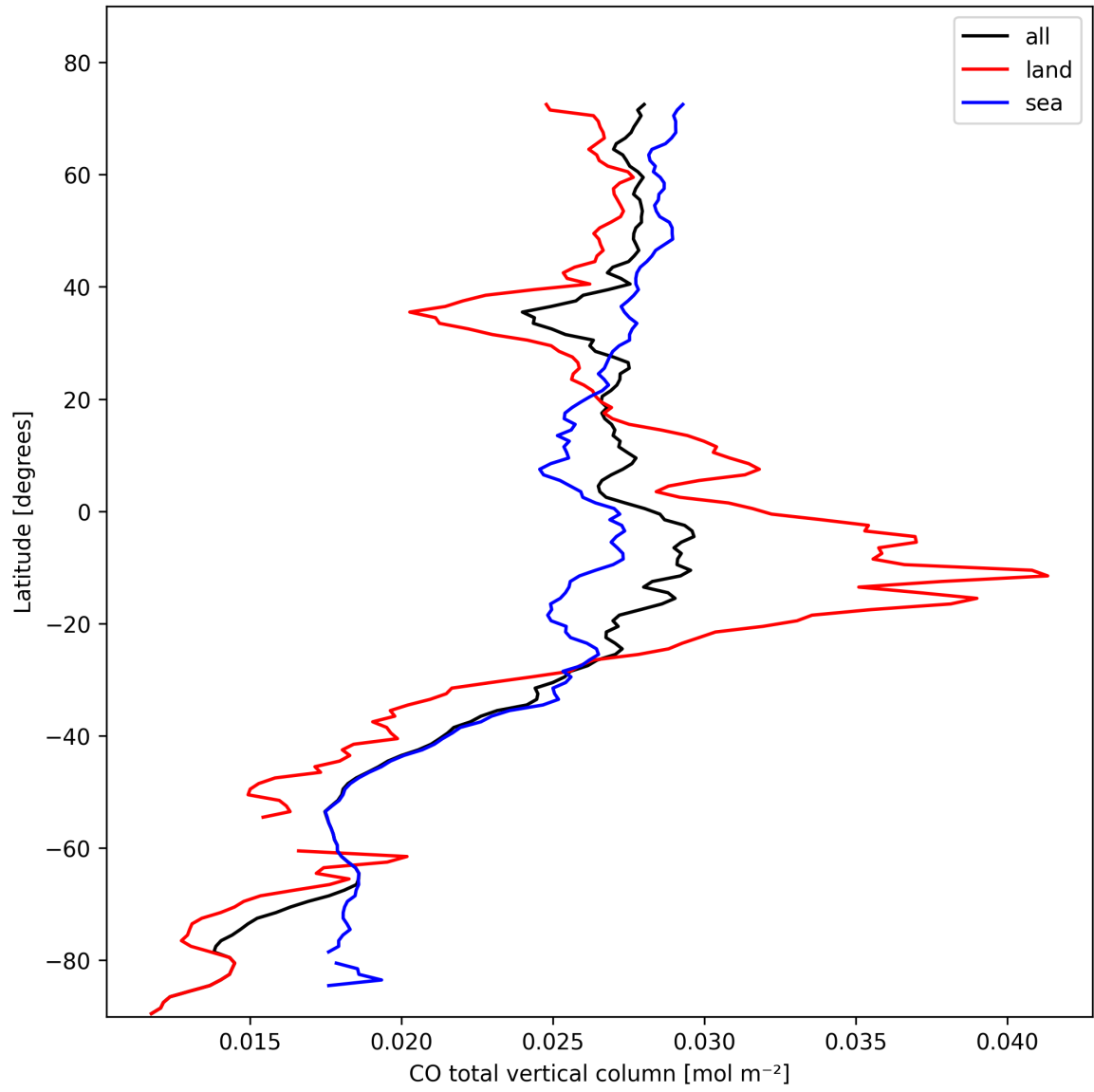
Figure 7: Zonal average of “CO total vertical column” for 2025-10-25 to 2025-10-25.
