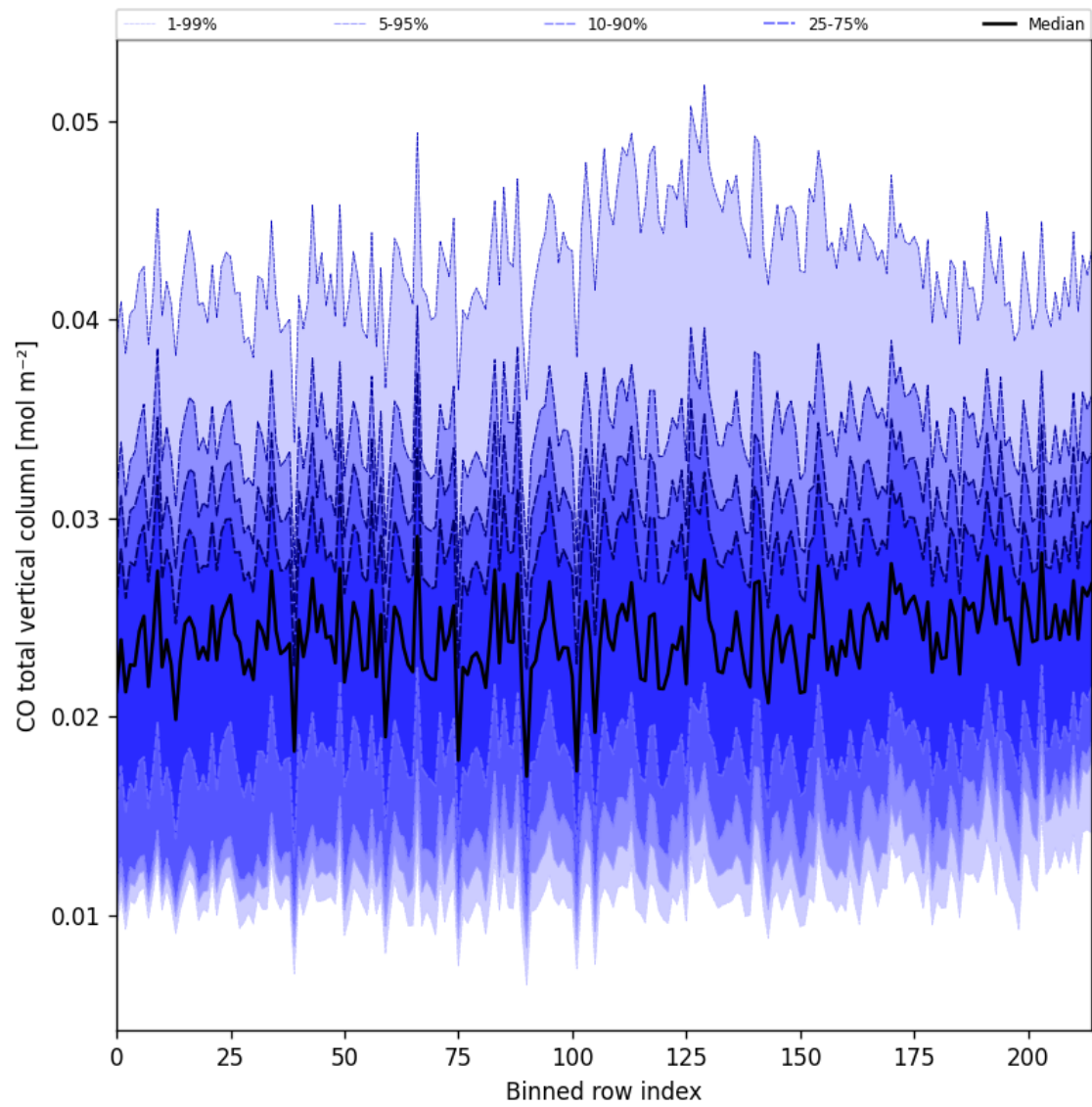
Figure 21: Along track statistics of “CO total vertical column” for 2025-10-25 to 2025-10-25
