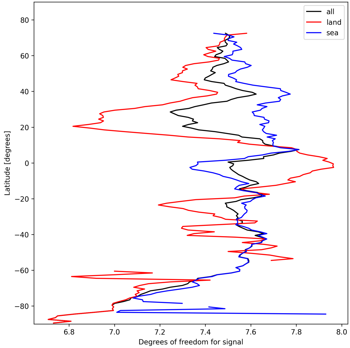
Figure 11: Zonal average of “Degrees of freedom for signal” for 2025-10-25 to 2025-10-25.
