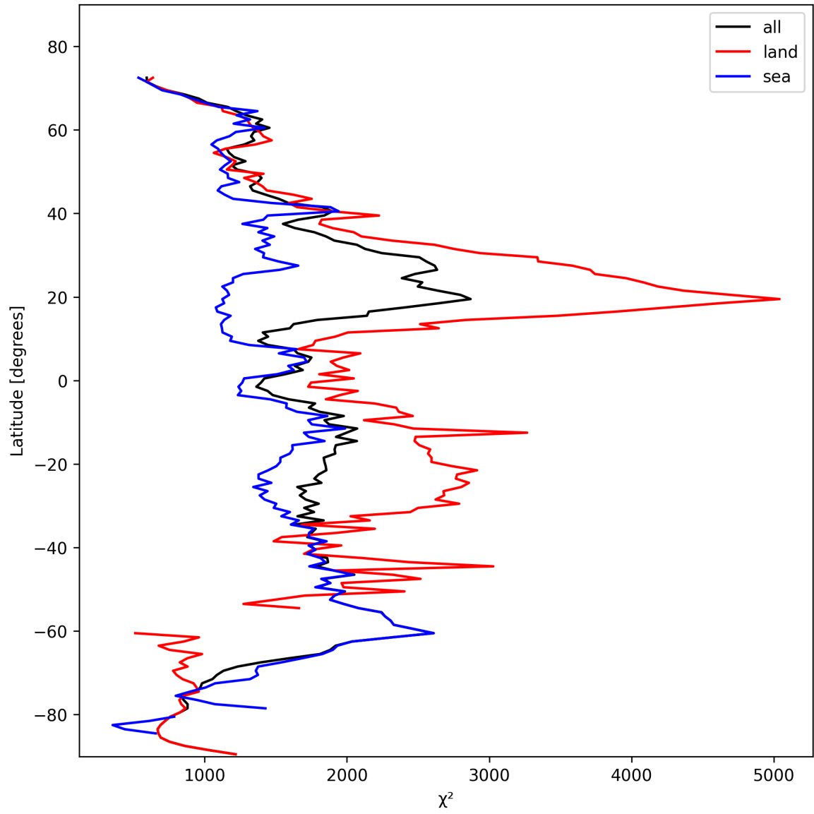
Figure 10: Zonal average of “ \chi^2 ” for 2025-10-25 to 2025-10-25.
