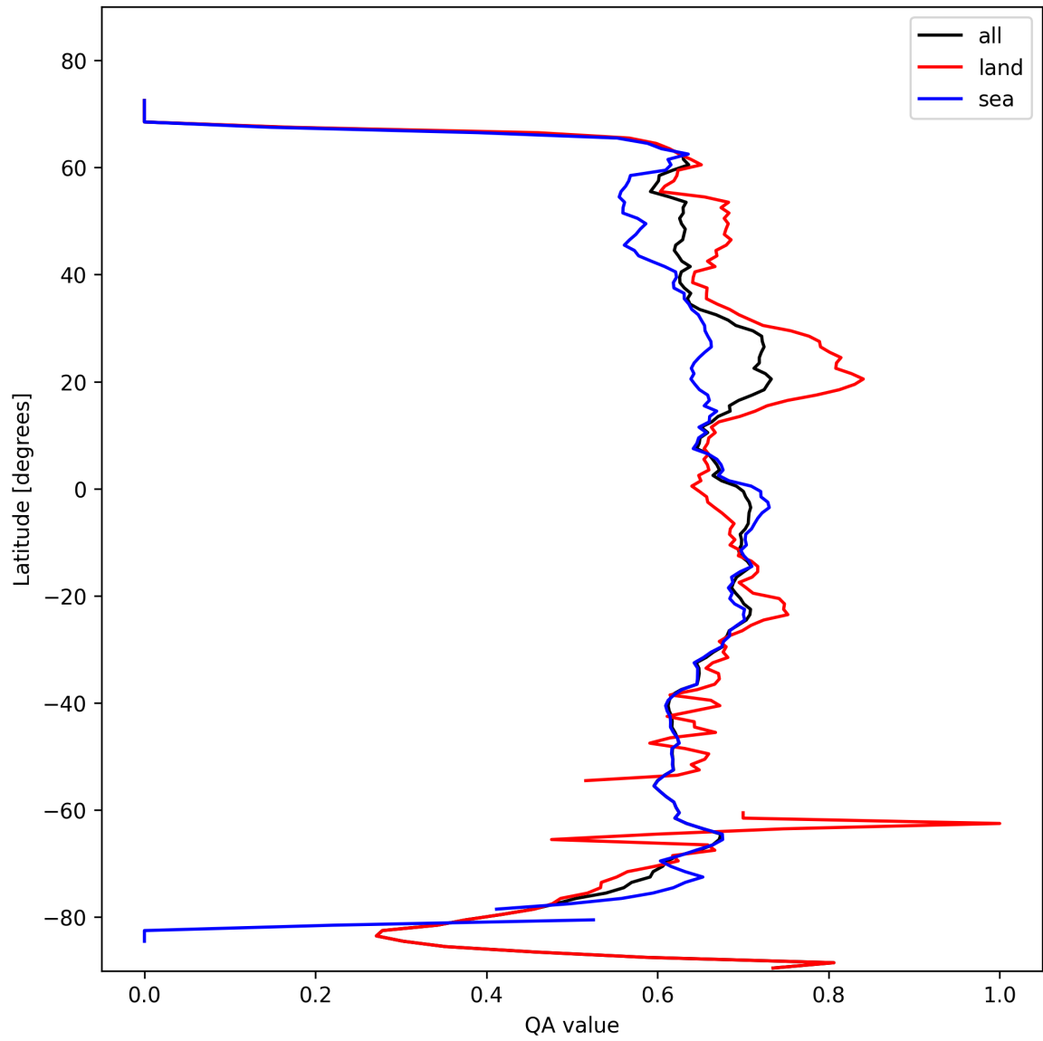
Figure 6: Zonal average of “QA value” for 2025-10-25 to 2025-10-25.
