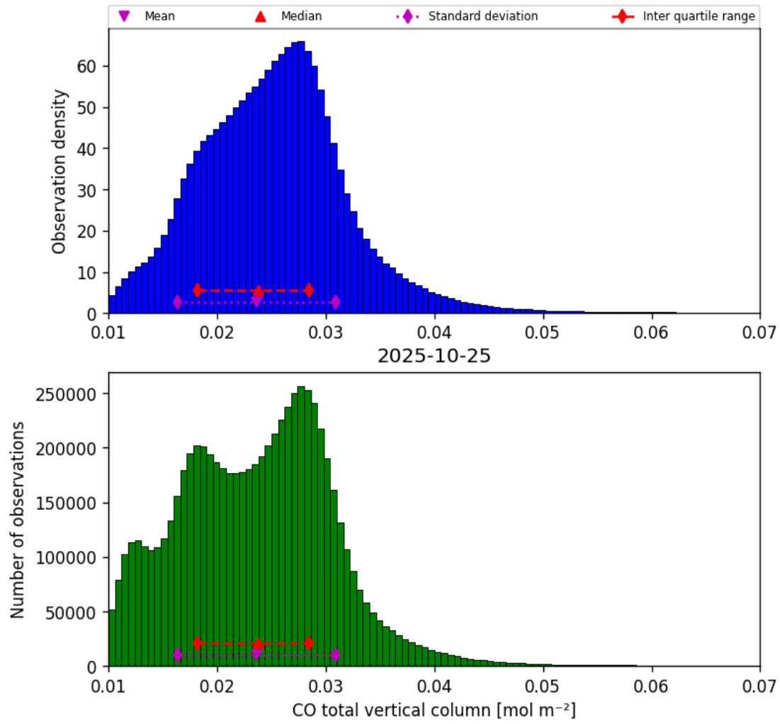
Figure 14: Histogram of “CO total vertical column” for 2025-10-25 to 2025-10-25
