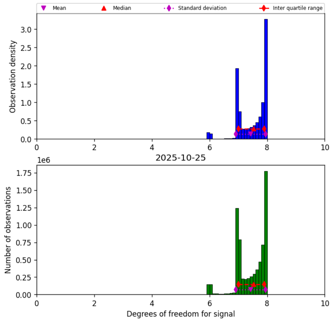
Figure 18: Histogram of “Degrees of freedom for signal” for 2025-10-25 to 2025-10-25
