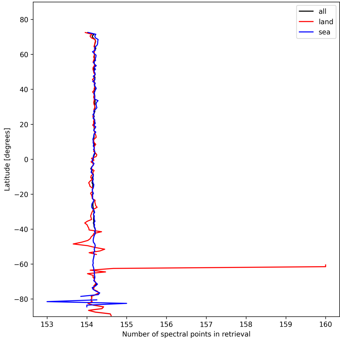
Figure 9: Zonal average of “Number of spectral points in retrieval” for 2025-10-25 to 2025-10-25.
