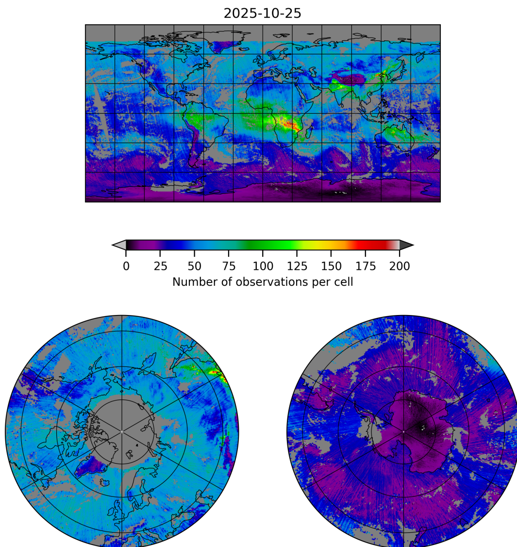
Figure 5: Map of the number of observations for 2025-10-25 to 2025-10-25
