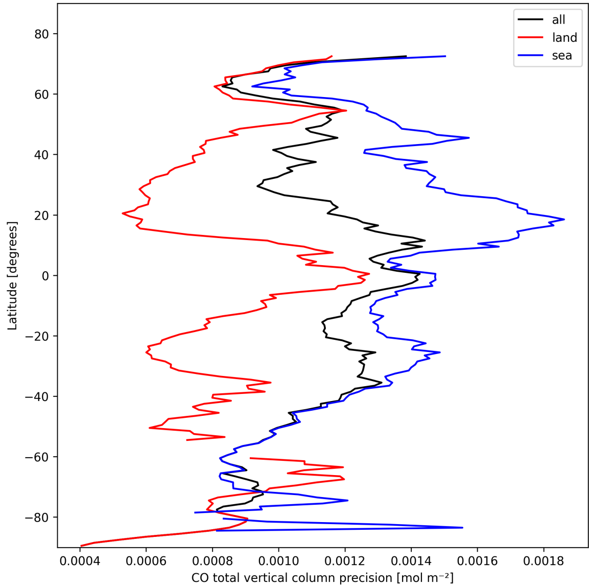
Figure 8: Zonal average of “CO total vertical column precision” for 2025-10-25 to 2025-10-25.
