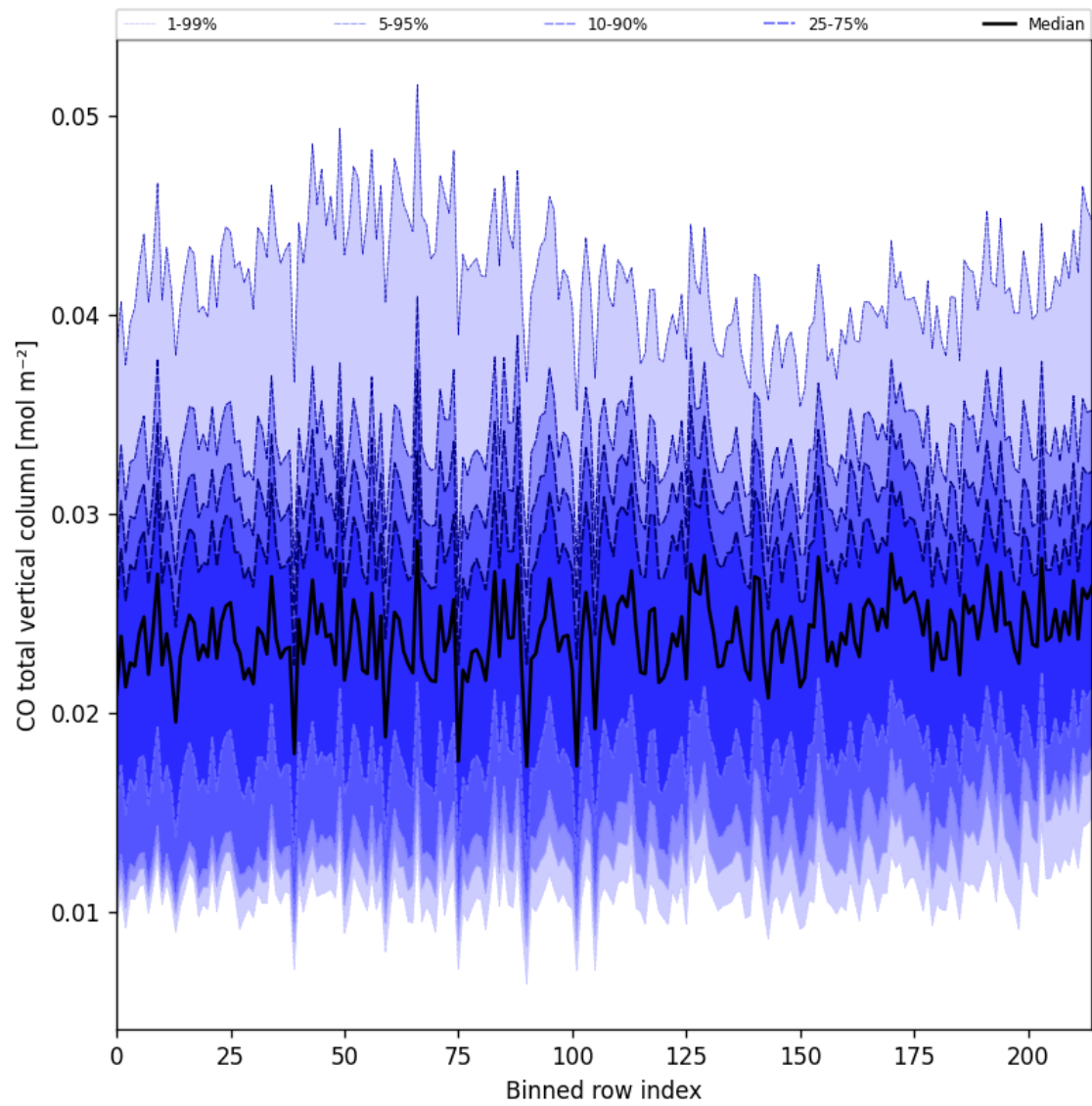
Figure 21: Along track statistics of “CO total vertical column” for 2025-10-26 to 2025-10-27
