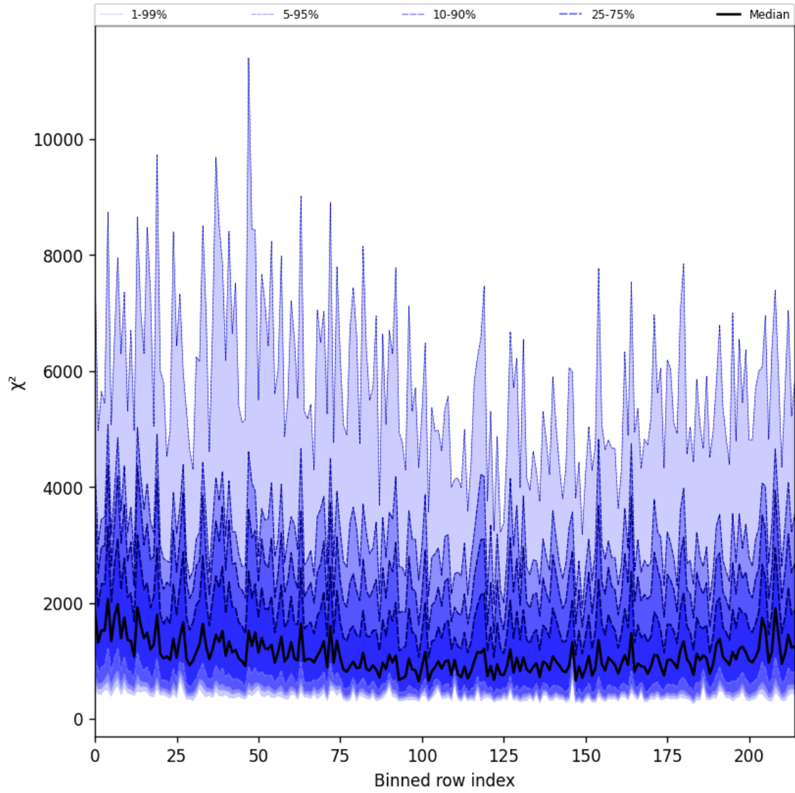
Figure 24: Along track statistics of “ \chi^2 ” for 2025-10-26 to 2025-10-27
