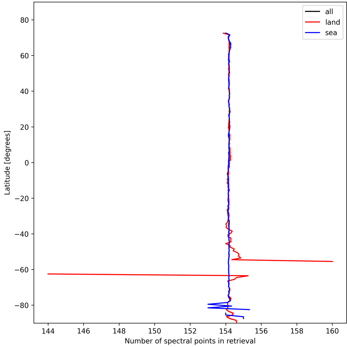
Figure 9: Zonal average of “Number of spectral points in retrieval” for 2025-10-26 to 2025-10-27.
