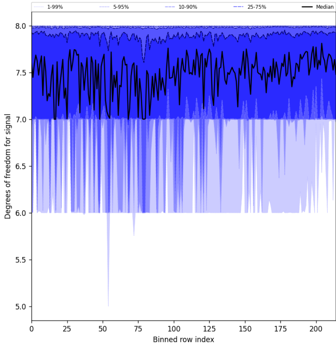
Figure 25: Along track statistics of “Degrees of freedom for signal” for 2025-10-26 to 2025-10-27
