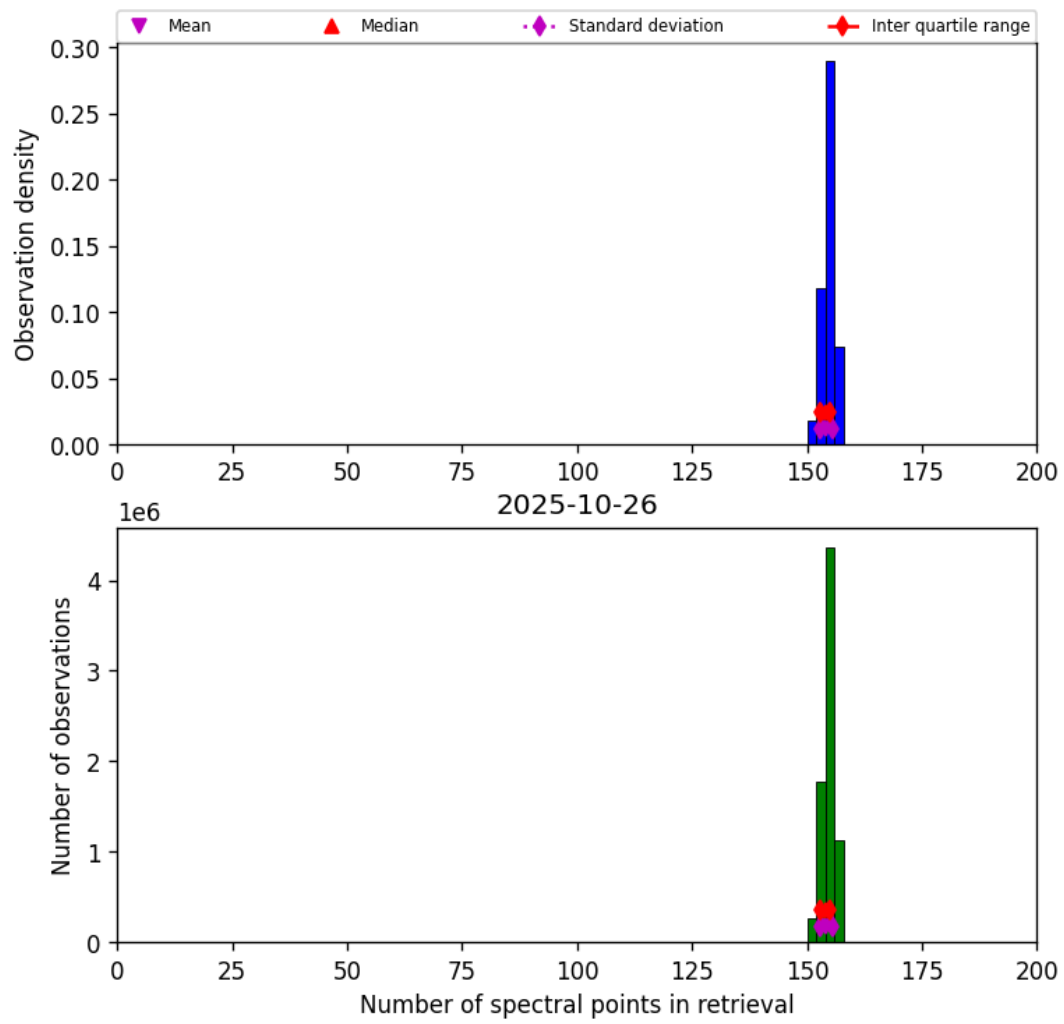
Figure 16: Histogram of “Number of spectral points in retrieval” for 2025-10-26 to 2025-10-27
