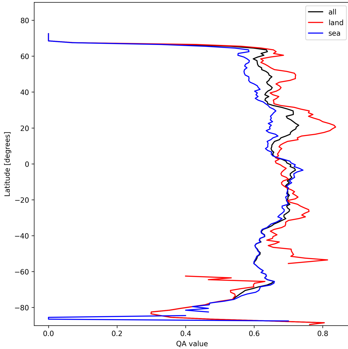
Figure 6: Zonal average of “QA value” for 2025-10-26 to 2025-10-27.
