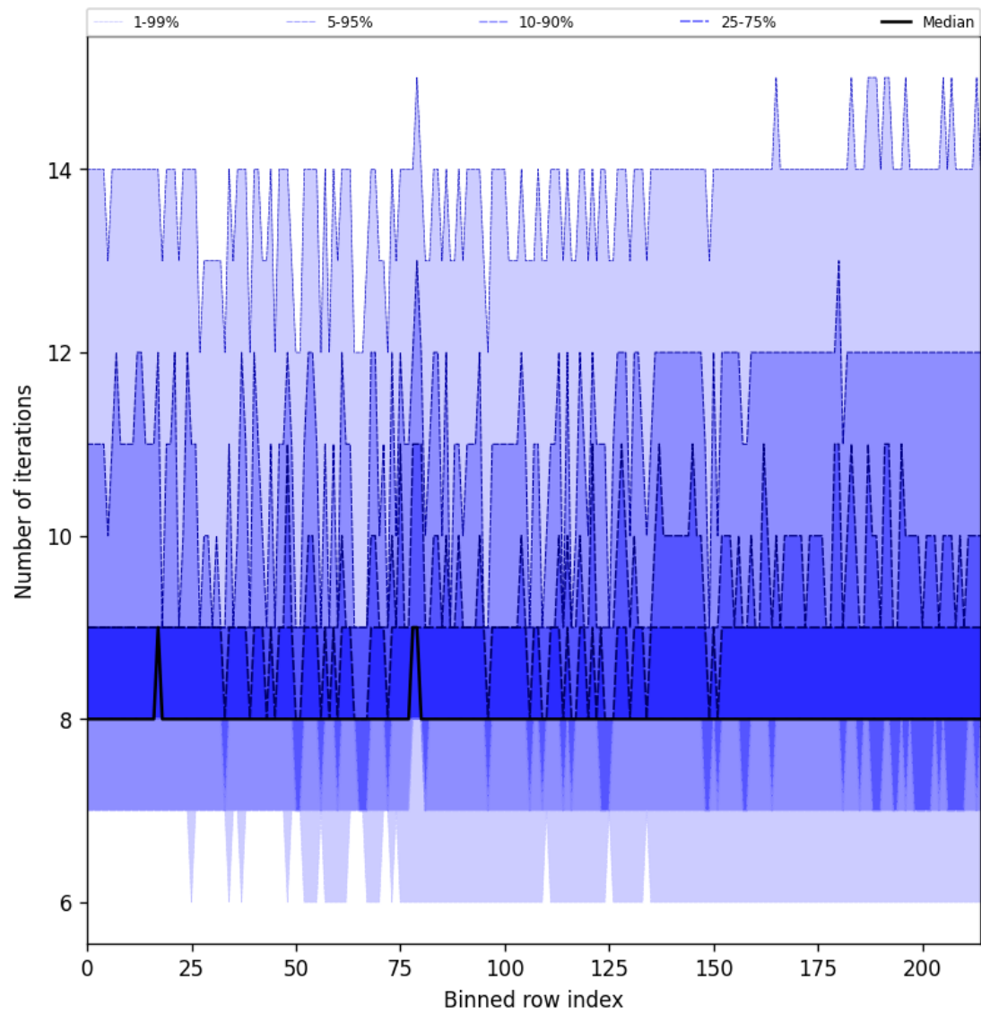
Figure 26: Along track statistics of “Number of iterations” for 2025-10-26 to 2025-10-27
