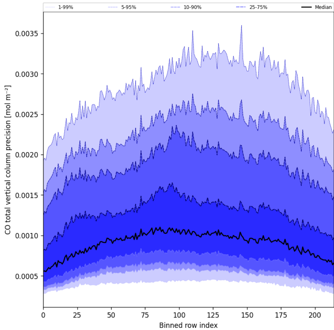
Figure 22: Along track statistics of “CO total vertical column precision” for 2025-10-26 to 2025-10-27
