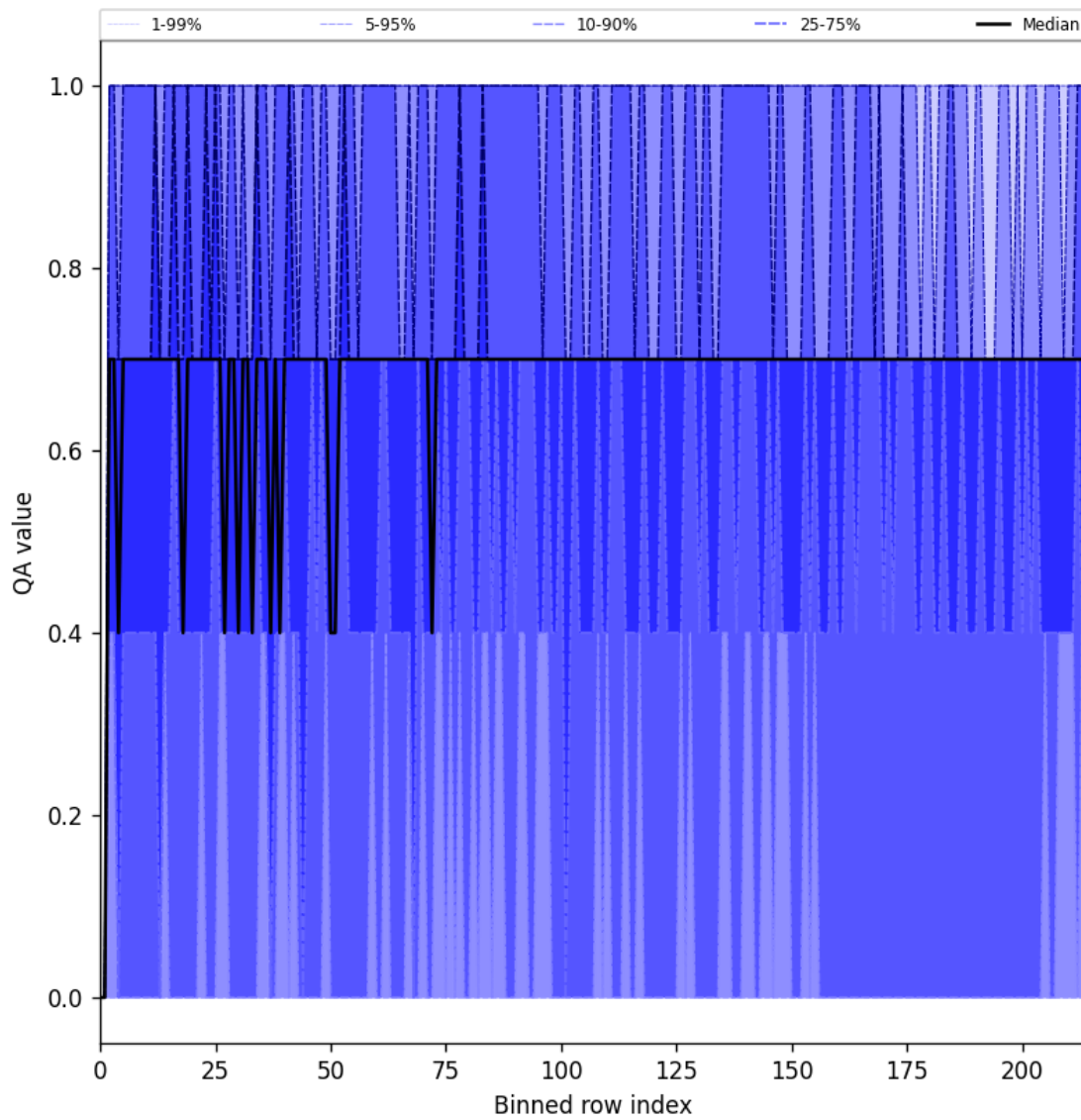
Figure 20: Along track statistics of “QA value” for 2025-10-26 to 2025-10-27
