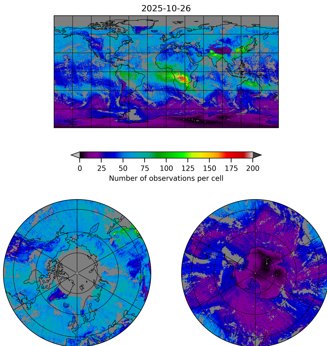
Figure 5: Map of the number of observations for 2025-10-26 to 2025-10-27
