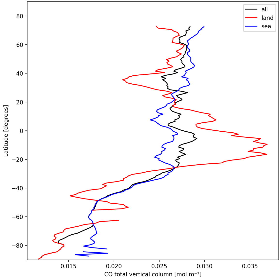
Figure 7: Zonal average of “CO total vertical column” for 2025-10-26 to 2025-10-27.
