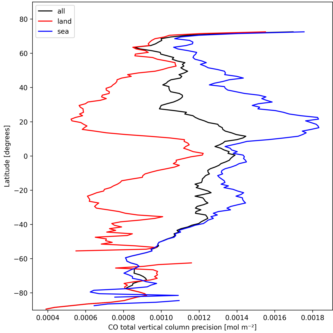
Figure 8: Zonal average of “CO total vertical column precision” for 2025-10-26 to 2025-10-27.
