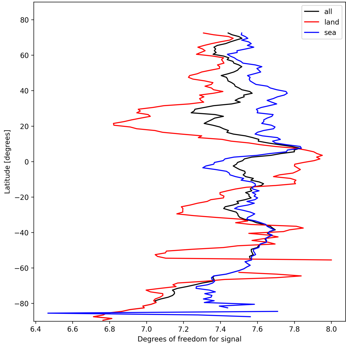
Figure 11: Zonal average of “Degrees of freedom for signal” for 2025-10-26 to 2025-10-27.
