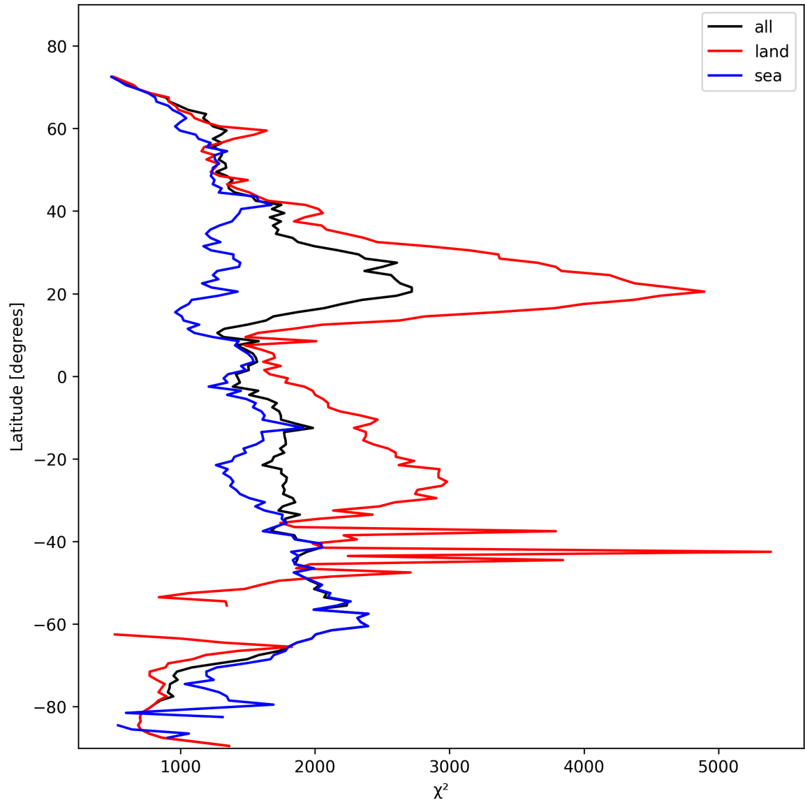
Figure 10: Zonal average of “ \chi^2 ” for 2025-10-26 to 2025-10-27.
