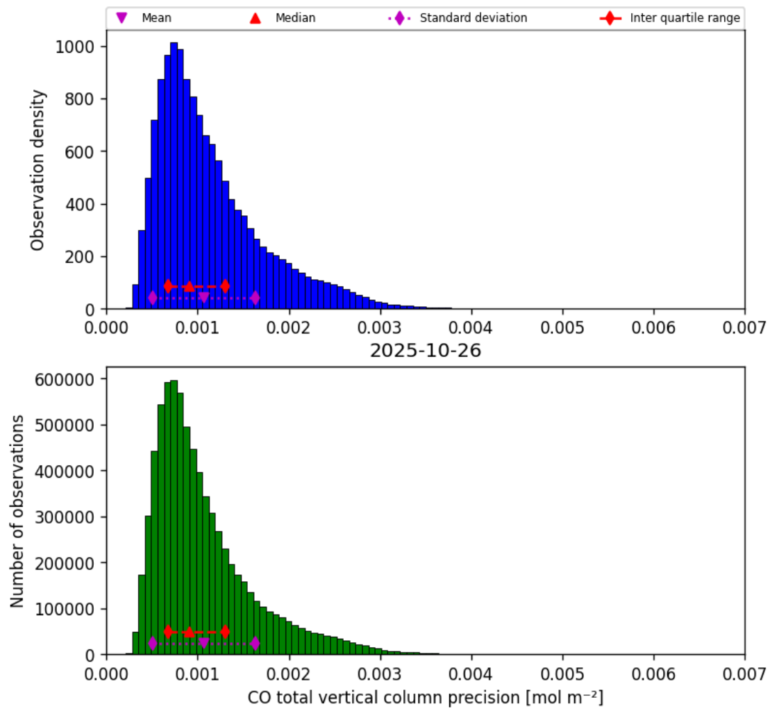
Figure 15: Histogram of “CO total vertical column precision” for 2025-10-26 to 2025-10-27
