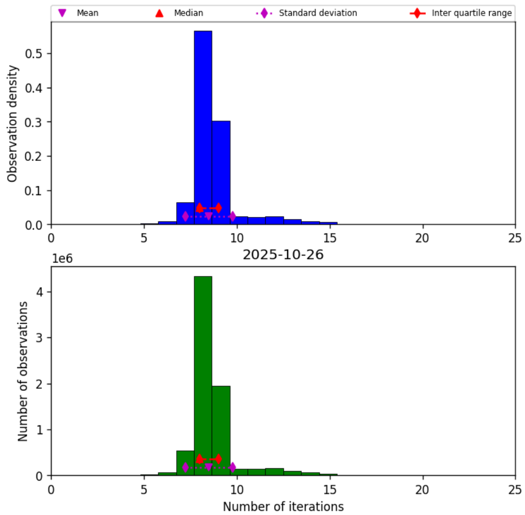
Figure 19: Histogram of “Number of iterations” for 2025-10-26 to 2025-10-27
