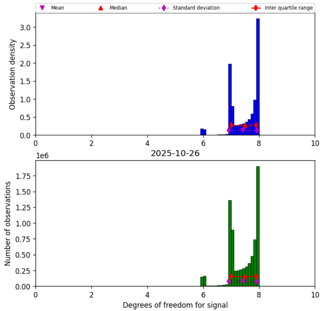
Figure 18: Histogram of “Degrees of freedom for signal” for 2025-10-26 to 2025-10-27
