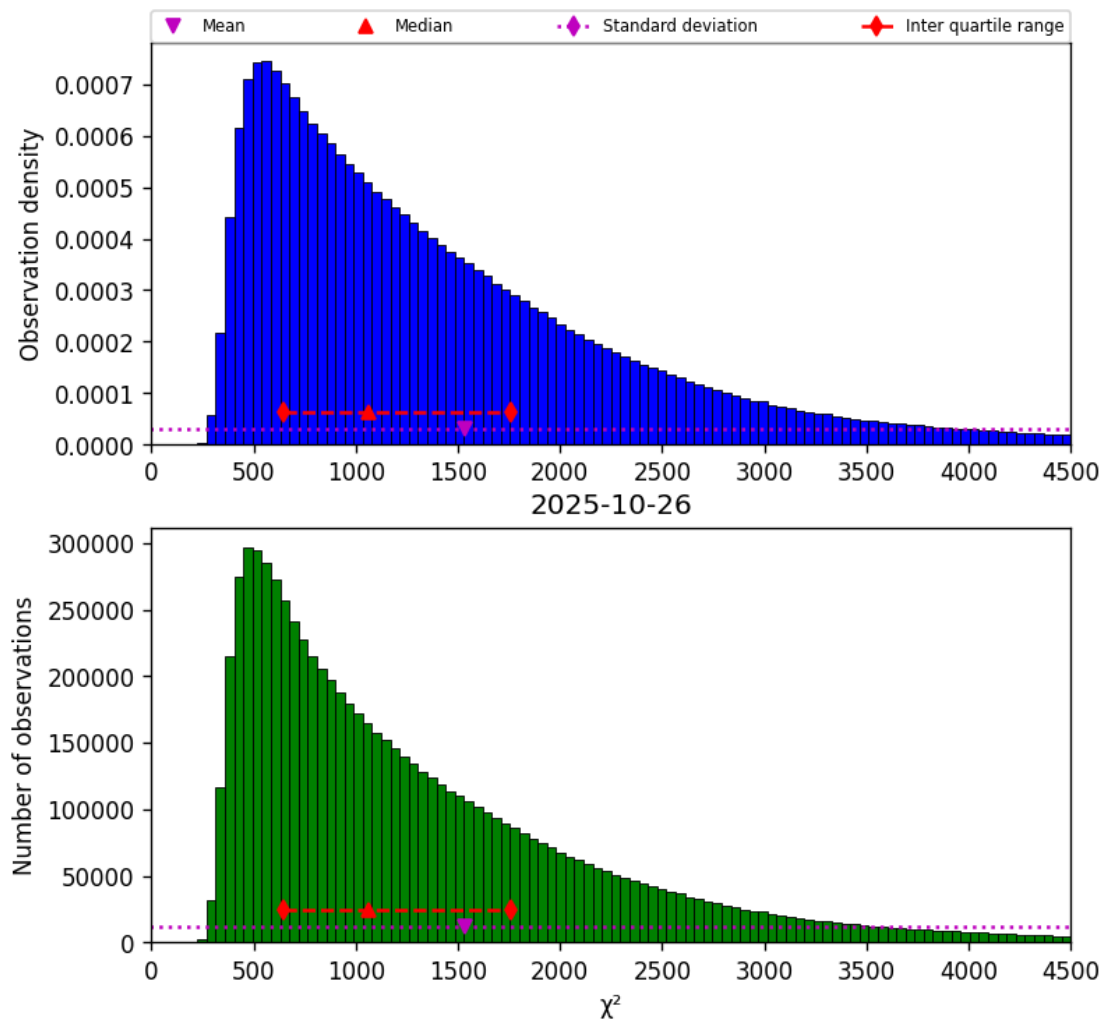
Figure 17: Histogram of “ \chi^2 ” for 2025-10-26 to 2025-10-27
