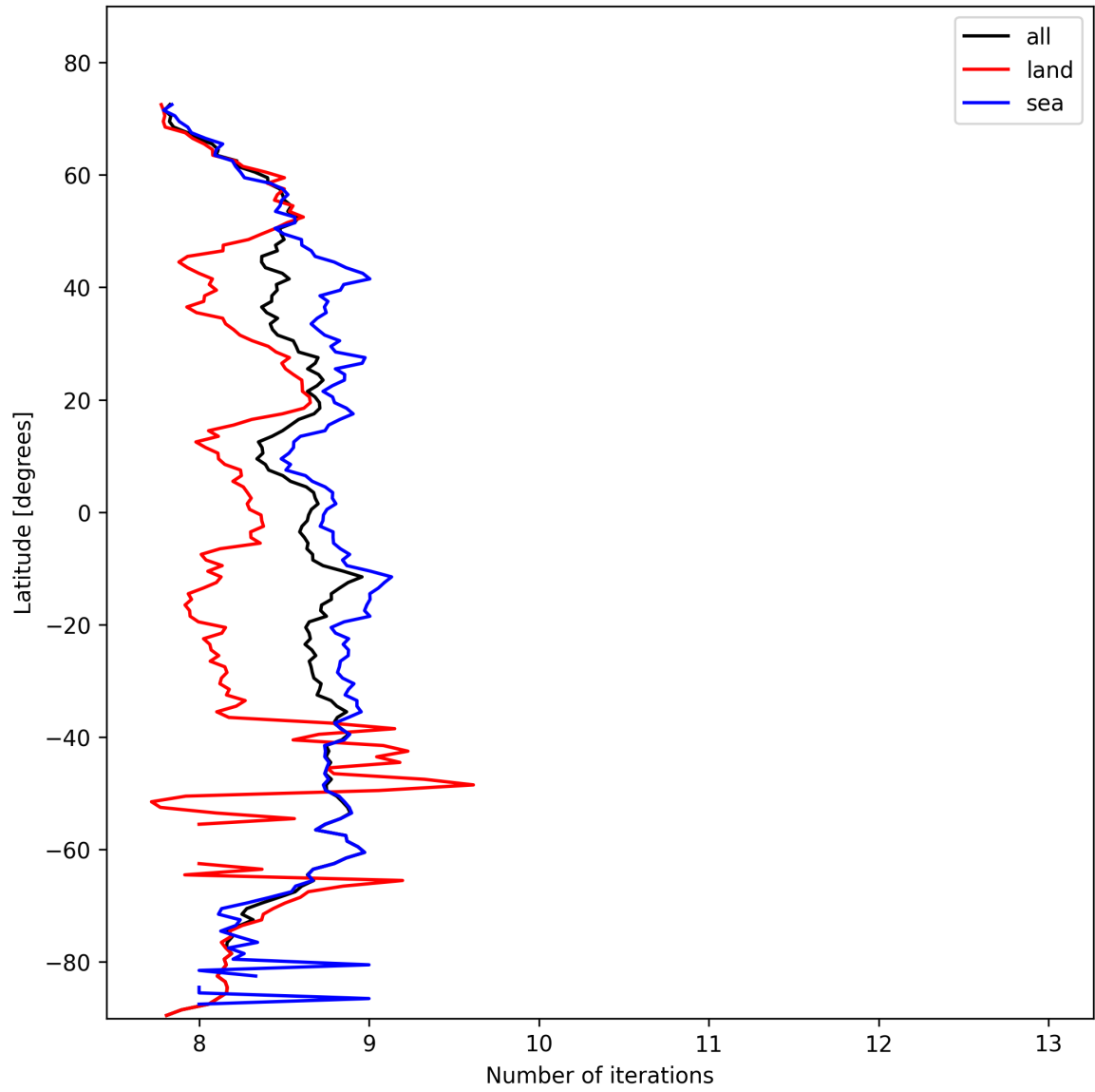
Figure 12: Zonal average of “Number of iterations” for 2025-10-26 to 2025-10-27.
