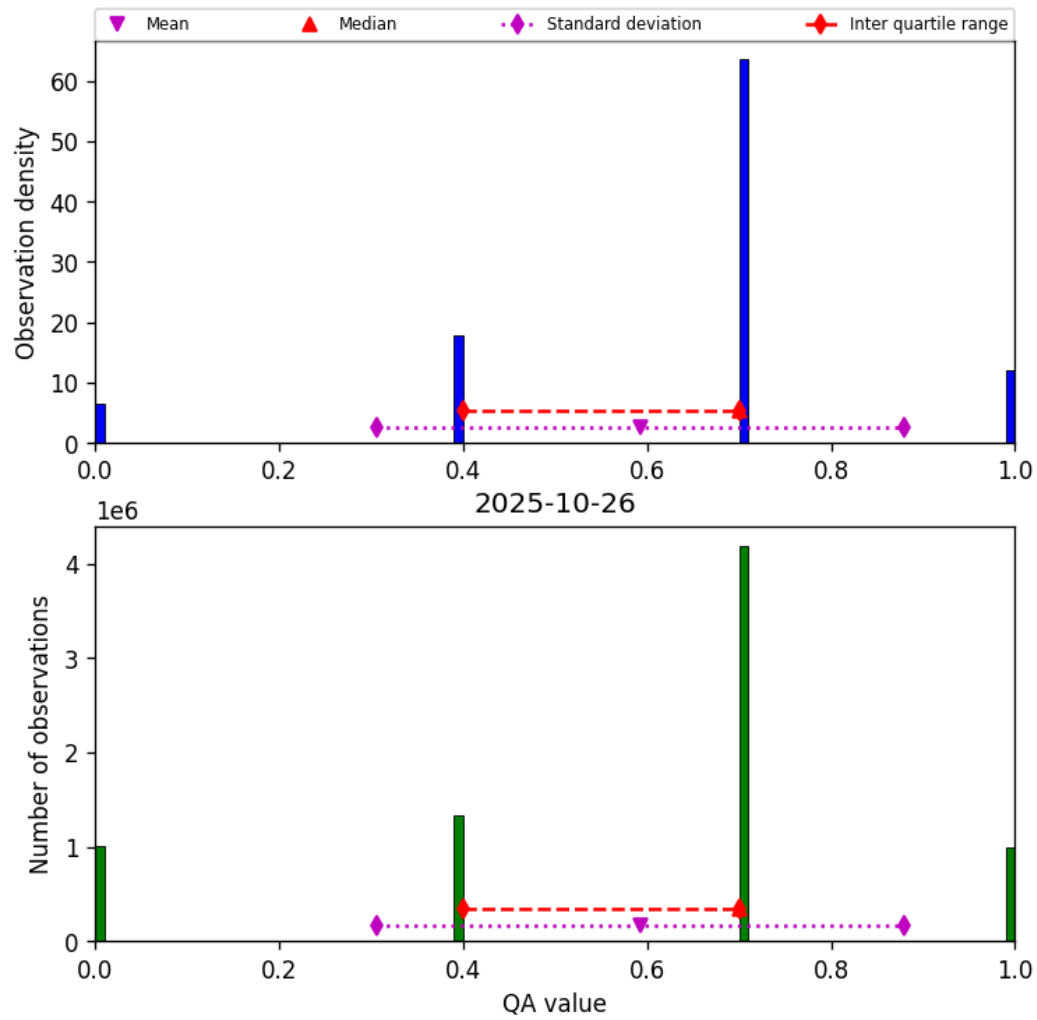
Figure 13: Histogram of “QA value” for 2025-10-26 to 2025-10-27
