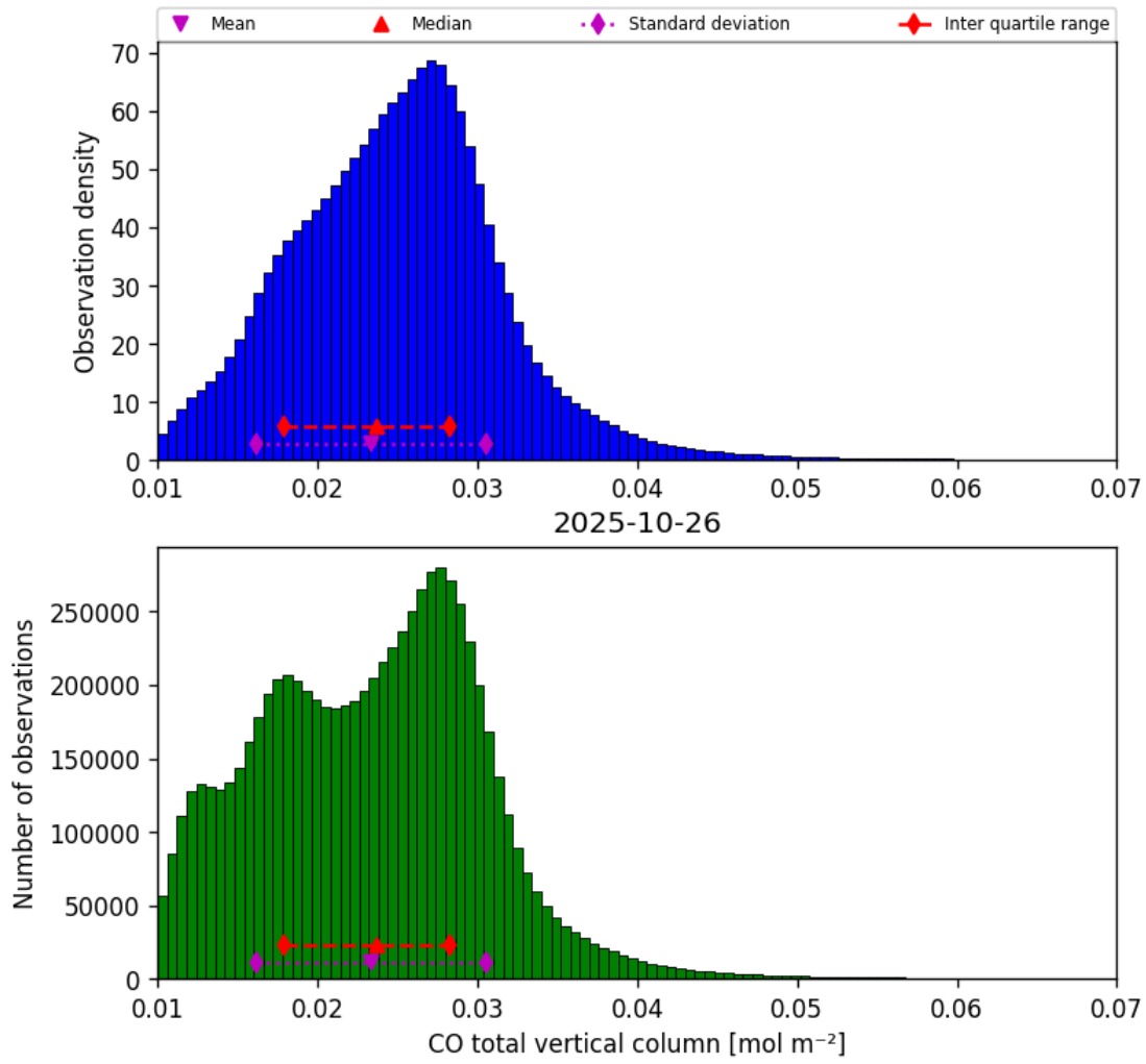
Figure 14: Histogram of “CO total vertical column” for 2025-10-26 to 2025-10-27
