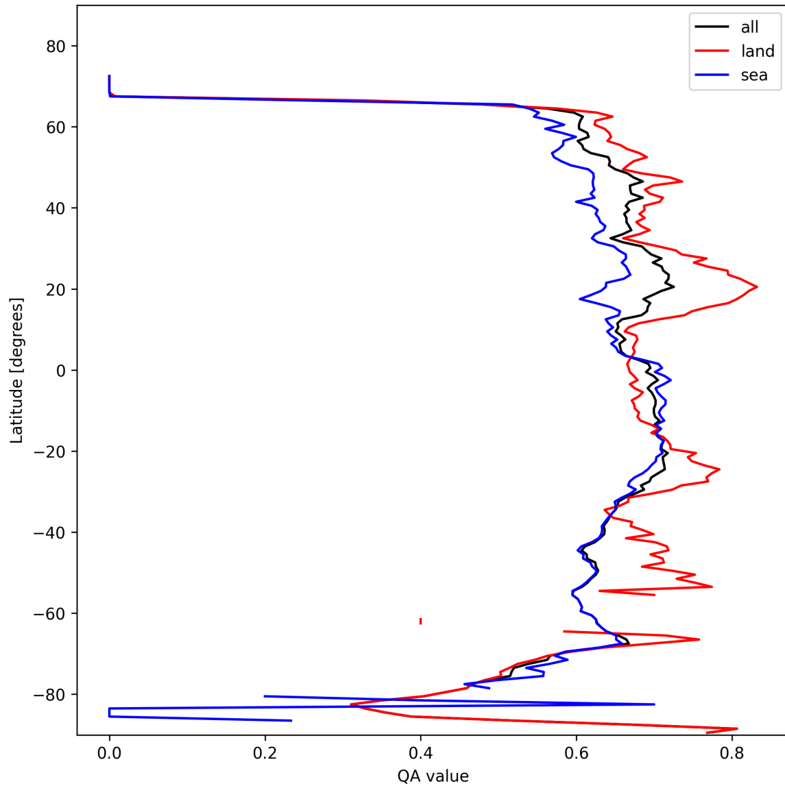
Figure 6: Zonal average of “QA value” for 2025-10-27 to 2025-10-28.
