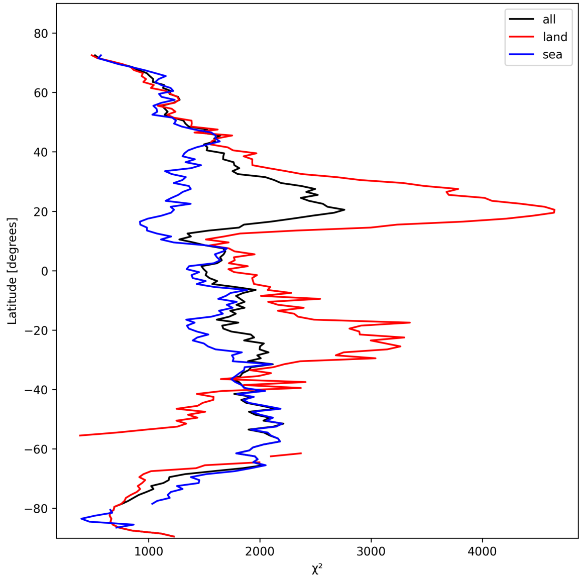
Figure 10: Zonal average of “ \chi^2 ” for 2025-10-27 to 2025-10-28.
