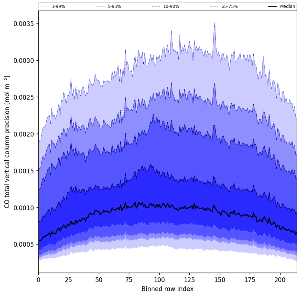
Figure 22: Along track statistics of “CO total vertical column precision” for 2025-10-27 to 2025-10-28
