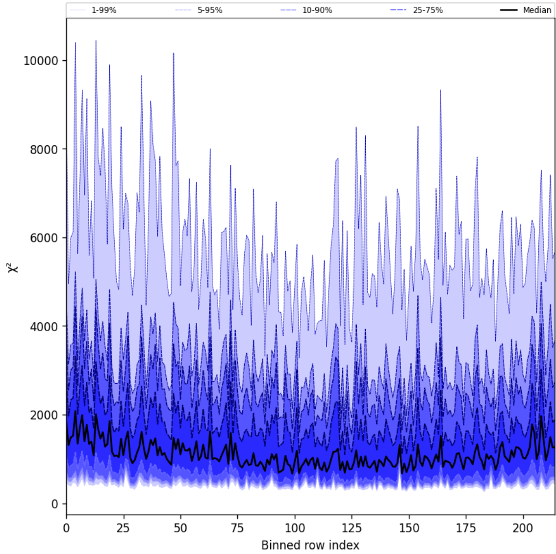
Figure 24: Along track statistics of “ \chi^2 ” for 2025-10-27 to 2025-10-28
