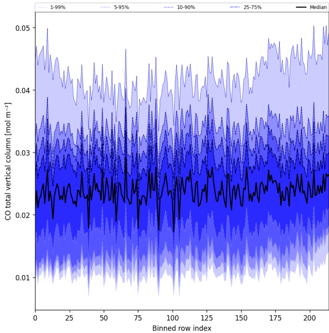
Figure 21: Along track statistics of “CO total vertical column” for 2025-10-27 to 2025-10-28
