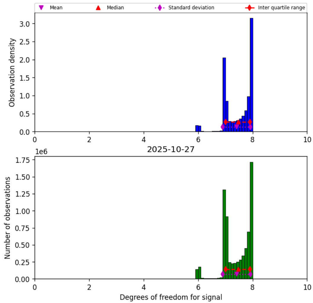
Figure 18: Histogram of “Degrees of freedom for signal” for 2025-10-27 to 2025-10-28
