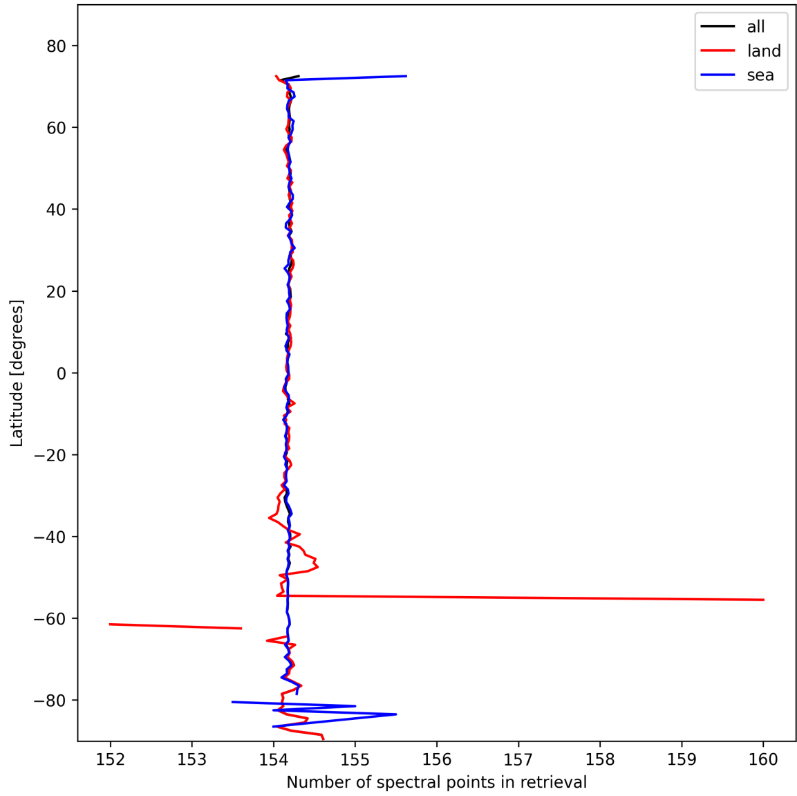
Figure 9: Zonal average of “Number of spectral points in retrieval” for 2025-10-27 to 2025-10-28.
