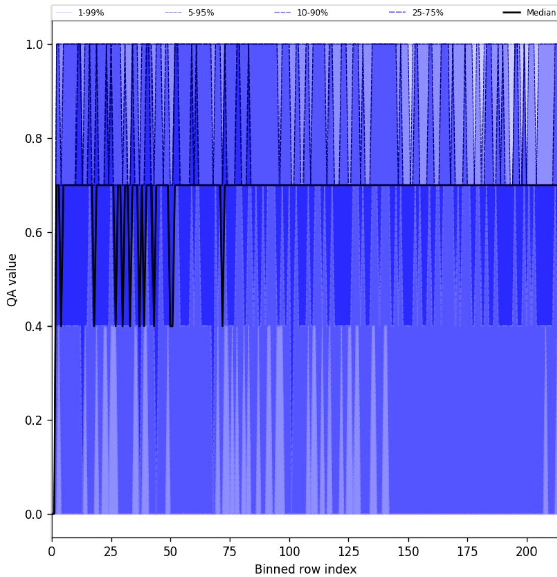
Figure 20: Along track statistics of “QA value” for 2025-10-27 to 2025-10-28
