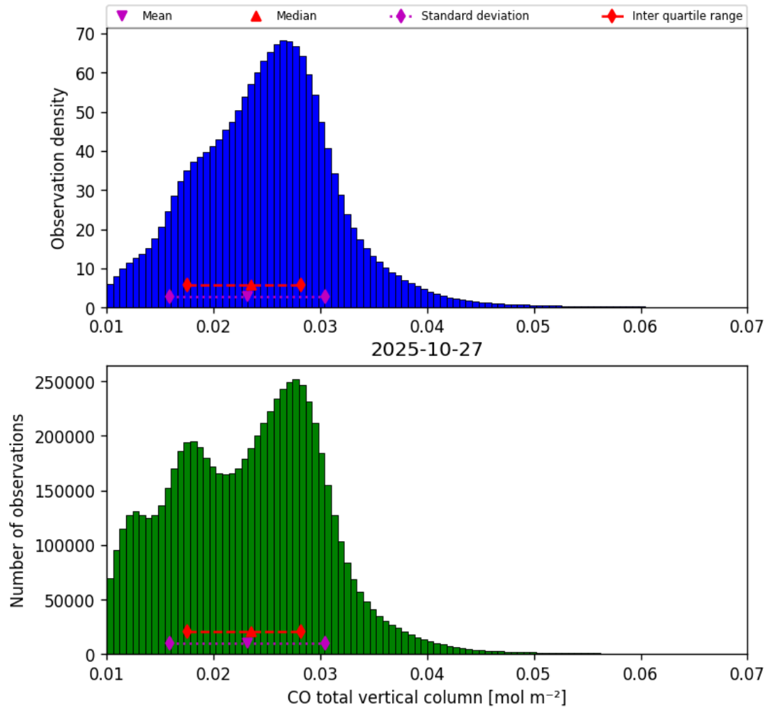
Figure 14: Histogram of “CO total vertical column” for 2025-10-27 to 2025-10-28
