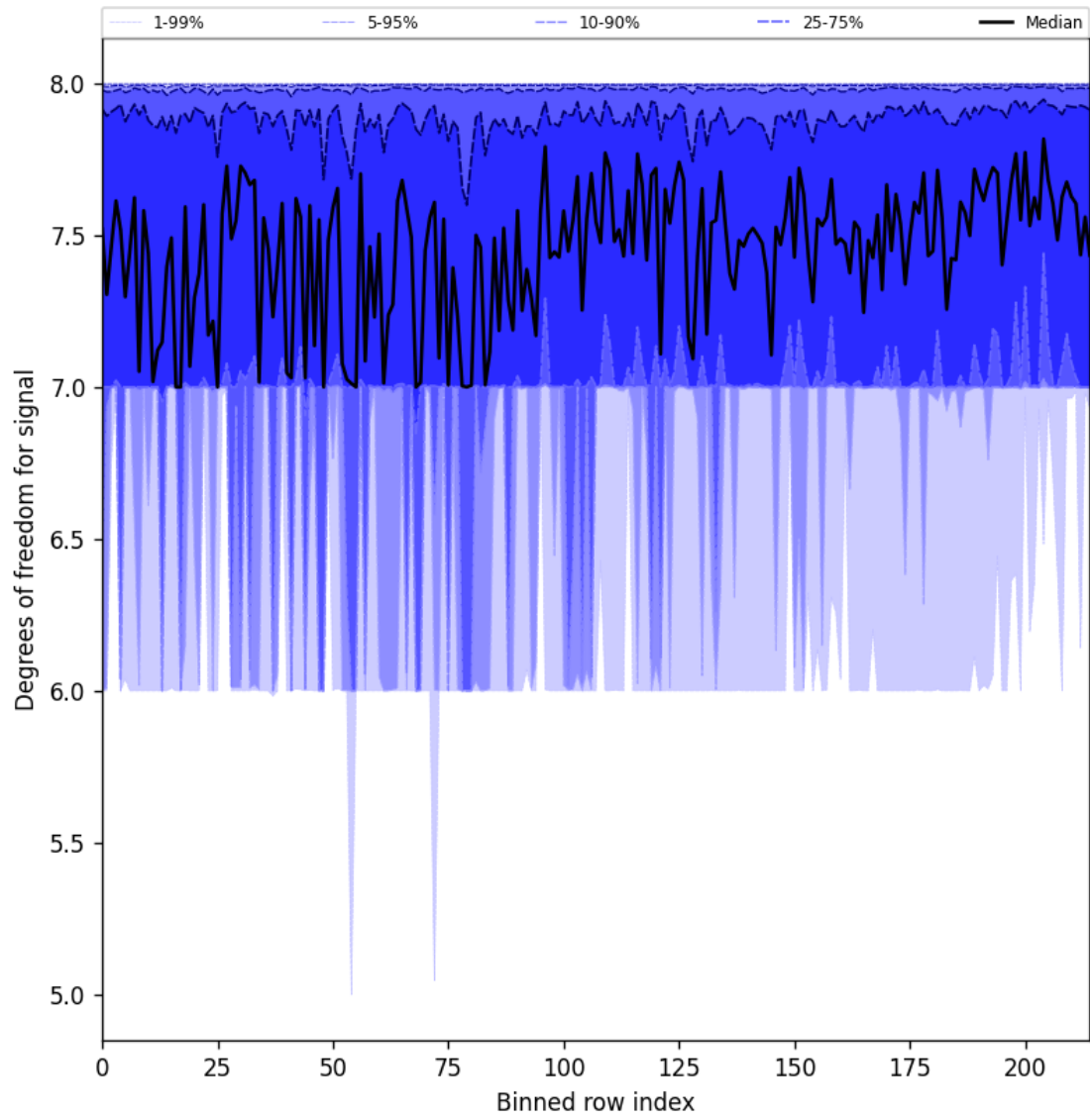
Figure 25: Along track statistics of “Degrees of freedom for signal” for 2025-10-27 to 2025-10-28
