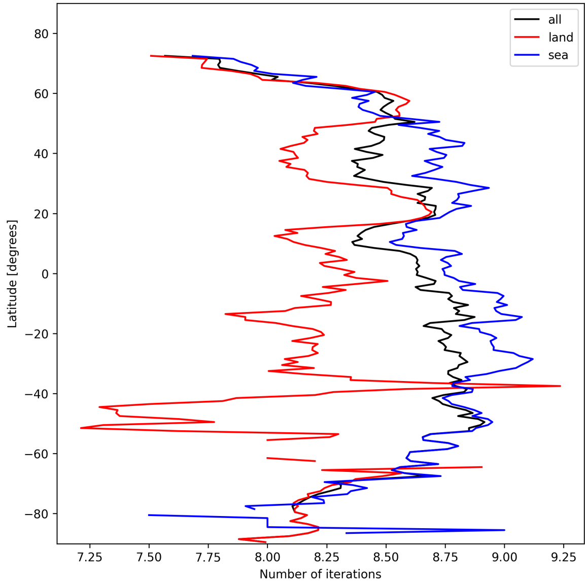
Figure 12: Zonal average of “Number of iterations” for 2025-10-27 to 2025-10-28.
