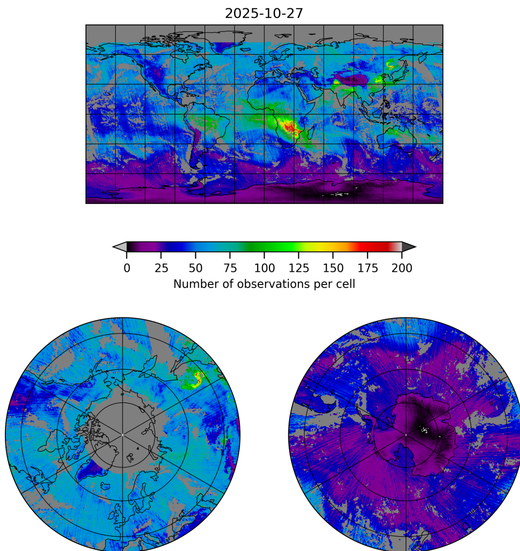
Figure 5: Map of the number of observations for 2025-10-27 to 2025-10-28
