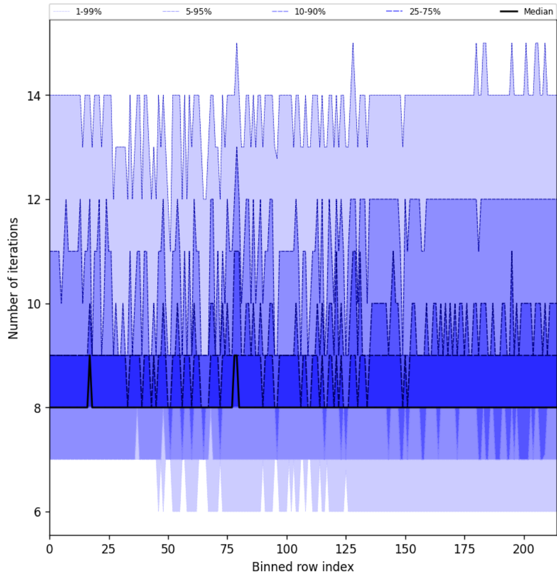
Figure 26: Along track statistics of “Number of iterations” for 2025-10-27 to 2025-10-28
