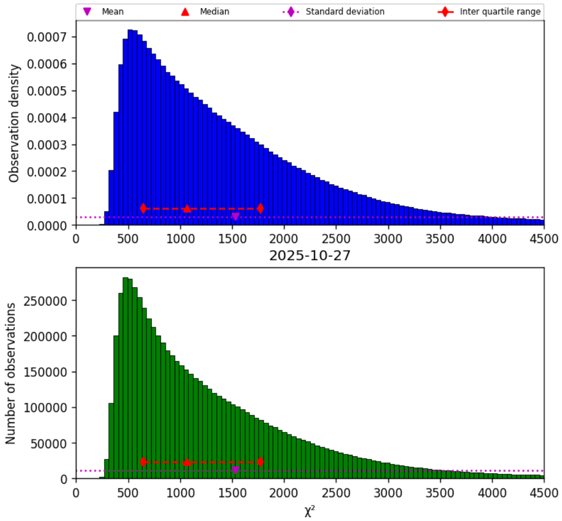
Figure 17: Histogram of “ \chi^2 ” for 2025-10-27 to 2025-10-28
