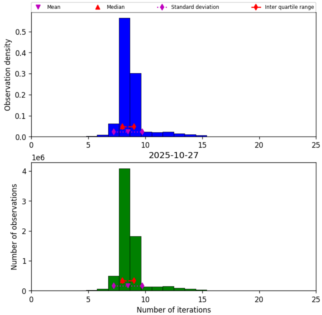
Figure 19: Histogram of “Number of iterations” for 2025-10-27 to 2025-10-28
