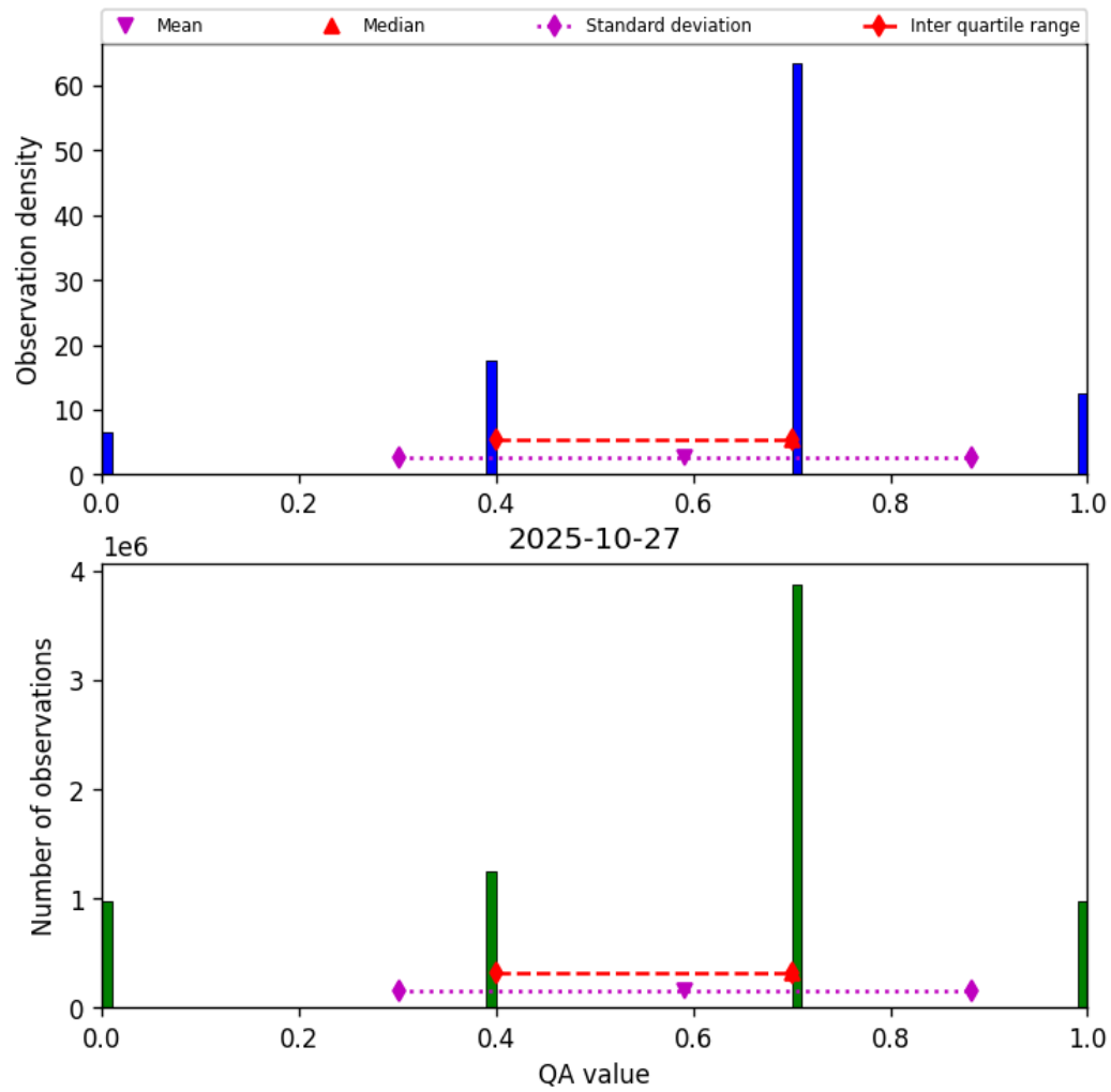
Figure 13: Histogram of “QA value” for 2025-10-27 to 2025-10-28
