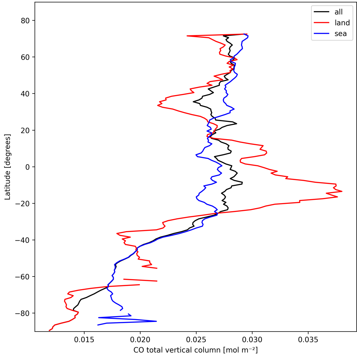
Figure 7: Zonal average of “CO total vertical column” for 2025-10-27 to 2025-10-28.
