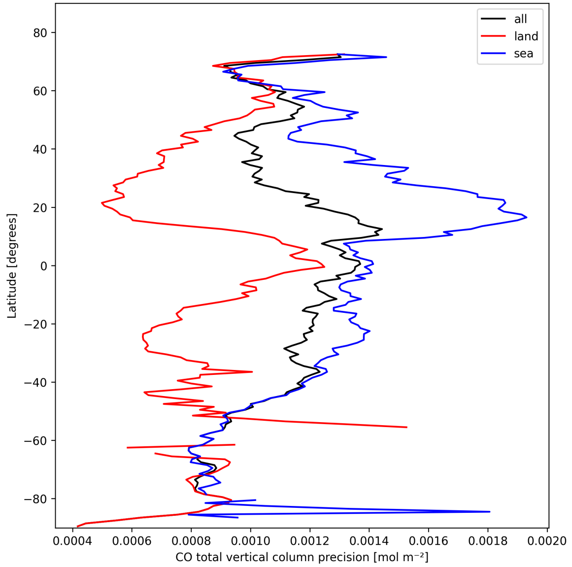
Figure 8: Zonal average of “CO total vertical column precision” for 2025-10-27 to 2025-10-28.
