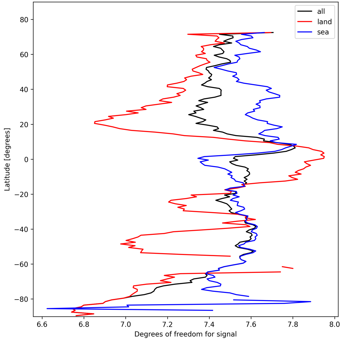
Figure 11: Zonal average of “Degrees of freedom for signal” for 2025-10-27 to 2025-10-28.
