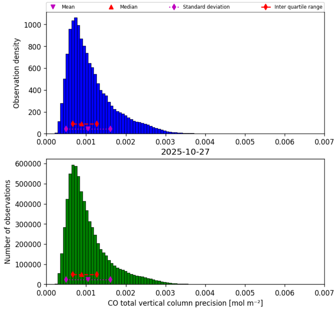
Figure 15: Histogram of “CO total vertical column precision” for 2025-10-27 to 2025-10-28
