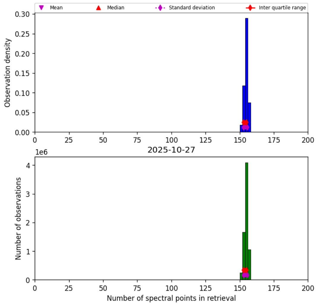
Figure 16: Histogram of “Number of spectral points in retrieval” for 2025-10-27 to 2025-10-28
