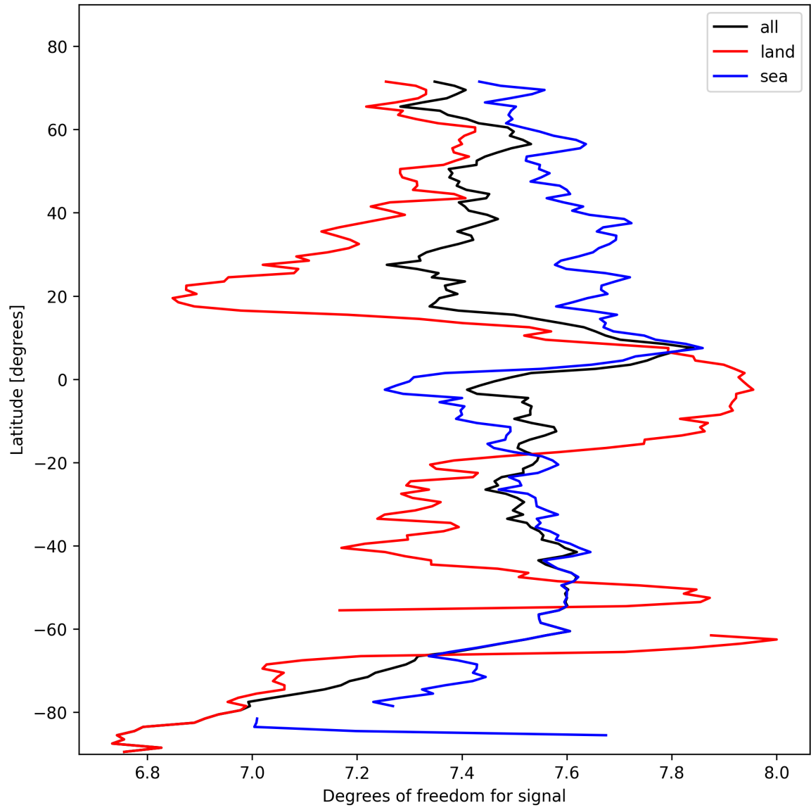
Figure 11: Zonal average of “Degrees of freedom for signal” for 2025-10-28 to 2025-10-29.
