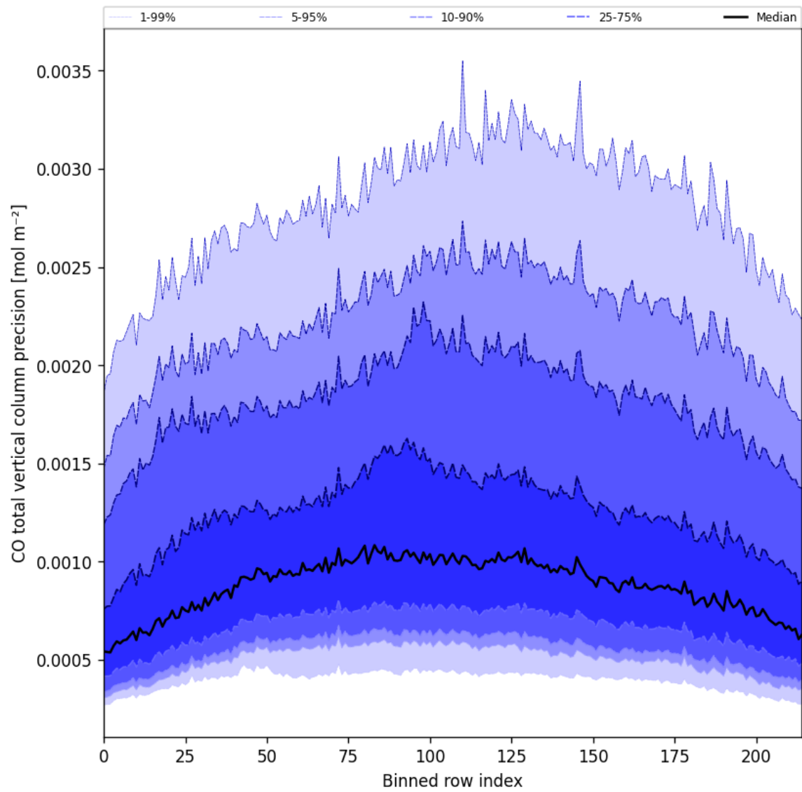
Figure 22: Along track statistics of “CO total vertical column precision” for 2025-10-28 to 2025-10-29
