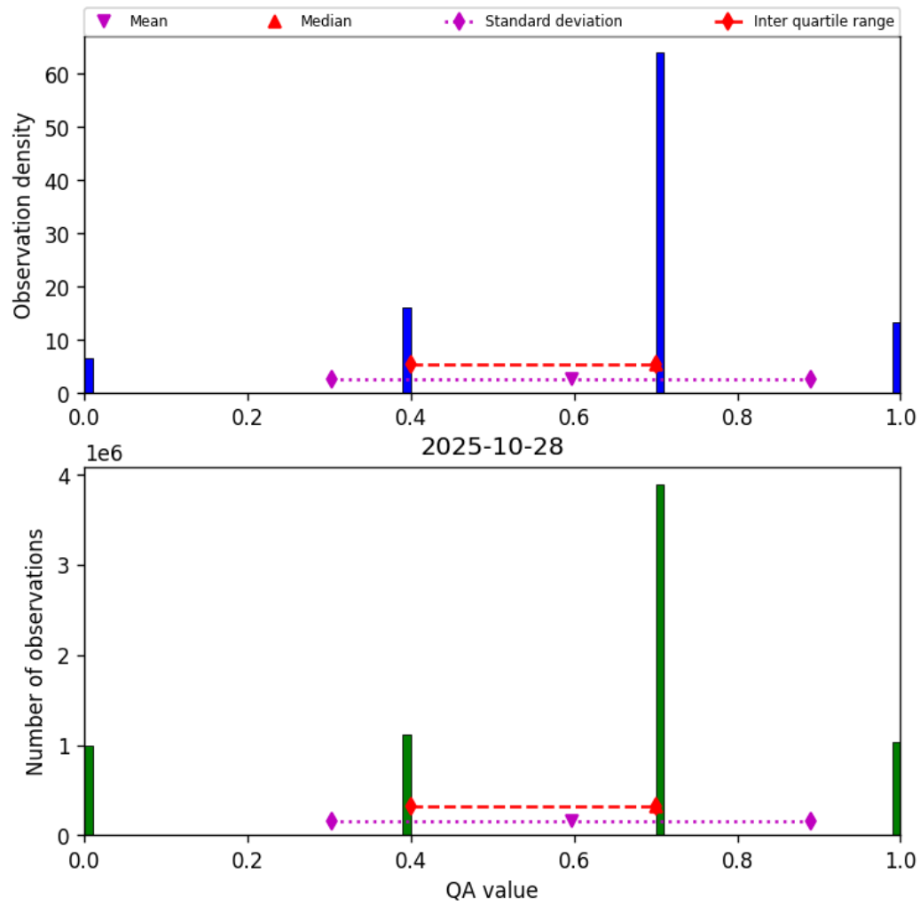
Figure 13: Histogram of “QA value” for 2025-10-28 to 2025-10-29
