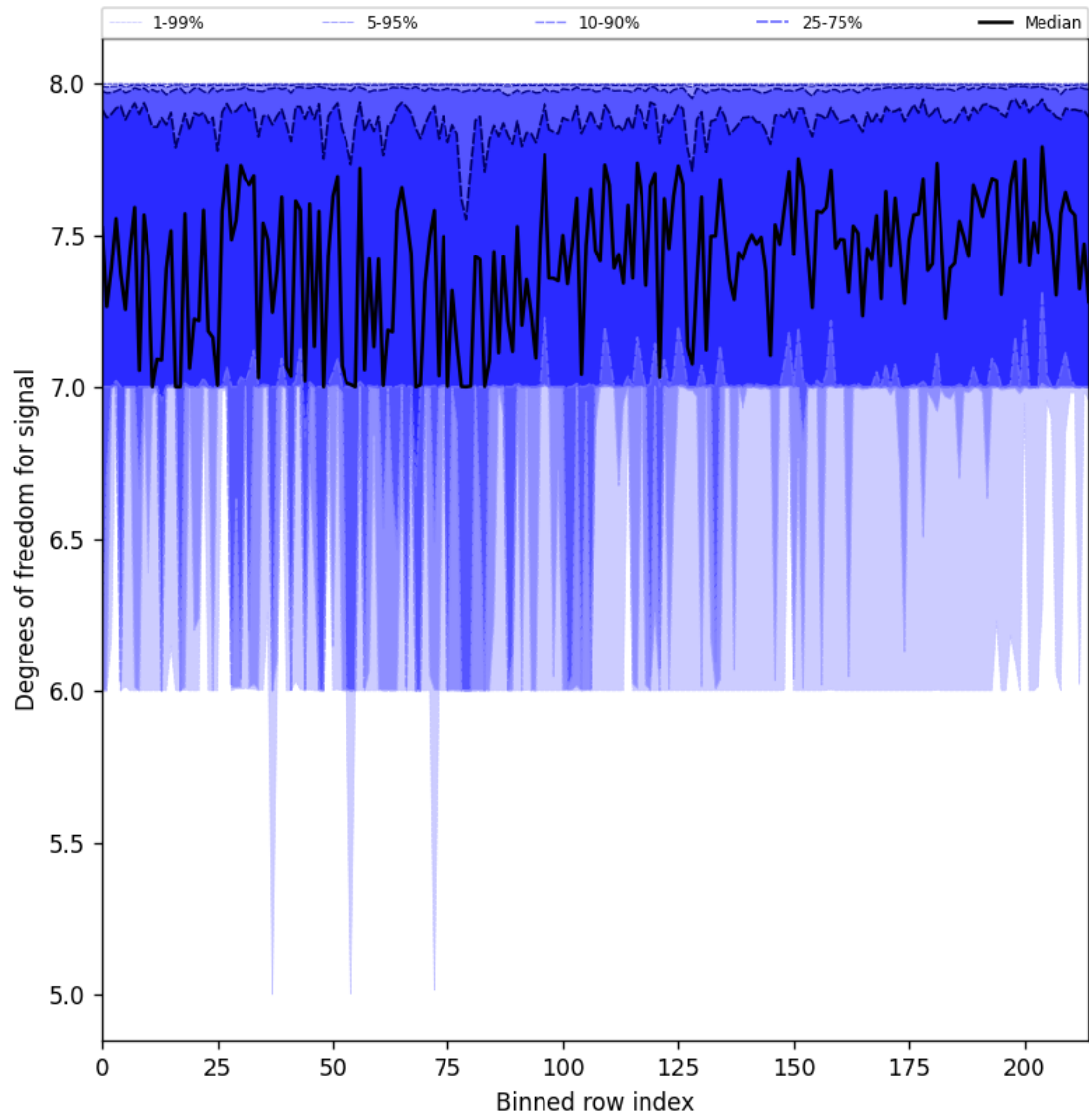
Figure 25: Along track statistics of “Degrees of freedom for signal” for 2025-10-28 to 2025-10-29
