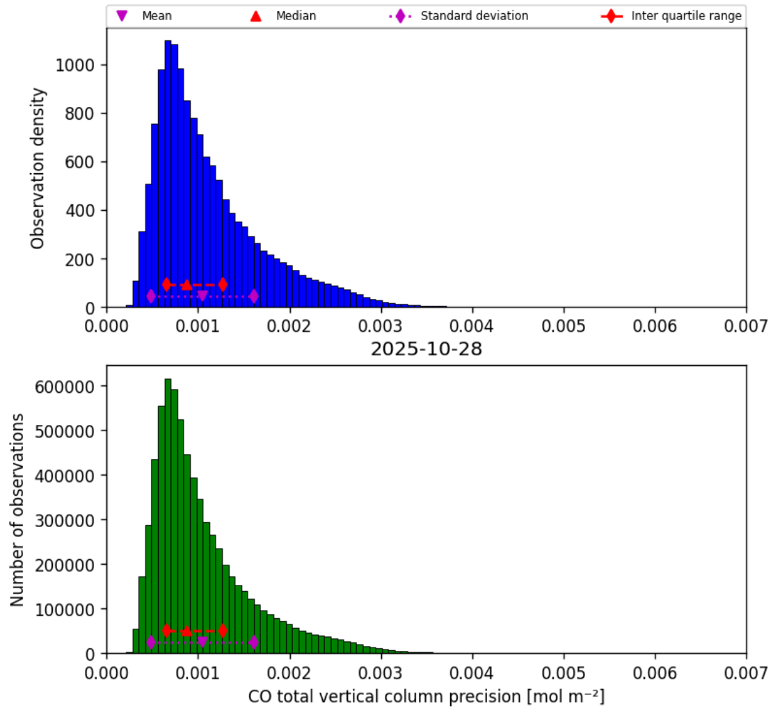
Figure 15: Histogram of “CO total vertical column precision” for 2025-10-28 to 2025-10-29
