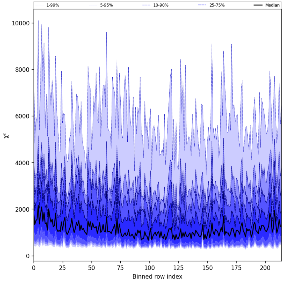
Figure 24: Along track statistics of “ \chi^2 ” for 2025-10-28 to 2025-10-29
