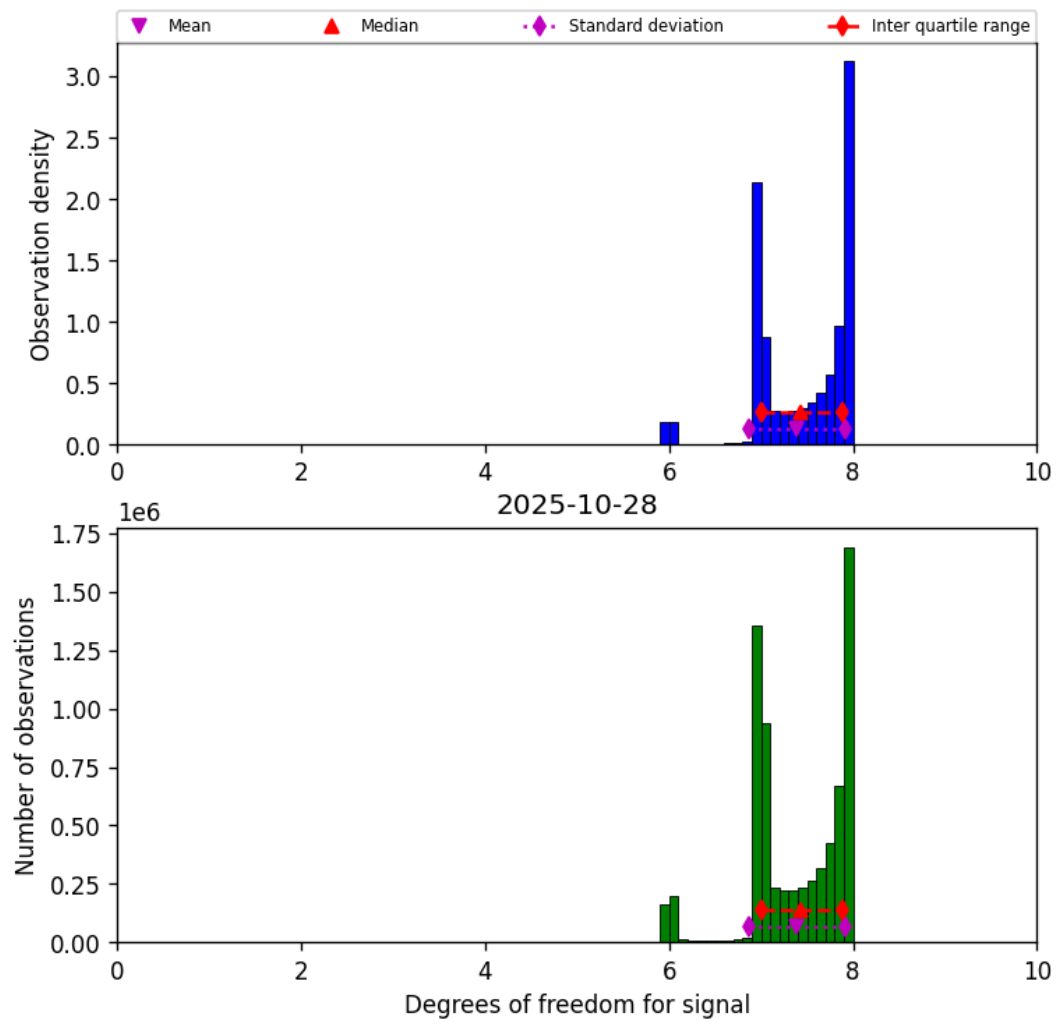
Figure 18: Histogram of “Degrees of freedom for signal” for 2025-10-28 to 2025-10-29
