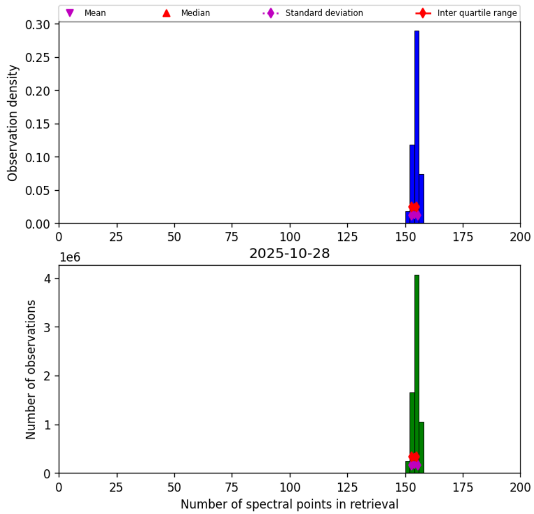
Figure 16: Histogram of “Number of spectral points in retrieval” for 2025-10-28 to 2025-10-29
