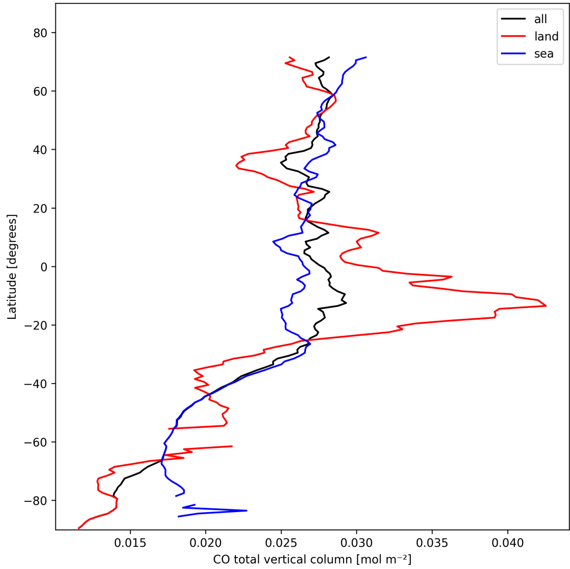
Figure 7: Zonal average of “CO total vertical column” for 2025-10-28 to 2025-10-29.
