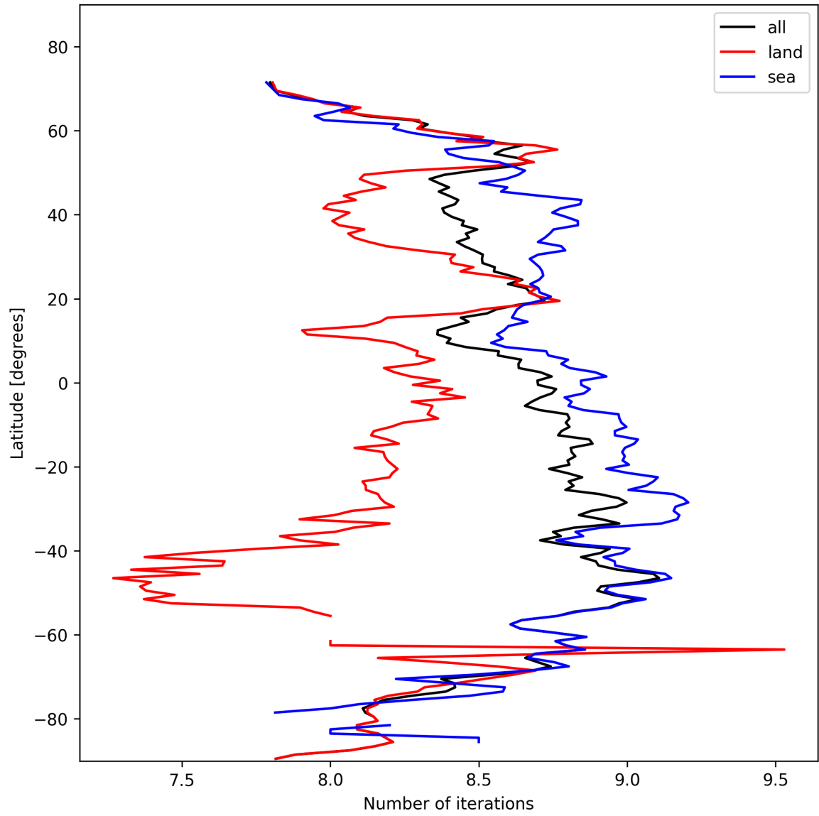
Figure 12: Zonal average of “Number of iterations” for 2025-10-28 to 2025-10-29.
