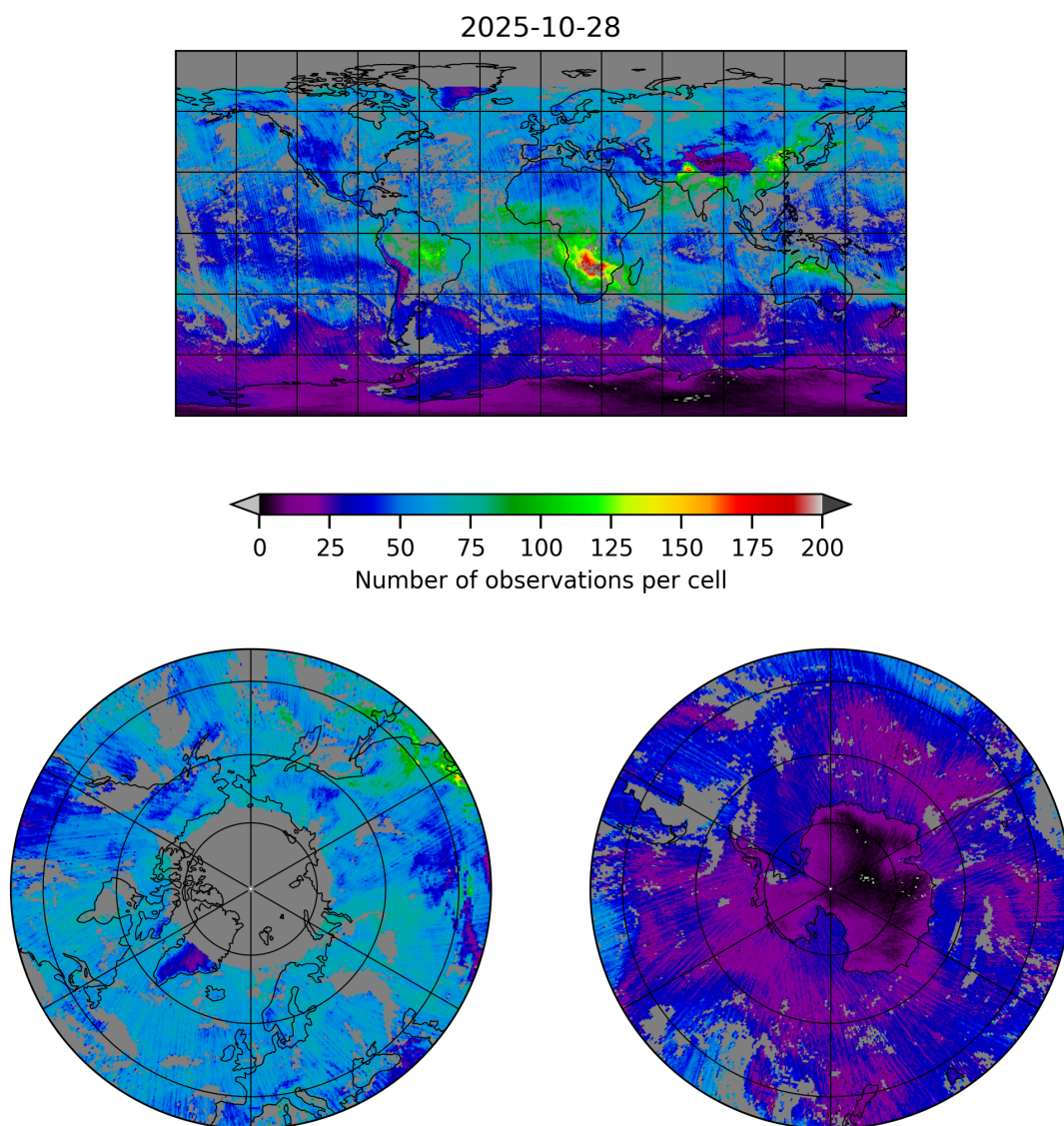
Figure 5: Map of the number of observations for 2025-10-28 to 2025-10-29
