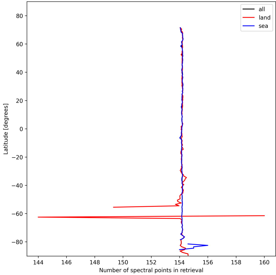
Figure 9: Zonal average of “Number of spectral points in retrieval” for 2025-10-28 to 2025-10-29.
