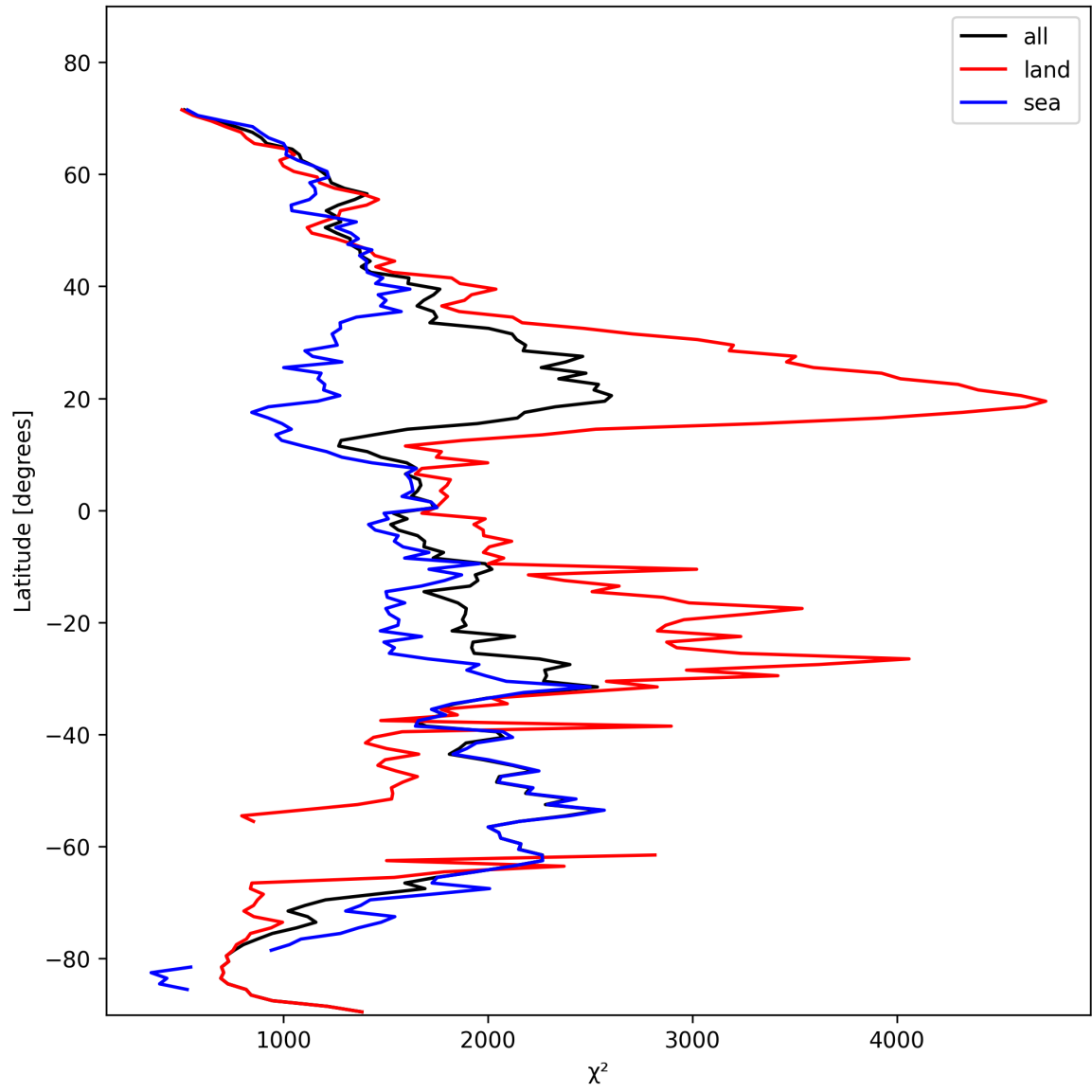
Figure 10: Zonal average of “ \chi^2 ” for 2025-10-28 to 2025-10-29.
