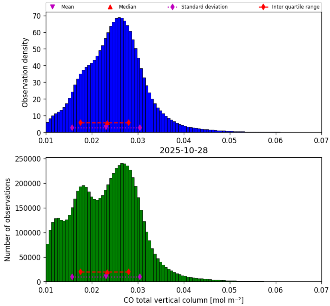
Figure 14: Histogram of “CO total vertical column” for 2025-10-28 to 2025-10-29
