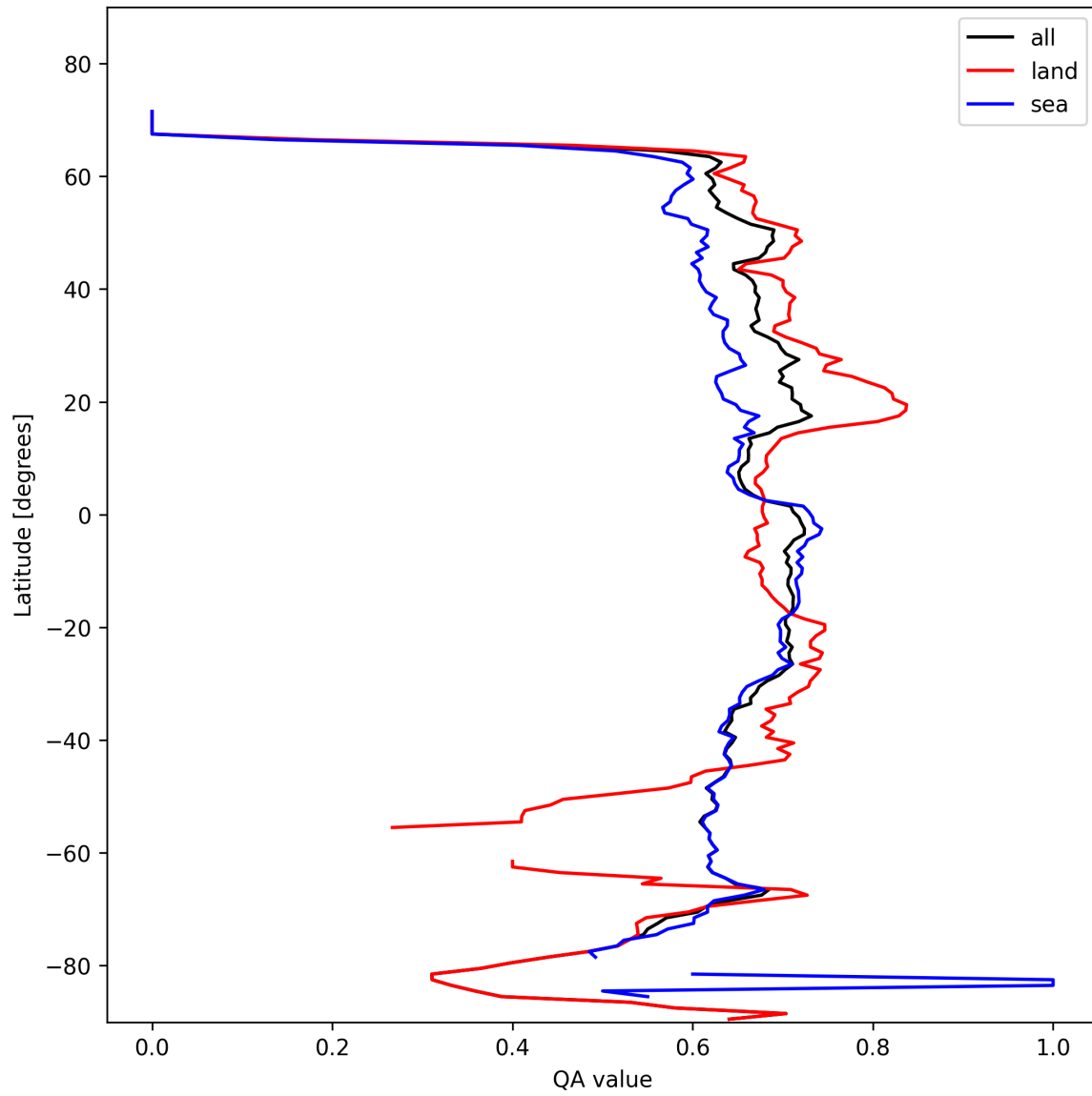
Figure 6: Zonal average of “QA value” for 2025-10-28 to 2025-10-29.
