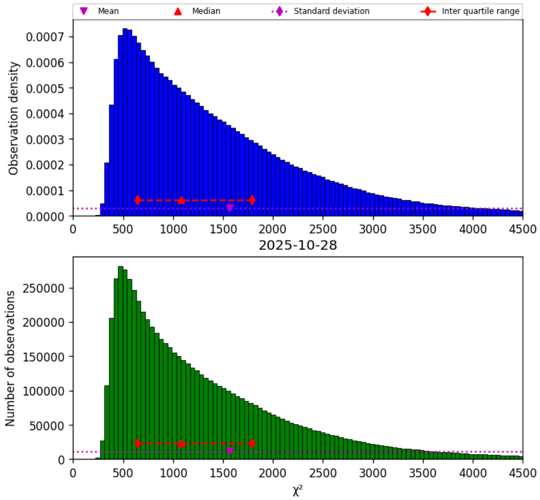
Figure 17: Histogram of “ \chi^2 ” for 2025-10-28 to 2025-10-29
