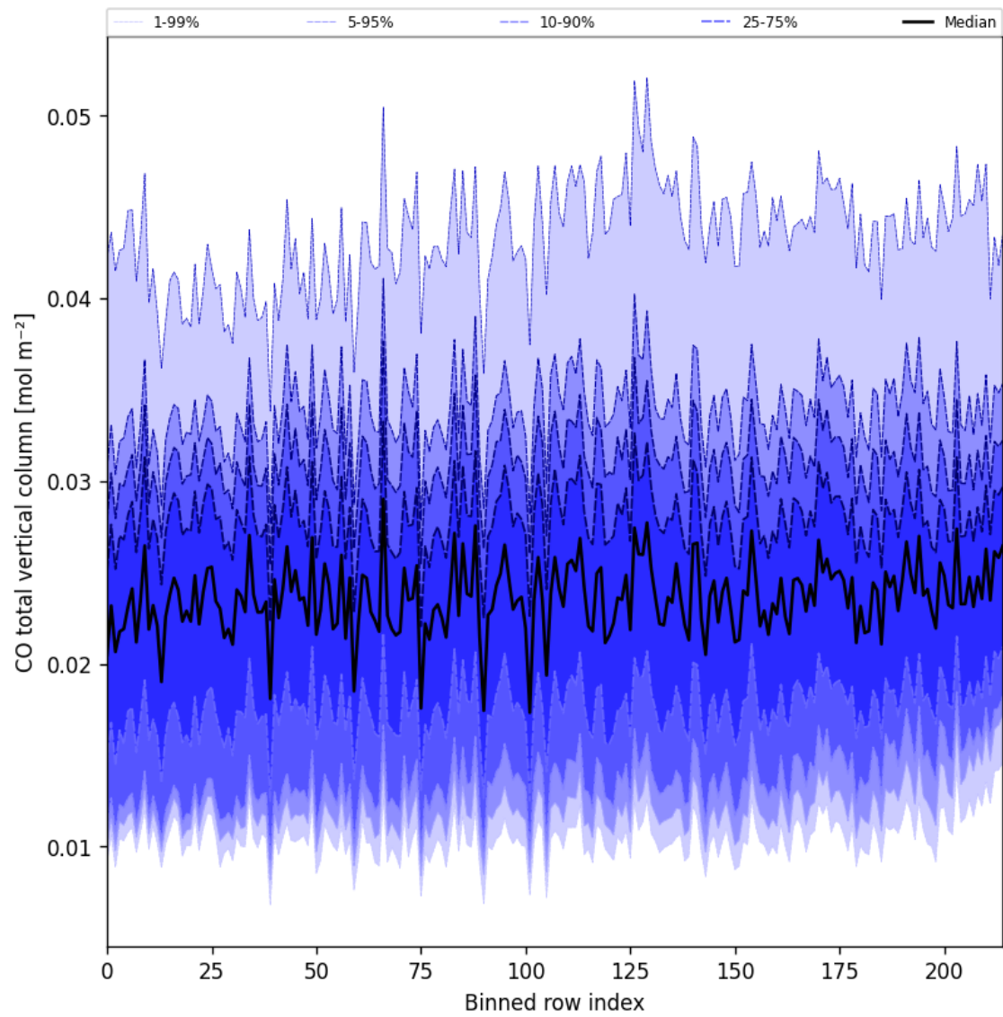
Figure 21: Along track statistics of “CO total vertical column” for 2025-10-28 to 2025-10-29
