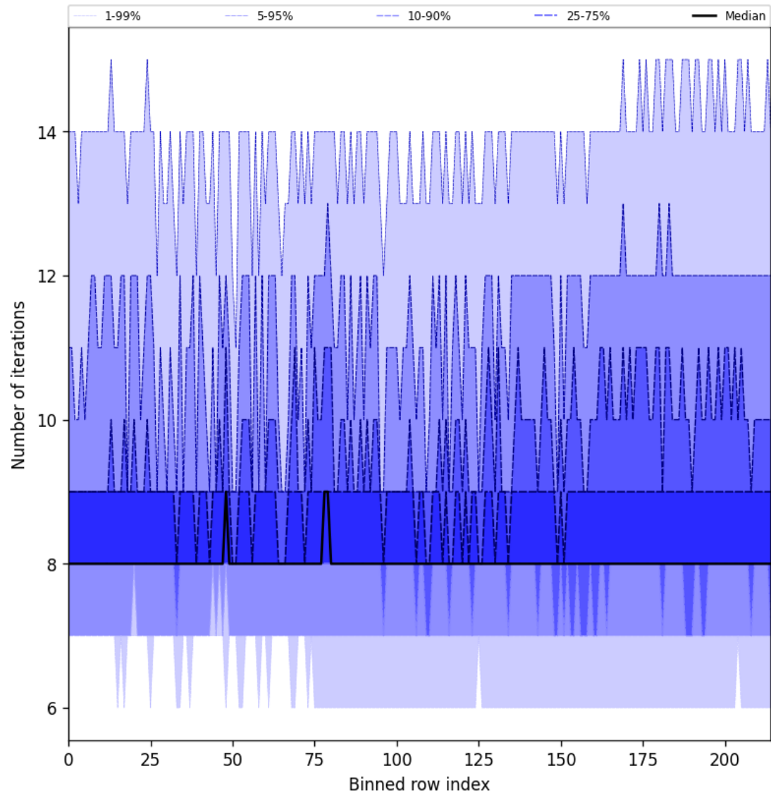
Figure 26: Along track statistics of “Number of iterations” for 2025-10-28 to 2025-10-29
