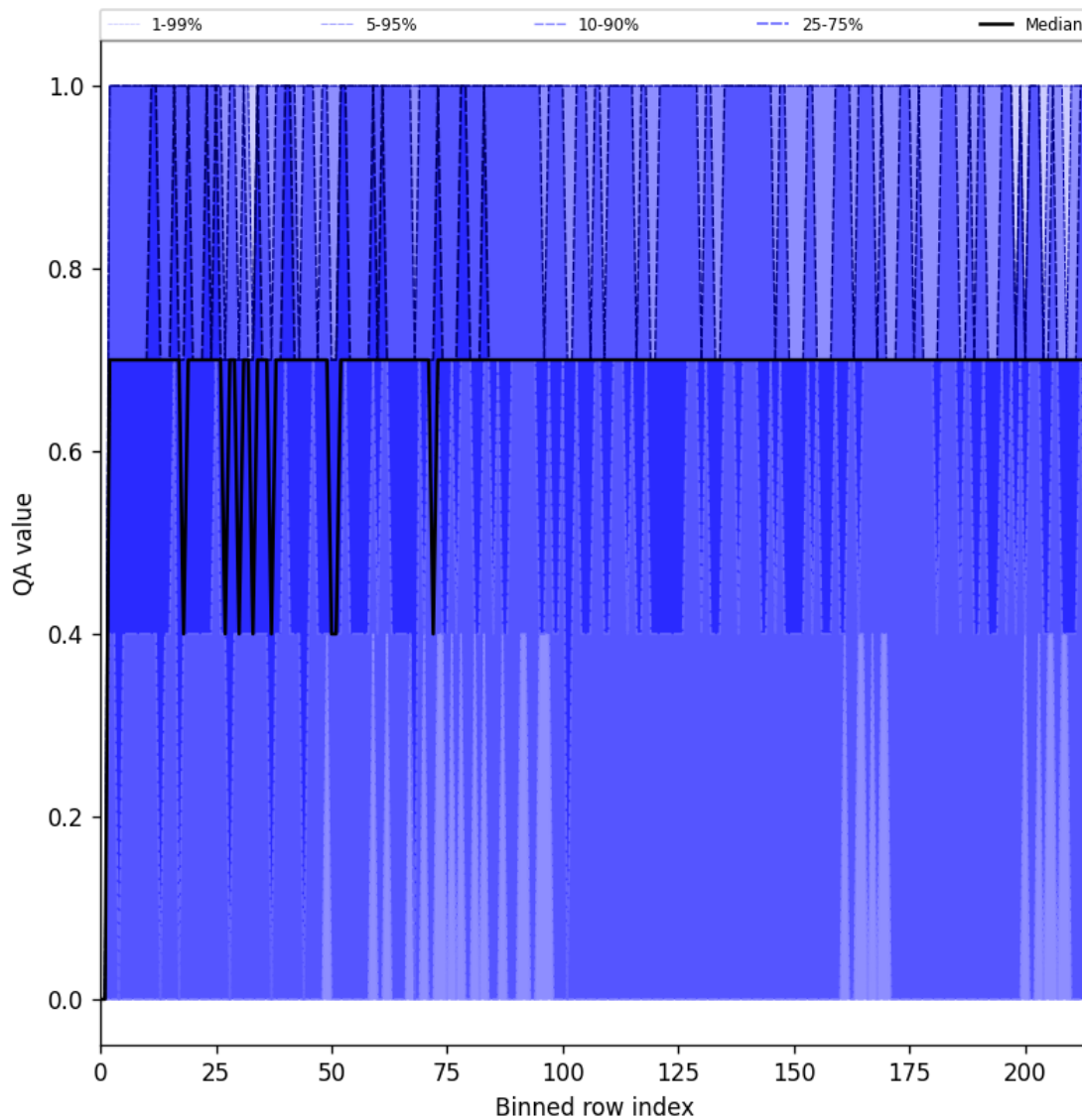
Figure 20: Along track statistics of “QA value” for 2025-10-28 to 2025-10-29
