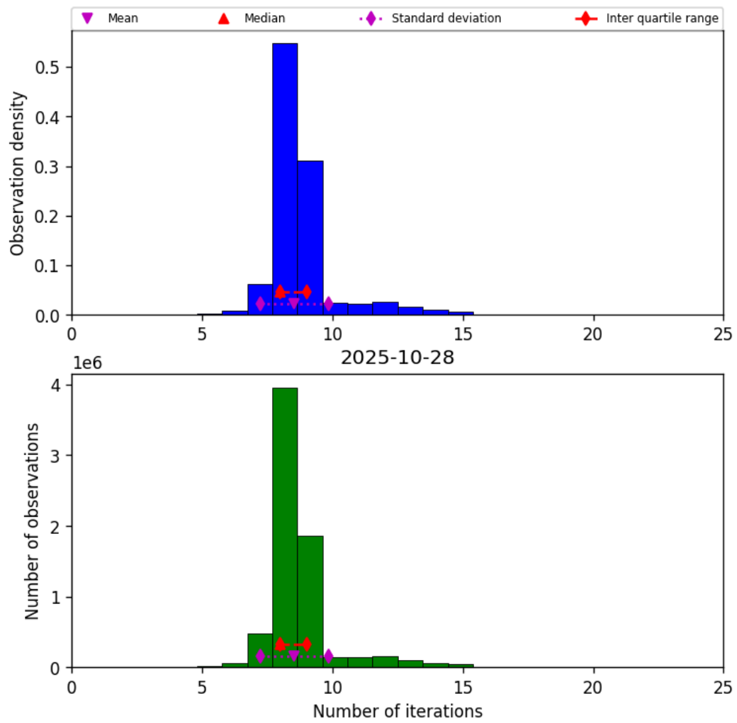
Figure 19: Histogram of “Number of iterations” for 2025-10-28 to 2025-10-29
