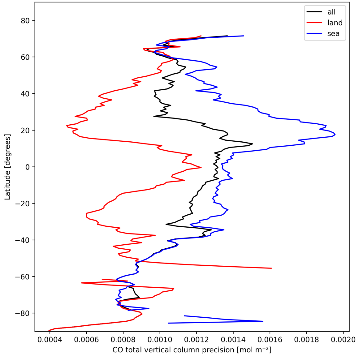
Figure 8: Zonal average of “CO total vertical column precision” for 2025-10-28 to 2025-10-29.
