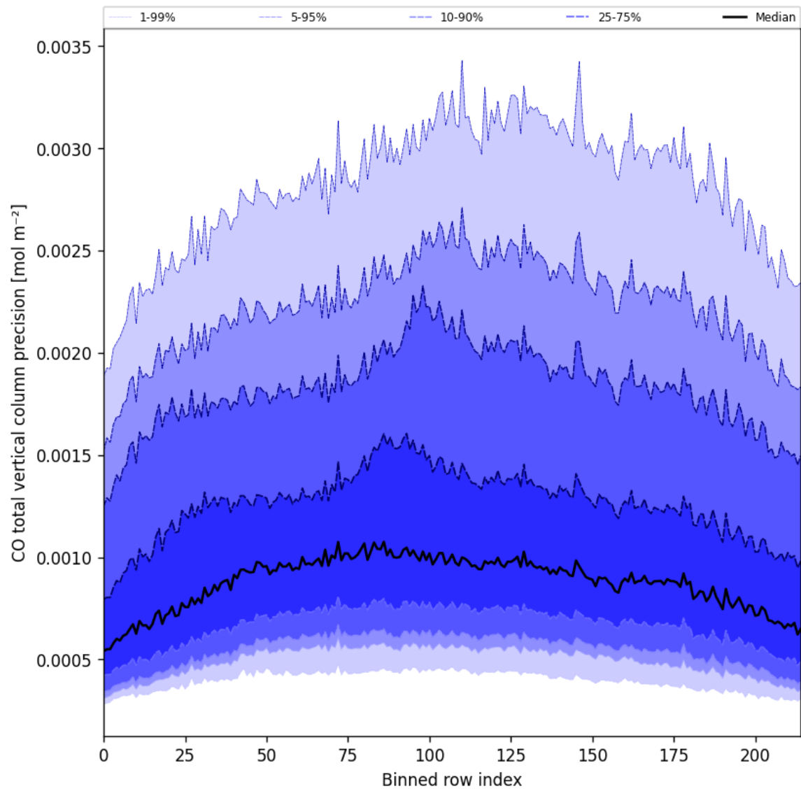
Figure 22: Along track statistics of “CO total vertical column precision” for 2025-10-29 to 2025-10-30
