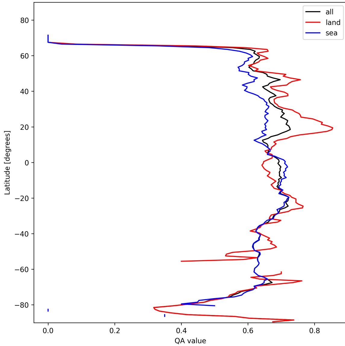
Figure 6: Zonal average of “QA value” for 2025-10-29 to 2025-10-30.
