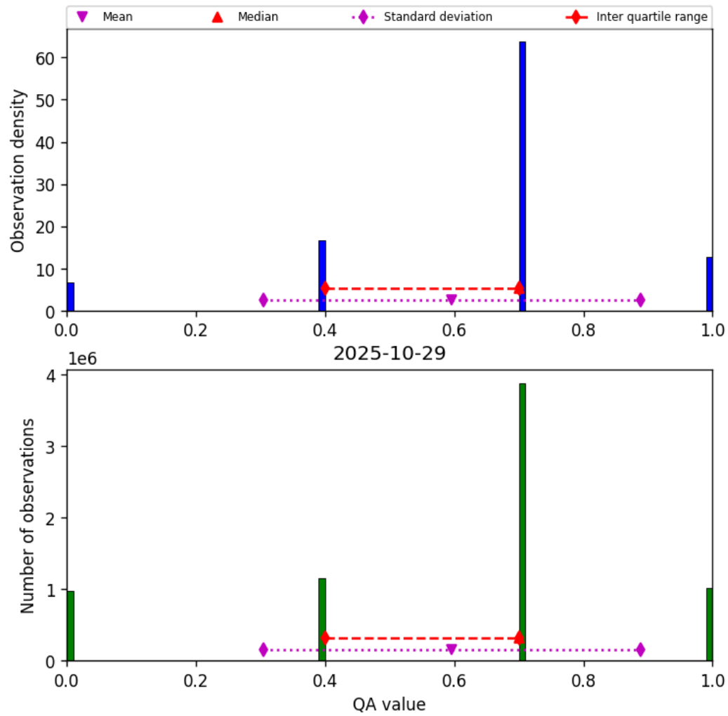
Figure 13: Histogram of “QA value” for 2025-10-29 to 2025-10-30
