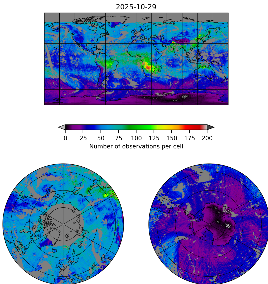
Figure 5: Map of the number of observations for 2025-10-29 to 2025-10-30
