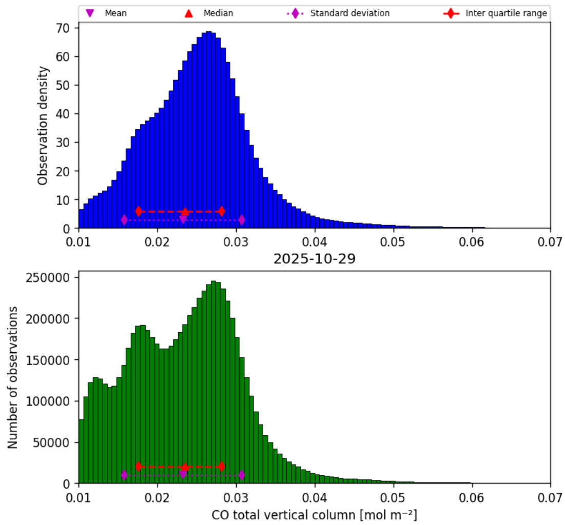
Figure 14: Histogram of “CO total vertical column” for 2025-10-29 to 2025-10-30
