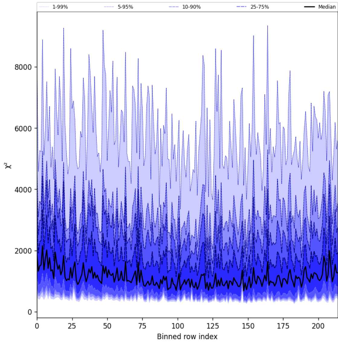
Figure 24: Along track statistics of “ \chi^2 ” for 2025-10-29 to 2025-10-30
