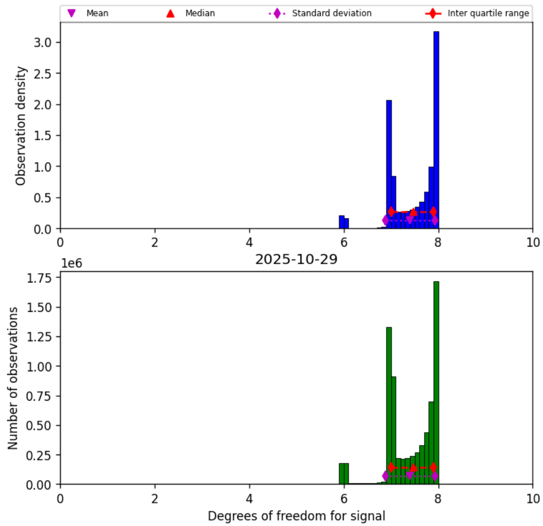
Figure 18: Histogram of “Degrees of freedom for signal” for 2025-10-29 to 2025-10-30
