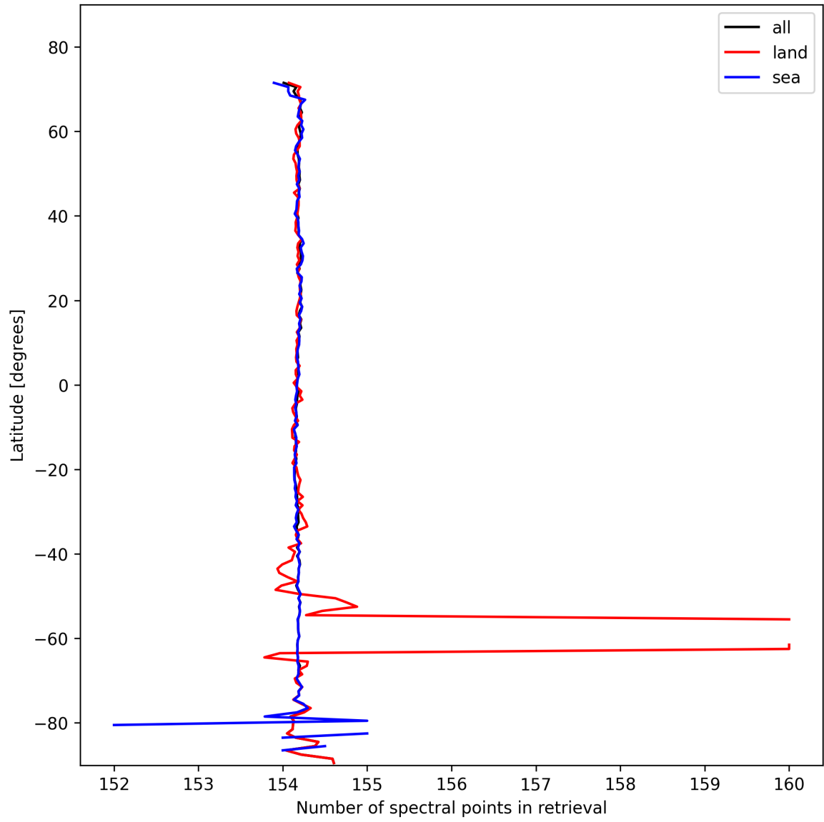
Figure 9: Zonal average of “Number of spectral points in retrieval” for 2025-10-29 to 2025-10-30.
