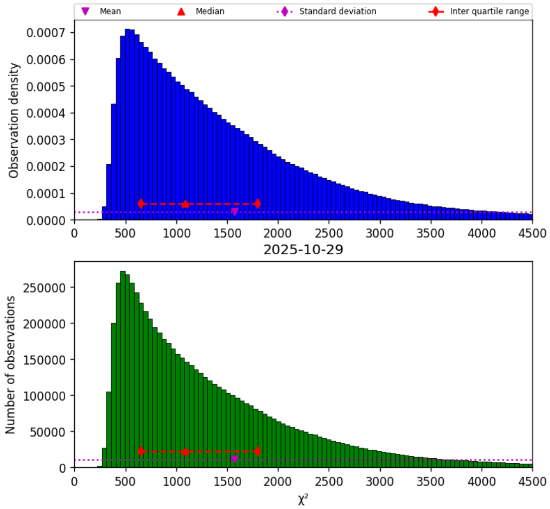
Figure 17: Histogram of “ \chi^2 ” for 2025-10-29 to 2025-10-30
