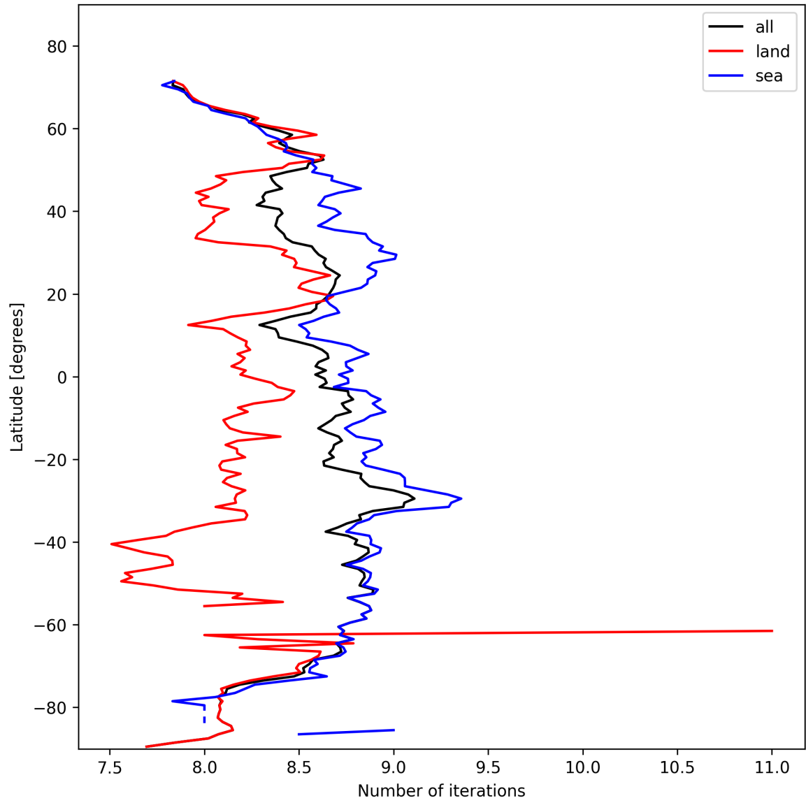
Figure 12: Zonal average of “Number of iterations” for 2025-10-29 to 2025-10-30.
