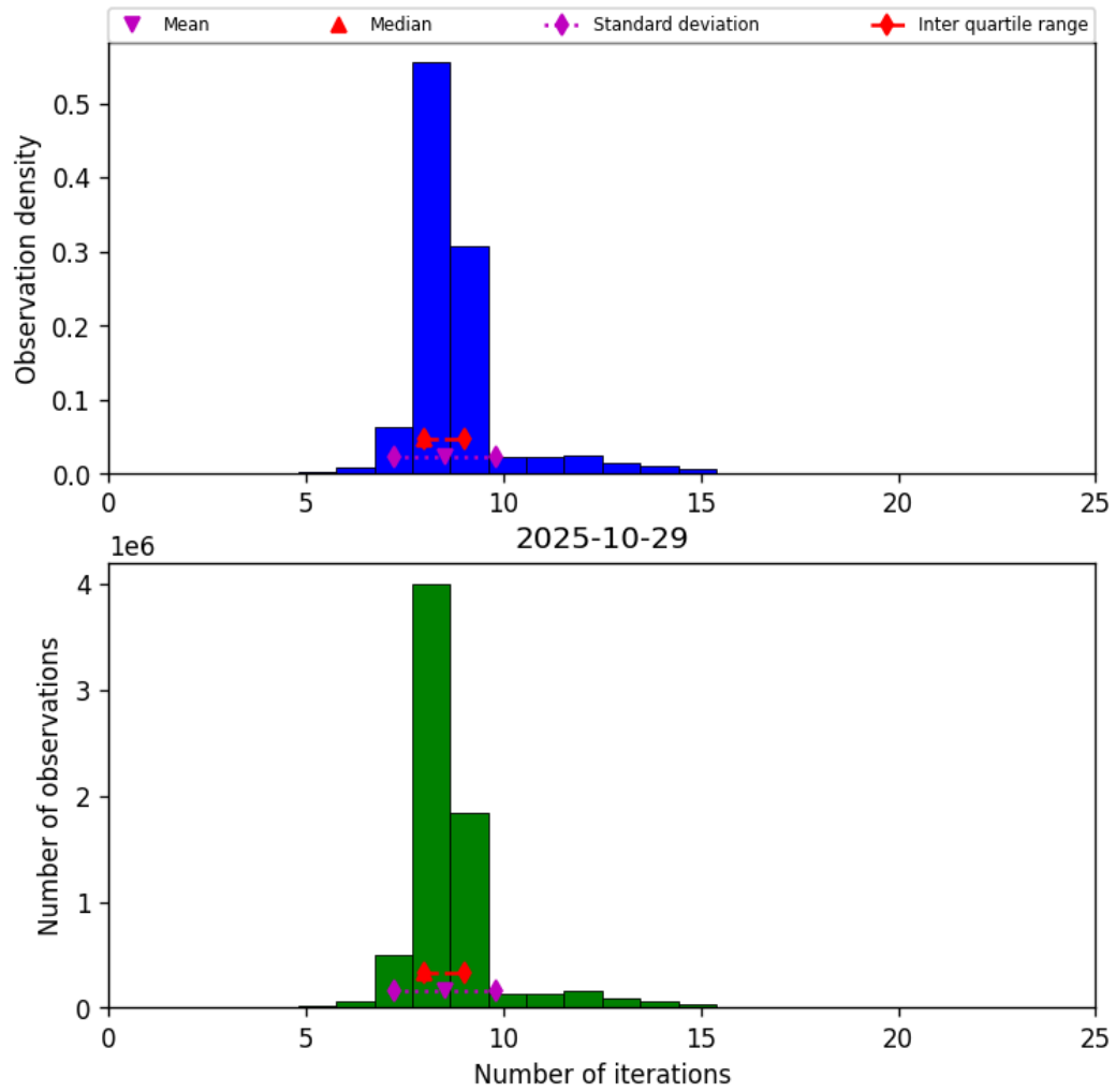
Figure 19: Histogram of “Number of iterations” for 2025-10-29 to 2025-10-30
