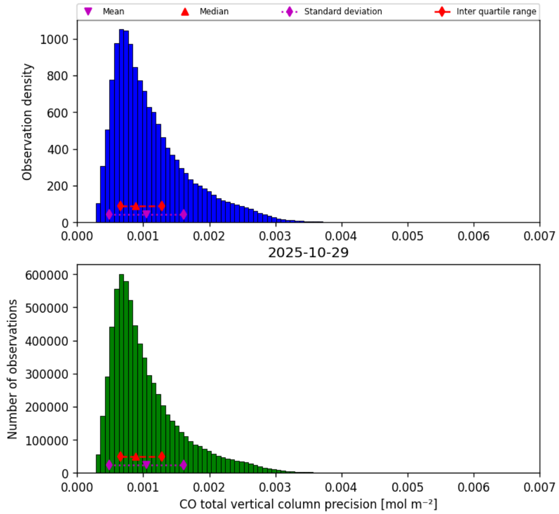
Figure 15: Histogram of “CO total vertical column precision” for 2025-10-29 to 2025-10-30
