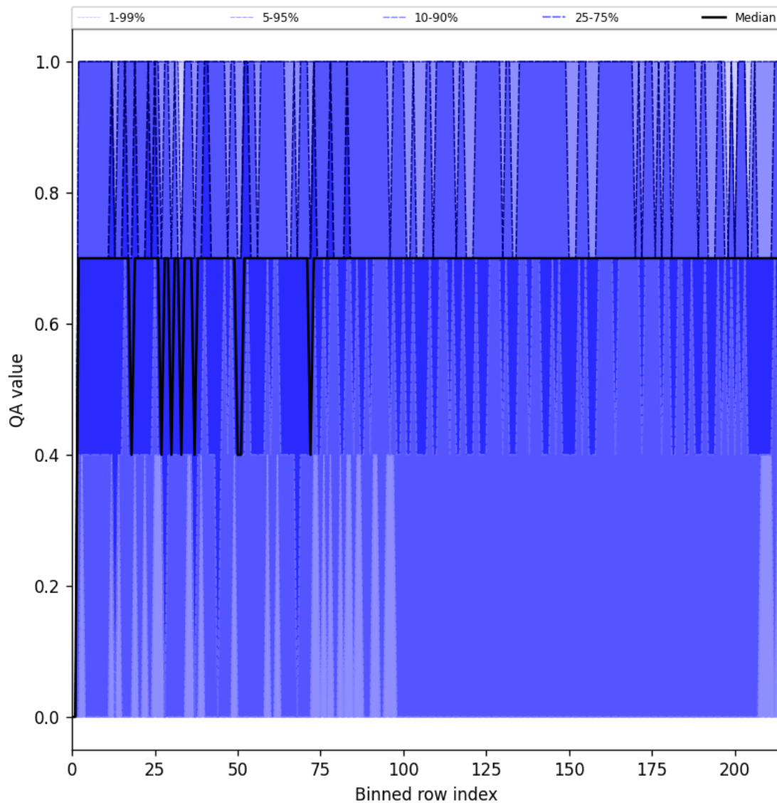
Figure 20: Along track statistics of “QA value” for 2025-10-29 to 2025-10-30
