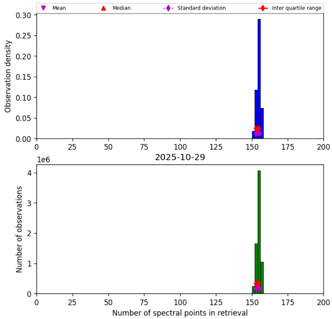
Figure 16: Histogram of “Number of spectral points in retrieval” for 2025-10-29 to 2025-10-30
