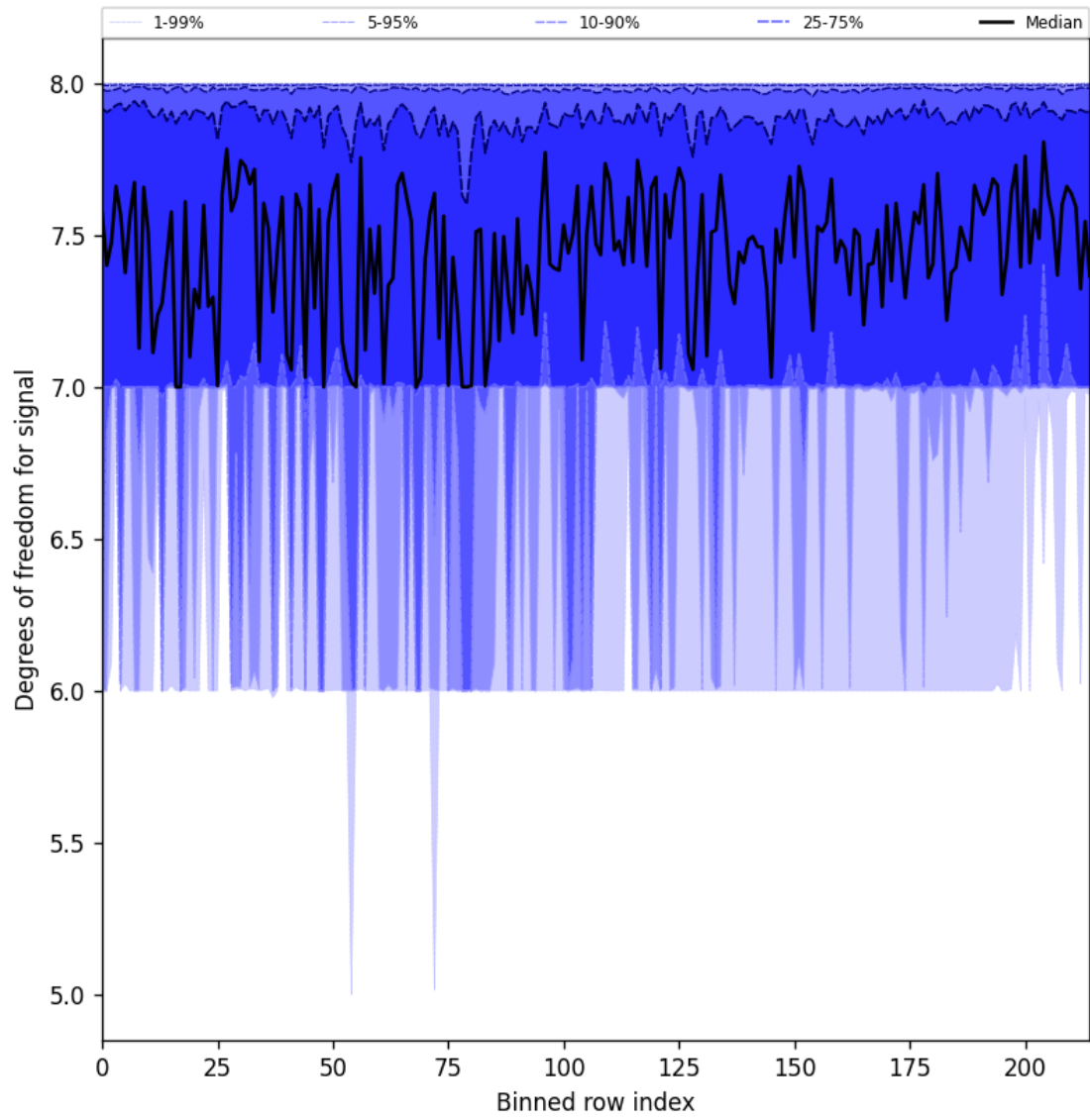
Figure 25: Along track statistics of “Degrees of freedom for signal” for 2025-10-29 to 2025-10-30
