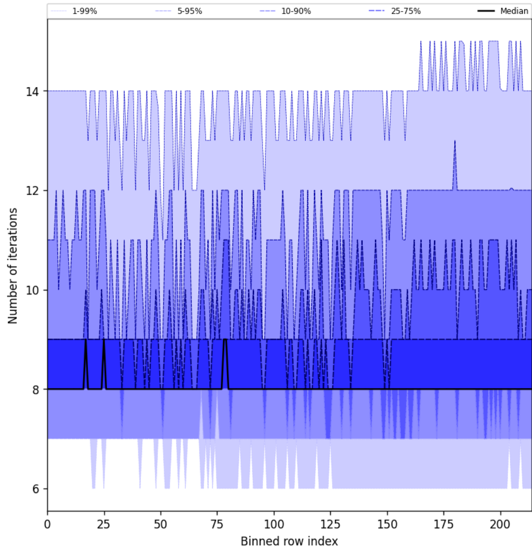
Figure 26: Along track statistics of “Number of iterations” for 2025-10-29 to 2025-10-30
