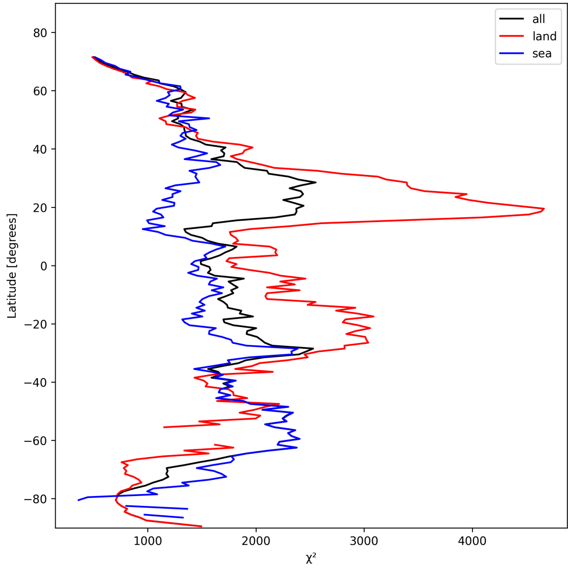
Figure 10: Zonal average of “ \chi^2 ” for 2025-10-29 to 2025-10-30.
