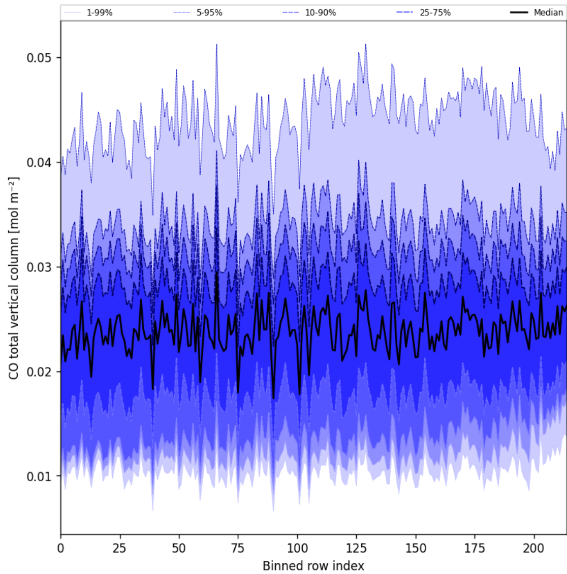
Figure 21: Along track statistics of “CO total vertical column” for 2025-10-29 to 2025-10-30
