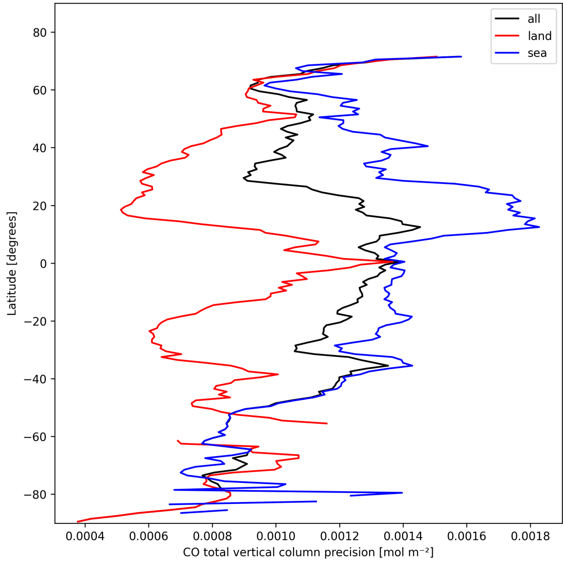
Figure 8: Zonal average of “CO total vertical column precision” for 2025-10-29 to 2025-10-30.
