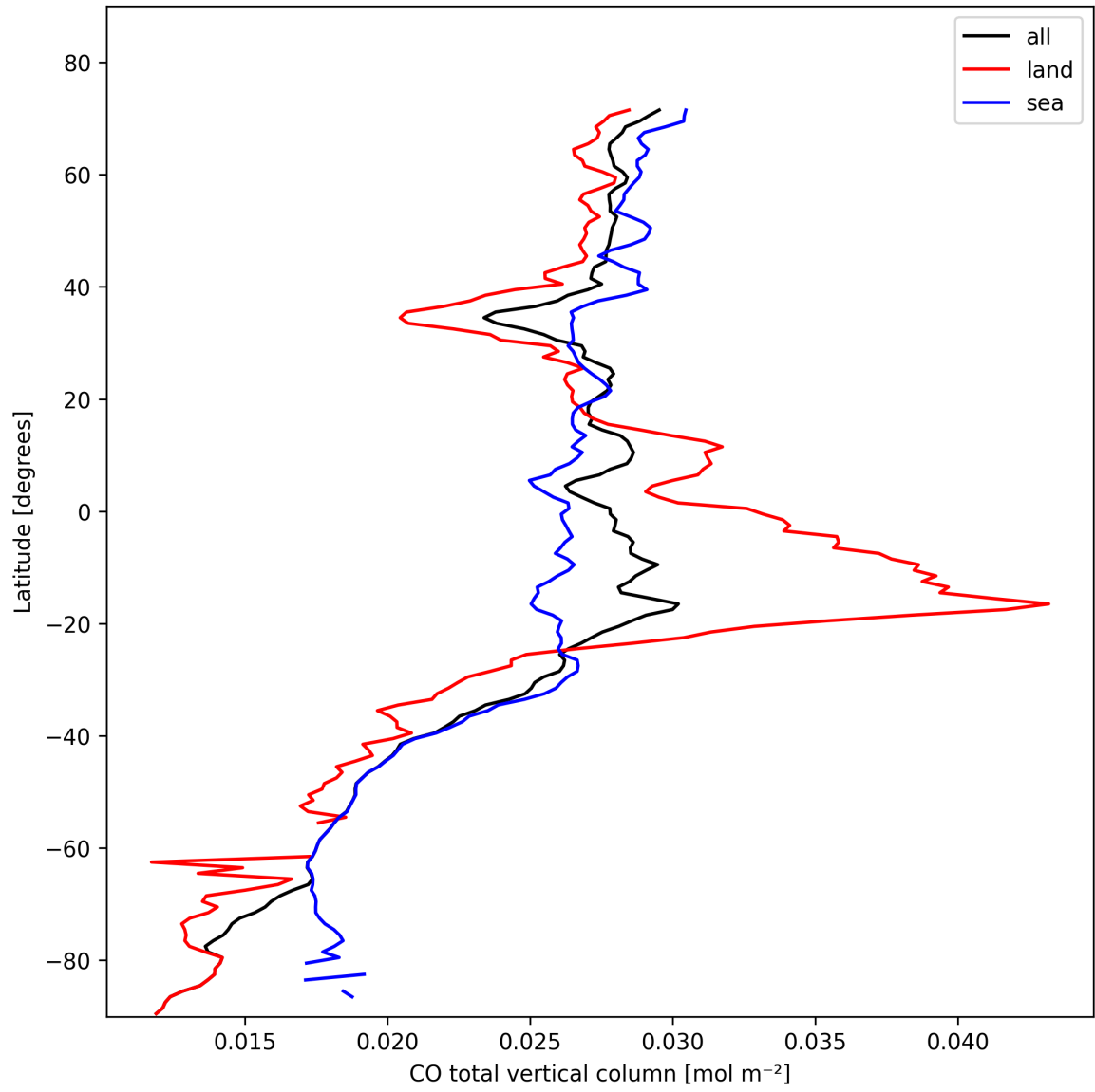
Figure 7: Zonal average of “CO total vertical column” for 2025-10-29 to 2025-10-30.
