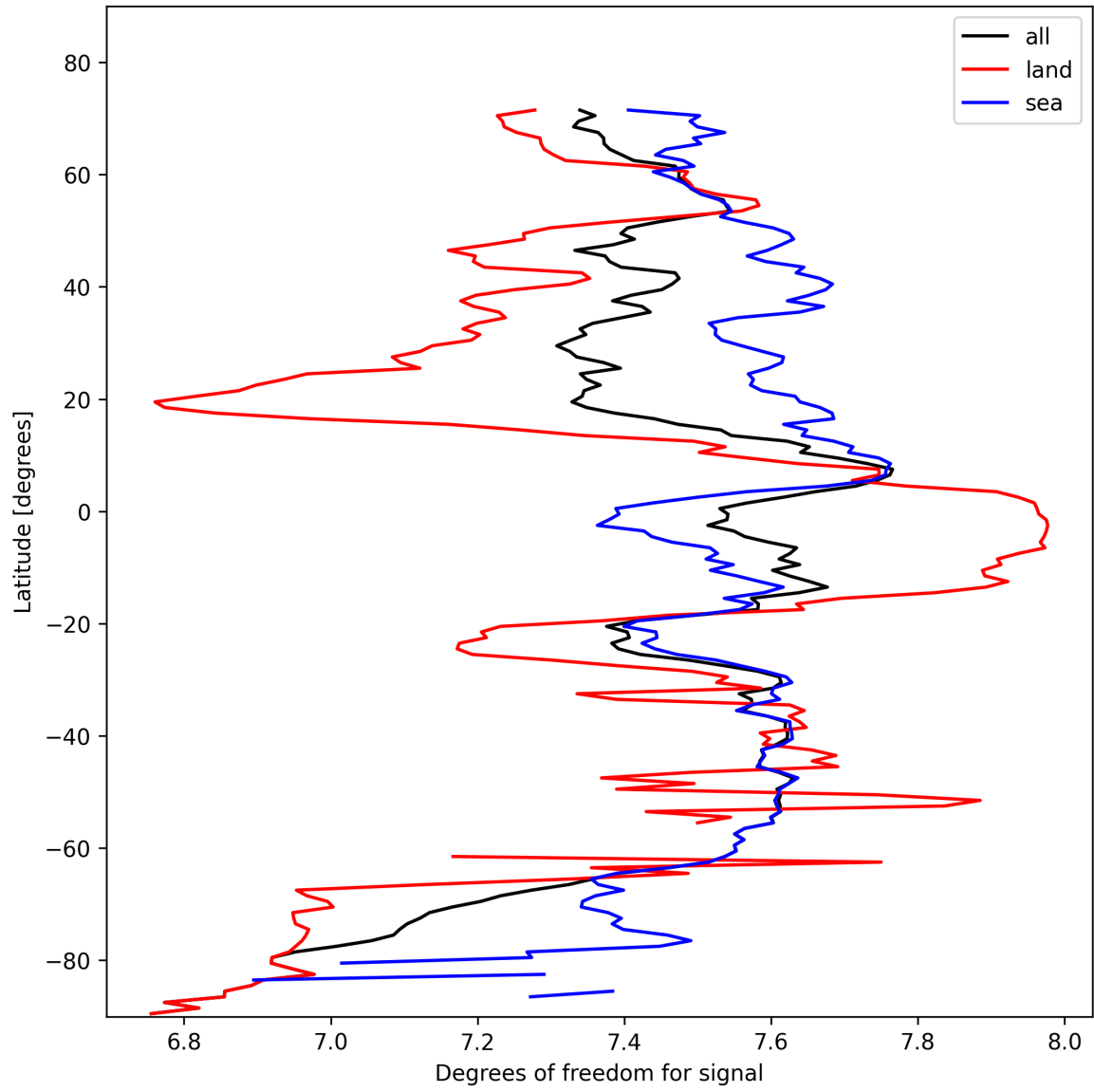
Figure 11: Zonal average of “Degrees of freedom for signal” for 2025-10-29 to 2025-10-30.
