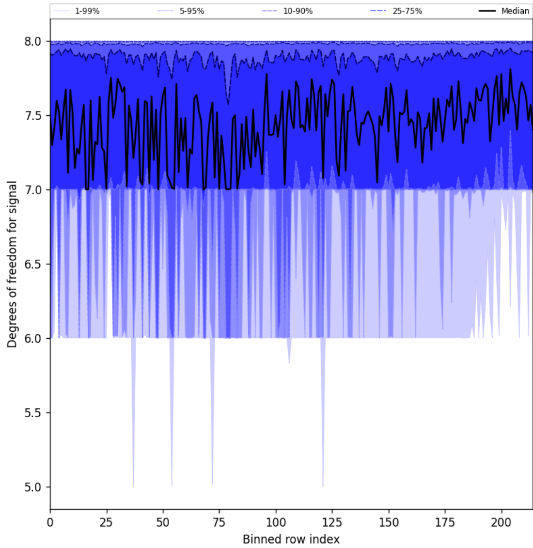
Figure 25: Along track statistics of “Degrees of freedom for signal” for 2025-10-30 to 2025-10-30
