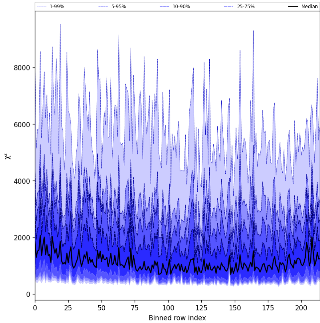
Figure 24: Along track statistics of “ \chi^2 ” for 2025-10-30 to 2025-10-30
