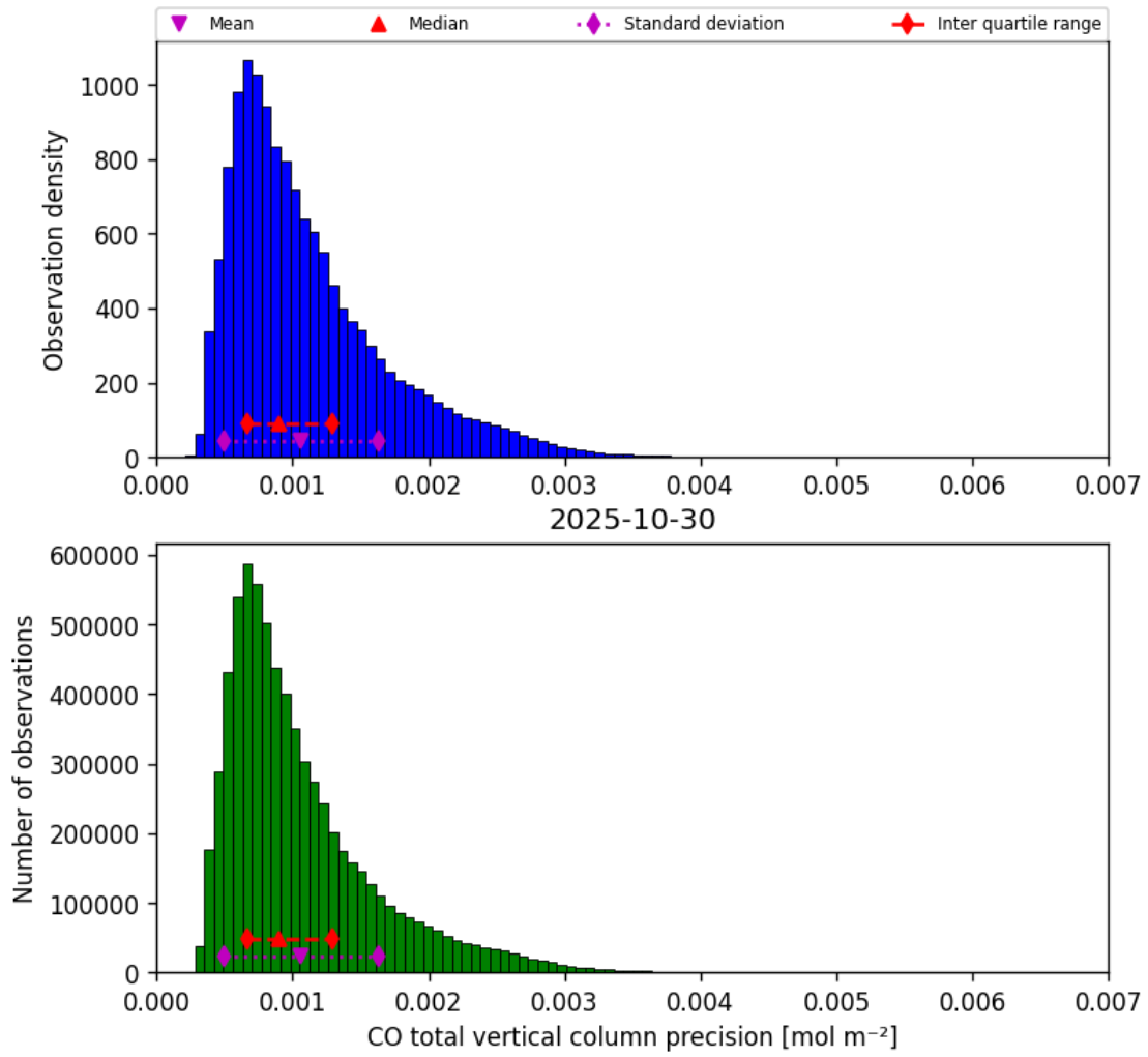
Figure 15: Histogram of “CO total vertical column precision” for 2025-10-30 to 2025-10-30
