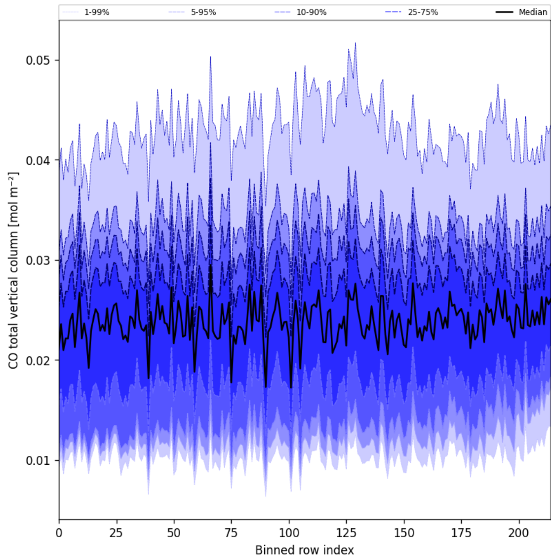
Figure 21: Along track statistics of “CO total vertical column” for 2025-10-30 to 2025-10-30
