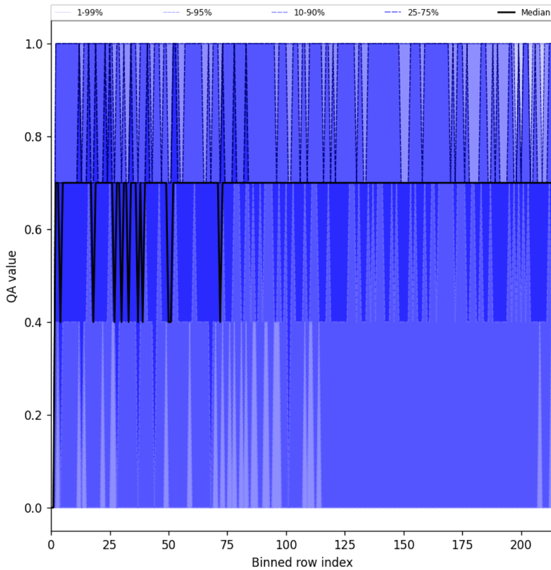
Figure 20: Along track statistics of “QA value” for 2025-10-30 to 2025-10-30
