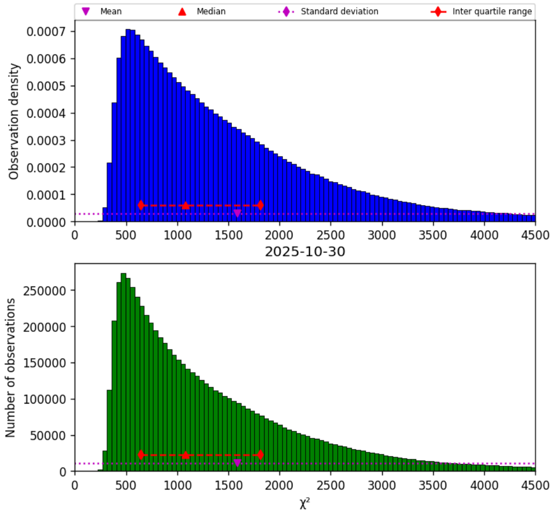
Figure 17: Histogram of " \chi^2 " for 2025-10-30 to 2025-10-30
