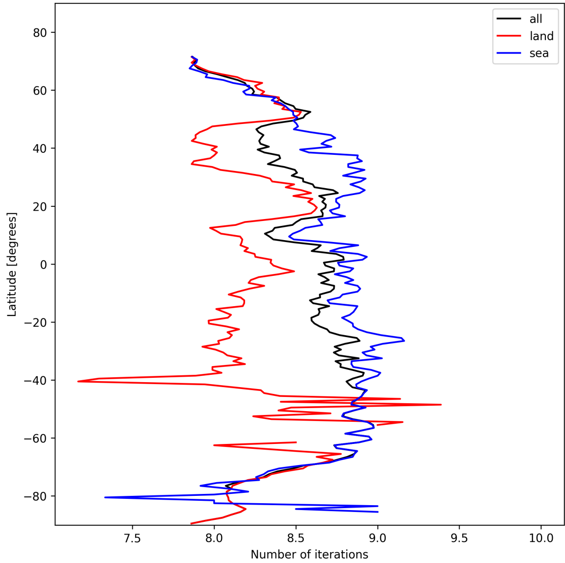
Figure 12: Zonal average of “Number of iterations” for 2025-10-30 to 2025-10-30.
