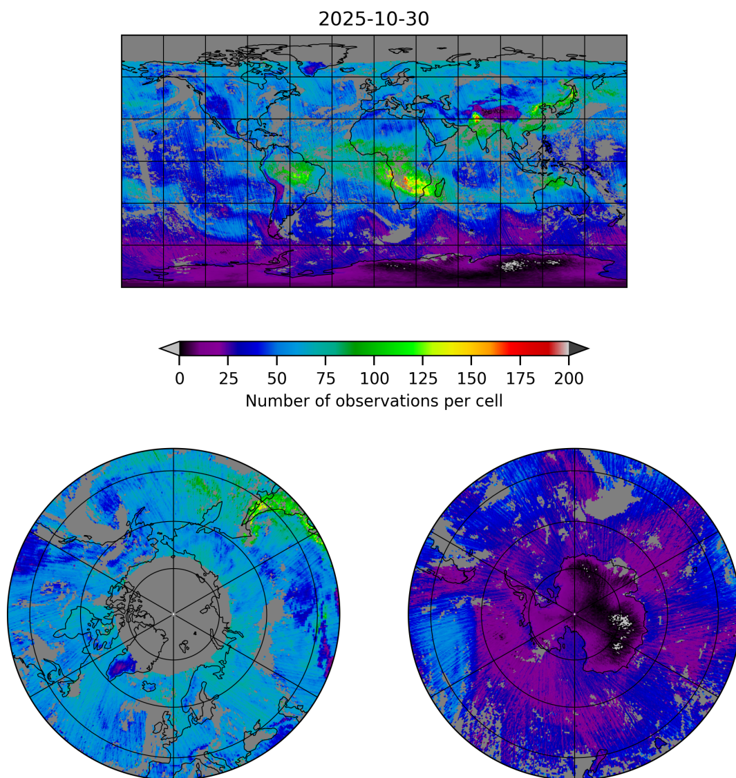
Figure 5: Map of the number of observations for 2025-10-30 to 2025-10-30
