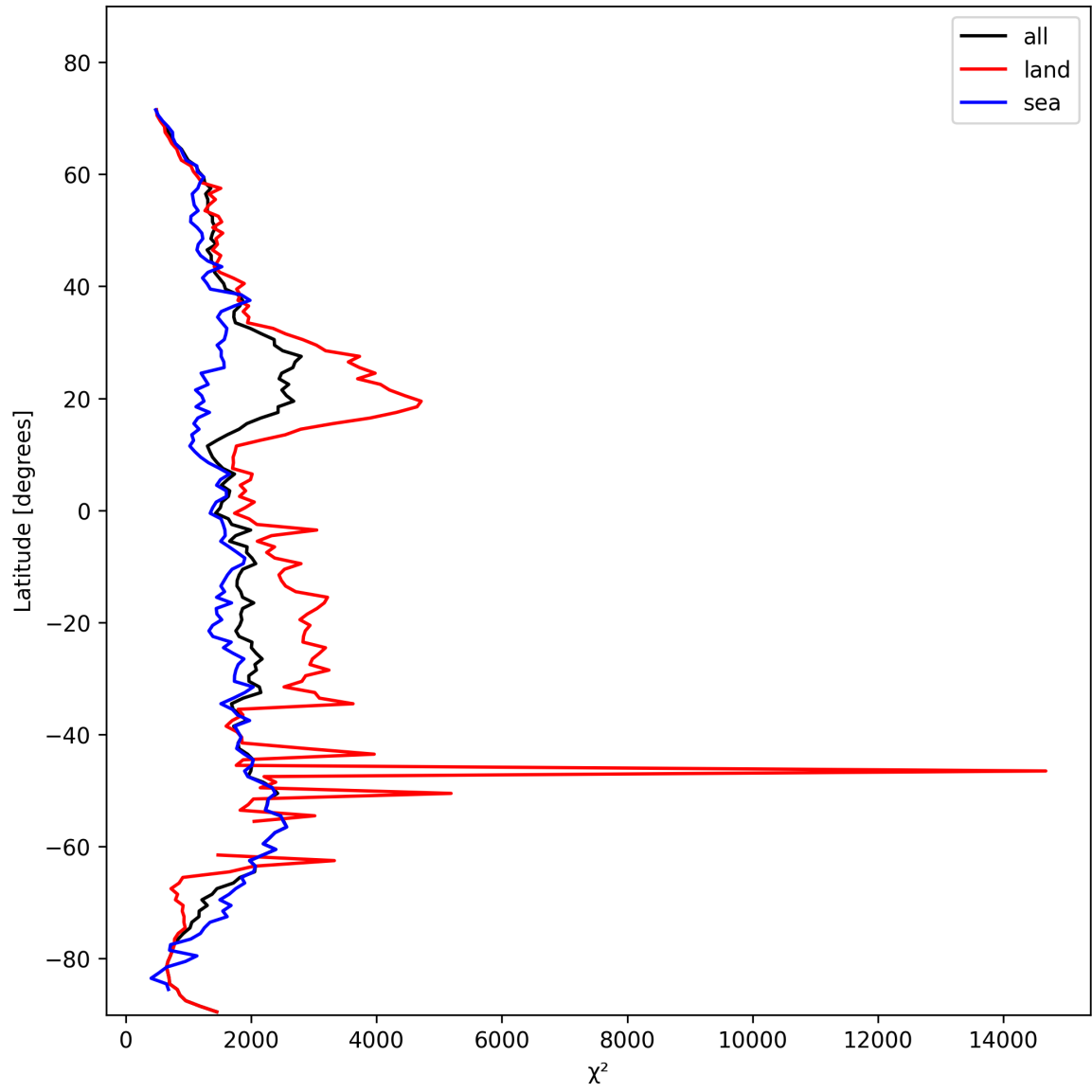
Figure 10: Zonal average of “ \chi^2 ” for 2025-10-30 to 2025-10-30.
