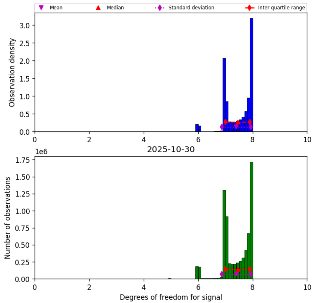
Figure 18: Histogram of “Degrees of freedom for signal” for 2025-10-30 to 2025-10-30
