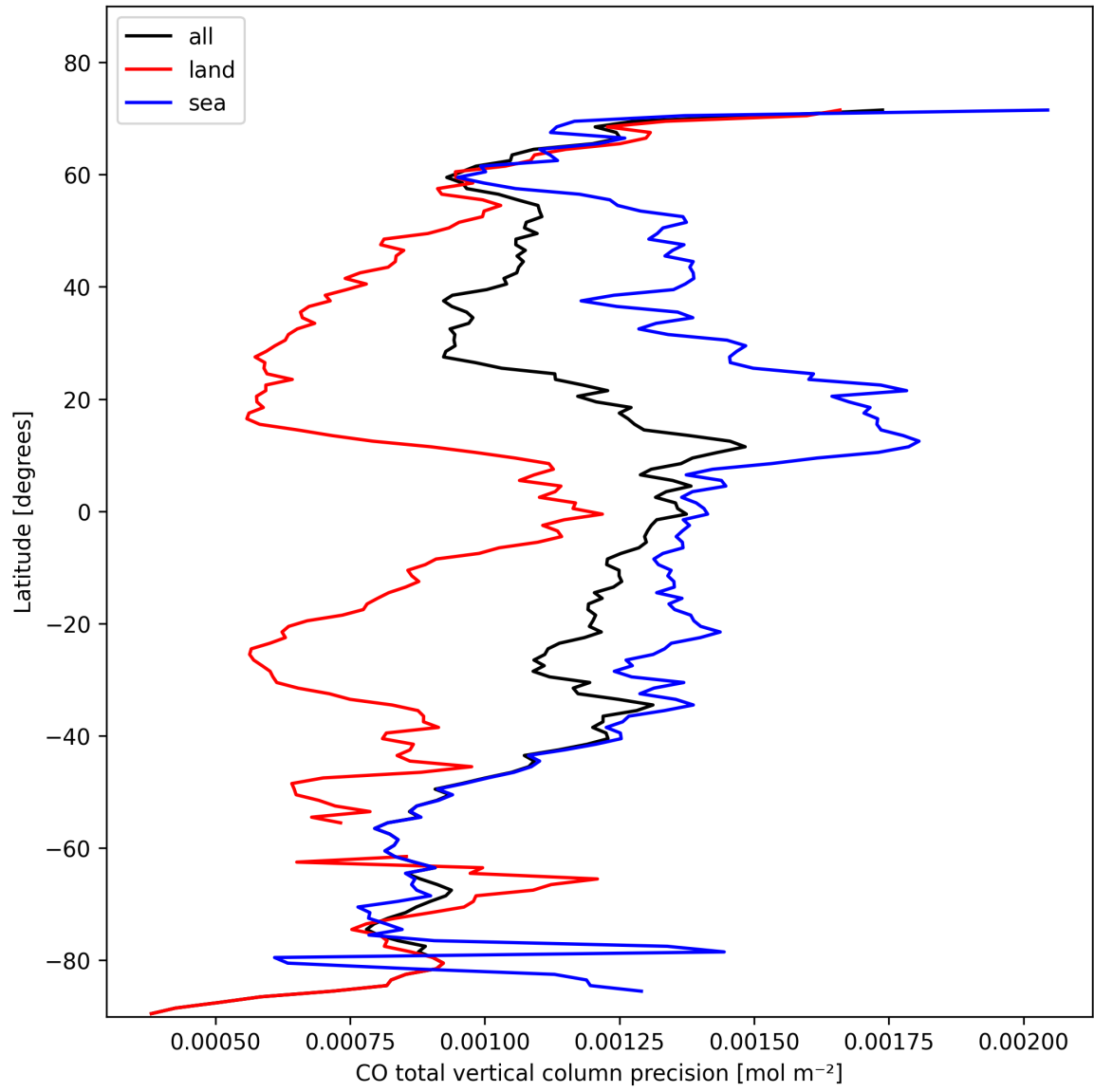
Figure 8: Zonal average of “CO total vertical column precision” for 2025-10-30 to 2025-10-30.
