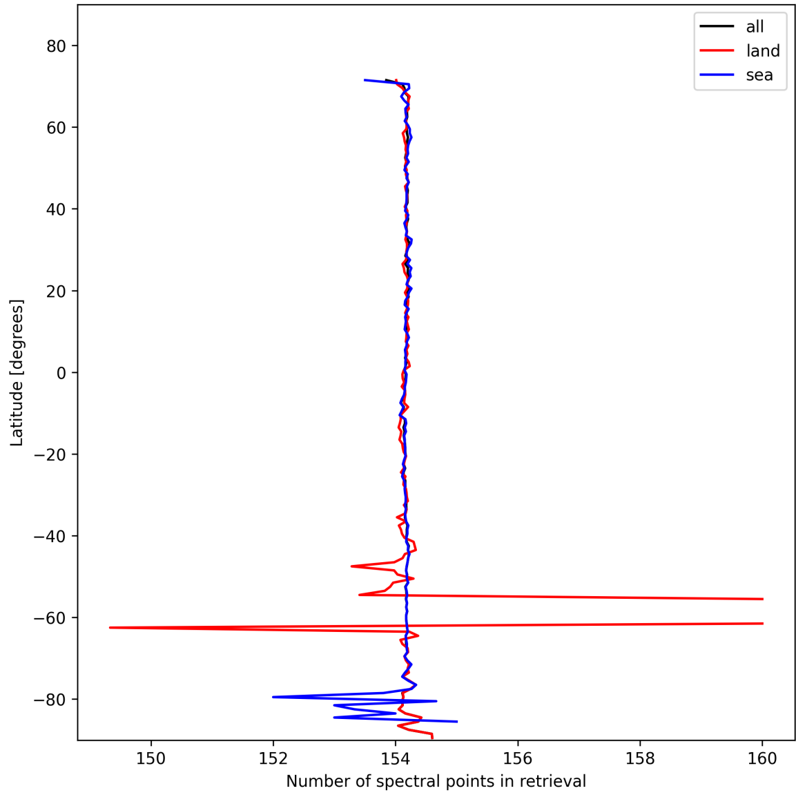
Figure 9: Zonal average of “Number of spectral points in retrieval” for 2025-10-30 to 2025-10-30.
