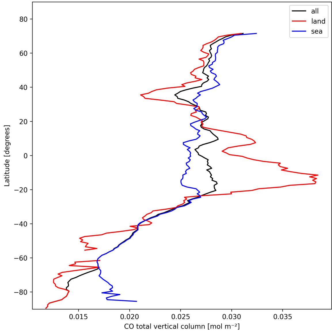
Figure 7: Zonal average of “CO total vertical column” for 2025-10-30 to 2025-10-30.
