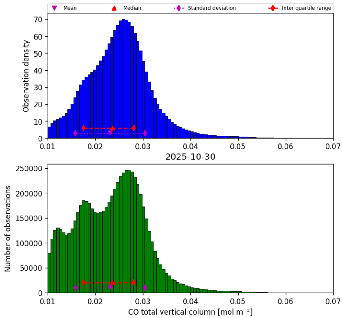
Figure 14: Histogram of “CO total vertical column” for 2025-10-30 to 2025-10-30
