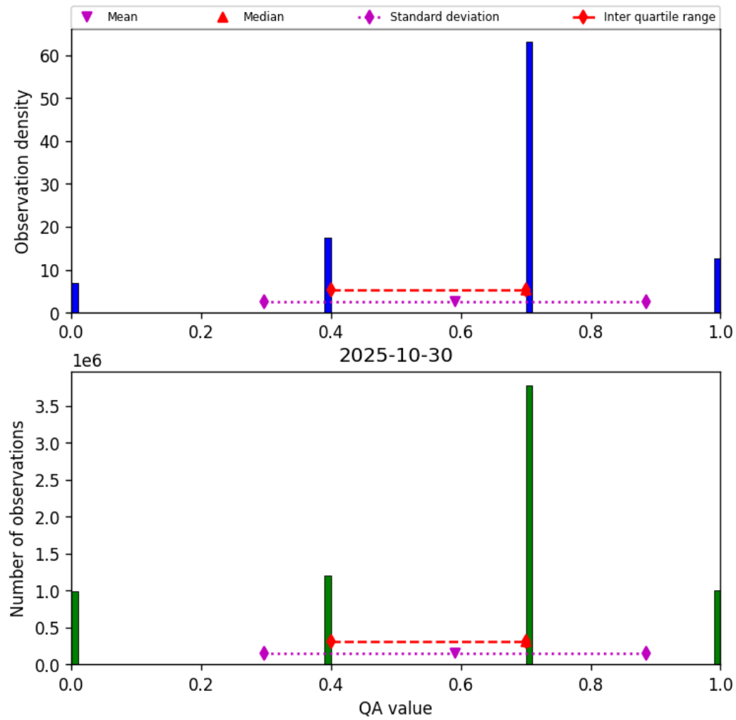
Figure 13: Histogram of “QA value” for 2025-10-30 to 2025-10-30
