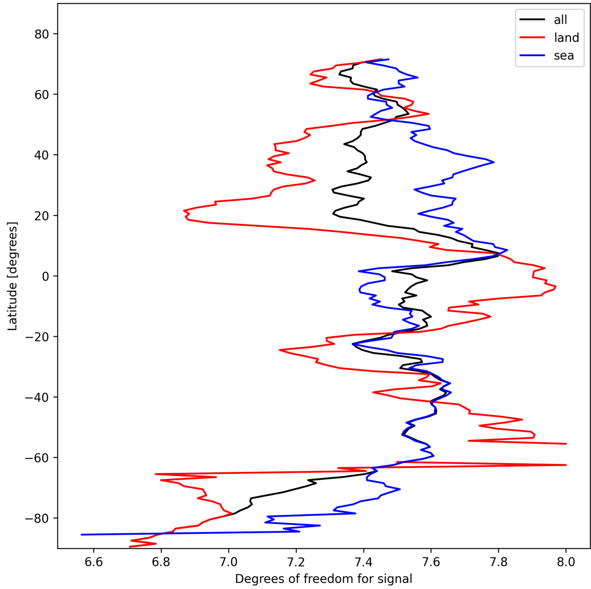
Figure 11: Zonal average of “Degrees of freedom for signal” for 2025-10-30 to 2025-10-30.
