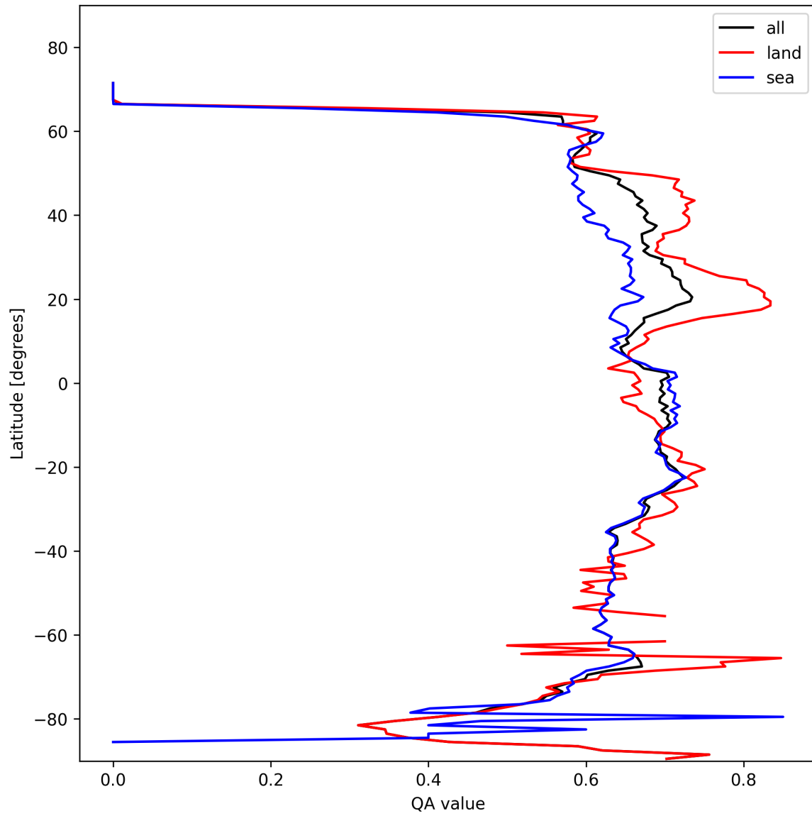
Figure 6: Zonal average of “QA value” for 2025-10-30 to 2025-10-30.
