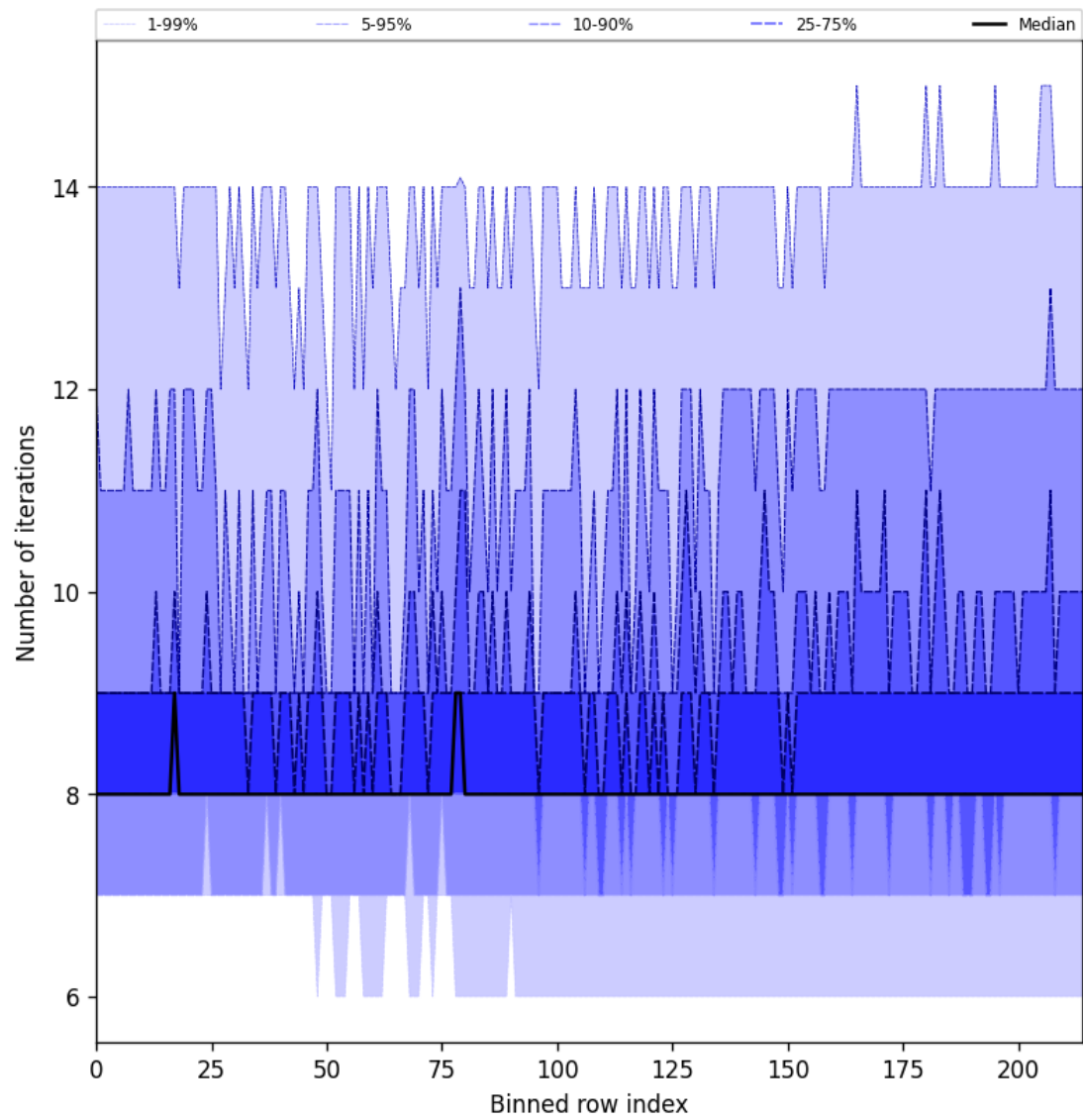
Figure 26: Along track statistics of “Number of iterations” for 2025-10-30 to 2025-10-30
