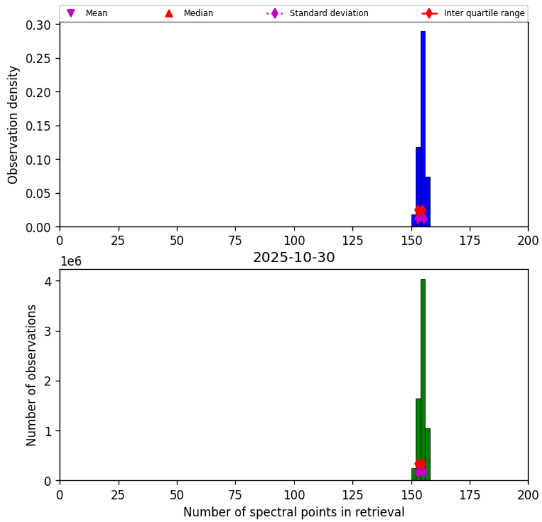
Figure 16: Histogram of “Number of spectral points in retrieval” for 2025-10-30 to 2025-10-30
