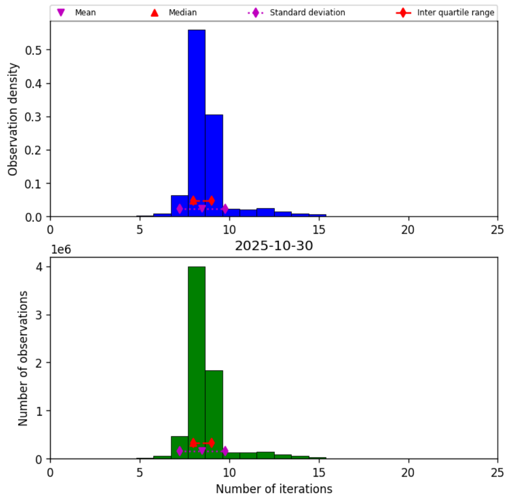
Figure 19: Histogram of “Number of iterations” for 2025-10-30 to 2025-10-30
