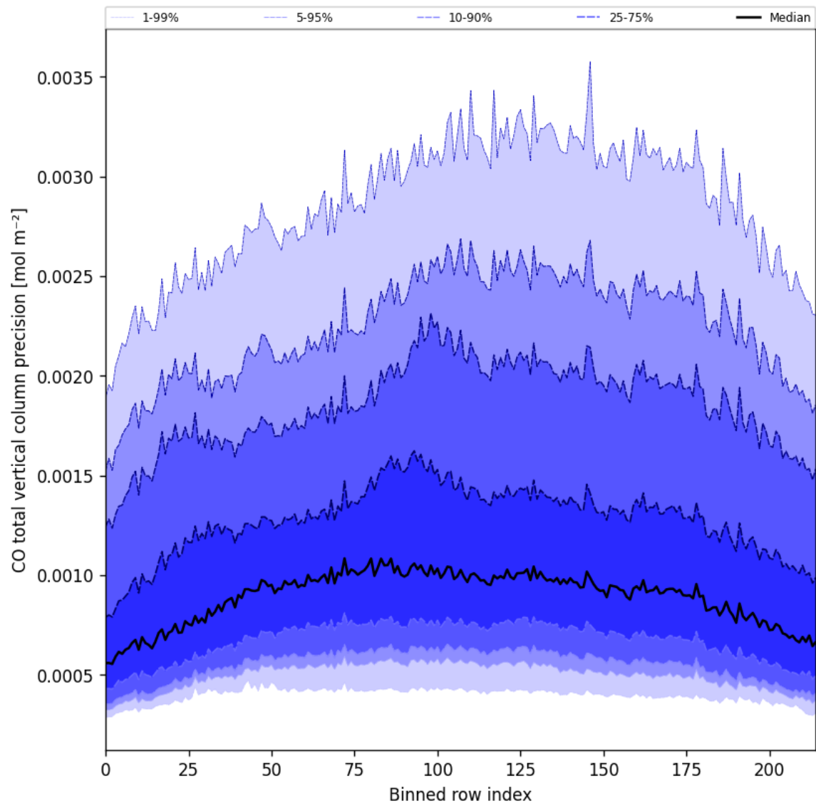
Figure 22: Along track statistics of “CO total vertical column precision” for 2025-10-30 to 2025-10-30
