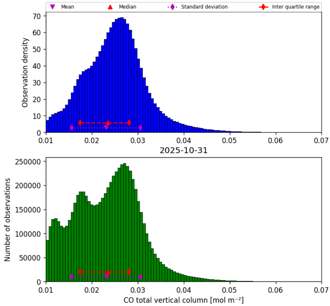
Figure 14: Histogram of “CO total vertical column” for 2025-10-31 to 2025-10-31
