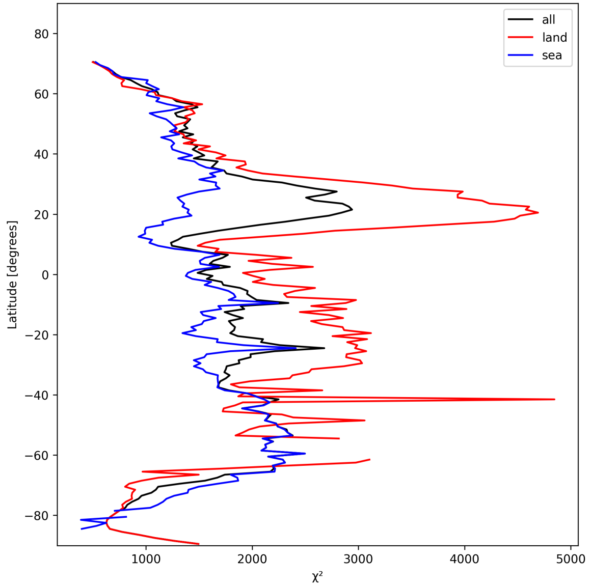
Figure 10: Zonal average of “ \chi^2 ” for 2025-10-31 to 2025-10-31.
