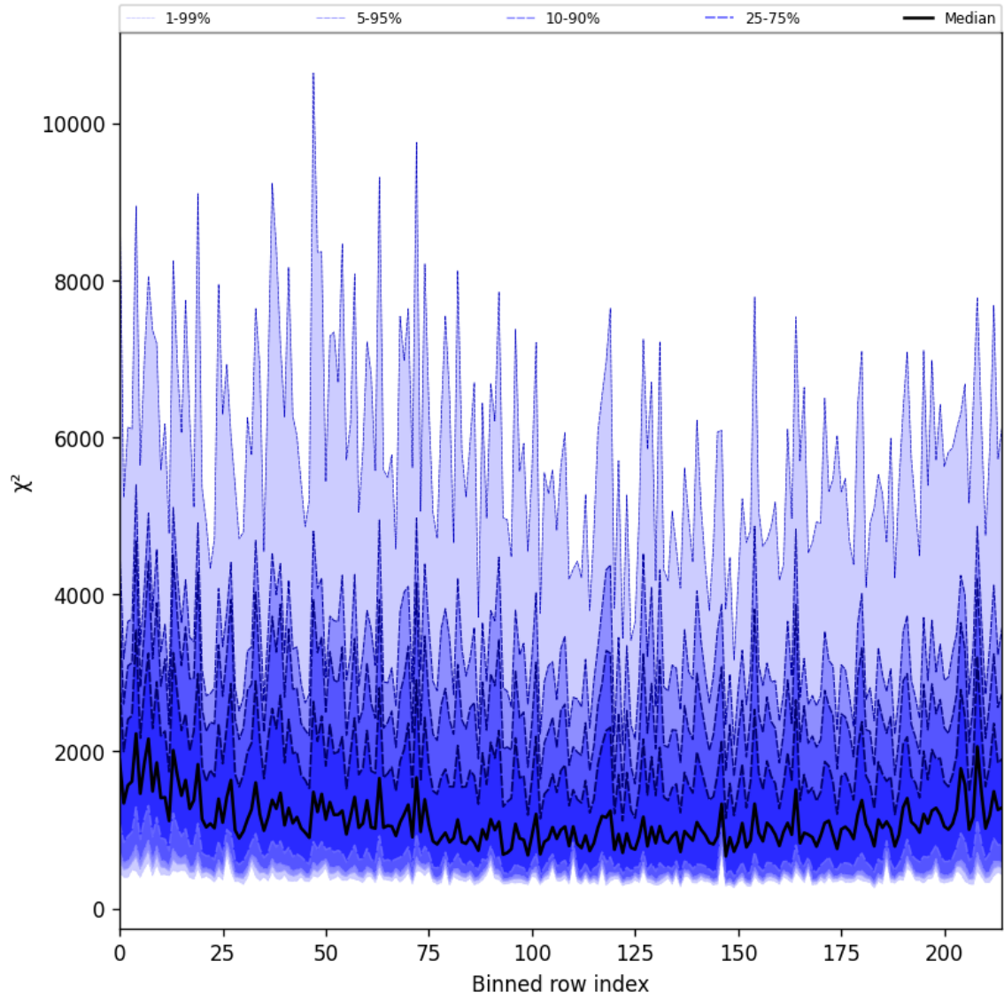
Figure 24: Along track statistics of “ \chi^2 ” for 2025-10-31 to 2025-10-31
