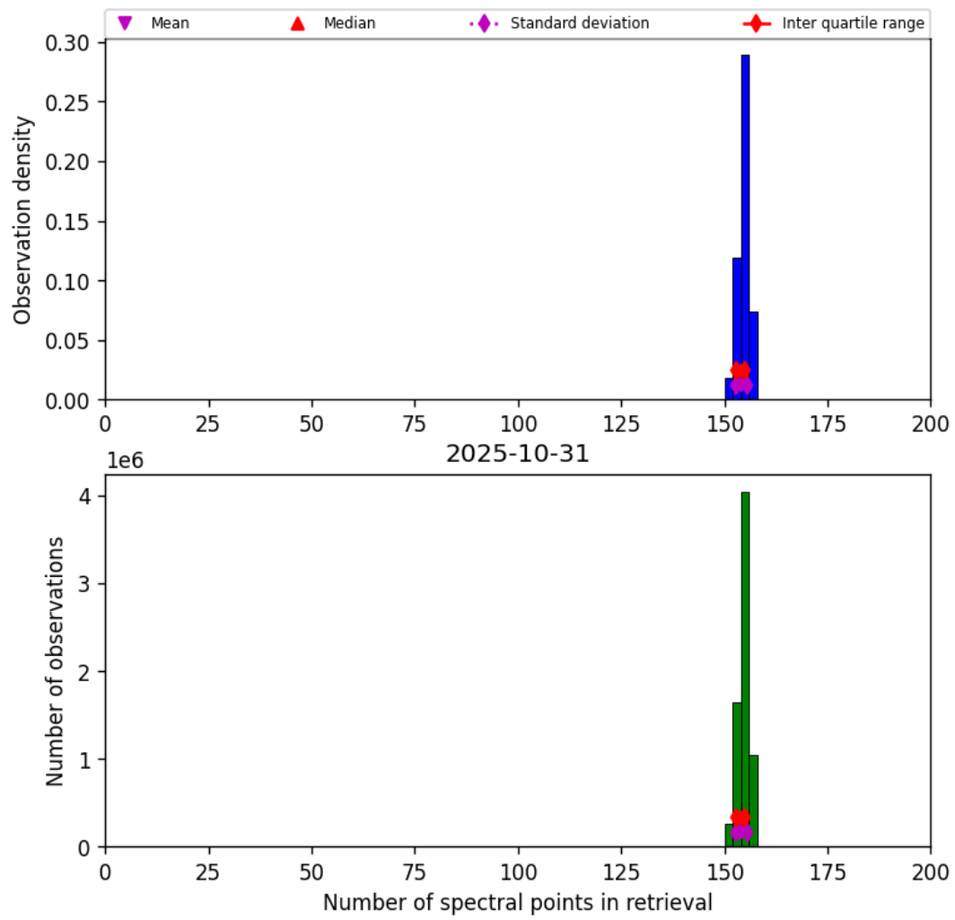
Figure 16: Histogram of “Number of spectral points in retrieval” for 2025-10-31 to 2025-10-31
