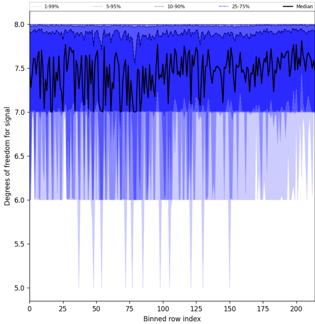
Figure 25: Along track statistics of “Degrees of freedom for signal” for 2025-10-31 to 2025-10-31
