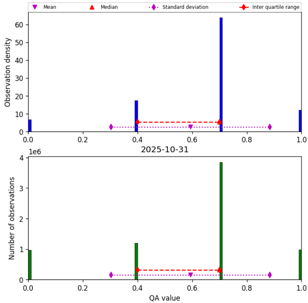
Figure 13: Histogram of “QA value” for 2025-10-31 to 2025-10-31
