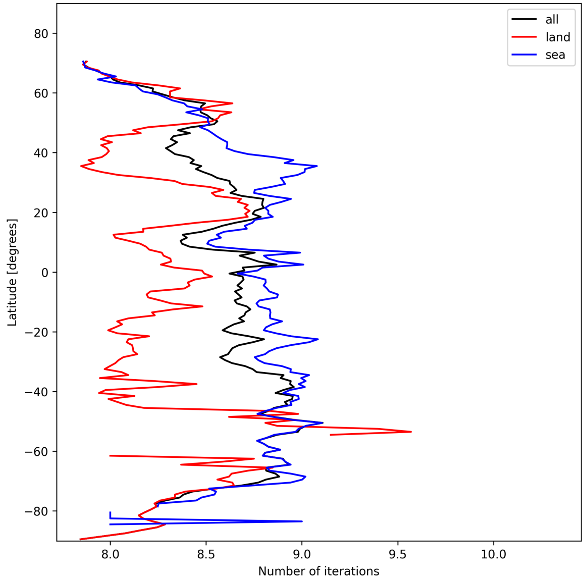
Figure 12: Zonal average of “Number of iterations” for 2025-10-31 to 2025-10-31.
