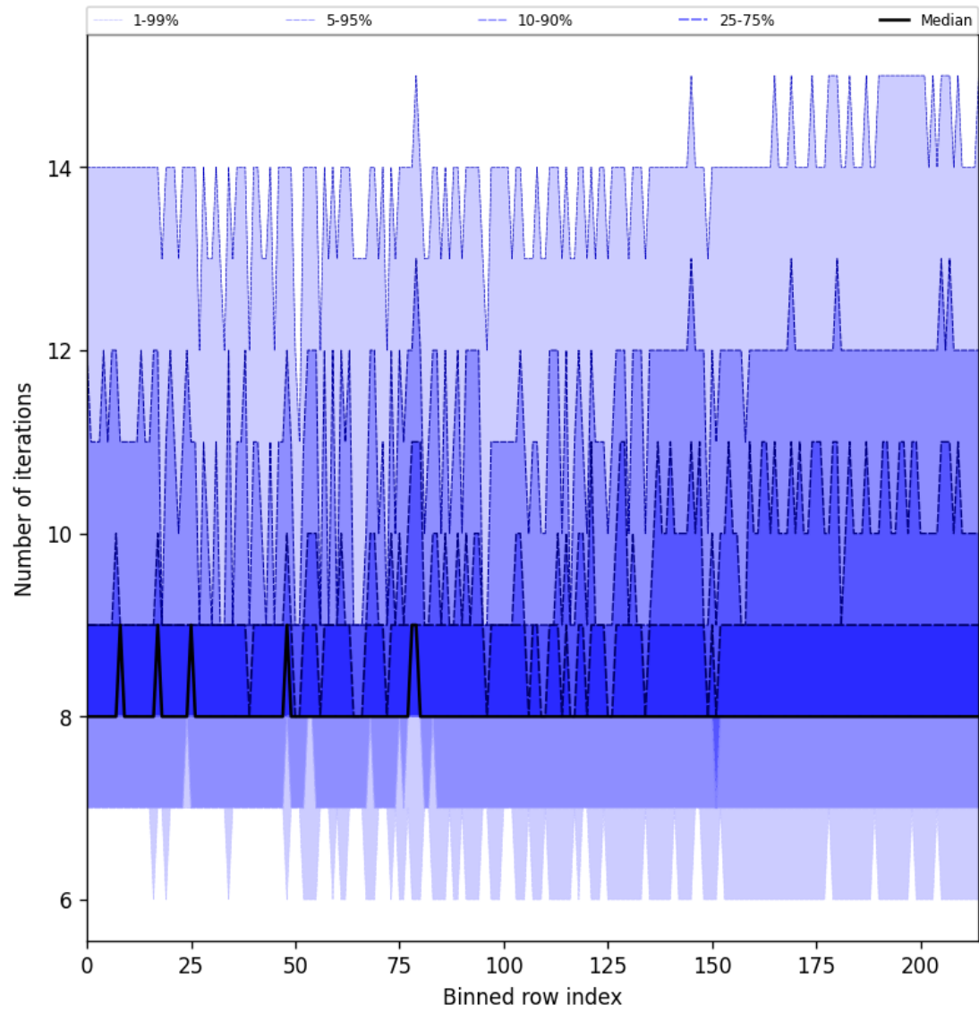
Figure 26: Along track statistics of “Number of iterations” for 2025-10-31 to 2025-10-31
