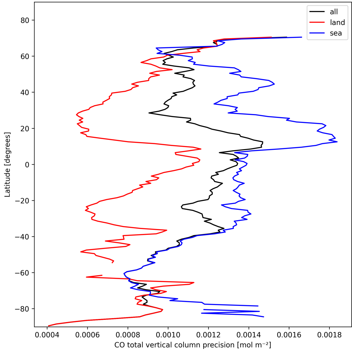
Figure 8: Zonal average of “CO total vertical column precision” for 2025-10-31 to 2025-10-31.
