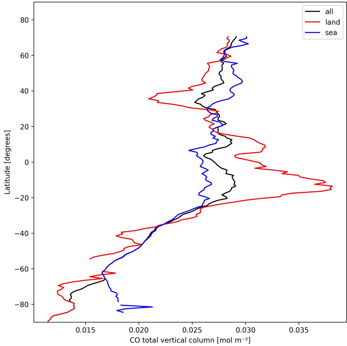
Figure 7: Zonal average of “CO total vertical column” for 2025-10-31 to 2025-10-31.
