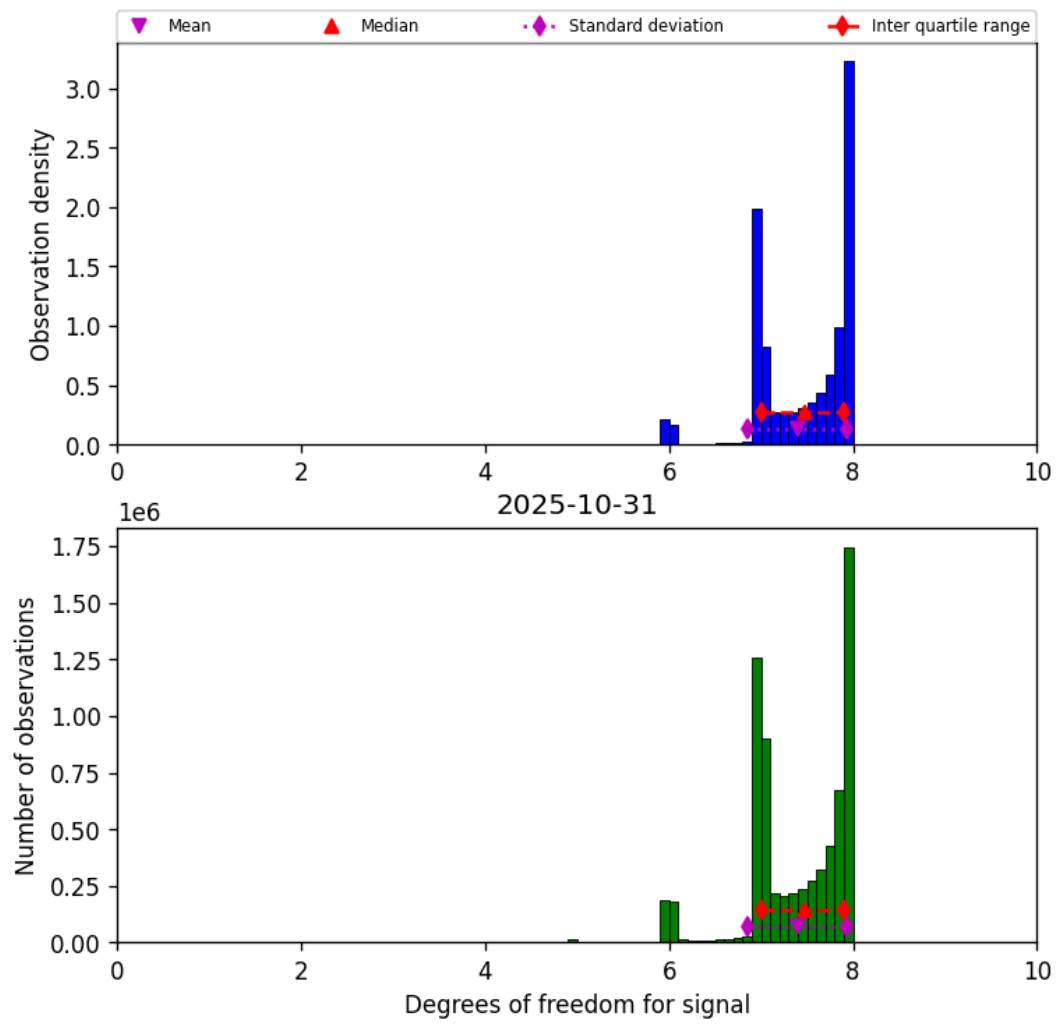
Figure 18: Histogram of “Degrees of freedom for signal” for 2025-10-31 to 2025-10-31
