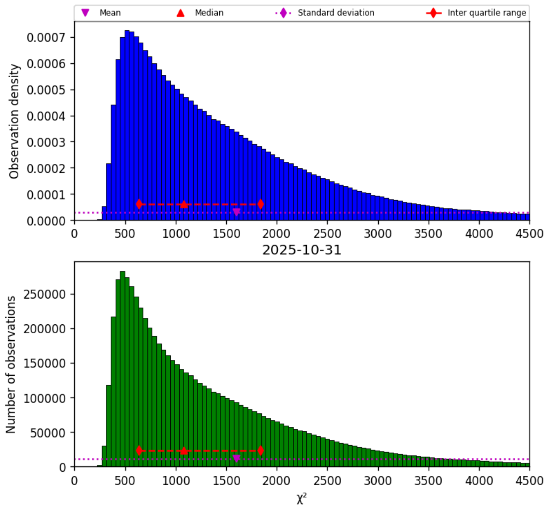
Figure 17: Histogram of “ \chi^2 ” for 2025-10-31 to 2025-10-31
