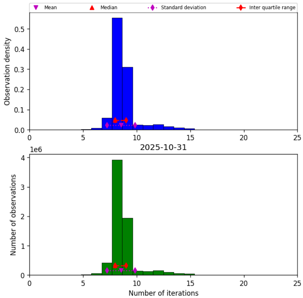
Figure 19: Histogram of “Number of iterations” for 2025-10-31 to 2025-10-31
