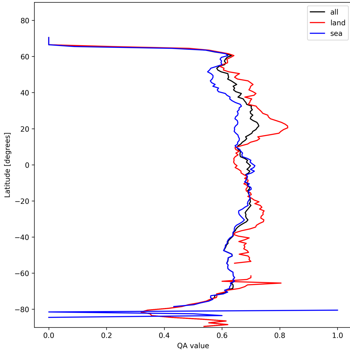
Figure 6: Zonal average of “QA value” for 2025-10-31 to 2025-10-31.
