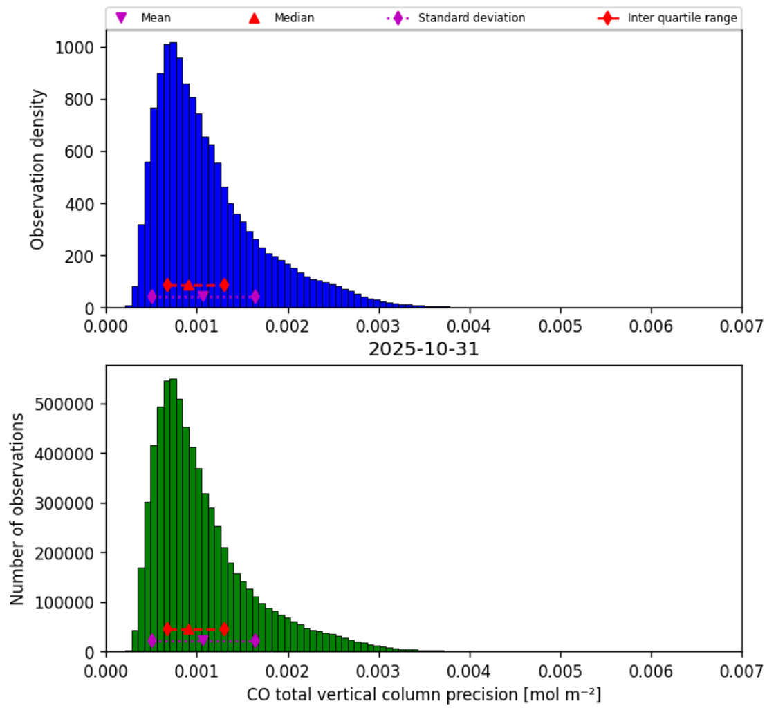
Figure 15: Histogram of “CO total vertical column precision” for 2025-10-31 to 2025-10-31
