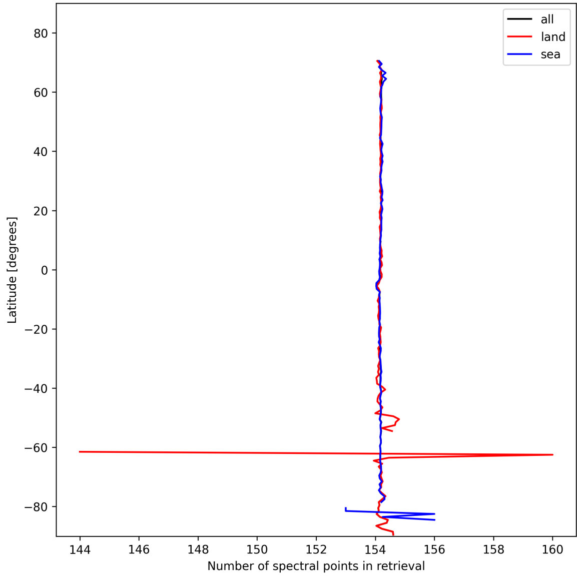
Figure 9: Zonal average of “Number of spectral points in retrieval” for 2025-10-31 to 2025-10-31.
