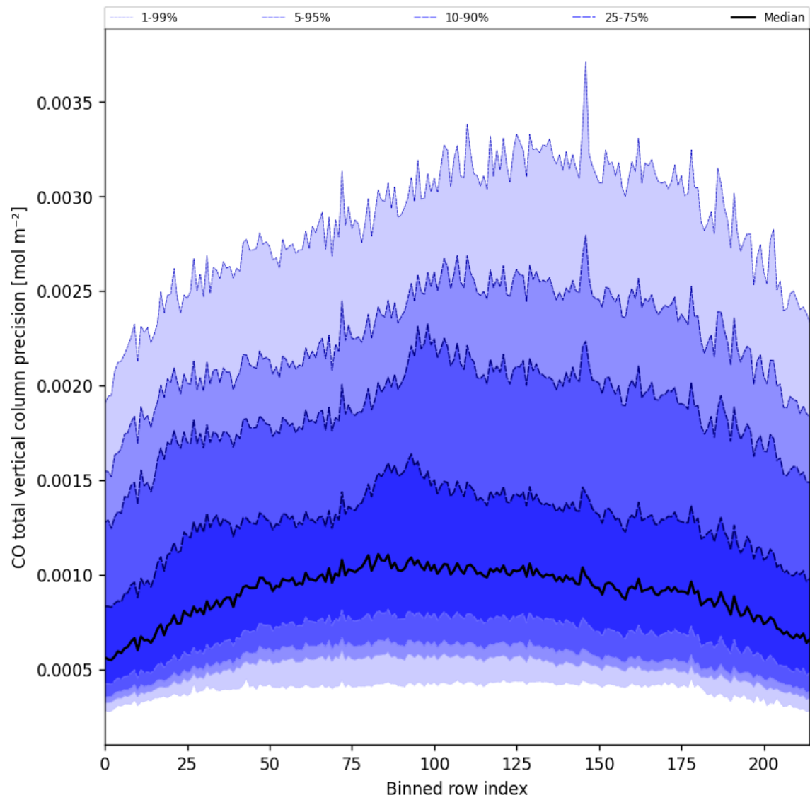
Figure 22: Along track statistics of “CO total vertical column precision” for 2025-10-31 to 2025-10-31
