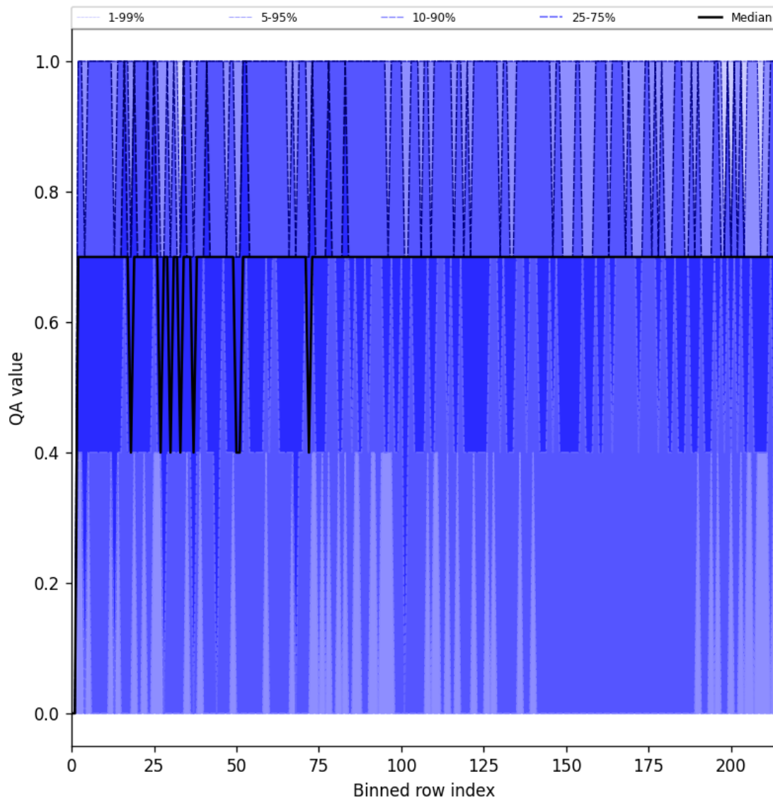
Figure 20: Along track statistics of “QA value” for 2025-10-31 to 2025-10-31
