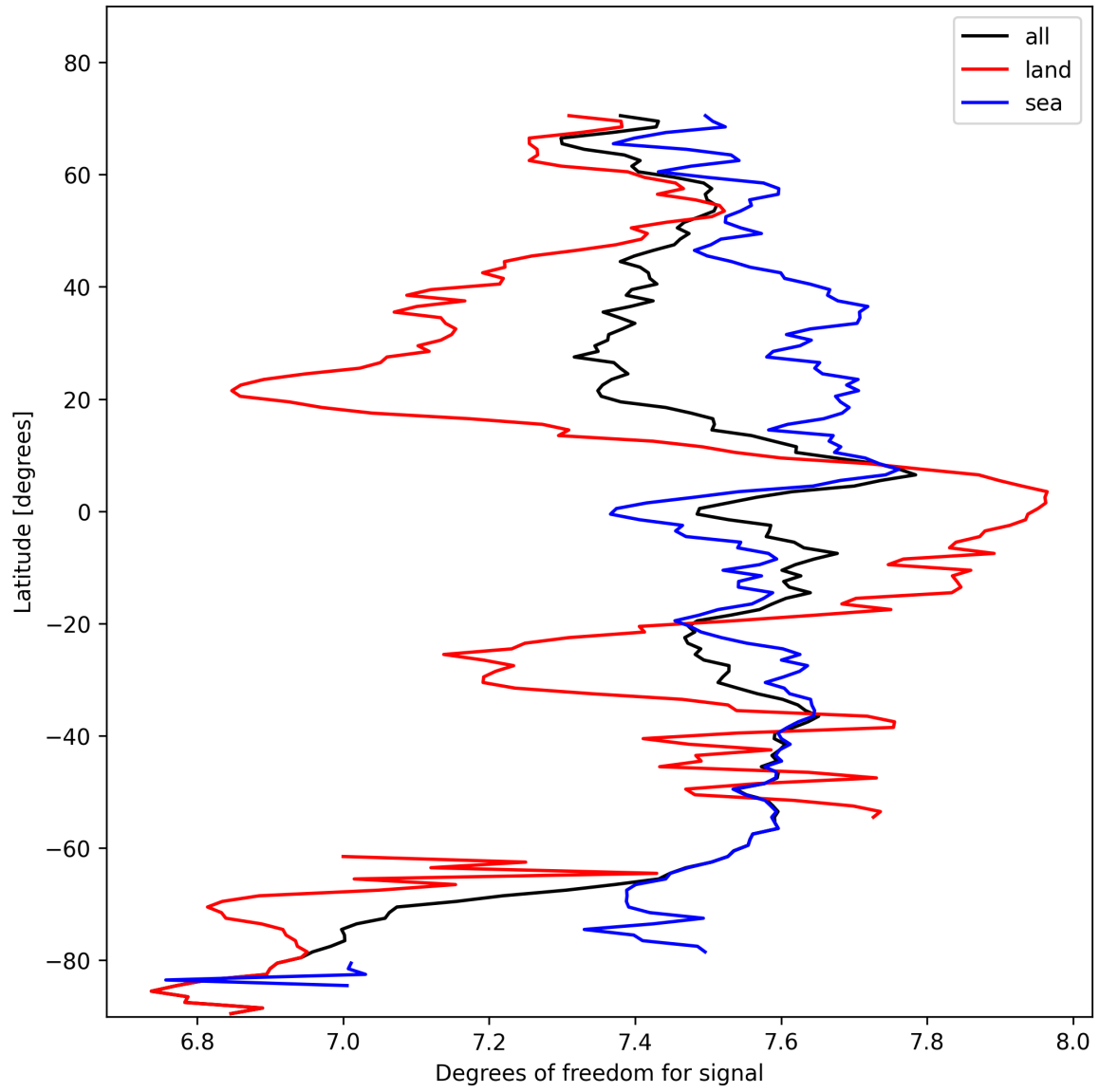
Figure 11: Zonal average of “Degrees of freedom for signal” for 2025-10-31 to 2025-10-31.
