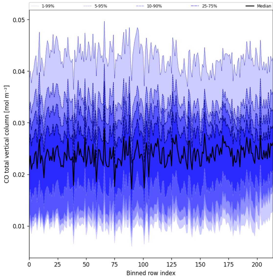
Figure 21: Along track statistics of “CO total vertical column” for 2025-10-31 to 2025-10-31
