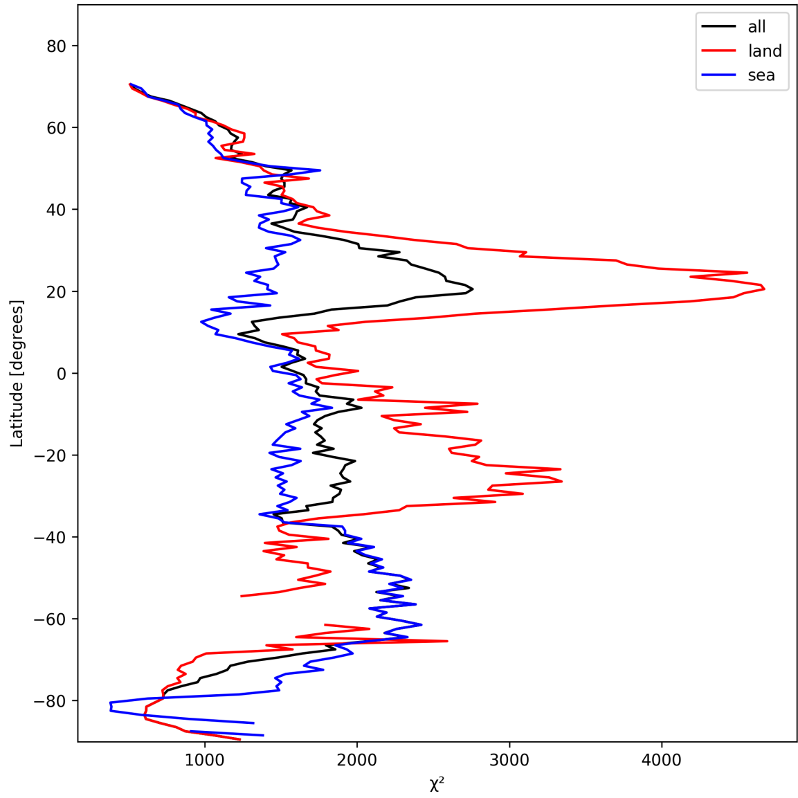
Figure 10: Zonal average of “ \chi^2 ” for 2025-11-01 to 2025-11-02.
