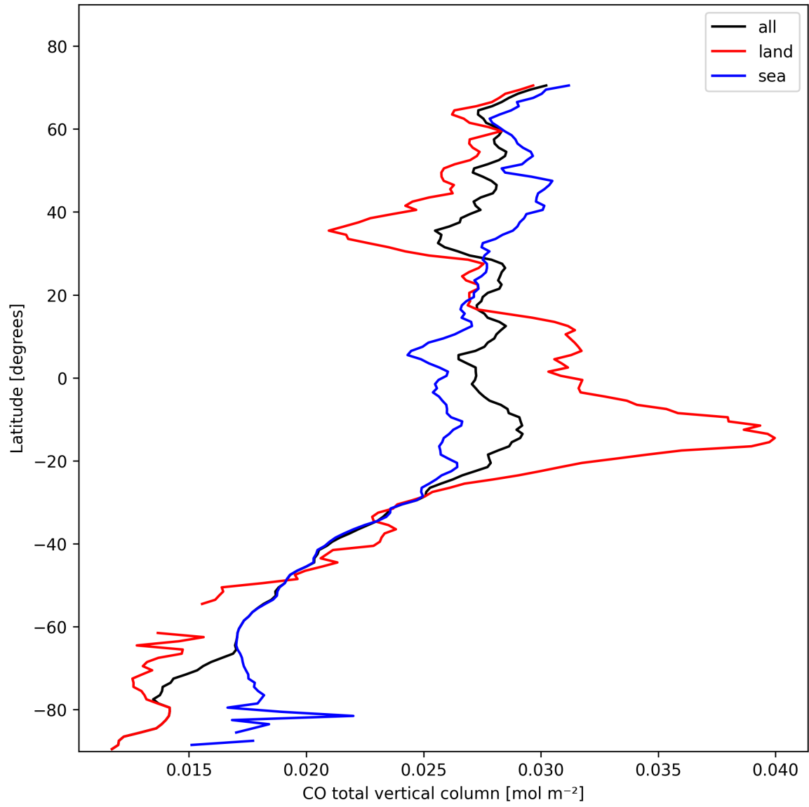
Figure 7: Zonal average of “CO total vertical column” for 2025-11-01 to 2025-11-02.
