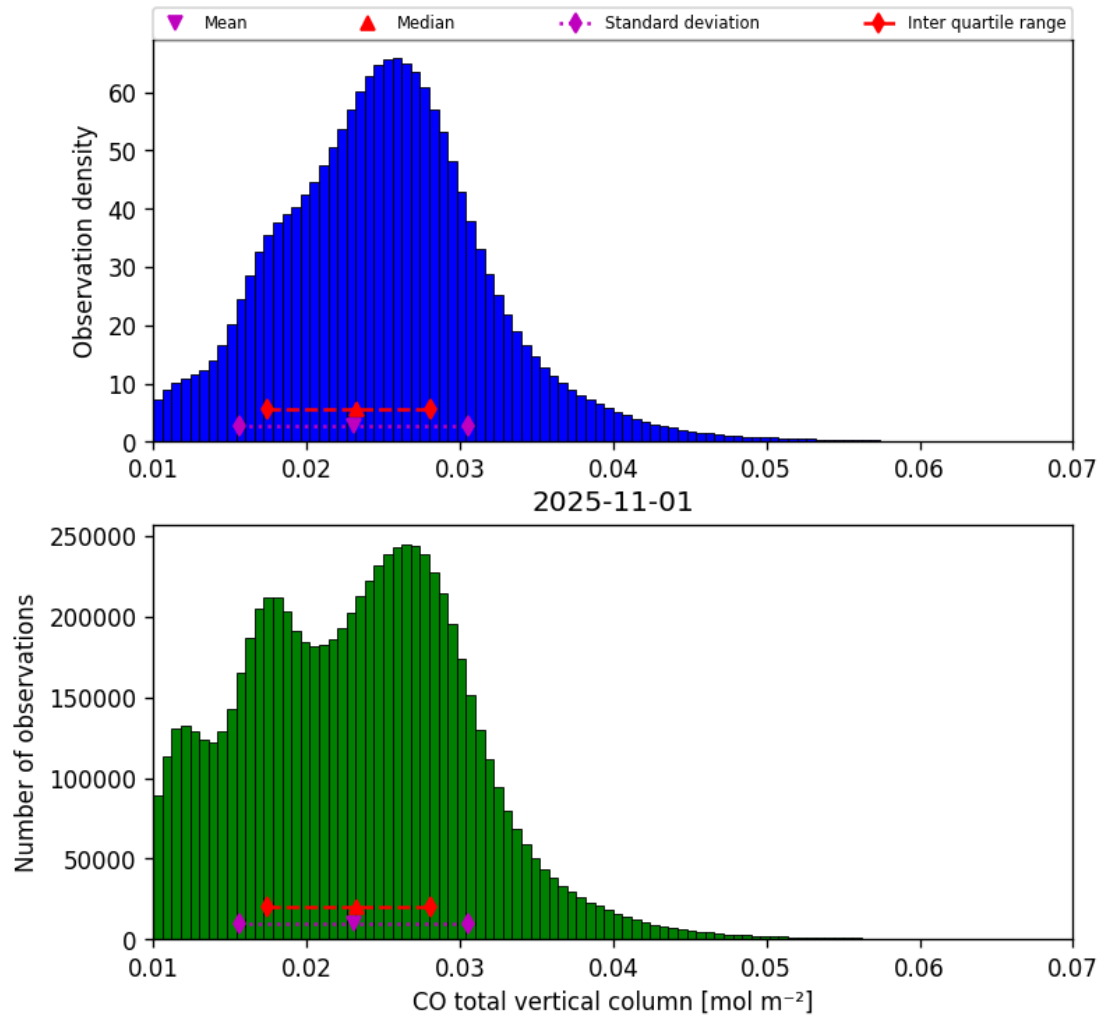
Figure 14: Histogram of “CO total vertical column” for 2025-11-01 to 2025-11-02
