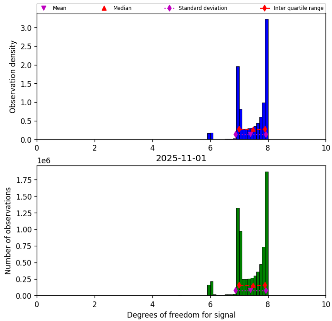
Figure 18: Histogram of “Degrees of freedom for signal” for 2025-11-01 to 2025-11-02
