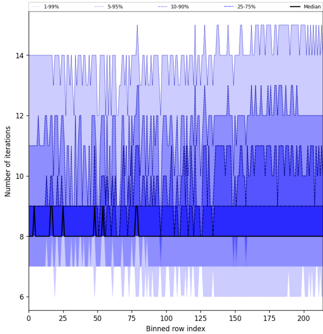
Figure 26: Along track statistics of “Number of iterations” for 2025-11-01 to 2025-11-02
