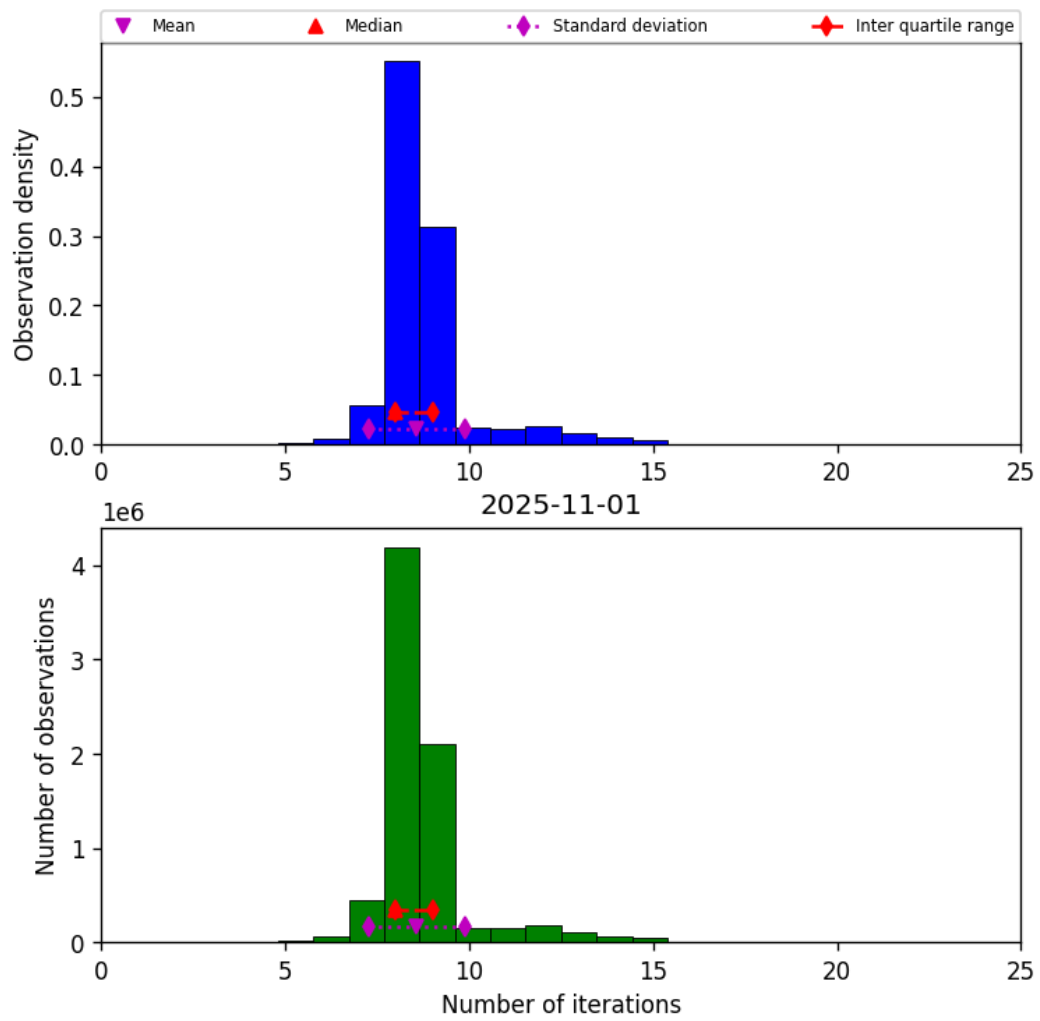
Figure 19: Histogram of “Number of iterations” for 2025-11-01 to 2025-11-02
