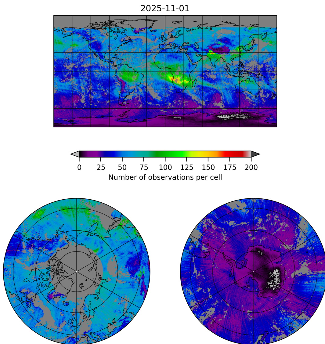
Figure 5: Map of the number of observations for 2025-11-01 to 2025-11-02
