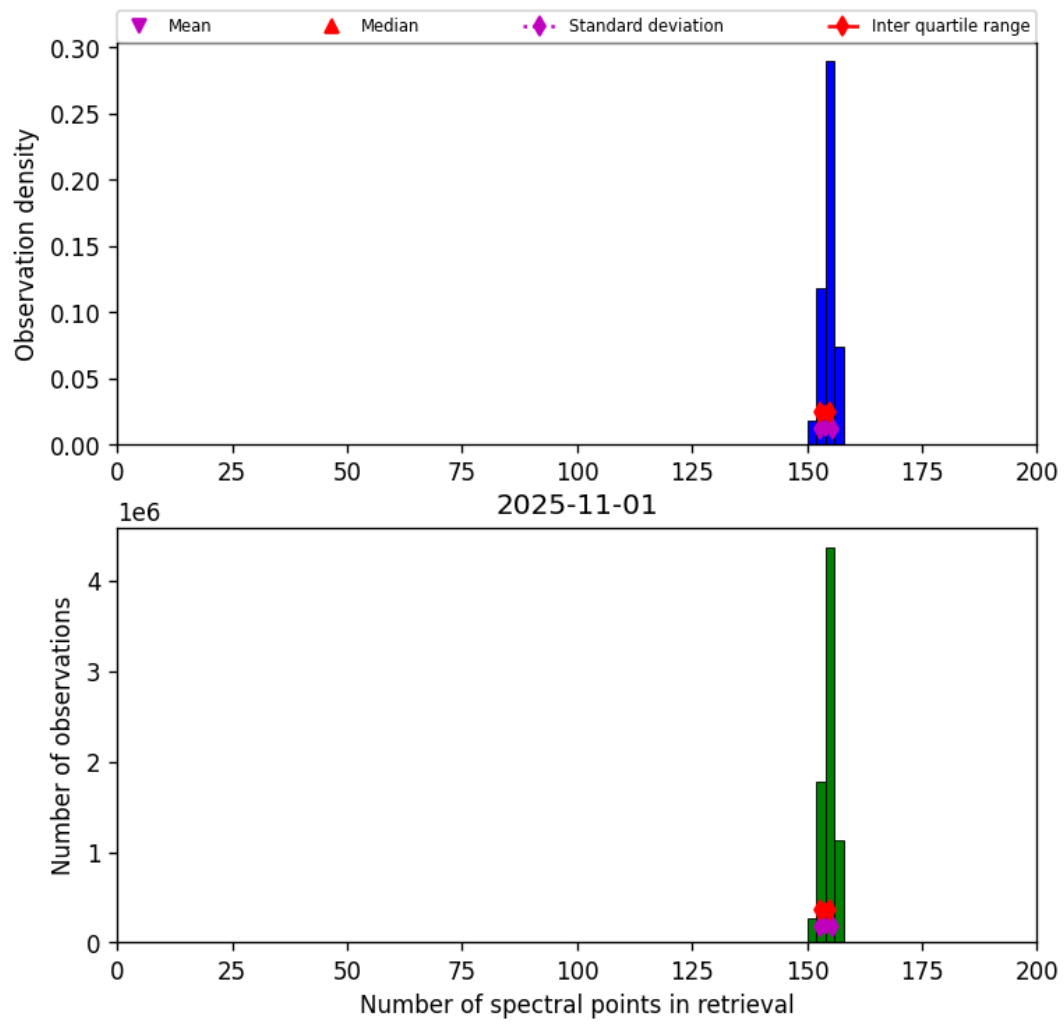
Figure 16: Histogram of “Number of spectral points in retrieval” for 2025-11-01 to 2025-11-02
