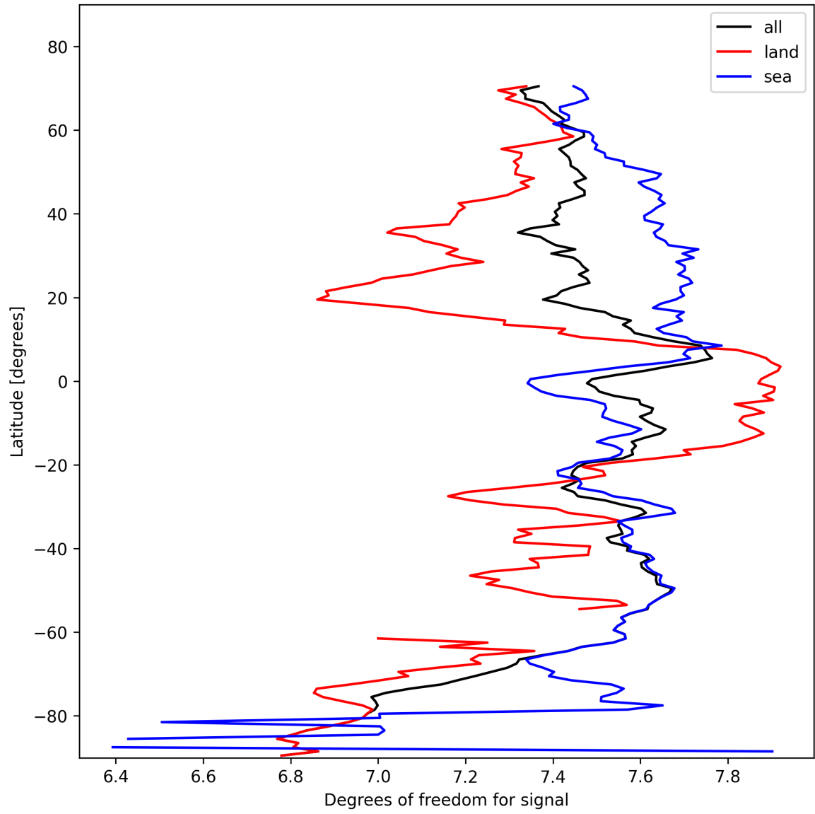
Figure 11: Zonal average of “Degrees of freedom for signal” for 2025-11-01 to 2025-11-02.
