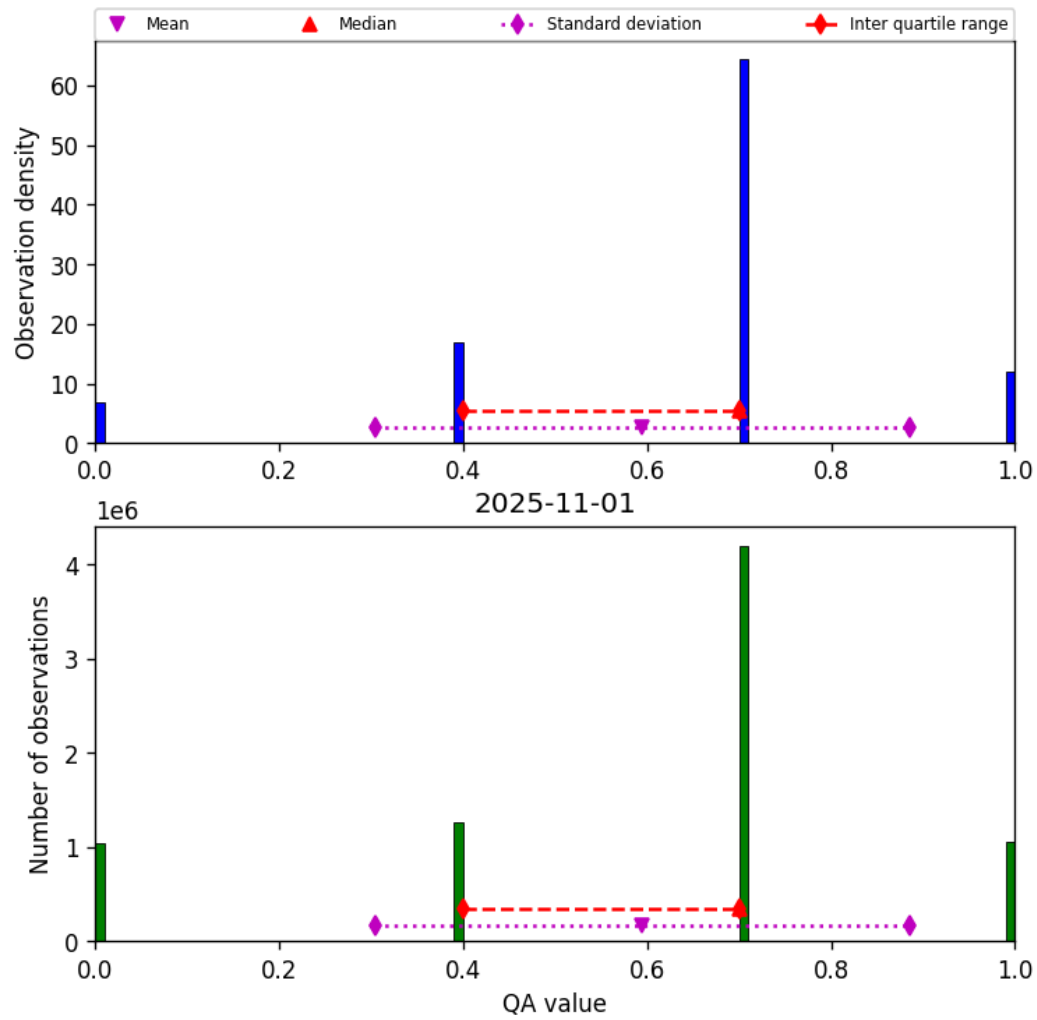
Figure 13: Histogram of “QA value” for 2025-11-01 to 2025-11-02
