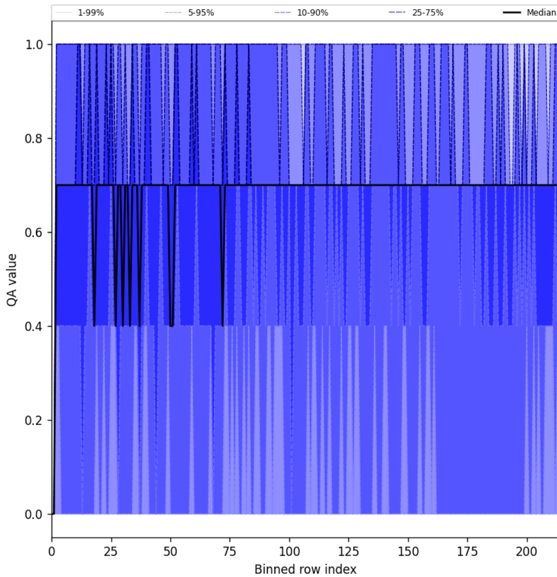
Figure 20: Along track statistics of “QA value” for 2025-11-01 to 2025-11-02
