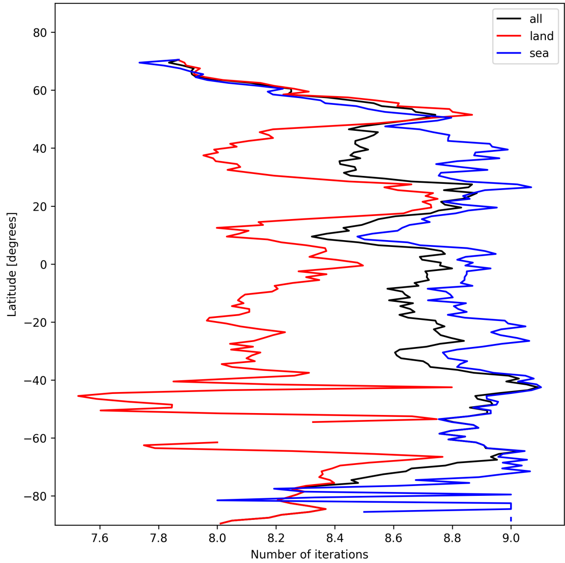
Figure 12: Zonal average of “Number of iterations” for 2025-11-01 to 2025-11-02.
