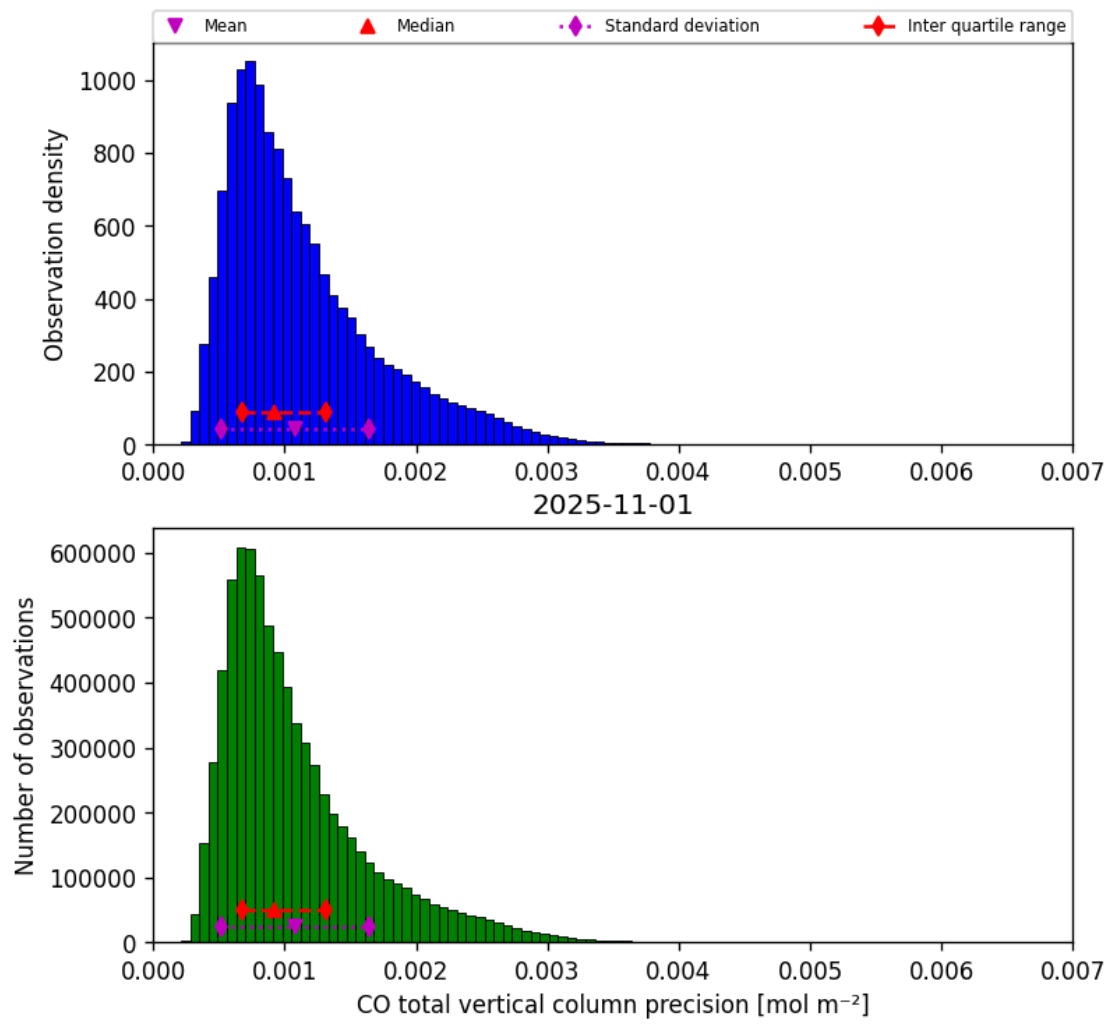
Figure 15: Histogram of “CO total vertical column precision” for 2025-11-01 to 2025-11-02
