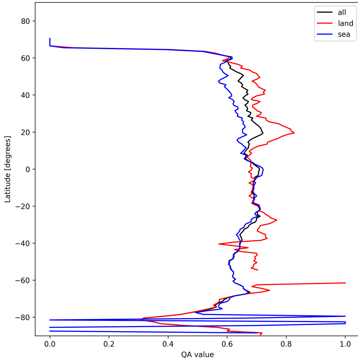
Figure 6: Zonal average of “QA value” for 2025-11-01 to 2025-11-02.
