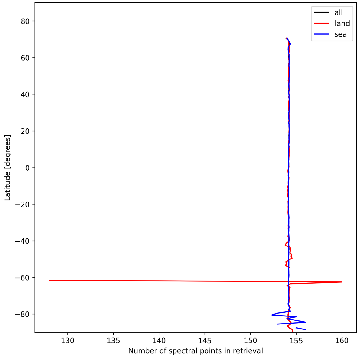
Figure 9: Zonal average of “Number of spectral points in retrieval” for 2025-11-01 to 2025-11-02.
