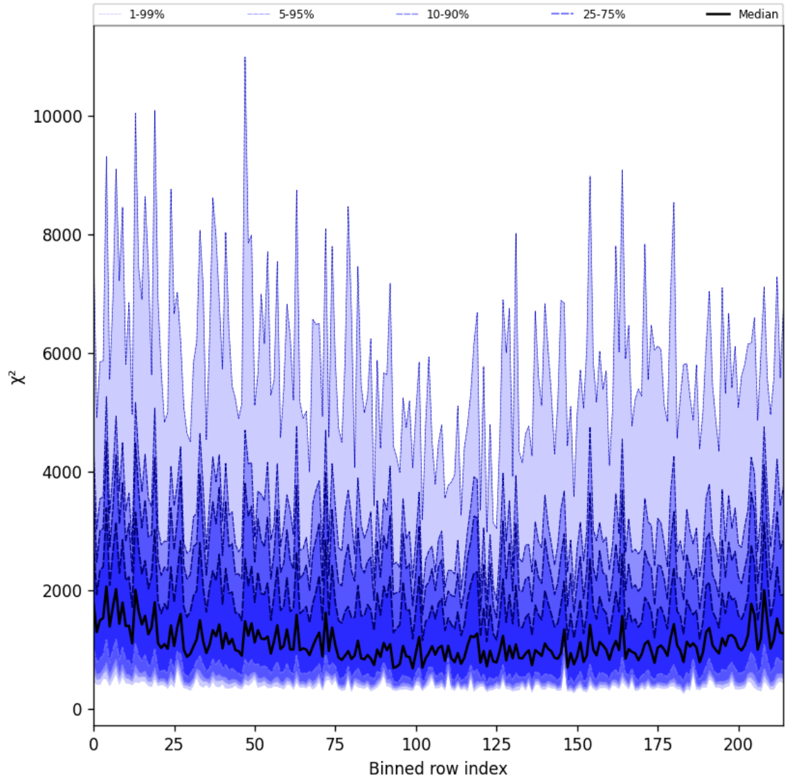
Figure 24: Along track statistics of “ \chi^2 ” for 2025-11-01 to 2025-11-02
