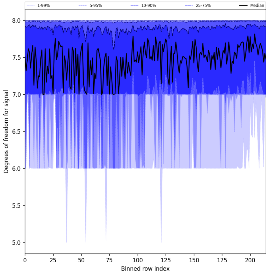
Figure 25: Along track statistics of “Degrees of freedom for signal” for 2025-11-01 to 2025-11-02
