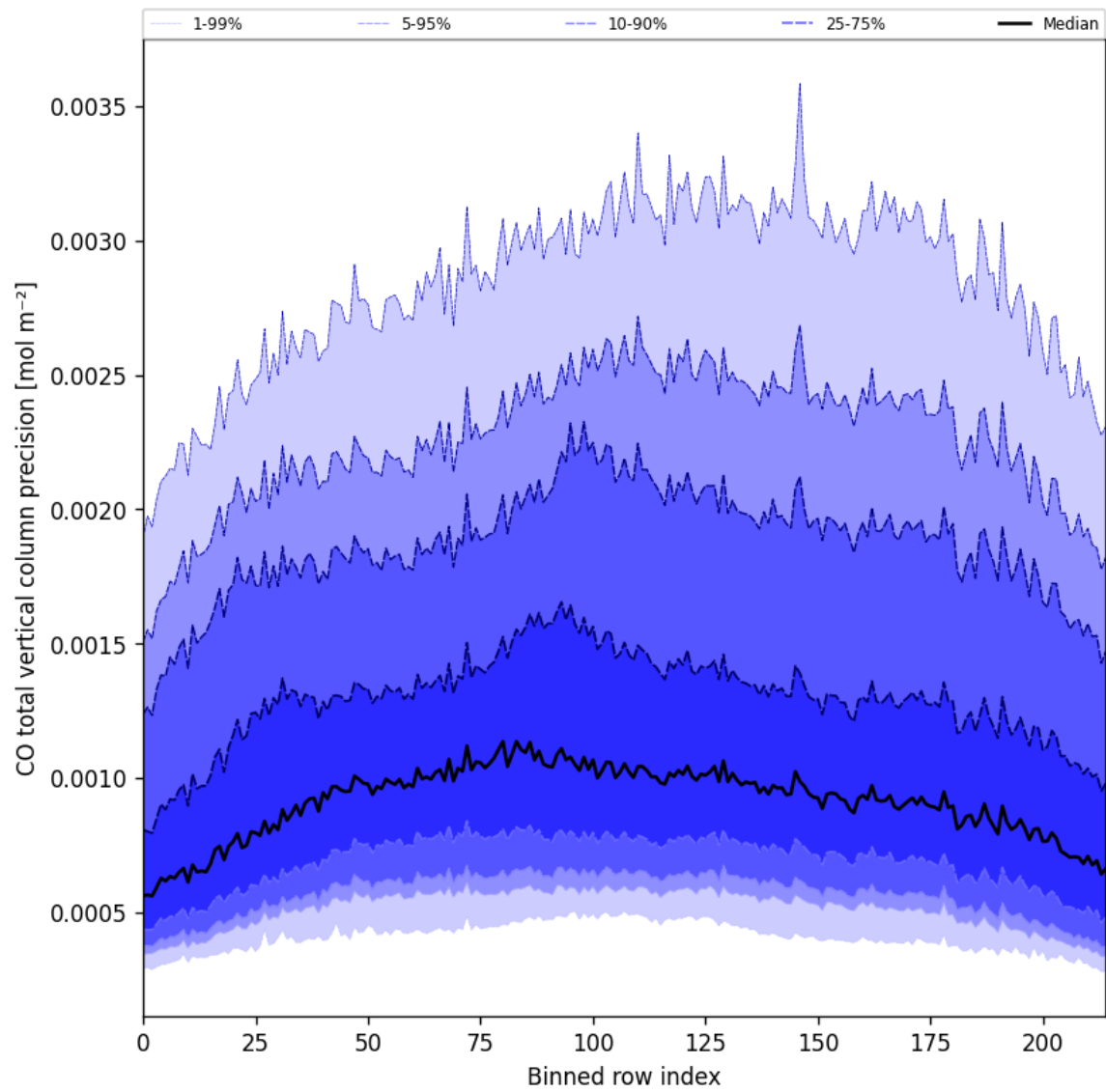
Figure 22: Along track statistics of “CO total vertical column precision” for 2025-11-01 to 2025-11-02
