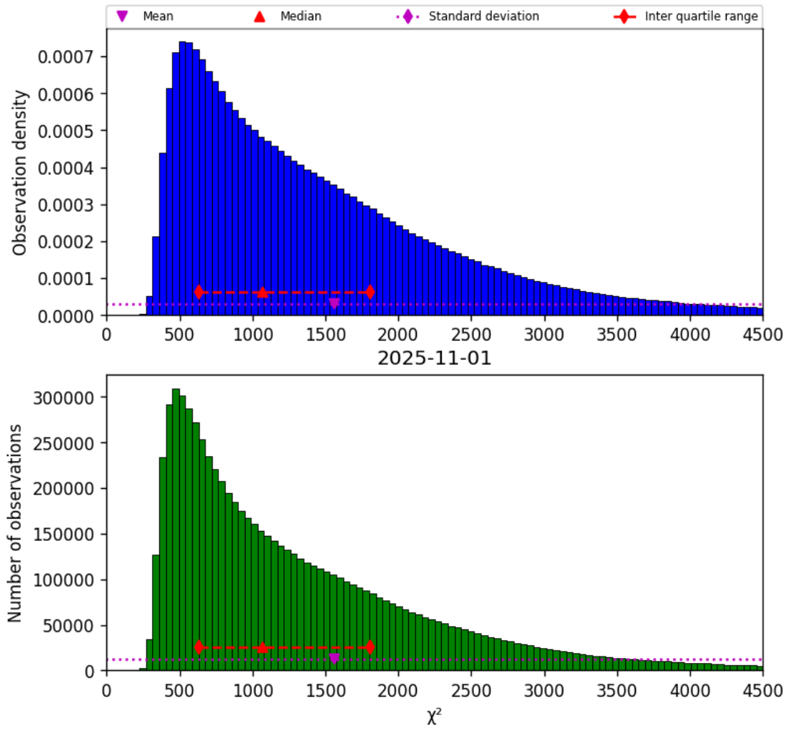
Figure 17: Histogram of “ \chi^2 ” for 2025-11-01 to 2025-11-02
