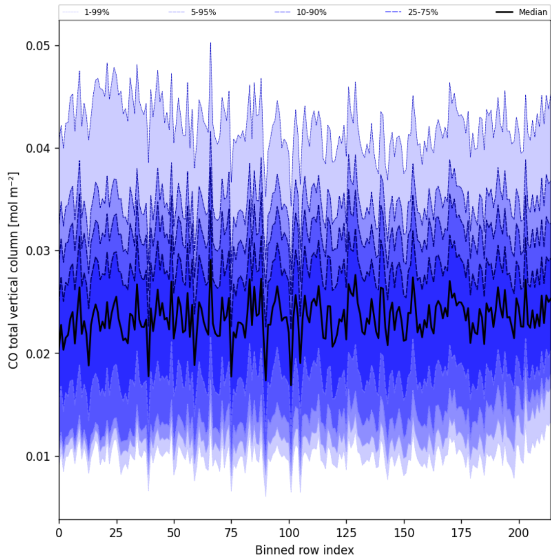
Figure 21: Along track statistics of “CO total vertical column” for 2025-11-01 to 2025-11-02
