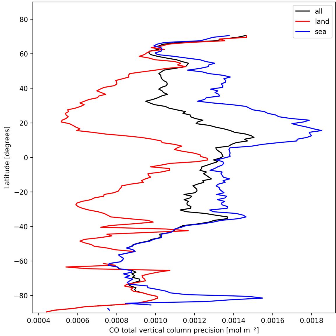
Figure 8: Zonal average of “CO total vertical column precision” for 2025-11-01 to 2025-11-02.
